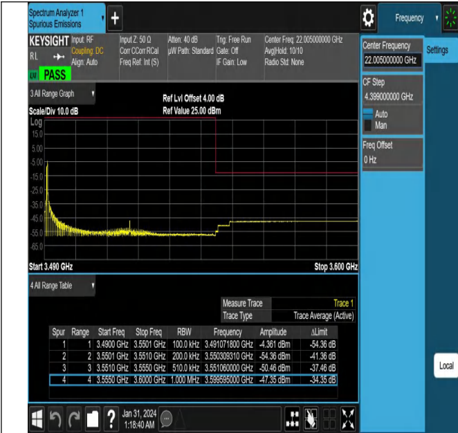
NTNV_N78-3450-3550_PC2_30_60_H_TID8_#1
