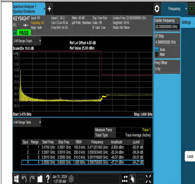
NTNV_N78-3450-3550_PC2_30_80_H_TID11_#1
