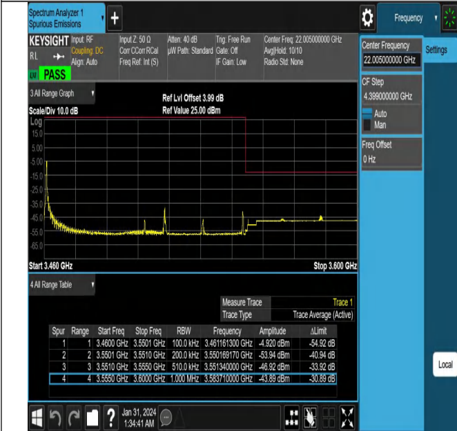
NTNV_N78-3450-3550_PC2_30_90_H_TID5_#1
