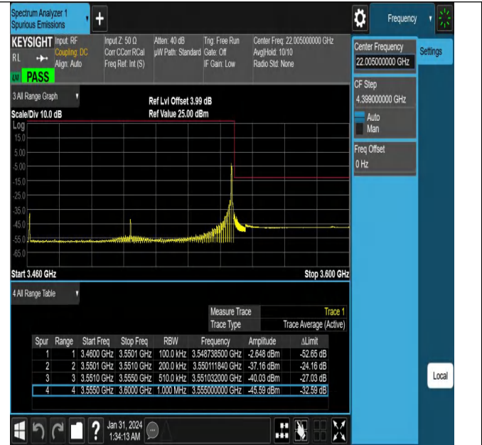
NTNV_N78-3450-3550_PC2_30_90_H_TID3_#1
