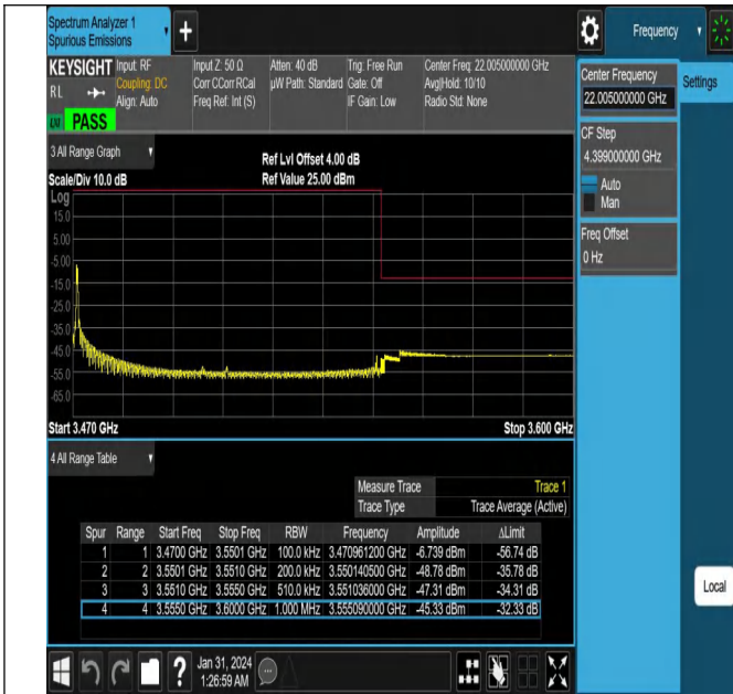
NTNV_N78-3450-3550_PC2_30_80_H_TID8_#1
