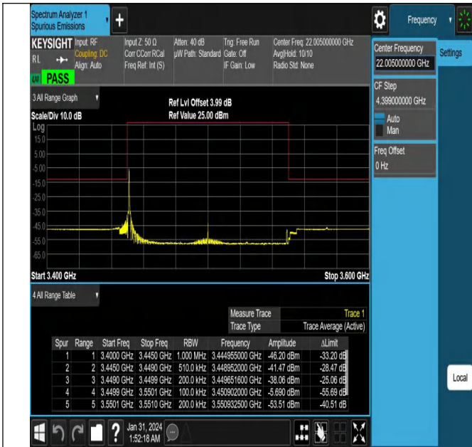
NTNV_N78-3450-3550_PC2_30_100_H_TID8_#1
