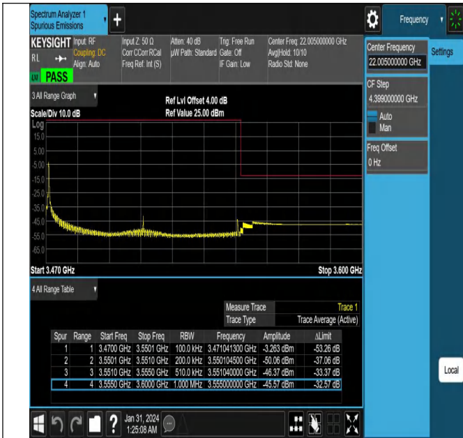
NTNV_N78-3450-3550_PC2_30_80_H_TID2_#1
