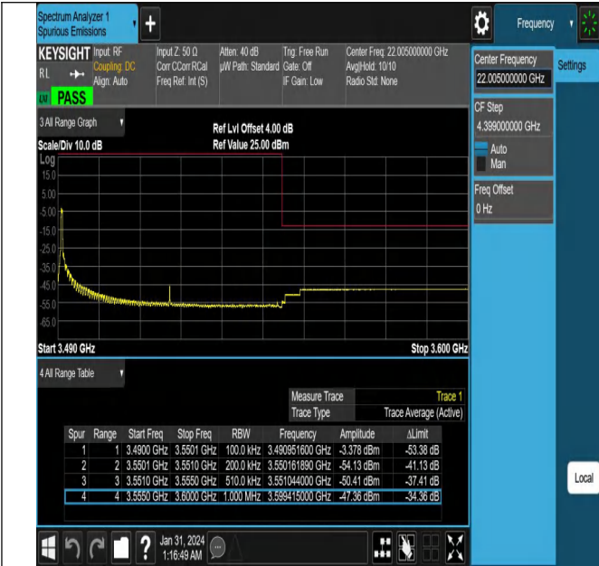
NTNV_N78-3450-3550_PC2_30_60_H_TID2_#1
