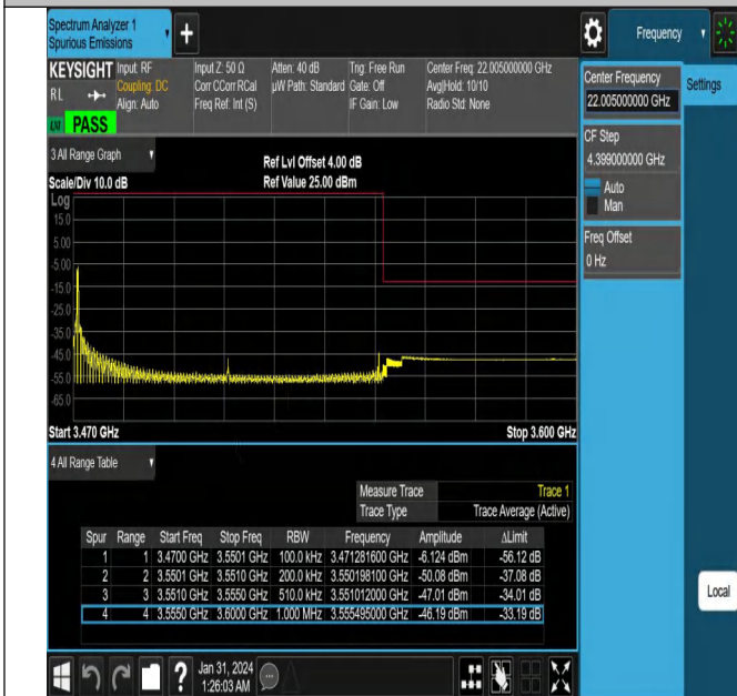
NTNV_N78-3450-3550_PC2_30_80_H_TID5_#1
