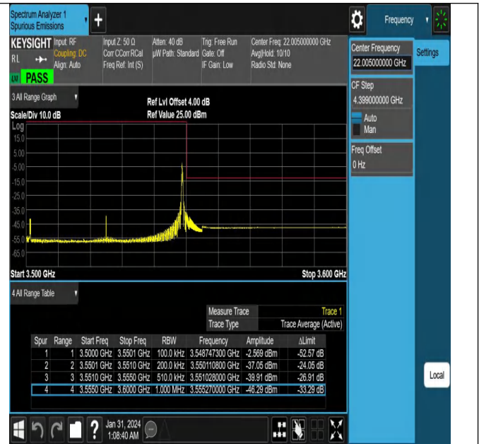
NTNV_N78-3450-3550_PC2_30_50_H_TID3_#1
