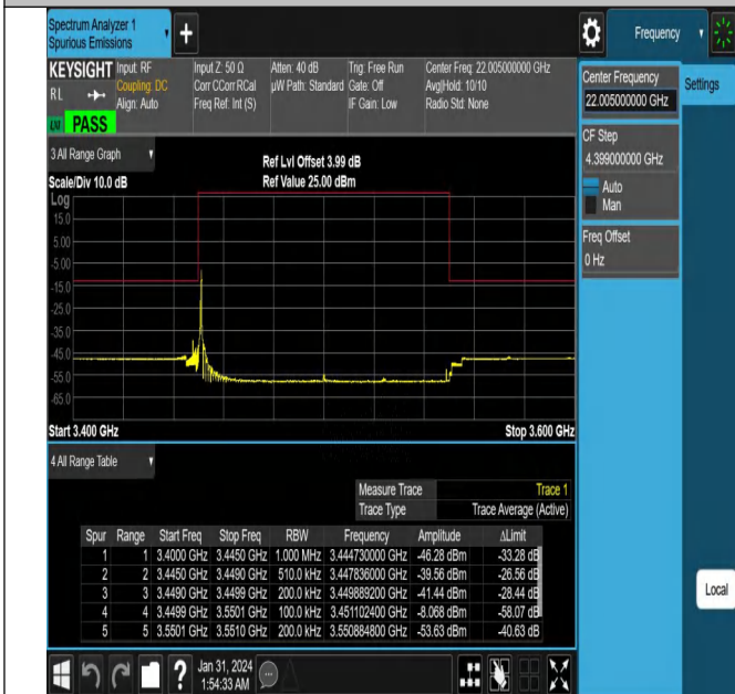
NTNV_N78-3450-3550_PC2_30_100_H_TID11_#1
