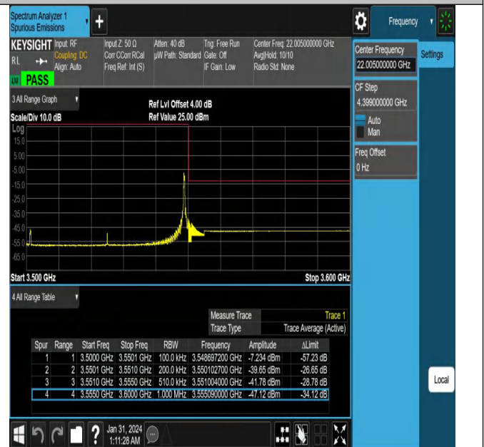
NTNV_N78-3450-3550_PC2_30_50_H_TID12_#1
