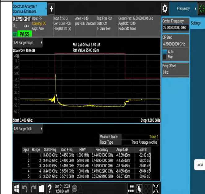
NTNV_N78-3450-3550_PC2_30_100_H_TID5_#1
