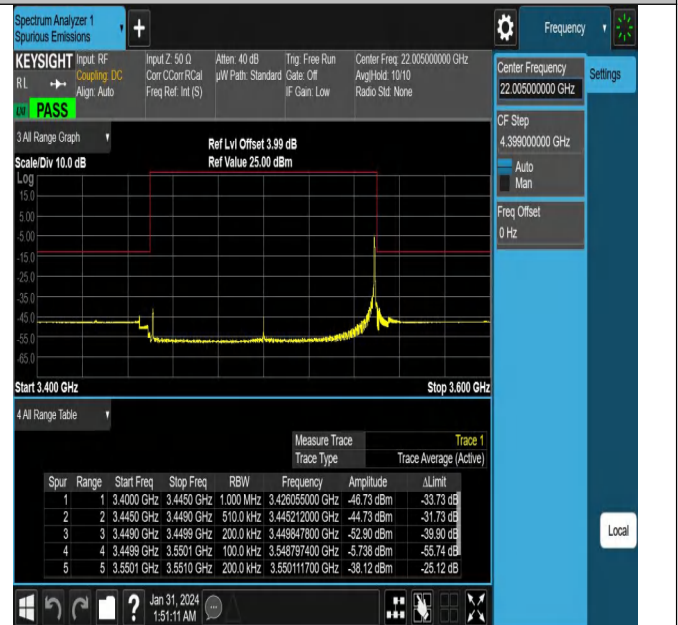
NTNV_N78-3450-3550_PC2_30_100_H_TID6_#1
