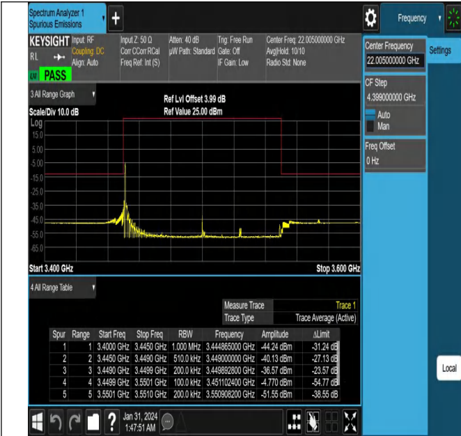
NTNV_N78-3450-3550_PC2_30_100_H_TID2_#1
