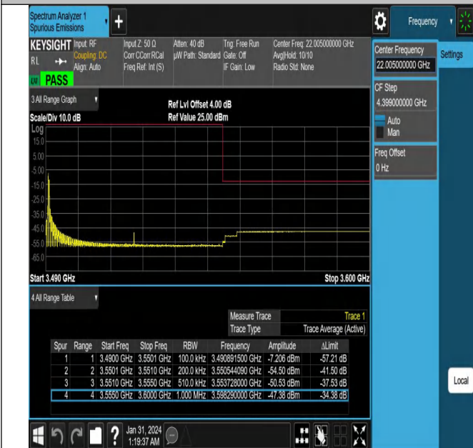
NTNV_N78-3450-3550_PC2_30_60_H_TID11_#1
