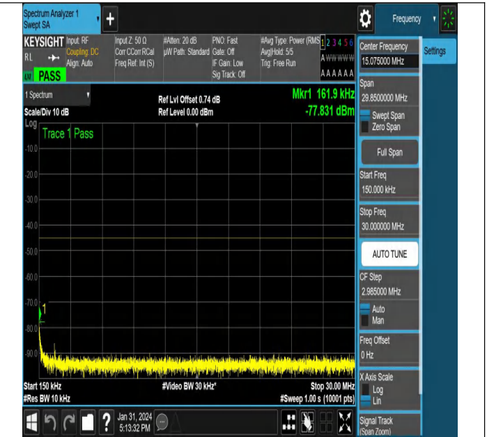
NTNV-N38-PC3-30-40-L-CP-QPSK-Edge_1RB_Left-Ant1-PAS
