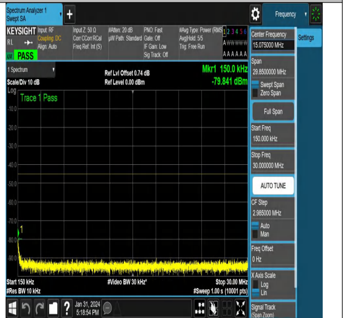
NTNV-N38-PC3-30-40-M-CP-QPSK-Edge_1RB_Right-Ant1-P
