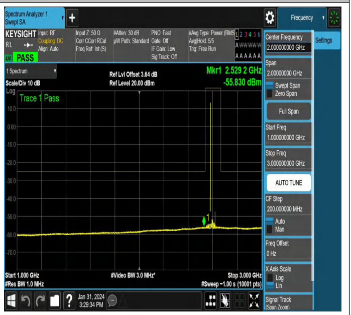
NTNV-N38-PC3-30-40-H-CP-QPSK-Edge_1RB_Left-Ant1-PAS
