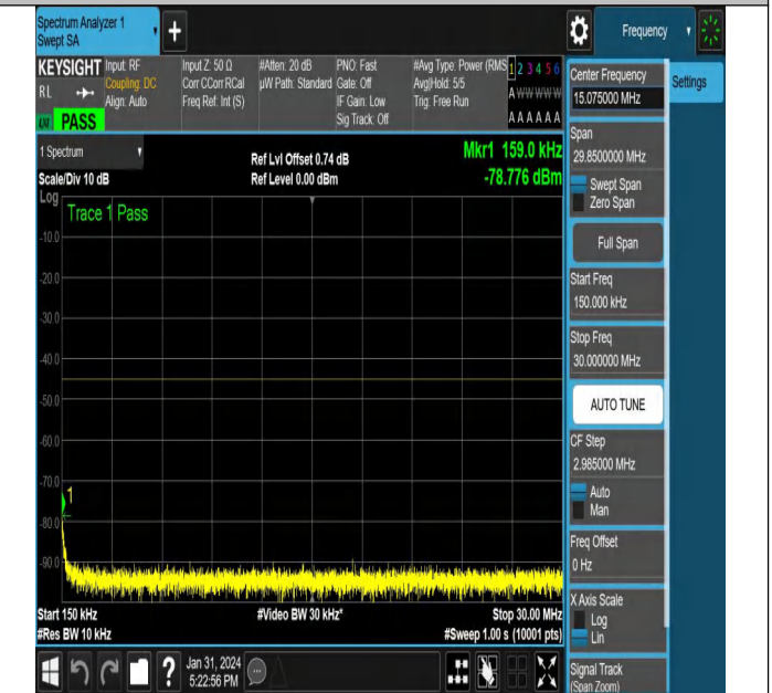
NTVN-N38-PC3-30-40-H-CP-QPSK-Edge_1RB_Right-Ant1-PA
