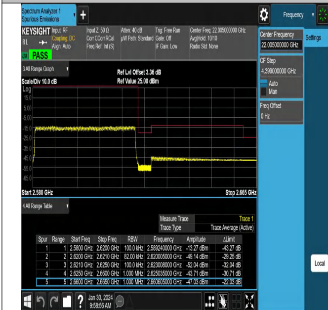
NTNV_N38_PC3_30_40_H_TID10_#1
