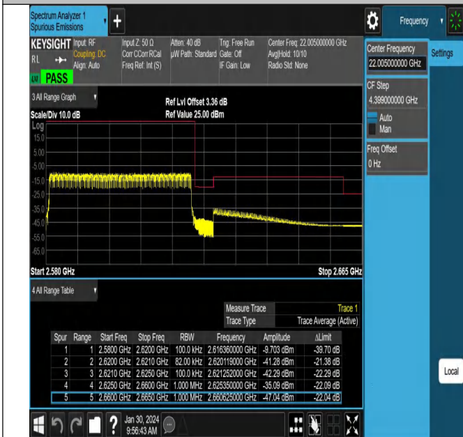
NTNV_N38_PC3_30_40_H_TID4_#1
