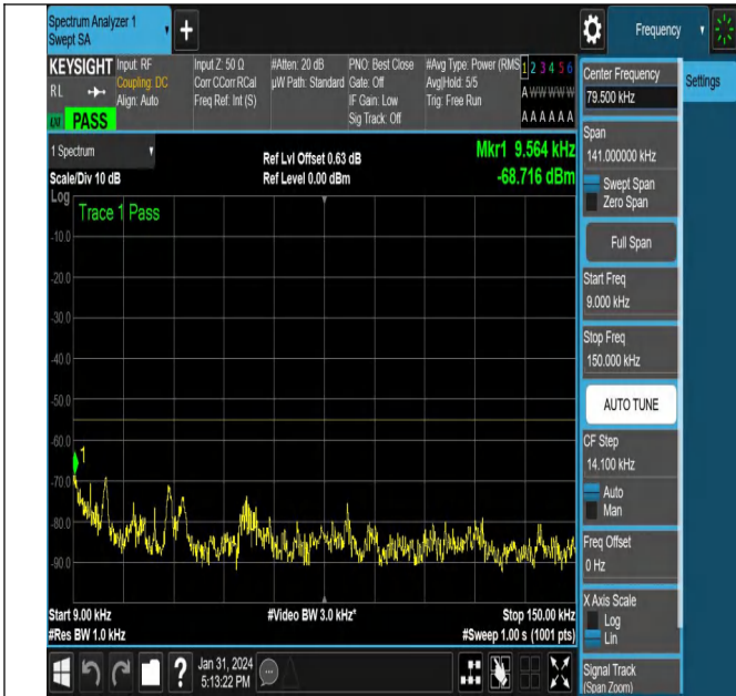
NTNV-N38-PC3-30-40-L-CP-QPSK-Edge_1RB_Left-Ant1-PAS
