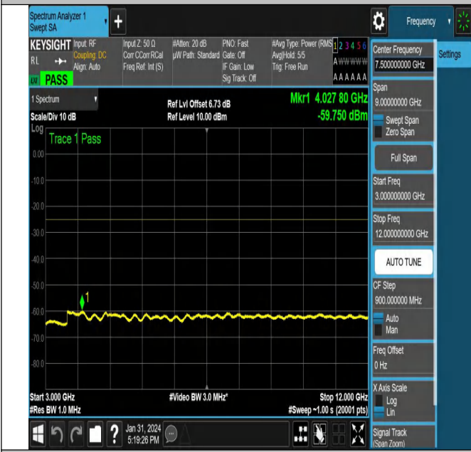
NTNV-N38-PC3-30-40-M-CP-QPSK-Edge_1RB_Right-Ant1-P ASS
