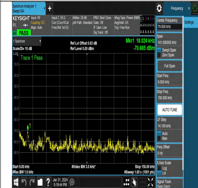
NTNV-N38-PC3-30-40-M-CP-QPSK-Edge_1RB_Right-Ant1-P
