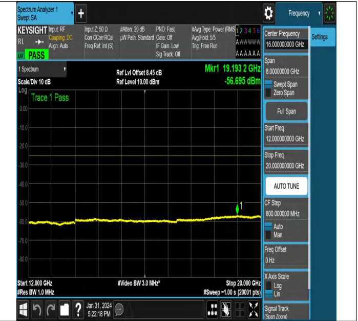
NTVN-N38-PC3-30-40-H-CP-QPSK-Edge_1RB_Left-Ant1-PAS
