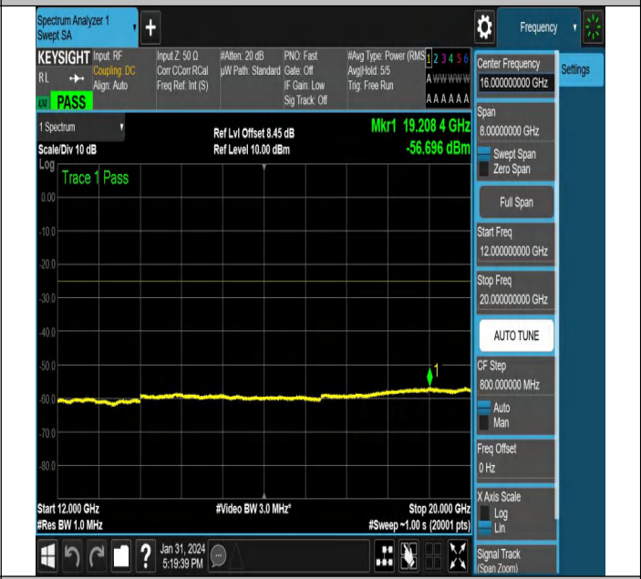
NTNV-N38-PC3-30-40-M-CP-QPSK-Edge_1RB_Right-Ant1-P ASS
