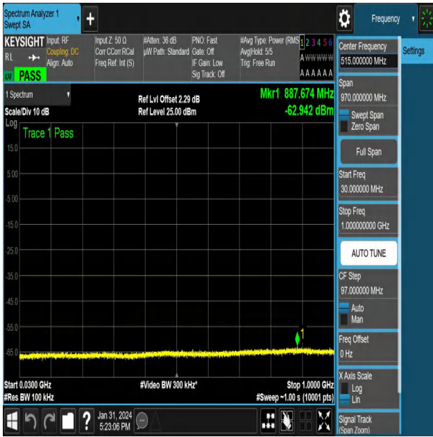
NTNV-N38-PC3-30-40-H-CP-QPSK-Edge_1RB_Right-Ant1-PA SS
