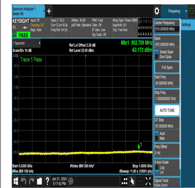
NTNV-N38-PC3-30-40-M-CP-QPSK-Edge_1RB_Left-Ant1-PA
