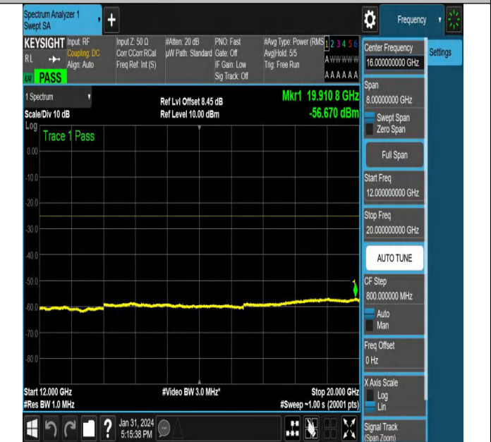
NTNV-N38-PC3-30-40-L-CP-QPSK-Edge_1RB_Right-Ant1-PA
