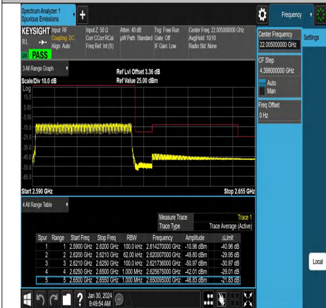
NTNV_N38_PC3_30_30_H_TID10_#1
