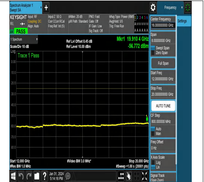
NTVN-N38-PC3-30-40-L-CP-QPSK-Edge_1RB_Left-Ant1-PAS
