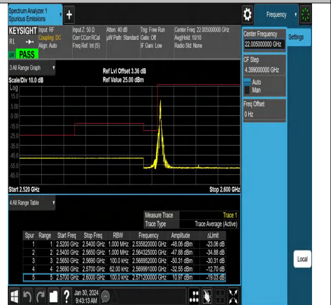
NTNV_N38_PC3_30_30_L_TID5_#1
