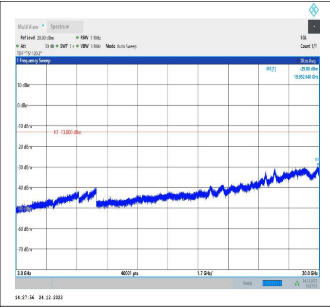
66-66-20MHz-15MHz-QPSK-QPSK-132423-132594-1RB#0-1RB#74-3000~20000MHz-PASS
