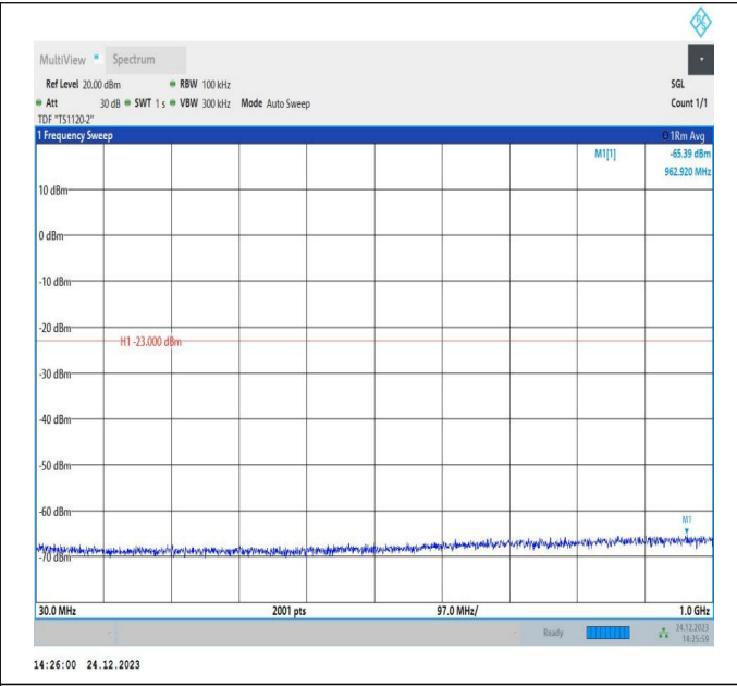
66-66-20MHz-15MHz-QPSK-QPSK-132423-132594-1RB#0-ORB#0-30~1000MHz-PASS
