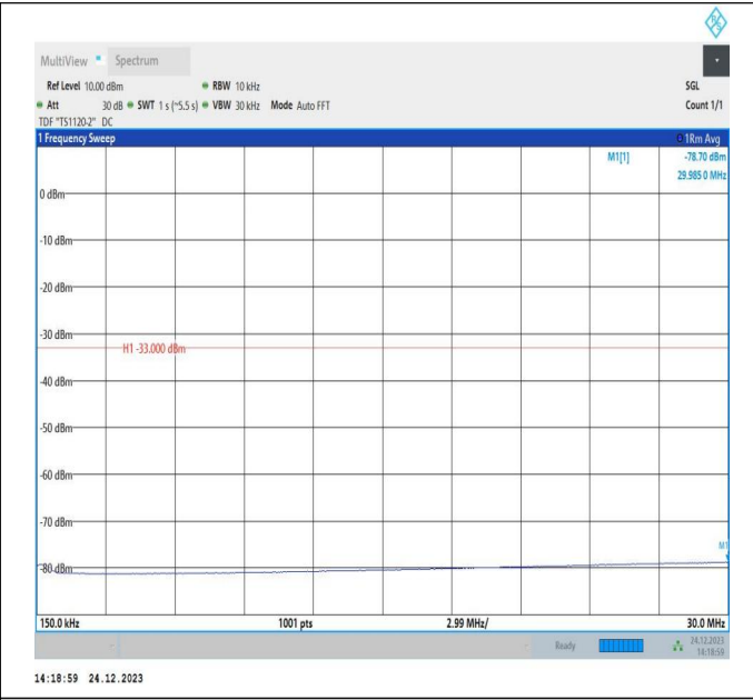
66-66-20MHz-15MHz-QPSK-QPSK-132072-132243-1RB#99 -ORB#0-0.15~30MHz-PASS
