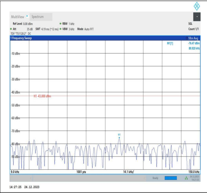
66-66-20MHz-15MHz-QPSK-QPSK-132423-132594-1RB#0-1RB#74-0.009~0.15MHz-PASS
