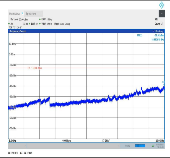
66-66-20MHz-15MHz-QPSK-QPSK-132072-132243-1RB#0-1RB#74-3000~20000MHz-PASS
