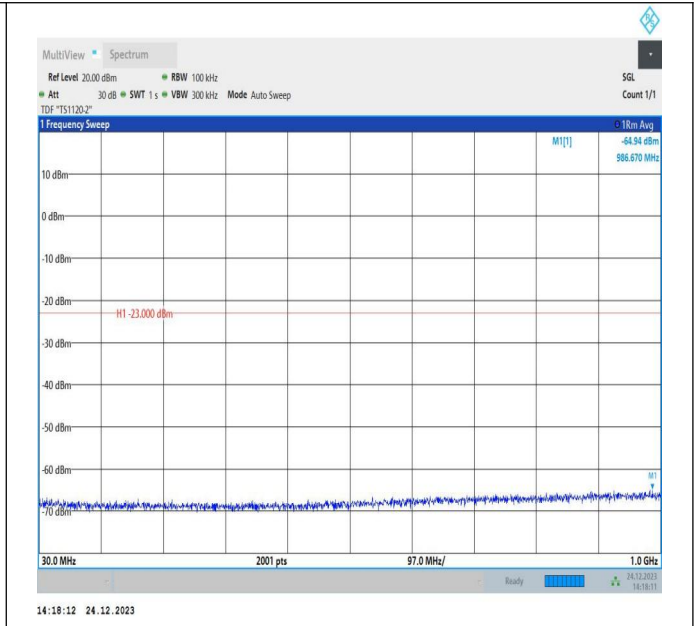
66-66-20MHz-15MHz-QPSK-QPSK-132072-132243-1RB#0-ORB#0-30~1000MHz-PASS
