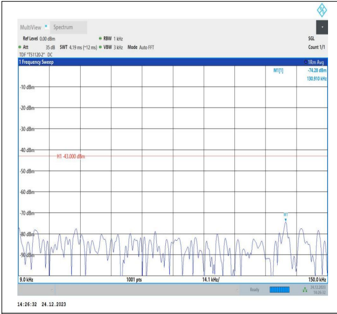
66-66-20MHz-15MHz-QPSK-QPSK-132423-132594-1RB#99 -ORB#0-0.009~0.15MHz-PASS
