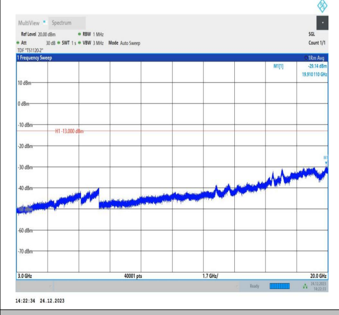
66-66-20MHz-15MHz-QPSK-QPSK-132348-132519-1RB#0-ORB#0-3000~20000MHz-PASS
