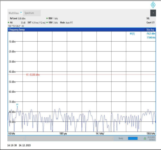
66-66-20MHz-15MHz-QPSK-QPSK-132072-132243-1RB#0-1RB#74-0.009~0.15MHz-PASS
