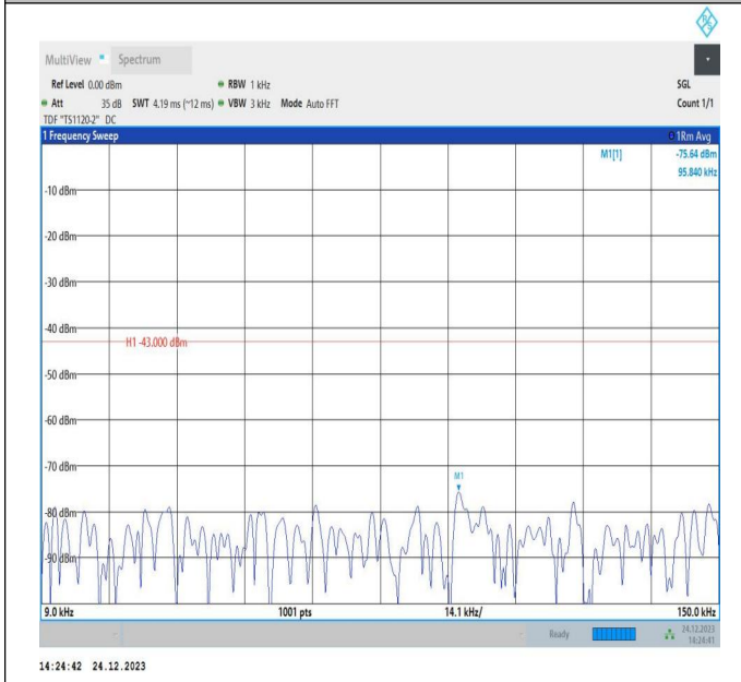
66-66-20MHz-15MHz-QPSK-QPSK-132348-132519-100RB#0-75RB#0-0.009~0.15MHz-PASS
