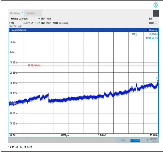
66-66-20MHz-15MHz-QPSK-QPSK-132423-132594-1RB#99-0RB#0-3000~20000MHz-PASS
