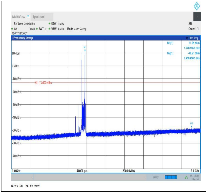
66-66-20MHz-15MHz-QPSK-QPSK-132423-132594-1RB#0-1RB#74-1000~3000MHz-PASS
