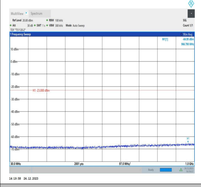
66-66-20MHz-15MHz-QPSK-QPSK-132072-132243-1RB#0-1RB#74-30~1000MHz-PASS
