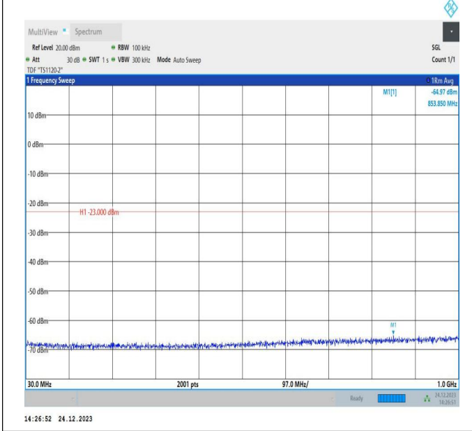
66-66-20MHz-15MHz-QPSK-QPSK-132423-132594-1RB#99 -ORB#0-30~1000MHz-PASS
