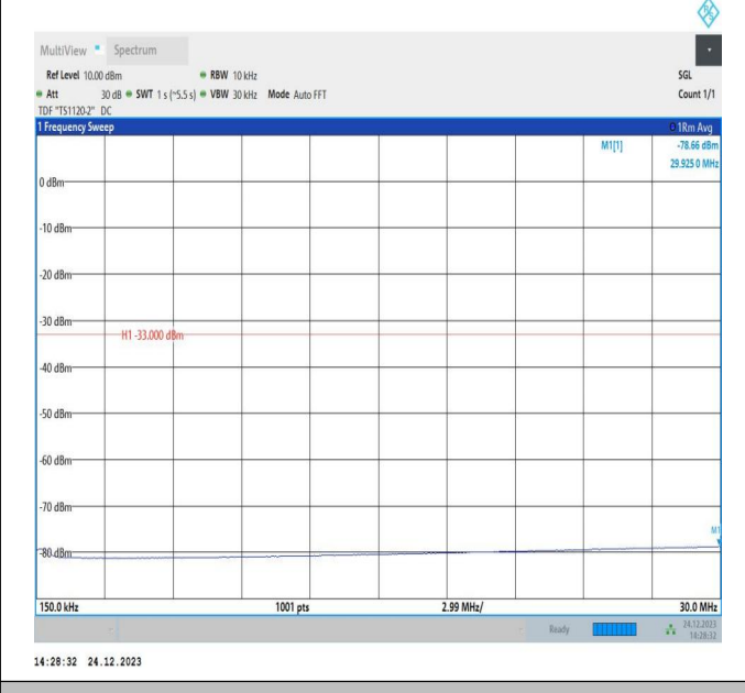
66-66-20MHz-15MHz-QPSK-QPSK-132423-132594-100RB#0-75RB#0-0.15~30MHz-PASS
