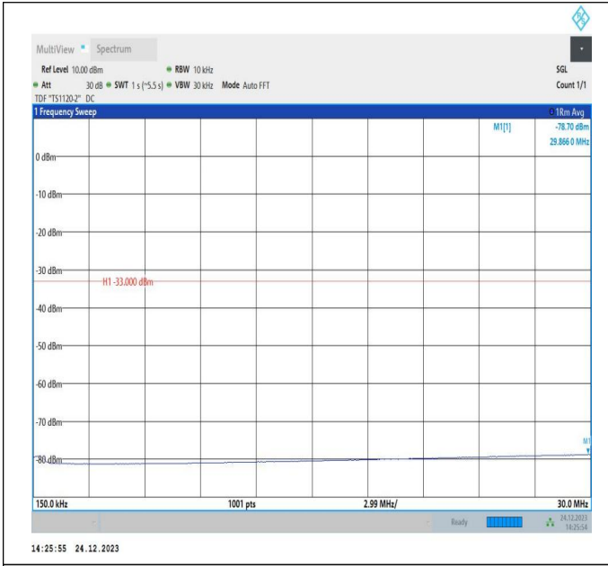
66-66-20MHz-15MHz-QPSK-QPSK-132423-132594-1RB#0-ORB#0-0.15~30MHz-PASS
