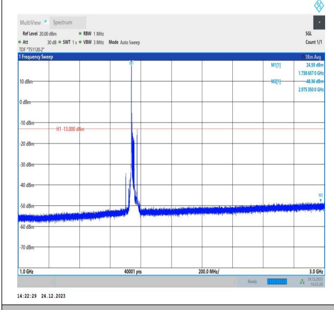
66-66-20MHz-15MHz-QPSK-QPSK-132348-132519-1RB#0-ORB#0-1000~3000MHz-PASS
