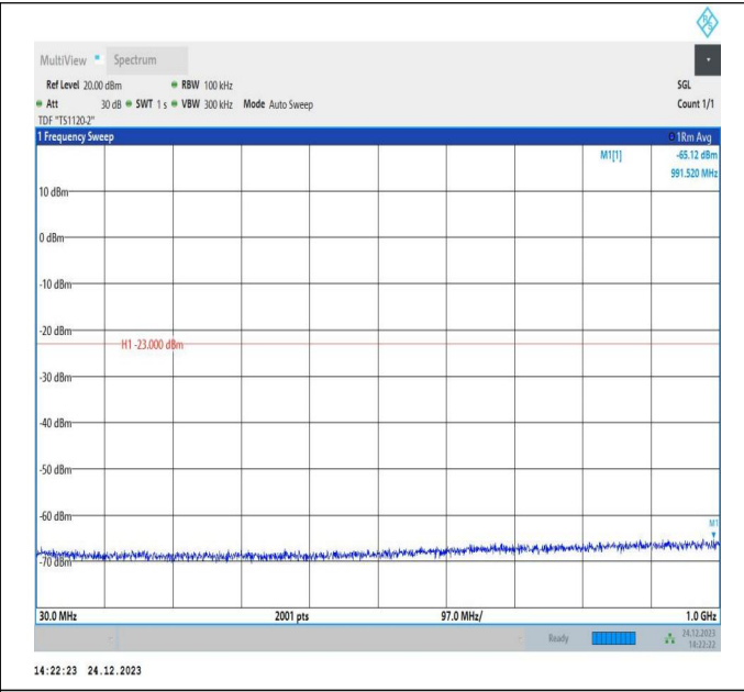
66-66-20MHz-15MHz-QPSK-QPSK-132348-132519-1RB#0-ORB#0-30~1000MHz-PASS
