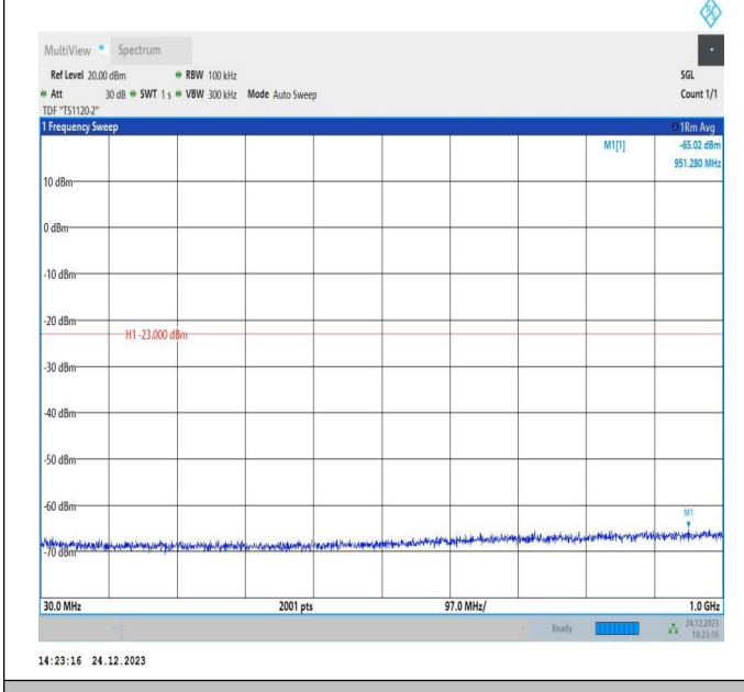
66-66-20MHz-15MHz-QPSK-QPSK-132348-132519-1RB#99 -ORB#0-30~1000MHz-PASS
