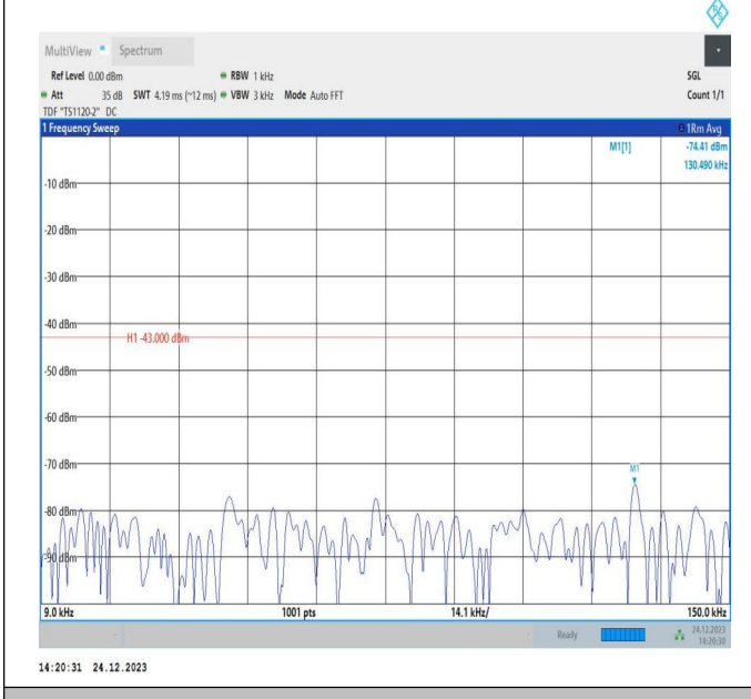
66-66-20MHz-15MHz-QPSK-QPSK-132072-132243-100RB#0-75RB#0-0.009~0.15MHz-PASS
