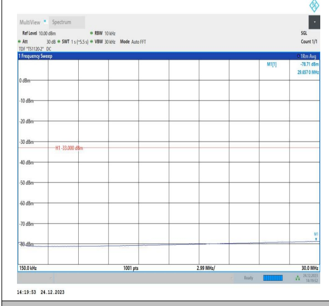
66-66-20MHz-15MHz-QPSK-QPSK-132072-132243-1RB#0-1RB#74-0.15~30MHz-PASS
