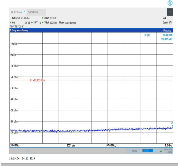
66-66-20MHz-15MHz-QPSK-QPSK-132072-132243-1RB#99 -ORB#0-30~1000MHz-PASS
