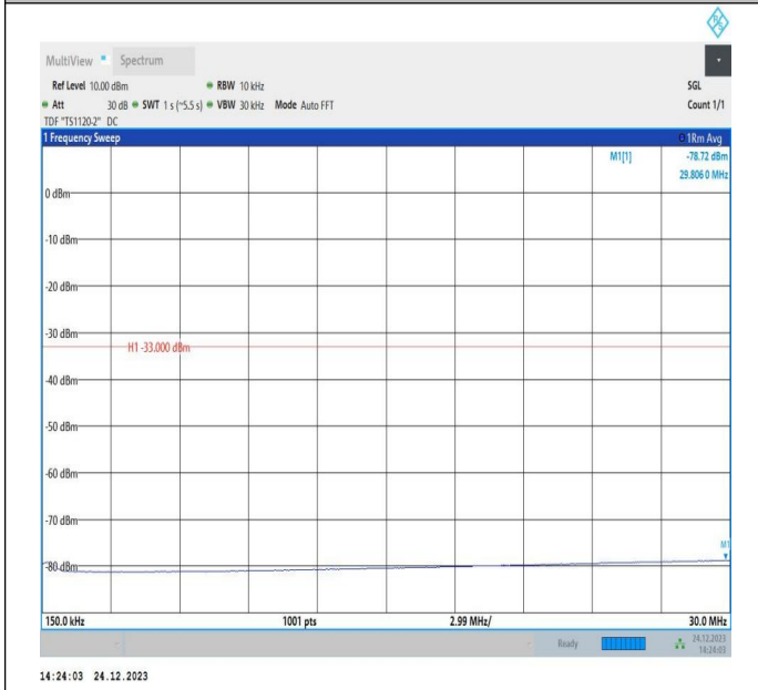
66-66-20MHz-15MHz-QPSK-QPSK-132348-132519-1RB#0- 1RB#74-0.15~30MHz-PASS
