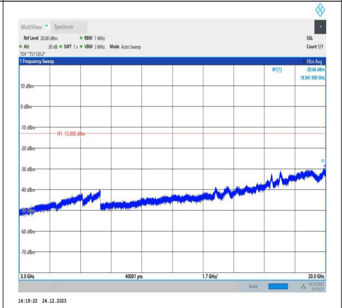
66-66-20MHz-15MHz-QPSK-QPSK-132072-132243-1RB#0-ORB#0-3000~20000MHz-PASS
