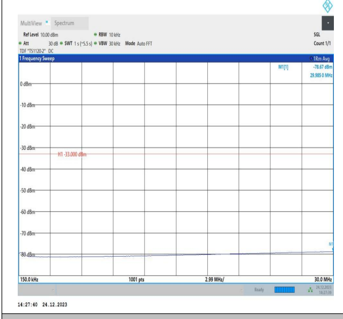
66-66-20MHz-15MHz-QPSK-QPSK-132423-132594-1RB#0-1RB#74-0.15~30MHz-PASS
