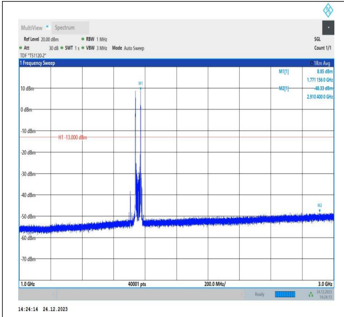
66-66-20MHz-15MHz-QPSK-QPSK-132348-132519-1RB#0-1RB#74-1000~3000MHz-PASS
