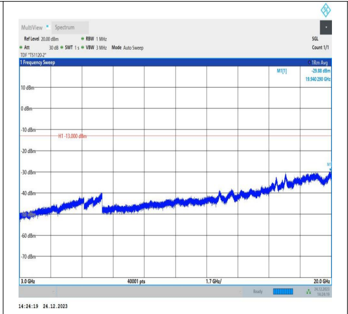
66-66-20MHz-15MHz-QPSK-QPSK-132348-132519-1RB#0-1RB#74-3000~20000MHz-PASS
