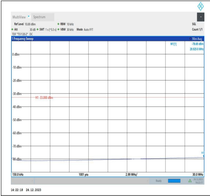
66-66-20MHz-15MHz-QPSK-QPSK-132348-132519-1RB#0-ORB#0-0.15~30MHz-PASS
