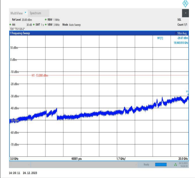
66-66-20MHz-15MHz-QPSK-QPSK-132423-132594-1RB#0-ORB#0-3000~20000MHz-PASS
