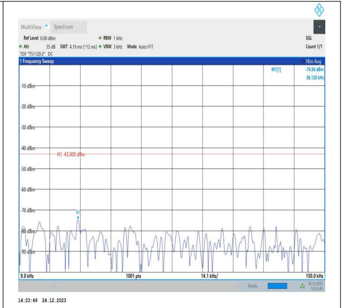
66-66-20MHz-15MHz-QPSK-QPSK-132348-132519-1RB#0- 1RB#74-0.009~0.15MHz-PASS
