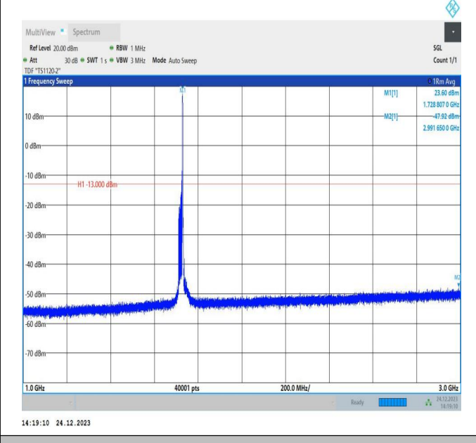
66-66-20MHz-15MHz-QPSK-QPSK-132072-132243-1RB#99 -ORB#0-1000~3000MHz-PASS
