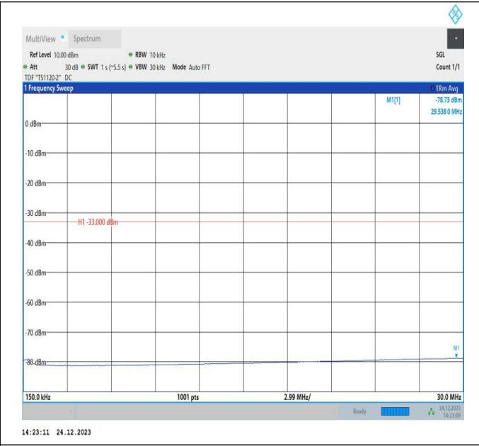
66-66-20MHz-15MHz-QPSK-QPSK-132348-132519-1RB#99 -ORB#0-0.15~30MHz-PASS
