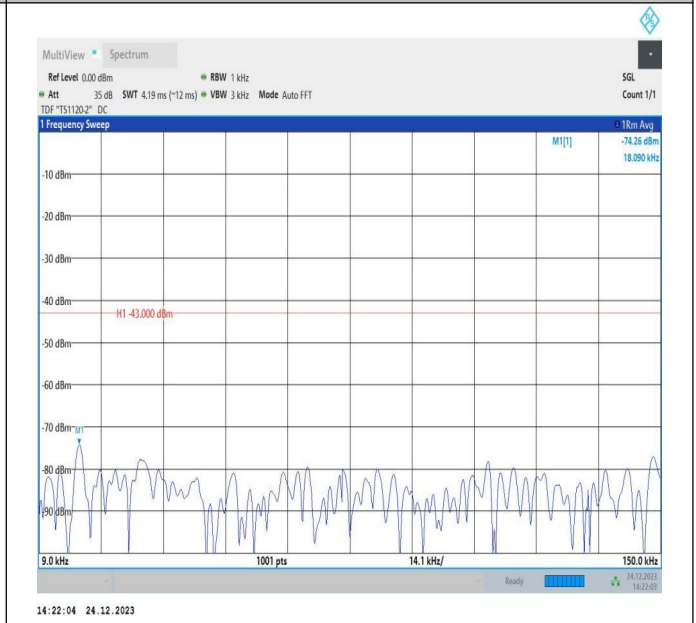
66-66-20MHz-15MHz-QPSK-QPSK-132348-132519-1RB#0- 0RB#0-0.009~0.15MHz-PASS
