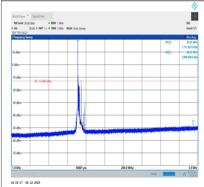
66-66-20MHz-15MHz-QPSK-QPSK-132072-132243-1RB#0-ORB#0-1000~3000MHz-PASS
