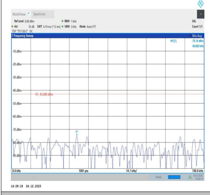
66-66-20MHz-15MHz-QPSK-QPSK-132423-132594-100RB#0-75RB#0-0.009~0.15MHz-PASS
