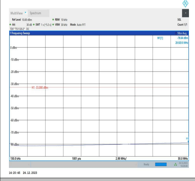
66-66-20MHz-15MHz-QPSK-QPSK-132072-132243-100RB#0-75RB#0-0.15~30MHz-PASS
