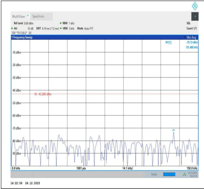
66-66-20MHz-15MHz-QPSK-QPSK-132348-132519-1RB#99 -ORB#0-0.009~0.15MHz-PASS
