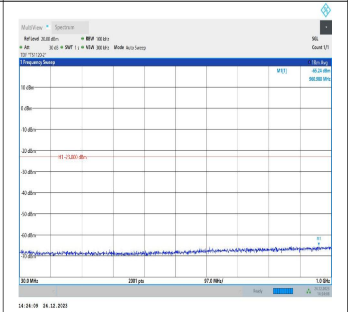
66-66-20MHz-15MHz-QPSK-QPSK-132348-132519-1RB#0- 1RB#74-30~1000MHz-PASS
