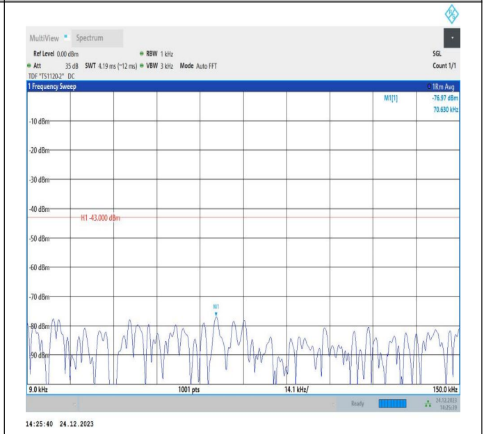
66-66-20MHz-15MHz-QPSK-QPSK-132423-132594-1RB#0- 0RB#0-0.009~0.15MHz-PASS
