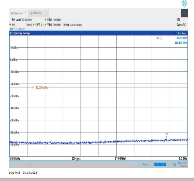
66-66-20MHz-15MHz-QPSK-QPSK-132423-132594-1RB#0-1RB#74-30~1000MHz-PASS
