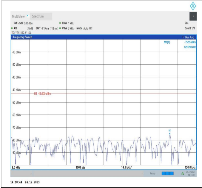
66-66-20MHz-15MHz-QPSK-QPSK-132072-132243-1RB#99 -ORB#0-0.009~0.15MHz-PASS
