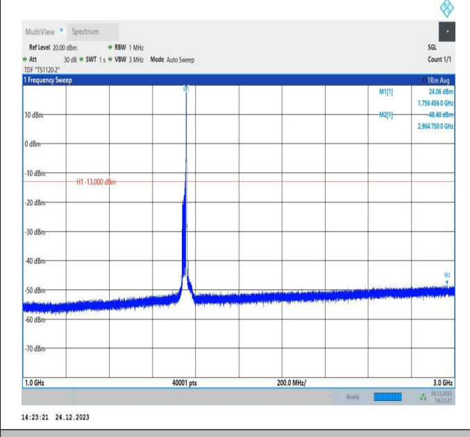
66-66-20MHz-15MHz-QPSK-QPSK-132348-132519-1RB#99 -ORB#0-1000~3000MHz-PASS
