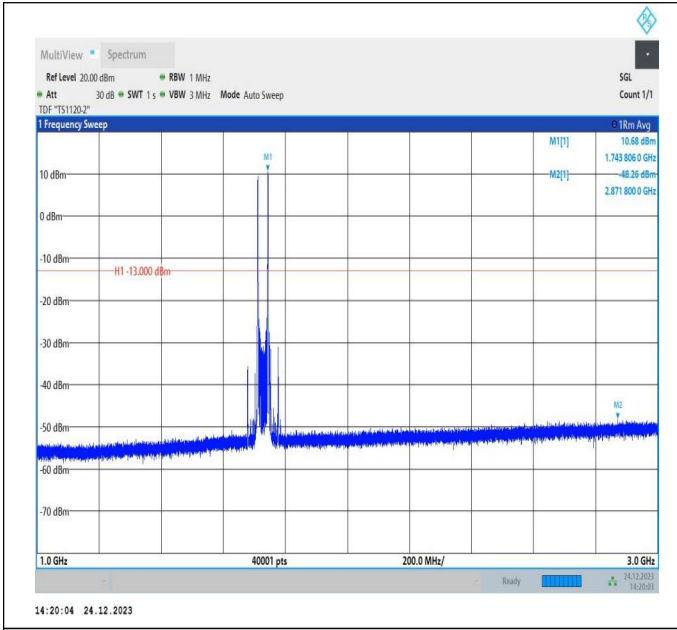
66-66-20MHz-15MHz-QPSK-QPSK-132072-132243-1RB#0-1RB#74-1000~3000MHz-PASS
