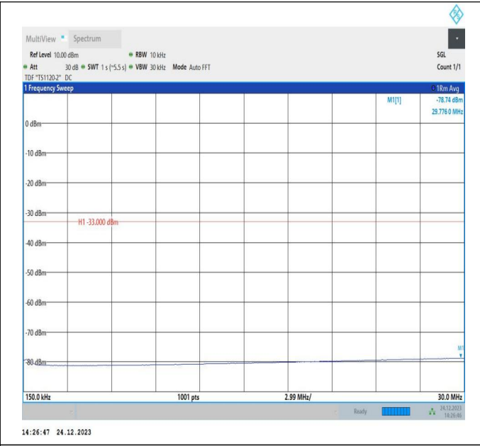
66-66-20MHz-15MHz-QPSK-QPSK-132423-132594-1RB#99 -ORB#0-0.15~30MHz-PASS
