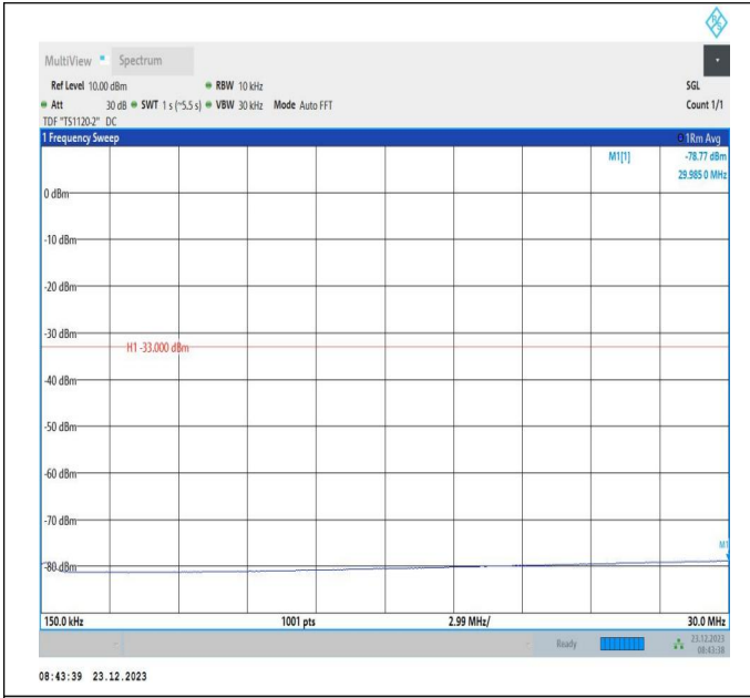
66-66-20MHz-5MHz-16QAM-16QAM-132522-132639-1RB#0 -1RB#24-0.15~30MHz-PASS
