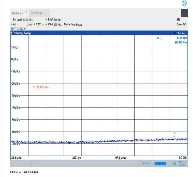
66-66-20MHz-5MHz-64QAM-64QAM-132522-132639-1RB#0 -1RB#24-30~1000MHz-PASS
