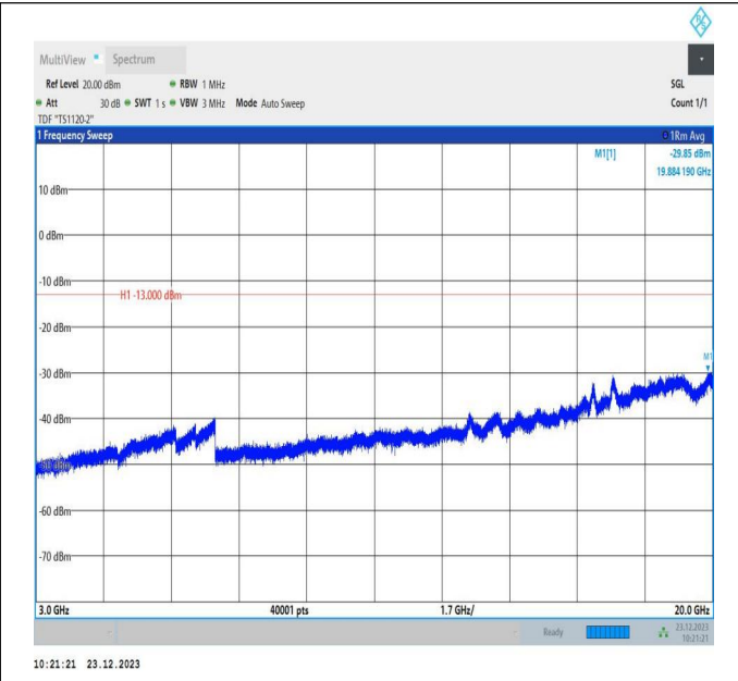
66-66-20MHz-10MHz-16QAM-16QAM-132072-132216-1RB# 0-ORB#0-3000~20000MHz-PASS
