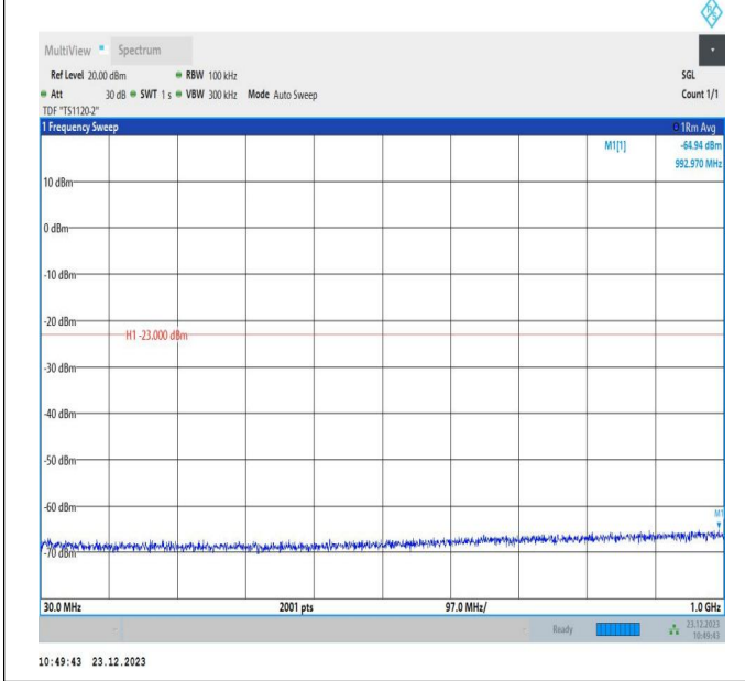
66-66-20MHz-10MHz-16QAM-16QAM-132072-132216-1RB# 99-ORB#0-30~1000MHz-PASS
