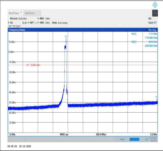
66-66-20MHz-5MHz-16QAM-16QAM-132522-132639-100RB #0-25RB#0-1000~3000MHz-PASS
