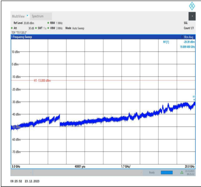
66-66-20MHz-5MHz-64QAM-64QAM-132522-132639-1RB#0 -1RB#24-3000~20000MHz-PASS
