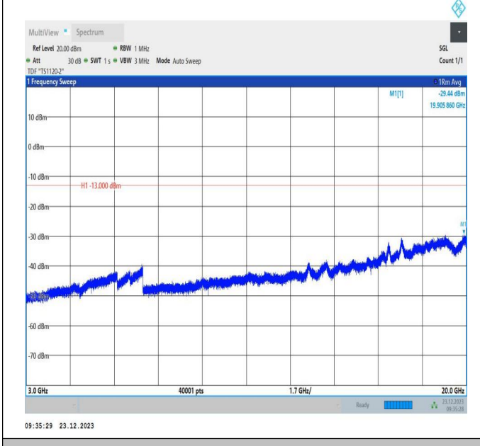
66-66-20MHz-5MHz-16QAM-16QAM-132522-132639-100RB #0-25RB#0-3000~20000MHz-PASS
