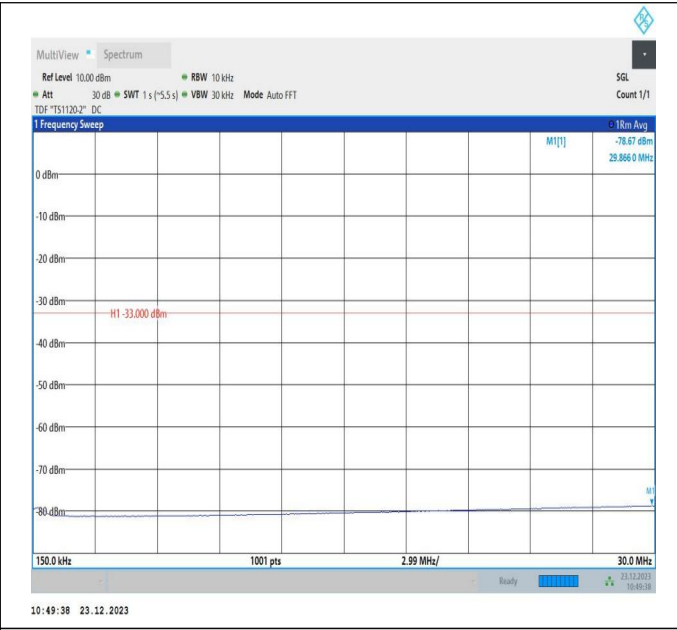
66-66-20MHz-10MHz-16QAM-16QAM-132072-132216-1RB# 99-ORB#0-0.15~30MHz-PASS
