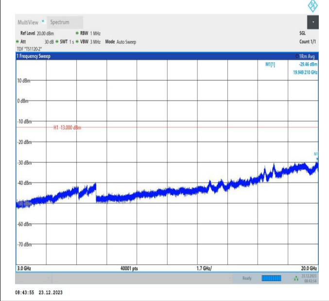
66-66-20MHz-5MHz-16QAM-16QAM-132522-132639-1RB#0 -1RB#24-3000~20000MHz-PASS
