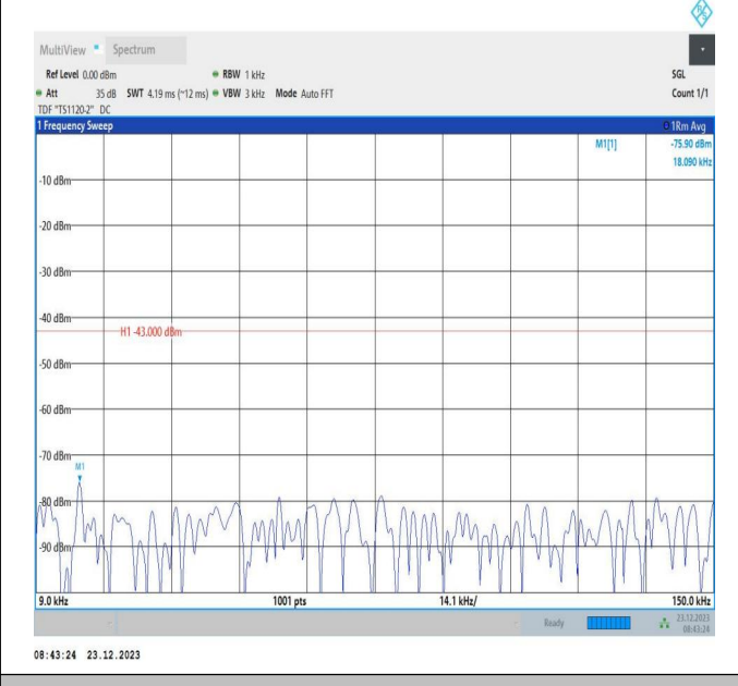
66-66-20MHz-5MHz-16QAM-16QAM-132522-132639-1RB#0-1 -1RB#24-0.009~0.15MHz-PASS
