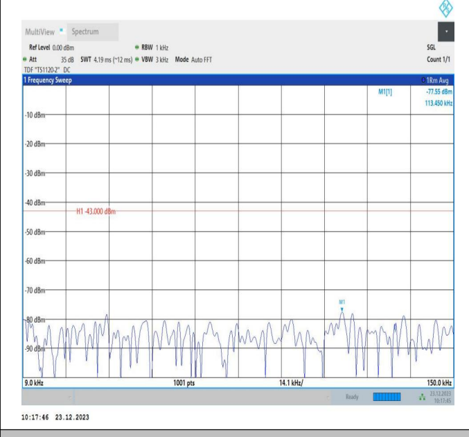
66-66-20MHz-5MHz-64QAM-64QAM-132522-132639-100RB #0-25RB#0-0.009~0.15MHz-PASS
