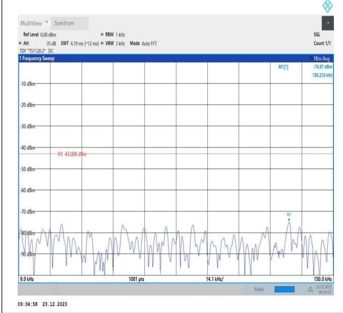
66-66-20MHz-5MHz-16QAM-16QAM-132522-132639-100RB #0-25RB#0-0.009~0.15MHz-PASS
