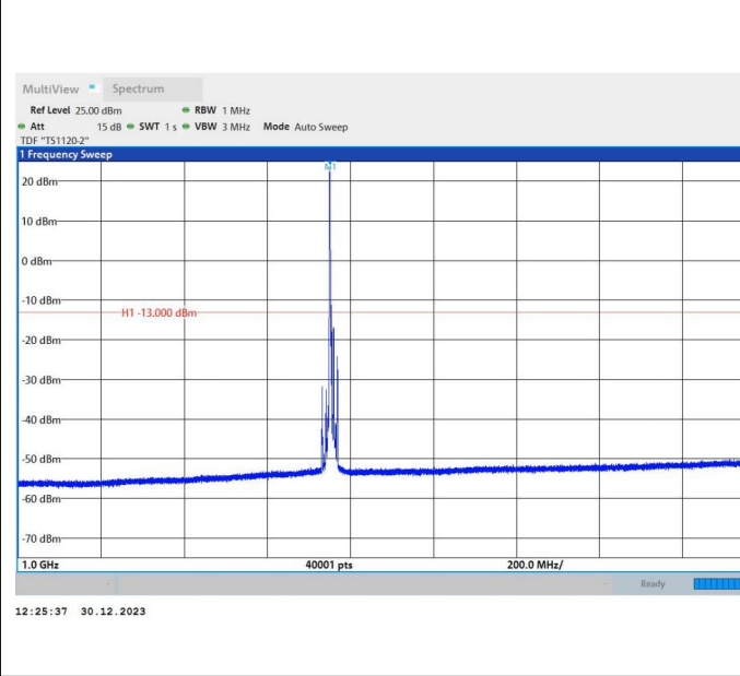
66-66-20MHz-5MHz-64QAM-64QAM-132522-132639-1RB#0 -1RB#24-1000~3000MHz-PASS
