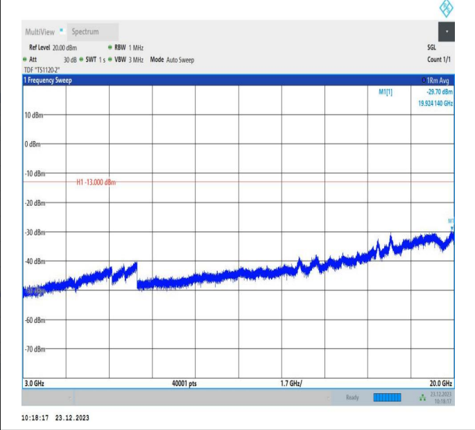
66-66-20MHz-5MHz-64QAM-64QAM-132522-132639-100RB #0-25RB#0-3000~20000MHz-PASS
