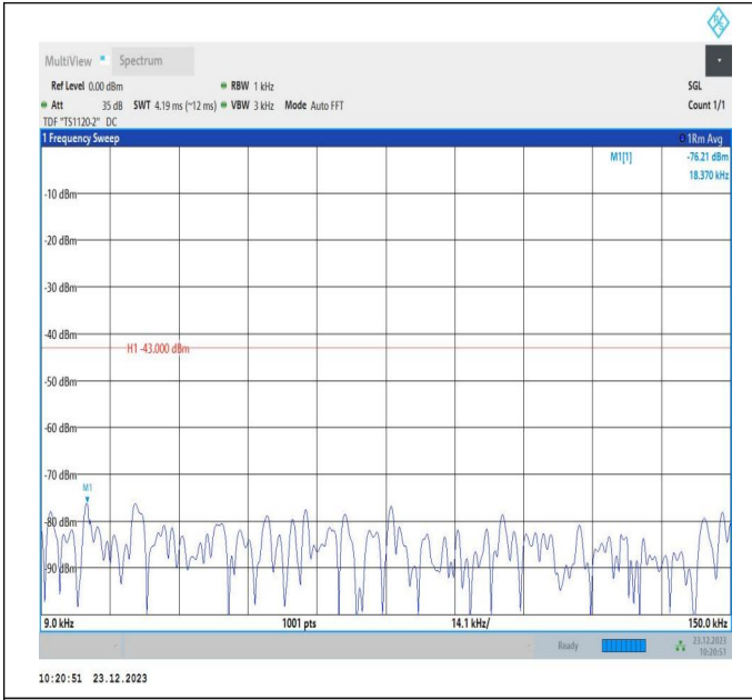
66-66-20MHz-10MHz-16QAM-16QAM-132072-132216-1RB#0-0RB#0-0.009~0.15MHz-PASS
