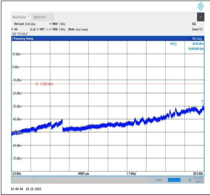
66-66-20MHz-10MHz-16QAM-16QAM-132072-132216-1RB# 99-0RB#0-3000~20000MHz-PASS
