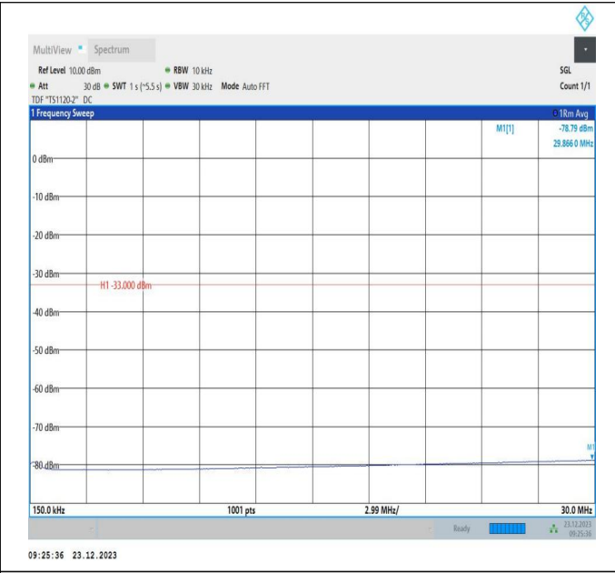
66-66-20MHz-5MHz-64QAM-64QAM-132522-132639-1RB#0 -1RB#24-0.15~30MHz-PASS
