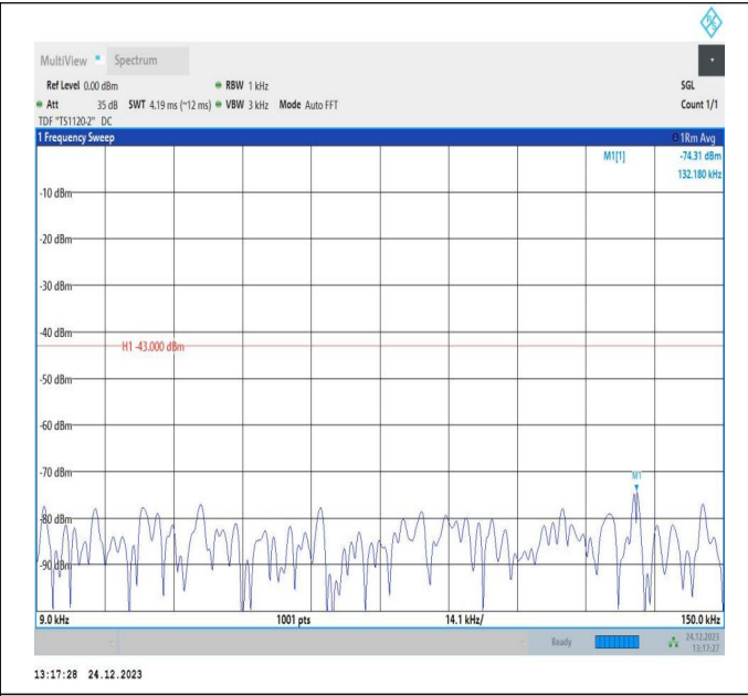
66-66-20MHz-10MHz-QPSK-QPSK-132072-132216-1RB#0- 1RB#49-0.009~0.15MHz-PASS
