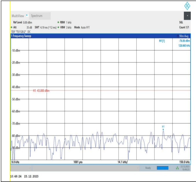
66-66-20MHz-10MHz-16QAM-16QAM-132072-132216-1RB# 99-ORB#0-0.009~0.15MHz-PASS
