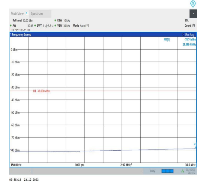
66-66-20MHz-5MHz-16QAM-16QAM-132522-132639-100RB #0-25RB#0-0.15~30MHz-PASS
