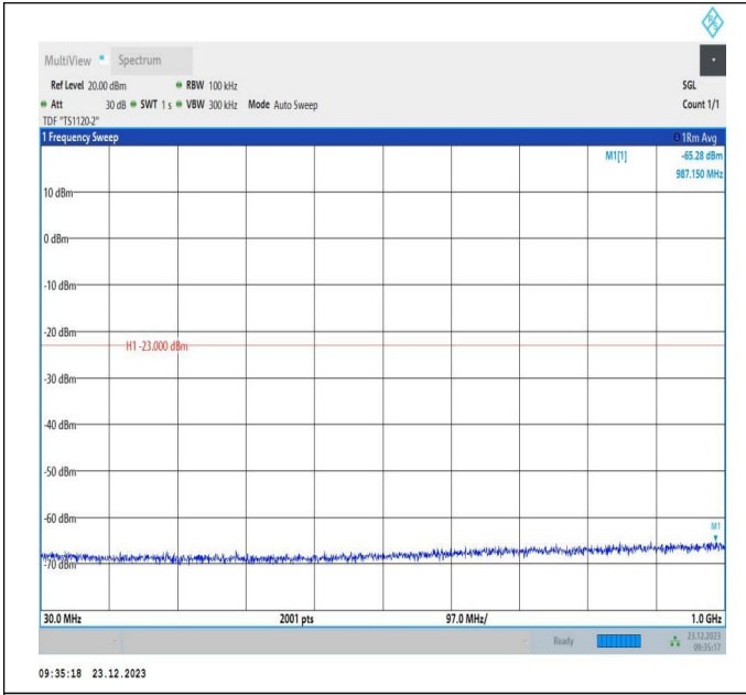
66-66-20MHz-5MHz-16QAM-16QAM-132522-132639-100RB #0-25RB#0-30~1000MHz-PASS
