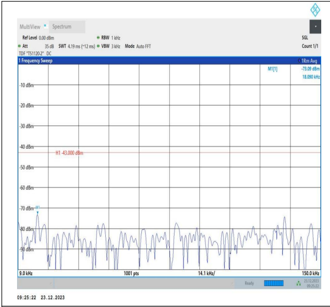
66-66-20MHz-5MHz-64QAM-64QAM-132522-132639-1RB#0 -1RB#24-0.009~0.15MHz-PASS
