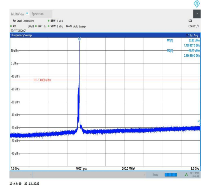
66-66-20MHz-10MHz-16QAM-16QAM-132072-132216-1RB# 99-ORB#0-1000~3000MHz-PASS
