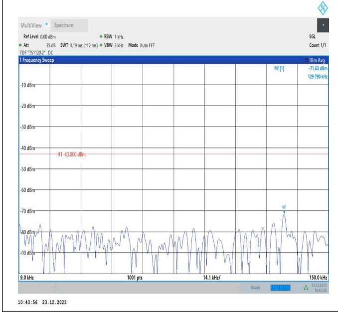
66-66-20MHz-10MHz-64QAM-64QAM-132072-132216-1RB# 0-ORB#0-0.009~0.15MHz-PASS
