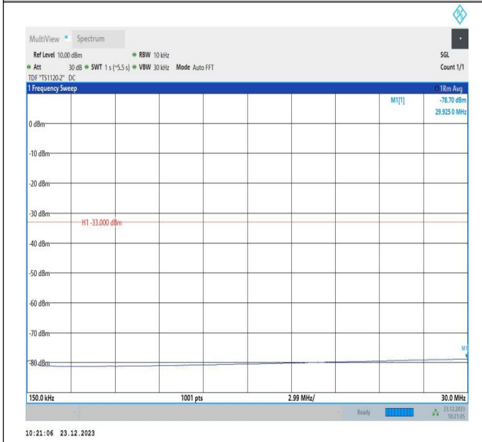
66-66-20MHz-10MHz-16QAM-16QAM-132072-132216-1RB#0-ORB#0-0.15~30MHz-PASS
