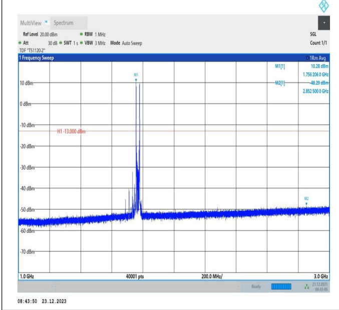
66-66-20MHz-5MHz-16QAM-16QAM-132522-132639-1RB#0 -1RB#24-1000~3000MHz-PASS
