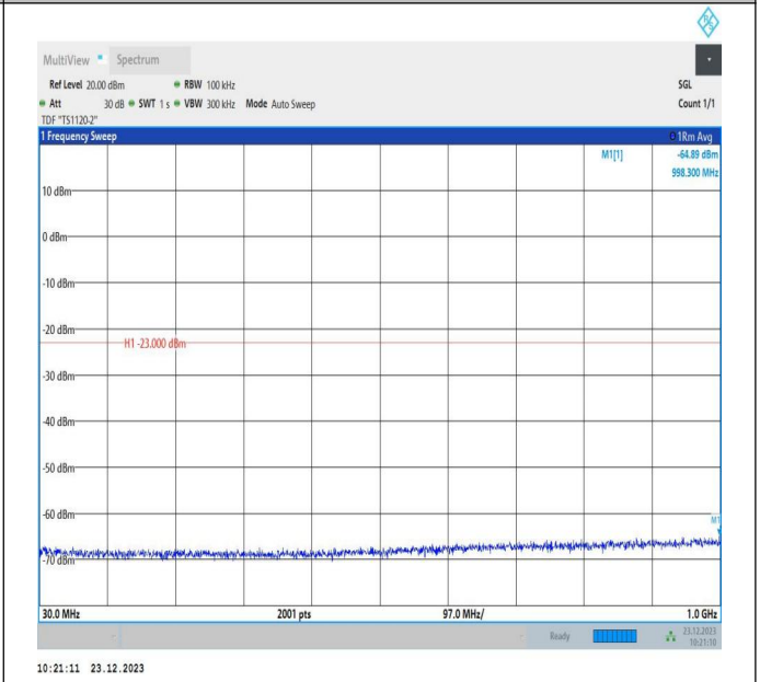
66-66-20MHz-10MHz-16QAM-16QAM-132072-132216-1RB#0-ORB#0-30~1000MHz-PASS
