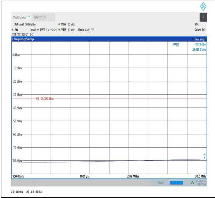
66-66-20MHz-5MHz-64QAM-64QAM-132522-132639-100RB #0-25RB#0-0.15~30MHz-PASS
