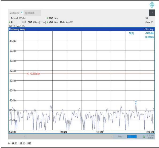
66-66-20MHz-5MHz-16QAM-16QAM-132397-132514-1RB#9 9-ORB#0-0.009~0.15MHz-PASS
