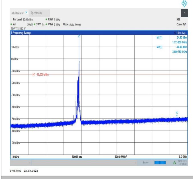
66-66-20MHz-5MHz-QPSK-QPSK-132522-132639-1RB#99-ORB#0-1000~3000MHz-PASS
