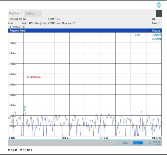
66-66-20MHz-5MHz-64QAM-64QAM-132522-132639-1RB#9 9-ORB#0-0.009~0.15MHz-PASS
