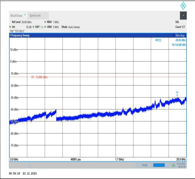
66-66-20MHz-5MHz-64QAM-64QAM-132522-132639-1RB#9 9-0RB#0-3000~20000MHz-PASS
