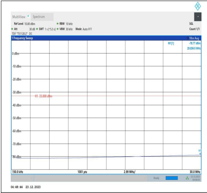
66-66-20MHz-5MHz-QPSK-QPSK-132397-132514-1RB#99-ORB#0-0.15~30MHz-PASS
