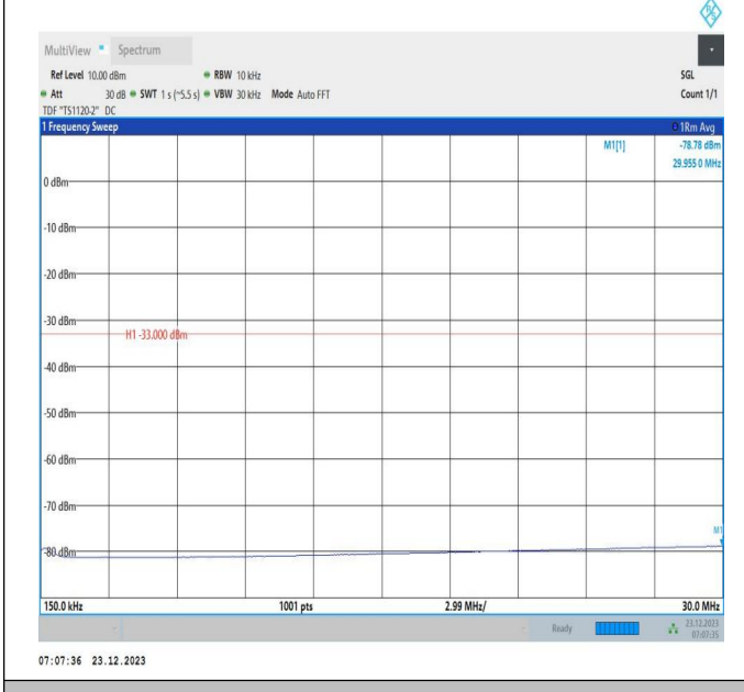
66-66-20MHz-5MHz-16QAM-16QAM-132522-132639-1RB#0-0-RB#0-0.15~30MHz-PASS
