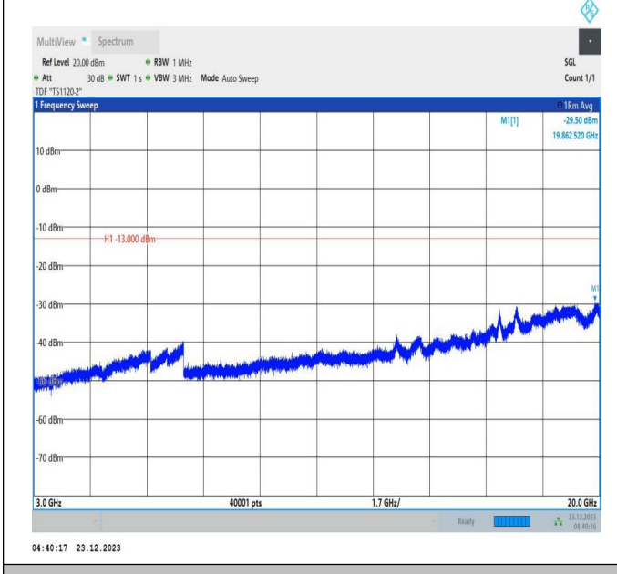
66-66-20MHz-5MHz-64QAM-64QAM-132397-132514-1RB#0 -ORB#0-3000~20000MHz-PASS
