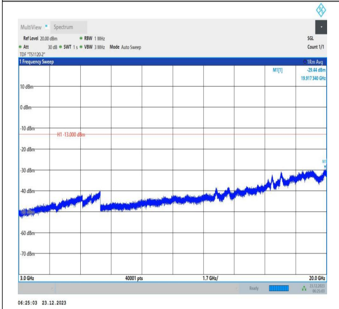
66-66-20MHz-5MHz-16QAM-16QAM-132397-132514-100RB #0-25RB#0-3000~20000MHz-PASS
