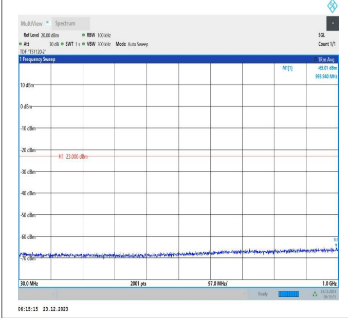
66-66-20MHz-5MHz-64QAM-64QAM-132397-132514-1RB#0 -1RB#24-30~1000MHz-PASS
