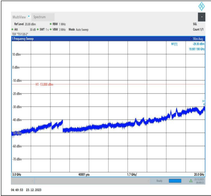
66-66-20MHz-5MHz-16QAM-16QAM-132397-132514-1RB#9 9-ORB#0-3000~20000MHz-PASS
