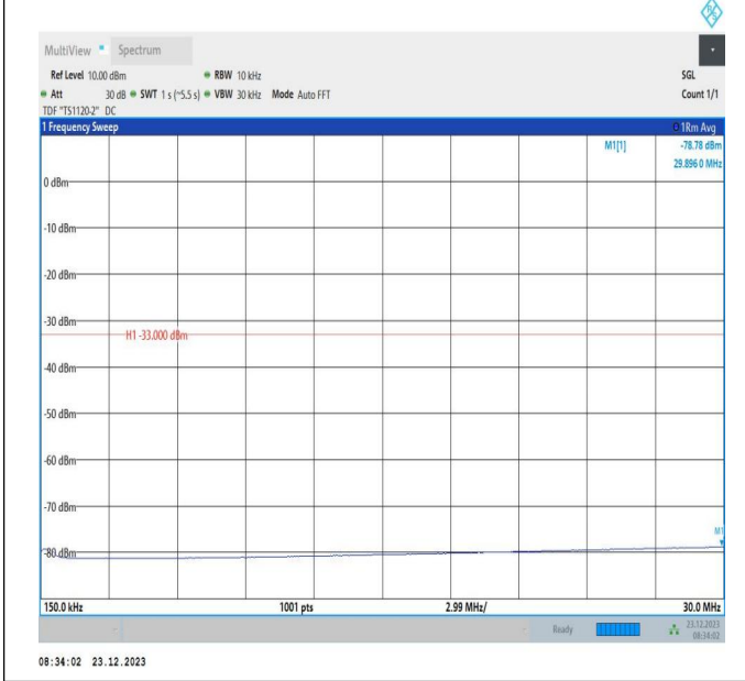
66-66-20MHz-5MHz-64QAM-64QAM-132522-132639-1RB#9 9-ORB#0-0.15~30MHz-PASS
