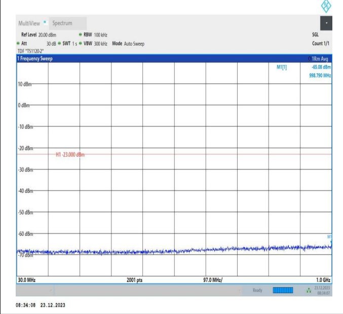
66-66-20MHz-5MHz-64QAM-64QAM-132522-132639-1RB#9 9-ORB#0-30~1000MHz-PASS
