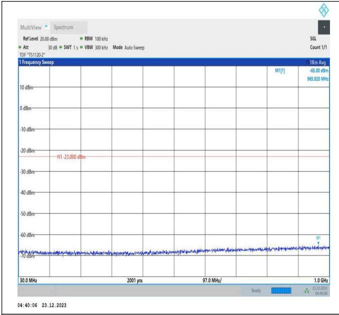
66-66-20MHz-5MHz-64QAM-64QAM-132397-132514-1RB#0 -ORB#0-30~1000MHz-PASS
