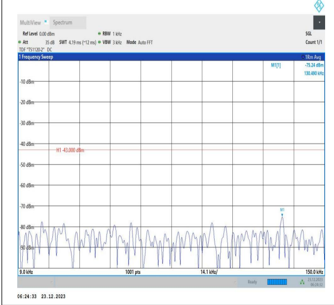
66-66-20MHz-5MHz-16QAM-16QAM-132397-132514-100RB #0-25RB#0-0.009~0.15MHz-PASS
