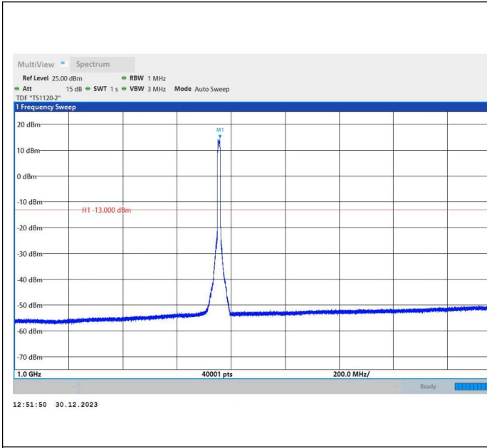
66-66-20MHz-5MHz-64QAM-64QAM-132522-132639-1RB#9 9-0RB#0-1000~3000MHz-PASS
