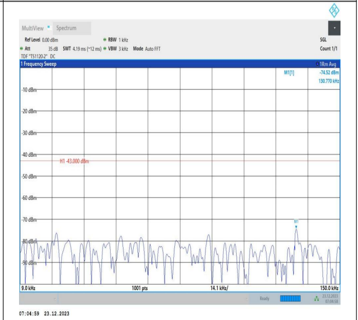
66-66-20MHz-5MHz-64QAM-64QAM-132397-132514-100RB #0-25RB#0-0.009~0.15MHz-PASS
