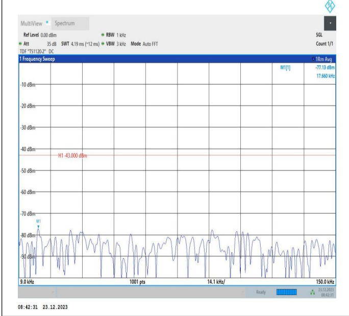
66-66-20MHz-5MHz-QPSK-QPSK-132522-132639-1RB#0-1 RB#24-0.009~0.15MHz-PASS
