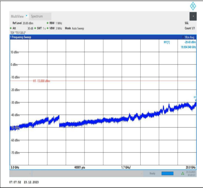
66-66-20MHz-5MHz-16QAM-16QAM-132522-132639-1RB#0 -ORB#0-3000~20000MHz-PASS
