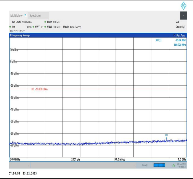
66-66-20MHz-5MHz-QPSK-QPSK-132522-132639-1RB#99-ORB#0-30~1000MHz-PASS
