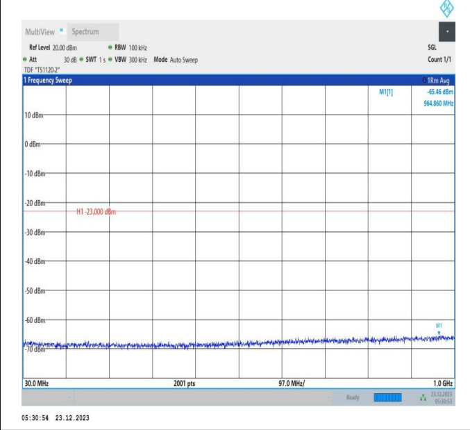
66-66-20MHz-5MHz-64QAM-64QAM-132397-132514-1RB#9 9-ORB#0-30~1000MHz-PASS
