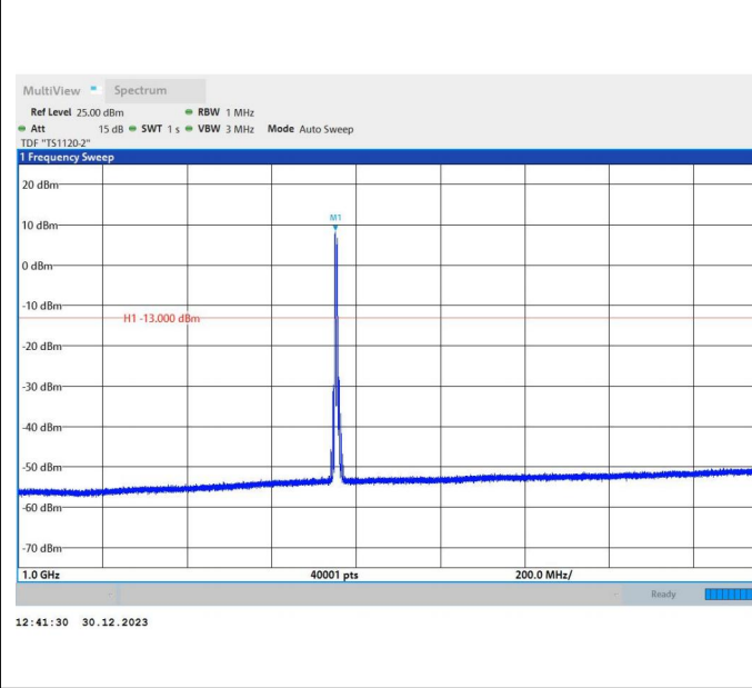
66-66-20MHz-5MHz-64QAM-64QAM-132397-132514-1RB#0 -1RB#24-1000~3000MHz-PASS
