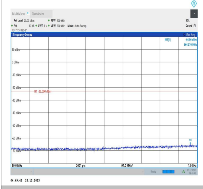
66-66-20MHz-5MHz-16QAM-16QAM-132397-132514-1RB#9 9-ORB#0-30~1000MHz-PASS
