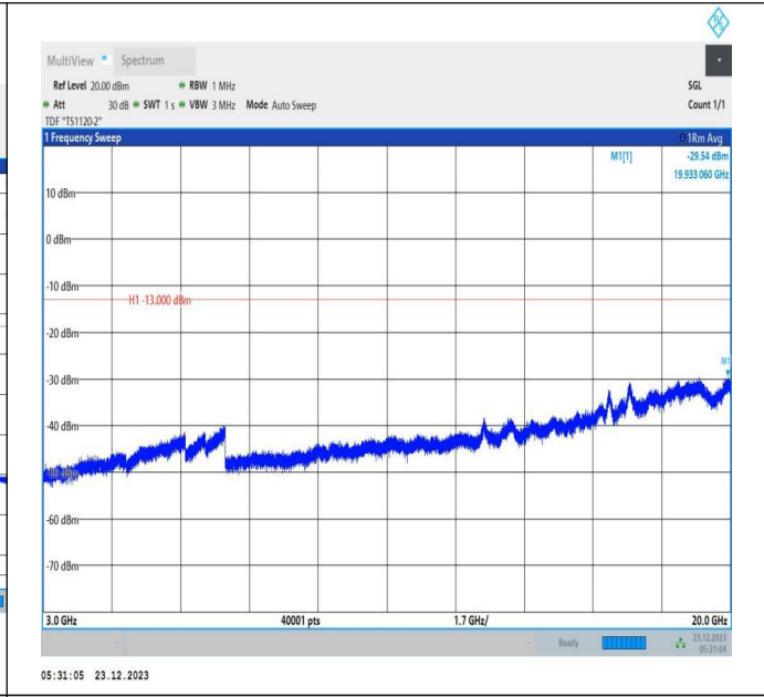
66-66-20MHz-5MHz-64QAM-64QAM-132397-132514-1RB#9 9-0RB#0-3000~20000MHz-PASS
