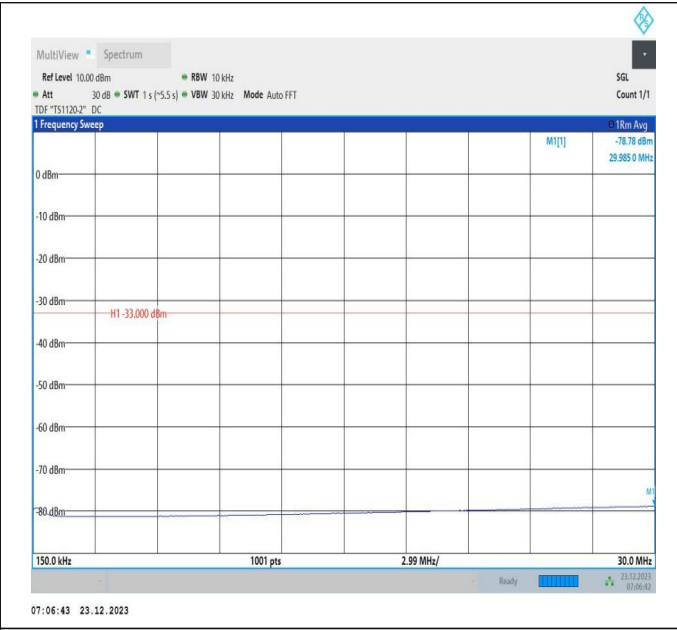
66-66-20MHz-5MHz-QPSK-QPSK-132522-132639-1RB#0-0 RB#0-0.15~30MHz-PASS
