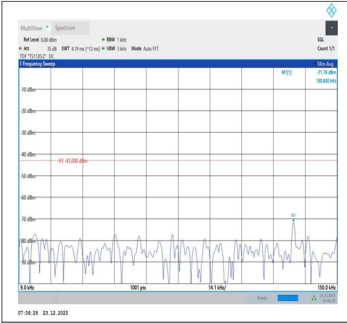
66-66-20MHz-5MHz-QPSK-QPSK-132522-132639-1RB#0-0 RB#0-0.009~0.15MHz-PASS
