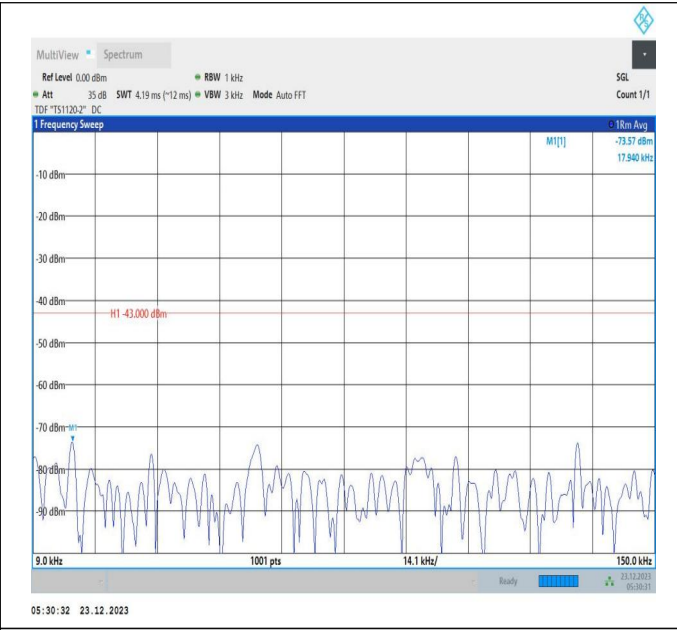
66-66-20MHz-5MHz-64QAM-64QAM-132397-132514-1RB#9 9-ORB#0-0.009~0.15MHz-PASS
