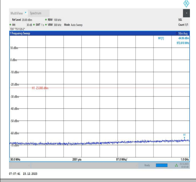
66-66-20MHz-5MHz-16QAM-16QAM-132522-132639-1RB#0-0-RB#0-30~1000MHz-PASS
