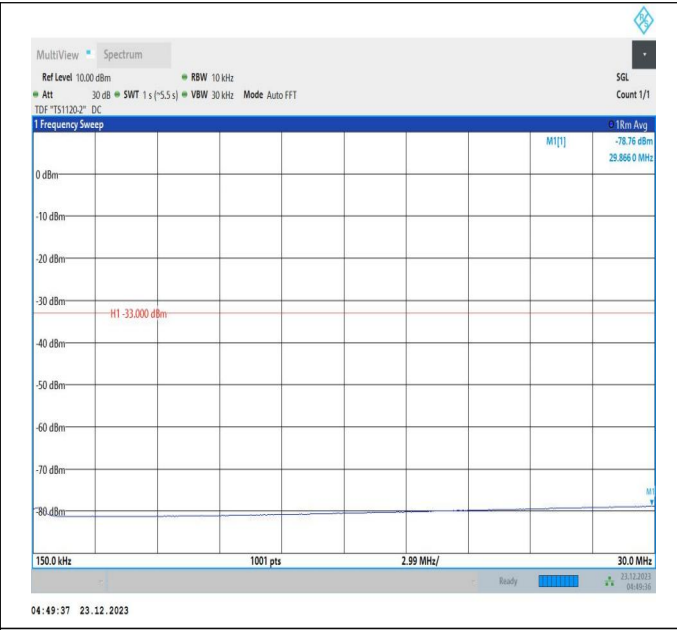
66-66-20MHz-5MHz-16QAM-16QAM-132397-132514-1RB#9 9-ORB#0-0.15~30MHz-PASS
