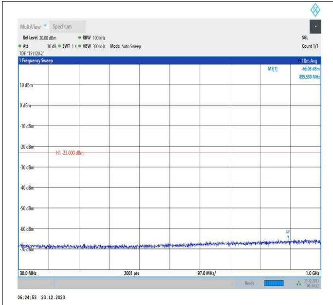
66-66-20MHz-5MHz-16QAM-16QAM-132397-132514-100RB #0-25RB#0-30~1000MHz-PASS
