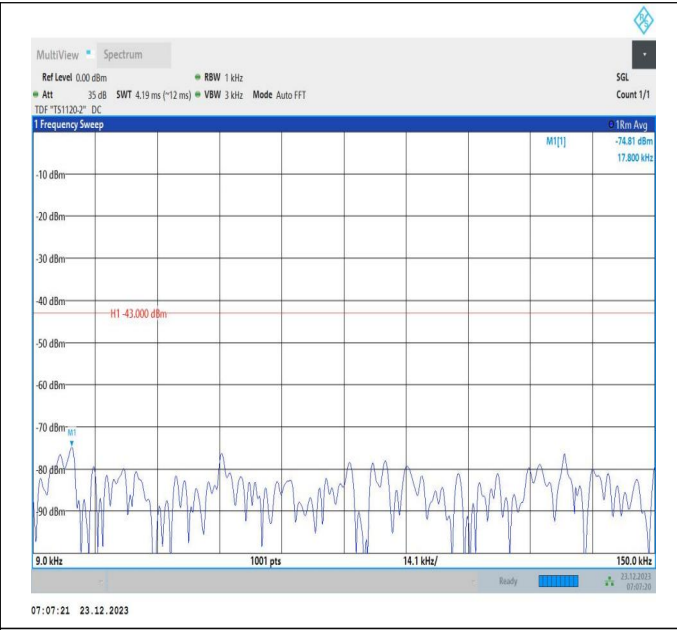
66-66-20MHz-5MHz-16QAM-16QAM-132522-132639-1RB#0-0-RB#0-0.009~0.15MHz-PASS
