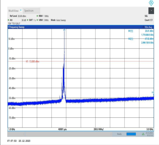
66-66-20MHz-5MHz-16QAM-16QAM-132522-132639-1RB#9 9-ORB#0-1000~3000MHz-PASS
