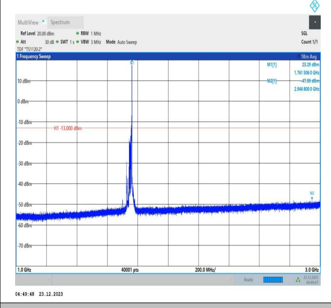
66-66-20MHz-5MHz-16QAM-16QAM-132397-132514-1RB#9 9-ORB#0-1000~3000MHz-PASS
