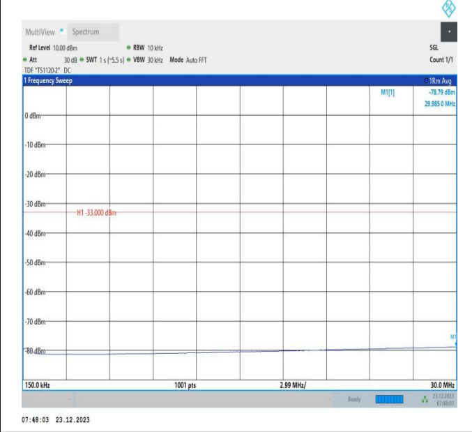
66-66-20MHz-5MHz-64QAM-64QAM-132522-132639-1RB#0 -ORB#0-0.15~30MHz-PASS
