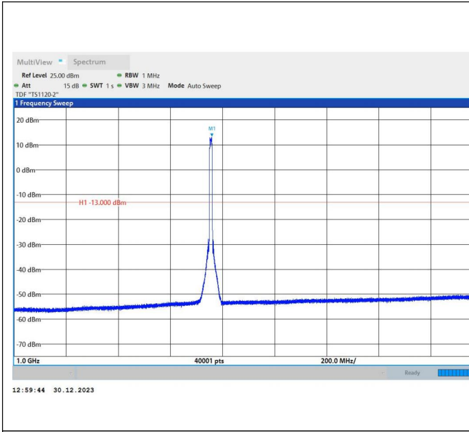
66-66-20MHz-5MHz-64QAM-64QAM-132397-132514-1RB#9 9-0RB#0-1000~3000MHz-PASS
