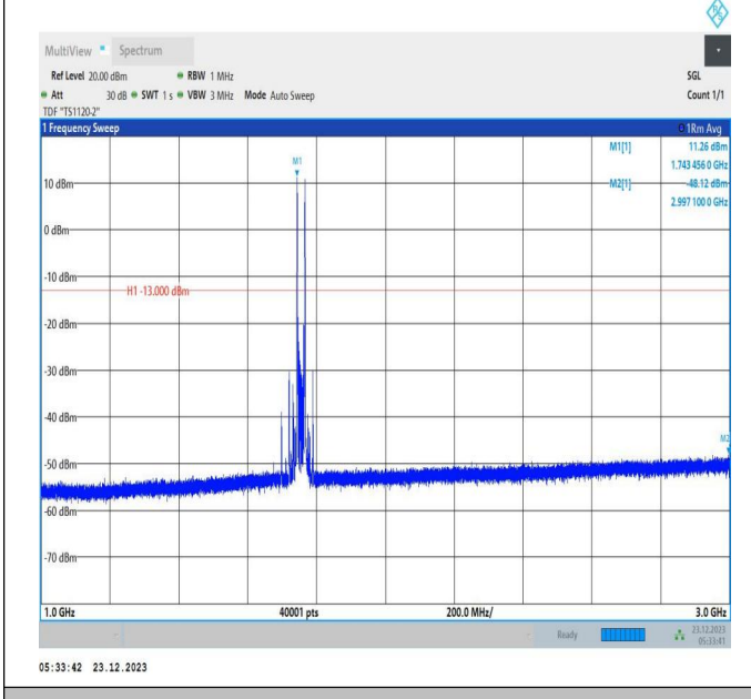
66-66-20MHz-5MHz-16QAM-16QAM-132397-132514-1RB#0 -1RB#24-1000~3000MHz-PASS
