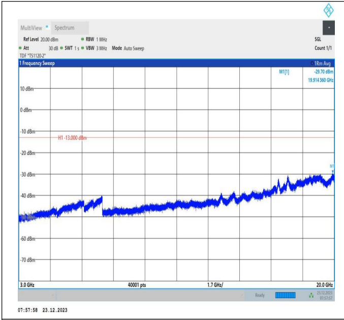
66-66-20MHz-5MHz-16QAM-16QAM-132522-132639-1RB#9 9-ORB#0-3000~20000MHz-PASS
