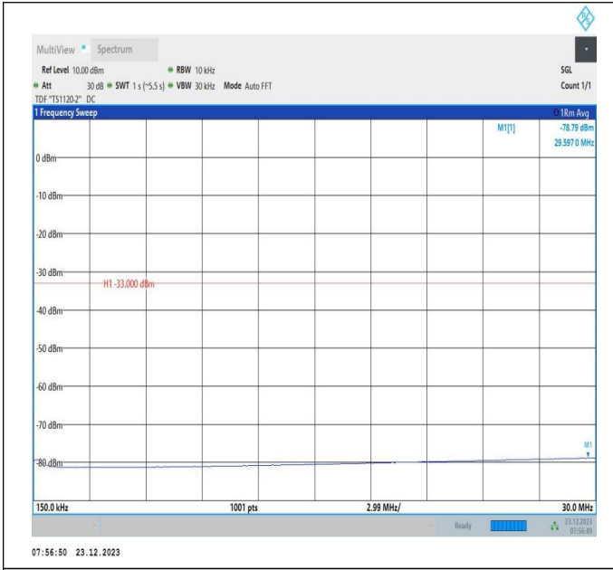
66-66-20MHz-5MHz-QPSK-QPSK-132522-132639-1RB#99-ORB#0-0.15~30MHz-PASS
