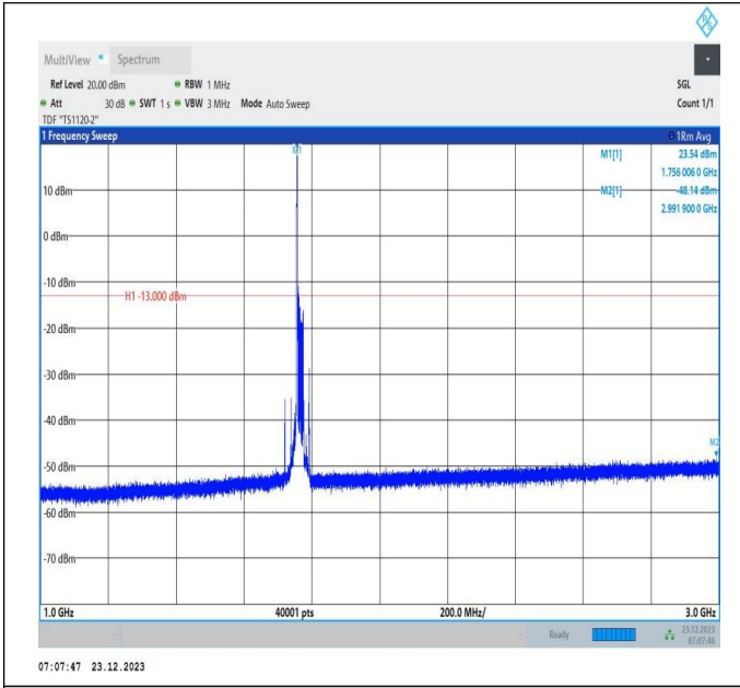
66-66-20MHz-5MHz-16QAM-16QAM-132522-132639-1RB#0 -ORB#0-1000~3000MHz-PASS
