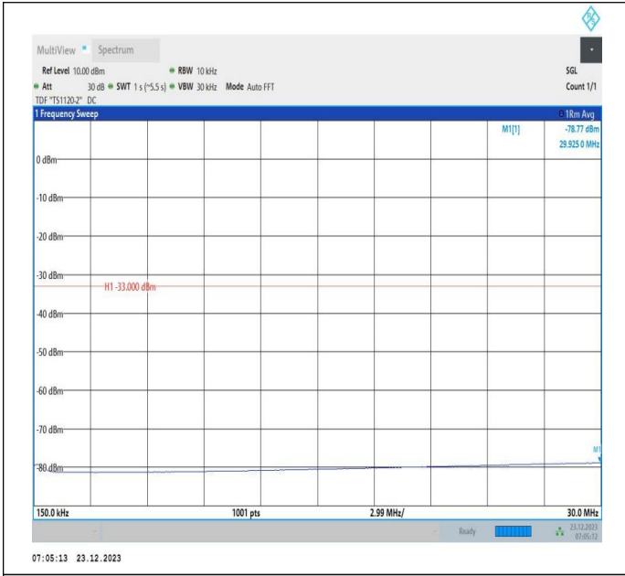
66-66-20MHz-5MHz-64QAM-64QAM-132397-132514-100RB #0-25RB#0-0.15~30MHz-PASS
