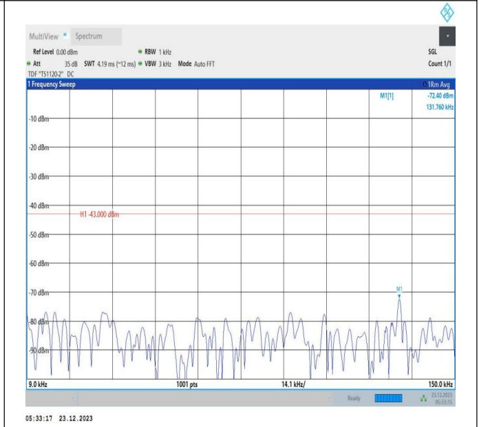
66-66-20MHz-5MHz-16QAM-16QAM-132397-132514-1RB#0-1 -1RB#24-0.009~0.15MHz-PASS
