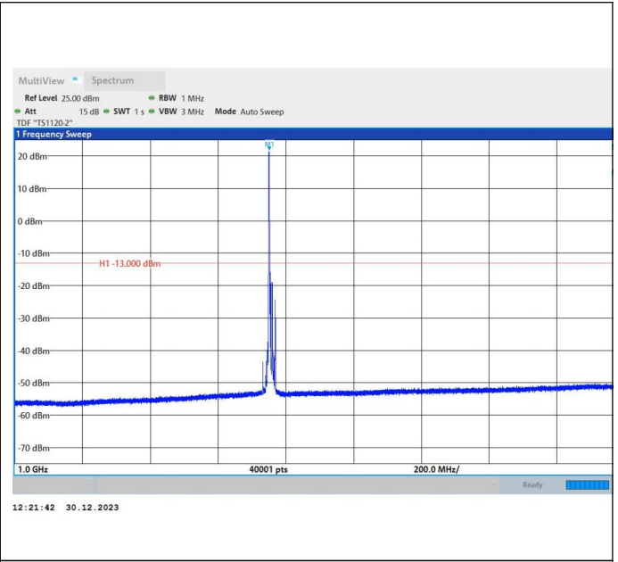
66-66-20MHz-5MHz-64QAM-64QAM-132522-132639-1RB#0 -ORB#0-1000~3000MHz-PASS
