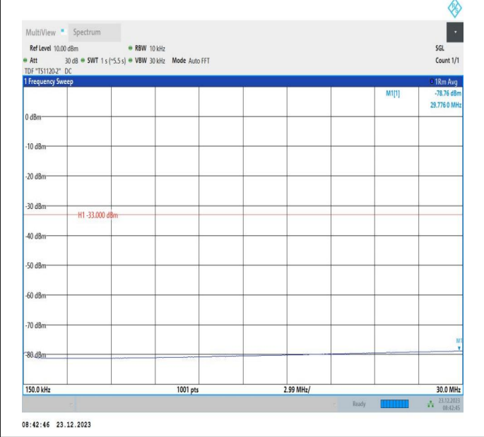
66-66-20MHz-5MHz-QPSK-QPSK-132522-132639-1RB#0-1 RB#24-0.15~30MHz-PASS
