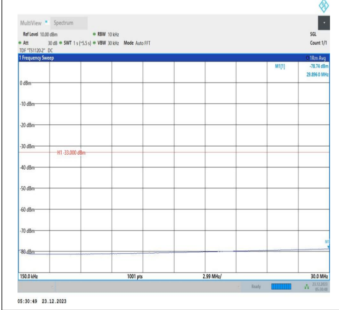
66-66-20MHz-5MHz-64QAM-64QAM-132397-132514-1RB#9 9-ORB#0-0.15~30MHz-PASS
