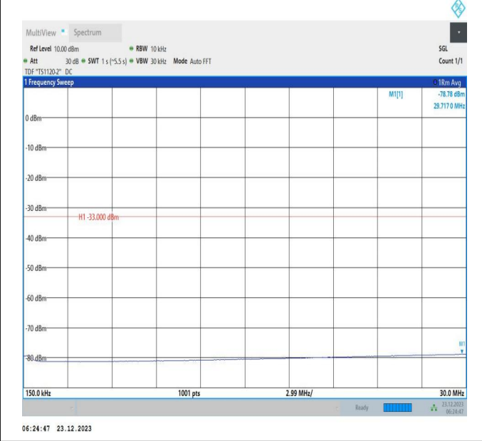
66-66-20MHz-5MHz-16QAM-16QAM-132397-132514-100RB #0-25RB#0-0.15~30MHz-PASS
