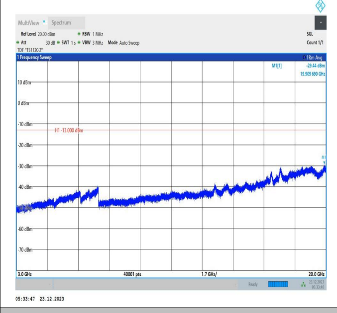
66-66-20MHz-5MHz-16QAM-16QAM-132397-132514-1RB#0 -1RB#24-3000~20000MHz-PASS
