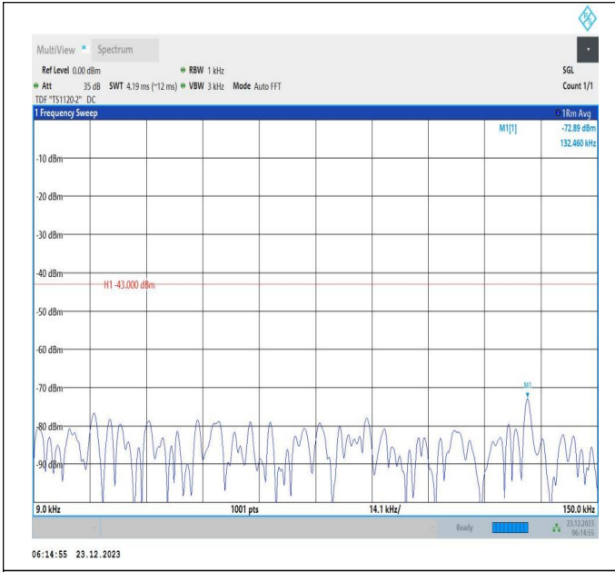
66-66-20MHz-5MHz-64QAM-64QAM-132397-132514-1RB#0 -1RB#24-0.009~0.15MHz-PASS
