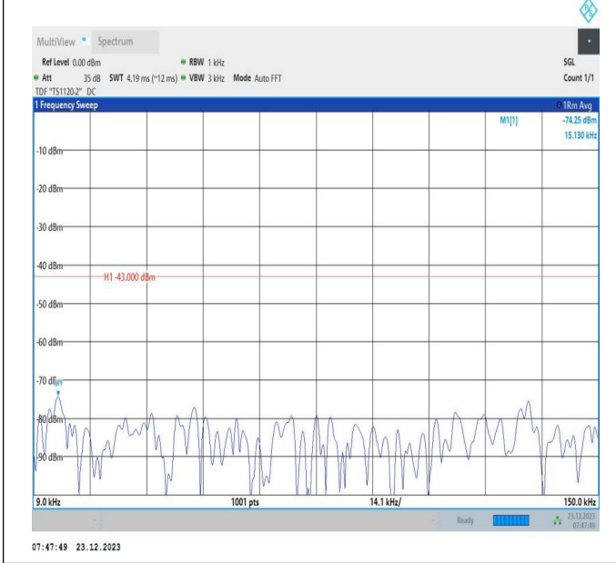
66-66-20MHz-5MHz-64QAM-64QAM-132522-132639-1RB#0 -ORB#0-0.009~0.15MHz-PASS
