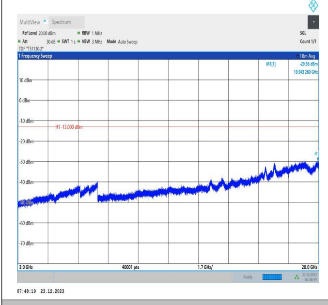
66-66-20MHz-5MHz-64QAM-64QAM-132522-132639-1RB#0 -ORB#0-3000~20000MHz-PASS
