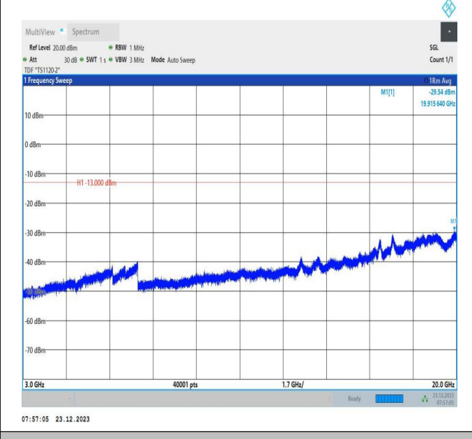
66-66-20MHz-5MHz-QPSK-QPSK-132522-132639-1RB#99-ORB#0-3000~20000MHz-PASS
