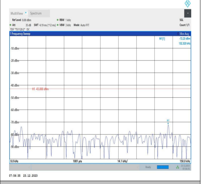
66-66-20MHz-5MHz-QPSK-QPSK-132522-132639-1RB#99- ORB#0-0.009~0.15MHz-PASS
