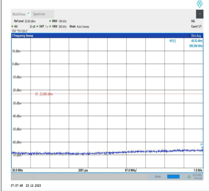
66-66-20MHz-5MHz-16QAM-16QAM-132522-132639-1RB#9 9-ORB#0-30~1000MHz-PASS
