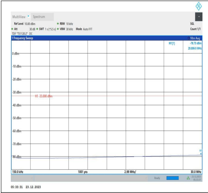
66-66-20MHz-5MHz-16QAM-16QAM-132397-132514-1RB#0 -1RB#24-0.15~30MHz-PASS
