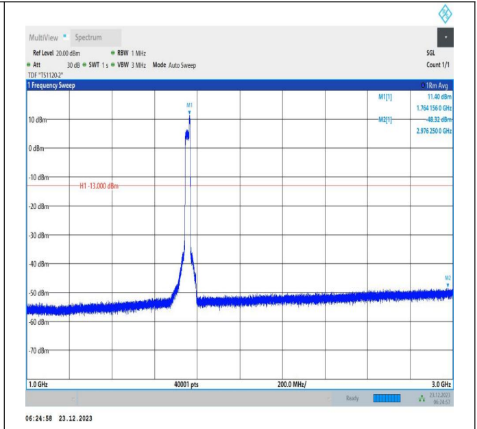
66-66-20MHz-5MHz-16QAM-16QAM-132397-132514-100RB #0-25RB#0-1000~3000MHz-PASS
