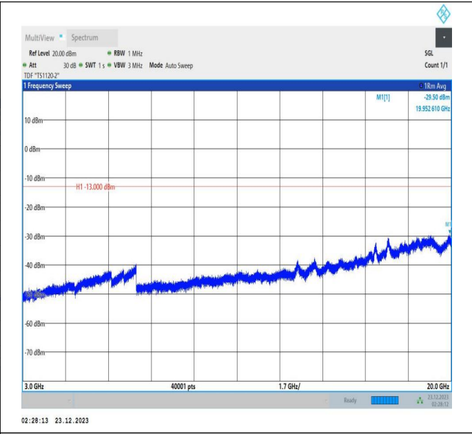
66-66-20MHz-5MHz-64QAM-64QAM-132072-132189-1RB#9 9-0RB#0-3000~20000MHz-PASS
