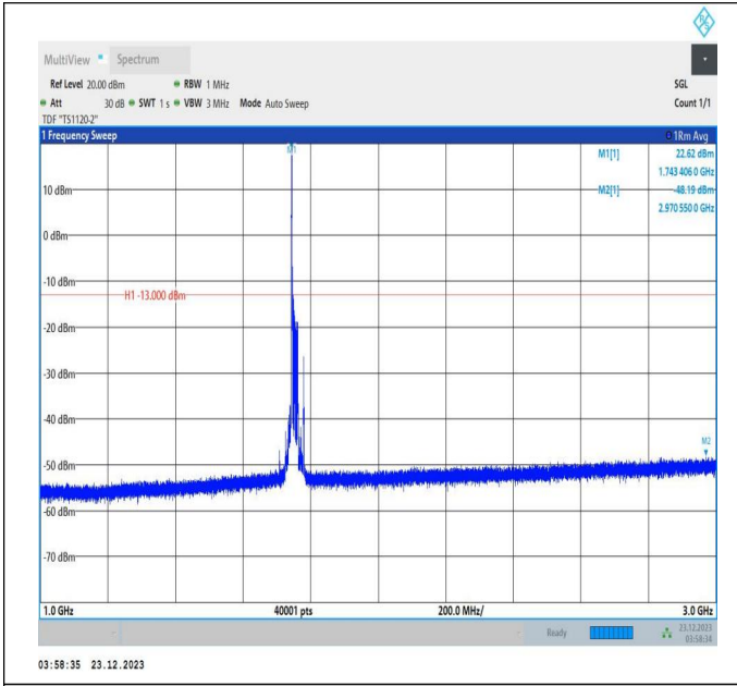
66-66-20MHz-5MHz-16QAM-16QAM-132397-132514-1RB#0 -ORB#0-1000~3000MHz-PASS
