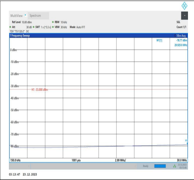
66-66-20MHz-5MHz-64QAM-64QAM-132072-132189-1RB#0 -1RB#24-0.15~30MHz-PASS
