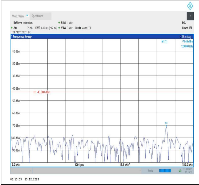
66-66-20MHz-5MHz-64QAM-64QAM-132072-132189-1RB#0 -1RB#24-0.009~0.15MHz-PASS
