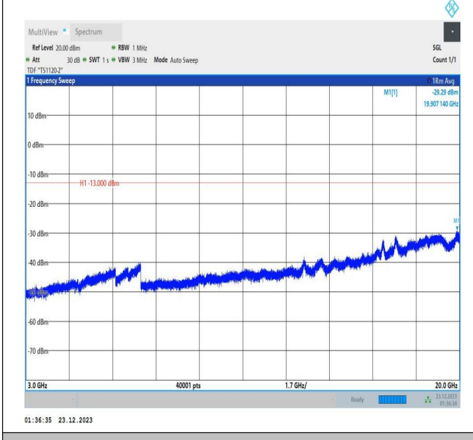
66-66-20MHz-5MHz-64QAM-64QAM-132072-132189-1RB#0 -ORB#0-3000~20000MHz-PASS
