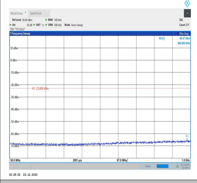
66-66-20MHz-5MHz-64QAM-64QAM-132072-132189-1RB#9 9-ORB#0-30~1000MHz-PASS
