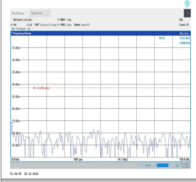
66-66-20MHz-5MHz-64QAM-64QAM-132072-132189-1RB#0 -ORB#0-0.009~0.15MHz-PASS
