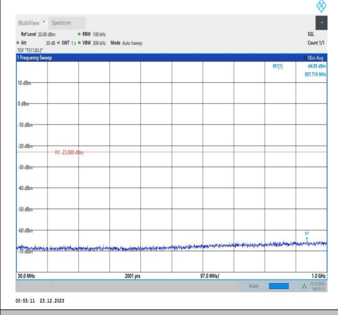
66-66-20MHz-5MHz-16QAM-16QAM-132072-132189-1RB#0-0 -ORB#0-30~1000MHz-PASS
