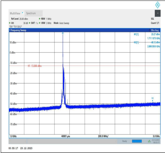
66-66-20MHz-5MHz-16QAM-16QAM-132072-132189-1RB#0 -ORB#0-1000~3000MHz-PASS
