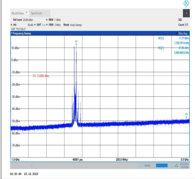
66-66-20MHz-5MHz-16QAM-16QAM-132072-132189-1RB#0 -1RB#24-1000~3000MHz-PASS
