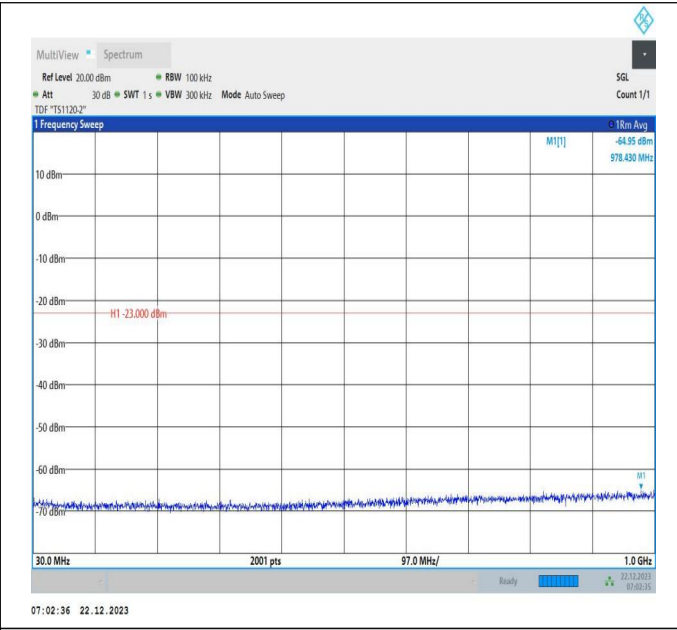
66-66-15MHz-20MHz-64QAM-64QAM-132401-132572-75RB #0-100RB#0-30~1000MHz-PASS
