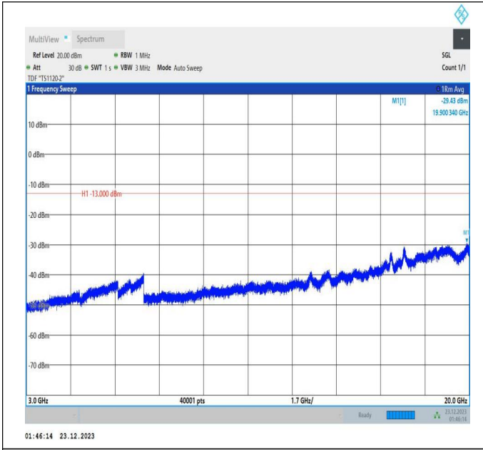
66-66-20MHz-5MHz-16QAM-16QAM-132072-132189-1RB#9 9-ORB#0-3000~20000MHz-PASS
