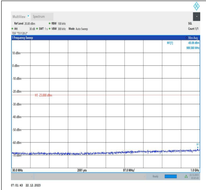
66-66-15MHz-20MHz-16QAM-16QAM-132401-132572-75RB #0-100RB#0-30~1000MHz-PASS
