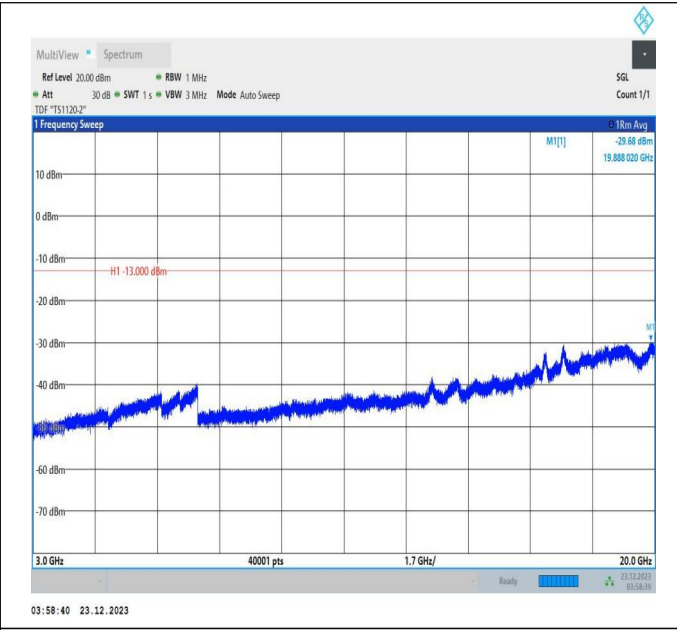
66-66-20MHz-5MHz-16QAM-16QAM-132397-132514-1RB#0 -ORB#0-3000~20000MHz-PASS
