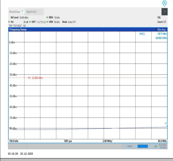
66-66-20MHz-5MHz-16QAM-16QAM-132072-132189-100RB #0-25RB#0-0.15~30MHz-PASS
