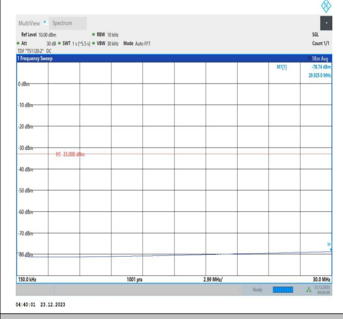
66-66-20MHz-5MHz-64QAM-64QAM-132397-132514-1RB#0 -ORB#0-0.15~30MHz-PASS
