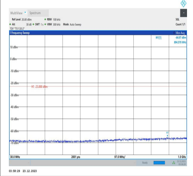
66-66-20MHz-5MHz-16QAM-16QAM-132397-132514-1RB#0-0 -ORB#0-30~1000MHz-PASS
