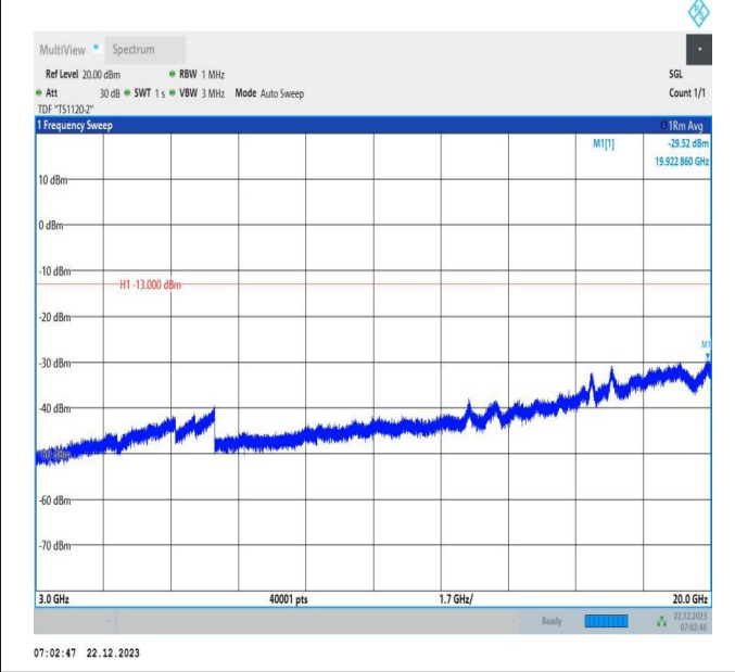
66-66-15MHz-20MHz-64QAM-64QAM-132401-132572-75RB #0-100RB#0-3000~20000MHz-PASS
