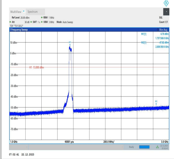
66-66-15MHz-20MHz-64QAM-64QAM-132401-132572-75RB #0-100RB#0-1000~3000MHz-PASS
