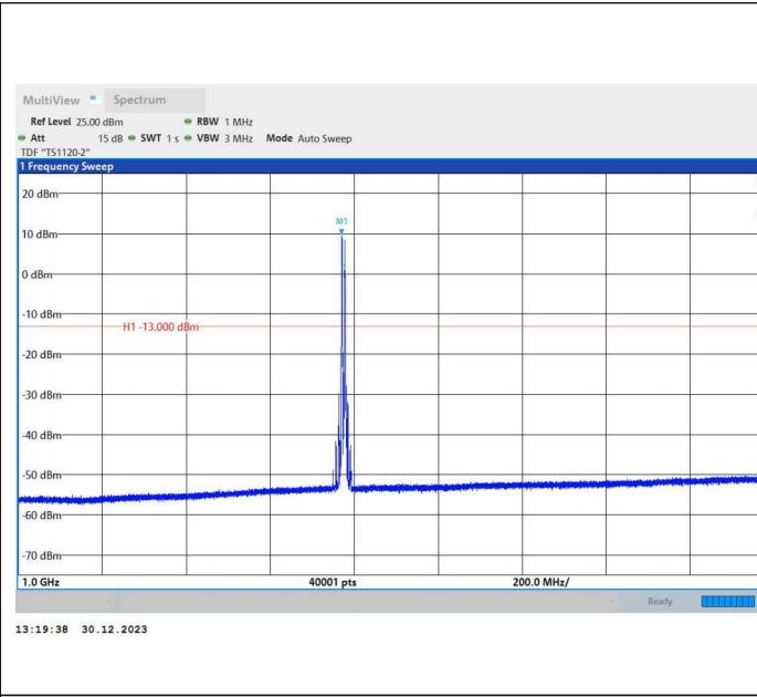
66-66-20MHz-5MHz-64QAM-64QAM-132072-132189-1RB#0 -ORB#0-1000~3000MHz-PASS
