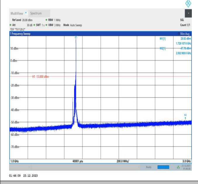
66-66-20MHz-5MHz-16QAM-16QAM-132072-132189-1RB#9 9-ORB#0-1000~3000MHz-PASS
