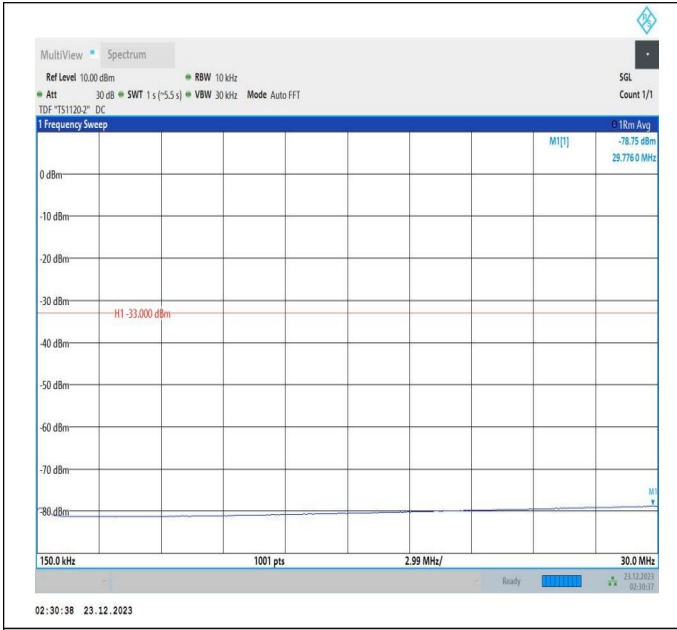
66-66-20MHz-5MHz-16QAM-16QAM-132072-132189-1RB#0 -1RB#24-0.15~30MHz-PASS
