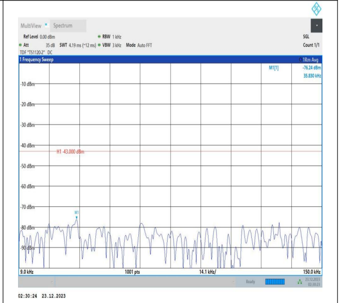
66-66-20MHz-5MHz-16QAM-16QAM-132072-132189-1RB#0-1 -1RB#24-0.009~0.15MHz-PASS
