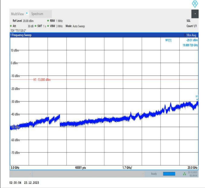
66-66-20MHz-5MHz-16QAM-16QAM-132072-132189-1RB#0 -1RB#24-3000~20000MHz-PASS
