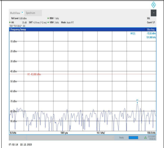
66-66-15MHz-20MHz-64QAM-64QAM-132401-132572-75RB #0-100RB#0-0.009~0.15MHz-PASS
