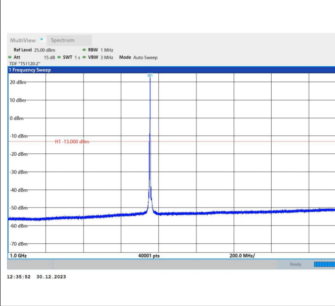
66-66-20MHz-5MHz-64QAM-64QAM-132072-132189-1RB#0 -1RB#24-1000~3000MHz-PASS
