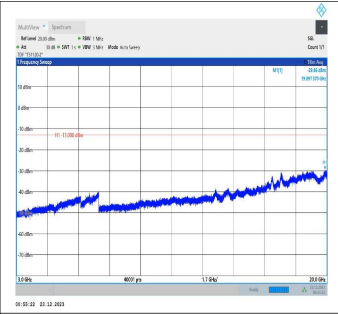
66-66-20MHz-5MHz-16QAM-16QAM-132072-132189-1RB#0 -ORB#0-3000~20000MHz-PASS
