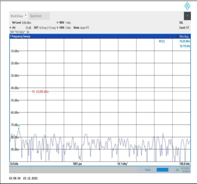
66-66-20MHz-5MHz-16QAM-16QAM-132397-132514-1RB#0-0 -ORB#0-0.009~0.15MHz-PASS
