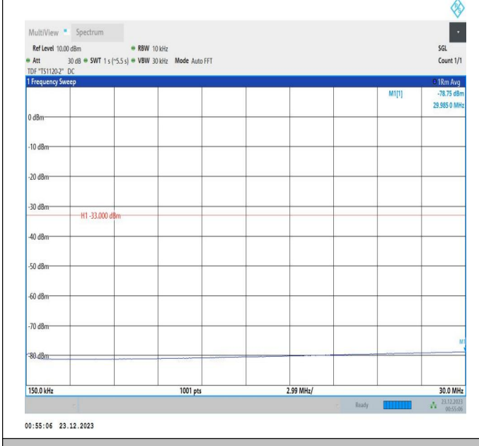
66-66-20MHz-5MHz-16QAM-16QAM-132072-132189-1RB#0-0 -ORB#0-0.15~30MHz-PASS
