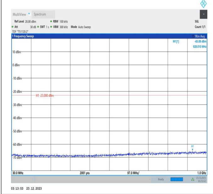
66-66-20MHz-5MHz-64QAM-64QAM-132072-132189-1RB#0 -1RB#24-30~1000MHz-PASS
