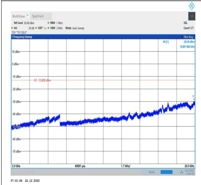
66-66-15MHz-20MHz-16QAM-16QAM-132401-132572-75RB #0-100RB#0-3000~20000MHz-PASS
