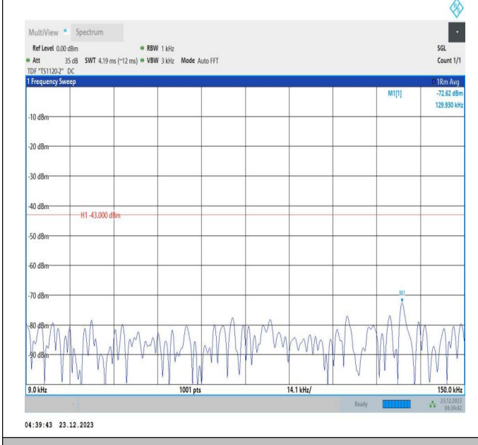
66-66-20MHz-5MHz-64QAM-64QAM-132397-132514-1RB#0 -ORB#0-0.009~0.15MHz-PASS
