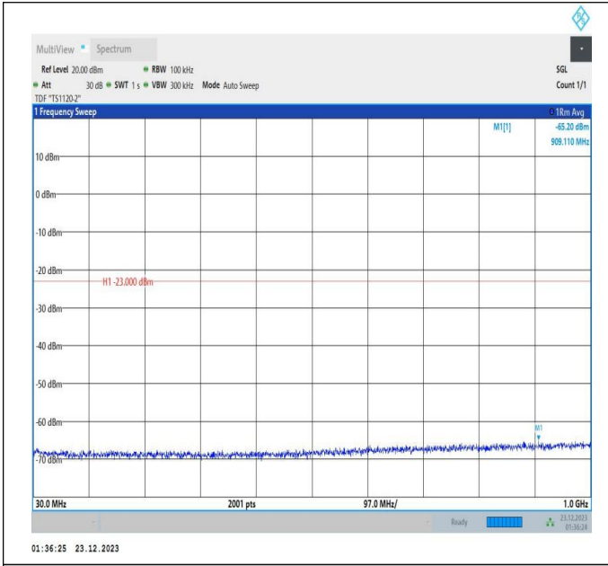
66-66-20MHz-5MHz-64QAM-64QAM-132072-132189-1RB#0 -ORB#0-30~1000MHz-PASS
