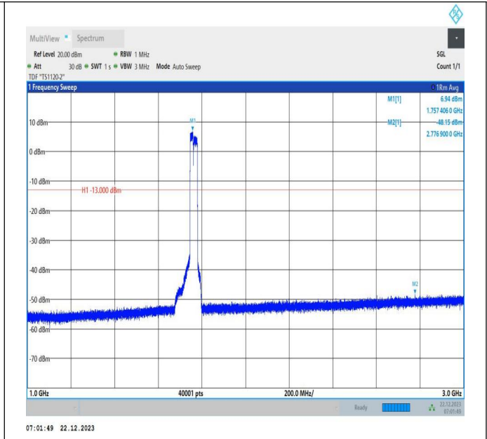
66-66-15MHz-20MHz-16QAM-16QAM-132401-132572-75RB #0-100RB#0-1000~3000MHz-PASS
