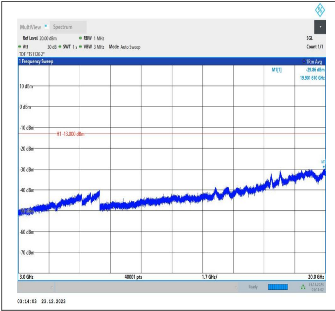
66-66-20MHz-5MHz-64QAM-64QAM-132072-132189-1RB#0 -1RB#24-3000~20000MHz-PASS
