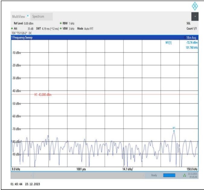
66-66-20MHz-5MHz-16QAM-16QAM-132072-132189-1RB#9 9-ORB#0-0.009~0.15MHz-PASS
