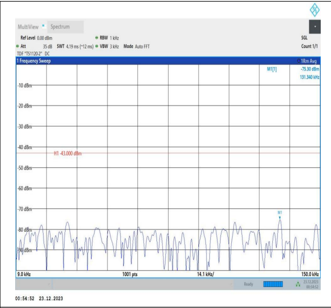
66-66-20MHz-5MHz-16QAM-16QAM-132072-132189-1RB#0-0 -ORB#0-0.009~0.15MHz-PASS
