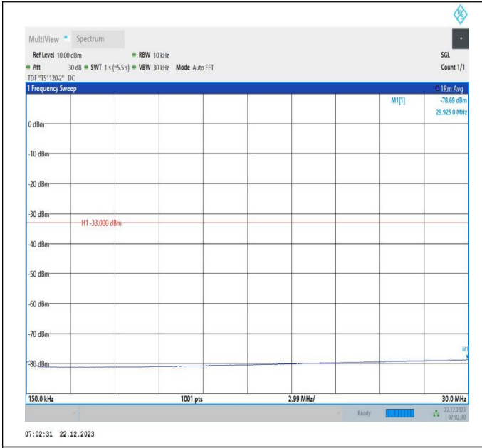
66-66-15MHz-20MHz-64QAM-64QAM-132401-132572-75RB #0-100RB#0-0.15~30MHz-PASS
