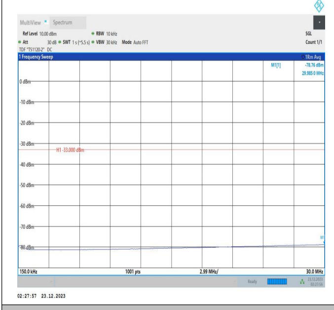
66-66-20MHz-5MHz-64QAM-64QAM-132072-132189-1RB#9 9-ORB#0-0.15~30MHz-PASS
