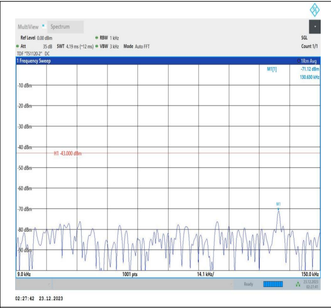
66-66-20MHz-5MHz-64QAM-64QAM-132072-132189-1RB#9 9-ORB#0-0.009~0.15MHz-PASS
