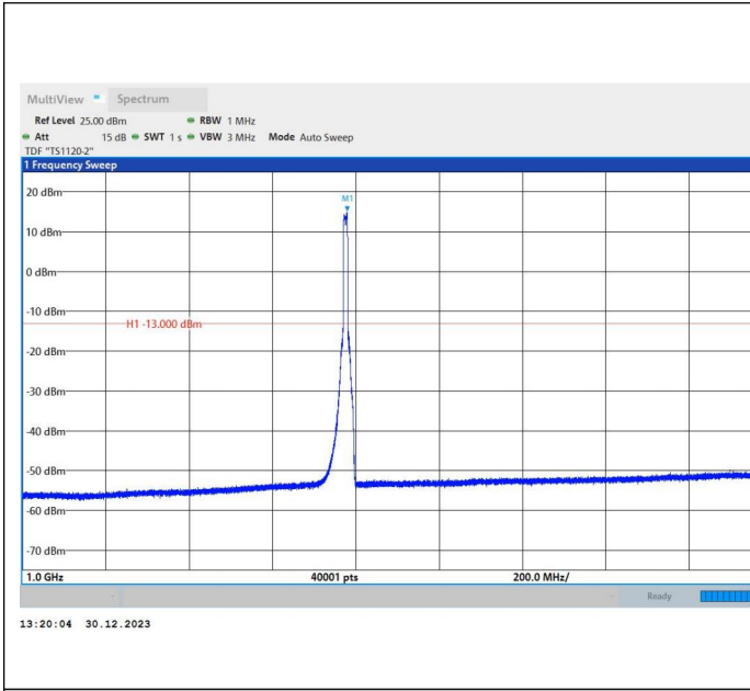
66-66-20MHz-5MHz-64QAM-64QAM-132072-132189-1RB#9 9-0RB#0-1000~3000MHz-PASS
