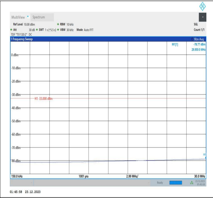
66-66-20MHz-5MHz-16QAM-16QAM-132072-132189-1RB#9 9-ORB#0-0.15~30MHz-PASS
