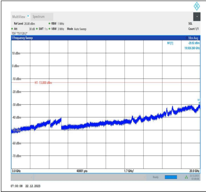
66-66-15MHz-20MHz-64QAM-64QAM-132401-132572-1RB# 0-1RB#99-3000~20000MHz-PASS
