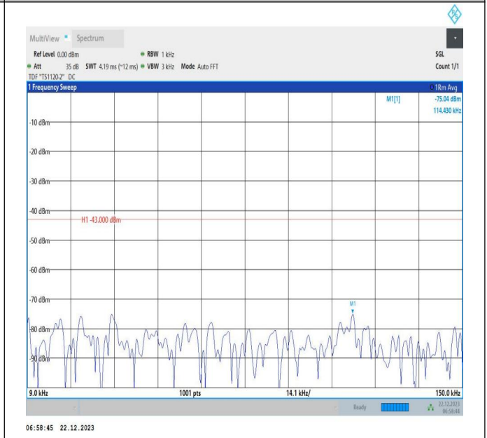
66-66-15MHz-20MHz-16QAM-16QAM-132401-132572-1RB#0-1RB#99-0.009~0.15MHz-PASS
