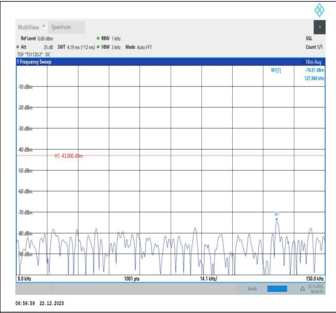
66-66-15MHz-20MHz-64QAM-64QAM-132401-132572-1RB# 74-ORB#0-0.009~0.15MHz-PASS
