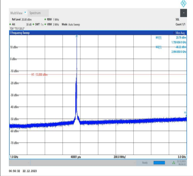
66-66-15MHz-20MHz-16QAM-16QAM-132401-132572-1RB# 74-ORB#0-1000~3000MHz-PASS
