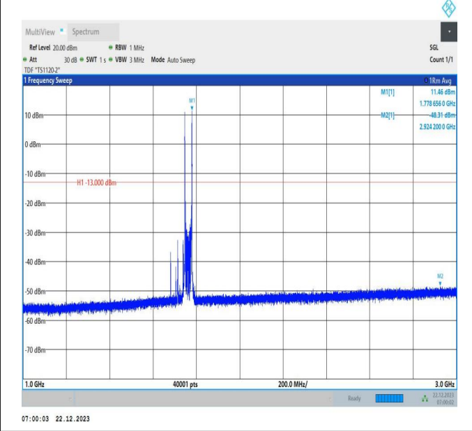
66-66-15MHz-20MHz-64QAM-64QAM-132401-132572-1RB# 0-1RB#99-1000~3000MHz-PASS
