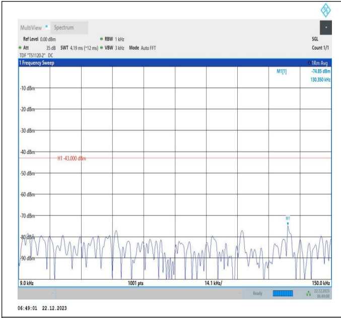
66-66-15MHz-20MHz-64QAM-64QAM-132325-132496-1RB# 0-1RB#99-0.009~0.15MHz-PASS
