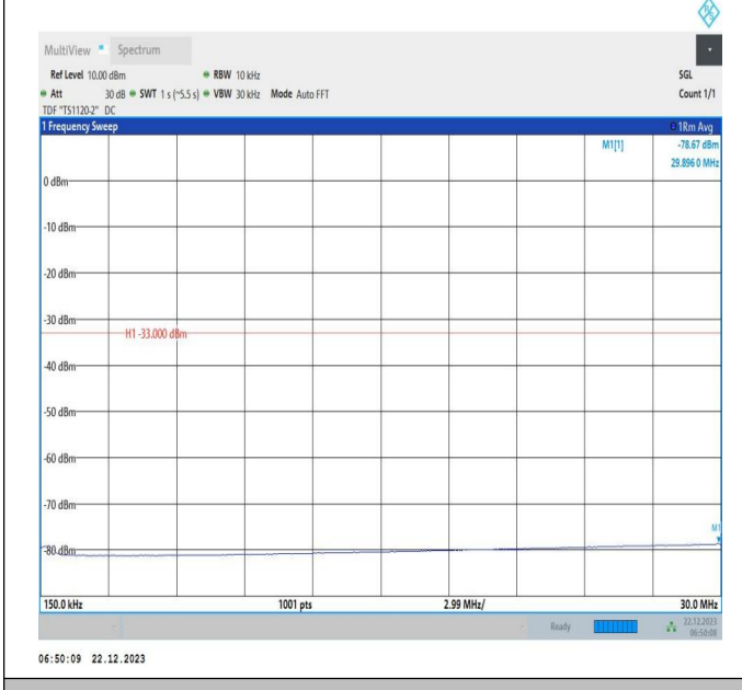
66-66-15MHz-20MHz-QPSK-QPSK-132325-132496-75RB#0 -100RB#0-0.15~30MHz-PASS
