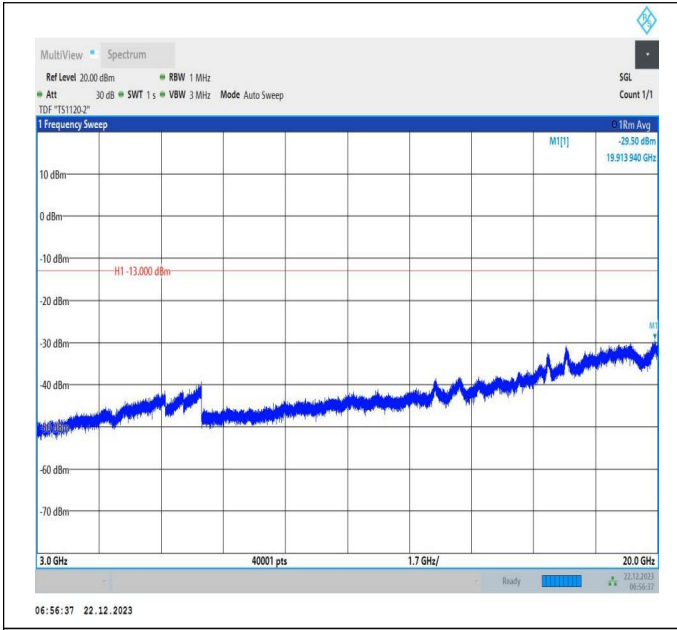
66-66-15MHz-20MHz-16QAM-16QAM-132401-132572-1RB# 74-ORB#0-3000~20000MHz-PASS
