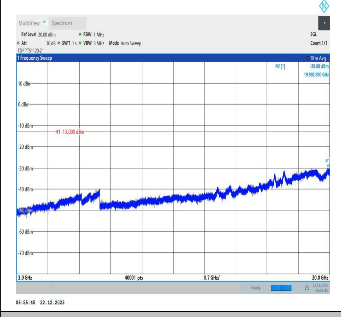
66-66-15MHz-20MHz-QPSK-QPSK-132401-132572-1RB#74 -ORB#0-3000~20000MHz-PASS
