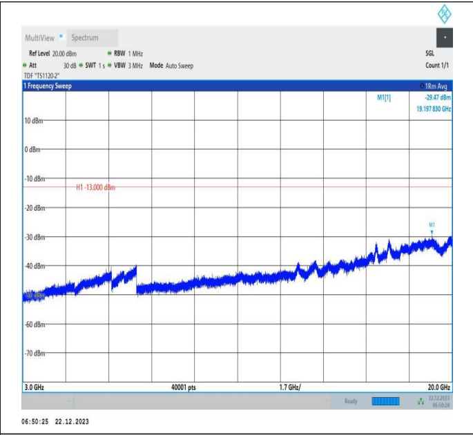
66-66-15MHz-20MHz-QPSK-QPSK-132325-132496-75RB#0 -100RB#0-3000~20000MHz-PASS
