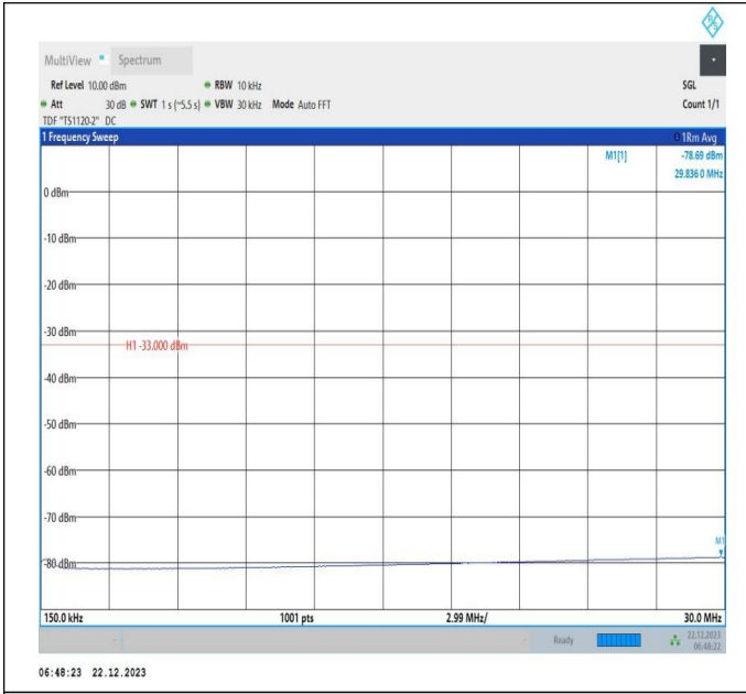
66-66-15MHz-20MHz-16QAM-16QAM-132325-132496-1RB# 0-1RB#99-0.15~30MHz-PASS
