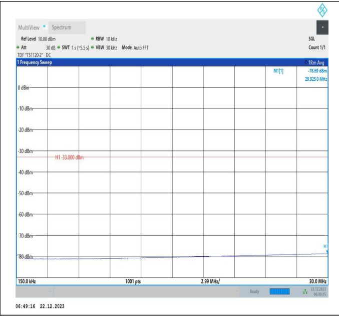
66-66-15MHz-20MHz-64QAM-64QAM-132325-132496-1RB# 0-1RB#99-0.15~30MHz-PASS
