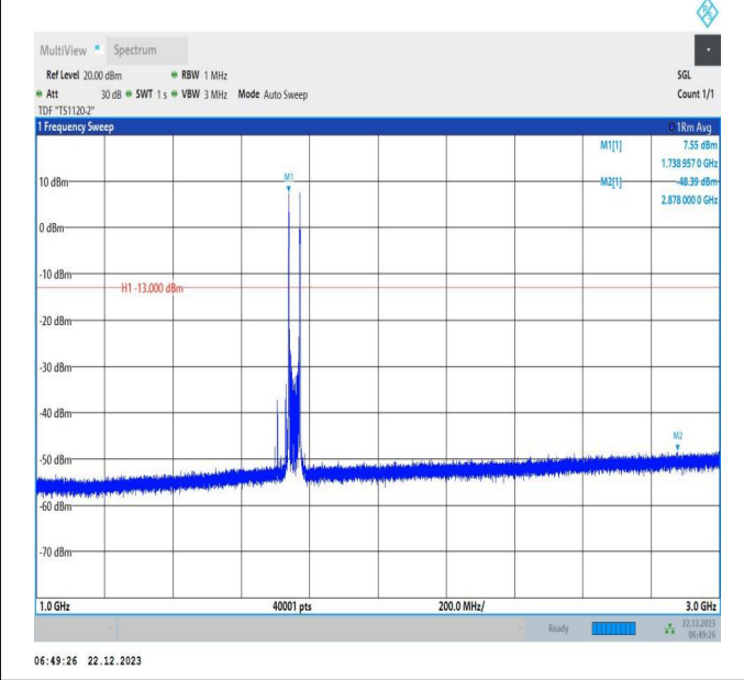
66-66-15MHz-20MHz-64QAM-64QAM-132325-132496-1RB# 0-1RB#99-1000~3000MHz-PASS
