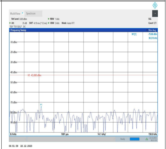
66-66-15MHz-20MHz-64QAM-64QAM-132325-132496-75RB #0-100RB#0-0.009~0.15MHz-PASS
