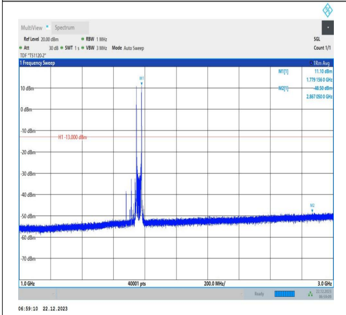
66-66-15MHz-20MHz-16QAM-16QAM-132401-132572-1RB# 0-1RB#99-1000~3000MHz-PASS
