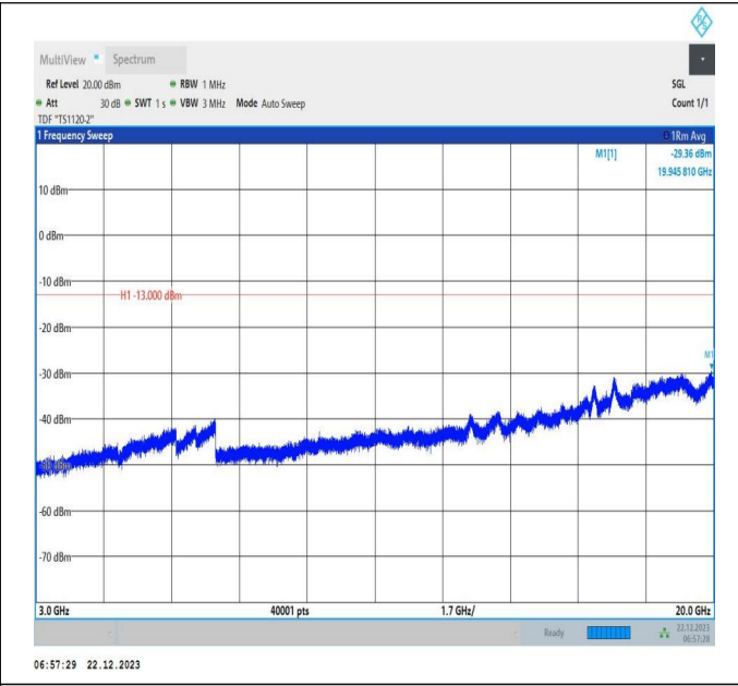
66-66-15MHz-20MHz-64QAM-64QAM-132401-132572-1RB# 74-ORB#0-3000~20000MHz-PASS
