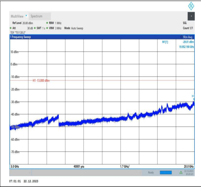
66-66-15MHz-20MHz-QPSK-QPSK-132401-132572-75RB#0 -100RB#0-3000~20000MHz-PASS
