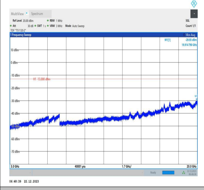
66-66-15MHz-20MHz-16QAM-16QAM-132325-132496-1RB# 0-1RB#99-3000~20000MHz-PASS
