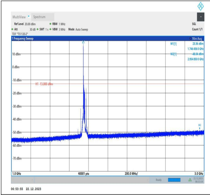
66-66-15MHz-20MHz-16QAM-16QAM-132401-132572-1RB# 0-ORB#0-1000~3000MHz-PASS
