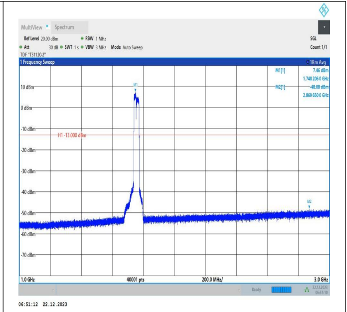
66-66-15MHz-20MHz-16QAM-16QAM-132325-132496-75RB #0-100RB#0-1000~3000MHz-PASS
