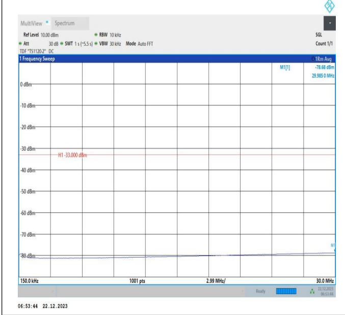
66-66-15MHz-20MHz-16QAM-16QAM-132401-132572-1RB#0-ORB#0-0.15~30MHz-PASS
