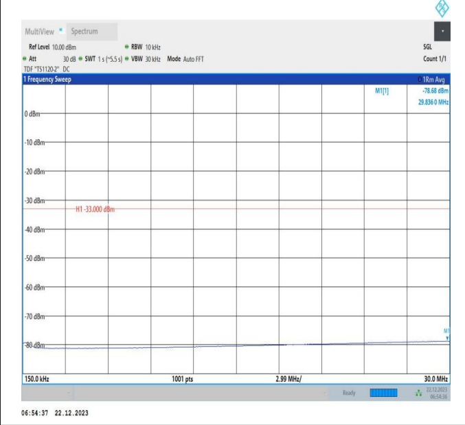
66-66-15MHz-20MHz-64QAM-64QAM-132401-132572-1RB# 0-ORB#0-0.15~30MHz-PASS
