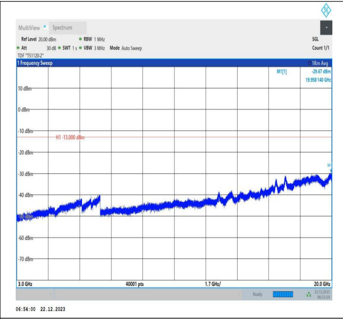
66-66-15MHz-20MHz-16QAM-16QAM-132401-132572-1RB# 0-ORB#0-3000~20000MHz-PASS
