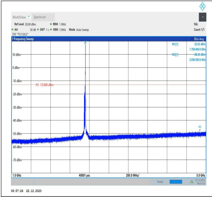
66-66-15MHz-20MHz-64QAM-64QAM-132401-132572-1RB# 74-ORB#0-1000~3000MHz-PASS
