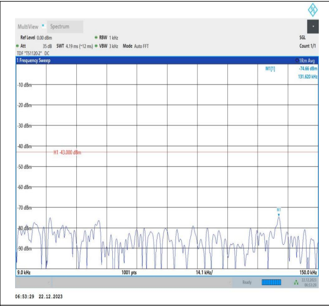
66-66-15MHz-20MHz-16QAM-16QAM-132401-132572-1RB#0-ORB#0-0.009~0.15MHz-PASS
