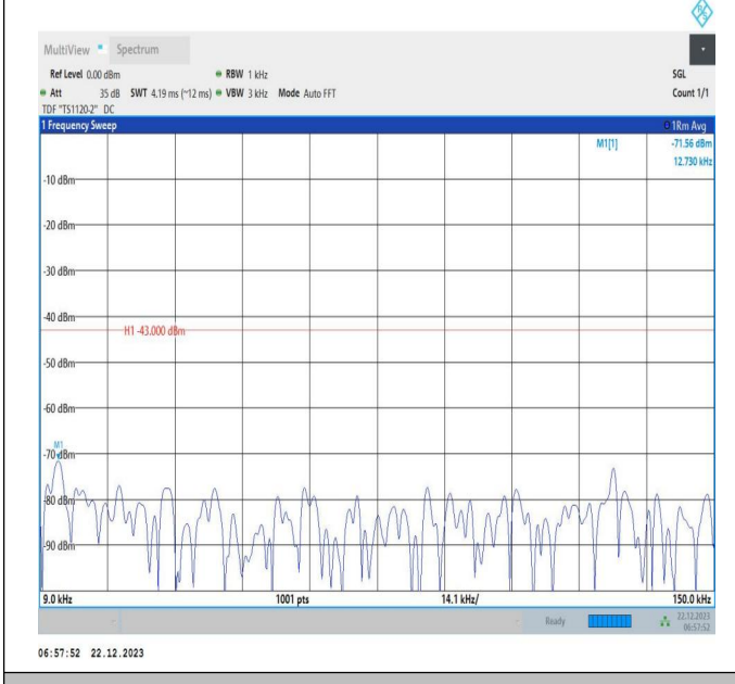
66-66-15MHz-20MHz-QPSK-QPSK-132401-132572-1RB#0- 1RB#99-0.009~0.15MHz-PASS
