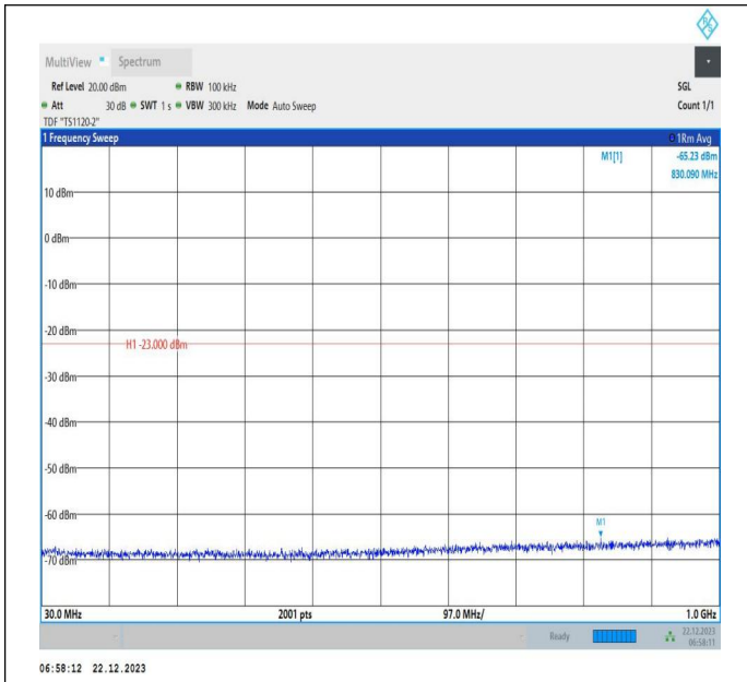
66-66-15MHz-20MHz-QPSK-QPSK-132401-132572-1RB#0-1RB#99-30~1000MHz-PASS
