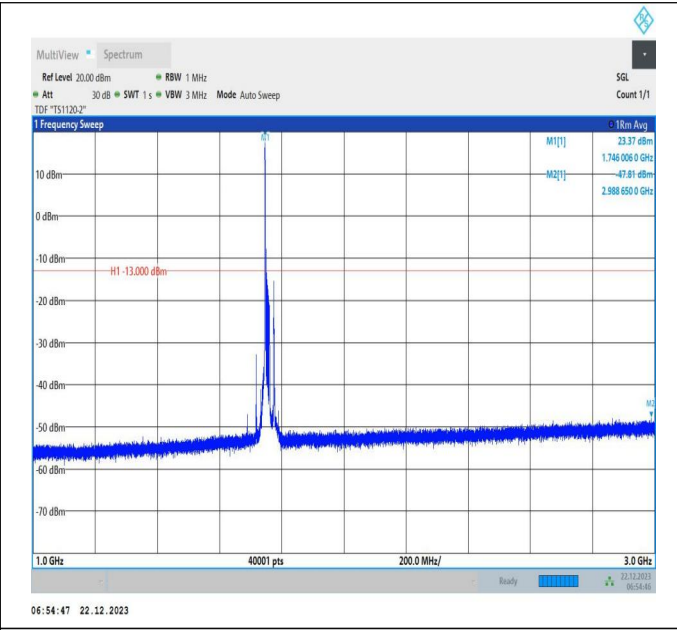
66-66-15MHz-20MHz-64QAM-64QAM-132401-132572-1RB# 0-ORB#0-1000~3000MHz-PASS
