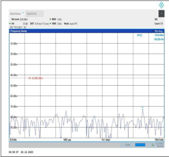
66-66-15MHz-20MHz-64QAM-64QAM-132401-132572-1RB# 0-1RB#99-0.009~0.15MHz-PASS
