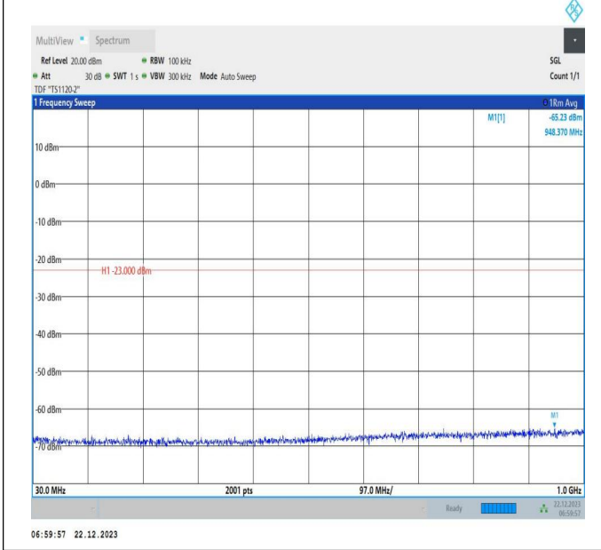
66-66-15MHz-20MHz-64QAM-64QAM-132401-132572-1RB# 0-1RB#99-30~1000MHz-PASS
