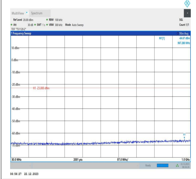
66-66-15MHz-20MHz-16QAM-16QAM-132401-132572-1RB# 74-ORB#0-30~1000MHz-PASS
