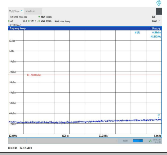
66-66-15MHz-20MHz-QPSK-QPSK-132325-132496-75RB#0 -100RB#0-30~1000MHz-PASS
