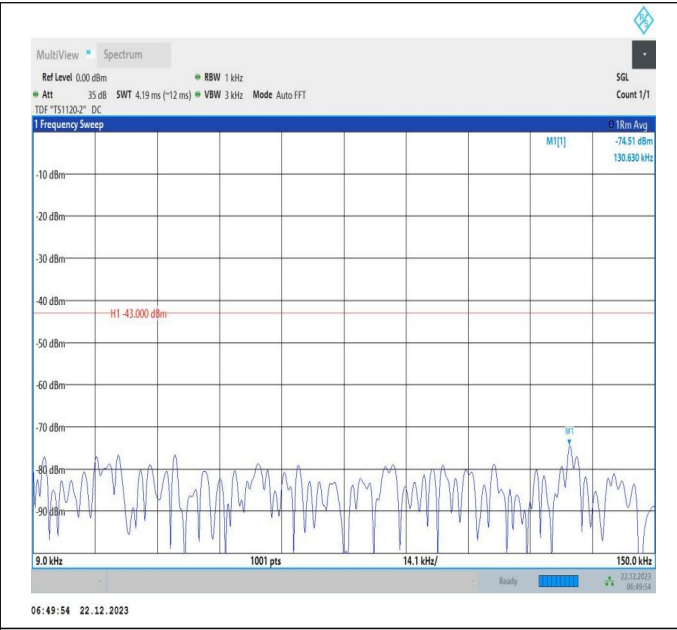
66-66-15MHz-20MHz-QPSK-QPSK-132325-132496-75RB#0 -100RB#0-0.009~0.15MHz-PASS
