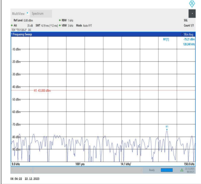
66-66-15MHz-20MHz-64QAM-64QAM-132401-132572-1RB# 0-ORB#0-0.009~0.15MHz-PASS
