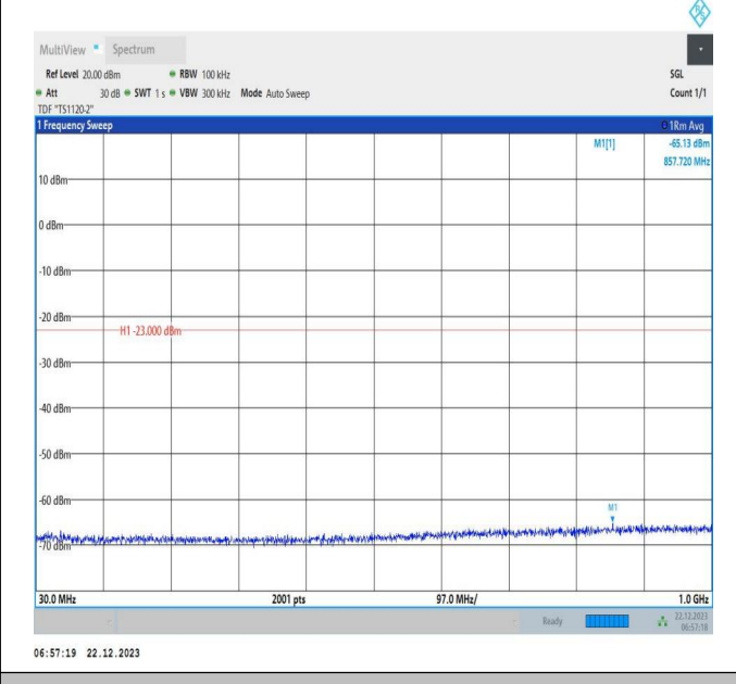
66-66-15MHz-20MHz-64QAM-64QAM-132401-132572-1RB# 74-ORB#0-30~1000MHz-PASS
