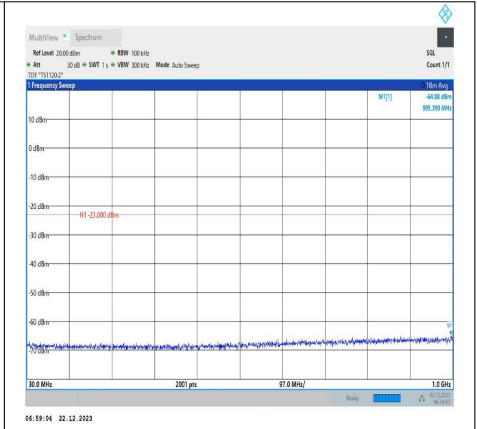
66-66-15MHz-20MHz-16QAM-16QAM-132401-132572-1RB# 0-1RB#99-30~1000MHz-PASS
