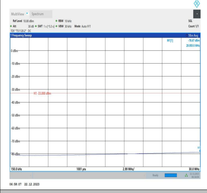
66-66-15MHz-20MHz-QPSK-QPSK-132401-132572-1RB#0- 1RB#99-0.15~30MHz-PASS
