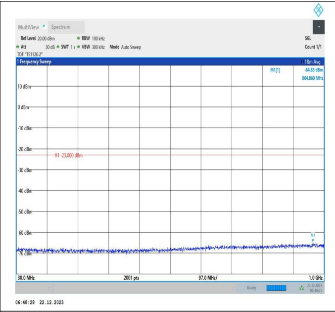
66-66-15MHz-20MHz-16QAM-16QAM-132325-132496-1RB# 0-1RB#99-30~1000MHz-PASS
