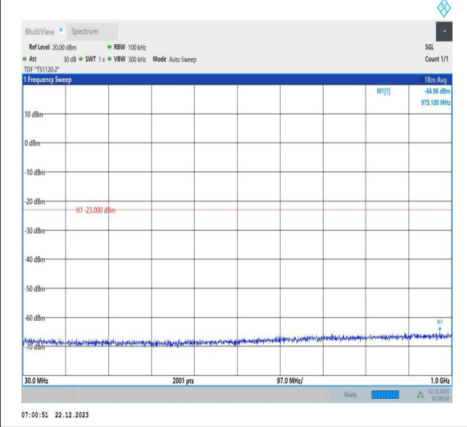
66-66-15MHz-20MHz-QPSK-QPSK-132401-132572-75RB#0 -100RB#0-30~1000MHz-PASS
