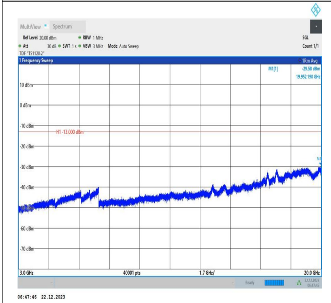
66-66-15MHz-20MHz-QPSK-QPSK-132325-132496-1RB#0-1RB#99-3000~20000MHz-PASS
