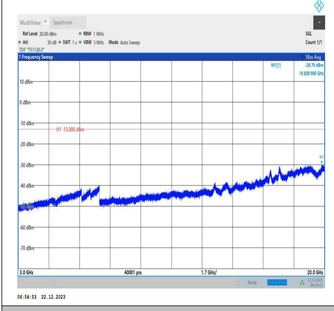
66-66-15MHz-20MHz-64QAM-64QAM-132401-132572-1RB# 0-ORB#0-3000~20000MHz-PASS
