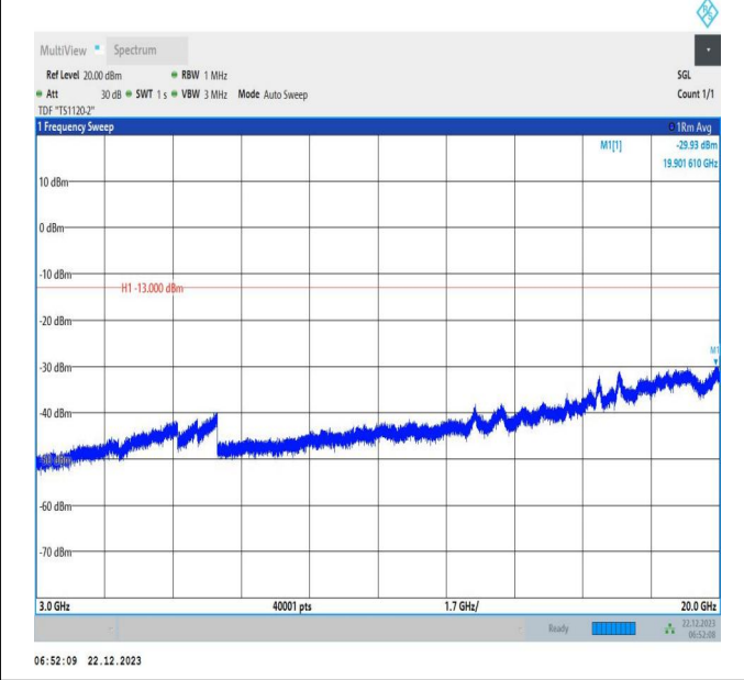
66-66-15MHz-20MHz-64QAM-64QAM-132325-132496-75RB #0-100RB#0-3000~20000MHz-PASS
