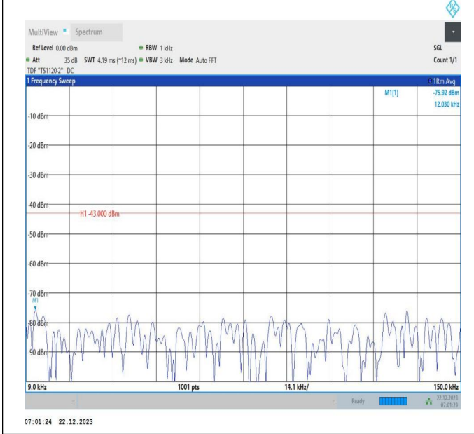
66-66-15MHz-20MHz-16QAM-16QAM-132401-132572-75RB #0-100RB#0-0.009~0.15MHz-PASS
