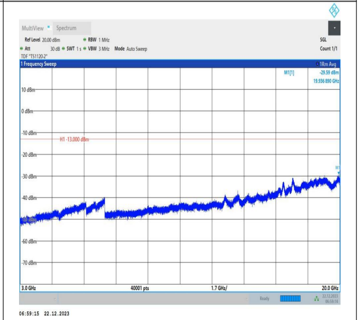
66-66-15MHz-20MHz-16QAM-16QAM-132401-132572-1RB# 0-1RB#99-3000~20000MHz-PASS
