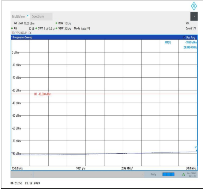
66-66-15MHz-20MHz-64QAM-64QAM-132325-132496-75RB #0-100RB#0-0.15~30MHz-PASS
