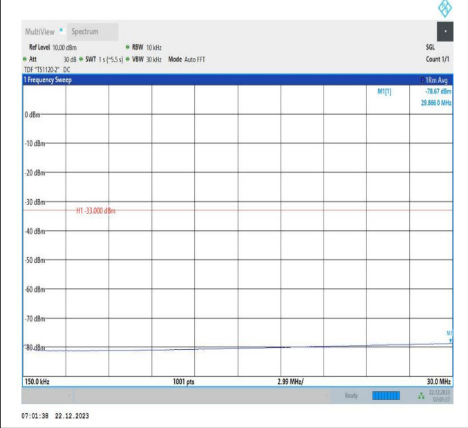
66-66-15MHz-20MHz-16QAM-16QAM-132401-132572-75RB #0-100RB#0-0.15~30MHz-PASS
