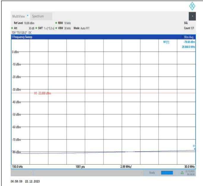
66-66-15MHz-20MHz-16QAM-16QAM-132401-132572-1RB# 0-1RB#99-0.15~30MHz-PASS
