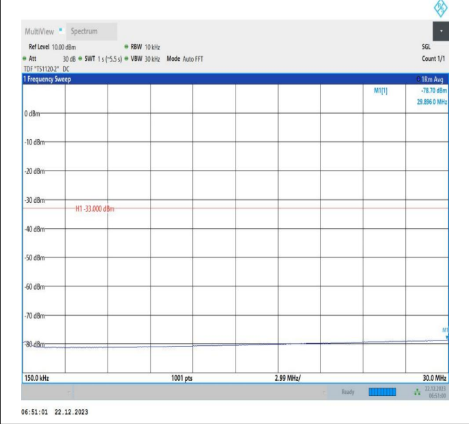
66-66-15MHz-20MHz-16QAM-16QAM-132325-132496-75RB #0-100RB#0-0.15~30MHz-PASS
