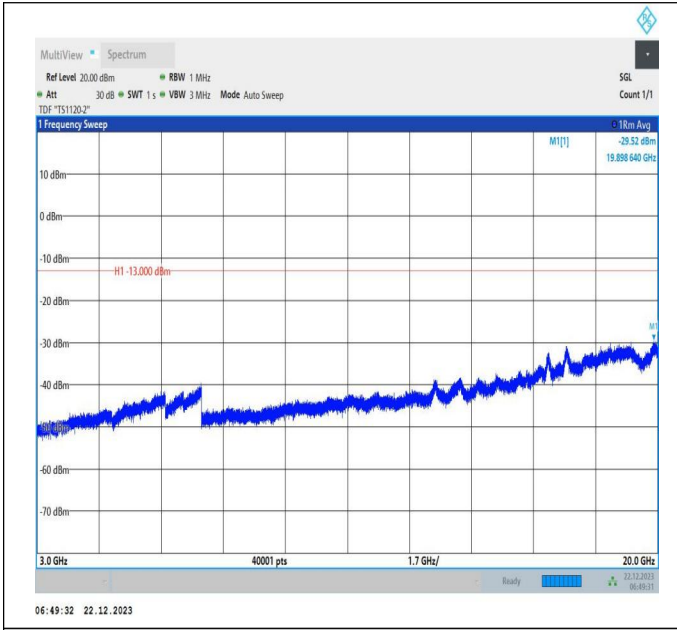
66-66-15MHz-20MHz-64QAM-64QAM-132325-132496-1RB# 0-1RB#99-3000~20000MHz-PASS
