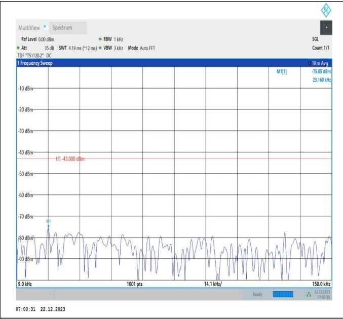
66-66-15MHz-20MHz-QPSK-QPSK-132401-132572-75RB#0 -100RB#0-0.009~0.15MHz-PASS
