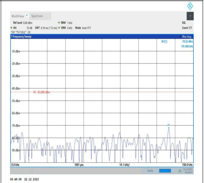
66-66-15MHz-20MHz-16QAM-16QAM-132325-132496-1RB#0-1RB#99-0.009~0.15MHz-PASS
