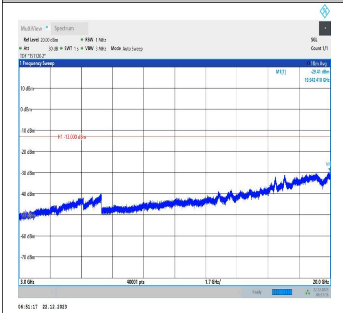
66-66-15MHz-20MHz-16QAM-16QAM-132325-132496-75RB #0-100RB#0-3000~20000MHz-PASS
