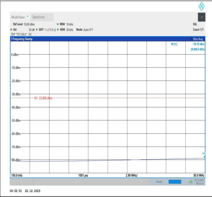
66-66-15MHz-20MHz-QPSK-QPSK-132401-132572-1RB#0-ORB#0-0.15~30MHz-PASS
