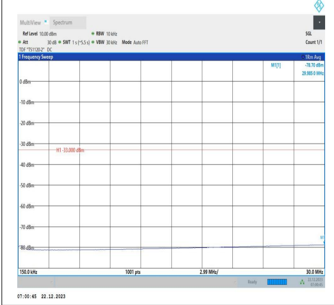
66-66-15MHz-20MHz-QPSK-QPSK-132401-132572-75RB#0 -100RB#0-0.15~30MHz-PASS
