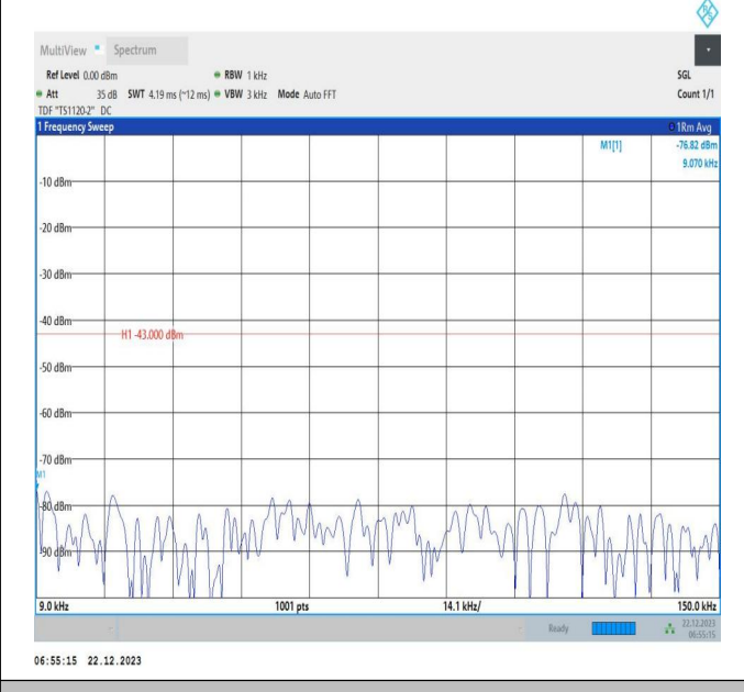
66-66-15MHz-20MHz-QPSK-QPSK-132401-132572-1RB#74 -ORB#0-0.009~0.15MHz-PASS
