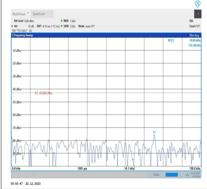
66-66-15MHz-20MHz-16QAM-16QAM-132325-132496-75RB #0-100RB#0-0.009~0.15MHz-PASS
