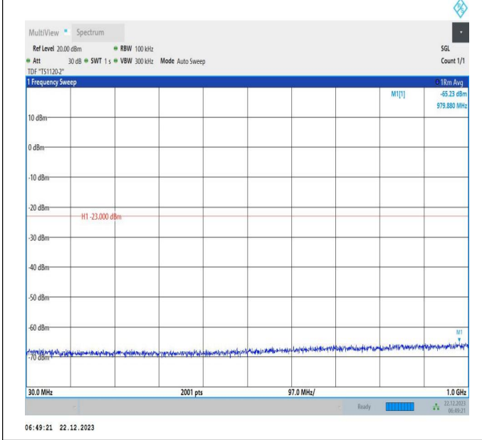
66-66-15MHz-20MHz-64QAM-64QAM-132325-132496-1RB# 0-1RB#99-30~1000MHz-PASS
