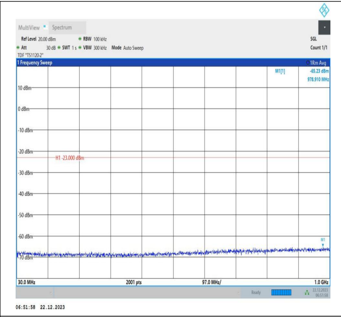
66-66-15MHz-20MHz-64QAM-64QAM-132325-132496-75RB #0-100RB#0-30~1000MHz-PASS
