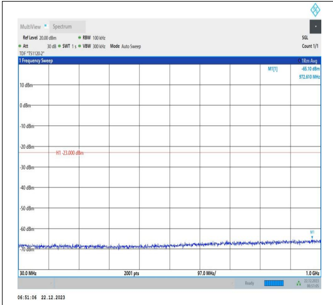
66-66-15MHz-20MHz-16QAM-16QAM-132325-132496-75RB #0-100RB#0-30~1000MHz-PASS
