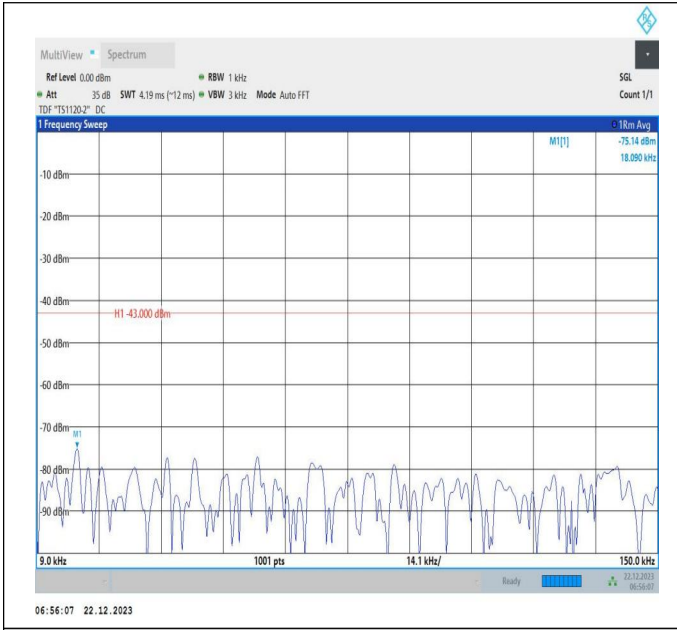
66-66-15MHz-20MHz-16QAM-16QAM-132401-132572-1RB# 74-ORB#0-0.009~0.15MHz-PASS
