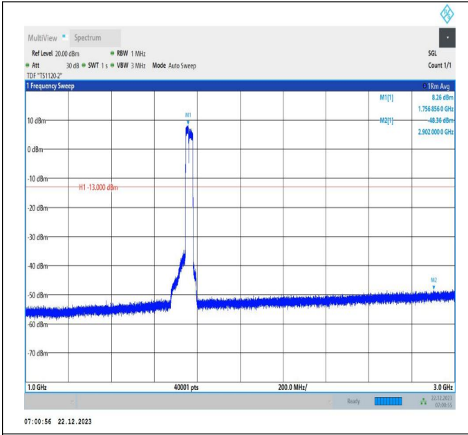
66-66-15MHz-20MHz-QPSK-QPSK-132401-132572-75RB#0 -100RB#0-1000~3000MHz-PASS
