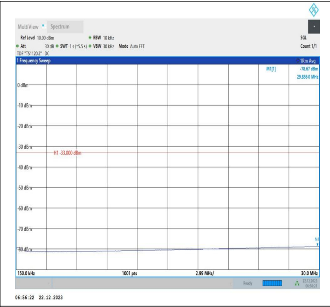
66-66-15MHz-20MHz-16QAM-16QAM-132401-132572-1RB# 74-ORB#0-0.15~30MHz-PASS
