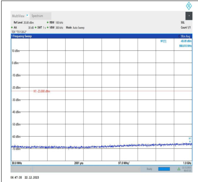
66-66-15MHz-20MHz-QPSK-QPSK-132325-132496-1RB#0-1RB#99-30~1000MHz-PASS
