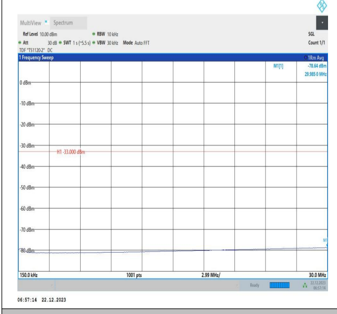
66-66-15MHz-20MHz-64QAM-64QAM-132401-132572-1RB# 74-ORB#0-0.15~30MHz-PASS
