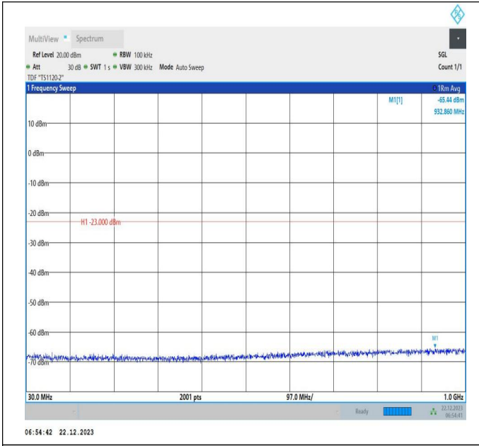
66-66-15MHz-20MHz-64QAM-64QAM-132401-132572-1RB# 0-ORB#0-30~1000MHz-PASS
