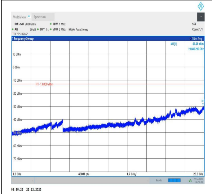
66-66-15MHz-20MHz-QPSK-QPSK-132401-132572-1RB#0-1RB#99-3000~20000MHz-PASS
