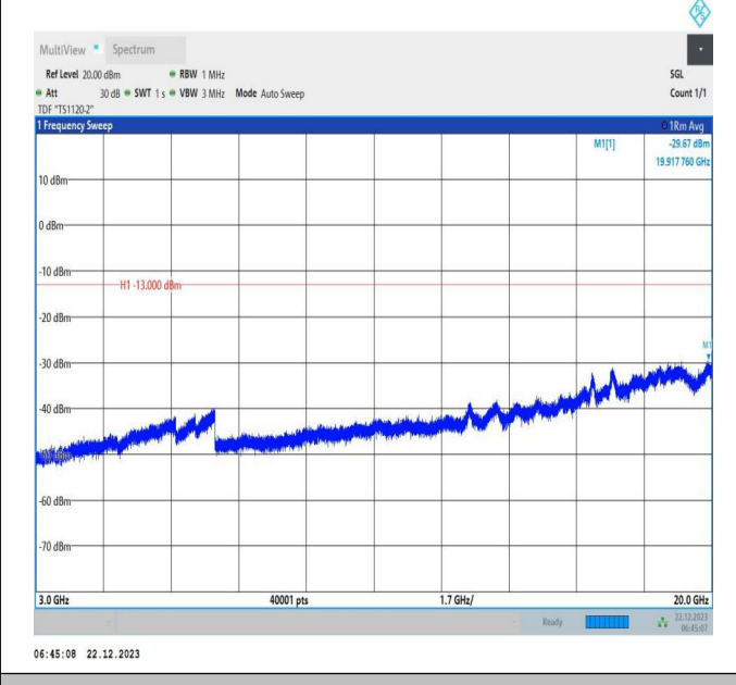
66-66-15MHz-20MHz-QPSK-QPSK-132325-132496-1RB#74 -ORB#0-3000~20000MHz-PASS
