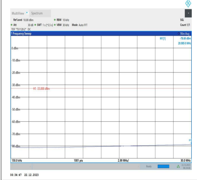
66-66-15MHz-20MHz-64QAM-64QAM-132050-132221-1RB# 74-ORB#0-0.15~30MHz-PASS
