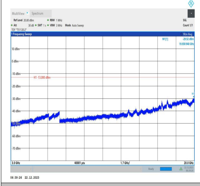
66-66-15MHz-20MHz-16QAM-16QAM-132050-132221-75RB #0-100RB#0-3000~20000MHz-PASS
