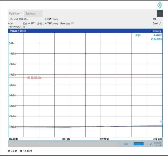
66-66-15MHz-20MHz-16QAM-16QAM-132325-132496-1RB# 74-ORB#0-0.15~30MHz-PASS
