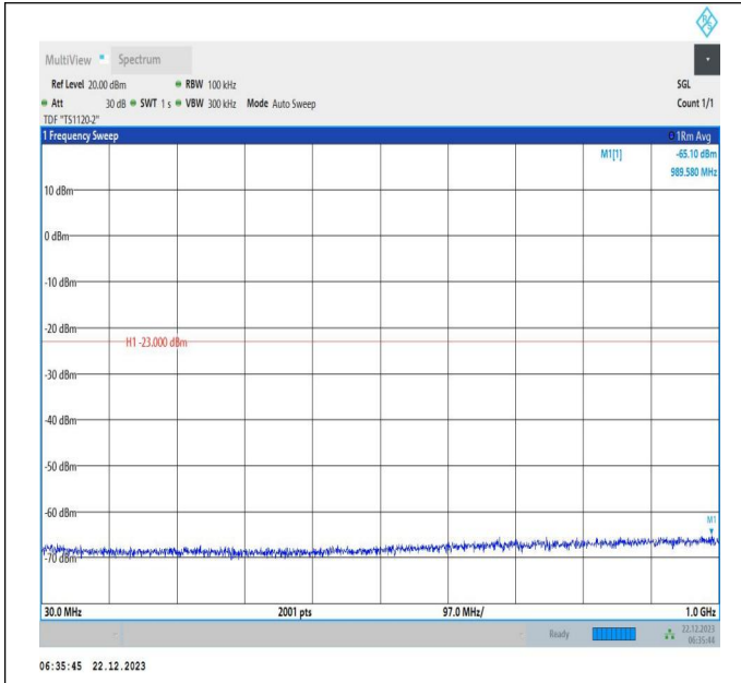
66-66-15MHz-20MHz-QPSK-QPSK-132050-132221-1RB#0-1RB#99-30~1000MHz-PASS
