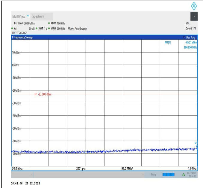
66-66-15MHz-20MHz-64QAM-64QAM-132325-132496-1RB# 0-ORB#0-30~1000MHz-PASS
