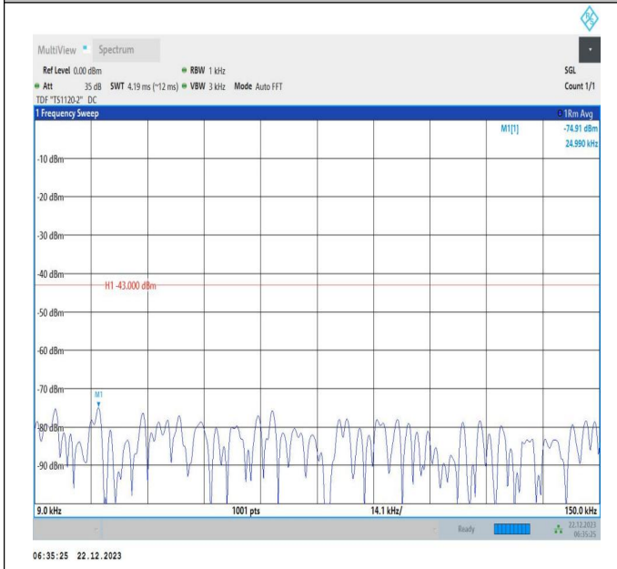
66-66-15MHz-20MHz-QPSK-QPSK-132050-132221-1RB#0- 1RB#99-0.009~0.15MHz-PASS
