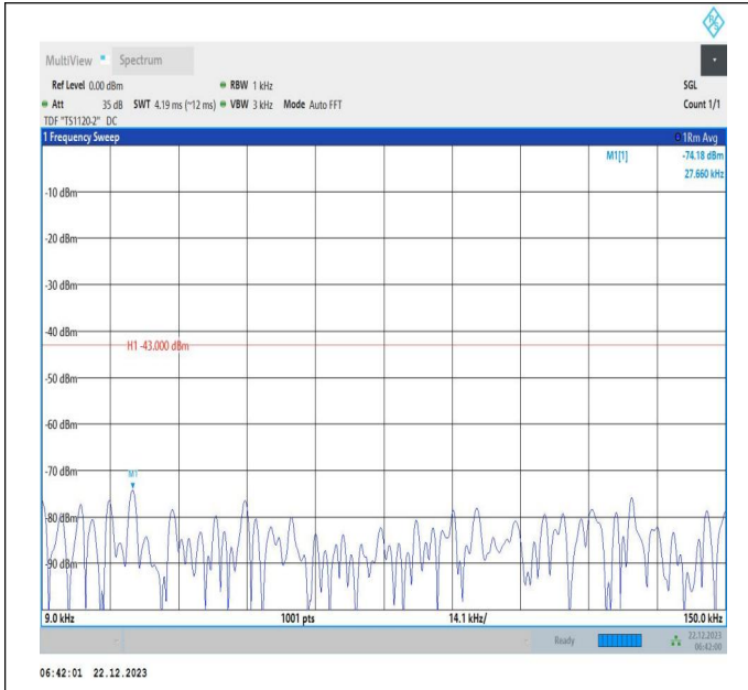
66-66-15MHz-20MHz-QPSK-QPSK-132325-132496-1RB#0-ORB#0-0.009~0.15MHz-PASS
