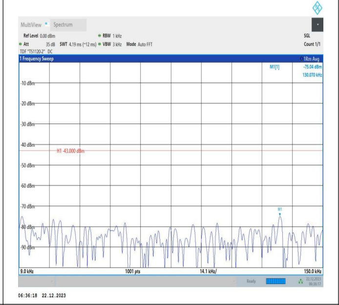
66-66-15MHz-20MHz-16QAM-16QAM-132050-132221-1RB#0-1RB#99-0.009~0.15MHz-PASS
