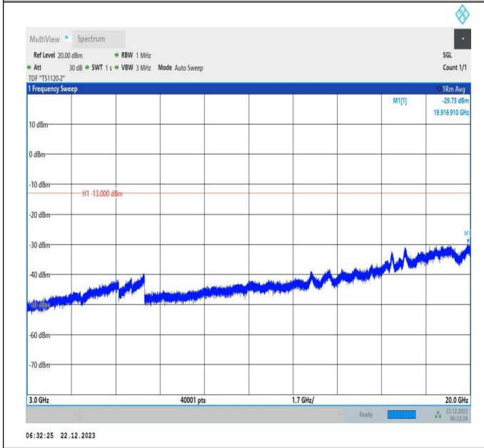
66-66-15MHz-20MHz-64QAM-64QAM-132050-132221-1RB# 0-ORB#0-3000~20000MHz-PASS
