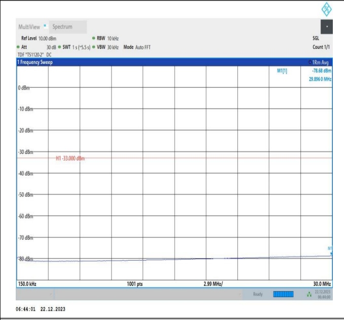
66-66-15MHz-20MHz-64QAM-64QAM-132325-132496-1RB# 0-ORB#0-0.15~30MHz-PASS
