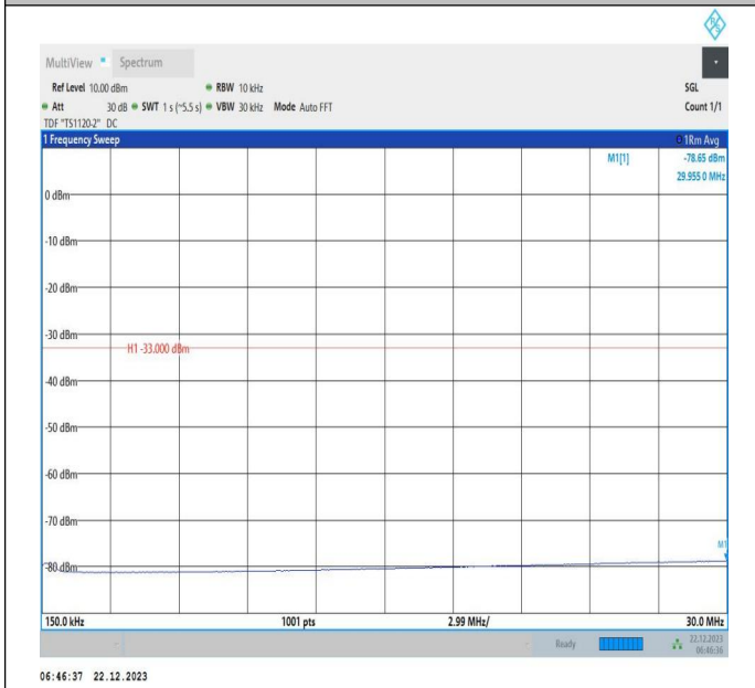
66-66-15MHz-20MHz-64QAM-64QAM-132325-132496-1RB# 74-ORB#0-0.15~30MHz-PASS
