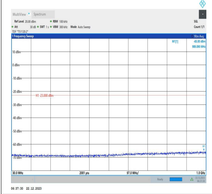
66-66-15MHz-20MHz-64QAM-64QAM-132050-132221-1RB# 0-1RB#99-30~1000MHz-PASS
