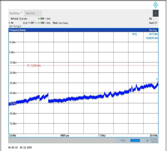
66-66-15MHz-20MHz-64QAM-64QAM-132050-132221-75RB #0-100RB#0-3000~20000MHz-PASS
