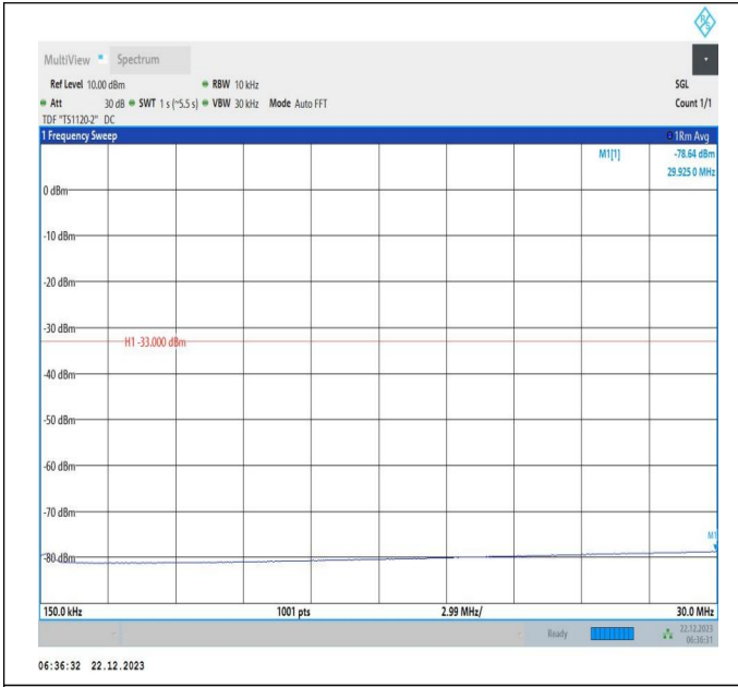
66-66-15MHz-20MHz-16QAM-16QAM-132050-132221-1RB# 0-1RB#99-0.15~30MHz-PASS
