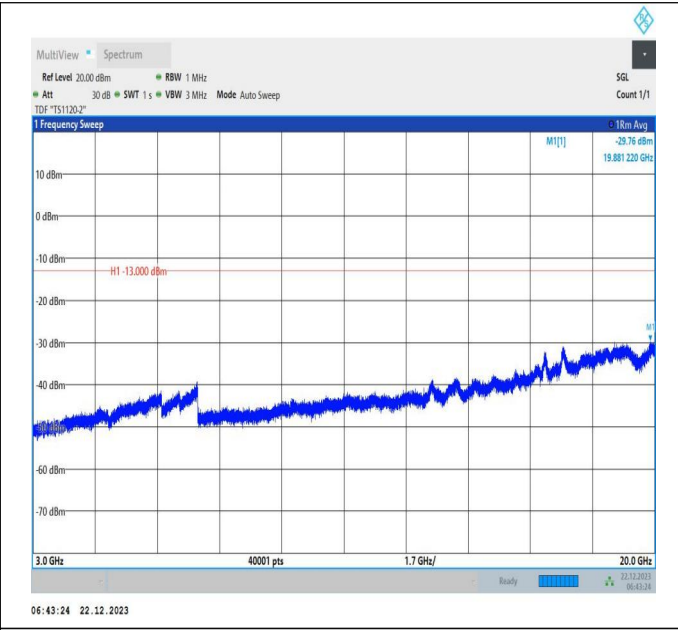
66-66-15MHz-20MHz-16QAM-16QAM-132325-132496-1RB# 0-ORB#0-3000~20000MHz-PASS
