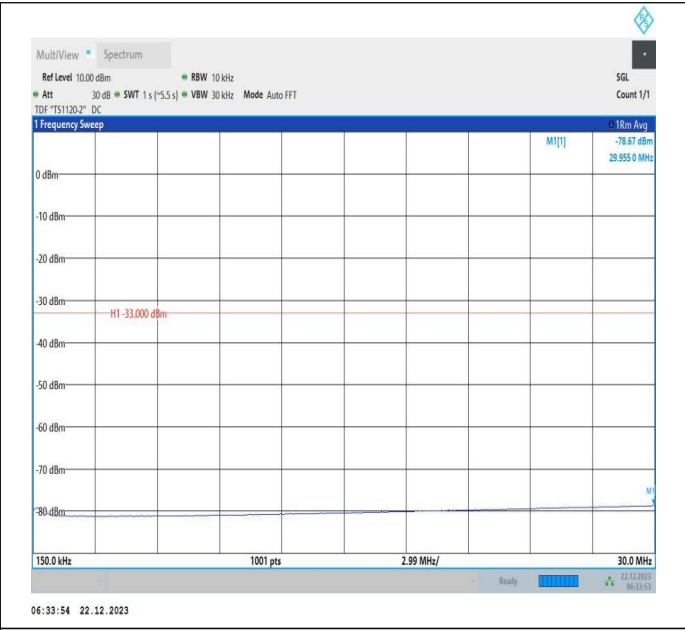
66-66-15MHz-20MHz-16QAM-16QAM-132050-132221-1RB# 74-ORB#0-0.15~30MHz-PASS
