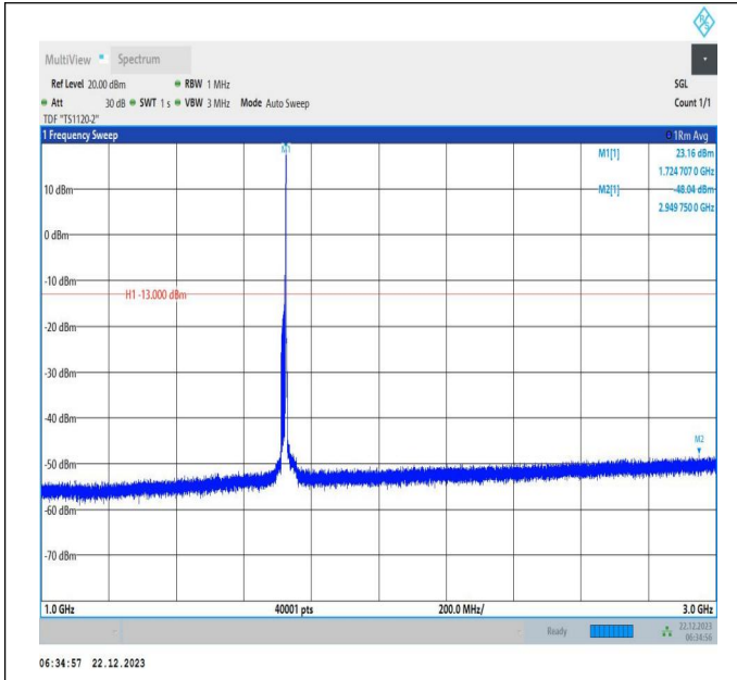
66-66-15MHz-20MHz-64QAM-64QAM-132050-132221-1RB# 74-ORB#0-1000~3000MHz-PASS
