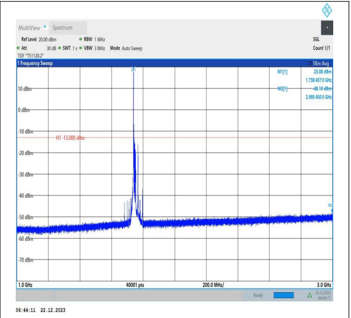
66-66-15MHz-20MHz-64QAM-64QAM-132325-132496-1RB# 0-ORB#0-1000~3000MHz-PASS
