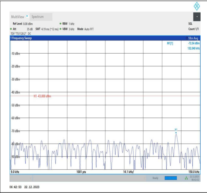
66-66-15MHz-20MHz-16QAM-16QAM-132325-132496-1RB#0-ORB#0-0.009~0.15MHz-PASS
