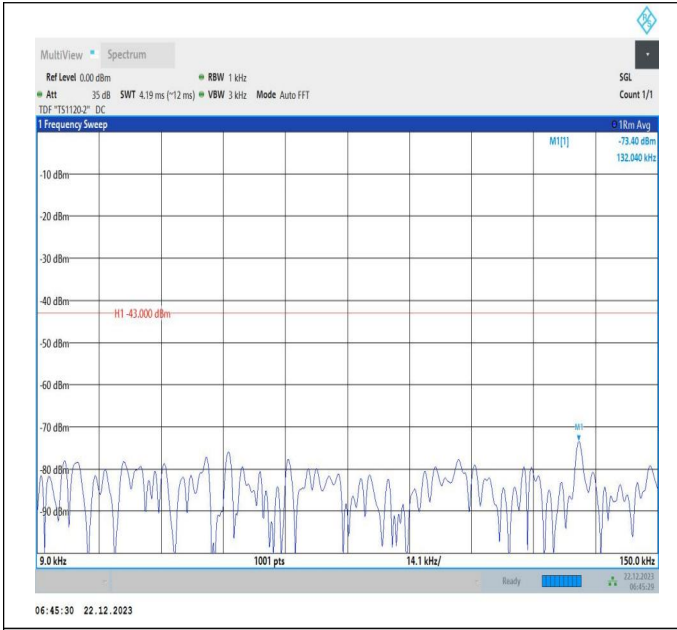
66-66-15MHz-20MHz-16QAM-16QAM-132325-132496-1RB# 74-ORB#0-0.009~0.15MHz-PASS
