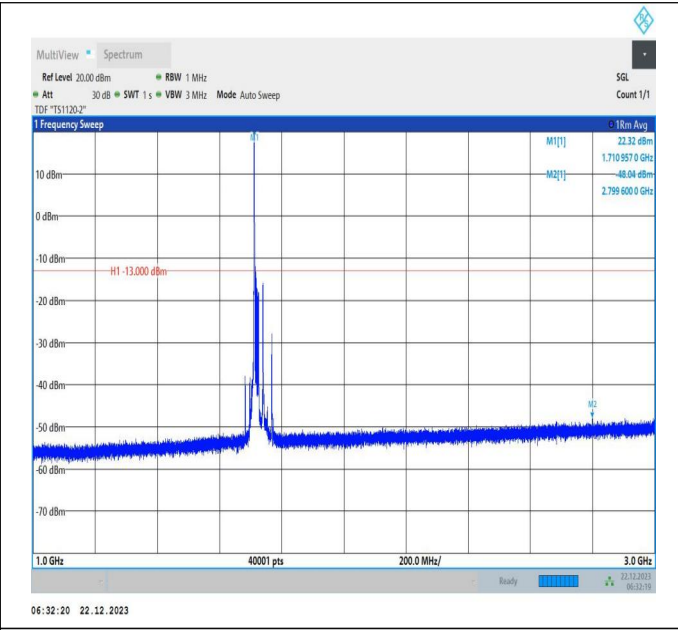
66-66-15MHz-20MHz-64QAM-64QAM-132050-132221-1RB# 0-ORB#0-1000~3000MHz-PASS
