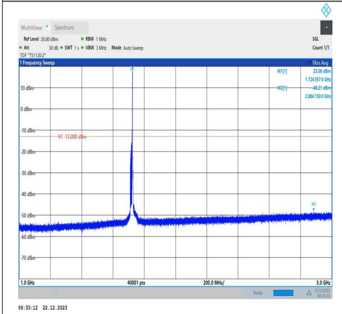
66-66-15MHz-20MHz-QPSK-QPSK-132050-132221-1RB#74 -ORB#0-1000~3000MHz-PASS
