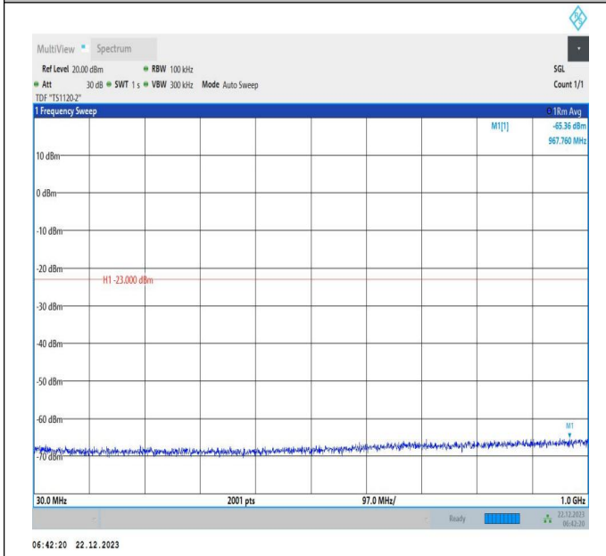
66-66-15MHz-20MHz-QPSK-QPSK-132325-132496-1RB#0-ORB#0-30~1000MHz-PASS
