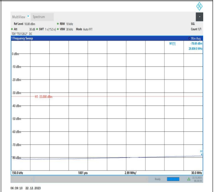
66-66-15MHz-20MHz-16QAM-16QAM-132050-132221-75RB #0-100RB#0-0.15~30MHz-PASS
