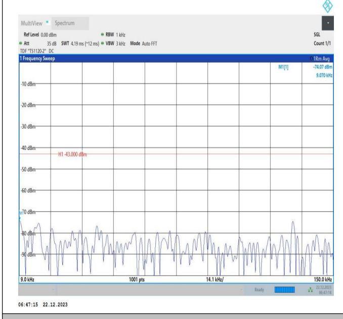
66-66-15MHz-20MHz-QPSK-QPSK-132325-132496-1RB#0- 1RB#99-0.009~0.15MHz-PASS
