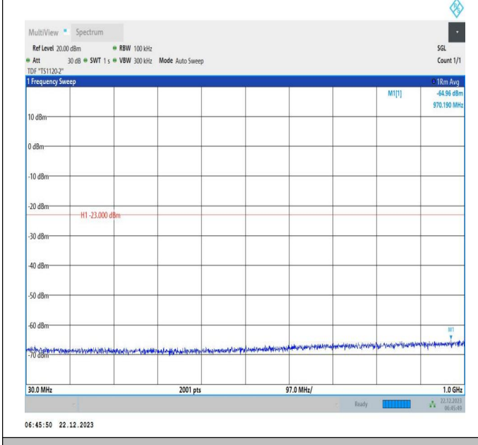
66-66-15MHz-20MHz-16QAM-16QAM-132325-132496-1RB# 74-ORB#0-30~1000MHz-PASS
