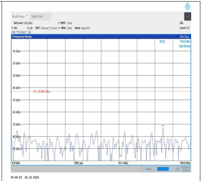
66-66-15MHz-20MHz-64QAM-64QAM-132325-132496-1RB# 74-ORB#0-0.009~0.15MHz-PASS
