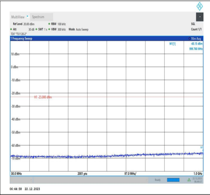
66-66-15MHz-20MHz-QPSK-QPSK-132325-132496-1RB#74 -ORB#0-30~1000MHz-PASS
