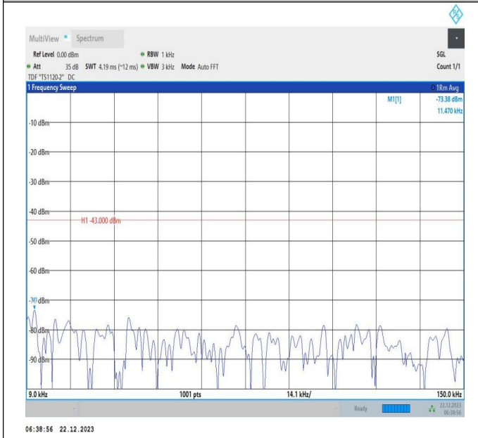
66-66-15MHz-20MHz-16QAM-16QAM-132050-132221-75RB #0-100RB#0-0.009~0.15MHz-PASS
