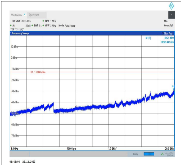
66-66-15MHz-20MHz-16QAM-16QAM-132325-132496-1RB# 74-ORB#0-3000~20000MHz-PASS
