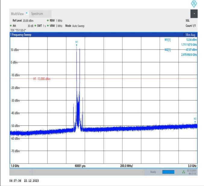
66-66-15MHz-20MHz-64QAM-64QAM-132050-132221-1RB# 0-1RB#99-1000~3000MHz-PASS
