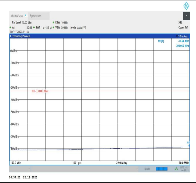
66-66-15MHz-20MHz-64QAM-64QAM-132050-132221-1RB# 0-1RB#99-0.15~30MHz-PASS
