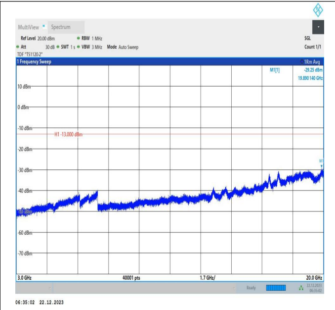
66-66-15MHz-20MHz-64QAM-64QAM-132050-132221-1RB# 74-ORB#0-3000~20000MHz-PASS
