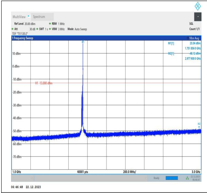
66-66-15MHz-20MHz-64QAM-64QAM-132325-132496-1RB# 74-0RB#0-1000~3000MHz-PASS
