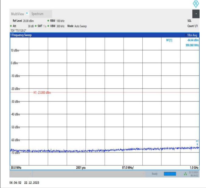
66-66-15MHz-20MHz-64QAM-64QAM-132050-132221-1RB# 74-ORB#0-30~1000MHz-PASS
