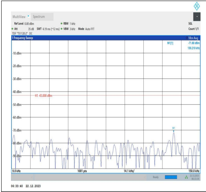
66-66-15MHz-20MHz-16QAM-16QAM-132050-132221-1RB# 74-ORB#0-0.009~0.15MHz-PASS
