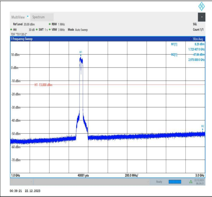
66-66-15MHz-20MHz-16QAM-16QAM-132050-132221-75RB #0-100RB#0-1000~3000MHz-PASS
