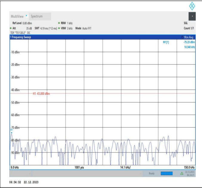
66-66-15MHz-20MHz-64QAM-64QAM-132050-132221-1RB# 74-ORB#0-0.009~0.15MHz-PASS
