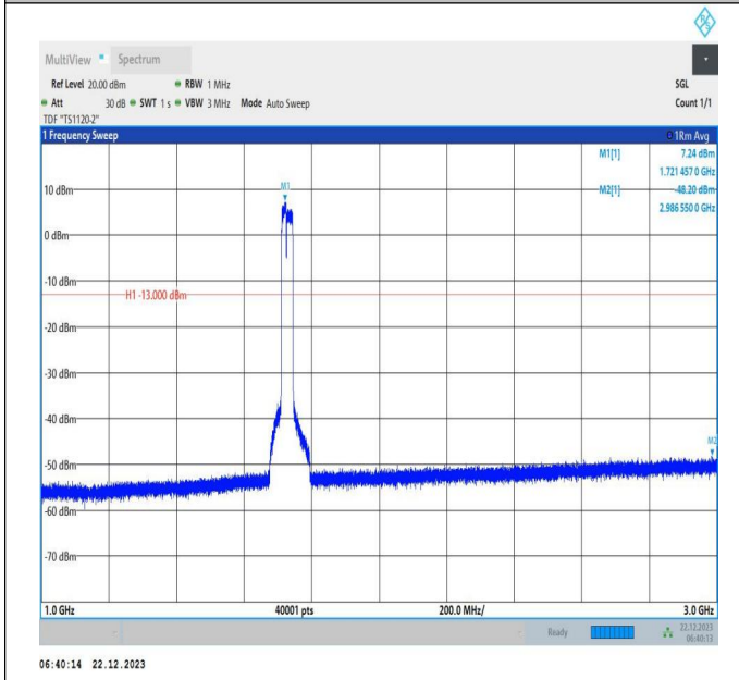
66-66-15MHz-20MHz-64QAM-64QAM-132050-132221-75RB #0-100RB#0-1000~3000MHz-PASS
