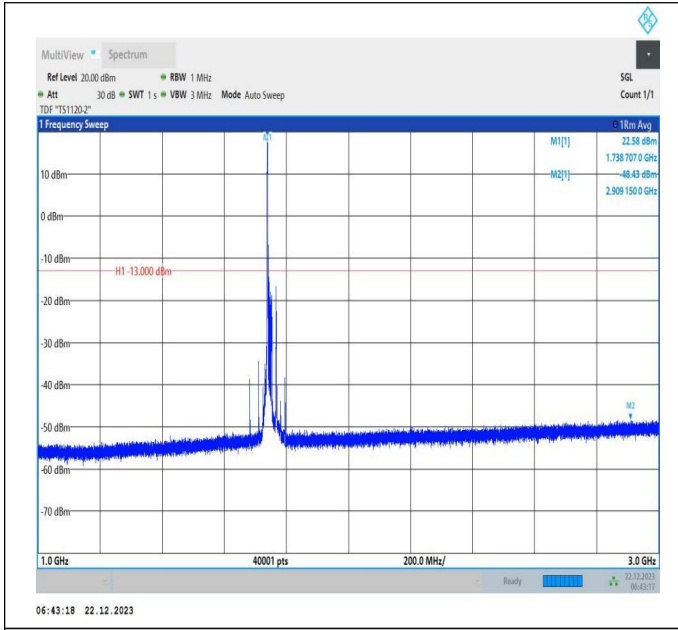
66-66-15MHz-20MHz-16QAM-16QAM-132325-132496-1RB# 0-ORB#0-1000~3000MHz-PASS
