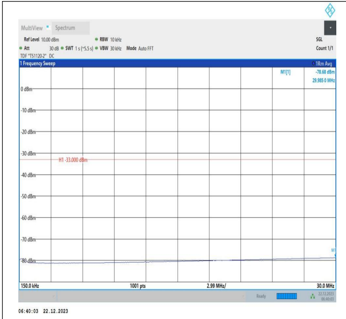
66-66-15MHz-20MHz-64QAM-64QAM-132050-132221-75RB #0-100RB#0-0.15~30MHz-PASS
