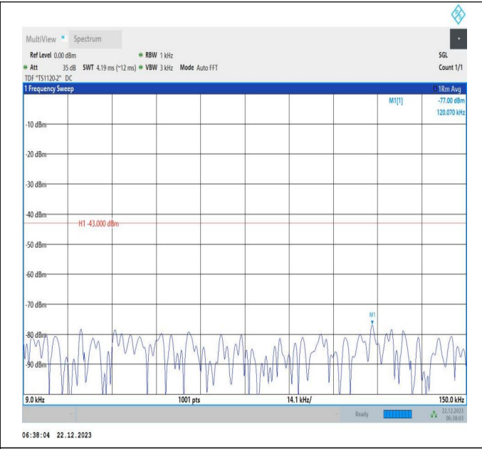
66-66-15MHz-20MHz-QPSK-QPSK-132050-132221-75RB#0-100RB#0-0.009~0.15MHz-PASS
