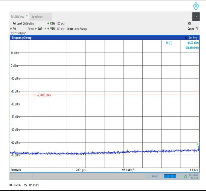
66-66-15MHz-20MHz-16QAM-16QAM-132050-132221-1RB# 0-1RB#99-30~1000MHz-PASS
