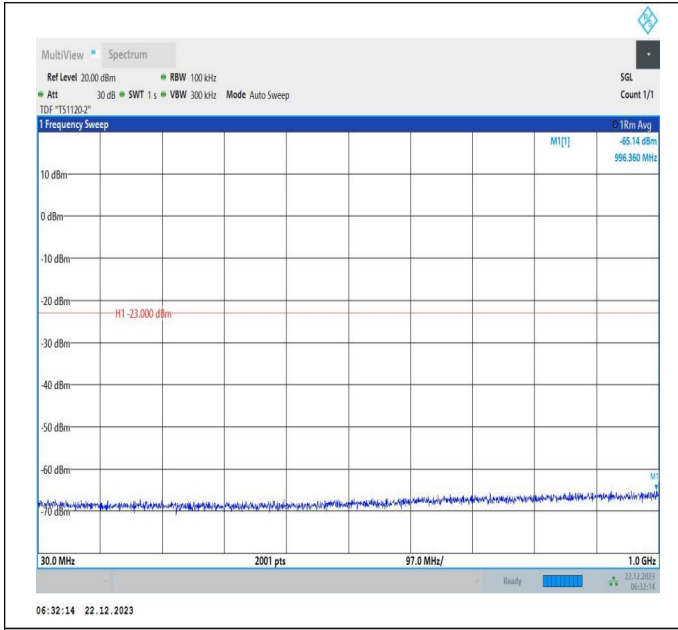
66-66-15MHz-20MHz-64QAM-64QAM-132050-132221-1RB# 0-ORB#0-30~1000MHz-PASS
