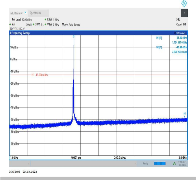
66-66-15MHz-20MHz-16QAM-16QAM-132050-132221-1RB# 74-ORB#0-1000~3000MHz-PASS
