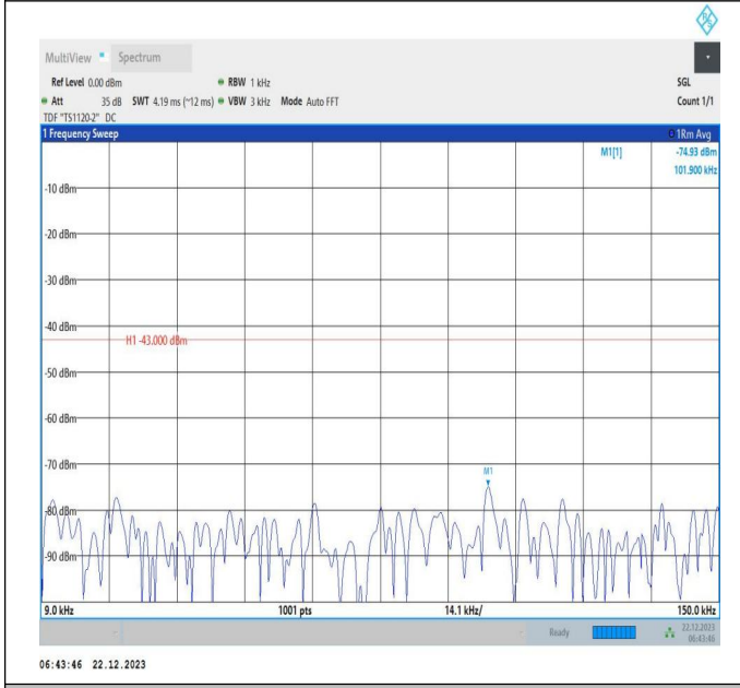
66-66-15MHz-20MHz-64QAM-64QAM-132325-132496-1RB# 0-ORB#0-0.009~0.15MHz-PASS
