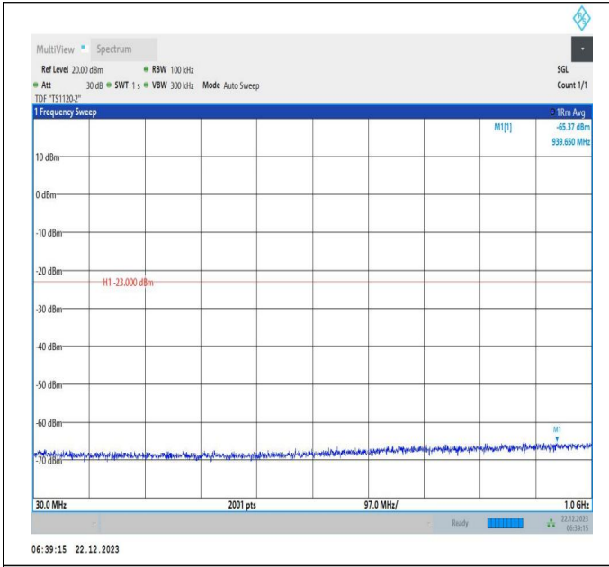
66-66-15MHz-20MHz-16QAM-16QAM-132050-132221-75RB #0-100RB#0-30~1000MHz-PASS
