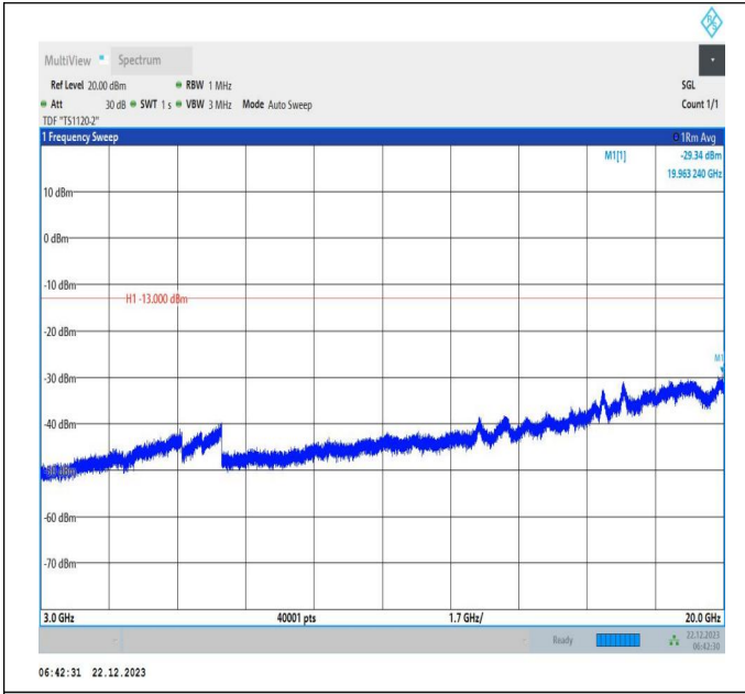
66-66-15MHz-20MHz-QPSK-QPSK-132325-132496-1RB#0-ORB#0-3000~20000MHz-PASS
