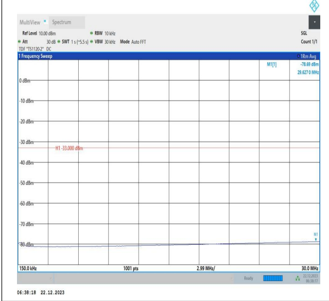
66-66-15MHz-20MHz-QPSK-QPSK-132050-132221-75RB#0-100RB#0-0.15~30MHz-PASS
