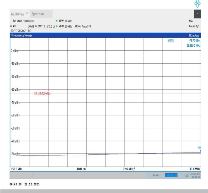
66-66-15MHz-20MHz-QPSK-QPSK-132325-132496-1RB#0- 1RB#99-0.15~30MHz-PASS
