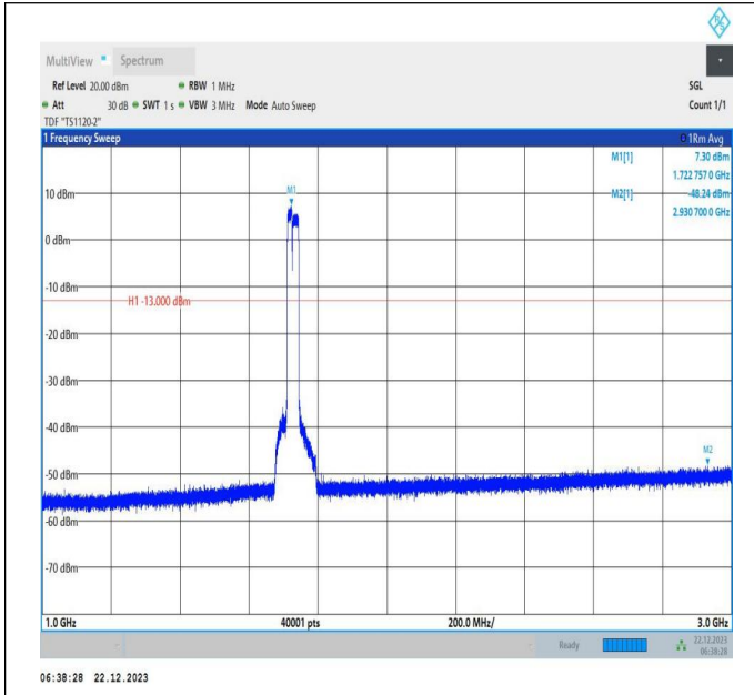
66-66-15MHz-20MHz-QPSK-QPSK-132050-132221-75RB#0 -100RB#0-1000~3000MHz-PASS
