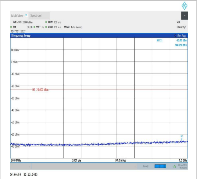
66-66-15MHz-20MHz-64QAM-64QAM-132050-132221-75RB #0-100RB#0-30~1000MHz-PASS
