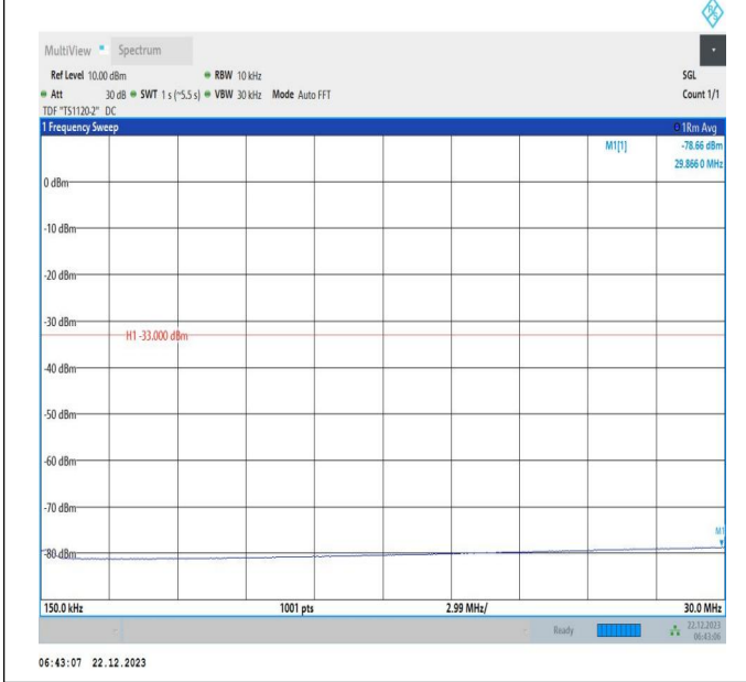
66-66-15MHz-20MHz-16QAM-16QAM-132325-132496-1RB#0-ORB#0-0.15~30MHz-PASS
