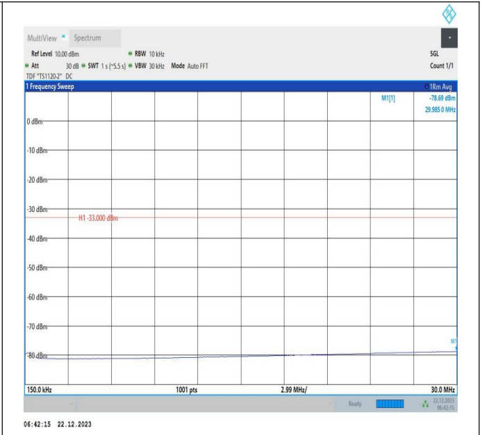
66-66-15MHz-20MHz-QPSK-QPSK-132325-132496-1RB#0-ORB#0-0.15~30MHz-PASS
