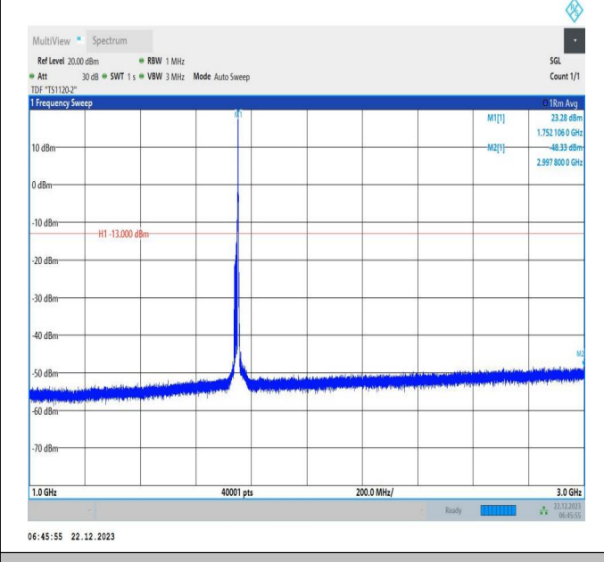
66-66-15MHz-20MHz-16QAM-16QAM-132325-132496-1RB# 74-ORB#0-1000~3000MHz-PASS
