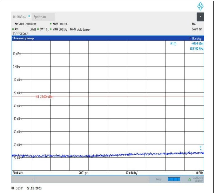
66-66-15MHz-20MHz-QPSK-QPSK-132050-132221-1RB#74 -ORB#0-30~1000MHz-PASS
