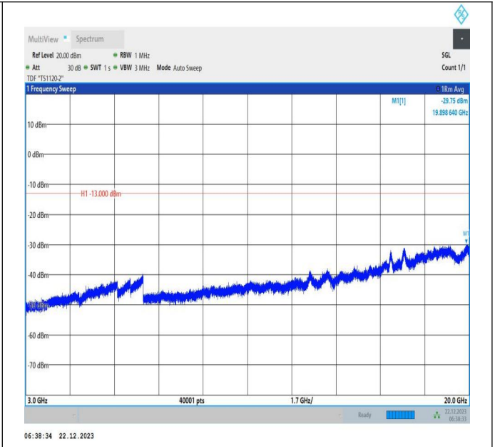
66-66-15MHz-20MHz-QPSK-QPSK-132050-132221-75RB#0 -100RB#0-3000~20000MHz-PASS
