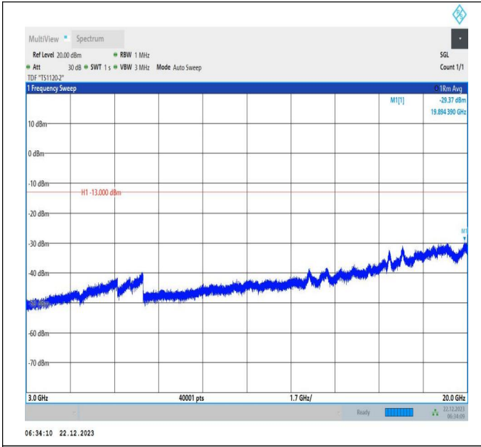
66-66-15MHz-20MHz-16QAM-16QAM-132050-132221-1RB# 74-ORB#0-3000~20000MHz-PASS
