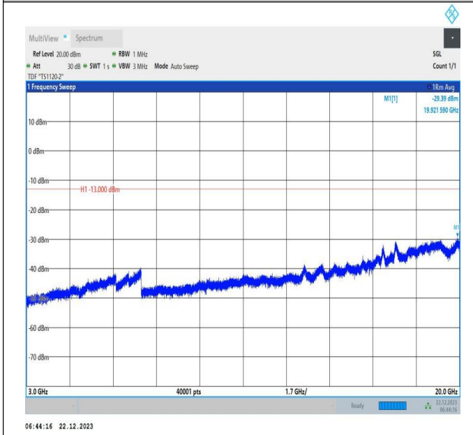
66-66-15MHz-20MHz-64QAM-64QAM-132325-132496-1RB# 0-ORB#0-3000~20000MHz-PASS
