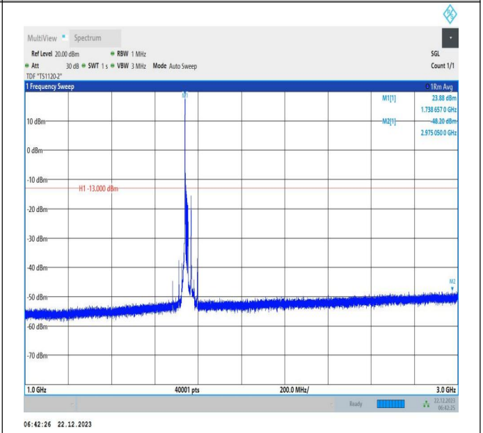
66-66-15MHz-20MHz-QPSK-QPSK-132325-132496-1RB#0-ORB#0-1000~3000MHz-PASS
