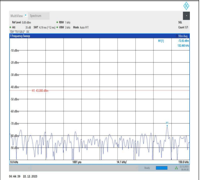
66-66-15MHz-20MHz-QPSK-QPSK-132325-132496-1RB#74 -ORB#0-0.009~0.15MHz-PASS
