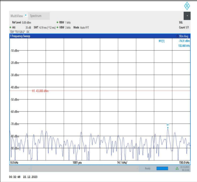
66-66-15MHz-20MHz-QPSK-QPSK-132050-132221-1RB#74 -ORB#0-0.009~0.15MHz-PASS
