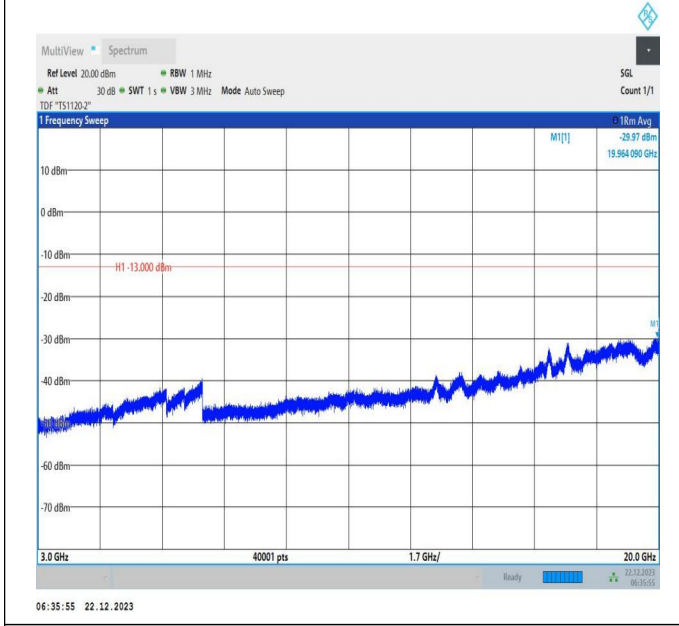
66-66-15MHz-20MHz-QPSK-QPSK-132050-132221-1RB#0-1RB#99-3000~20000MHz-PASS
