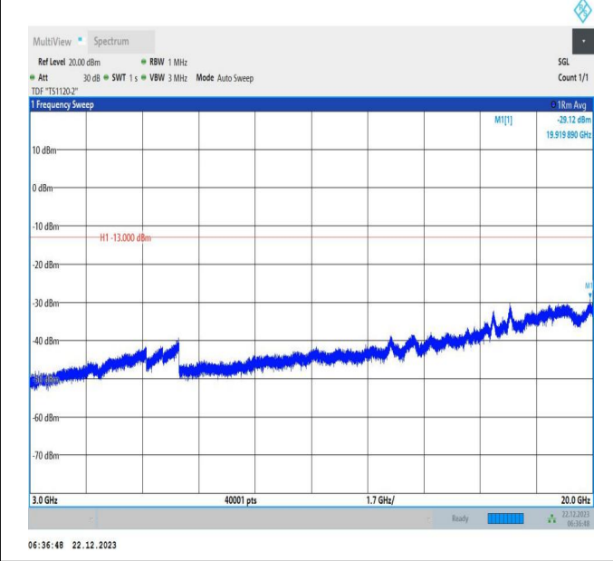
66-66-15MHz-20MHz-16QAM-16QAM-132050-132221-1RB# 0-1RB#99-3000~20000MHz-PASS
