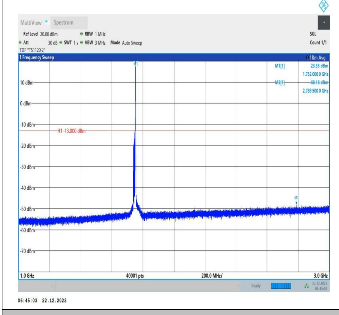
66-66-15MHz-20MHz-QPSK-QPSK-132325-132496-1RB#74 -ORB#0-1000~3000MHz-PASS
