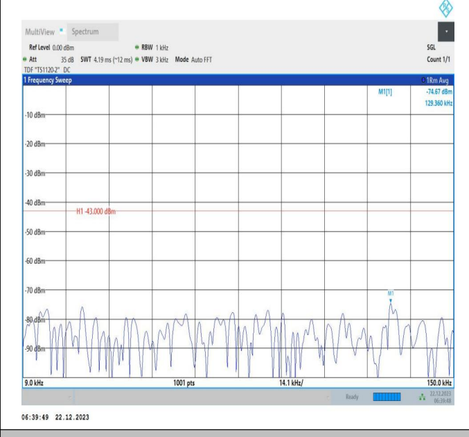
66-66-15MHz-20MHz-64QAM-64QAM-132050-132221-75RB #0-100RB#0-0.009~0.15MHz-PASS
