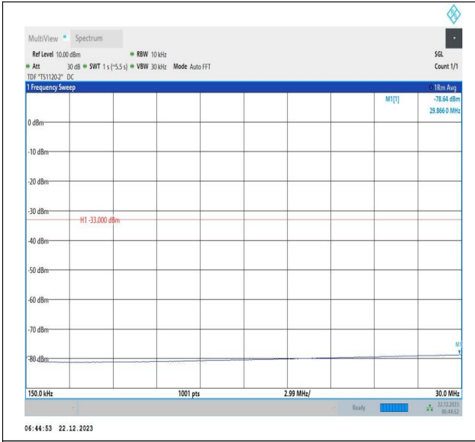
66-66-15MHz-20MHz-QPSK-QPSK-132325-132496-1RB#74 -ORB#0-0.15~30MHz-PASS
