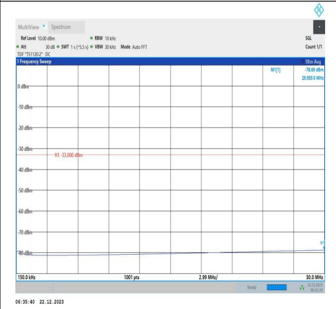
66-66-15MHz-20MHz-QPSK-QPSK-132050-132221-1RB#0- 1RB#99-0.15~30MHz-PASS
