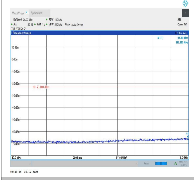
66-66-15MHz-20MHz-16QAM-16QAM-132050-132221-1RB# 74-ORB#0-30~1000MHz-PASS
