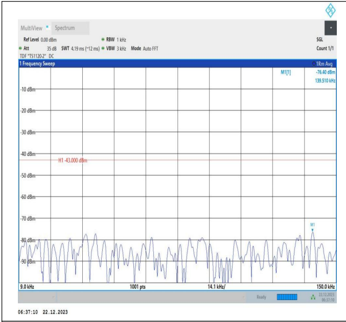
66-66-15MHz-20MHz-64QAM-64QAM-132050-132221-1RB# 0-1RB#99-0.009~0.15MHz-PASS
