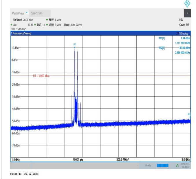
66-66-15MHz-20MHz-16QAM-16QAM-132050-132221-1RB# 0-1RB#99-1000~3000MHz-PASS
