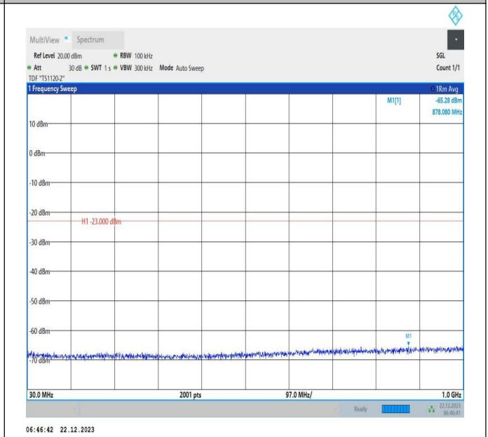
66-66-15MHz-20MHz-64QAM-64QAM-132325-132496-1RB# 74-ORB#0-30~1000MHz-PASS
