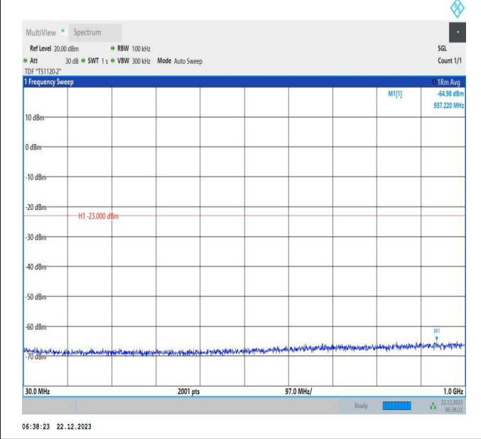
66-66-15MHz-20MHz-QPSK-QPSK-132050-132221-75RB#0-100RB#0-30~1000MHz-PASS
