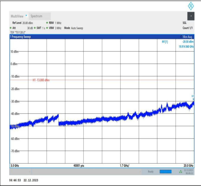
66-66-15MHz-20MHz-64QAM-64QAM-132325-132496-1RB# 74-0RB#0-3000~20000MHz-PASS
