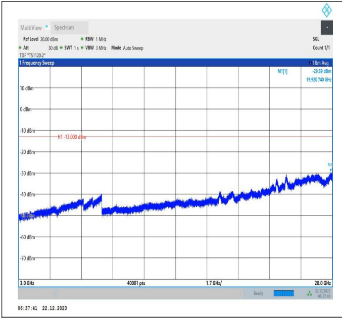
66-66-15MHz-20MHz-64QAM-64QAM-132050-132221-1RB#0-1RB#99-3000~20000MHz-PASS
