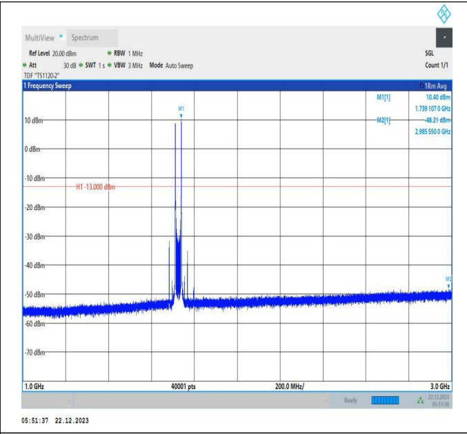
66-66-15MHz-15MHz-QPSK-QPSK-132047-132197-1RB#0-1RB#74-1000~3000MHz-PASS
