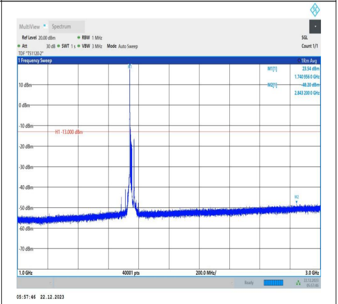
66-66-15MHz-15MHz-QPSK-QPSK-132347-132497-1RB#0-ORB#0-1000~3000MHz-PASS
