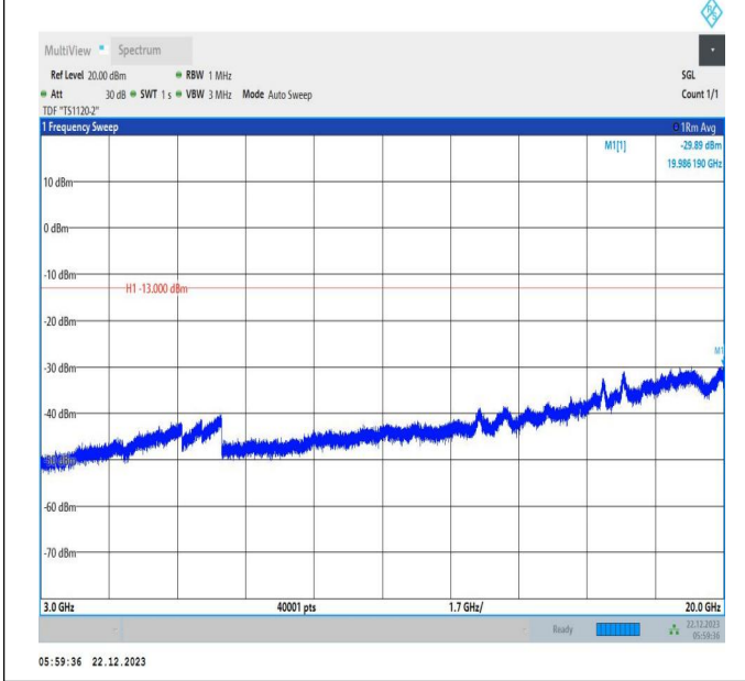
66-66-15MHz-15MHz-64QAM-64QAM-132347-132497-1RB# 0-ORB#0-3000~20000MHz-PASS
