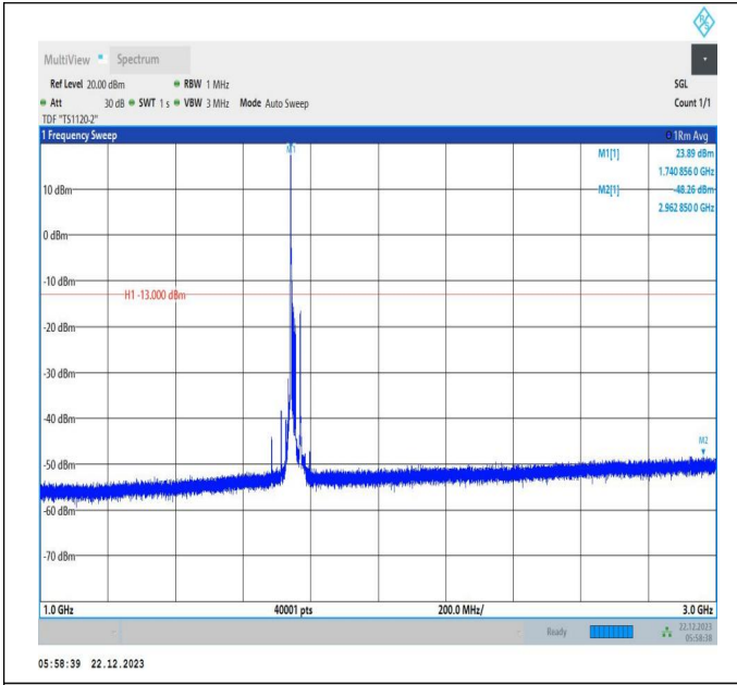
66-66-15MHz-15MHz-16QAM-16QAM-132347-132497-1RB# 0-ORB#0-1000~3000MHz-PASS
