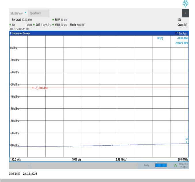
66-66-15MHz-15MHz-16QAM-16QAM-132047-132197-75RB #0-75RB#0-0.15~30MHz-PASS
