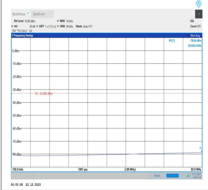
66-66-15MHz-15MHz-QPSK-QPSK-132347-132497-75RB#0-75RB#0-0.15~30MHz-PASS
