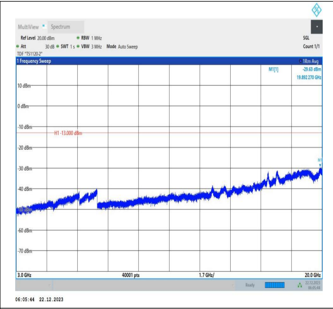
66-66-15MHz-15MHz-QPSK-QPSK-132347-132497-75RB#0 -75RB#0-3000~20000MHz-PASS
