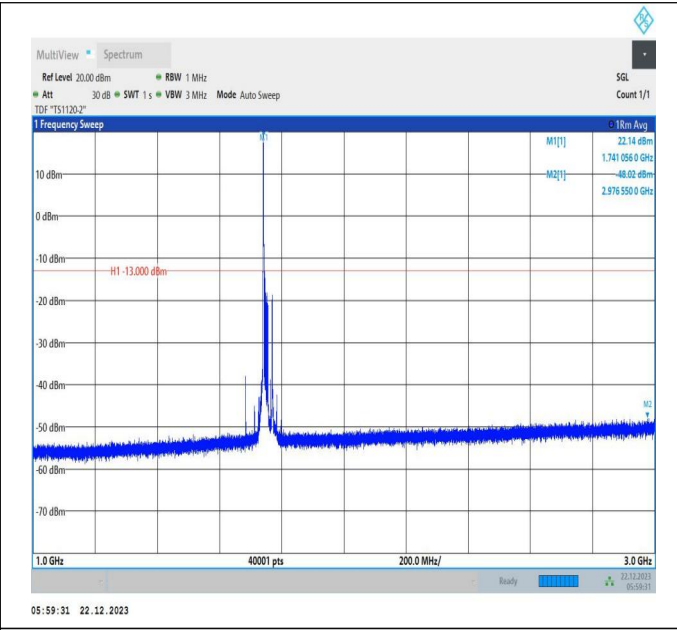
66-66-15MHz-15MHz-64QAM-64QAM-132347-132497-1RB# 0-ORB#0-1000~3000MHz-PASS
