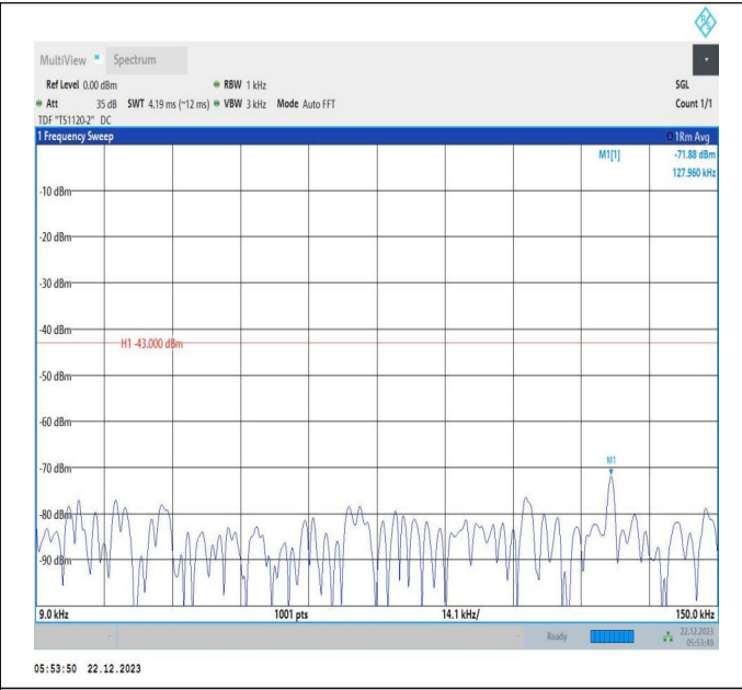
66-66-15MHz-15MHz-QPSK-QPSK-132047-132197-75RB#0-75RB#0-0.009~0.15MHz-PASS
