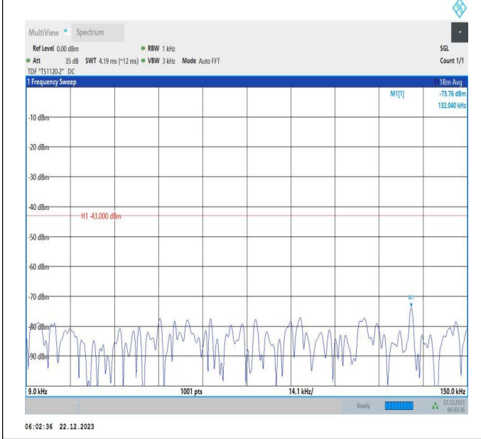
66-66-15MHz-15MHz-QPSK-QPSK-132347-132497-1RB#0- 1RB#74-0.009~0.15MHz-PASS
