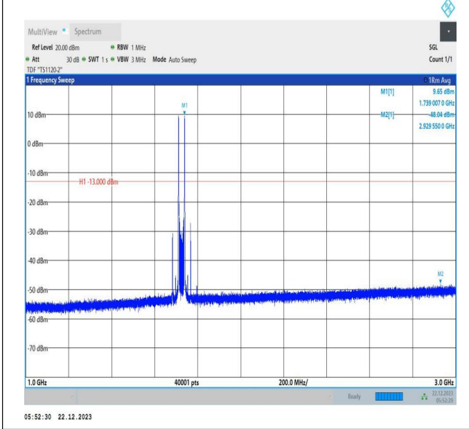
66-66-15MHz-15MHz-16QAM-16QAM-132047-132197-1RB# 0-1RB#74-1000~3000MHz-PASS
