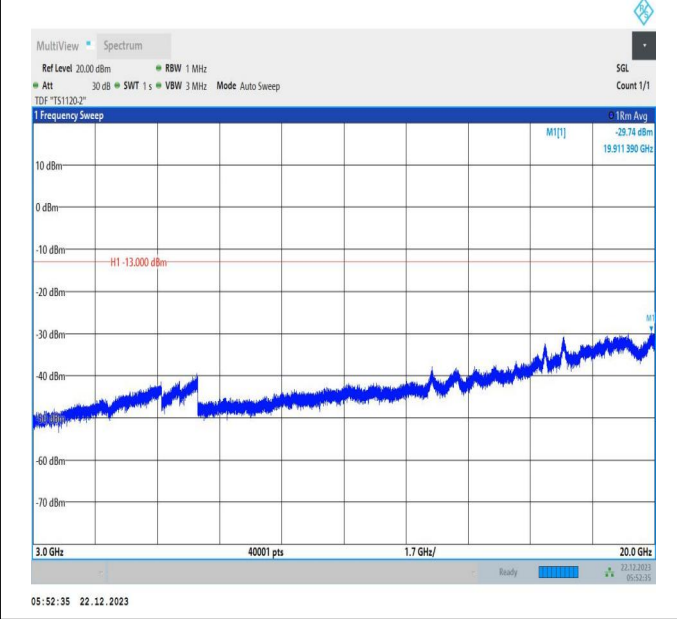
66-66-15MHz-15MHz-16QAM-16QAM-132047-132197-1RB# 0-1RB#74-3000~20000MHz-PASS
