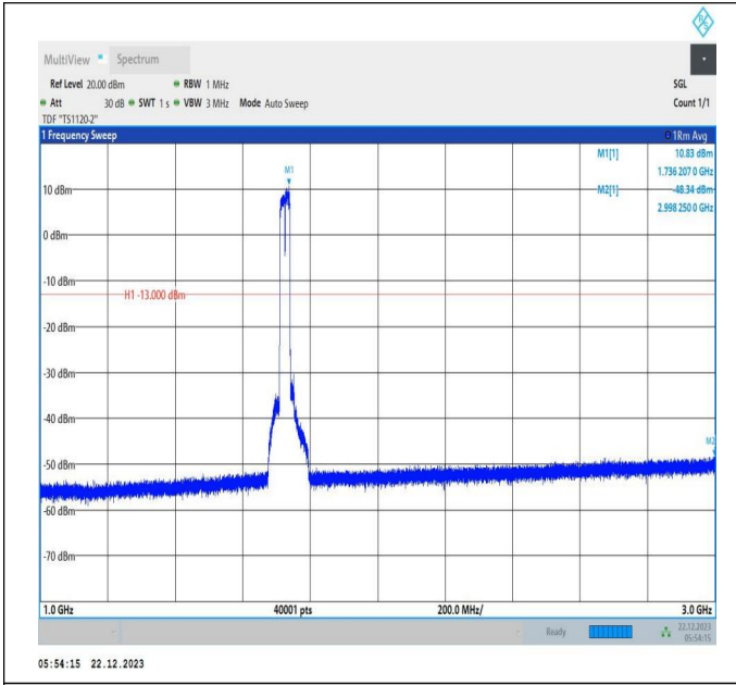
66-66-15MHz-15MHz-QPSK-QPSK-132047-132197-75RB#0 -75RB#0-1000~3000MHz-PASS
