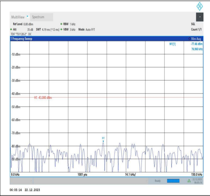
66-66-15MHz-15MHz-QPSK-QPSK-132347-132497-75RB#0-75RB#0-0.009~0.15MHz-PASS
