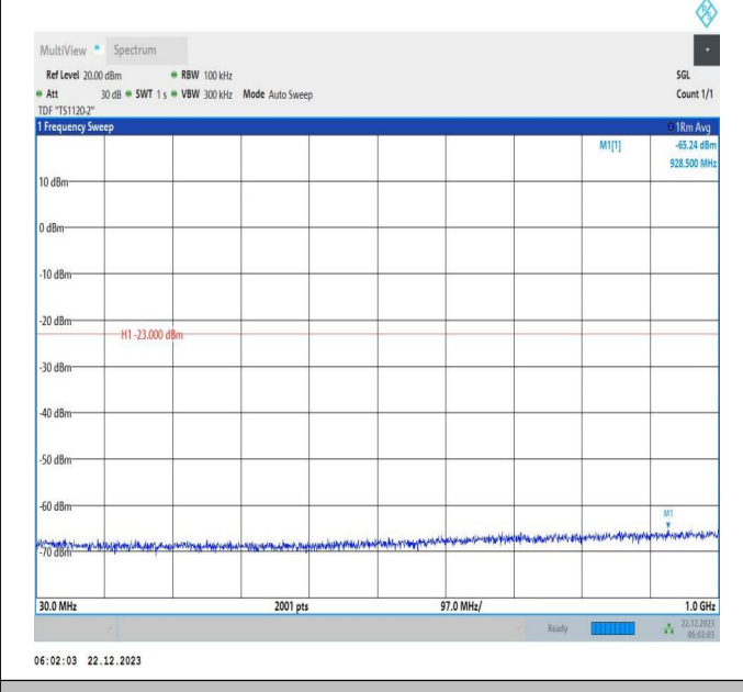
66-66-15MHz-15MHz-64QAM-64QAM-132347-132497-1RB# 74-ORB#0-30~1000MHz-PASS
