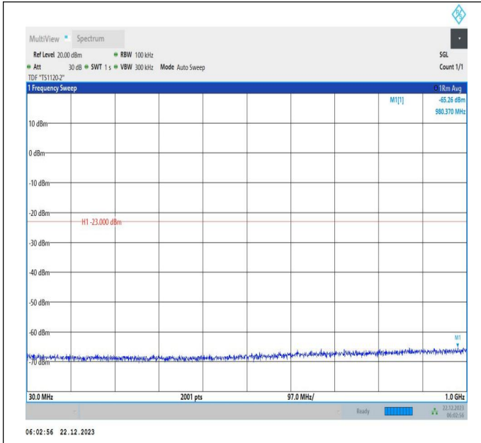
66-66-15MHz-15MHz-QPSK-QPSK-132347-132497-1RB#0-1RB#74-30~1000MHz-PASS
