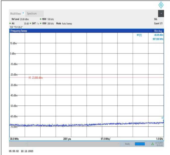
66-66-15MHz-15MHz-16QAM-16QAM-132047-132197-75RB #0-75RB#0-30~1000MHz-PASS
