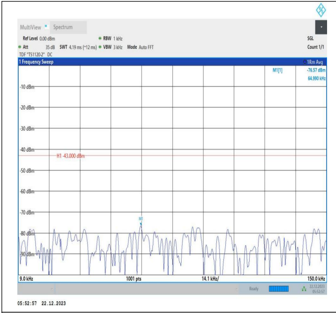
66-66-15MHz-15MHz-64QAM-64QAM-132047-132197-1RB# 0-1RB#74-0.009~0.15MHz-PASS
