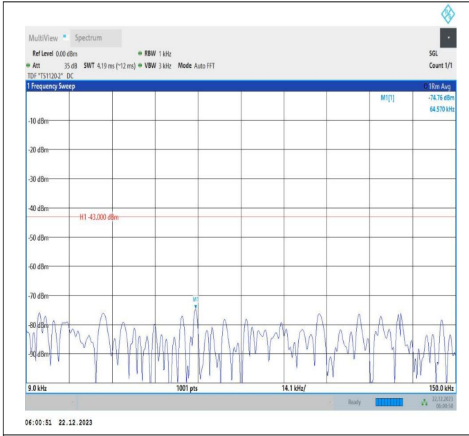
66-66-15MHz-15MHz-16QAM-16QAM-132347-132497-1RB# 74-ORB#0-0.009~0.15MHz-PASS
