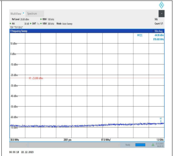
66-66-15MHz-15MHz-QPSK-QPSK-132347-132497-1RB#74 -ORB#0-30~1000MHz-PASS
