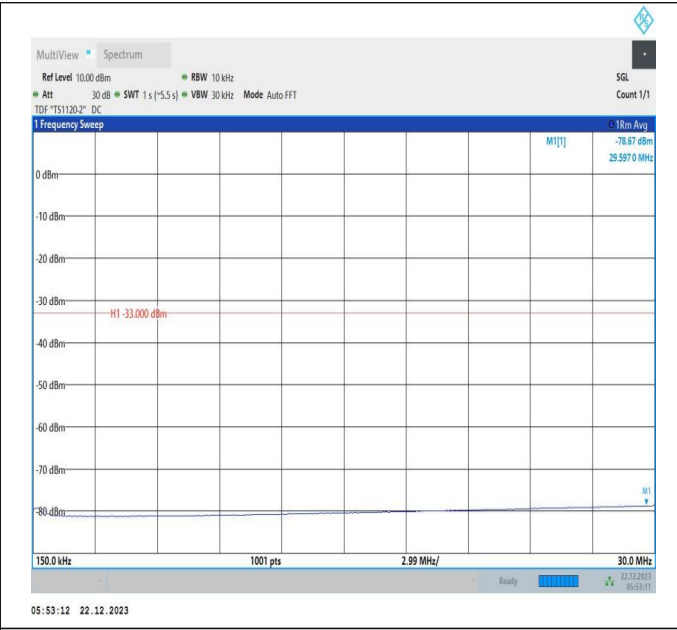
66-66-15MHz-15MHz-64QAM-64QAM-132047-132197-1RB# 0-1RB#74-0.15~30MHz-PASS
