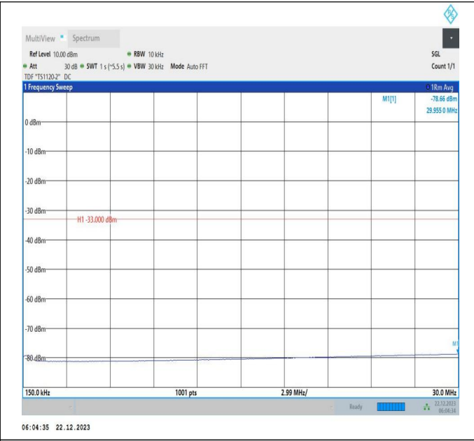
66-66-15MHz-15MHz-64QAM-64QAM-132347-132497-1RB# 0-1RB#74-0.15~30MHz-PASS
