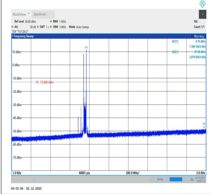
66-66-15MHz-15MHz-16QAM-16QAM-132347-132497-1RB# 0-1RB#74-1000~3000MHz-PASS
