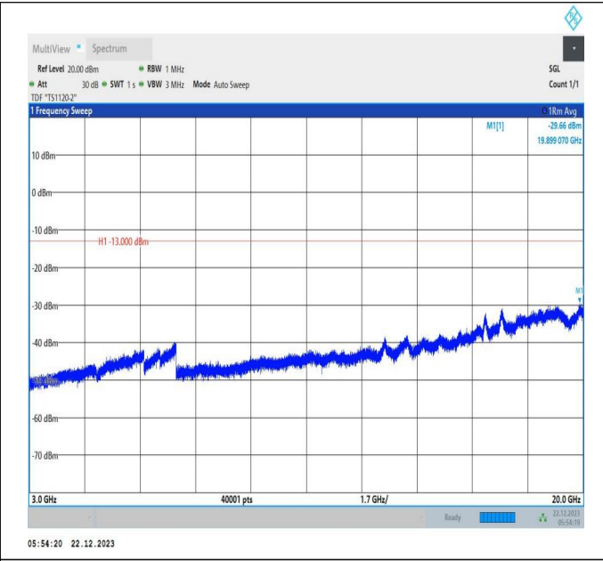
66-66-15MHz-15MHz-QPSK-QPSK-132047-132197-75RB#0 -75RB#0-3000~20000MHz-PASS
