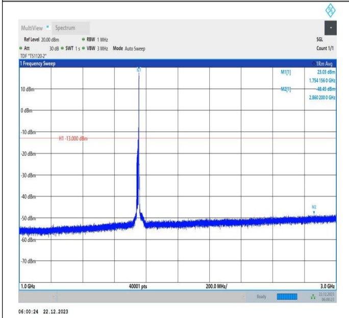
66-66-15MHz-15MHz-QPSK-QPSK-132347-132497-1RB#74 -ORB#0-1000~3000MHz-PASS
