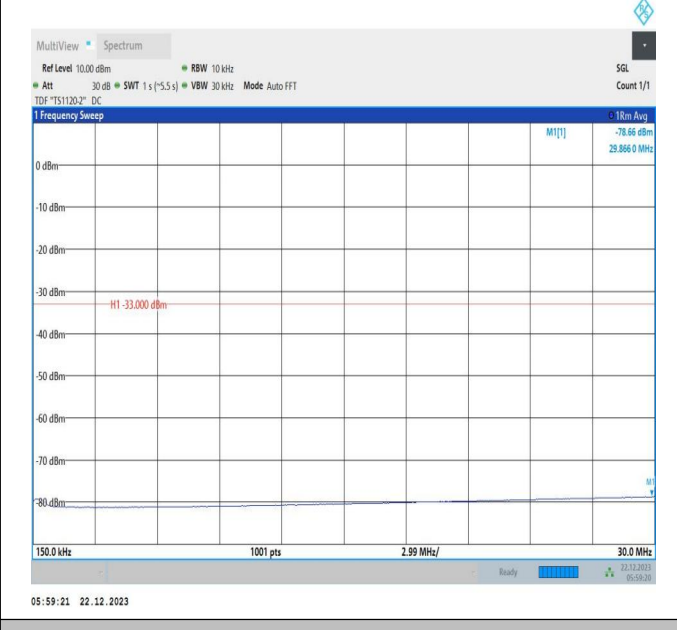
66-66-15MHz-15MHz-64QAM-64QAM-132347-132497-1RB# 0-ORB#0-0.15~30MHz-PASS
