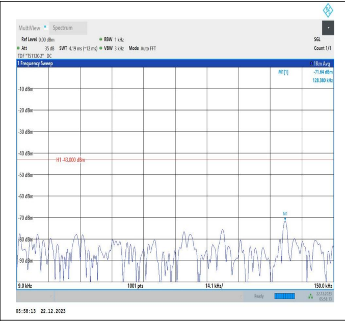
66-66-15MHz-15MHz-16QAM-16QAM-132347-132497-1RB#0-ORB#0-0.009~0.15MHz-PASS
