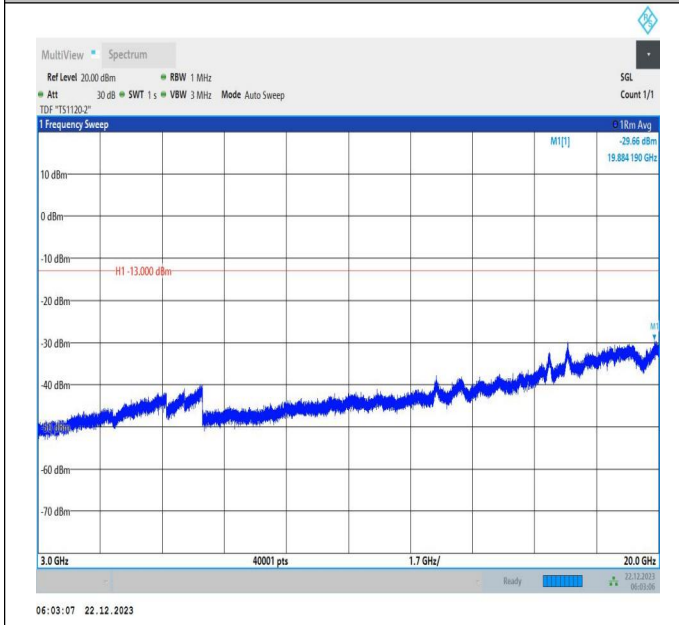
66-66-15MHz-15MHz-QPSK-QPSK-132347-132497-1RB#0-1RB#74-3000~20000MHz-PASS
