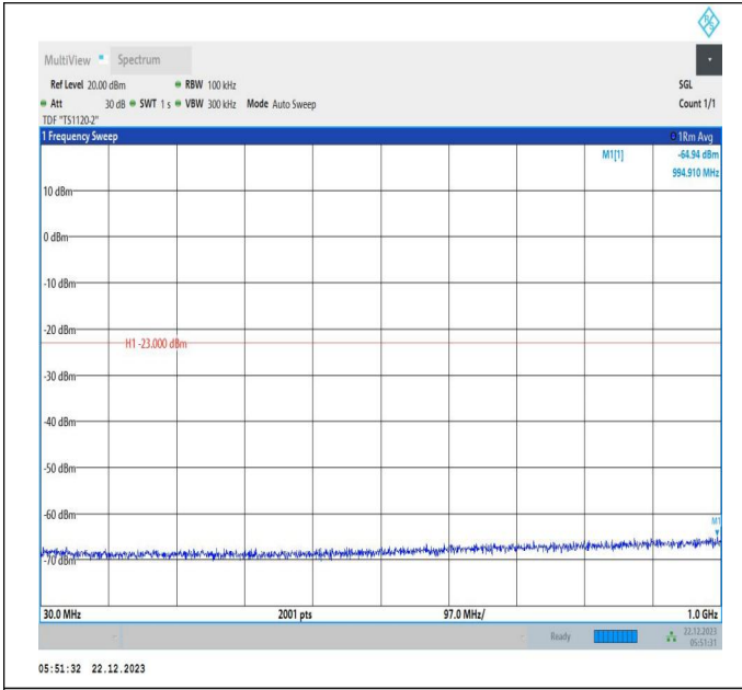
66-66-15MHz-15MHz-QPSK-QPSK-132047-132197-1RB#0-1RB#74-30~1000MHz-PASS
