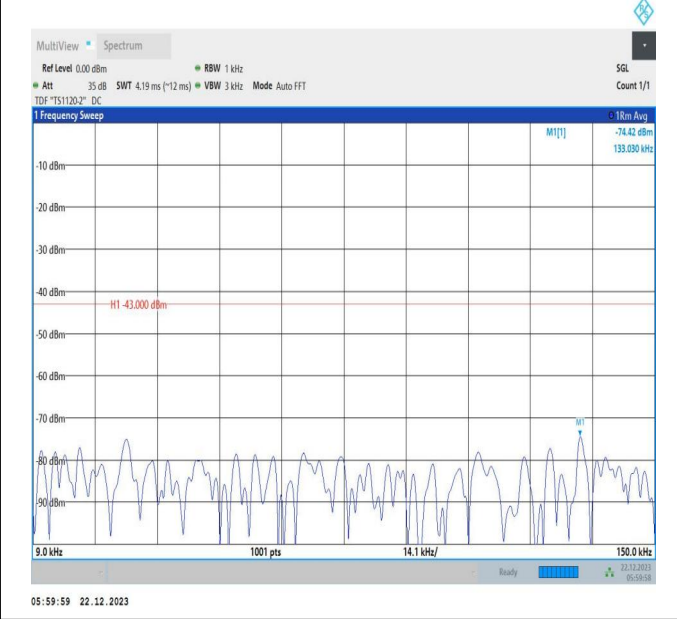
66-66-15MHz-15MHz-QPSK-QPSK-132347-132497-1RB#74 -ORB#0-0.009~0.15MHz-PASS
