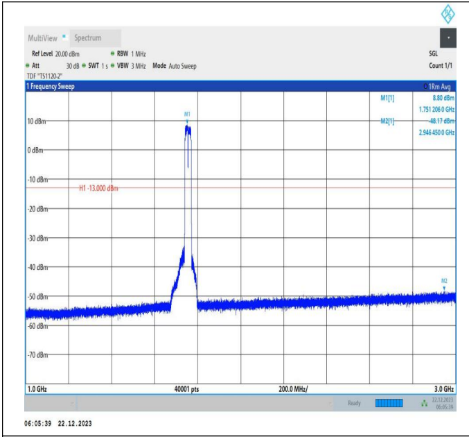
66-66-15MHz-15MHz-QPSK-QPSK-132347-132497-75RB#0 -75RB#0-1000~3000MHz-PASS
