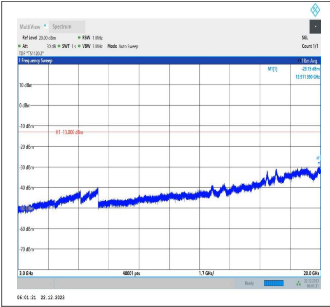
66-66-15MHz-15MHz-16QAM-16QAM-132347-132497-1RB# 74-ORB#0-3000~20000MHz-PASS
