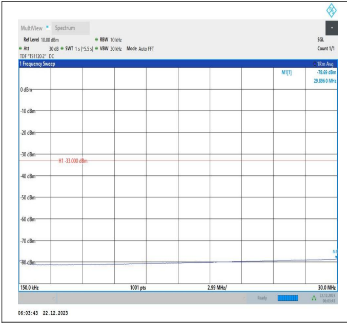
66-66-15MHz-15MHz-16QAM-16QAM-132347-132497-1RB# 0-1RB#74-0.15~30MHz-PASS
