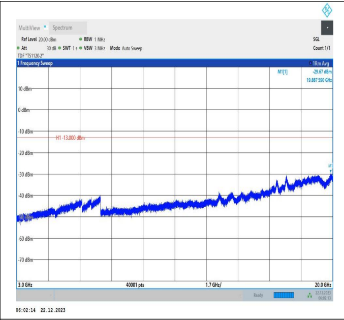
66-66-15MHz-15MHz-64QAM-64QAM-132347-132497-1RB# 74-0RB#0-3000~20000MHz-PASS
