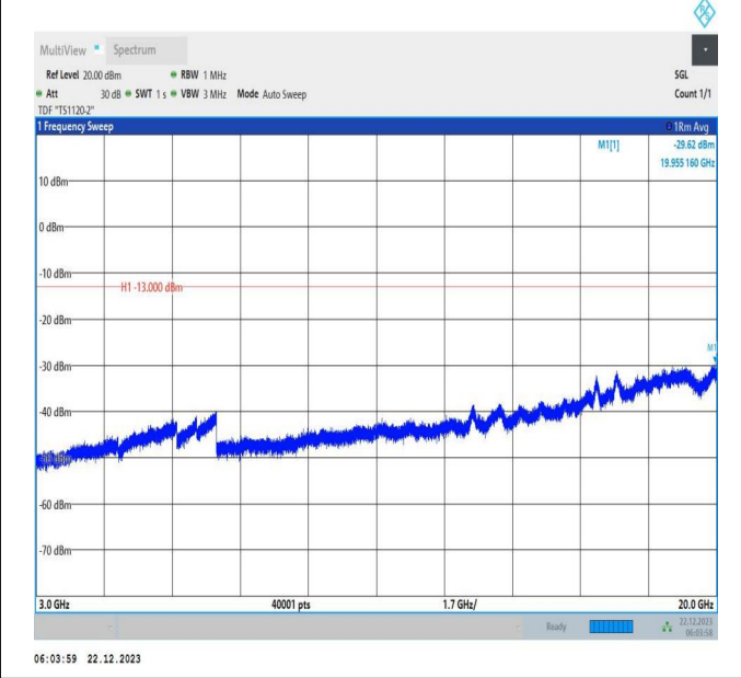
66-66-15MHz-15MHz-16QAM-16QAM-132347-132497-1RB# 0-1RB#74-3000~20000MHz-PASS
