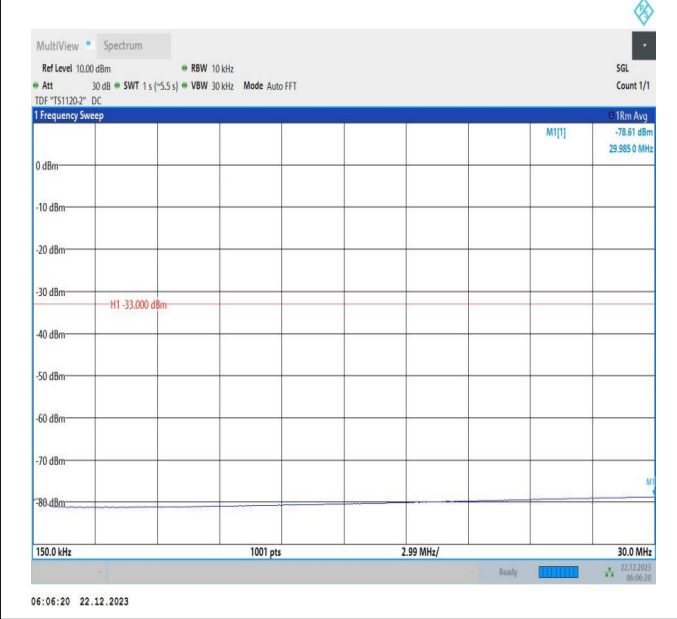
66-66-15MHz-15MHz-16QAM-16QAM-132347-132497-75RB #0-75RB#0-0.15~30MHz-PASS
