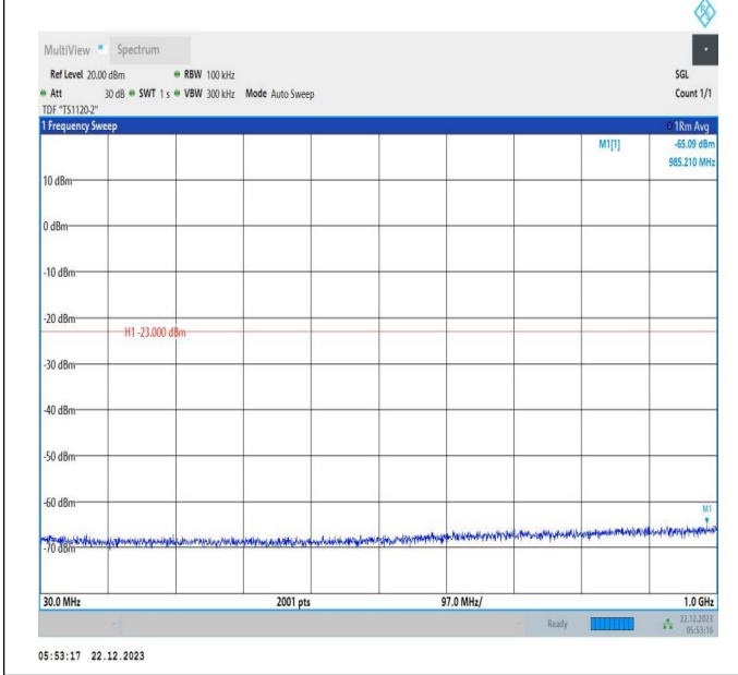
66-66-15MHz-15MHz-64QAM-64QAM-132047-132197-1RB# 0-1RB#74-30~1000MHz-PASS
