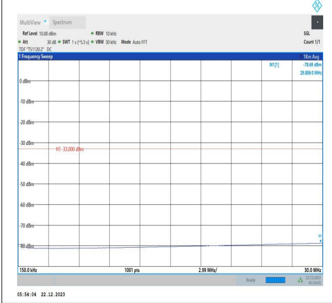
66-66-15MHz-15MHz-QPSK-QPSK-132047-132197-75RB#0-75RB#0-0.15~30MHz-PASS
