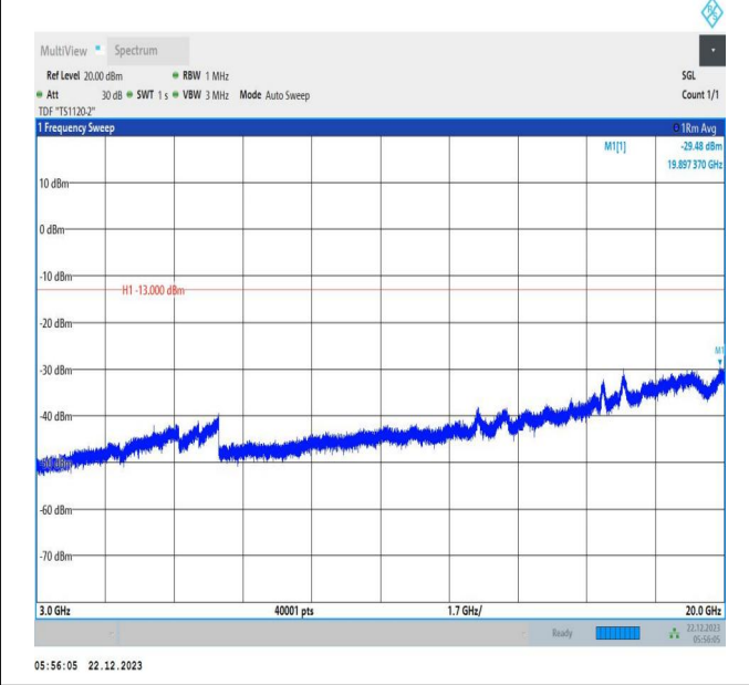
66-66-15MHz-15MHz-64QAM-64QAM-132047-132197-75RB #0-75RB#0-3000~20000MHz-PASS
