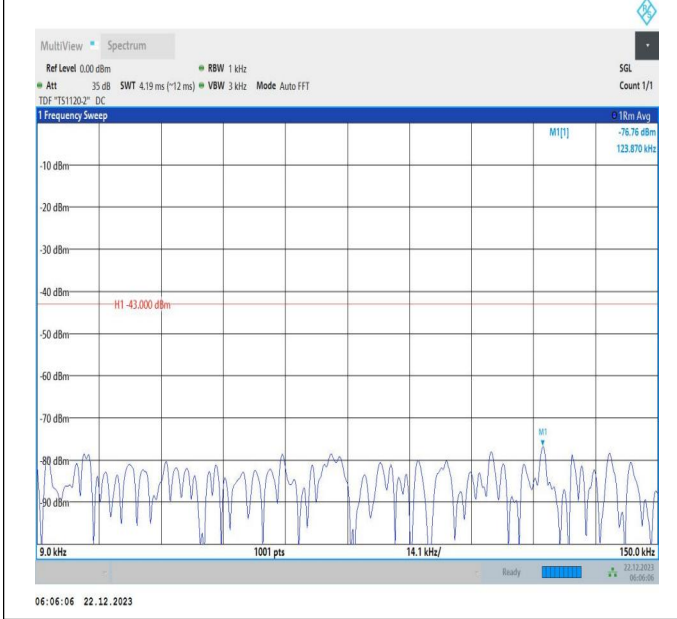
66-66-15MHz-15MHz-16QAM-16QAM-132347-132497-75RB #0-75RB#0-0.009~0.15MHz-PASS
