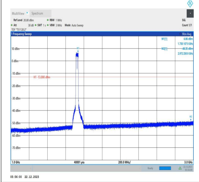
66-66-15MHz-15MHz-64QAM-64QAM-132047-132197-75RB #0-75RB#0-1000~3000MHz-PASS
