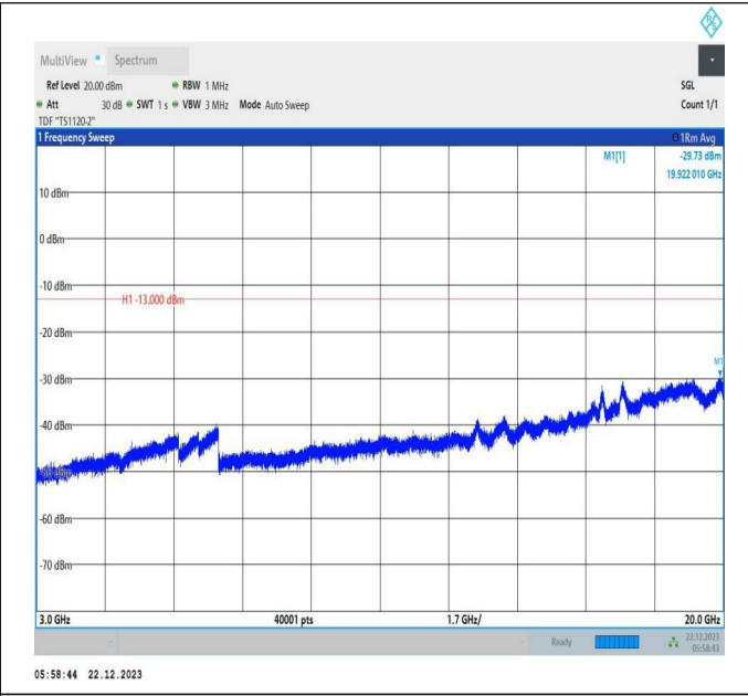
66-66-15MHz-15MHz-16QAM-16QAM-132347-132497-1RB# 0-ORB#0-3000~20000MHz-PASS
