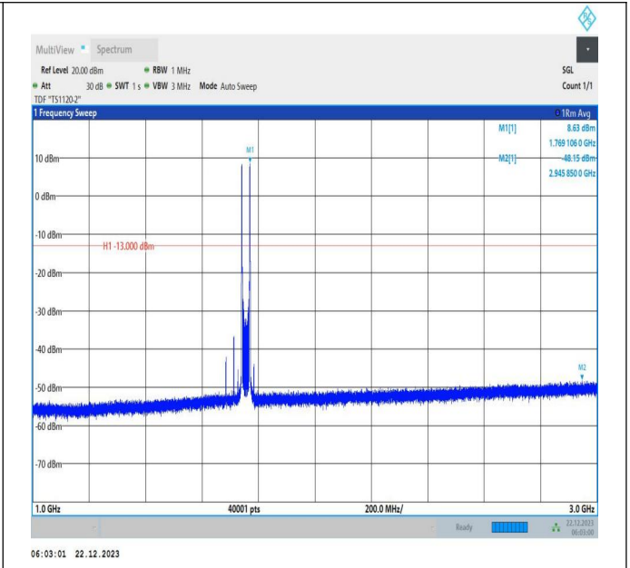
66-66-15MHz-15MHz-QPSK-QPSK-132347-132497-1RB#0-1RB#74-1000~3000MHz-PASS
