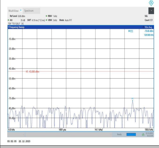
66-66-15MHz-15MHz-16QAM-16QAM-132047-132197-1RB#0-1RB#74-0.009~0.15MHz-PASS
