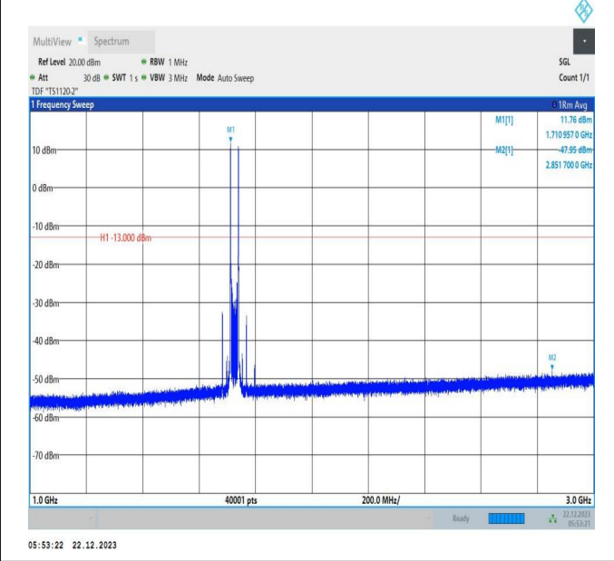
66-66-15MHz-15MHz-64QAM-64QAM-132047-132197-1RB# 0-1RB#74-1000~3000MHz-PASS
