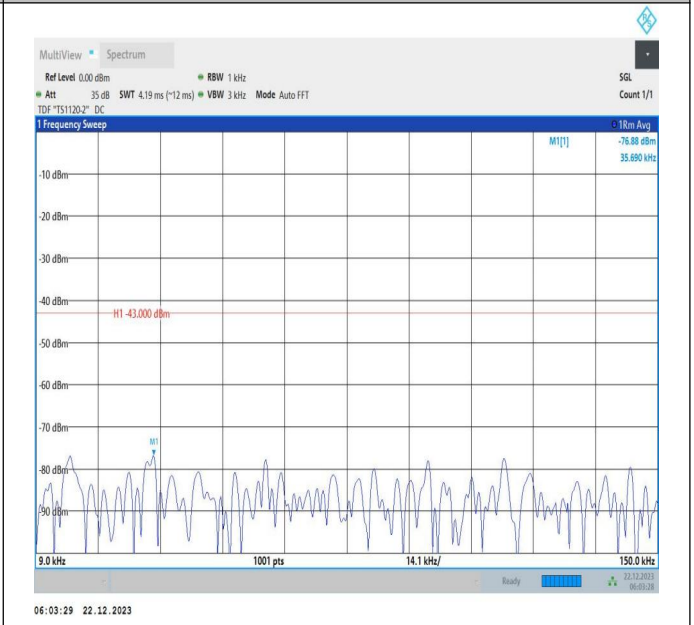
66-66-15MHz-15MHz-16QAM-16QAM-132347-132497-1RB#0-1RB#74-0.009~0.15MHz-PASS
