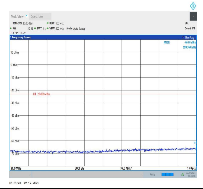
66-66-15MHz-15MHz-16QAM-16QAM-132347-132497-1RB# 0-1RB#74-30~1000MHz-PASS
