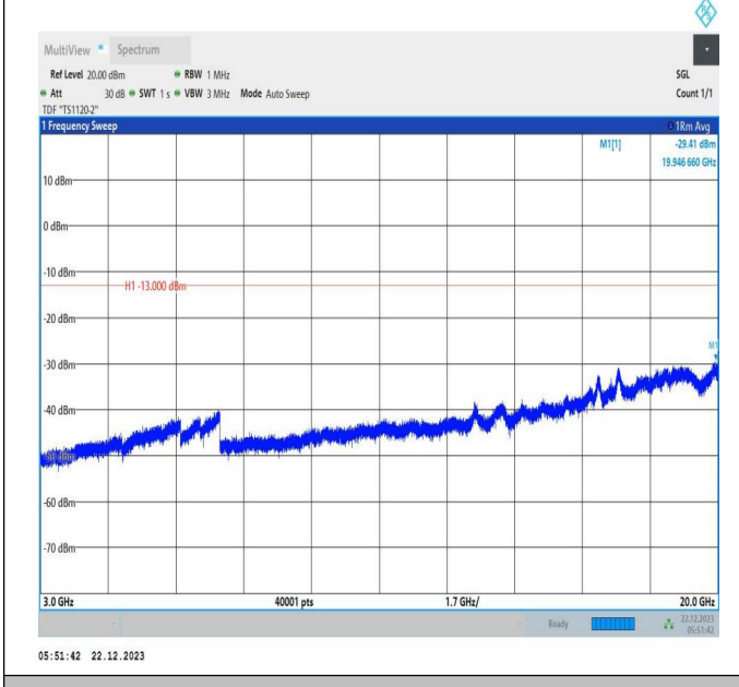
66-66-15MHz-15MHz-QPSK-QPSK-132047-132197-1RB#0-1RB#74-3000~20000MHz-PASS
