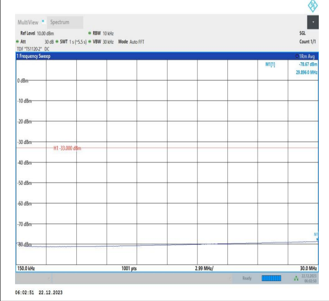
66-66-15MHz-15MHz-QPSK-QPSK-132347-132497-1RB#0- 1RB#74-0.15~30MHz-PASS
