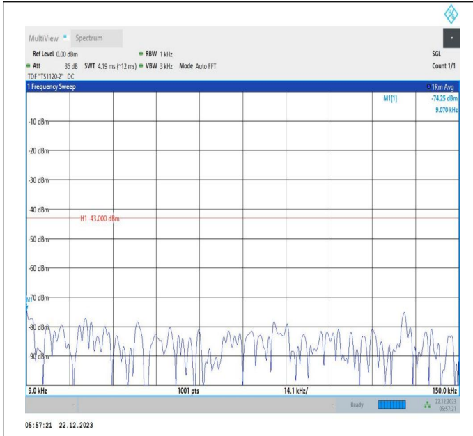
66-66-15MHz-15MHz-QPSK-QPSK-132347-132497-1RB#0-ORB#0-0.009~0.15MHz-PASS
