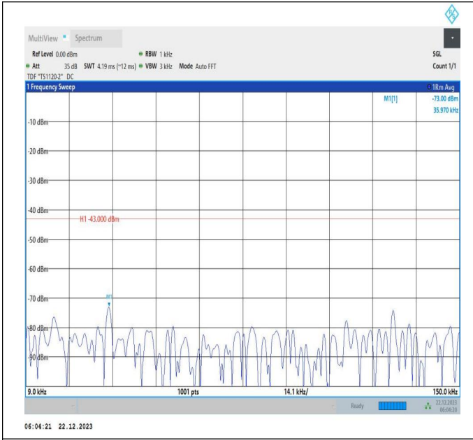
66-66-15MHz-15MHz-64QAM-64QAM-132347-132497-1RB# 0-1RB#74-0.009~0.15MHz-PASS
