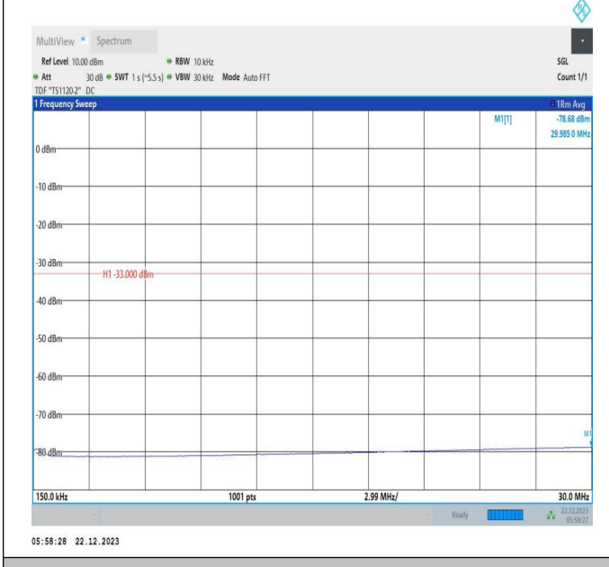
66-66-15MHz-15MHz-16QAM-16QAM-132347-132497-1RB#0-ORB#0-0.15~30MHz-PASS
