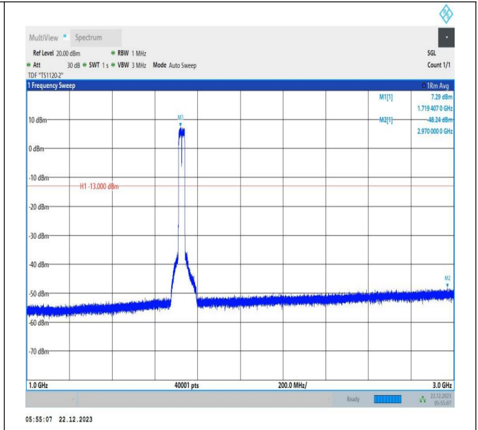
66-66-15MHz-15MHz-16QAM-16QAM-132047-132197-75RB #0-75RB#0-1000~3000MHz-PASS
