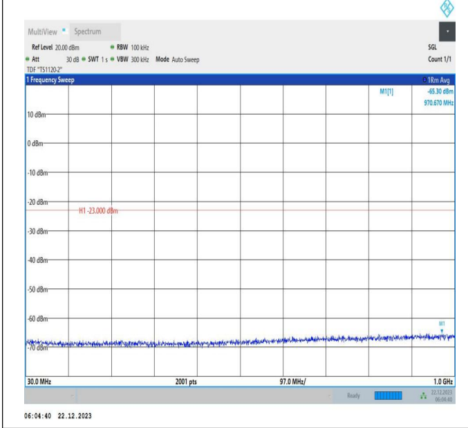
66-66-15MHz-15MHz-64QAM-64QAM-132347-132497-1RB# 0-1RB#74-30~1000MHz-PASS
