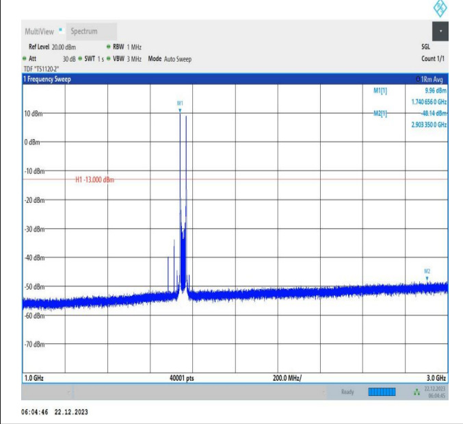
66-66-15MHz-15MHz-64QAM-64QAM-132347-132497-1RB# 0-1RB#74-1000~3000MHz-PASS
