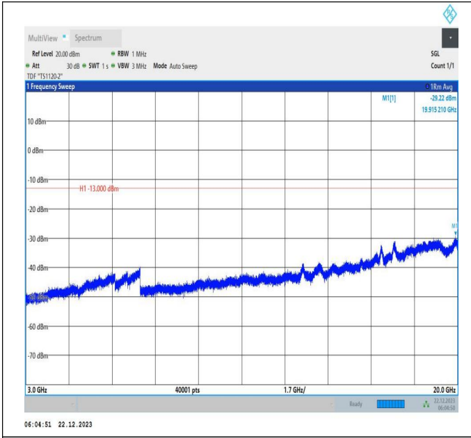
66-66-15MHz-15MHz-64QAM-64QAM-132347-132497-1RB#0-1RB#74-3000~20000MHz-PASS
