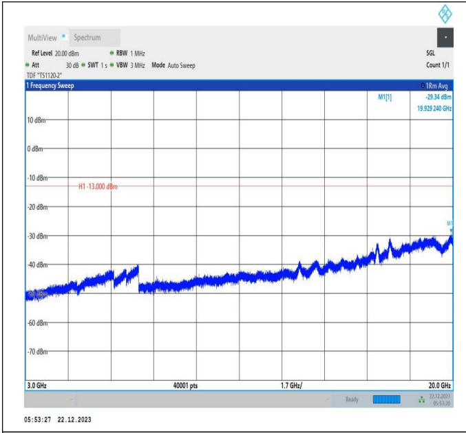
66-66-15MHz-15MHz-64QAM-64QAM-132047-132197-1RB#0-1RB#74-3000~20000MHz-PASS
