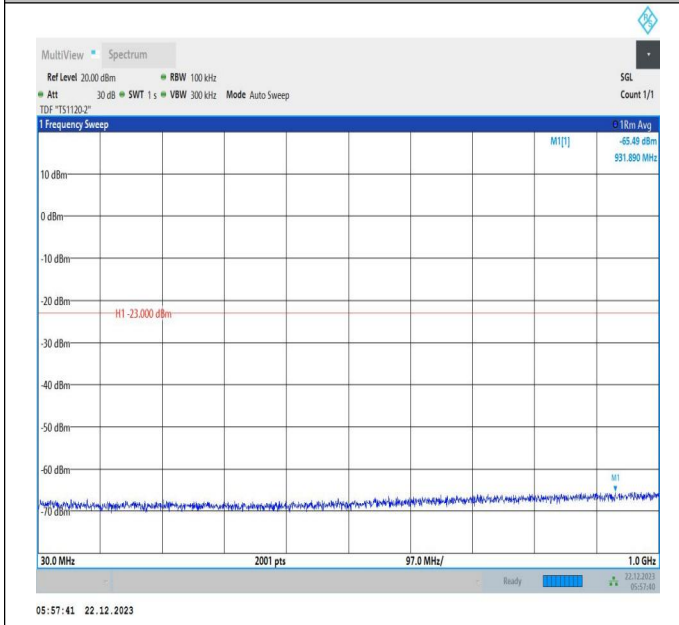
66-66-15MHz-15MHz-QPSK-QPSK-132347-132497-1RB#0-ORB#0-30~1000MHz-PASS
