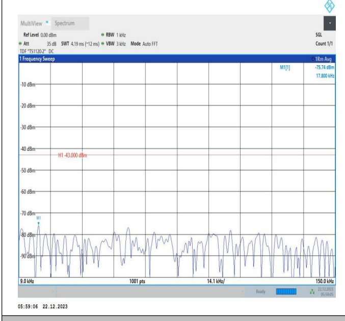
66-66-15MHz-15MHz-64QAM-64QAM-132347-132497-1RB# 0-ORB#0-0.009~0.15MHz-PASS
