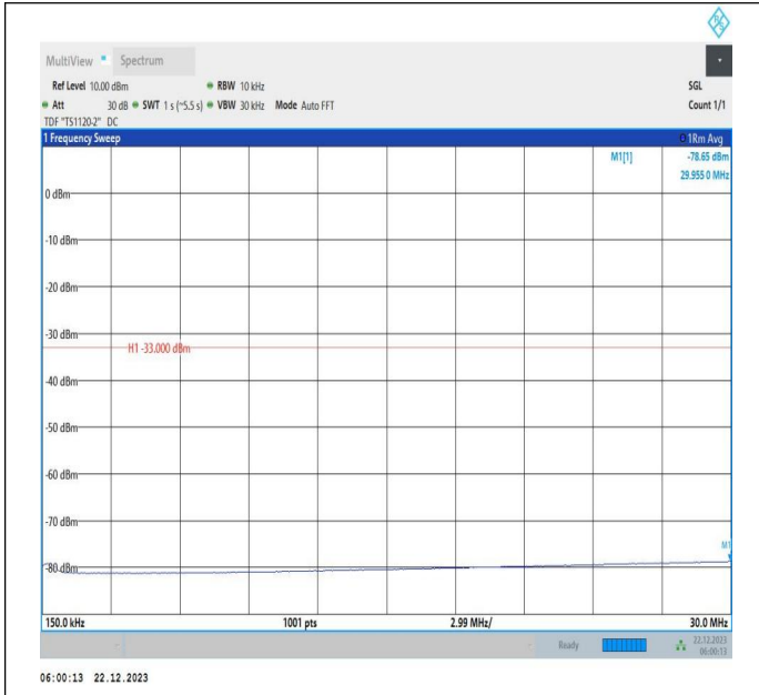
66-66-15MHz-15MHz-QPSK-QPSK-132347-132497-1RB#74 -ORB#0-0.15~30MHz-PASS
