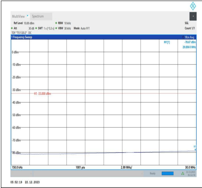
66-66-15MHz-15MHz-16QAM-16QAM-132047-132197-1RB# 0-1RB#74-0.15~30MHz-PASS
