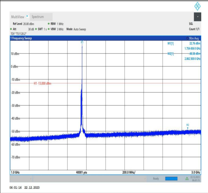
66-66-15MHz-15MHz-16QAM-16QAM-132347-132497-1RB# 74-ORB#0-1000~3000MHz-PASS
