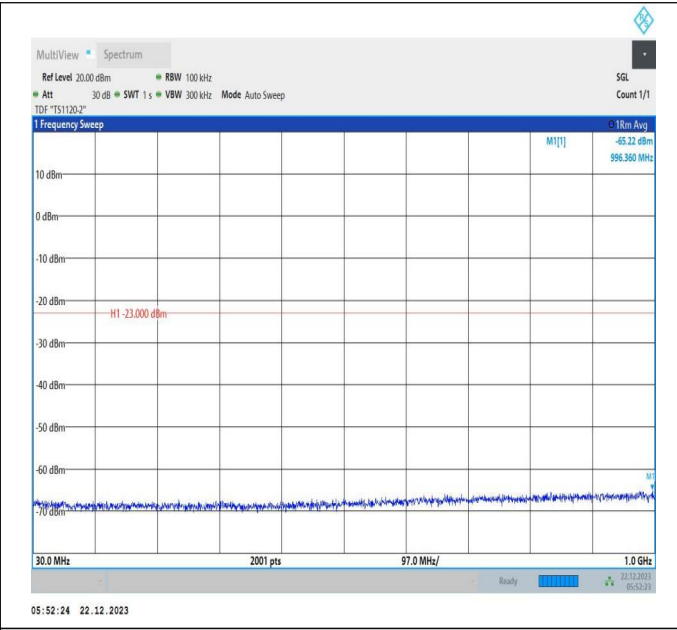
66-66-15MHz-15MHz-16QAM-16QAM-132047-132197-1RB# 0-1RB#74-30~1000MHz-PASS
