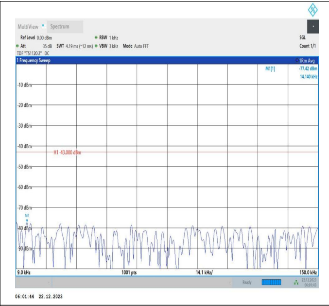
66-66-15MHz-15MHz-64QAM-64QAM-132347-132497-1RB# 74-ORB#0-0.009~0.15MHz-PASS
