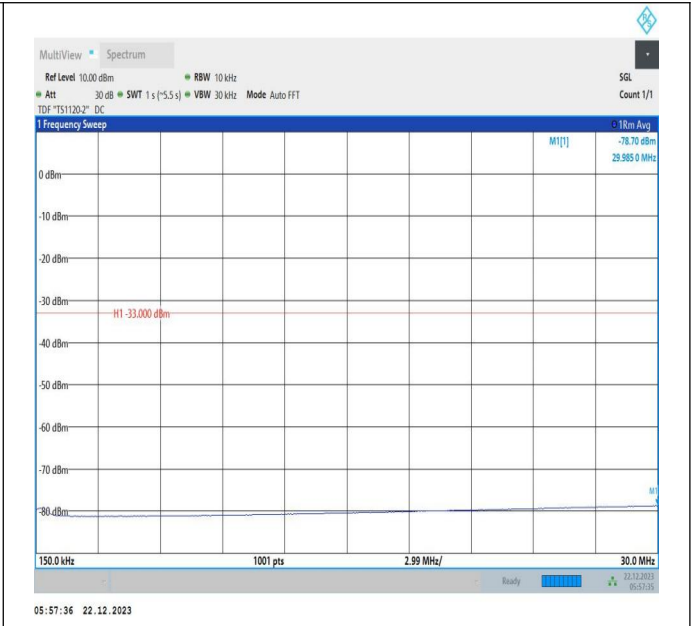
66-66-15MHz-15MHz-QPSK-QPSK-132347-132497-1RB#0-ORB#0-0.15~30MHz-PASS
