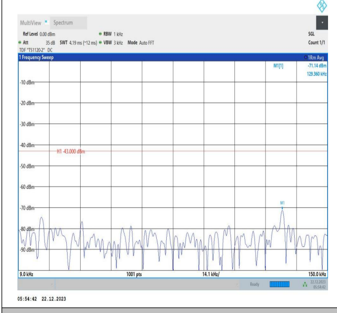
66-66-15MHz-15MHz-16QAM-16QAM-132047-132197-75RB #0-75RB#0-0.009~0.15MHz-PASS
