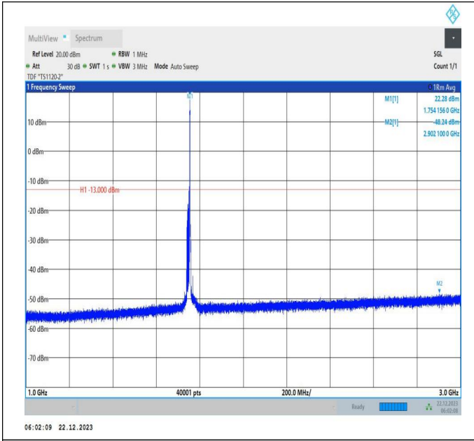
66-66-15MHz-15MHz-64QAM-64QAM-132347-132497-1RB# 74-0RB#0-1000~3000MHz-PASS
