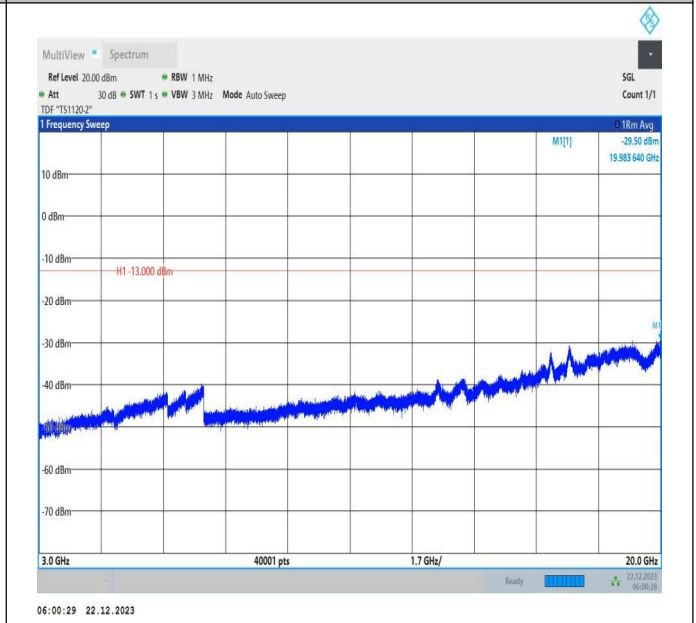
66-66-15MHz-15MHz-QPSK-QPSK-132347-132497-1RB#74 -ORB#0-3000~20000MHz-PASS
