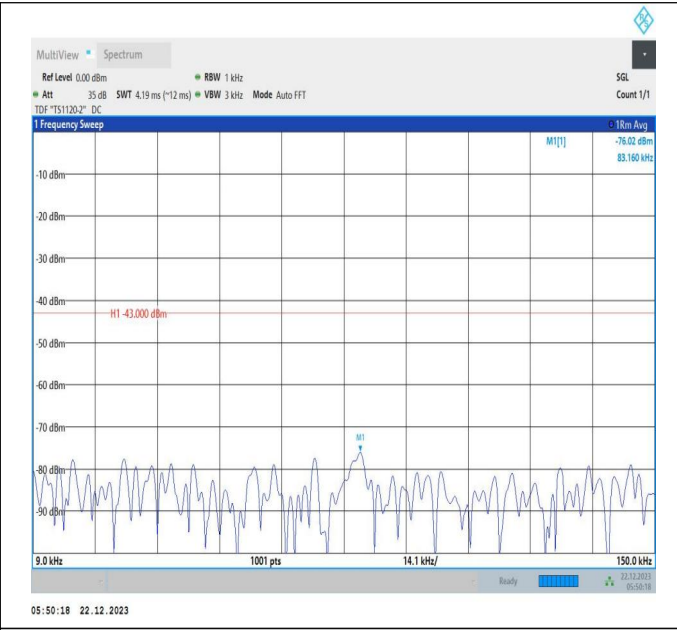
66-66-15MHz-15MHz-64QAM-64QAM-132047-132197-1RB# 74-ORB#0-0.009~0.15MHz-PASS
