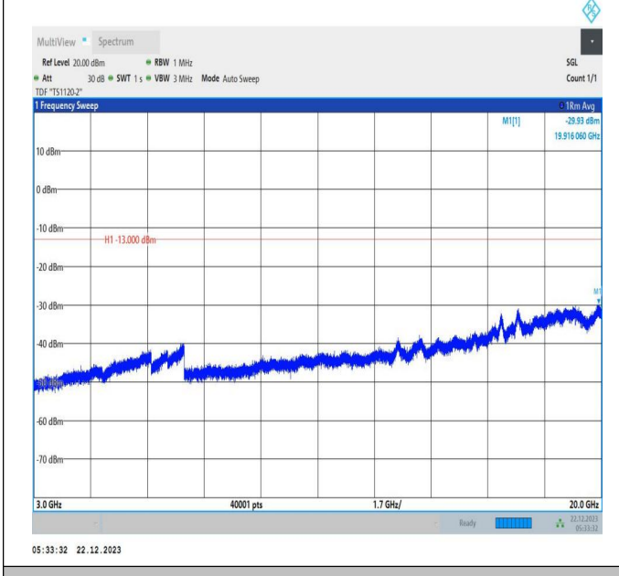
66-66-15MHz-10MHz-16QAM-16QAM-132499-132619-75RB #0-50RB#0-3000~20000MHz-PASS
