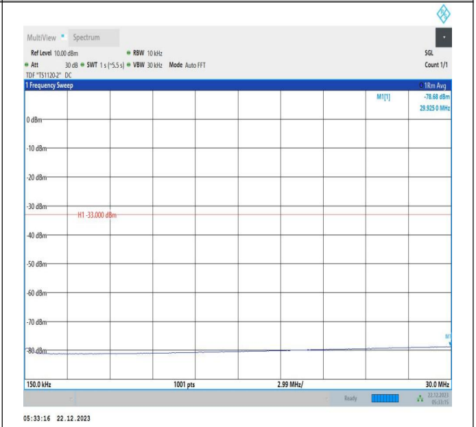
66-66-15MHz-10MHz-16QAM-16QAM-132499-132619-75RB #0-50RB#0-0.15~30MHz-PASS
