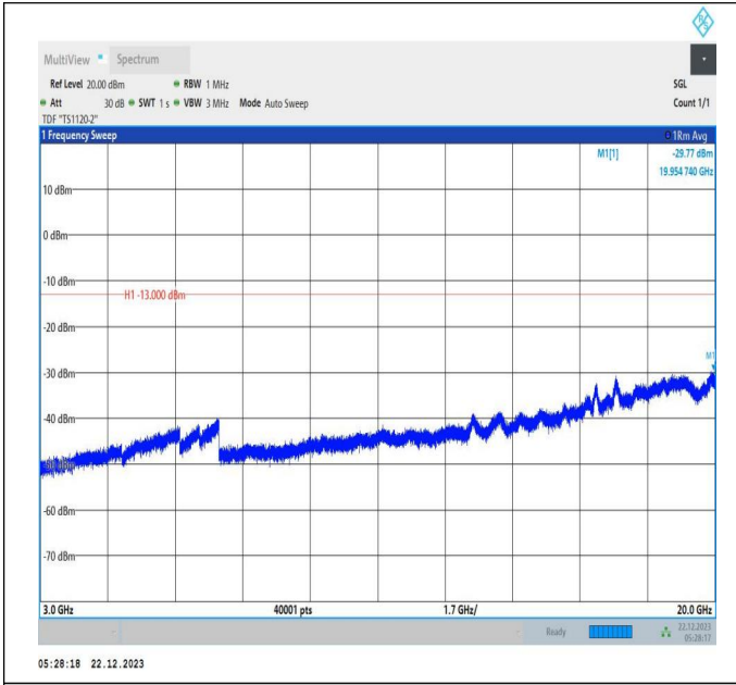
66-66-15MHz-10MHz-16QAM-16QAM-132499-132619-1RB# 74-ORB#0-3000~20000MHz-PASS
