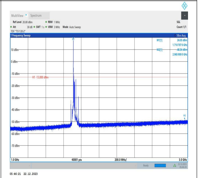
66-66-15MHz-15MHz-QPSK-QPSK-132047-132197-1RB#0-ORB#0-1000~3000MHz-PASS
