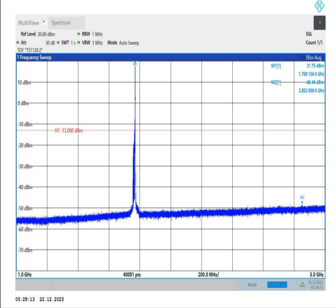
66-66-15MHz-10MHz-16QAM-16QAM-132499-132619-1RB# 74-ORB#0-1000~3000MHz-PASS
