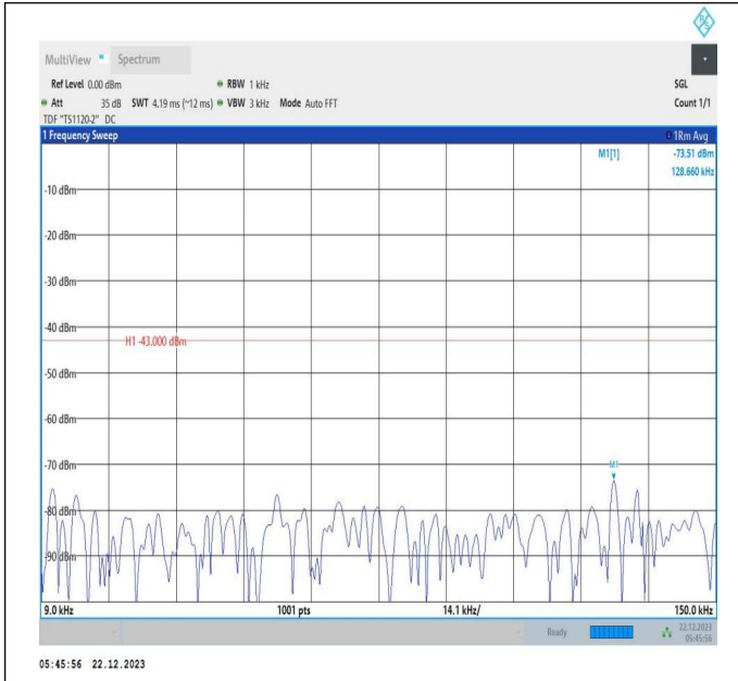
66-66-15MHz-15MHz-QPSK-QPSK-132047-132197-1RB#0-ORB#0-0.009~0.15MHz-PASS
