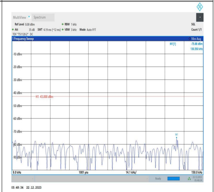
66-66-15MHz-15MHz-QPSK-QPSK-132047-132197-1RB#74 -ORB#0-0.009~0.15MHz-PASS
