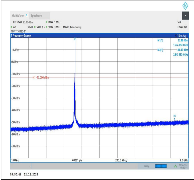
66-66-15MHz-15MHz-64QAM-64QAM-132047-132197-1RB# 74-0RB#0-1000~3000MHz-PASS
