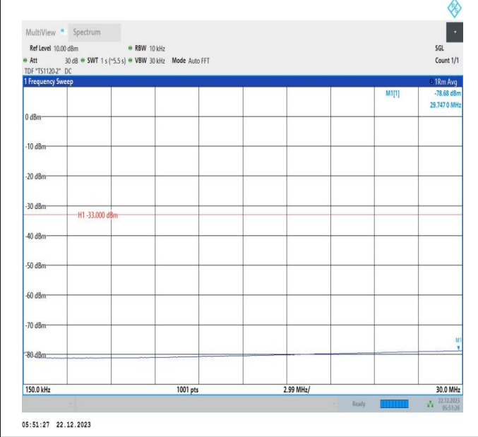
66-66-15MHz-15MHz-QPSK-QPSK-132047-132197-1RB#0- 1RB#74-0.15~30MHz-PASS
