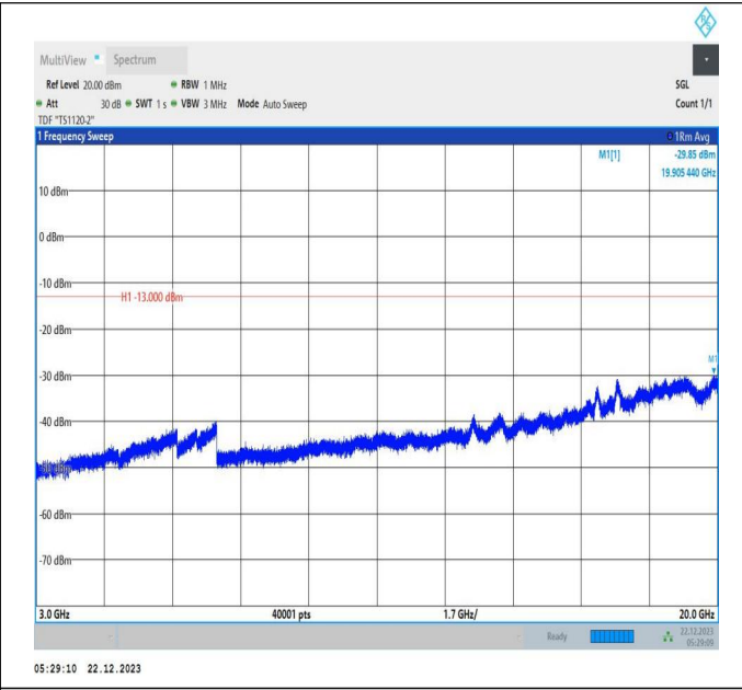
66-66-15MHz-10MHz-64QAM-64QAM-132499-132619-1RB# 74-ORB#0-3000~20000MHz-PASS
