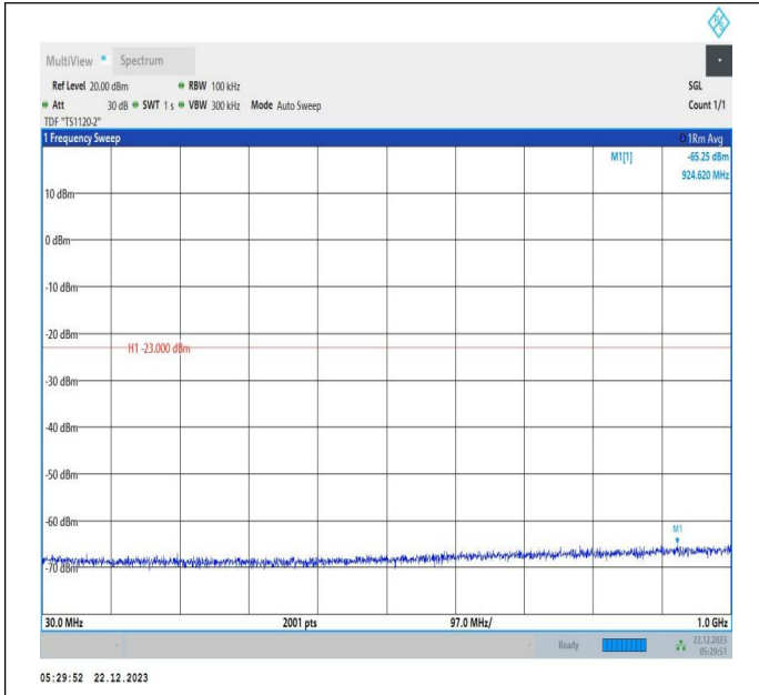
66-66-15MHz-10MHz-QPSK-QPSK-132499-132619-1RB#0-1RB#49-30~1000MHz-PASS
