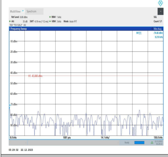
66-66-15MHz-10MHz-QPSK-QPSK-132499-132619-1RB#0- 1RB#49-0.009~0.15MHz-PASS
