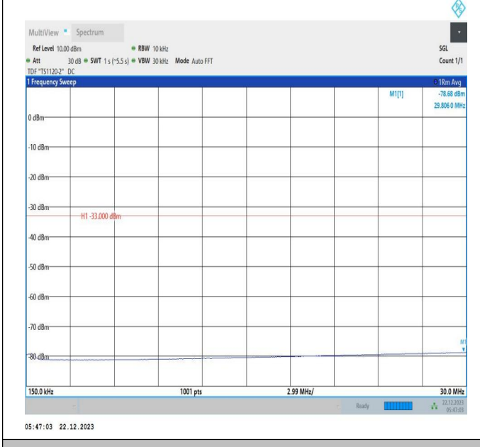
66-66-15MHz-15MHz-16QAM-16QAM-132047-132197-1RB#0-0RB#0-0.15~30MHz-PASS
