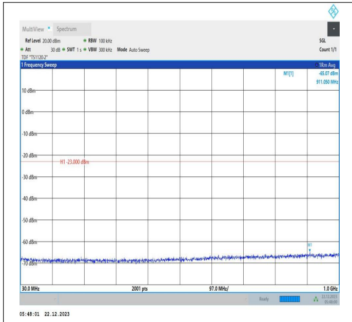
66-66-15MHz-15MHz-64QAM-64QAM-132047-132197-1RB# 0-ORB#0-30~1000MHz-PASS
