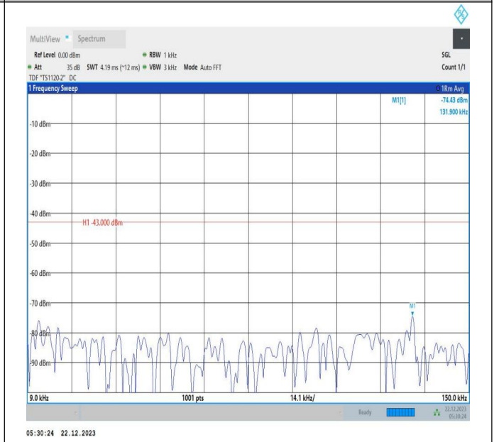
66-66-15MHz-10MHz-16QAM-16QAM-132499-132619-1RB#0-1RB#49-0.009~0.15MHz-PASS
