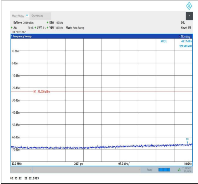
66-66-15MHz-10MHz-16QAM-16QAM-132499-132619-75RB #0-50RB#0-30~1000MHz-PASS
