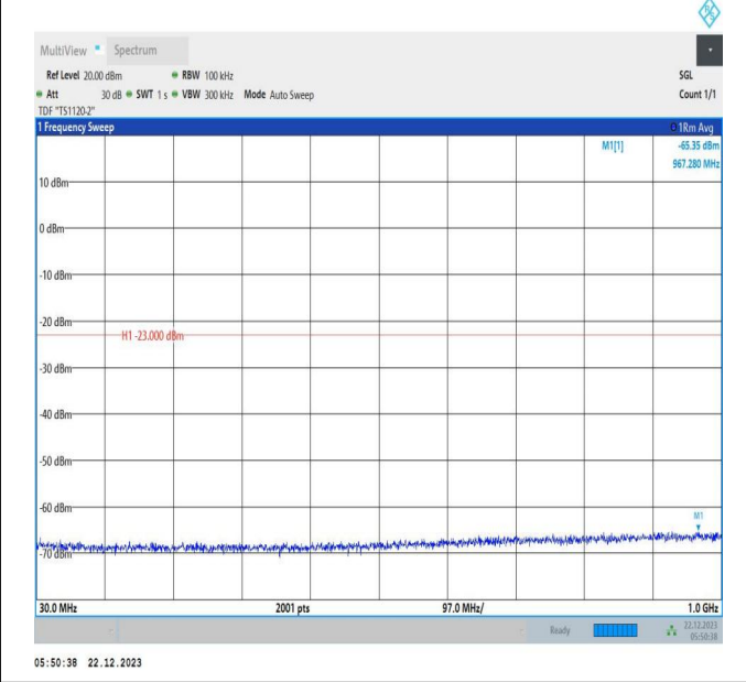
66-66-15MHz-15MHz-64QAM-64QAM-132047-132197-1RB# 74-ORB#0-30~1000MHz-PASS
