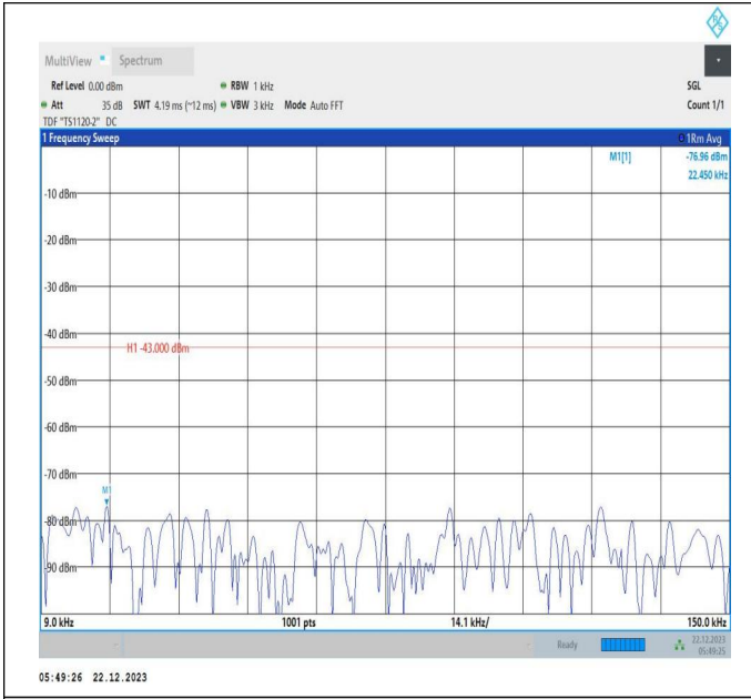
66-66-15MHz-15MHz-16QAM-16QAM-132047-132197-1RB# 74-ORB#0-0.009~0.15MHz-PASS
