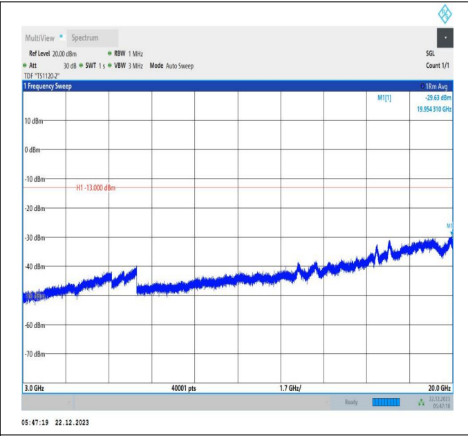
66-66-15MHz-15MHz-16QAM-16QAM-132047-132197-1RB# 0-ORB#0-3000~20000MHz-PASS
