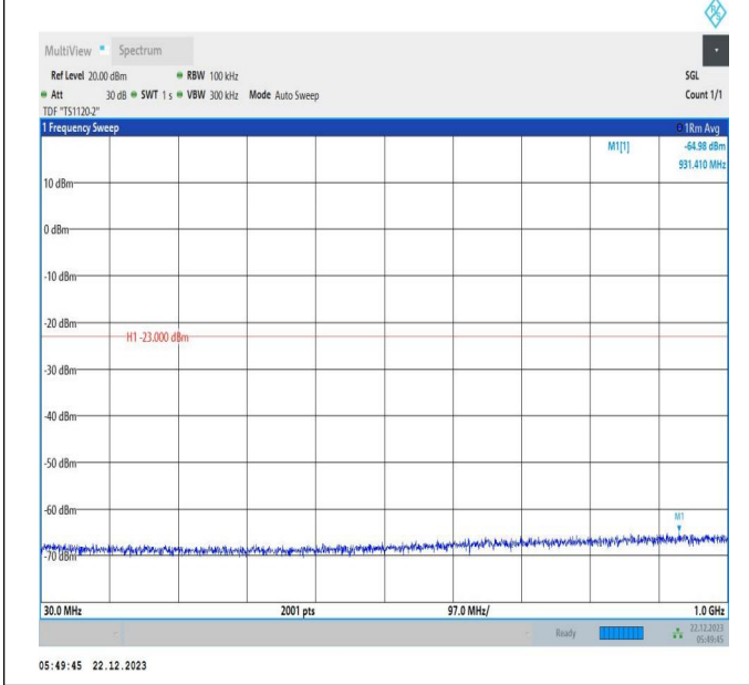
66-66-15MHz-15MHz-16QAM-16QAM-132047-132197-1RB# 74-ORB#0-30~1000MHz-PASS
