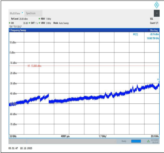
66-66-15MHz-10MHz-64QAM-64QAM-132499-132619-1RB# 0-1RB#49-3000~20000MHz-PASS
