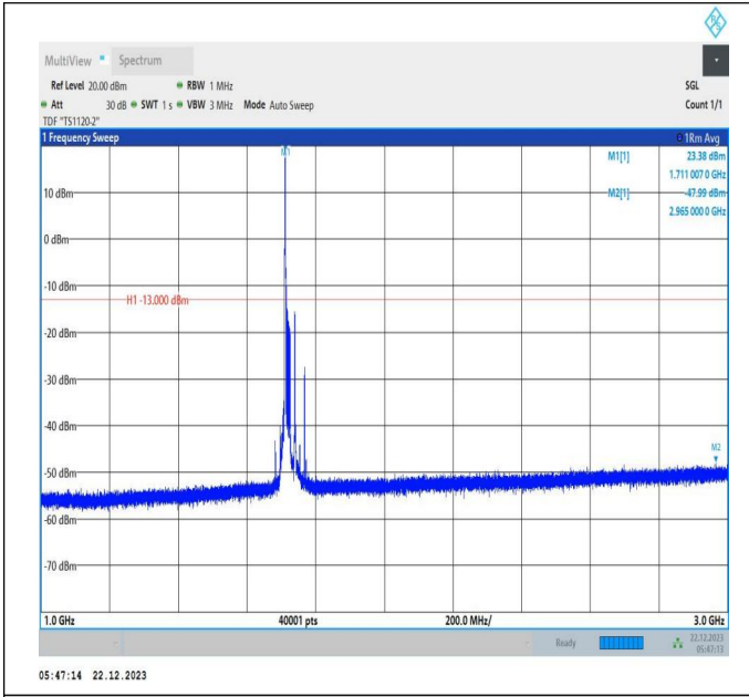
66-66-15MHz-15MHz-16QAM-16QAM-132047-132197-1RB# 0-ORB#0-1000~3000MHz-PASS
