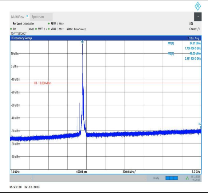
66-66-15MHz-10MHz-64QAM-64QAM-132499-132619-1RB# 0-ORB#0-1000~3000MHz-PASS
