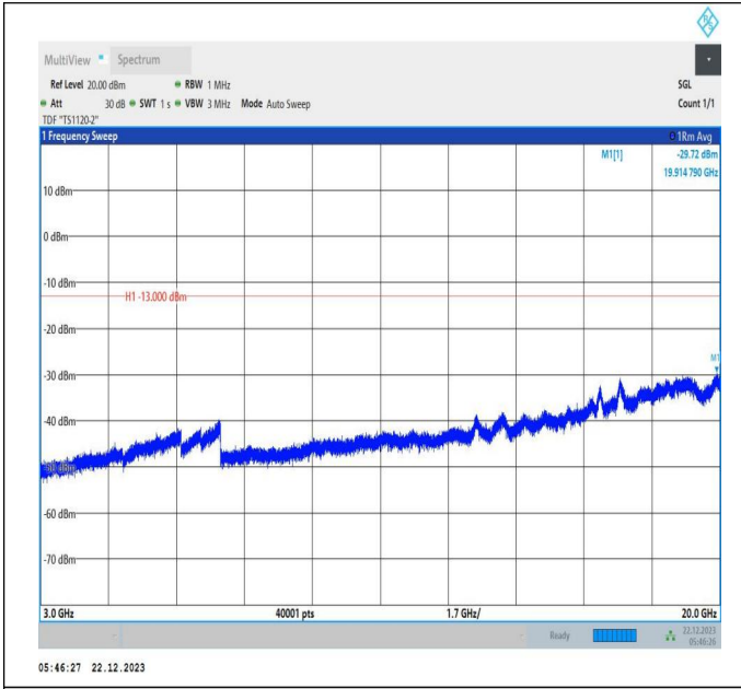
66-66-15MHz-15MHz-QPSK-QPSK-132047-132197-1RB#-0RB#0-3000~20000MHz-PASS
