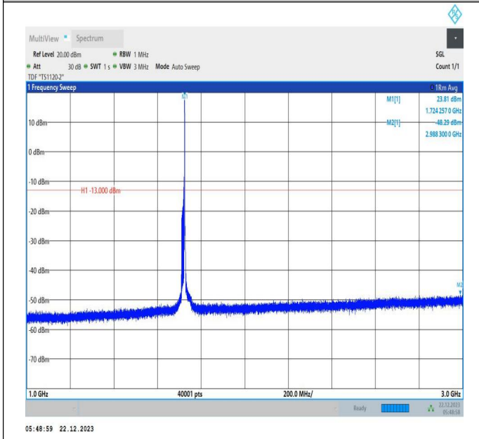
66-66-15MHz-15MHz-QPSK-QPSK-132047-132197-1RB#74 -ORB#0-1000~3000MHz-PASS
