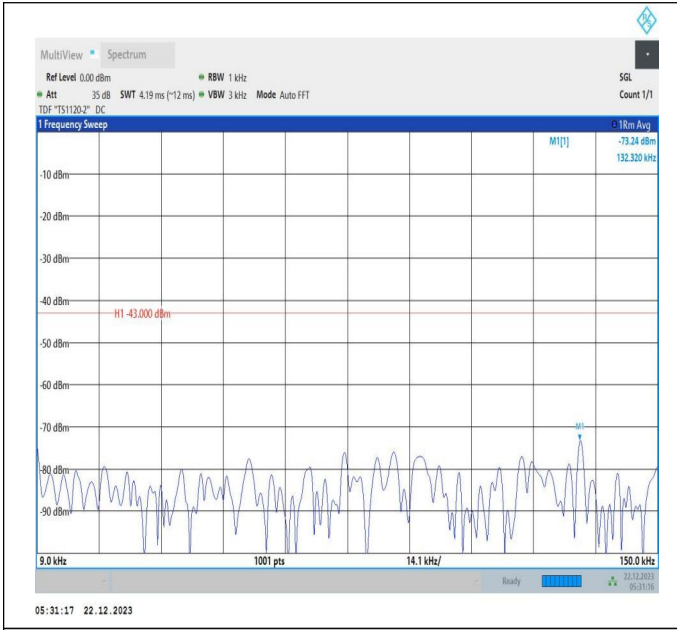
66-66-15MHz-10MHz-64QAM-64QAM-132499-132619-1RB# 0-1RB#49-0.009~0.15MHz-PASS
