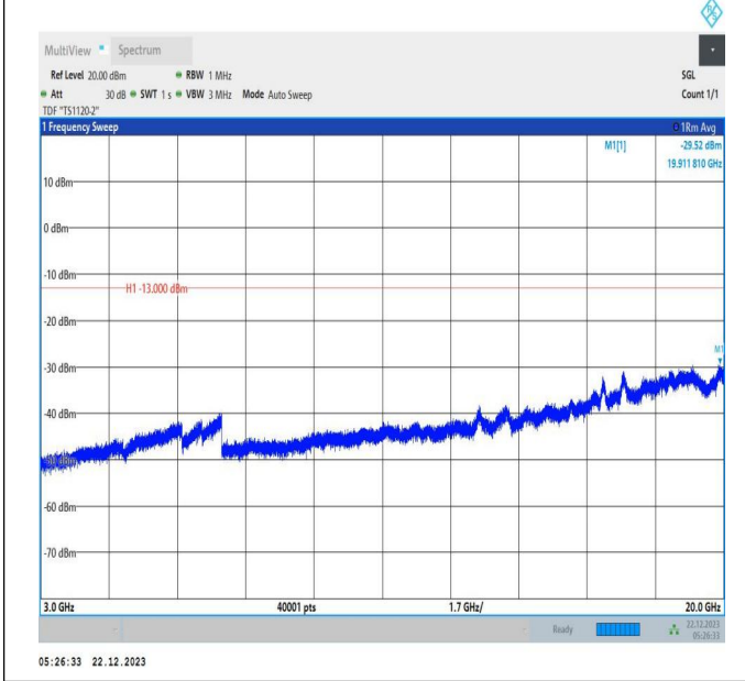
66-66-15MHz-10MHz-64QAM-64QAM-132499-132619-1RB# 0-ORB#0-3000~20000MHz-PASS
