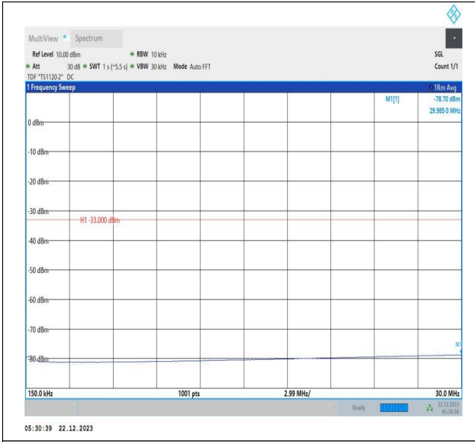
66-66-15MHz-10MHz-16QAM-16QAM-132499-132619-1RB# 0-1RB#49-0.15~30MHz-PASS
