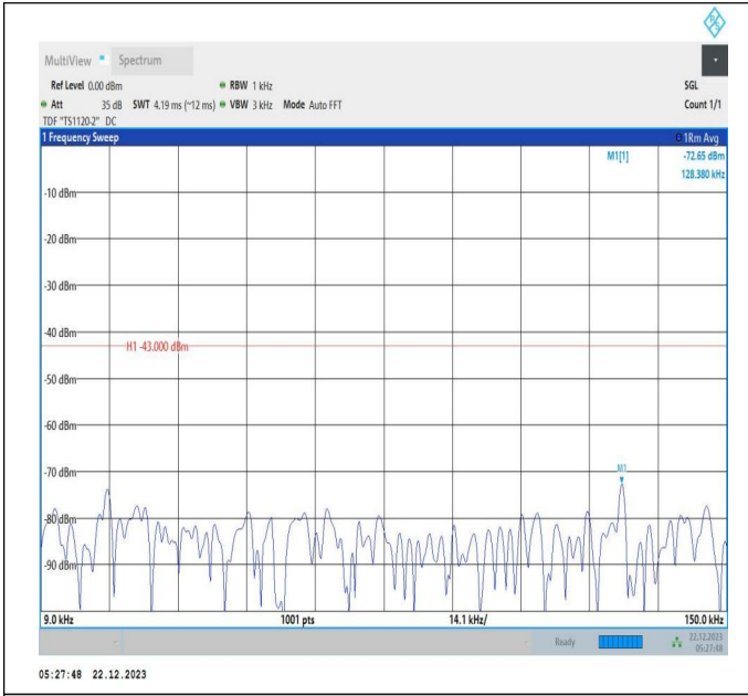
66-66-15MHz-10MHz-16QAM-16QAM-132499-132619-1RB# 74-ORB#0-0.009~0.15MHz-PASS
