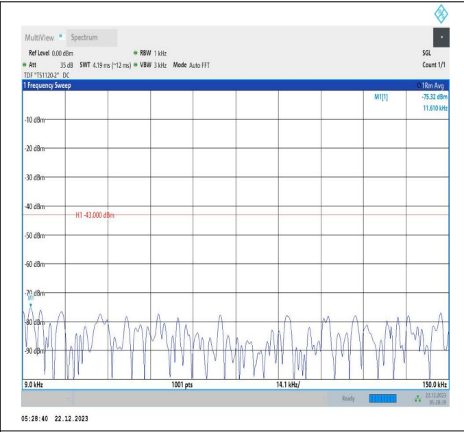
66-66-15MHz-10MHz-64QAM-64QAM-132499-132619-1RB# 74-ORB#0-0.009~0.15MHz-PASS
