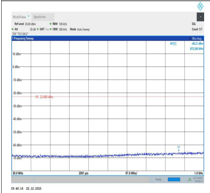
66-66-15MHz-15MHz-QPSK-QPSK-132047-132197-1RB#0-ORB#0-30~1000MHz-PASS
