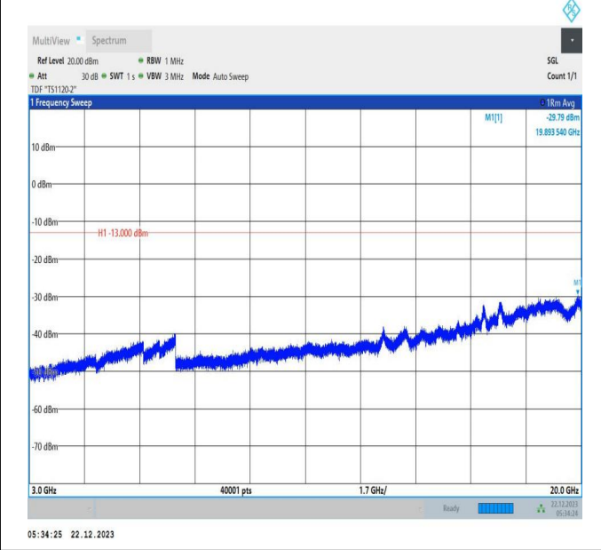
66-66-15MHz-10MHz-64QAM-64QAM-132499-132619-75RB #0-50RB#0-3000~20000MHz-PASS
