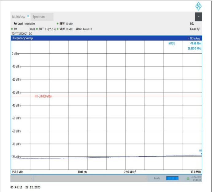
66-66-15MHz-15MHz-QPSK-QPSK-132047-132197-1RB#0-ORB#0-0.15~30MHz-PASS
