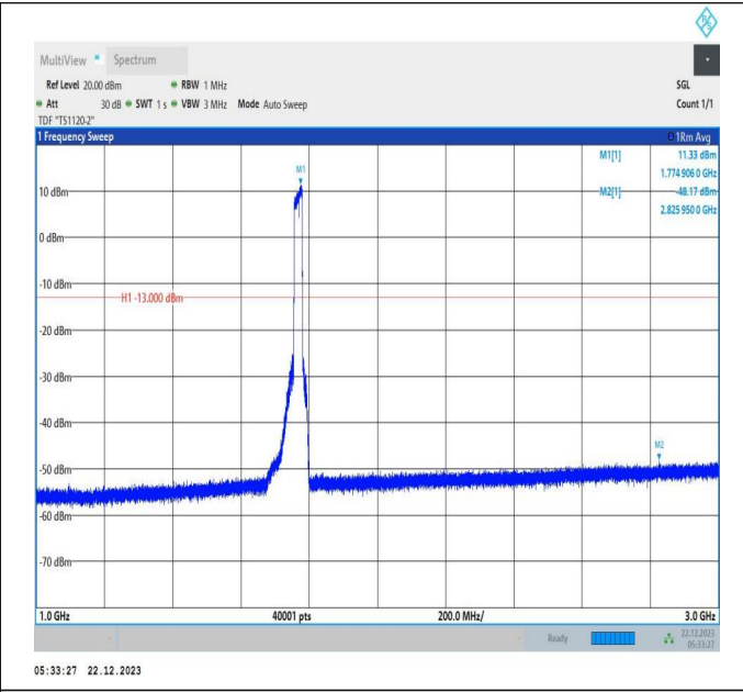
66-66-15MHz-10MHz-16QAM-16QAM-132499-132619-75RB #0-50RB#0-1000~3000MHz-PASS
