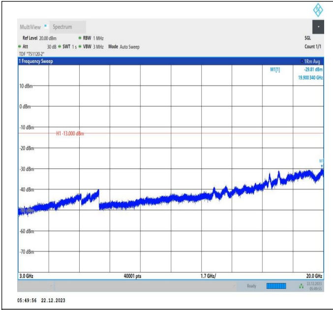
66-66-15MHz-15MHz-16QAM-16QAM-132047-132197-1RB# 74-ORB#0-3000~20000MHz-PASS
