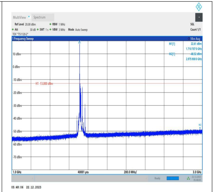
66-66-15MHz-15MHz-64QAM-64QAM-132047-132197-1RB# 0-ORB#0-1000~3000MHz-PASS
