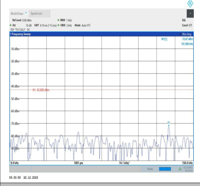
66-66-15MHz-10MHz-64QAM-64QAM-132499-132619-75RB #0-50RB#0-0.009~0.15MHz-PASS
