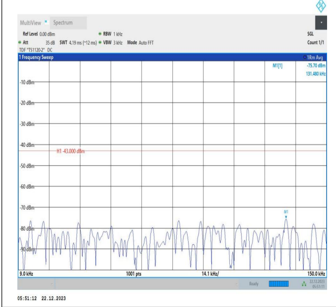
66-66-15MHz-15MHz-QPSK-QPSK-132047-132197-1RB#0- 1RB#74-0.009~0.15MHz-PASS
