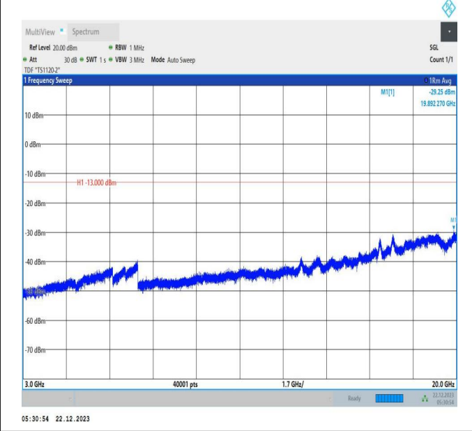
66-66-15MHz-10MHz-16QAM-16QAM-132499-132619-1RB# 0-1RB#49-3000~20000MHz-PASS
