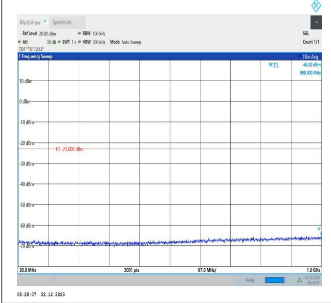
66-66-15MHz-10MHz-16QAM-16QAM-132499-132619-1RB# 74-ORB#0-30~1000MHz-PASS
