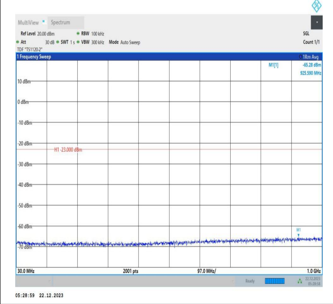
66-66-15MHz-10MHz-64QAM-64QAM-132499-132619-1RB# 74-ORB#0-30~1000MHz-PASS
