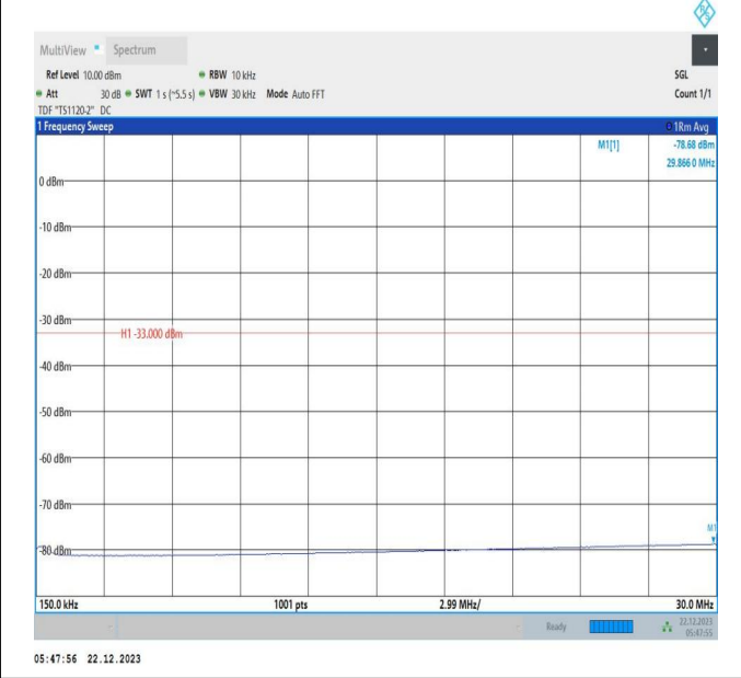
66-66-15MHz-15MHz-64QAM-64QAM-132047-132197-1RB# 0-ORB#0-0.15~30MHz-PASS
