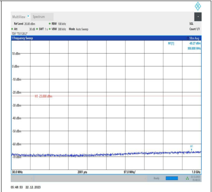
66-66-15MHz-15MHz-QPSK-QPSK-132047-132197-1RB#74 -ORB#0-30~1000MHz-PASS
