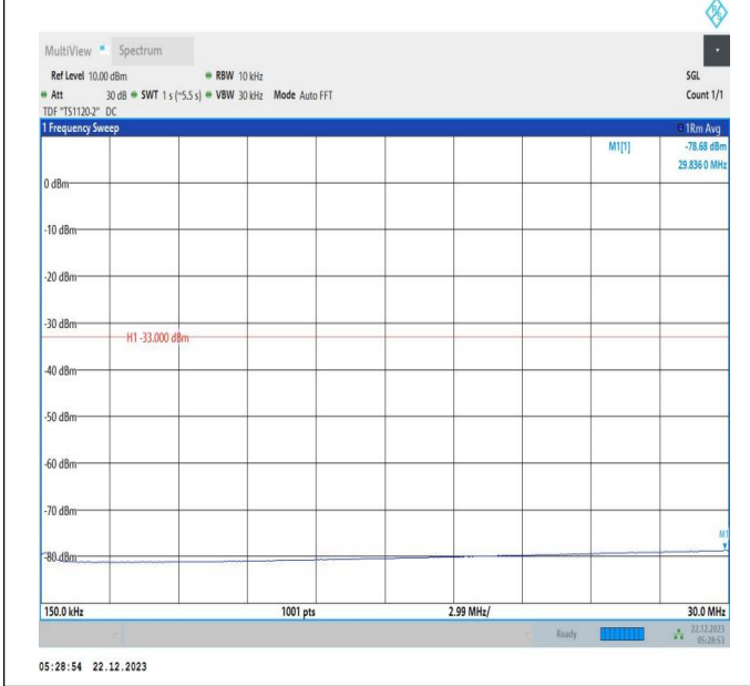
66-66-15MHz-10MHz-64QAM-64QAM-132499-132619-1RB# 74-ORB#0-0.15~30MHz-PASS
