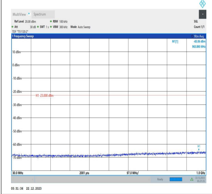
66-66-15MHz-10MHz-64QAM-64QAM-132499-132619-1RB# 0-1RB#49-30~1000MHz-PASS
