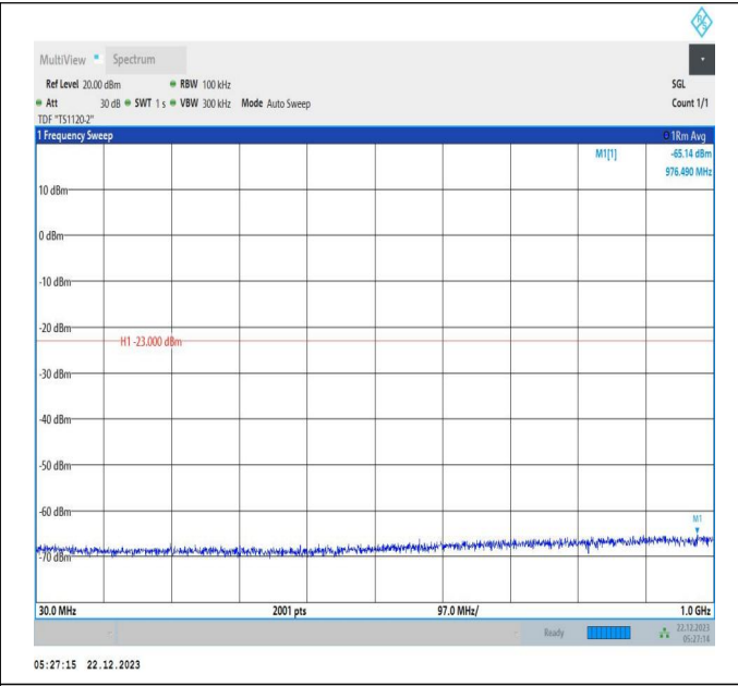
66-66-15MHz-10MHz-QPSK-QPSK-132499-132619-1RB#74 -ORB#0-30~1000MHz-PASS
