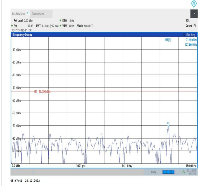
66-66-15MHz-15MHz-64QAM-64QAM-132047-132197-1RB# 0-ORB#0-0.009~0.15MHz-PASS
