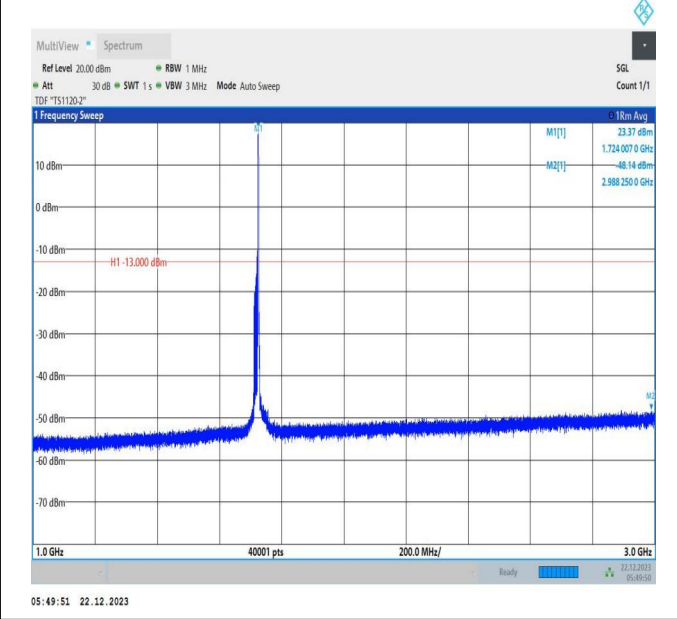
66-66-15MHz-15MHz-16QAM-16QAM-132047-132197-1RB# 74-ORB#0-1000~3000MHz-PASS
