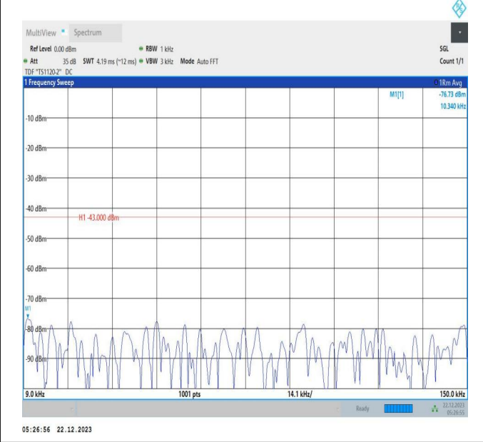
66-66-15MHz-10MHz-QPSK-QPSK-132499-132619-1RB#74 -ORB#0-0.009~0.15MHz-PASS
