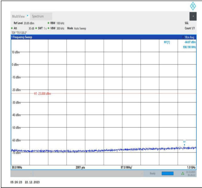
66-66-15MHz-10MHz-64QAM-64QAM-132499-132619-1RB# 0-ORB#0-30~1000MHz-PASS
