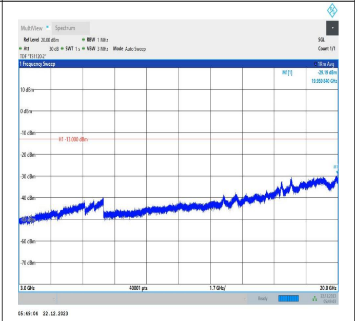
66-66-15MHz-15MHz-QPSK-QPSK-132047-132197-1RB#74 -ORB#0-3000~20000MHz-PASS
