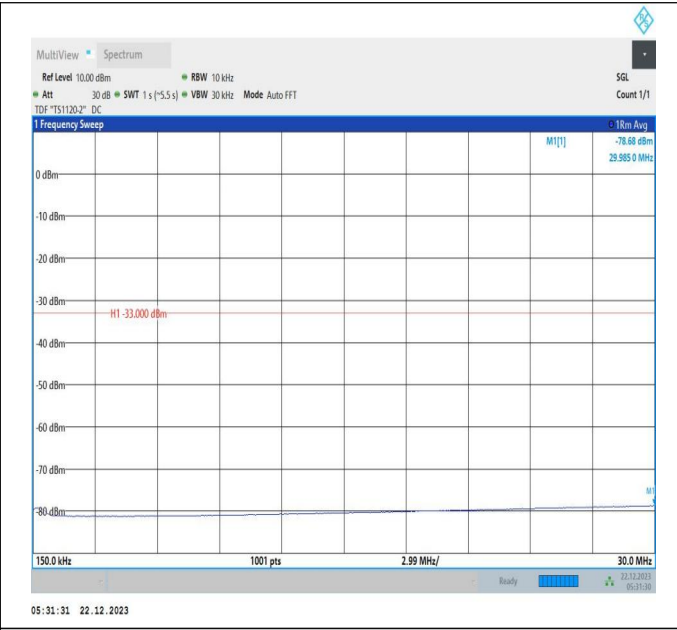
66-66-15MHz-10MHz-64QAM-64QAM-132499-132619-1RB# 0-1RB#49-0.15~30MHz-PASS
