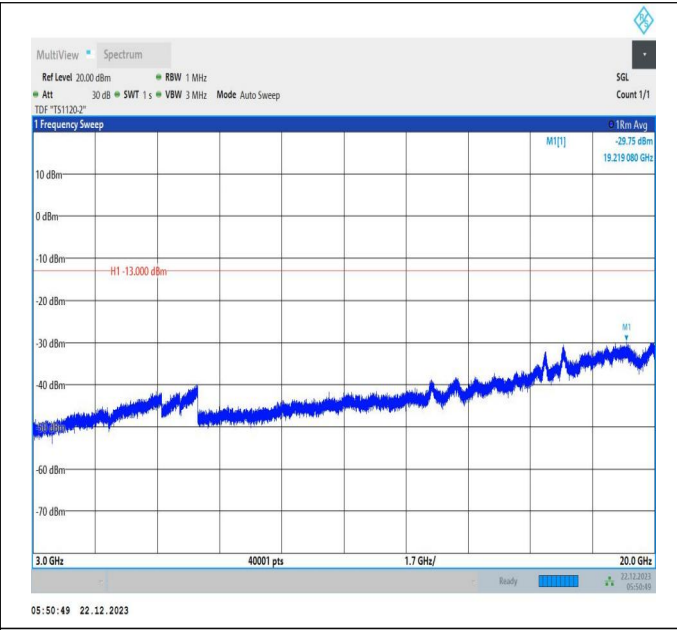
66-66-15MHz-15MHz-64QAM-64QAM-132047-132197-1RB# 74-0RB#0-3000~20000MHz-PASS
