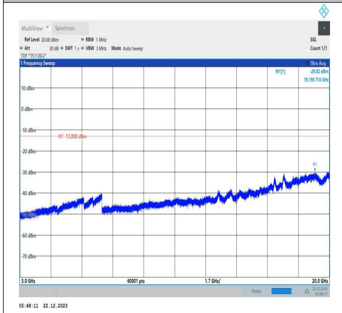
66-66-15MHz-15MHz-64QAM-64QAM-132047-132197-1RB# 0-ORB#0-3000~20000MHz-PASS
