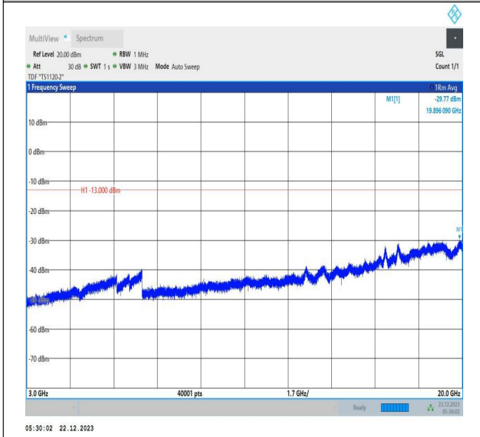
66-66-15MHz-10MHz-QPSK-QPSK-132499-132619-1RB#0-1RB#49-3000~20000MHz-PASS
