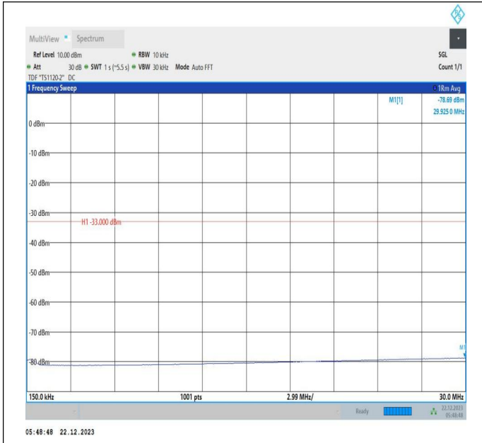
66-66-15MHz-15MHz-QPSK-QPSK-132047-132197-1RB#74 -ORB#0-0.15~30MHz-PASS
