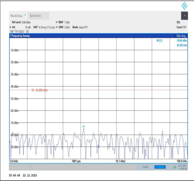
66-66-15MHz-15MHz-16QAM-16QAM-132047-132197-1RB#0-0RB#0-0.009~0.15MHz-PASS
