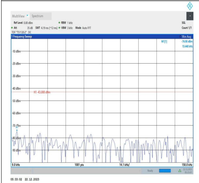
66-66-15MHz-10MHz-16QAM-16QAM-132499-132619-75RB #0-50RB#0-0.009~0.15MHz-PASS
