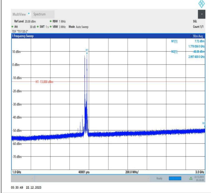
66-66-15MHz-10MHz-16QAM-16QAM-132499-132619-1RB# 0-1RB#49-1000~3000MHz-PASS
