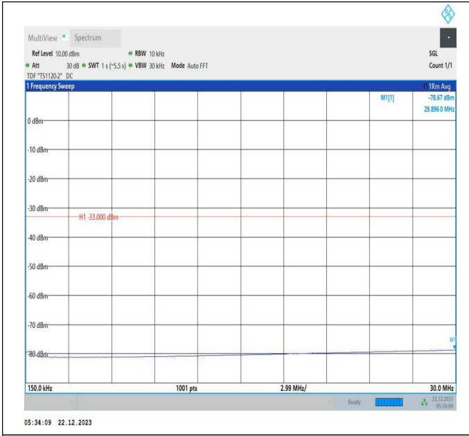
66-66-15MHz-10MHz-64QAM-64QAM-132499-132619-75RB #0-50RB#0-0.15~30MHz-PASS
