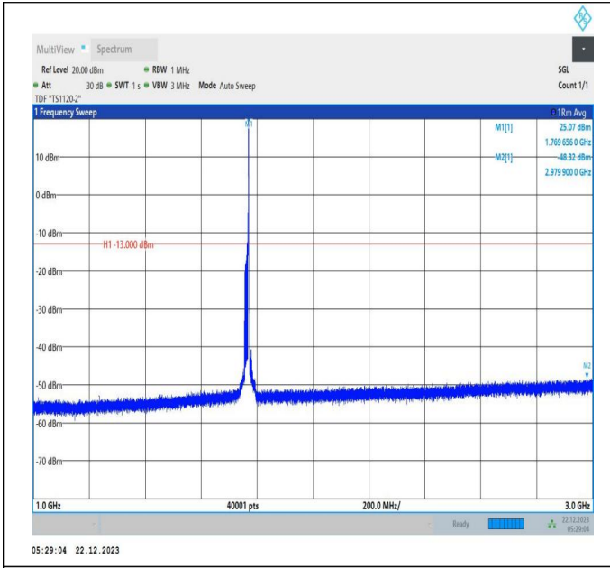
66-66-15MHz-10MHz-64QAM-64QAM-132499-132619-1RB# 74-ORB#0-1000~3000MHz-PASS
