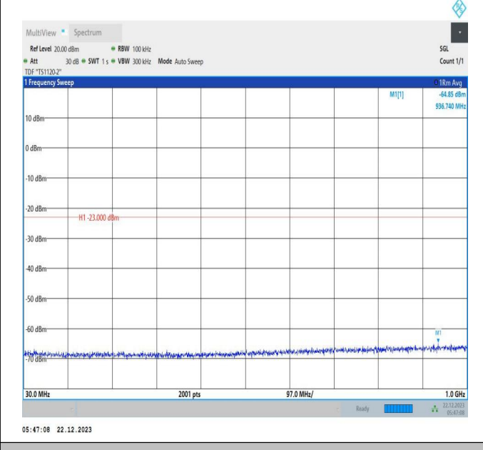
66-66-15MHz-15MHz-16QAM-16QAM-132047-132197-1RB#0-0RB#0-30~1000MHz-PASS
