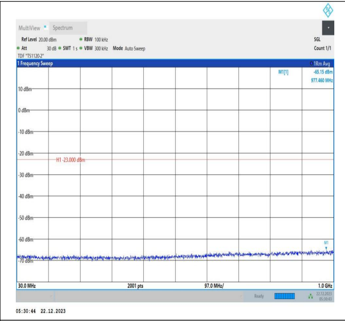
66-66-15MHz-10MHz-16QAM-16QAM-132499-132619-1RB# 0-1RB#49-30~1000MHz-PASS
