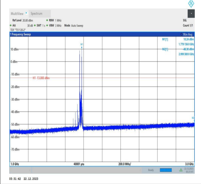
66-66-15MHz-10MHz-64QAM-64QAM-132499-132619-1RB# 0-1RB#49-1000~3000MHz-PASS
