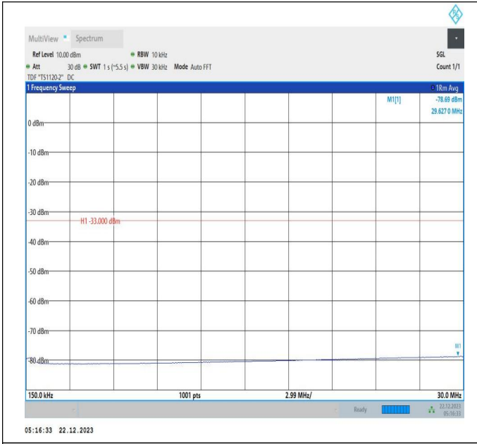
66-66-15MHz-10MHz-QPSK-QPSK-132373-132493-1RB#74 -ORB#0-0.15~30MHz-PASS
