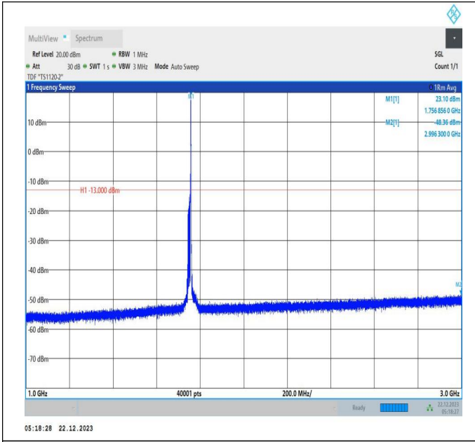
66-66-15MHz-10MHz-64QAM-64QAM-132373-132493-1RB# 74-0RB#0-1000~3000MHz-PASS
