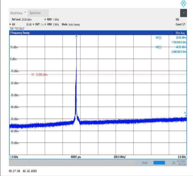
66-66-15MHz-10MHz-16QAM-16QAM-132373-132493-1RB# 74-ORB#0-1000~3000MHz-PASS
