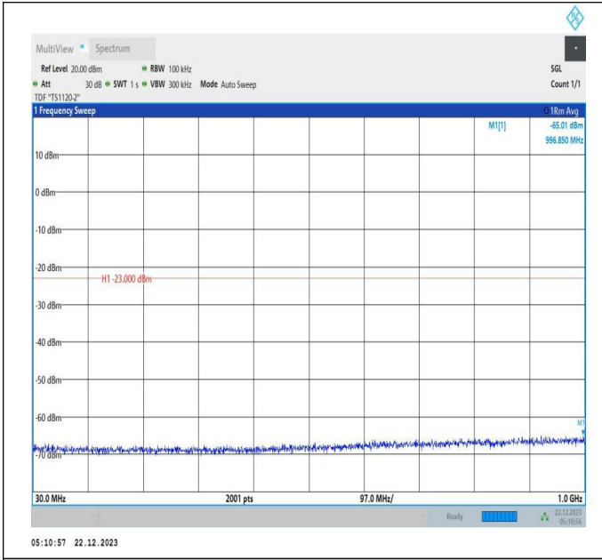
66-66-15MHz-10MHz-16QAM-16QAM-132047-132167-75RB #0-50RB#0-30~1000MHz-PASS
