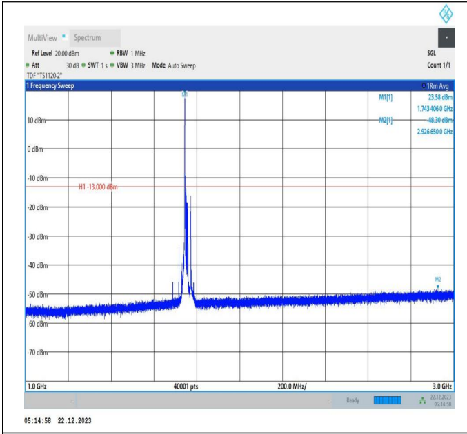
66-66-15MHz-10MHz-16QAM-16QAM-132373-132493-1RB# 0-ORB#0-1000~3000MHz-PASS
