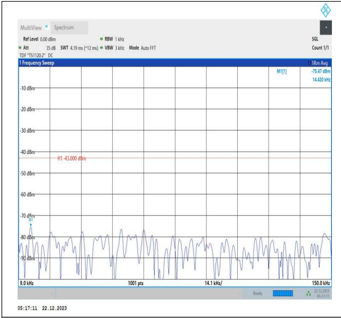
66-66-15MHz-10MHz-16QAM-16QAM-132373-132493-1RB# 74-ORB#0-0.009~0.15MHz-PASS
