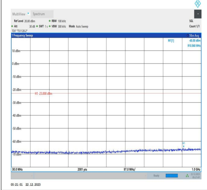
66-66-15MHz-10MHz-64QAM-64QAM-132373-132493-1RB# 0-1RB#49-30~1000MHz-PASS
