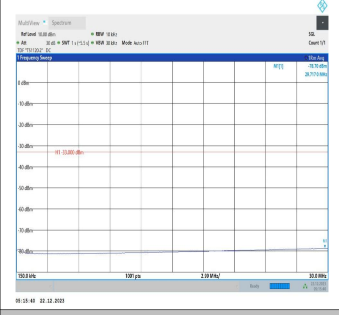
66-66-15MHz-10MHz-64QAM-64QAM-132373-132493-1RB# 0-ORB#0-0.15~30MHz-PASS
