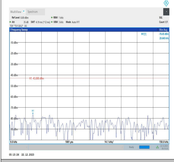
66-66-15MHz-10MHz-64QAM-64QAM-132373-132493-1RB# 0-ORB#0-0.009~0.15MHz-PASS
