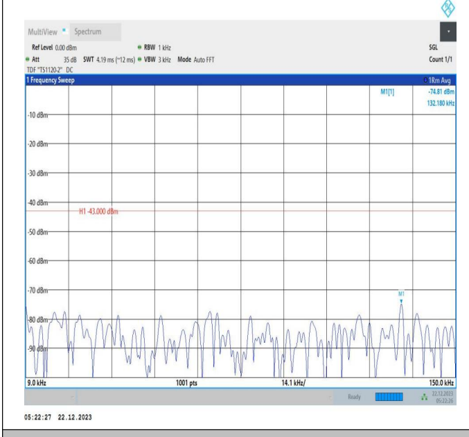
66-66-15MHz-10MHz-16QAM-16QAM-132373-132493-75RB #0-50RB#0-0.009~0.15MHz-PASS
