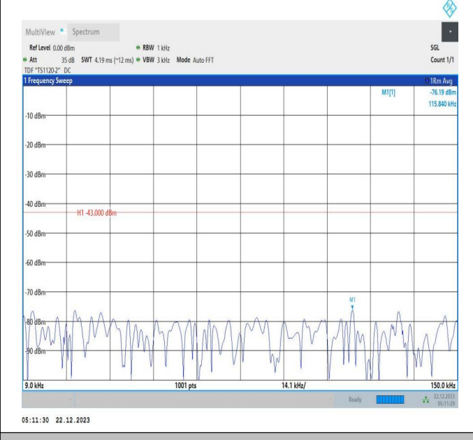
66-66-15MHz-10MHz-64QAM-64QAM-132047-132167-75RB #0-50RB#0-0.009~0.15MHz-PASS
