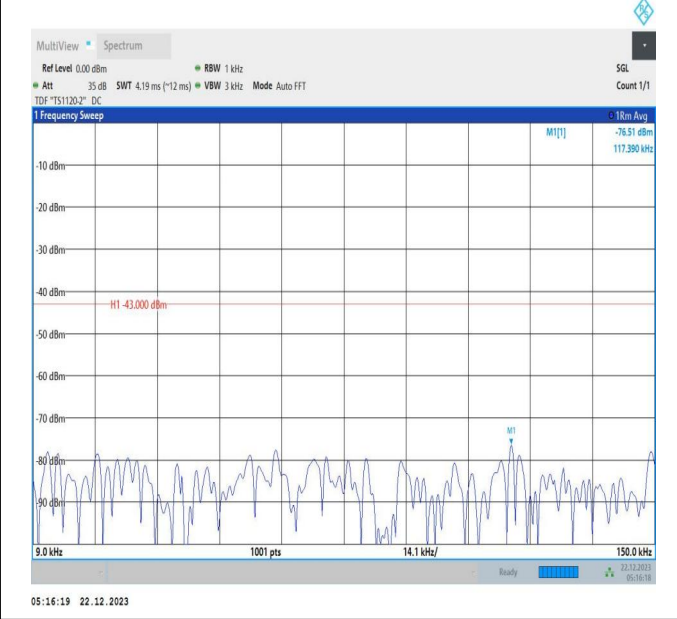
66-66-15MHz-10MHz-QPSK-QPSK-132373-132493-1RB#74 -ORB#0-0.009~0.15MHz-PASS
