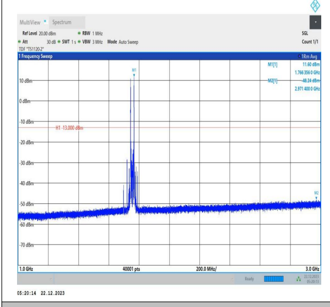
66-66-15MHz-10MHz-16QAM-16QAM-132373-132493-1RB# 0-1RB#49-1000~3000MHz-PASS
