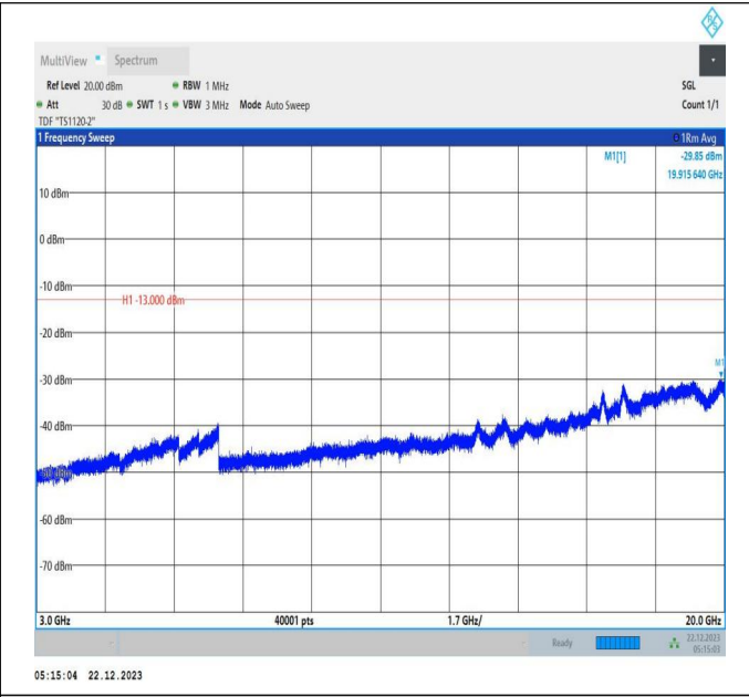
66-66-15MHz-10MHz-16QAM-16QAM-132373-132493-1RB# 0-ORB#0-3000~20000MHz-PASS
