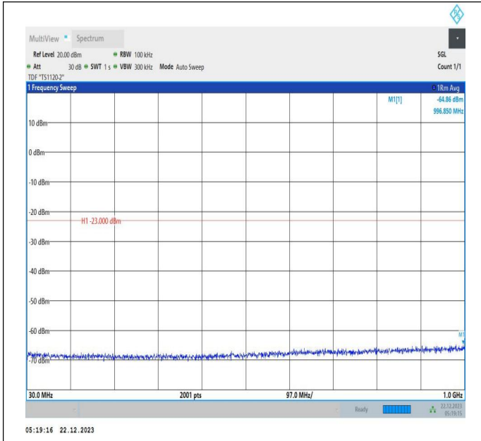
66-66-15MHz-10MHz-QPSK-QPSK-132373-132493-1RB#0-1RB#49-30~1000MHz-PASS
