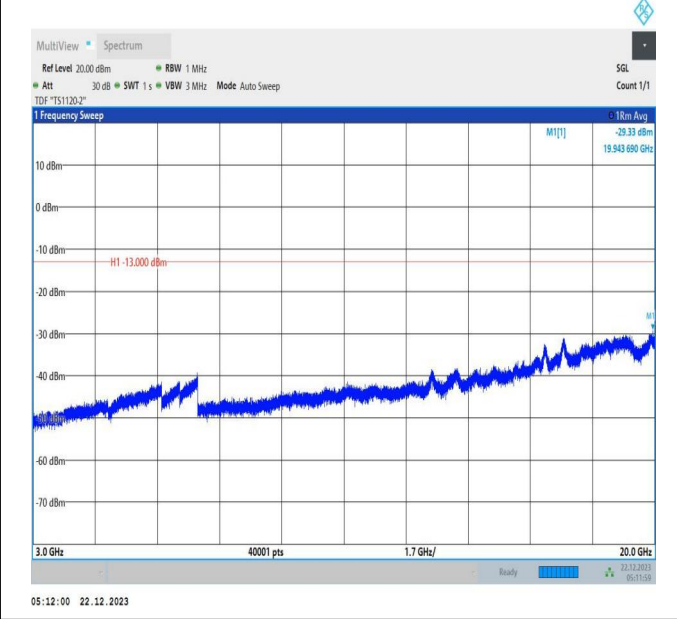
66-66-15MHz-10MHz-64QAM-64QAM-132047-132167-75RB #0-50RB#0-3000~20000MHz-PASS
