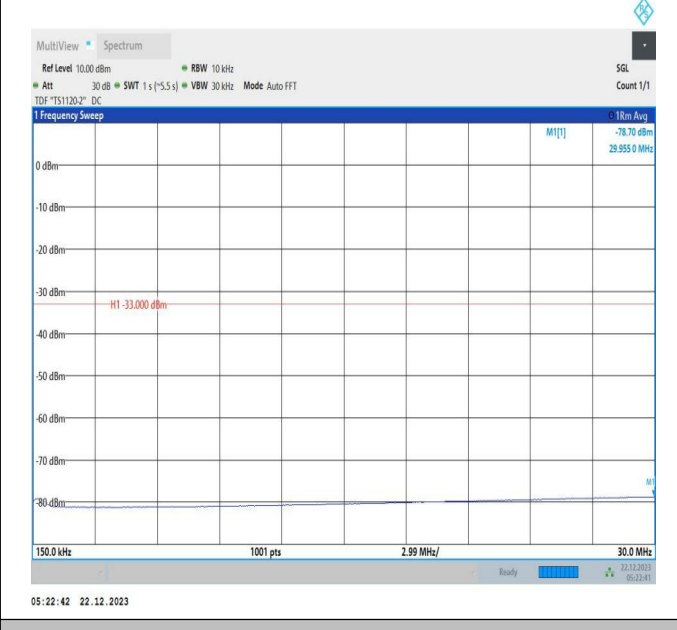
66-66-15MHz-10MHz-16QAM-16QAM-132373-132493-75RB #0-50RB#0-0.15~30MHz-PASS
