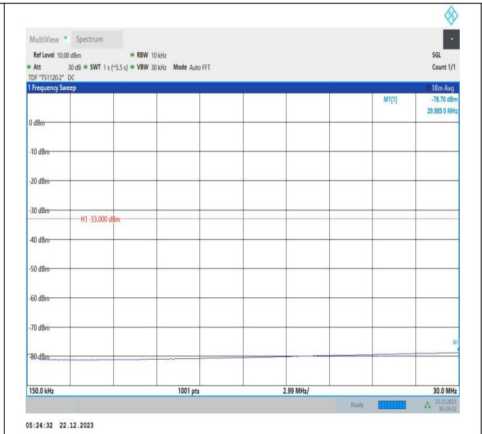
66-66-15MHz-10MHz-QPSK-QPSK-132499-132619-1RB#0-ORB#0-0.15~30MHz-PASS
