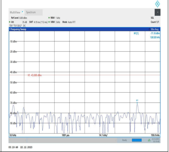
66-66-15MHz-10MHz-16QAM-16QAM-132373-132493-1RB#0-1RB#49-0.009~0.15MHz-PASS
