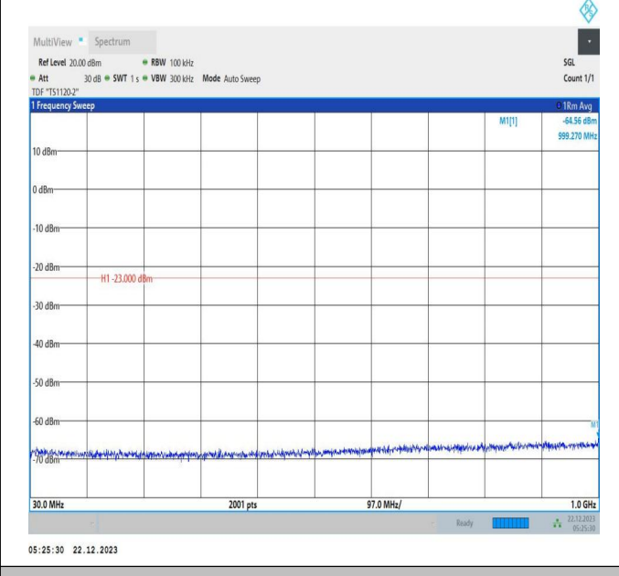
66-66-15MHz-10MHz-16QAM-16QAM-132499-132619-1RB#0-ORB#0-30~1000MHz-PASS
