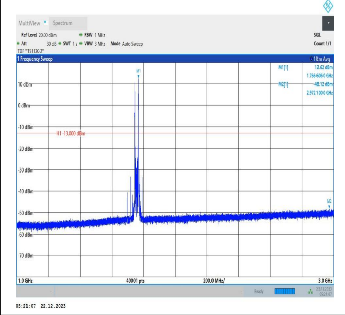
66-66-15MHz-10MHz-64QAM-64QAM-132373-132493-1RB# 0-1RB#49-1000~3000MHz-PASS
