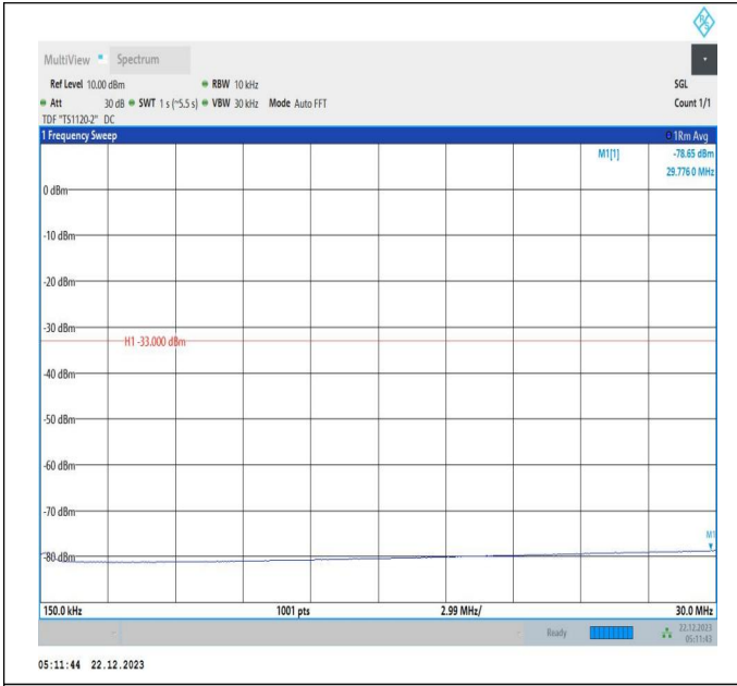
66-66-15MHz-10MHz-64QAM-64QAM-132047-132167-75RB #0-50RB#0-0.15~30MHz-PASS
