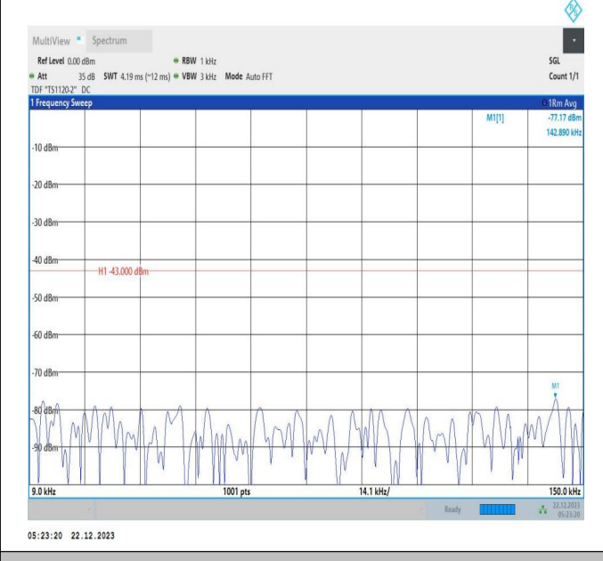
66-66-15MHz-10MHz-64QAM-64QAM-132373-132493-75RB #0-50RB#0-0.009~0.15MHz-PASS
