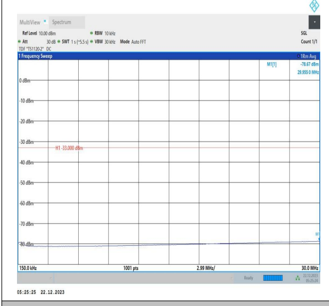
66-66-15MHz-10MHz-16QAM-16QAM-132499-132619-1RB#0-ORB#0-0.15~30MHz-PASS
