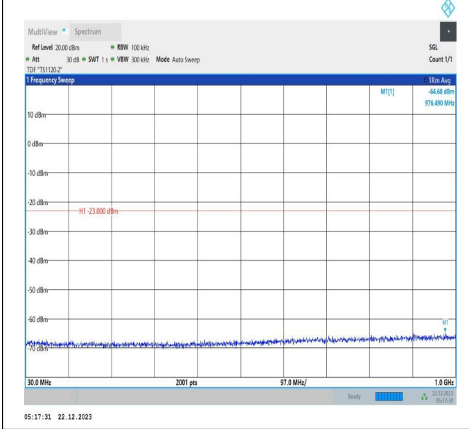
66-66-15MHz-10MHz-16QAM-16QAM-132373-132493-1RB# 74-ORB#0-30~1000MHz-PASS
