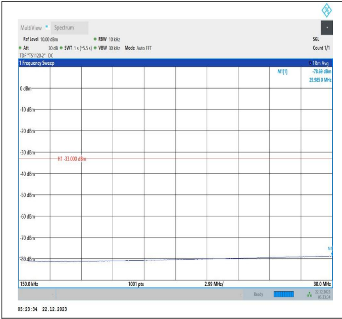
66-66-15MHz-10MHz-64QAM-64QAM-132373-132493-75RB #0-50RB#0-0.15~30MHz-PASS
