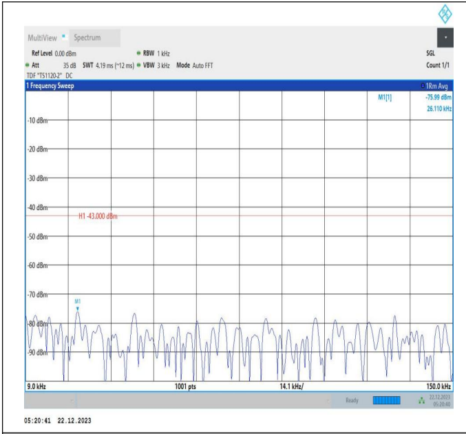
66-66-15MHz-10MHz-64QAM-64QAM-132373-132493-1RB# 0-1RB#49-0.009~0.15MHz-PASS
