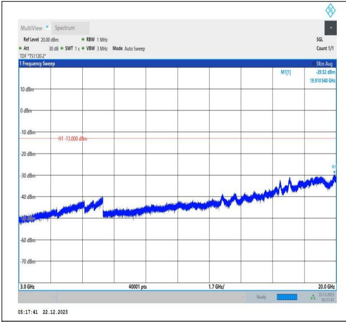
66-66-15MHz-10MHz-16QAM-16QAM-132373-132493-1RB# 74-ORB#0-3000~20000MHz-PASS
