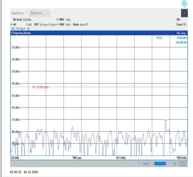
66-66-15MHz-10MHz-64QAM-64QAM-132499-132619-1RB# 0-ORB#0-0.009~0.15MHz-PASS
