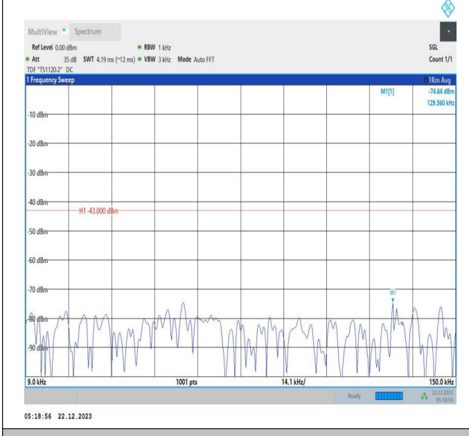
66-66-15MHz-10MHz-QPSK-QPSK-132373-132493-1RB#0- 1RB#49-0.009~0.15MHz-PASS
