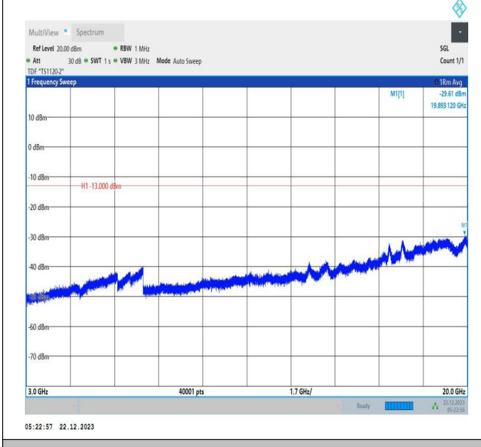
66-66-15MHz-10MHz-16QAM-16QAM-132373-132493-75RB #0-50RB#0-3000~20000MHz-PASS
