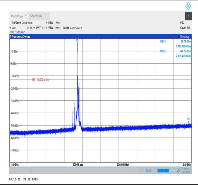
66-66-15MHz-10MHz-64QAM-64QAM-132373-132493-1RB# 0-ORB#0-1000~3000MHz-PASS
