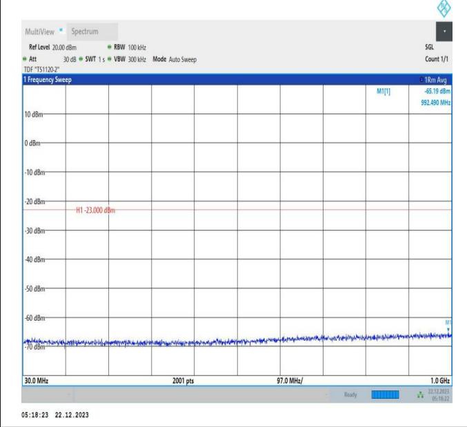
66-66-15MHz-10MHz-64QAM-64QAM-132373-132493-1RB# 74-ORB#0-30~1000MHz-PASS
