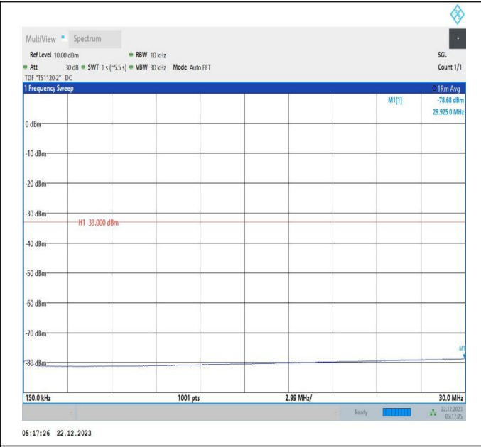
66-66-15MHz-10MHz-16QAM-16QAM-132373-132493-1RB# 74-ORB#0-0.15~30MHz-PASS
