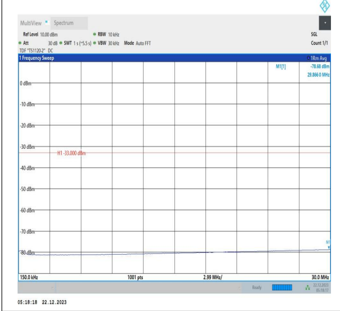
66-66-15MHz-10MHz-64QAM-64QAM-132373-132493-1RB# 74-ORB#0-0.15~30MHz-PASS
