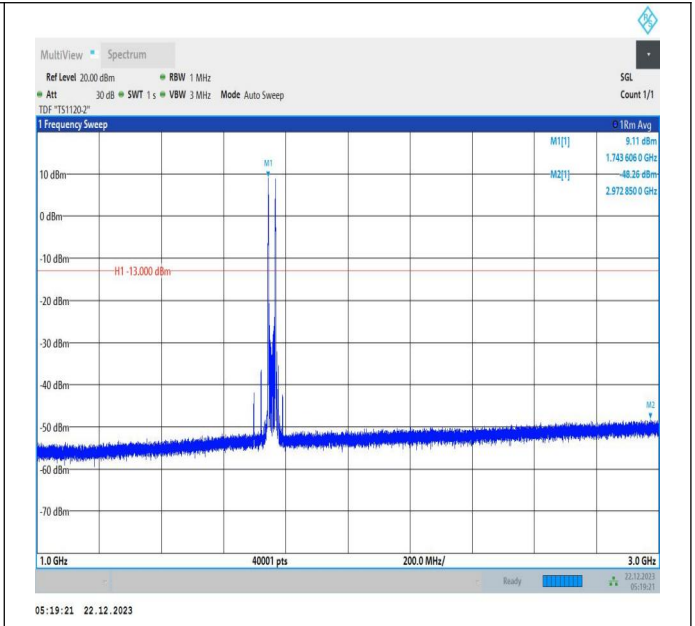
66-66-15MHz-10MHz-QPSK-QPSK-132373-132493-1RB#0-1RB#49-1000~3000MHz-PASS
