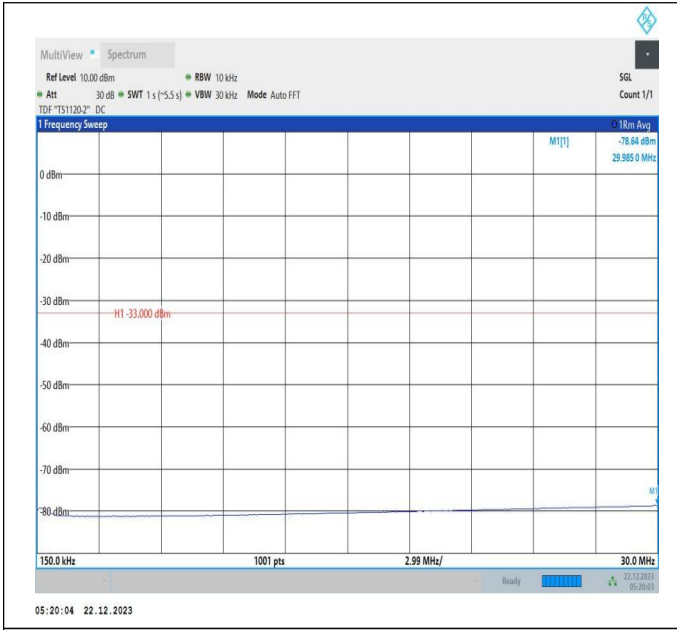
66-66-15MHz-10MHz-16QAM-16QAM-132373-132493-1RB# 0-1RB#49-0.15~30MHz-PASS
