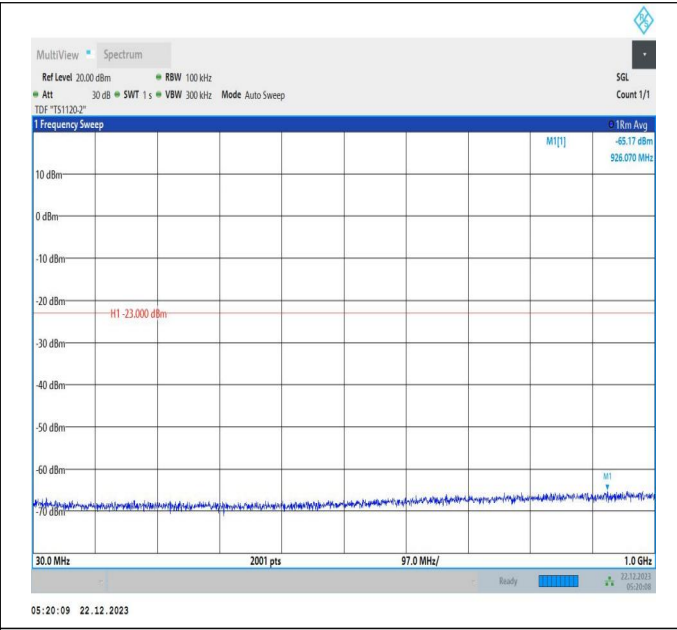
66-66-15MHz-10MHz-16QAM-16QAM-132373-132493-1RB# 0-1RB#49-30~1000MHz-PASS
