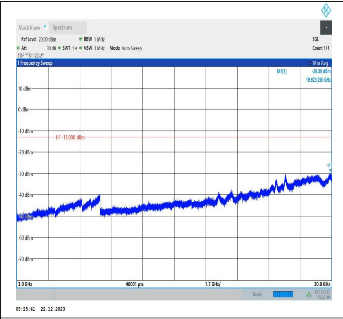
66-66-15MHz-10MHz-16QAM-16QAM-132499-132619-1RB# 0-ORB#0-3000~20000MHz-PASS
