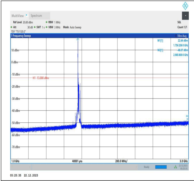
66-66-15MHz-10MHz-16QAM-16QAM-132499-132619-1RB# 0-ORB#0-1000~3000MHz-PASS
