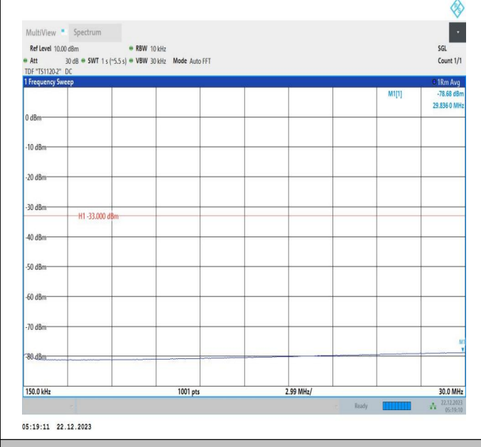
66-66-15MHz-10MHz-QPSK-QPSK-132373-132493-1RB#0- 1RB#49-0.15~30MHz-PASS
