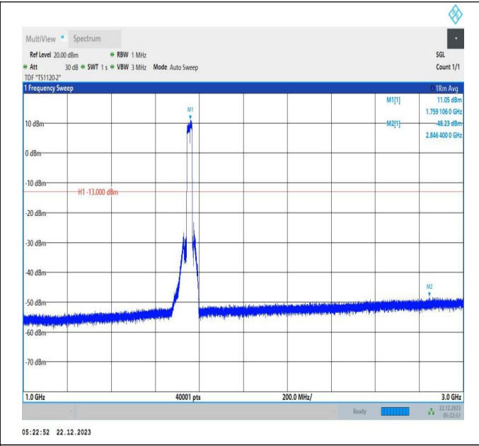
66-66-15MHz-10MHz-16QAM-16QAM-132373-132493-75RB #0-50RB#0-1000~3000MHz-PASS
