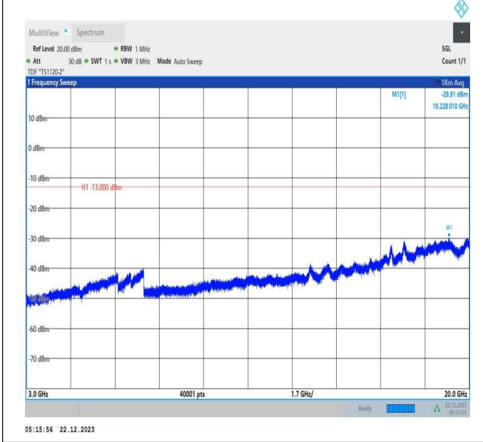
66-66-15MHz-10MHz-64QAM-64QAM-132373-132493-1RB# 0-ORB#0-3000~20000MHz-PASS
