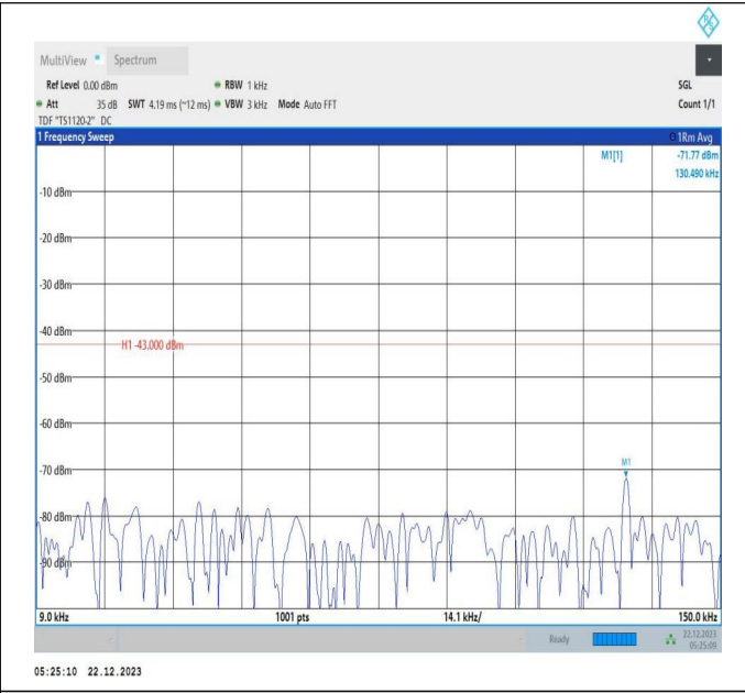
66-66-15MHz-10MHz-16QAM-16QAM-132499-132619-1RB#0-ORB#0-0.009~0.15MHz-PASS
