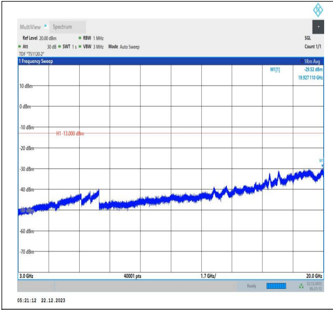
66-66-15MHz-10MHz-64QAM-64QAM-132373-132493-1RB#0-1RB#49-3000~20000MHz-PASS
