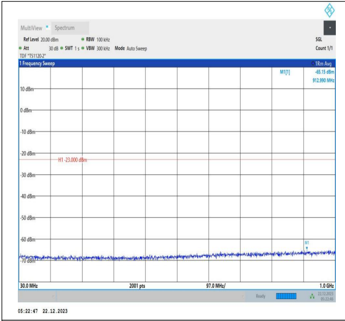
66-66-15MHz-10MHz-16QAM-16QAM-132373-132493-75RB #0-50RB#0-30~1000MHz-PASS
