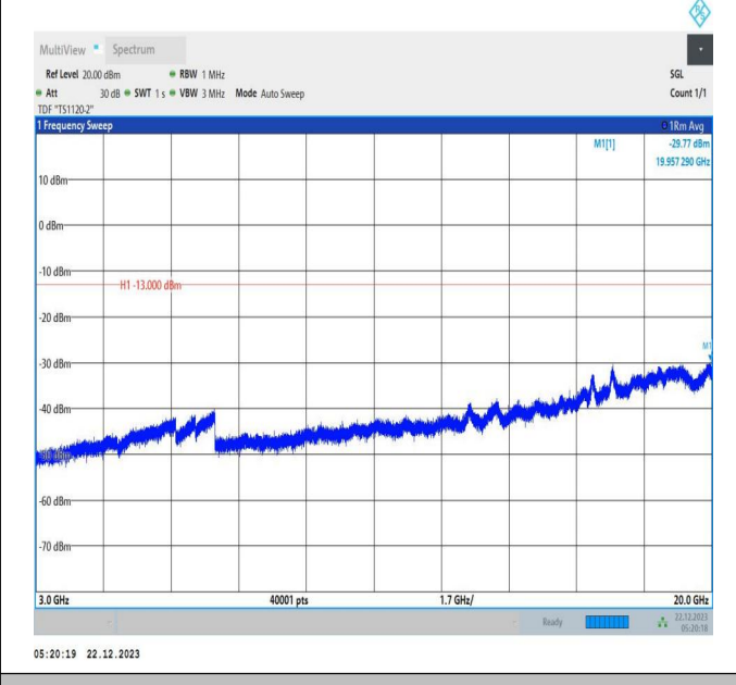
66-66-15MHz-10MHz-16QAM-16QAM-132373-132493-1RB# 0-1RB#49-3000~20000MHz-PASS
