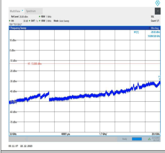
66-66-15MHz-10MHz-16QAM-16QAM-132047-132167-75RB #0-50RB#0-3000~20000MHz-PASS
