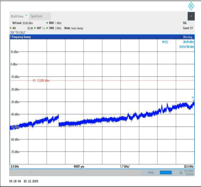
66-66-15MHz-10MHz-64QAM-64QAM-132373-132493-1RB# 74-0RB#0-3000~20000MHz-PASS
