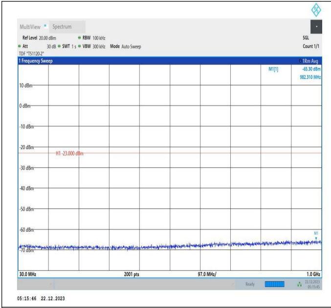
66-66-15MHz-10MHz-64QAM-64QAM-132373-132493-1RB# 0-ORB#0-30~1000MHz-PASS
