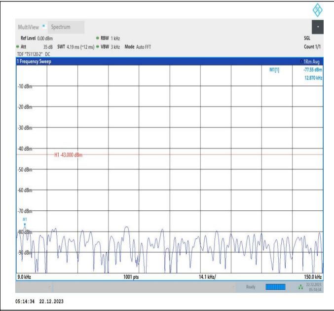
66-66-15MHz-10MHz-16QAM-16QAM-132373-132493-1RB#0-ORB#0-0.009~0.15MHz-PASS
