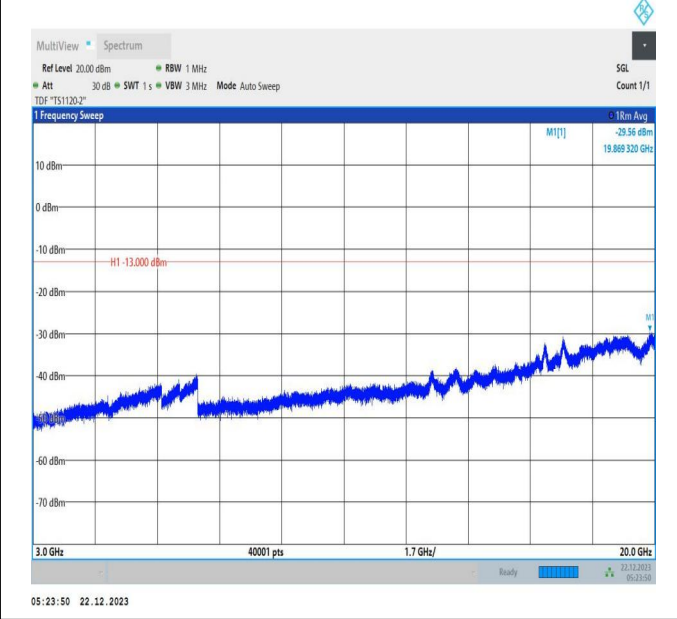
66-66-15MHz-10MHz-64QAM-64QAM-132373-132493-75RB #0-50RB#0-3000~20000MHz-PASS
