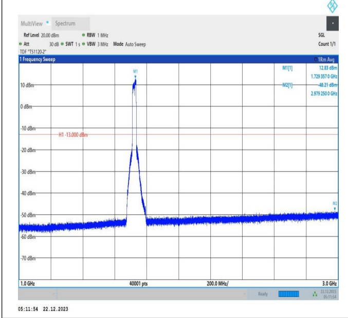
66-66-15MHz-10MHz-64QAM-64QAM-132047-132167-75RB #0-50RB#0-1000~3000MHz-PASS
