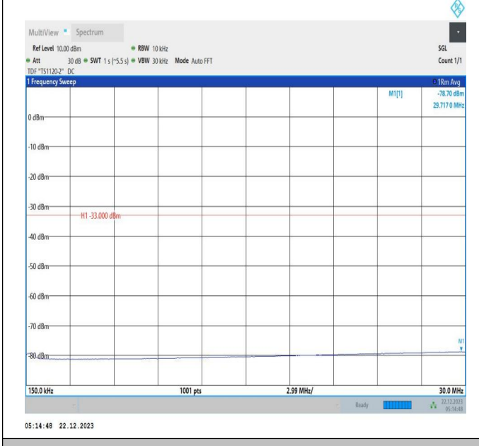
66-66-15MHz-10MHz-16QAM-16QAM-132373-132493-1RB#0-ORB#0-0.15~30MHz-PASS
