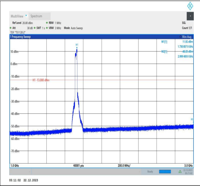
66-66-15MHz-10MHz-16QAM-16QAM-132047-132167-75RB #0-50RB#0-1000~3000MHz-PASS
