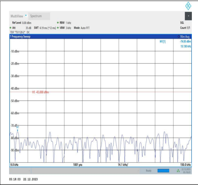
66-66-15MHz-10MHz-64QAM-64QAM-132373-132493-1RB# 74-ORB#0-0.009~0.15MHz-PASS
