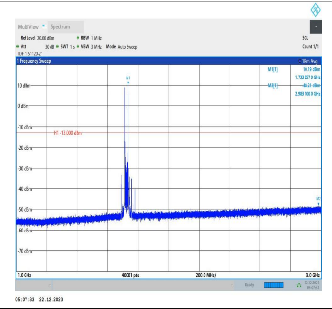
66-66-15MHz-10MHz-QPSK-QPSK-132047-132167-1RB#0-1RB#49-1000~3000MHz-PASS
