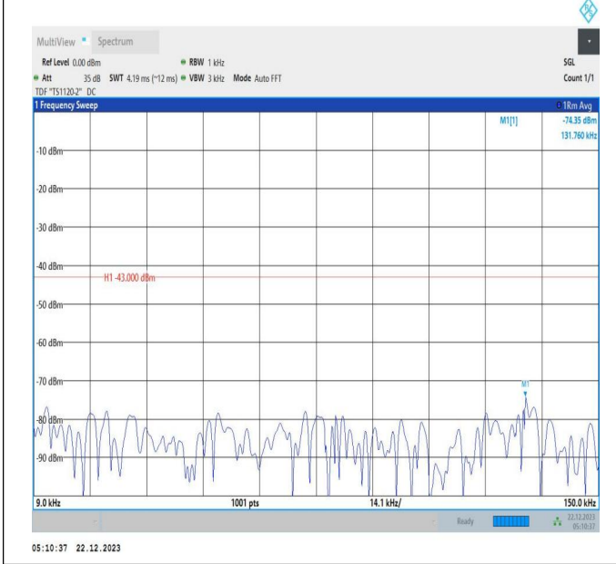
66-66-15MHz-10MHz-16QAM-16QAM-132047-132167-75RB #0-50RB#0-0.009~0.15MHz-PASS
