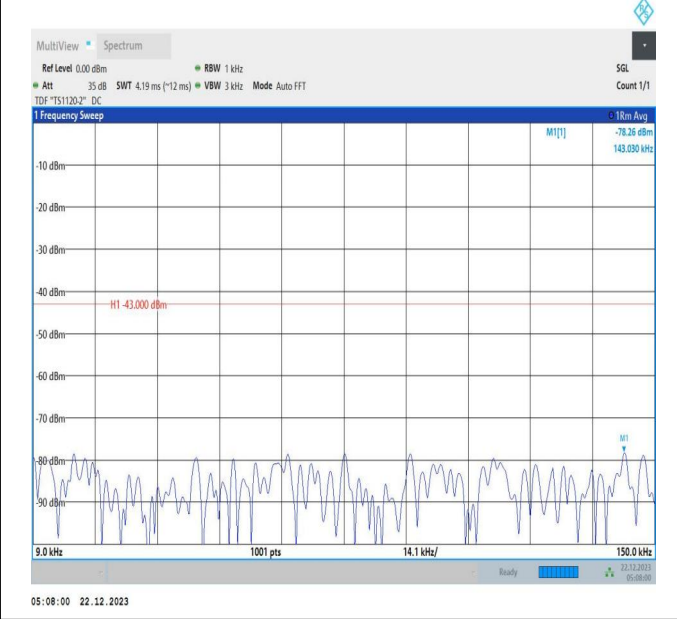
66-66-15MHz-10MHz-16QAM-16QAM-132047-132167-1RB#0-1RB#49-0.009~0.15MHz-PASS
