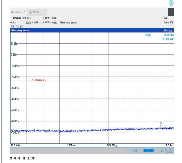
66-66-15MHz-10MHz-64QAM-64QAM-132047-132167-1RB# 74-ORB#0-30~1000MHz-PASS
