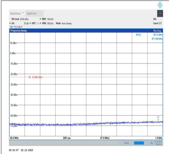
66-66-15MHz-10MHz-64QAM-64QAM-132047-132167-1RB# 0-ORB#0-30~1000MHz-PASS
