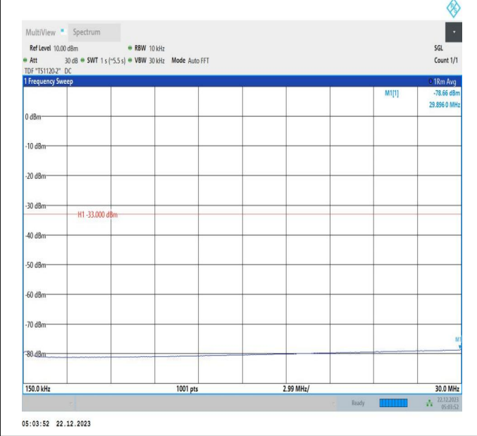
66-66-15MHz-10MHz-64QAM-64QAM-132047-132167-1RB# 0-ORB#0-0.15~30MHz-PASS
