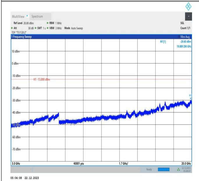
66-66-15MHz-10MHz-64QAM-64QAM-132047-132167-1RB# 0-ORB#0-3000~20000MHz-PASS
