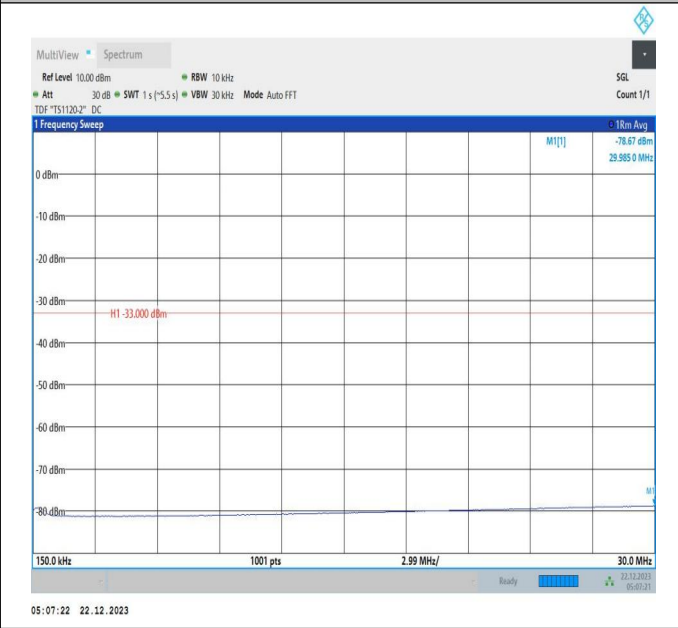
66-66-15MHz-10MHz-QPSK-QPSK-132047-132167-1RB#0- 1RB#49-0.15~30MHz-PASS
