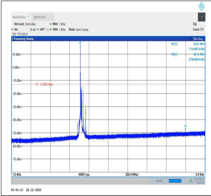
66-66-15MHz-10MHz-16QAM-16QAM-132047-132167-1RB# 0-ORB#0-1000~3000MHz-PASS
