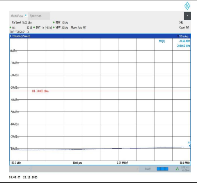
66-66-15MHz-10MHz-64QAM-64QAM-132047-132167-1RB# 0-1RB#49-0.15~30MHz-PASS
