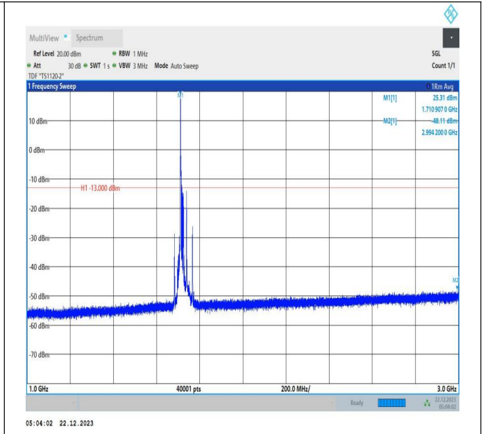
66-66-15MHz-10MHz-64QAM-64QAM-132047-132167-1RB# 0-ORB#0-1000~3000MHz-PASS
