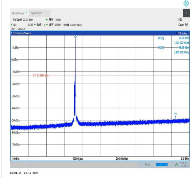
66-66-15MHz-10MHz-QPSK-QPSK-132047-132167-1RB#74 -ORB#0-1000~3000MHz-PASS
