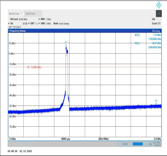
66-66-10MHz-20MHz-16QAM-16QAM-132428-132572-50RB #0-100RB#0-1000~3000MHz-PASS
