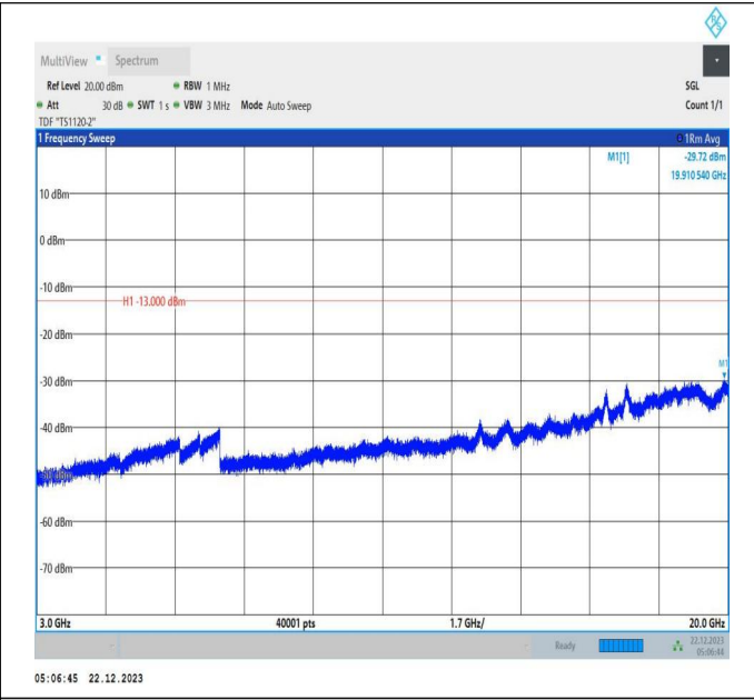
66-66-15MHz-10MHz-64QAM-64QAM-132047-132167-1RB# 74-0RB#0-3000~20000MHz-PASS
