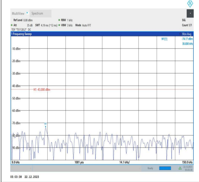
66-66-15MHz-10MHz-64QAM-64QAM-132047-132167-1RB# 0-ORB#0-0.009~0.15MHz-PASS
