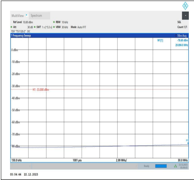
66-66-15MHz-10MHz-QPSK-QPSK-132047-132167-1RB#74 -ORB#0-0.15~30MHz-PASS
