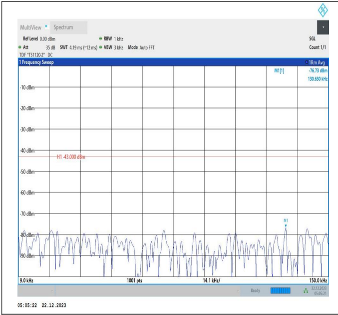
66-66-15MHz-10MHz-16QAM-16QAM-132047-132167-1RB# 74-ORB#0-0.009~0.15MHz-PASS
