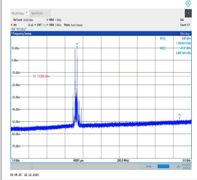
66-66-15MHz-10MHz-16QAM-16QAM-132047-132167-1RB# 0-1RB#49-1000~3000MHz-PASS
