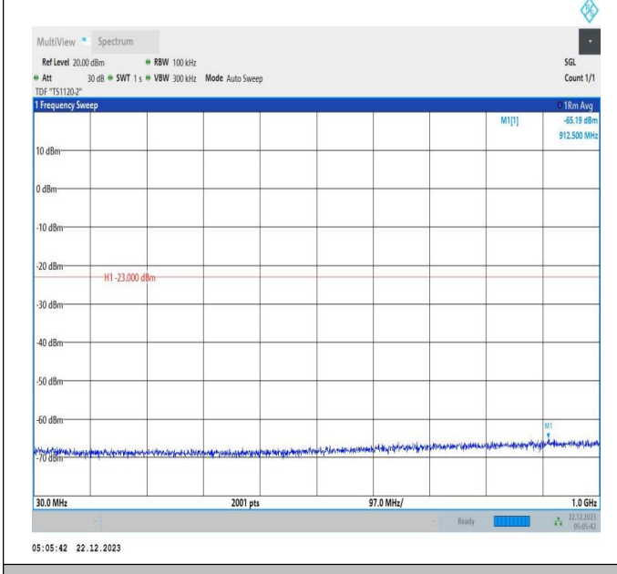
66-66-15MHz-10MHz-16QAM-16QAM-132047-132167-1RB# 74-ORB#0-30~1000MHz-PASS
