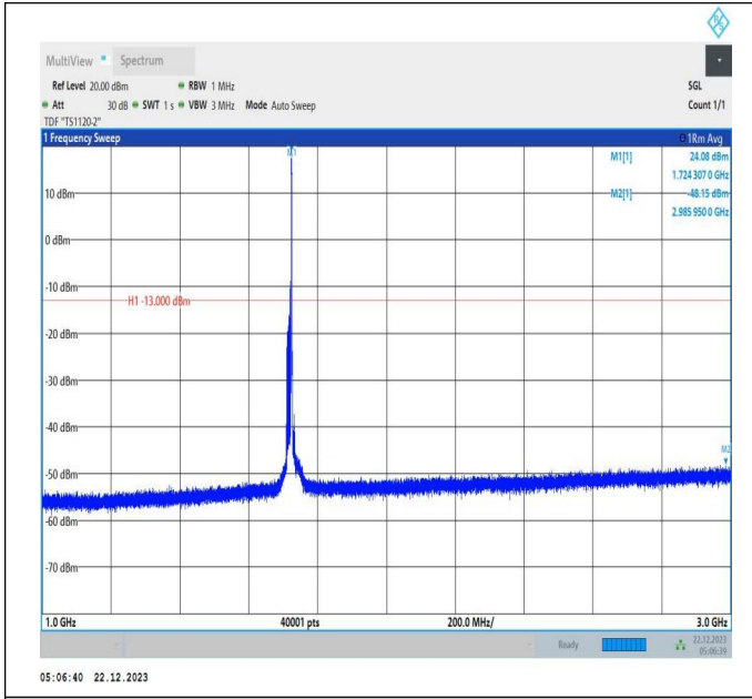
66-66-15MHz-10MHz-64QAM-64QAM-132047-132167-1RB# 74-0RB#0-1000~3000MHz-PASS
