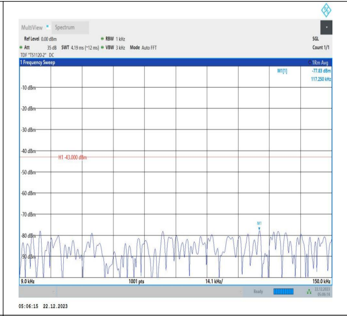
66-66-15MHz-10MHz-64QAM-64QAM-132047-132167-1RB# 74-ORB#0-0.009~0.15MHz-PASS
