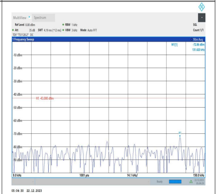
66-66-15MHz-10MHz-QPSK-QPSK-132047-132167-1RB#74 -ORB#0-0.009~0.15MHz-PASS
