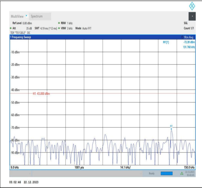
66-66-15MHz-10MHz-16QAM-16QAM-132047-132167-1RB#0-ORB#0-0.009~0.15MHz-PASS
