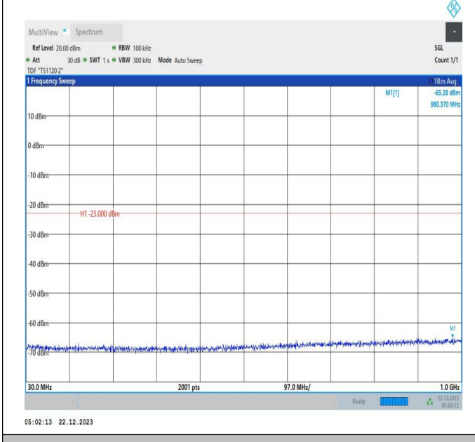
66-66-15MHz-10MHz-QPSK-QPSK-132047-132167-1RB#0-ORB#0-30~1000MHz-PASS
