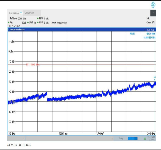
66-66-15MHz-10MHz-16QAM-16QAM-132047-132167-1RB# 0-ORB#0-3000~20000MHz-PASS
