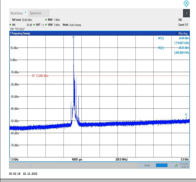
66-66-15MHz-10MHz-QPSK-QPSK-132047-132167-1RB#0-ORB#0-1000~3000MHz-PASS
