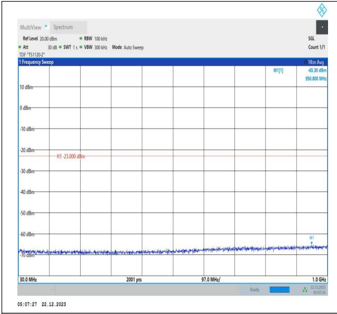
66-66-15MHz-10MHz-QPSK-QPSK-132047-132167-1RB#0-1RB#49-30~1000MHz-PASS
