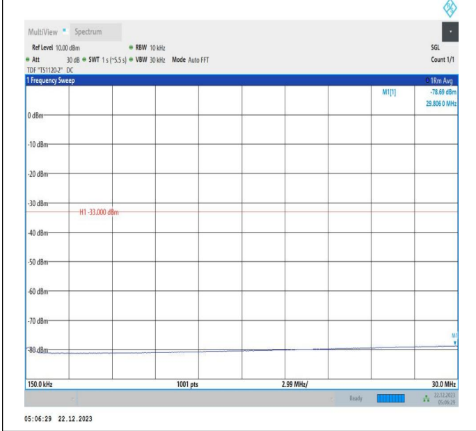
66-66-15MHz-10MHz-64QAM-64QAM-132047-132167-1RB# 74-ORB#0-0.15~30MHz-PASS
