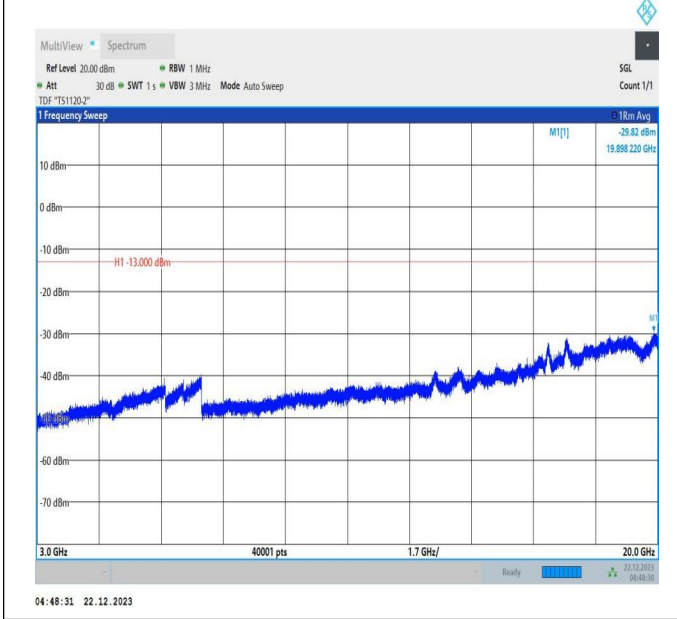
66-66-10MHz-20MHz-16QAM-16QAM-132428-132572-50RB #0-100RB#0-3000~20000MHz-PASS
