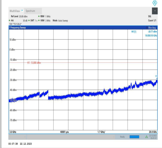
66-66-15MHz-10MHz-QPSK-QPSK-132047-132167-1RB#0-1RB#49-3000~20000MHz-PASS
