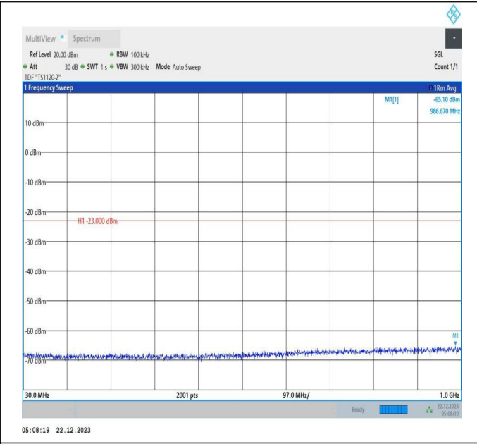
66-66-15MHz-10MHz-16QAM-16QAM-132047-132167-1RB# 0-1RB#49-30~1000MHz-PASS
