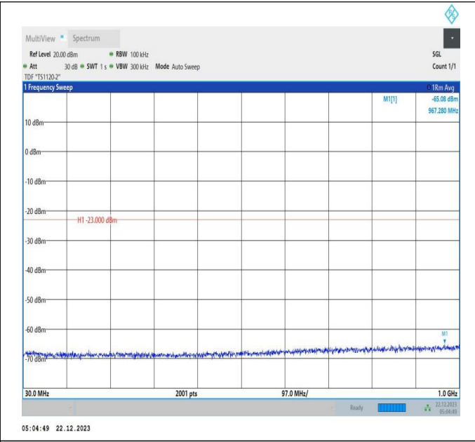
66-66-15MHz-10MHz-QPSK-QPSK-132047-132167-1RB#74 -ORB#0-30~1000MHz-PASS
