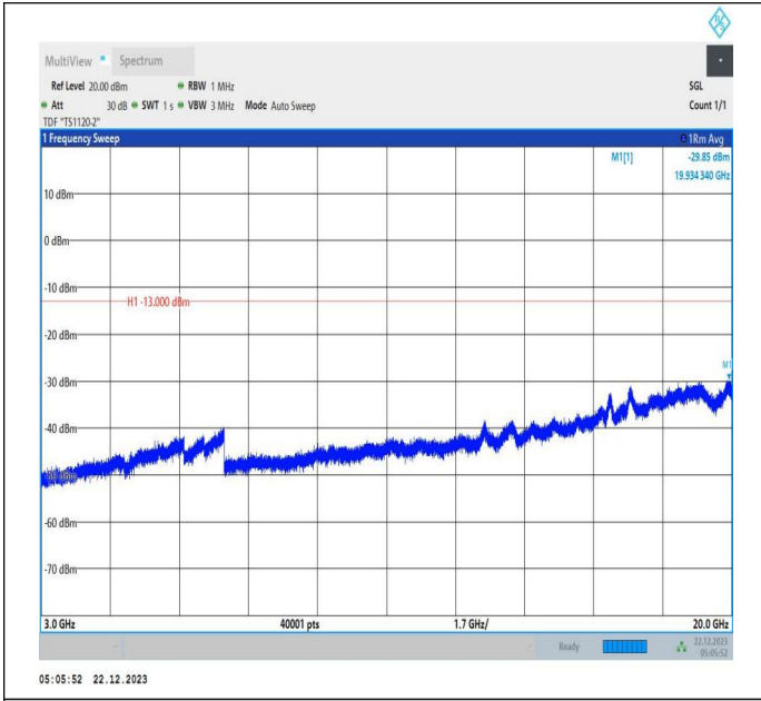
66-66-15MHz-10MHz-16QAM-16QAM-132047-132167-1RB# 74-ORB#0-3000~20000MHz-PASS
