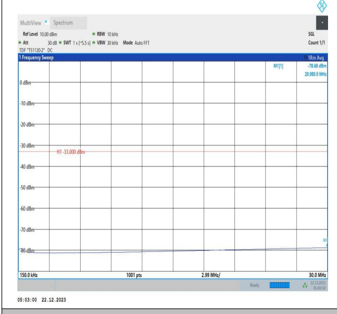
66-66-15MHz-10MHz-16QAM-16QAM-132047-132167-1RB#0-ORB#0-0.15~30MHz-PASS
