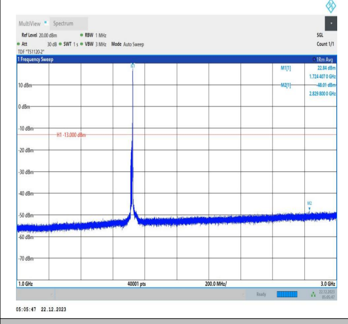
66-66-15MHz-10MHz-16QAM-16QAM-132047-132167-1RB# 74-ORB#0-1000~3000MHz-PASS
