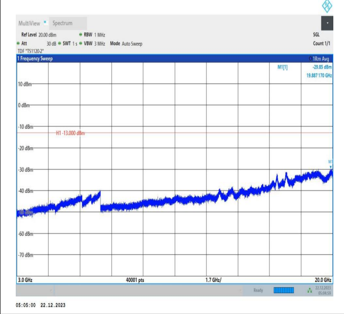
66-66-15MHz-10MHz-QPSK-QPSK-132047-132167-1RB#74 -ORB#0-3000~20000MHz-PASS
