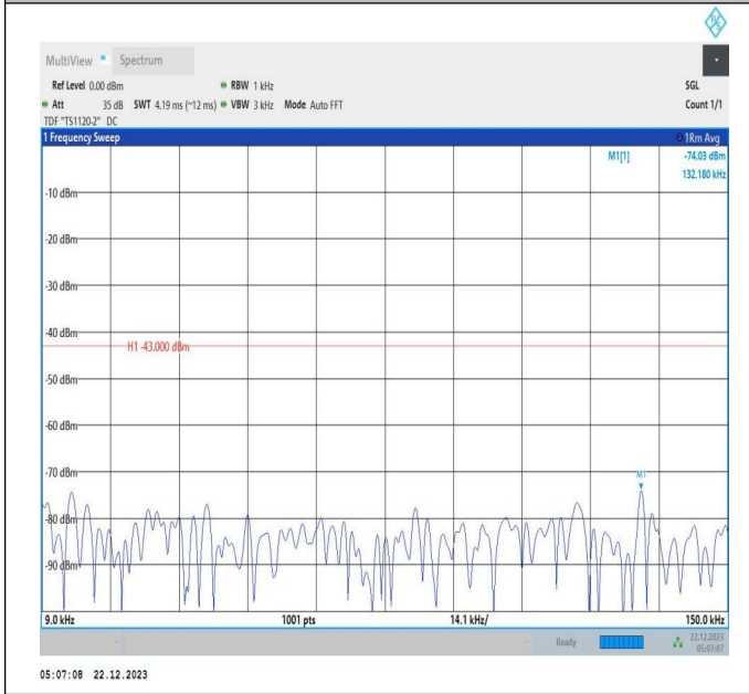
66-66-15MHz-10MHz-QPSK-QPSK-132047-132167-1RB#0- 1RB#49-0.009~0.15MHz-PASS
