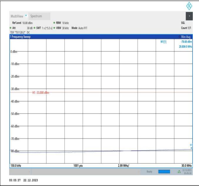
66-66-15MHz-10MHz-16QAM-16QAM-132047-132167-1RB# 74-ORB#0-0.15~30MHz-PASS
