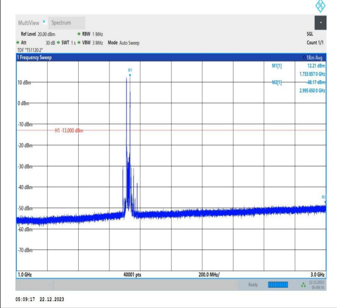
66-66-15MHz-10MHz-64QAM-64QAM-132047-132167-1RB# 0-1RB#49-1000~3000MHz-PASS
