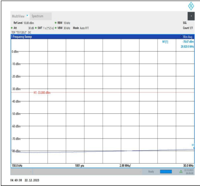
66-66-10MHz-20MHz-64QAM-64QAM-132428-132572-50RB #0-100RB#0-0.15~30MHz-PASS
