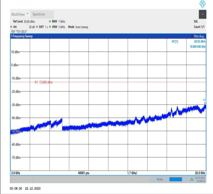
66-66-15MHz-10MHz-16QAM-16QAM-132047-132167-1RB# 0-1RB#49-3000~20000MHz-PASS
