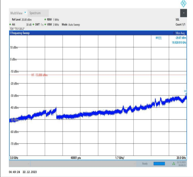
66-66-10MHz-20MHz-64QAM-64QAM-132428-132572-50RB #0-100RB#0-3000~20000MHz-PASS
