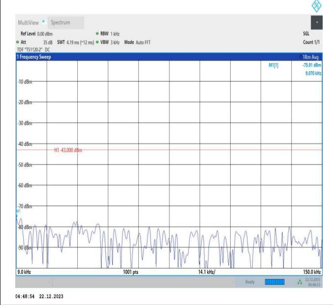
66-66-10MHz-20MHz-64QAM-64QAM-132428-132572-50RB #0-100RB#0-0.009~0.15MHz-PASS
