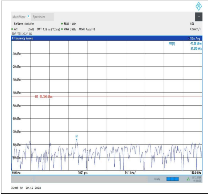
66-66-15MHz-10MHz-64QAM-64QAM-132047-132167-1RB# 0-1RB#49-0.009~0.15MHz-PASS
