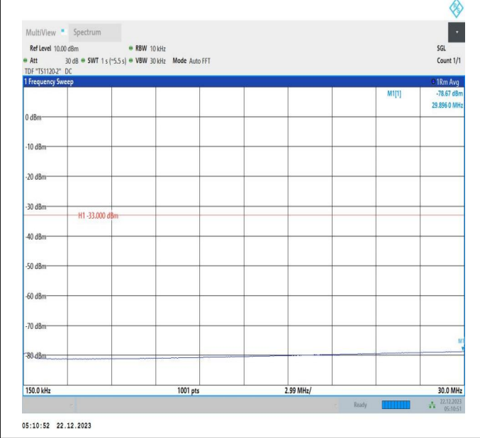
66-66-15MHz-10MHz-16QAM-16QAM-132047-132167-75RB #0-50RB#0-0.15~30MHz-PASS
