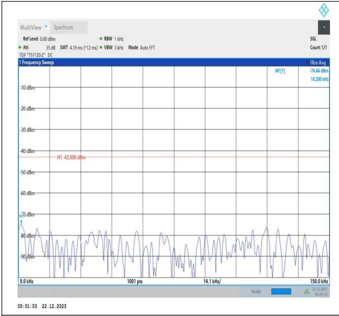
66-66-15MHz-10MHz-QPSK-QPSK-132047-132167-1RB#0-ORB#0-0.009~0.15MHz-PASS
