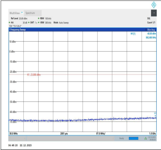
66-66-10MHz-20MHz-16QAM-16QAM-132428-132572-50RB #0-100RB#0-30~1000MHz-PASS
