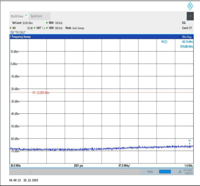
66-66-10MHz-20MHz-64QAM-64QAM-132428-132572-50RB #0-100RB#0-30~1000MHz-PASS
