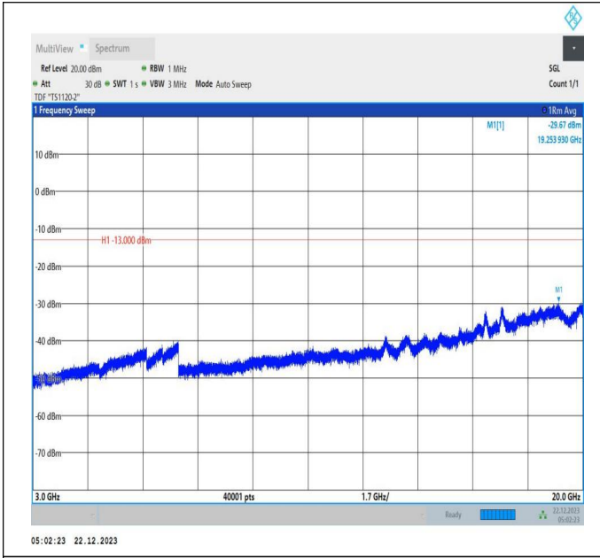
66-66-15MHz-10MHz-QPSK-QPSK-132047-132167-1RB#0-ORB#0-3000~20000MHz-PASS
