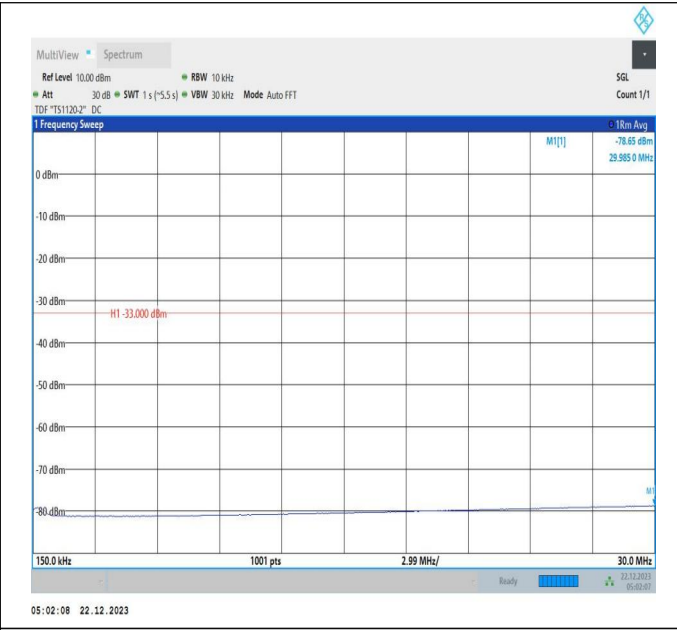
66-66-15MHz-10MHz-QPSK-QPSK-132047-132167-1RB#0-ORB#0-0.15~30MHz-PASS
