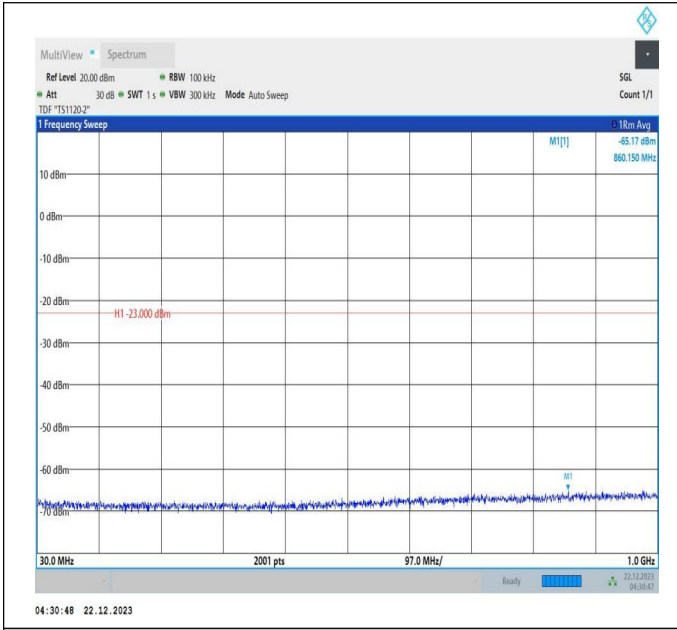
66-66-10MHz-20MHz-64QAM-64QAM-132328-132472-1RB# 0-ORB#0-30~1000MHz-PASS
