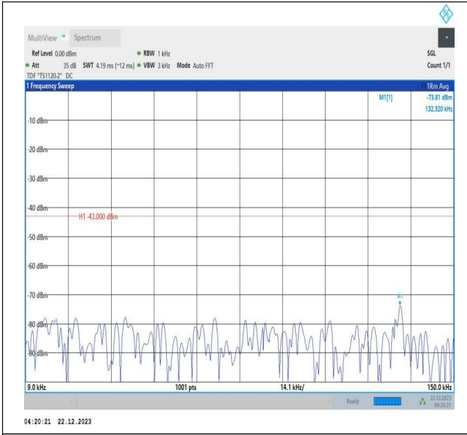
66-66-10MHz-20MHz-16QAM-16QAM-132027-132171-1RB# 49-ORB#0-0.009~0.15MHz-PASS
