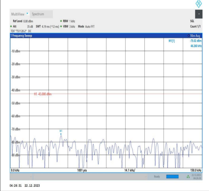
66-66-10MHz-20MHz-64QAM-64QAM-132027-132171-50RB #0-100RB#0-0.009~0.15MHz-PASS
