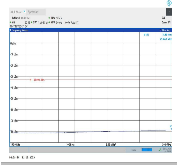
66-66-10MHz-20MHz-16QAM-16QAM-132328-132472-1RB#0-ORB#0-0.15~30MHz-PASS
