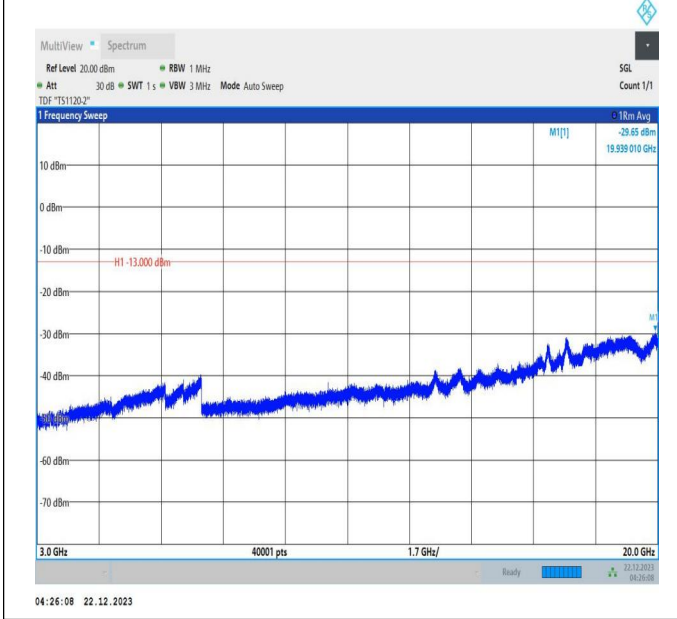
66-66-10MHz-20MHz-16QAM-16QAM-132027-132171-50RB #0-100RB#0-3000~20000MHz-PASS
