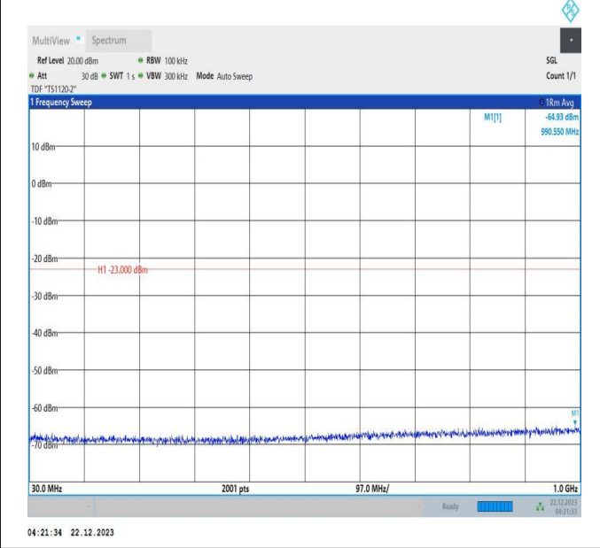
66-66-10MHz-20MHz-64QAM-64QAM-132027-132171-1RB# 49-ORB#0-30~1000MHz-PASS
