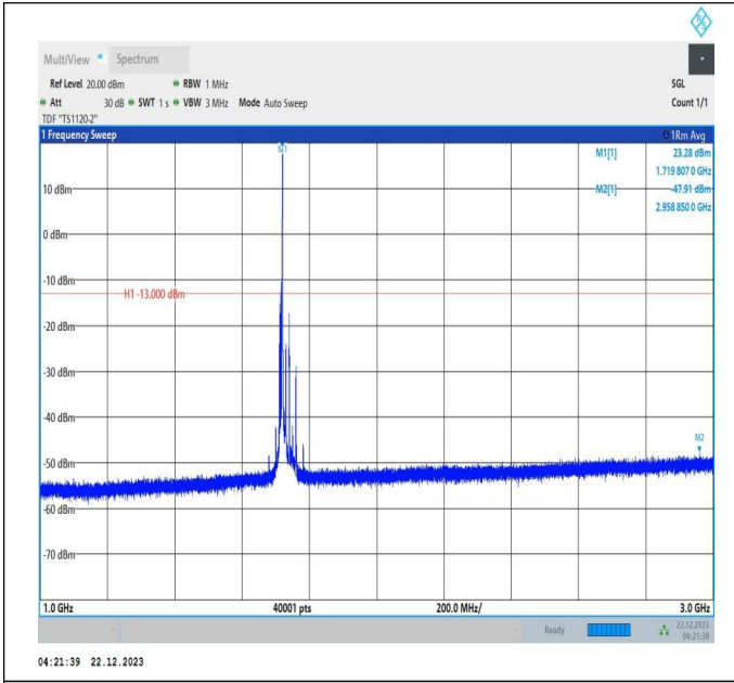
66-66-10MHz-20MHz-64QAM-64QAM-132027-132171-1RB# 49-ORB#0-1000~3000MHz-PASS
