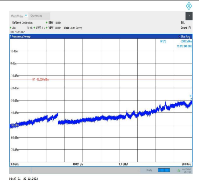
66-66-10MHz-20MHz-64QAM-64QAM-132027-132171-50RB #0-100RB#0-3000~20000MHz-PASS
