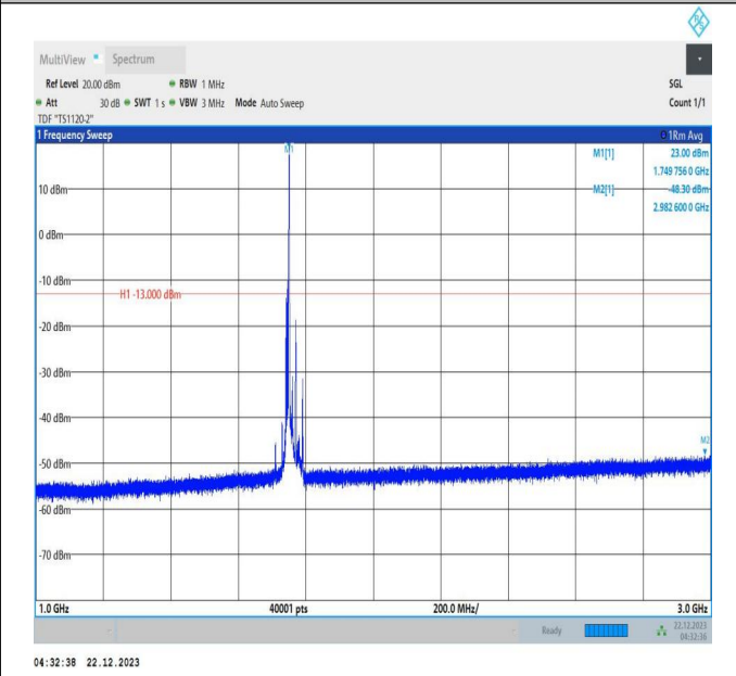
66-66-10MHz-20MHz-16QAM-16QAM-132328-132472-1RB# 49-ORB#0-1000~3000MHz-PASS
