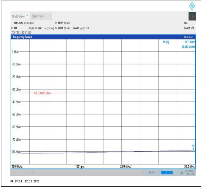
66-66-10MHz-20MHz-16QAM-16QAM-132027-132171-1RB# 0-1RB#99-0.15~30MHz-PASS
