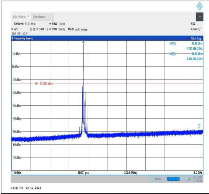
66-66-10MHz-20MHz-64QAM-64QAM-132328-132472-1RB# 49-ORB#0-1000~3000MHz-PASS
