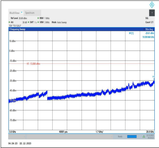
66-66-10MHz-20MHz-64QAM-64QAM-132027-132171-1RB#0-1RB#99-3000~20000MHz-PASS
