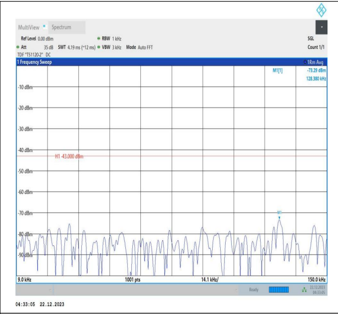
66-66-10MHz-20MHz-64QAM-64QAM-132328-132472-1RB# 49-ORB#0-0.009~0.15MHz-PASS
