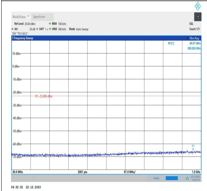
66-66-10MHz-20MHz-16QAM-16QAM-132328-132472-1RB# 49-ORB#0-30~1000MHz-PASS
