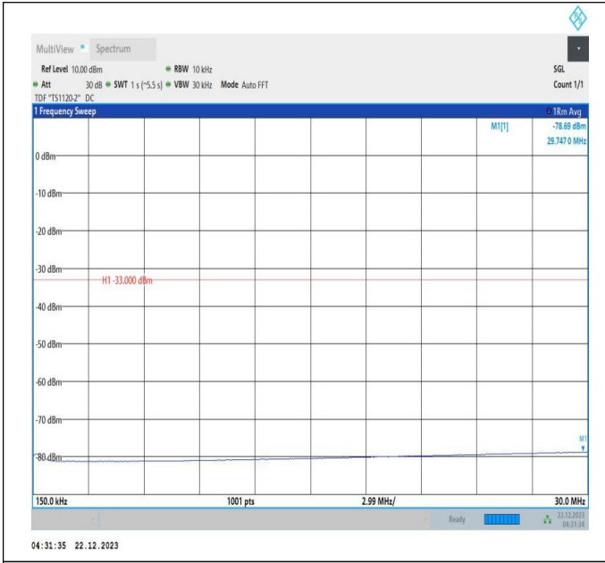
66-66-10MHz-20MHz-QPSK-QPSK-132328-132472-1RB#49 -ORB#0-0.15~30MHz-PASS
