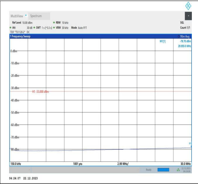
66-66-10MHz-20MHz-64QAM-64QAM-132027-132171-1RB# 0-1RB#99-0.15~30MHz-PASS
