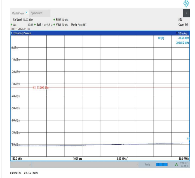
66-66-10MHz-20MHz-64QAM-64QAM-132027-132171-1RB# 49-ORB#0-0.15~30MHz-PASS
