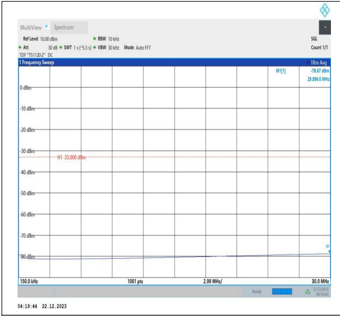
66-66-10MHz-20MHz-QPSK-QPSK-132027-132171-1RB#49 -ORB#0-0.15~30MHz-PASS
