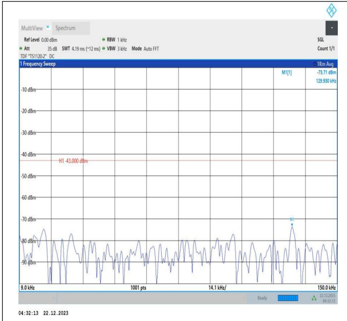
66-66-10MHz-20MHz-16QAM-16QAM-132328-132472-1RB# 49-ORB#0-0.009~0.15MHz-PASS
