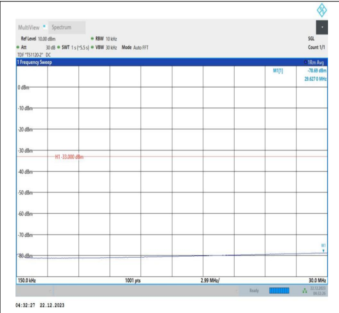
66-66-10MHz-20MHz-16QAM-16QAM-132328-132472-1RB# 49-ORB#0-0.15~30MHz-PASS
