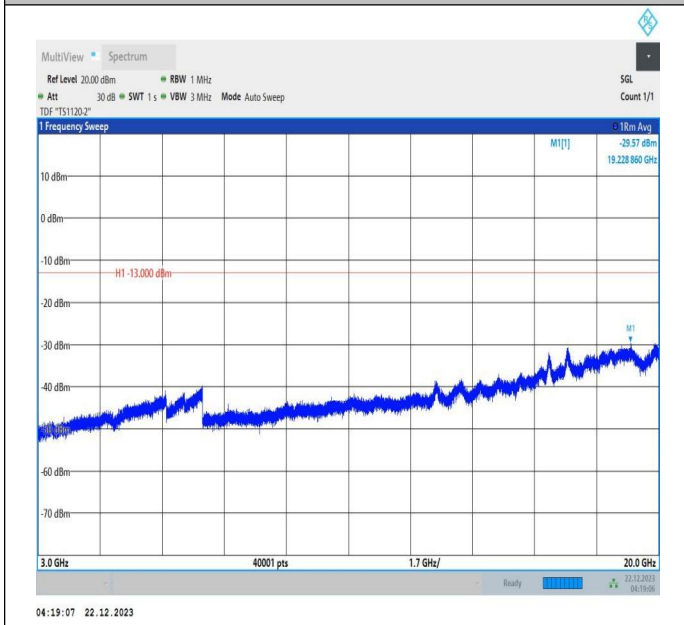
66-66-10MHz-20MHz-64QAM-64QAM-132027-132171-1RB# 0-ORB#0-3000~20000MHz-PASS
