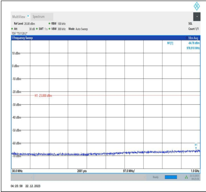
66-66-10MHz-20MHz-16QAM-16QAM-132027-132171-50RB #0-100RB#0-30~1000MHz-PASS
