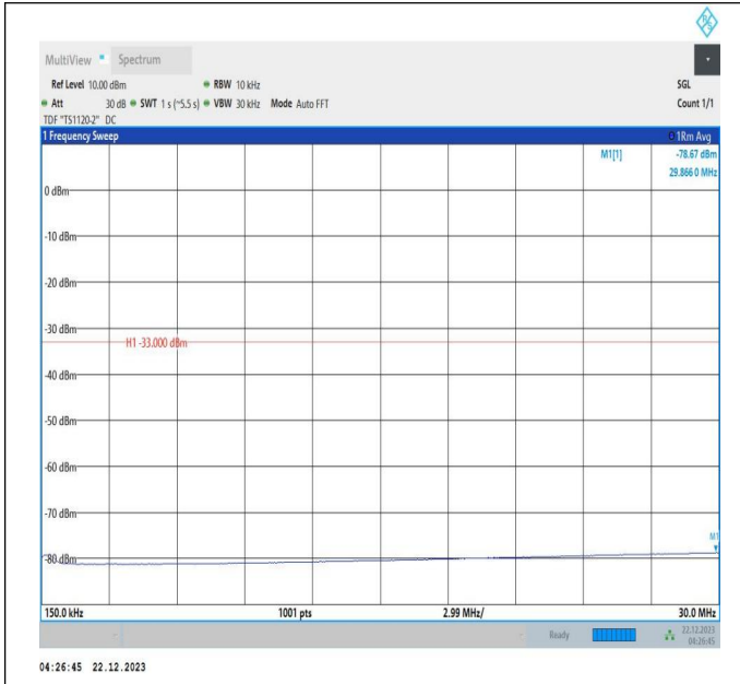
66-66-10MHz-20MHz-64QAM-64QAM-132027-132171-50RB #0-100RB#0-0.15~30MHz-PASS
