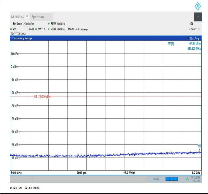
66-66-10MHz-20MHz-16QAM-16QAM-132027-132171-1RB# 0-1RB#99-30~1000MHz-PASS
