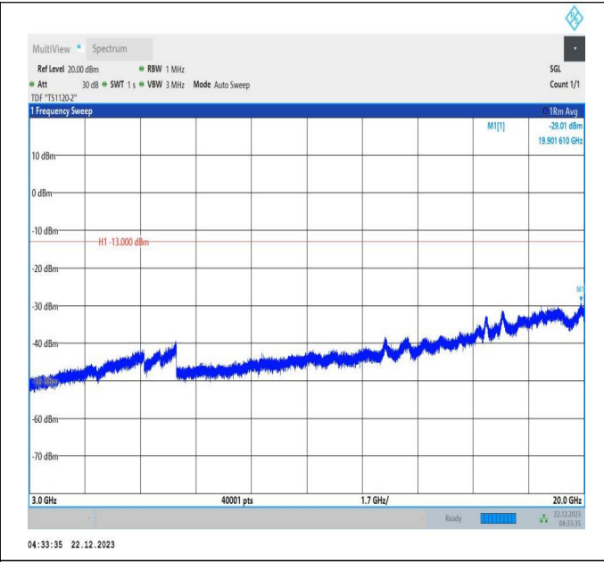
66-66-10MHz-20MHz-64QAM-64QAM-132328-132472-1RB# 49-ORB#0-3000~20000MHz-PASS
