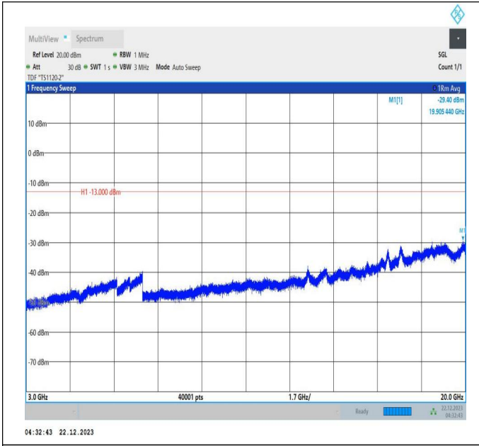
66-66-10MHz-20MHz-16QAM-16QAM-132328-132472-1RB# 49-ORB#0-3000~20000MHz-PASS
