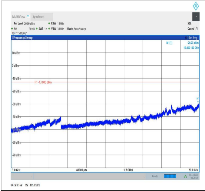
66-66-10MHz-20MHz-16QAM-16QAM-132027-132171-1RB# 49-ORB#0-3000~20000MHz-PASS
