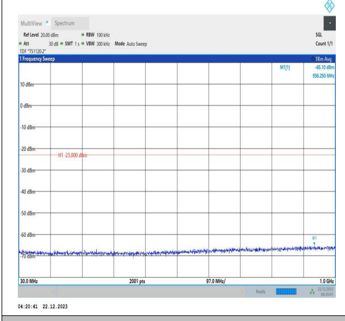
66-66-10MHz-20MHz-16QAM-16QAM-132027-132171-1RB# 49-ORB#0-30~1000MHz-PASS
