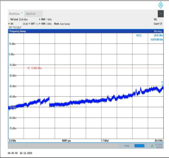
66-66-10MHz-20MHz-16QAM-16QAM-132328-132472-1RB# 0-ORB#0-3000~20000MHz-PASS
