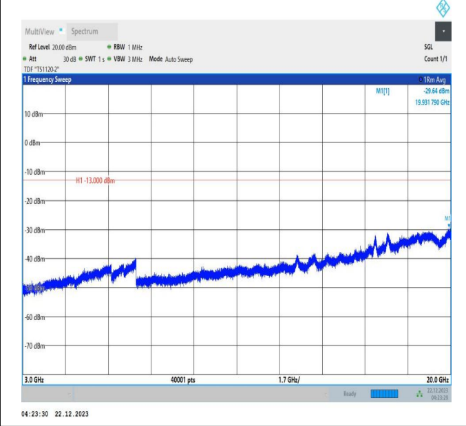
66-66-10MHz-20MHz-16QAM-16QAM-132027-132171-1RB# 0-1RB#99-3000~20000MHz-PASS
