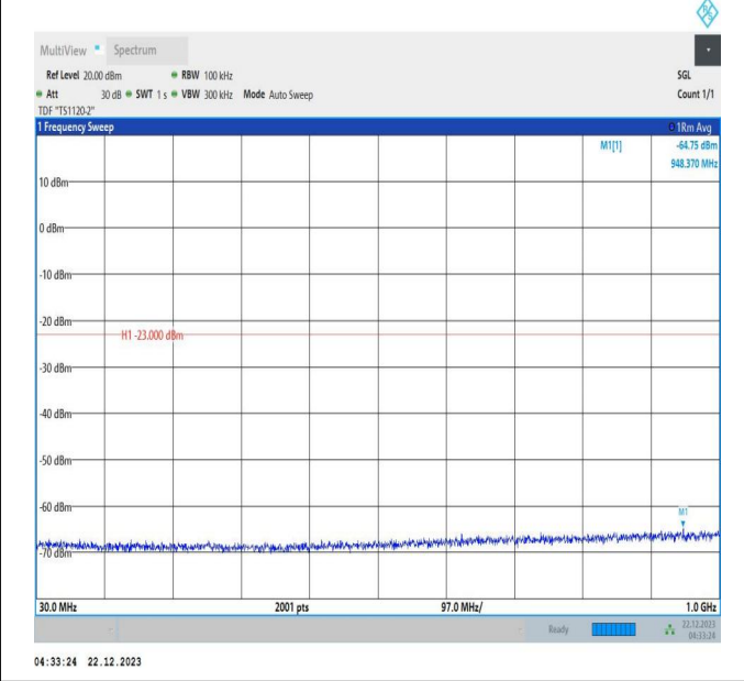
66-66-10MHz-20MHz-64QAM-64QAM-132328-132472-1RB# 49-ORB#0-30~1000MHz-PASS
