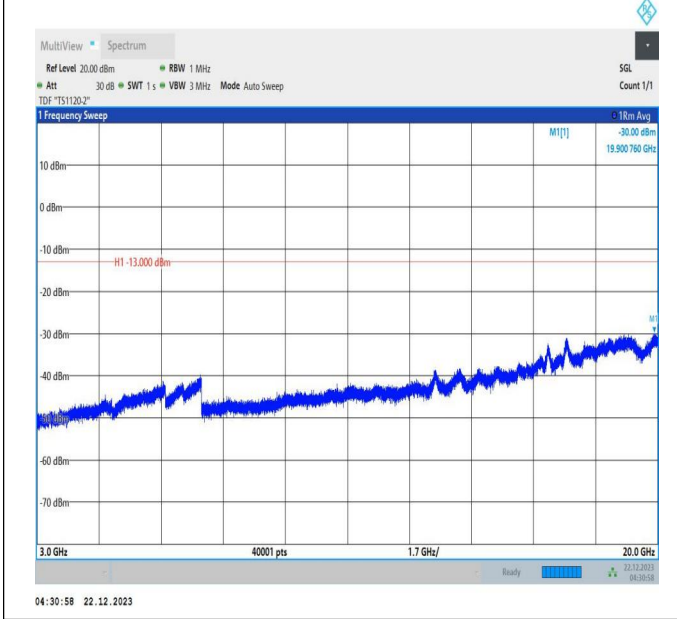
66-66-10MHz-20MHz-64QAM-64QAM-132328-132472-1RB# 0-ORB#0-3000~20000MHz-PASS
