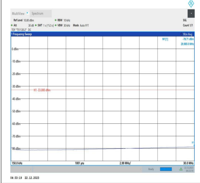
66-66-10MHz-20MHz-64QAM-64QAM-132328-132472-1RB# 49-ORB#0-0.15~30MHz-PASS
