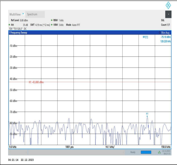
66-66-10MHz-20MHz-64QAM-64QAM-132027-132171-1RB# 49-ORB#0-0.009~0.15MHz-PASS
