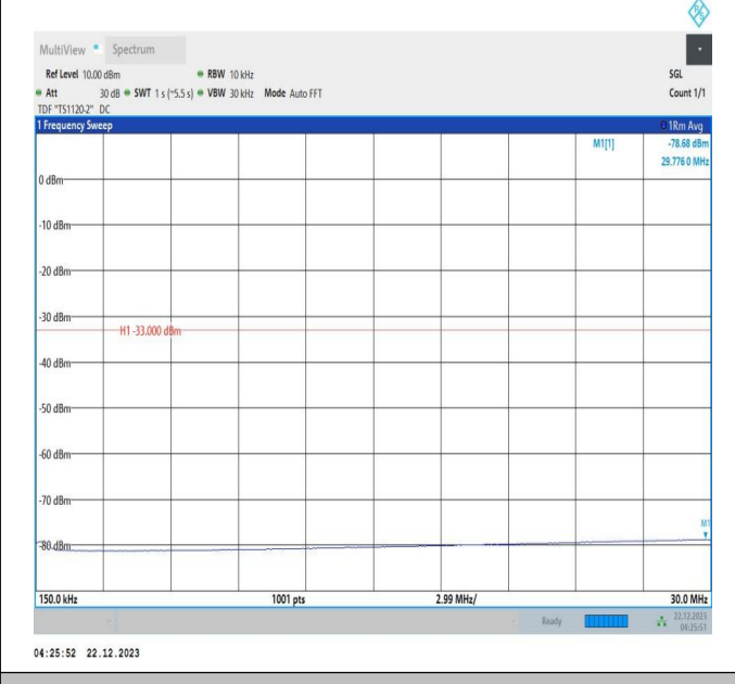
66-66-10MHz-20MHz-16QAM-16QAM-132027-132171-50RB#0-100RB#0-0.15~30MHz-PASS
