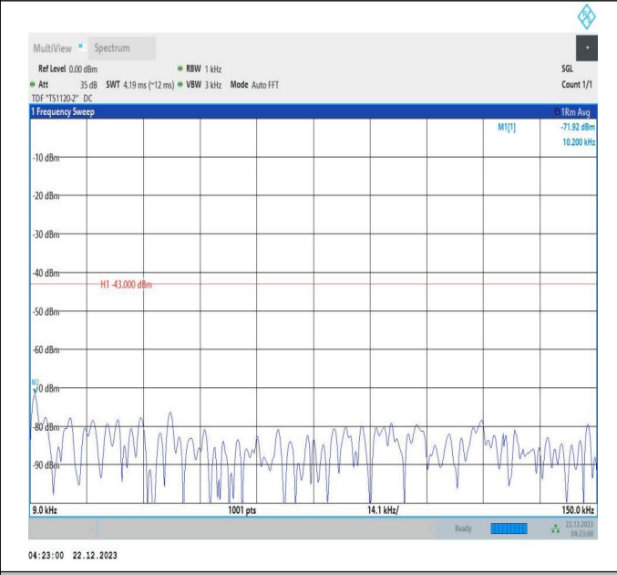
66-66-10MHz-20MHz-16QAM-16QAM-132027-132171-1RB#0-1RB#99-0.009~0.15MHz-PASS
