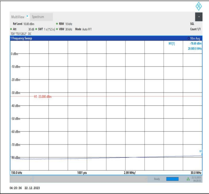
66-66-10MHz-20MHz-16QAM-16QAM-132027-132171-1RB# 49-ORB#0-0.15~30MHz-PASS
