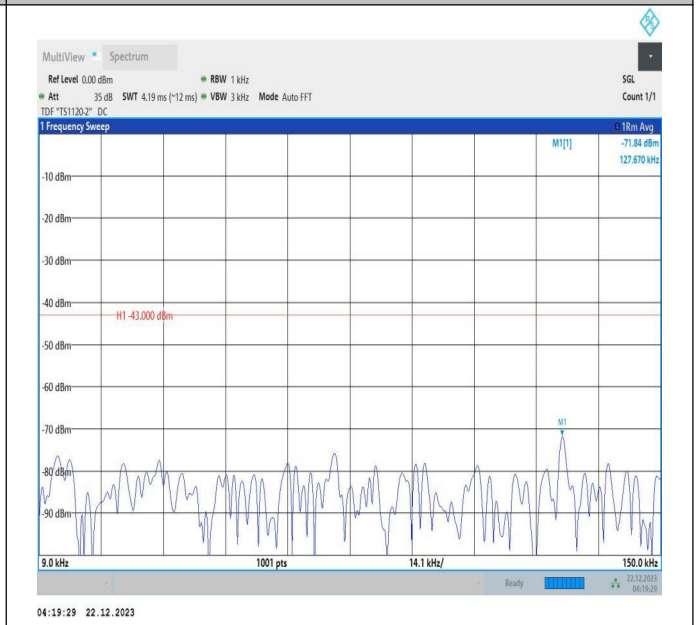
66-66-10MHz-20MHz-QPSK-QPSK-132027-132171-1RB#49 -ORB#0-0.009~0.15MHz-PASS
