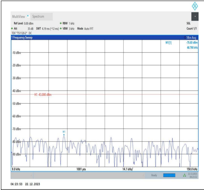
66-66-10MHz-20MHz-64QAM-64QAM-132027-132171-1RB# 0-1RB#99-0.009~0.15MHz-PASS
