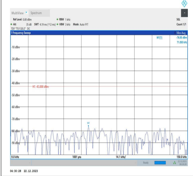
66-66-10MHz-20MHz-64QAM-64QAM-132328-132472-1RB# 0-ORB#0-0.009~0.15MHz-PASS
