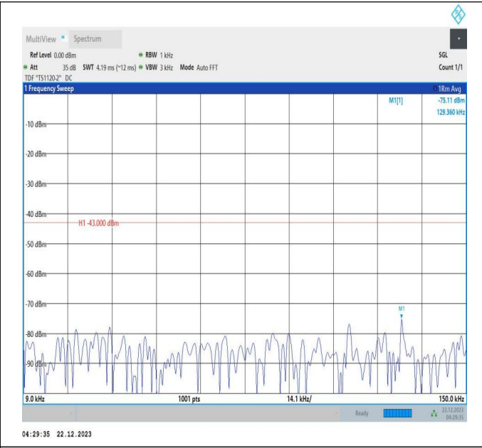
66-66-10MHz-20MHz-16QAM-16QAM-132328-132472-1RB#0-ORB#0-0.009~0.15MHz-PASS
