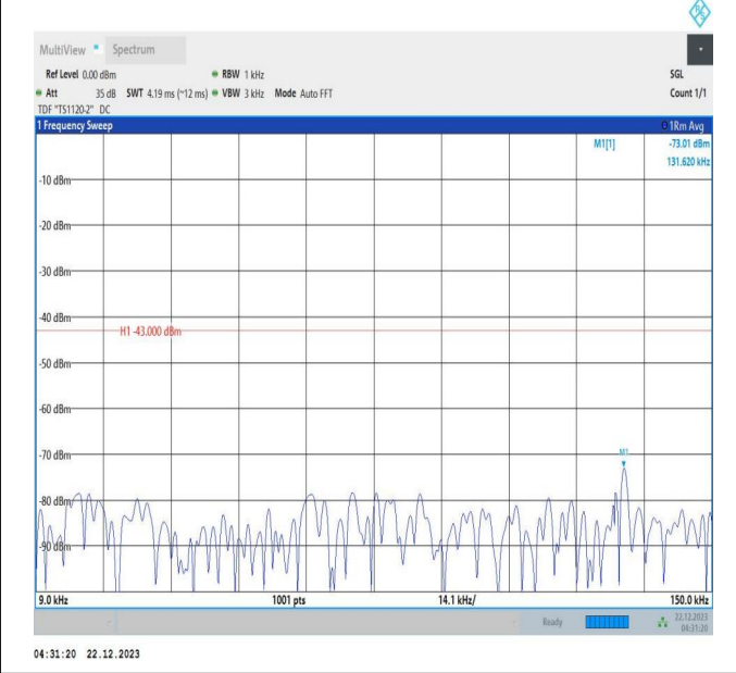
66-66-10MHz-20MHz-QPSK-QPSK-132328-132472-1RB#49 -ORB#0-0.009~0.15MHz-PASS
