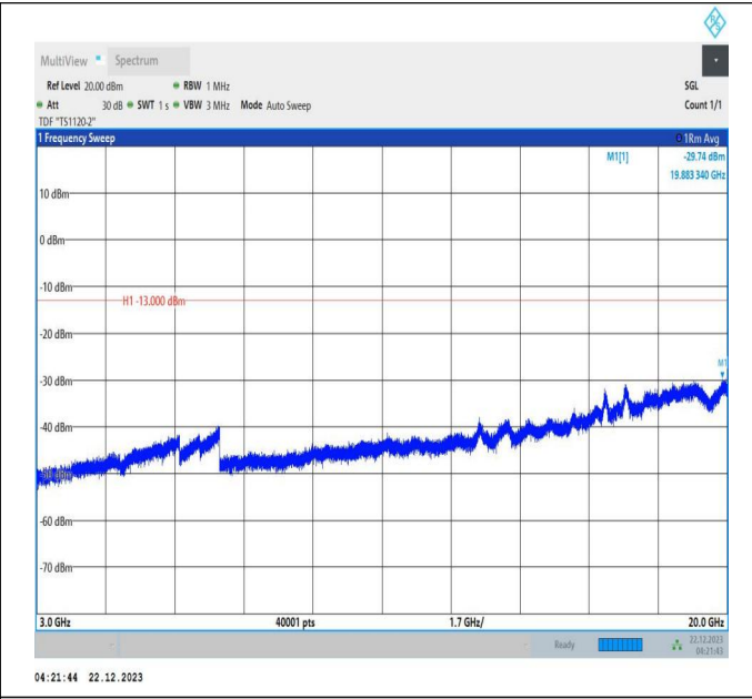
66-66-10MHz-20MHz-64QAM-64QAM-132027-132171-1RB# 49-ORB#0-3000~20000MHz-PASS
