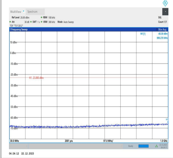
66-66-10MHz-20MHz-64QAM-64QAM-132027-132171-1RB# 0-1RB#99-30~1000MHz-PASS
