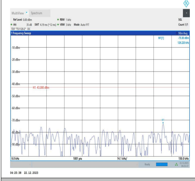
66-66-10MHz-20MHz-16QAM-16QAM-132027-132171-50RB#0-100RB#0-0.009~0.15MHz-PASS
