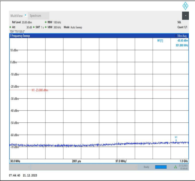
66-66-10MHz-15MHz-16QAM-16QAM-132477-132597-1RB# 0-1RB#74-30~1000MHz-PASS
