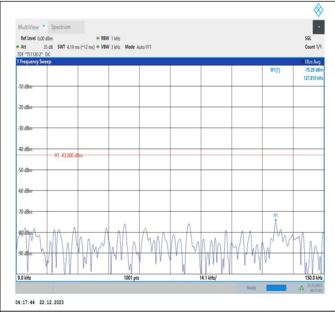
66-66-10MHz-20MHz-16QAM-16QAM-132027-132171-1RB#0-ORB#0-0.009~0.15MHz-PASS
