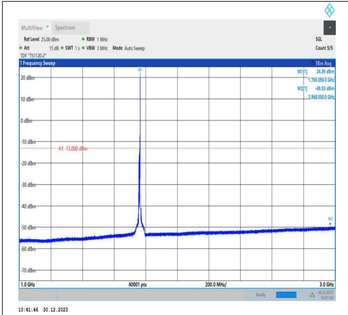
66-66-10MHz-15MHz-64QAM-64QAM-132477-132597-1RB# 49-ORB#0-1000~3000MHz-PASS
