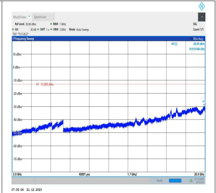
66-66-10MHz-15MHz-64QAM-64QAM-132477-132597-1RB# 49-ORB#0-3000~20000MHz-PASS
