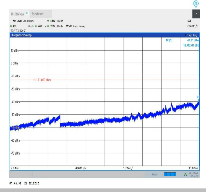
66-66-10MHz-15MHz-16QAM-16QAM-132477-132597-1RB# 0-1RB#74-3000~20000MHz-PASS
