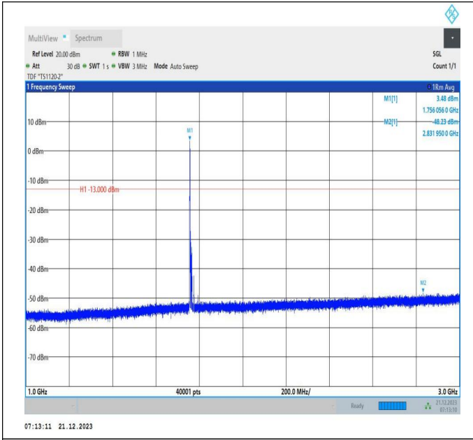
66-66-10MHz-15MHz-16QAM-16QAM-132477-132597-1RB# 0-ORB#0-1000~3000MHz-PASS
