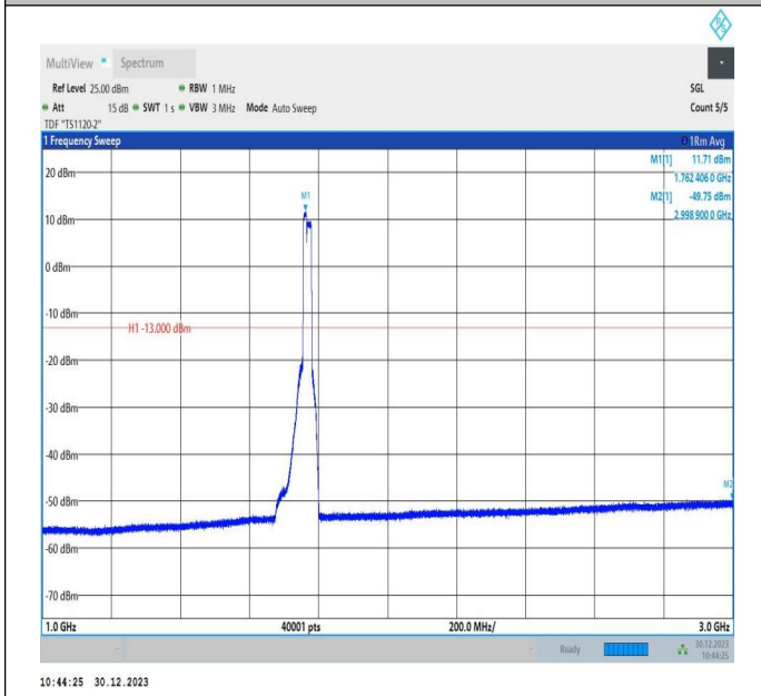
66-66-10MHz-15MHz-64QAM-64QAM-132477-132597-50RB #0-75RB#0-1000~3000MHz-PASS
