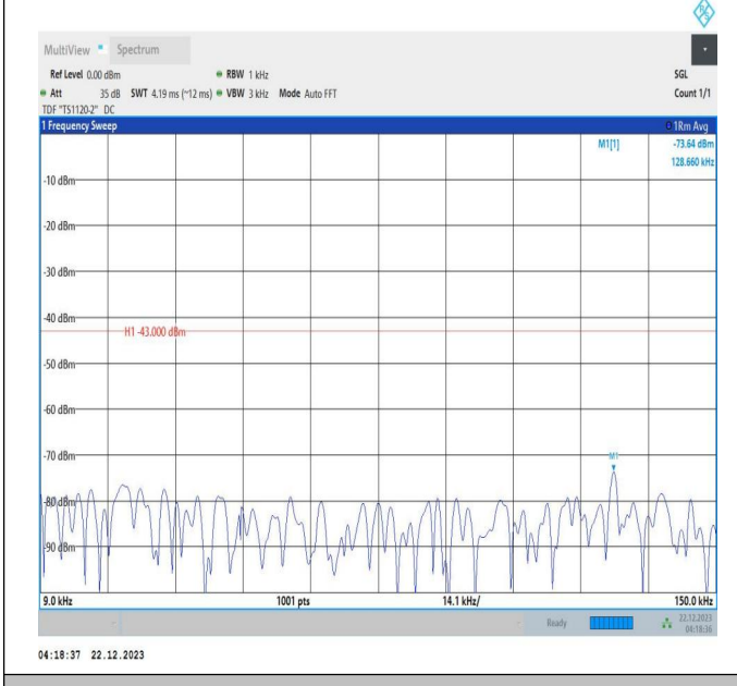
66-66-10MHz-20MHz-64QAM-64QAM-132027-132171-1RB# 0-ORB#0-0.009~0.15MHz-PASS
