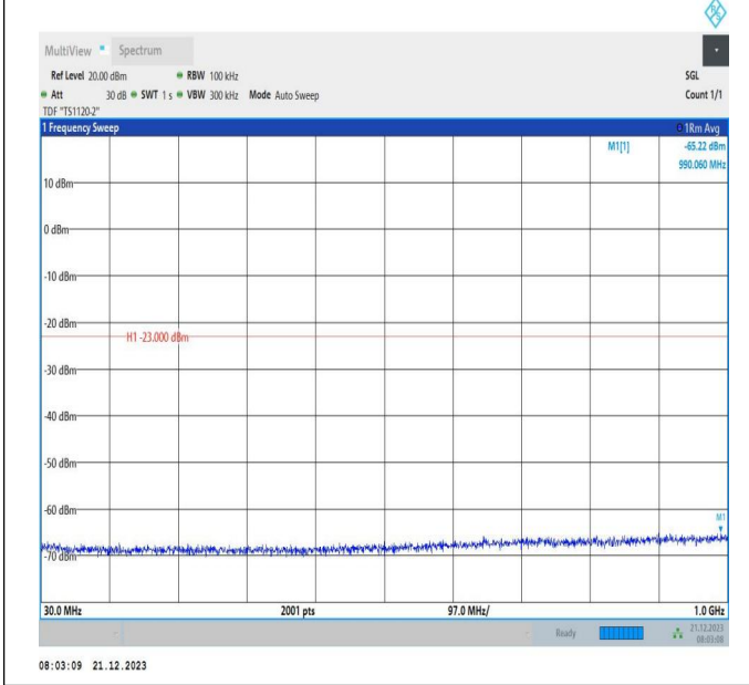
66-66-10MHz-15MHz-64QAM-64QAM-132477-132597-1RB# 0-1RB#74-30~1000MHz-PASS
