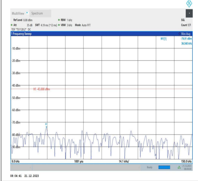
66-66-10MHz-15MHz-16QAM-16QAM-132477-132597-50RB#0-75RB#0-0.009~0.15MHz-PASS
