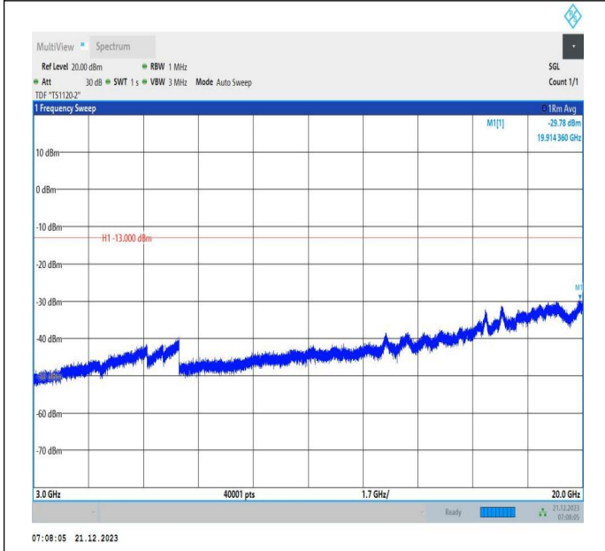
66-66-10MHz-15MHz-16QAM-16QAM-132351-132471-50RB #0-75RB#0-3000~20000MHz-PASS
