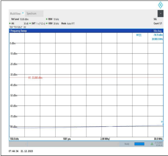
66-66-10MHz-15MHz-16QAM-16QAM-132477-132597-1RB# 0-1RB#74-0.15~30MHz-PASS
