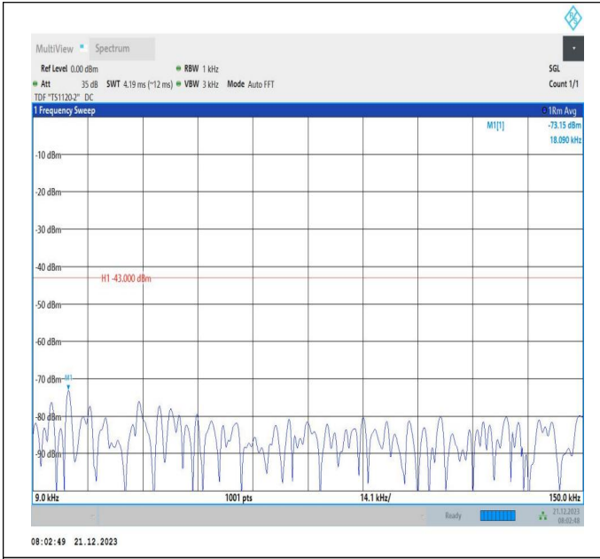
66-66-10MHz-15MHz-64QAM-64QAM-132477-132597-1RB# 0-1RB#74-0.009~0.15MHz-PASS
