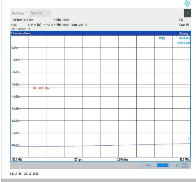
66-66-10MHz-20MHz-16QAM-16QAM-132027-132171-1RB#0-ORB#0-0.15~30MHz-PASS
