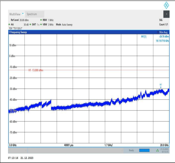
66-66-10MHz-15MHz-16QAM-16QAM-132477-132597-1RB# 0-ORB#0-3000~20000MHz-PASS
