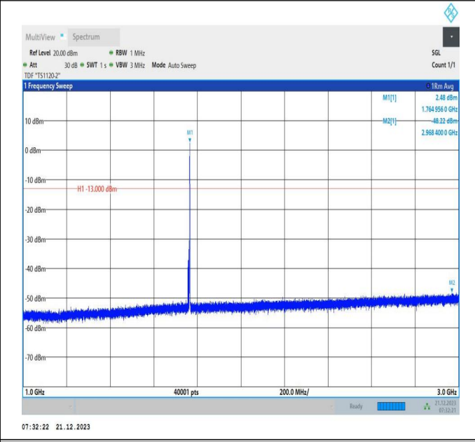
66-66-10MHz-15MHz-16QAM-16QAM-132477-132597-1RB# 49-ORB#0-1000~3000MHz-PASS
