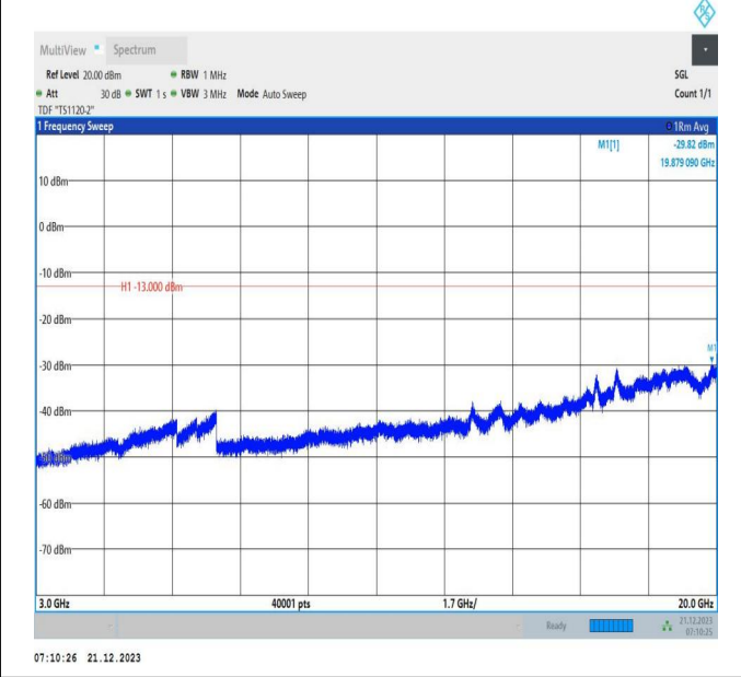
66-66-10MHz-15MHz-64QAM-64QAM-132351-132471-50RB #0-75RB#0-3000~20000MHz-PASS
