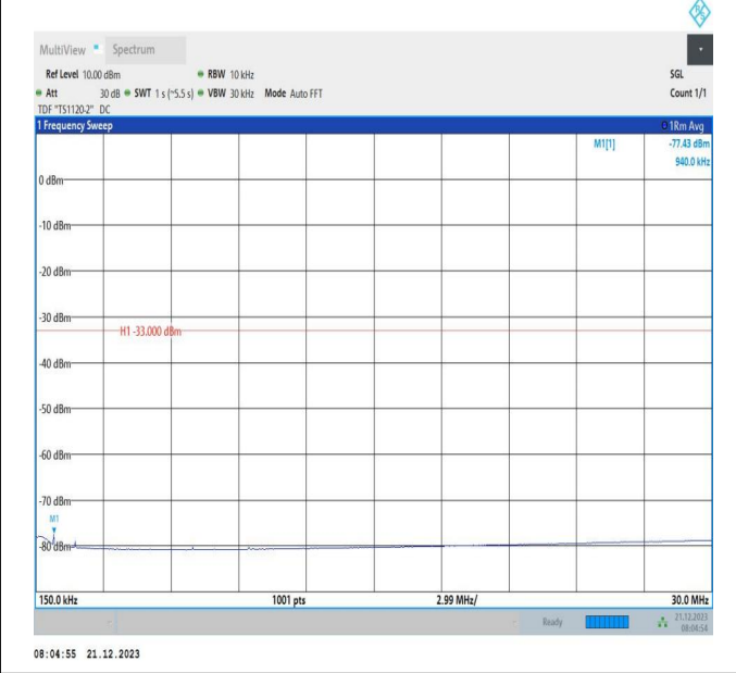
66-66-10MHz-15MHz-16QAM-16QAM-132477-132597-50RB#0-75RB#0-0.15~30MHz-PASS
