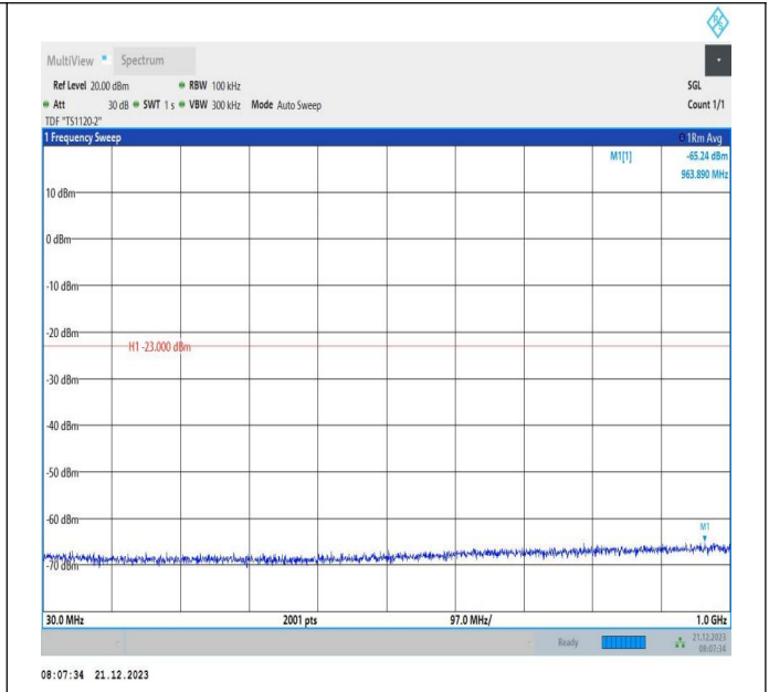
66-66-10MHz-15MHz-64QAM-64QAM-132477-132597-50RB #0-75RB#0-30~1000MHz-PASS
