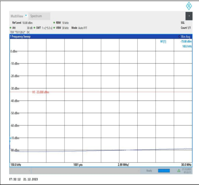
66-66-10MHz-15MHz-16QAM-16QAM-132477-132597-1RB# 49-ORB#0-0.15~30MHz-PASS
