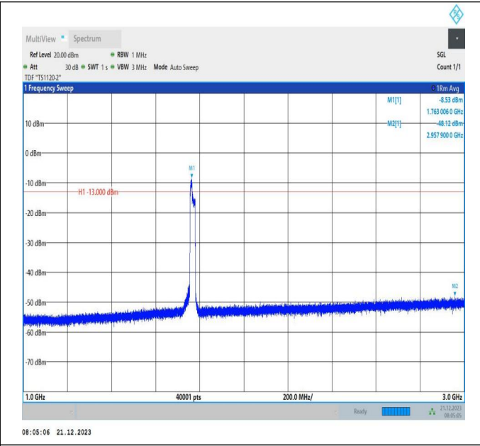
66-66-10MHz-15MHz-16QAM-16QAM-132477-132597-50RB #0-75RB#0-1000~3000MHz-PASS
