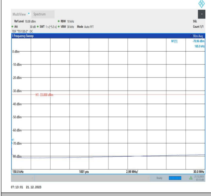
66-66-10MHz-15MHz-16QAM-16QAM-132477-132597-1RB#-0-ORB#0-0.15~30MHz-PASS
