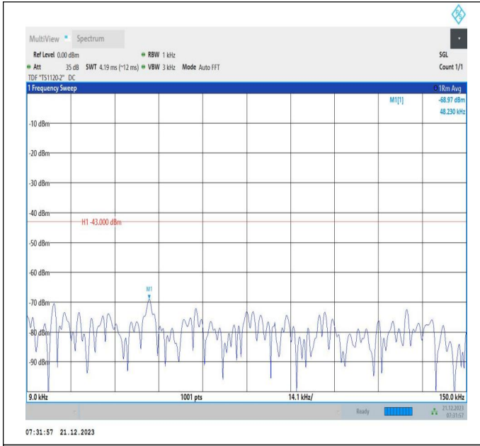
66-66-10MHz-15MHz-16QAM-16QAM-132477-132597-1RB# 49-ORB#0-0.009~0.15MHz-PASS
