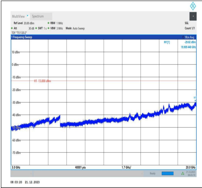
66-66-10MHz-15MHz-64QAM-64QAM-132477-132597-1RB# 0-1RB#74-3000~20000MHz-PASS
