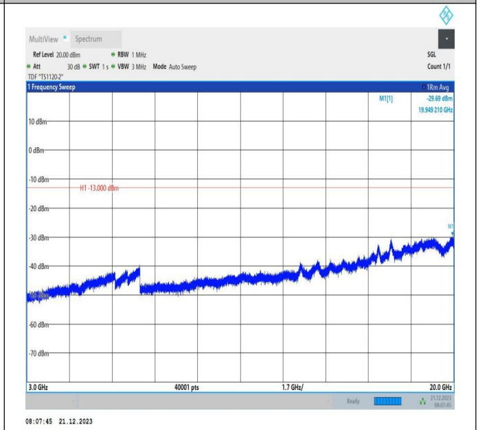
66-66-10MHz-15MHz-64QAM-64QAM-132477-132597-50RB #0-75RB#0-3000~20000MHz-PASS
