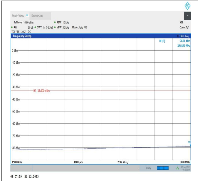
66-66-10MHz-15MHz-64QAM-64QAM-132477-132597-50RB #0-75RB#0-0.15~30MHz-PASS
