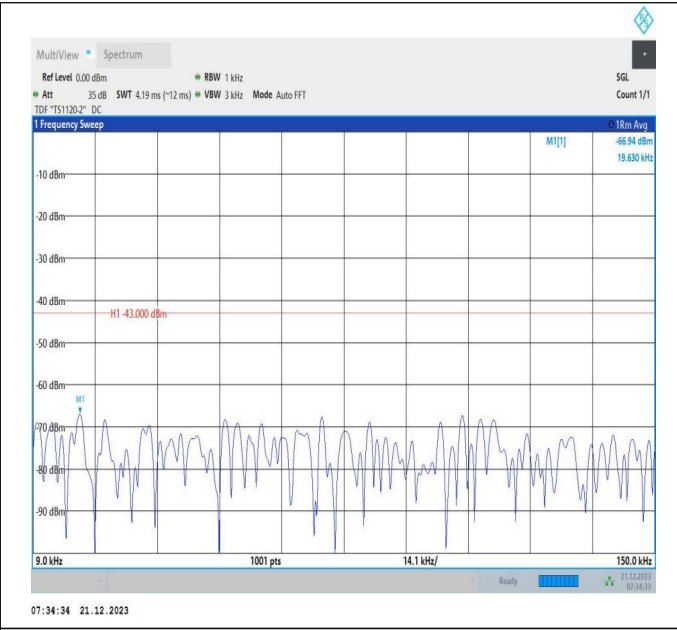
66-66-10MHz-15MHz-64QAM-64QAM-132477-132597-1RB# 49-ORB#0-0.009~0.15MHz-PASS
