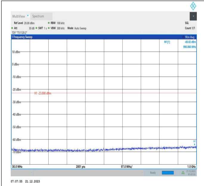
66-66-10MHz-15MHz-16QAM-16QAM-132351-132471-50RB #0-75RB#0-30~1000MHz-PASS
