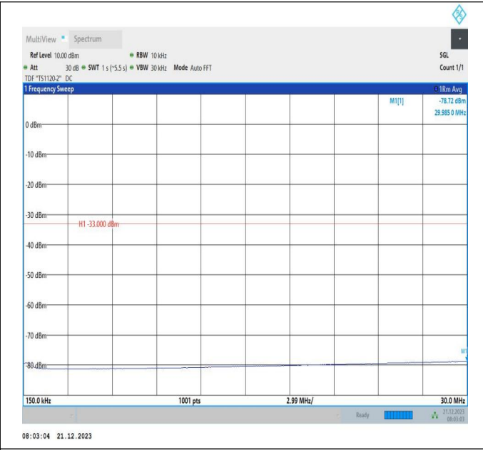
66-66-10MHz-15MHz-64QAM-64QAM-132477-132597-1RB# 0-1RB#74-0.15~30MHz-PASS
