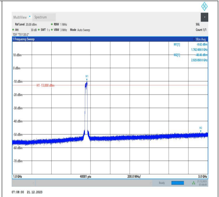
66-66-10MHz-15MHz-16QAM-16QAM-132351-132471-50RB #0-75RB#0-1000~3000MHz-PASS
