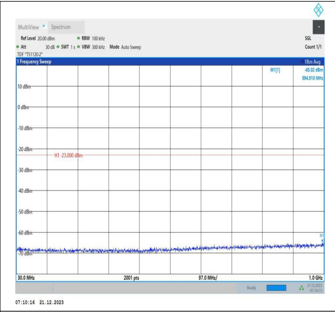
66-66-10MHz-15MHz-64QAM-64QAM-132351-132471-50RB #0-75RB#0-30~1000MHz-PASS
