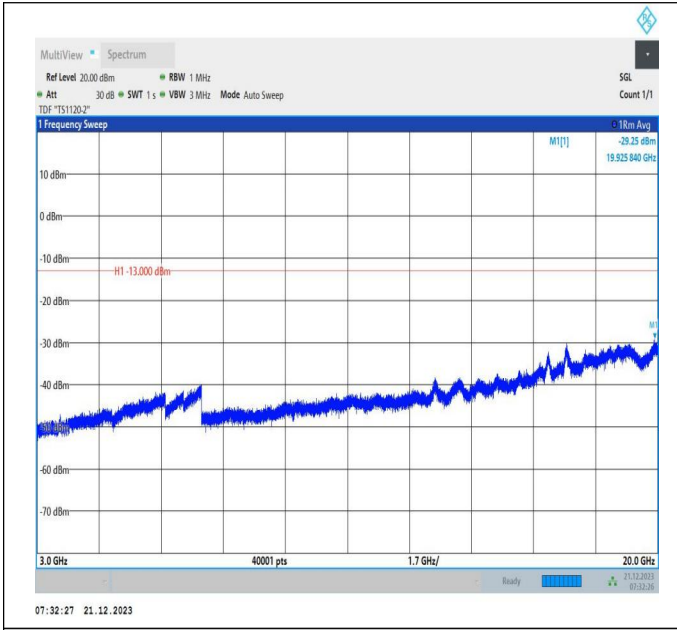
66-66-10MHz-15MHz-16QAM-16QAM-132477-132597-1RB# 49-ORB#0-3000~20000MHz-PASS
