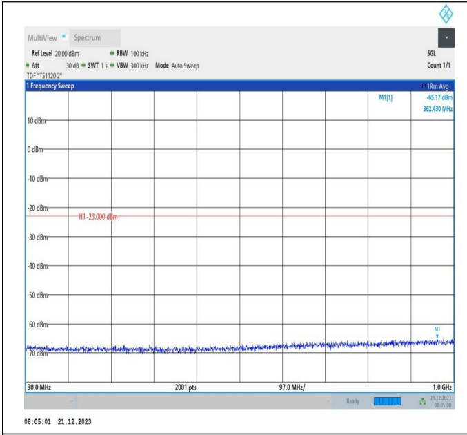
66-66-10MHz-15MHz-16QAM-16QAM-132477-132597-50RB #0-75RB#0-30~1000MHz-PASS
