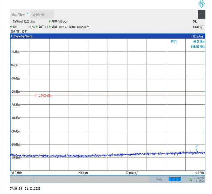
66-66-10MHz-15MHz-64QAM-64QAM-132477-132597-1RB# 49-ORB#0-30~1000MHz-PASS
