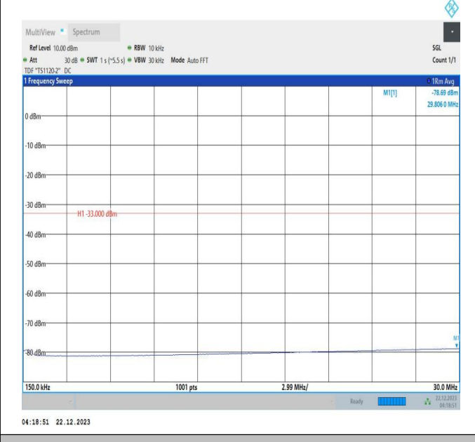
66-66-10MHz-20MHz-64QAM-64QAM-132027-132171-1RB# 0-ORB#0-0.15~30MHz-PASS
