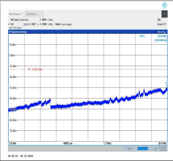
66-66-10MHz-20MHz-16QAM-16QAM-132027-132171-1RB# 0-ORB#0-3000~20000MHz-PASS
