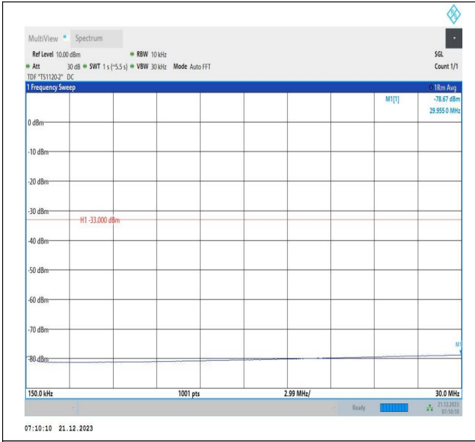
66-66-10MHz-15MHz-64QAM-64QAM-132351-132471-50RB #0-75RB#0-0.15~30MHz-PASS
