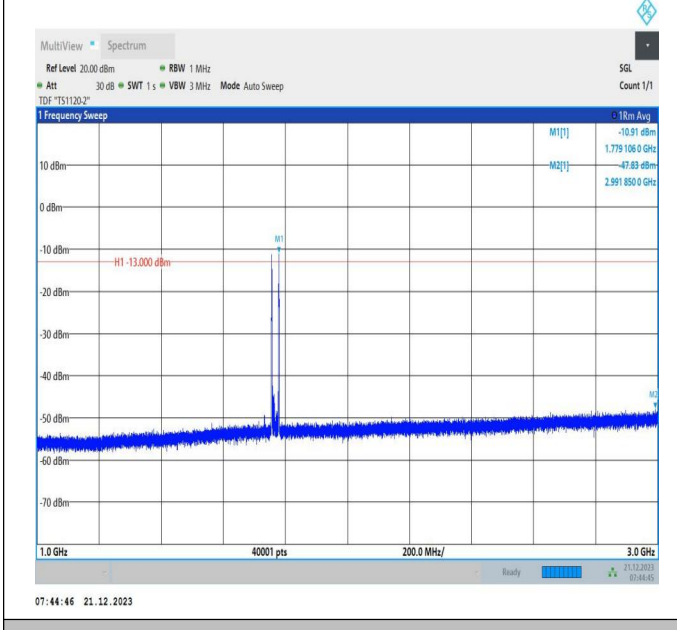
66-66-10MHz-15MHz-16QAM-16QAM-132477-132597-1RB# 0-1RB#74-1000~3000MHz-PASS
