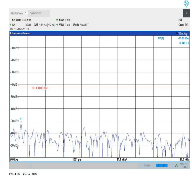
66-66-10MHz-15MHz-16QAM-16QAM-132477-132597-1RB#0-1RB#74-0.009~0.15MHz-PASS
