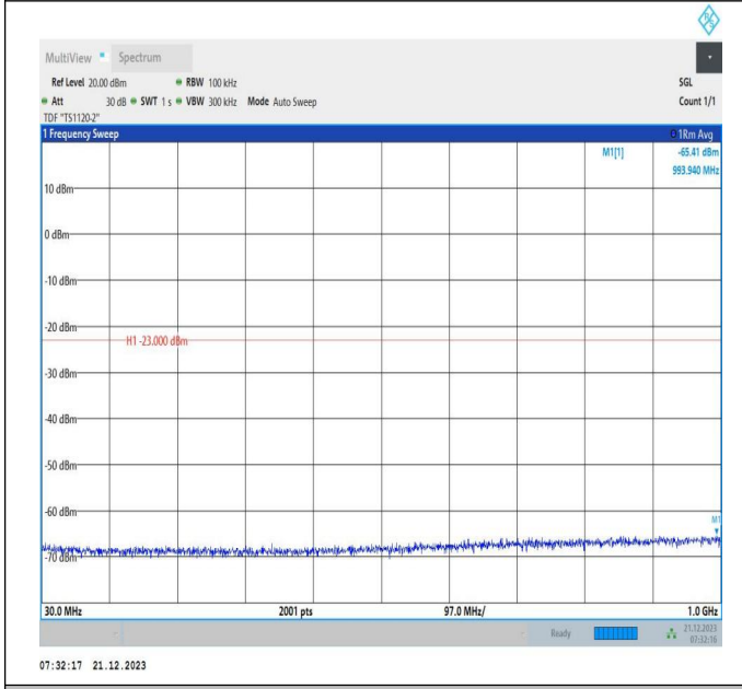
66-66-10MHz-15MHz-16QAM-16QAM-132477-132597-1RB# 49-ORB#0-30~1000MHz-PASS
