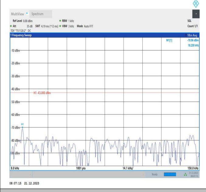
66-66-10MHz-15MHz-64QAM-64QAM-132477-132597-50RB #0-75RB#0-0.009~0.15MHz-PASS
