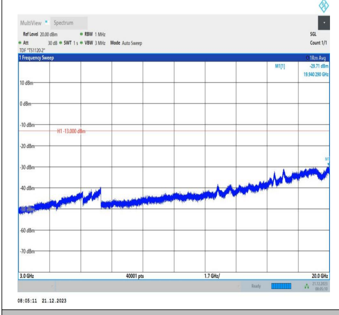
66-66-10MHz-15MHz-16QAM-16QAM-132477-132597-50RB #0-75RB#0-3000~20000MHz-PASS
