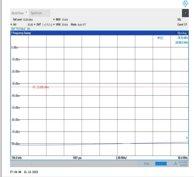
66-66-10MHz-15MHz-64QAM-64QAM-132477-132597-1RB# 49-ORB#0-0.15~30MHz-PASS
