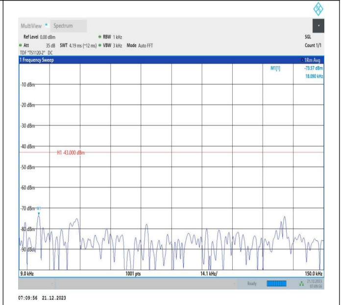
66-66-10MHz-15MHz-64QAM-64QAM-132351-132471-50RB #0-75RB#0-0.009~0.15MHz-PASS
