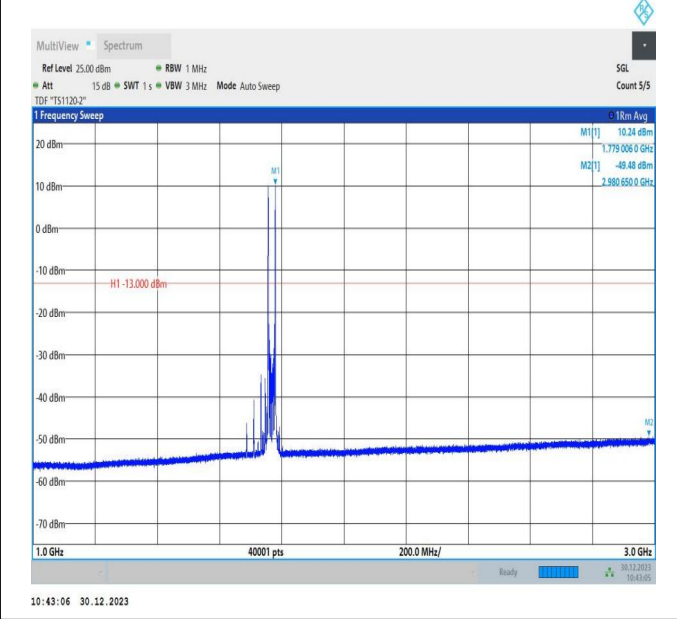
66-66-10MHz-15MHz-64QAM-64QAM-132477-132597-1RB# 0-1RB#74-1000~3000MHz-PASS
