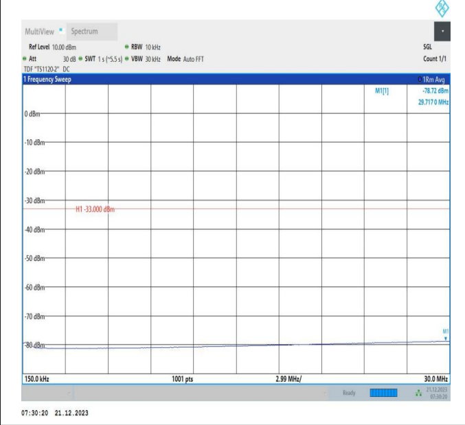
66-66-10MHz-15MHz-64QAM-64QAM-132477-132597-1RB# 0-ORB#0-0.15~30MHz-PASS
