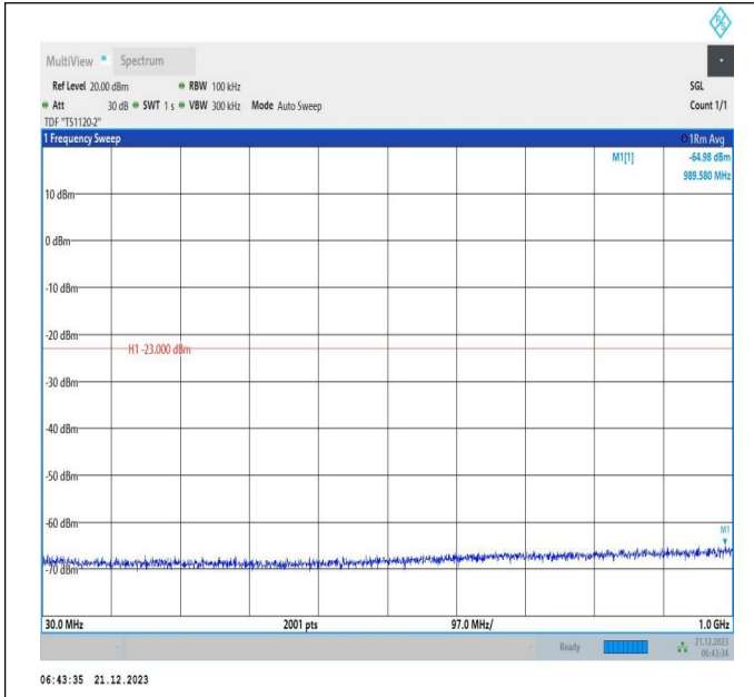
66-66-10MHz-15MHz-16QAM-16QAM-132025-132145-50RB #0-75RB#0-30~1000MHz-PASS
