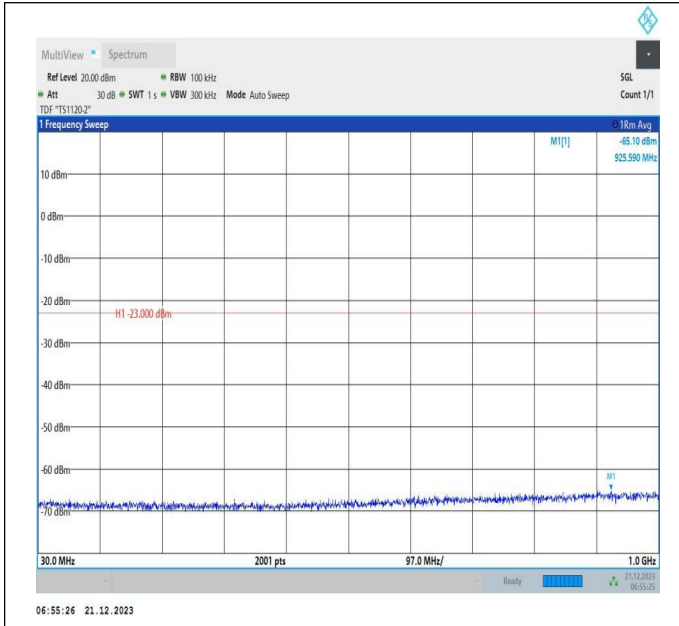
66-66-10MHz-15MHz-QPSK-QPSK-132351-132471-1RB#0-1RB#74-30~1000MHz-PASS
