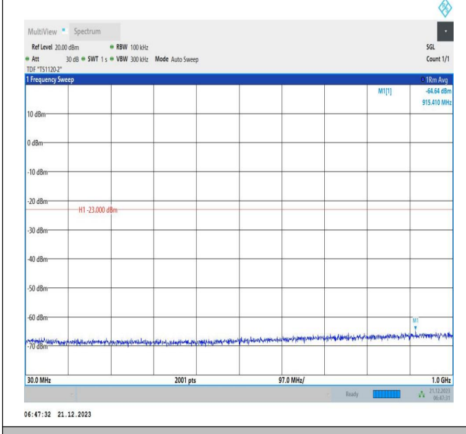
66-66-10MHz-15MHz-QPSK-QPSK-132351-132471-1RB#0-ORB#0-30~1000MHz-PASS
