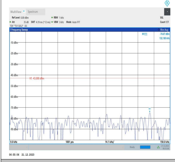
66-66-10MHz-15MHz-QPSK-QPSK-132351-132471-1RB#0- 1RB#74-0.009~0.15MHz-PASS
