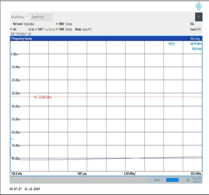
66-66-10MHz-15MHz-QPSK-QPSK-132351-132471-1RB#0-ORB#0-0.15~30MHz-PASS
