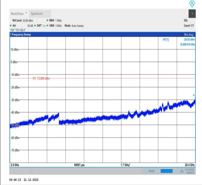
66-66-10MHz-15MHz-64QAM-64QAM-132025-132145-50RB #0-75RB#0-3000~20000MHz-PASS
