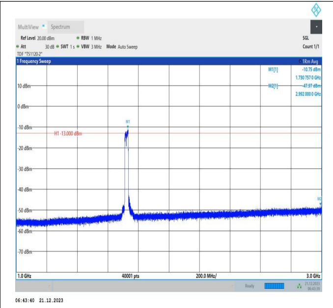
66-66-10MHz-15MHz-16QAM-16QAM-132025-132145-50RB #0-75RB#0-1000~3000MHz-PASS
