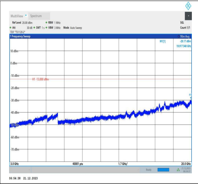
66-66-10MHz-15MHz-64QAM-64QAM-132351-132471-1RB# 49-ORB#0-3000~20000MHz-PASS
