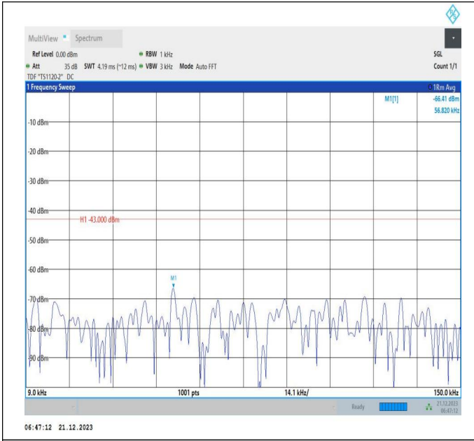
66-66-10MHz-15MHz-QPSK-QPSK-132351-132471-1RB#0-ORB#0-0.009~0.15MHz-PASS
