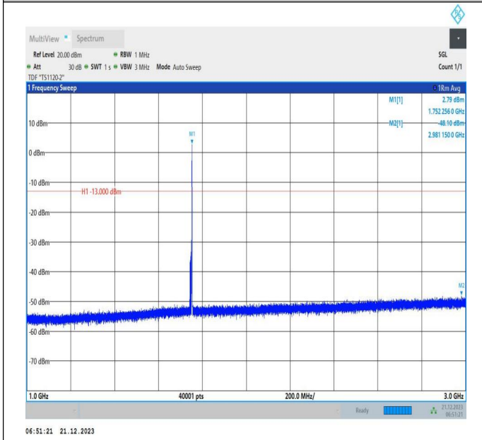
66-66-10MHz-15MHz-QPSK-QPSK-132351-132471-1RB#49 -ORB#0-1000~3000MHz-PASS
