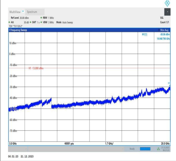
66-66-10MHz-15MHz-16QAM-16QAM-132025-132145-1RB# 0-1RB#74-3000~20000MHz-PASS
