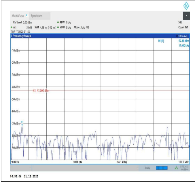
66-66-10MHz-15MHz-64QAM-64QAM-132351-132471-1RB# 0-1RB#74-0.009~0.15MHz-PASS
