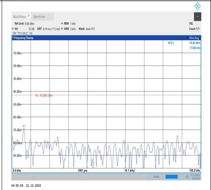
66-66-10MHz-15MHz-16QAM-16QAM-132351-132471-1RB#0-1RB#74-0.009~0.15MHz-PASS
