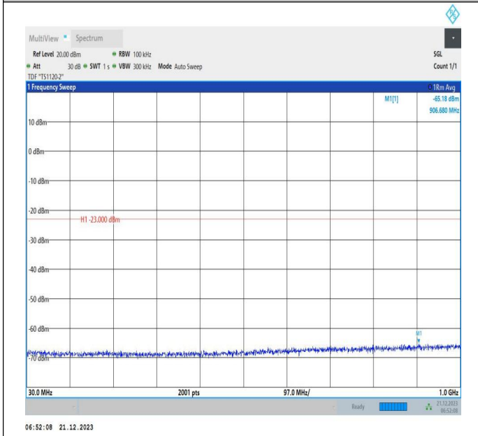
66-66-10MHz-15MHz-16QAM-16QAM-132351-132471-1RB# 49-ORB#0-30~1000MHz-PASS
