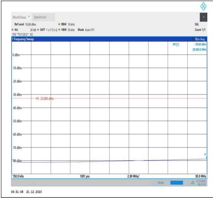
66-66-10MHz-15MHz-16QAM-16QAM-132025-132145-1RB# 0-1RB#74-0.15~30MHz-PASS
