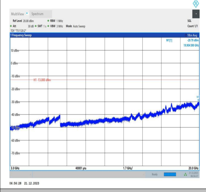
66-66-10MHz-15MHz-16QAM-16QAM-132351-132471-1RB# 0-1RB#74-3000~20000MHz-PASS
