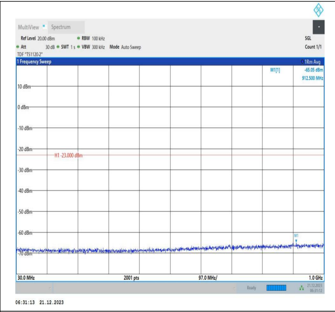
66-66-10MHz-15MHz-16QAM-16QAM-132025-132145-1RB# 0-1RB#74-30~1000MHz-PASS
