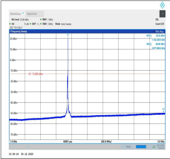
66-66-10MHz-15MHz-64QAM-64QAM-132351-132471-1RB# 49-ORB#0-1000~3000MHz-PASS
