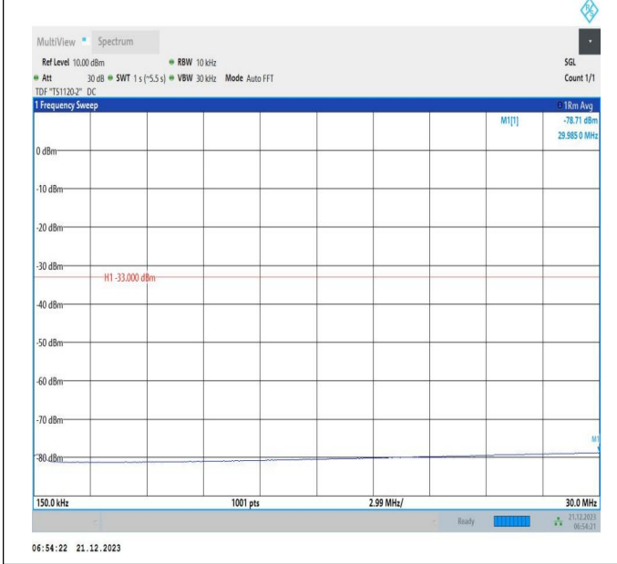
66-66-10MHz-15MHz-64QAM-64QAM-132351-132471-1RB# 49-ORB#0-0.15~30MHz-PASS
