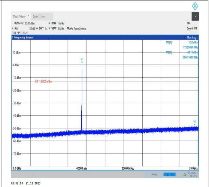
66-66-10MHz-15MHz-16QAM-16QAM-132351-132471-1RB# 49-ORB#0-1000~3000MHz-PASS
