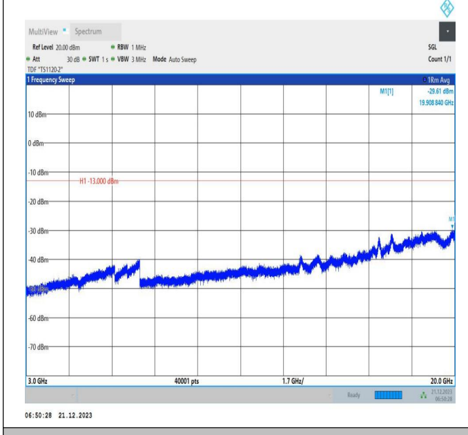
66-66-10MHz-15MHz-64QAM-64QAM-132351-132471-1RB# 0-ORB#0-3000~20000MHz-PASS
