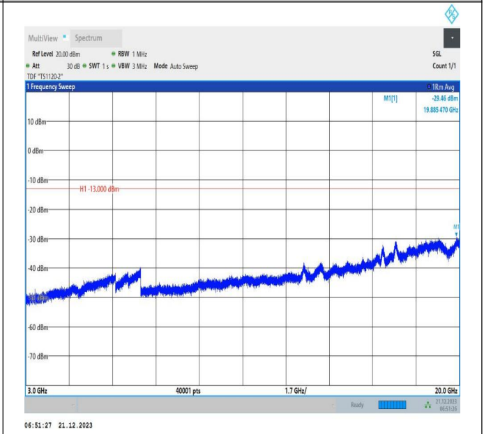
66-66-10MHz-15MHz-QPSK-QPSK-132351-132471-1RB#49 -ORB#0-3000~20000MHz-PASS
