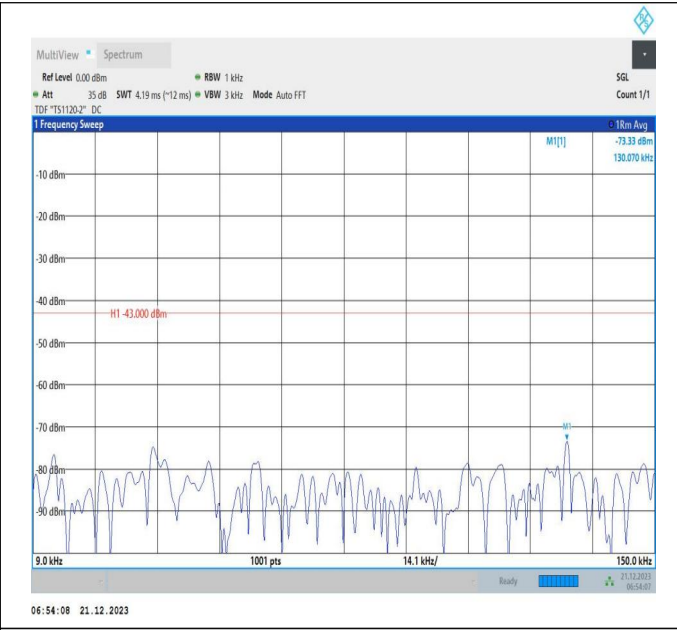
66-66-10MHz-15MHz-64QAM-64QAM-132351-132471-1RB# 49-ORB#0-0.009~0.15MHz-PASS
