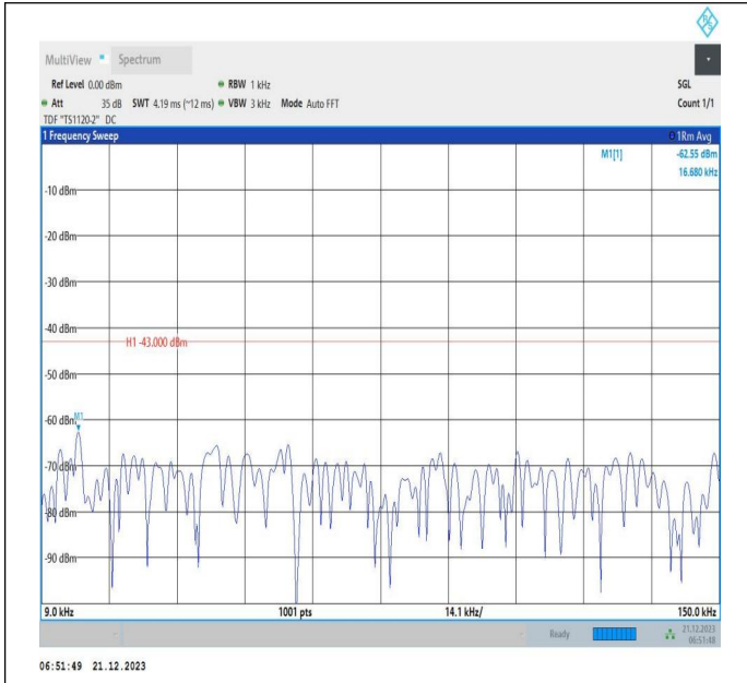
66-66-10MHz-15MHz-16QAM-16QAM-132351-132471-1RB# 49-ORB#0-0.009~0.15MHz-PASS
