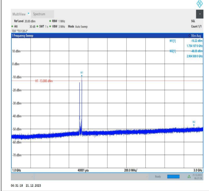
66-66-10MHz-15MHz-16QAM-16QAM-132025-132145-1RB# 0-1RB#74-1000~3000MHz-PASS
