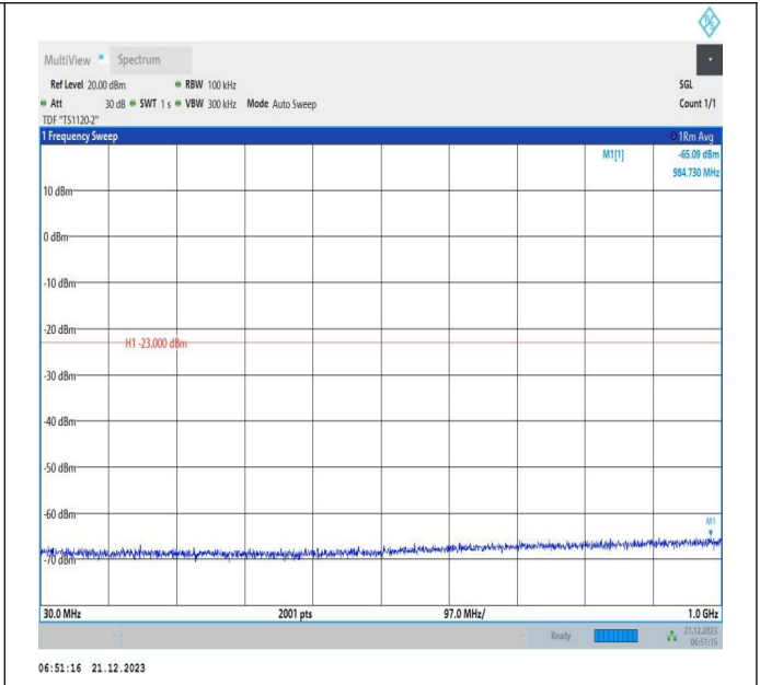
66-66-10MHz-15MHz-QPSK-QPSK-132351-132471-1RB#49 -ORB#0-30~1000MHz-PASS
