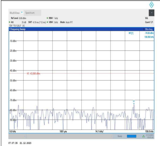
66-66-10MHz-15MHz-16QAM-16QAM-132351-132471-50RB #0-75RB#0-0.009~0.15MHz-PASS
