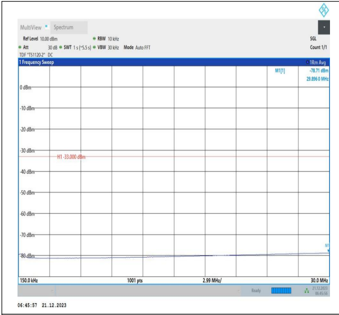
66-66-10MHz-15MHz-64QAM-64QAM-132025-132145-50RB #0-75RB#0-0.15~30MHz-PASS
