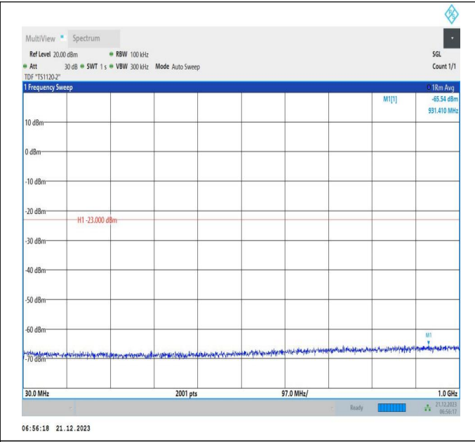
66-66-10MHz-15MHz-16QAM-16QAM-132351-132471-1RB# 0-1RB#74-30~1000MHz-PASS
