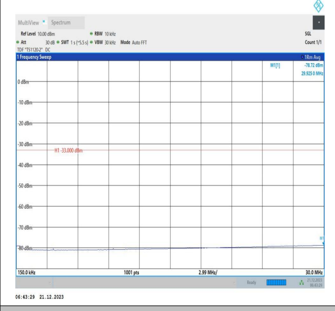
66-66-10MHz-15MHz-16QAM-16QAM-132025-132145-50RB#0-75RB#0-0.15~30MHz-PASS
