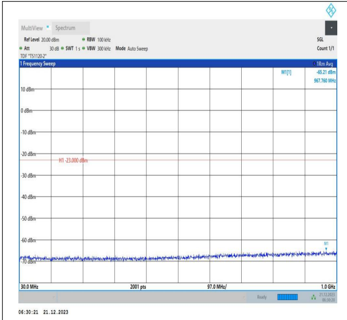
66-66-10MHz-15MHz-QPSK-QPSK-132025-132145-1RB#0-1RB#74-30~1000MHz-PASS
