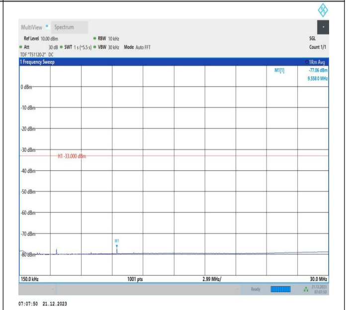
66-66-10MHz-15MHz-16QAM-16QAM-132351-132471-50RB #0-75RB#0-0.15~30MHz-PASS
