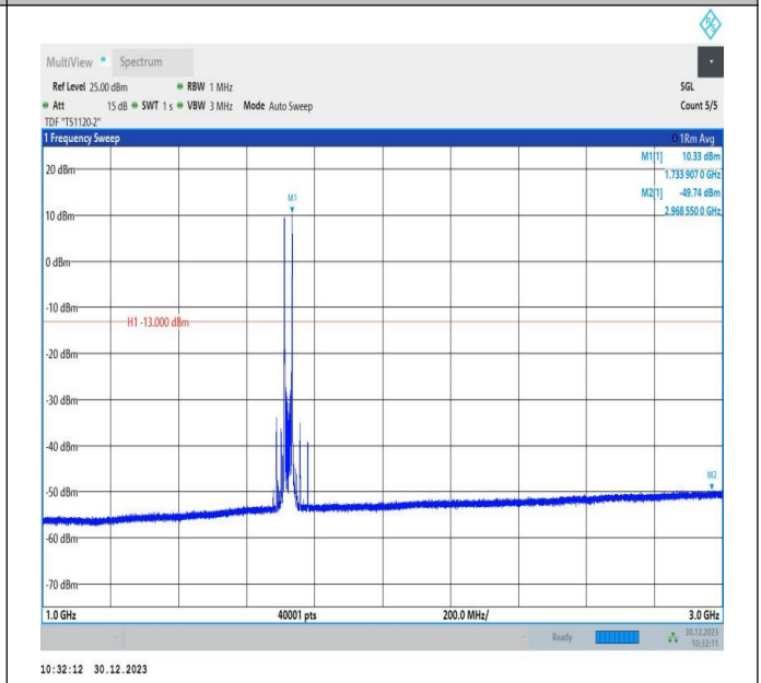
66-66-10MHz-15MHz-64QAM-64QAM-132025-132145-1RB# 0-1RB#74-1000~3000MHz-PASS
