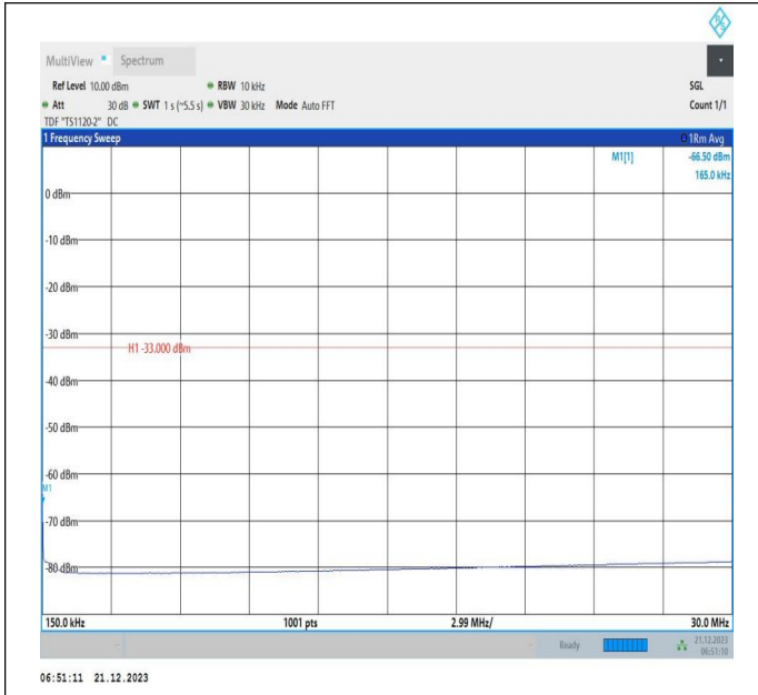
66-66-10MHz-15MHz-QPSK-QPSK-132351-132471-1RB#49 -ORB#0-0.15~30MHz-PASS
