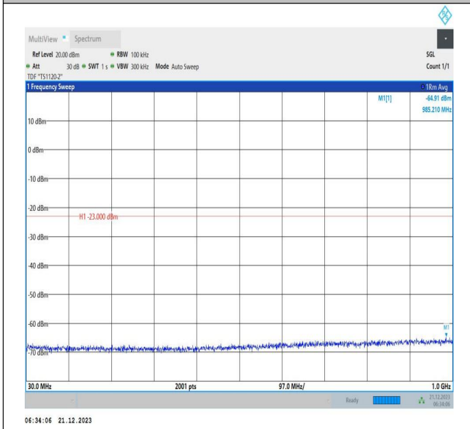
66-66-10MHz-15MHz-64QAM-64QAM-132025-132145-1RB# 0-1RB#74-30~1000MHz-PASS
