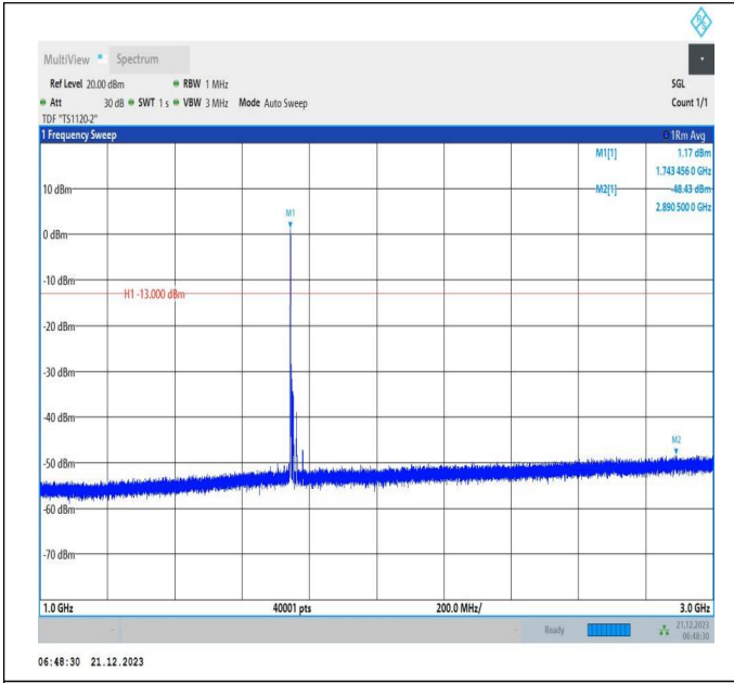
66-66-10MHz-15MHz-16QAM-16QAM-132351-132471-1RB# 0-ORB#0-1000~3000MHz-PASS
