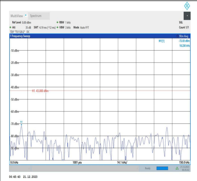
66-66-10MHz-15MHz-64QAM-64QAM-132025-132145-50RB #0-75RB#0-0.009~0.15MHz-PASS
