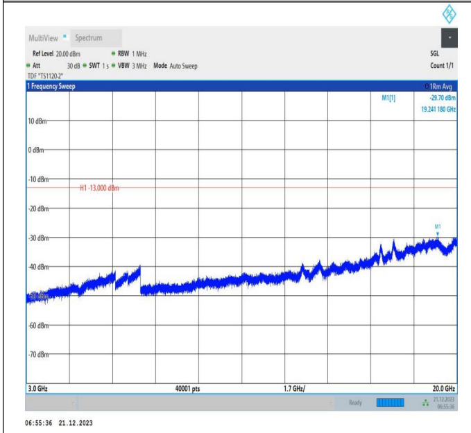
66-66-10MHz-15MHz-QPSK-QPSK-132351-132471-1RB#0-1RB#74-3000~20000MHz-PASS
