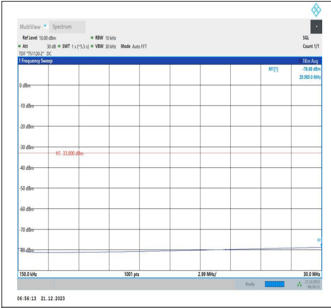
66-66-10MHz-15MHz-16QAM-16QAM-132351-132471-1RB# 0-1RB#74-0.15~30MHz-PASS
