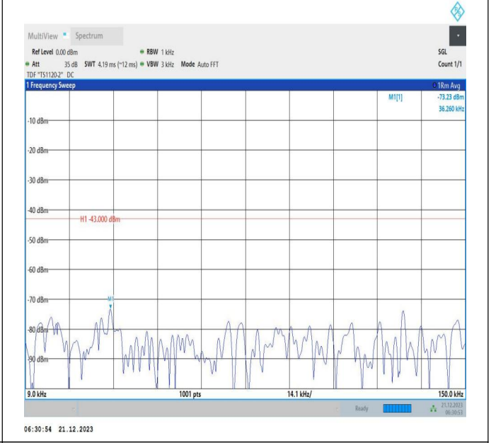
66-66-10MHz-15MHz-16QAM-16QAM-132025-132145-1RB#0-1RB#74-0.009~0.15MHz-PASS
