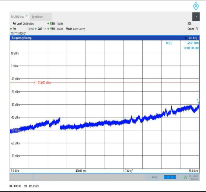
66-66-10MHz-15MHz-16QAM-16QAM-132351-132471-1RB# 0-ORB#0-3000~20000MHz-PASS
