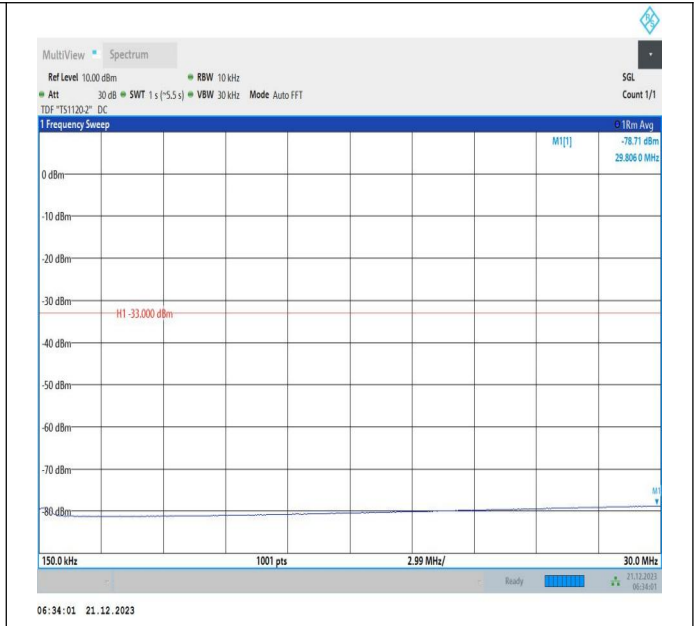
66-66-10MHz-15MHz-64QAM-64QAM-132025-132145-1RB# 0-1RB#74-0.15~30MHz-PASS
