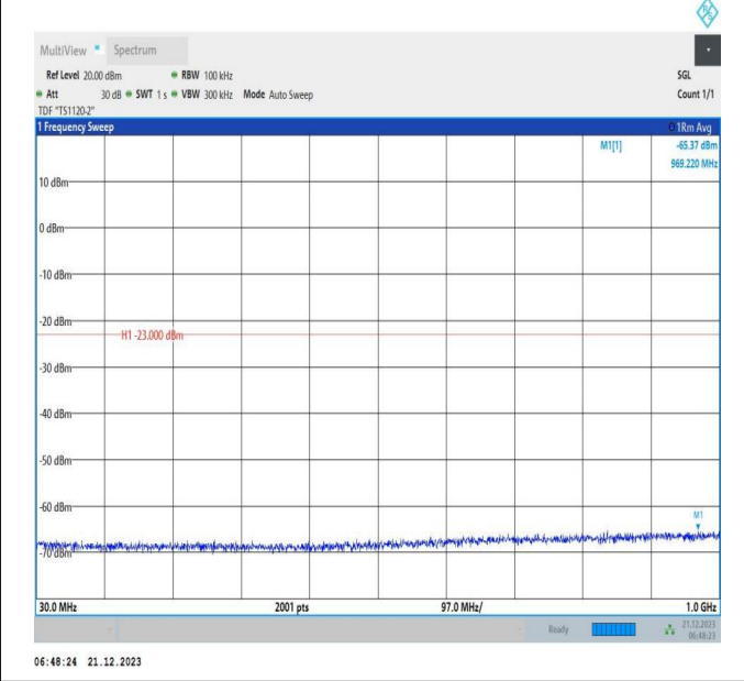
66-66-10MHz-15MHz-16QAM-16QAM-132351-132471-1RB#0-0RB#0-30~1000MHz-PASS
