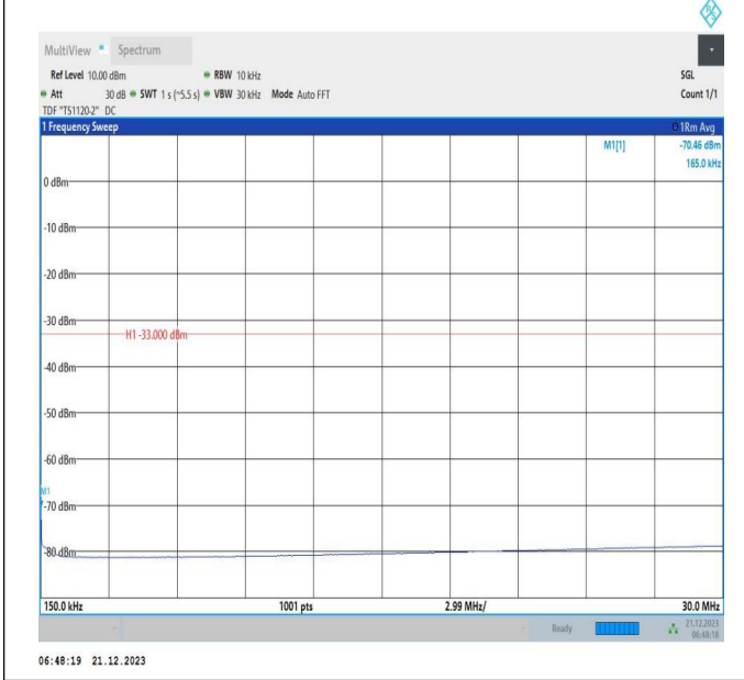
66-66-10MHz-15MHz-16QAM-16QAM-132351-132471-1RB#0-0RB#0-0.15~30MHz-PASS
