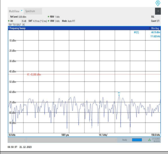
66-66-10MHz-15MHz-QPSK-QPSK-132351-132471-1RB#49 -ORB#0-0.009~0.15MHz-PASS
