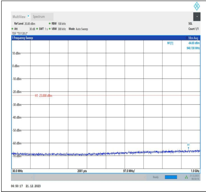
66-66-10MHz-15MHz-64QAM-64QAM-132351-132471-1RB# 0-ORB#0-30~1000MHz-PASS
