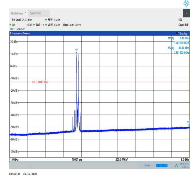
66-66-10MHz-15MHz-64QAM-64QAM-132351-132471-1RB# 0-1RB#74-1000~3000MHz-PASS
