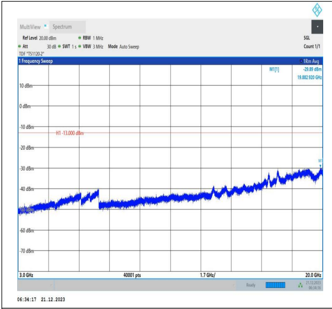
66-66-10MHz-15MHz-64QAM-64QAM-132025-132145-1RB#0-1RB#74-3000~20000MHz-PASS
