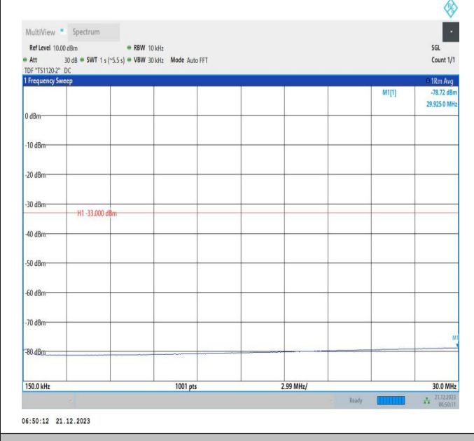
66-66-10MHz-15MHz-64QAM-64QAM-132351-132471-1RB# 0-ORB#0-0.15~30MHz-PASS
