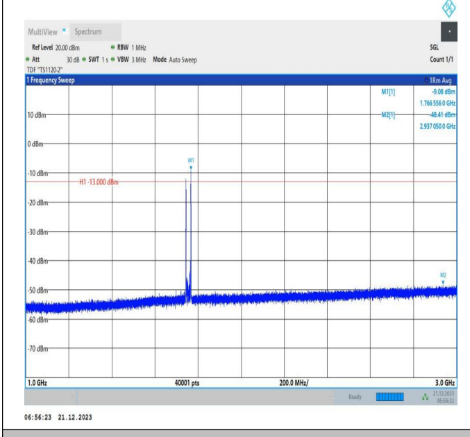
66-66-10MHz-15MHz-16QAM-16QAM-132351-132471-1RB# 0-1RB#74-1000~3000MHz-PASS
