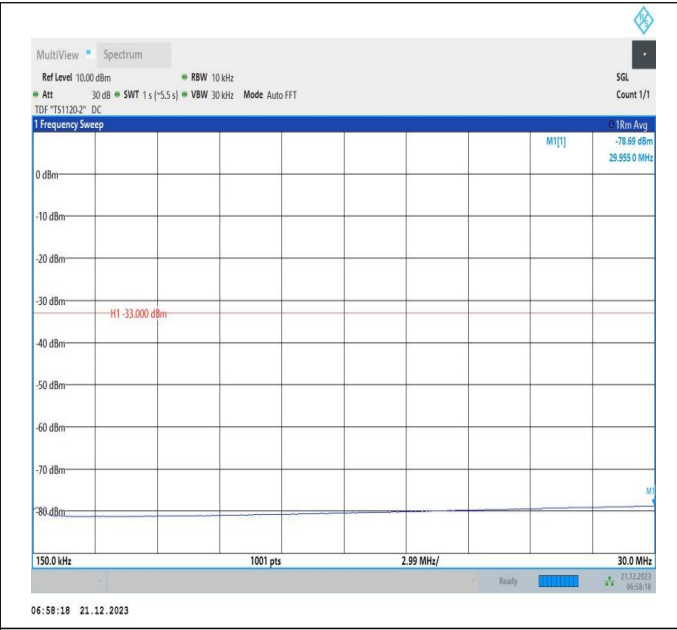
66-66-10MHz-15MHz-64QAM-64QAM-132351-132471-1RB# 0-1RB#74-0.15~30MHz-PASS
