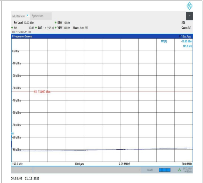
66-66-10MHz-15MHz-16QAM-16QAM-132351-132471-1RB# 49-ORB#0-0.15~30MHz-PASS
