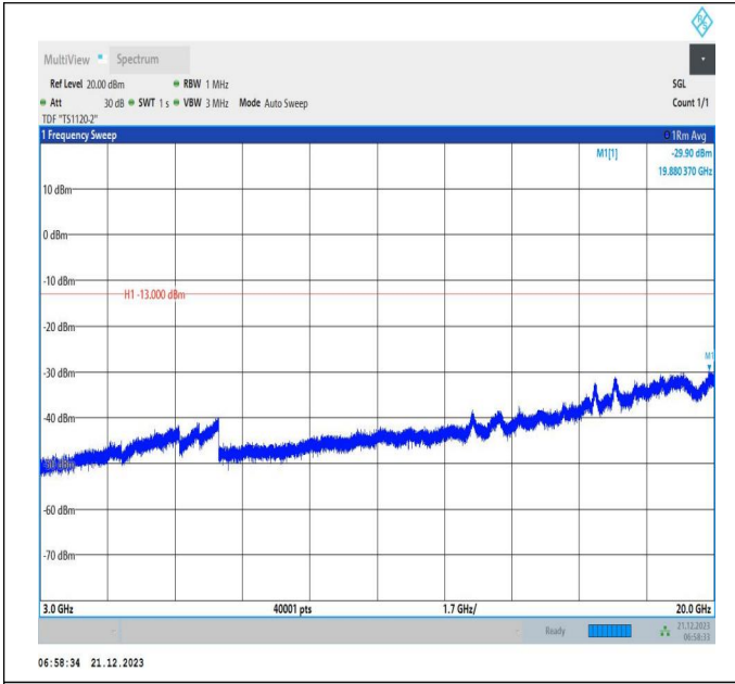
66-66-10MHz-15MHz-64QAM-64QAM-132351-132471-1RB#0-1RB#74-3000~20000MHz-PASS
