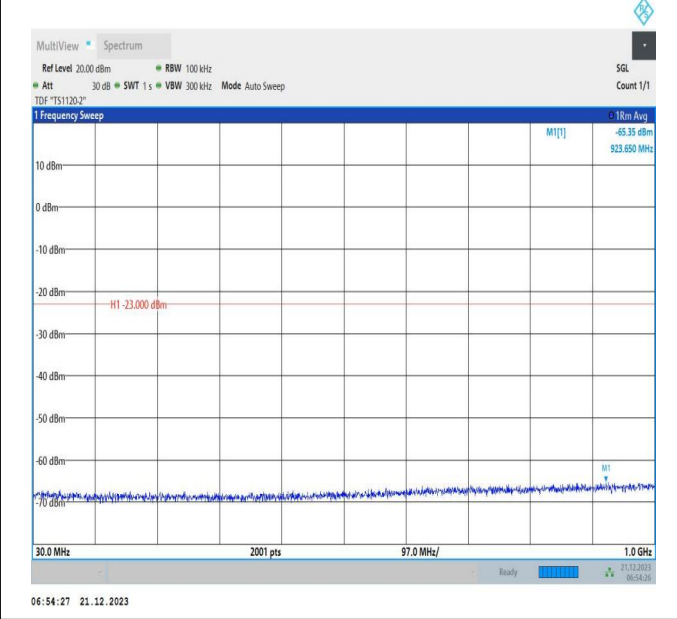
66-66-10MHz-15MHz-64QAM-64QAM-132351-132471-1RB# 49-ORB#0-30~1000MHz-PASS
