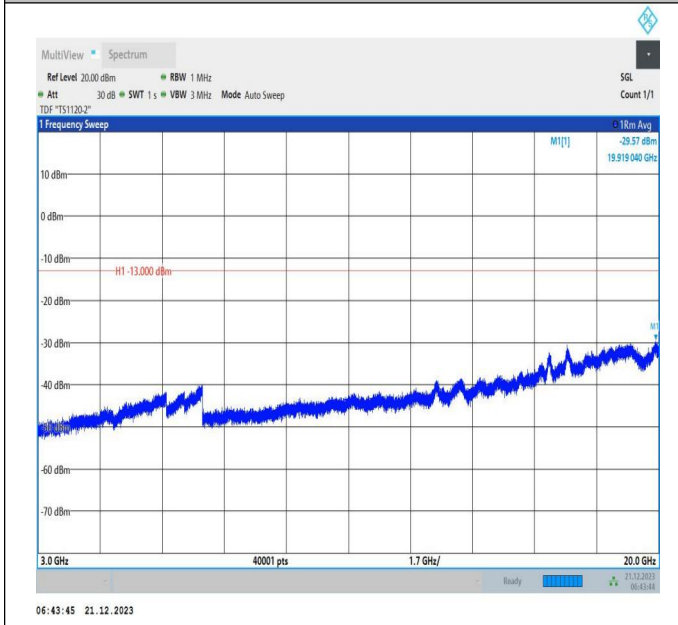
66-66-10MHz-15MHz-16QAM-16QAM-132025-132145-50RB #0-75RB#0-3000~20000MHz-PASS
