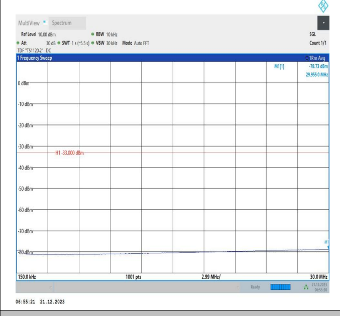
66-66-10MHz-15MHz-QPSK-QPSK-132351-132471-1RB#0- 1RB#74-0.15~30MHz-PASS
