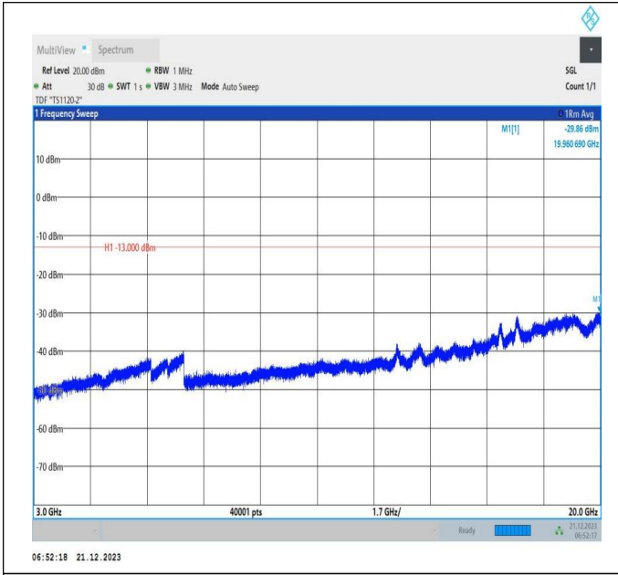
66-66-10MHz-15MHz-16QAM-16QAM-132351-132471-1RB# 49-ORB#0-3000~20000MHz-PASS
