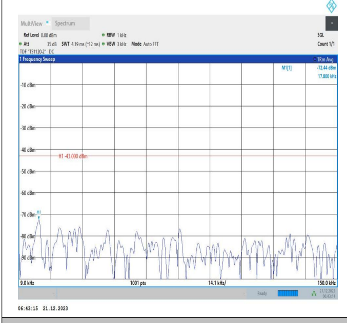
66-66-10MHz-15MHz-16QAM-16QAM-132025-132145-50RB#0-75RB#0-0.009~0.15MHz-PASS
