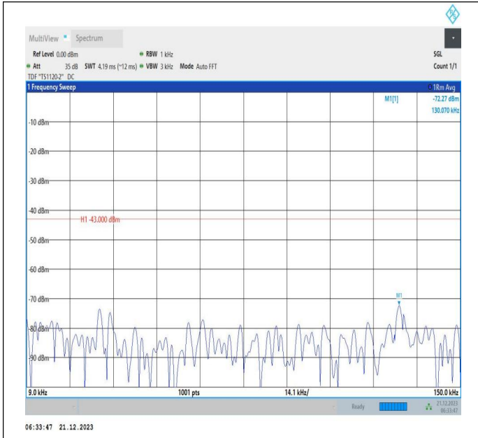
66-66-10MHz-15MHz-64QAM-64QAM-132025-132145-1RB# 0-1RB#74-0.009~0.15MHz-PASS
