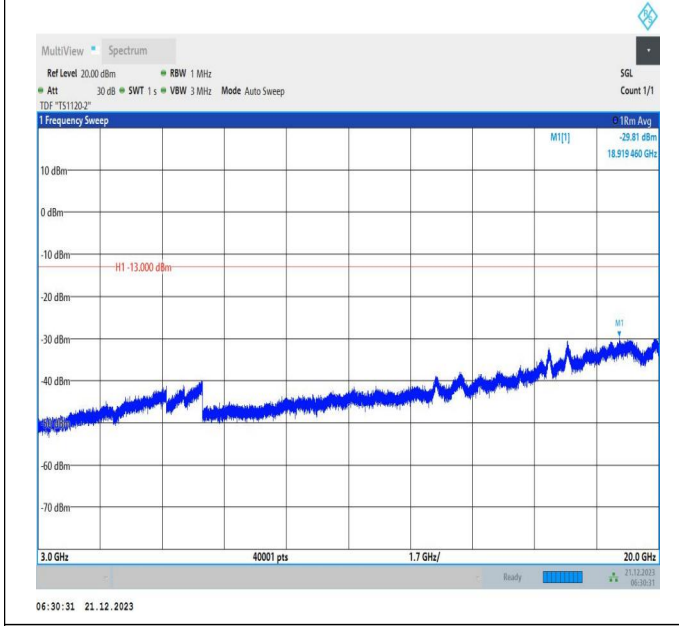
66-66-10MHz-15MHz-QPSK-QPSK-132025-132145-1RB#0-1RB#74-3000~20000MHz-PASS
