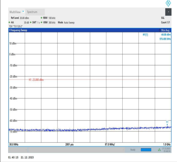
66-66-5MHz-20MHz-16QAM-16QAM-132328-132472-1RB#0 -ORB#0-30~1000MHz-PASS
