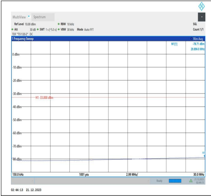
66-66-5MHz-20MHz-64QAM-64QAM-132328-132472-25RB# 0-100RB#0-0.15~30MHz-PASS
