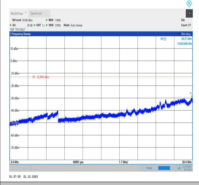
66-66-5MHz-20MHz-64QAM-64QAM-132027-132171-25RB# 0-100RB#0-3000~20000MHz-PASS
