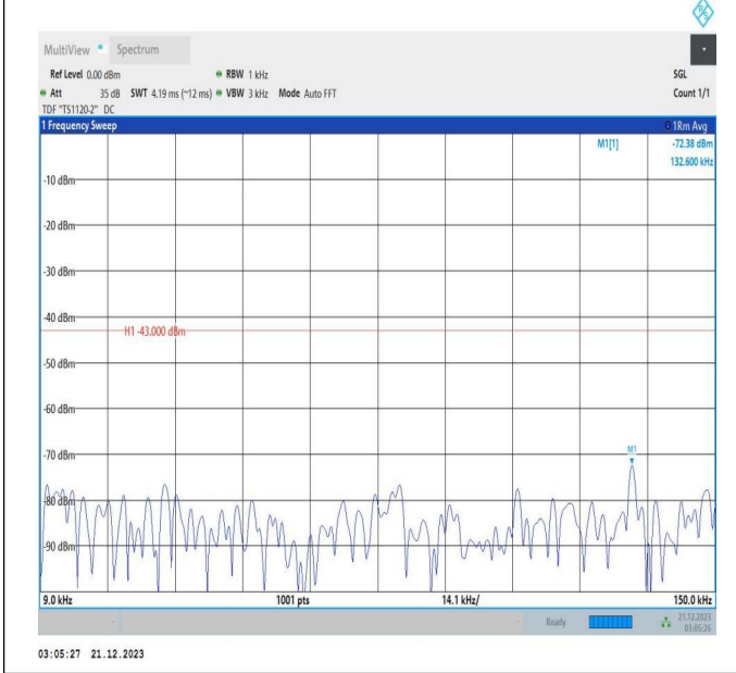
66-66-5MHz-20MHz-64QAM-64QAM-132428-132572-1RB#0 -ORB#0-0.009~0.15MHz-PASS
