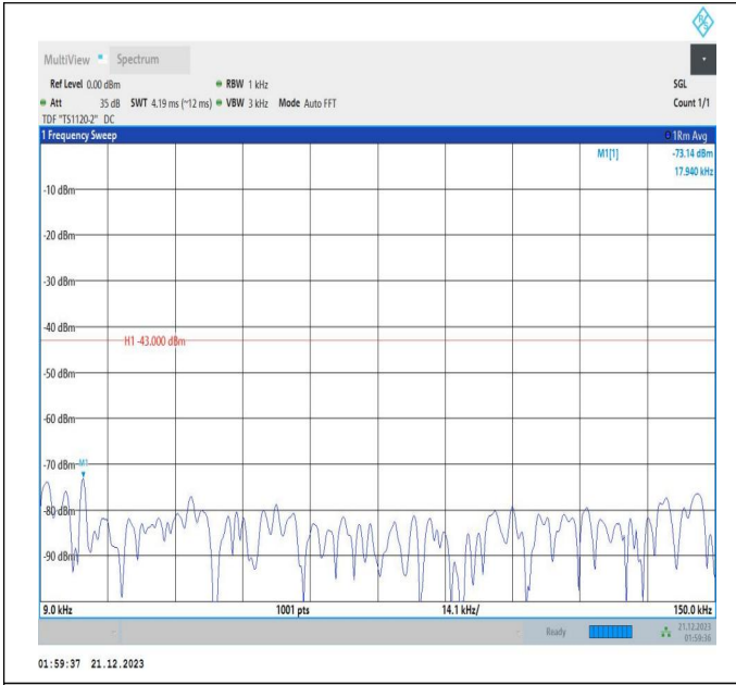
66-66-5MHz-20MHz-16QAM-16QAM-132328-132472-1RB#2 4-ORB#0-0.009~0.15MHz-PASS
