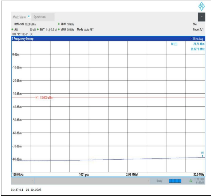
66-66-5MHz-20MHz-64QAM-64QAM-132027-132171-25RB# 0-100RB#0-0.15~30MHz-PASS
