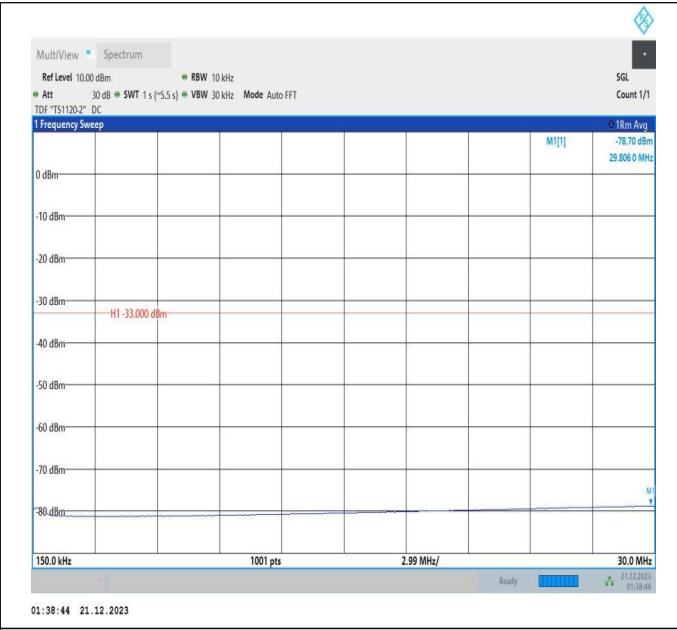
66-66-5MHz-20MHz-QPSK-QPSK-132328-132472-1RB#0-0 RB#0-0.15~30MHz-PASS
