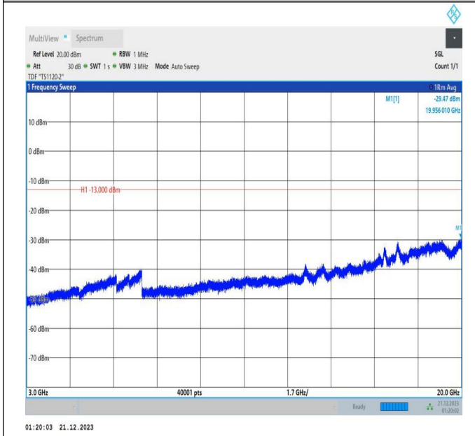
66-66-5MHz-20MHz-16QAM-16QAM-132027-132171-25RB# 0-100RB#0-3000~20000MHz-PASS
