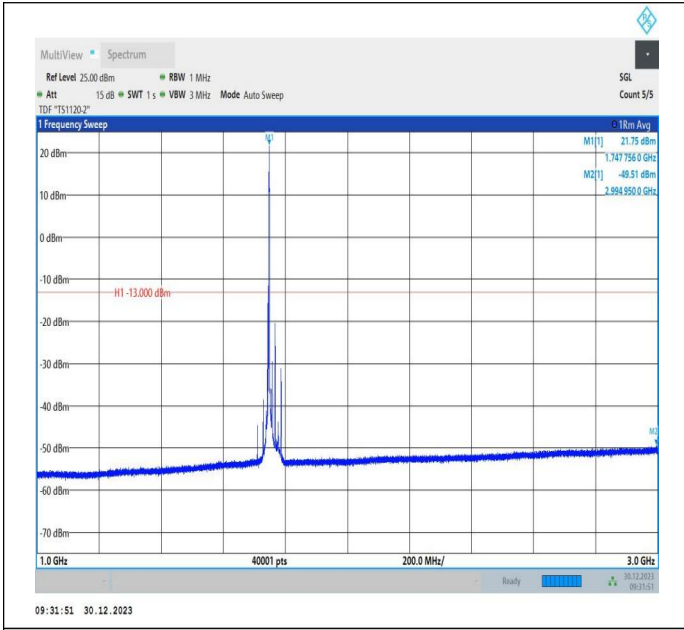
66-66-5MHz-20MHz-64QAM-64QAM-132328-132472-1RB#2 4-ORB#0-1000~3000MHz-PASS
