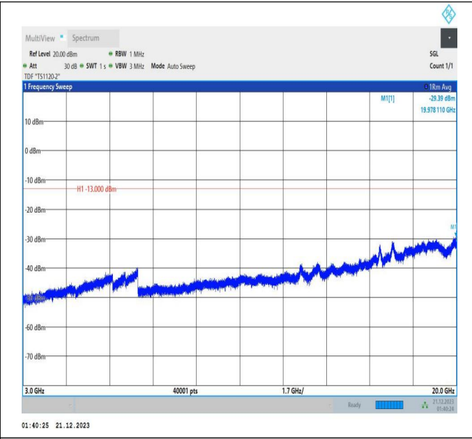
66-66-5MHz-20MHz-16QAM-16QAM-132328-132472-1RB#0 -ORB#0-3000~20000MHz-PASS
