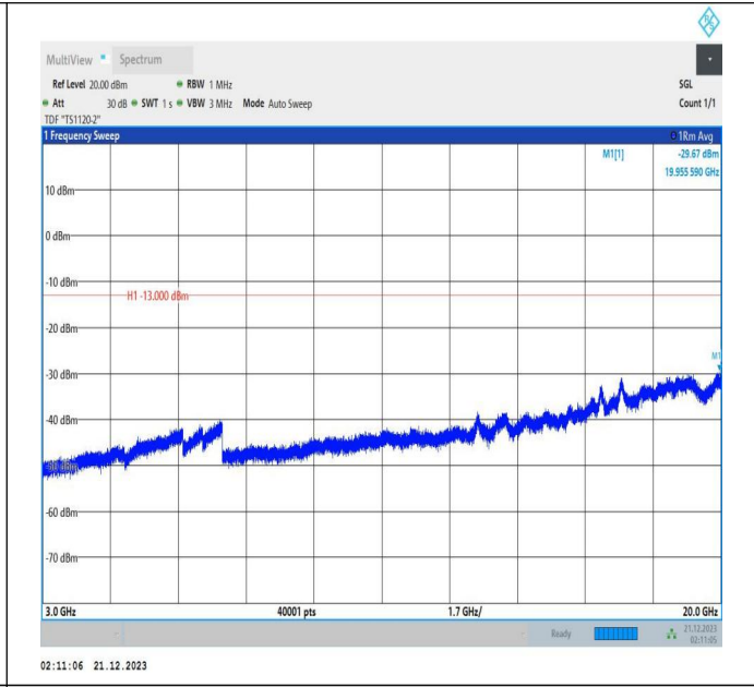
66-66-5MHz-20MHz-64QAM-64QAM-132328-132472-1RB#2 4-ORB#0-3000~20000MHz-PASS
