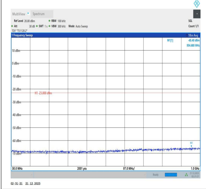
66-66-5MHz-20MHz-64QAM-64QAM-132328-132472-1RB#0 -1RB#99-30~1000MHz-PASS
