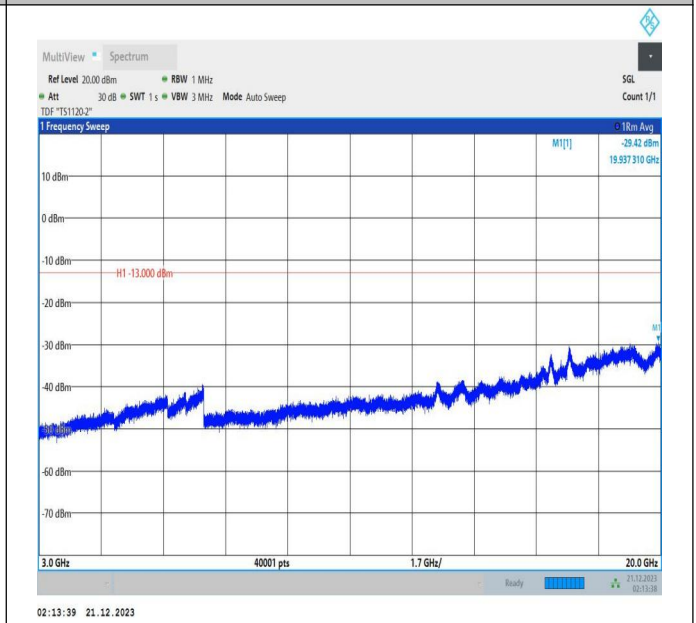
66-66-5MHz-20MHz-16QAM-16QAM-132328-132472-1RB#0 -1RB#99-3000~20000MHz-PASS
