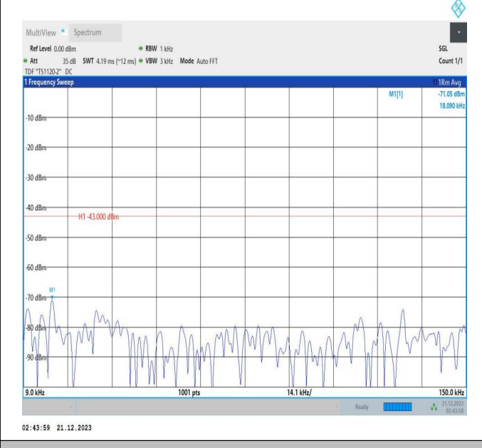
66-66-5MHz-20MHz-64QAM-64QAM-132328-132472-25RB# 0-100RB#0-0.009~0.15MHz-PASS
