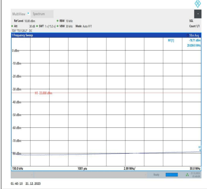
66-66-5MHz-20MHz-16QAM-16QAM-132328-132472-1RB#0 -ORB#0-0.15~30MHz-PASS
