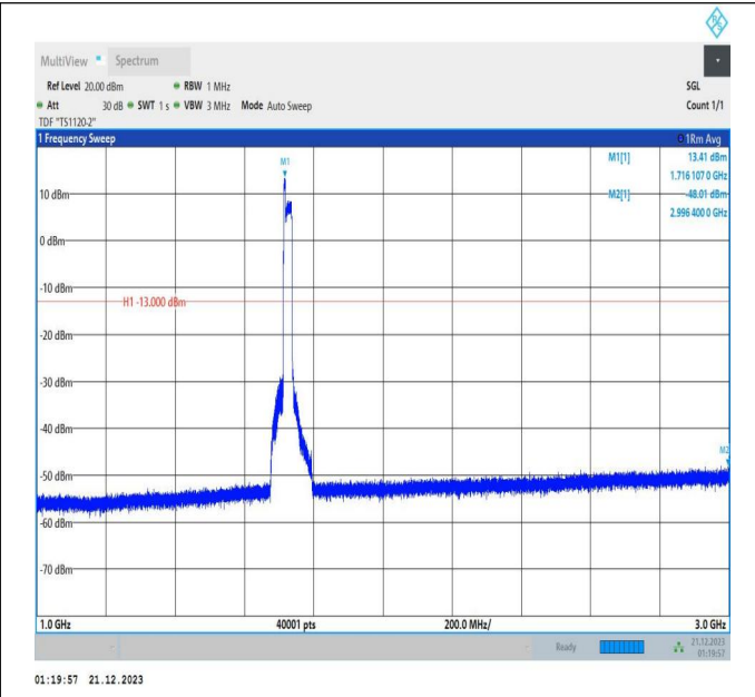
66-66-5MHz-20MHz-16QAM-16QAM-132027-132171-25RB# 0-100RB#0-1000~3000MHz-PASS
