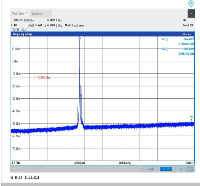
66-66-5MHz-20MHz-QPSK-QPSK-132328-132472-1RB#24-ORB#0-1000~3000MHz-PASS
