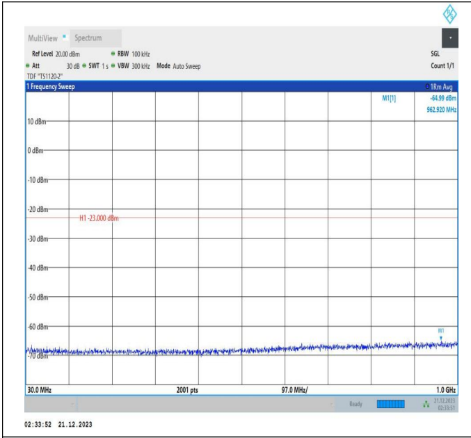
66-66-5MHz-20MHz-16QAM-16QAM-132328-132472-25RB# 0-100RB#0-30~1000MHz-PASS
