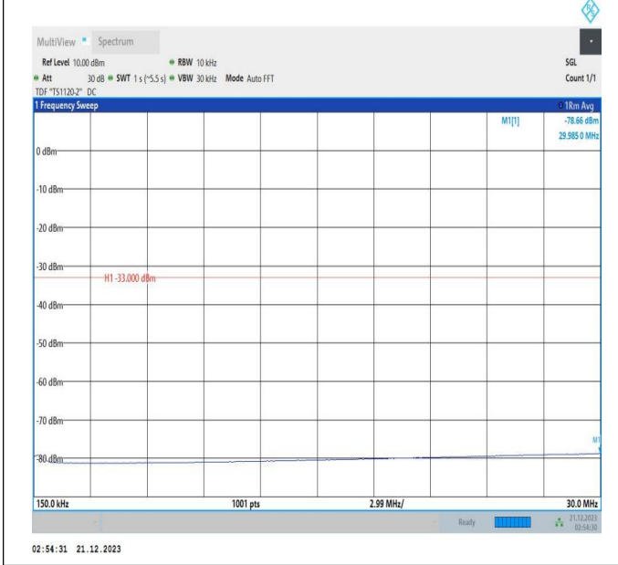
66-66-5MHz-20MHz-16QAM-16QAM-132428-132572-1RB#0 -ORB#0-0.15~30MHz-PASS
