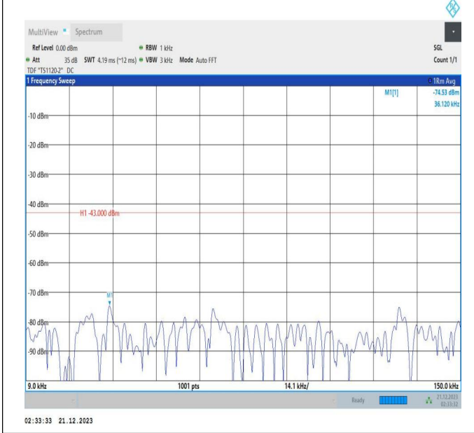
66-66-5MHz-20MHz-16QAM-16QAM-132328-132472-25RB#0-100RB#0-0.009~0.15MHz-PASS
