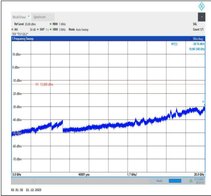
66-66-5MHz-20MHz-64QAM-64QAM-132328-132472-1RB#0-1RB#99-3000~20000MHz-PASS
