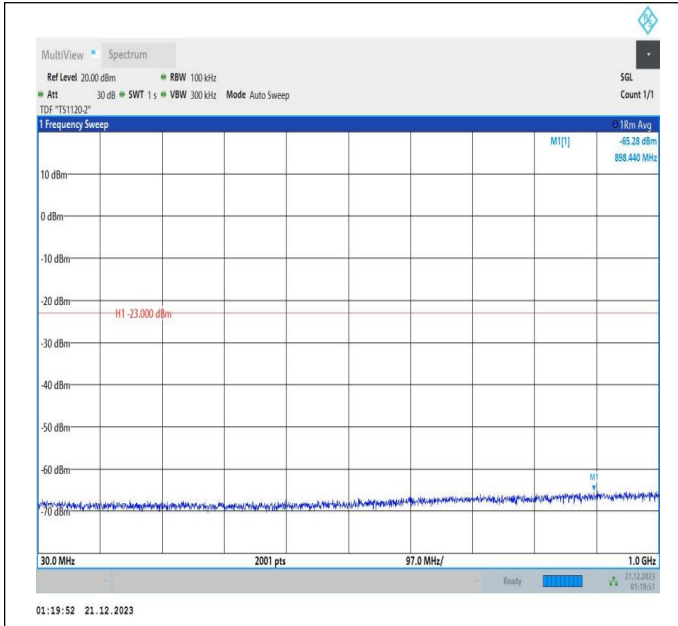
66-66-5MHz-20MHz-16QAM-16QAM-132027-132171-25RB# 0-100RB#0-30~1000MHz-PASS
