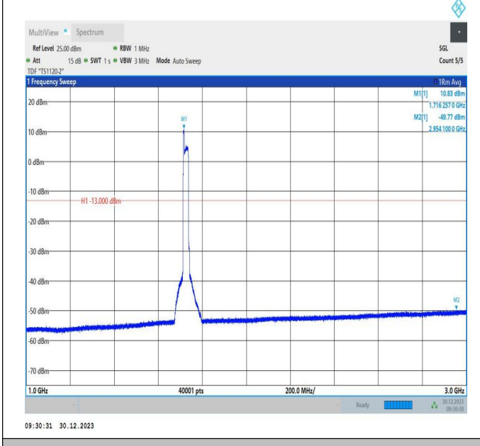
66-66-5MHz-20MHz-64QAM-64QAM-132027-132171-25RB# 0-100RB#0-1000~3000MHz-PASS
