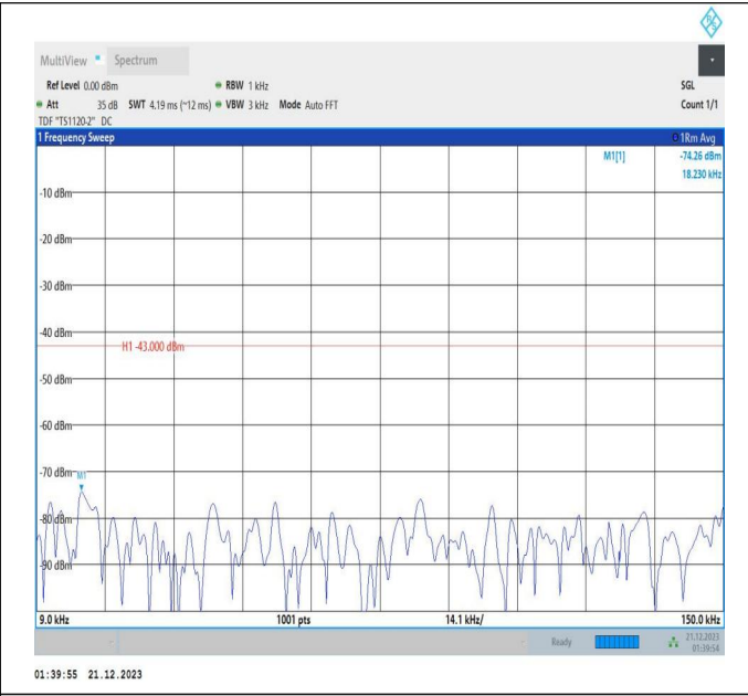
66-66-5MHz-20MHz-16QAM-16QAM-132328-132472-1RB#0 -ORB#0-0.009~0.15MHz-PASS
