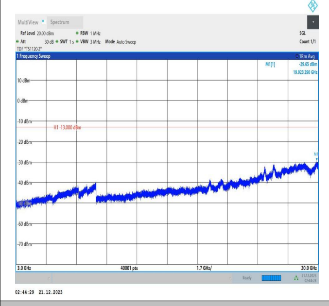
66-66-5MHz-20MHz-64QAM-64QAM-132328-132472-25RB# 0-100RB#0-3000~20000MHz-PASS
