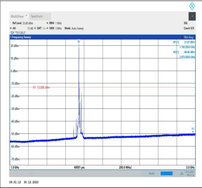
66-66-5MHz-20MHz-64QAM-64QAM-132328-132472-1RB#0 -ORB#0-1000~3000MHz-PASS
