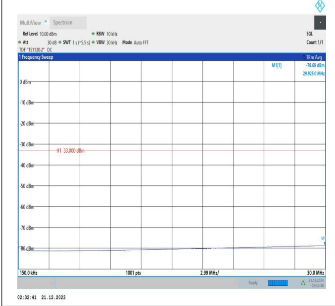
66-66-5MHz-20MHz-QPSK-QPSK-132328-132472-25RB#0-100RB#0-0.15~30MHz-PASS
