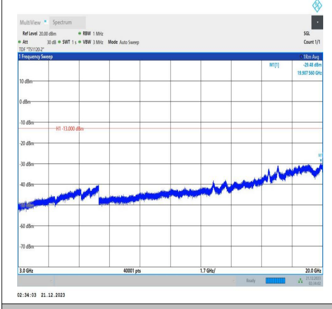
66-66-5MHz-20MHz-16QAM-16QAM-132328-132472-25RB# 0-100RB#0-3000~20000MHz-PASS
