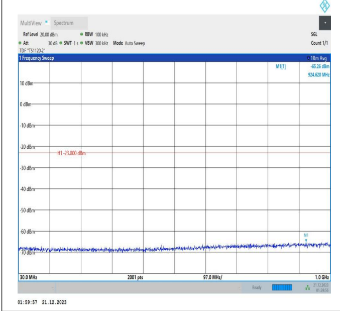
66-66-5MHz-20MHz-16QAM-16QAM-132328-132472-1RB#2 4-ORB#0-30~1000MHz-PASS
