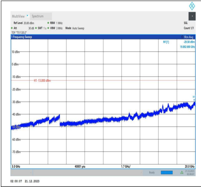
66-66-5MHz-20MHz-16QAM-16QAM-132328-132472-1RB#2 4-ORB#0-3000~20000MHz-PASS
