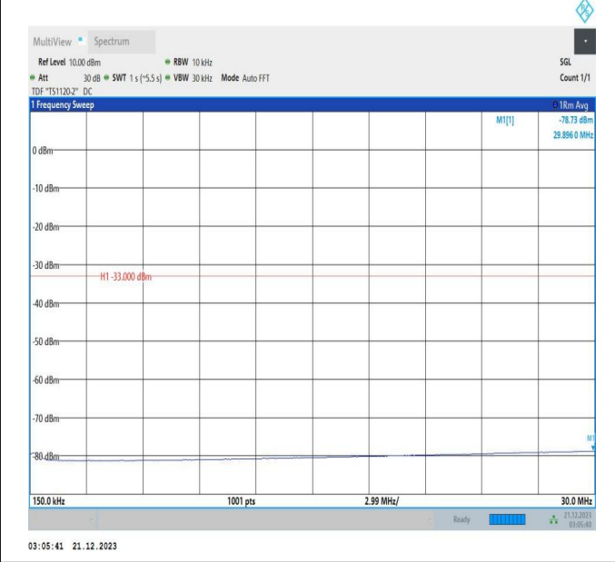
66-66-5MHz-20MHz-64QAM-64QAM-132428-132572-1RB#0 -ORB#0-0.15~30MHz-PASS
