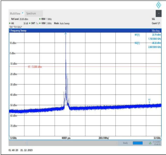
66-66-5MHz-20MHz-16QAM-16QAM-132328-132472-1RB#0 -ORB#0-1000~3000MHz-PASS
