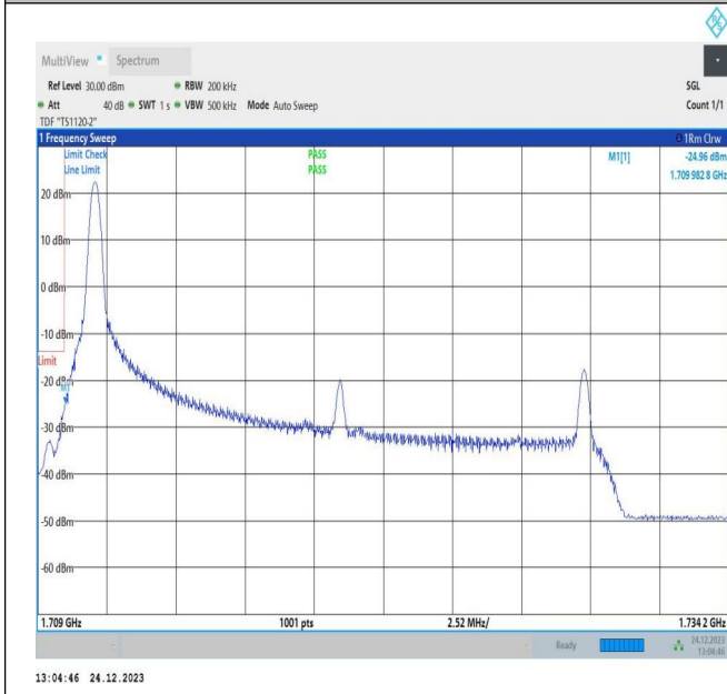
20MHz-5MHz_QPSK@QPSK-QPSK@QPSK_132072-132189_1RB#0@100RB#0-0RB#0@25RB#0
