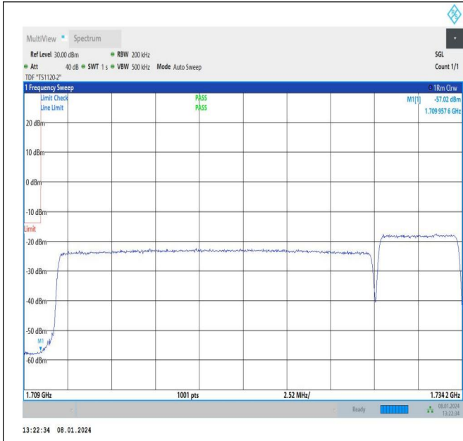
20MHz-5MHz_QPSK@QPSK-QPSK@QPSK_132072-132189_100RB#0@100RB#0-25RB#0@25RB#0
