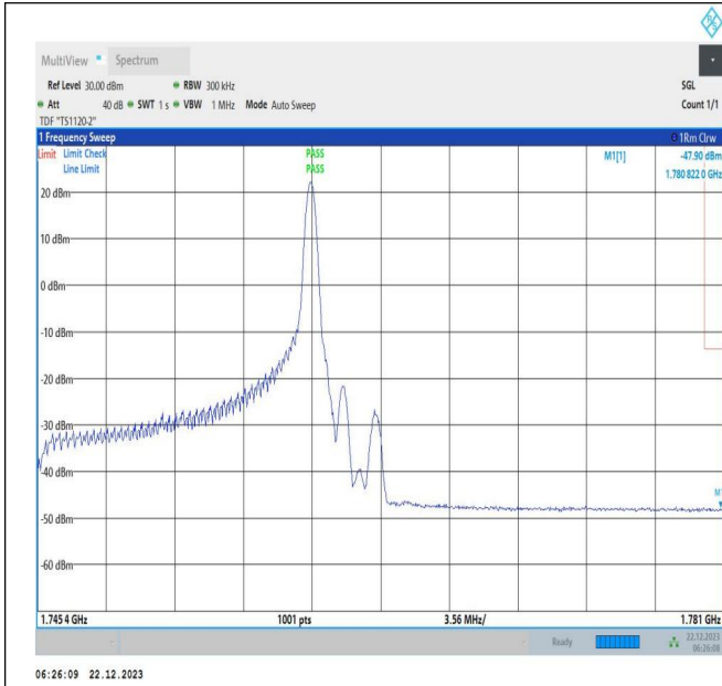
15MHz-20MHz_16QAM@16QAM-16QAM@16QAM_132401-132572_1RB#74@75RB#0-0RB#0@100RB#0
