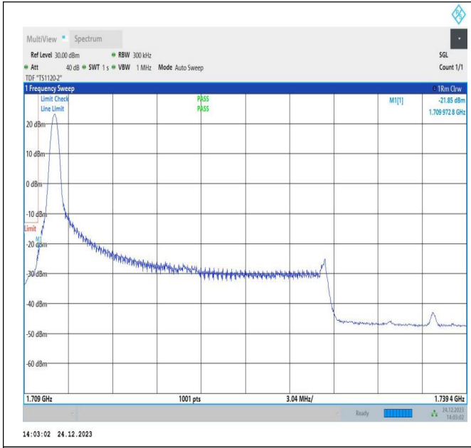
20MHz-10MHz_QPSK@QPSK-QPSK@QPSK_132072-132216_1RB#0@100RB#0-0RB#0@50RB#0
