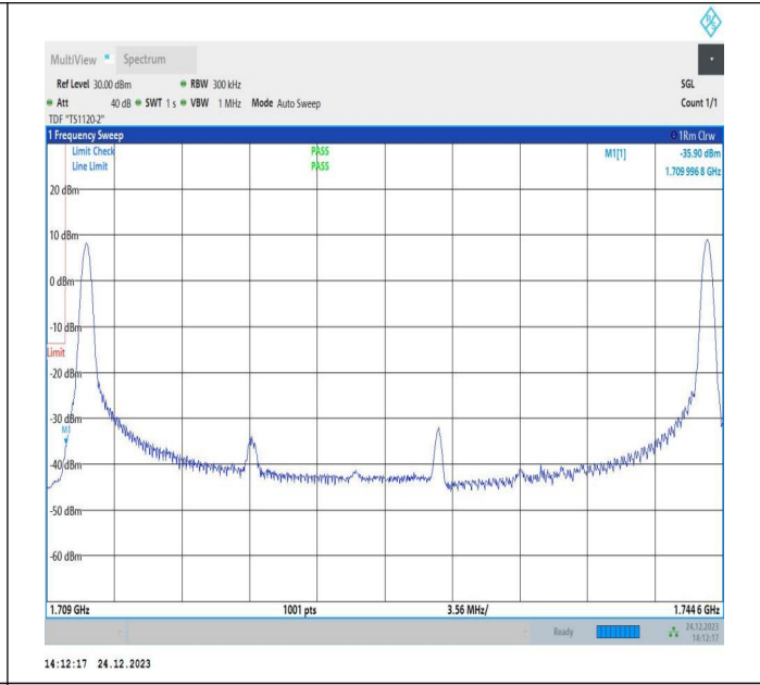
20MHz-15MHz_16QAM@16QAM-16QAM@16QAM_132072-132243_1RB#0@100RB#0-1RB#74@75RB#0
