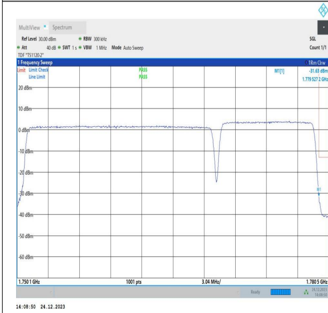
20MHz-10MHz_QPSK@QPSK-QPSK@QPSK_132473-132617_100RB#0@100RB#0-50RB#0@50RB#0
