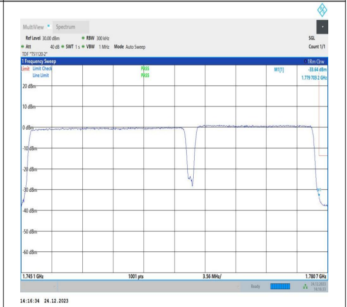
20MHz-15MHz_16QAM@16QAM-16QAM@16QAM_132423-132594_100RB#0@100RB#0-75RB#0@75RB#0
