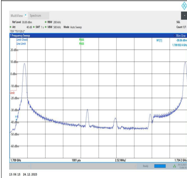
20MHz-5MHz_QPSK@QPSK-QPSK@QPSK_132072-1321 89_1RB#0@100RB#0-1RB#24@25RB#0
