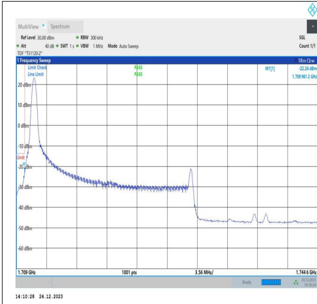
20MHz-15MHz_QPSK@QPSK-QPSK@QPSK_132072-132243_1RB#0@100RB#0-0RB#0@75RB#0
