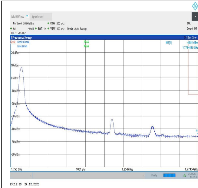
20MHz-5MHz_16QAM@16QAM-16QAM@16QAM_132522-132572_1RB#0@100RB#0-1RB#24@25RB#0
