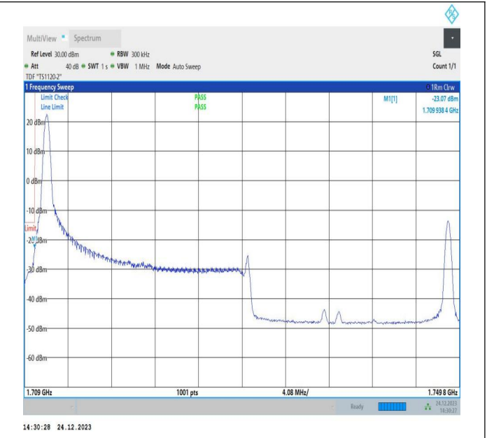
20MHz-20MHz_16QAM@16QAM-16QAM@16QAM_132072-132270_1RB#0@100RB#0-0RB#0@100RB#0
