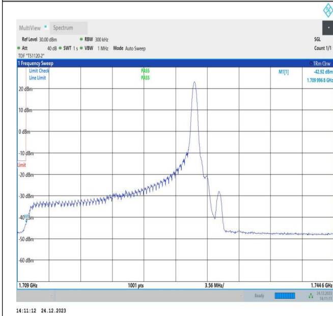
20MHz-15MHz_QPSK@QPSK-QPSK@QPSK_132072-132243_1RB#99@100RB#0-0RB#0@75RB#0
