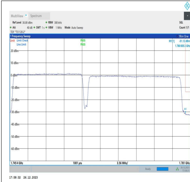
15MHz-20MHz_64QAM@64QAM-64QAM_132401 -132572_75RB#0@75RB#0-100RB#0@100RB#0
