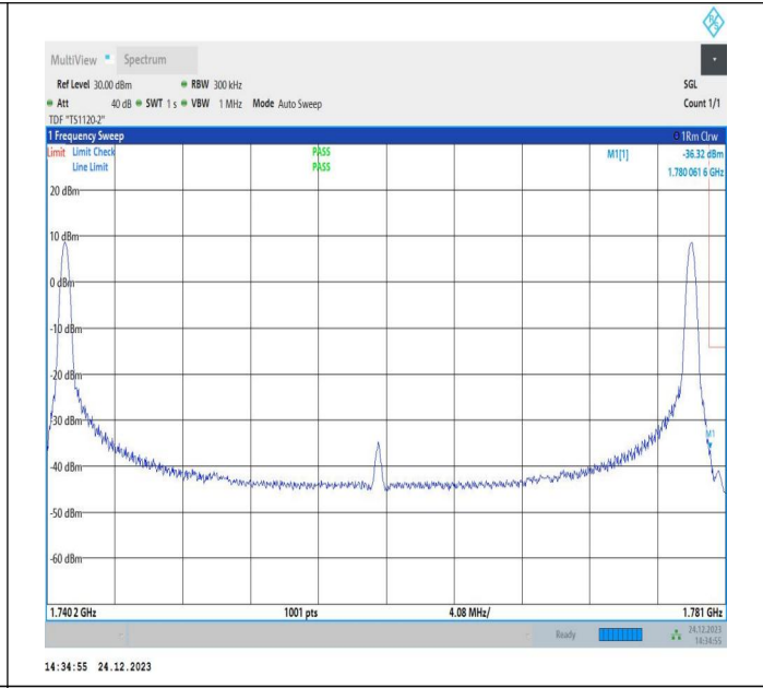
20MHz-20MHz_16QAM@16QAM-16QAM@16QAM_132374-132572_1RB#0@100RB#0-1RB#99@100RB#0
