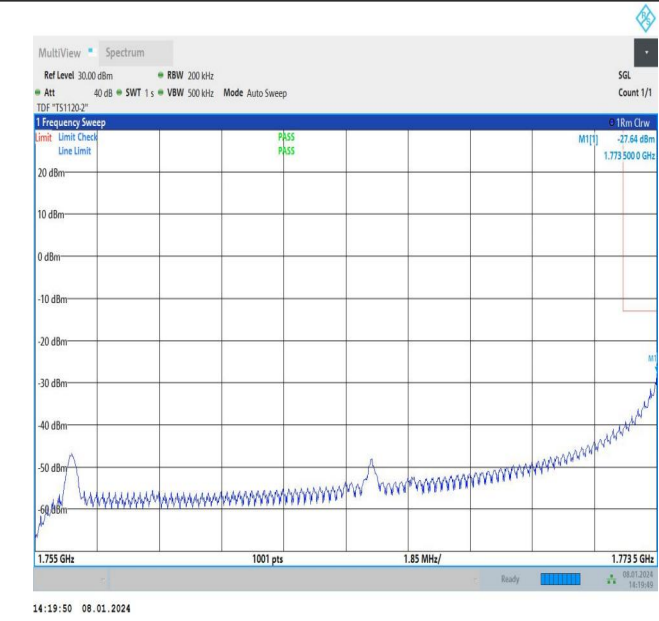
20MHz-5MHz_16QAM@16QAM-16QAM@16QAM_132522-132572_1RB#99@100RB#0-0RB#0@25RB#0
