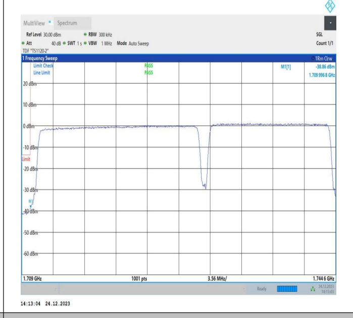
20MHz-15MHz_16QAM@16QAM-16QAM@16QAM_132072-132243_100RB#0@100RB#0-75RB#0@75RB#0
