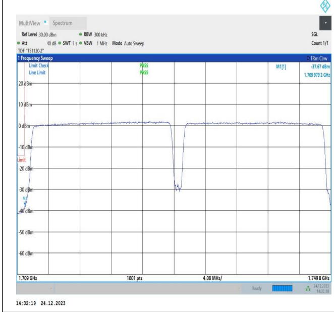
20MHz-20MHz_QPSK@QPSK-QPSK@QPSK_132072-132270_100RB#0@100RB#0-100RB#0@100RB#0
