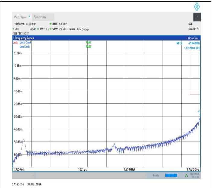
20MHz-5MHz_64QAM@64QAM-64QAM@64QAM_132522-132572_1RB#99@100RB#0-0RB#0@25RB#0
