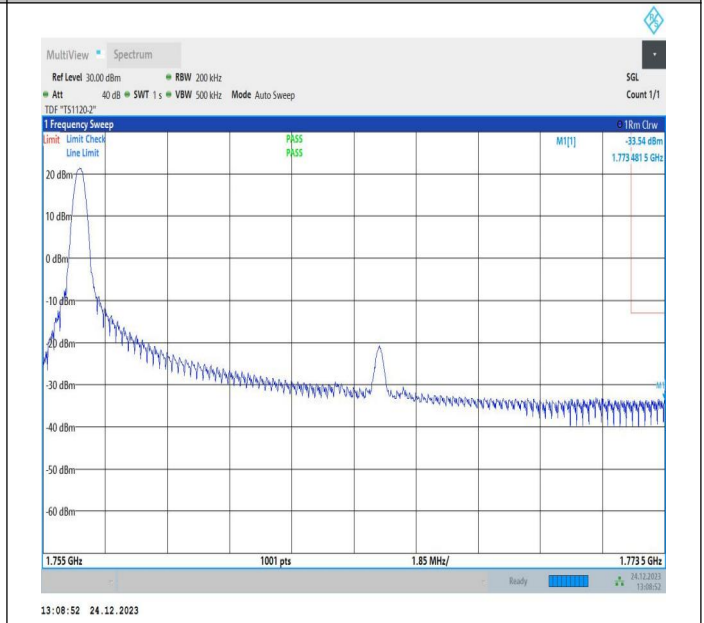
20MHz-5MHz_16QAM@16QAM-16QAM@16QAM_132522-132572_1RB#0@100RB#0-0RB#0@25RB#0
