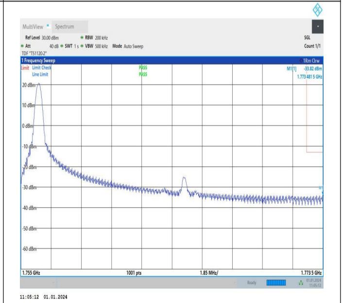
20MHz-5MHz_64QAM@64QAM-64QAM@64QAM_132522-132572_1RB#0@100RB#0-0RB#0@25RB#0
