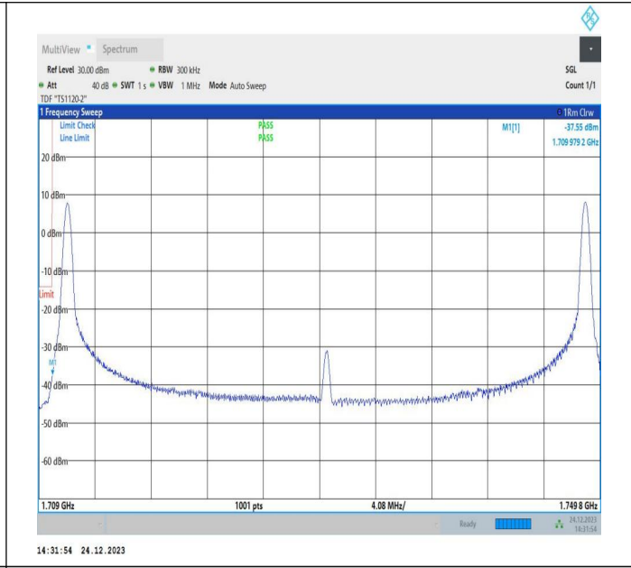
20MHz-20MHz_16QAM@16QAM-16QAM@16QAM_132072-132270_1RB#0@100RB#0-1RB#99@100RB#0
