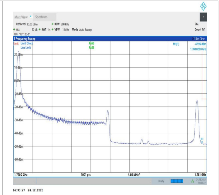
20MHz-20MHz_16QAM@16QAM-16QAM@16QAM_132374-132572_1RB#0@100RB#0-0RB#0@100RB#0
