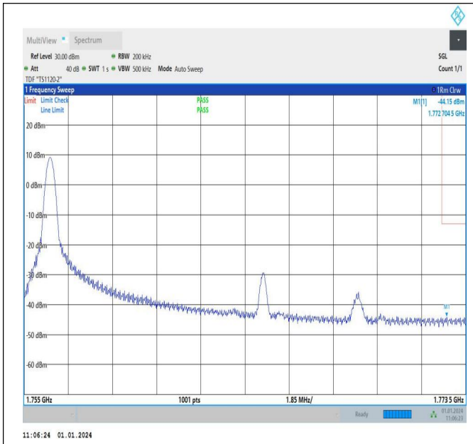
20MHz-5MHz_64QAM@64QAM-64QAM@64QAM_132522-132572_1RB#0@100RB#0-1RB#24@25RB#0
