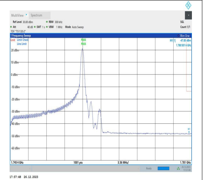
15MHz-20MHz_64QAM@64QAM-64QAM@64QAM_132401-132572_1RB#74@75RB#0-0RB#0@100RB#0
