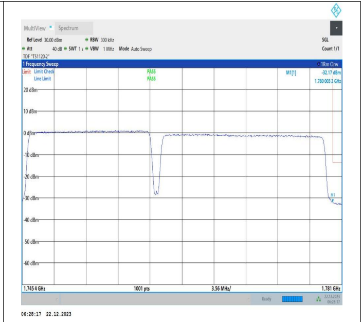
15MHz-20MHz_16QAM@16QAM-16QAM@16QAM_132401-132572_75RB#0@75RB#0-100RB#0@100RB#0
