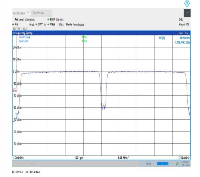
20MHz-20MHz_16QAM@16QAM-16QAM@16QAM_132072-132270_100RB#0@100RB#0-100RB#0@100RB#0
