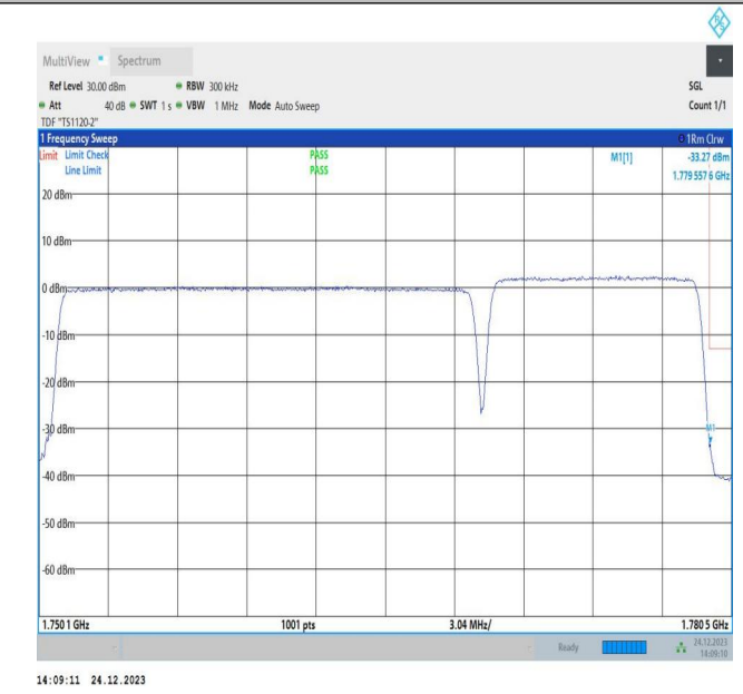
20MHz-10MHz_16QAM@16QAM-16QAM@16QAM_132473-132617_100RB#0@100RB#0-50RB#0@50RB#0
