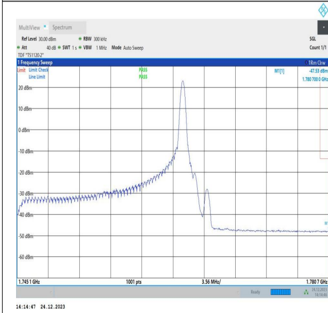
20MHz-15MHz_QPSK@QPSK-QPSK@QPSK_132423-132594_1RB#99@100RB#0-0RB#0@75RB#0
