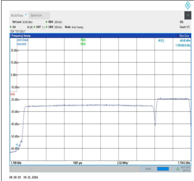
20MHz-5MHz_64QAM@64QAM-64QAM@64QAM_132072-132189_100RB#0@100RB#0-25RB#0@25RB#0
