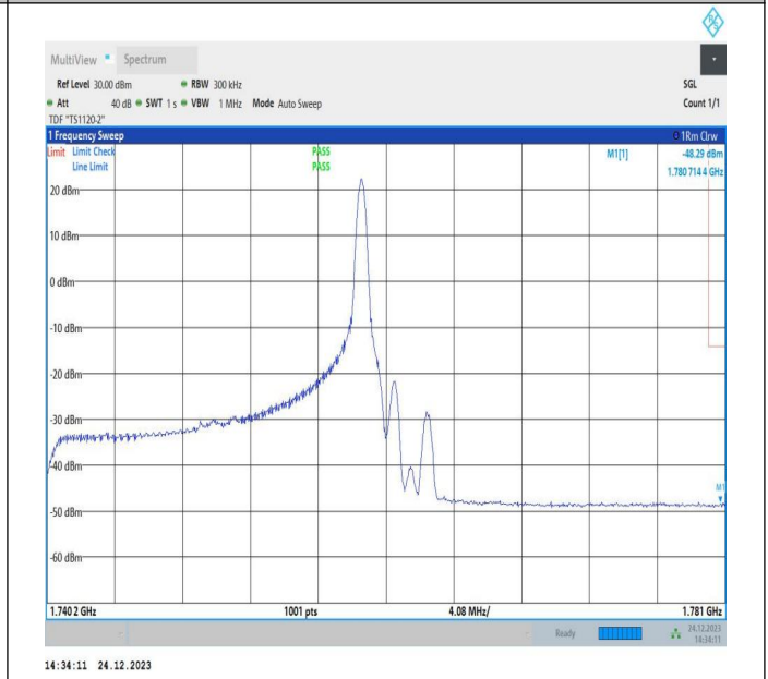
20MHz-20MHz_16QAM@16QAM-16QAM@16QAM_132374-132572_1RB#99@100RB#0-0RB#0@100RB#0
