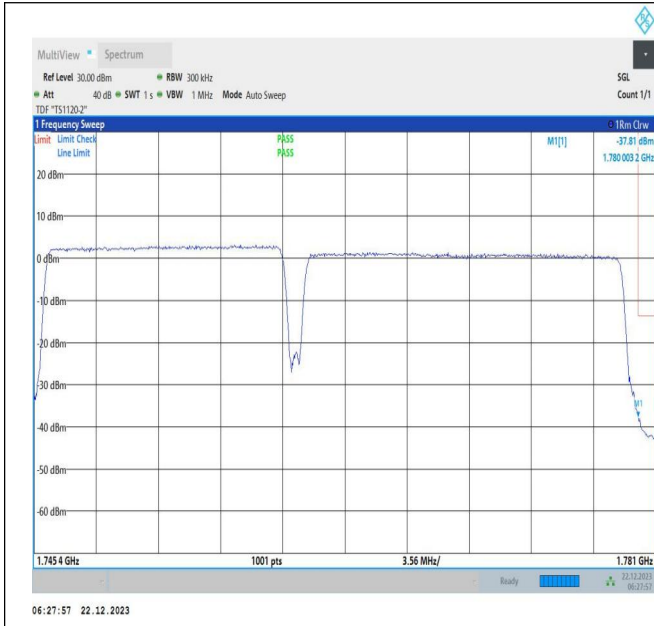
15MHz-20MHz_QPSK@QPSK-QPSK@QPSK_132401-132572_75RB#0@75RB#0-100RB#0@100RB#0
