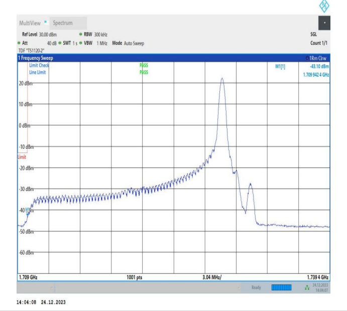
20MHz-10MHz_16QAM@16QAM-16QAM@16QAM_132072-132216_1RB#99@100RB#0-0RB#0@50RB#0
