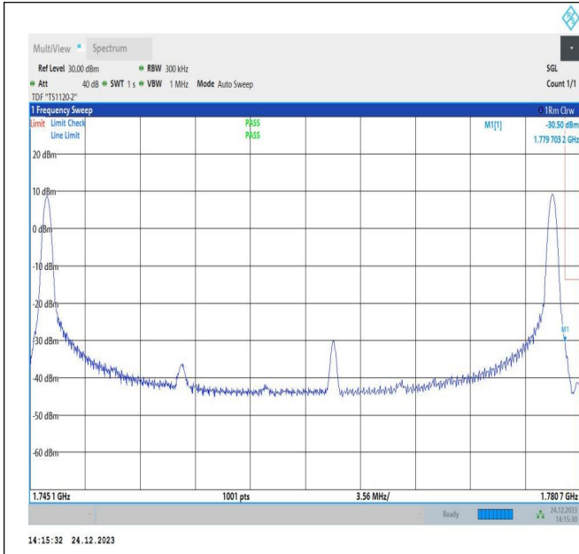
20MHz-15MHz_QPSK@QPSK-QPSK@QPSK_132423-132594_1RB#0@100RB#0-1RB#74@75RB#0
