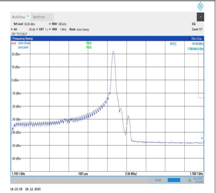
20MHz-15MHz_16QAM@16QAM-16QAM@16QAM_132423-132594_1RB#99@100RB#0-0RB#0@75RB#0
