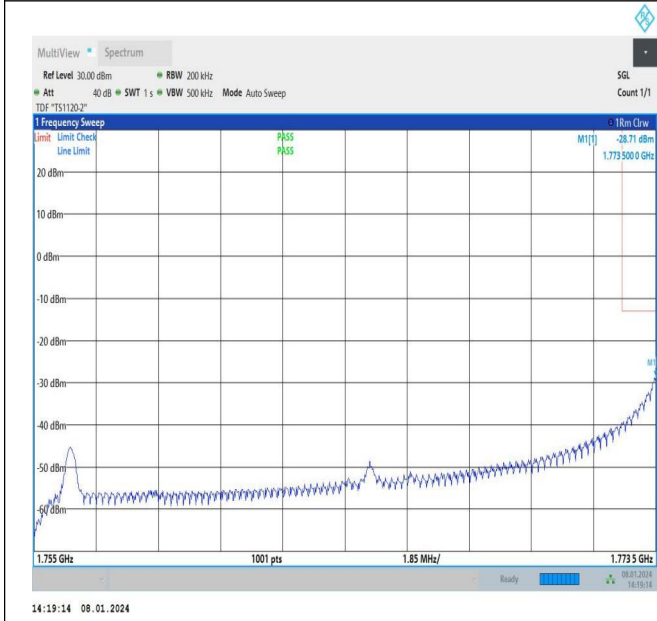
20MHz-5MHz_QPSK@QPSK-QPSK@QPSK_132522-132572_1RB#99@100RB#0-0RB#0@25RB#0
