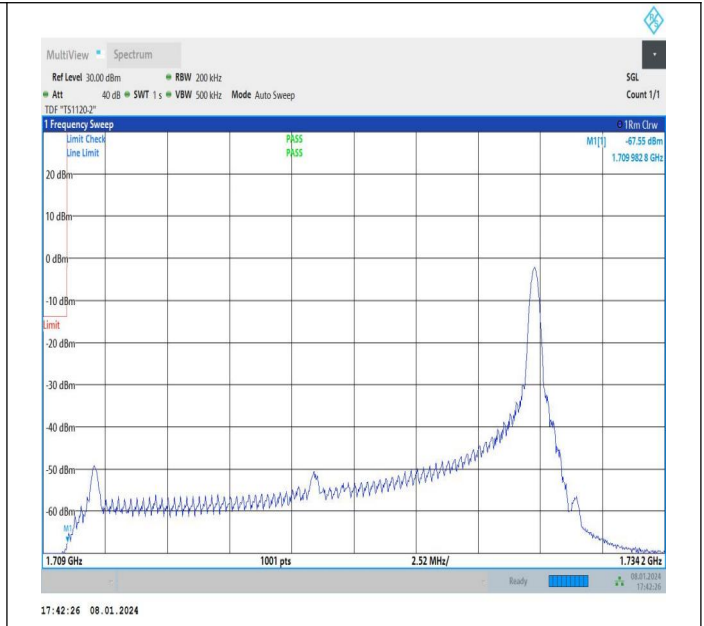
20MHz-5MHz_64QAM@64QAM-64QAM@64QAM_132072-132189_1RB#99@100RB#0-0RB#0@25RB#0
