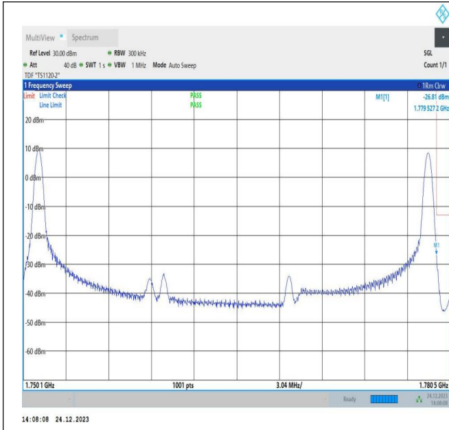
20MHz-10MHz_QPSK@QPSK-QPSK@QPSK_132473-132617_1RB#0@100RB#0-1RB#49@50RB#0
