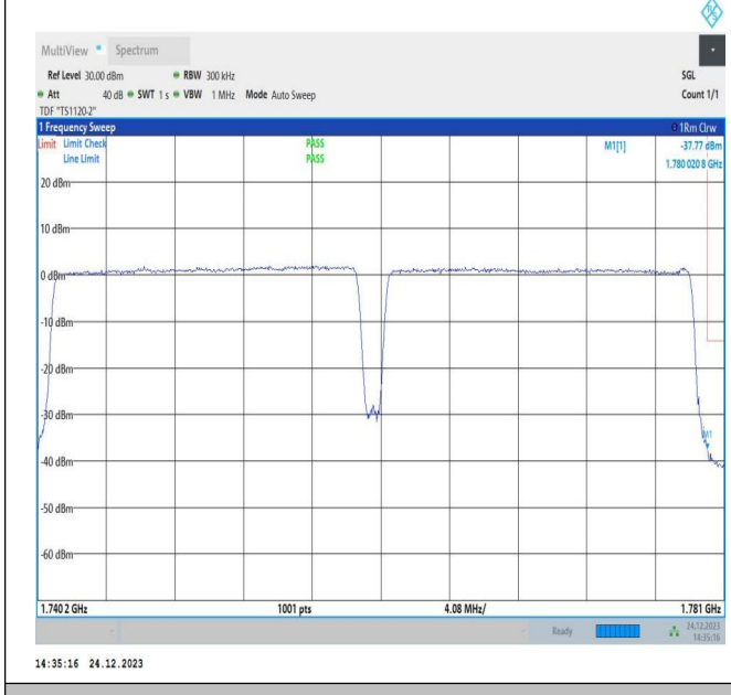
20MHz-20MHz_QPSK@QPSK-QPSK@QPSK_132374-132572_100RB#0@100RB#0-100RB#0@100RB#0
