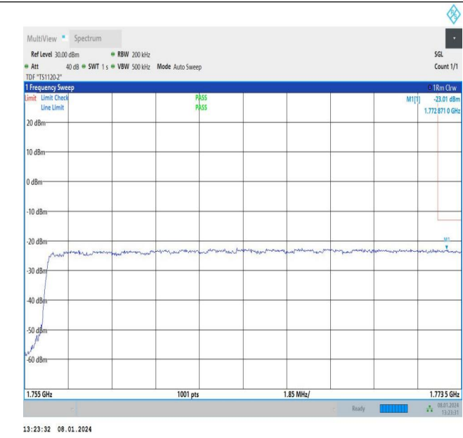
20MHz-5MHz_QPSK@QPSK-QPSK@QPSK_132522-132572_100RB#0@100RB#0-25RB#0@25RB#0
