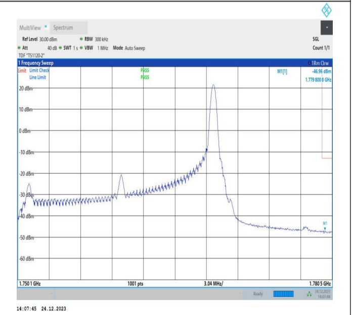
20MHz-10MHz_16QAM@16QAM-16QAM@16QAM_132473-132617_1RB#99@100RB#0-0RB#0@50RB#0
