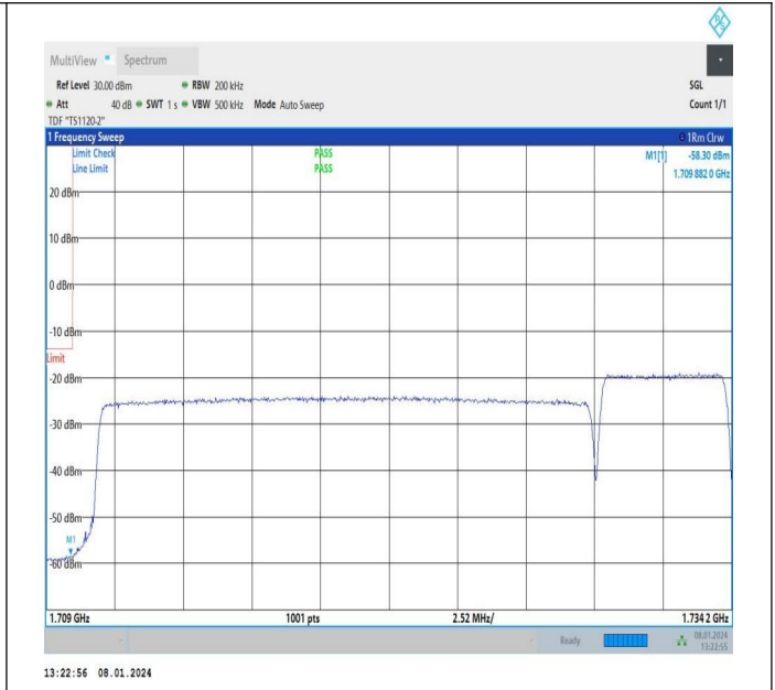
20MHz-5MHz_16QAM@16QAM-16QAM@16QAM_132072-132189_100RB#0@100RB#0-25RB#0@25RB#0
