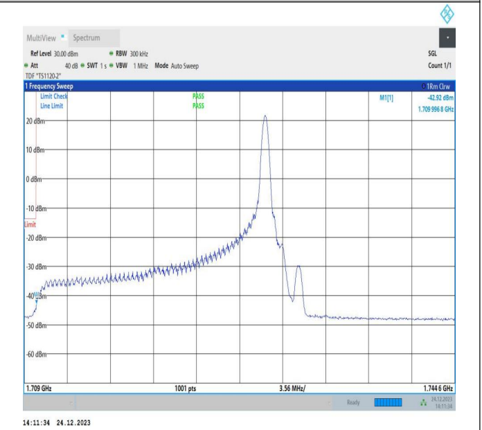
20MHz-15MHz_16QAM@16QAM-16QAM@16QAM_132072-132243_1RB#99@100RB#0-0RB#0@75RB#0
