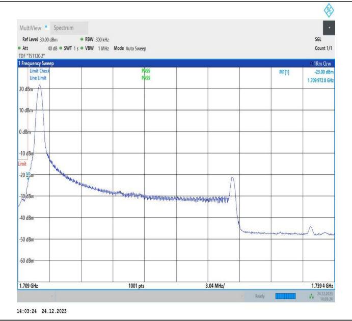
20MHz-10MHz_16QAM@16QAM-16QAM@16QAM_132072-132216_1RB#0@100RB#0-0RB#0@50RB#0
