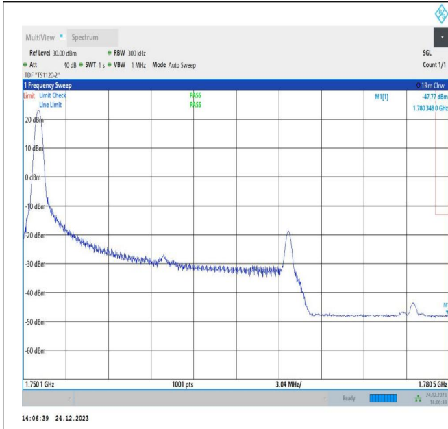
20MHz-10MHz_QPSK@QPSK-QPSK@QPSK_132473-132617_1RB#0@100RB#0-0RB#0@50RB#0
