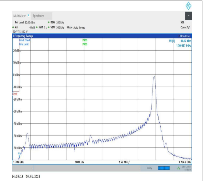
20MHz-5MHz_16QAM@16QAM-16QAM@16QAM_132072-132189_1RB#99@100RB#0-0RB#0@25RB#0
