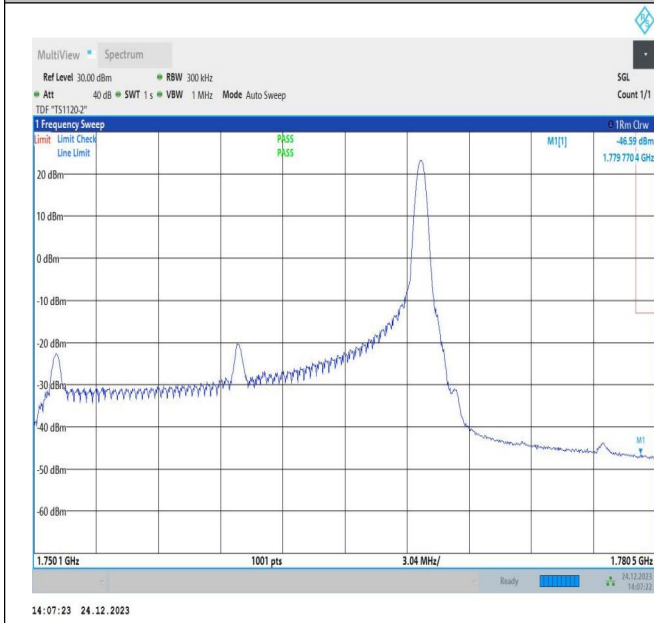
20MHz-10MHz_QPSK@QPSK-QPSK@QPSK_132473-132617_1RB#99@100RB#0-0RB#0@50RB#0
