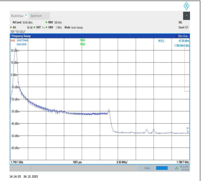
20MHz-15MHz_16QAM@16QAM-16QAM@16QAM_132423-132594_1RB#0@100RB#0-0RB#0@75RB#0
