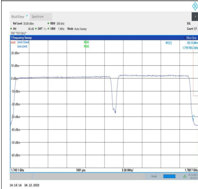
20MHz-15MHz_QPSK@QPSK-QPSK@QPSK_132423-132594_100RB#0@100RB#0-75RB#0@75RB#0
