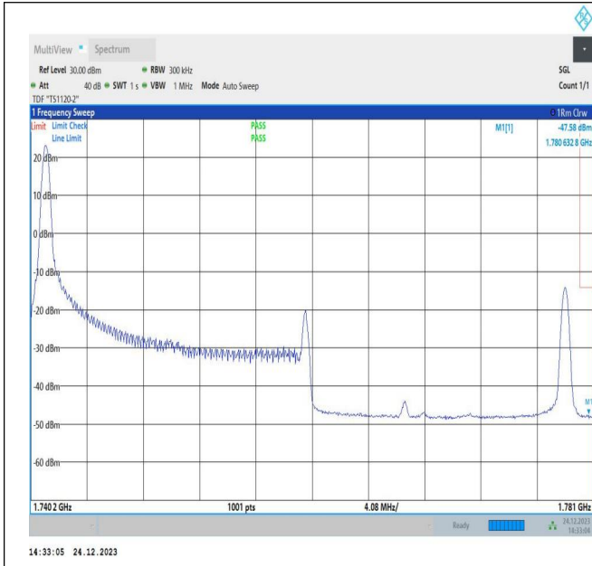
20MHz-20MHz_QPSK@QPSK-QPSK@QPSK_132374-132572_1RB#0@100RB#0-0RB#0@100RB#0
