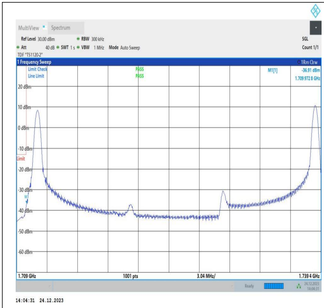
20MHz-10MHz_QPSK@QPSK-QPSK@QPSK_132072-132216_1RB#0@100RB#0-1RB#49@50RB#0
