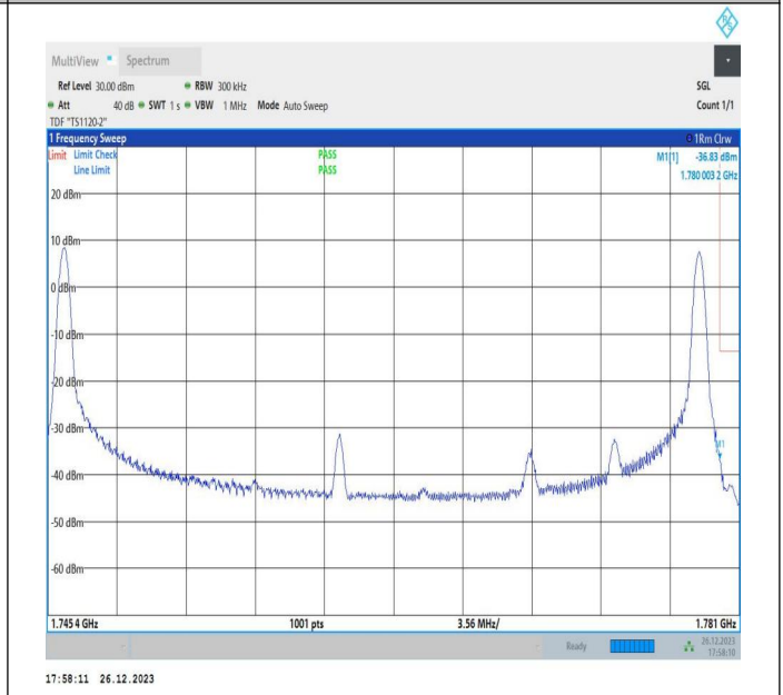
15MHz-20MHz_64QAM@64QAM-64QAM@64QAM_132401-132572_1RB#0@75RB#0-1RB#99@100RB#0
