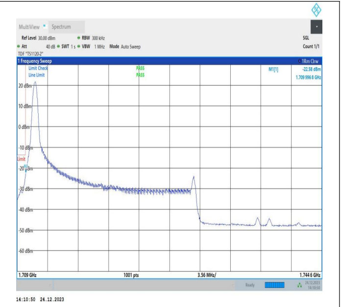
20MHz-15MHz_16QAM@16QAM-16QAM@16QAM_132072-132243_1RB#0@100RB#0-0RB#0@75RB#0
