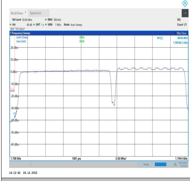
20MHz-15MHz_QPSK@QPSK-QPSK@QPSK_132072-132243_100RB#0@100RB#0-75RB#0@75RB#0
