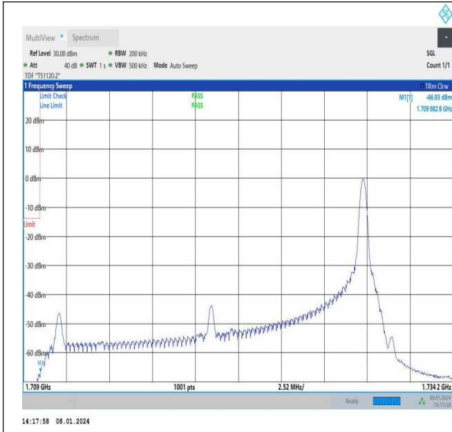
20MHz-5MHz_QPSK@QPSK-QPSK@QPSK_132072-132189_1RB#99@100RB#0-0RB#0@25RB#0
