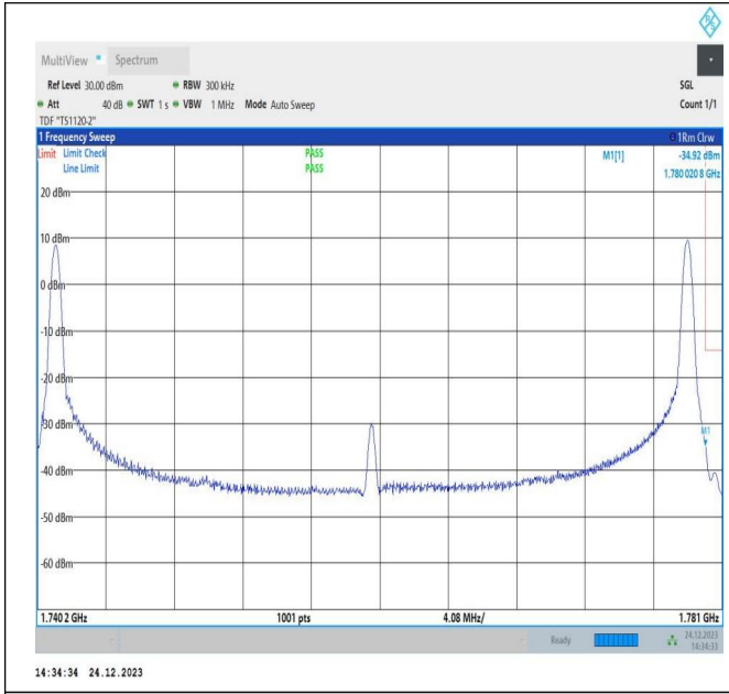
20MHz-20MHz_QPSK@QPSK-QPSK@QPSK_132374-132572_1RB#0@100RB#0-1RB#99@100RB#0
