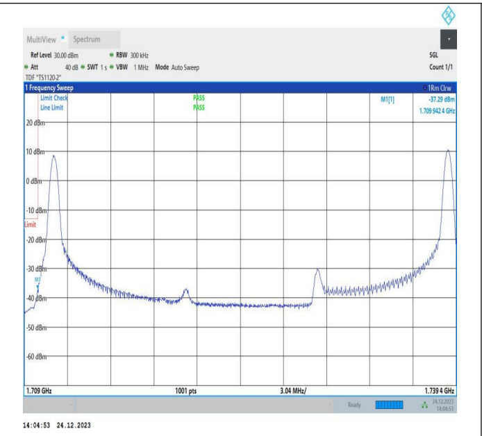
20MHz-10MHz_16QAM@16QAM-16QAM@16QAM_132072-132216_1RB#0@100RB#0-1RB#49@50RB#0
