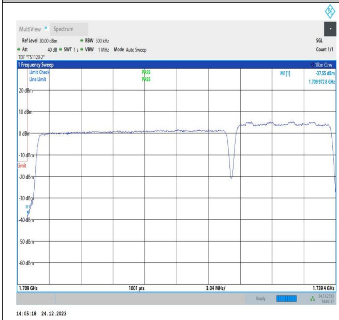
20MHz-10MHz_QPSK@QPSK-QPSK@QPSK_132072-132216_100RB#0@100RB#0-50RB#0@50RB#0
