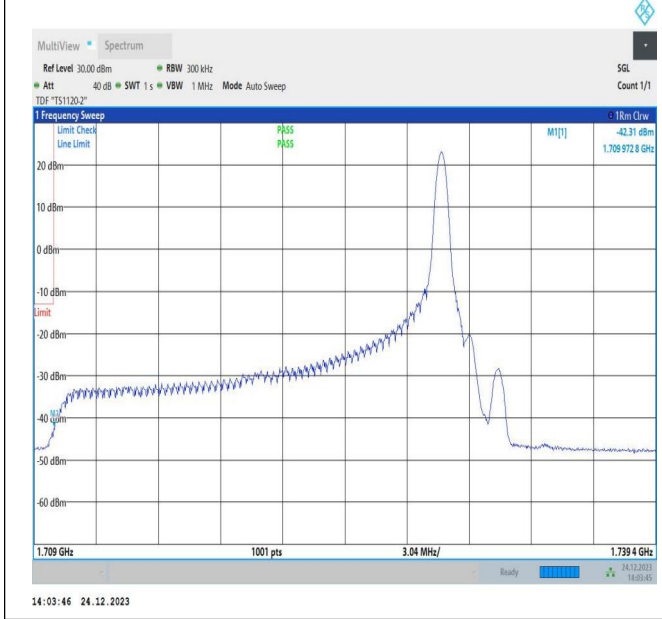
20MHz-10MHz_QPSK@QPSK-QPSK@QPSK_132072-132216_1RB#99@100RB#0-0RB#0@50RB#0
