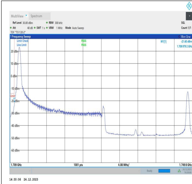
20MHz-20MHz_QPSK@QPSK-QPSK@QPSK_132072-132270_1RB#0@100RB#0-0RB#0@100RB#0
