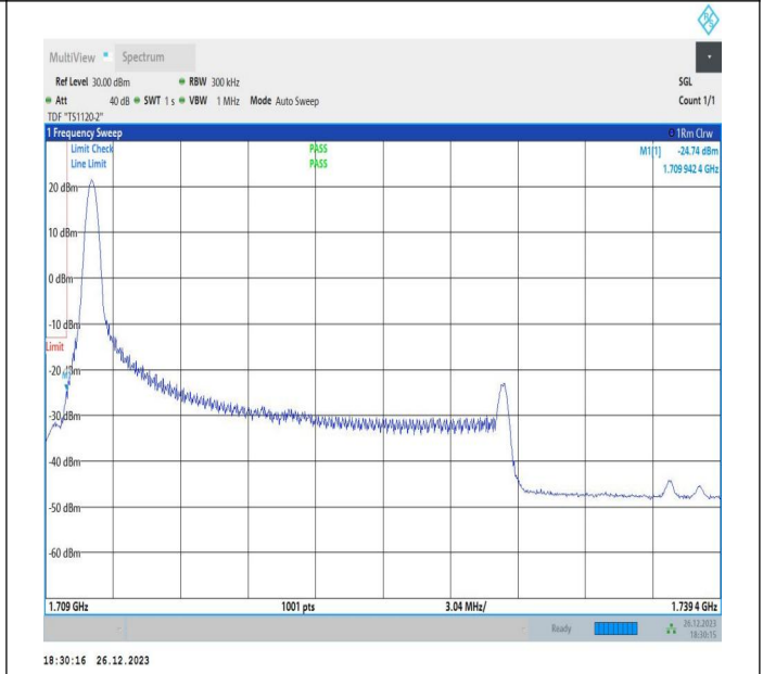
20MHz-10MHz_64QAM@64QAM-64QAM@64QAM_132072-132216_1RB#0@100RB#0-0RB#0@50RB#0
