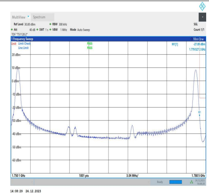
20MHz-10MHz_16QAM@16QAM-16QAM@16QAM_132473-132617_1RB#0@100RB#0-1RB#49@50RB#0
