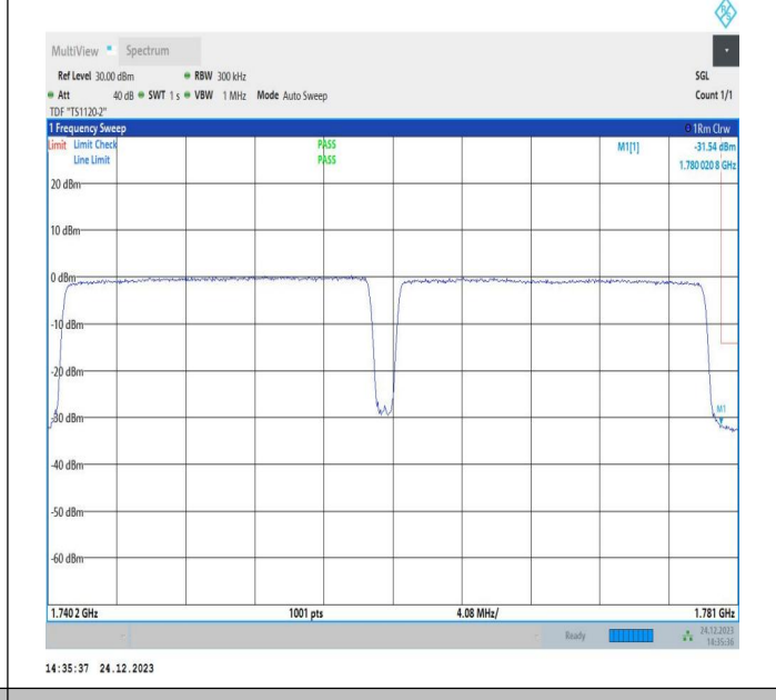
20MHz-20MHz_16QAM@16QAM-16QAM@16QAM_132374-132572_100RB#0@100RB#0-100RB#0@100RB#0
