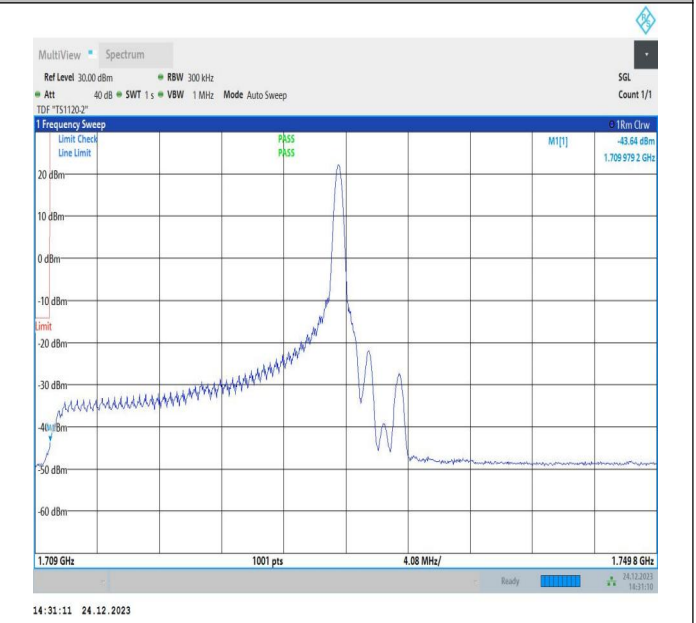
20MHz-20MHz_16QAM@16QAM-16QAM@16QAM_132072-132270_1RB#99@100RB#0-0RB#0@100RB#0
