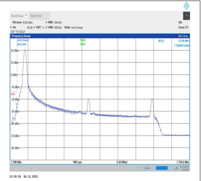
20MHz-5MHz_16QAM@16QAM-16QAM@16QAM_132072-1 32189_1RB#0@100RB#0-0RB#0@25RB#0
