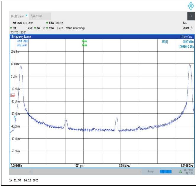
20MHz-15MHz_QPSK@QPSK-QPSK@QPSK_132072-132243_1RB#0@100RB#0-1RB#74@75RB#0
