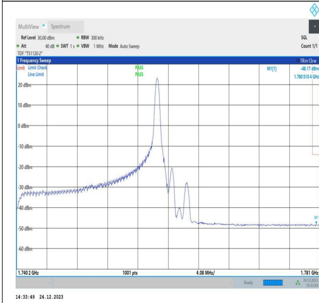
20MHz-20MHz_QPSK@QPSK-QPSK@QPSK_132374-132572_1RB#99@100RB#0-0RB#0@100RB#0
