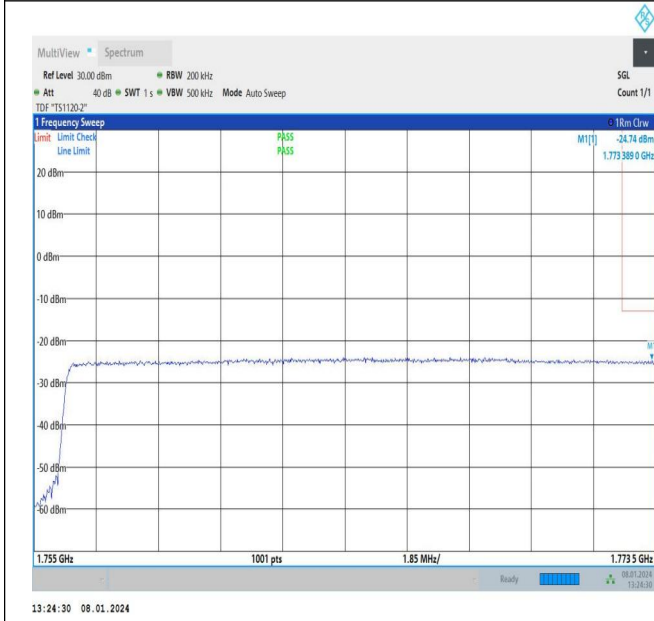
20MHz-5MHz_16QAM@16QAM-16QAM@16QAM_132522-132572_100RB#0@100RB#0-25RB#0@25RB#0
