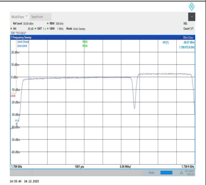
20MHz-10MHz_16QAM@16QAM-16QAM@16QAM_132072-132216_100RB#0@100RB#0-50RB#0@50RB#0
