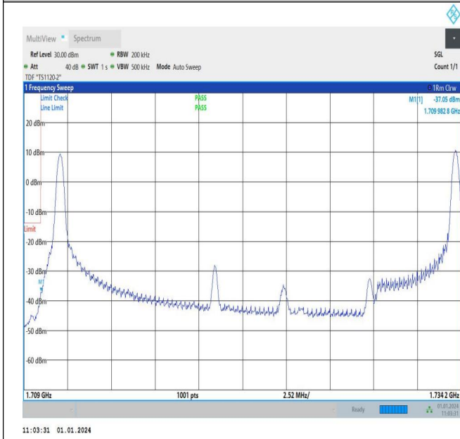
20MHz-5MHz_64QAM@64QAM-64QAM@64QAM_132072-132189_1RB#0@100RB#0-1RB#24@25RB#0
