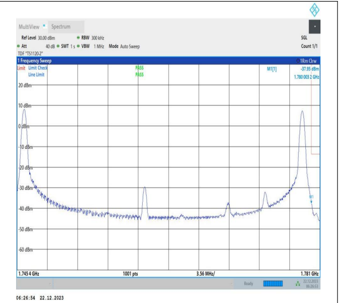
15MHz-20MHz_QPSK@QPSK-QPSK@QPSK_132401-132572_1RB#0@75RB#0-1RB#99@100RB#0
