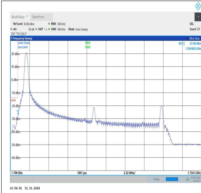
20MHz-5MHz_64QAM@64QAM-64QAM@64QAM_132072-132189_1RB#0@100RB#0-0RB#0@25RB#0
