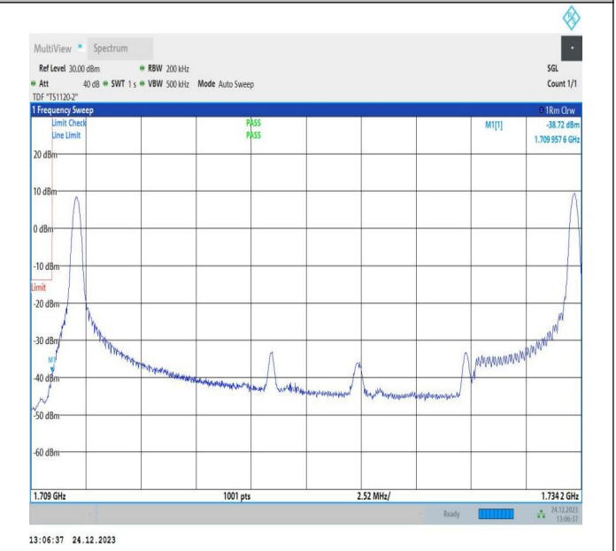
20MHz-5MHz_16QAM@16QAM-16QAM@16QAM_132072-1 32189_1RB#0@100RB#0-1RB#24@25RB#0
