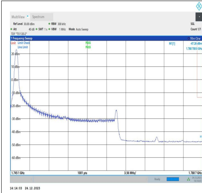
20MHz-15MHz_QPSK@QPSK-QPSK@QPSK_132423-132594_1RB#0@100RB#0-0RB#0@75RB#0
