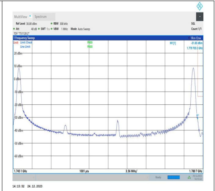
20MHz-15MHz_16QAM@16QAM-16QAM@16QAM_132423-132594_1RB#0@100RB#0-1RB#74@75RB#0
