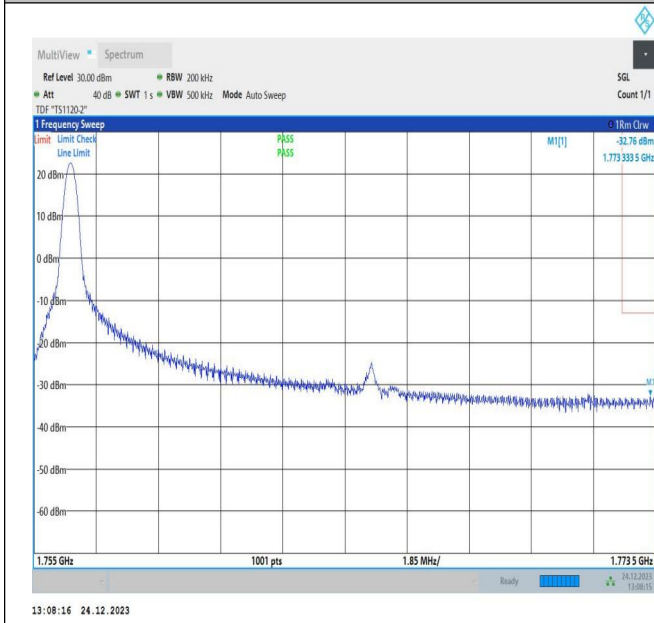
20MHz-5MHz_QPSK@QPSK-QPSK@QPSK_132522-132572_1RB#0@100RB#0-0RB#0@25RB#0
