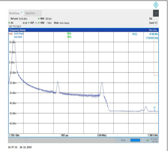
20MHz-10MHz_16QAM@16QAM-16QAM@16QAM_132473-132617_1RB#0@100RB#0-0RB#0@50RB#0
