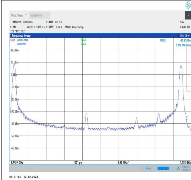
15MHz-20MHz_16QAM@16QAM-16QAM@16QAM_132401-132572_1RB#0@75RB#0-1RB#99@100RB#0
