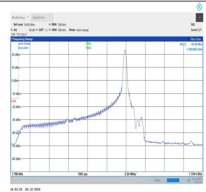
15MHz-10MHz_64QAM@64QAM-64QAM@64QAM_132047-132167_1RB#74@75RB#0-0RB#0@50RB#0
