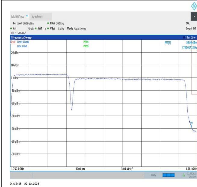
10MHz-20MHz_16QAM@16QAM-16QAM@16QAM_132428-132572_50RB#0@50RB#0-100RB#0@100RB#0
