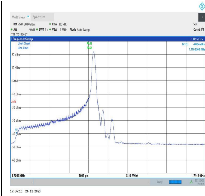
15MHz-20MHz_64QAM@64QAM-64QAM@64QAM_132050-132221_1RB#74@75RB#0-0RB#0@100RB#0
