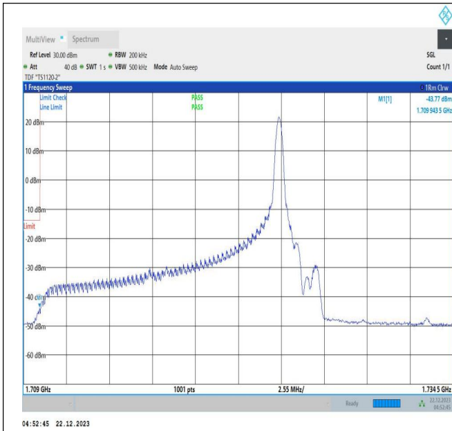
15MHz-10MHz_16QAM@16QAM-16QAM@16QAM_132047-132167_1RB#0@75RB#0-0RB#0@50RB#0
