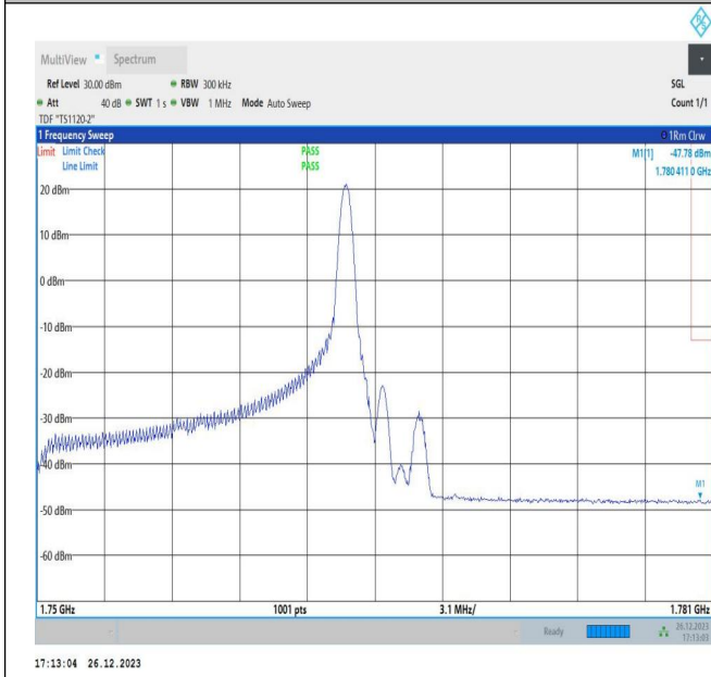
15MHz-15MHz_64QAM@64QAM-64QAM@64QAM_132447-132597_1RB#74@75RB#0-0RB#0@75RB#0
