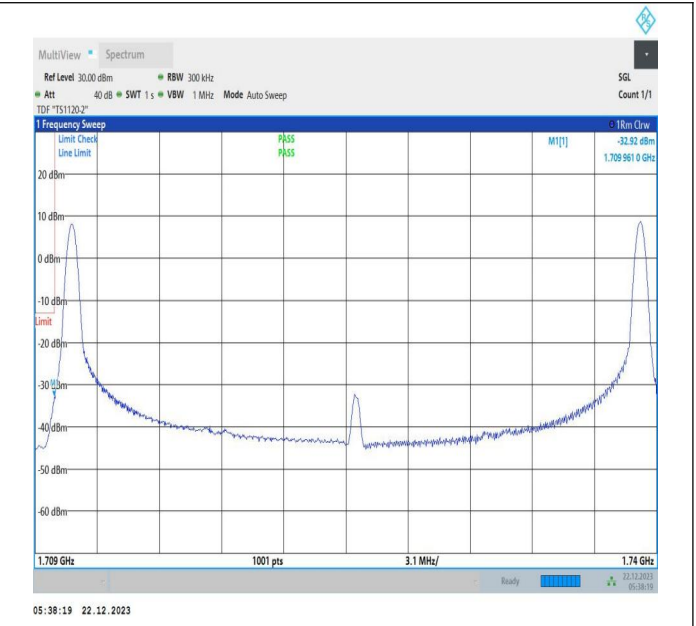
15MHz-15MHz_QPSK@QPSK-QPSK@QPSK_132047-132197_1RB#0@75RB#0-1RB#74@75RB#0
