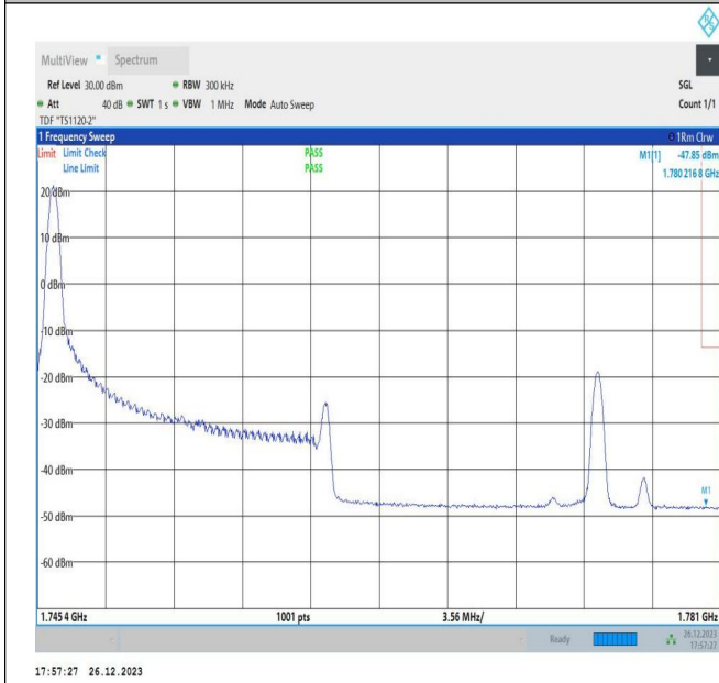
15MHz-20MHz_64QAM@64QAM-64QAM@64QAM_132401 -132572_1RB#0@75RB#0-0RB#0@100RB#0
