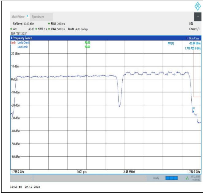
15MHz-10MHz_QPSK@QPSK-QPSK@QPSK_132499-132619_75RB#0@75RB#0-50RB#0@50RB#0
