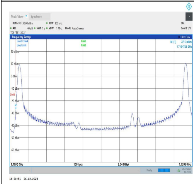
10MHz-20MHz_64QAM@64QAM-64QAM@64QAM_132027-132171_1RB#0@50RB#0-1RB#99@100RB#0
