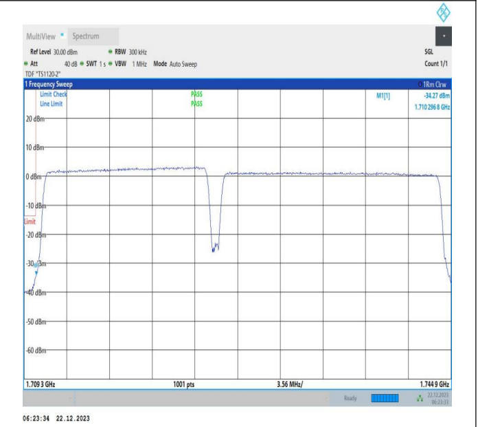
15MHz-20MHz_QPSK@QPSK-QPSK@QPSK_132050-1322 21_75RB#0@75RB#0-100RB#0@100RB#0
