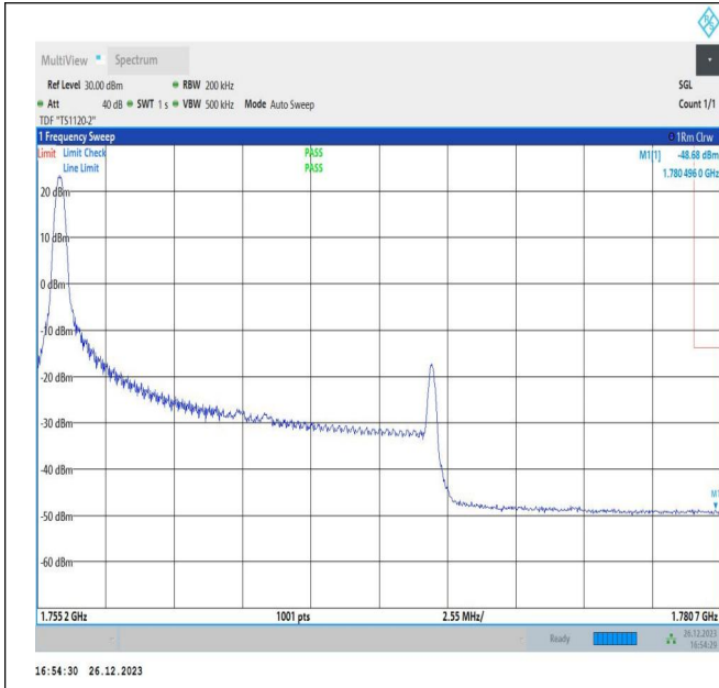
15MHz-10MHz_64QAM@64QAM-64QAM_132499-132619_1RB#0@75RB#0-0RB#0@50RB#0
