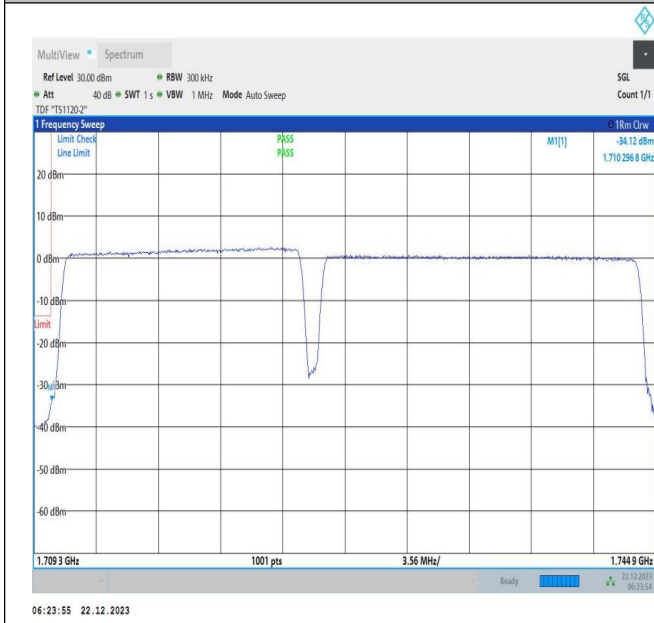
15MHz-20MHz_16QAM@16QAM-16QAM@16QAM_132050-132221_75RB#0@75RB#0-100RB#0@100RB#0
