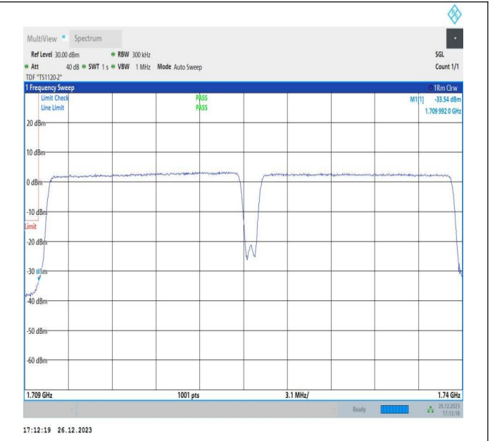
15MHz-15MHz_64QAM@64QAM-64QAM@64QAM_132047-132197_75RB#0@75RB#0-75RB#0@75RB#0
