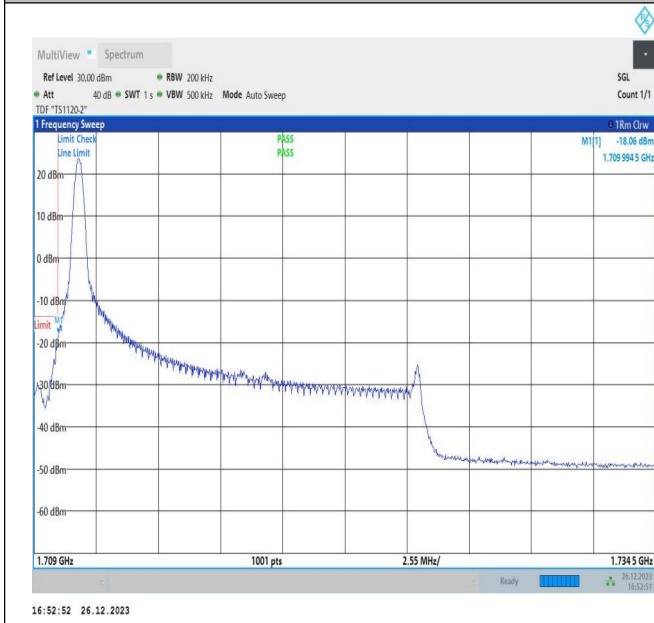
15MHz-10MHz_64QAM@64QAM-64QAM@64QAM_132047-132167_1RB#0@75RB#0-0RB#0@50RB#0
