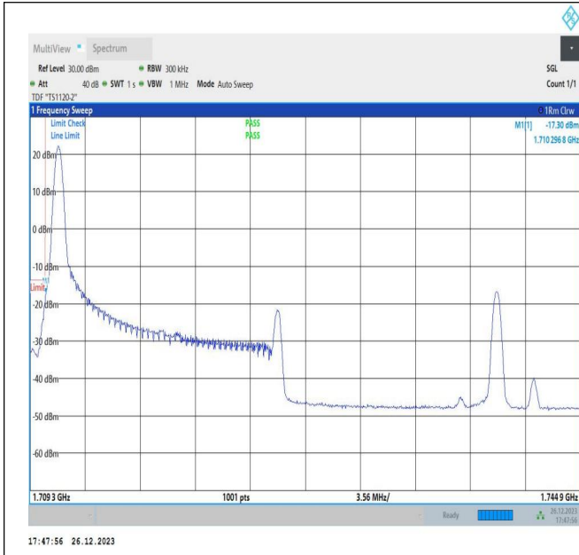
15MHz-20MHz_64QAM@64QAM-64QAM@64QAM_132050 -132221_1RB#0@75RB#0-0RB#0@100RB#0
