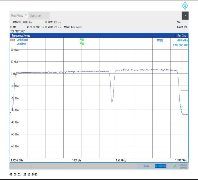
15MHz-10MHz_16QAM@16QAM-16QAM@16QAM_132499-132619_75RB#0@75RB#0-50RB#0@50RB#0
