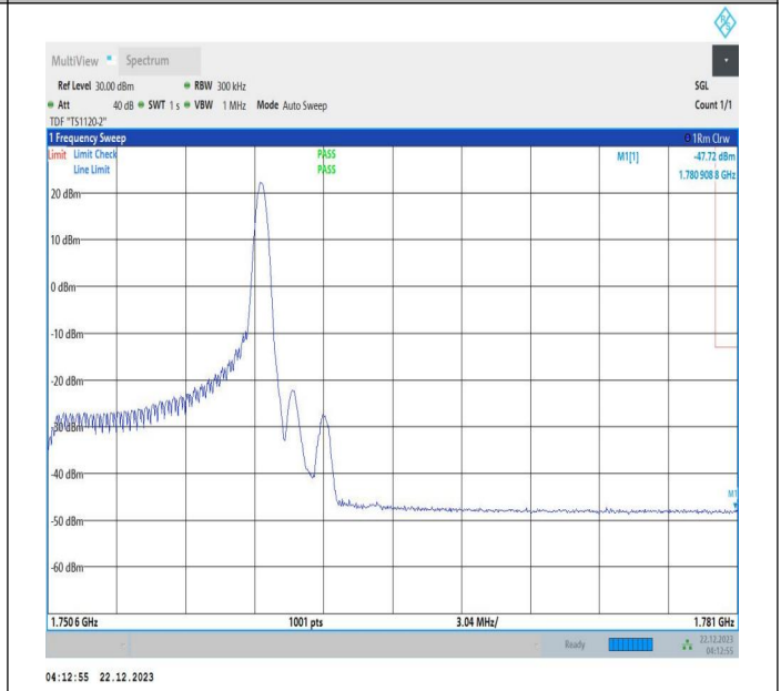
10MHz-20MHz_16QAM@16QAM-16QAM@16QAM_132428-132572_1RB#49@50RB#0-0RB#0@100RB#0
