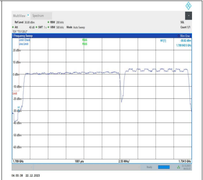
15MHz-10MHz_16QAM@16QAM-16QAM@16QAM_132047-132167_75RB#0@75RB#0-50RB#0@50RB#0
