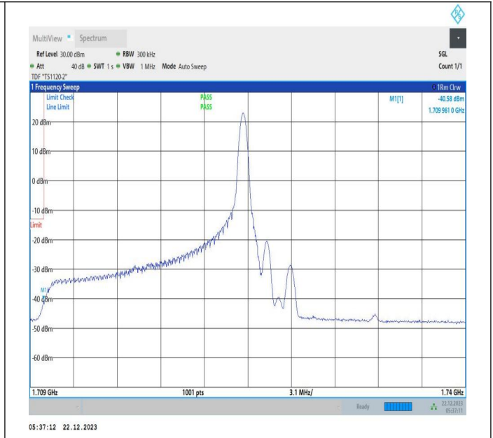
15MHz-15MHz_QPSK@QPSK-QPSK@QPSK_132047-132197_1RB#74@75RB#0-0RB#0@75RB#0
