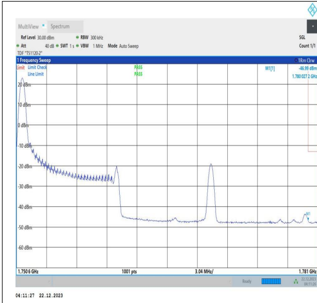
10MHz-20MHz_QPSK@QPSK-QPSK@QPSK_132428-132572_1RB#0@50RB#0-0RB#0@100RB#0
