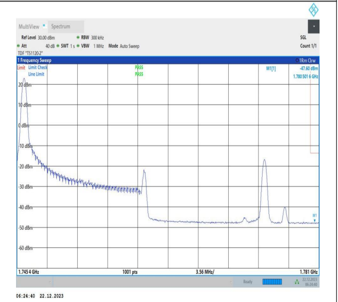
15MHz-20MHz_QPSK@QPSK-QPSK@QPSK_132401-132572_1RB#0@75RB#0-0RB#0@100RB#0
