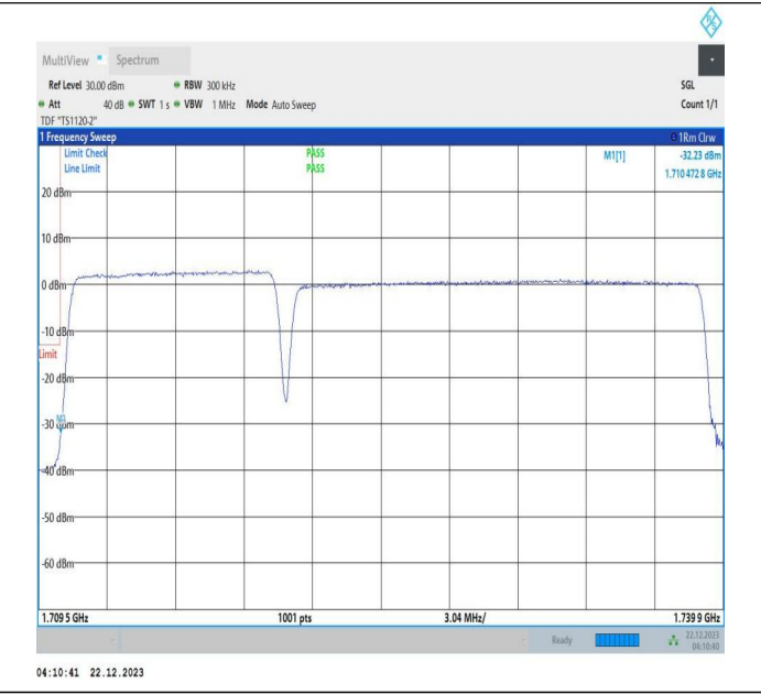
10MHz-20MHz_16QAM@16QAM-16QAM@16QAM_132027-132171_50RB#0@50RB#0-100RB#0@100RB#0
