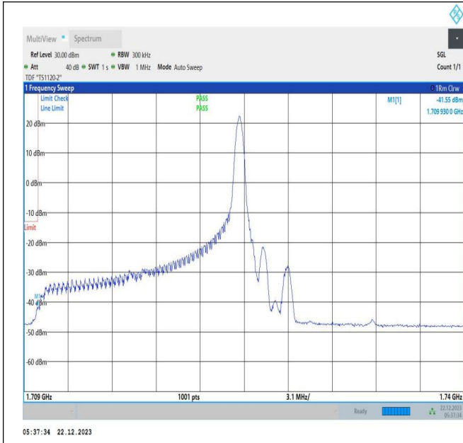
15MHz-15MHz_16QAM@16QAM-16QAM@16QAM_132047-132197_1RB#74@75RB#0-0RB#0@75RB#0
