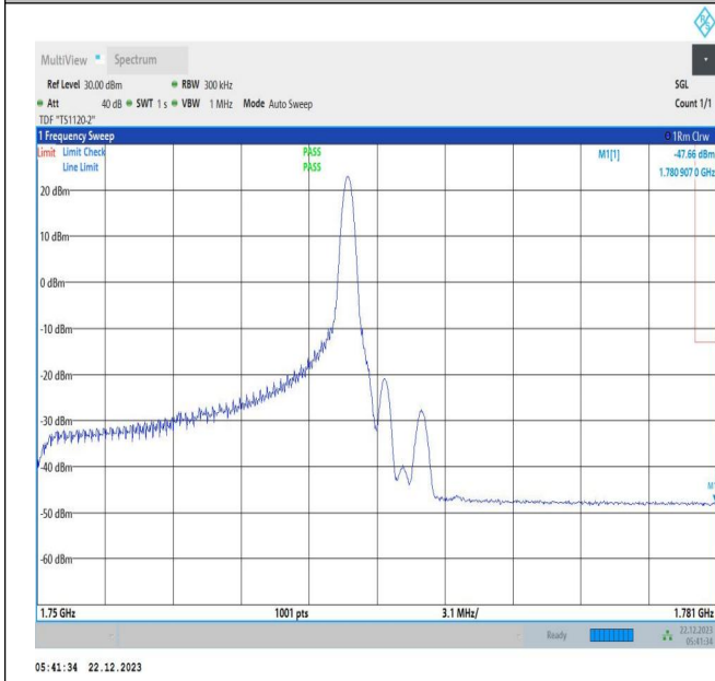
15MHz-15MHz_QPSK@QPSK-QPSK@QPSK_132447-132597_1RB#74@75RB#0-0RB#0@75RB#0
