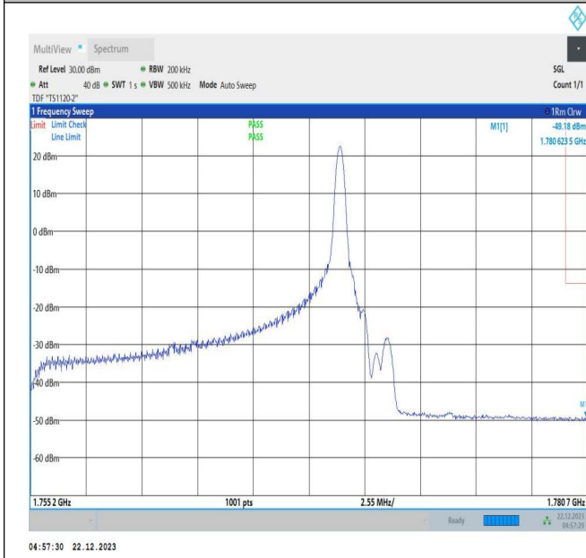
15MHz-10MHz_QPSK@QPSK-QPSK@QPSK_132499-132619_1RB#74@75RB#0-0RB#0@50RB#0
