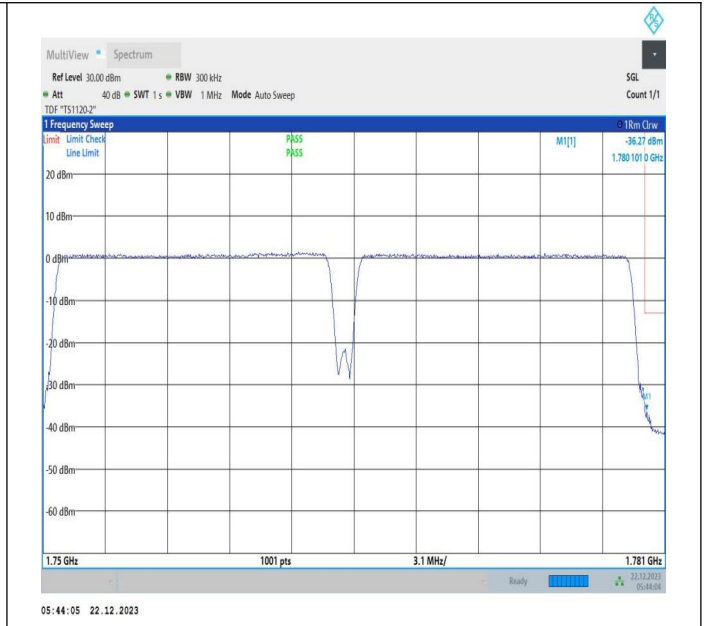
15MHz-15MHz_16QAM@16QAM-16QAM@16QAM_132447-132597_75RB#0@75RB#0-75RB#0@75RB#0
