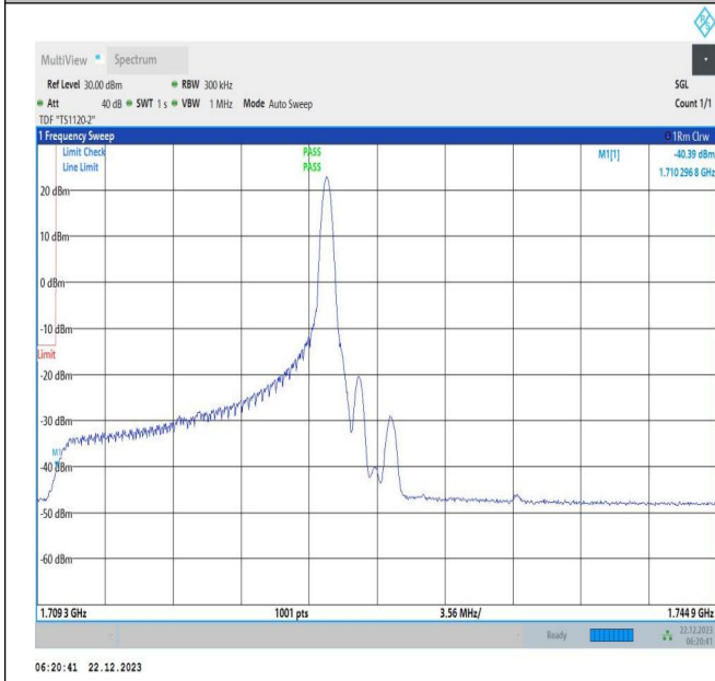
15MHz-20MHz_QPSK@QPSK-QPSK@QPSK_132050-13221_1RB#74@75RB#0-0RB#0@100RB#0
