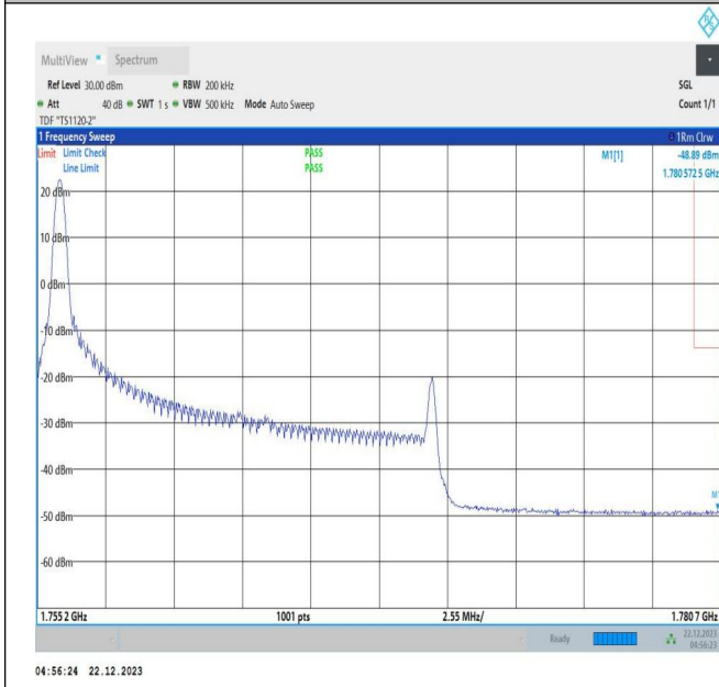
15MHz-10MHz_QPSK@QPSK-QPSK@QPSK_132499-132619_1RB#0@75RB#0-0RB#0@50RB#0
