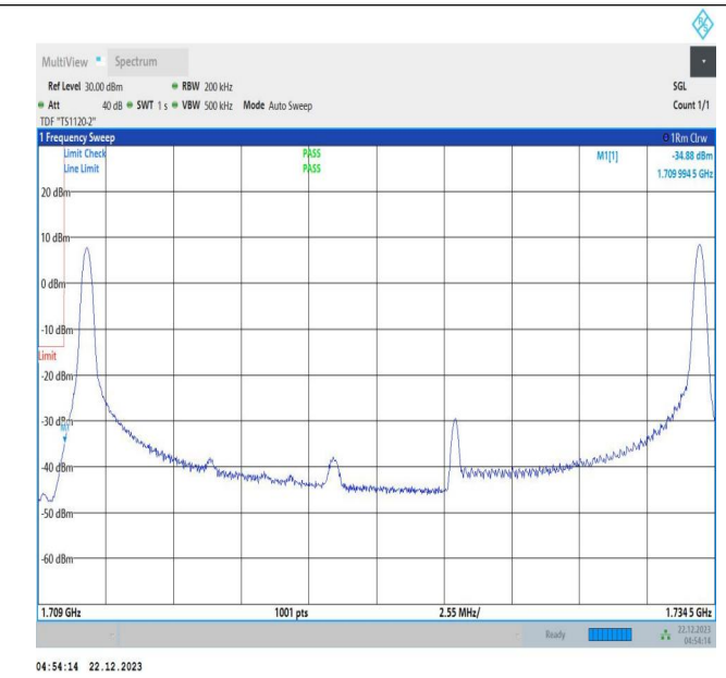
15MHz-10MHz_QPSK@QPSK-QPSK@QPSK_132047-132167_1RB#0@75RB#0-1RB#49@50RB#0
