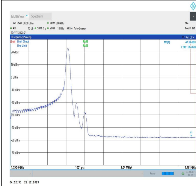
10MHz-20MHz_QPSK@QPSK-QPSK@QPSK_132428-132572_1RB#49@50RB#0-0RB#0@100RB#0
