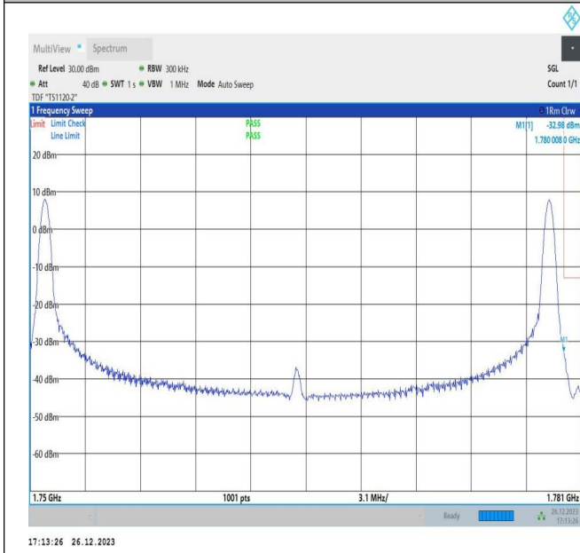
15MHz-15MHz_64QAM@64QAM-64QAM@64QAM_132447-132597_1RB#0@75RB#0-1RB#74@75RB#0
