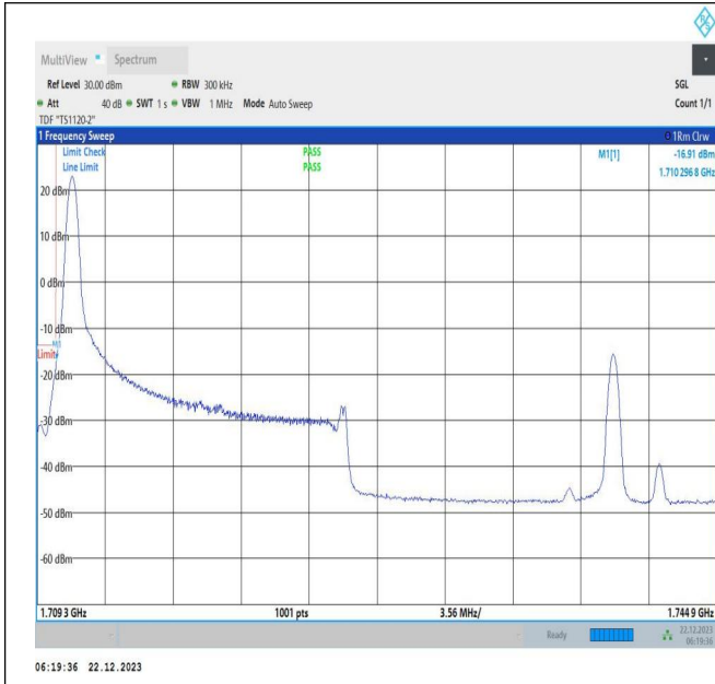
15MHz-20MHz_QPSK@QPSK-QPSK@QPSK_132050-13221_1RB#0@75RB#0-0RB#0@100RB#0
