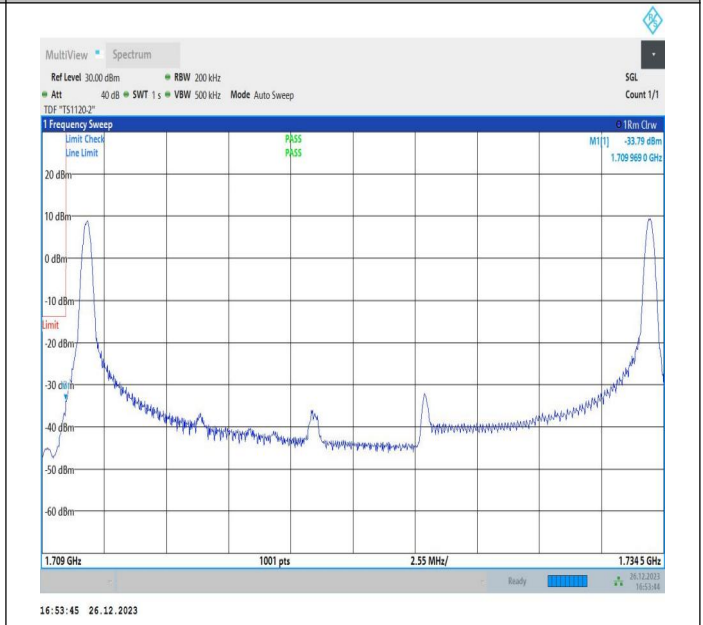
15MHz-10MHz_64QAM@64QAM-64QAM@64QAM_132047-132167_1RB#0@75RB#0-1RB#49@50RB#0
