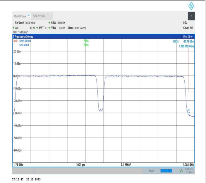
15MHz-15MHz_64QAM@64QAM-64QAM@64QAM_132447-132597_75RB#0@75RB#0-75RB#0@75RB#0
