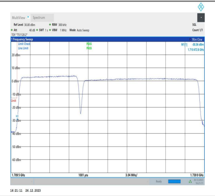
10MHz-20MHz_64QAM@64QAM-64QAM@64QAM_132027-132171_50RB#0@50RB#0-100RB#0@100RB#0
