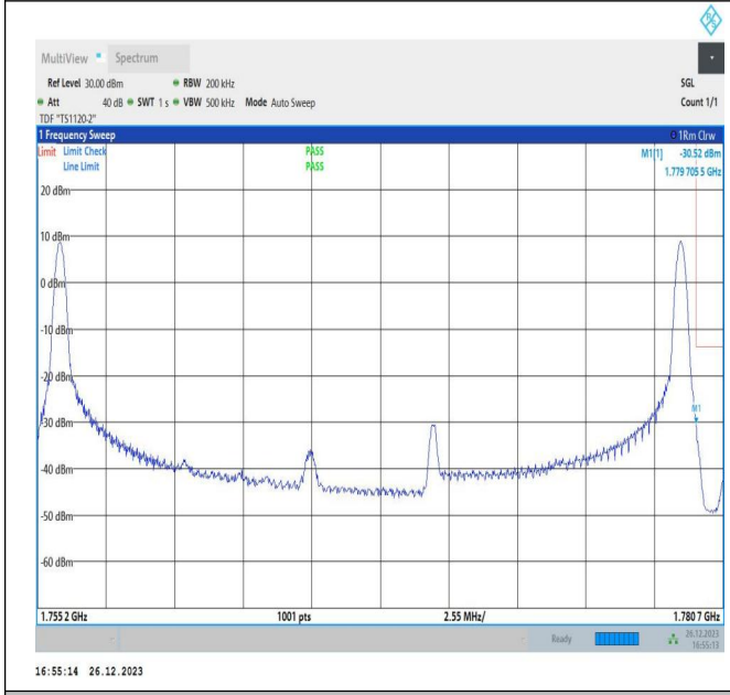
15MHz-10MHz_64QAM@64QAM-64QAM@64QAM_132499-132619_1RB#0@75RB#0-1RB#49@50RB#0
