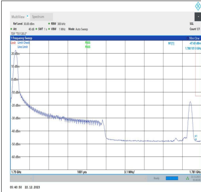
15MHz-15MHz_16QAM@16QAM-16QAM_132447-132597_1RB#0@75RB#0-0RB#0@75RB#0
