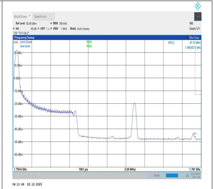
10MHz-20MHz_16QAM@16QAM-16QAM@16QAM_132428-132572_1RB#0@50RB#0-0RB#0@100RB#0
