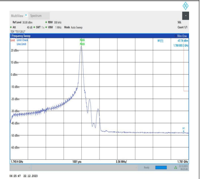
15MHz-20MHz_QPSK@QPSK-QPSK@QPSK_132401-1325 72_1RB#74@75RB#0-0RB#0@100RB#0
