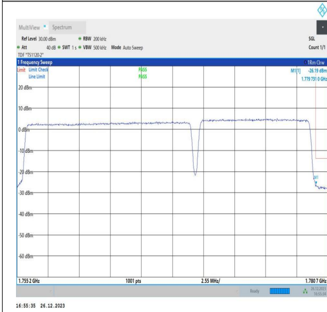
15MHz-10MHz_64QAM@64QAM-64QAM@64QAM_132499-132619_75RB#0@75RB#0-50RB#0@50RB#0
