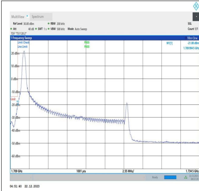
15MHz-10MHz_16QAM@16QAM-16QAM@16QAM_132047-132167_1RB#0@75RB#0-0RB#0@50RB#0
