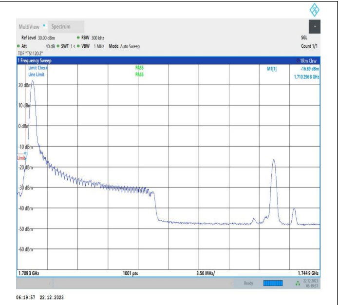
15MHz-20MHz_16QAM@16QAM-16QAM@16QAM_132050-132221_1RB#0@75RB#0-0RB#0@100RB#0
