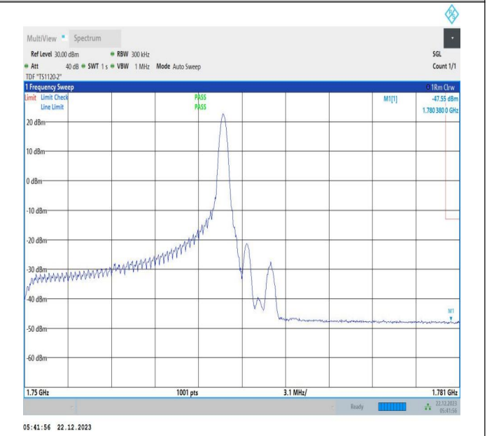
15MHz-15MHz_16QAM@16QAM-16QAM@16QAM_132447-132597_1RB#74@75RB#0-0RB#0@75RB#0
