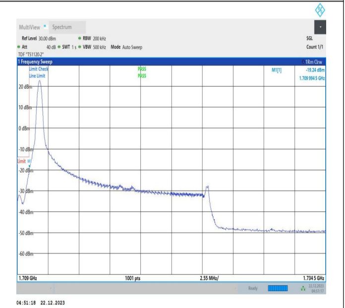
15MHz-10MHz_QPSK@QPSK-QPSK@QPSK_132047-132167_1RB#0@75RB#0-0RB#0@50RB#0
