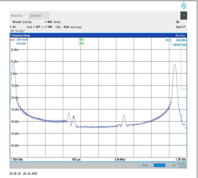
10MHz-20MHz_64QAM@64QAM-64QAM_132428-132572_1RB#0@50RB#0-1RB#99@100RB#0
