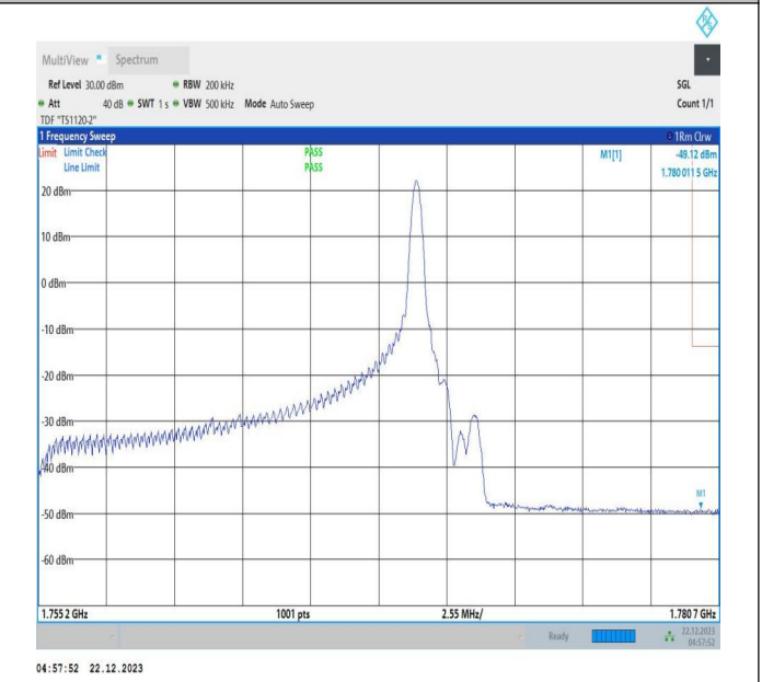
15MHz-10MHz_16QAM@16QAM-16QAM@16QAM_132499-132619_1RB#74@75RB#0-0RB#0@50RB#0
