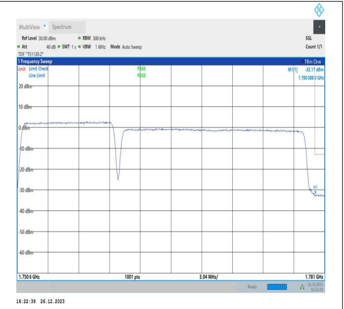
10MHz-20MHz_64QAM@64QAM-64QAM@64QAM_132428-132572_50RB#0@50RB#0-100RB#0@100RB#0
