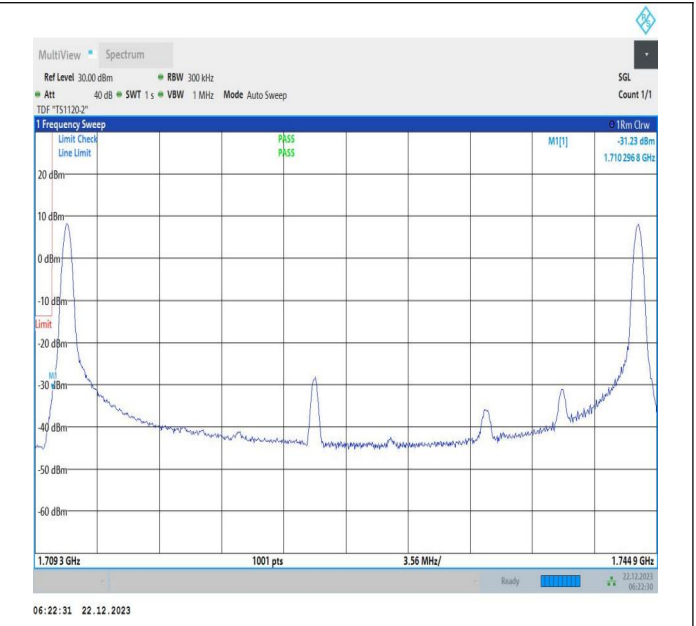
15MHz-20MHz_QPSK@QPSK-QPSK@QPSK_132050-1322 21_1RB#0@75RB#0-1RB#99@100RB#0
