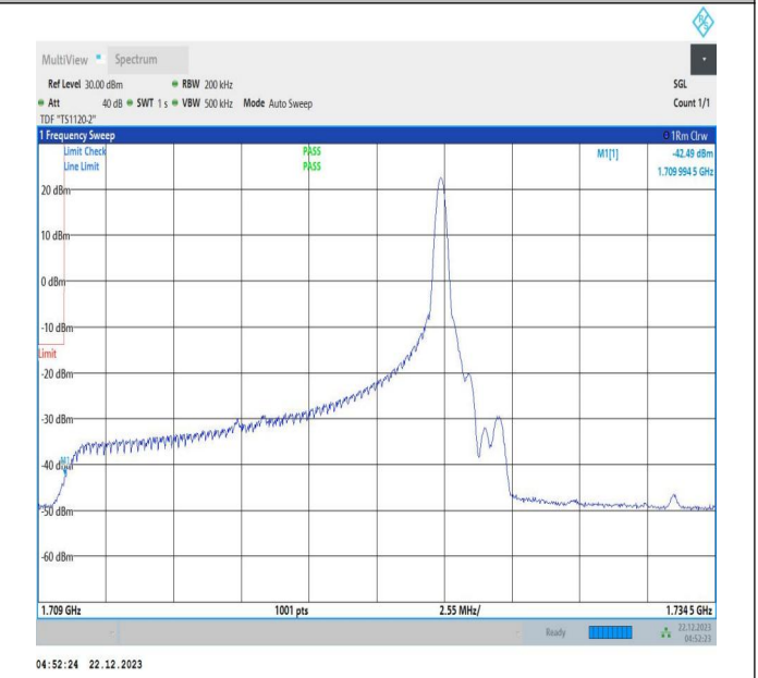
15MHz-10MHz_QPSK@QPSK-QPSK@QPSK_132047-132167_1RB#74@75RB#0-0RB#0@50RB#0
