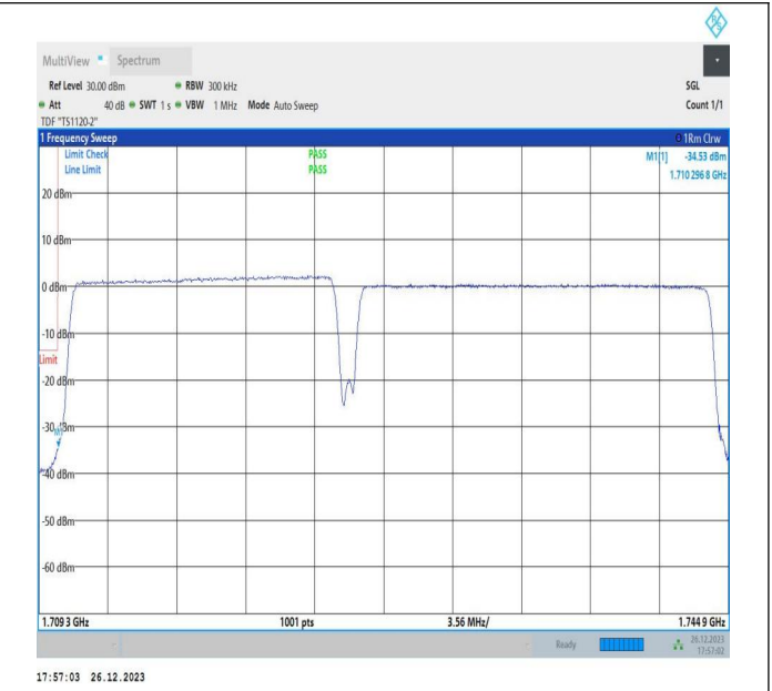
15MHz-20MHz_64QAM@64QAM-64QAM@64QAM_132050- 132221_75RB#0@75RB#0-100RB#0@100RB#0
