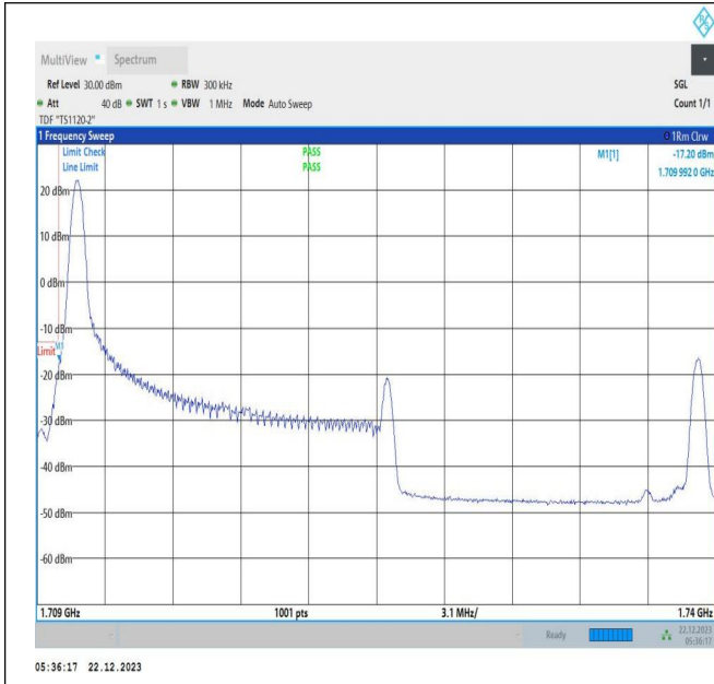
15MHz-15MHz_16QAM@16QAM-16QAM@16QAM_132047-132197_1RB#0@75RB#0-0RB#0@75RB#0
