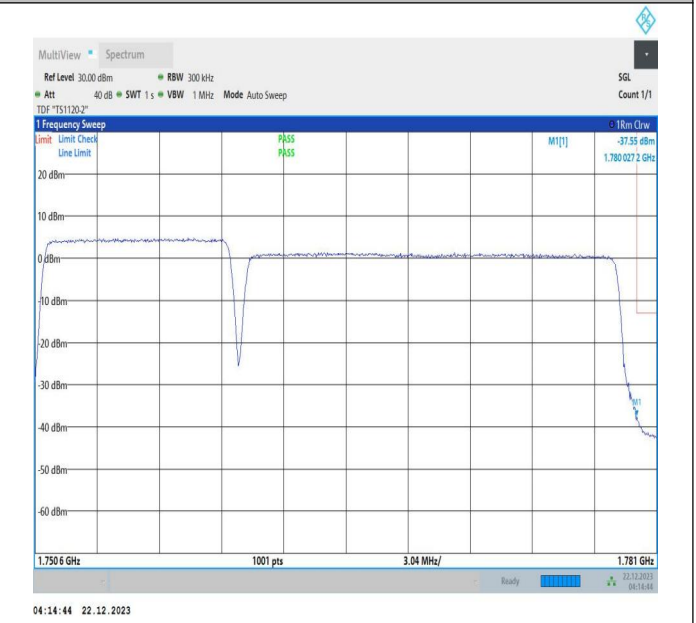
10MHz-20MHz_QPSK@QPSK-QPSK@QPSK_132428-1325 72_50RB#0@50RB#0-100RB#0@100RB#0
