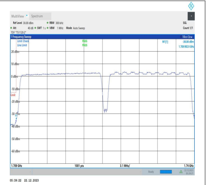
15MHz-15MHz_QPSK@QPSK-QPSK@QPSK_132047-1321 97_75RB#0@75RB#0-75RB#0@75RB#0
