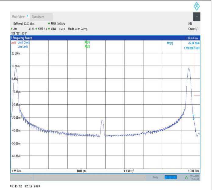
15MHz-15MHz_16QAM@16QAM-16QAM@16QAM_132447-132597_1RB#0@75RB#0-1RB#74@75RB#0
