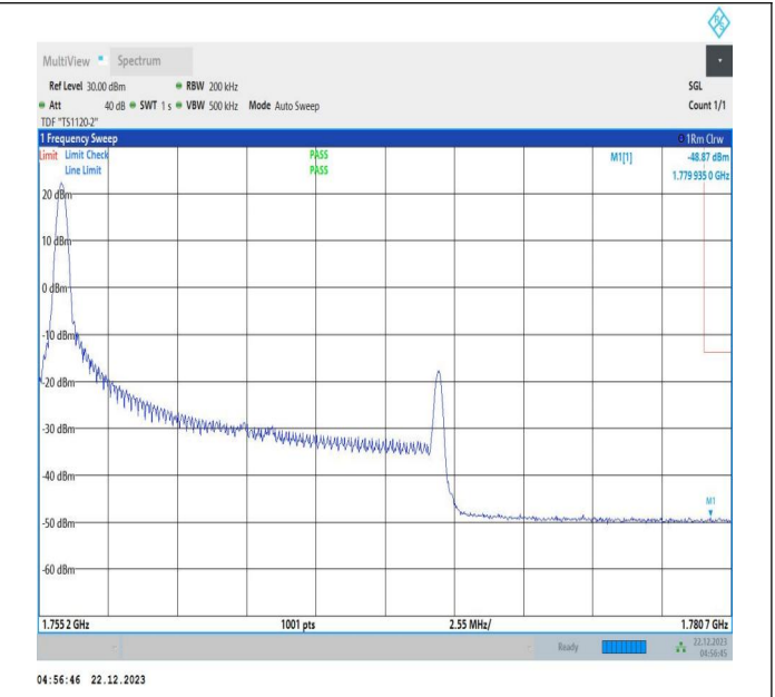
15MHz-10MHz_16QAM@16QAM-16QAM@16QAM_132499-132619_1RB#0@75RB#0-0RB#0@50RB#0
