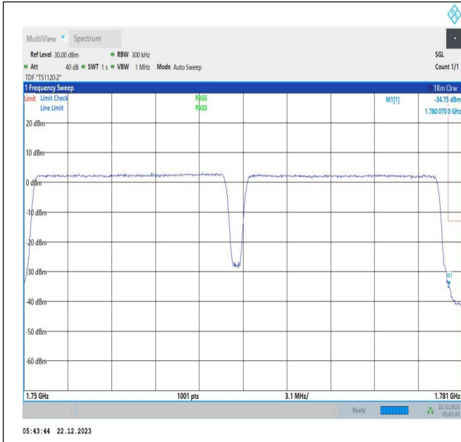
15MHz-15MHz_QPSK@QPSK-QPSK@QPSK_132447-132597_75RB#0@75RB#0-75RB#0@75RB#0
