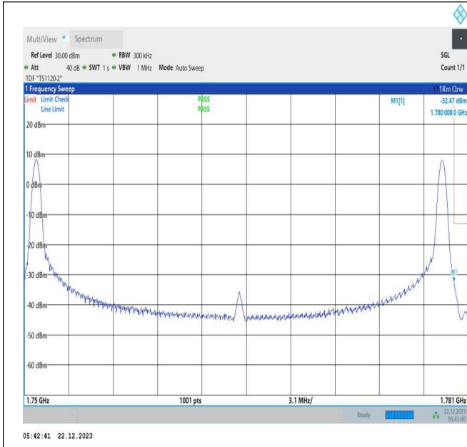
15MHz-15MHz_QPSK@QPSK-QPSK@QPSK_132447-132597_1RB#0@75RB#0-1RB#74@75RB#0
