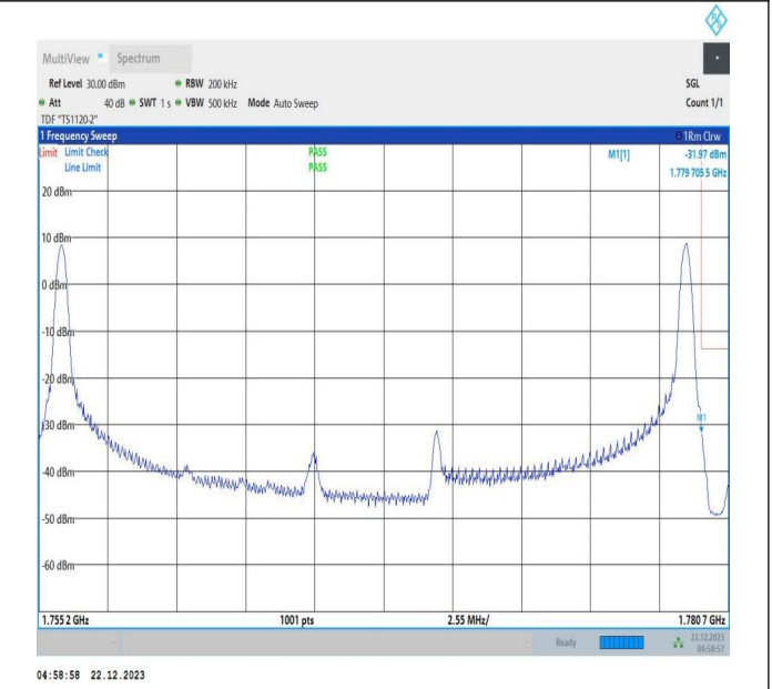
15MHz-10MHz_16QAM@16QAM-16QAM@16QAM_132499-132619_1RB#0@75RB#0-1RB#49@50RB#0
