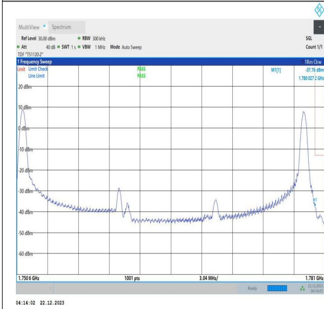
10MHz-20MHz_16QAM@16QAM-16QAM@16QAM_132428 -132572_1RB#0@50RB#0-1RB#99@100RB#0
