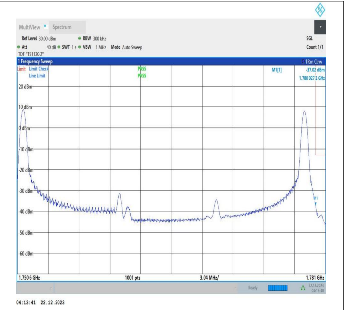
10MHz-20MHz_QPSK@QPSK-QPSK@QPSK_132428-1325 72_1RB#0@50RB#0-1RB#99@100RB#0
