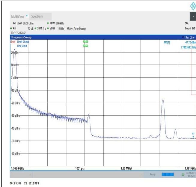
15MHz-20MHz_16QAM@16QAM-16QAM@16QAM_132401 -132572_1RB#0@75RB#0-0RB#0@100RB#0
