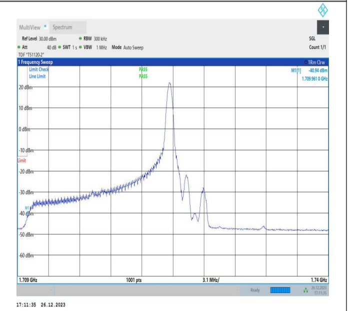
15MHz-15MHz_64QAM@64QAM-64QAM@64QAM_132047-132197_1RB#74@75RB#0-0RB#0@75RB#0
