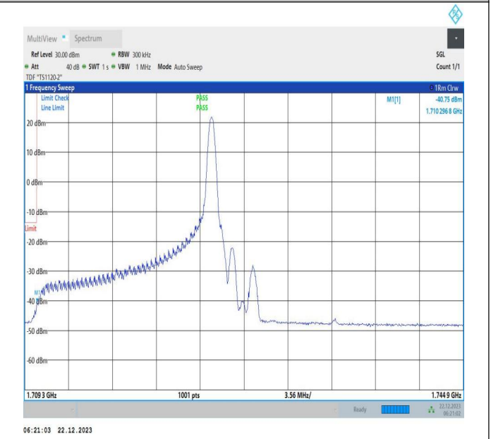
15MHz-20MHz_16QAM@16QAM-16QAM@16QAM_132050-132221_1RB#74@75RB#0-0RB#0@100RB#0
