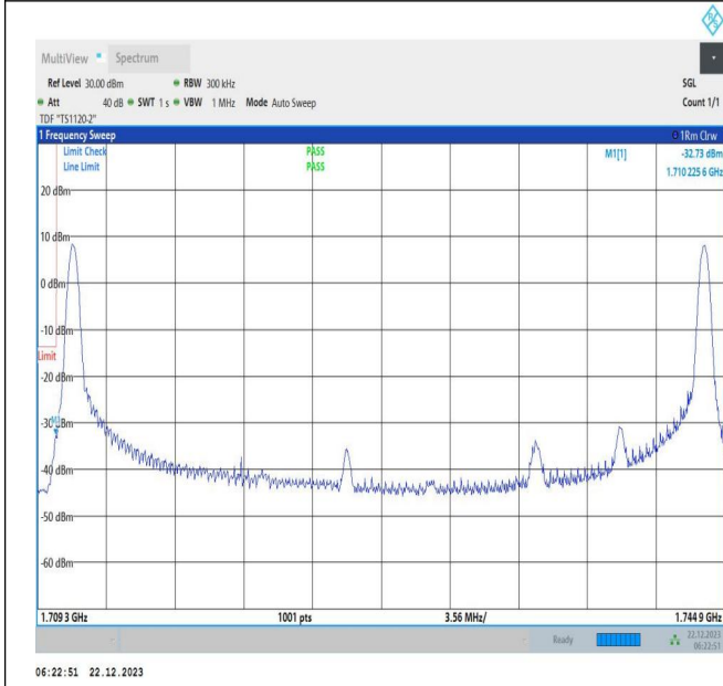
15MHz-20MHz_16QAM@16QAM-16QAM@16QAM_132050 -132221_1RB#0@75RB#0-1RB#99@100RB#0
