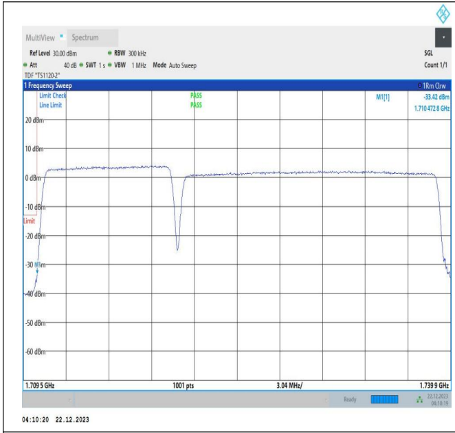
10MHz-20MHz_QPSK@QPSK-QPSK@QPSK_132027-132171_50RB#0@50RB#0-100RB#0@100RB#0
