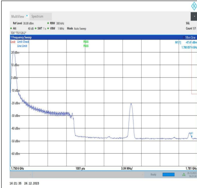
10MHz-20MHz_64QAM@64QAM-64QAM_132428 -132572_1RB#0@50RB#0-0RB#0@100RB#0
