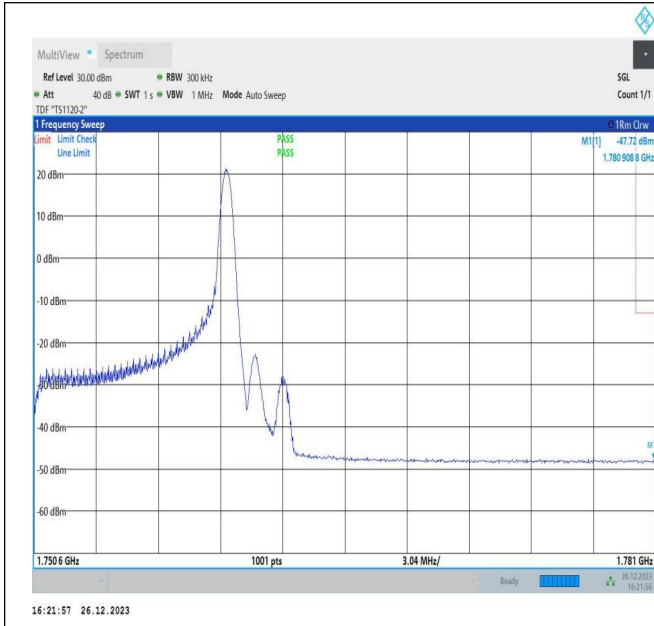
10MHz-20MHz_64QAM@64QAM-64QAM_132428-132572_1RB#49@50RB#0-0RB#0@100RB#0
