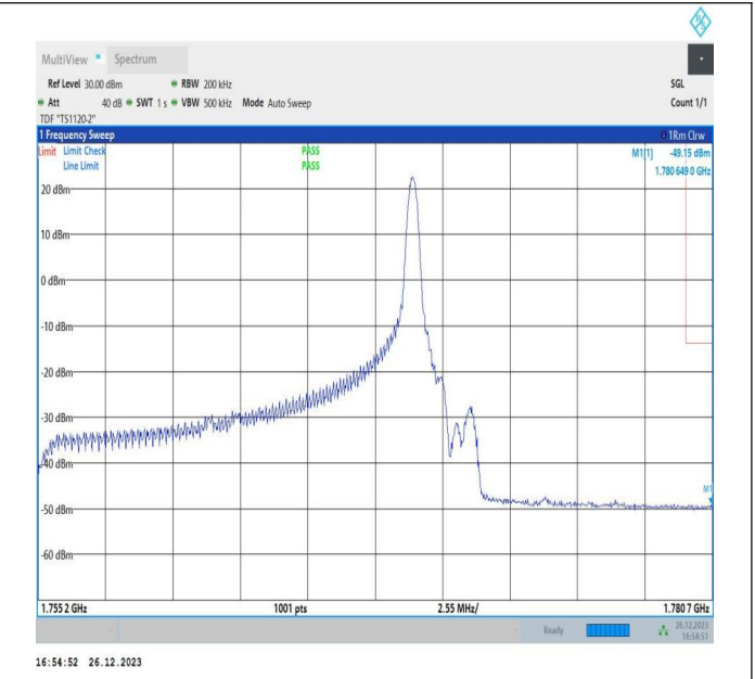
15MHz-10MHz_64QAM@64QAM-64QAM_132499-132619_1RB#74@75RB#0-0RB#0@50RB#0
