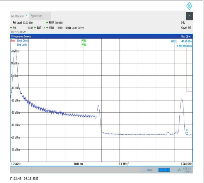
15MHz-15MHz_64QAM@64QAM-64QAM@64QAM_132447-132597_1RB#0@75RB#0-0RB#0@75RB#0
