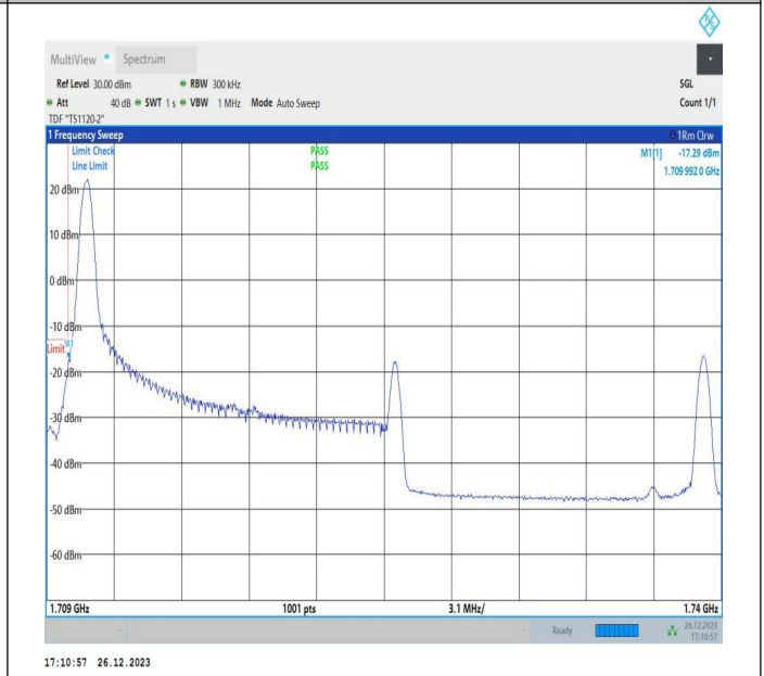
15MHz-15MHz_64QAM@64QAM-64QAM@64QAM_132047-132197_1RB#0@75RB#0-0RB#0@75RB#0
