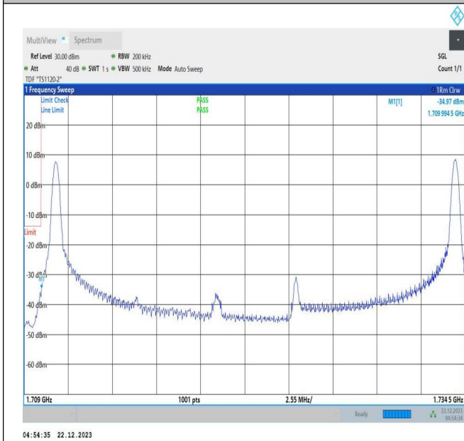
15MHz-10MHz_16QAM@16QAM-16QAM@16QAM_132047-132167_1RB#0@75RB#0-1RB#49@50RB#0
