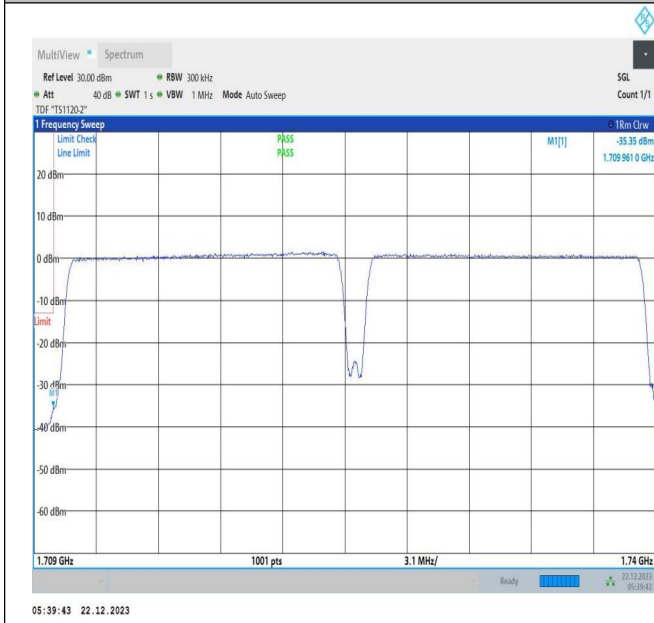
15MHz-15MHz_16QAM@16QAM-16QAM@16QAM_132047 -132197_75RB#0@75RB#0-75RB#0@75RB#0
