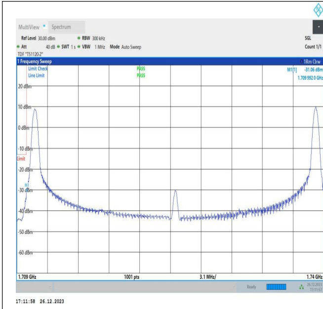
15MHz-15MHz_64QAM@64QAM-64QAM_132047 -132197_1RB#0@75RB#0-1RB#74@75RB#0
