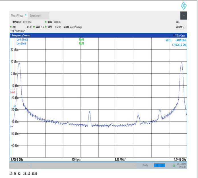
15MHz-20MHz_64QAM@64QAM-64QAM@64QAM_132050-132221_1RB#0@75RB#0-1RB#99@100RB#0
