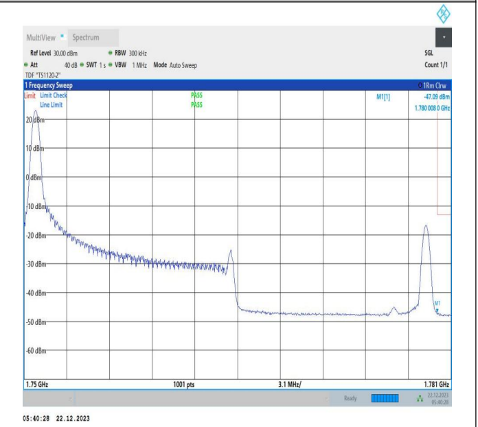
15MHz-15MHz_QPSK@QPSK-QPSK@QPSK_132447-1325 97_1RB#0@75RB#0-0RB#0@75RB#0
