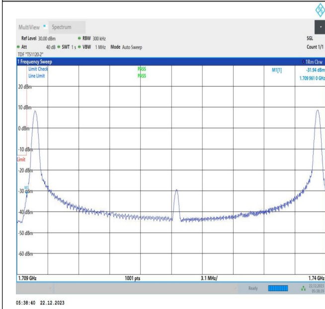
15MHz-15MHz_16QAM@16QAM-16QAM@16QAM_132047-132197_1RB#0@75RB#0-1RB#74@75RB#0
