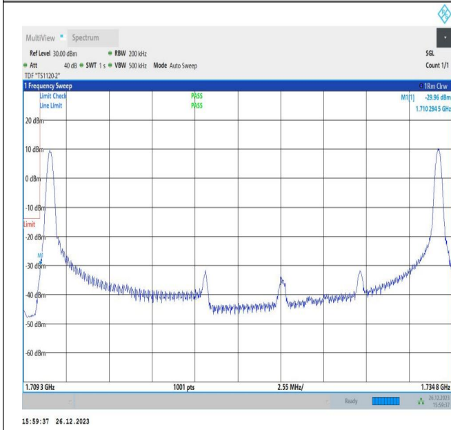
10MHz-15MHz_64QAM@64QAM-64QAM@64QAM_132025-132145_1RB#0@50RB#0-1RB#74@75RB#0
