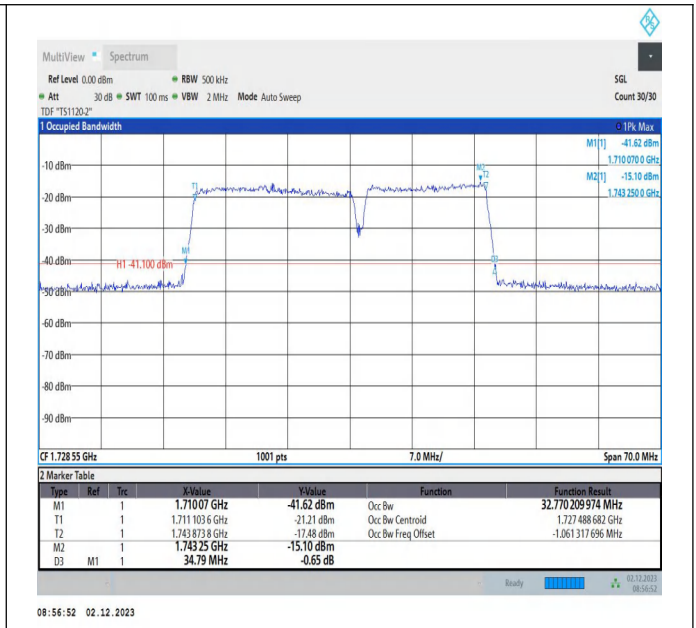
66-66-20MHz-15MHz-16QAM-16QAM-132072-132243-100R B#0-75RB#0-PASS
