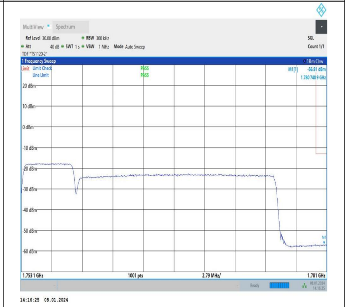
5MHz-20MHz_16QAM@16QAM-16QAM@16QAM_132428-132572_25RB#0@25RB#0-100RB#0@100RB#0
