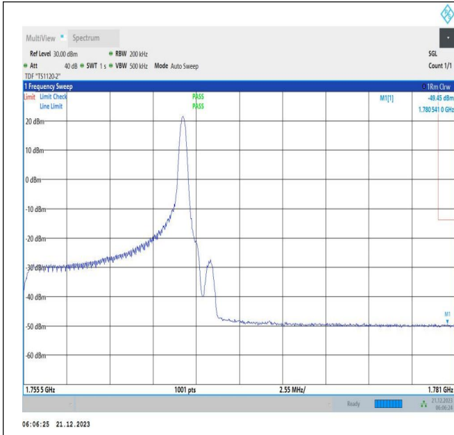
10MHz-15MHz_16QAM@16QAM-16QAM@16QAM_132477-132597_1RB#49@50RB#0-0RB#0@75RB#0
