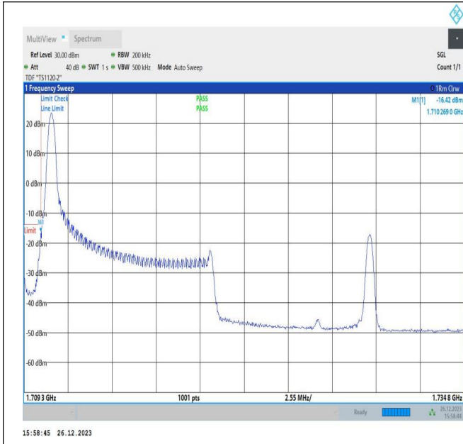
10MHz-15MHz_64QAM@64QAM-64QAM_132025-132145_1RB#0@50RB#0-0RB#0@75RB#0
