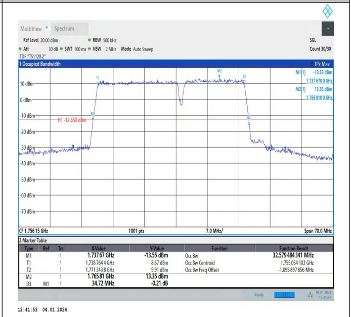
66-66-20MHz-15MHz-64QAM-64QAM-132348-132519-100RB#0-75RB#0-PASS
