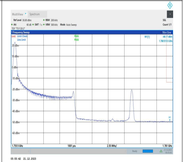
10MHz-15MHz_QPSK@QPSK-QPSK@QPSK_132477-132597_1RB#0@50RB#0-0RB#0@75RB#0
