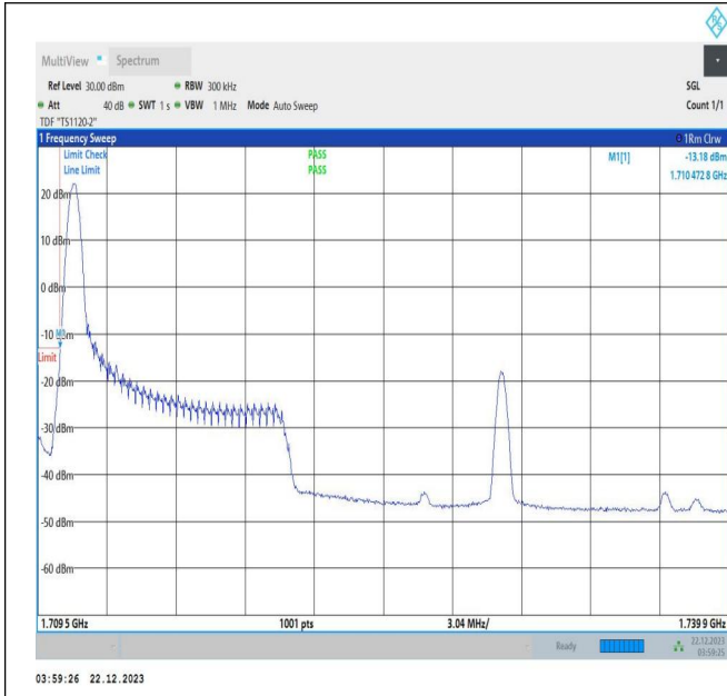
10MHz-20MHz_16QAM@16QAM-16QAM@16QAM_132027-132171_1RB#0@50RB#0-0RB#0@100RB#0
