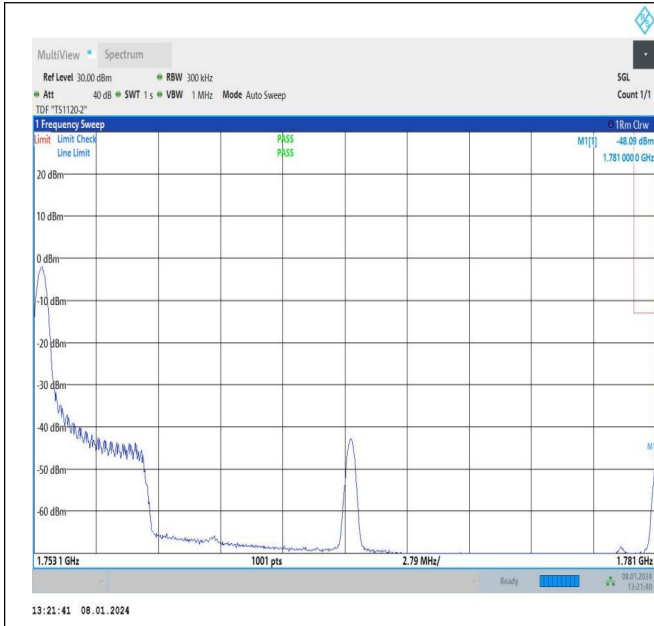
5MHz-20MHz_64QAM@64QAM-64QAM@64QAM_132428-132572_1RB#0@25RB#0-0RB#0@100RB#0
