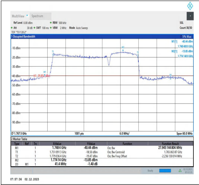
66-66-20MHz-10MHz-16QAM-16QAM-132473-132617-100R B#0-50RB#0-PASS
