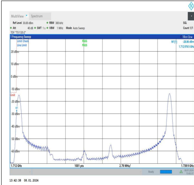
5MHz-20MHz_64QAM@64QAM-64QAM@64QAM_132027-132171_1RB#0@25RB#0-1RB#99@100RB#0
