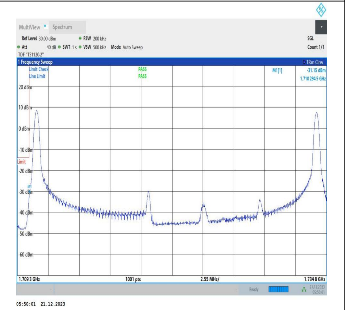
10MHz-15MHz_16QAM@16QAM-16QAM_132025-132145_1RB#0@50RB#0-1RB#74@75RB#0
