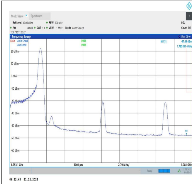
5MHz-20MHz_16QAM@16QAM-16QAM@16QAM_132428-132572_1RB#24@25RB#0-0RB#0@100RB#0
