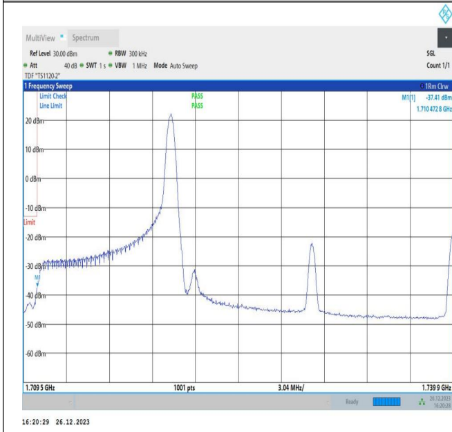
10MHz-20MHz_64QAM@64QAM-64QAM@64QAM_132027-132171_1RB#49@50RB#0-0RB#0@100RB#0
