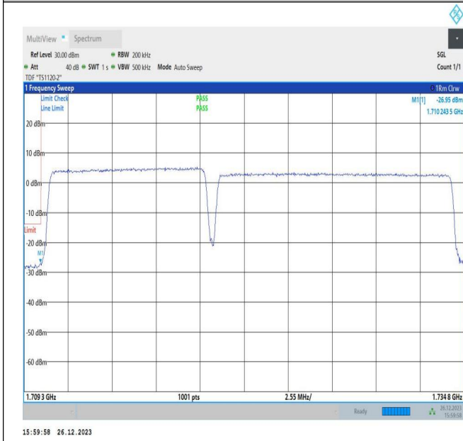
10MHz-15MHz_64QAM@64QAM-64QAM@64QAM_132025-132145_50RB#0@50RB#0-75RB#0@75RB#0
