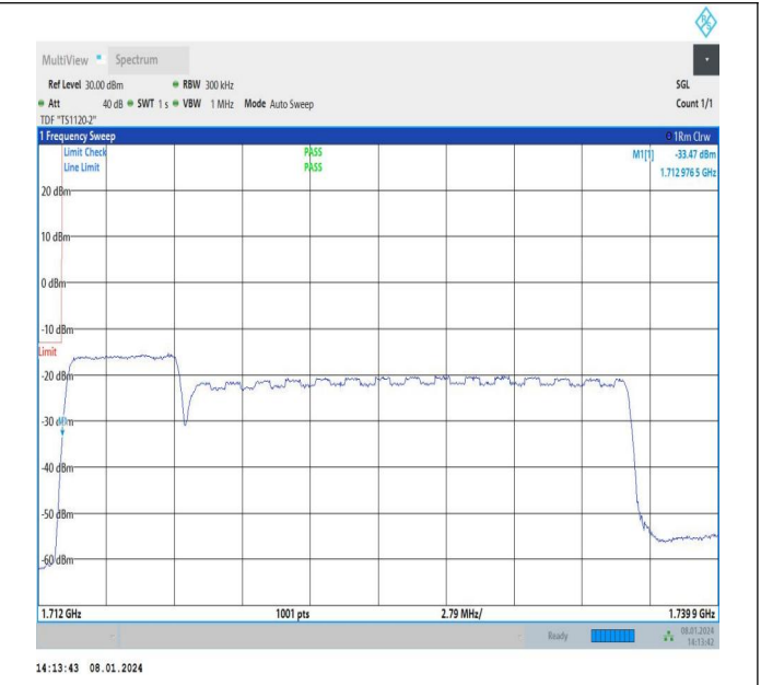
5MHz-20MHz_QPSK@QPSK-QPSK@QPSK_132027-132171_25RB#0@25RB#0-100RB#0@100RB#0
