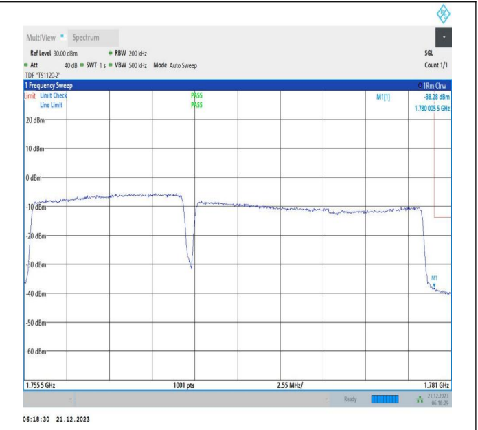
10MHz-15MHz_QPSK@QPSK-QPSK@QPSK_132477-1325 97_50RB#0@50RB#0-75RB#0@75RB#0
