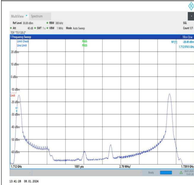
5MHz-20MHz_QPSK@QPSK-QPSK@QPSK_132027-132171_1RB#0@25RB#0-1RB#99@100RB#0
