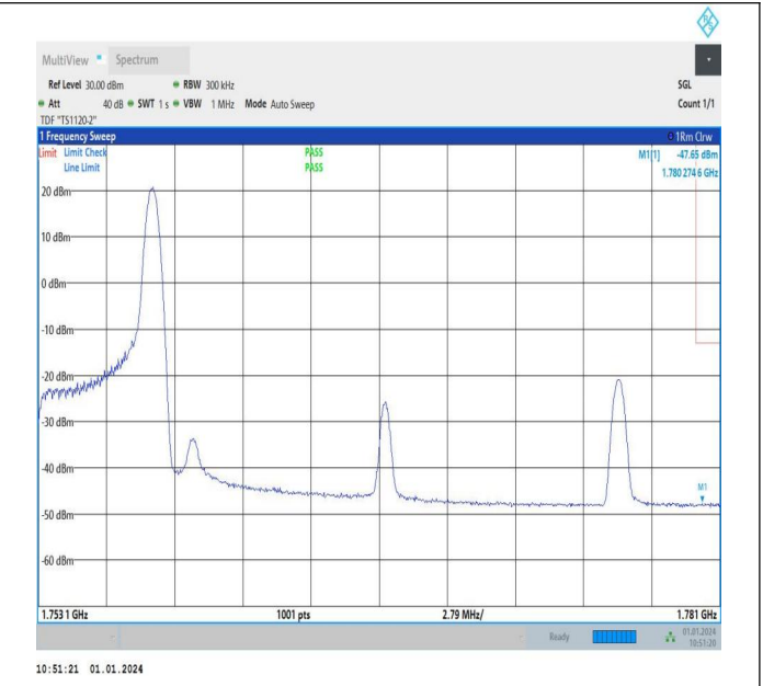
5MHz-20MHz_64QAM@64QAM-64QAM@64QAM_132428-132572_1RB#24@25RB#0-0RB#0@100RB#0
