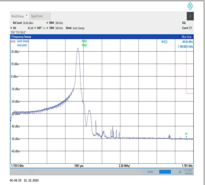
10MHz-15MHz_QPSK@QPSK-QPSK@QPSK_132477-132597_1RB#49@50RB#0-0RB#0@75RB#0
