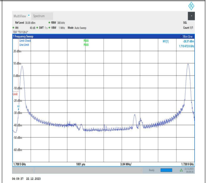
10MHz-20MHz_16QAM@16QAM-16QAM@16QAM_132027-132171_1RB#0@50RB#0-1RB#99@100RB#0
