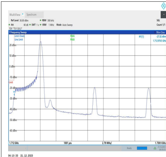
5MHz-20MHz_QPSK@QPSK-QPSK@QPSK_132027-1321 71_1RB#24@25RB#0-0RB#0@100RB#0
