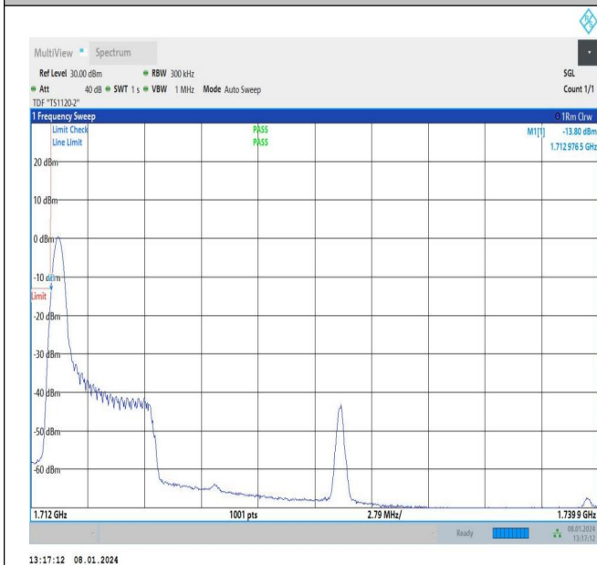
5MHz-20MHz_QPSK@QPSK-QPSK@QPSK_132027-1321 71_1RB#0@25RB#0-0RB#0@100RB#0
