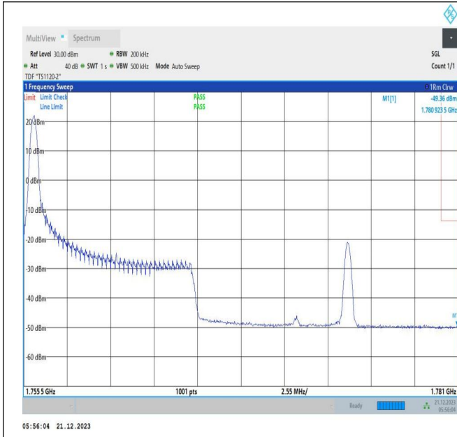
10MHz-15MHz_16QAM@16QAM-16QAM@16QAM_132477-132597_1RB#0@50RB#0-0RB#0@75RB#0
