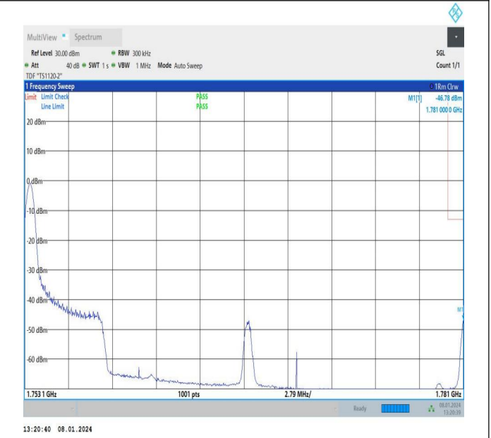
5MHz-20MHz_16QAM@16QAM-16QAM@16QAM_132428-132572_1RB#0@25RB#0-0RB#0@100RB#0
