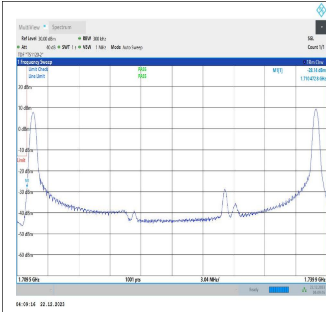
10MHz-20MHz_QPSK@QPSK-QPSK@QPSK_132027-132171_1RB#0@50RB#0-1RB#99@100RB#0
