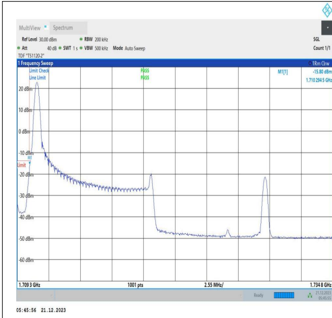
10MHz-15MHz_QPSK@QPSK-QPSK@QPSK_132025-132145_1RB#0@50RB#0-0RB#0@75RB#0
