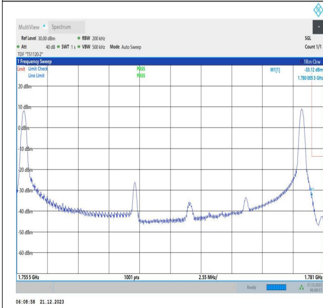
10MHz-15MHz_16QAM@16QAM-16QAM@16QAM_132477-132597_1RB#0@50RB#0-1RB#74@75RB#0
