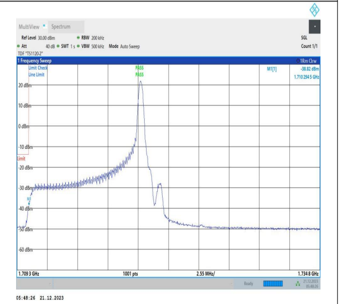
10MHz-15MHz_16QAM@16QAM-16QAM@16QAM_132025-132145_1RB#49@50RB#0-0RB#0@75RB#0
