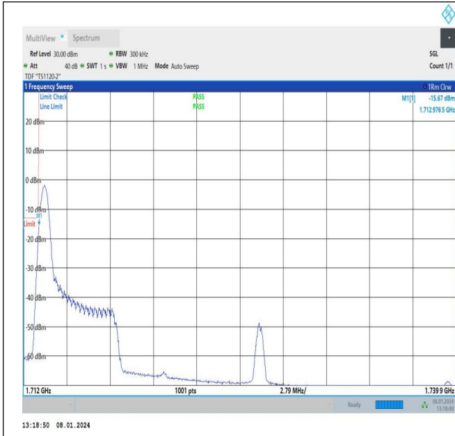
5MHz-20MHz_64QAM@64QAM-64QAM@64QAM_132027-132171_1RB#0@25RB#0-0RB#0@100RB#0
