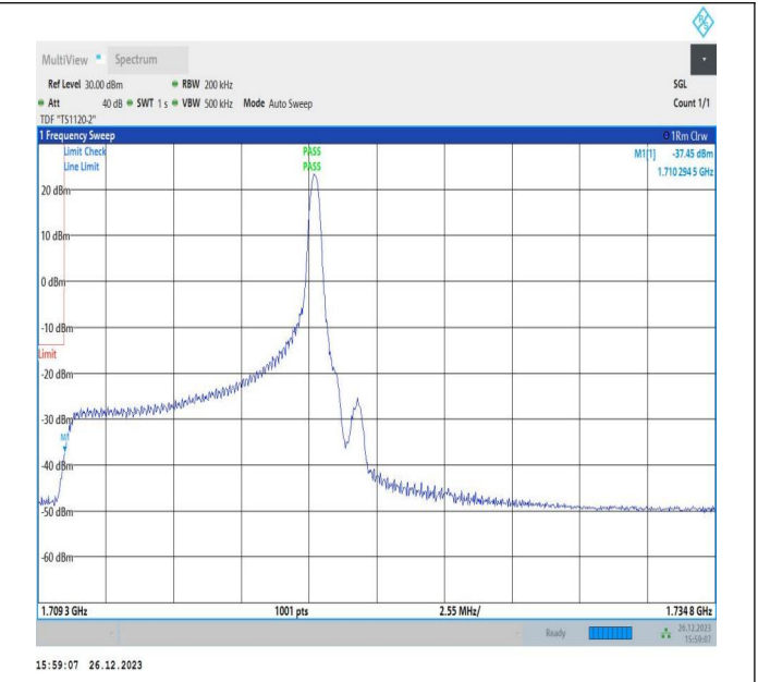
10MHz-15MHz_64QAM@64QAM-64QAM_132025-132145_1RB#49@50RB#0-0RB#0@75RB#0
