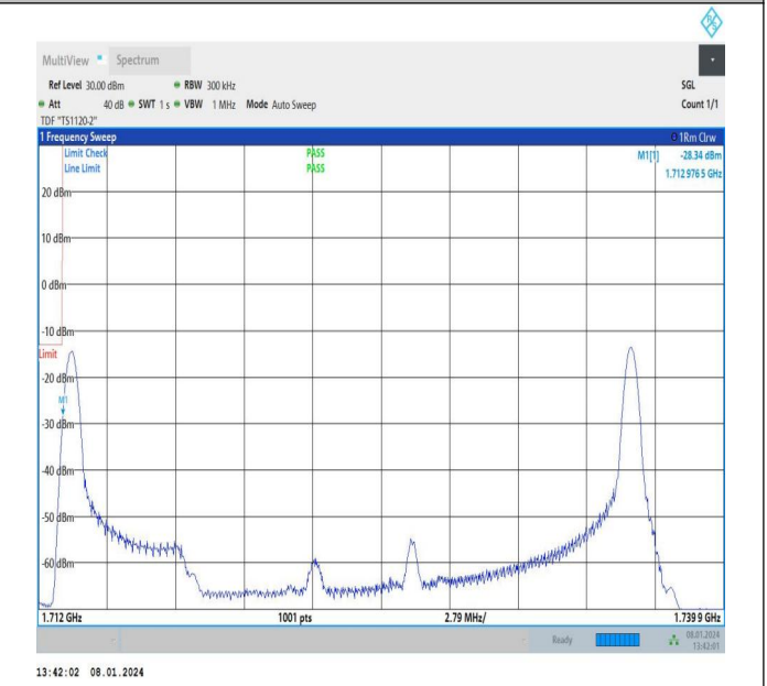
5MHz-20MHz_16QAM@16QAM-16QAM@16QAM_132027-132171_1RB#0@25RB#0-1RB#99@100RB#0
