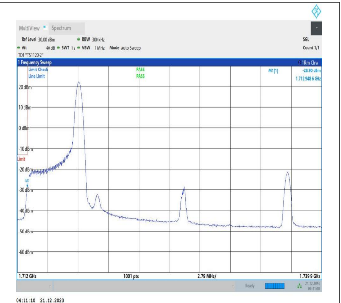
5MHz-20MHz_16QAM@16QAM-16QAM@16QAM_132027-1 32171_1RB#24@25RB#0-0RB#0@100RB#0
