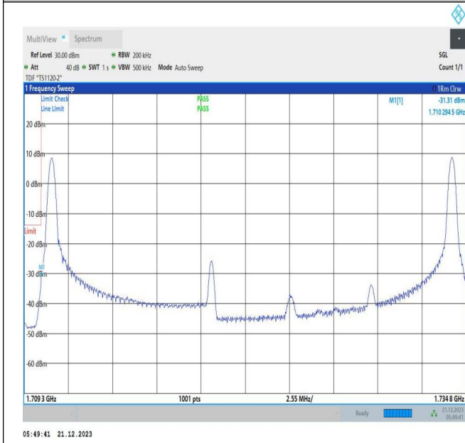
10MHz-15MHz_QPSK@QPSK-QPSK_132025-132145_1RB#0@50RB#0-1RB#74@75RB#0
