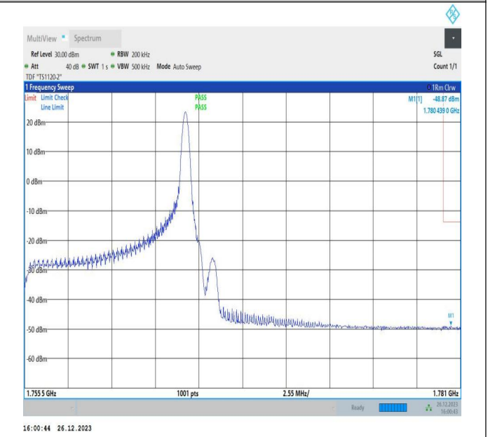
10MHz-15MHz_64QAM@64QAM-64QAM@64QAM_132477-132597_1RB#49@50RB#0-0RB#0@75RB#0
