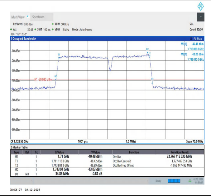
66-66-20MHz-15MHz-QPSK-QPSK-132072-132243-100RB#0-75RB#0-PASS
