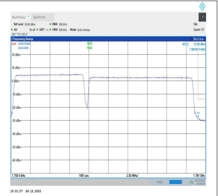
10MHz-15MHz_64QAM@64QAM-64QAM@64QAM_132477-132597_50RB#0@50RB#0-75RB#0@75RB#0
