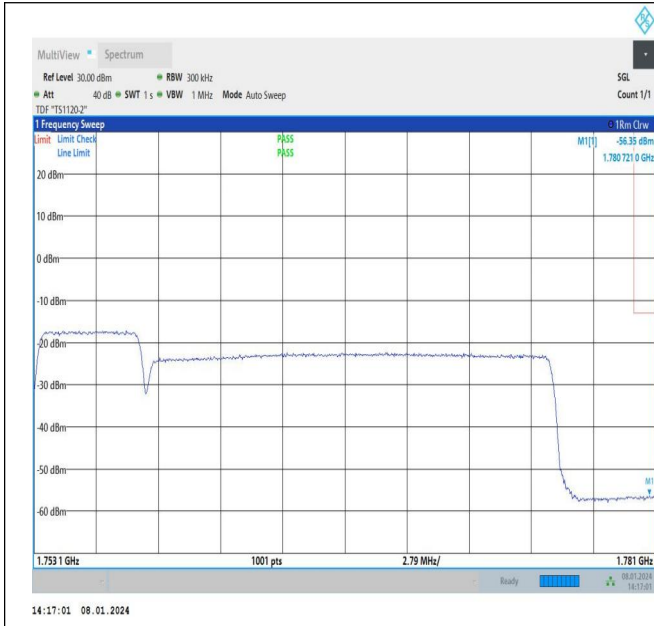
5MHz-20MHz_64QAM@64QAM-64QAM@64QAM_132428-132572_25RB#0@25RB#0-100RB#0@100RB#0
