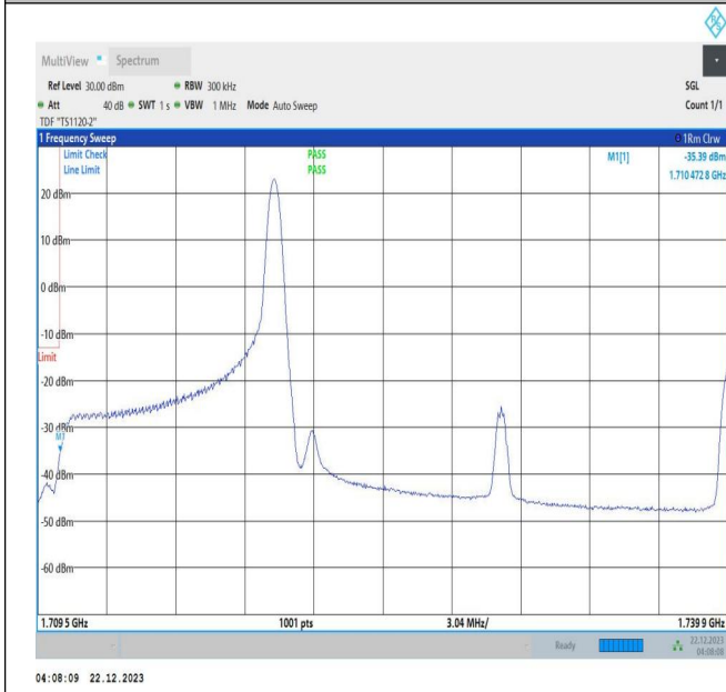
10MHz-20MHz_QPSK@QPSK-QPSK@QPSK_132027-132171_1RB#49@50RB#0-0RB#0@100RB#0
