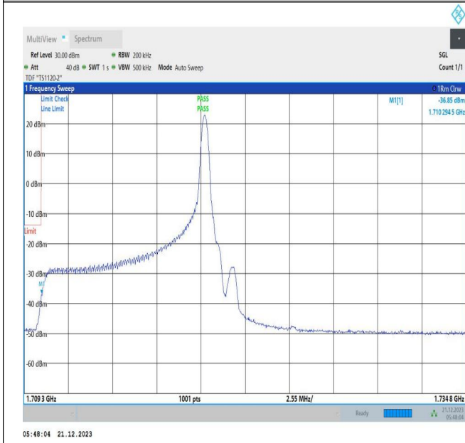
10MHz-15MHz_QPSK@QPSK-QPSK@QPSK_132025-132145_1RB#49@50RB#0-0RB#0@75RB#0
