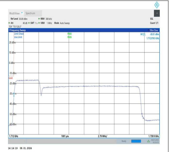
5MHz-20MHz_16QAM@16QAM-16QAM@16QAM_132027-132171_25RB#0@25RB#0-100RB#0@100RB#0
