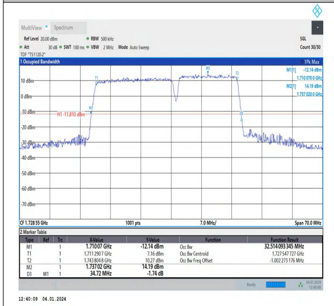
66-66-20MHz-15MHz-64QAM-64QAM-132072-132243-100RB#0-75RB#0-PASS
