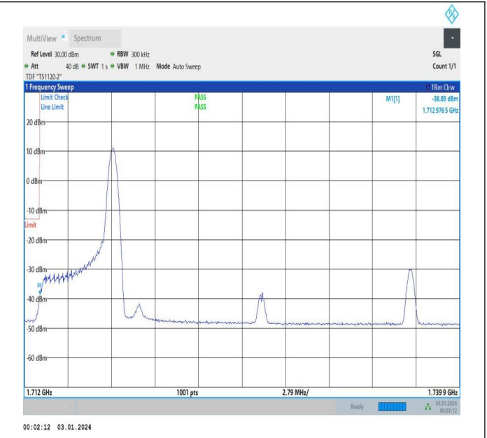
5MHz-20MHz_64QAM@64QAM-64QAM@64QAM_132027-132171_1RB#24@25RB#0-0RB#0@100RB#0
