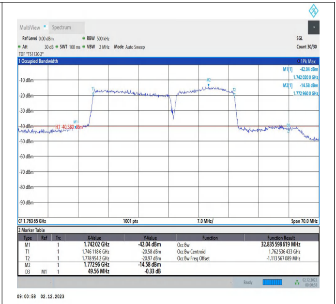
66-66-20MHz-15MHz-16QAM-16QAM-132423-132594-100RB#0-75RB#0-PASS
