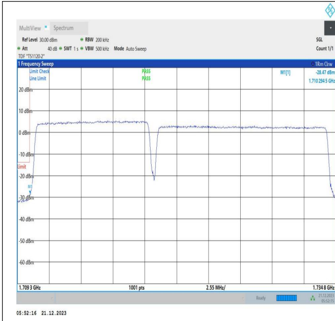
10MHz-15MHz_QPSK@QPSK-QPSK@QPSK_132025-132145_50RB#0@50RB#0-75RB#0@75RB#0
