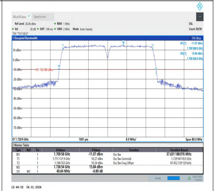
66-66-20MHz-20MHz-64QAM-64QAM-132072-132270-100R B#0-100RB#0-PASS
