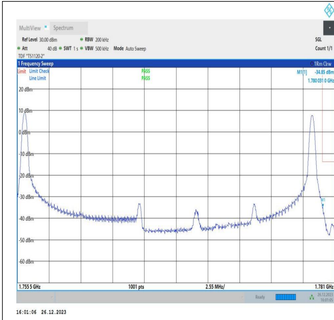
10MHz-15MHz_64QAM@64QAM-64QAM_132477 -132597_1RB#0@50RB#0-1RB#74@75RB#0
