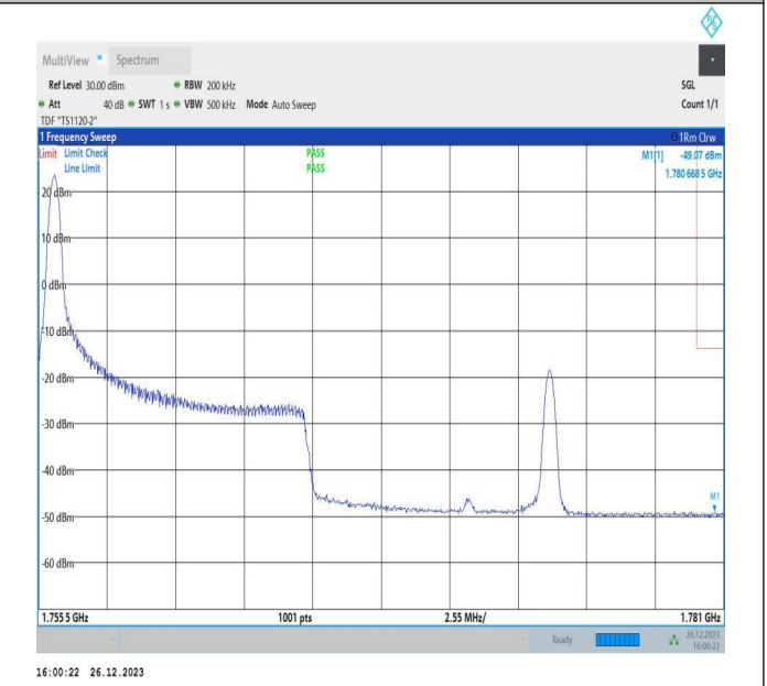
10MHz-15MHz_64QAM@64QAM-64QAM@64QAM_132477-132597_1RB#0@50RB#0-0RB#0@75RB#0
