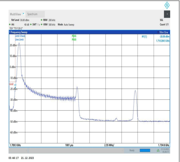
10MHz-15MHz_16QAM@16QAM-16QAM@16QAM_132025-132145_1RB#0@50RB#0-0RB#0@75RB#0
