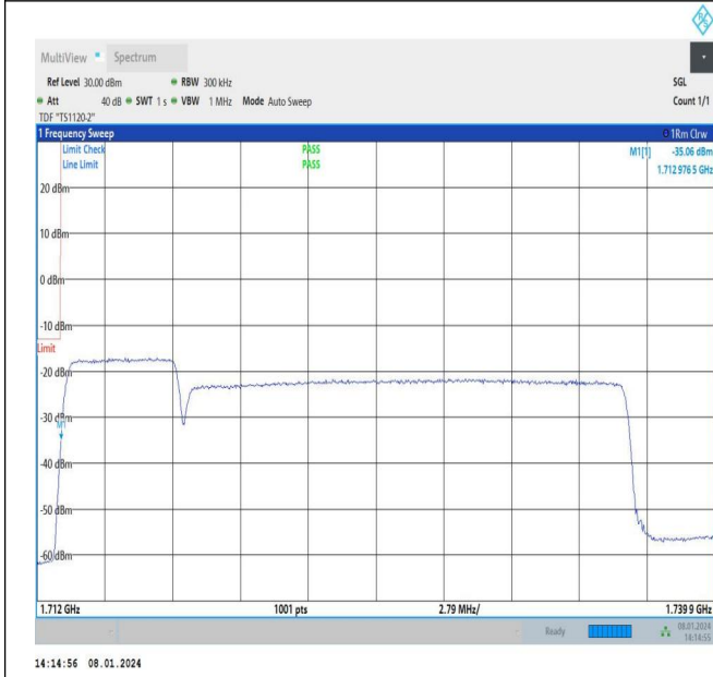
5MHz-20MHz_64QAM@64QAM-64QAM@64QAM_132027-132171_25RB#0@25RB#0-100RB#0@100RB#0
