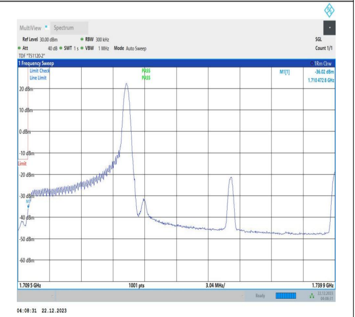
10MHz-20MHz_16QAM@16QAM-16QAM@16QAM_132027-132171_1RB#49@50RB#0-0RB#0@100RB#0
