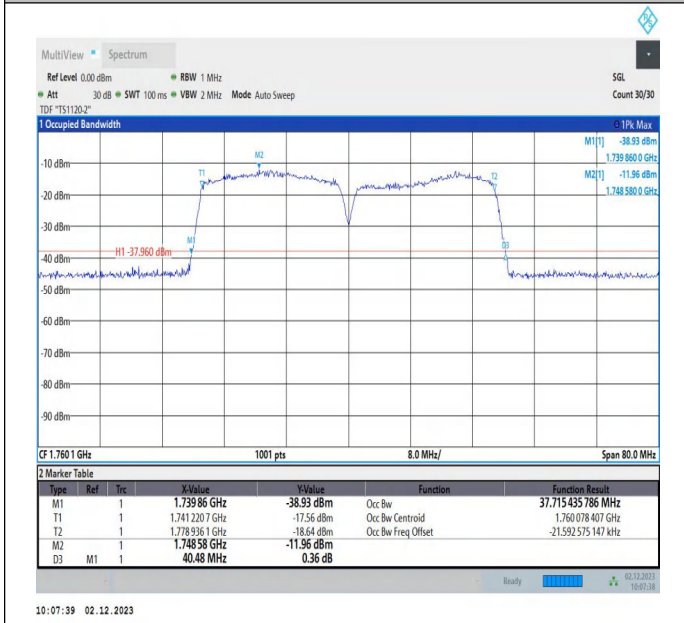
66-66-20MHz-20MHz-16QAM-16QAM-132374-132572-100R B#0-100RB#0-PASS
