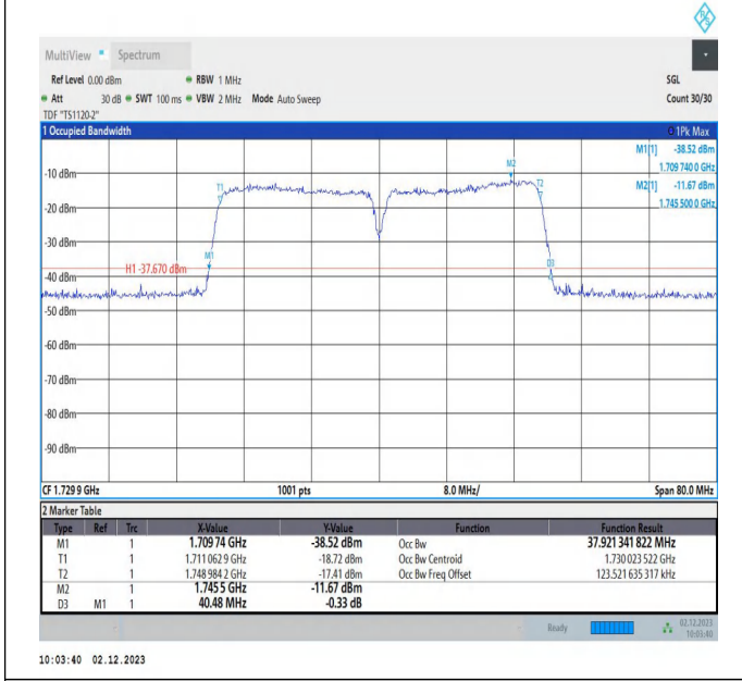
66-66-20MHz-20MHz-16QAM-16QAM-132072-132270-100R B#0-100RB#0-PASS
