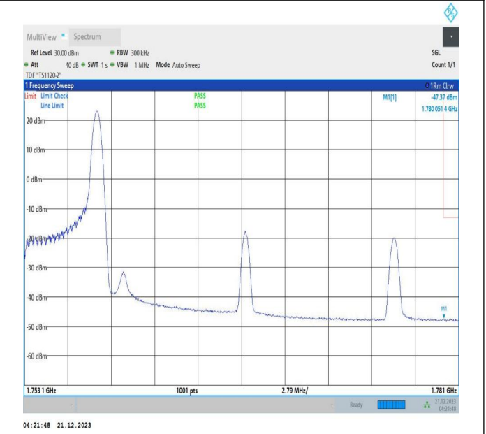
5MHz-20MHz_QPSK@QPSK-QPSK@QPSK_132428-132572_1RB#24@25RB#0-0RB#0@100RB#0
