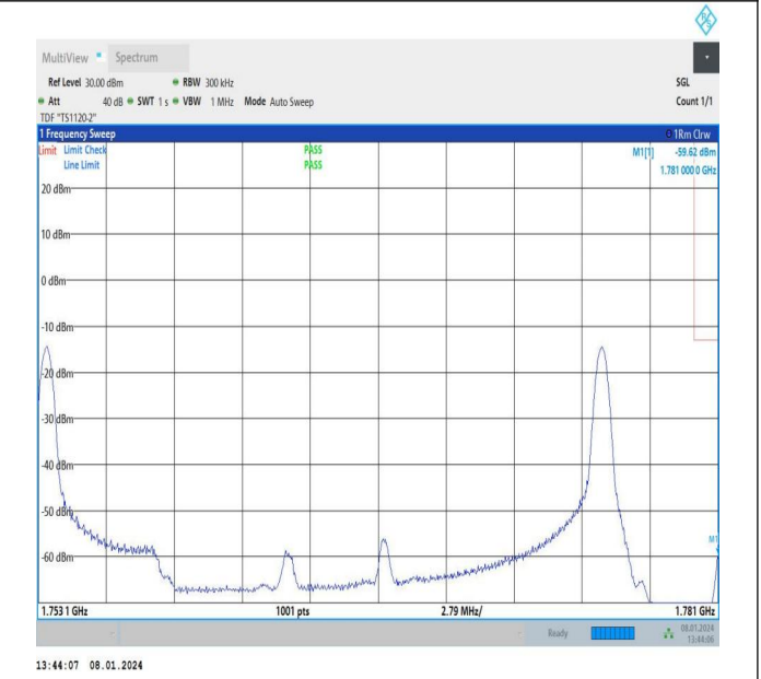
5MHz-20MHz_16QAM@16QAM-16QAM@16QAM_132428-132572_1RB#0@25RB#0-1RB#99@100RB#0
