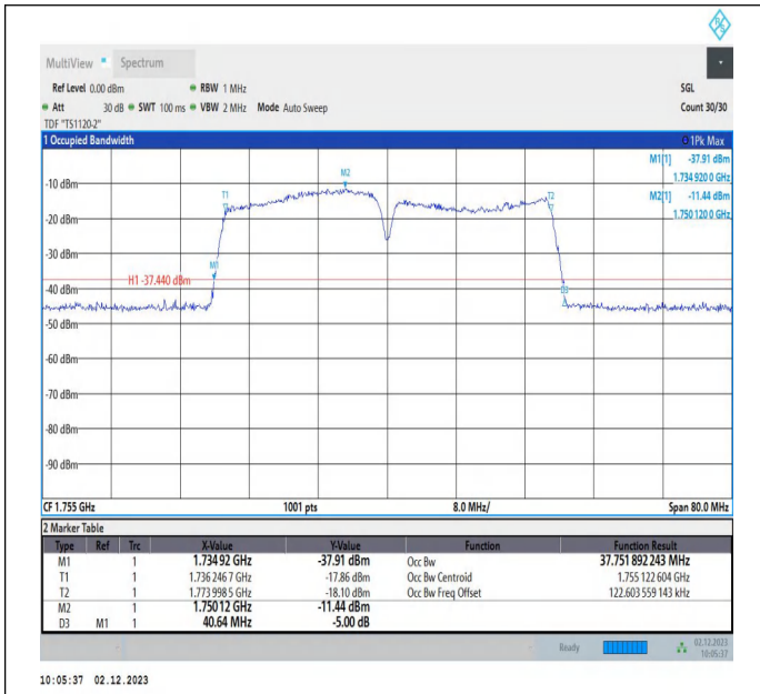
66-66-20MHz-20MHz-16QAM-16QAM-132323-132521-100R B#0-100RB#0-PASS
