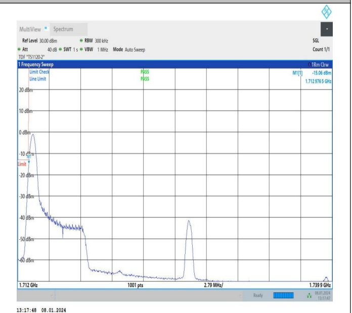
5MHz-20MHz_16QAM@16QAM-16QAM@16QAM_132027-1 32171_1RB#0@25RB#0-0RB#0@100RB#0
