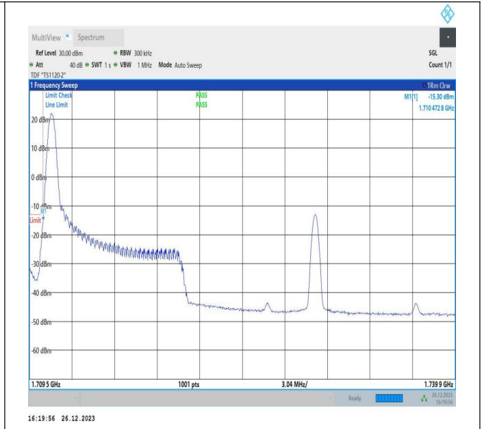
10MHz-20MHz_64QAM@64QAM-64QAM@64QAM_132027-132171_1RB#0@50RB#0-0RB#0@100RB#0
