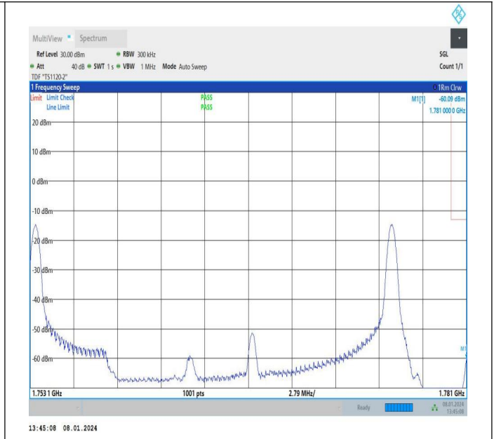
5MHz-20MHz_64QAM@64QAM-64QAM@64QAM_132428-132572_1RB#0@25RB#0-1RB#99@100RB#0
