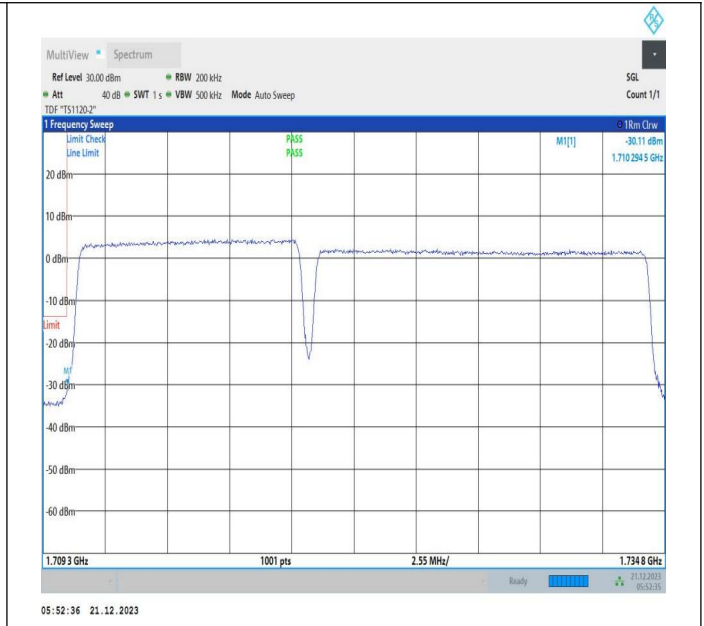
10MHz-15MHz_16QAM@16QAM-16QAM@16QAM_132025-132145_50RB#0@50RB#0-75RB#0@75RB#0
