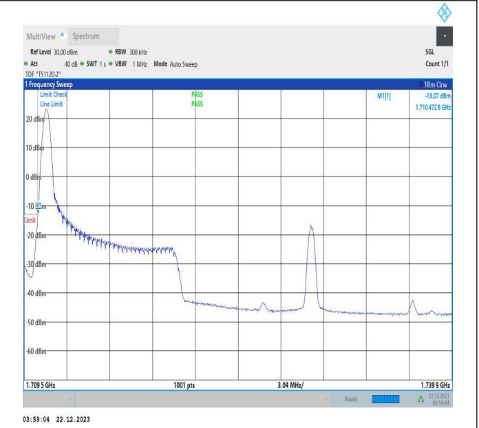
10MHz-20MHz_QPSK@QPSK-QPSK@QPSK_132027-1321 71_1RB#0@50RB#0-0RB#0@100RB#0
