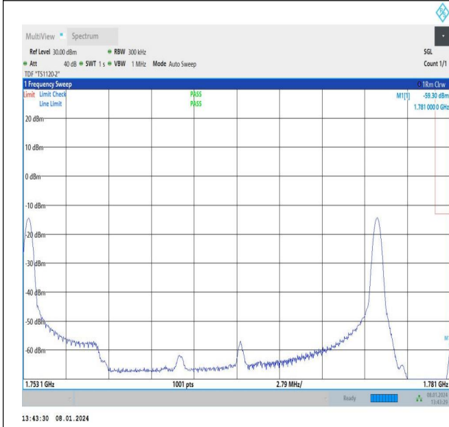
5MHz-20MHz_QPSK@QPSK-QPSK@QPSK_132428-132572_1RB#0@25RB#0-1RB#99@100RB#0
