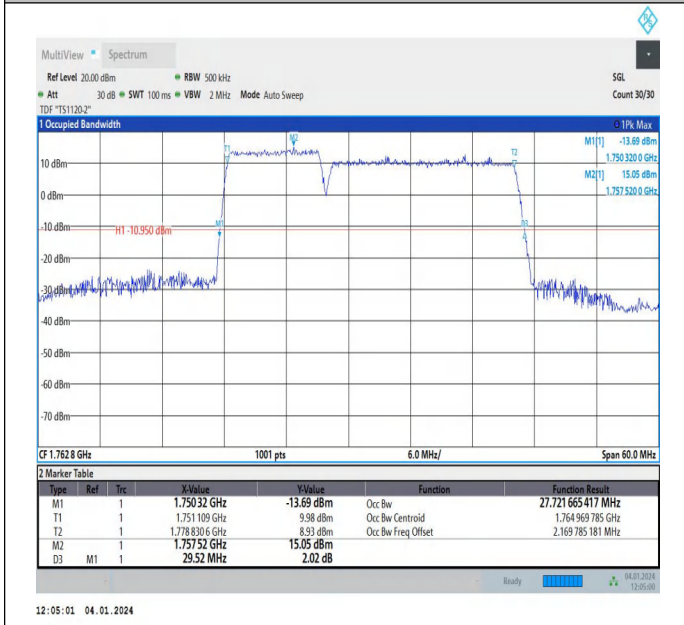
66-66-10MHz-20MHz-64QAM-64QAM-132428-132572-50RB#0-100RB#0-PASS
