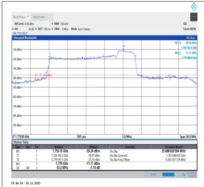
66-66-20MHz-5MHz-16QAM-16QAM-132522-132639-100RB #0-25RB#0-PASS
