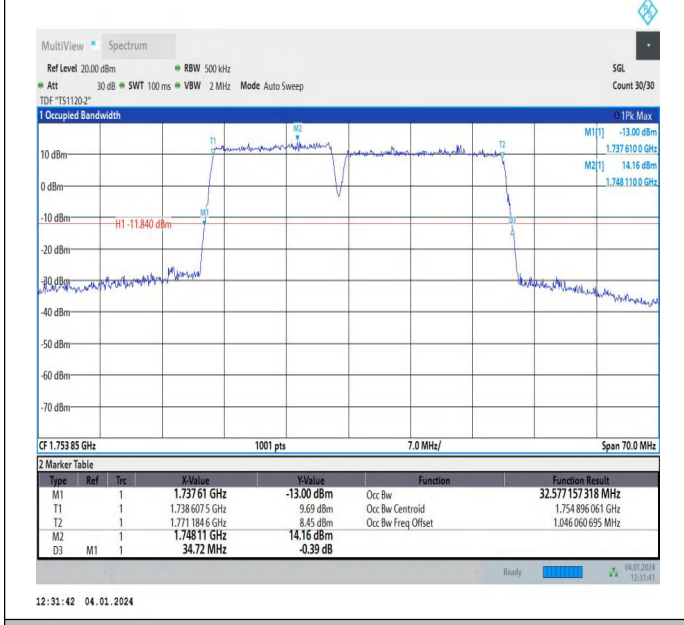
66-66-15MHz-20MHz-64QAM-64QAM-132325-132496-75RB#0-100RB#0-PASS
