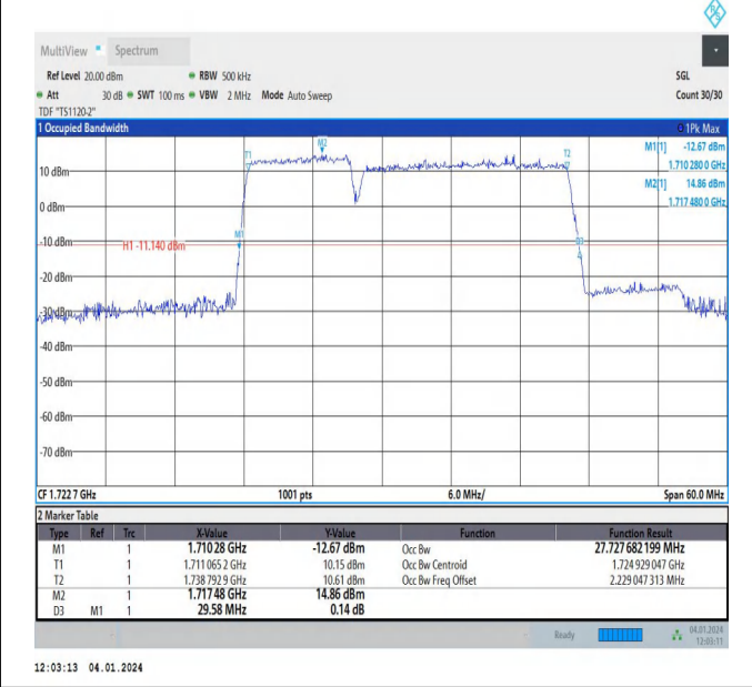
66-66-10MHz-20MHz-64QAM-64QAM-132027-132171-50RB #0-100RB#0-PASS
