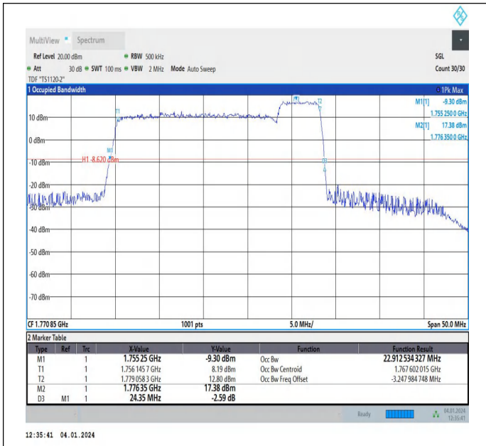
66-66-20MHz-5MHz-64QAM-64QAM-132522-132639-100RB #0-25RB#0-PASS
