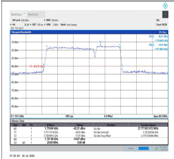
66-66-20MHz-10MHz-16QAM-16QAM-132072-132216-100R B#0-50RB#0-PASS
