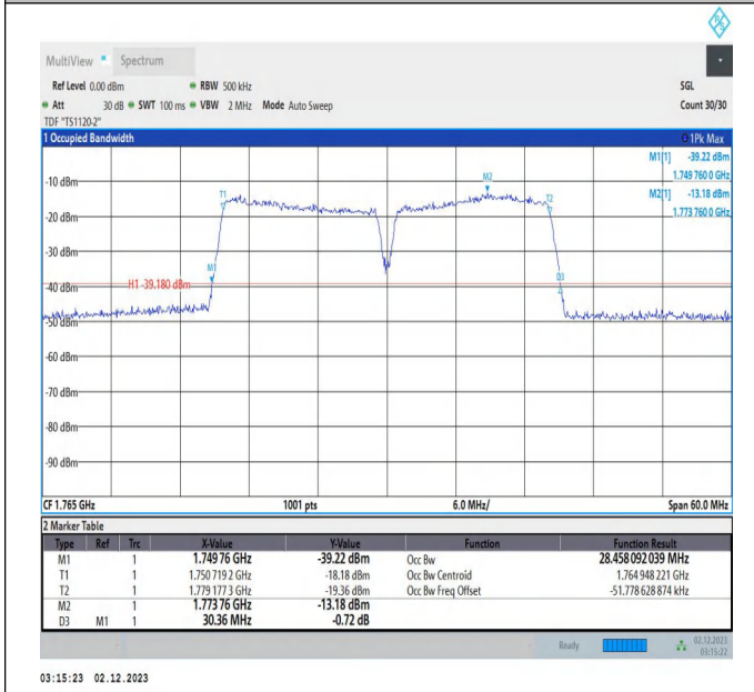
66-66-15MHz-15MHz-16QAM-16QAM-132447-132597-75RB #0-75RB#0-PASS
