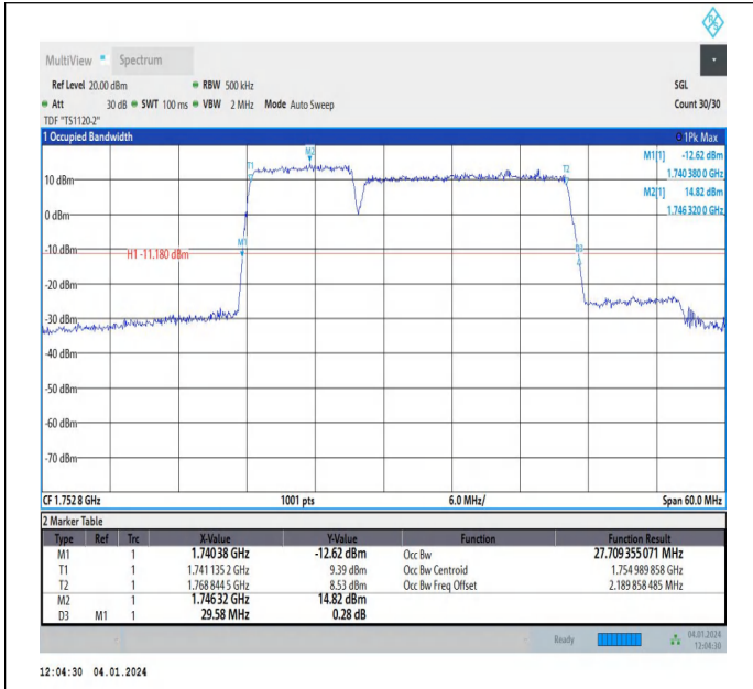
66-66-10MHz-20MHz-64QAM-64QAM-132328-132472-50RB #0-100RB#0-PASS
