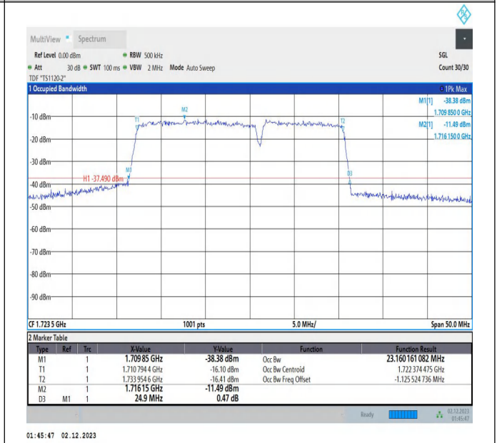
66-66-15MHz-10MHz-16QAM-16QAM-132047-132167-75RB #0-50RB#0-PASS
