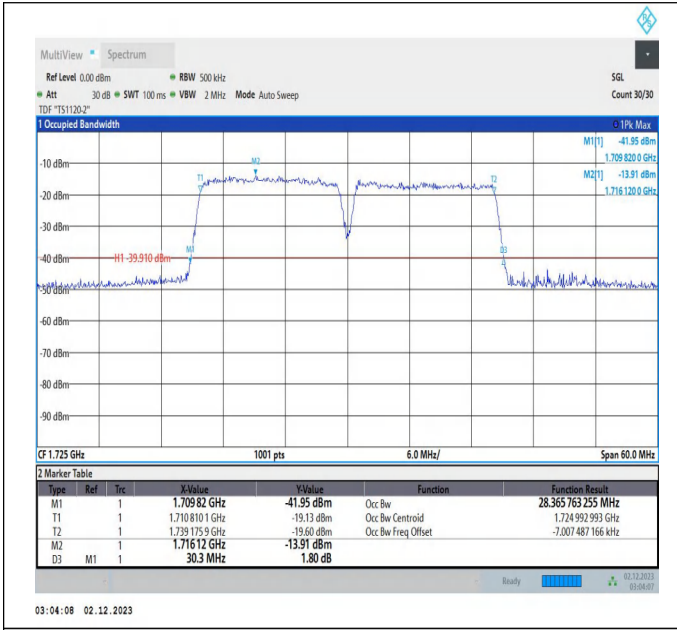
66-66-15MHz-15MHz-16QAM-16QAM-132047-132197-75RB #0-75RB#0-PASS
