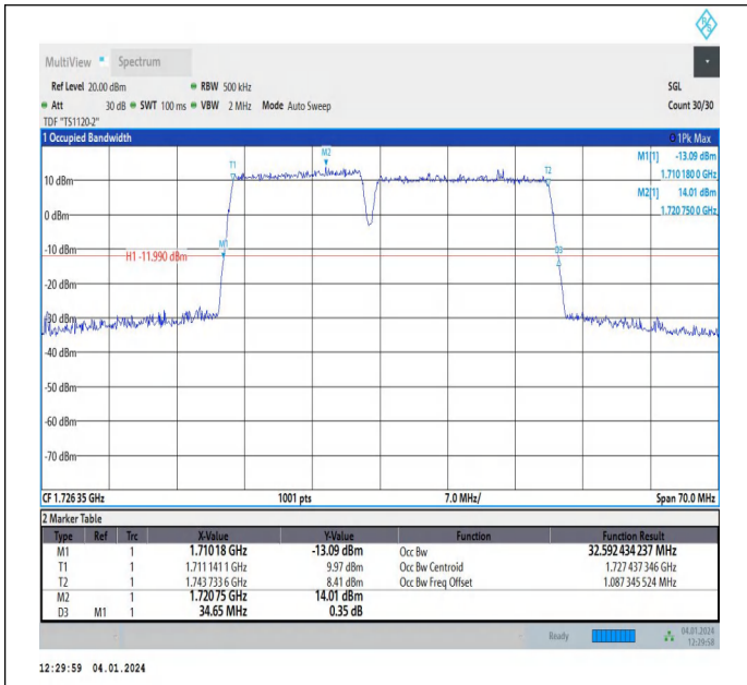
66-66-15MHz-20MHz-64QAM-64QAM-132050-132221-75RB #0-100RB#0-PASS
