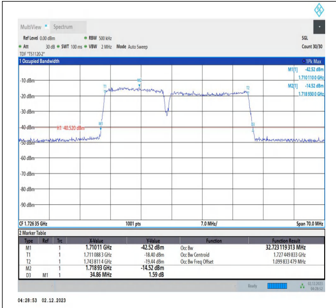
66-66-15MHz-20MHz-16QAM-16QAM-132050-132221-75RB #0-100RB#0-PASS
