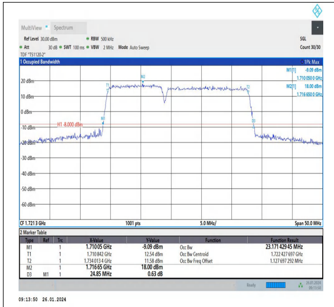
66-66-10MHz-15MHz-16QAM-16QAM-132025-132145-50RB #0-75RB#0-PASS
