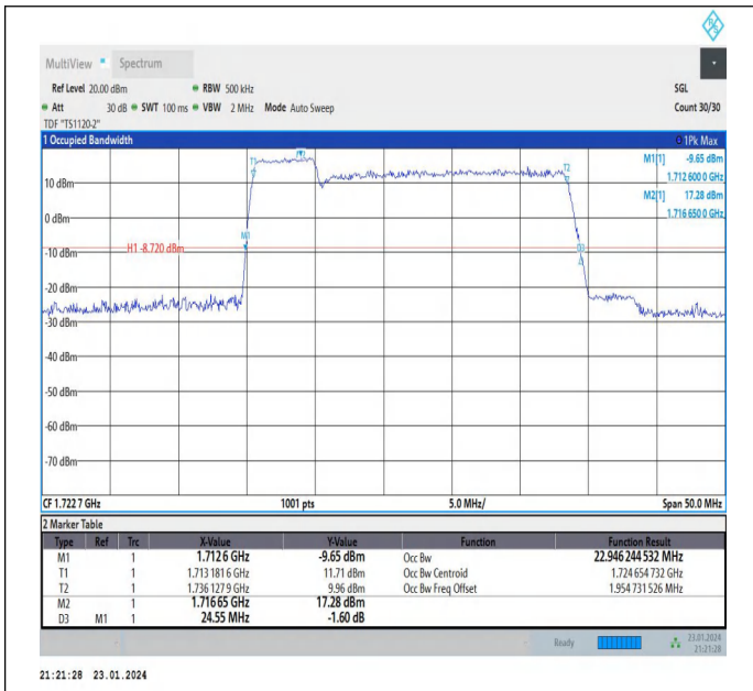
66-66-5MHz-20MHz-QPSK-QPSK-132027-132171-25RB#-100RB#0-PASS
