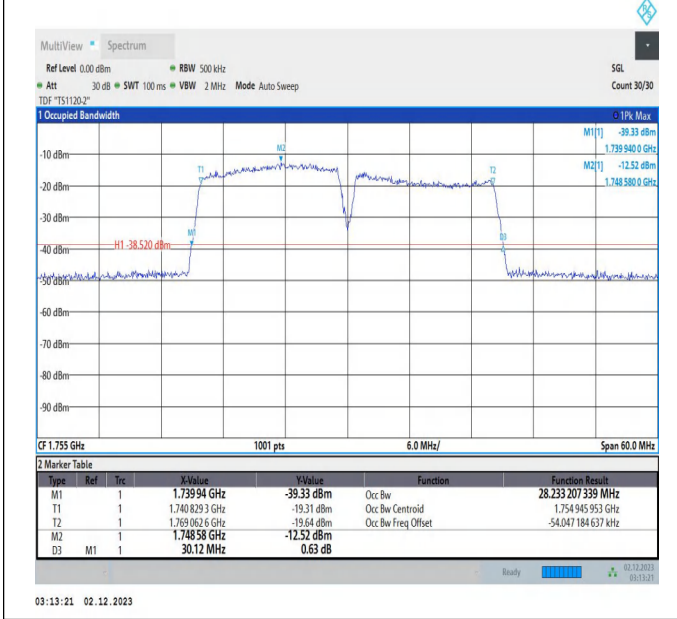
66-66-15MHz-15MHz-16QAM-16QAM-132347-132497-75RB #0-75RB#0-PASS
