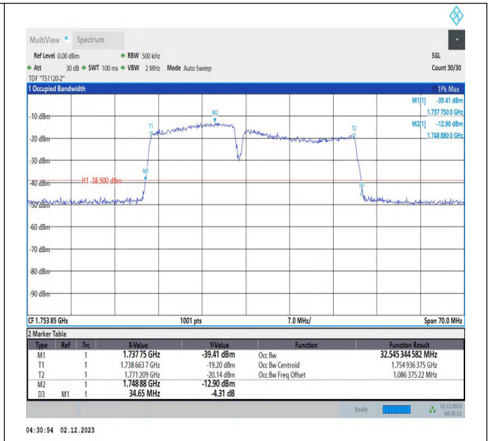
66-66-15MHz-20MHz-16QAM-16QAM-132325-132496-75RB #0-100RB#0-PASS
