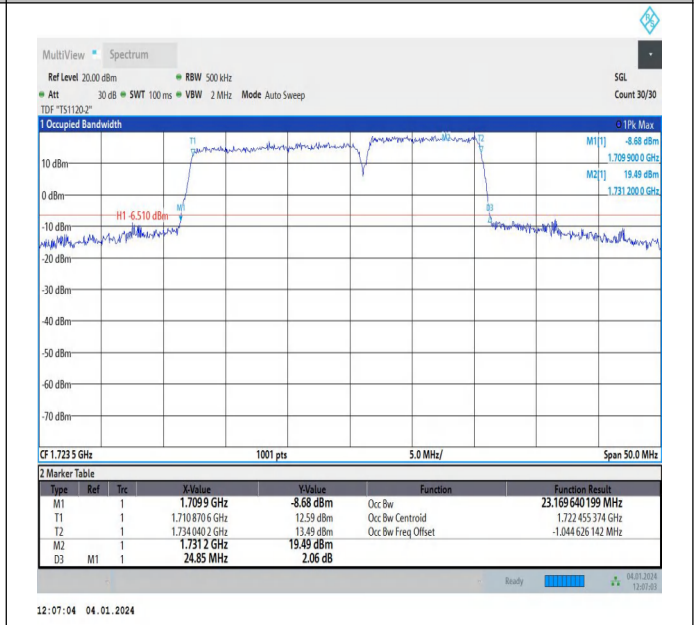
66-66-15MHz-10MHz-64QAM-64QAM-132047-132167-75RB#0-50RB#0-PASS
