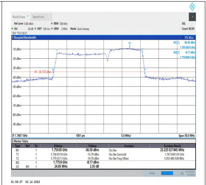
66-66-15MHz-10MHz-QPSK-QPSK-132499-132619-75RB#0-50RB#0-PASS
