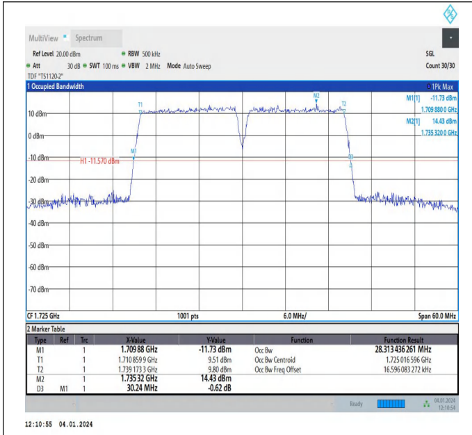
66-66-15MHz-15MHz-64QAM-64QAM-132047-132197-75RB #0-75RB#0-PASS
