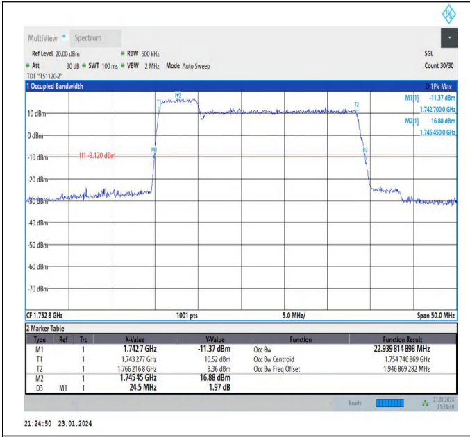
66-66-5MHz-20MHz-16QAM-16QAM-132328-132472-25RB# 0-100RB#0-PASS
