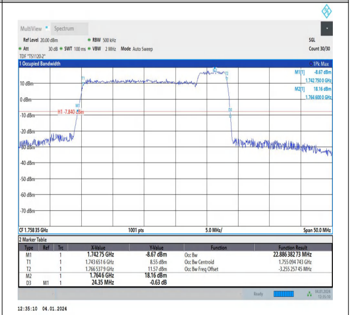
66-66-20MHz-5MHz-64QAM-64QAM-132397-132514-100RB #0-25RB#0-PASS
