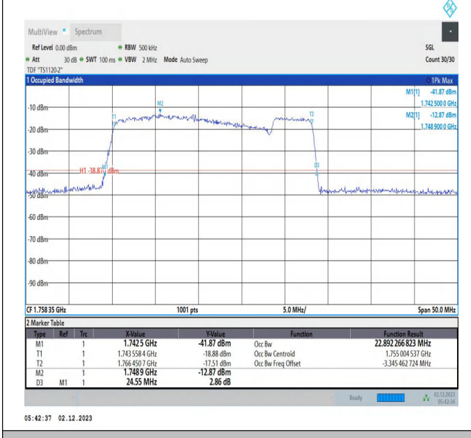
66-66-20MHz-5MHz-16QAM-16QAM-132397-132514-100RB #0-25RB#0-PASS
