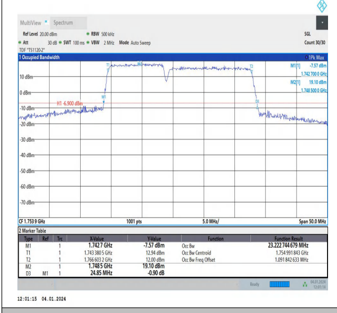
66-66-10MHz-15MHz-64QAM-64QAM-132351-132471-50RB #0-75RB#0-PASS
