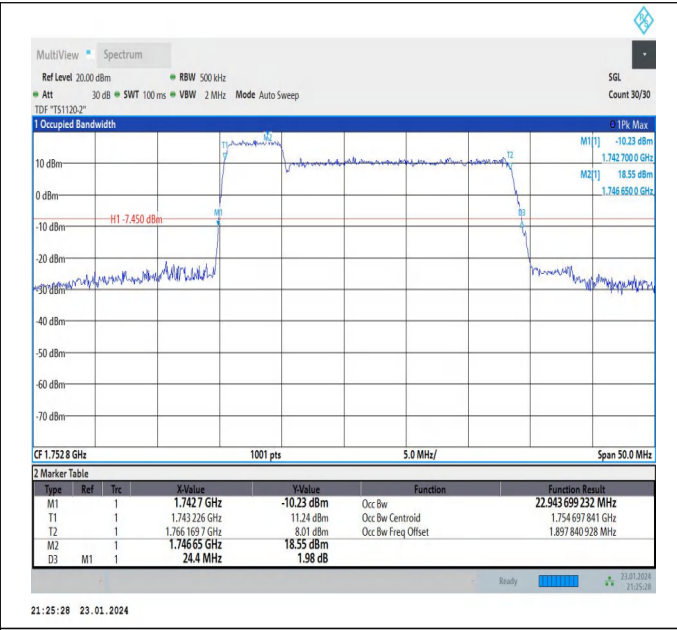
66-66-5MHz-20MHz-64QAM-64QAM-132328-132472-25RB# 0-100RB#0-PASS
