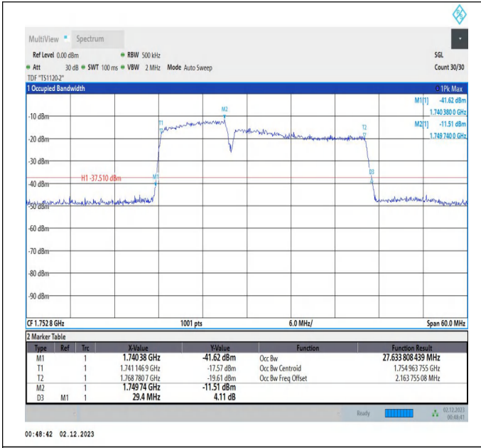
66-66-10MHz-20MHz-16QAM-16QAM-132328-132472-50RB #0-100RB#0-PASS
