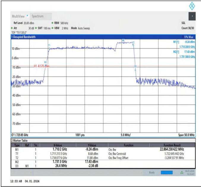
66-66-20MHz-5MHz-64QAM-64QAM-132072-132189-100RB #0-25RB#0-PASS
