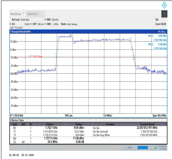
66-66-5MHz-20MHz-64QAM-64QAM-132428-132572-25RB#0-100RB#0-PASS
