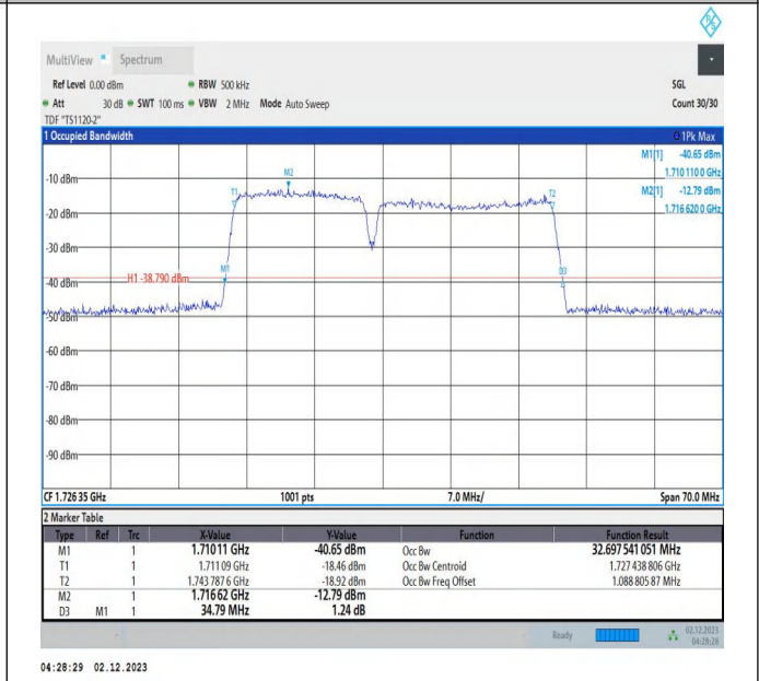
66-66-15MHz-20MHz-QPSK-QPSK-132050-132221-75RB#0-100RB#0-PASS
