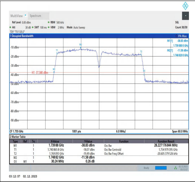
66-66-15MHz-15MHz-QPSK-QPSK-132347-132497-75RB#0-75RB#0-PASS
