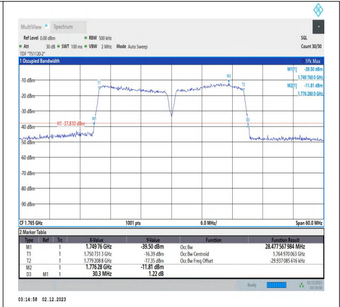
66-66-15MHz-15MHz-QPSK-QPSK-132447-132597-75RB#0-75RB#0-PASS
