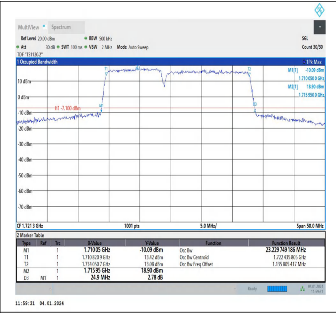
66-66-10MHz-15MHz-64QAM-64QAM-132025-132145-50RB #0-75RB#0-PASS
