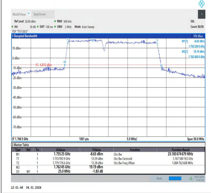
66-66-10MHz-15MHz-64QAM-64QAM-132477-132597-50RB #0-75RB#0-PASS
