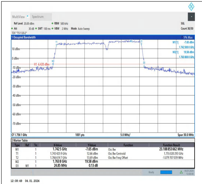
66-66-15MHz-10MHz-64QAM-64QAM-132373-132493-75RB #0-50RB#0-PASS
