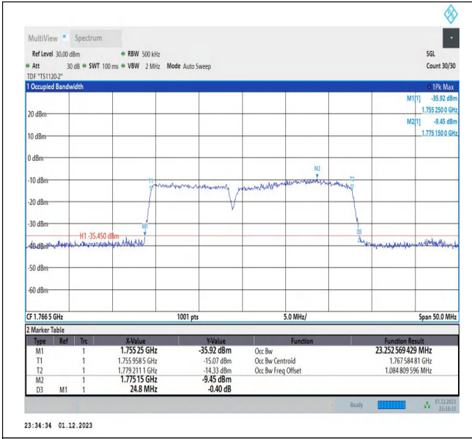
66-66-10MHz-15MHz-16QAM-16QAM-132477-132597-50RB #0-75RB#0-PASS
