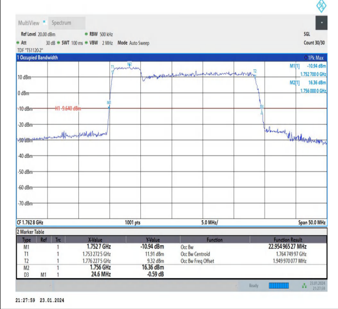
66-66-5MHz-20MHz-16QAM-16QAM-132428-132572-25RB# 0-100RB#0-PASS
