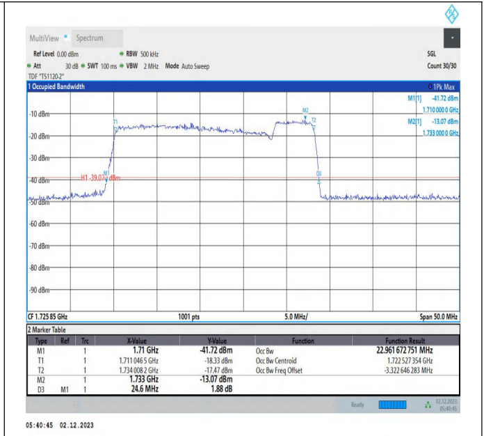
66-66-20MHz-5MHz-16QAM-16QAM-132072-132189-100RB#0-25RB#0-PASS
