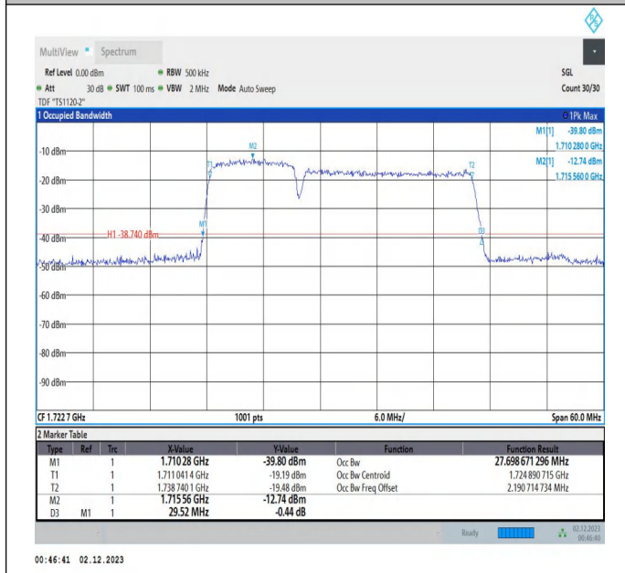
66-66-10MHz-20MHz-16QAM-16QAM-132027-132171-50RB #0-100RB#0-PASS
