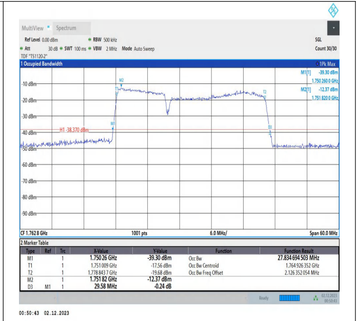
66-66-10MHz-20MHz-16QAM-16QAM-132428-132572-50RB #0-100RB#0-PASS
