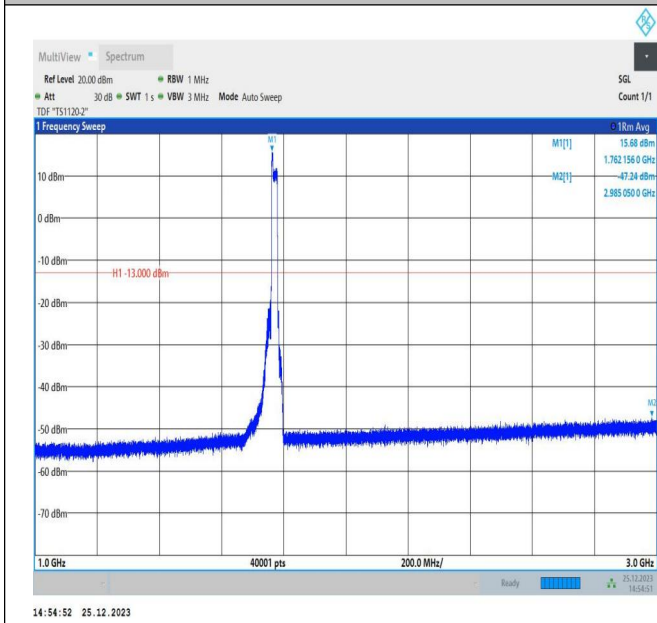
66-66-5MHz-15MHz-16QAM-16QAM-132504-132597-25RB# 0-75RB#0-1000~3000MHz-PASS
