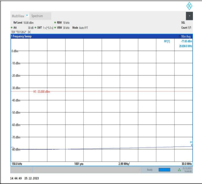
66-66-5MHz-15MHz-QPSK-QPSK-132353-132446-1RB#0-1R B#74-0.15~30MHz-PASS
