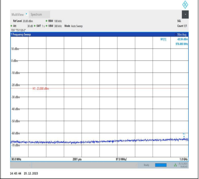
66-66-5MHz-15MHz-16QAM-16QAM-132353-132446-1RB#0- 1RB#74-30~1000MHz-PASS
