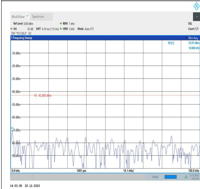
66-66-5MHz-15MHz-QPSK-QPSK-132504-132597-25RB#0-75RB#0-0.009~0.15MHz-PASS
