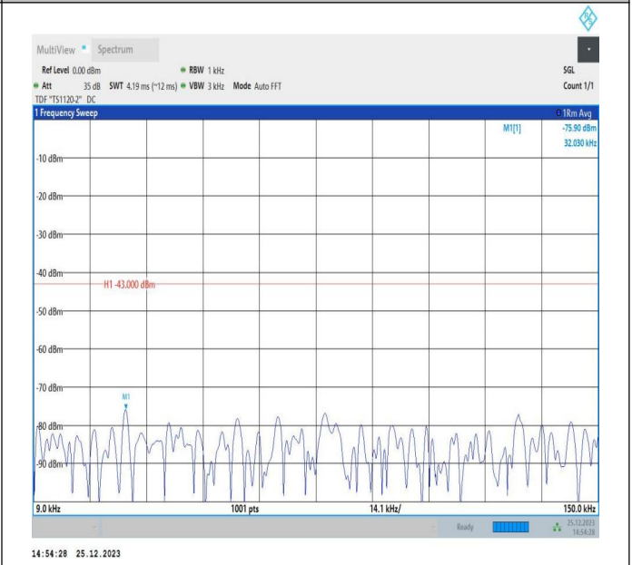
66-66-5MHz-15MHz-16QAM-16QAM-132504-132597-25RB#0-75RB#0-0.009~0.15MHz-PASS
