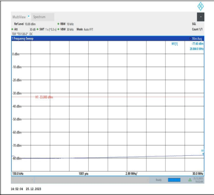
66-66-5MHz-15MHz-QPSK-QPSK-132504-132597-1RB#0-1R B#74-0.15~30MHz-PASS
