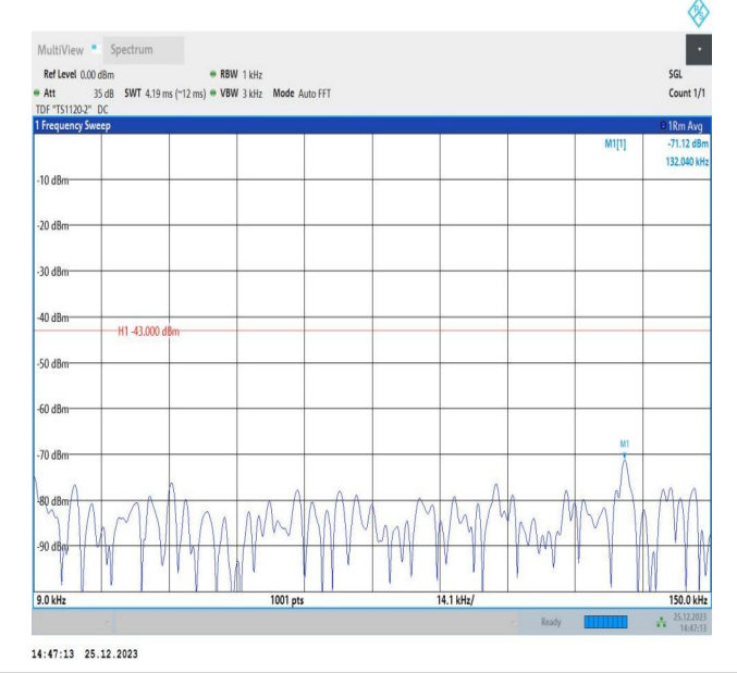
66-66-5MHz-15MHz-16QAM-16QAM-132353-132446-25RB#0-75RB#0-0.009~0.15MHz-PASS
