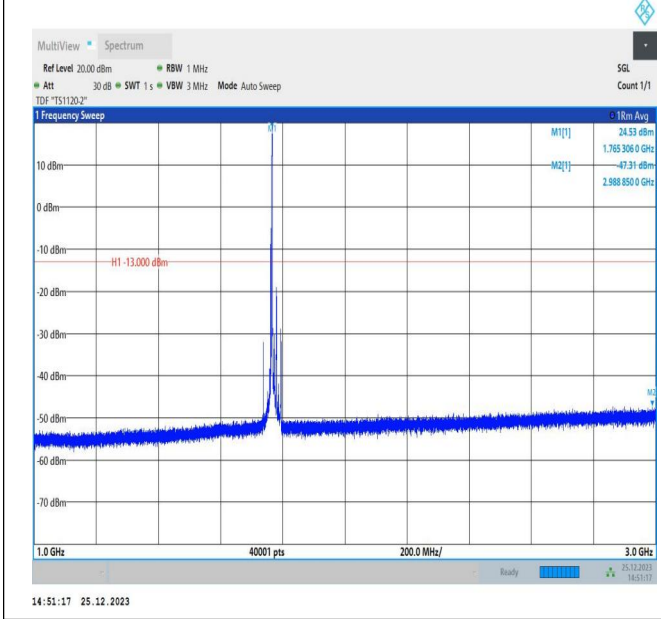
66-66-5MHz-15MHz-16QAM-16QAM-132504-132597-1RB#2 4-ORB#0-1000~3000MHz-PASS
