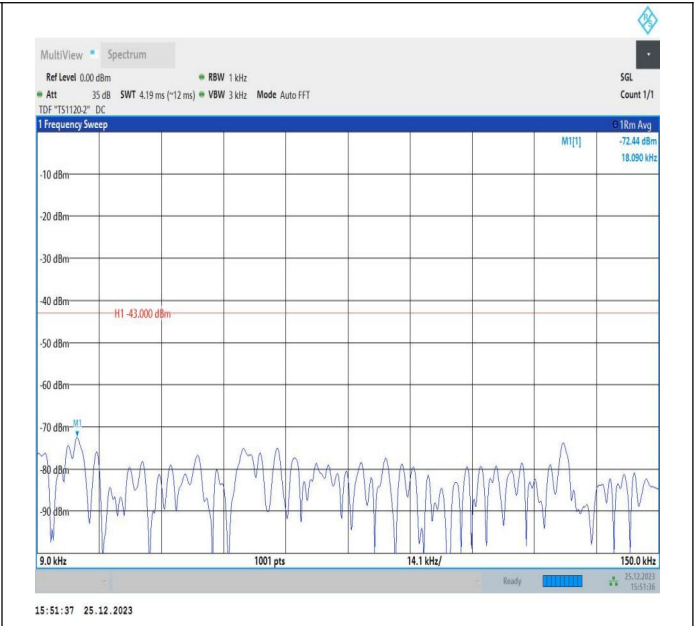
66-66-15MHz-5MHz-16QAM-16QAM-132047-132140-1RB#0-0 ORB#0-0.009~0.15MHz-PASS
