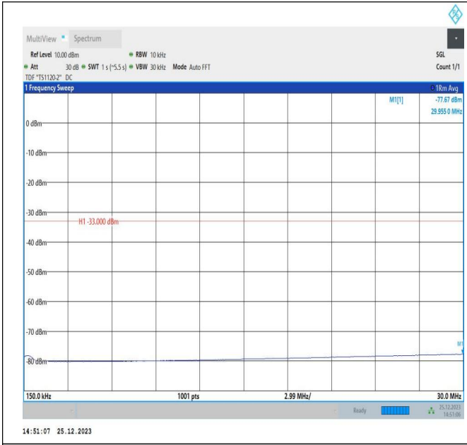
66-66-5MHz-15MHz-16QAM-16QAM-132504-132597-1RB#2 4-ORB#0-0.15~30MHz-PASS
