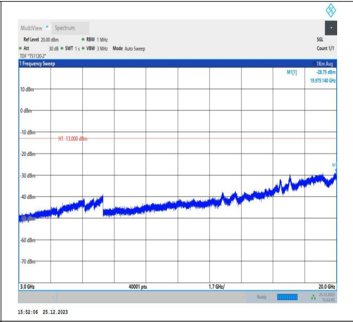
66-66-15MHz-5MHz-16QAM-16QAM-132047-132140-1RB#0-ORB#0-3000~20000MHz-PASS
