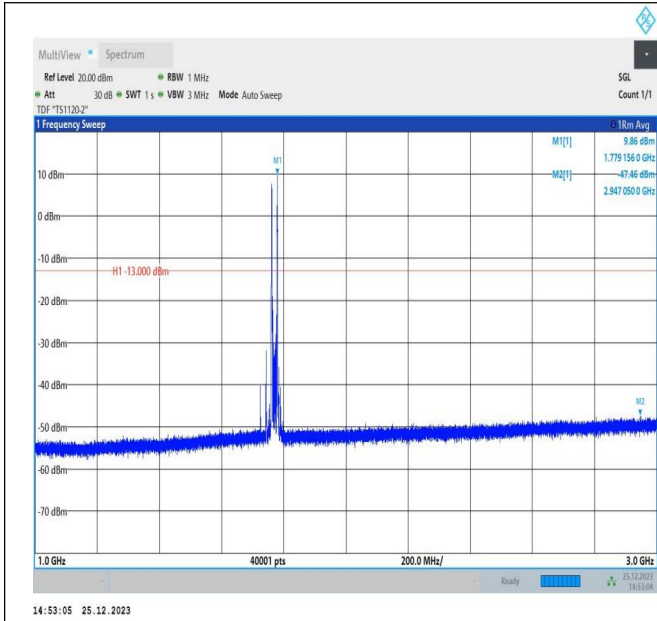
66-66-5MHz-15MHz-16QAM-16QAM-132504-132597-1RB#0-1RB#74-1000~3000MHz-PASS
