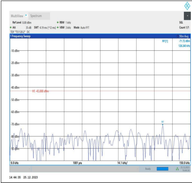
66-66-5MHz-15MHz-QPSK-QPSK-132353-132446-1RB#0-1 RB#74-0.009~0.15MHz-PASS
