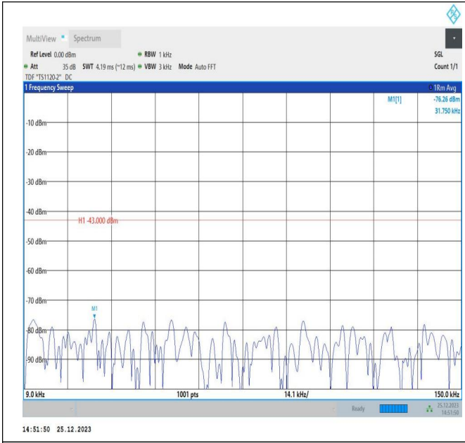
66-66-5MHz-15MHz-QPSK-QPSK-132504-132597-1RB#0-1 RB#74-0.009~0.15MHz-PASS
