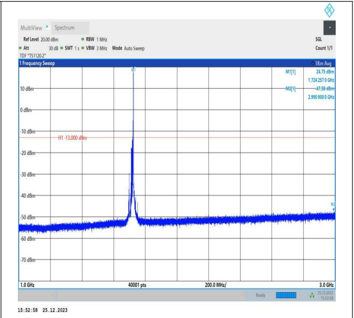
66-66-15MHz-5MHz-QPSK-QPSK-132047-132140-1RB#74-0RB#0-1000~3000MHz-PASS
