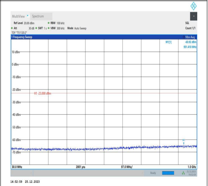
66-66-5MHz-15MHz-16QAM-16QAM-132504-132597-1RB#0- 1RB#74-30~1000MHz-PASS
