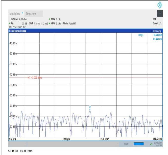
66-66-5MHz-15MHz-QPSK-QPSK-132353-132446-1RB#0-0 RB#0-0.009~0.15MHz-PASS
