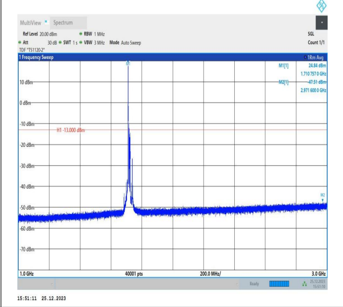
66-66-15MHz-5MHz-QPSK-QPSK-132047-132140-1RB#0-0RB#0-1000~3000MHz-PASS
