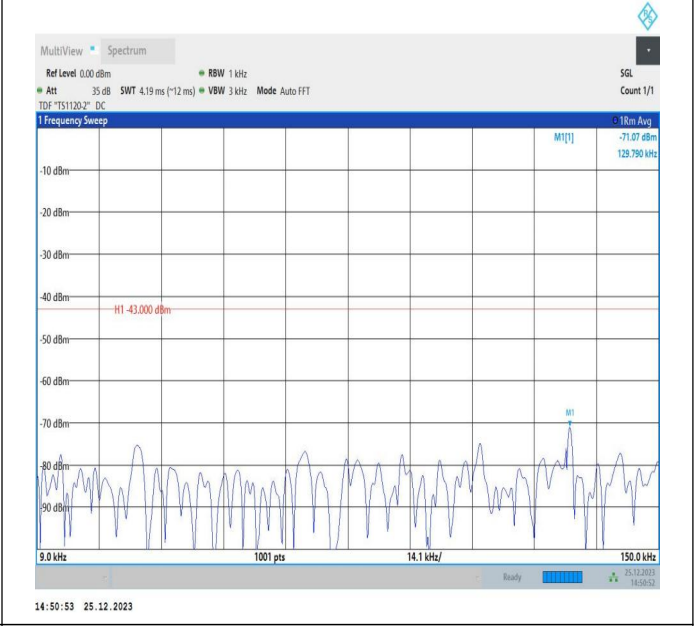
66-66-5MHz-15MHz-16QAM-16QAM-132504-132597-1RB#24-ORB#0-0.009~0.15MHz-PASS
