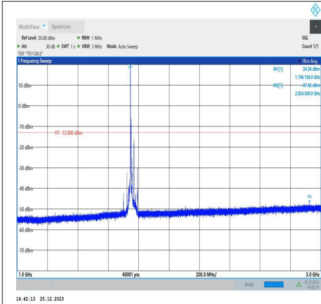
66-66-5MHz-15MHz-16QAM-16QAM-132353-132446-1RB#0-ORB#0-1000~3000MHz-PASS
