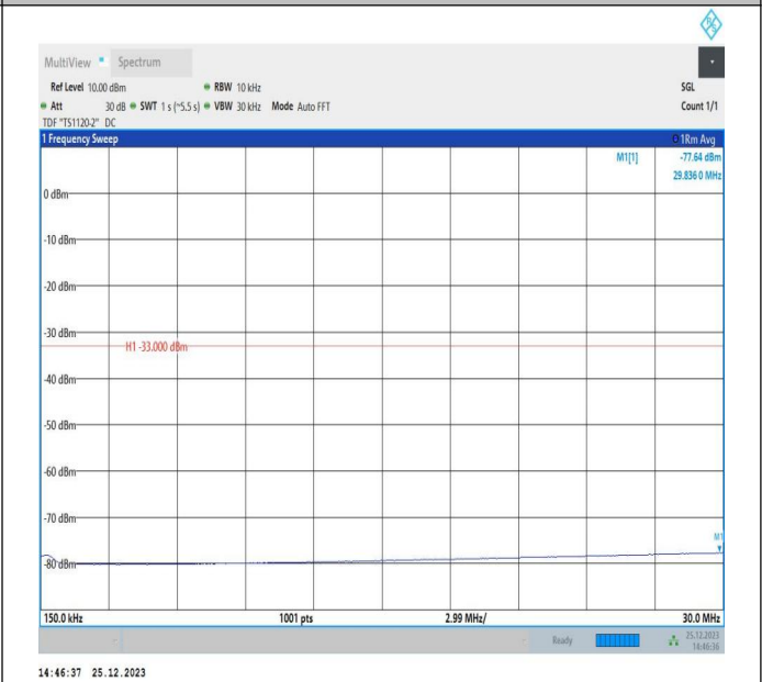
66-66-5MHz-15MHz-QPSK-QPSK-132353-132446-25RB#0-75RB#0-0.15~30MHz-PASS
