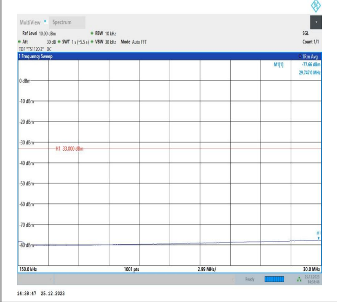
66-66-5MHz-15MHz-QPSK-QPSK-132002-132095-25RB#0-75RB#0-0.15~30MHz-PASS
