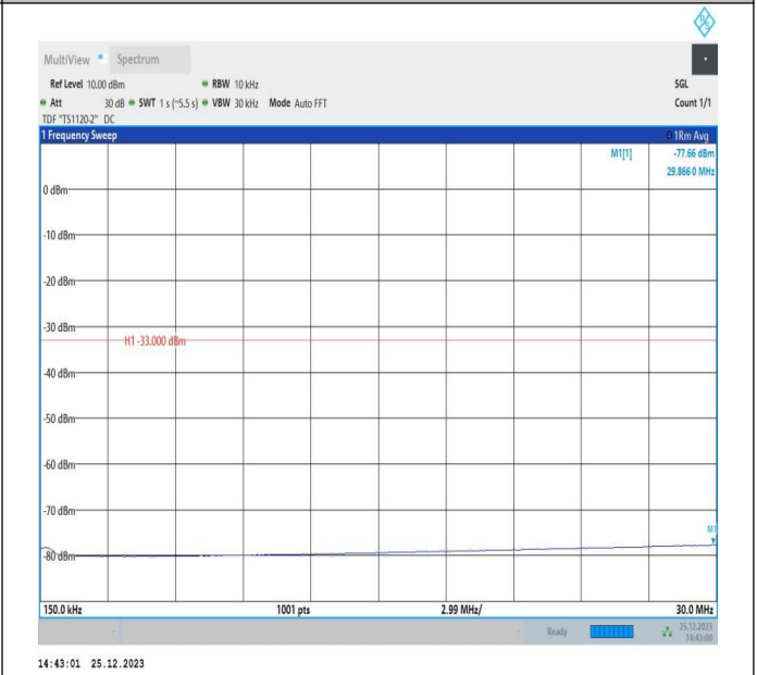
66-66-5MHz-15MHz-QPSK-QPSK-132353-132446-1RB#24-ORB#0-0.15~30MHz-PASS
