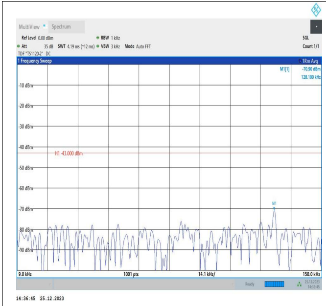
66-66-5MHz-15MHz-QPSK-QPSK-132002-132095-1RB#0-1 RB#74-0.009~0.15MHz-PASS
