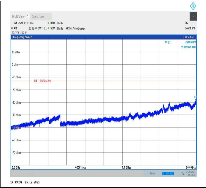
66-66-5MHz-15MHz-16QAM-16QAM-132504-132597-1RB#0-ORB#0-3000~20000MHz-PASS
