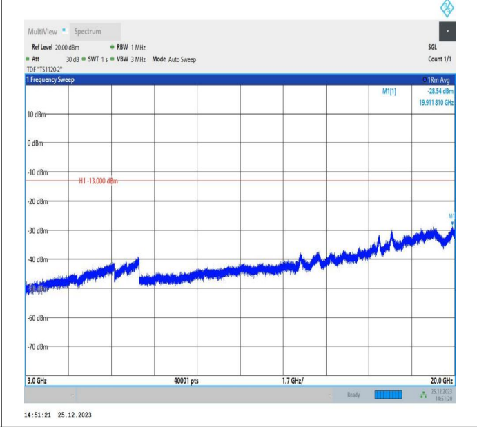
66-66-5MHz-15MHz-16QAM-16QAM-132504-132597-1RB#2 4-ORB#0-3000~20000MHz-PASS
