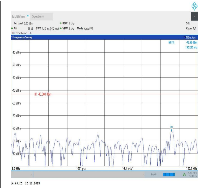
66-66-5MHz-15MHz-16QAM-16QAM-132353-132446-1RB#0- 1RB#74-0.009~0.15MHz-PASS
