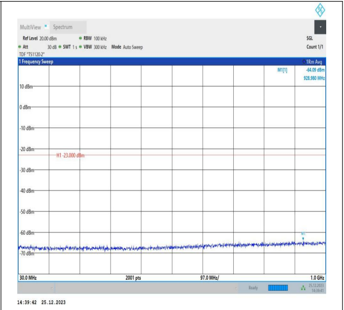
66-66-5MHz-15MHz-16QAM-16QAM-132002-132095-25RB# 0-75RB#0-30~1000MHz-PASS
