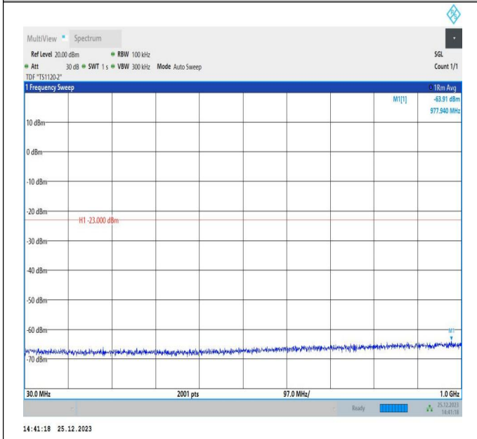
66-66-5MHz-15MHz-QPSK-QPSK-132353-132446-1RB#0-0 RB#0-30~1000MHz-PASS
