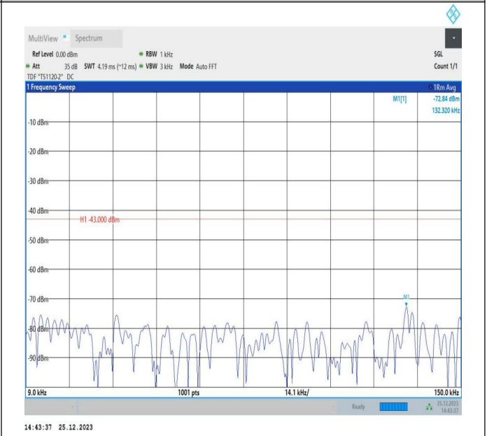
66-66-5MHz-15MHz-16QAM-16QAM-132353-132446-1RB#24-ORB#0-0.009~0.15MHz-PASS
