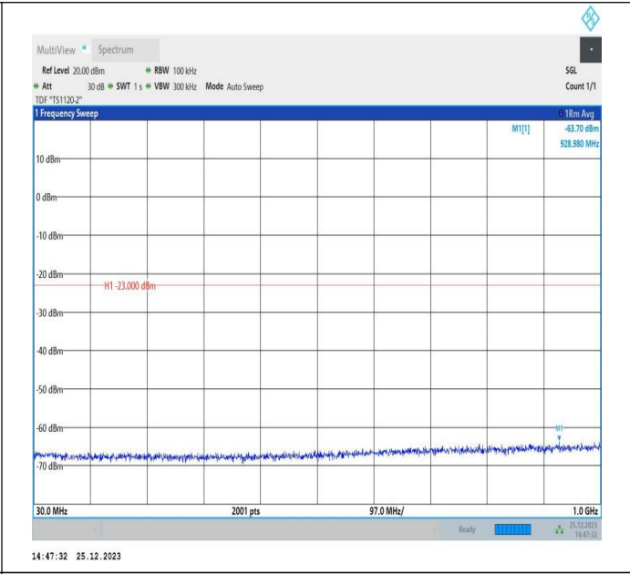
66-66-5MHz-15MHz-16QAM-16QAM-132353-132446-25RB# 0-75RB#0-30~1000MHz-PASS
