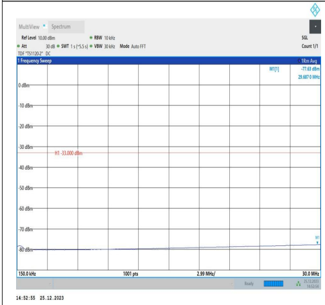
66-66-5MHz-15MHz-16QAM-16QAM-132504-132597-1RB#0 -1RB#74-0.15~30MHz-PASS
