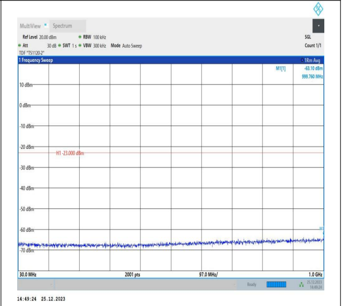
66-66-5MHz-15MHz-16QAM-16QAM-132504-132597-1RB#0-0ORB#0-30~1000MHz-PASS
