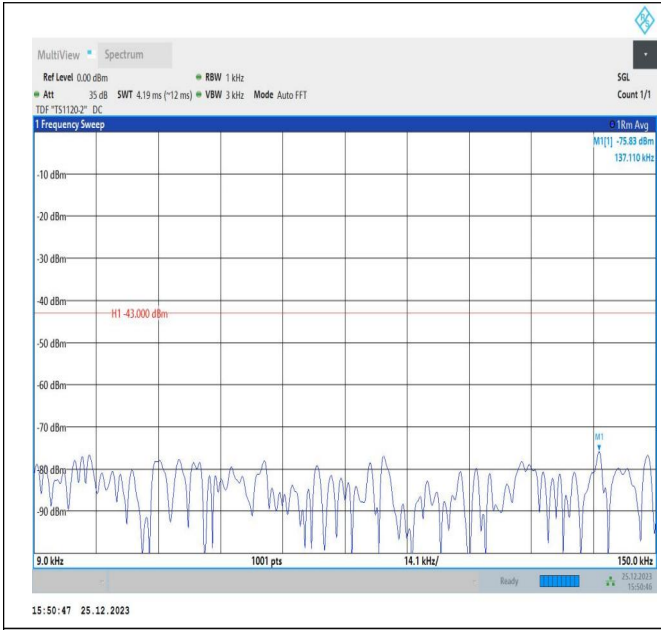
66-66-15MHz-5MHz-QPSK-QPSK-132047-132140-1RB#0-0RB#0-0.009~0.15MHz-PASS
