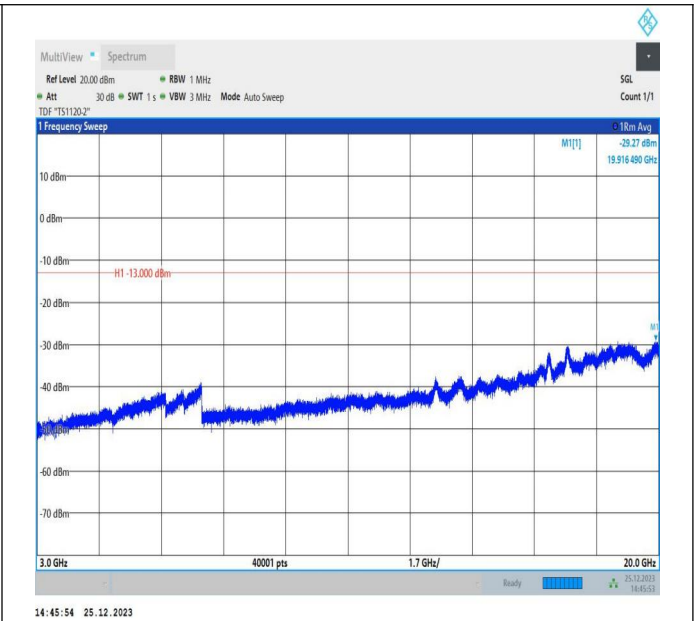
66-66-5MHz-15MHz-16QAM-16QAM-132353-132446-1RB#0-1RB#74-3000~20000MHz-PASS
