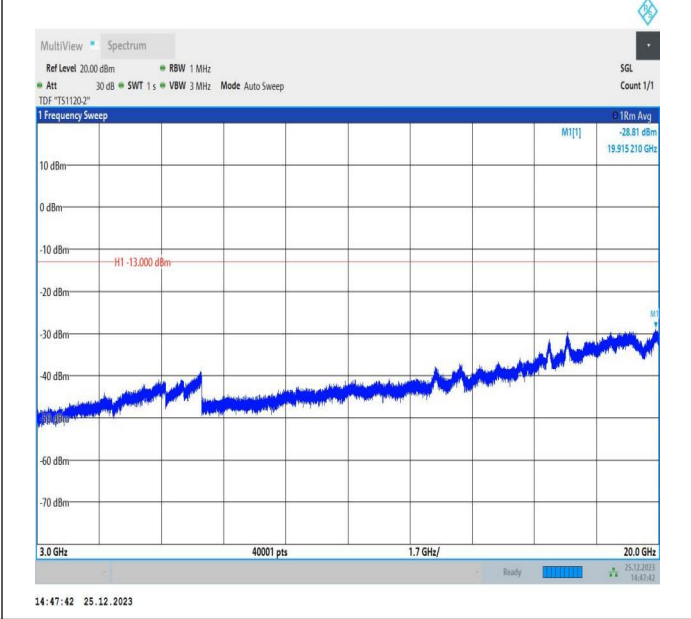
66-66-5MHz-15MHz-16QAM-16QAM-132353-132446-25RB# 0-75RB#0-3000~20000MHz-PASS
