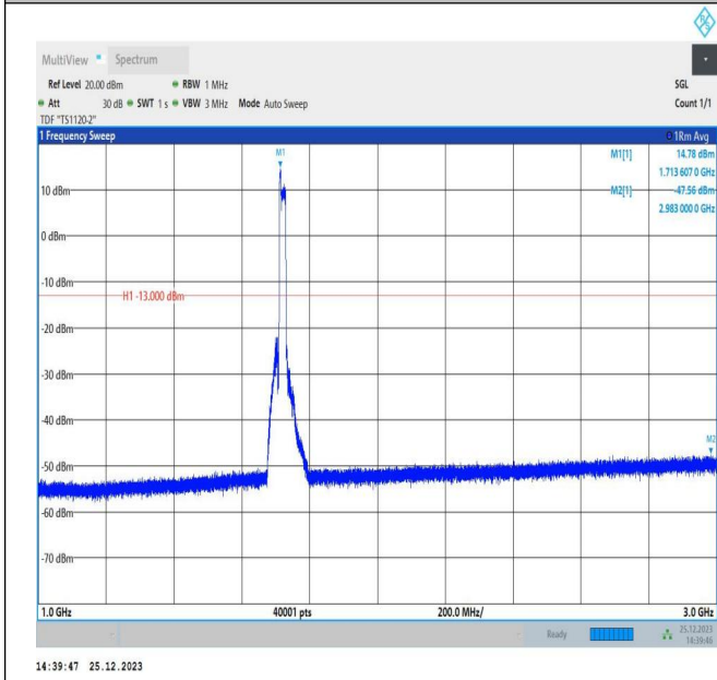
66-66-5MHz-15MHz-16QAM-16QAM-132002-132095-25RB# 0-75RB#0-1000~3000MHz-PASS
