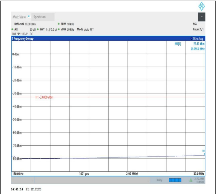
66-66-5MHz-15MHz-QPSK-QPSK-132353-132446-1RB#0-0R B#0-0.15~30MHz-PASS
