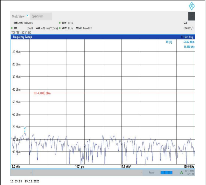
66-66-15MHz-5MHz-16QAM-16QAM-132047-132140-1RB#74-0RB#0-0.009~0.15MHz-PASS
