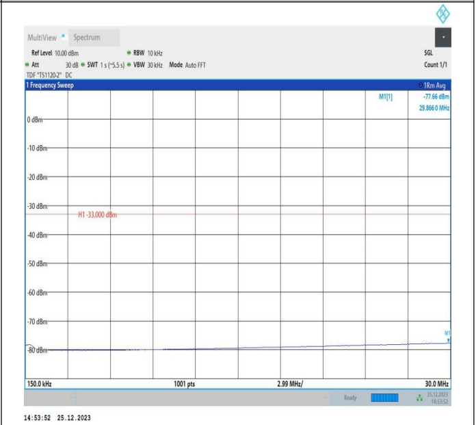
66-66-5MHz-15MHz-QPSK-QPSK-132504-132597-25RB#0-75RB#0-0.15~30MHz-PASS
