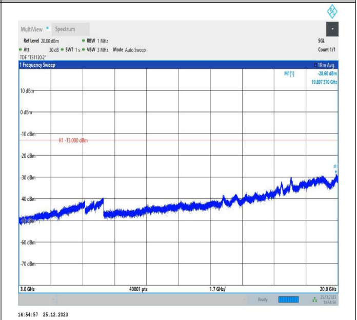
66-66-5MHz-15MHz-16QAM-16QAM-132504-132597-25RB# 0-75RB#0-3000~20000MHz-PASS
