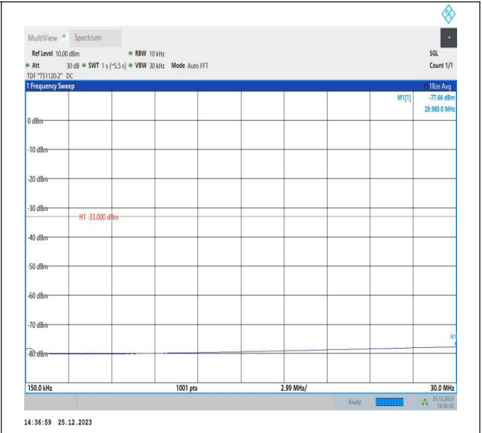
66-66-5MHz-15MHz-QPSK-QPSK-132002-132095-1RB#0-1R B#74-0.15~30MHz-PASS
