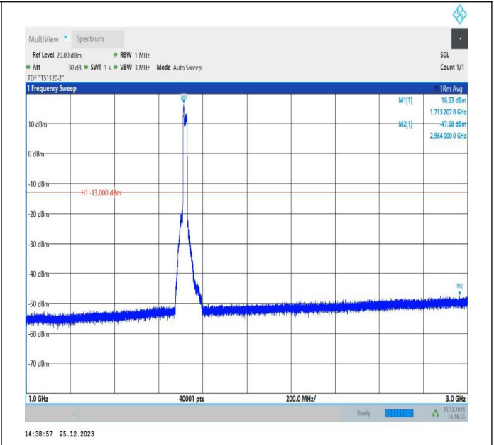
66-66-5MHz-15MHz-QPSK-QPSK-132002-132095-25RB#0-75RB#0-1000~3000MHz-PASS
