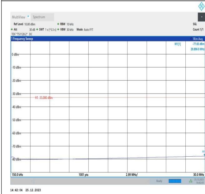
66-66-5MHz-15MHz-16QAM-16QAM-132353-132446-1RB#0-0ORB#0-0.15~30MHz-PASS
