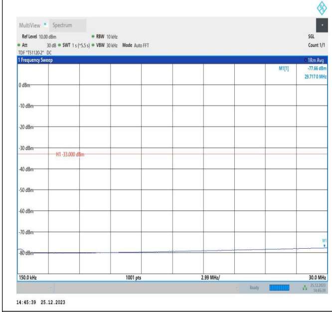
66-66-5MHz-15MHz-16QAM-16QAM-132353-132446-1RB#0 -1RB#74-0.15~30MHz-PASS
