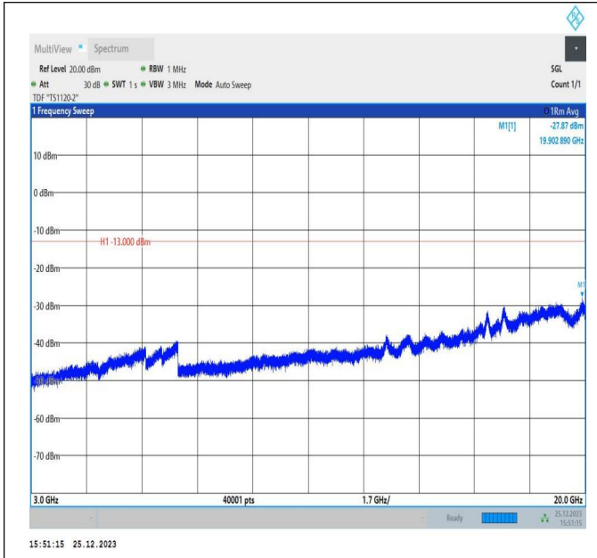
66-66-15MHz-5MHz-QPSK-QPSK-132047-132140-1RB#0-0 RB#0-3000~20000MHz-PASS
