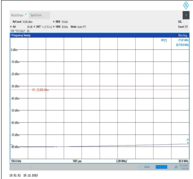
66-66-15MHz-5MHz-16QAM-16QAM-132047-132140-1RB#0-0 -ORB#0-0.15~30MHz-PASS
