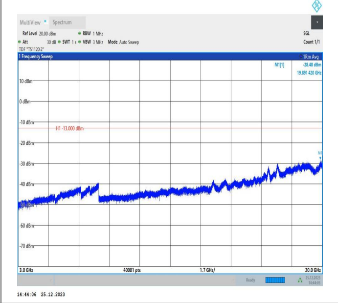
66-66-5MHz-15MHz-16QAM-16QAM-132353-132446-1RB#2 4-ORB#0-3000~20000MHz-PASS
