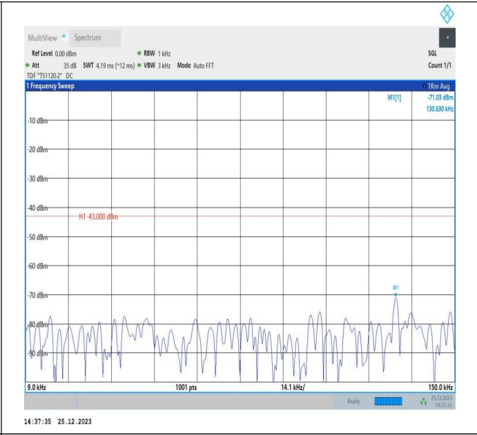
66-66-5MHz-15MHz-16QAM-16QAM-132002-132095-1RB#0- 1RB#74-0.009~0.15MHz-PASS
