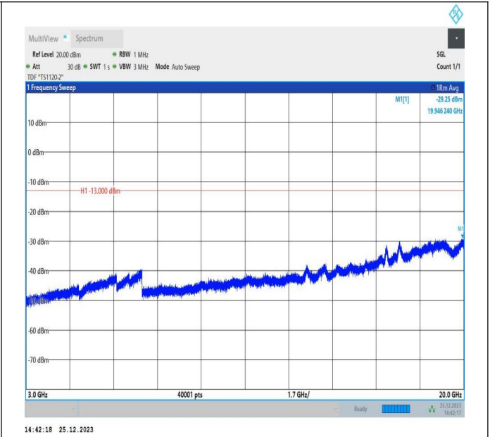
66-66-5MHz-15MHz-16QAM-16QAM-132353-132446-1RB#0-ORB#0-3000~20000MHz-PASS
