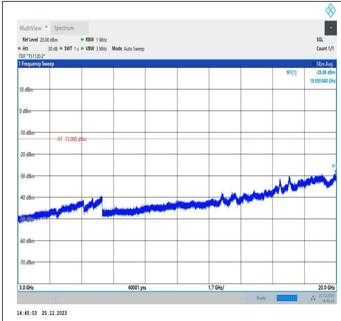
66-66-5MHz-15MHz-QPSK-QPSK-132353-132446-1RB#0-1 RB#74-3000~20000MHz-PASS
