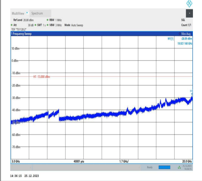
66-66-5MHz-15MHz-16QAM-16QAM-132002-132095-1RB#2 4-ORB#0-3000~20000MHz-PASS
