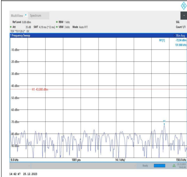
66-66-5MHz-15MHz-QPSK-QPSK-132353-132446-1RB#24-ORB#0-0.009~0.15MHz-PASS
