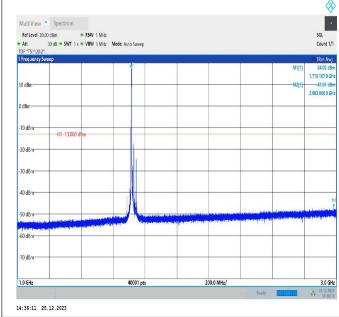
66-66-5MHz-15MHz-16QAM-16QAM-132002-132095-1RB#2 4-ORB#0-1000~3000MHz-PASS
