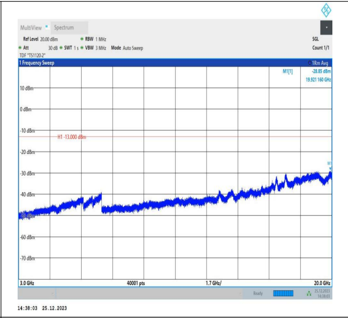
66-66-5MHz-15MHz-16QAM-16QAM-132002-132095-1RB#0-1RB#74-3000~20000MHz-PASS
