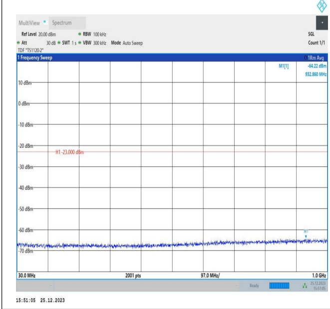
66-66-15MHz-5MHz-QPSK-QPSK-132047-132140-1RB#0-0RB#0-30~1000MHz-PASS
