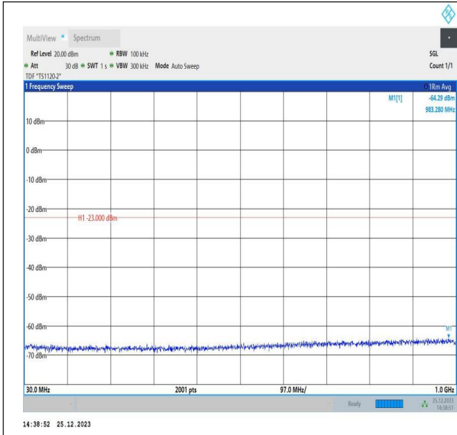
66-66-5MHz-15MHz-QPSK-QPSK-132002-132095-25RB#0-75RB#0-30~1000MHz-PASS
