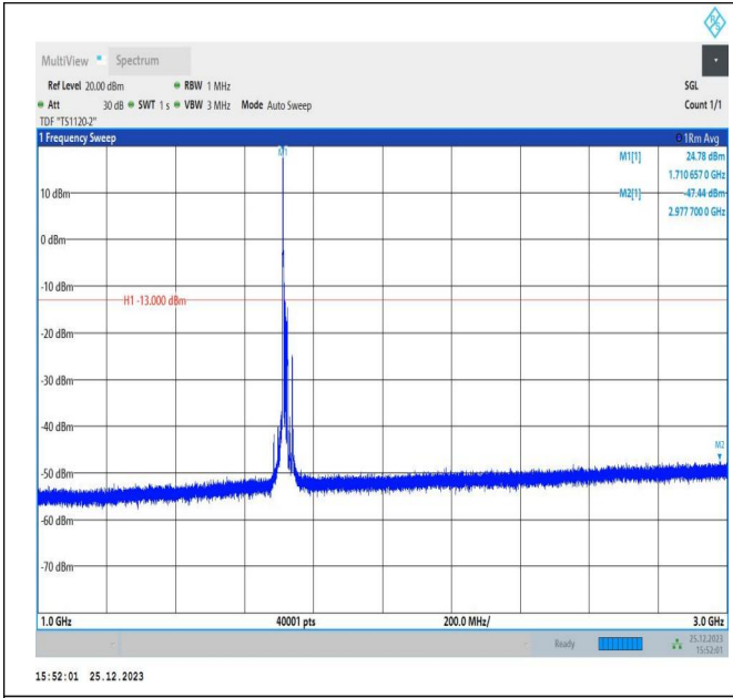
66-66-15MHz-5MHz-16QAM-16QAM-132047-132140-1RB#0-ORB#0-1000~3000MHz-PASS
