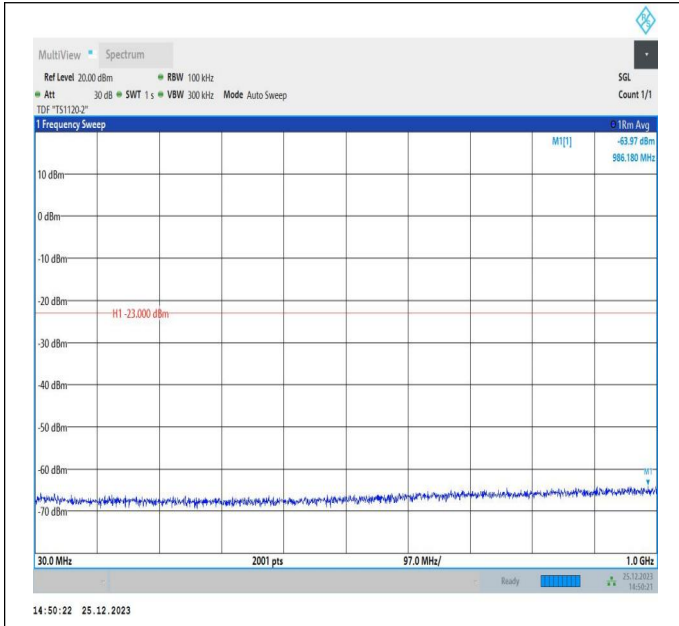
66-66-5MHz-15MHz-QPSK-QPSK-132504-132597-1RB#24-ORB#0-30~1000MHz-PASS
