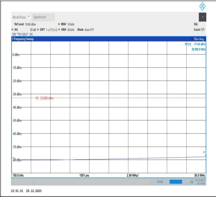
66-66-15MHz-5MHz-QPSK-QPSK-132047-132140-1RB#0-0RB#0-0.15~30MHz-PASS
