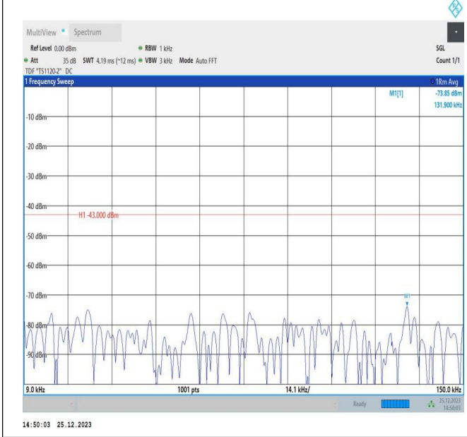
66-66-5MHz-15MHz-QPSK-QPSK-132504-132597-1RB#24-ORB#0-0.009~0.15MHz-PASS
