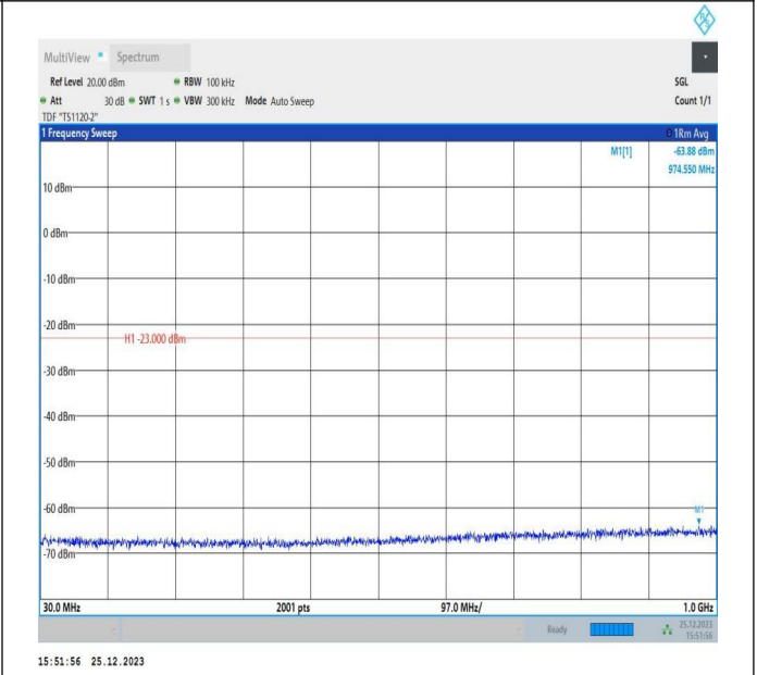
66-66-15MHz-5MHz-16QAM-16QAM-132047-132140-1RB#0-0 ORB#0-30~1000MHz-PASS
