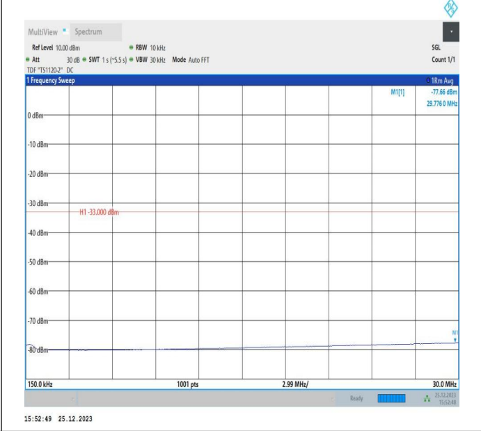
66-66-15MHz-5MHz-QPSK-QPSK-132047-132140-1RB#74-ORB#0-0.15~30MHz-PASS
