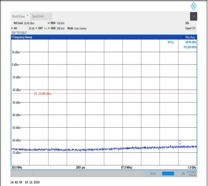
66-66-5MHz-15MHz-16QAM-16QAM-132353-132446-1RB#0-0ORB#0-30~1000MHz-PASS
