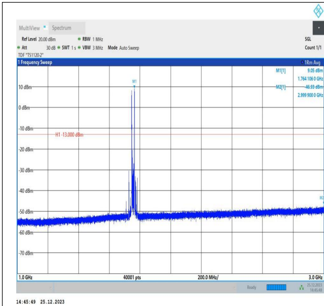
66-66-5MHz-15MHz-16QAM-16QAM-132353-132446-1RB#0-1RB#74-1000~3000MHz-PASS
