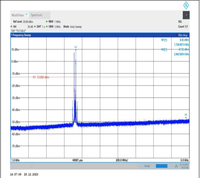
66-66-5MHz-15MHz-QPSK-QPSK-132002-132095-1RB#0-1R B#74-1000~3000MHz-PASS
