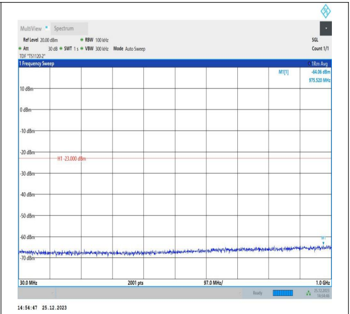
66-66-5MHz-15MHz-16QAM-16QAM-132504-132597-25RB# 0-75RB#0-30~1000MHz-PASS
