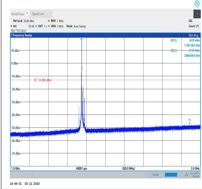
66-66-5MHz-15MHz-16QAM-16QAM-132353-132446-1RB#2 4-ORB#0-1000~3000MHz-PASS
