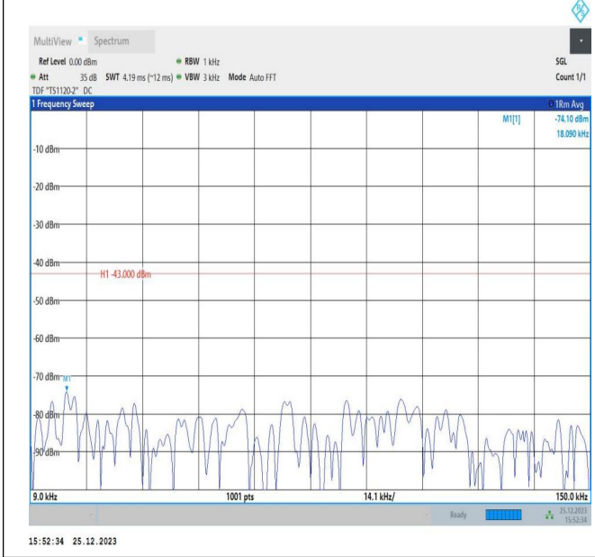
66-66-15MHz-5MHz-QPSK-QPSK-132047-132140-1RB#74-ORB#0-0.009~0.15MHz-PASS
