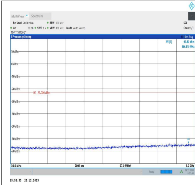
66-66-15MHz-5MHz-QPSK-QPSK-132047-132140-1RB#74-ORB#0-30~1000MHz-PASS
