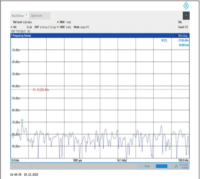
66-66-5MHz-15MHz-16QAM-16QAM-132504-132597-1RB#0-0ORB#0-0.009~0.15MHz-PASS
