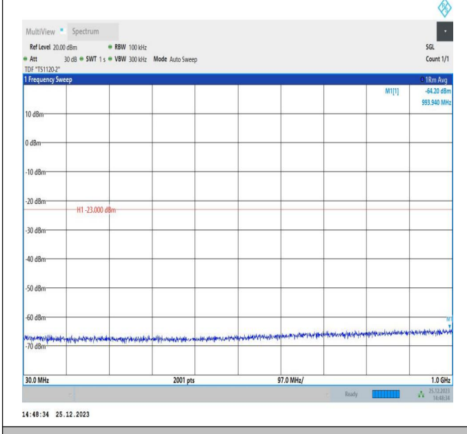
66-66-5MHz-15MHz-QPSK-QPSK-132504-132597-1RB#0-0 RB#0-30~1000MHz-PASS
