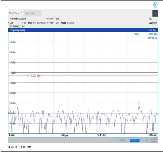
66-66-5MHz-15MHz-QPSK-QPSK-132504-132597-1RB#0-0 RB#0-0.009~0.15MHz-PASS
