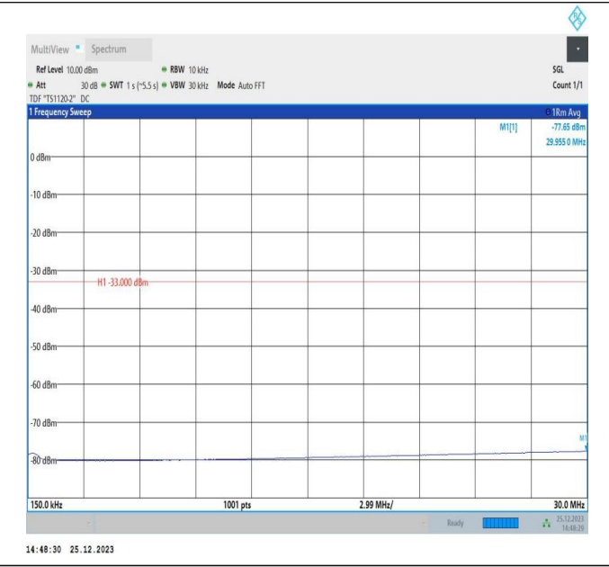
66-66-5MHz-15MHz-QPSK-QPSK-132504-132597-1RB#0-0R B#0-0.15~30MHz-PASS
