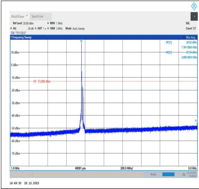
66-66-5MHz-15MHz-16QAM-16QAM-132504-132597-1RB#0-ORB#0-1000~3000MHz-PASS
