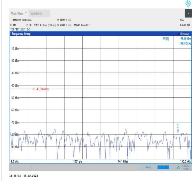
66-66-5MHz-15MHz-QPSK-QPSK-132002-132095-25RB#0-75RB#0-0.009~0.15MHz-PASS
