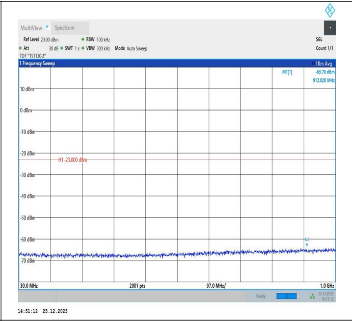
66-66-5MHz-15MHz-16QAM-16QAM-132504-132597-1RB#2 4-ORB#0-30~1000MHz-PASS
