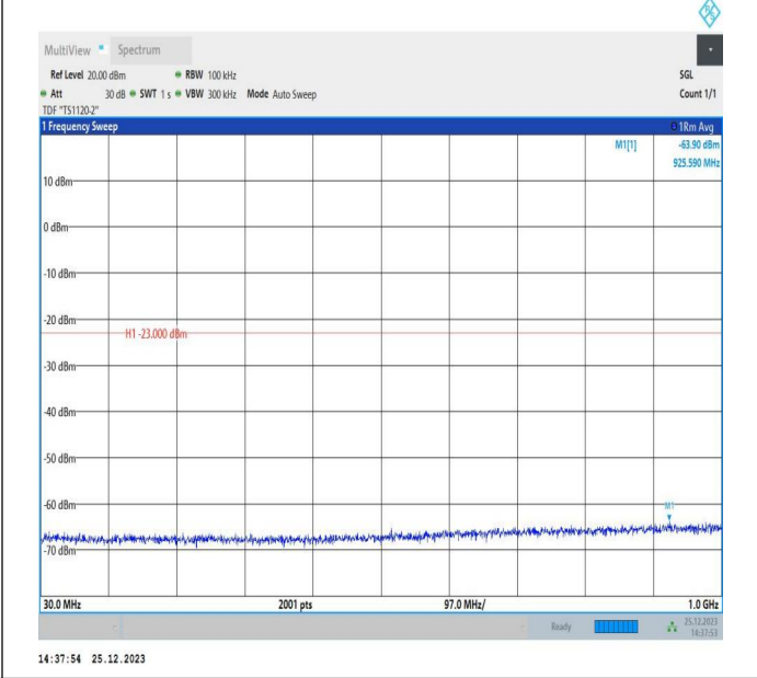
66-66-5MHz-15MHz-16QAM-16QAM-132002-132095-1RB#0- 1RB#74-30~1000MHz-PASS
