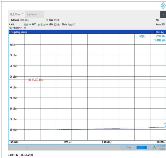
66-66-5MHz-15MHz-16QAM-16QAM-132504-132597-25RB# 0-75RB#0-0.15~30MHz-PASS
