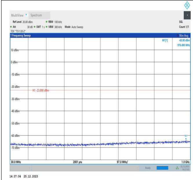
66-66-5MHz-15MHz-QPSK-QPSK-132002-132095-1RB#0-1 RB#74-30~1000MHz-PASS
