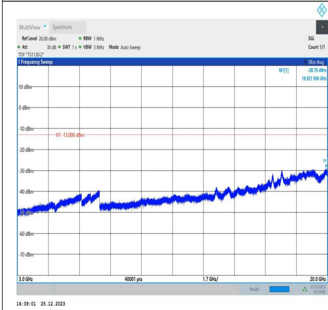
66-66-5MHz-15MHz-QPSK-QPSK-132002-132095-25RB#0-75RB#0-3000~20000MHz-PASS
