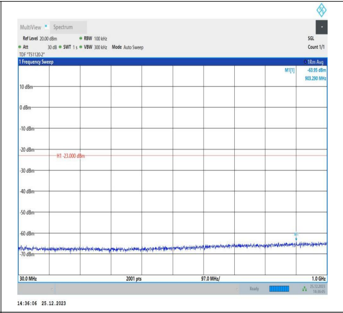
66-66-5MHz-15MHz-16QAM-16QAM-132002-132095-1RB#2 4-ORB#0-30~1000MHz-PASS
