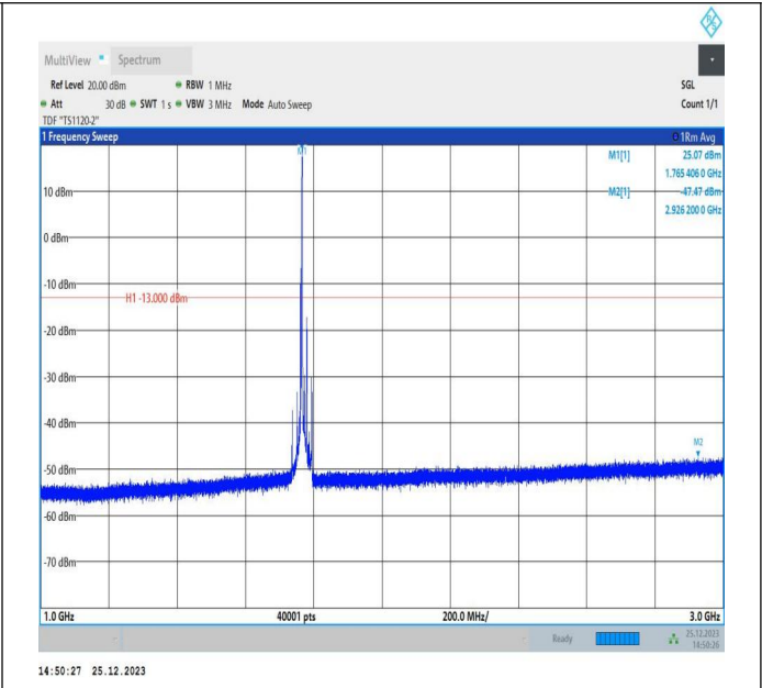
66-66-5MHz-15MHz-QPSK-QPSK-132504-132597-1RB#24-ORB#0-1000~3000MHz-PASS
