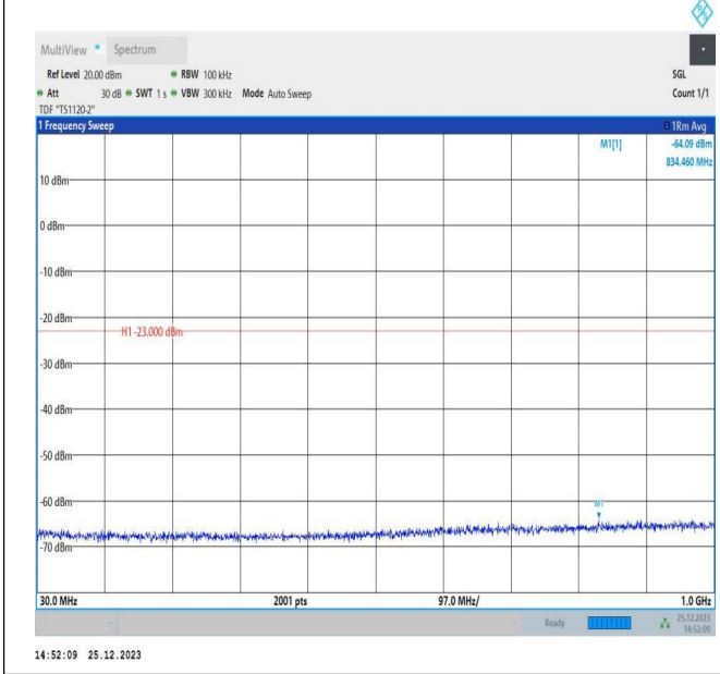
66-66-5MHz-15MHz-QPSK-QPSK-132504-132597-1RB#0-1 RB#74-30~1000MHz-PASS
