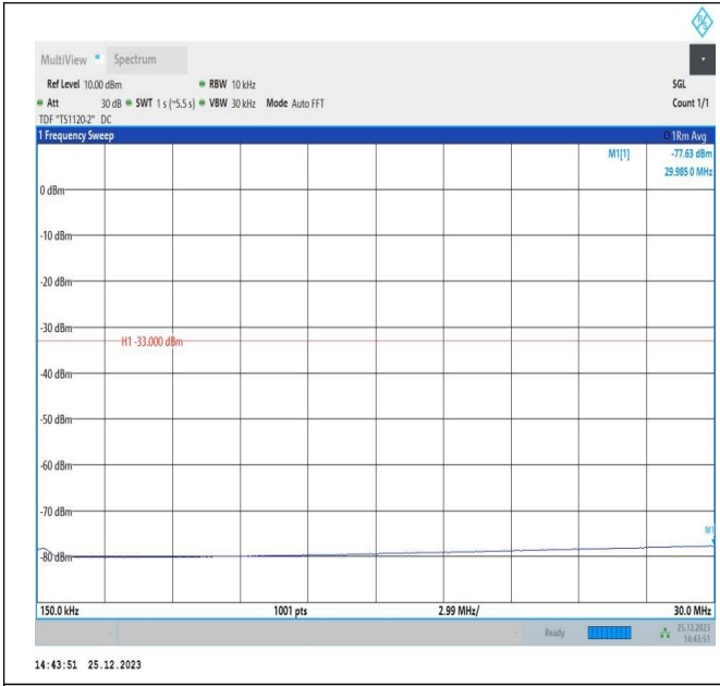
66-66-5MHz-15MHz-16QAM-16QAM-132353-132446-1RB#2 4-ORB#0-0.15~30MHz-PASS
