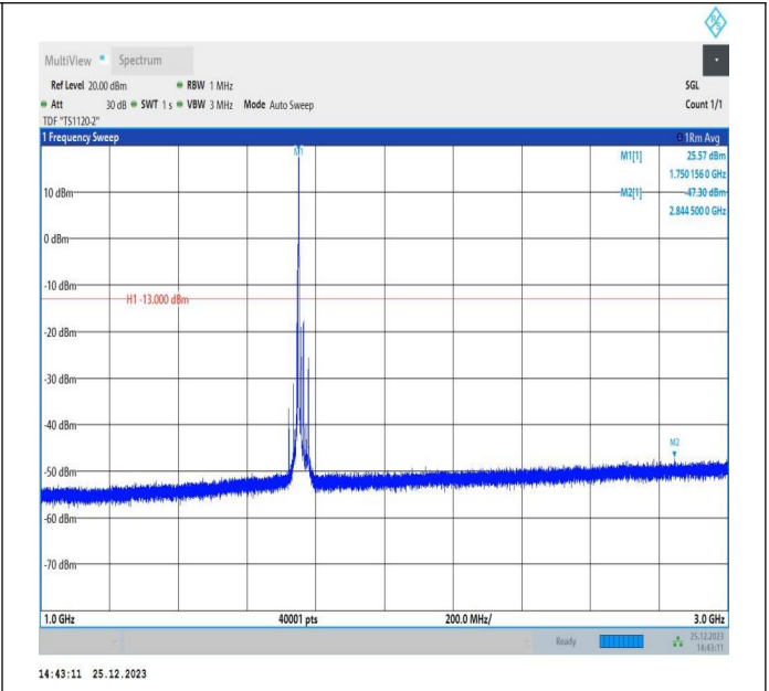
66-66-5MHz-15MHz-QPSK-QPSK-132353-132446-1RB#24-ORB#0-1000~3000MHz-PASS
