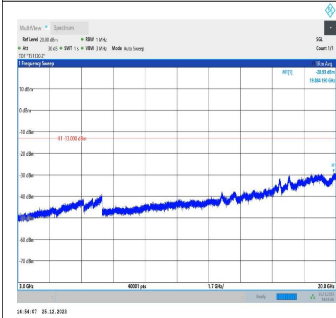
66-66-5MHz-15MHz-QPSK-QPSK-132504-132597-25RB#0-75RB#0-3000~20000MHz-PASS
