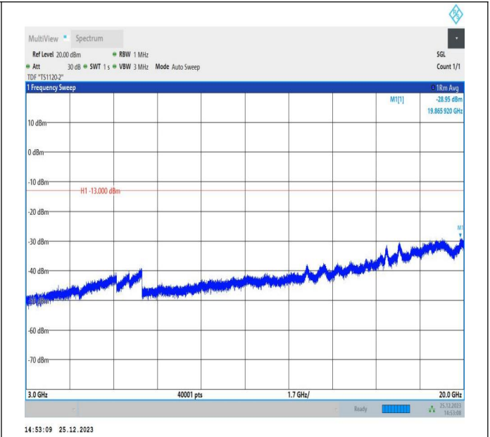
66-66-5MHz-15MHz-16QAM-16QAM-132504-132597-1RB#0-1RB#74-3000~20000MHz-PASS
