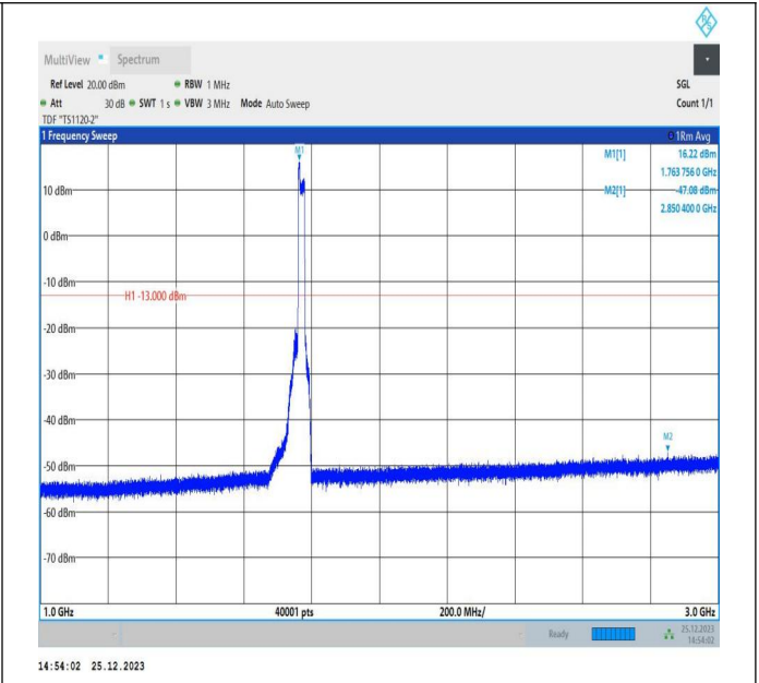
66-66-5MHz-15MHz-QPSK-QPSK-132504-132597-25RB#0-75RB#0-1000~3000MHz-PASS
