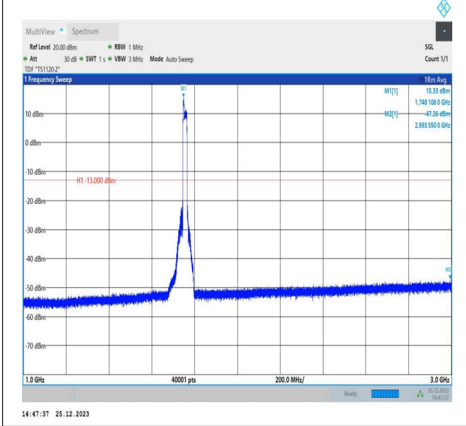
66-66-5MHz-15MHz-16QAM-16QAM-132353-132446-25RB# 0-75RB#0-1000~3000MHz-PASS
