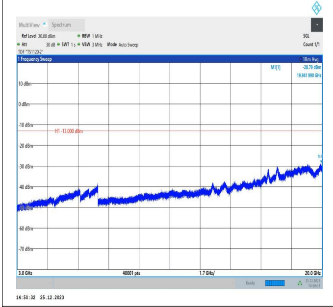
66-66-5MHz-15MHz-QPSK-QPSK-132504-132597-1RB#24-ORB#0-3000~20000MHz-PASS
