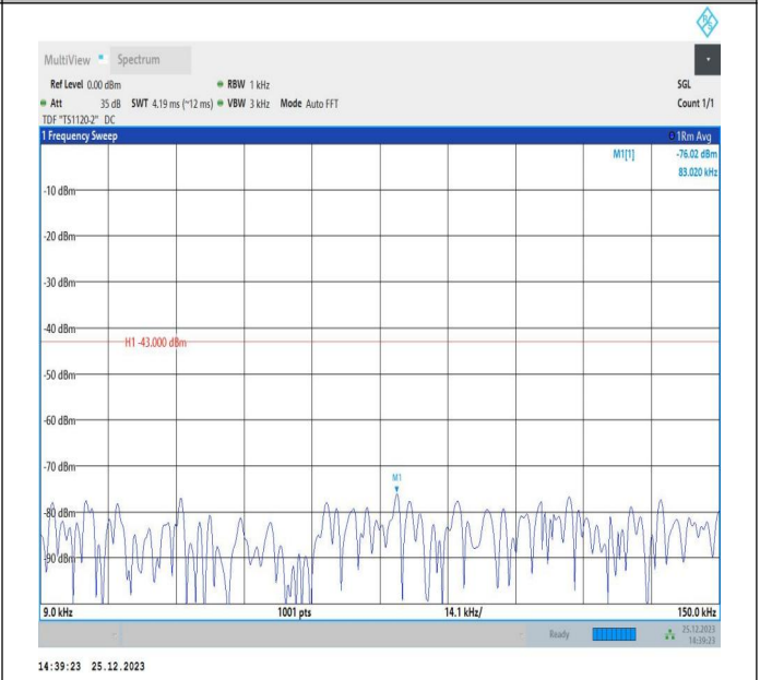
66-66-5MHz-15MHz-16QAM-16QAM-132002-132095-25RB#0-75RB#0-0.009~0.15MHz-PASS
