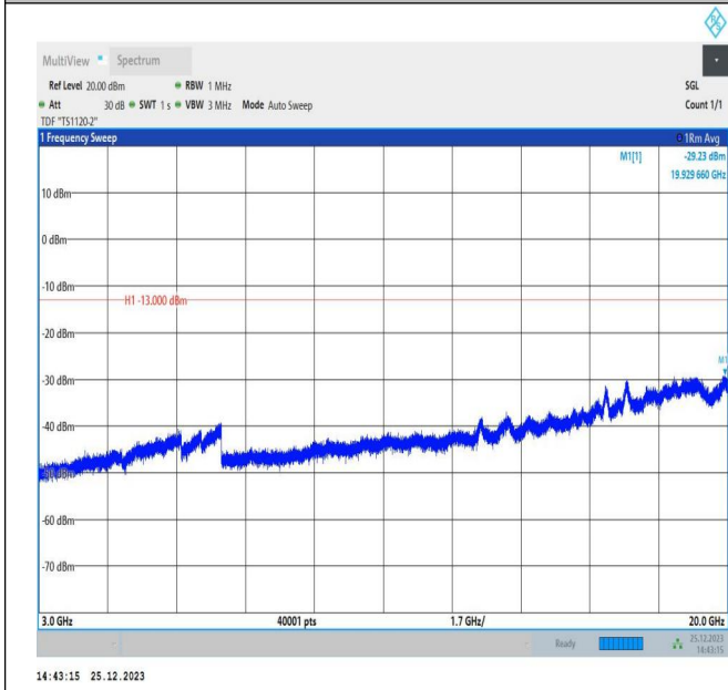
66-66-5MHz-15MHz-QPSK-QPSK-132353-132446-1RB#24-ORB#0-3000~20000MHz-PASS
