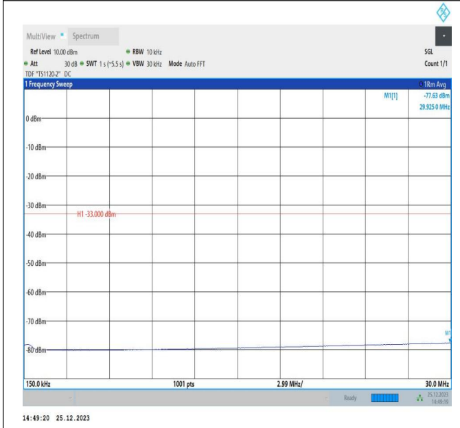
66-66-5MHz-15MHz-16QAM-16QAM-132504-132597-1RB#0-0ORB#0-0.15~30MHz-PASS
