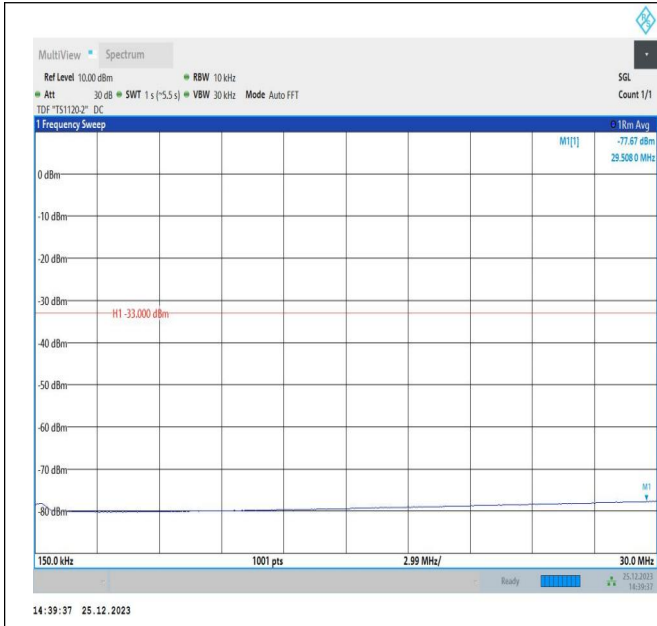
66-66-5MHz-15MHz-16QAM-16QAM-132002-132095-25RB# 0-75RB#0-0.15~30MHz-PASS
