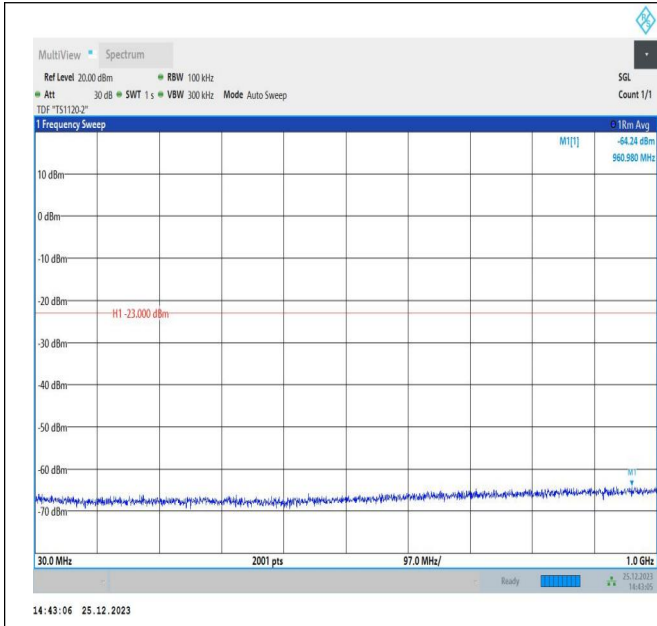
66-66-5MHz-15MHz-QPSK-QPSK-132353-132446-1RB#24-ORB#0-30~1000MHz-PASS
