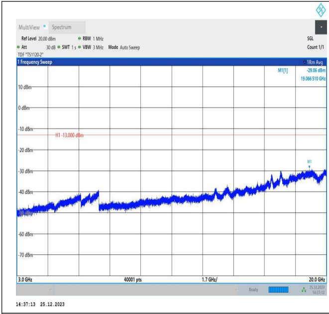
66-66-5MHz-15MHz-QPSK-QPSK-132002-132095-1RB#0-1 RB#74-3000~20000MHz-PASS
