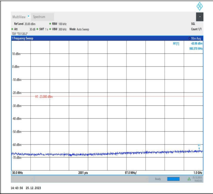
66-66-5MHz-15MHz-16QAM-16QAM-132353-132446-1RB#2 4-ORB#0-30~1000MHz-PASS
