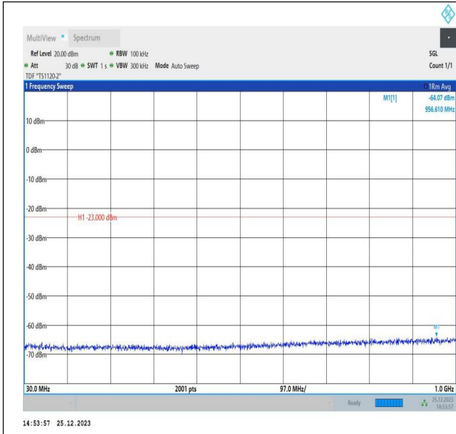
66-66-5MHz-15MHz-QPSK-QPSK-132504-132597-25RB#0-75RB#0-30~1000MHz-PASS
