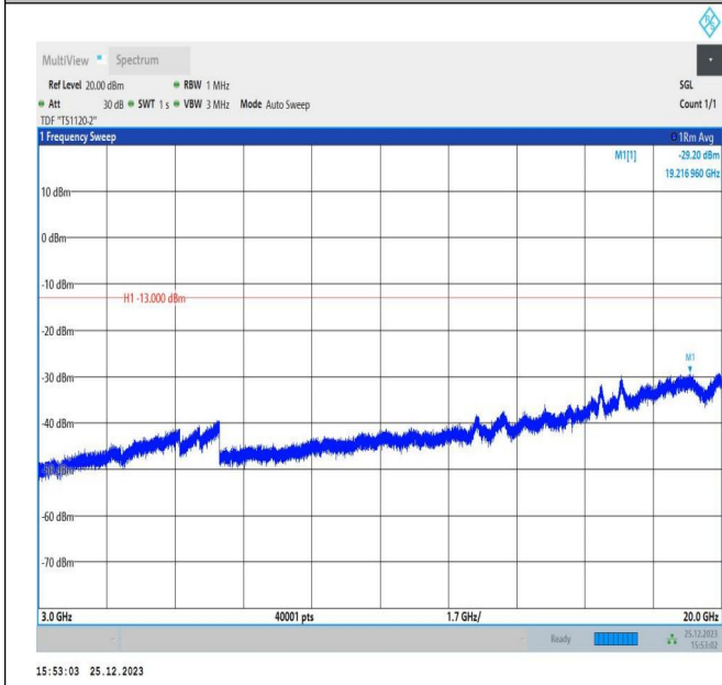
66-66-15MHz-5MHz-QPSK-QPSK-132047-132140-1RB#74-ORB#0-3000~20000MHz-PASS
