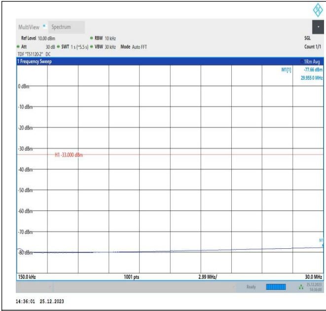
66-66-5MHz-15MHz-16QAM-16QAM-132002-132095-1RB#2 4-ORB#0-0.15~30MHz-PASS
