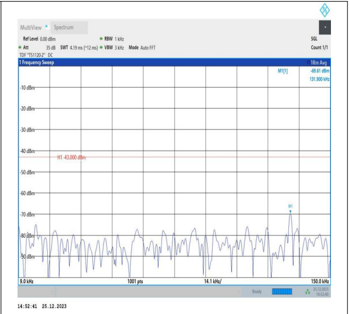
66-66-5MHz-15MHz-16QAM-16QAM-132504-132597-1RB#0- 1RB#74-0.009~0.15MHz-PASS
