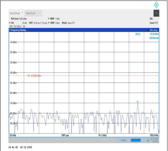
66-66-5MHz-15MHz-16QAM-16QAM-132353-132446-1RB#0-0ORB#0-0.009~0.15MHz-PASS
