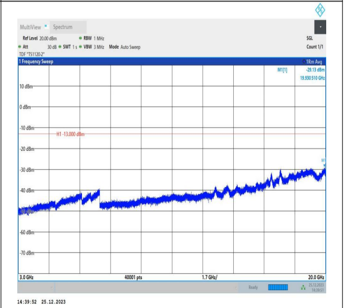
66-66-5MHz-15MHz-16QAM-16QAM-132002-132095-25RB# 0-75RB#0-3000~20000MHz-PASS
