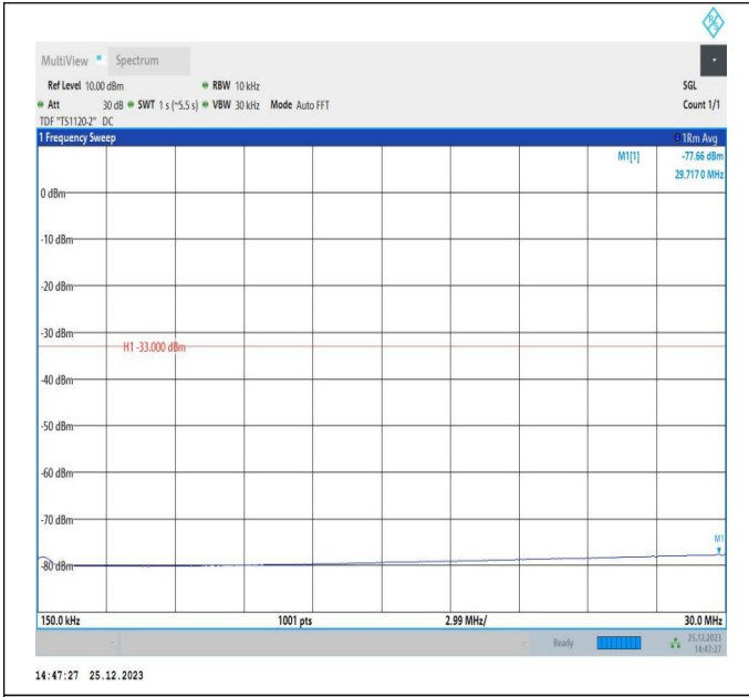
66-66-5MHz-15MHz-16QAM-16QAM-132353-132446-25RB# 0-75RB#0-0.15~30MHz-PASS
