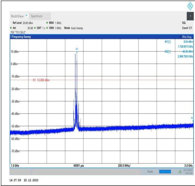
66-66-5MHz-15MHz-16QAM-16QAM-132002-132095-1RB#0-1RB#74-1000~3000MHz-PASS
