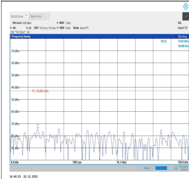
66-66-5MHz-15MHz-QPSK-QPSK-132353-132446-25RB#0-75RB#0-0.009~0.15MHz-PASS
