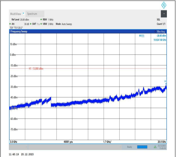
66-66-10MHz-5MHz-16QAM-16QAM-132022-132094-1RB#0-1RB#24-3000~20000MHz-PASS
