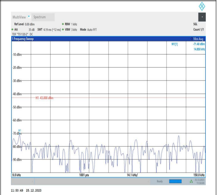
66-66-10MHz-5MHz-16QAM-16QAM-132397-132469-1RB#49-ORB#0-0.009~0.15MHz-PASS
