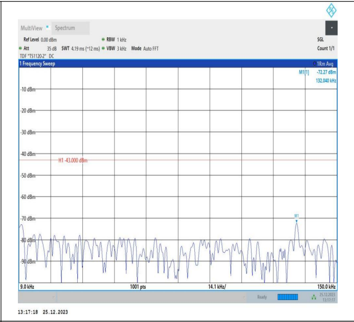
66-66-10MHz-10MHz-16QAM-16QAM-132022-132121-1RB#0-ORB#0-0.009~0.15MHz-PASS
