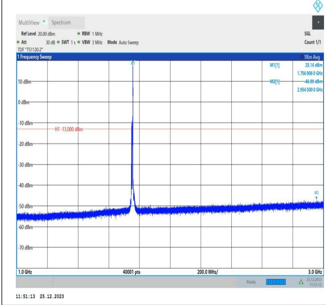
66-66-10MHz-5MHz-16QAM-16QAM-132397-132469-1RB#4 9-ORB#0-1000~3000MHz-PASS
