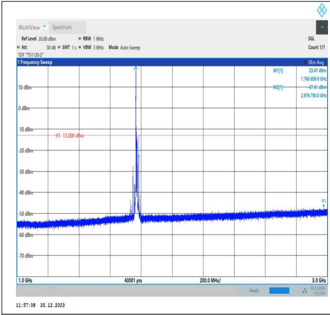
66-66-10MHz-5MHz-16QAM-16QAM-132572-132644-1RB#0-ORB#0-1000~3000MHz-PASS
