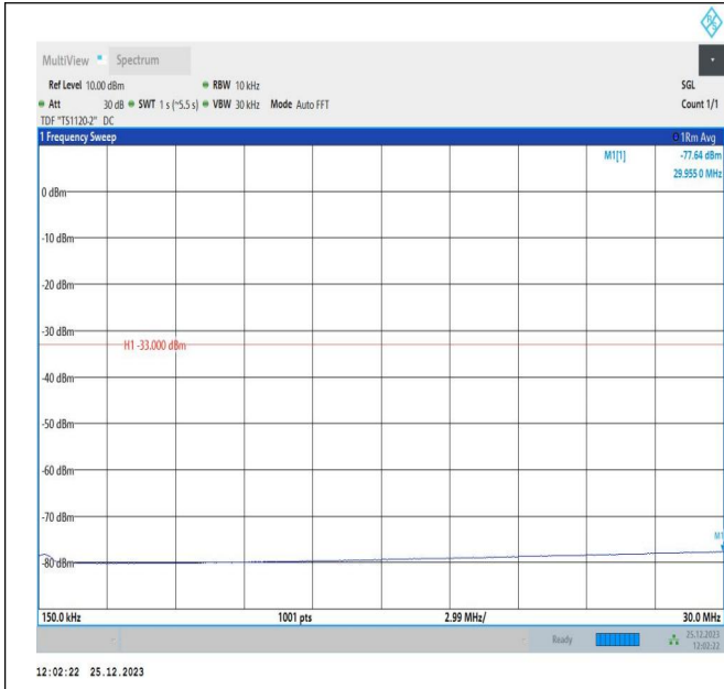
66-66-10MHz-5MHz-16QAM-16QAM-132572-132644-50RB# 0-25RB#0-0.15~30MHz-PASS
