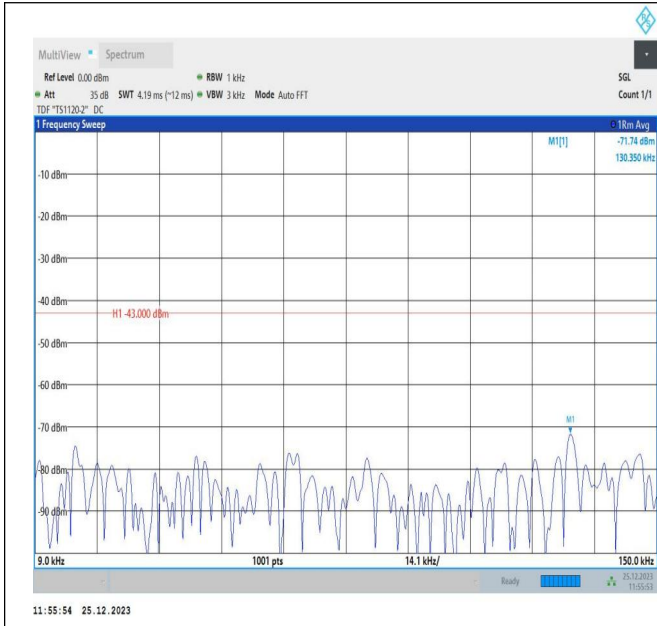
66-66-10MHz-5MHz-QPSK-QPSK-132572-132644-1RB#0-0 RB#0-0.009~0.15MHz-PASS
