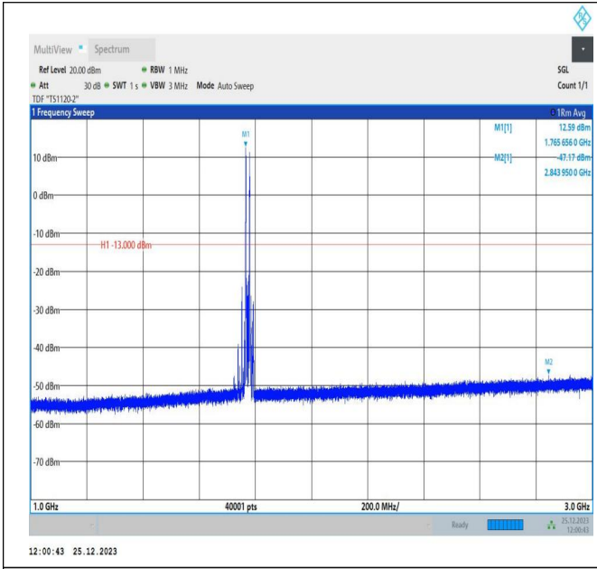
66-66-10MHz-5MHz-16QAM-16QAM-132572-132644-1RB#0-1RB#24-1000~3000MHz-PASS
