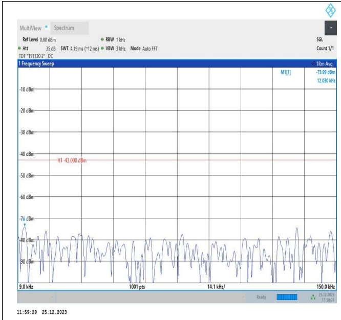
66-66-10MHz-5MHz-QPSK-QPSK-132572-132644-1RB#0-1 RB#24-0.009~0.15MHz-PASS
