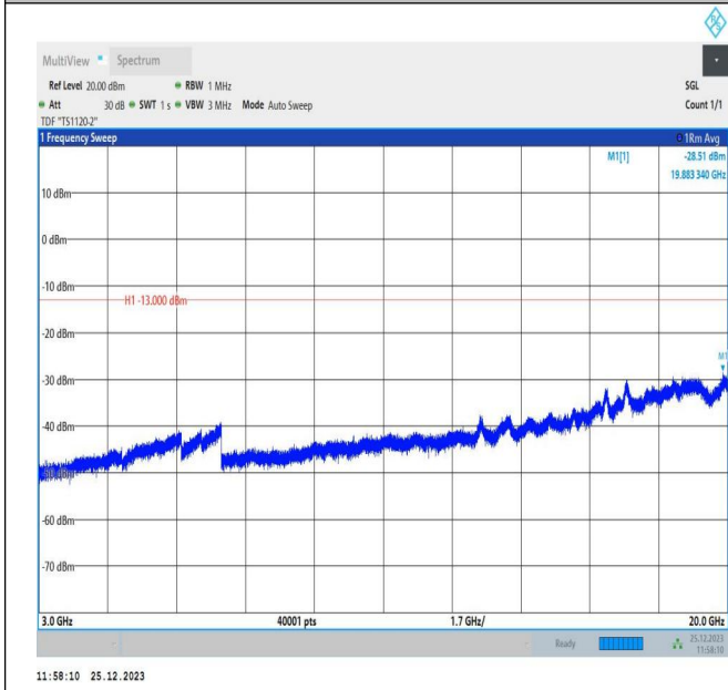
66-66-10MHz-5MHz-QPSK-QPSK-132572-132644-1RB#49-ORB#0-3000~20000MHz-PASS
