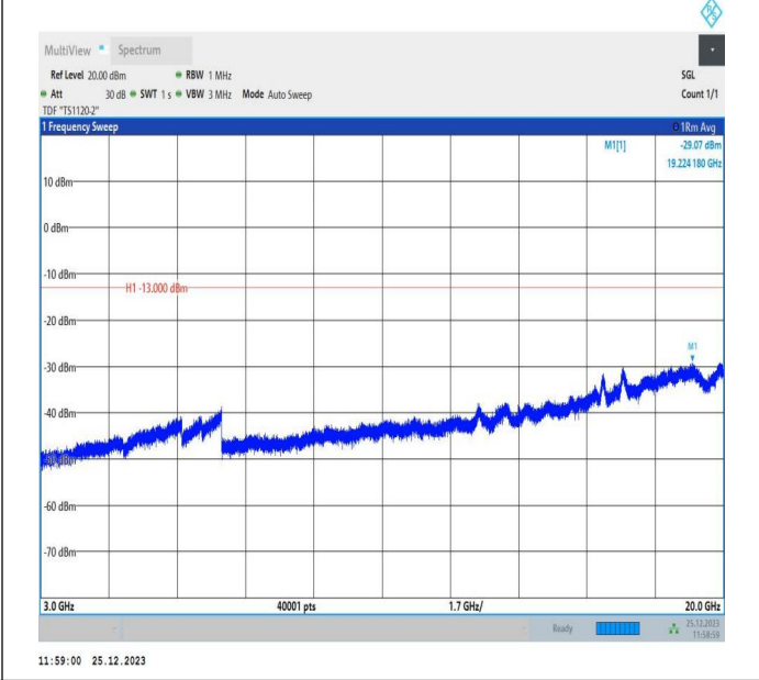
66-66-10MHz-5MHz-16QAM-16QAM-132572-132644-1RB#4 9-ORB#0-3000~20000MHz-PASS
