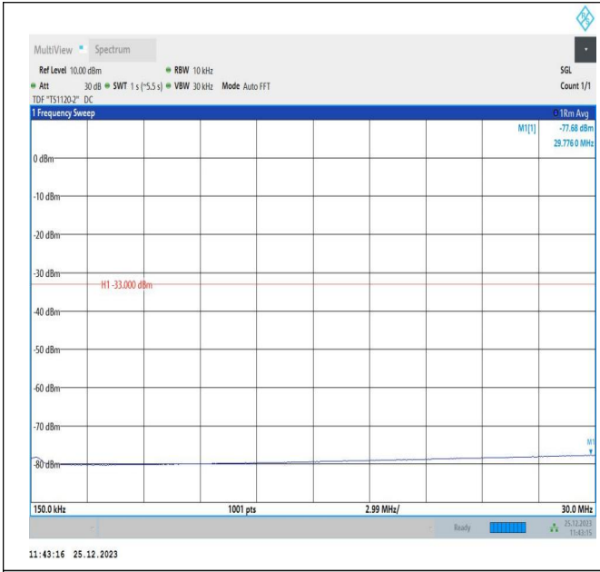
66-66-10MHz-5MHz-16QAM-16QAM-132022-132094-1RB#4 9-ORB#0-0.15~30MHz-PASS
