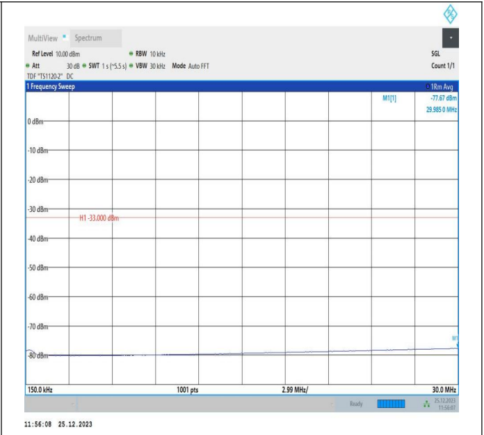
66-66-10MHz-5MHz-QPSK-QPSK-132572-132644-1RB#0-0R B#0-0.15~30MHz-PASS
