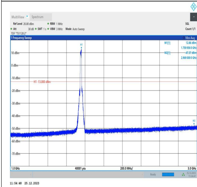
66-66-10MHz-5MHz-16QAM-16QAM-132397-132469-50RB# 0-25RB#0-1000~3000MHz-PASS
