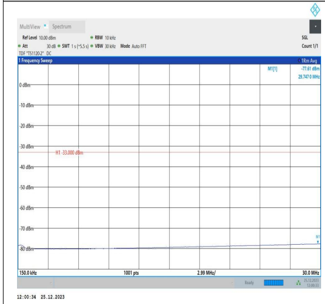
66-66-10MHz-5MHz-16QAM-16QAM-132572-132644-1RB#0 -1RB#24-0.15~30MHz-PASS
