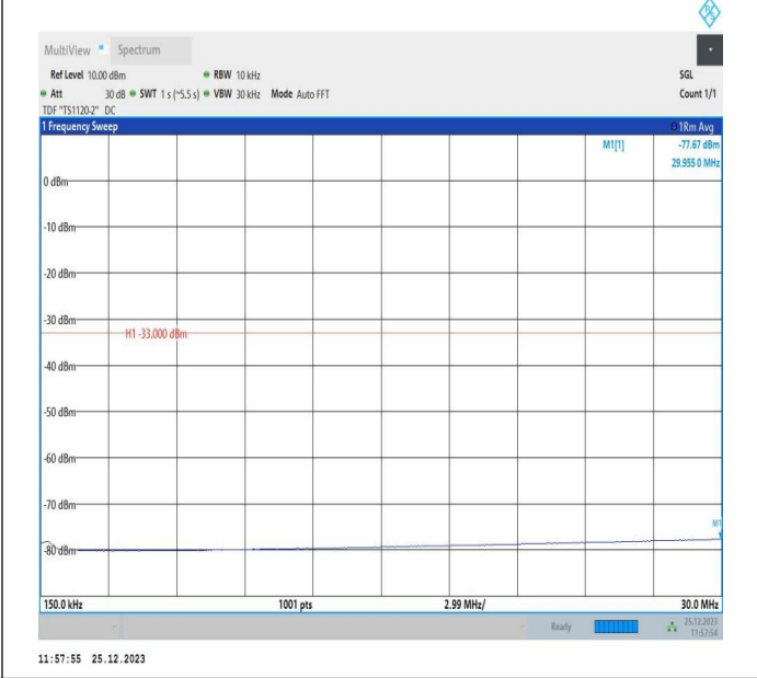
66-66-10MHz-5MHz-QPSK-QPSK-132572-132644-1RB#49-ORB#0-0.15~30MHz-PASS
