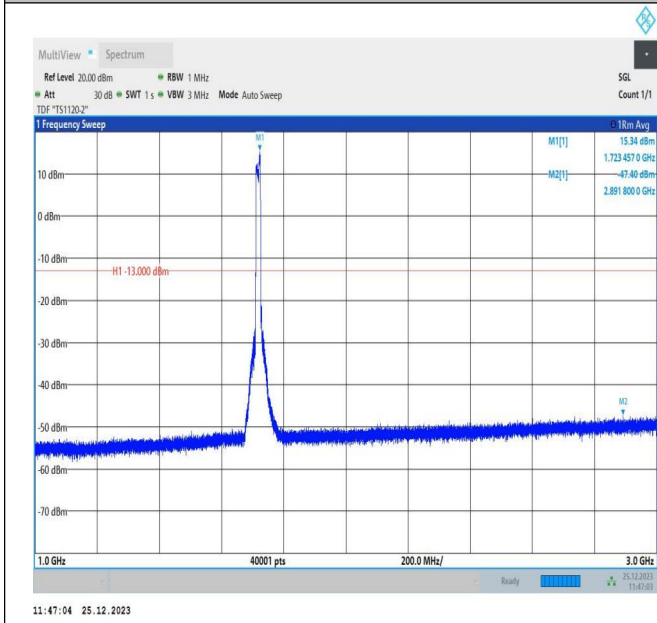
66-66-10MHz-5MHz-16QAM-16QAM-132022-132094-50RB# 0-25RB#0-1000~3000MHz-PASS
