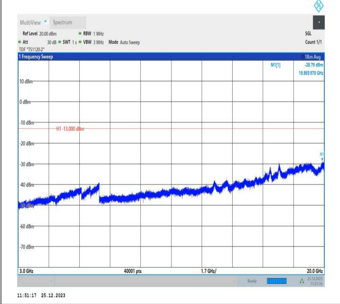
66-66-10MHz-5MHz-16QAM-16QAM-132397-132469-1RB#4 9-ORB#0-3000~20000MHz-PASS
