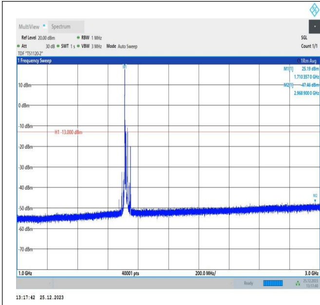
66-66-10MHz-10MHz-16QAM-16QAM-132022-132121-1RB# 0-ORB#0-1000~3000MHz-PASS
