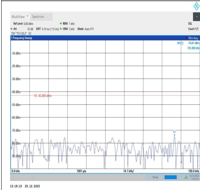
66-66-10MHz-10MHz-QPSK-QPSK-132022-132121-1RB#49 -ORB#0-0.009~0.15MHz-PASS
