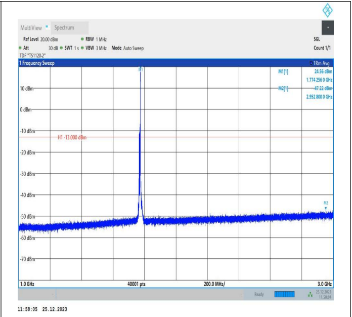
66-66-10MHz-5MHz-QPSK-QPSK-132572-132644-1RB#49-ORB#0-1000~3000MHz-PASS
