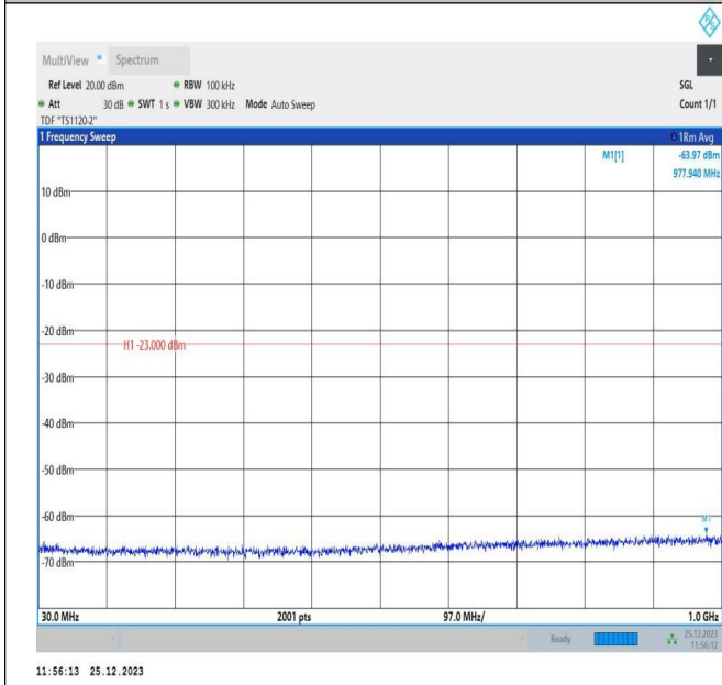
66-66-10MHz-5MHz-QPSK-QPSK-132572-132644-1RB#0-0 RB#0-30~1000MHz-PASS
