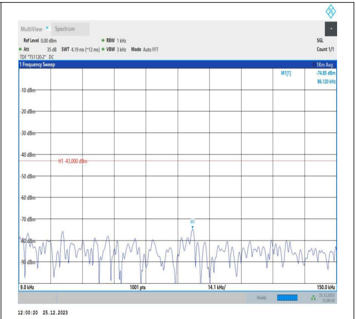
66-66-10MHz-5MHz-16QAM-16QAM-132572-132644-1RB#0- 1RB#24-0.009~0.15MHz-PASS
