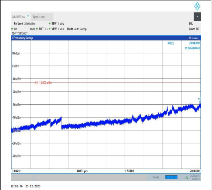
66-66-10MHz-5MHz-16QAM-16QAM-132572-132644-50RB# 0-25RB#0-3000~20000MHz-PASS
