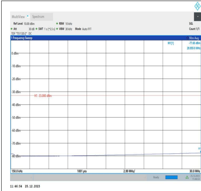
66-66-10MHz-5MHz-16QAM-16QAM-132022-132094-50RB# 0-25RB#0-0.15~30MHz-PASS
