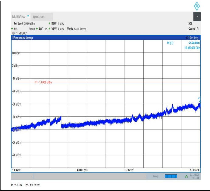
66-66-10MHz-5MHz-16QAM-16QAM-132397-132469-1RB#0-1RB#24-3000~20000MHz-PASS
