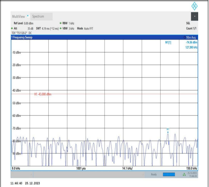
66-66-10MHz-5MHz-16QAM-16QAM-132022-132094-50RB#0-25RB#0-0.009~0.15MHz-PASS
