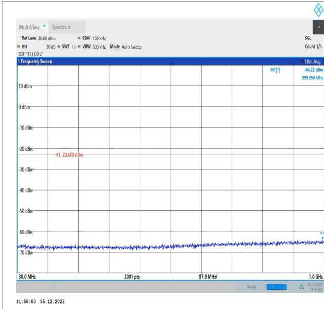
66-66-10MHz-5MHz-QPSK-QPSK-132572-132644-1RB#49-ORB#0-30~1000MHz-PASS
