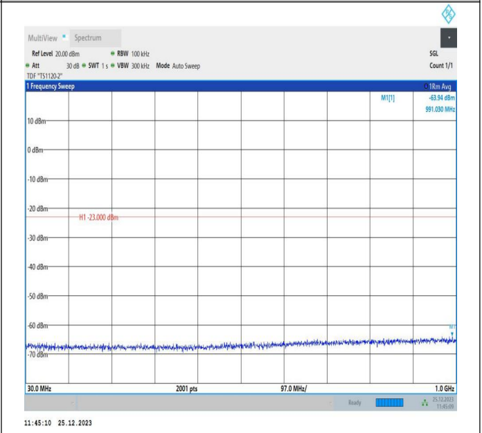
66-66-10MHz-5MHz-16QAM-16QAM-132022-132094-1RB#0- 1RB#24-30~1000MHz-PASS
