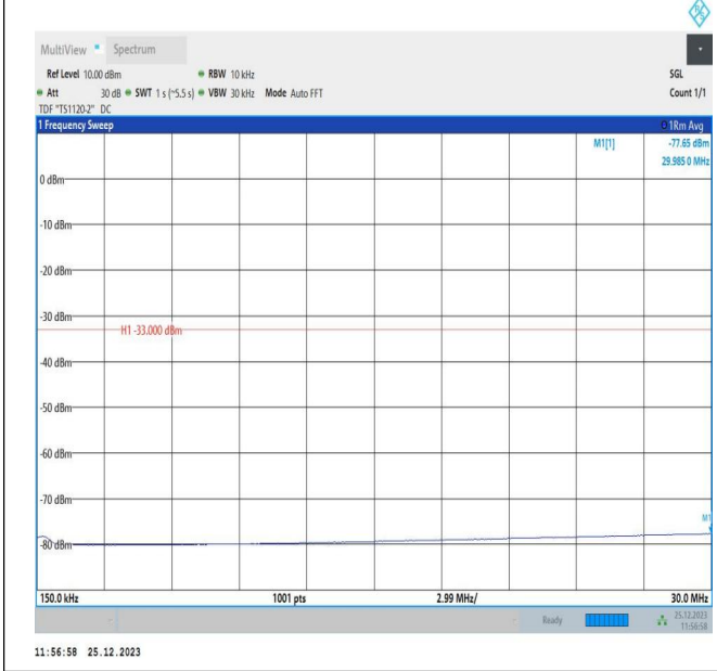
66-66-10MHz-5MHz-16QAM-16QAM-132572-132644-1RB#0-0 -ORB#0-0.15~30MHz-PASS
