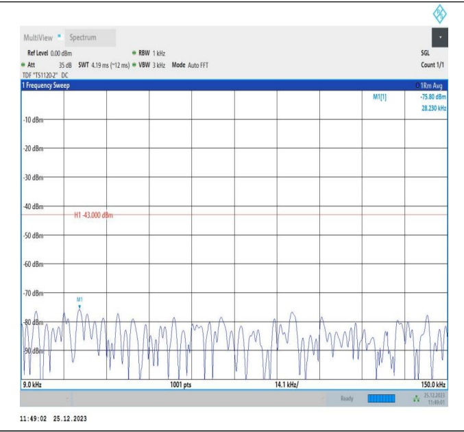
66-66-10MHz-5MHz-16QAM-16QAM-132397-132469-1RB#0-0RB#0-0.009~0.15MHz-PASS
