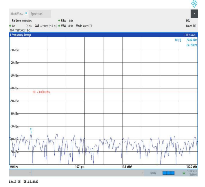
66-66-10MHz-10MHz-16QAM-16QAM-132022-132121-1RB# 49-ORB#0-0.009~0.15MHz-PASS
