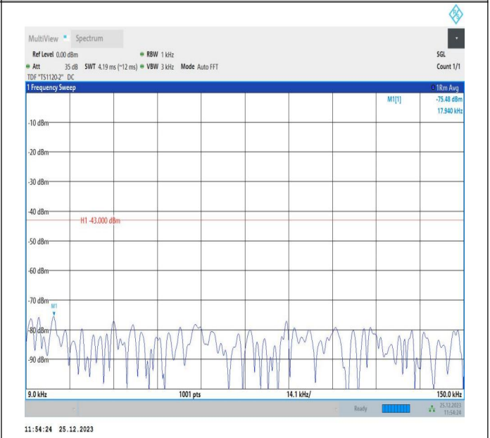
66-66-10MHz-5MHz-16QAM-16QAM-132397-132469-50RB#0-25RB#0-0.009~0.15MHz-PASS
