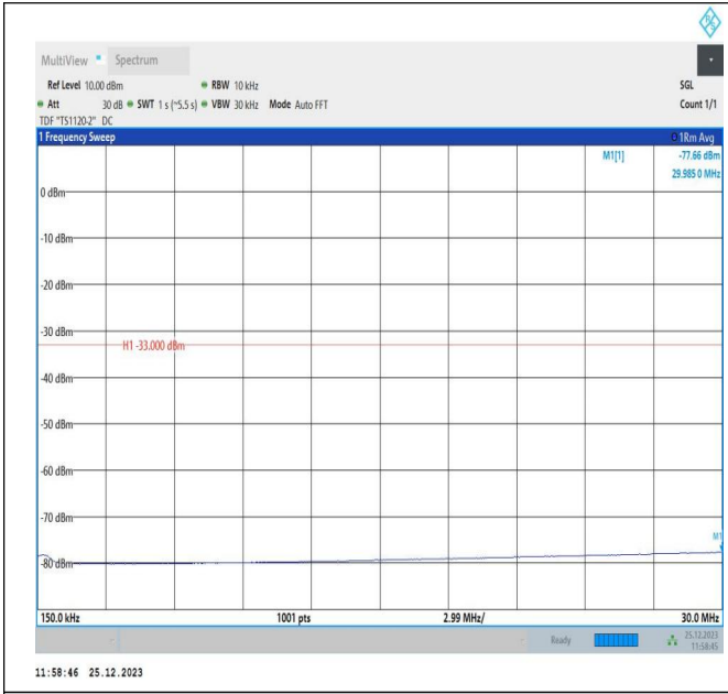
66-66-10MHz-5MHz-16QAM-16QAM-132572-132644-1RB#4 9-ORB#0-0.15~30MHz-PASS
