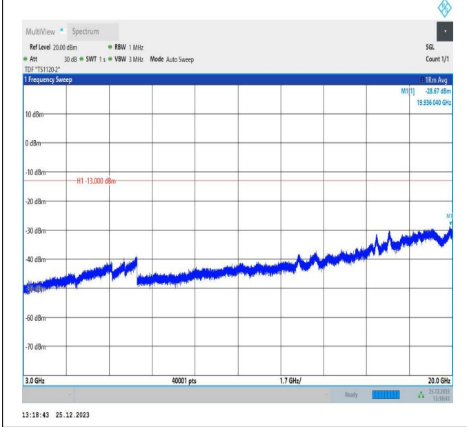
66-66-10MHz-10MHz-QPSK-QPSK-132022-132121-1RB#49 -ORB#0-3000~20000MHz-PASS
