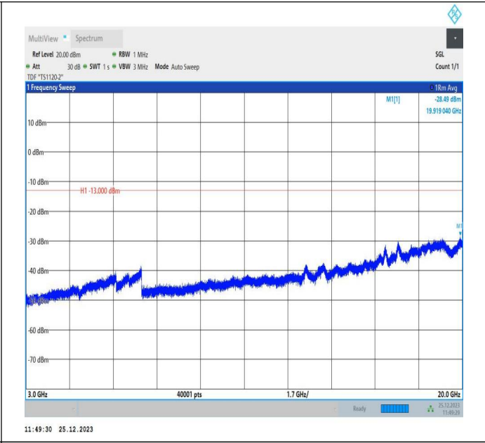
66-66-10MHz-5MHz-16QAM-16QAM-132397-132469-1RB#0-ORB#0-3000~20000MHz-PASS
