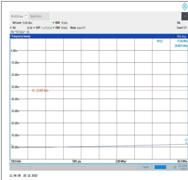
66-66-10MHz-5MHz-16QAM-16QAM-132397-132469-50RB# 0-25RB#0-0.15~30MHz-PASS
