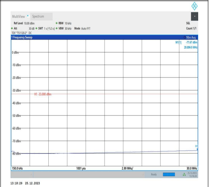
66-66-10MHz-10MHz-QPSK-QPSK-132022-132121-1RB#49- ORB#0-0.15~30MHz-PASS
