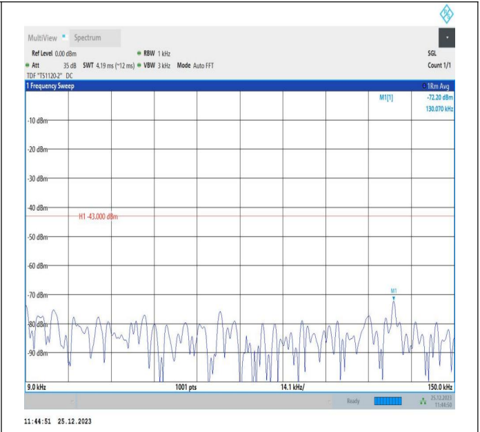
66-66-10MHz-5MHz-16QAM-16QAM-132022-132094-1RB#0- 1RB#24-0.009~0.15MHz-PASS
