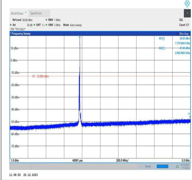
66-66-10MHz-5MHz-16QAM-16QAM-132572-132644-1RB#4 9-ORB#0-1000~3000MHz-PASS
