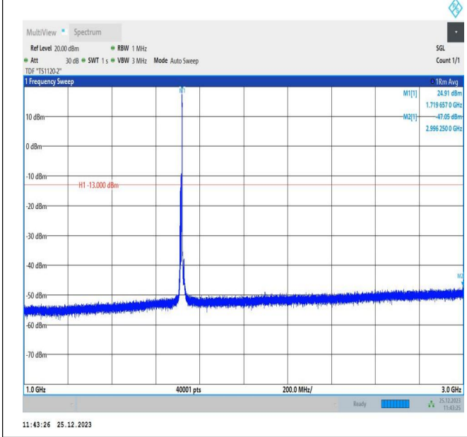
66-66-10MHz-5MHz-16QAM-16QAM-132022-132094-1RB#4 9-ORB#0-1000~3000MHz-PASS
