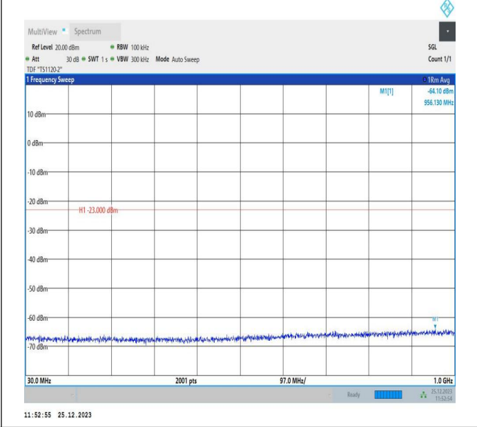
66-66-10MHz-5MHz-16QAM-16QAM-132397-132469-1RB#0- 1RB#24-30~1000MHz-PASS
