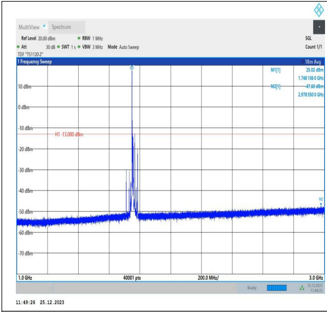
66-66-10MHz-5MHz-16QAM-16QAM-132397-132469-1RB#0-0RB#0-1000~3000MHz-PASS
