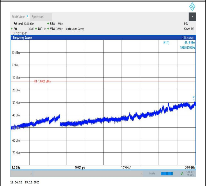
66-66-10MHz-5MHz-16QAM-16QAM-132397-132469-50RB# 0-25RB#0-3000~20000MHz-PASS
