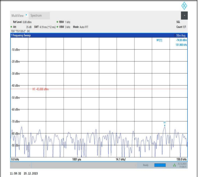
66-66-10MHz-5MHz-16QAM-16QAM-132572-132644-1RB#49-ORB#0-0.009~0.15MHz-PASS
