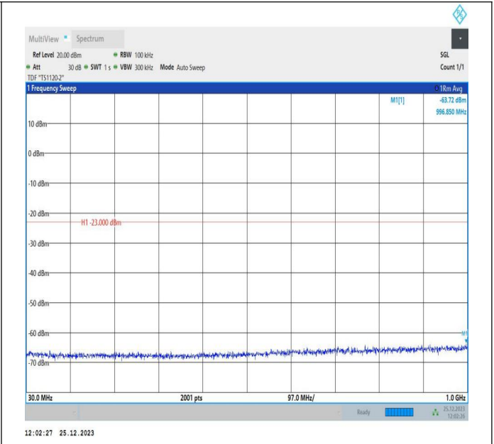
66-66-10MHz-5MHz-16QAM-16QAM-132572-132644-50RB# 0-25RB#0-30~1000MHz-PASS
