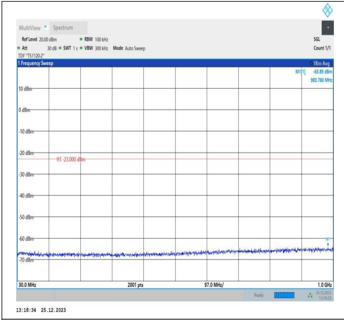
66-66-10MHz-10MHz-QPSK-QPSK-132022-132121-1RB#49 -ORB#0-30~1000MHz-PASS
