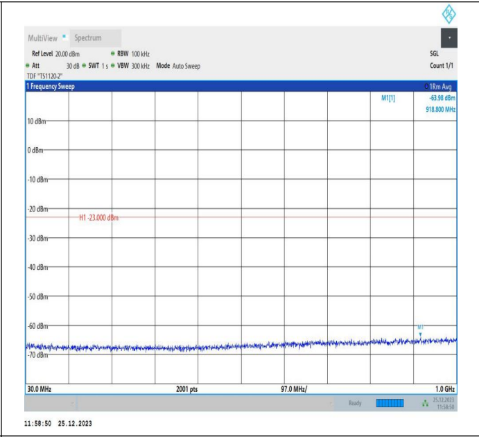
66-66-10MHz-5MHz-16QAM-16QAM-132572-132644-1RB#4 9-ORB#0-30~1000MHz-PASS
