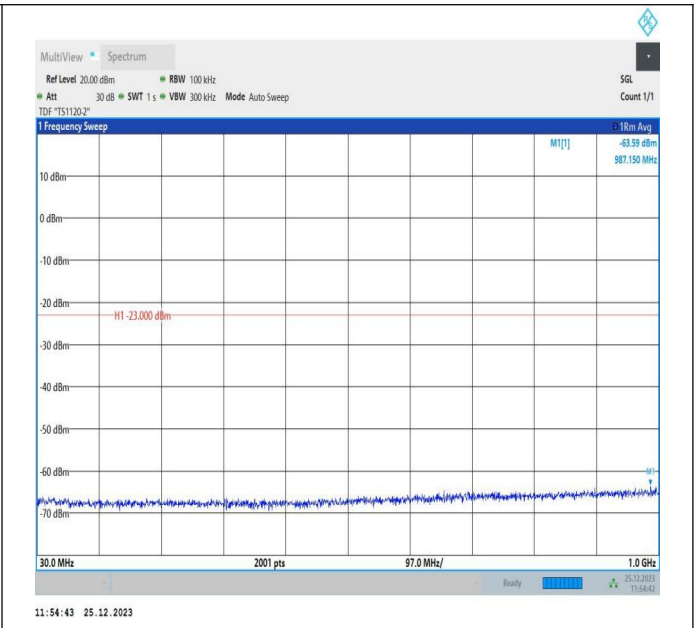
66-66-10MHz-5MHz-16QAM-16QAM-132397-132469-50RB# 0-25RB#0-30~1000MHz-PASS
