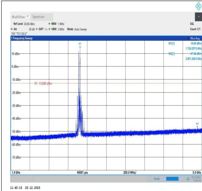
66-66-10MHz-5MHz-16QAM-16QAM-132022-132094-1RB#0-1RB#24-1000~3000MHz-PASS
