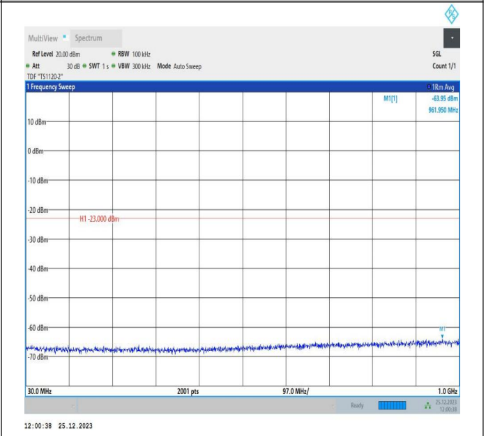
66-66-10MHz-5MHz-16QAM-16QAM-132572-132644-1RB#0- 1RB#24-30~1000MHz-PASS
