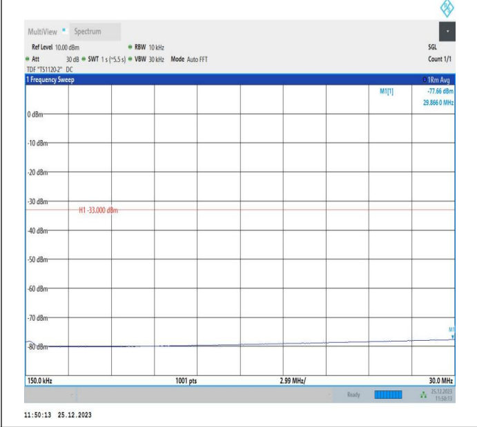
66-66-10MHz-5MHz-QPSK-QPSK-132397-132469-1RB#49-0RB#0-0.15~30MHz-PASS
