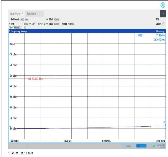
66-66-10MHz-5MHz-16QAM-16QAM-132022-132094-1RB#0 -1RB#24-0.15~30MHz-PASS
