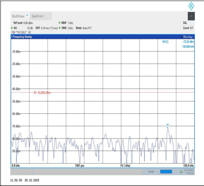
66-66-10MHz-5MHz-16QAM-16QAM-132397-132469-1RB#0- 1RB#24-0.009~0.15MHz-PASS
