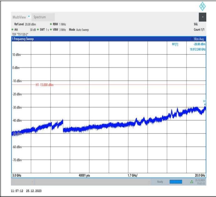
66-66-10MHz-5MHz-16QAM-16QAM-132572-132644-1RB#0-ORB#0-3000~20000MHz-PASS
