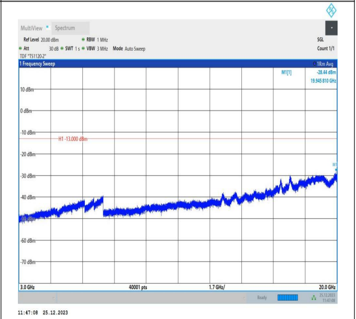
66-66-10MHz-5MHz-16QAM-16QAM-132022-132094-50RB# 0-25RB#0-3000~20000MHz-PASS
