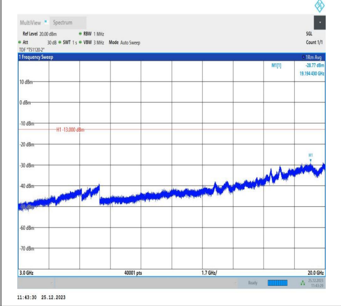
66-66-10MHz-5MHz-16QAM-16QAM-132022-132094-1RB#4 9-ORB#0-3000~20000MHz-PASS
