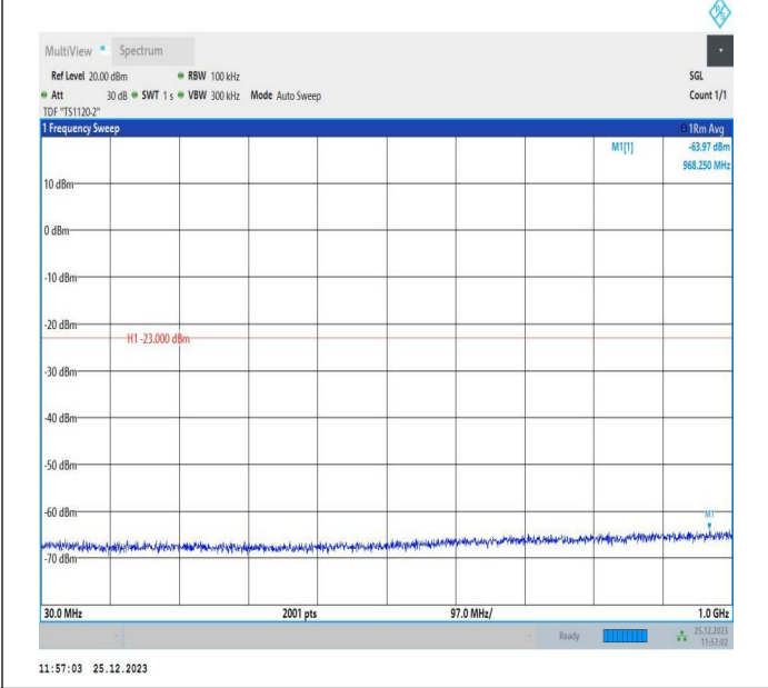
66-66-10MHz-5MHz-16QAM-16QAM-132572-132644-1RB#0-0 ORB#0-30~1000MHz-PASS
