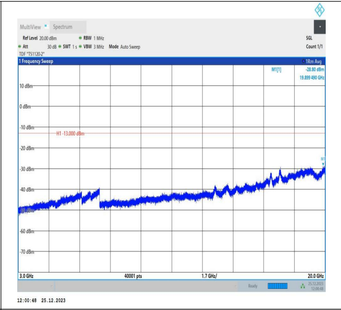
66-66-10MHz-5MHz-16QAM-16QAM-132572-132644-1RB#0-1RB#24-3000~20000MHz-PASS
