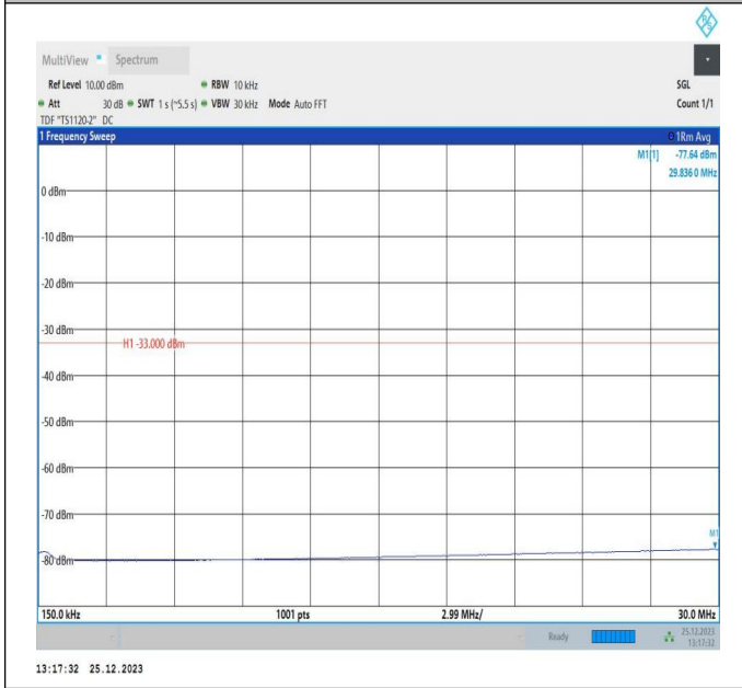
66-66-10MHz-10MHz-16QAM-16QAM-132022-132121-1RB#0-ORB#0-0.15~30MHz-PASS
