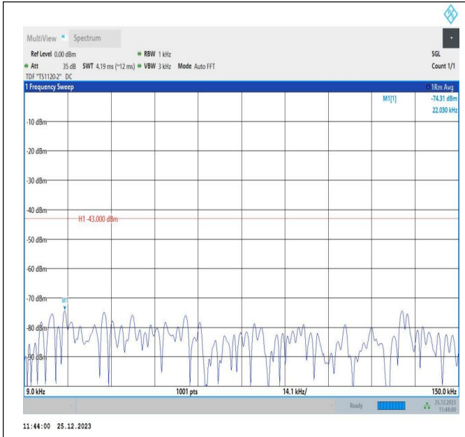
66-66-10MHz-5MHz-QPSK-QPSK-132022-132094-1RB#0-1 RB#24-0.009~0.15MHz-PASS
