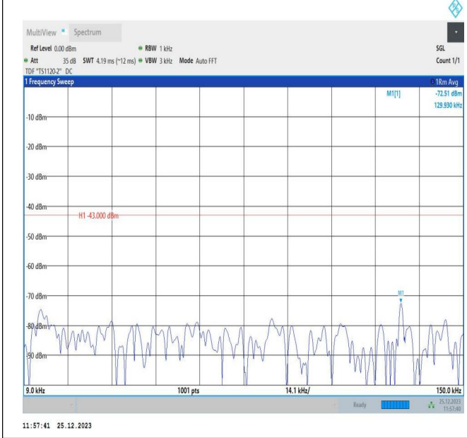
66-66-10MHz-5MHz-QPSK-QPSK-132572-132644-1RB#49-ORB#0-0.009~0.15MHz-PASS
