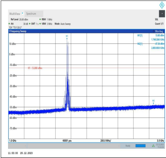
66-66-10MHz-5MHz-16QAM-16QAM-132397-132469-1RB#0-1RB#24-1000~3000MHz-PASS
