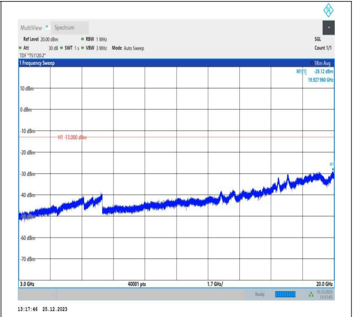
66-66-10MHz-10MHz-16QAM-16QAM-132022-132121-1RB# 0-ORB#0-3000~20000MHz-PASS
