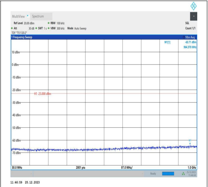
66-66-10MHz-5MHz-16QAM-16QAM-132022-132094-50RB# 0-25RB#0-30~1000MHz-PASS
