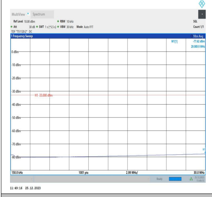
66-66-10MHz-5MHz-16QAM-16QAM-132397-132469-1RB#0-0RB#0-0.15~30MHz-PASS
