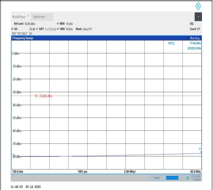
66-66-10MHz-5MHz-QPSK-QPSK-132022-132094-50RB#0-25RB#0-0.15~30MHz-PASS
