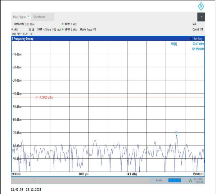
66-66-10MHz-5MHz-16QAM-16QAM-132572-132644-50RB#0-25RB#0-0.009~0.15MHz-PASS
