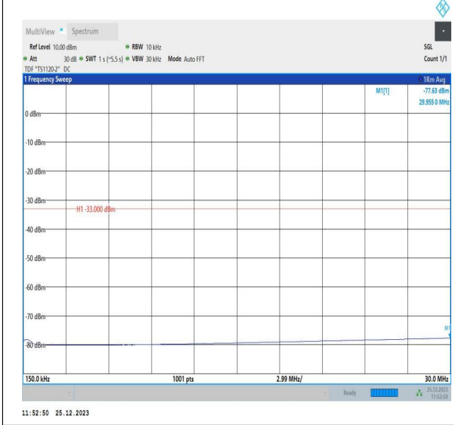
66-66-10MHz-5MHz-16QAM-16QAM-132397-132469-1RB#0 -1RB#24-0.15~30MHz-PASS
