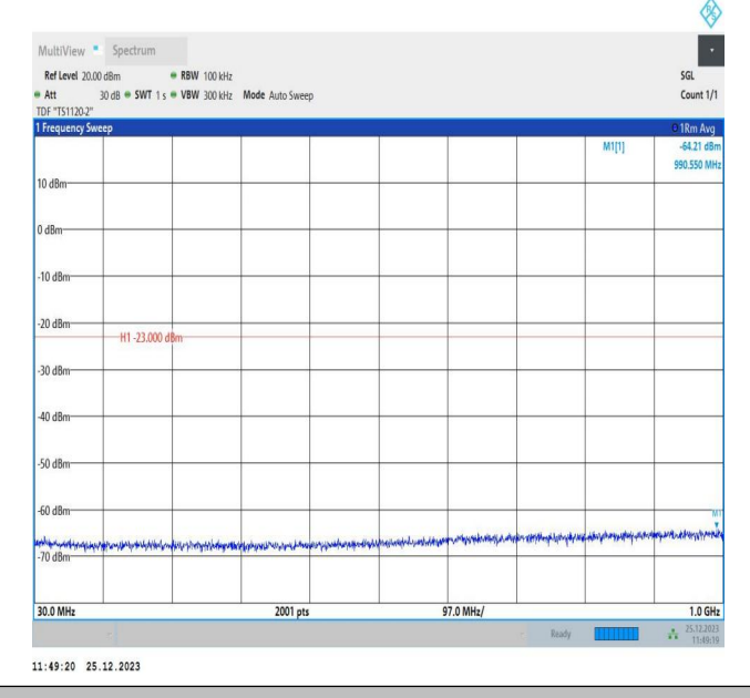
66-66-10MHz-5MHz-16QAM-16QAM-132397-132469-1RB#0-0RB#0-30~1000MHz-PASS
