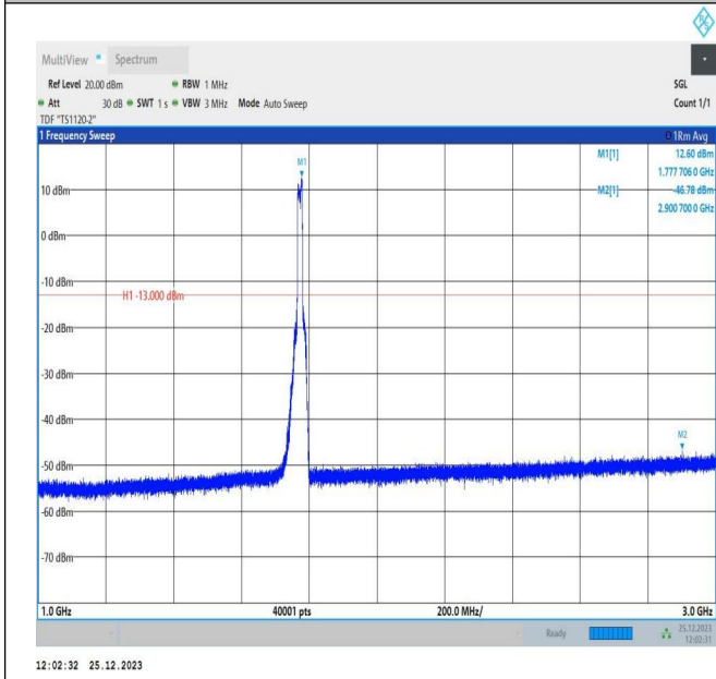
66-66-10MHz-5MHz-16QAM-16QAM-132572-132644-50RB# 0-25RB#0-1000~3000MHz-PASS
