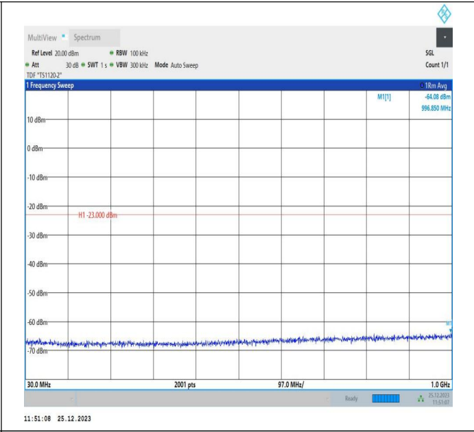
66-66-10MHz-5MHz-16QAM-16QAM-132397-132469-1RB#4 9-ORB#0-30~1000MHz-PASS
