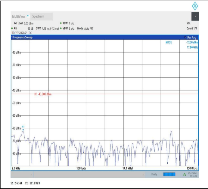
66-66-10MHz-5MHz-16QAM-16QAM-132572-132644-1RB#0-0 ORB#0-0.009~0.15MHz-PASS
