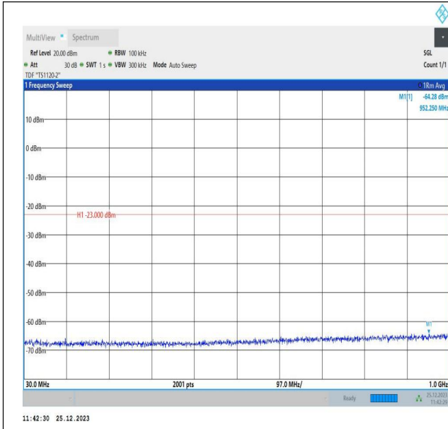
66-66-10MHz-5MHz-QPSK-QPSK-132022-132094-1RB#49-ORB#0-30~1000MHz-PASS
