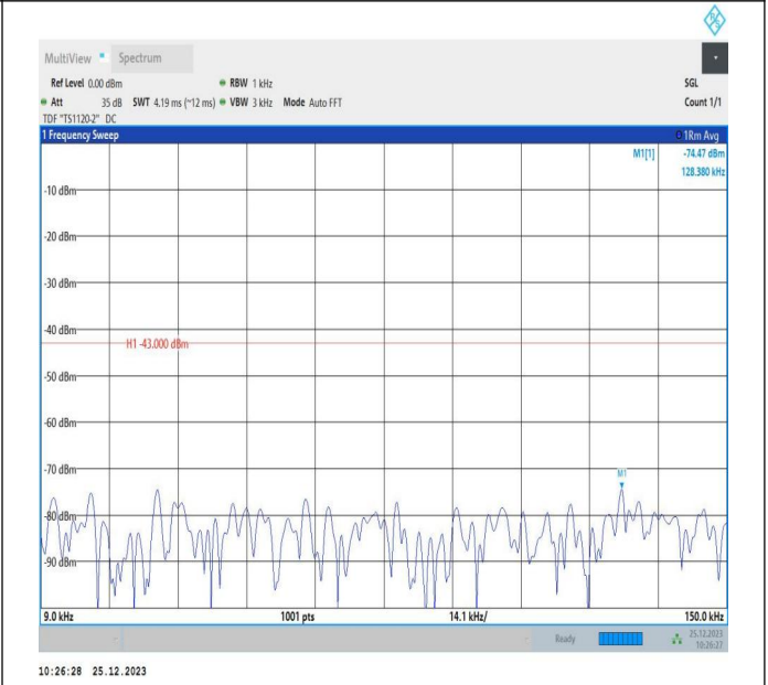
66-66-5MHz-10MHz-16QAM-16QAM-132375-132447-25RB#0-50RB#0-0.009~0.15MHz-PASS
