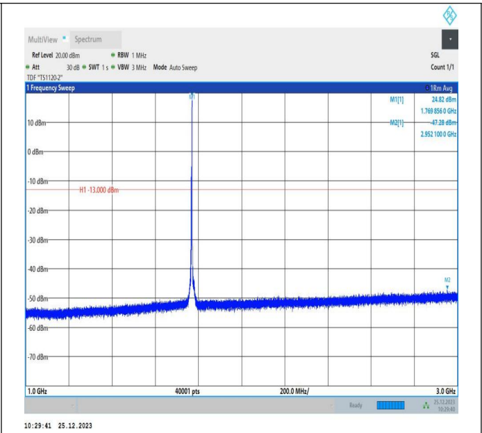
66-66-5MHz-10MHz-QPSK-QPSK-132550-132622-1RB#24-ORB#0-1000~3000MHz-PASS
