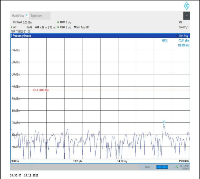
66-66-5MHz-10MHz-16QAM-16QAM-132550-132622-1RB#24-ORB#0-0.009~0.15MHz-PASS
