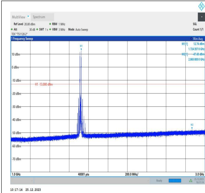
66-66-5MHz-10MHz-16QAM-16QAM-132000-132072-1RB#0-1RB#49-1000~3000MHz-PASS
