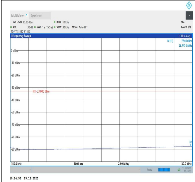
66-66-5MHz-10MHz-16QAM-16QAM-132375-132447-1RB#0 -1RB#49-0.15~30MHz-PASS
