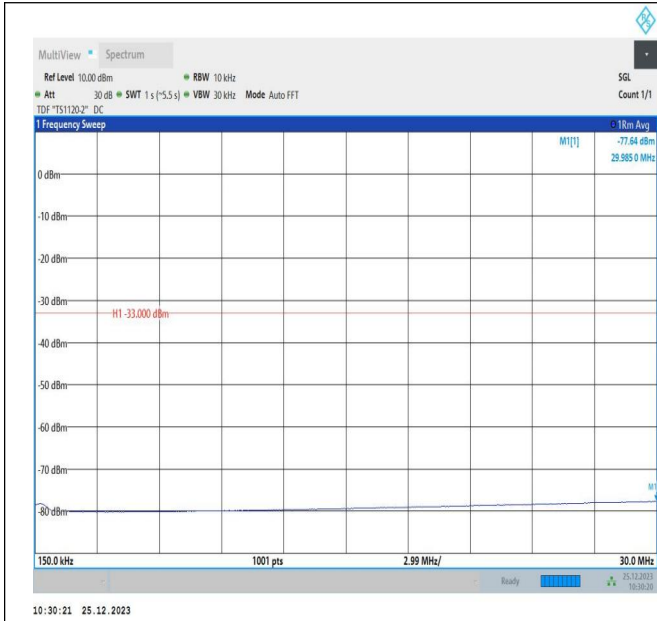
66-66-5MHz-10MHz-16QAM-16QAM-132550-132622-1RB#2 4-ORB#0-0.15~30MHz-PASS
