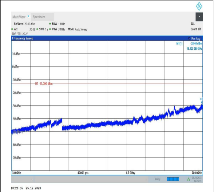
66-66-5MHz-10MHz-16QAM-16QAM-132375-132447-25RB# 0-50RB#0-3000~20000MHz-PASS
