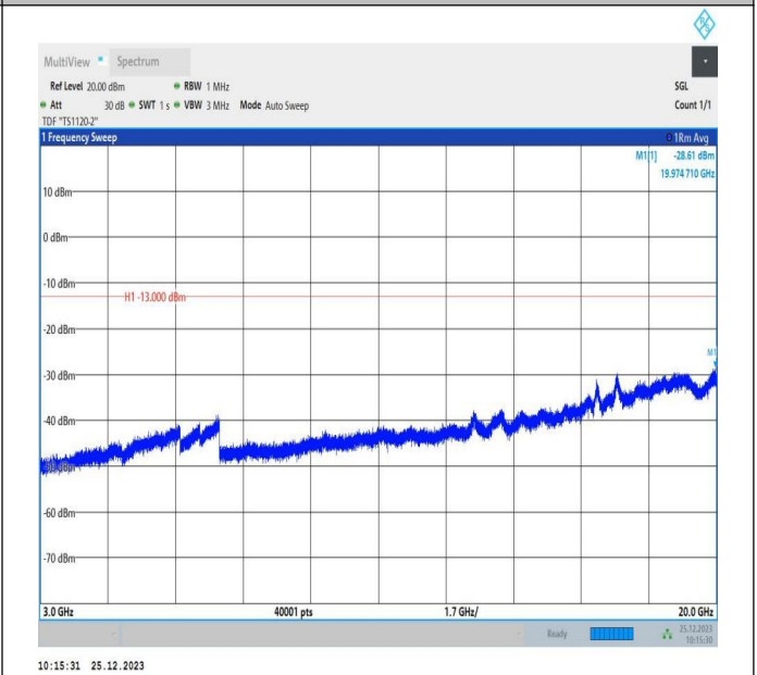
66-66-5MHz-10MHz-16QAM-16QAM-132000-132072-1RB#2 4-ORB#0-3000~20000MHz-PASS
