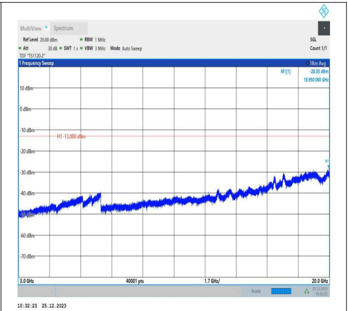
66-66-5MHz-10MHz-16QAM-16QAM-132550-132622-1RB#0-1RB#49-3000~20000MHz-PASS
