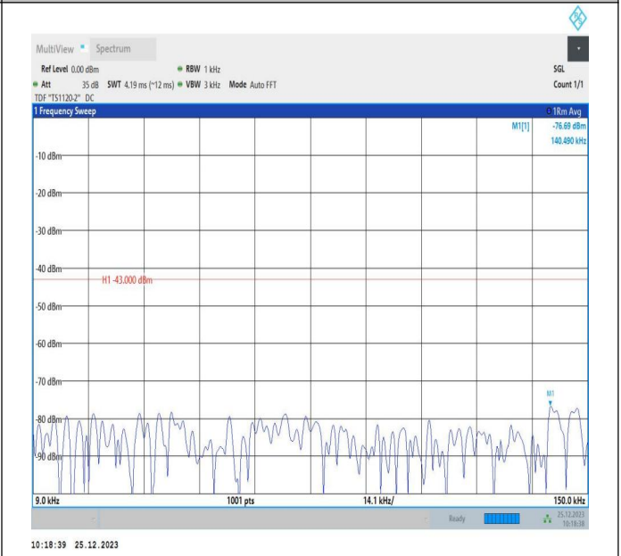
66-66-5MHz-10MHz-16QAM-16QAM-132000-132072-25RB#0-50RB#0-0.009~0.15MHz-PASS
