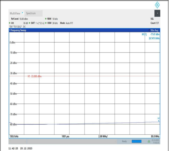
66-66-10MHz-5MHz-QPSK-QPSK-132022-132094-1RB#49-ORB#0-0.15~30MHz-PASS
