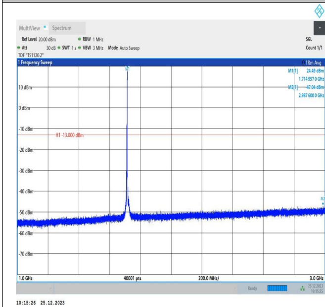
66-66-5MHz-10MHz-16QAM-16QAM-132000-132072-1RB#2 4-ORB#0-1000~3000MHz-PASS
