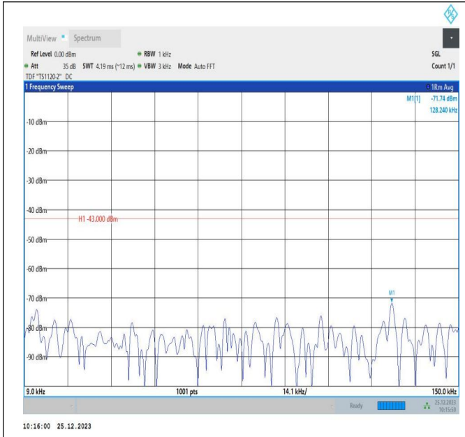
66-66-5MHz-10MHz-QPSK-QPSK-132000-132072-1RB#0-1 RB#49-0.009~0.15MHz-PASS
