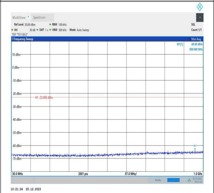
66-66-5MHz-10MHz-16QAM-16QAM-132375-132447-1RB#0-0ORB#0-30~1000MHz-PASS
