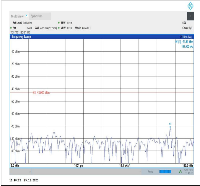
66-66-10MHz-5MHz-QPSK-QPSK-132022-132094-1RB#0-0 RB#0-0.009~0.15MHz-PASS
