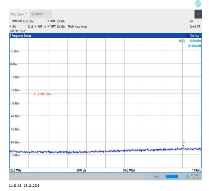
66-66-10MHz-5MHz-16QAM-16QAM-132022-132094-1RB#0-0RB#0-30~1000MHz-PASS
