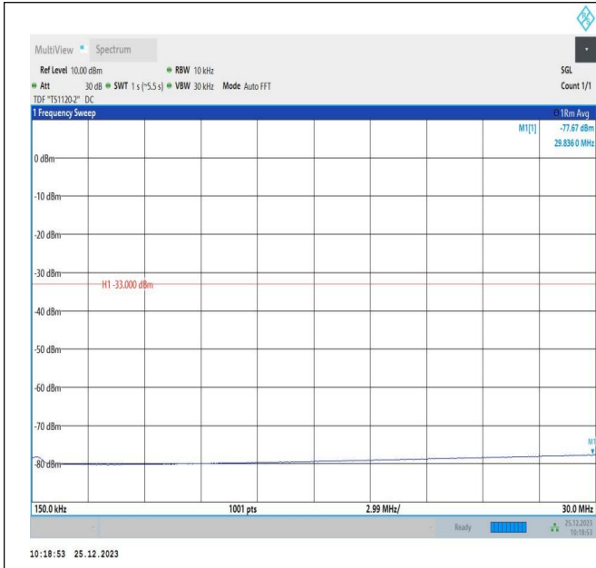
66-66-5MHz-10MHz-16QAM-16QAM-132000-132072-25RB# 0-50RB#0-0.15~30MHz-PASS
