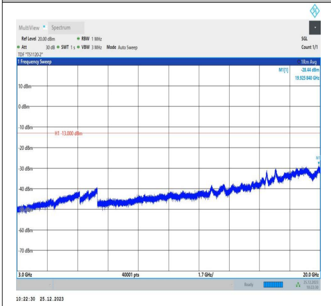
66-66-5MHz-10MHz-QPSK-QPSK-132375-132447-1RB#24-ORB#0-3000~20000MHz-PASS
