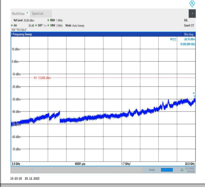
66-66-5MHz-10MHz-16QAM-16QAM-132375-132447-1RB#2 4-ORB#0-3000~20000MHz-PASS
