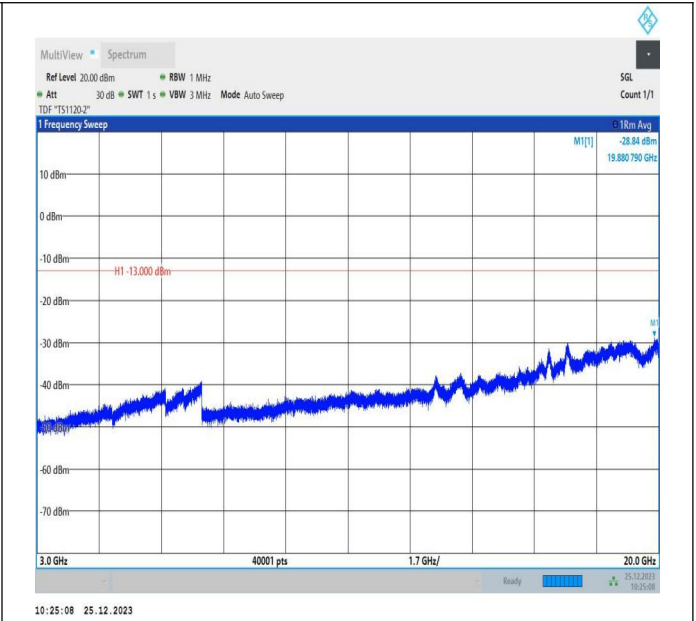
66-66-5MHz-10MHz-16QAM-16QAM-132375-132447-1RB#0-1RB#49-3000~20000MHz-PASS
