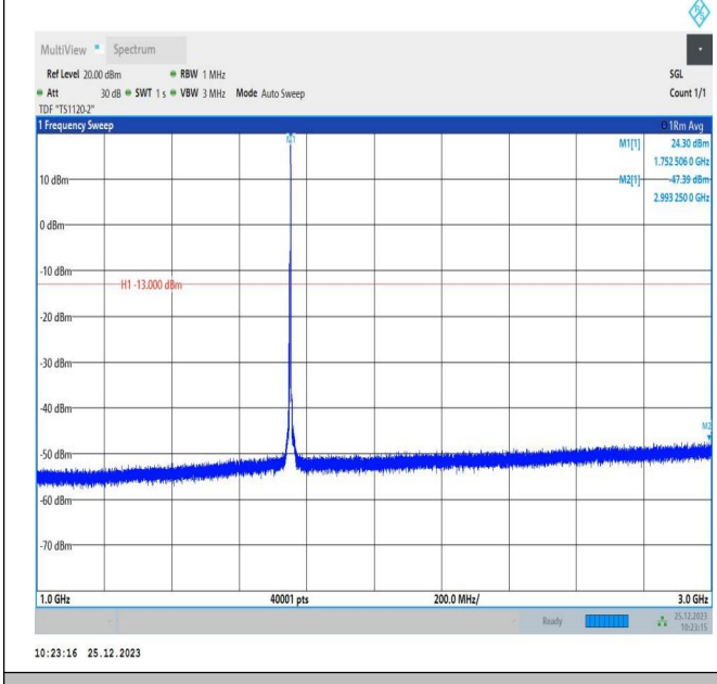
66-66-5MHz-10MHz-16QAM-16QAM-132375-132447-1RB#2 4-ORB#0-1000~3000MHz-PASS
