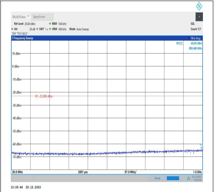
66-66-5MHz-10MHz-16QAM-16QAM-132375-132447-25RB# 0-50RB#0-30~1000MHz-PASS
