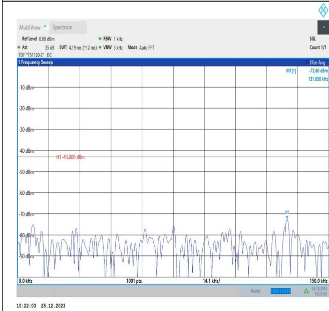
66-66-5MHz-10MHz-QPSK-QPSK-132375-132447-1RB#24-ORB#0-0.009~0.15MHz-PASS
