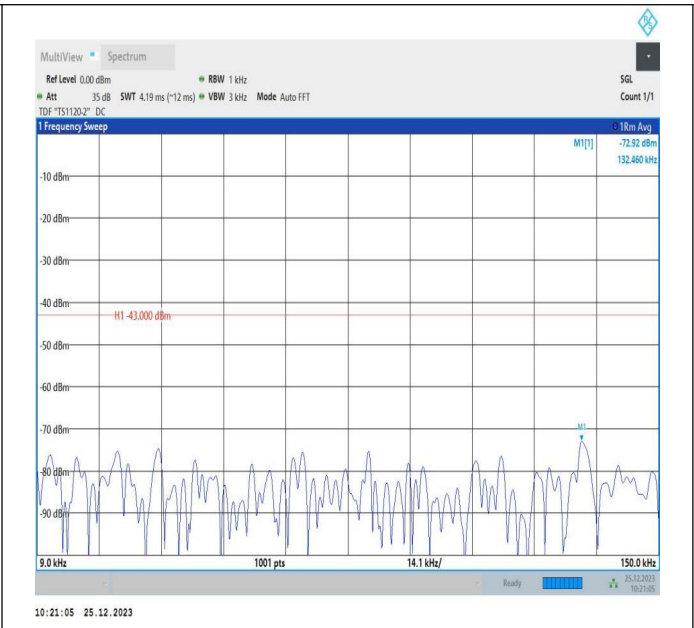
66-66-5MHz-10MHz-16QAM-16QAM-132375-132447-1RB#0-0ORB#0-0.009~0.15MHz-PASS
