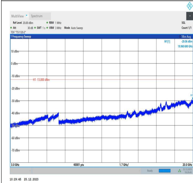
66-66-5MHz-10MHz-QPSK-QPSK-132550-132622-1RB#24-ORB#0-3000~20000MHz-PASS
