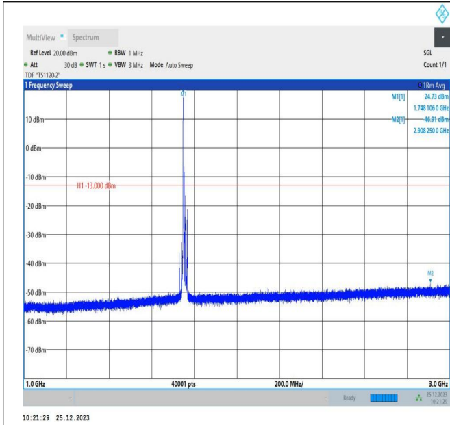
66-66-5MHz-10MHz-16QAM-16QAM-132375-132447-1RB#0-ORB#0-1000~3000MHz-PASS
