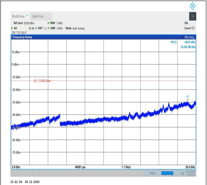
66-66-5MHz-10MHz-16QAM-16QAM-132375-132447-1RB#0-ORB#0-3000~20000MHz-PASS
