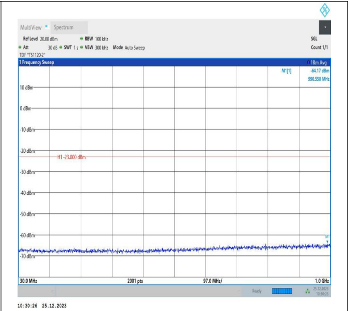
66-66-5MHz-10MHz-16QAM-16QAM-132550-132622-1RB#2 4-ORB#0-30~1000MHz-PASS
