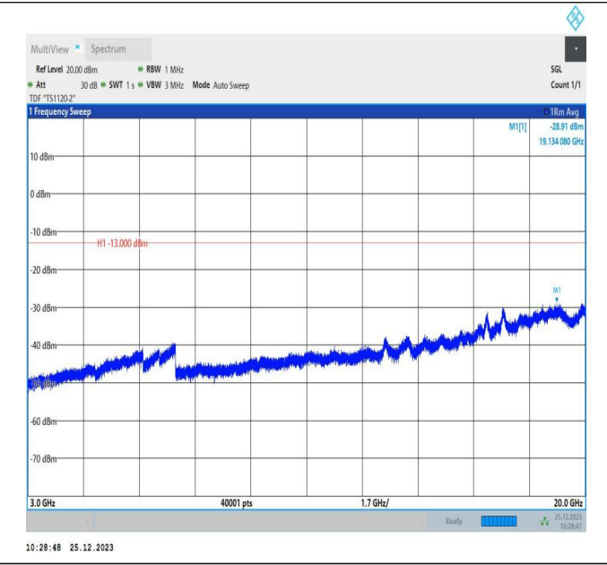
66-66-5MHz-10MHz-16QAM-16QAM-132550-132622-1RB#0-ORB#0-3000~20000MHz-PASS
