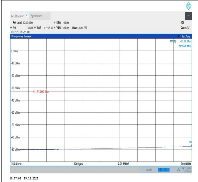
66-66-5MHz-10MHz-16QAM-16QAM-132000-132072-1RB#0 -1RB#49-0.15~30MHz-PASS
