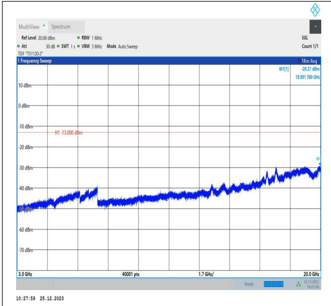
66-66-5MHz-10MHz-QPSK-QPSK-132550-132622-1RB#0-0RB#0-3000~20000MHz-PASS
