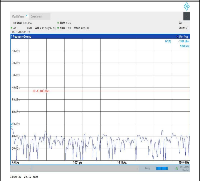
66-66-5MHz-10MHz-16QAM-16QAM-132375-132447-1RB#24-ORB#0-0.009~0.15MHz-PASS
