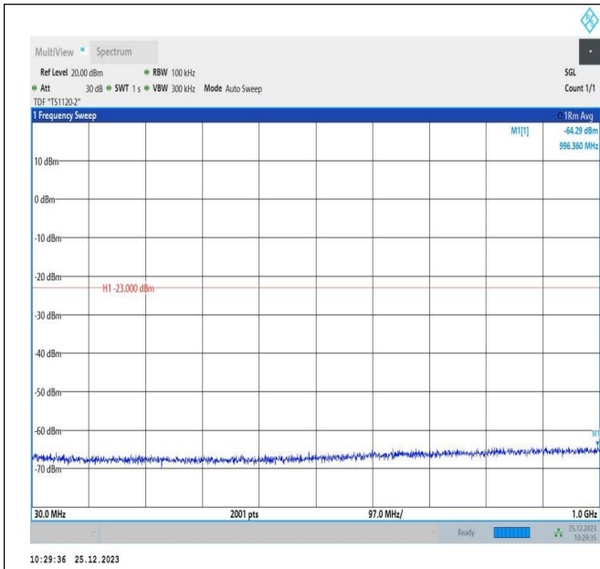
66-66-5MHz-10MHz-QPSK-QPSK-132550-132622-1RB#24-ORB#0-30~1000MHz-PASS
