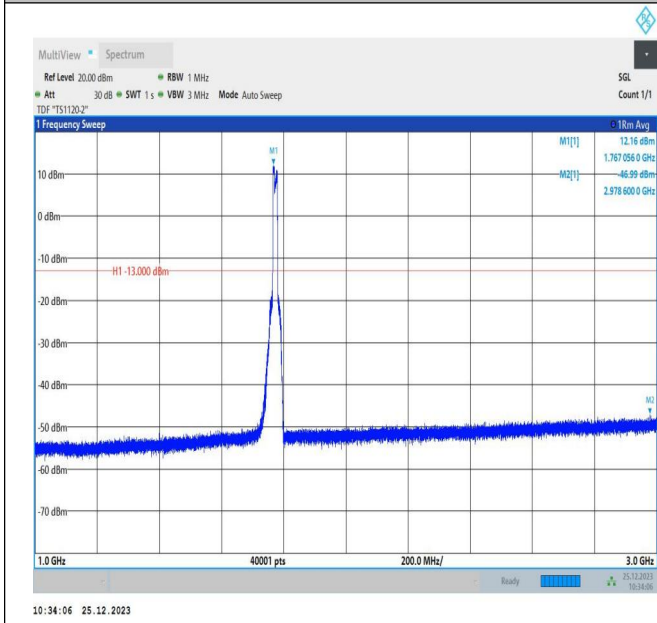
66-66-5MHz-10MHz-16QAM-16QAM-132550-132622-25RB# 0-50RB#0-1000~3000MHz-PASS
