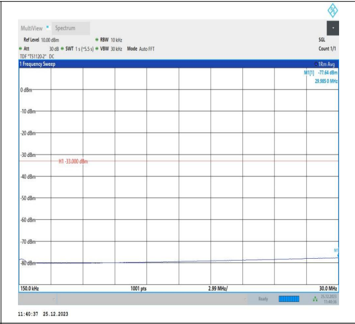
66-66-10MHz-5MHz-QPSK-QPSK-132022-132094-1RB#0-0R B#0-0.15~30MHz-PASS
