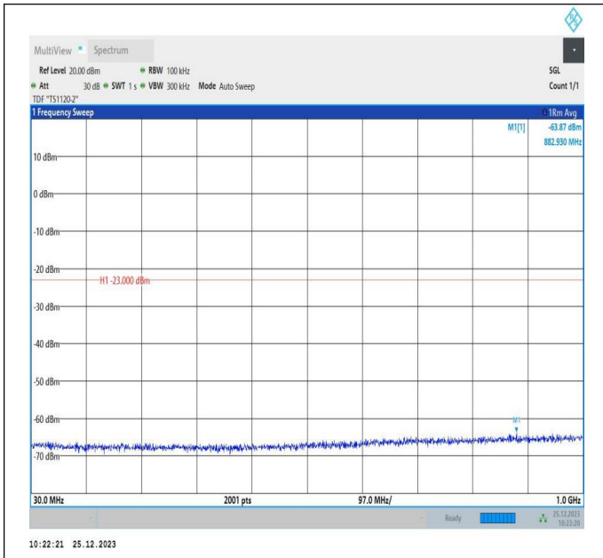
66-66-5MHz-10MHz-QPSK-QPSK-132375-132447-1RB#24-ORB#0-30~1000MHz-PASS
