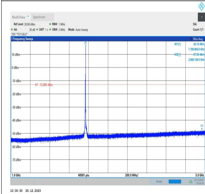
66-66-5MHz-10MHz-16QAM-16QAM-132550-132622-1RB#2 4-ORB#0-1000~3000MHz-PASS
