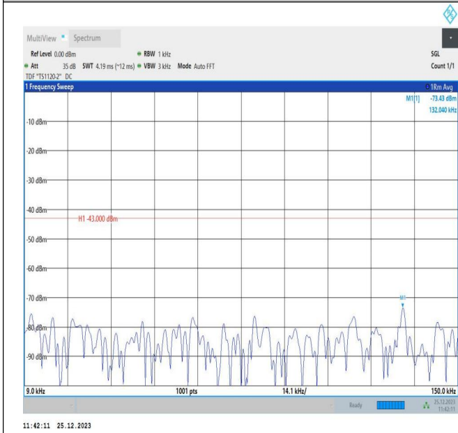
66-66-10MHz-5MHz-QPSK-QPSK-132022-132094-1RB#49-ORB#0-0.009~0.15MHz-PASS
