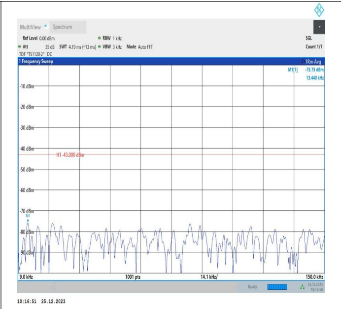
66-66-5MHz-10MHz-16QAM-16QAM-132000-132072-1RB#0- 1RB#49-0.009~0.15MHz-PASS
