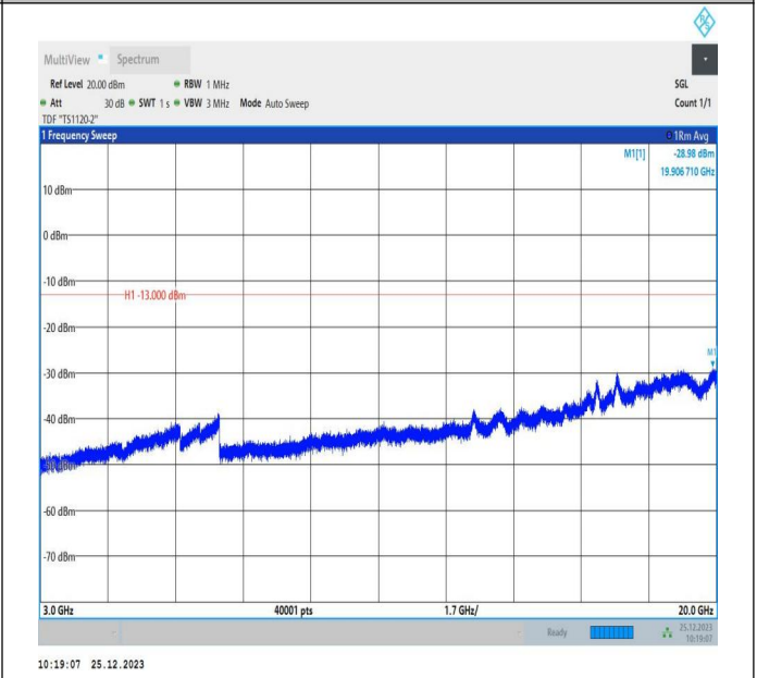
66-66-5MHz-10MHz-16QAM-16QAM-132000-132072-25RB# 0-50RB#0-3000~20000MHz-PASS
