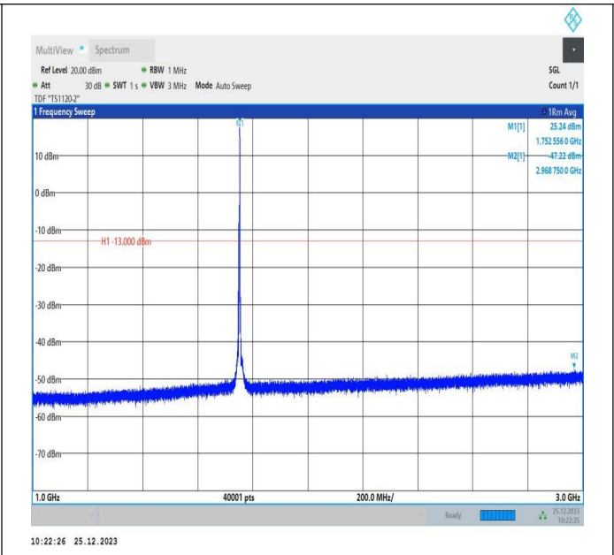
66-66-5MHz-10MHz-QPSK-QPSK-132375-132447-1RB#24-ORB#0-1000~3000MHz-PASS
