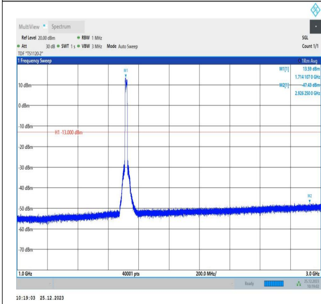
66-66-5MHz-10MHz-16QAM-16QAM-132000-132072-25RB# 0-50RB#0-1000~3000MHz-PASS
