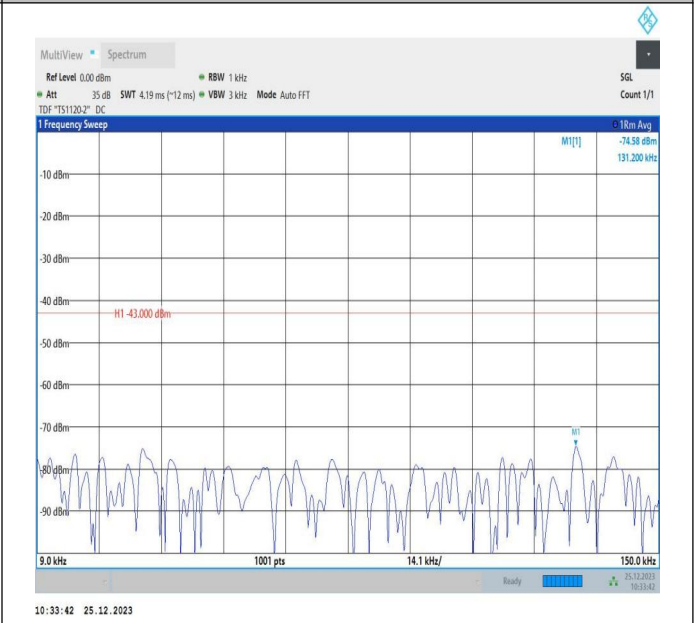
66-66-5MHz-10MHz-16QAM-16QAM-132550-132622-25RB#0-50RB#0-0.009~0.15MHz-PASS
