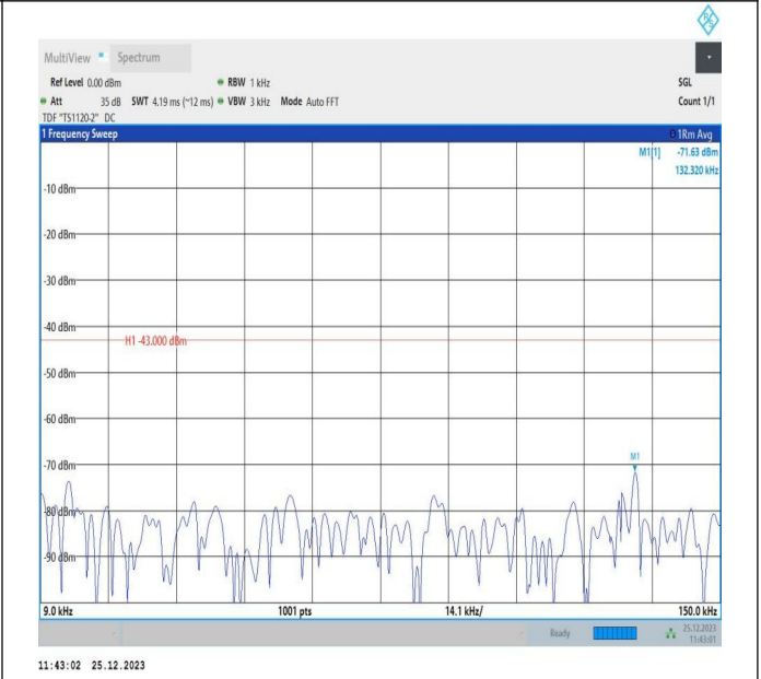
66-66-10MHz-5MHz-16QAM-16QAM-132022-132094-1RB#49-0RB#0-0.009~0.15MHz-PASS
