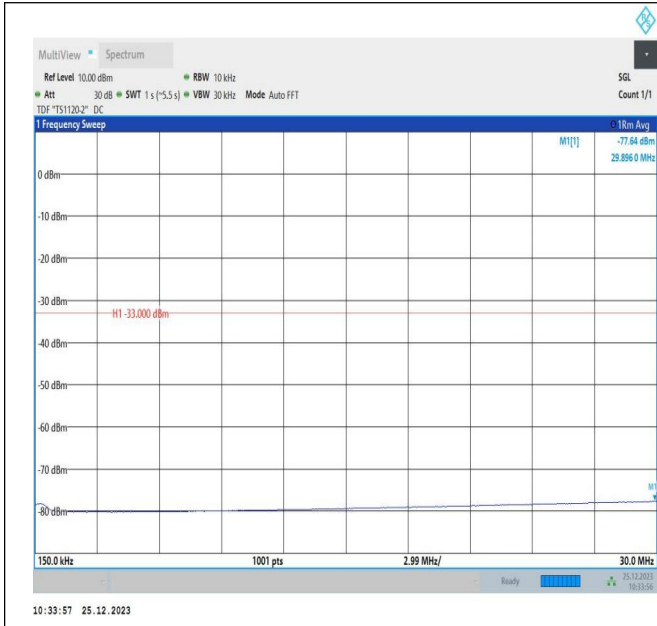
66-66-5MHz-10MHz-16QAM-16QAM-132550-132622-25RB# 0-50RB#0-0.15~30MHz-PASS
