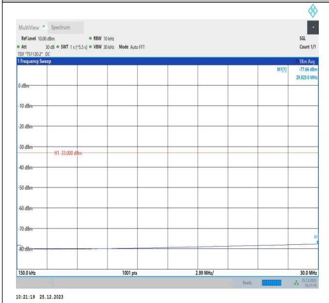
66-66-5MHz-10MHz-16QAM-16QAM-132375-132447-1RB#0-0ORB#0-0.15~30MHz-PASS
