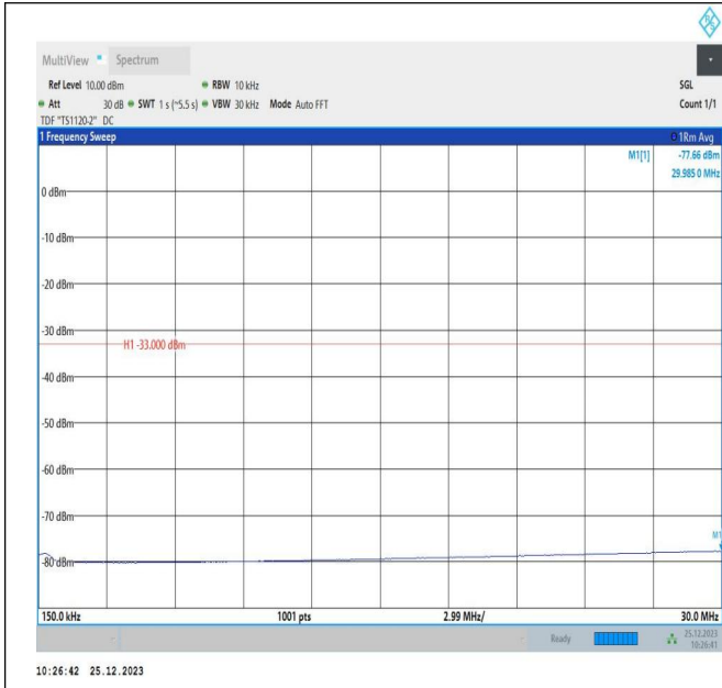
66-66-5MHz-10MHz-16QAM-16QAM-132375-132447-25RB# 0-50RB#0-0.15~30MHz-PASS
