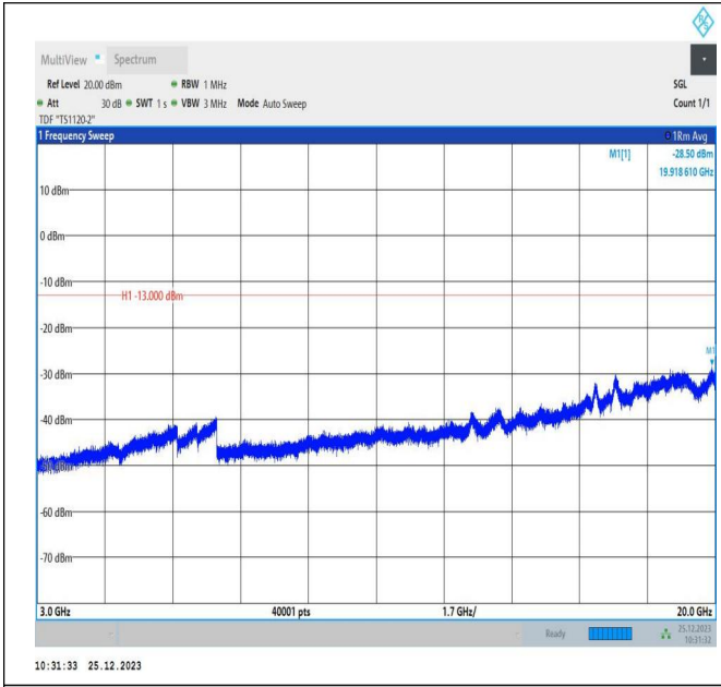
66-66-5MHz-10MHz-QPSK-QPSK-132550-132622-1RB#0-1 RB#49-3000~20000MHz-PASS
