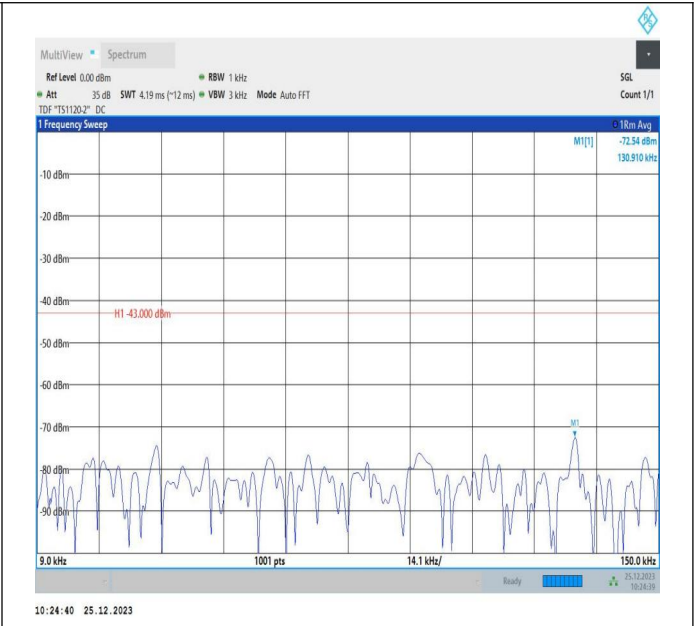
66-66-5MHz-10MHz-16QAM-16QAM-132375-132447-1RB#0- 1RB#49-0.009~0.15MHz-PASS
