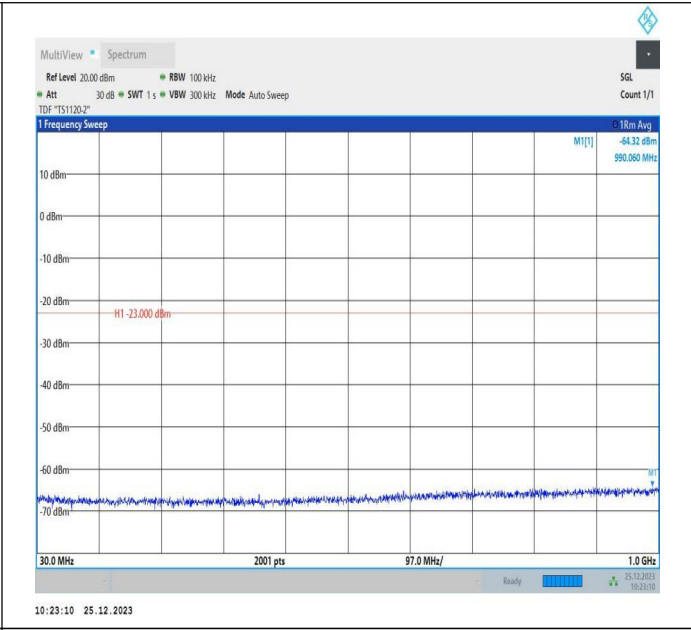
66-66-5MHz-10MHz-16QAM-16QAM-132375-132447-1RB#2 4-ORB#0-30~1000MHz-PASS
