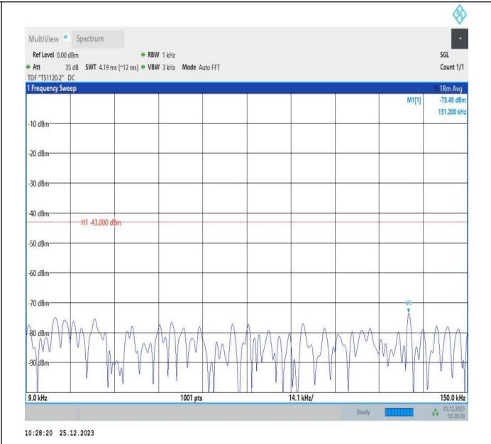
66-66-5MHz-10MHz-16QAM-16QAM-132550-132622-1RB#0-0ORB#0-0.009~0.15MHz-PASS
