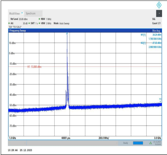
66-66-5MHz-10MHz-16QAM-16QAM-132550-132622-1RB#0-ORB#0-1000~3000MHz-PASS
