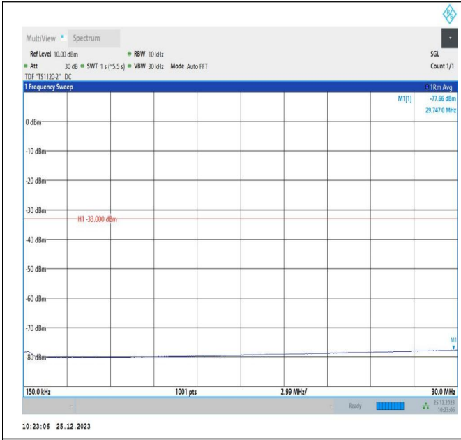
66-66-5MHz-10MHz-16QAM-16QAM-132375-132447-1RB#2 4-ORB#0-0.15~30MHz-PASS
