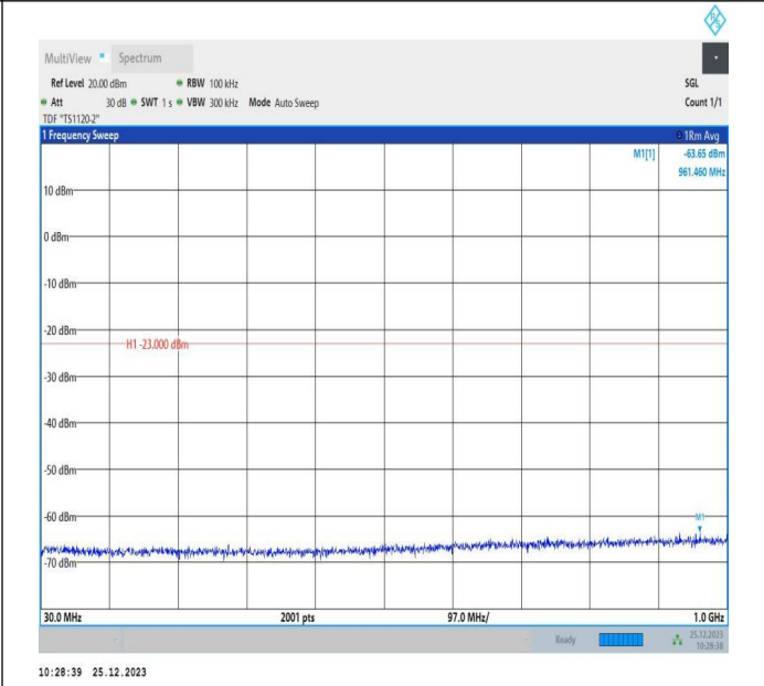
66-66-5MHz-10MHz-16QAM-16QAM-132550-132622-1RB#0-0ORB#0-30~1000MHz-PASS
