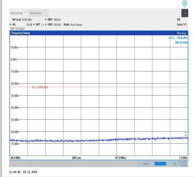
66-66-10MHz-5MHz-QPSK-QPSK-132022-132094-1RB#0-0 RB#0-30~1000MHz-PASS
