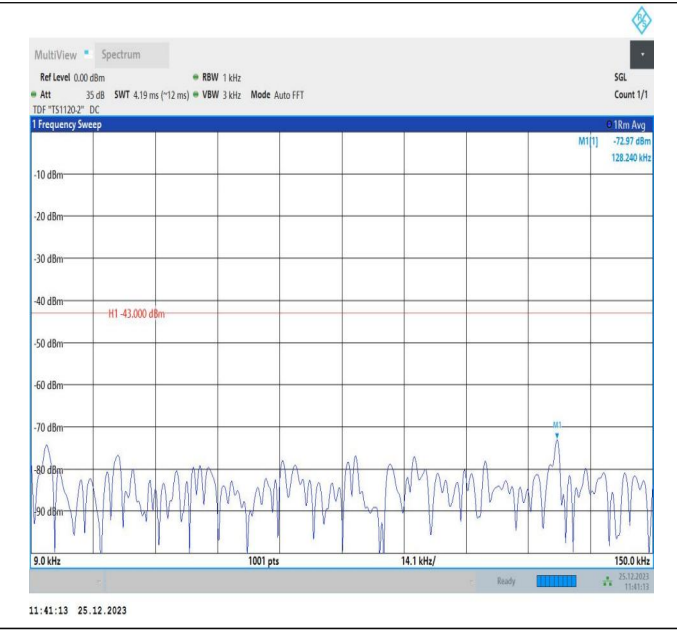
66-66-10MHz-5MHz-16QAM-16QAM-132022-132094-1RB#0-0RB#0-0.009~0.15MHz-PASS
