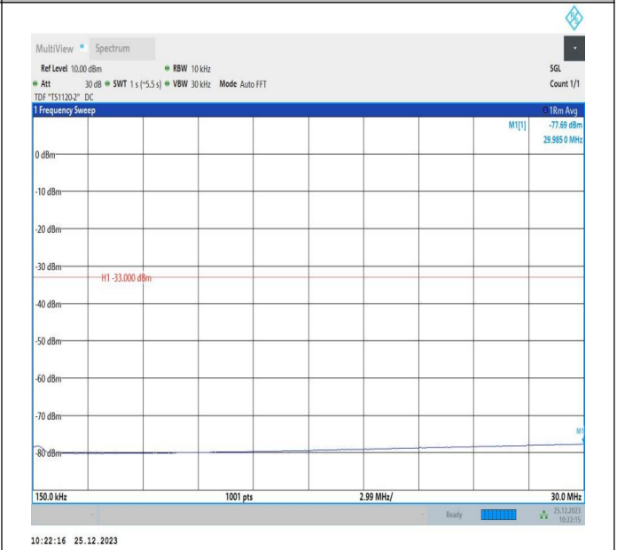
66-66-5MHz-10MHz-QPSK-QPSK-132375-132447-1RB#24-ORB#0-0.15~30MHz-PASS
