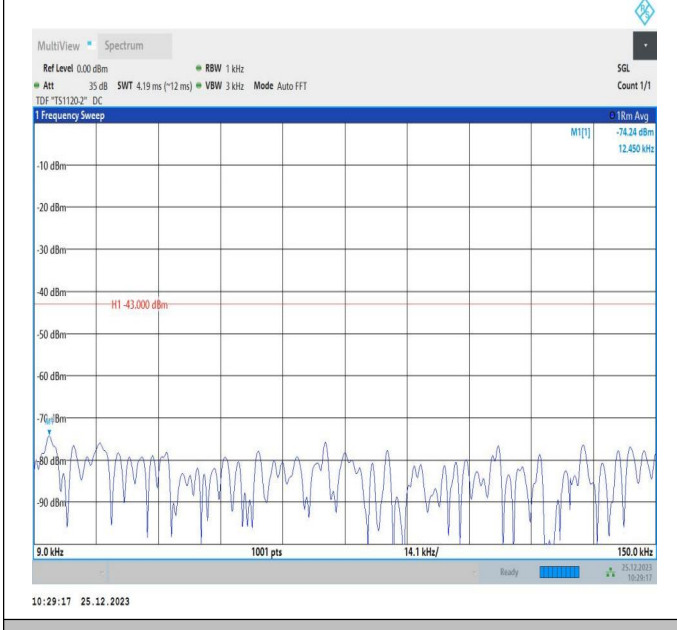
66-66-5MHz-10MHz-QPSK-QPSK-132550-132622-1RB#24-ORB#0-0.009~0.15MHz-PASS
