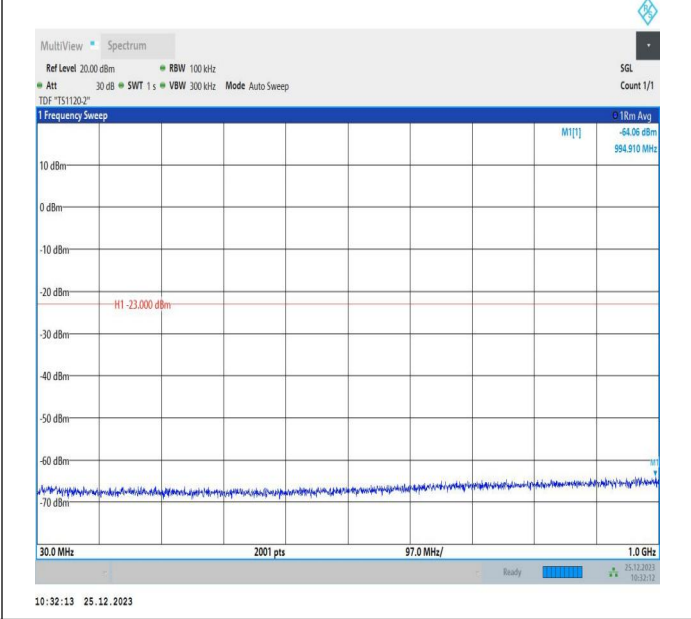
66-66-5MHz-10MHz-16QAM-16QAM-132550-132622-1RB#0- 1RB#49-30~1000MHz-PASS
