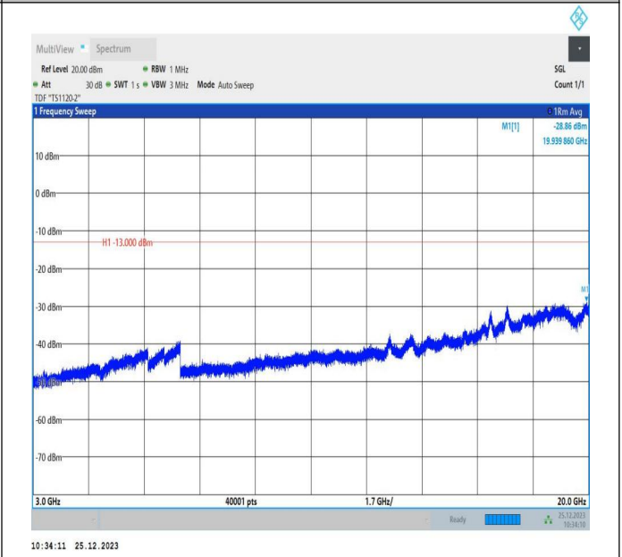
66-66-5MHz-10MHz-16QAM-16QAM-132550-132622-25RB# 0-50RB#0-3000~20000MHz-PASS
