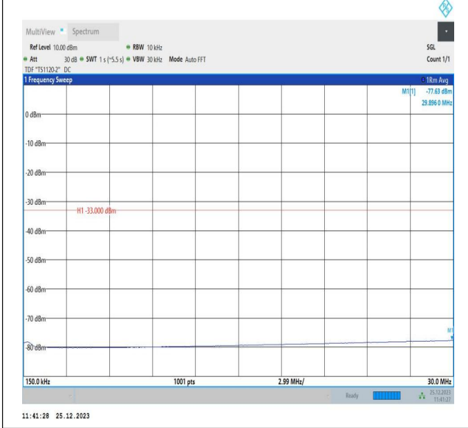
66-66-10MHz-5MHz-16QAM-16QAM-132022-132094-1RB#0-0RB#0-0.15~30MHz-PASS
