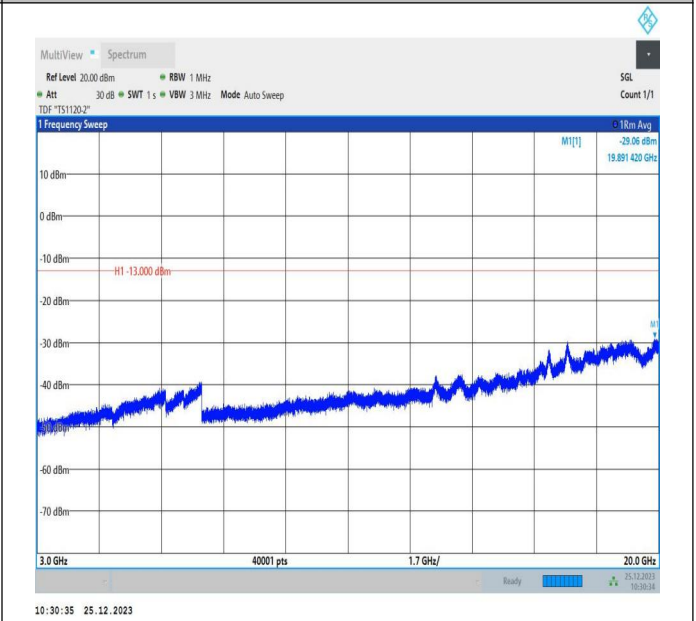
66-66-5MHz-10MHz-16QAM-16QAM-132550-132622-1RB#2 4-ORB#0-3000~20000MHz-PASS
