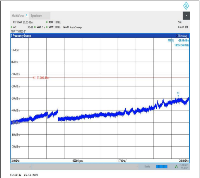
66-66-10MHz-5MHz-16QAM-16QAM-132022-132094-1RB#0-ORB#0-3000~20000MHz-PASS
