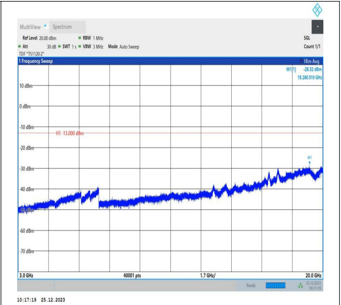
66-66-5MHz-10MHz-16QAM-16QAM-132000-132072-1RB#0-1RB#49-3000~20000MHz-PASS
