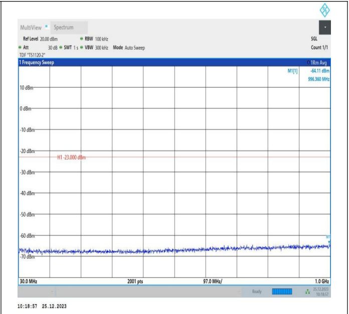
66-66-5MHz-10MHz-16QAM-16QAM-132000-132072-25RB# 0-50RB#0-30~1000MHz-PASS
