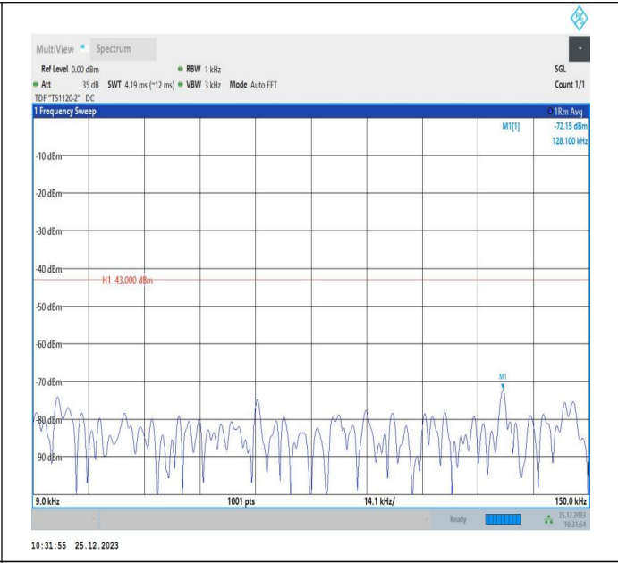
66-66-5MHz-10MHz-16QAM-16QAM-132550-132622-1RB#0- 1RB#49-0.009~0.15MHz-PASS
