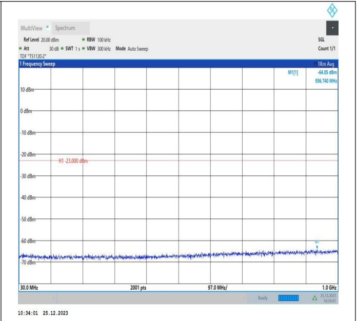
66-66-5MHz-10MHz-16QAM-16QAM-132550-132622-25RB# 0-50RB#0-30~1000MHz-PASS
