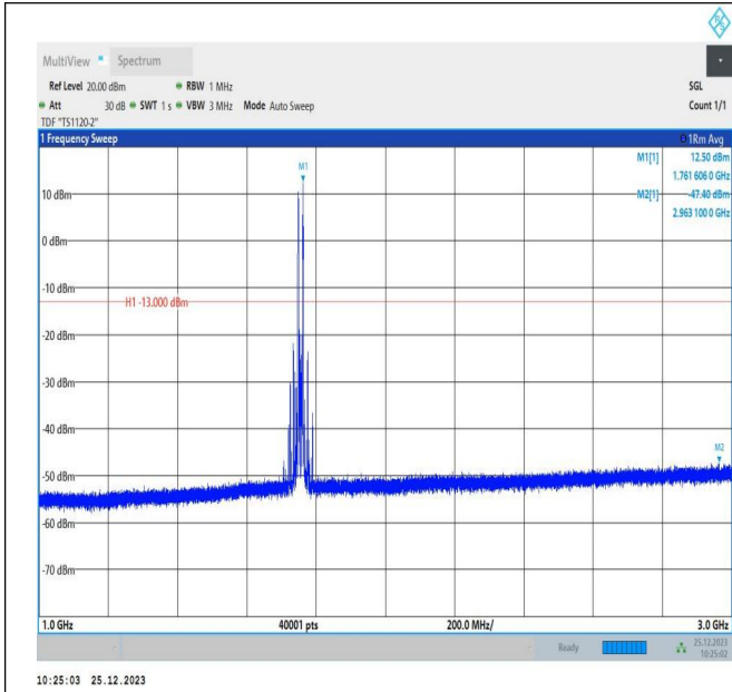
66-66-5MHz-10MHz-16QAM-16QAM-132375-132447-1RB#0-1RB#49-1000~3000MHz-PASS
