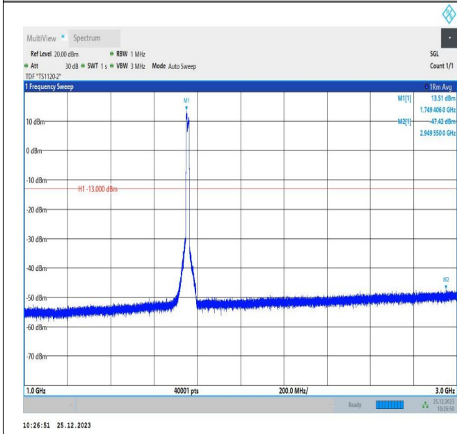
66-66-5MHz-10MHz-16QAM-16QAM-132375-132447-25RB# 0-50RB#0-1000~3000MHz-PASS
