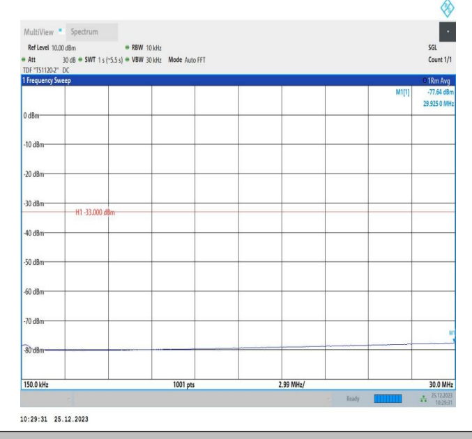
66-66-5MHz-10MHz-QPSK-QPSK-132550-132622-1RB#24-ORB#0-0.15~30MHz-PASS
