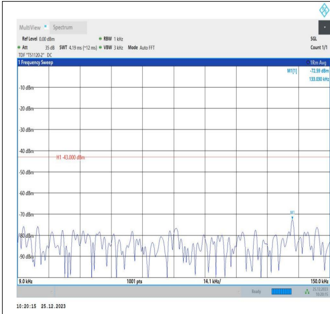
66-66-5MHz-10MHz-QPSK-QPSK-132375-132447-1RB#0-0 RB#0-0.009~0.15MHz-PASS
