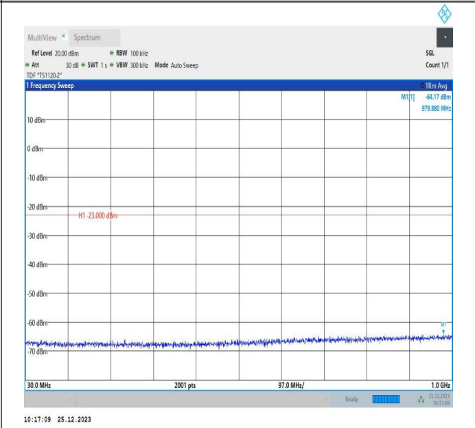
66-66-5MHz-10MHz-16QAM-16QAM-132000-132072-1RB#0- 1RB#49-30~1000MHz-PASS
