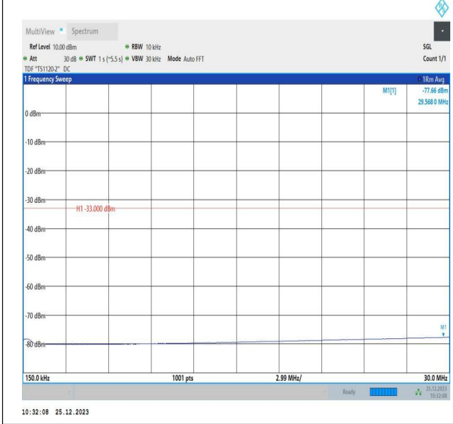
66-66-5MHz-10MHz-16QAM-16QAM-132550-132622-1RB#0 -1RB#49-0.15~30MHz-PASS
