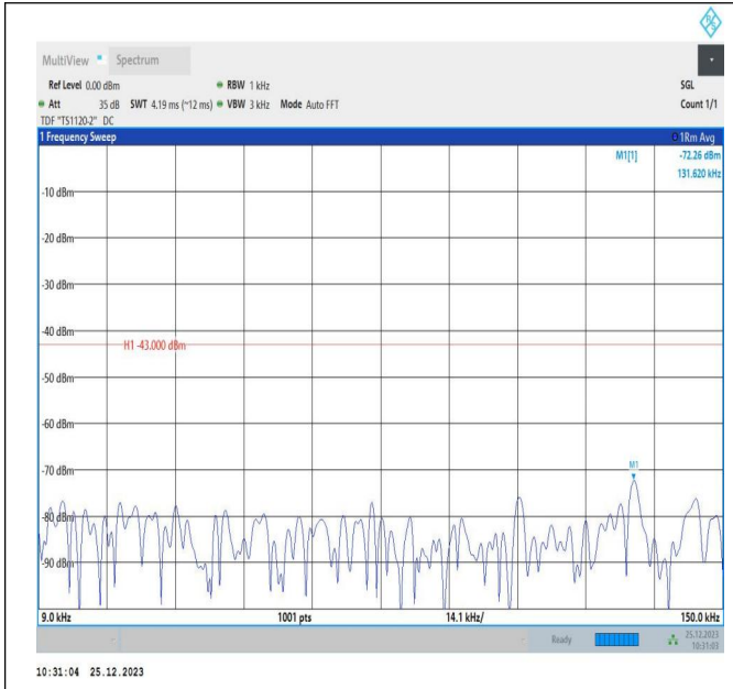
66-66-5MHz-10MHz-QPSK-QPSK-132550-132622-1RB#0-1 RB#49-0.009~0.15MHz-PASS
