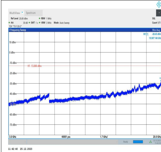
66-66-10MHz-5MHz-QPSK-QPSK-132022-132094-1RB#49-0RB#0-3000~20000MHz-PASS
