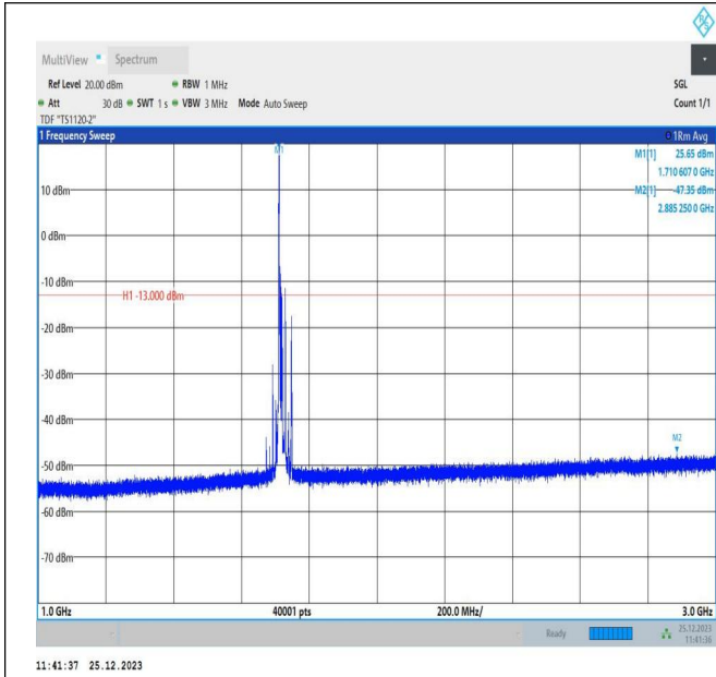
66-66-10MHz-5MHz-16QAM-16QAM-132022-132094-1RB#0-ORB#0-1000~3000MHz-PASS
