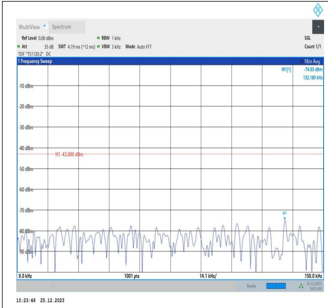
66-66-5MHz-10MHz-QPSK-QPSK-132375-132447-1RB#0-1 RB#49-0.009~0.15MHz-PASS
