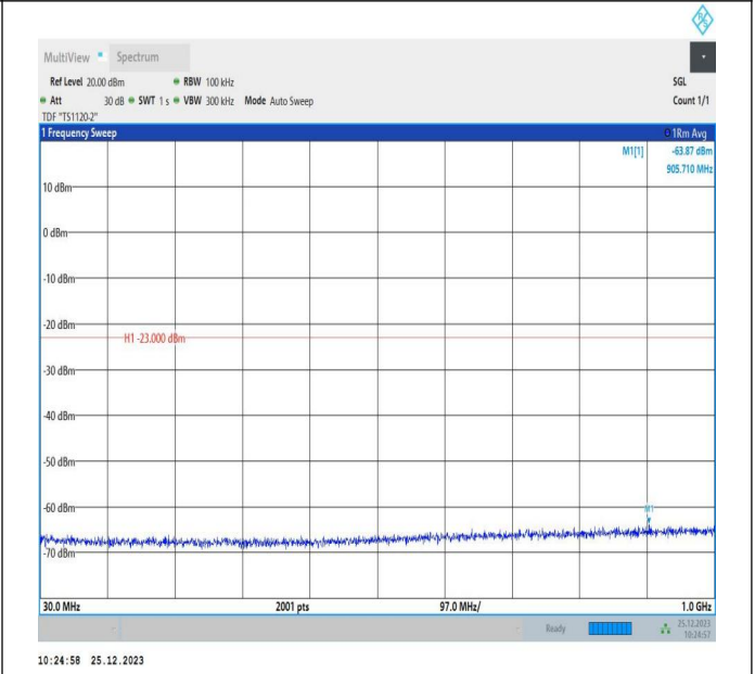
66-66-5MHz-10MHz-16QAM-16QAM-132375-132447-1RB#0- 1RB#49-30~1000MHz-PASS
