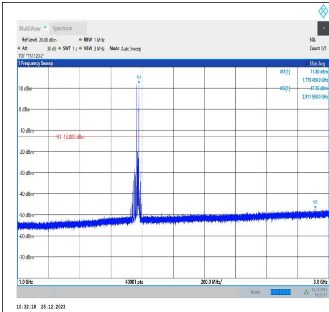
66-66-5MHz-10MHz-16QAM-16QAM-132550-132622-1RB#0-1RB#49-1000~3000MHz-PASS
