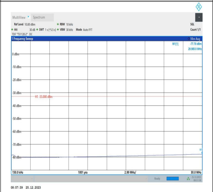
66-66-5MHz-5MHz-QPSK-QPSK-132599-132647-1RB#24-0RB#0-0.15~30MHz-PASS
