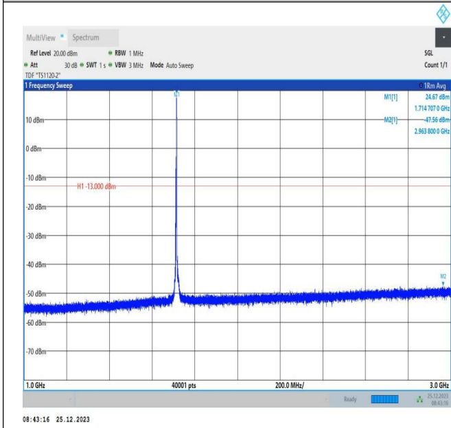
66-66-5MHz-5MHz-16QAM-16QAM-131997-132045-1RB#24 -ORB#0-1000~3000MHz-PASS
