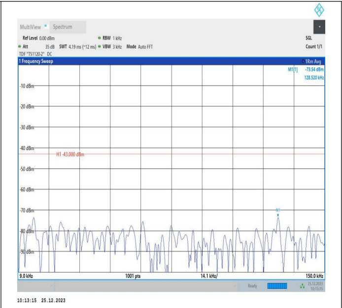
66-66-5MHz-10MHz-16QAM-16QAM-132000-132072-1RB#0-0ORB#0-0.009~0.15MHz-PASS
