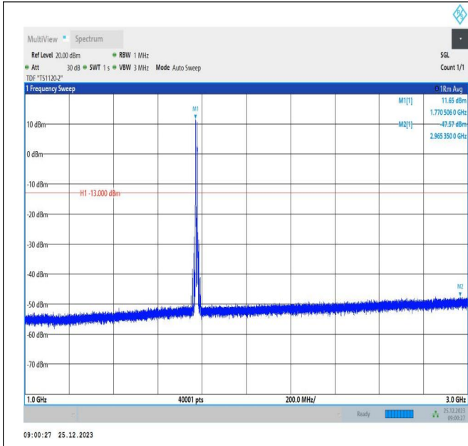
66-66-5MHz-5MHz-16QAM-16QAM-132599-132647-1RB#0-1RB#15-1000~3000MHz-PASS
