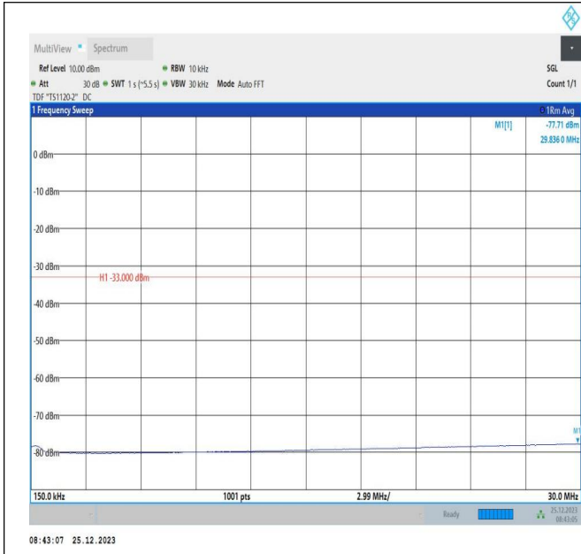
66-66-5MHz-5MHz-16QAM-16QAM-131997-132045-1RB#24 -ORB#0-0.15~30MHz-PASS
