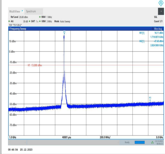
66-66-5MHz-5MHz-16QAM-16QAM-131997-132045-25RB#0-25RB#0-1000~3000MHz-PASS
