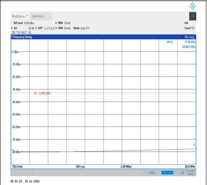
66-66-5MHz-5MHz-QPSK-QPSK-132398-132446-1RB#24-0RB#0-0.15~30MHz-PASS
