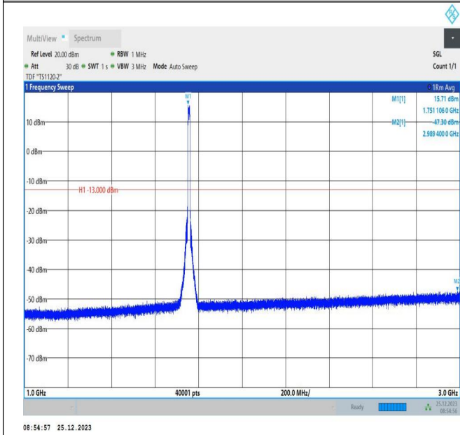
66-66-5MHz-5MHz-16QAM-16QAM-132398-132446-25RB#0-25RB#0-1000~3000MHz-PASS
