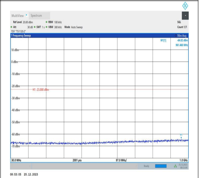
66-66-5MHz-5MHz-16QAM-16QAM-132398-132446-1RB#0-1 RB#15-30~1000MHz-PASS
