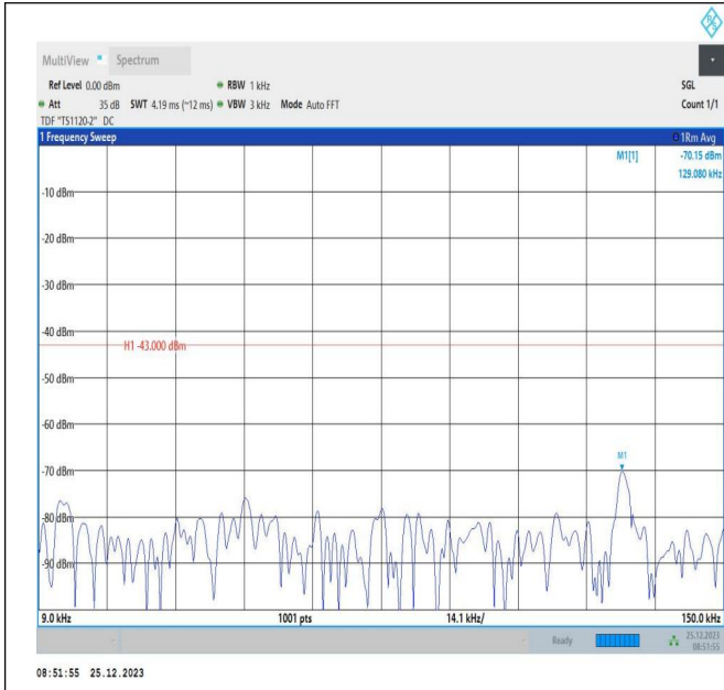
66-66-5MHz-5MHz-QPSK-QPSK-132398-132446-1RB#0-1R B#15-0.009~0.15MHz-PASS
