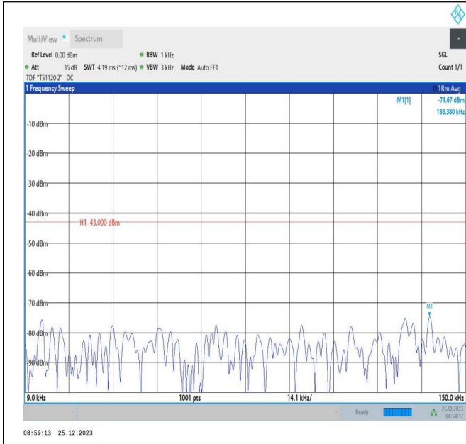
66-66-5MHz-5MHz-QPSK-QPSK-132599-132647-1RB#0-1R B#15-0.009~0.15MHz-PASS
