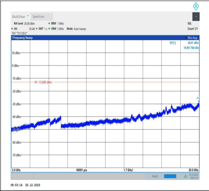
66-66-5MHz-5MHz-16QAM-16QAM-132398-132446-1RB#0-1RB#15-3000~20000MHz-PASS
