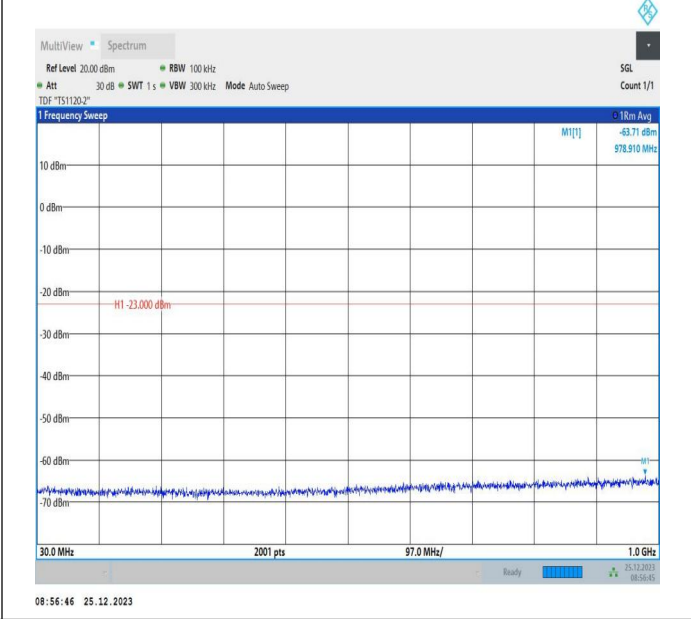
66-66-5MHz-5MHz-16QAM-16QAM-132599-132647-1RB#0-0 RB#0-30~1000MHz-PASS
