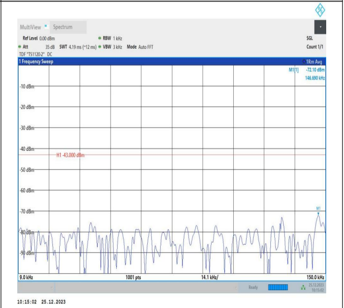
66-66-5MHz-10MHz-16QAM-16QAM-132000-132072-1RB#24-ORB#0-0.009~0.15MHz-PASS
