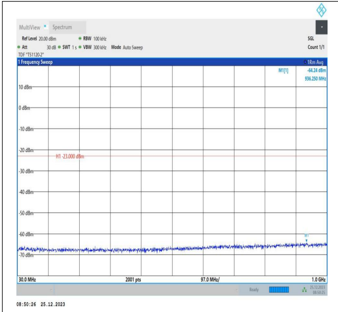
66-66-5MHz-5MHz-QPSK-QPSK-132398-132446-1RB#24-0 RB#0-30~1000MHz-PASS
