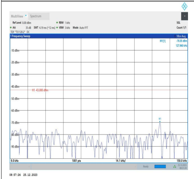
66-66-5MHz-5MHz-QPSK-QPSK-132599-132647-1RB#24-0RB#0-0.009~0.15MHz-PASS
