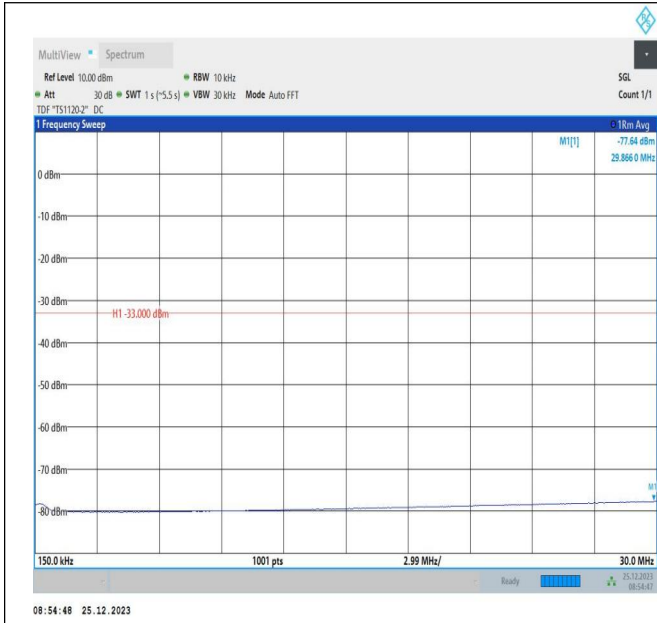
66-66-5MHz-5MHz-16QAM-16QAM-132398-132446-25RB#0-25RB#0-0.15~30MHz-PASS
