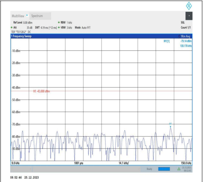
66-66-5MHz-5MHz-16QAM-16QAM-132398-132446-1RB#0-1 RB#15-0.009~0.15MHz-PASS
