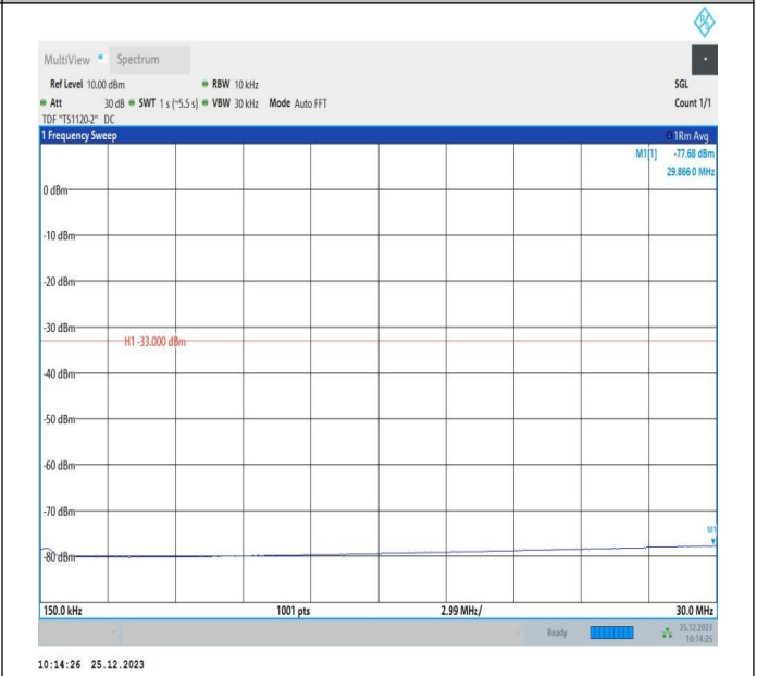
66-66-5MHz-10MHz-QPSK-QPSK-132000-132072-1RB#24-ORB#0-0.15~30MHz-PASS
