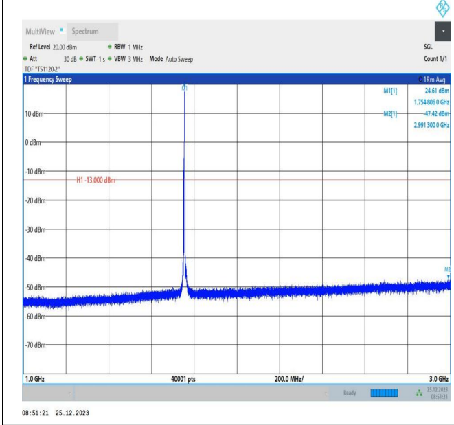
66-66-5MHz-5MHz-16QAM-16QAM-132398-132446-1RB#24-0RB#0-1000~3000MHz-PASS
