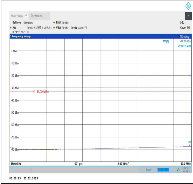
66-66-5MHz-5MHz-16QAM-16QAM-132599-132647-1RB#24-0RB#0-0.15~30MHz-PASS
