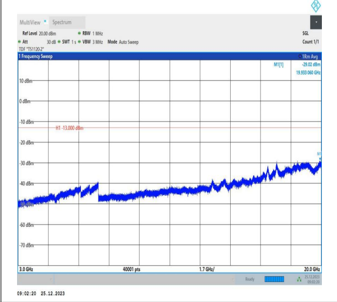
66-66-5MHz-5MHz-16QAM-16QAM-132599-132647-25RB#0-25RB#0-3000~20000MHz-PASS
