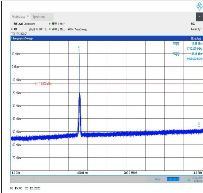
66-66-5MHz-5MHz-16QAM-16QAM-131997-132045-1RB#0-1RB#15-1000~3000MHz-PASS
