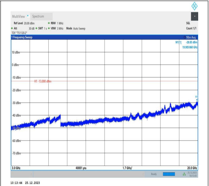
66-66-5MHz-10MHz-16QAM-16QAM-132000-132072-1RB#0-ORB#0-3000~20000MHz-PASS
