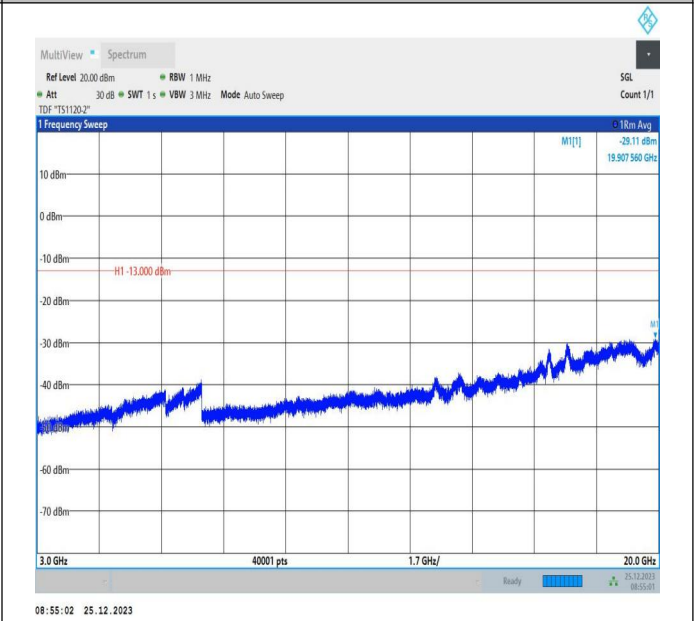
66-66-5MHz-5MHz-16QAM-16QAM-132398-132446-25RB#0-25RB#0-3000~20000MHz-PASS
