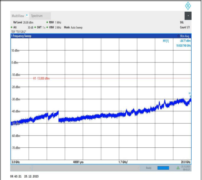
66-66-5MHz-5MHz-16QAM-16QAM-131997-132045-1RB#24- ORB#0-3000~20000MHz-PASS
