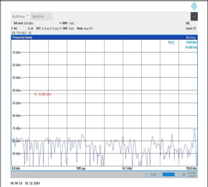
66-66-5MHz-5MHz-16QAM-16QAM-132599-132647-1RB#24-0 RB#0-0.009~0.15MHz-PASS
