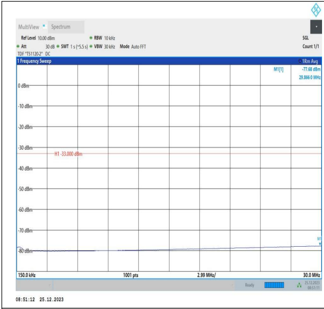
66-66-5MHz-5MHz-16QAM-16QAM-132398-132446-1RB#24-0RB#0-0.15~30MHz-PASS
