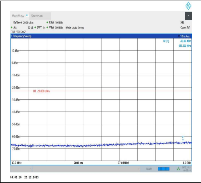
66-66-5MHz-5MHz-16QAM-16QAM-132599-132647-25RB#0-25RB#0-30~1000MHz-PASS
