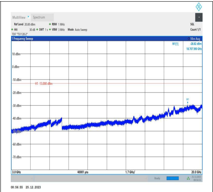
66-66-5MHz-5MHz-16QAM-16QAM-132599-132647-1RB#0-0RB#0-3000~20000MHz-PASS
