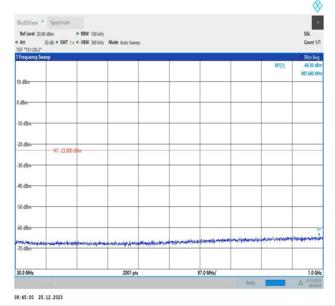
66-66-5MHz-5MHz-16QAM-16QAM-131997-132045-1RB#0-1 RB#15-30~1000MHz-PASS
