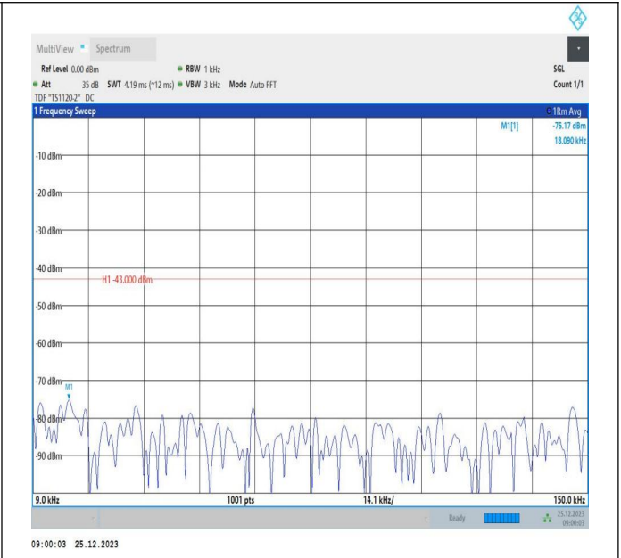
66-66-5MHz-5MHz-16QAM-16QAM-132599-132647-1RB#0-1 RB#15-0.009~0.15MHz-PASS
