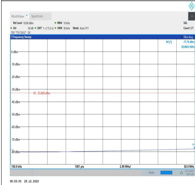
66-66-5MHz-5MHz-16QAM-16QAM-132398-132446-1RB#0-1 1RB#15-0.15~30MHz-PASS
