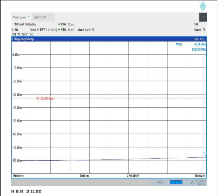
66-66-5MHz-5MHz-QPSK-QPSK-131997-132045-25RB#0-25RB#0-0.15~30MHz-PASS
