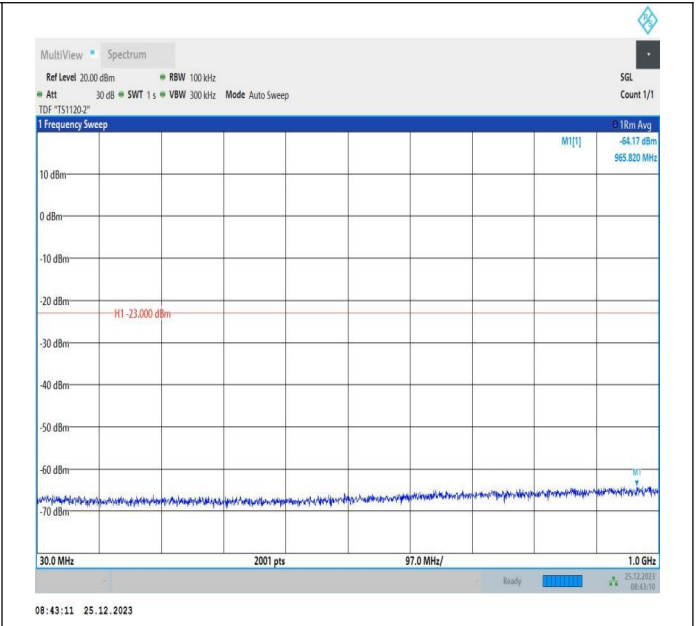
66-66-5MHz-5MHz-16QAM-16QAM-131997-132045-1RB#24- ORB#0-30~1000MHz-PASS
