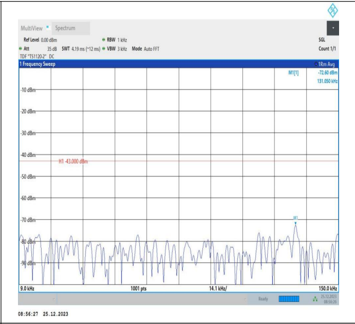
66-66-5MHz-5MHz-16QAM-16QAM-132599-132647-1RB#0-0 RB#0-0.009~0.15MHz-PASS
