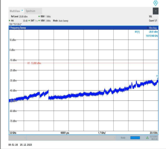
66-66-5MHz-5MHz-16QAM-16QAM-132398-132446-1RB#24-0RB#0-3000~20000MHz-PASS
