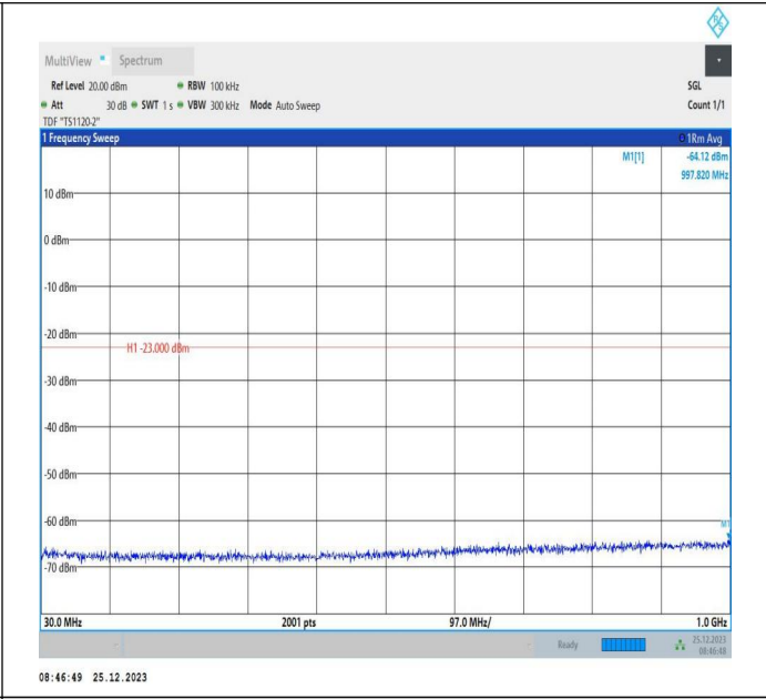
66-66-5MHz-5MHz-16QAM-16QAM-131997-132045-25RB#0-25RB#0-30~1000MHz-PASS
