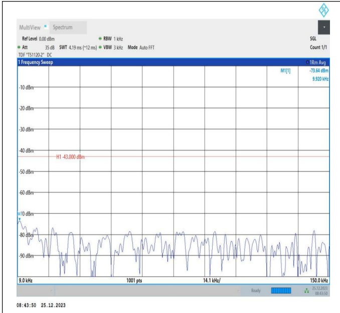
66-66-5MHz-5MHz-QPSK-QPSK-131997-132045-1RB#0-1R B#15-0.009~0.15MHz-PASS
