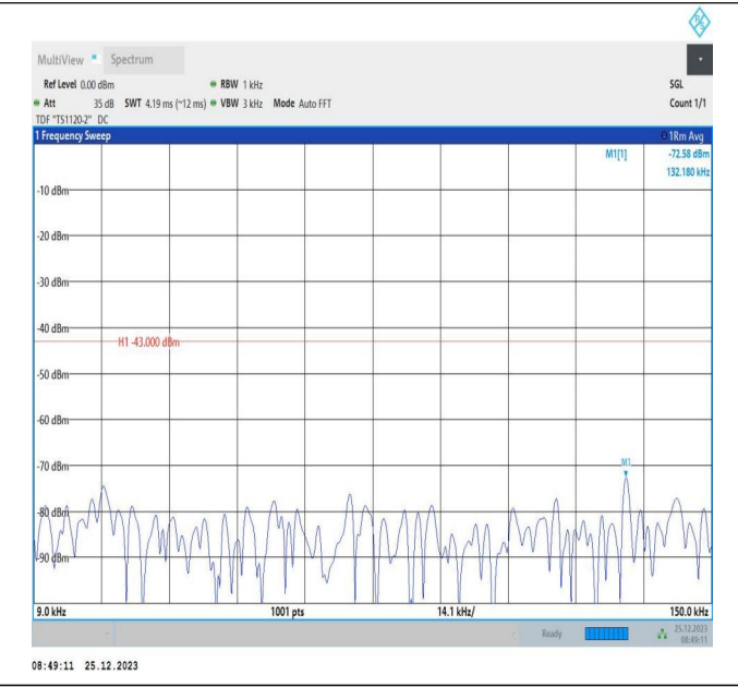
66-66-5MHz-5MHz-16QAM-16QAM-132398-132446-1RB#0-0 RB#0-0.009~0.15MHz-PASS
