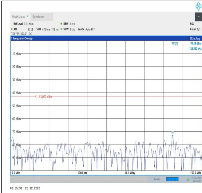
66-66-5MHz-5MHz-QPSK-QPSK-132599-132647-1RB#0-0R B#0-0.009~0.15MHz-PASS
