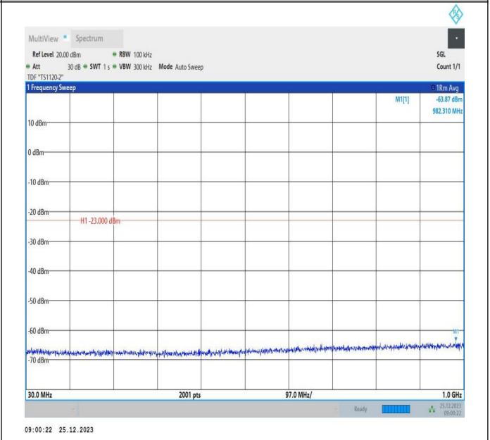
66-66-5MHz-5MHz-16QAM-16QAM-132599-132647-1RB#0-1 RB#15-30~1000MHz-PASS
