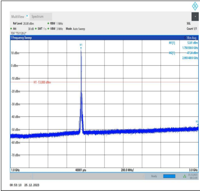
66-66-5MHz-5MHz-16QAM-16QAM-132398-132446-1RB#0-1RB#15-1000~3000MHz-PASS
