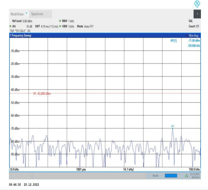
66-66-5MHz-5MHz-16QAM-16QAM-131997-132045-25RB#0- 25RB#0-0.009~0.15MHz-PASS
