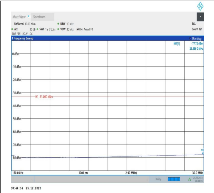
66-66-5MHz-5MHz-QPSK-QPSK-131997-132045-1RB#0-1R B#15-0.15~30MHz-PASS
