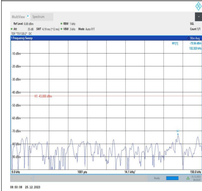
66-66-5MHz-5MHz-QPSK-QPSK-132398-132446-1RB#24-0RB#0-0.009~0.15MHz-PASS
