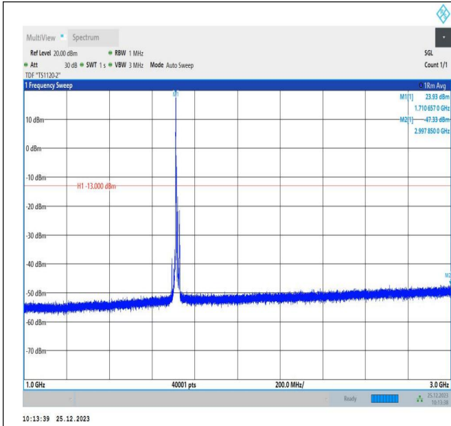
66-66-5MHz-10MHz-16QAM-16QAM-132000-132072-1RB#0-ORB#0-1000~3000MHz-PASS
