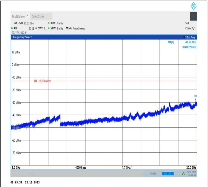
66-66-5MHz-5MHz-16QAM-16QAM-132398-132446-1RB#0-0RB#0-3000~20000MHz-PASS
