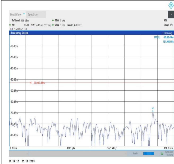
66-66-5MHz-10MHz-QPSK-QPSK-132000-132072-1RB#24-ORB#0-0.009~0.15MHz-PASS
