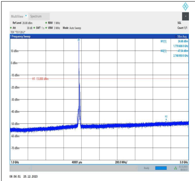
66-66-5MHz-5MHz-16QAM-16QAM-132599-132647-1RB#0-ORB#0-1000~3000MHz-PASS
