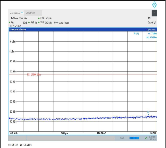
66-66-5MHz-5MHz-16QAM-16QAM-132398-132446-25RB#0-25RB#0-30~1000MHz-PASS
