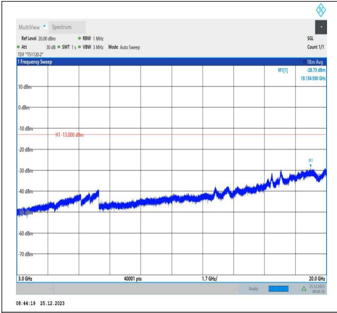
66-66-5MHz-5MHz-QPSK-QPSK-131997-132045-1RB#0-1R B#15-3000~20000MHz-PASS
