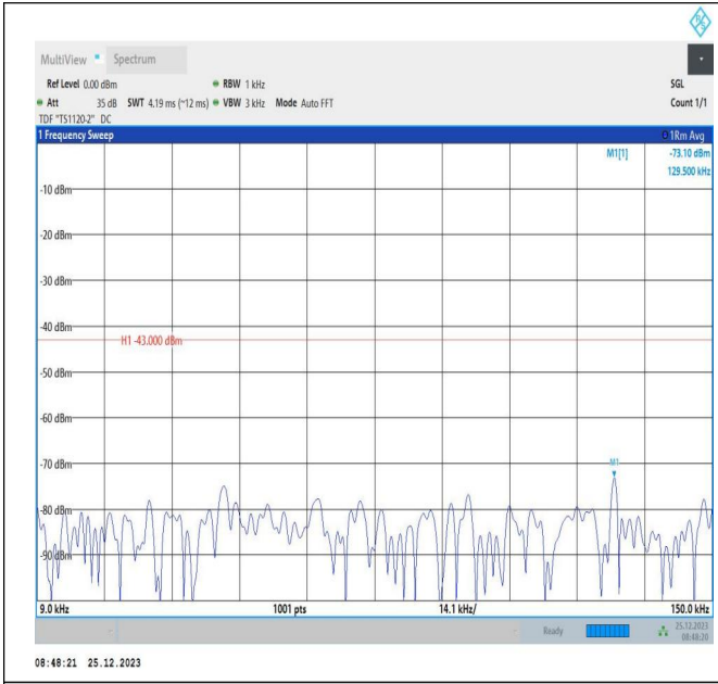
66-66-5MHz-5MHz-QPSK-QPSK-132398-132446-1RB#0-0R B#0-0.009~0.15MHz-PASS
