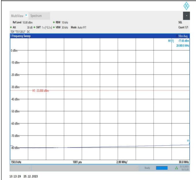
66-66-5MHz-10MHz-16QAM-16QAM-132000-132072-1RB#0-0ORB#0-0.15~30MHz-PASS
