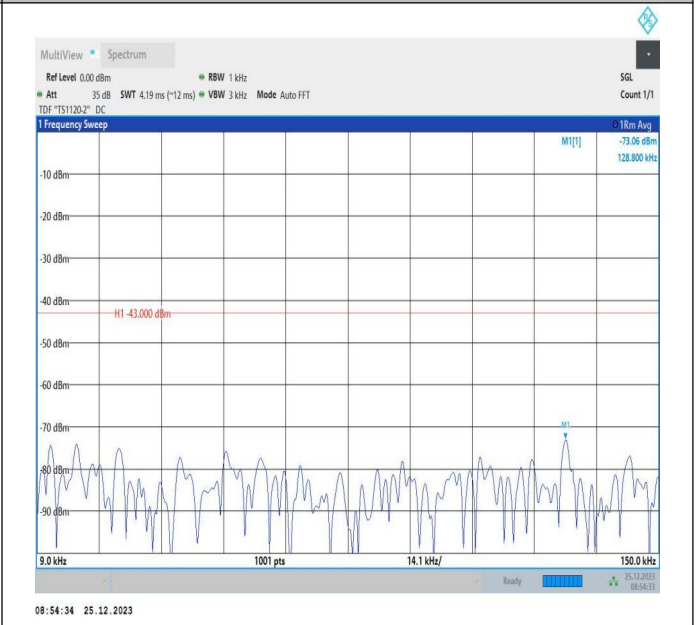
66-66-5MHz-5MHz-16QAM-16QAM-132398-132446-25RB#0-25 25RB#0-0.009~0.15MHz-PASS
