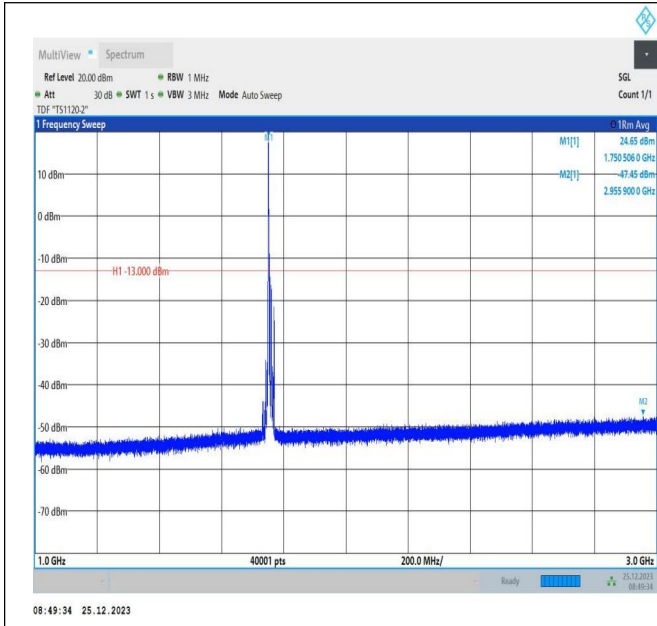
66-66-5MHz-5MHz-16QAM-16QAM-132398-132446-1RB#0-ORB#0-1000~3000MHz-PASS
