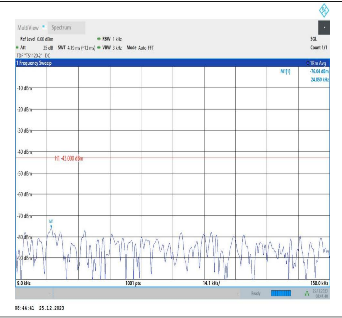
66-66-5MHz-5MHz-16QAM-16QAM-131997-132045-1RB#0-1 RB#15-0.009~0.15MHz-PASS
