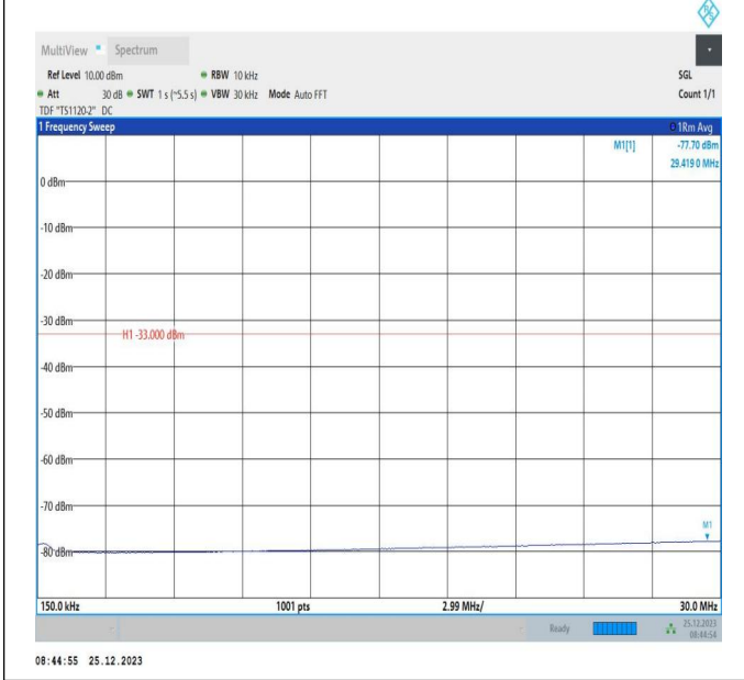
66-66-5MHz-5MHz-16QAM-16QAM-131997-132045-1RB#0-1 1RB#15-0.15~30MHz-PASS
