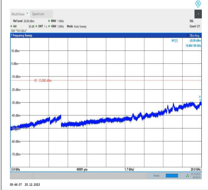
66-66-5MHz-5MHz-QPSK-QPSK-131997-132045-25RB#0-2 5RB#0-3000~20000MHz-PASS
