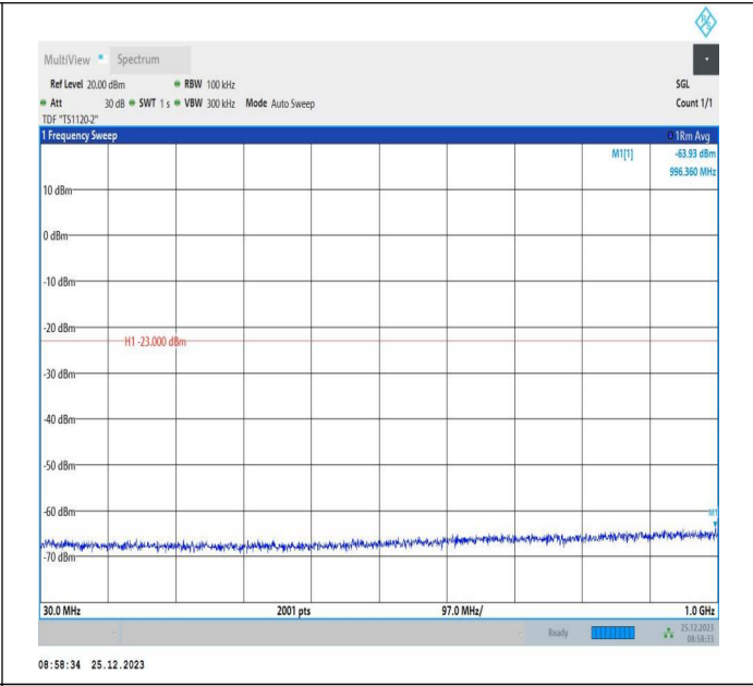
66-66-5MHz-5MHz-16QAM-16QAM-132599-132647-1RB#24-0RB#0-30~1000MHz-PASS
