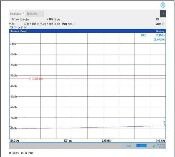
66-66-5MHz-5MHz-QPSK-QPSK-132599-132647-1RB#0-0R B#0-0.15~30MHz-PASS
