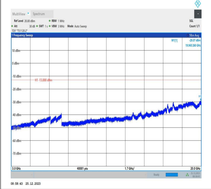
66-66-5MHz-5MHz-16QAM-16QAM-132599-132647-1RB#24-0RB#0-3000~20000MHz-PASS
