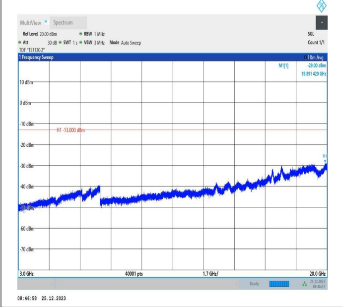
66-66-5MHz-5MHz-16QAM-16QAM-131997-132045-25RB#0-25RB#0-3000~20000MHz-PASS
