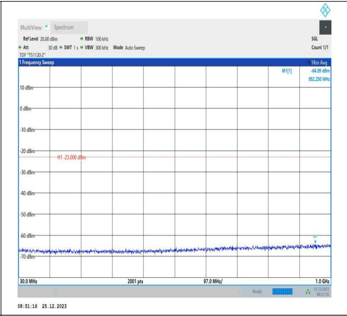
66-66-5MHz-5MHz-16QAM-16QAM-132398-132446-1RB#24-0RB#0-30~1000MHz-PASS
