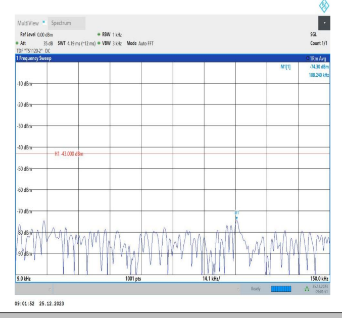
66-66-5MHz-5MHz-16QAM-16QAM-132599-132647-25RB#0- 25RB#0-0.009~0.15MHz-PASS
