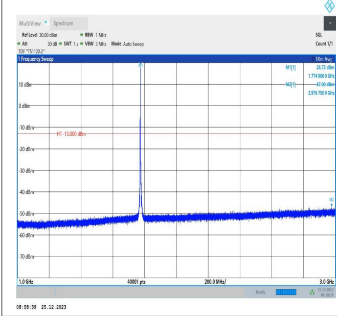
66-66-5MHz-5MHz-16QAM-16QAM-132599-132647-1RB#24-0RB#0-1000~3000MHz-PASS
