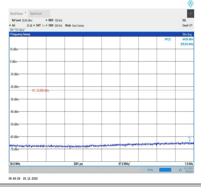
66-66-5MHz-5MHz-16QAM-16QAM-132398-132446-1RB#0-0 RB#0-30~1000MHz-PASS
