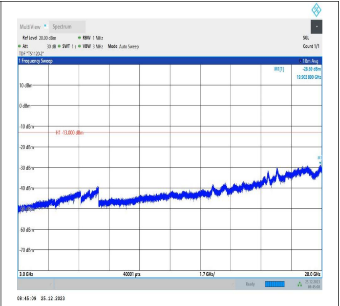
66-66-5MHz-5MHz-16QAM-16QAM-131997-132045-1RB#0-1RB#15-3000~20000MHz-PASS
