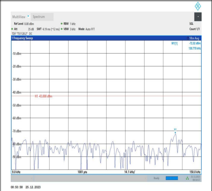
66-66-5MHz-5MHz-16QAM-16QAM-132398-132446-1RB#24-0 RB#0-0.009~0.15MHz-PASS
