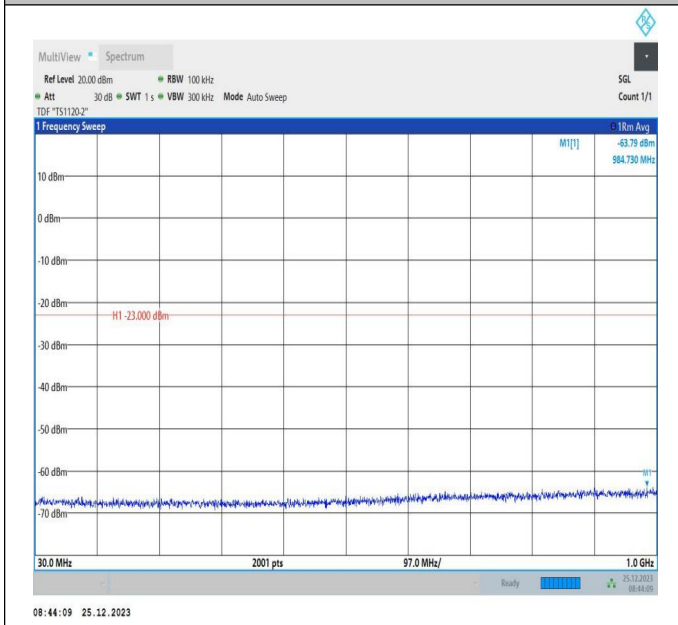
66-66-5MHz-5MHz-QPSK-QPSK-131997-132045-1RB#0-1R B#15-30~1000MHz-PASS
