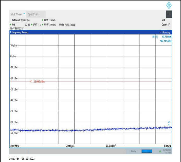
66-66-5MHz-10MHz-16QAM-16QAM-132000-132072-1RB#0-0ORB#0-30~1000MHz-PASS
