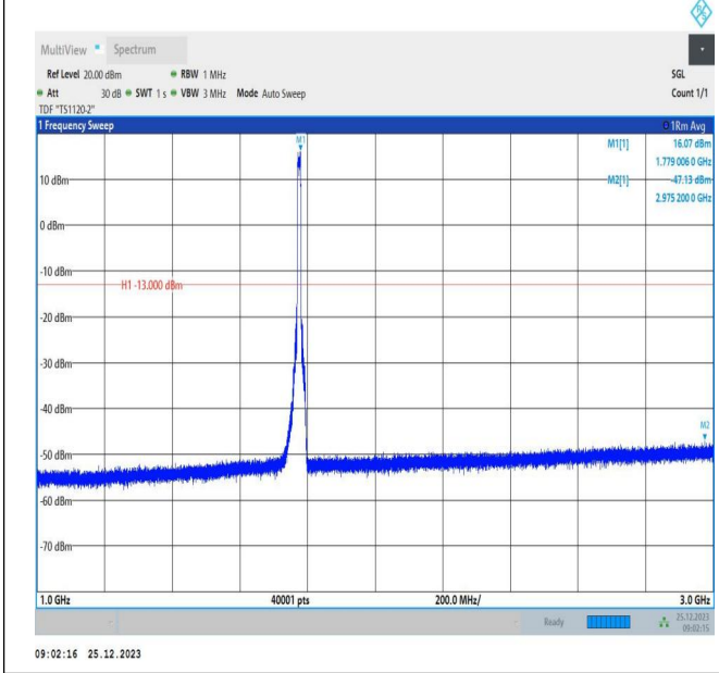
66-66-5MHz-5MHz-16QAM-16QAM-132599-132647-25RB#0-25RB#0-1000~3000MHz-PASS
