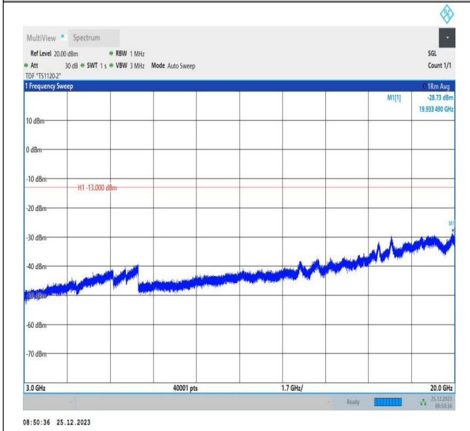
66-66-5MHz-5MHz-QPSK-QPSK-132398-132446-1RB#24-0 RB#0-3000~20000MHz-PASS
