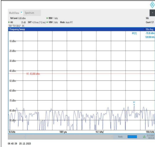
66-66-5MHz-5MHz-QPSK-QPSK-131997-132045-25RB#0-25RB#0-0.009~0.15MHz-PASS
