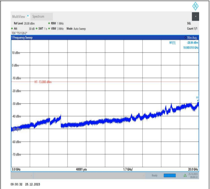
66-66-5MHz-5MHz-16QAM-16QAM-132599-132647-1RB#0-1RB#15-3000~20000MHz-PASS
