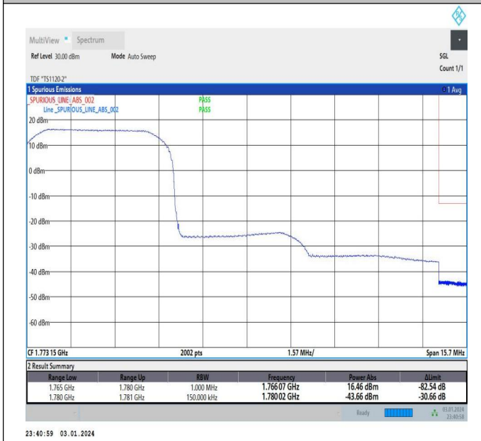
5MHz-10MHz_16QAM@16QAM-16QAM@16QAM_132550-132622_1RB#0@25RB#0-0RB#0@50RB#0
