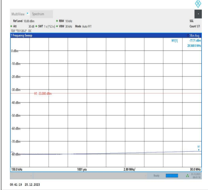
66-66-5MHz-5MHz-16QAM-16QAM-131997-132045-1RB#0-0 ORB#0-0.15~30MHz-PASS
