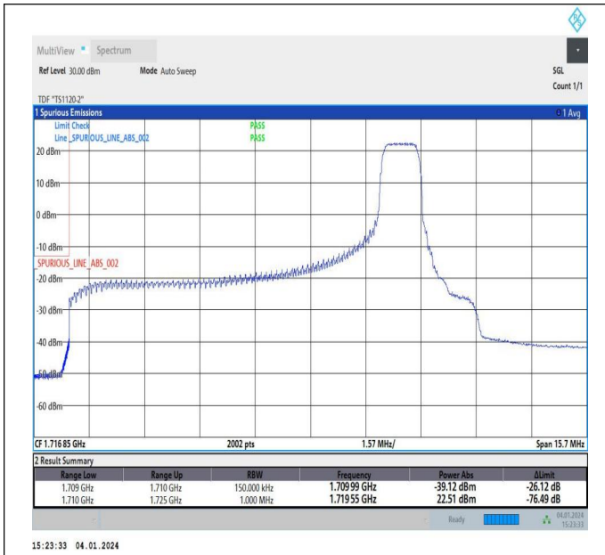
10MHz-5MHz_64QAM@64QAM-64QAM@64QAM_132022-1 32094_1RB#49@50RB#0-0RB#0@25RB#0
