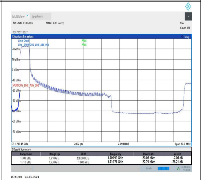
10MHz-10MHz_64QAM@64QAM-64QAM@64QAM_132022- 132121_1RB#0@50RB#0-0RB#0@50RB#0
