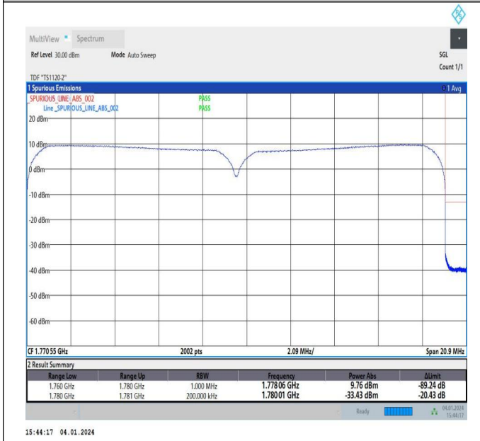
10MHz-10MHz_64QAM@64QAM-64QAM@64QAM_132523-132622_50RB#0@50RB#0-50RB#0@50RB#0
