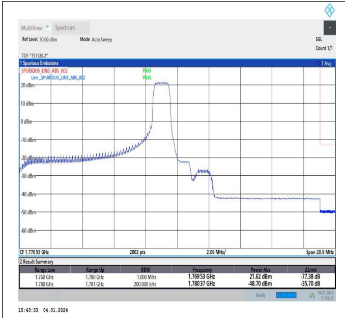
10MHz-10MHz_64QAM@64QAM-64QAM@64QAM_132523-132622_1RB#49@50RB#0-0RB#0@50RB#0
