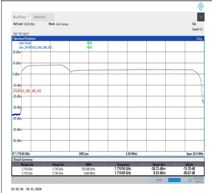
5MHz-15MHz_QPSK@QPSK-QPSK@QPSK_132002-13209_5_25RB#0@25RB#0-75RB#0@75RB#0
