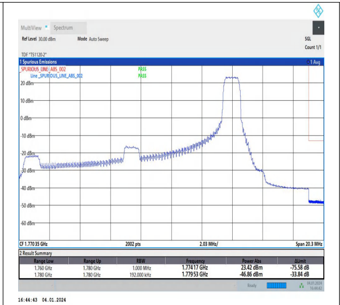
15MHz-5MHz_64QAM@64QAM-64QAM@64QAM_132549-1 32642_1RB#74@75RB#0-0RB#0@25RB#0
