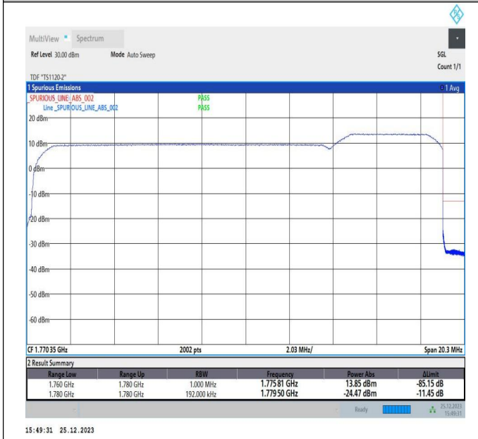
15MHz-5MHz_16QAM@16QAM-16QAM@16QAM_132549-1 32642_75RB#0@75RB#0-25RB#0@25RB#0
