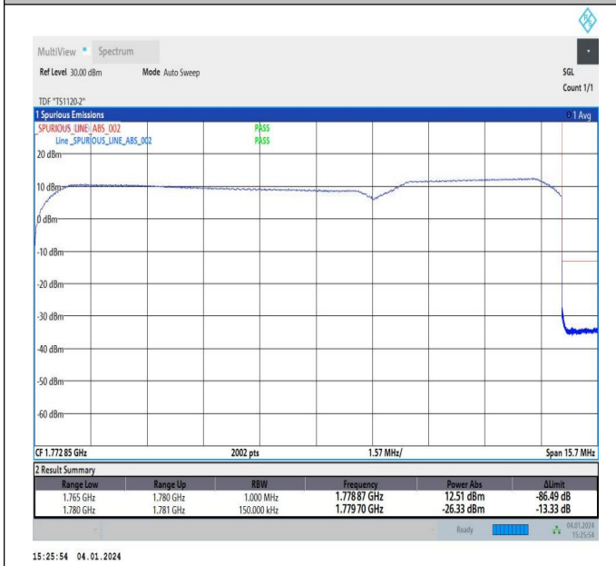
10MHz-5MHz_64QAM@64QAM-64QAM@64QAM_132572-1 32644_50RB#0@50RB#0-25RB#0@25RB#0
