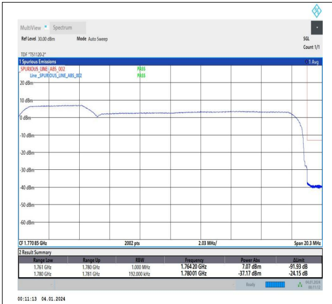
5MHz-15MHz_16QAM@16QAM-16QAM@16QAM_132504-1 32597_25RB#0@25RB#0-75RB#0@75RB#0
