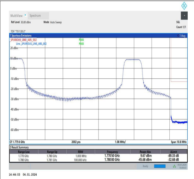
5MHz-5MHz_64QAM@64QAM-64QAM@64QAM_132599-13 2647_1RB#0@25RB#0-1RB#15@25RB#0
