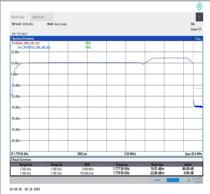
15MHz-5MHz_QPSK@QPSK-QPSK@QPSK_132549-13264 2_75RB#0@75RB#0-25RB#0@25RB#0
