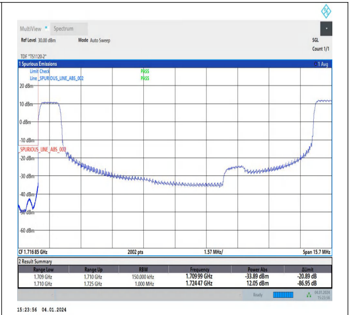
10MHz-5MHz_64QAM@64QAM-64QAM@64QAM_132022-1 32094_1RB#0@50RB#0-1RB#24@25RB#0
