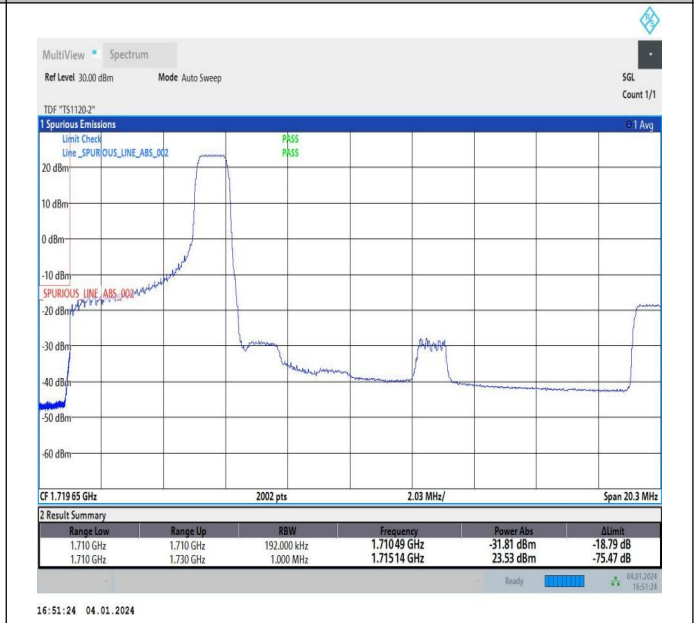
5MHz-15MHz_64QAM@64QAM-64QAM@64QAM_132002-132095_1RB#24@25RB#0-0RB#0@75RB#0
