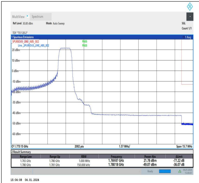
5MHz-10MHz_64QAM@64QAM-64QAM@64QAM_132550-1 32622_1RB#24@25RB#0-0RB#0@50RB#0
