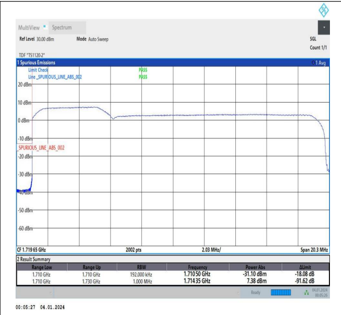
5MHz-15MHz_16QAM@16QAM-16QAM@16QAM_132002-1 32095_25RB#0@25RB#0-75RB#0@75RB#0
