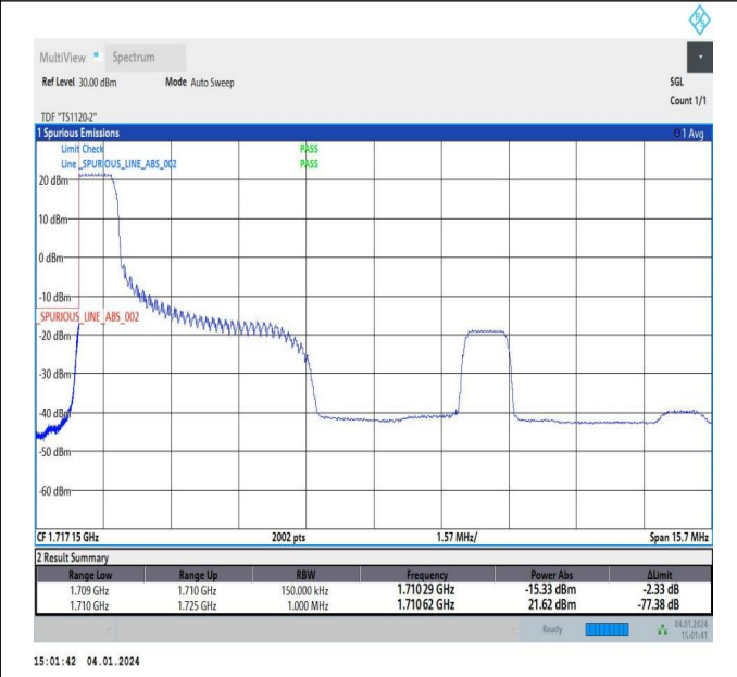
5MHz-10MHz_64QAM@64QAM-64QAM@64QAM_132000-1 32072_1RB#0@25RB#0-0RB#0@50RB#0
