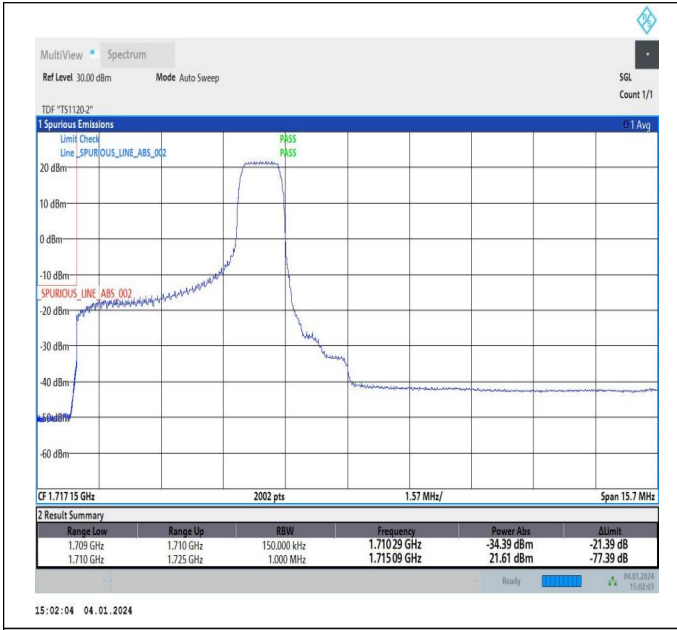
5MHz-10MHz_64QAM@64QAM-64QAM@64QAM_132000-1 32072_1RB#24@25RB#0-0RB#0@50RB#0
