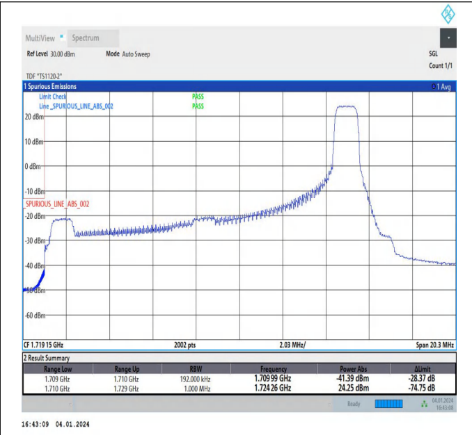
15MHz-5MHz_64QAM@64QAM-64QAM@64QAM_132047-132140_1RB#74@75RB#0-0RB#0@25RB#0
