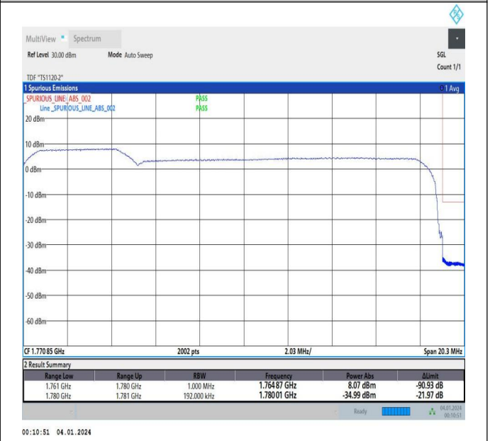
5MHz-15MHz_QPSK@QPSK-QPSK@QPSK_132504-132597_25RB#0@25RB#0-75RB#0@75RB#0
