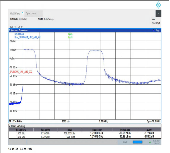
5MHz-5MHz_64QAM@64QAM-64QAM@64QAM_131997-13 2045_1RB#0@25RB#0-1RB#15@25RB#0
