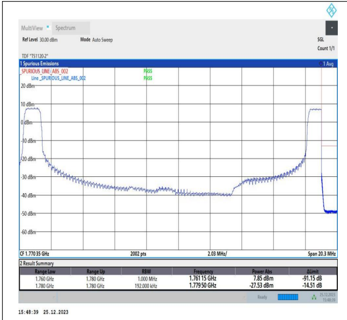
15MHz-5MHz_16QAM@16QAM-16QAM@16QAM_132549-1 32642_1RB#0@75RB#0-1RB#24@25RB#0
