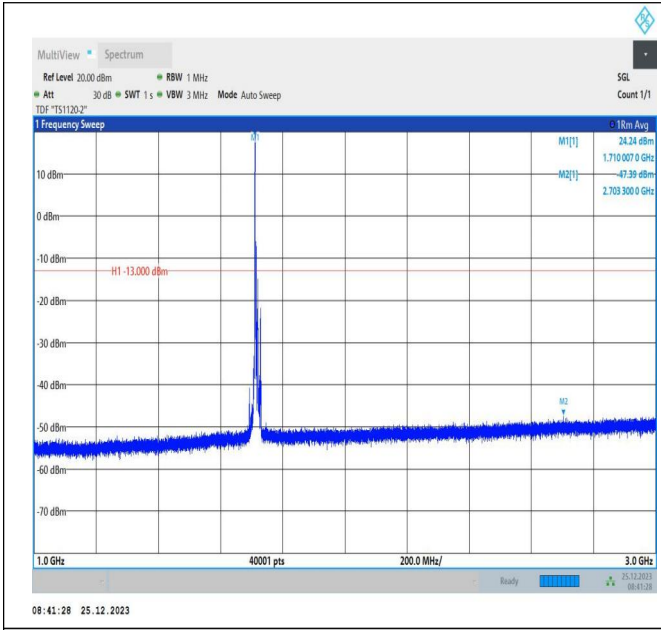
66-66-5MHz-5MHz-16QAM-16QAM-131997-132045-1RB#0-ORB#0-1000~3000MHz-PASS
