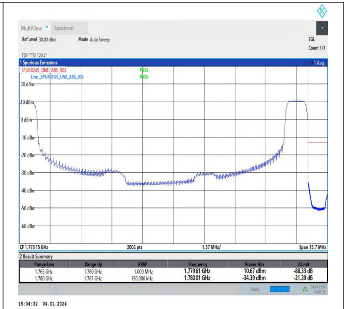
5MHz-10MHz_64QAM@64QAM-64QAM@64QAM_132550-1 32622_1RB#0@25RB#0-1RB#49@50RB#0
