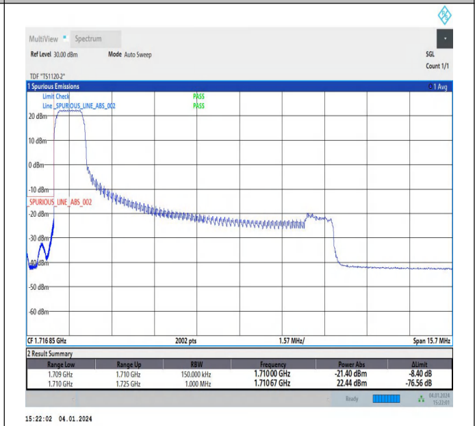
10MHz-5MHz_64QAM@64QAM-64QAM@64QAM_132022-1 32094_1RB#0@50RB#0-0RB#0@25RB#0
