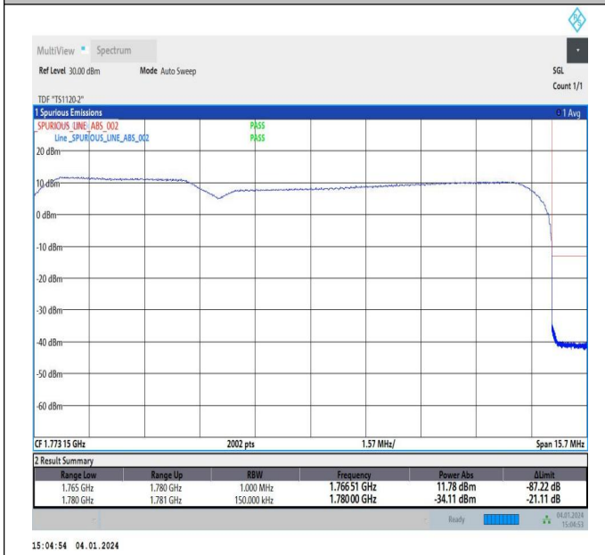
5MHz-10MHz_64QAM@64QAM-64QAM@64QAM_132550-1 32622_25RB#0@25RB#0-50RB#0@50RB#0
