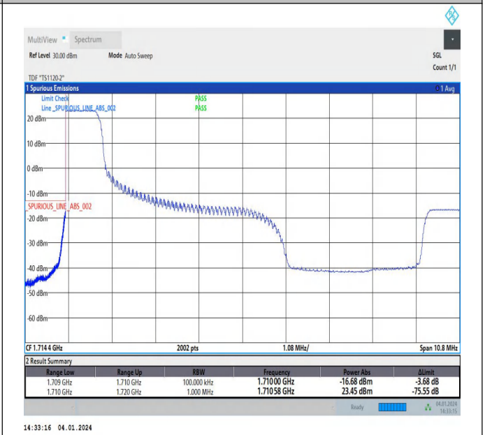
5MHz-5MHz_64QAM@64QAM-64QAM@64QAM_131997-13 2045_1RB#0@25RB#0-0RB#0@25RB#0
