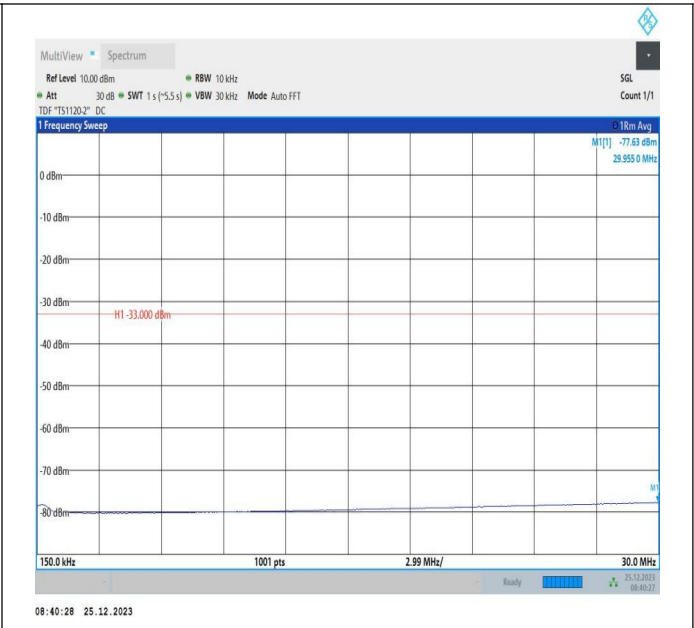
66-66-5MHz-5MHz-QPSK-QPSK-131997-132045-1RB#0-0R B#0-0.15~30MHz-PASS
