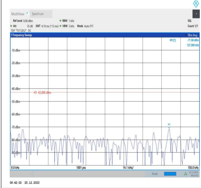
66-66-5MHz-5MHz-QPSK-QPSK-131997-132045-1RB#24-0RB#0-0.009~0.15MHz-PASS
