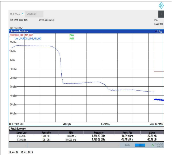
5MHz-10MHz_QPSK@QPSK-QPSK@QPSK_132550-132622_1RB#0@25RB#0-0RB#0@50RB#0
