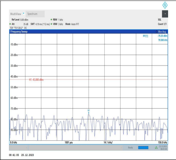
66-66-5MHz-5MHz-16QAM-16QAM-131997-132045-1RB#0-0 RB#0-0.009~0.15MHz-PASS
