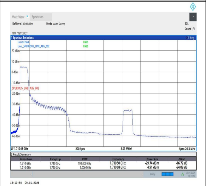
5MHz-15MHz_64QAM@64QAM-64QAM@64QAM_132002-132095_1RB#0@25RB#0-0RB#0@75RB#0
