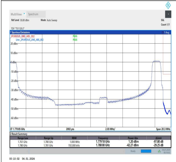
5MHz-15MHz_16QAM@16QAM-16QAM@16QAM_132504-1 32597_1RB#0@25RB#0-1RB#74@75RB#0
