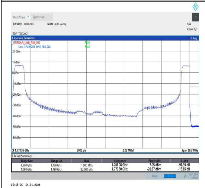
15MHz-5MHz_64QAM@64QAM-64QAM@64QAM_132549-1 32642_1RB#0@75RB#0-1RB#24@25RB#0
