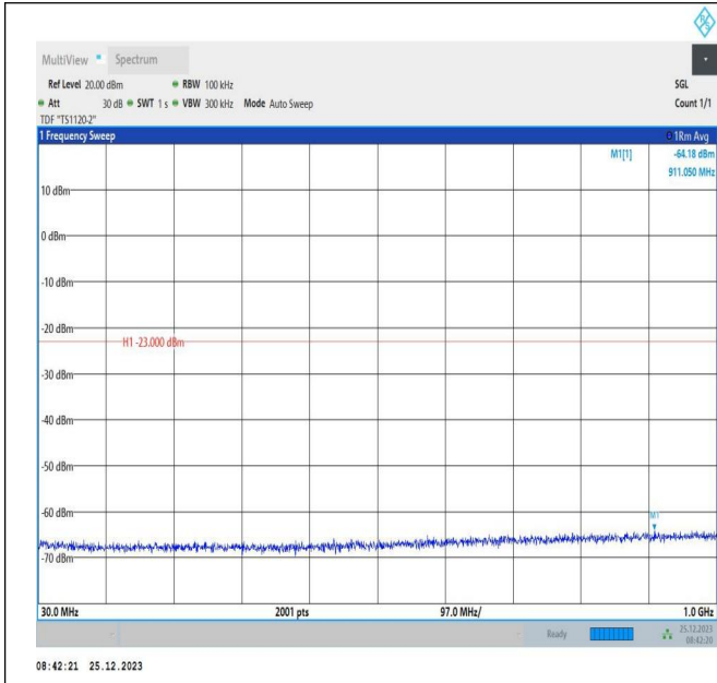
66-66-5MHz-5MHz-QPSK-QPSK-131997-132045-1RB#24-0 RB#0-30~1000MHz-PASS
