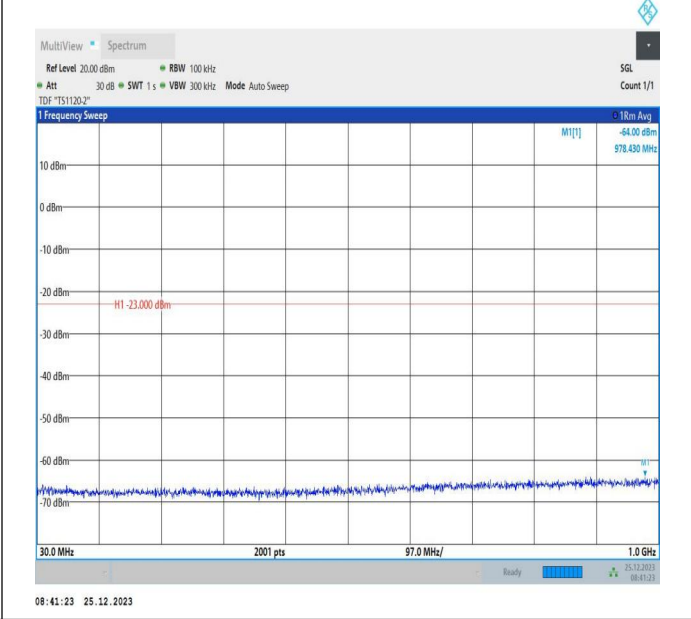
66-66-5MHz-5MHz-16QAM-16QAM-131997-132045-1RB#0-0 RB#0-30~1000MHz-PASS
