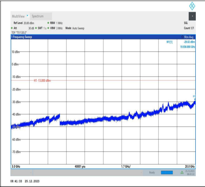
66-66-5MHz-5MHz-16QAM-16QAM-131997-132045-1RB#0-0RB#0-3000~20000MHz-PASS
