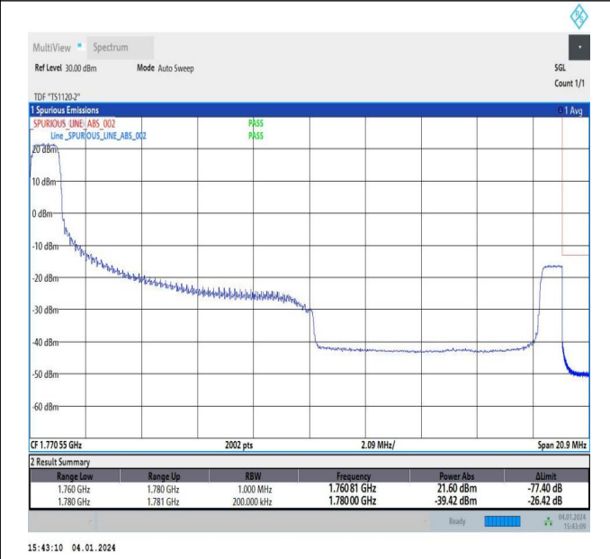
10MHz-10MHz_64QAM@64QAM-64QAM@64QAM_132523-132622_1RB#0@50RB#0-0RB#0@50RB#0
