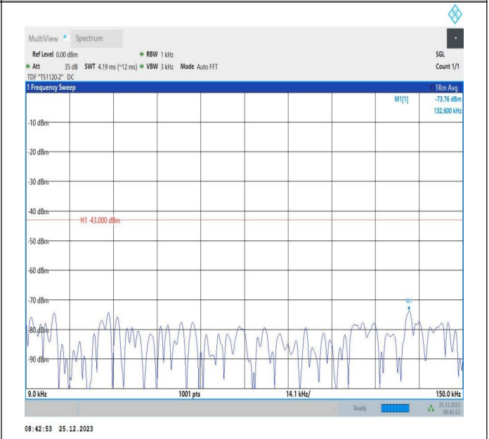
66-66-5MHz-5MHz-16QAM-16QAM-131997-132045-1RB#24-0 RB#0-0.009~0.15MHz-PASS
