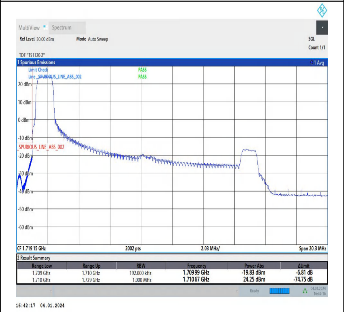
15MHz-5MHz_64QAM@64QAM-64QAM@64QAM_132047-32140_1RB#0@75RB#0-0RB#0@25RB#0
