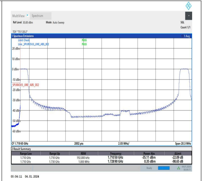
5MHz-15MHz_16QAM@16QAM-16QAM@16QAM_132002-132095_1RB#0@25RB#0-1RB#74@75RB#0
