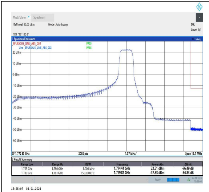
10MHz-5MHz_64QAM@64QAM-64QAM@64QAM_132572-1 32644_1RB#49@50RB#0-0RB#0@25RB#0
