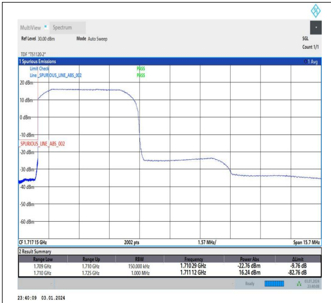
5MHz-10MHz_16QAM@16QAM-16QAM@16QAM_132000-132072_1RB#0@25RB#0-0RB#0@50RB#0
