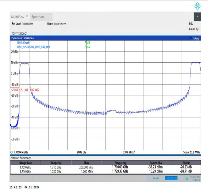
10MHz-10MHz_64QAM@64QAM-64QAM@64QAM_132022-132121_1RB#0@50RB#0-1RB#49@50RB#0
