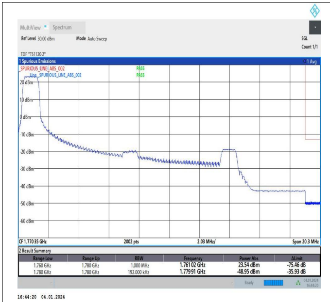
15MHz-5MHz_64QAM@64QAM-64QAM@64QAM_132549-1 32642_1RB#0@75RB#0-0RB#0@25RB#0
