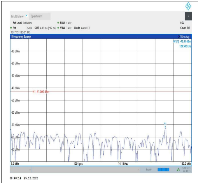
66-66-5MHz-5MHz-QPSK-QPSK-131997-132045-1RB#0-0R B#0-0.009~0.15MHz-PASS
