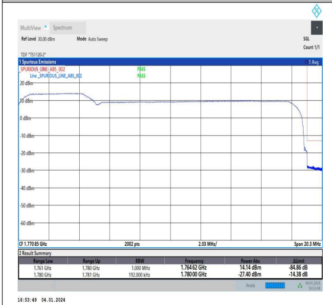
5MHz-15MHz_64QAM@64QAM-64QAM@64QAM_132504-1 32597_25RB#0@25RB#0-75RB#0@75RB#0
