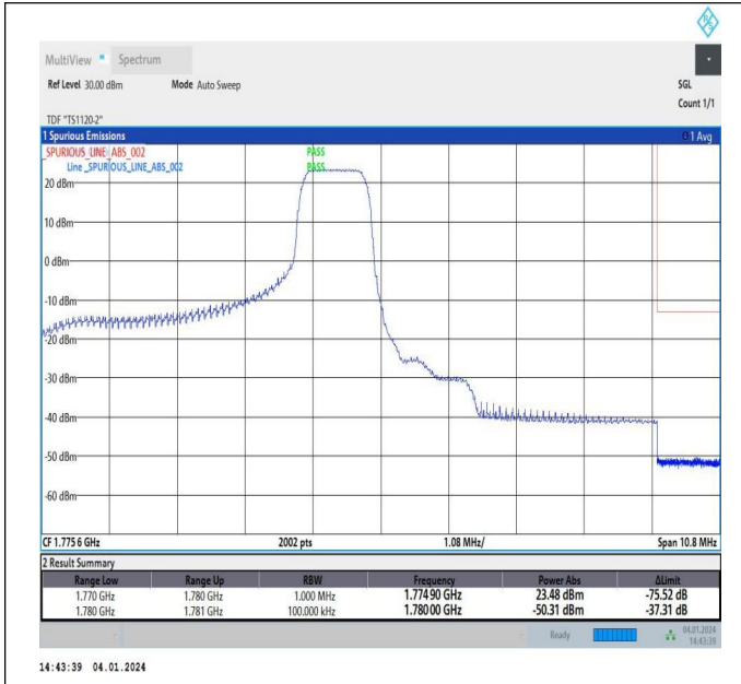
5MHz-5MHz_64QAM@64QAM-64QAM@64QAM_132599-13 2647_1RB#24@25RB#0-0RB#0@25RB#0
