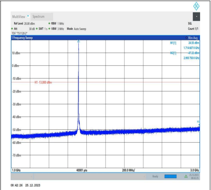
66-66-5MHz-5MHz-QPSK-QPSK-131997-132045-1RB#24-0R B#0-1000~3000MHz-PASS
