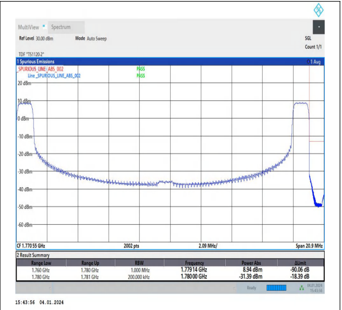
10MHz-10MHz_64QAM@64QAM-64QAM@64QAM_132523-132622_1RB#0@50RB#0-1RB#49@50RB#0
