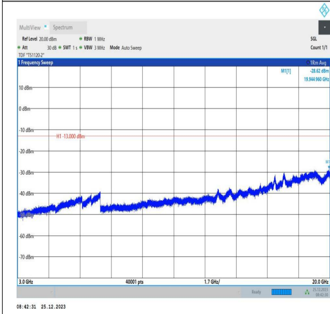
66-66-5MHz-5MHz-QPSK-QPSK-131997-132045-1RB#24-0 RB#0-3000~20000MHz-PASS
