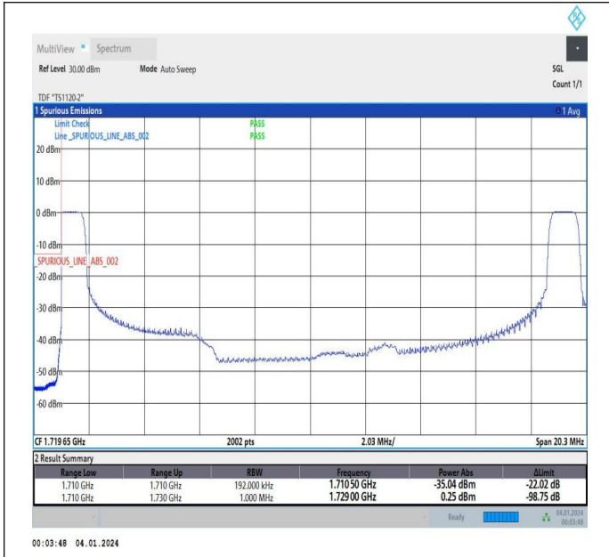
5MHz-15MHz_QPSK@QPSK-QPSK@QPSK_132002-13209_5_1RB#0@25RB#0-1RB#74@75RB#0
