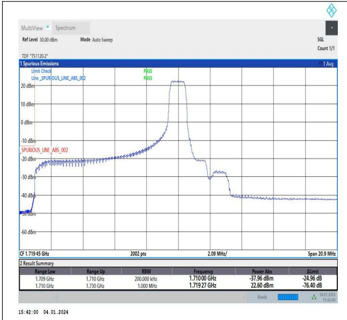
10MHz-10MHz_64QAM@64QAM-64QAM@64QAM_132022-132121_1RB#49@50RB#0-0RB#0@50RB#0
