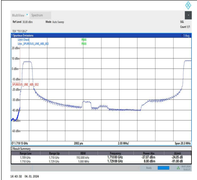
15MHz-5MHz_64QAM@64QAM-64QAM@64QAM_132047-132140_1RB#0@75RB#0-1RB#24@25RB#0
