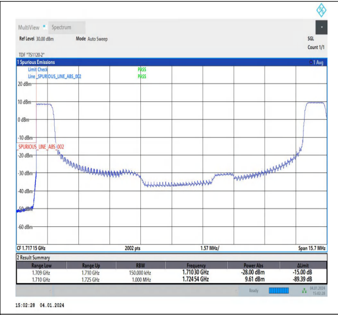
5MHz-10MHz_64QAM@64QAM-64QAM@64QAM_132000-1 32072_1RB#0@25RB#0-1RB#49@50RB#0
