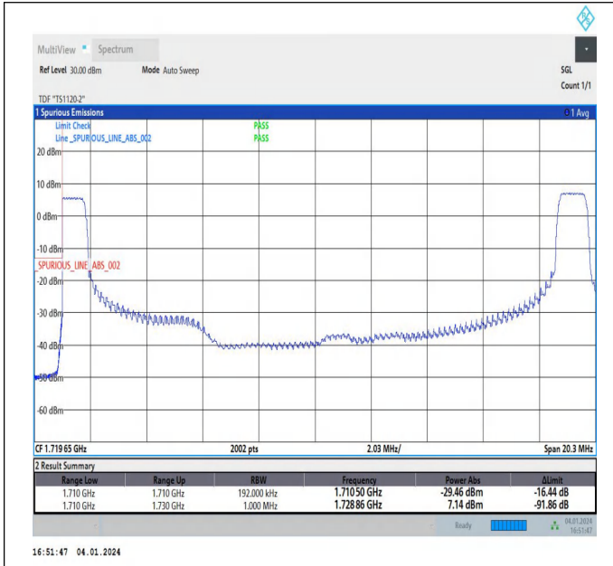
5MHz-15MHz_64QAM@64QAM-64QAM@64QAM_132002-1 32095_1RB#0@25RB#0-1RB#74@75RB#0
