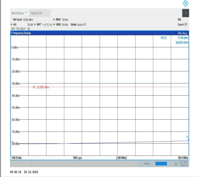
66-66-5MHz-5MHz-QPSK-QPSK-131997-132045-1RB#24-0RB#0-0.15~30MHz-PASS
