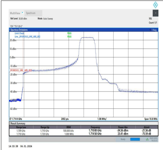
5MHz-5MHz_64QAM@64QAM-64QAM@64QAM_131997-13 2045_1RB#24@25RB#0-0RB#0@25RB#0
