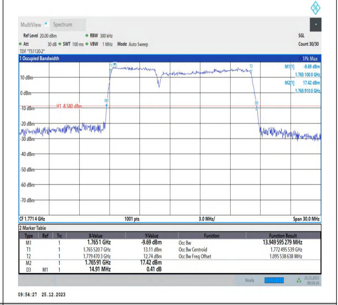
66-66-5MHz-10MHz-16QAM-16QAM-132550-132622-25RB#0-50RB#0-PASS
