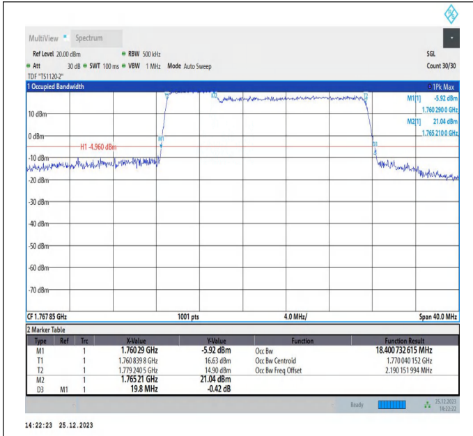
66-66-5MHz-15MHz-QPSK-QPSK-132504-132597-25RB#0-75RB#0-PASS
