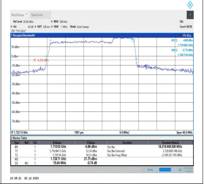
66-66-15MHz-5MHz-16QAM-16QAM-132047-132140-75RB#0-25RB#0-PASS
