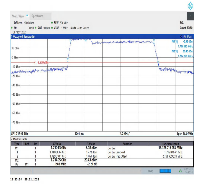
66-66-5MHz-15MHz-16QAM-16QAM-132002-132095-25RB#0-75RB#0-PASS
