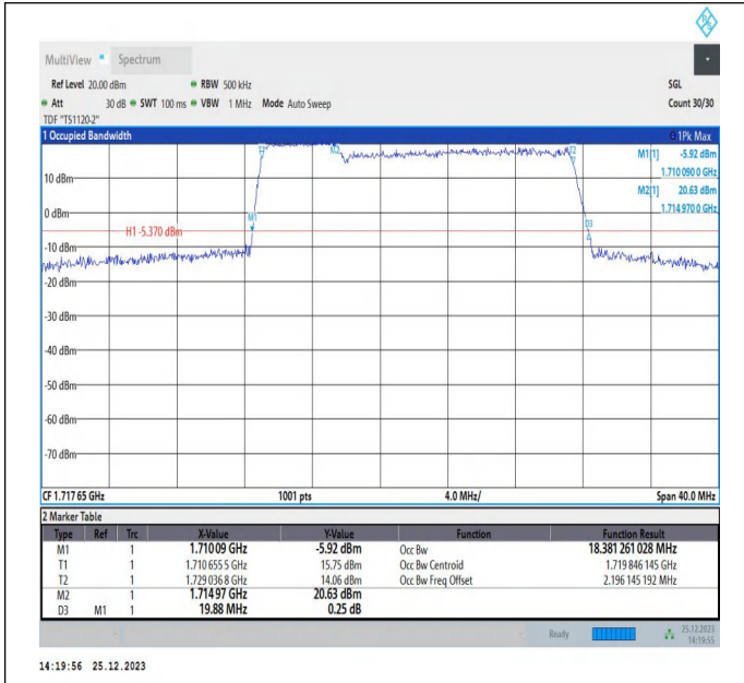
66-66-5MHz-15MHz-QPSK-QPSK-132002-132095-25RB#0-75RB#0-PASS
