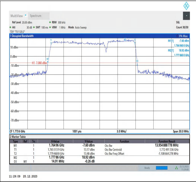
66-66-10MHz-5MHz-16QAM-16QAM-132572-132644-50RB#0-25RB#0-PASS
