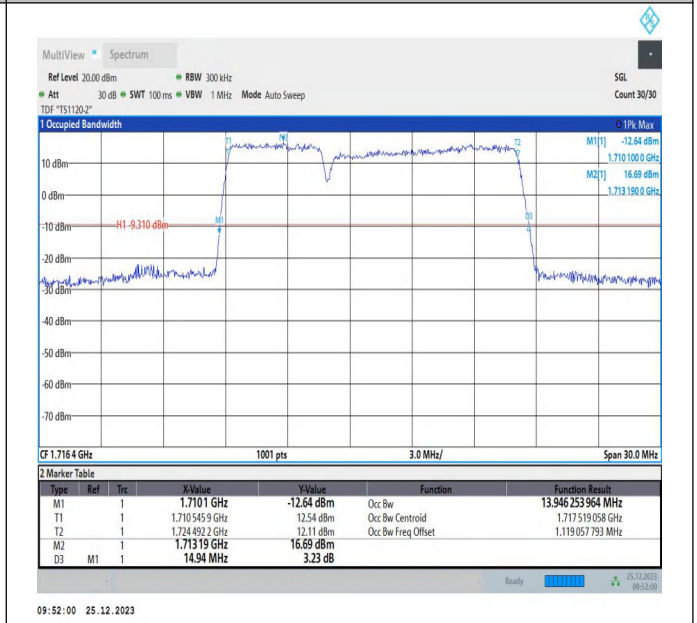
66-66-5MHz-10MHz-16QAM-16QAM-132000-132072-25RB#0-50RB#0-PASS
