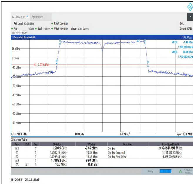
66-66-5MHz-5MHz-QPSK-QPSK-131997-132045-25RB#0-2 5RB#0-PASS
