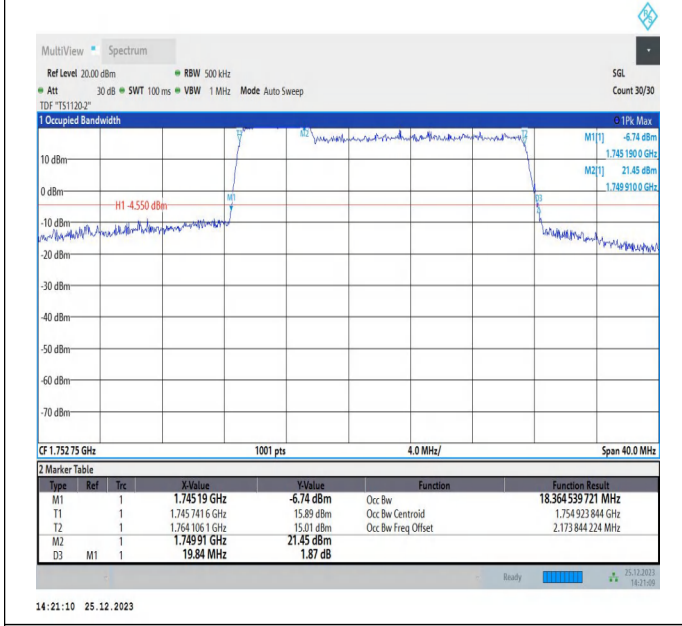
66-66-5MHz-15MHz-QPSK-QPSK-132353-132446-25RB#0-75RB#0-PASS
