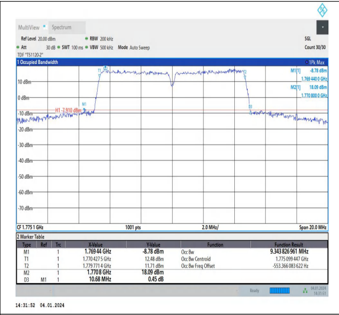
66-66-5MHz-5MHz-64QAM-64QAM-132599-132647-25RB#0 -25RB#0-PASS
