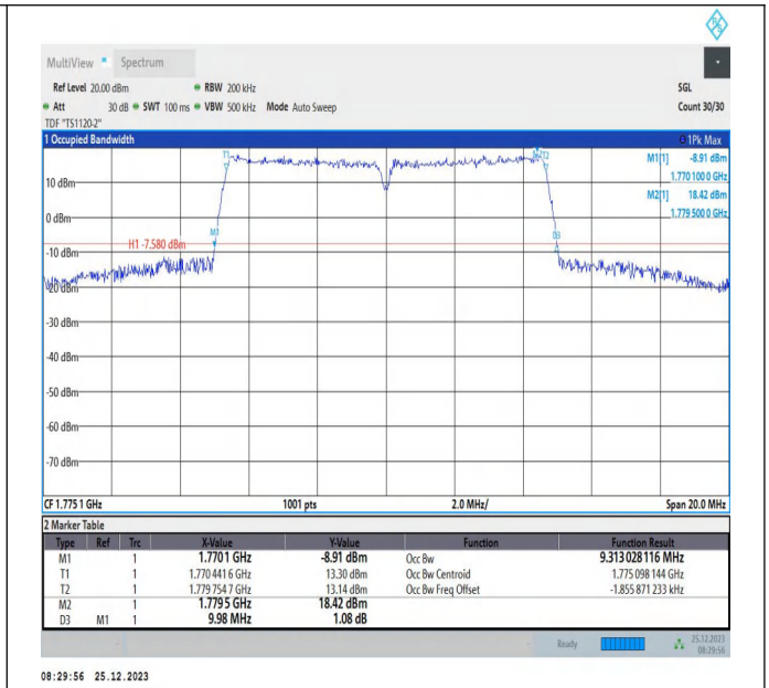
66-66-5MHz-5MHz-16QAM-16QAM-132599-132647-25RB#0-25RB#0-PASS
