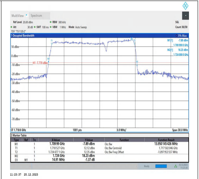
66-66-10MHz-5MHz-16QAM-16QAM-132022-132094-50RB#0-25RB#0-PASS
