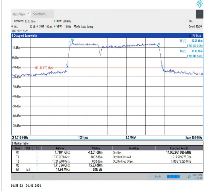
66-66-5MHz-10MHz-64QAM-64QAM-132000-132072-25RB#0 0-50RB#0-PASS
