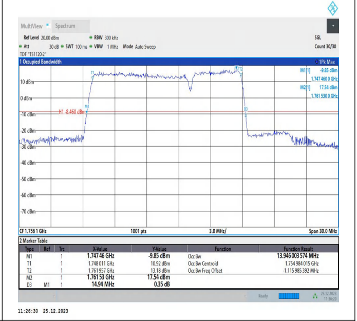
66-66-10MHz-5MHz-16QAM-16QAM-132397-132469-50RB#0-25RB#0-PASS
