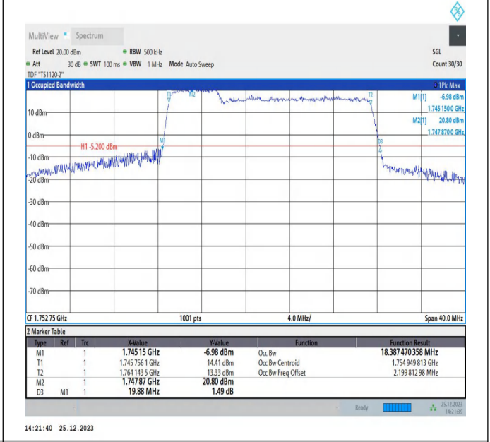
66-66-5MHz-15MHz-16QAM-16QAM-132353-132446-25RB#0-75RB#0-PASS
