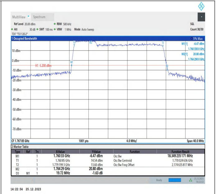
66-66-5MHz-15MHz-16QAM-16QAM-132504-132597-25RB#0-75RB#0-PASS
