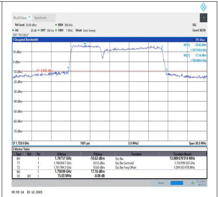
66-66-5MHz-10MHz-16QAM-16QAM-132375-132447-25RB#0-50RB#0-PASS
