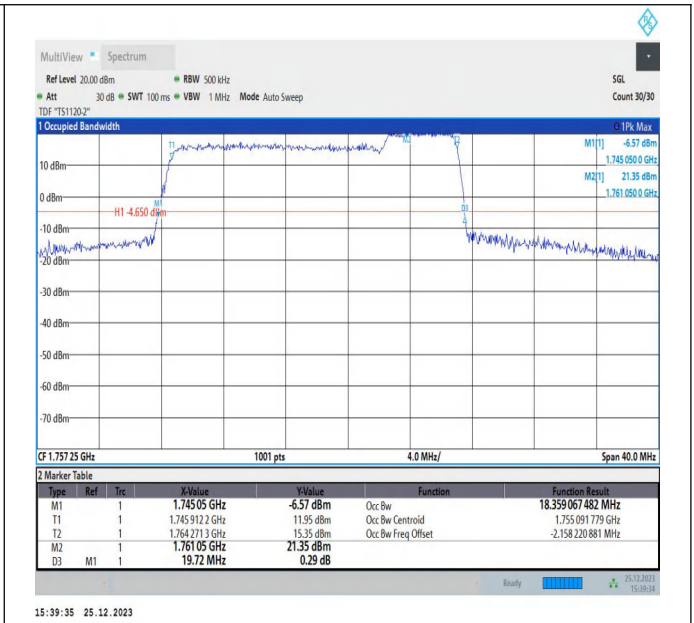
66-66-15MHz-5MHz-16QAM-16QAM-132398-132491-75RB#0-25RB#0-PASS
