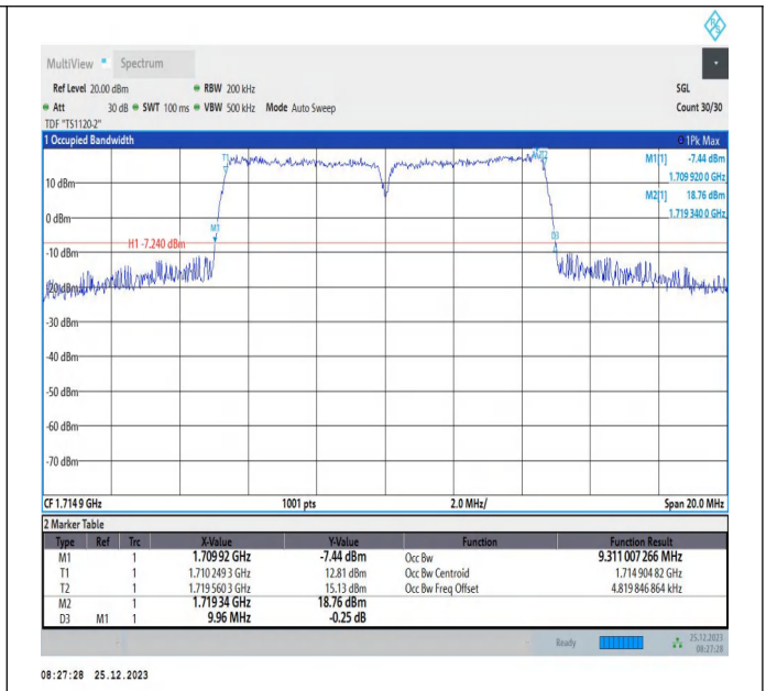
66-66-5MHz-5MHz-16QAM-16QAM-131997-132045-25RB#0-2 -25RB#0-PASS
