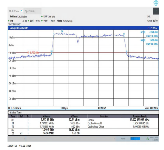
66-66-5MHz-10MHz-64QAM-64QAM-132375-132447-25RB#0 0-50RB#0-PASS
