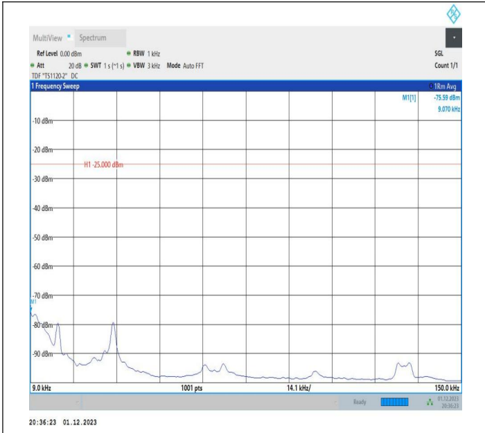
7-7-20MHz-20MHz-16QAM-16QAM-20850-21048-1RB#99-0R B#0-0.009~0.15MHz-PASS
