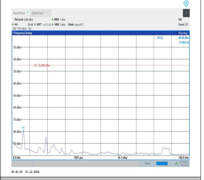
7-7-20MHz-20MHz-64QAM-64QAM-20850-21048-100RB#0-1 00RB#0-0.009~0.15MHz-PASS
