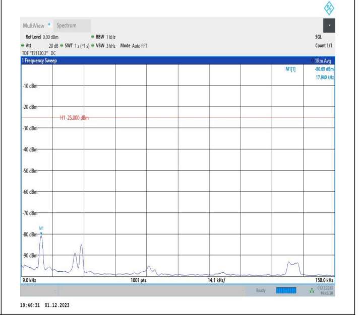
7-7-20MHz-15MHz-16QAM-16QAM-21201-21372-1RB#0-1RB #74-0.009~0.15MHz-PASS
