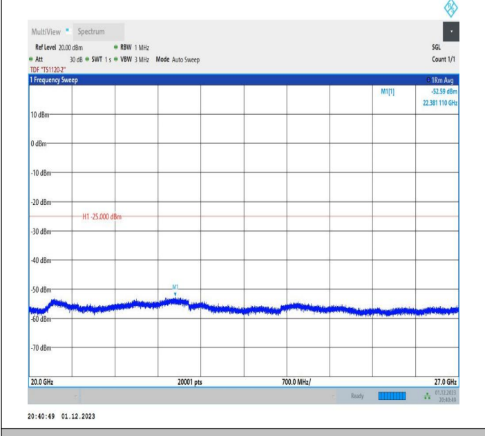
7-7-20MHz-20MHz-16QAM-16QAM-20850-21048-100RB#0-1 00RB#0-20000~27000MHz-PASS
