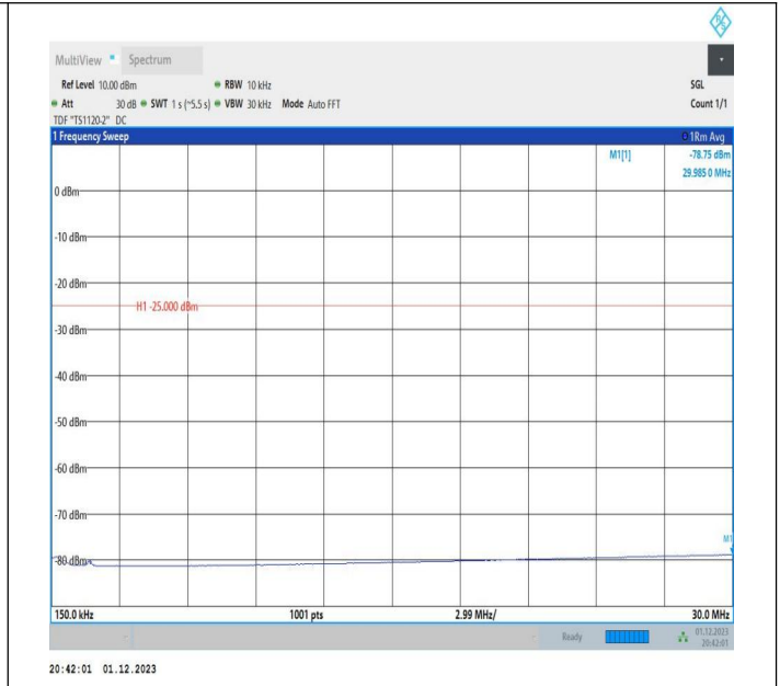
7-7-20MHz-20MHz-QPSK-QPSK-21001-21199-1RB#0-ORB#0-0.15~30MHz-PASS
