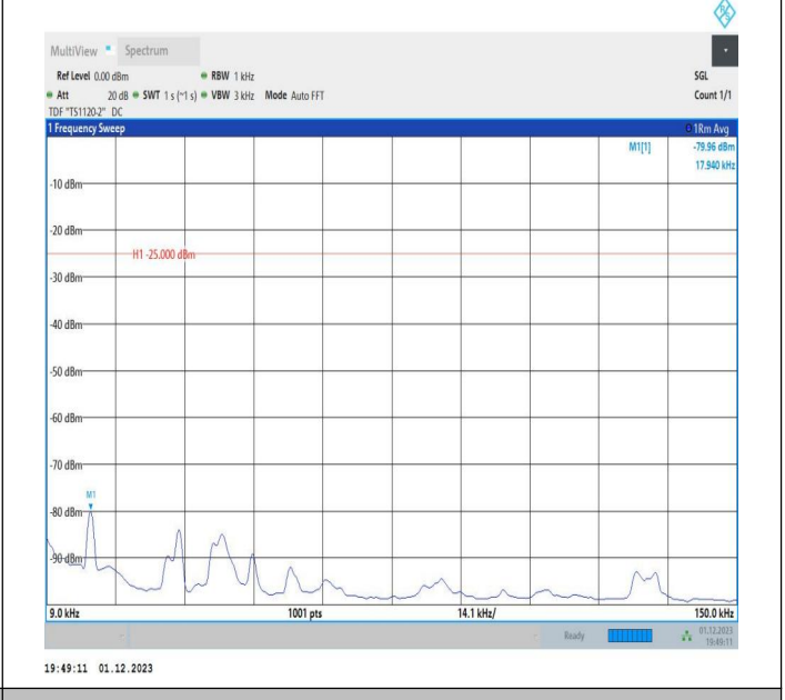
7-7-20MHz-15MHz-64QAM-64QAM-21201-21372-100RB#0-7 5RB#0-0.009~0.15MHz-PASS
