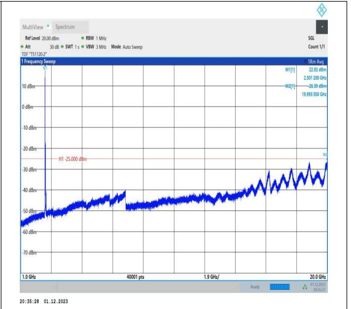
7-7-20MHz-20MHz-64QAM-64QAM-20850-21048-1RB#0-ORB #0-1000~20000MHz-PASS
