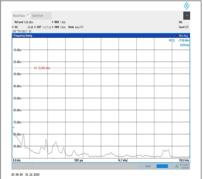
7-7-20MHz-20MHz-16QAM-16QAM-20850-21048-1RB#0-0RB #0-0.009~0.15MHz-PASS
