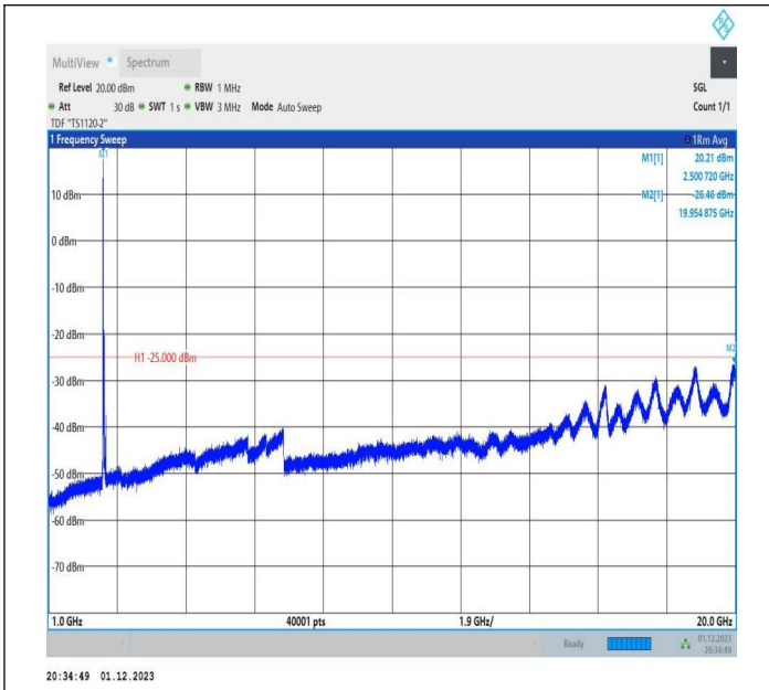
7-7-20MHz-20MHz-16QAM-16QAM-20850-21048-1RB#0-ORB #0-1000~20000MHz-PASS
