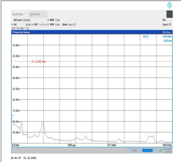
7-7-20MHz-20MHz-QPSK-QPSK-21001-21199-1RB#0-ORB#0-0.009~0.15MHz-PASS
