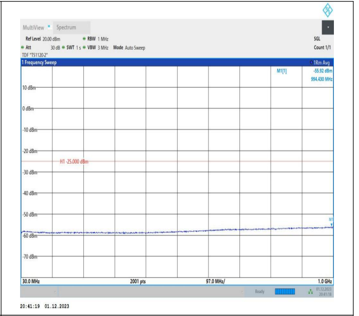
7-7-20MHz-20MHz-64QAM-64QAM-20850-21048-100RB#0-1 00RB#0-30~1000MHz-PASS
