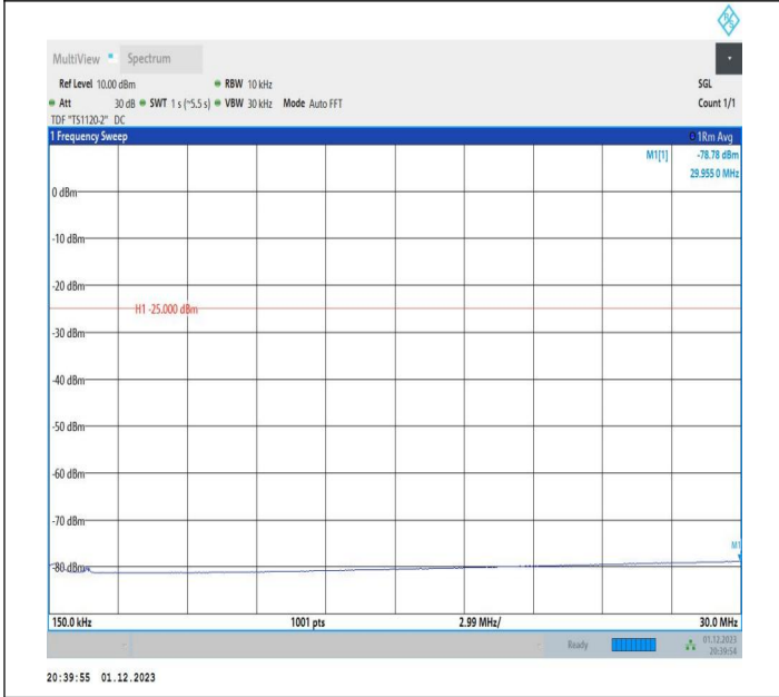
7-7-20MHz-20MHz-QPSK-QPSK-20850-21048-100RB#0-100 RB#0-0.15~30MHz-PASS
