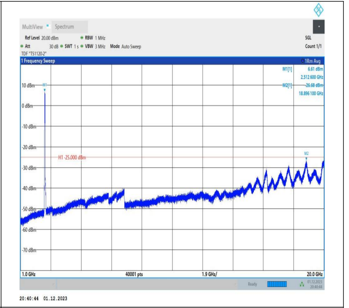
7-7-20MHz-20MHz-16QAM-16QAM-20850-21048-100RB#0-1 00RB#0-1000~20000MHz-PASS
