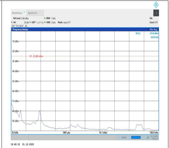
7-7-20MHz-15MHz-64QAM-64QAM-21201-21372-1RB#99-0R B#0-0.009~0.15MHz-PASS
