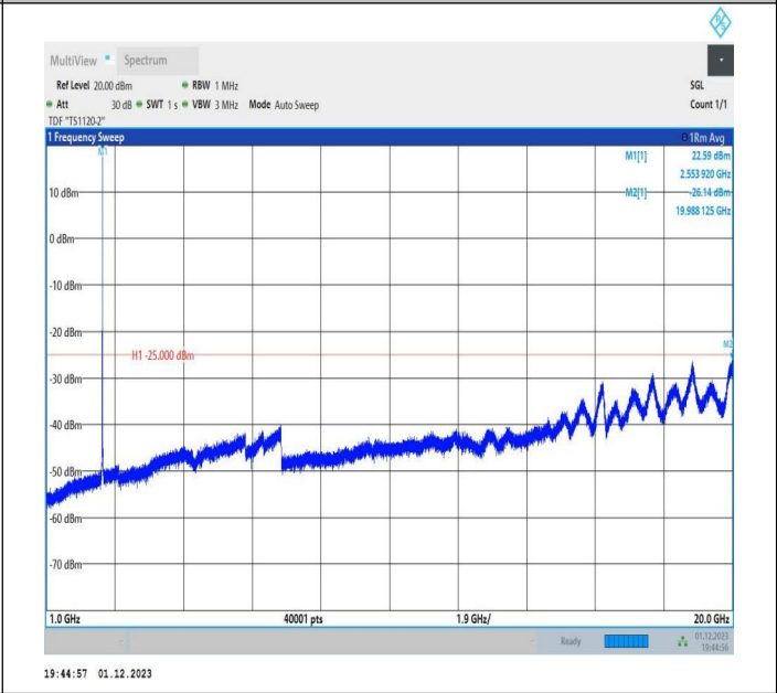
7-7-20MHz-15MHz-16QAM-16QAM-21201-21372-1RB#99-0R B#0-1000~20000MHz-PASS
