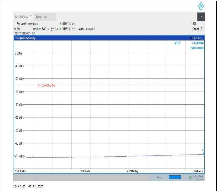
7-7-20MHz-15MHz-64QAM-64QAM-21201-21372-1RB#0-1RB #74-0.15~30MHz-PASS
