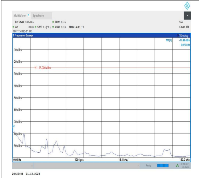
7-7-20MHz-20MHz-64QAM-64QAM-20850-21048-1RB#0-ORB #0-0.009~0.15MHz-PASS
