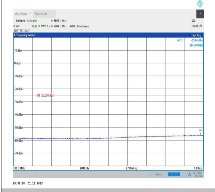
7-7-20MHz-20MHz-64QAM-64QAM-20850-21048-1RB#0-1RB #99-30~1000MHz-PASS
