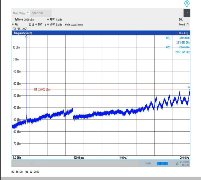
7-7-20MHz-20MHz-QPSK-QPSK-20850-21048-1RB#99-0RB# 0-1000~20000MHz-PASS
