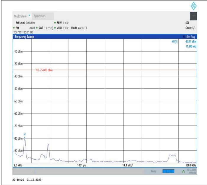
7-7-20MHz-20MHz-16QAM-16QAM-20850-21048-100RB#0-1 00RB#0-0.009~0.15MHz-PASS
