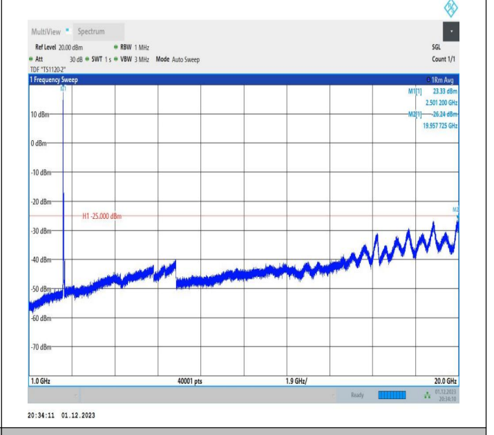
7-7-20MHz-20MHz-QPSK-QPSK-20850-21048-1RB#0-0RB#0 -1000~20000MHz-PASS
