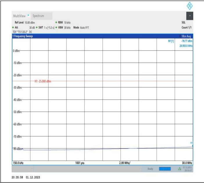
7-7-20MHz-20MHz-QPSK-QPSK-20850-21048-1RB#99-0RB# 0-0.15~30MHz-PASS
