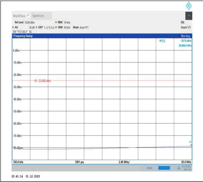
7-7-20MHz-20MHz-64QAM-64QAM-20850-21048-100RB#0-1 00RB#0-0.15~30MHz-PASS
