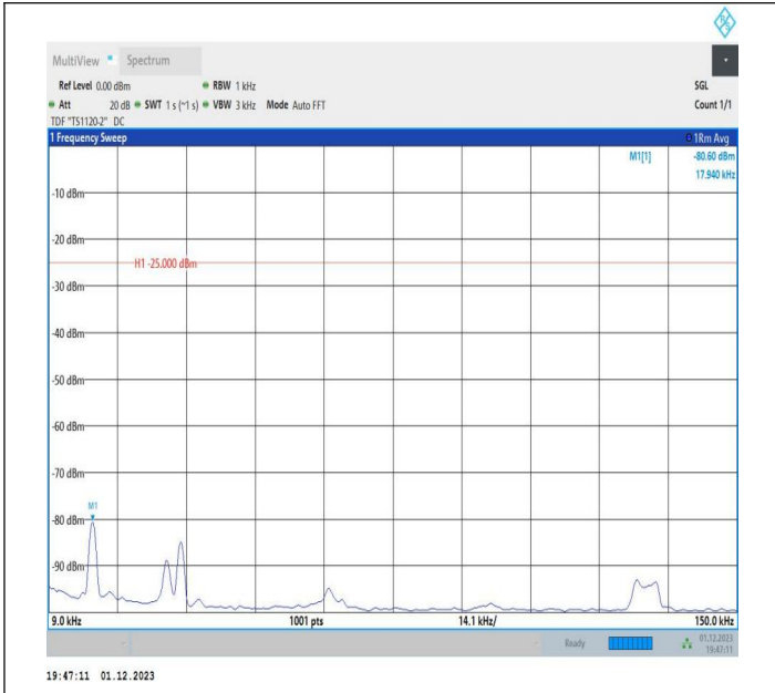
7-7-20MHz-15MHz-64QAM-64QAM-21201-21372-1RB#0-1RB #74-0.009~0.15MHz-PASS
