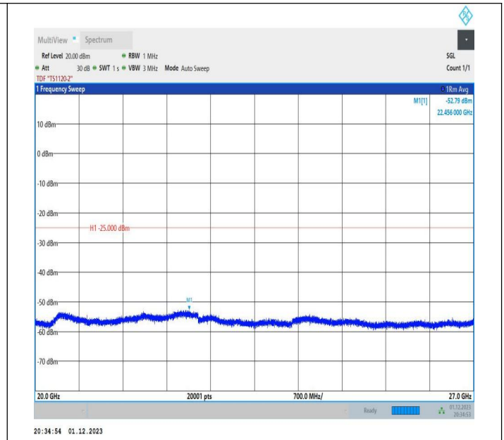
7-7-20MHz-20MHz-16QAM-16QAM-20850-21048-1RB#0-ORB #0-20000~27000MHz-PASS
