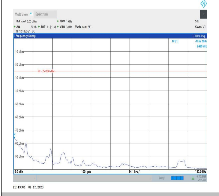
7-7-20MHz-20MHz-64QAM-64QAM-21001-21199-1RB#0-ORB #0-0.009~0.15MHz-PASS
