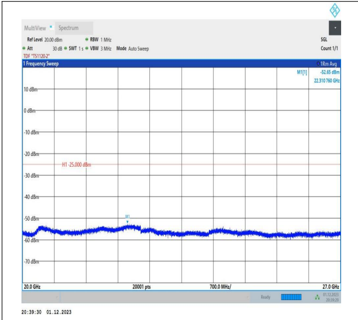
7-7-20MHz-20MHz-64QAM-64QAM-20850-21048-1RB#0-1RB #99-20000~27000MHz-PASS
