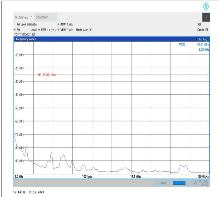
7-7-20MHz-15MHz-16QAM-16QAM-21201-21372-1RB#99-0R B#0-0.009~0.15MHz-PASS
