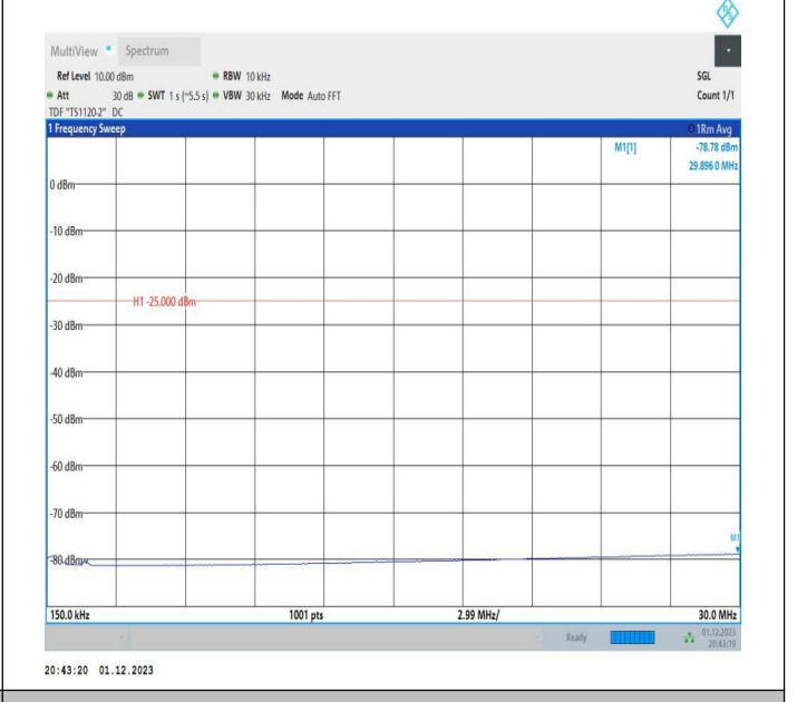
7-7-20MHz-20MHz-64QAM-64QAM-21001-21199-1RB#0-ORB #0-0.15~30MHz-PASS
