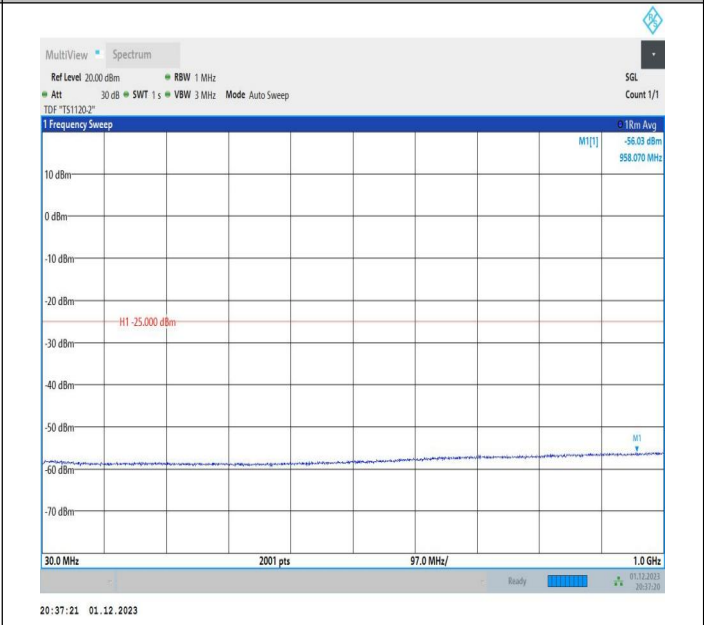
7-7-20MHz-20MHz-64QAM-64QAM-20850-21048-1RB#99-0R B#0-30~1000MHz-PASS
