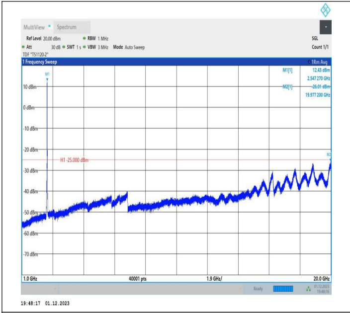
7-7-20MHz-15MHz-QPSK-QPSK-21201-21372-100RB#0-75R B#0-1000~20000MHz-PASS
