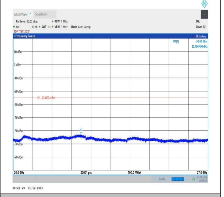
7-7-20MHz-20MHz-64QAM-64QAM-20850-21048-100RB#0-1 00RB#0-20000~27000MHz-PASS
