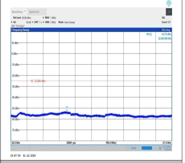
7-7-20MHz-15MHz-16QAM-16QAM-21201-21372-1RB#0-1RB #74-20000~27000MHz-PASS
