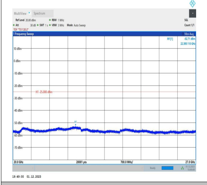
7-7-20MHz-15MHz-16QAM-16QAM-21201-21372-100RB#0-7 5RB#0-20000~27000MHz-PASS
