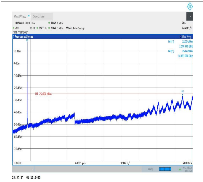
7-7-20MHz-20MHz-64QAM-64QAM-20850-21048-1RB#99-0R B#0-1000~20000MHz-PASS
