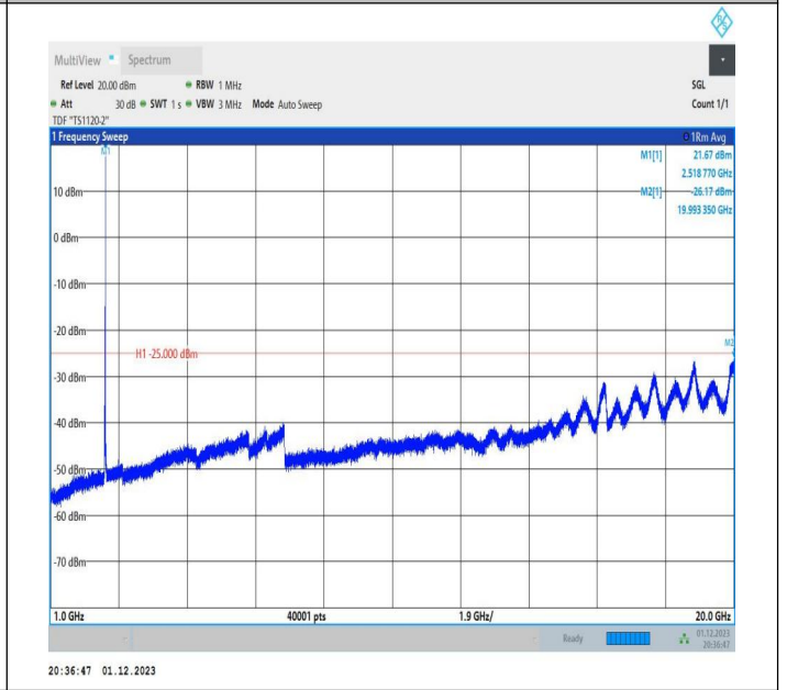
7-7-20MHz-20MHz-16QAM-16QAM-20850-21048-1RB#99-0R B#0-1000~20000MHz-PASS
