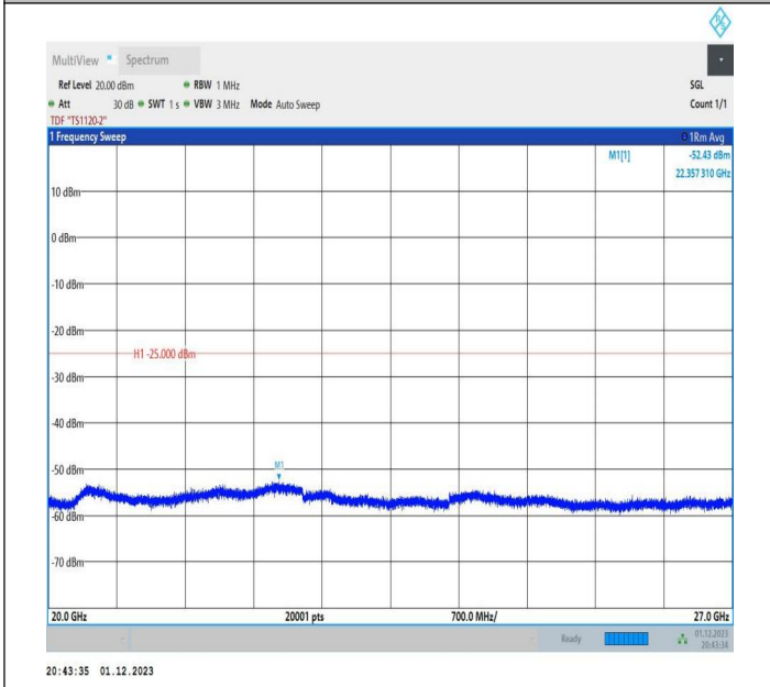
7-7-20MHz-20MHz-64QAM-64QAM-21001-21199-1RB#0-ORB #0-20000~27000MHz-PASS
