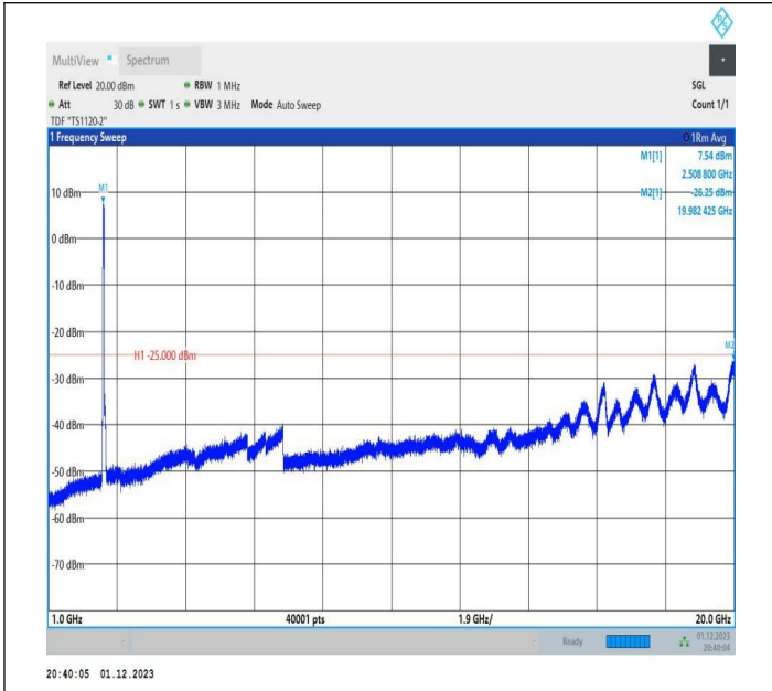
7-7-20MHz-20MHz-QPSK-QPSK-20850-21048-100RB#0-100 RB#0-1000~20000MHz-PASS
