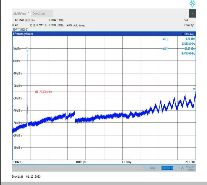
7-7-20MHz-20MHz-64QAM-64QAM-20850-21048-100RB#0-1 00RB#0-1000~20000MHz-PASS
