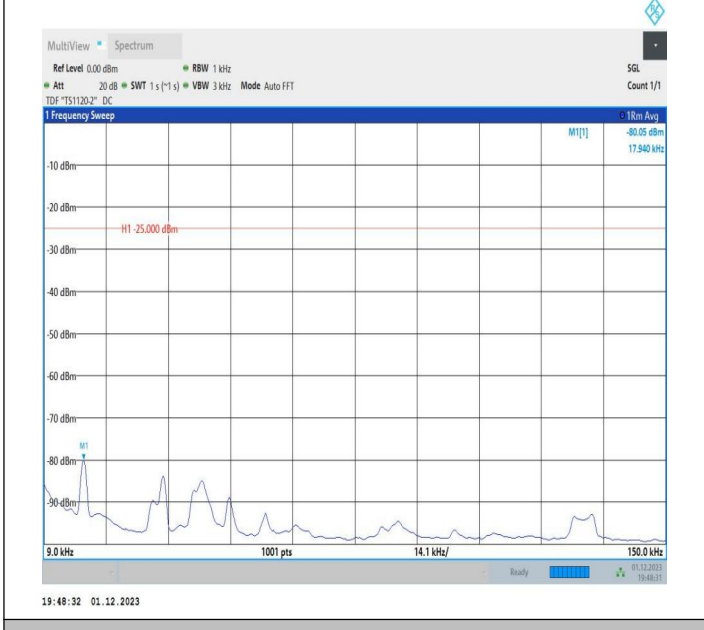
7-7-20MHz-15MHz-16QAM-16QAM-21201-21372-100RB#0-7 5RB#0-0.009~0.15MHz-PASS
