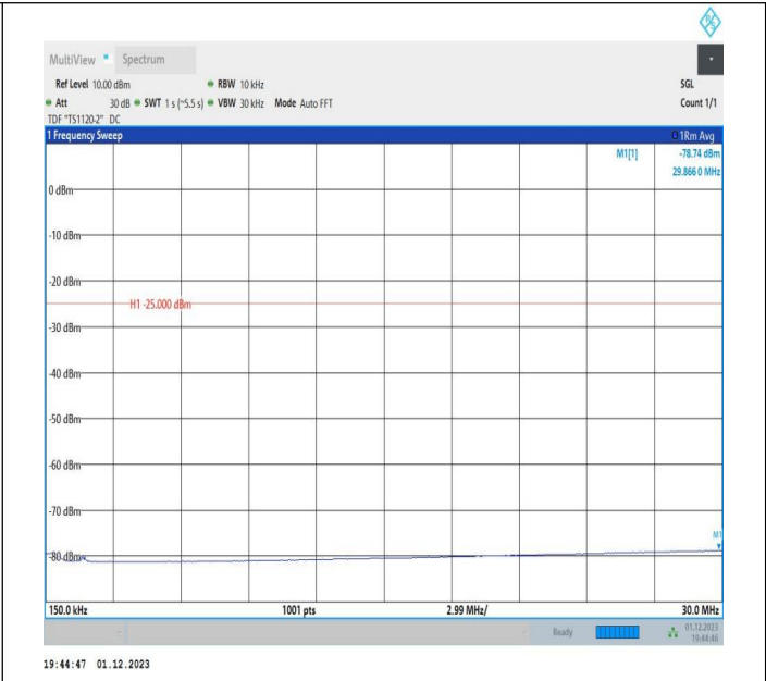
7-7-20MHz-15MHz-16QAM-16QAM-21201-21372-1RB#99-0R B#0-0.15~30MHz-PASS
