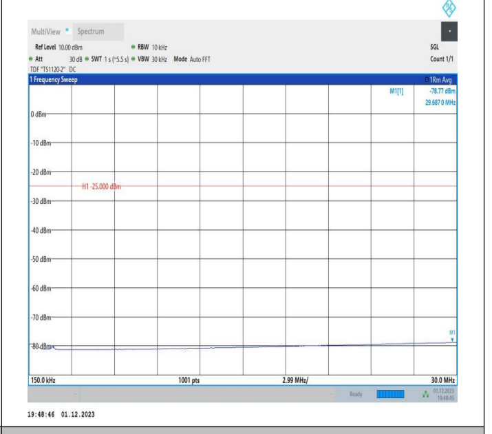
7-7-20MHz-15MHz-16QAM-16QAM-21201-21372-100RB#0-7 5RB#0-0.15~30MHz-PASS
