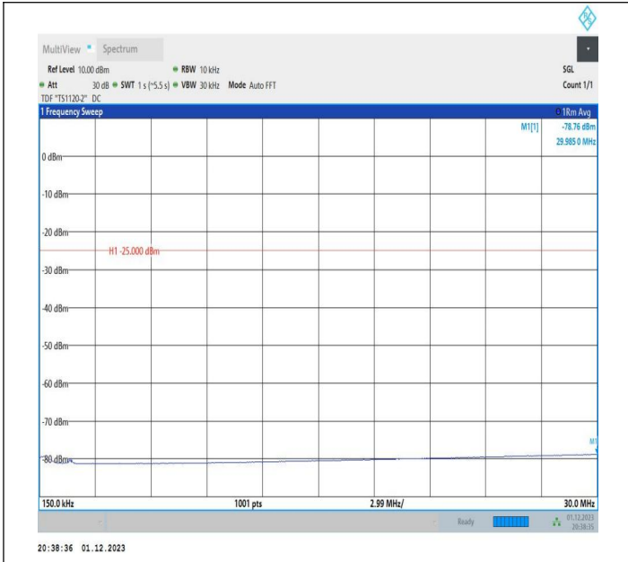
7-7-20MHz-20MHz-16QAM-16QAM-20850-21048-1RB#0-1RB #99-0.15~30MHz-PASS
