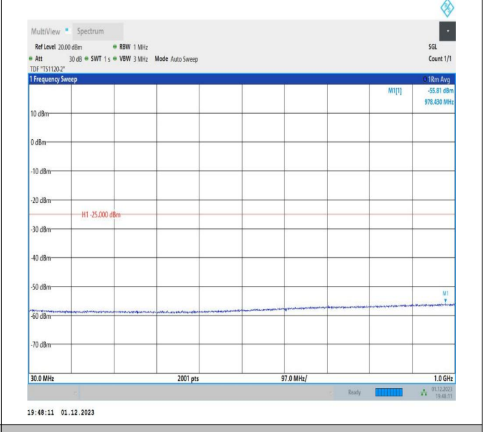
7-7-20MHz-15MHz-QPSK-QPSK-21201-21372-100RB#0-75R B#0-30~1000MHz-PASS
