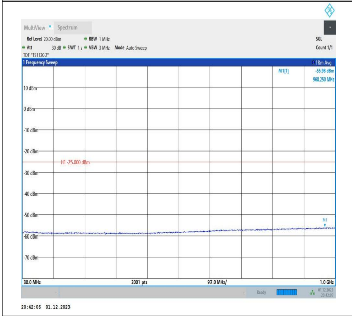
7-7-20MHz-20MHz-QPSK-QPSK-21001-21199-1RB#0-ORB#0-30~1000MHz-PASS
