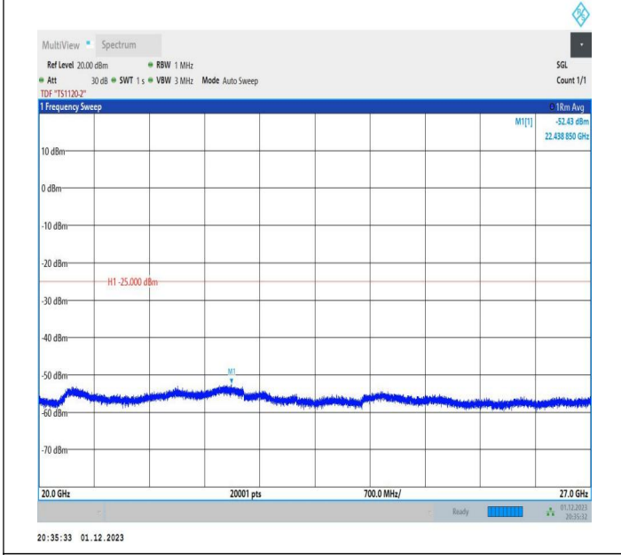
7-7-20MHz-20MHz-64QAM-64QAM-20850-21048-1RB#0-ORB #0-20000~27000MHz-PASS
