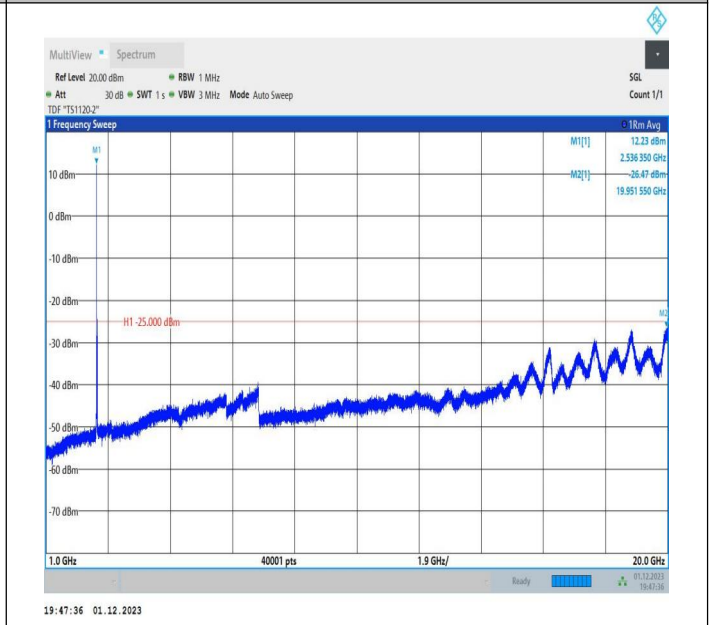
7-7-20MHz-15MHz-64QAM-64QAM-21201-21372-1RB#0-1RB #74-1000~20000MHz-PASS
