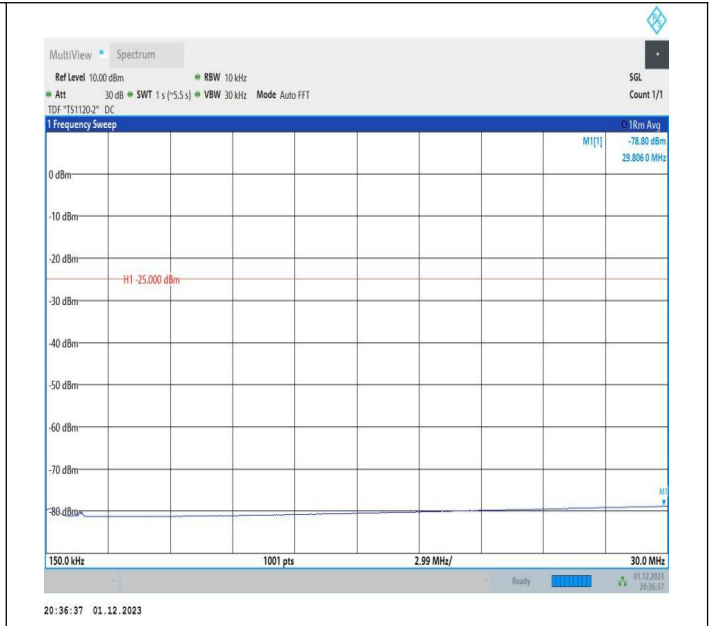
7-7-20MHz-20MHz-16QAM-16QAM-20850-21048-1RB#99-0R B#0-0.15~30MHz-PASS
