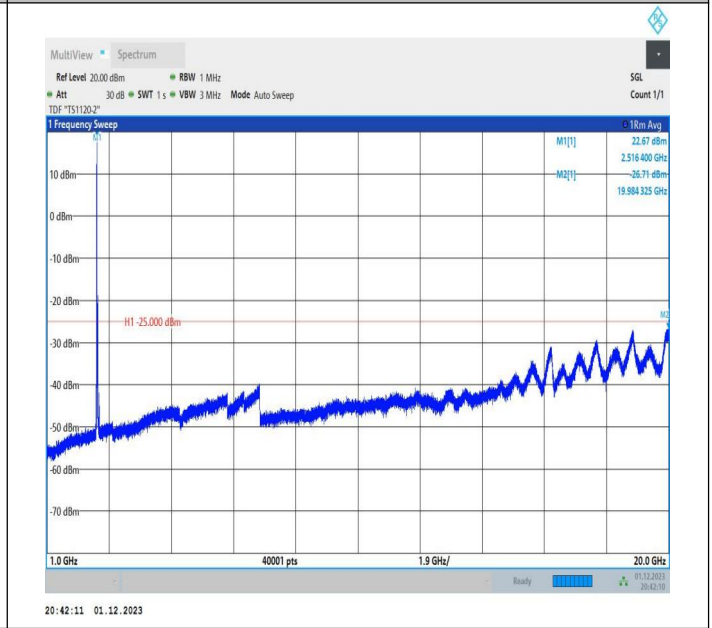
7-7-20MHz-20MHz-QPSK-QPSK-21001-21199-1RB#0-ORB#0-1000~20000MHz-PASS
