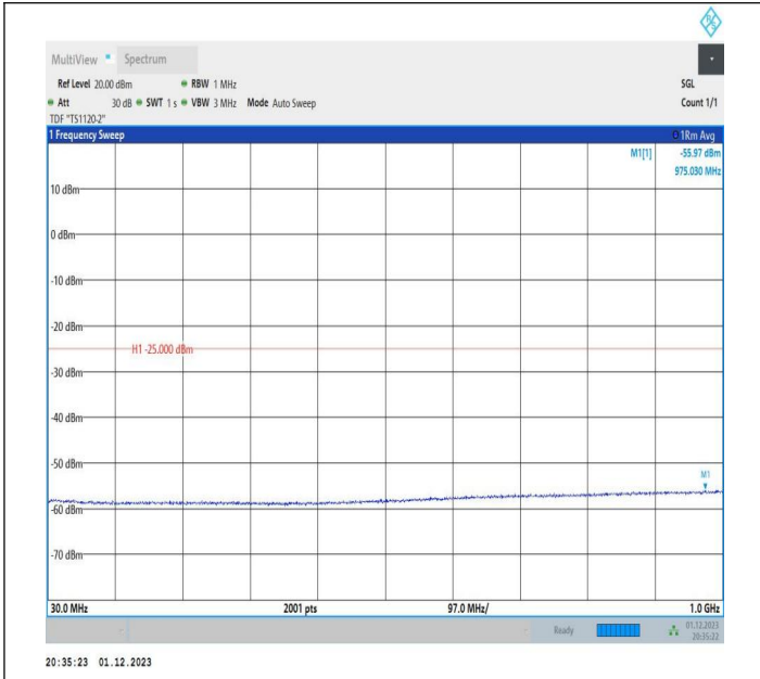
7-7-20MHz-20MHz-64QAM-64QAM-20850-21048-1RB#0-ORB #0-30~1000MHz-PASS
