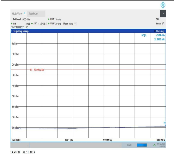
7-7-20MHz-15MHz-64QAM-64QAM-21201-21372-1RB#99-0R B#0-0.15~30MHz-PASS
