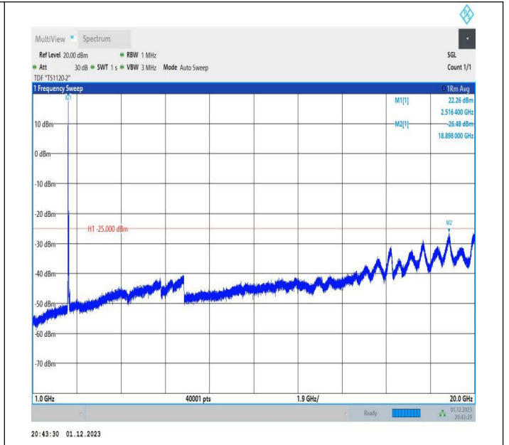
7-7-20MHz-20MHz-64QAM-64QAM-21001-21199-1RB#0-ORB #0-1000~20000MHz-PASS
