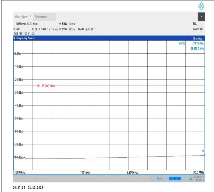
7-7-20MHz-20MHz-64QAM-64QAM-20850-21048-1RB#99-0R B#0-0.15~30MHz-PASS
