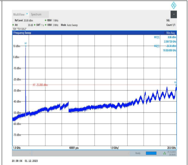
7-7-20MHz-20MHz-QPSK-QPSK-20850-21048-1RB#0-1RB#9 9-1000~20000MHz-PASS
