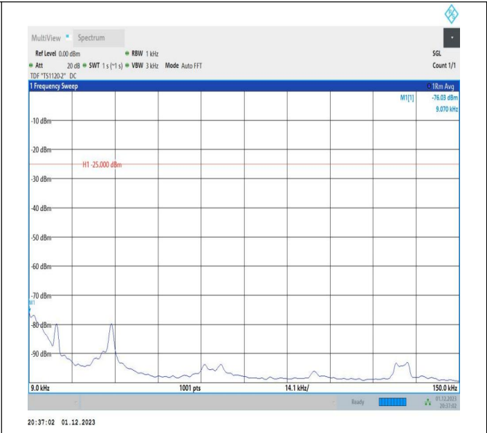
7-7-20MHz-20MHz-64QAM-64QAM-20850-21048-1RB#99-0R B#0-0.009~0.15MHz-PASS
