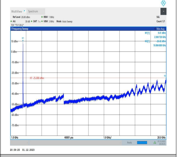
7-7-20MHz-20MHz-64QAM-64QAM-20850-21048-1RB#0-1RB #99-1000~20000MHz-PASS
