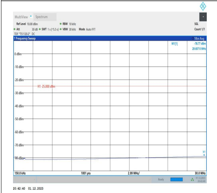
7-7-20MHz-20MHz-16QAM-16QAM-21001-21199-1RB#0-ORB#0-0-0.15~30MHz-PASS
