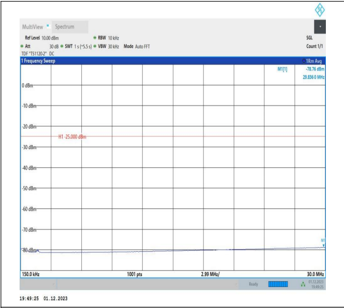
7-7-20MHz-15MHz-64QAM-64QAM-21201-21372-100RB#0-7 5RB#0-0.15~30MHz-PASS
