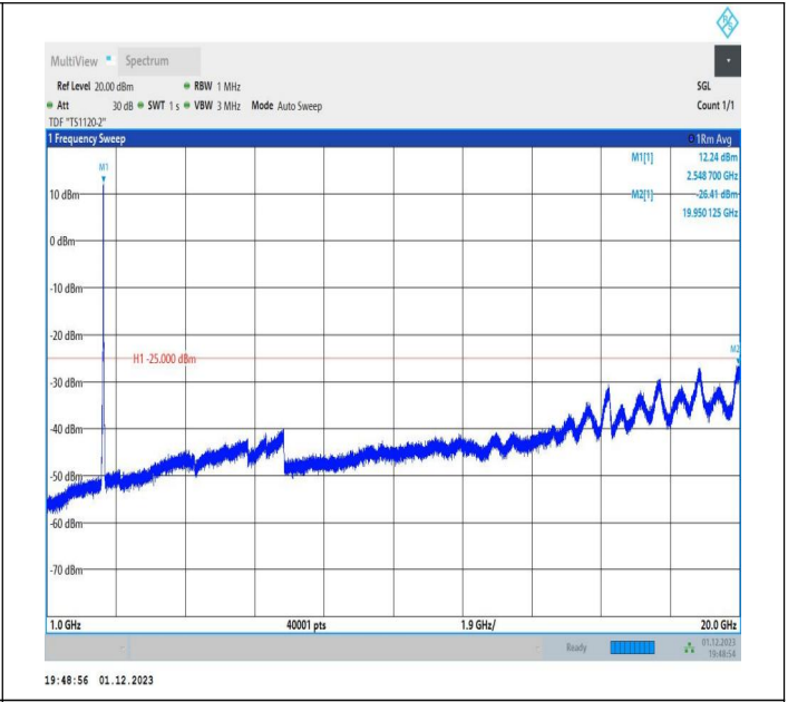
7-7-20MHz-15MHz-16QAM-16QAM-21201-21372-100RB#0-7 5RB#0-1000~20000MHz-PASS
