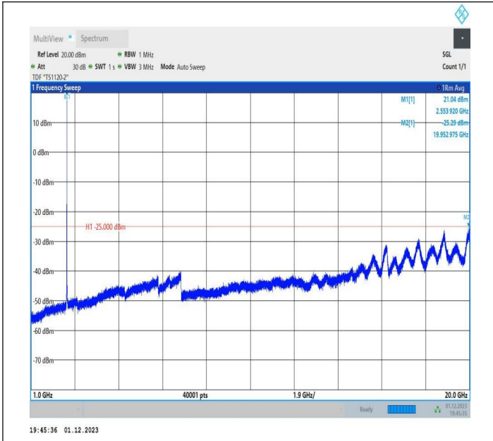
7-7-20MHz-15MHz-64QAM-64QAM-21201-21372-1RB#99-0R B#0-1000~20000MHz-PASS
