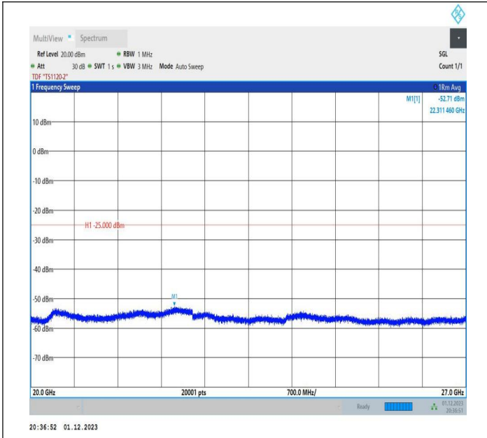
7-7-20MHz-20MHz-16QAM-16QAM-20850-21048-1RB#99-0R B#0-20000~27000MHz-PASS
