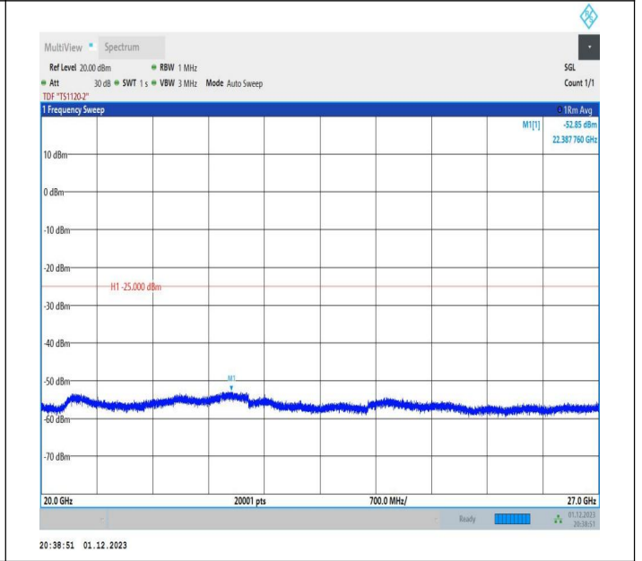
7-7-20MHz-20MHz-16QAM-16QAM-20850-21048-1RB#0-1RB #99-20000~27000MHz-PASS
