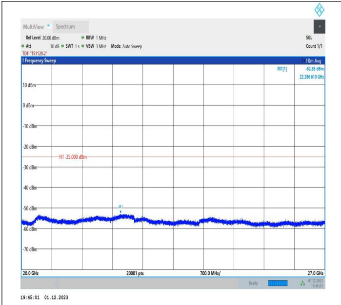
7-7-20MHz-15MHz-16QAM-16QAM-21201-21372-1RB#99-0R B#0-20000~27000MHz-PASS
