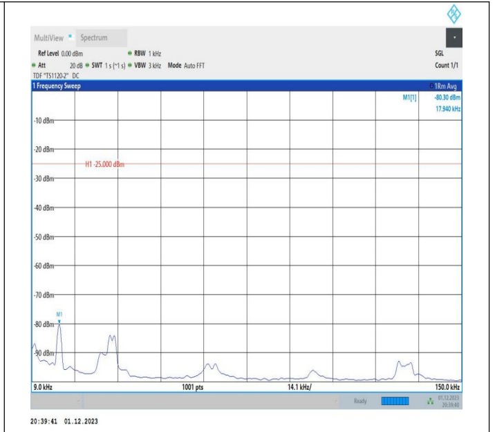
7-7-20MHz-20MHz-QPSK-QPSK-20850-21048-100RB#0-100 RB#0-0.009~0.15MHz-PASS
