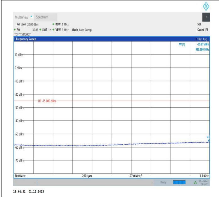
7-7-20MHz-15MHz-16QAM-16QAM-21201-21372-1RB#99-0R B#0-30~1000MHz-PASS
