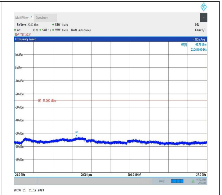
7-7-20MHz-20MHz-64QAM-64QAM-20850-21048-1RB#99-0R B#0-20000~27000MHz-PASS
