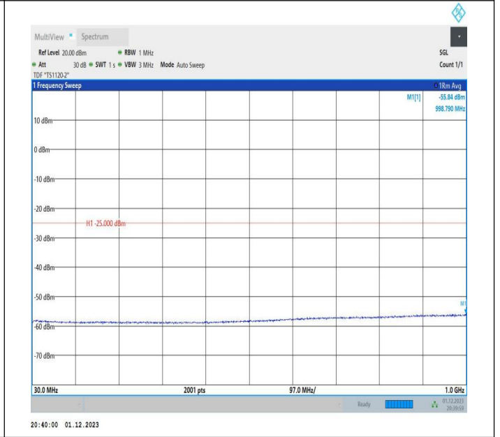
7-7-20MHz-20MHz-QPSK-QPSK-20850-21048-100RB#0-100 RB#0-30~1000MHz-PASS
