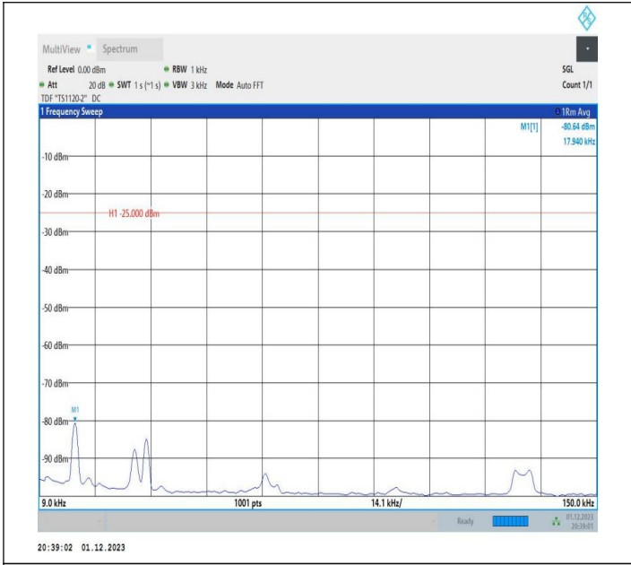
7-7-20MHz-20MHz-64QAM-64QAM-20850-21048-1RB#0-1RB #99-0.009~0.15MHz-PASS
