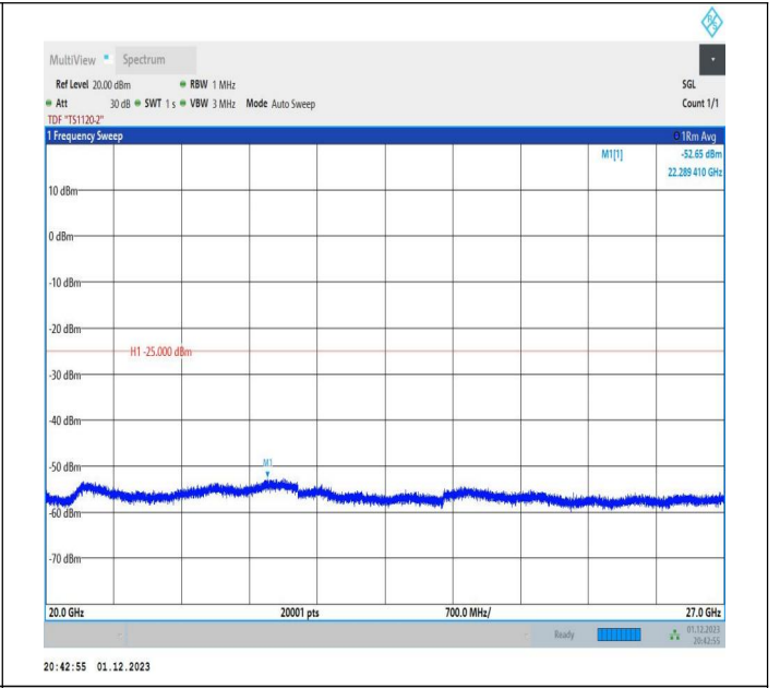
7-7-20MHz-20MHz-16QAM-16QAM-21001-21199-1RB#0-ORB #0-20000~27000MHz-PASS
