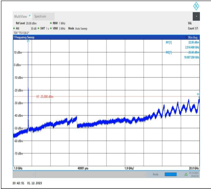
7-7-20MHz-20MHz-16QAM-16QAM-21001-21199-1RB#0-ORB #0-1000~20000MHz-PASS
