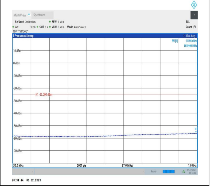
7-7-20MHz-20MHz-16QAM-16QAM-20850-21048-1RB#0-0RB #0-30~1000MHz-PASS
