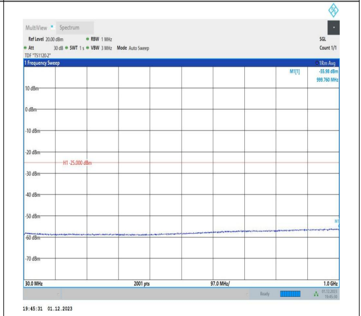
7-7-20MHz-15MHz-64QAM-64QAM-21201-21372-1RB#99-0R B#0-30~1000MHz-PASS
