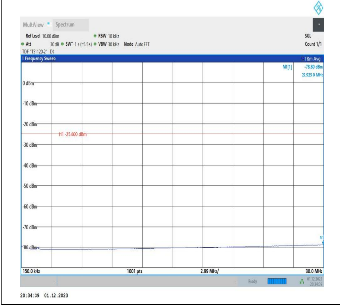
7-7-20MHz-20MHz-16QAM-16QAM-20850-21048-1RB#0-0RB #0-0.15~30MHz-PASS
