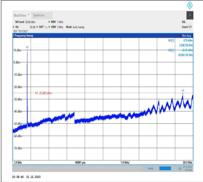
7-7-20MHz-20MHz-16QAM-16QAM-20850-21048-1RB#0-1RB #99-1000~20000MHz-PASS
