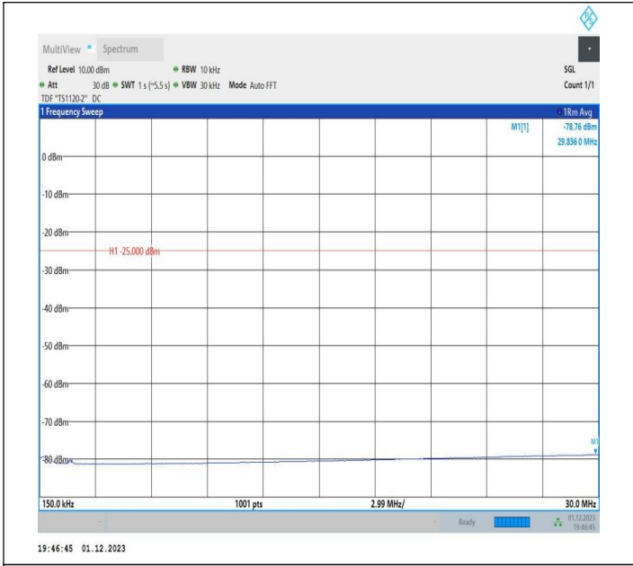
7-7-20MHz-15MHz-16QAM-16QAM-21201-21372-1RB#0-1RB #74-0.15~30MHz-PASS
