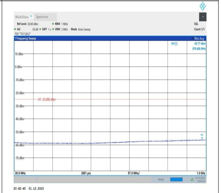
7-7-20MHz-20MHz-16QAM-16QAM-21001-21199-1RB#0-ORB#0-0-30~1000MHz-PASS
