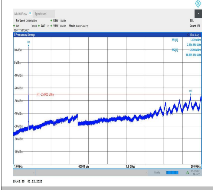
7-7-20MHz-15MHz-16QAM-16QAM-21201-21372-1RB#0-1RB #74-1000~20000MHz-PASS
