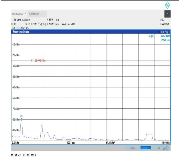
7-7-20MHz-20MHz-QPSK-QPSK-20850-21048-1RB#0-1RB#9 9-0.009~0.15MHz-PASS
