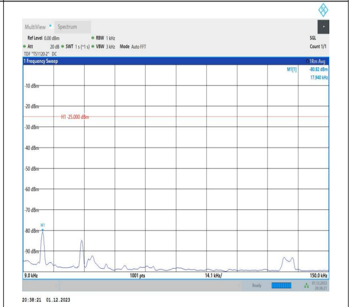
7-7-20MHz-20MHz-16QAM-16QAM-20850-21048-1RB#0-1RB #99-0.009~0.15MHz-PASS
