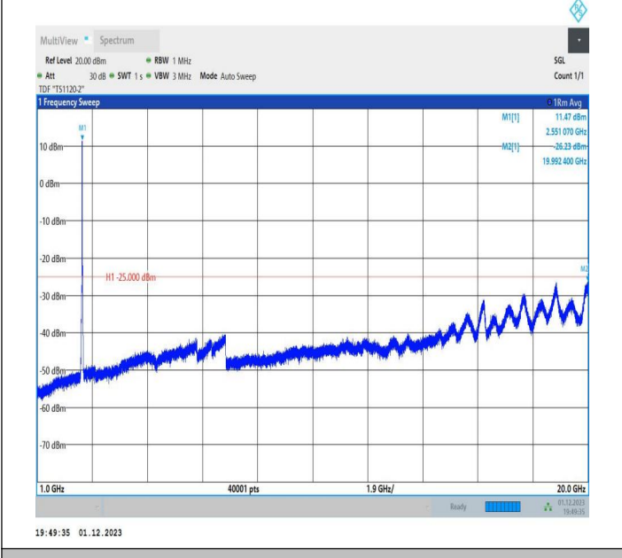
7-7-20MHz-15MHz-64QAM-64QAM-21201-21372-100RB#0-7 5RB#0-1000~20000MHz-PASS
