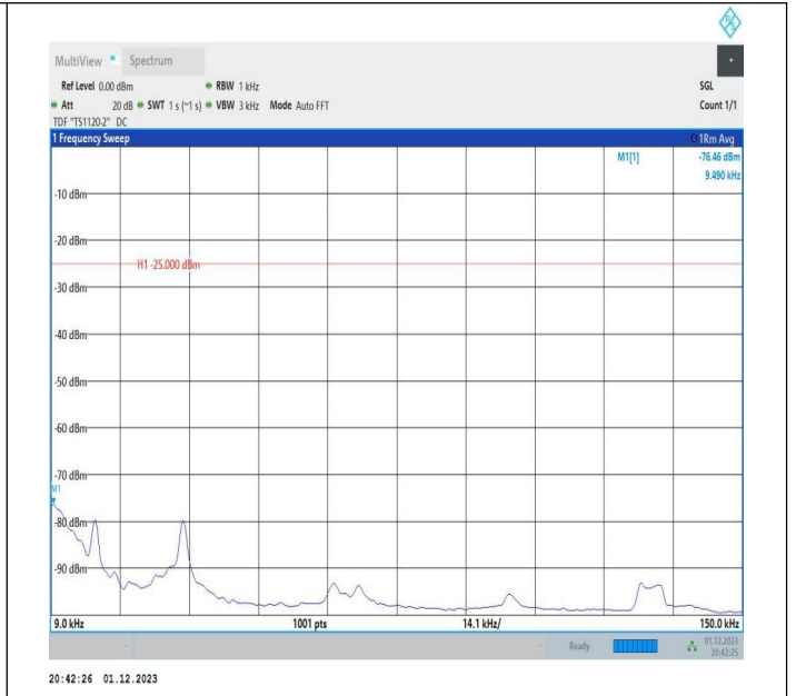
7-7-20MHz-20MHz-16QAM-16QAM-21001-21199-1RB#0-ORB#0-0-0.009~0.15MHz-PASS
