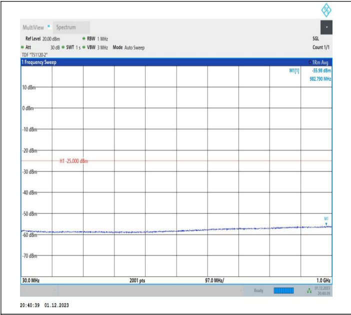
7-7-20MHz-20MHz-16QAM-16QAM-20850-21048-100RB#0-1 00RB#0-30~1000MHz-PASS
