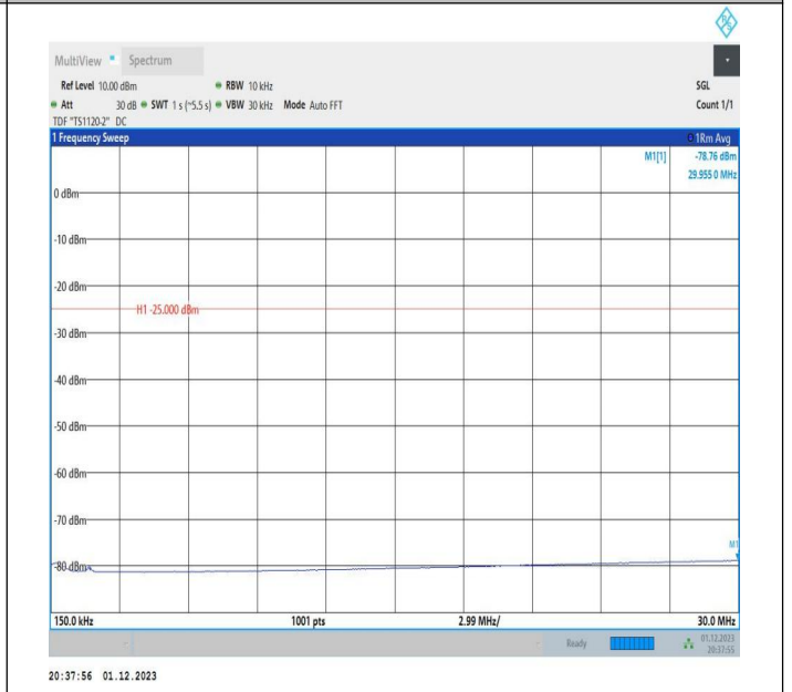
7-7-20MHz-20MHz-QPSK-QPSK-20850-21048-1RB#0-1RB#9 9-0.15~30MHz-PASS
