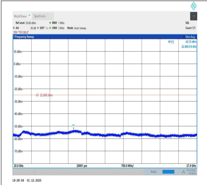
7-7-20MHz-15MHz-16QAM-16QAM-20850-21021-1RB#99-0R B#0-20000~27000MHz-PASS
