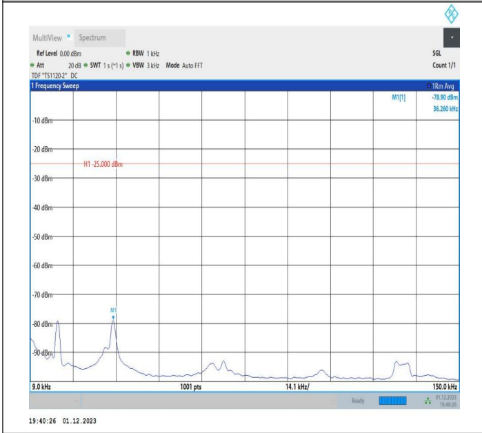
7-7-20MHz-15MHz-16QAM-16QAM-21026-21197-100RB#0-75 RB#0-0.009~0.15MHz-PASS
