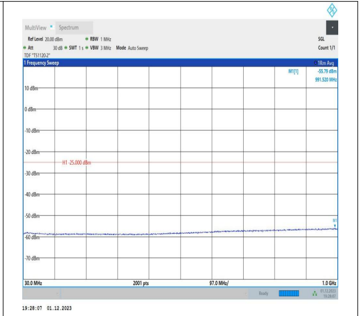
7-7-20MHz-15MHz-QPSK-QPSK-20850-21021-1RB#99-0RB# 0-30~1000MHz-PASS
