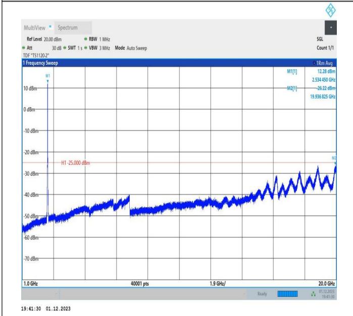
7-7-20MHz-15MHz-64QAM-64QAM-21026-21197-100RB#0-75 RB#0-1000~20000MHz-PASS
