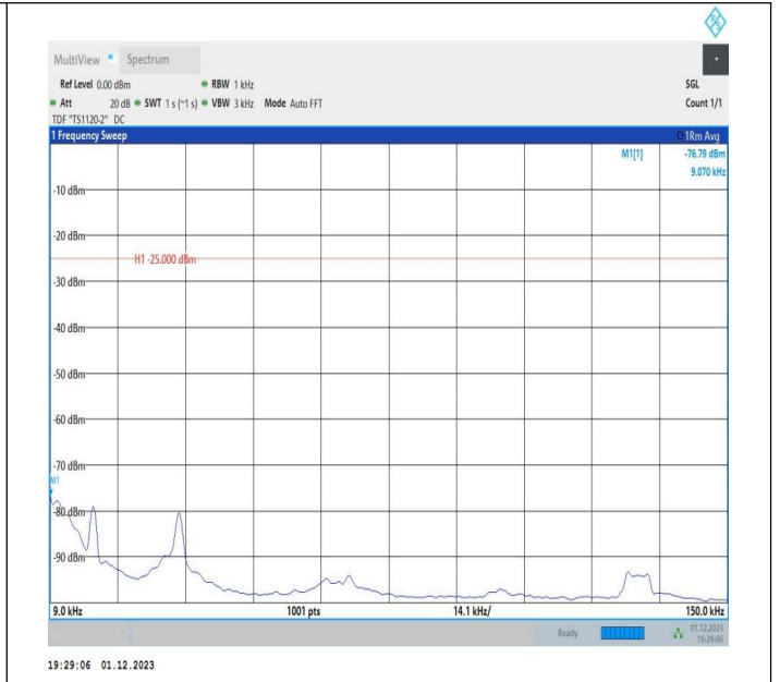
7-7-20MHz-15MHz-64QAM-64QAM-20850-21021-1RB#99-0R B#0-0.009~0.15MHz-PASS
