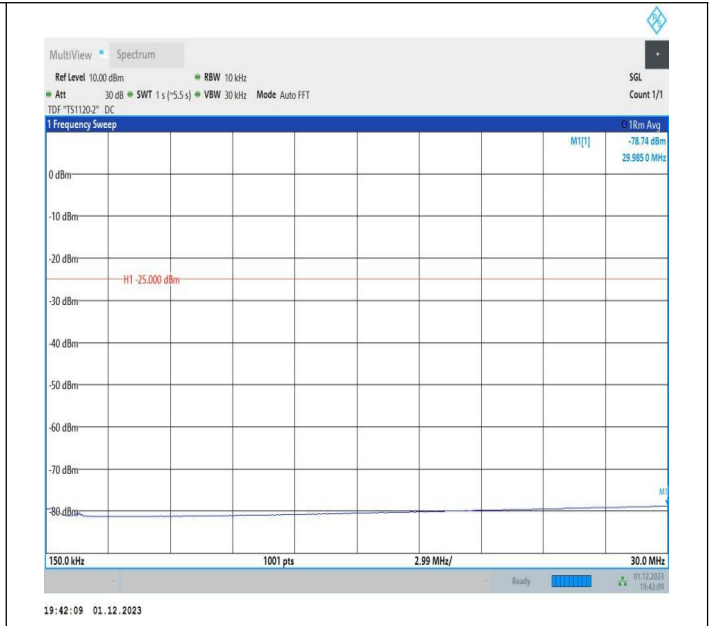
7-7-20MHz-15MHz-QPSK-QPSK-21201-21372-1RB#0-0RB#0 -0.15~30MHz-PASS
