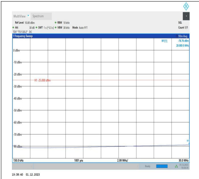
7-7-20MHz-15MHz-16QAM-16QAM-21026-21197-1RB#0-1RB #74-0.15~30MHz-PASS
