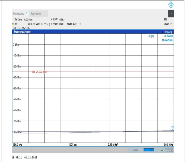
7-7-20MHz-15MHz-64QAM-64QAM-21026-21197-1RB#0-ORB #0-0.15~30MHz-PASS
