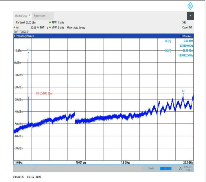
7-7-20MHz-15MHz-64QAM-64QAM-20850-21021-1RB#0-1RB #74-1000~20000MHz-PASS
