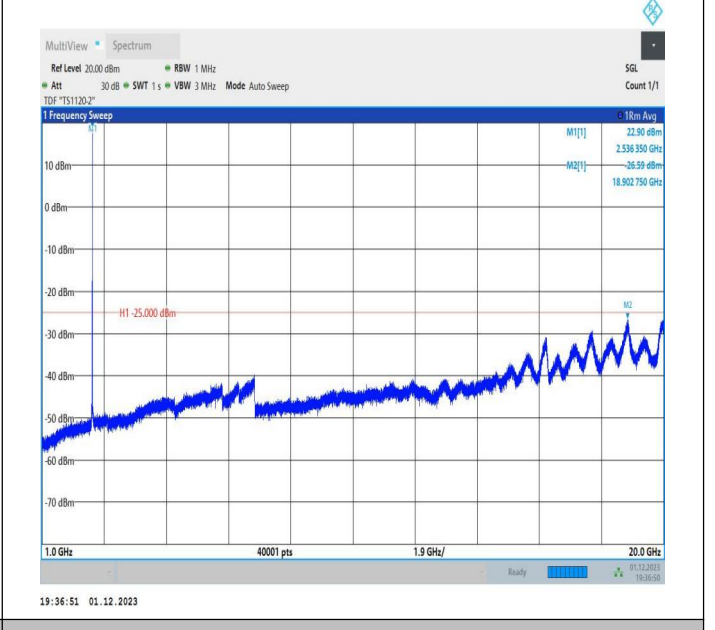
7-7-20MHz-15MHz-16QAM-16QAM-21026-21197-1RB#99-0R B#0-1000~20000MHz-PASS
