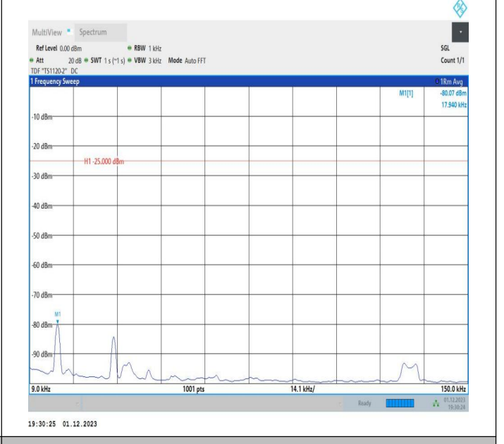
7-7-20MHz-15MHz-16QAM-16QAM-20850-21021-1RB#0-1RB#7 #74-0.009~0.15MHz-PASS
