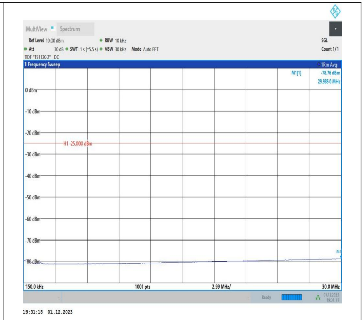
7-7-20MHz-15MHz-64QAM-64QAM-20850-21021-1RB#0-1RB #74-0.15~30MHz-PASS
