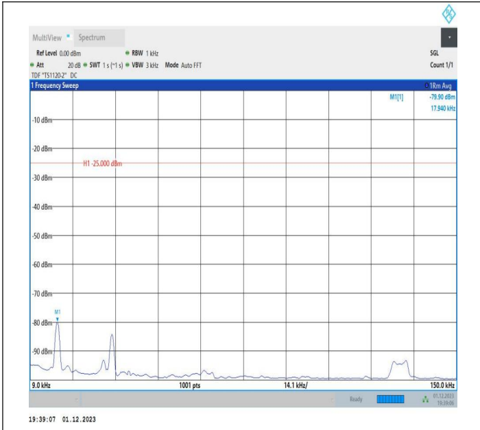
7-7-20MHz-15MHz-64QAM-64QAM-21026-21197-1RB#0-1RB #74-0.009~0.15MHz-PASS
