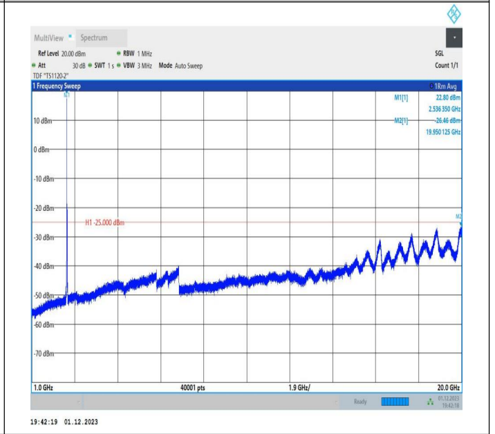
7-7-20MHz-15MHz-QPSK-QPSK-21201-21372-1RB#0-0RB#0 -1000~20000MHz-PASS
