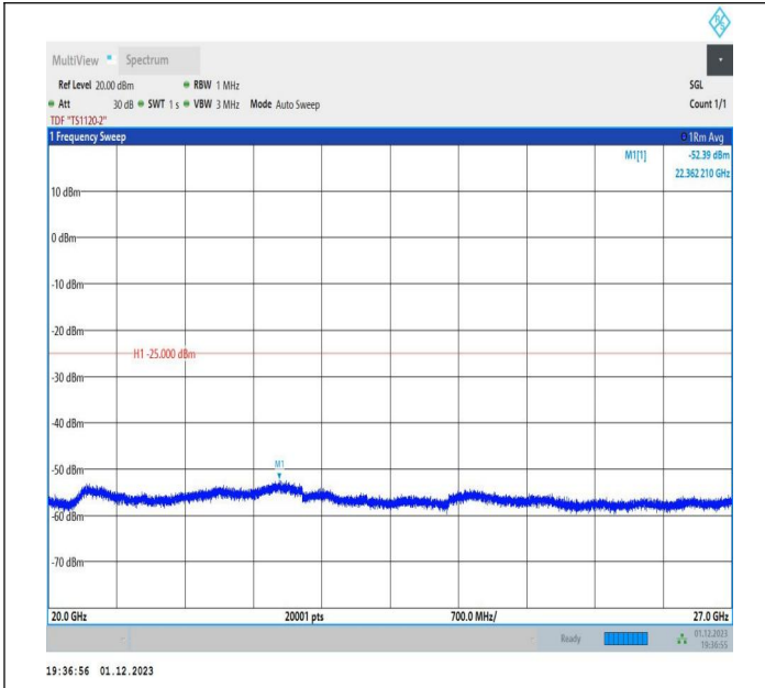
7-7-20MHz-15MHz-16QAM-16QAM-21026-21197-1RB#99-0R B#0-20000~27000MHz-PASS
