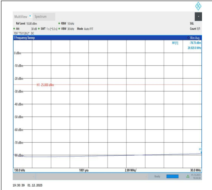
7-7-20MHz-15MHz-16QAM-16QAM-20850-21021-1RB#0-1RB #74-0.15~30MHz-PASS
