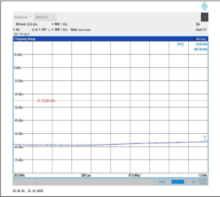
7-7-20MHz-15MHz-16QAM-16QAM-20850-21021-100RB#0-7 5RB#0-30~1000MHz-PASS
