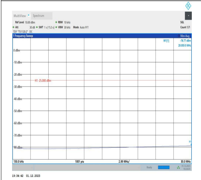
7-7-20MHz-15MHz-16QAM-16QAM-21026-21197-1RB#0-ORB#0-0.15~30MHz-PASS
