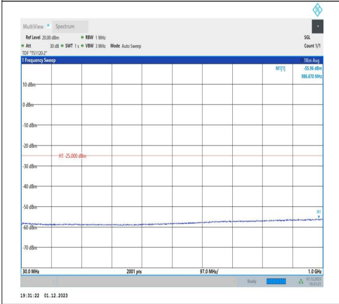
7-7-20MHz-15MHz-64QAM-64QAM-20850-21021-1RB#0-1RB #74-30~1000MHz-PASS
