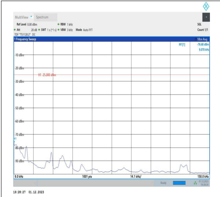
7-7-20MHz-15MHz-16QAM-16QAM-20850-21021-1RB#99-OR B#0-0.009~0.15MHz-PASS
