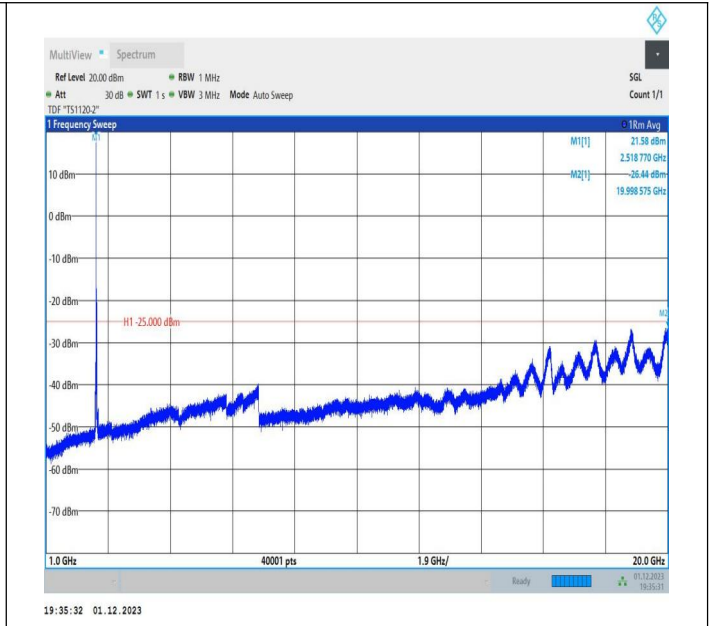
7-7-20MHz-15MHz-64QAM-64QAM-21026-21197-1RB#0-ORB #0-1000~20000MHz-PASS
