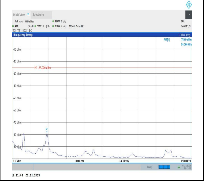
7-7-20MHz-15MHz-64QAM-64QAM-21026-21197-100RB#0-75 RB#0-0.009~0.15MHz-PASS
