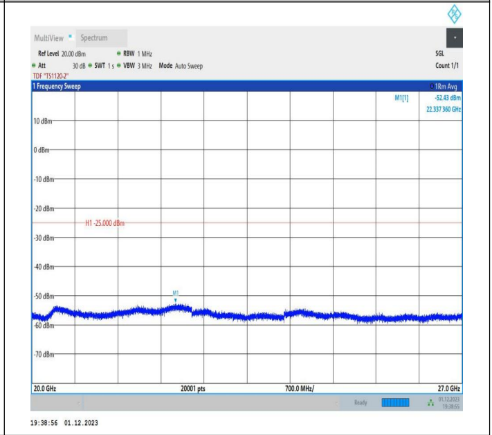
7-7-20MHz-15MHz-16QAM-16QAM-21026-21197-1RB#0-1RB #74-20000~27000MHz-PASS
