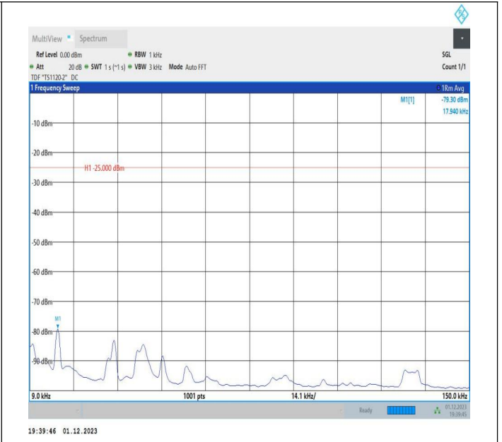
7-7-20MHz-15MHz-QPSK-QPSK-21026-21197-100RB#0-75R B#0-0.009~0.15MHz-PASS
