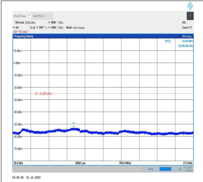
7-7-20MHz-15MHz-64QAM-64QAM-21026-21197-1RB#0-1RB #74-20000~27000MHz-PASS
