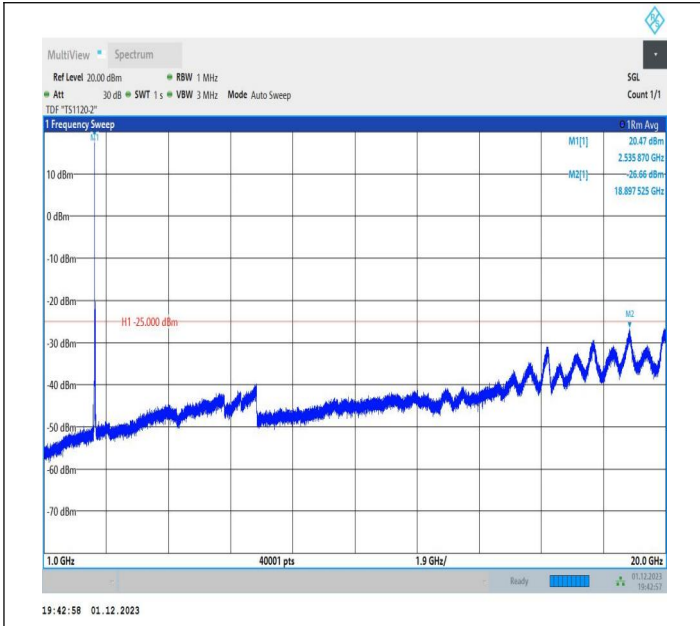
7-7-20MHz-15MHz-16QAM-16QAM-21201-21372-1RB#0-ORB #0-1000~20000MHz-PASS
