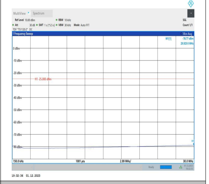
7-7-20MHz-15MHz-16QAM-16QAM-20850-21021-100RB#0-7 5RB#0-0.15~30MHz-PASS
