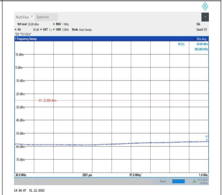
7-7-20MHz-15MHz-16QAM-16QAM-21026-21197-1RB#0-ORB#0-30~1000MHz-PASS
