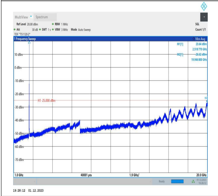
7-7-20MHz-15MHz-QPSK-QPSK-20850-21021-1RB#99-0RB# 0-1000~20000MHz-PASS
