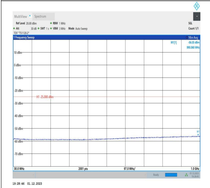
7-7-20MHz-15MHz-16QAM-16QAM-20850-21021-1RB#99-OR B#0-30~1000MHz-PASS
