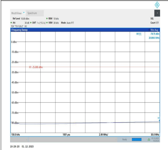
7-7-20MHz-15MHz-64QAM-64QAM-20850-21021-1RB#99-0R B#0-0.15~30MHz-PASS
