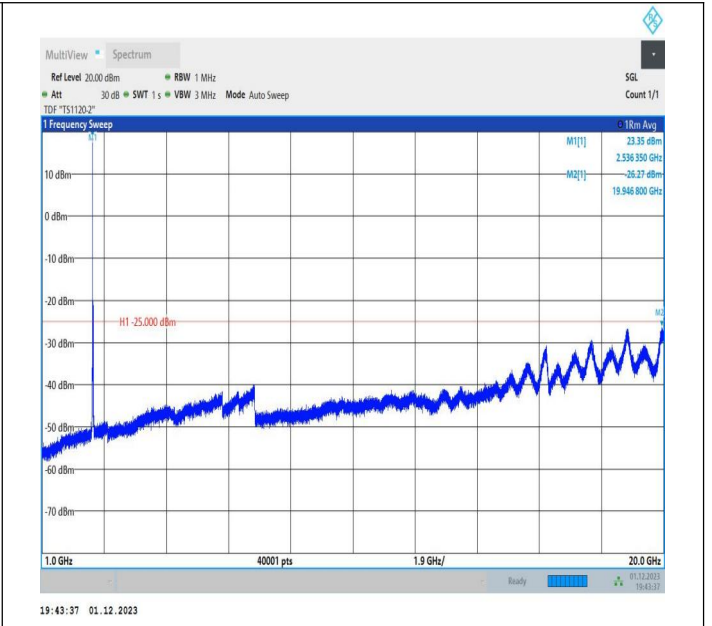
7-7-20MHz-15MHz-64QAM-64QAM-21201-21372-1RB#0-ORB #0-1000~20000MHz-PASS
