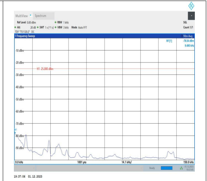
7-7-20MHz-15MHz-64QAM-64QAM-21026-21197-1RB#99-0R B#0-0.009~0.15MHz-PASS
