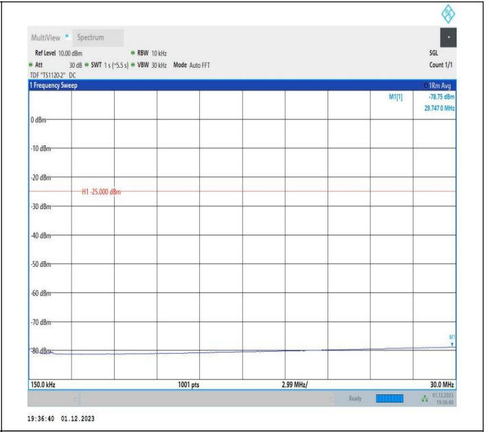
7-7-20MHz-15MHz-16QAM-16QAM-21026-21197-1RB#99-0R B#0-0.15~30MHz-PASS
