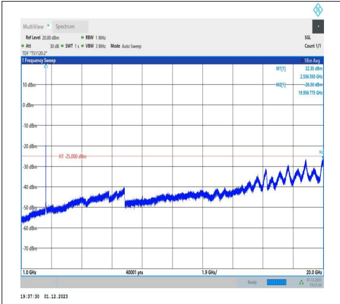
7-7-20MHz-15MHz-64QAM-64QAM-21026-21197-1RB#99-0R B#0-1000~20000MHz-PASS
