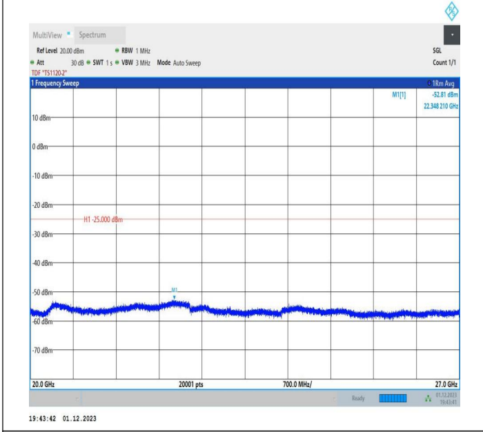
7-7-20MHz-15MHz-64QAM-64QAM-21201-21372-1RB#0-ORB #0-20000~27000MHz-PASS
