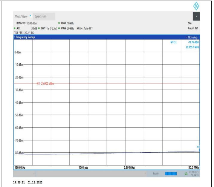
7-7-20MHz-15MHz-64QAM-64QAM-21026-21197-1RB#0-1RB #74-0.15~30MHz-PASS
