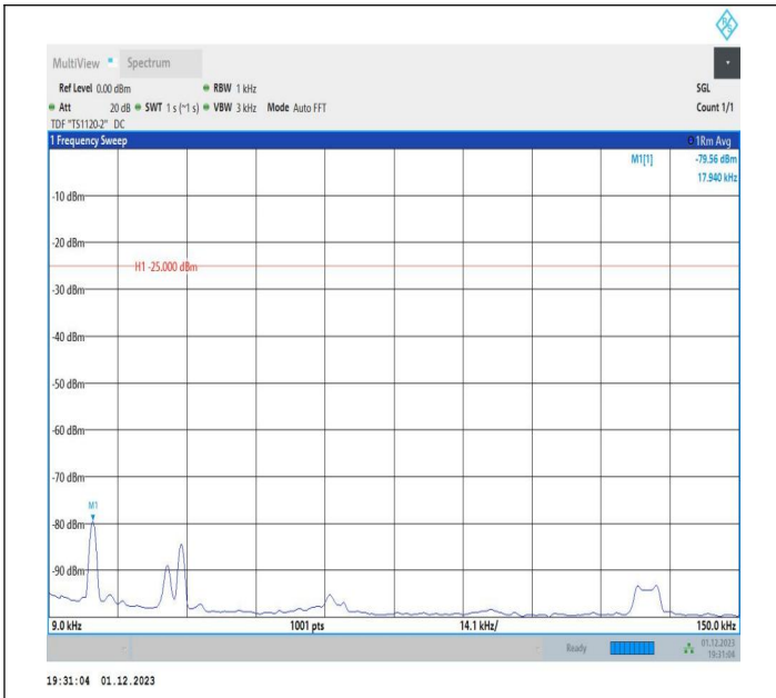
7-7-20MHz-15MHz-64QAM-64QAM-20850-21021-1RB#0-1RB #74-0.009~0.15MHz-PASS
