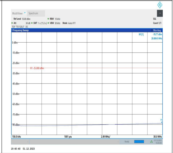
7-7-20MHz-15MHz-16QAM-16QAM-21026-21197-100RB#0-75 RB#0-0.15~30MHz-PASS
