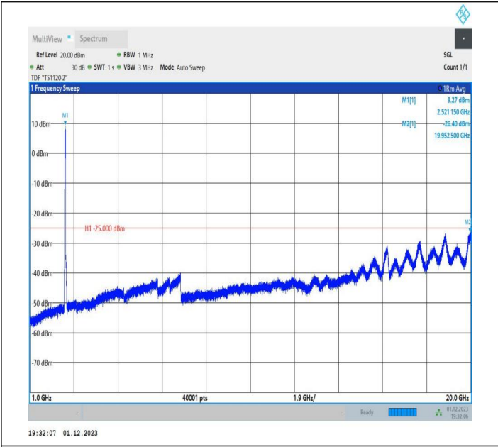
7-7-20MHz-15MHz-QPSK-QPSK-20850-21021-100RB#0-75R B#0-1000~20000MHz-PASS
