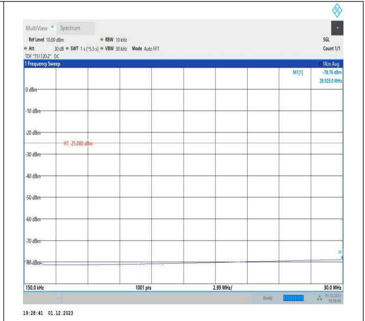
7-7-20MHz-15MHz-16QAM-16QAM-20850-21021-1RB#99-OR B#0-0.15~30MHz-PASS
