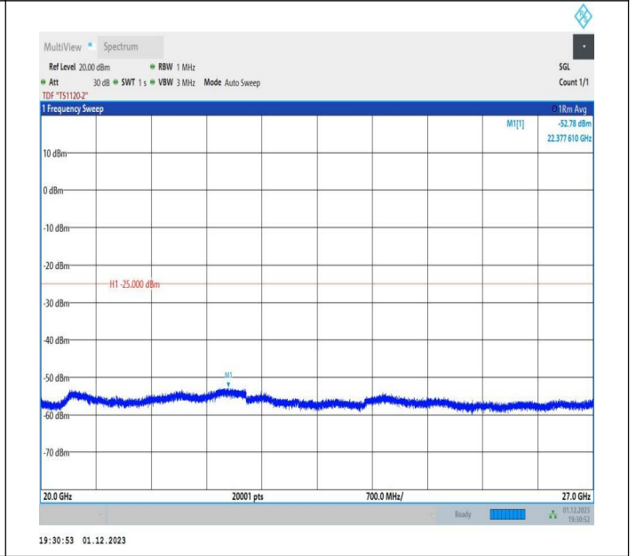
7-7-20MHz-15MHz-16QAM-16QAM-20850-21021-1RB#0-1RB #74-20000~27000MHz-PASS
