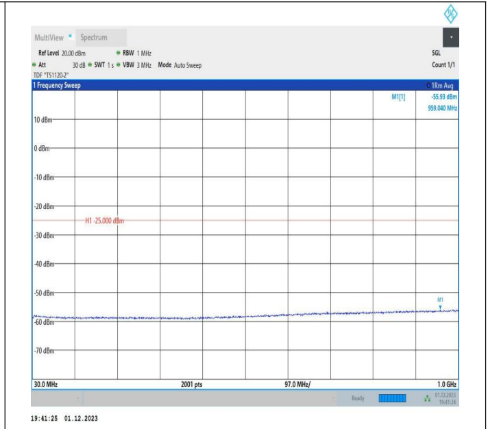
7-7-20MHz-15MHz-64QAM-64QAM-21026-21197-100RB#0-75 RB#0-30~1000MHz-PASS
