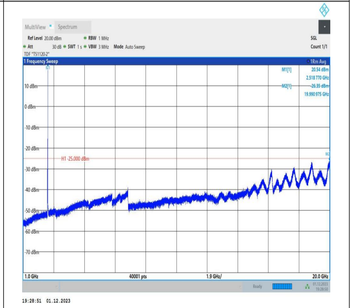
7-7-20MHz-15MHz-16QAM-16QAM-20850-21021-1RB#99-OR B#0-1000~20000MHz-PASS
