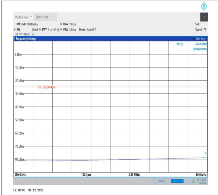
7-7-20MHz-15MHz-QPSK-QPSK-20850-21021-1RB#99-0RB# 0-0.15~30MHz-PASS
