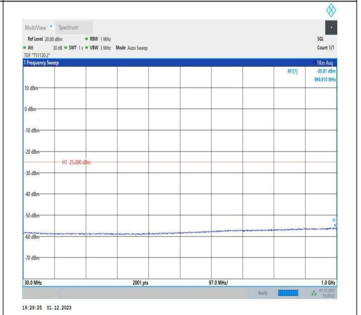
7-7-20MHz-15MHz-64QAM-64QAM-20850-21021-1RB#99-0R B#0-30~1000MHz-PASS
