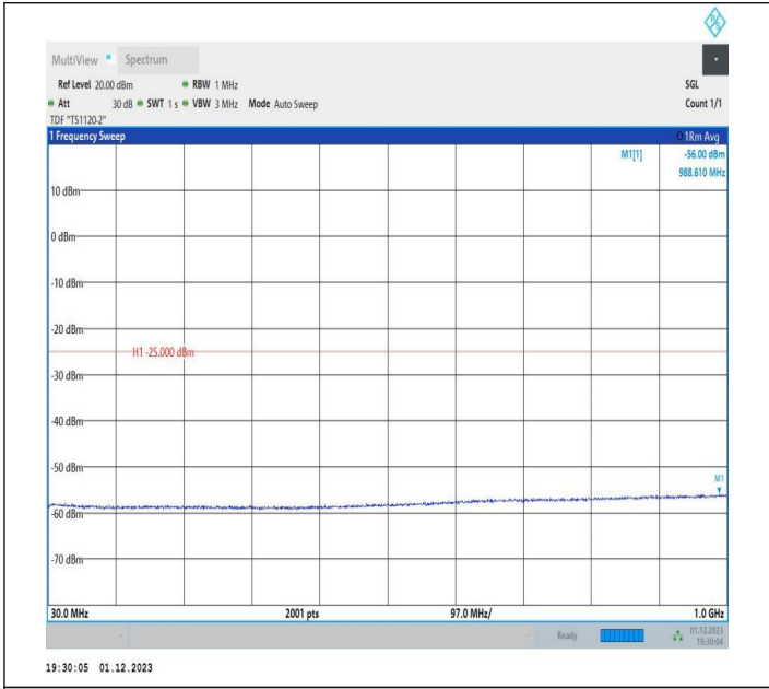
7-7-20MHz-15MHz-QPSK-QPSK-20850-21021-1RB#0-1RB#7 4-30~1000MHz-PASS
