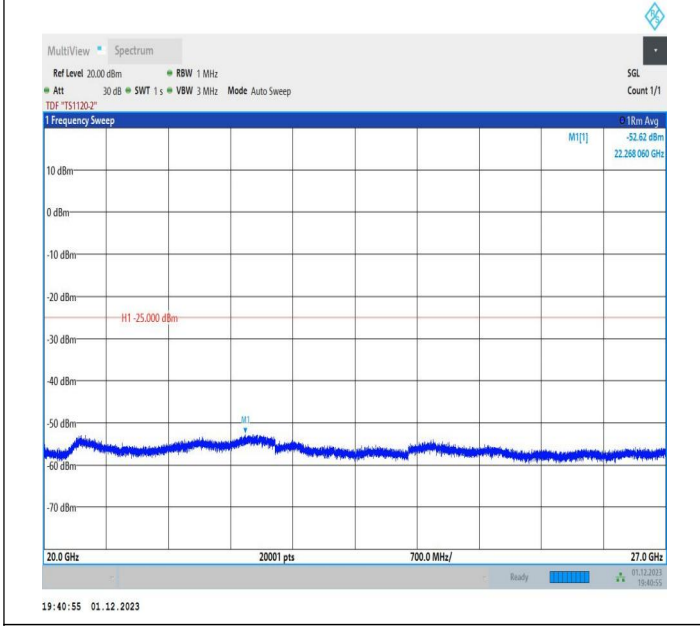
7-7-20MHz-15MHz-16QAM-16QAM-21026-21197-100RB#0-75 RB#0-20000~27000MHz-PASS
