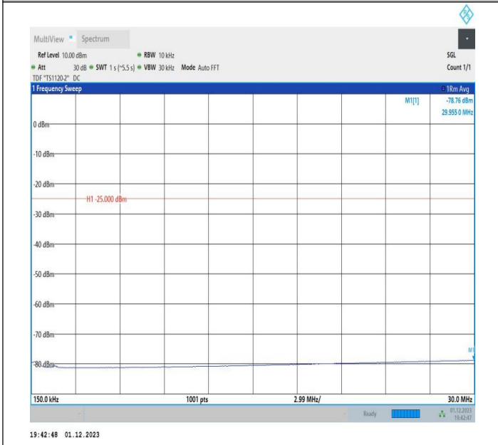
7-7-20MHz-15MHz-16QAM-16QAM-21201-21372-1RB#0-0RB #0-0.15~30MHz-PASS
