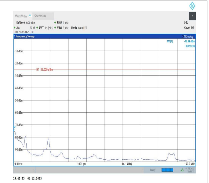
7-7-20MHz-15MHz-16QAM-16QAM-21201-21372-1RB#0-0RB #0-0.009~0.15MHz-PASS
