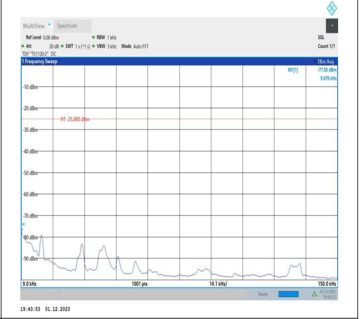
7-7-20MHz-15MHz-QPSK-QPSK-21201-21372-1RB#99-ORB# 0-0.009~0.15MHz-PASS
