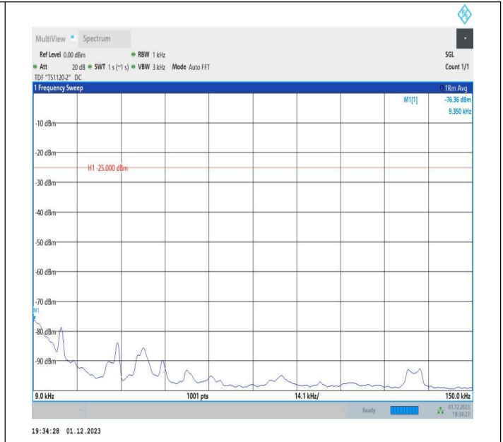
7-7-20MHz-15MHz-16QAM-16QAM-21026-21197-1RB#0-ORB#0-0.009~0.15MHz-PASS
