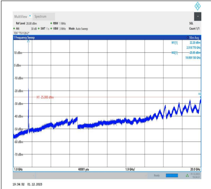
7-7-20MHz-15MHz-16QAM-16QAM-21026-21197-1RB#0-ORB #0-1000~20000MHz-PASS
