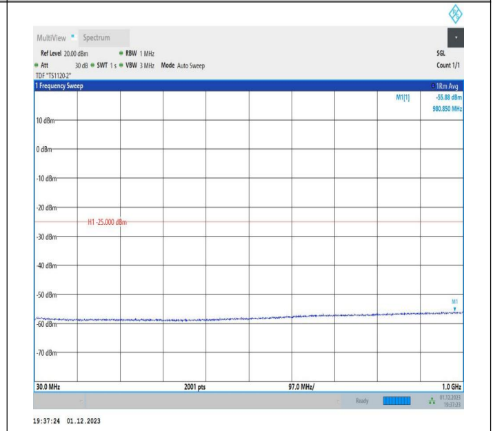
7-7-20MHz-15MHz-64QAM-64QAM-21026-21197-1RB#99-0R B#0-30~1000MHz-PASS
