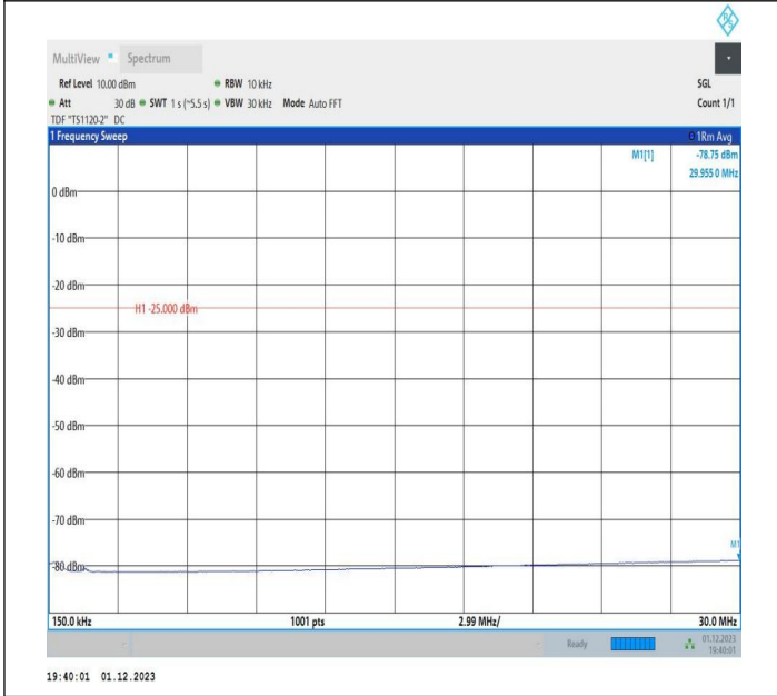
7-7-20MHz-15MHz-QPSK-QPSK-21026-21197-100RB#0-75R B#0-0.15~30MHz-PASS
