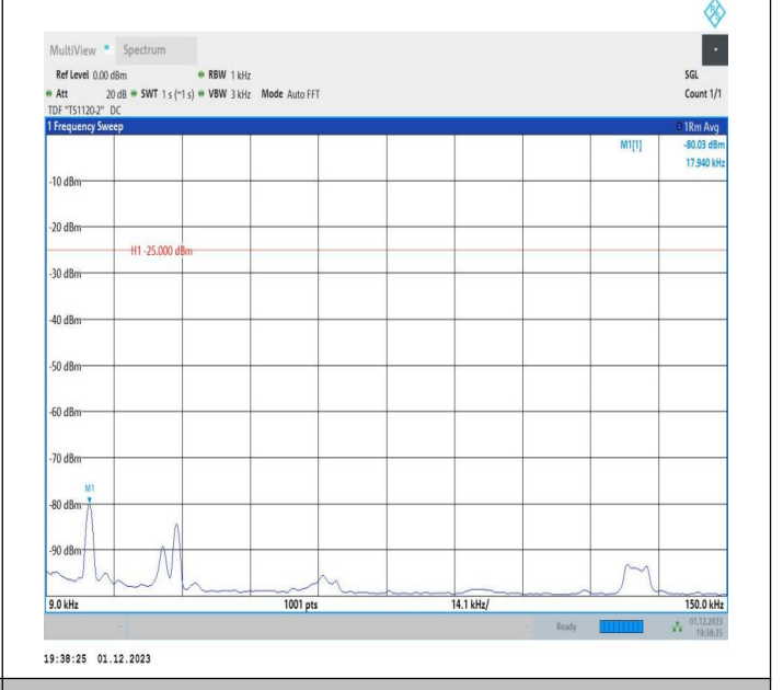
7-7-20MHz-15MHz-16QAM-16QAM-21026-21197-1RB#0-1RB #74-0.009~0.15MHz-PASS
