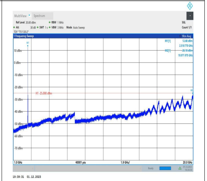
7-7-20MHz-15MHz-64QAM-64QAM-21026-21197-1RB#0-1RB #74-1000~20000MHz-PASS
