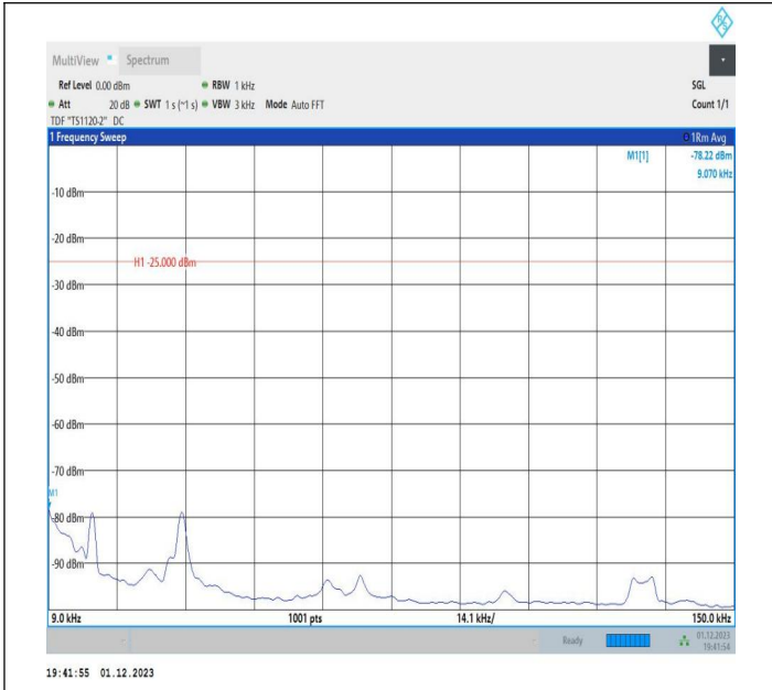
7-7-20MHz-15MHz-QPSK-QPSK-21201-21372-1RB#0-0RB#0 -0.009~0.15MHz-PASS
