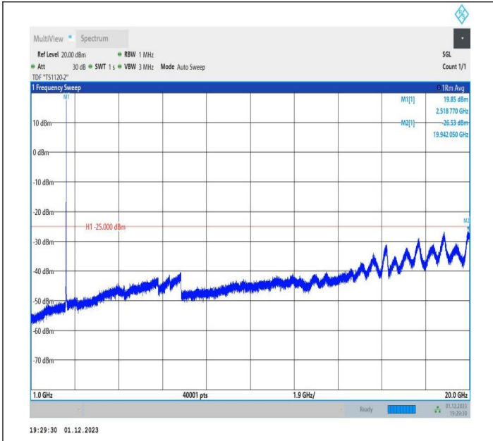
7-7-20MHz-15MHz-64QAM-64QAM-20850-21021-1RB#99-0R B#0-1000~20000MHz-PASS
