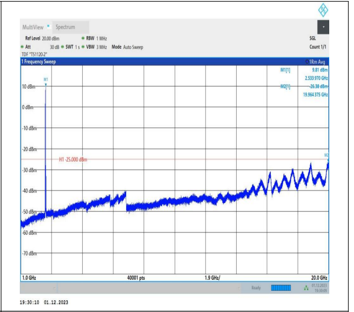
7-7-20MHz-15MHz-QPSK-QPSK-20850-21021-1RB#0-1RB#7 4-1000~20000MHz-PASS
