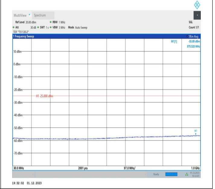
7-7-20MHz-15MHz-QPSK-QPSK-20850-21021-100RB#0-75R B#0-30~1000MHz-PASS
