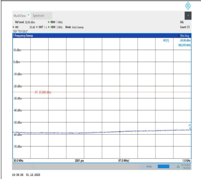
7-7-20MHz-15MHz-64QAM-64QAM-21026-21197-1RB#0-1RB #74-30~1000MHz-PASS
