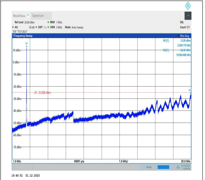
7-7-20MHz-15MHz-16QAM-16QAM-21026-21197-100RB#0-75 RB#0-1000~20000MHz-PASS
