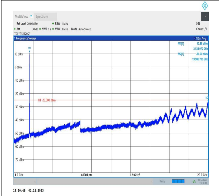
7-7-20MHz-15MHz-16QAM-16QAM-20850-21021-1RB#0-1RB #74-1000~20000MHz-PASS
