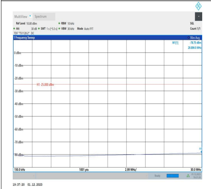
7-7-20MHz-15MHz-64QAM-64QAM-21026-21197-1RB#99-0R B#0-0.15~30MHz-PASS
