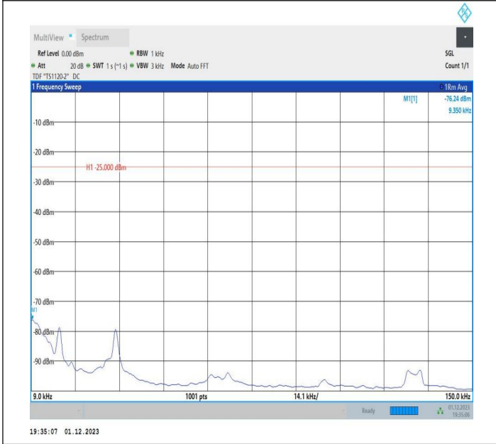
7-7-20MHz-15MHz-64QAM-64QAM-21026-21197-1RB#0-ORB #0-0.009~0.15MHz-PASS
