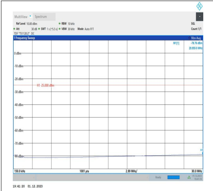
7-7-20MHz-15MHz-64QAM-64QAM-21026-21197-100RB#0-75 RB#0-0.15~30MHz-PASS
