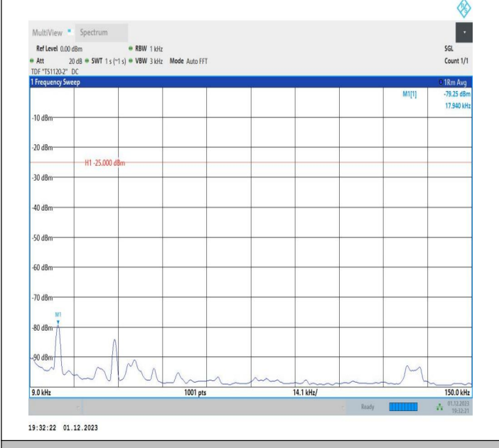
7-7-20MHz-15MHz-16QAM-16QAM-20850-21021-100RB#0-7 5RB#0-0.009~0.15MHz-PASS
