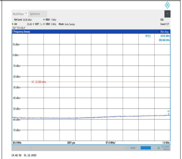
7-7-20MHz-15MHz-16QAM-16QAM-21201-21372-1RB#0-0RB #0-30~1000MHz-PASS
