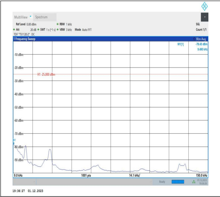
7-7-20MHz-15MHz-16QAM-16QAM-21026-21197-1RB#99-0R B#0-0.009~0.15MHz-PASS
