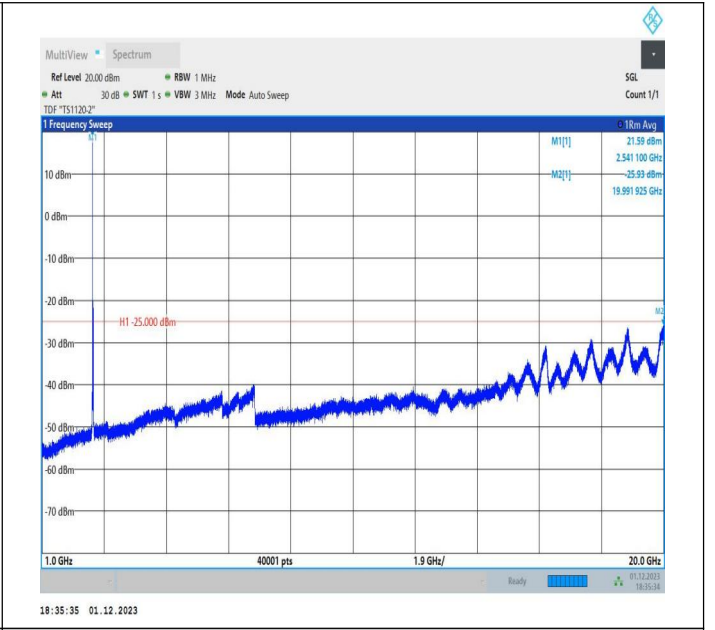
7-7-20MHz-10MHz-64QAM-64QAM-21251-21395-1RB#0-ORB #0-1000~20000MHz-PASS
