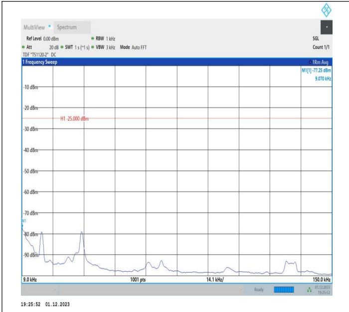
7-7-20MHz-15MHz-QPSK-QPSK-20850-21021-1RB#0-0RB#0 -0.009~0.15MHz-PASS
