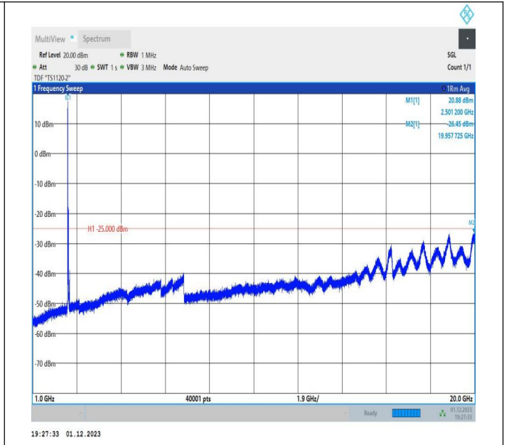
7-7-20MHz-15MHz-64QAM-64QAM-20850-21021-1RB#0-ORB #0-1000~20000MHz-PASS
