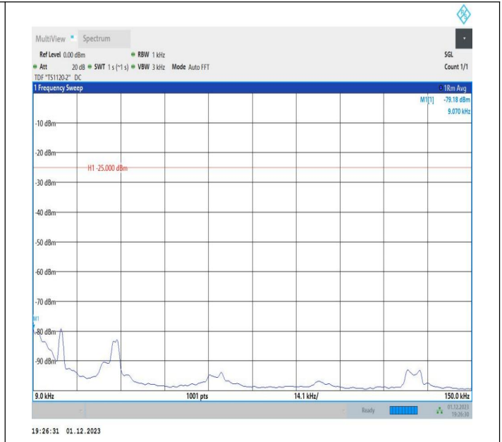
7-7-20MHz-15MHz-16QAM-16QAM-20850-21021-1RB#0-0RB #0-0.009~0.15MHz-PASS
