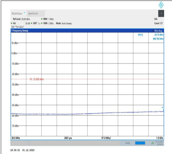
7-7-20MHz-10MHz-QPSK-QPSK-21051-21195-1RB#0-1RB#4 9-30~1000MHz-PASS
