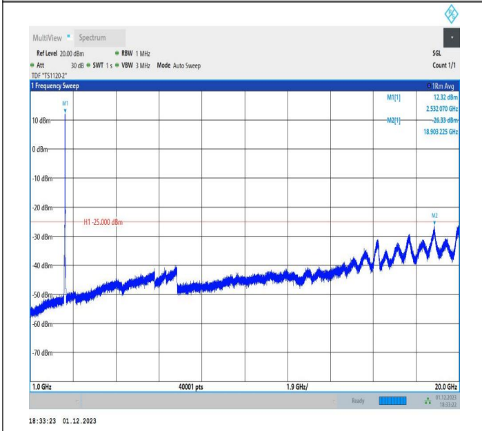
7-7-20MHz-10MHz-64QAM-64QAM-21051-21195-100RB#0-50 RB#0-1000~20000MHz-PASS
