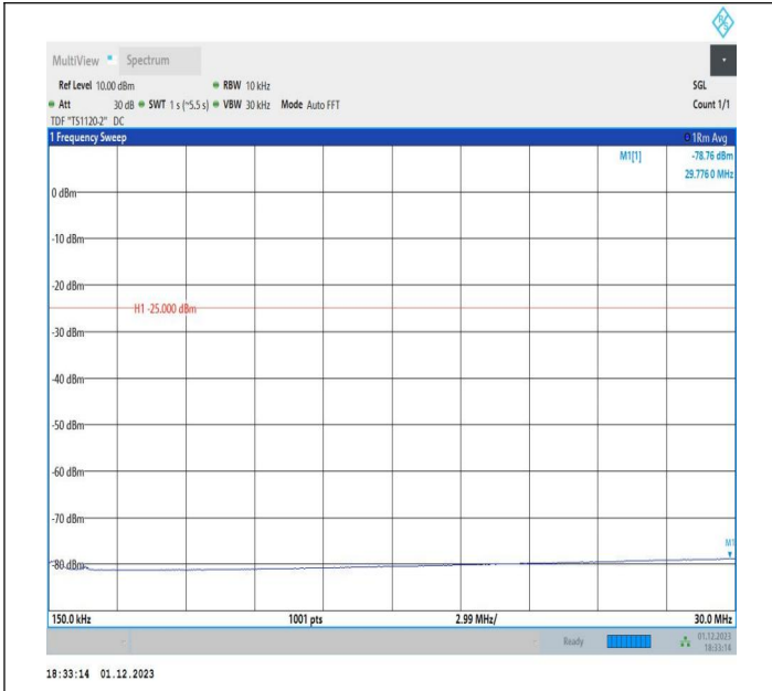
7-7-20MHz-10MHz-64QAM-64QAM-21051-21195-100RB#0-50 RB#0-0.15~30MHz-PASS
