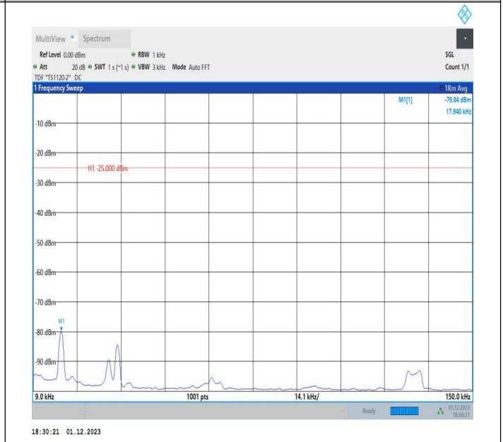
7-7-20MHz-10MHz-16QAM-16QAM-21051-21195-1RB#0-1RB #49-0.009~0.15MHz-PASS
