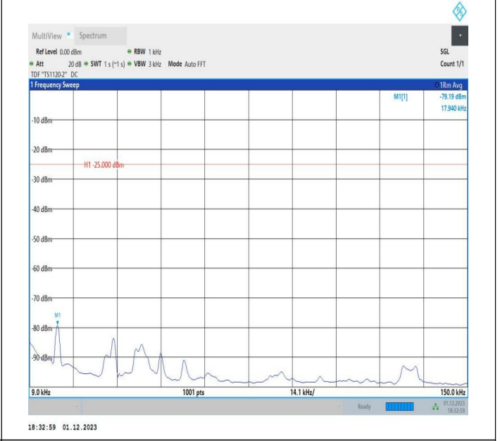
7-7-20MHz-10MHz-64QAM-64QAM-21051-21195-100RB#0-50 RB#0-0.009~0.15MHz-PASS
