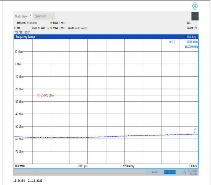
7-7-20MHz-15MHz-16QAM-16QAM-20850-21021-1RB#0-0RB #0-30~1000MHz-PASS
