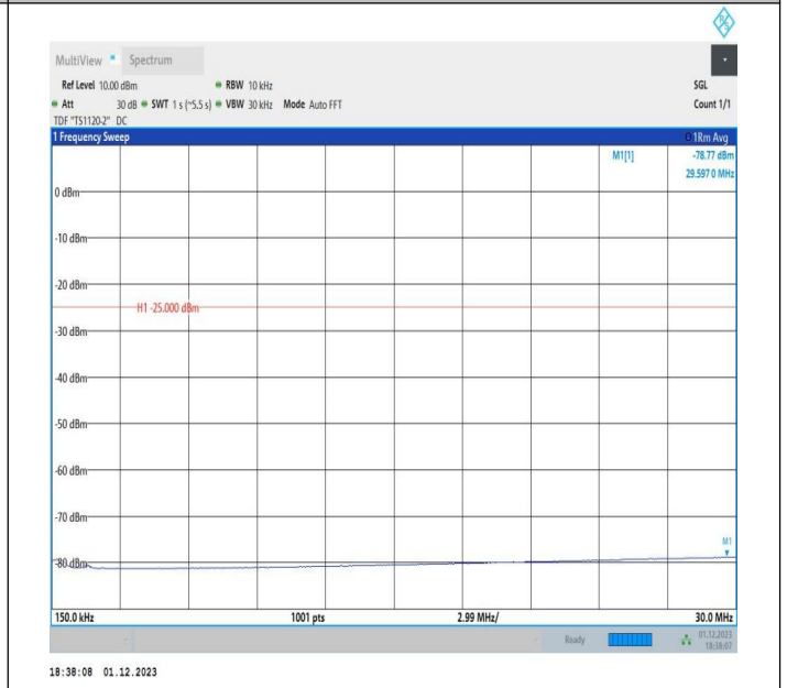
7-7-20MHz-10MHz-QPSK-QPSK-21251-21395-1RB#0-1RB#4 9-0.15~30MHz-PASS
