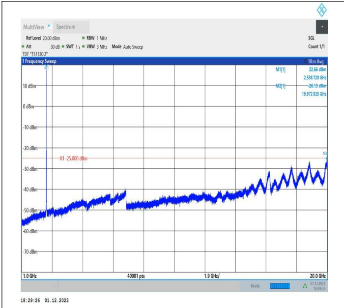
7-7-20MHz-10MHz-64QAM-64QAM-21051-21195-1RB#99-0R B#0-1000~20000MHz-PASS
