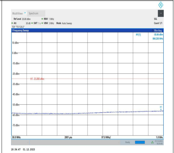
7-7-20MHz-10MHz-16QAM-16QAM-21251-21395-1RB#0-0RB #0-30~1000MHz-PASS
