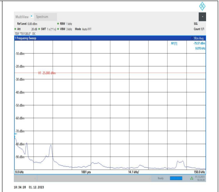
7-7-20MHz-10MHz-16QAM-16QAM-21251-21395-1RB#0-0RB #0-0.009~0.15MHz-PASS
