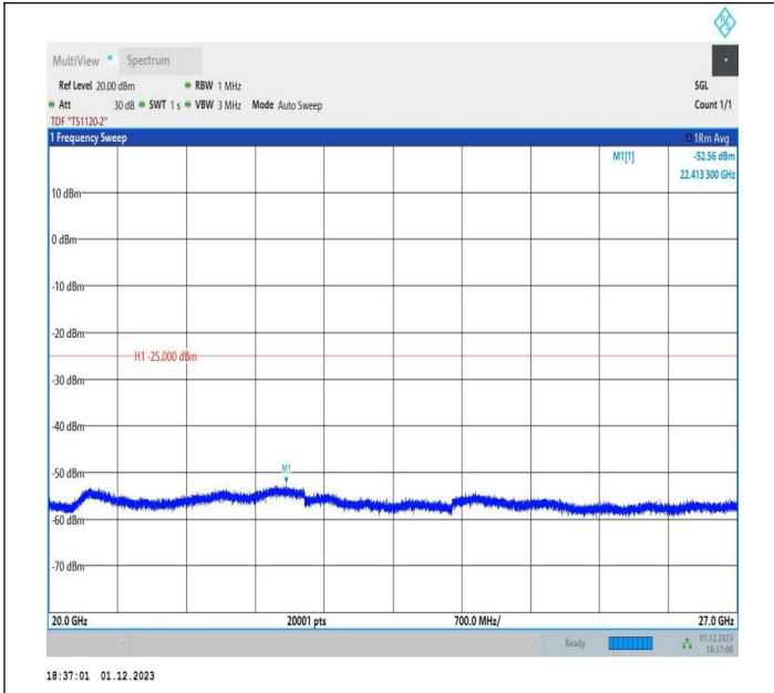
7-7-20MHz-10MHz-16QAM-16QAM-21251-21395-1RB#99-0R B#0-20000~27000MHz-PASS
