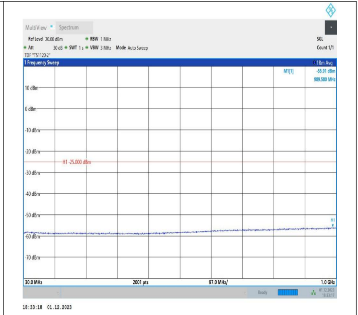
7-7-20MHz-10MHz-64QAM-64QAM-21051-21195-100RB#0-50 RB#0-30~1000MHz-PASS
