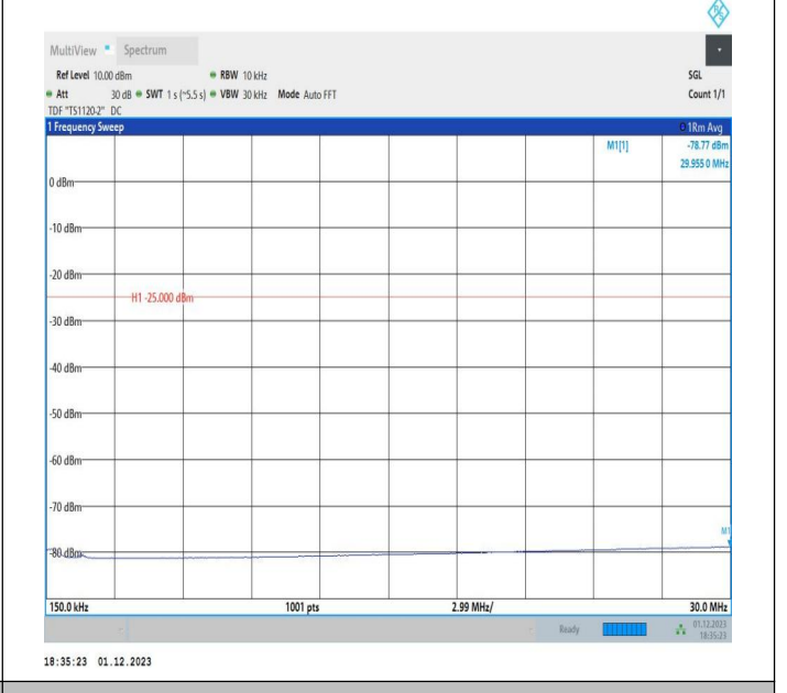
7-7-20MHz-10MHz-64QAM-64QAM-21251-21395-1RB#0-ORB #0-0.15~30MHz-PASS
