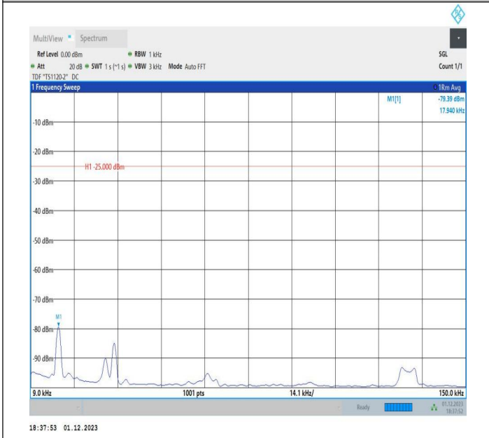
7-7-20MHz-10MHz-QPSK-QPSK-21251-21395-1RB#0-1RB#4 9-0.009~0.15MHz-PASS
