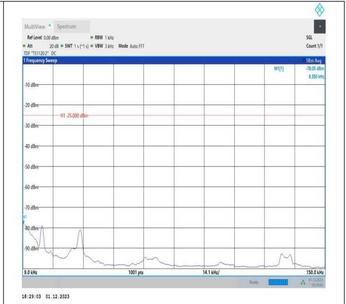
7-7-20MHz-10MHz-64QAM-64QAM-21051-21195-1RB#99-0R B#0-0.009~0.15MHz-PASS
