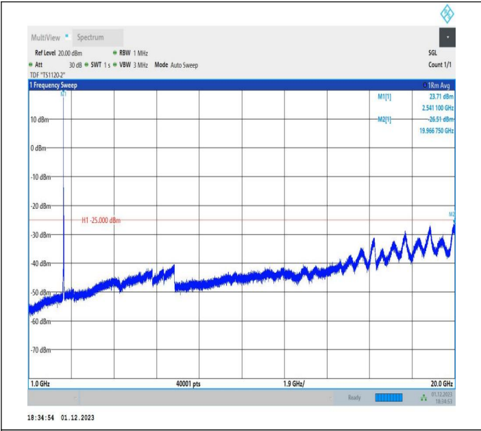
7-7-20MHz-10MHz-16QAM-16QAM-21251-21395-1RB#0-ORB #0-1000~20000MHz-PASS
