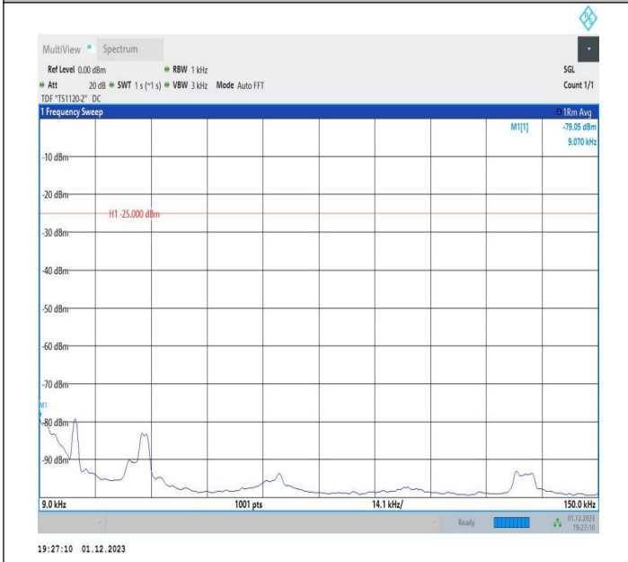
7-7-20MHz-15MHz-64QAM-64QAM-20850-21021-1RB#0-ORB #0-0.009~0.15MHz-PASS
