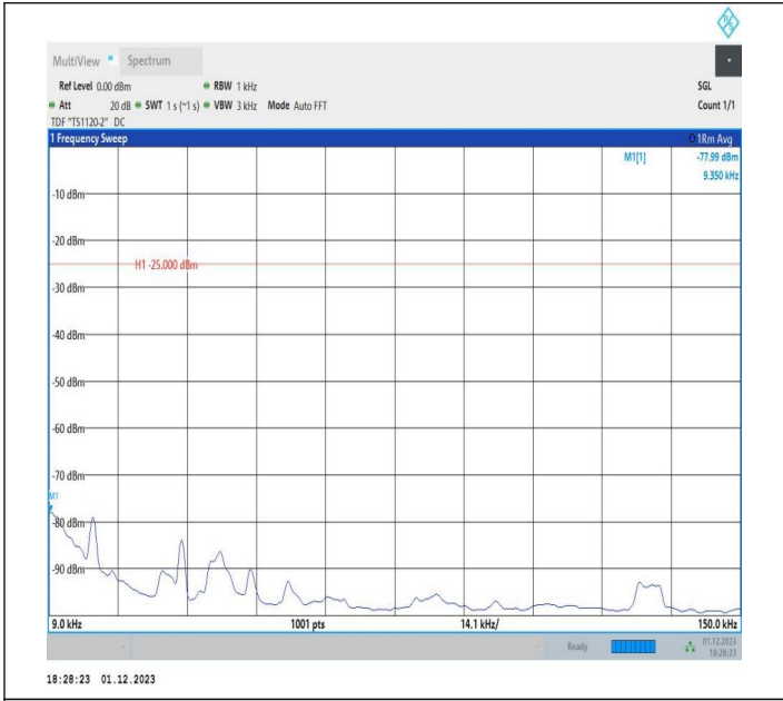
7-7-20MHz-10MHz-16QAM-16QAM-21051-21195-1RB#99-0R B#0-0.009~0.15MHz-PASS
