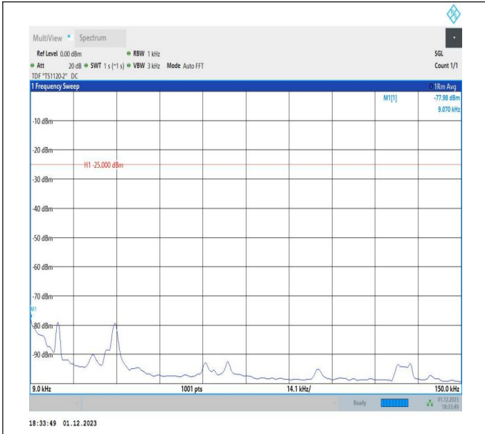
7-7-20MHz-10MHz-QPSK-QPSK-21251-21395-1RB#0-0RB#0 -0.009~0.15MHz-PASS
