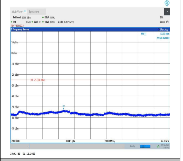
7-7-20MHz-10MHz-64QAM-64QAM-21251-21395-100RB#0-5 ORB#0-20000~27000MHz-PASS
