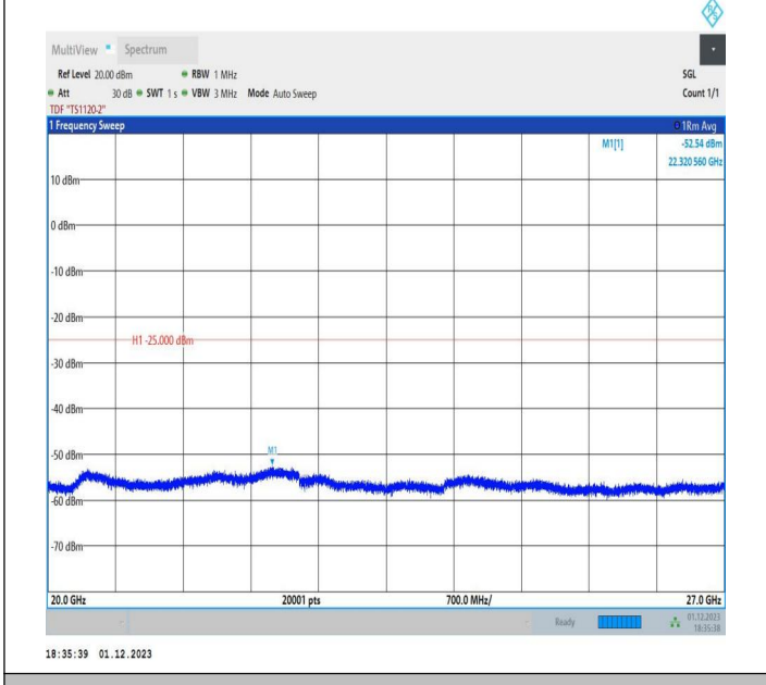
7-7-20MHz-10MHz-64QAM-64QAM-21251-21395-1RB#0-ORB #0-20000~27000MHz-PASS
