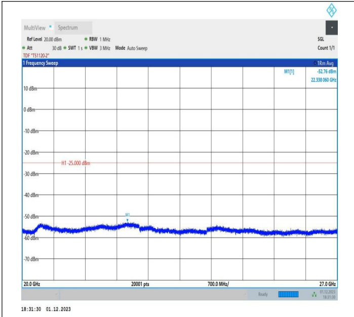
7-7-20MHz-10MHz-64QAM-64QAM-21051-21195-1RB#0-1RB #49-20000~27000MHz-PASS
