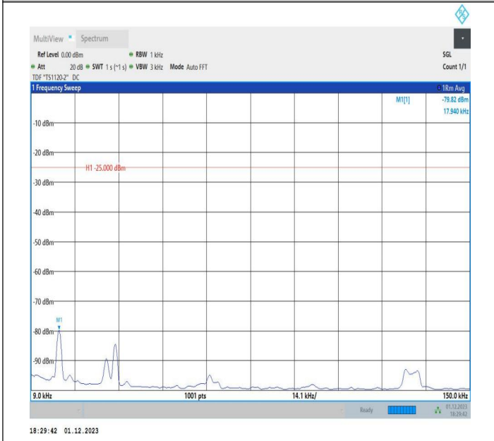
7-7-20MHz-10MHz-QPSK-QPSK-21051-21195-1RB#0-1RB#4 9-0.009~0.15MHz-PASS
