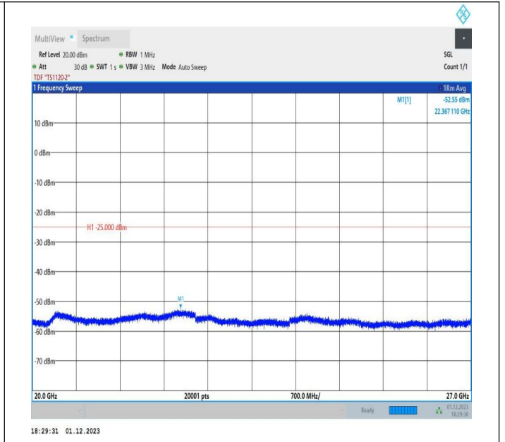
7-7-20MHz-10MHz-64QAM-64QAM-21051-21195-1RB#99-0R B#0-20000~27000MHz-PASS
