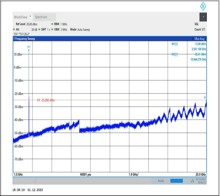
7-7-20MHz-10MHz-QPSK-QPSK-21251-21395-1RB#0-1RB#4 9-1000~20000MHz-PASS
