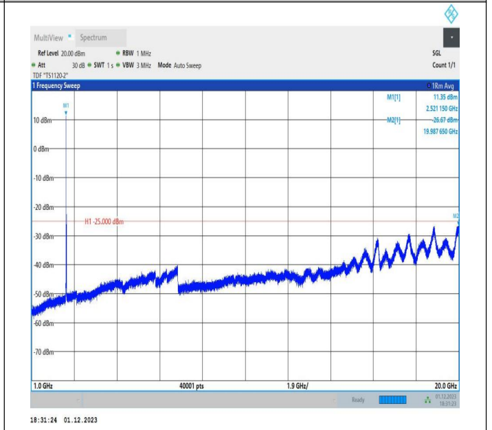
7-7-20MHz-10MHz-64QAM-64QAM-21051-21195-1RB#0-1RB #49-1000~20000MHz-PASS
