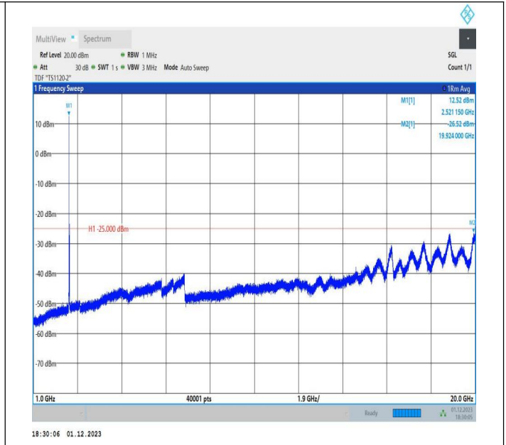
7-7-20MHz-10MHz-QPSK-QPSK-21051-21195-1RB#0-1RB#4 9-1000~20000MHz-PASS
