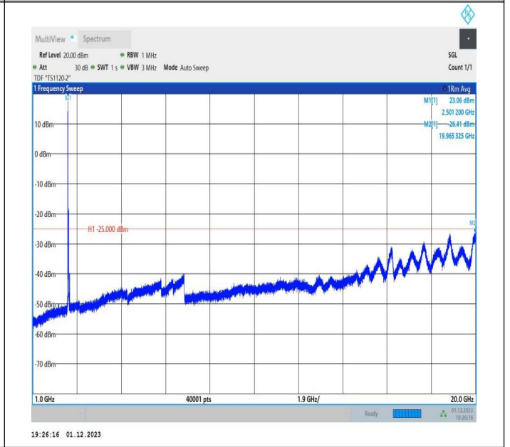
7-7-20MHz-15MHz-QPSK-QPSK-20850-21021-1RB#0-0RB#0 -1000~20000MHz-PASS
