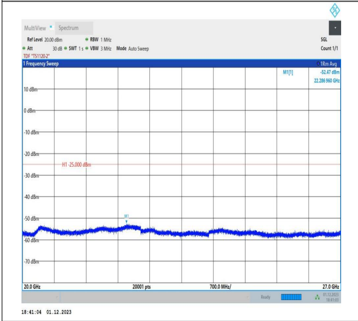
7-7-20MHz-10MHz-16QAM-16QAM-21251-21395-100RB#0-5 ORB#0-20000~27000MHz-PASS
