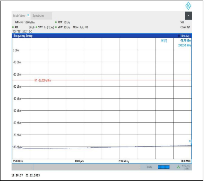
7-7-20MHz-10MHz-16QAM-16QAM-21051-21195-1RB#99-0R B#0-0.15~30MHz-PASS
