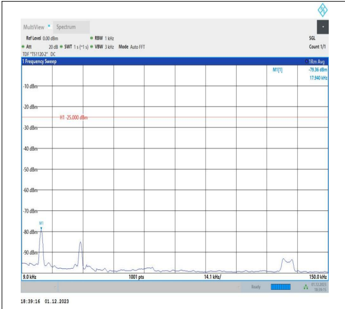
7-7-20MHz-10MHz-64QAM-64QAM-21251-21395-1RB#0-1RB #49-0.009~0.15MHz-PASS
