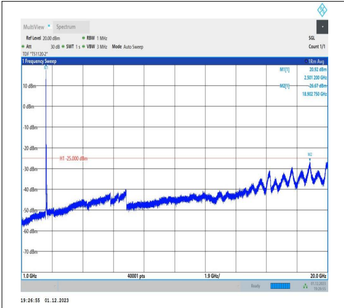
7-7-20MHz-15MHz-16QAM-16QAM-20850-21021-1RB#0-ORB #0-1000~20000MHz-PASS
