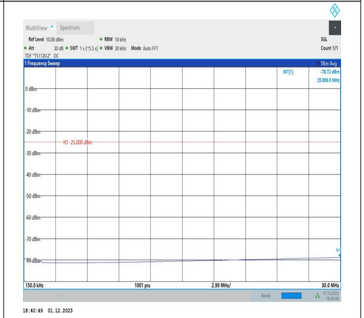
7-7-20MHz-10MHz-16QAM-16QAM-21251-21395-100RB#0-5 ORB#0-0.15~30MHz-PASS
