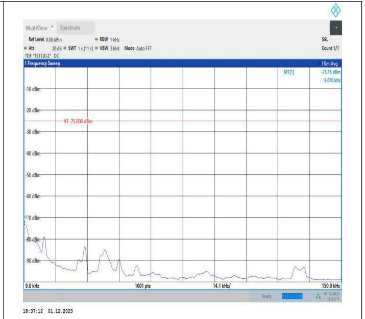
7-7-20MHz-10MHz-64QAM-64QAM-21251-21395-1RB#99-0R B#0-0.009~0.15MHz-PASS
