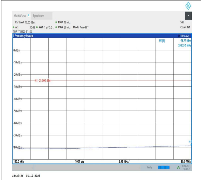
7-7-20MHz-10MHz-64QAM-64QAM-21251-21395-1RB#99-0R B#0-0.15~30MHz-PASS
