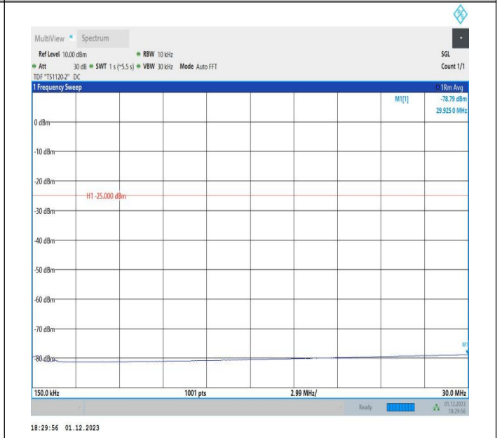
7-7-20MHz-10MHz-QPSK-QPSK-21051-21195-1RB#0-1RB#4 9-0.15~30MHz-PASS
