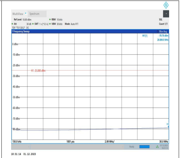
7-7-20MHz-10MHz-64QAM-64QAM-21051-21195-1RB#0-1RB #49-0.15~30MHz-PASS
