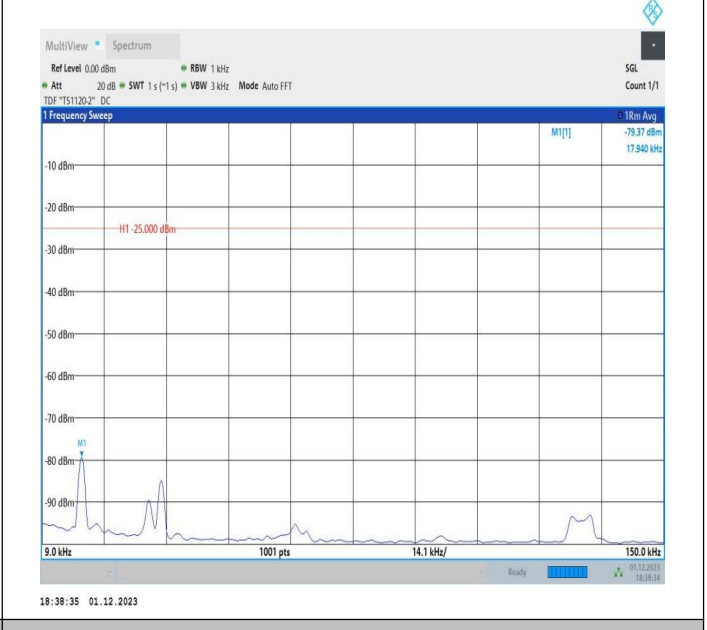
7-7-20MHz-10MHz-16QAM-16QAM-21251-21395-1RB#0-1RB #49-0.009~0.15MHz-PASS
