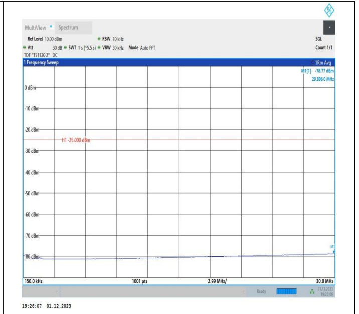
7-7-20MHz-15MHz-QPSK-QPSK-20850-21021-1RB#0-0RB#0 -0.15~30MHz-PASS
