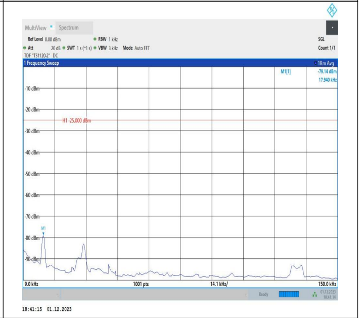
7-7-20MHz-10MHz-64QAM-64QAM-21251-21395-100RB#0-5 ORB#0-0.009~0.15MHz-PASS
