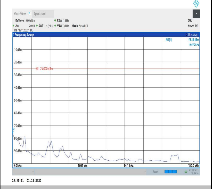
7-7-20MHz-10MHz-QPSK-QPSK-21251-21395-1RB#99-ORB# 0-0.009~0.15MHz-PASS
