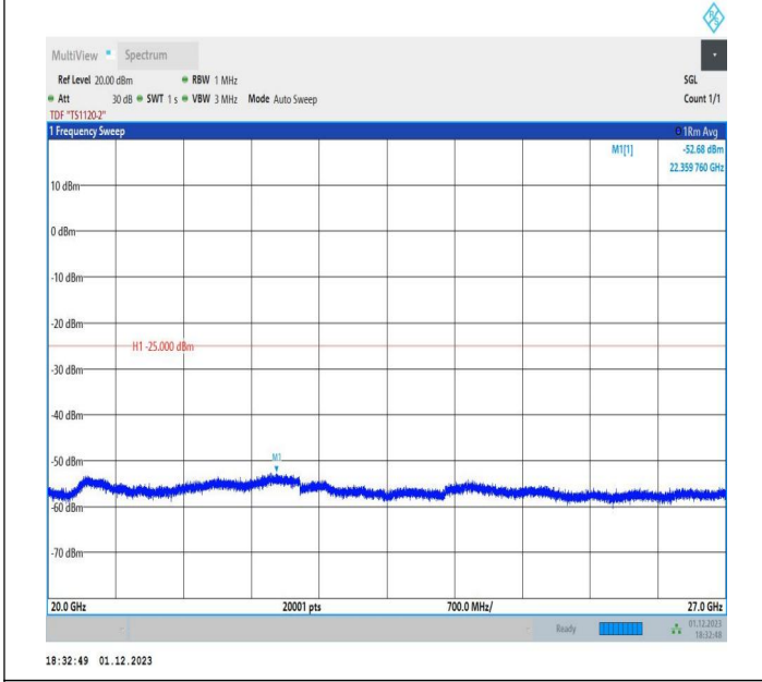
7-7-20MHz-10MHz-16QAM-16QAM-21051-21195-100RB#0-50 RB#0-20000~27000MHz-PASS
