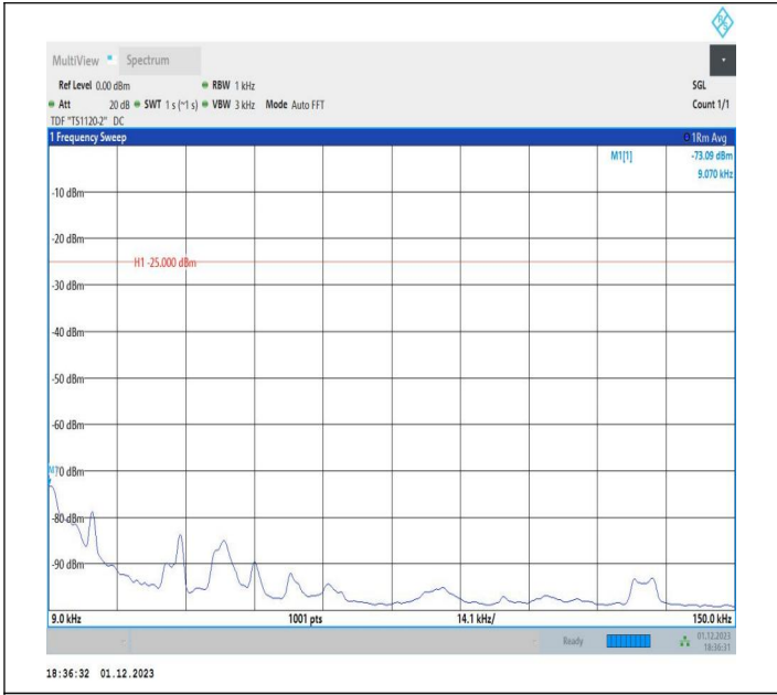
7-7-20MHz-10MHz-16QAM-16QAM-21251-21395-1RB#99-0R B#0-0.009~0.15MHz-PASS
