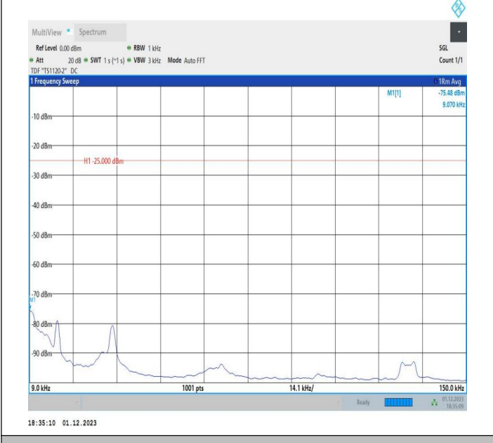
7-7-20MHz-10MHz-64QAM-64QAM-21251-21395-1RB#0-ORB #0-0.009~0.15MHz-PASS
