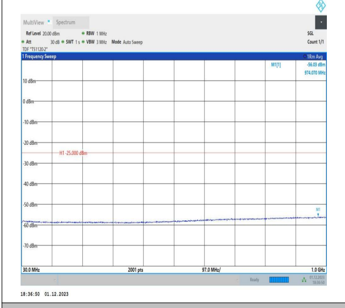
7-7-20MHz-10MHz-16QAM-16QAM-21251-21395-1RB#99-0R B#0-30~1000MHz-PASS
