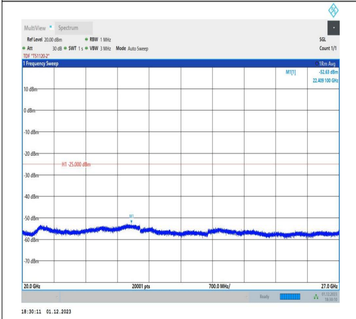
7-7-20MHz-10MHz-QPSK-QPSK-21051-21195-1RB#0-1RB#4 9-20000~27000MHz-PASS
