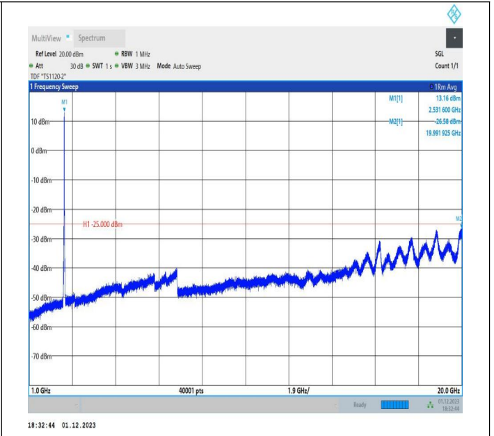
7-7-20MHz-10MHz-16QAM-16QAM-21051-21195-100RB#0-50 RB#0-1000~20000MHz-PASS
