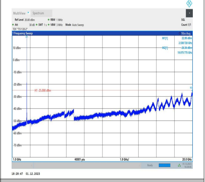
7-7-20MHz-10MHz-16QAM-16QAM-21051-21195-1RB#99-0R B#0-1000~20000MHz-PASS
