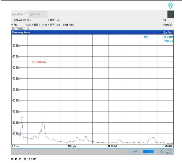
7-7-20MHz-10MHz-16QAM-16QAM-21251-21395-100RB#0-5 ORB#0-0.009~0.15MHz-PASS
