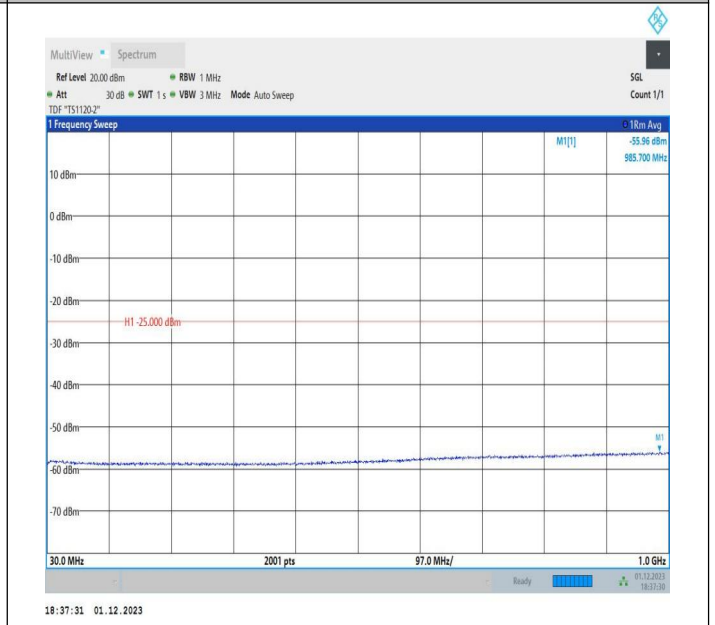
7-7-20MHz-10MHz-64QAM-64QAM-21251-21395-1RB#99-0R B#0-30~1000MHz-PASS
