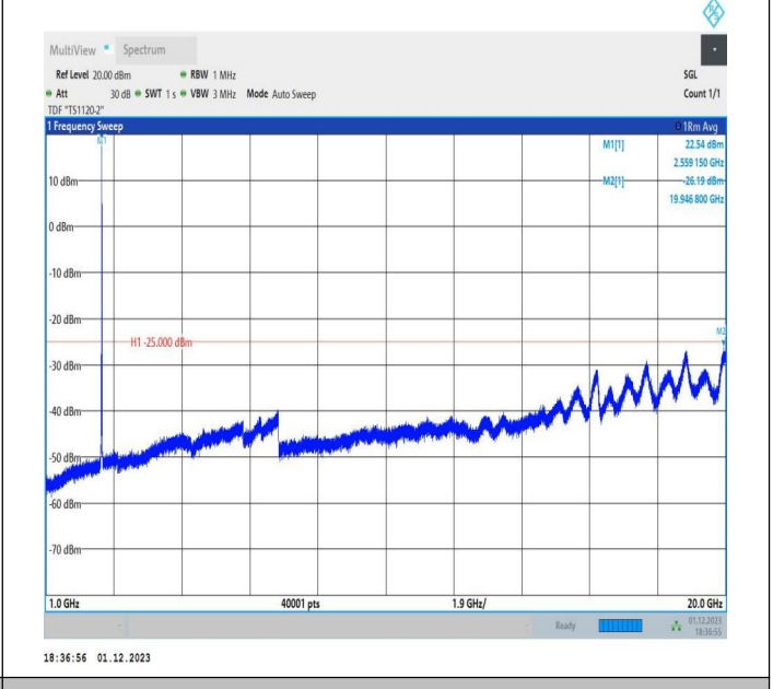
7-7-20MHz-10MHz-16QAM-16QAM-21251-21395-1RB#99-0R B#0-1000~20000MHz-PASS
