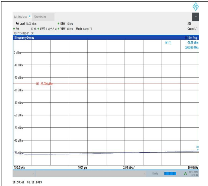
7-7-20MHz-10MHz-16QAM-16QAM-21251-21395-1RB#0-1RB #49-0.15~30MHz-PASS
