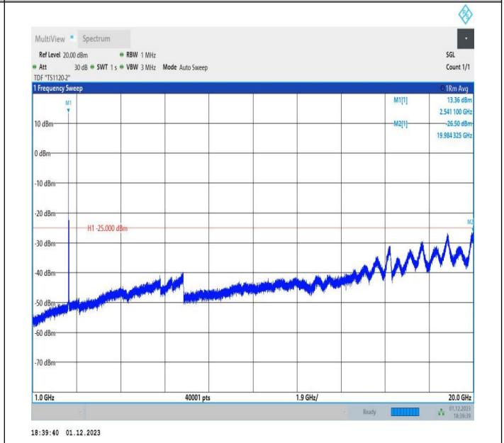
7-7-20MHz-10MHz-64QAM-64QAM-21251-21395-1RB#0-1RB #49-1000~20000MHz-PASS
