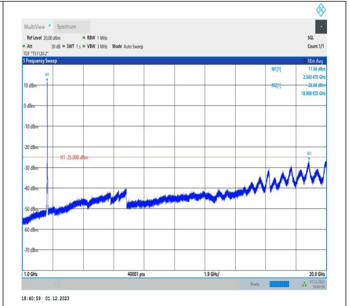
7-7-20MHz-10MHz-16QAM-16QAM-21251-21395-100RB#0-5 ORB#0-1000~20000MHz-PASS
