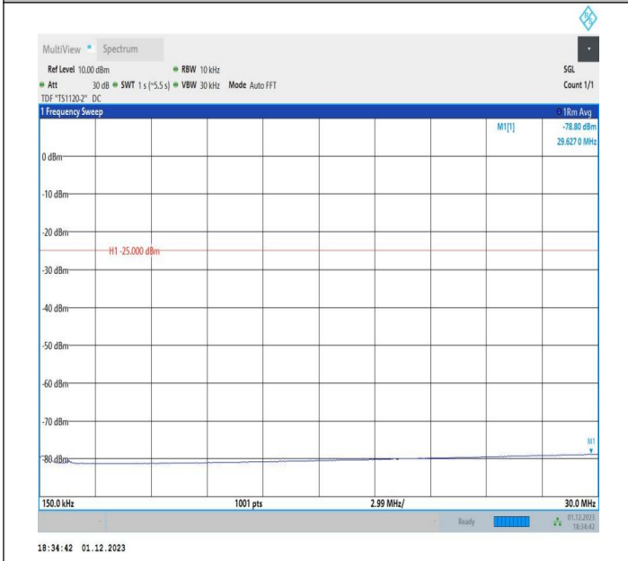
7-7-20MHz-10MHz-16QAM-16QAM-21251-21395-1RB#0-0RB #0-0.15~30MHz-PASS
