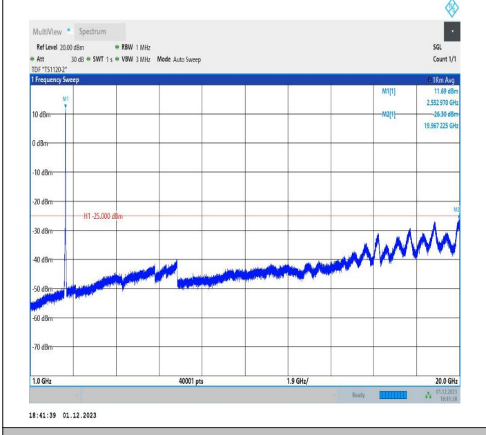
7-7-20MHz-10MHz-64QAM-64QAM-21251-21395-100RB#0-5 ORB#0-1000~20000MHz-PASS
