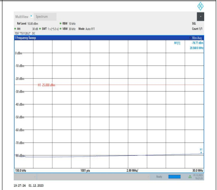
7-7-20MHz-15MHz-64QAM-64QAM-20850-21021-1RB#0-ORB #0-0.15~30MHz-PASS
