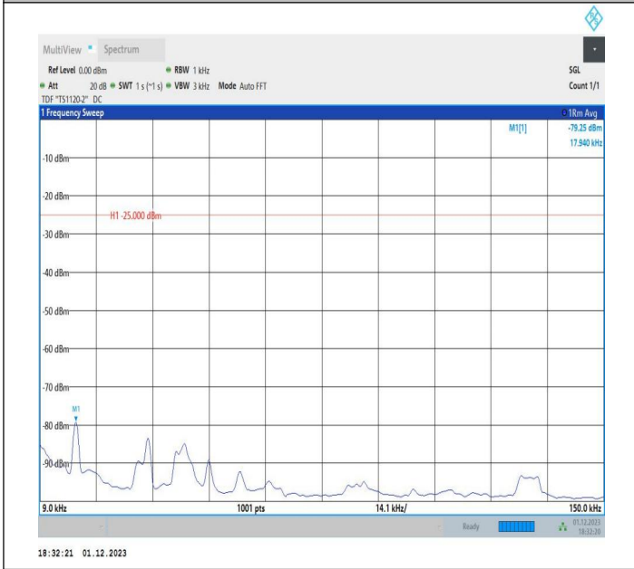
7-7-20MHz-10MHz-16QAM-16QAM-21051-21195-100RB#0-50 RB#0-0.009~0.15MHz-PASS
