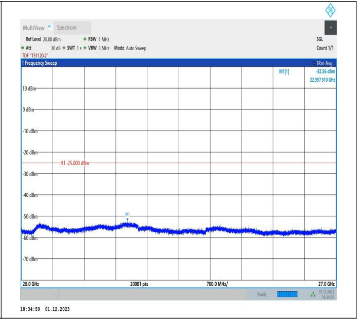
7-7-20MHz-10MHz-16QAM-16QAM-21251-21395-1RB#0-ORB #0-20000~27000MHz-PASS
