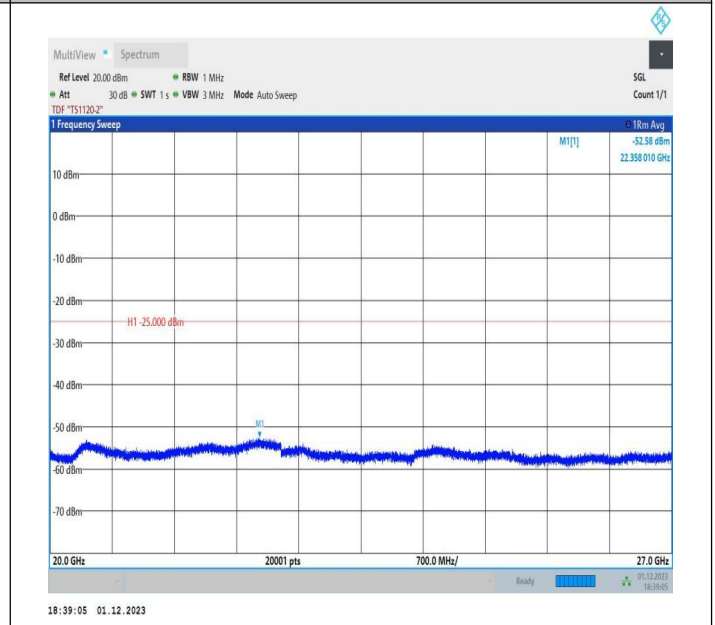
7-7-20MHz-10MHz-16QAM-16QAM-21251-21395-1RB#0-1RB #49-20000~27000MHz-PASS
