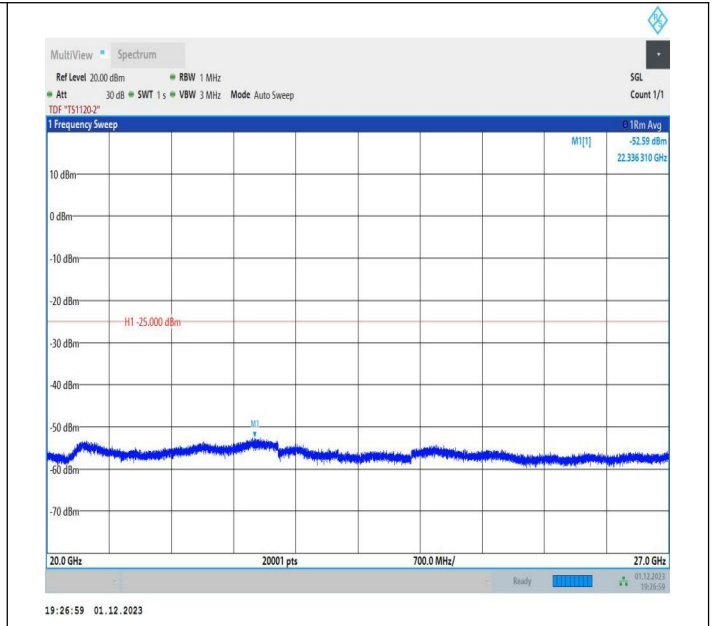
7-7-20MHz-15MHz-16QAM-16QAM-20850-21021-1RB#0-ORB #0-20000~27000MHz-PASS
