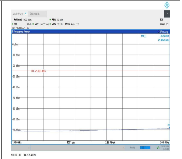
7-7-20MHz-10MHz-QPSK-QPSK-21251-21395-1RB#0-0RB#0 -0.15~30MHz-PASS
