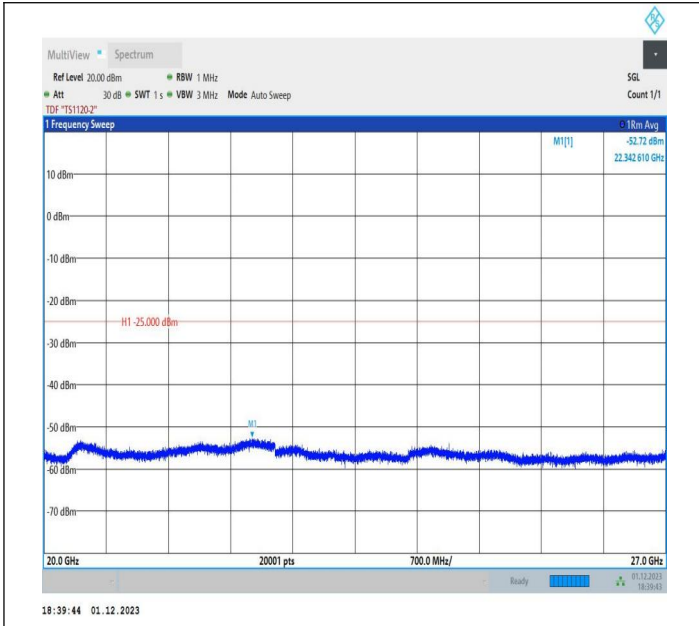
7-7-20MHz-10MHz-64QAM-64QAM-21251-21395-1RB#0-1RB #49-20000~27000MHz-PASS
