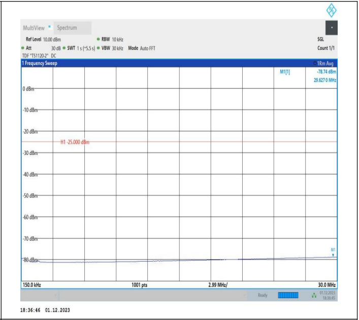
7-7-20MHz-10MHz-16QAM-16QAM-21251-21395-1RB#99-0R B#0-0.15~30MHz-PASS
