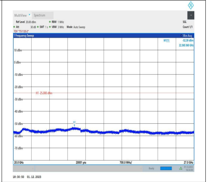
7-7-20MHz-10MHz-16QAM-16QAM-21051-21195-1RB#0-1RB #49-20000~27000MHz-PASS
