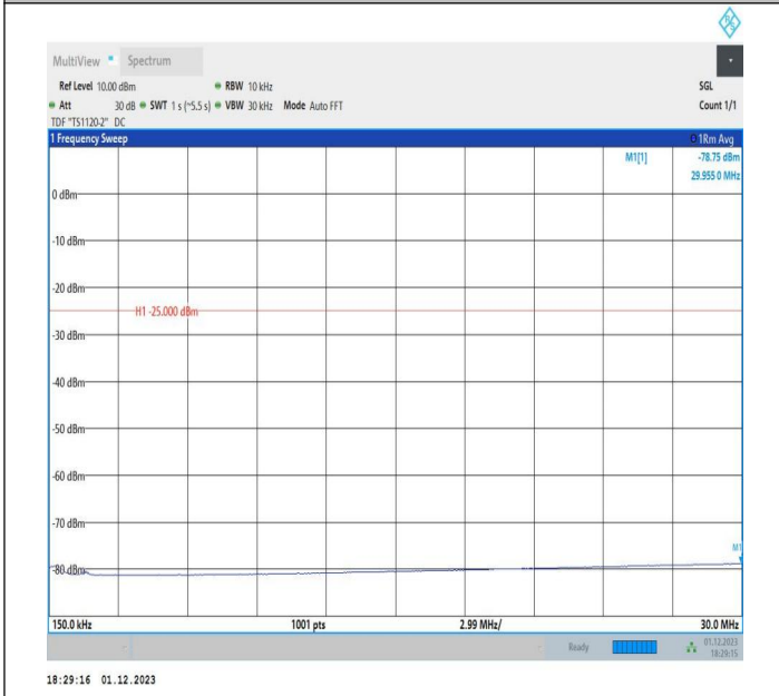
7-7-20MHz-10MHz-64QAM-64QAM-21051-21195-1RB#99-0R B#0-0.15~30MHz-PASS
