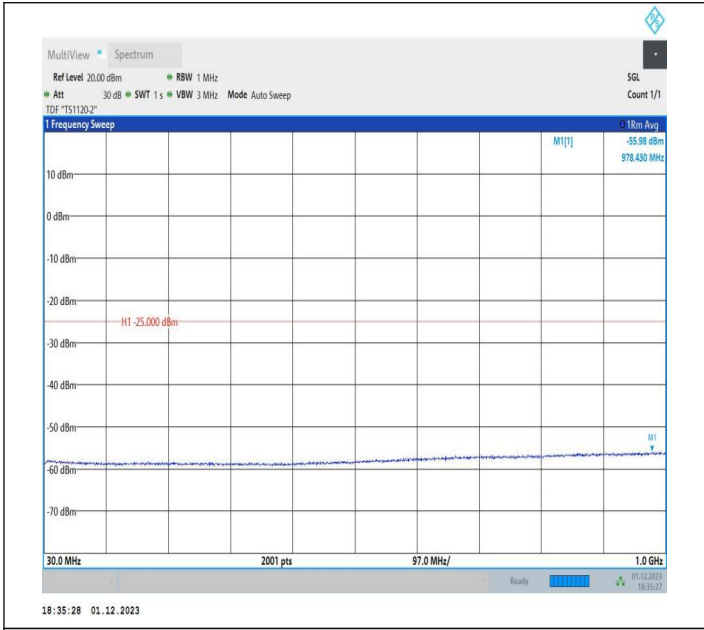
7-7-20MHz-10MHz-64QAM-64QAM-21251-21395-1RB#0-ORB #0-30~1000MHz-PASS
