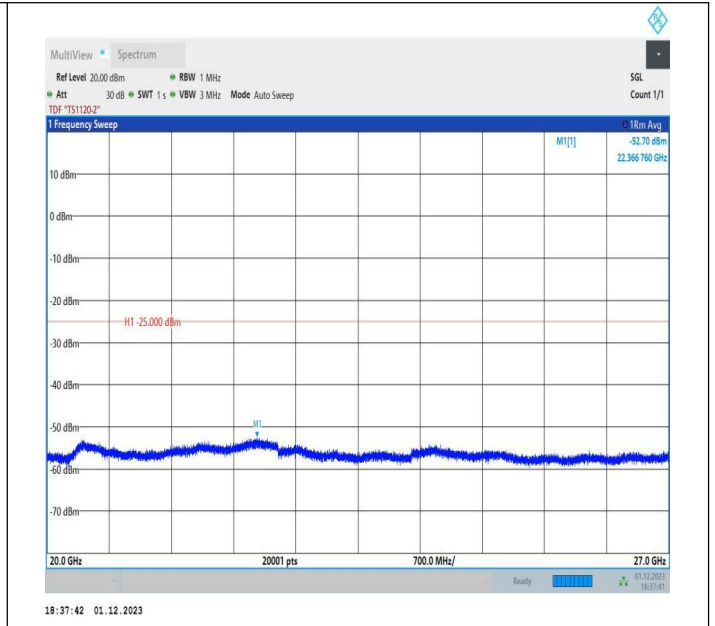
7-7-20MHz-10MHz-64QAM-64QAM-21251-21395-1RB#99-0R B#0-20000~27000MHz-PASS
