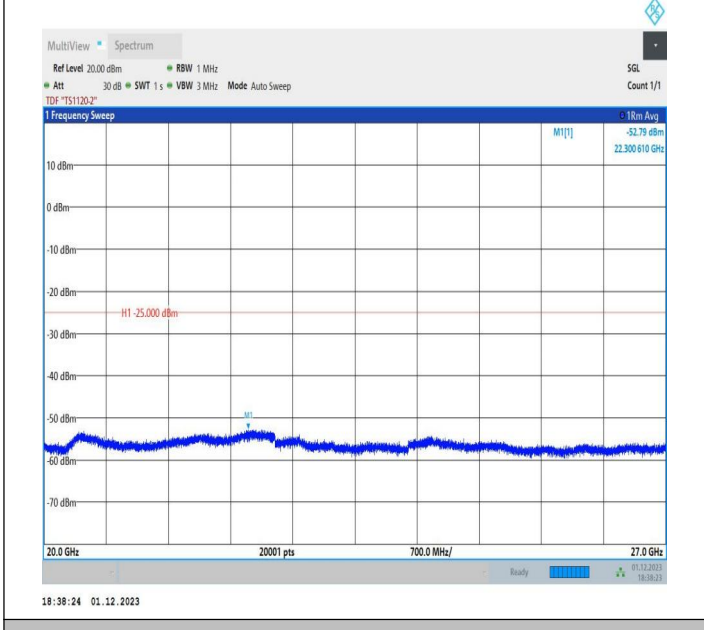
7-7-20MHz-10MHz-QPSK-QPSK-21251-21395-1RB#0-1RB#4 9-20000~27000MHz-PASS
