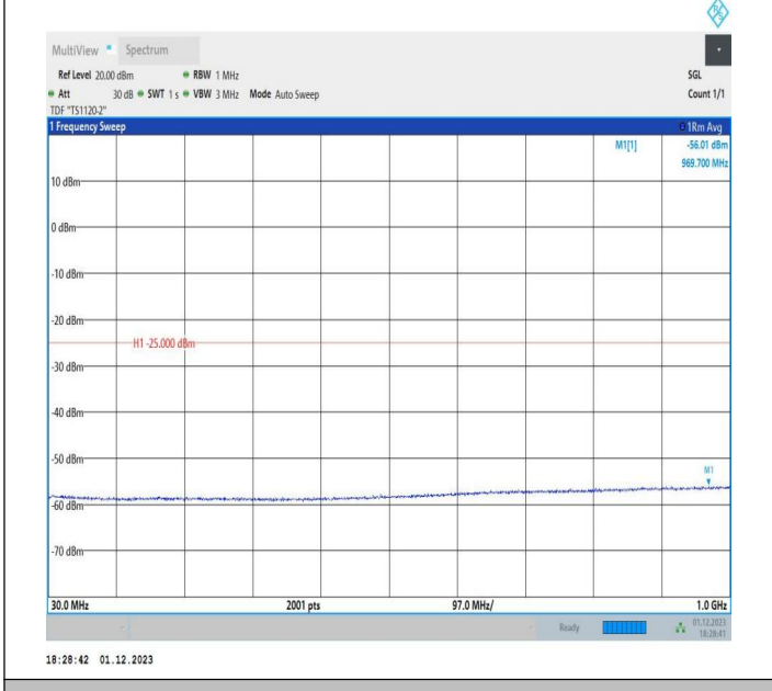
7-7-20MHz-10MHz-16QAM-16QAM-21051-21195-1RB#99-0R B#0-30~1000MHz-PASS
