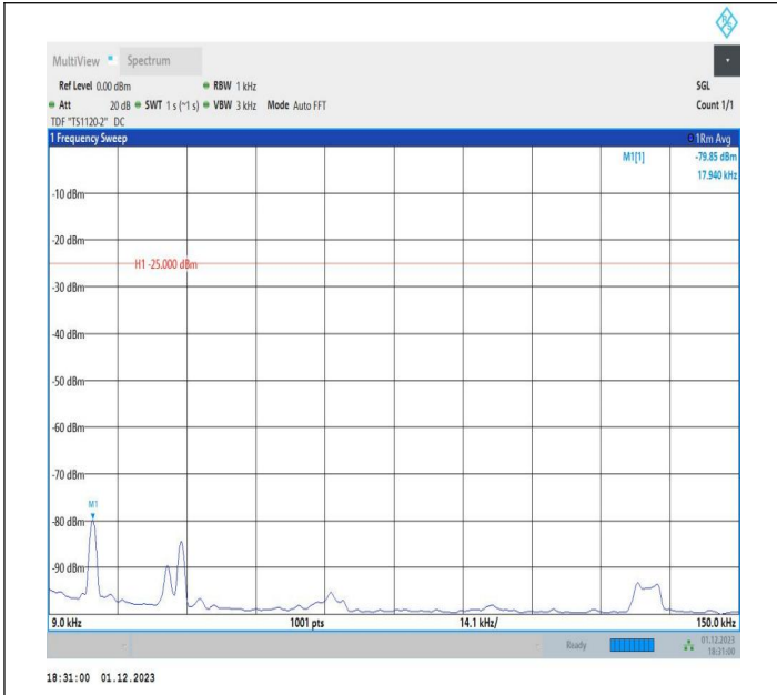
7-7-20MHz-10MHz-64QAM-64QAM-21051-21195-1RB#0-1RB #49-0.009~0.15MHz-PASS
