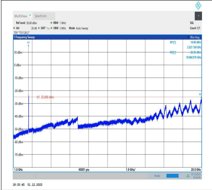
7-7-20MHz-10MHz-16QAM-16QAM-21051-21195-1RB#0-1RB #49-1000~20000MHz-PASS
