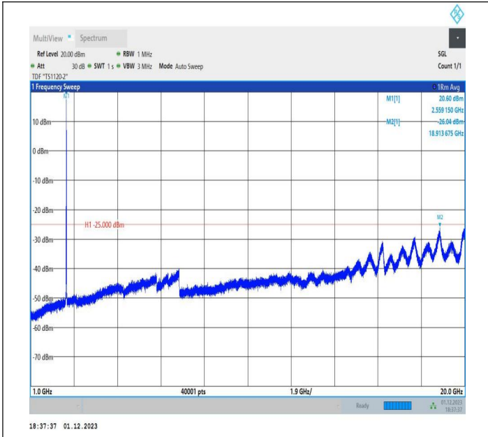
7-7-20MHz-10MHz-64QAM-64QAM-21251-21395-1RB#99-0R B#0-1000~20000MHz-PASS
