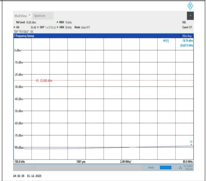
7-7-20MHz-10MHz-16QAM-16QAM-21051-21195-100RB#0-50 RB#0-0.15~30MHz-PASS
