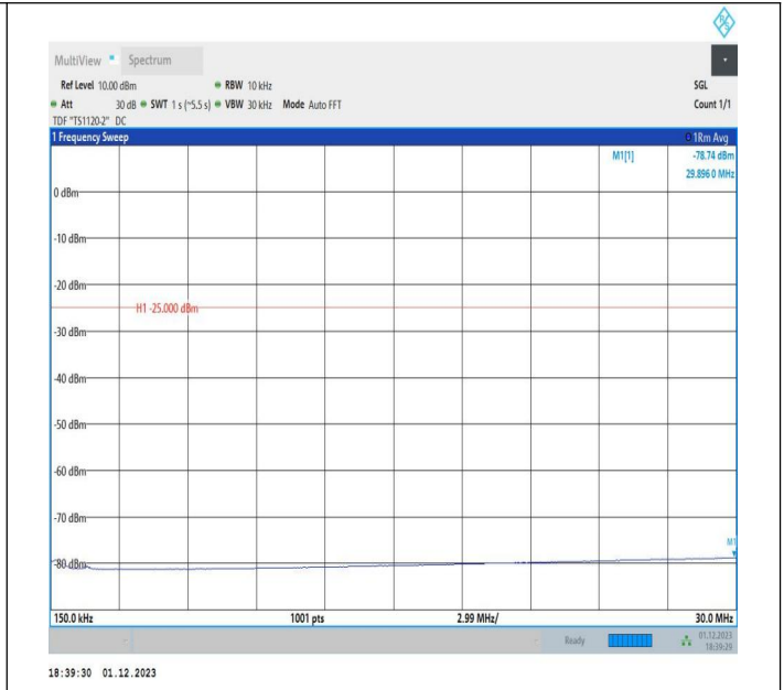
7-7-20MHz-10MHz-64QAM-64QAM-21251-21395-1RB#0-1RB #49-0.15~30MHz-PASS
