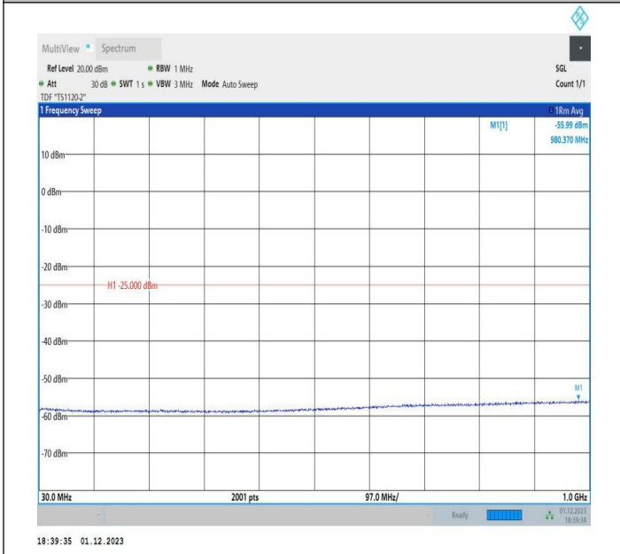
7-7-20MHz-10MHz-64QAM-64QAM-21251-21395-1RB#0-1RB #49-30~1000MHz-PASS
