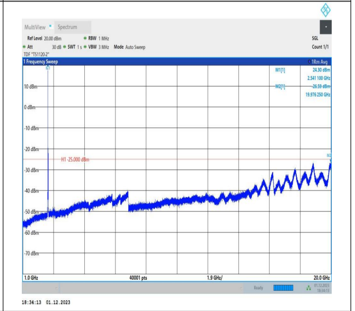
7-7-20MHz-10MHz-QPSK-QPSK-21251-21395-1RB#0-0RB#0 -1000~20000MHz-PASS
