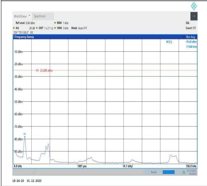
7-7-20MHz-10MHz-16QAM-16QAM-20850-20994-100RB#0-5 ORB#0-0.009~0.15MHz-PASS
