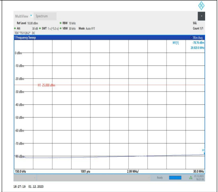
7-7-20MHz-10MHz-64QAM-64QAM-21051-21195-1RB#0-ORB #0-0.15~30MHz-PASS
