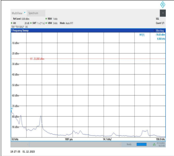
7-7-20MHz-10MHz-64QAM-64QAM-21051-21195-1RB#0-ORB #0-0.009~0.15MHz-PASS
