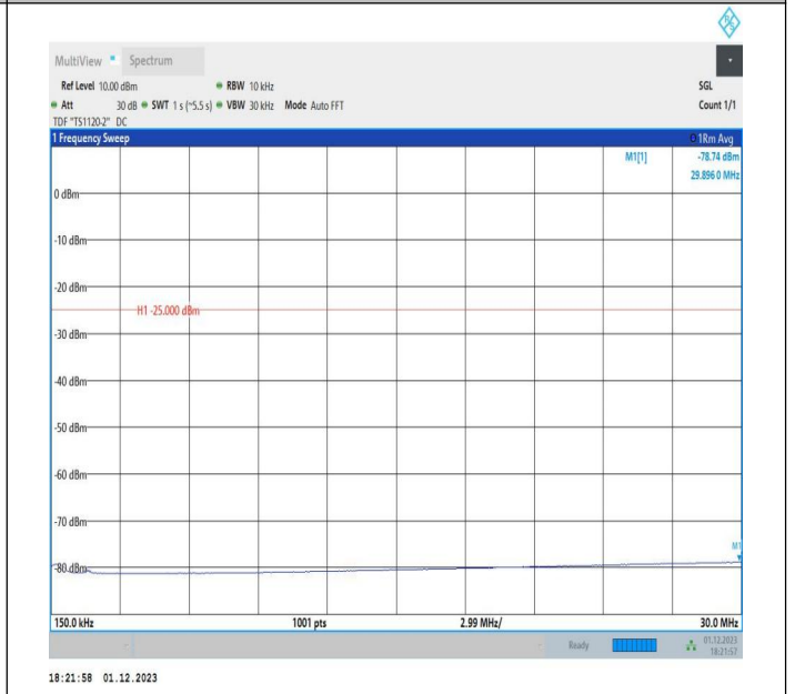
7-7-20MHz-10MHz-QPSK-QPSK-20850-20994-1RB#0-1RB#4 9-0.15~30MHz-PASS
