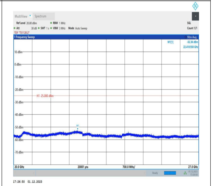
7-7-15MHz-20MHz-16QAM-16QAM-21179-21350-1RB#0-1RB #99-20000~27000MHz-PASS
