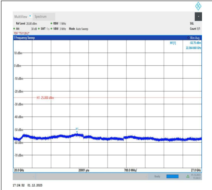
7-7-15MHz-20MHz-16QAM-16QAM-21179-21350-1RB#74-0R B#0-20000~27000MHz-PASS
