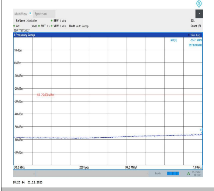
7-7-20MHz-10MHz-16QAM-16QAM-20850-20994-1RB#99-0R B#0-30~1000MHz-PASS
