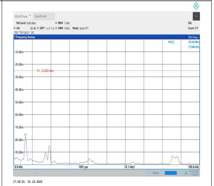
7-7-15MHz-20MHz-16QAM-16QAM-21179-21350-1RB#0-1RB #99-0.009~0.15MHz-PASS
