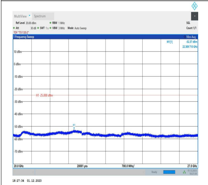
7-7-20MHz-10MHz-64QAM-64QAM-21051-21195-1RB#0-ORB #0-20000~27000MHz-PASS
