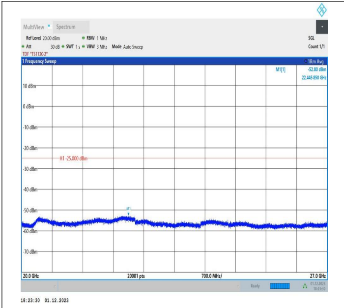
7-7-20MHz-10MHz-64QAM-64QAM-20850-20994-1RB#0-1RB #49-20000~27000MHz-PASS
