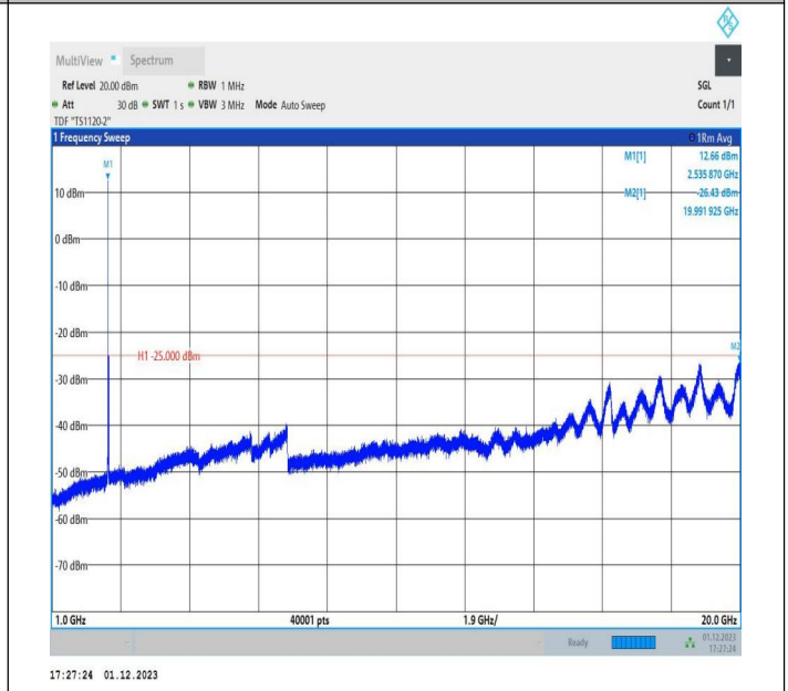
7-7-15MHz-20MHz-64QAM-64QAM-21179-21350-1RB#0-1RB #99-1000~20000MHz-PASS
