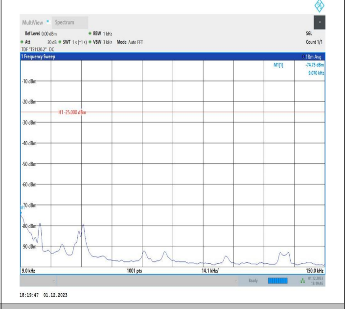
7-7-20MHz-10MHz-QPSK-QPSK-20850-20994-1RB#99-ORB# 0-0.009~0.15MHz-PASS
