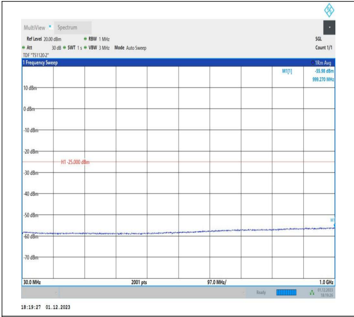
7-7-20MHz-10MHz-64QAM-64QAM-20850-20994-1RB#0-ORB #0-30~1000MHz-PASS
