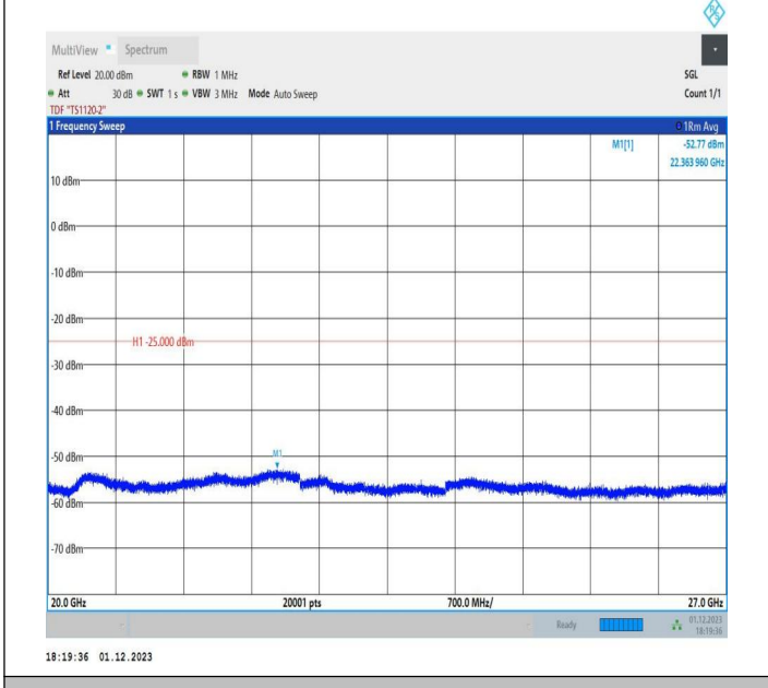
7-7-20MHz-10MHz-64QAM-64QAM-20850-20994-1RB#0-ORB #0-20000~27000MHz-PASS
