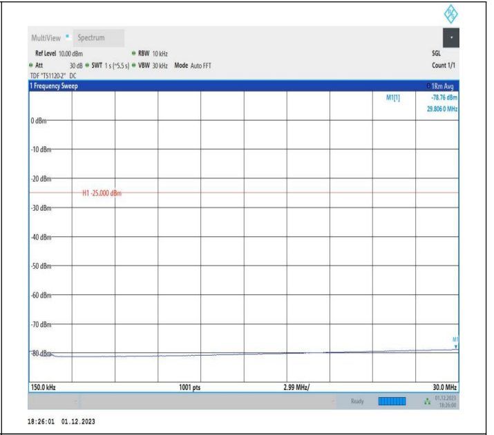
7-7-20MHz-10MHz-QPSK-QPSK-21051-21195-1RB#0-ORB#0-0.15~30MHz-PASS
