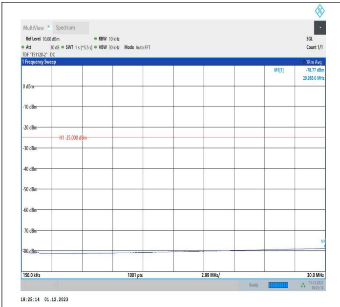
7-7-20MHz-10MHz-64QAM-64QAM-20850-20994-100RB#0-5 ORB#0-0.15~30MHz-PASS
