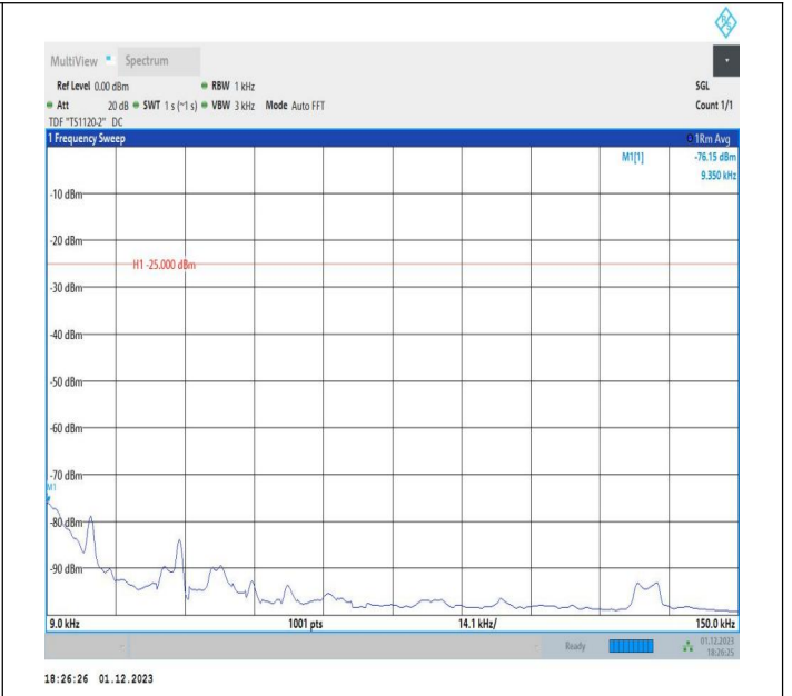
7-7-20MHz-10MHz-16QAM-16QAM-21051-21195-1RB#0-ORB#0-0.009~0.15MHz-PASS
