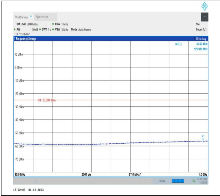
7-7-20MHz-10MHz-QPSK-QPSK-20850-20994-1RB#0-1RB#4 9-30~1000MHz-PASS
