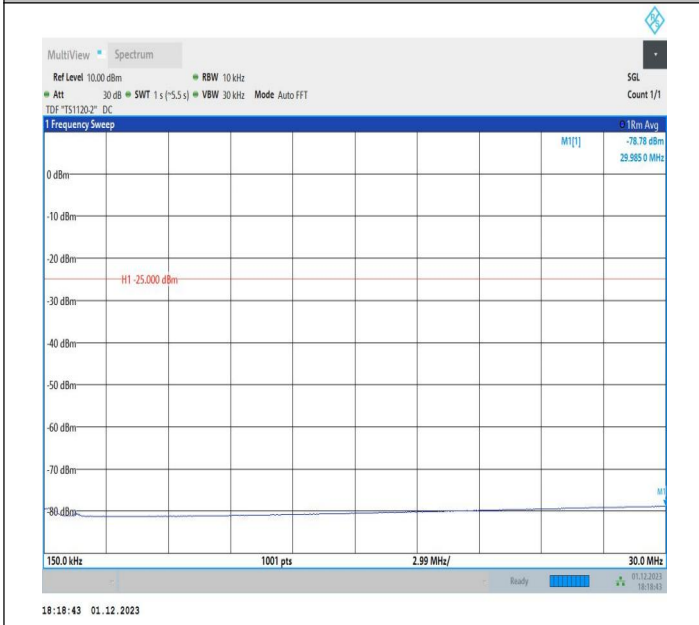
7-7-20MHz-10MHz-16QAM-16QAM-20850-20994-1RB#0-0RB #0-0.15~30MHz-PASS
