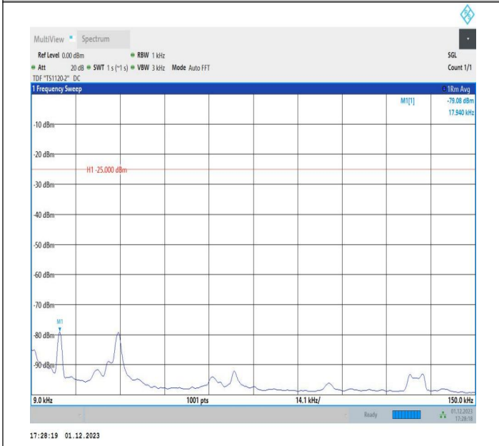
7-7-15MHz-20MHz-16QAM-16QAM-21179-21350-75RB#0-100 RB#0-0.009~0.15MHz-PASS
