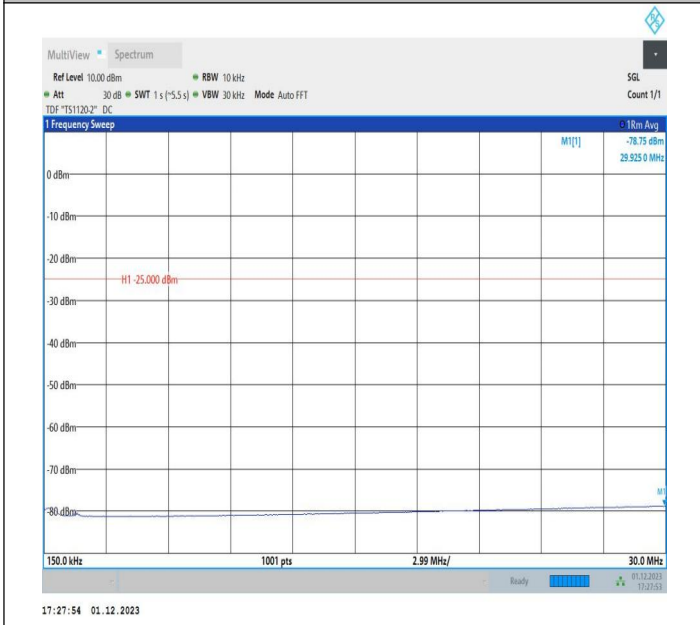
7-7-15MHz-20MHz-QPSK-QPSK-21179-21350-75RB#0-100R B#0-0.15~30MHz-PASS
