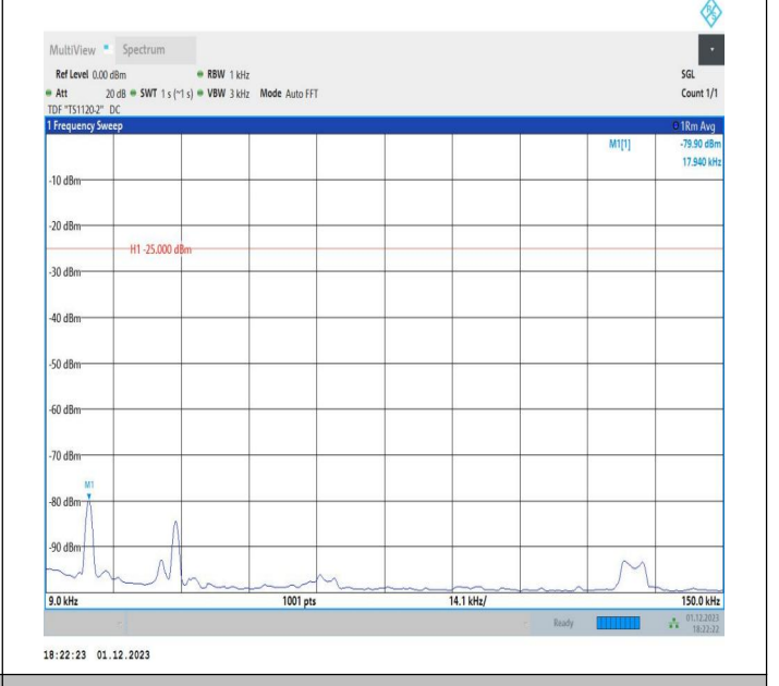
7-7-20MHz-10MHz-16QAM-16QAM-20850-20994-1RB#0-1RB #49-0.009~0.15MHz-PASS
