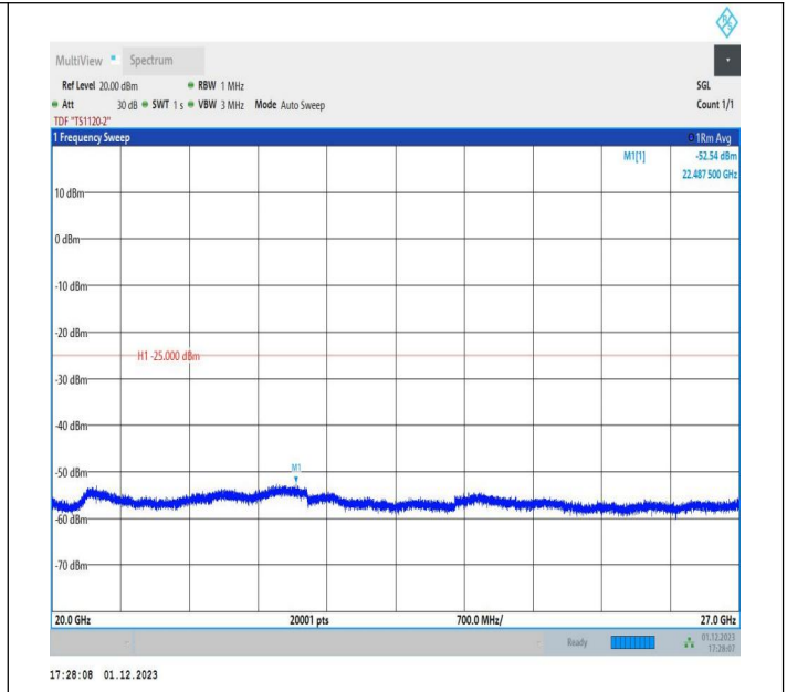
7-7-15MHz-20MHz-QPSK-QPSK-21179-21350-75RB#0-100R B#0-20000~27000MHz-PASS
