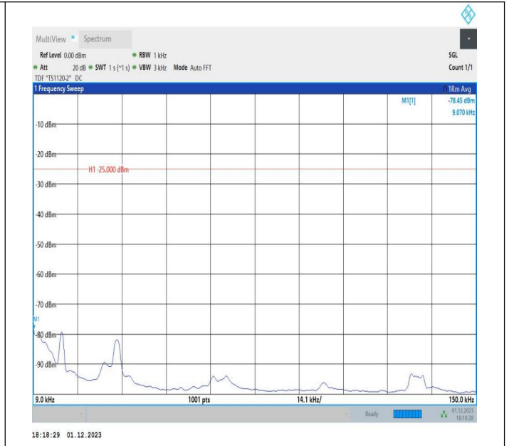
7-7-20MHz-10MHz-16QAM-16QAM-20850-20994-1RB#0-0RB #0-0.009~0.15MHz-PASS
