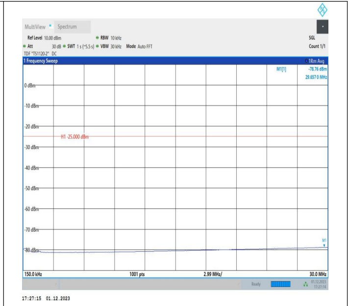
7-7-15MHz-20MHz-64QAM-64QAM-21179-21350-1RB#0-1RB #99-0.15~30MHz-PASS
