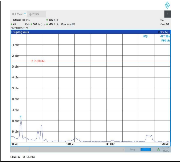
7-7-20MHz-10MHz-64QAM-64QAM-20850-20994-1RB#0-1RB #49-0.009~0.15MHz-PASS
