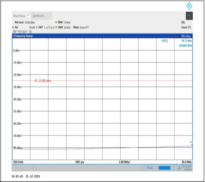
7-7-20MHz-10MHz-16QAM-16QAM-20850-20994-1RB#99-0R B#0-0.15~30MHz-PASS
