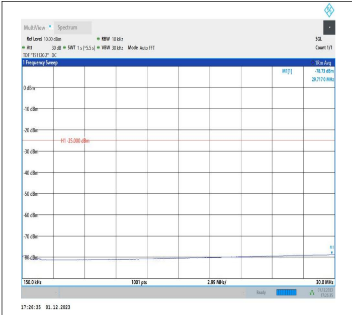
7-7-15MHz-20MHz-16QAM-16QAM-21179-21350-1RB#0-1RB #99-0.15~30MHz-PASS
