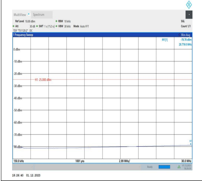
7-7-20MHz-10MHz-16QAM-16QAM-21051-21195-1RB#0-ORB#0-0.15~30MHz-PASS
