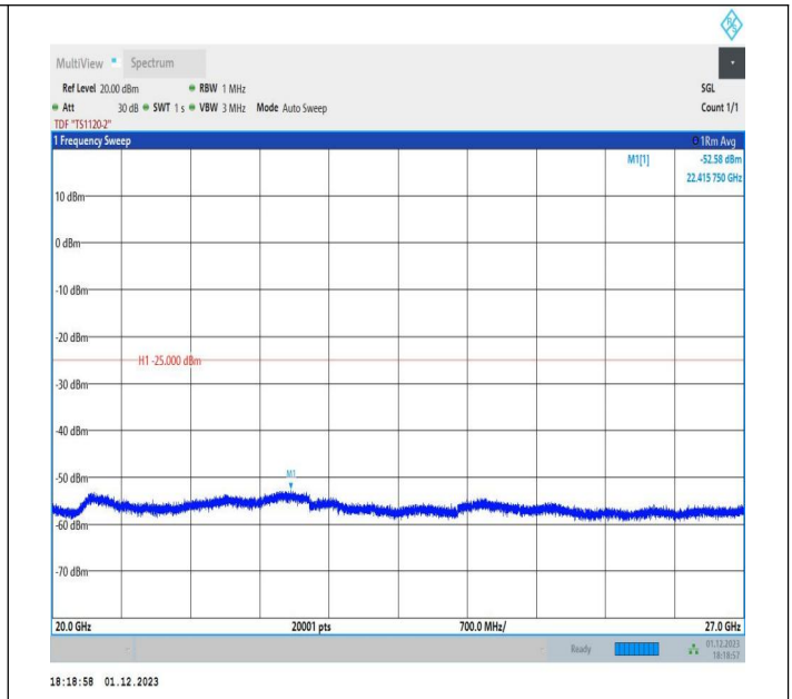
7-7-20MHz-10MHz-16QAM-16QAM-20850-20994-1RB#0-ORB #0-20000~27000MHz-PASS
