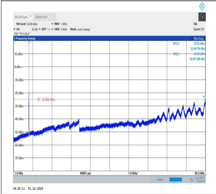
7-7-20MHz-10MHz-QPSK-QPSK-20850-20994-1RB#99-0RB# 0-1000~20000MHz-PASS
