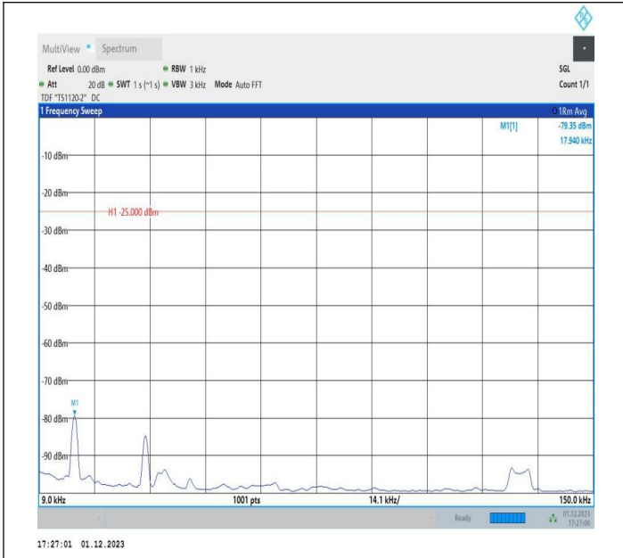
7-7-15MHz-20MHz-64QAM-64QAM-21179-21350-1RB#0-1RB #99-0.009~0.15MHz-PASS
