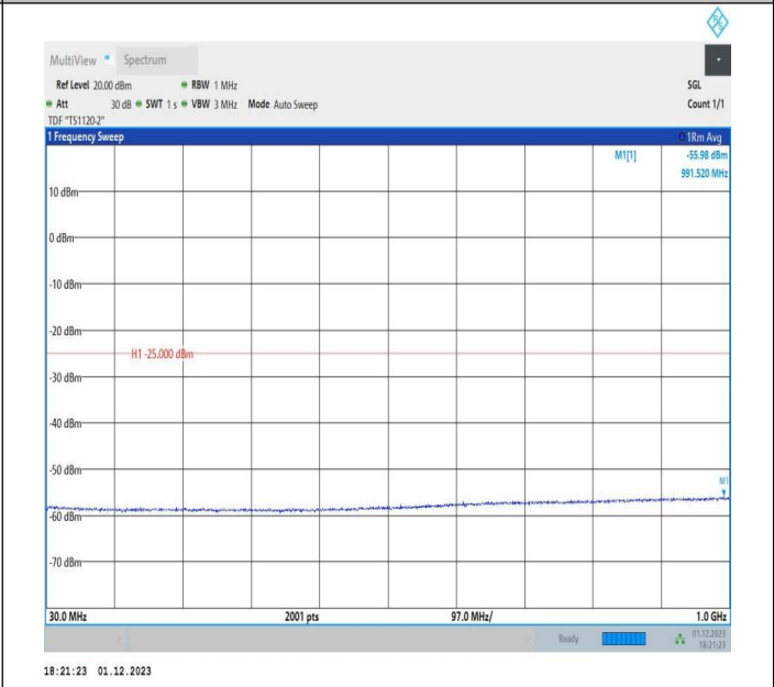
7-7-20MHz-10MHz-64QAM-64QAM-20850-20994-1RB#99-0R B#0-30~1000MHz-PASS
