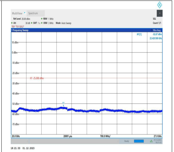
7-7-20MHz-10MHz-64QAM-64QAM-20850-20994-1RB#99-0R B#0-20000~27000MHz-PASS
