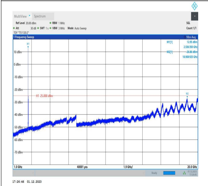
7-7-15MHz-20MHz-16QAM-16QAM-21179-21350-1RB#0-1RB #99-1000~20000MHz-PASS
