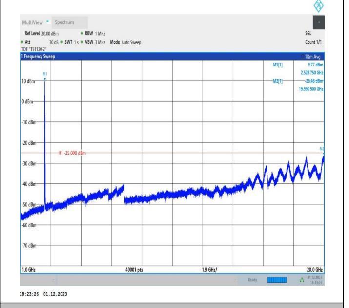
7-7-20MHz-10MHz-64QAM-64QAM-20850-20994-1RB#0-1RB #49-1000~20000MHz-PASS
