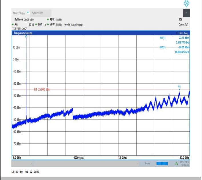
7-7-20MHz-10MHz-16QAM-16QAM-20850-20994-1RB#99-0R B#0-1000~20000MHz-PASS
