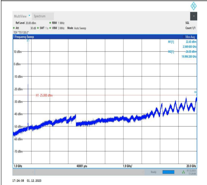
7-7-15MHz-20MHz-QPSK-QPSK-21179-21350-1RB#74-0RB# 0-1000~20000MHz-PASS
