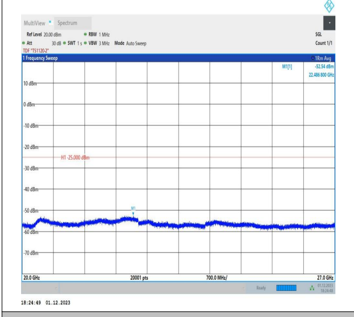
7-7-20MHz-10MHz-16QAM-16QAM-20850-20994-100RB#0-5 ORB#0-20000~27000MHz-PASS
