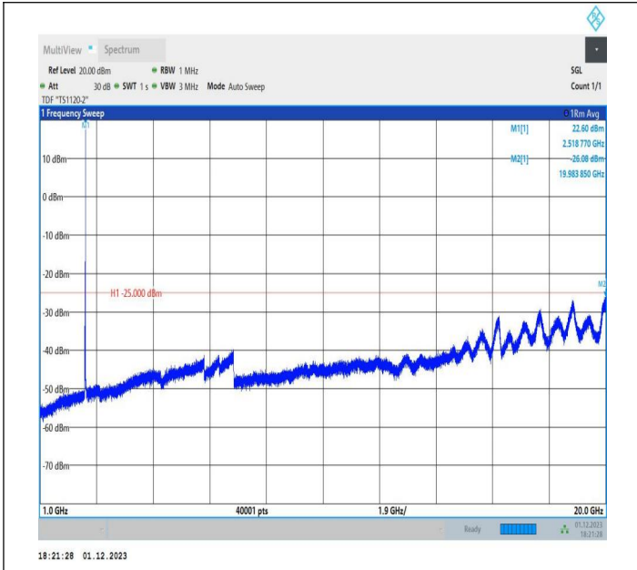
7-7-20MHz-10MHz-64QAM-64QAM-20850-20994-1RB#99-0R B#0-1000~20000MHz-PASS
