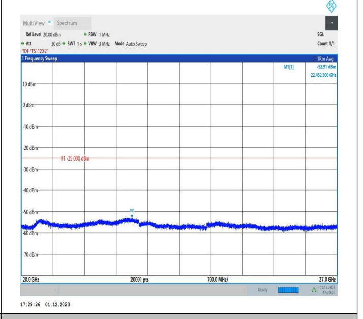
7-7-15MHz-20MHz-64QAM-64QAM-21179-21350-75RB#0-100 RB#0-20000~27000MHz-PASS
