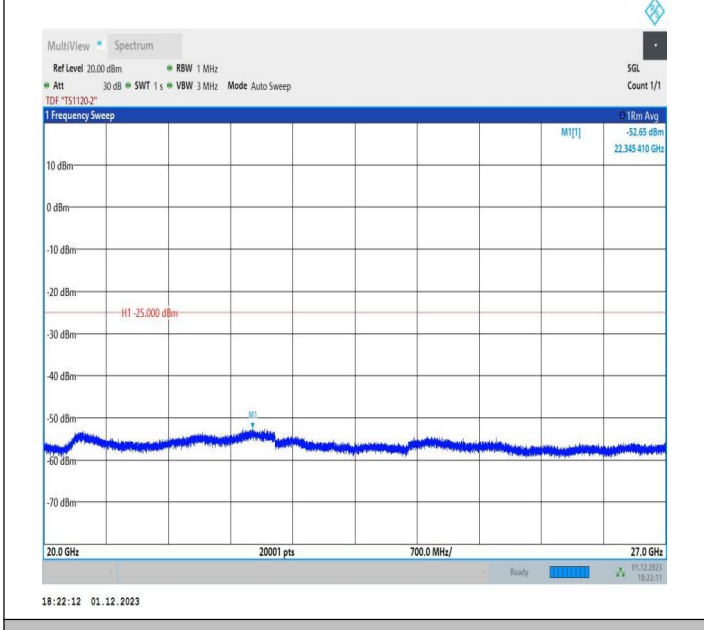
7-7-20MHz-10MHz-QPSK-QPSK-20850-20994-1RB#0-1RB#4 9-20000~27000MHz-PASS
