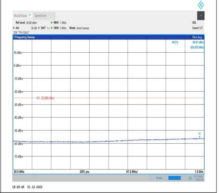
7-7-20MHz-10MHz-16QAM-16QAM-21051-21195-1RB#0-ORB#0-30~1000MHz-PASS
