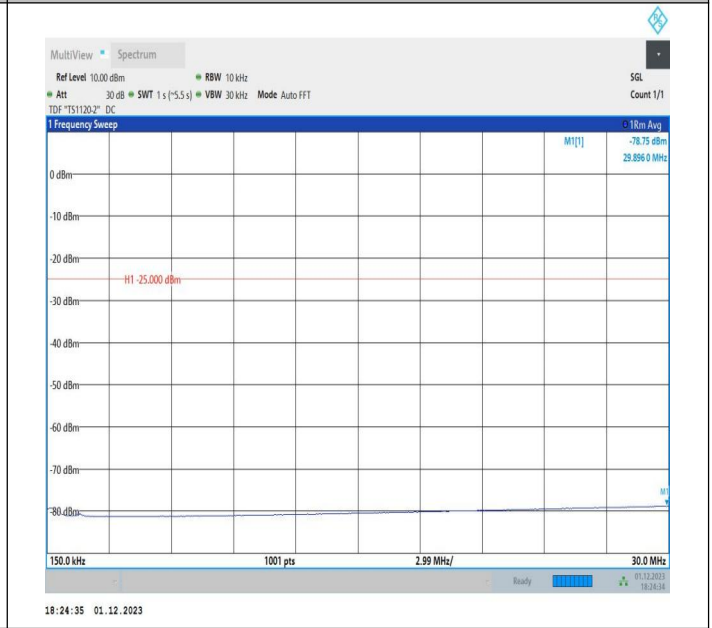
7-7-20MHz-10MHz-16QAM-16QAM-20850-20994-100RB#0-5 ORB#0-0.15~30MHz-PASS
