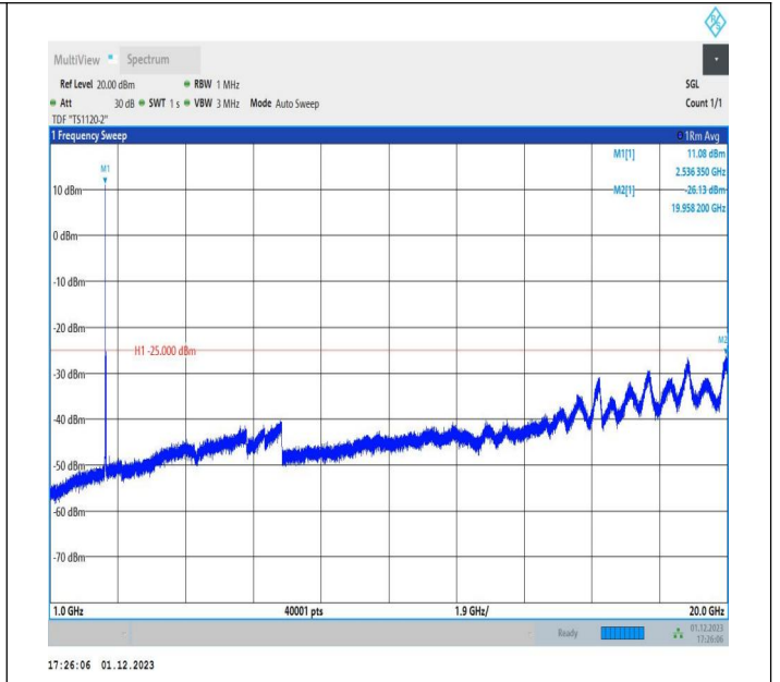
7-7-15MHz-20MHz-QPSK-QPSK-21179-21350-1RB#0-1RB#9 9-1000~20000MHz-PASS
