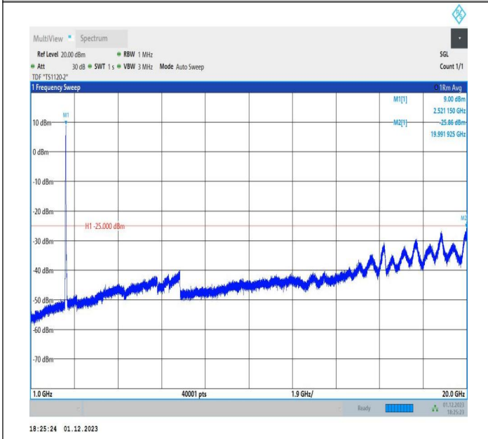
7-7-20MHz-10MHz-64QAM-64QAM-20850-20994-100RB#0-5 ORB#0-1000~20000MHz-PASS
