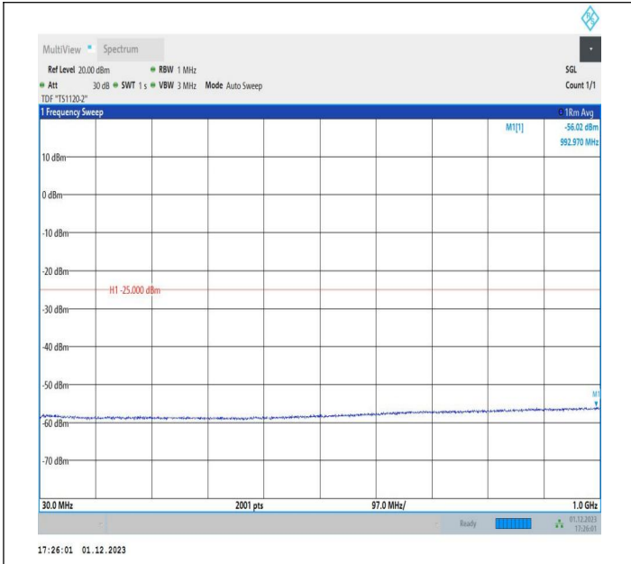
7-7-15MHz-20MHz-QPSK-QPSK-21179-21350-1RB#0-1RB#9 9-30~1000MHz-PASS
