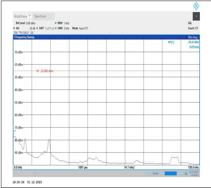
7-7-20MHz-10MHz-16QAM-16QAM-20850-20994-1RB#99-0R B#0-0.009~0.15MHz-PASS
