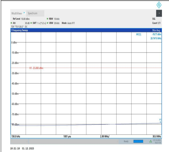
7-7-20MHz-10MHz-64QAM-64QAM-20850-20994-1RB#99-0R B#0-0.15~30MHz-PASS
