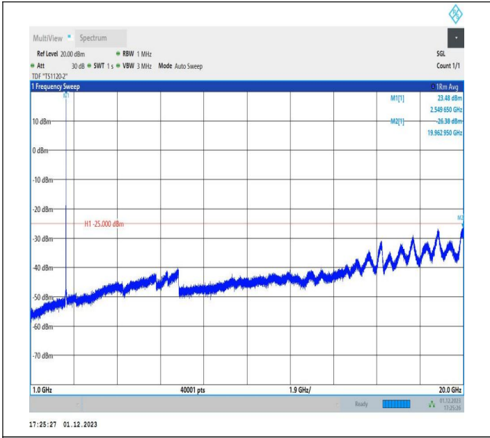
7-7-15MHz-20MHz-64QAM-64QAM-21179-21350-1RB#74-0R B#0-1000~20000MHz-PASS
