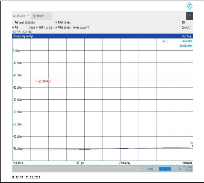
7-7-20MHz-10MHz-16QAM-16QAM-20850-20994-1RB#0-1RB #49-0.15~30MHz-PASS
