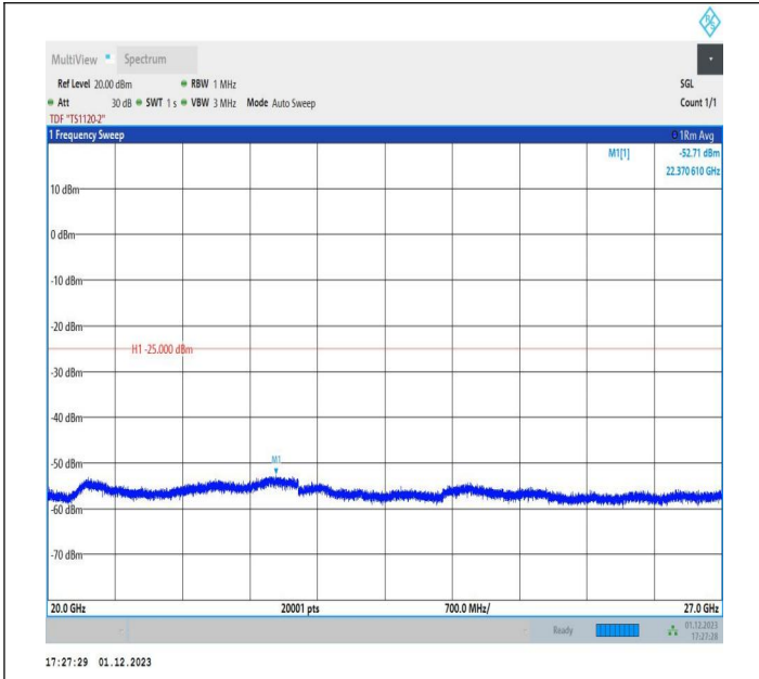
7-7-15MHz-20MHz-64QAM-64QAM-21179-21350-1RB#0-1RB #99-20000~27000MHz-PASS
