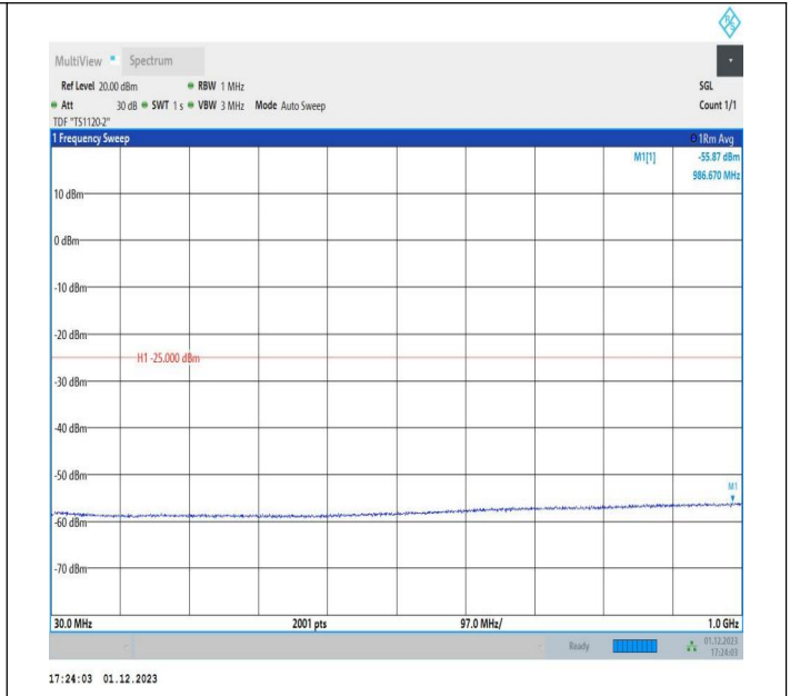
7-7-15MHz-20MHz-QPSK-QPSK-21179-21350-1RB#74-0RB# 0-30~1000MHz-PASS
