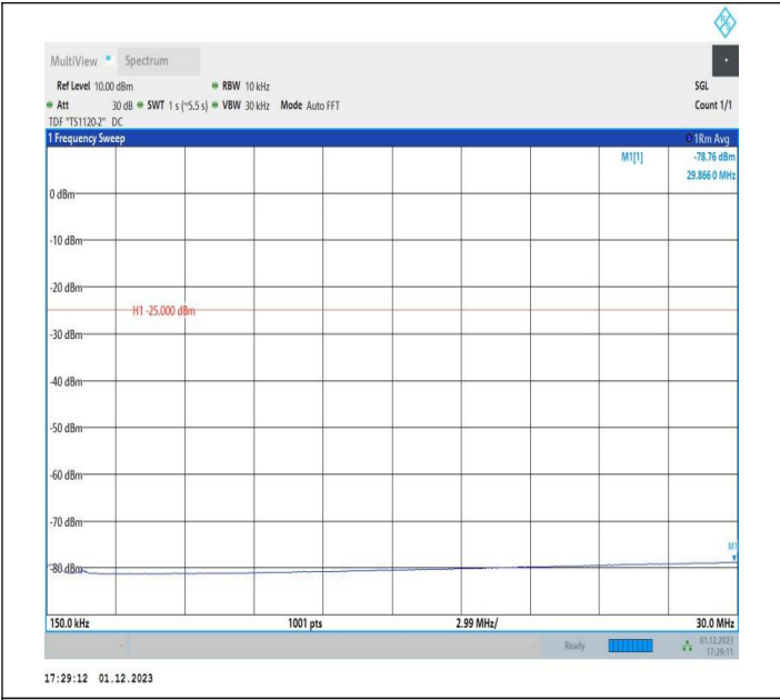
7-7-15MHz-20MHz-64QAM-64QAM-21179-21350-75RB#0-100 RB#0-0.15~30MHz-PASS
