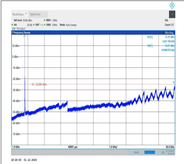
7-7-20MHz-10MHz-16QAM-16QAM-21051-21195-1RB#0-ORB #0-1000~20000MHz-PASS
