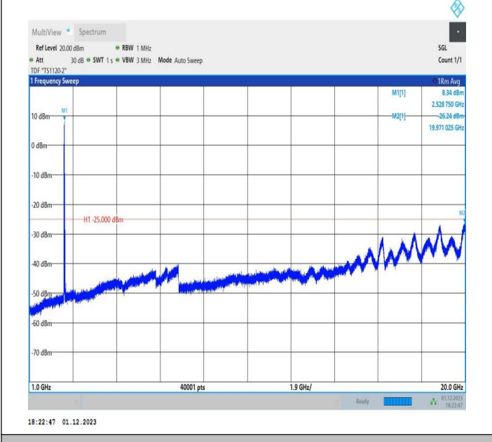
7-7-20MHz-10MHz-16QAM-16QAM-20850-20994-1RB#0-1RB #49-1000~20000MHz-PASS
