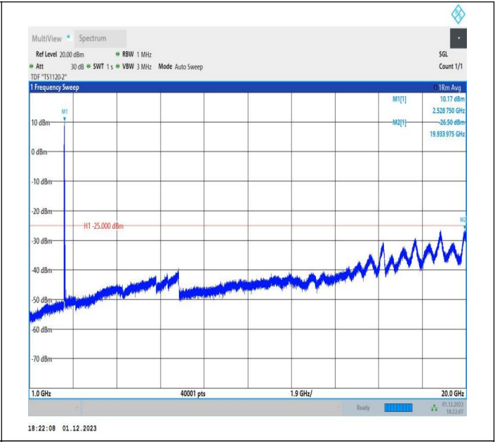
7-7-20MHz-10MHz-QPSK-QPSK-20850-20994-1RB#0-1RB#4 9-1000~20000MHz-PASS
