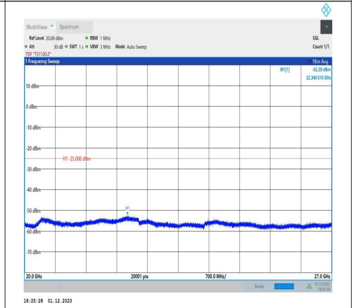
7-7-20MHz-10MHz-64QAM-64QAM-20850-20994-100RB#0-5 ORB#0-20000~27000MHz-PASS
