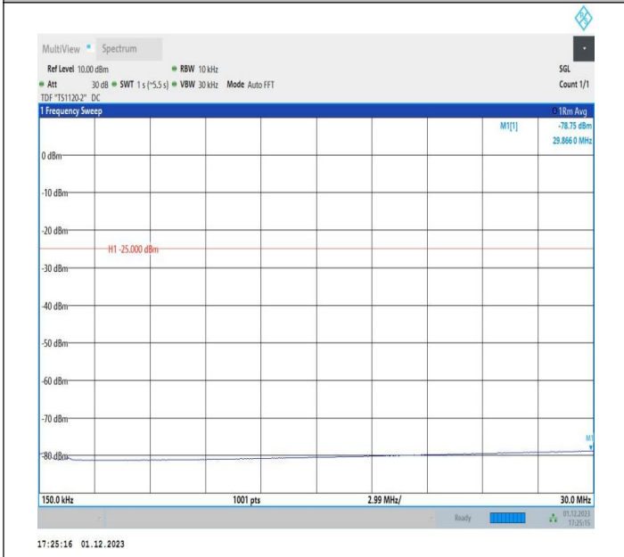
7-7-15MHz-20MHz-64QAM-64QAM-21179-21350-1RB#74-0R B#0-0.15~30MHz-PASS
