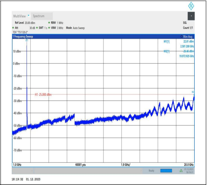
7-7-20MHz-10MHz-64QAM-64QAM-20850-20994-1RB#0-ORB #0-1000~20000MHz-PASS
