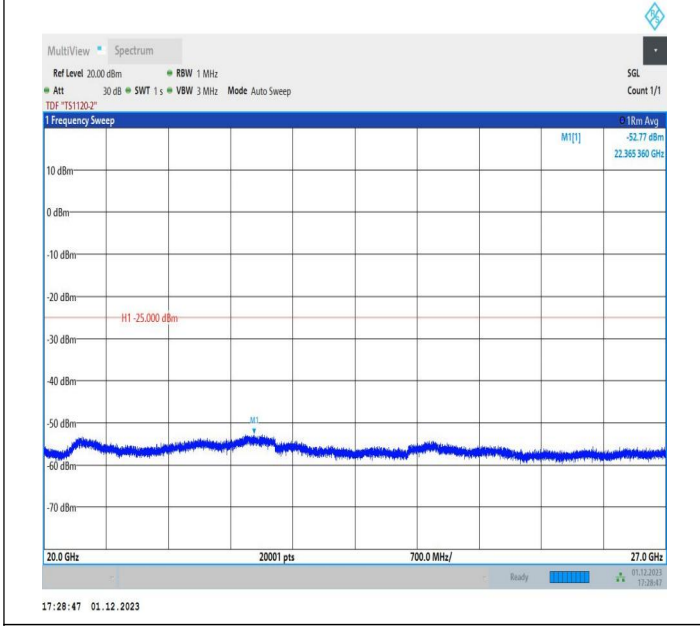
7-7-15MHz-20MHz-16QAM-16QAM-21179-21350-75RB#0-100 RB#0-20000~27000MHz-PASS
