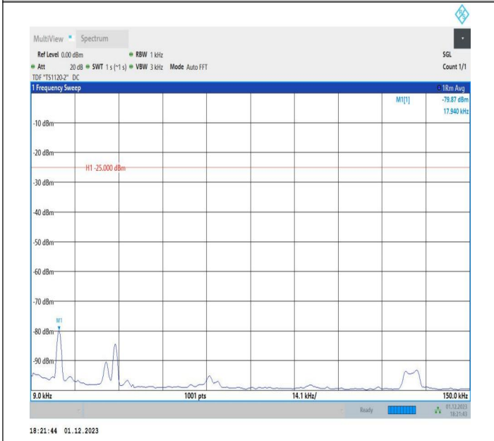
7-7-20MHz-10MHz-QPSK-QPSK-20850-20994-1RB#0-1RB#4 9-0.009~0.15MHz-PASS
