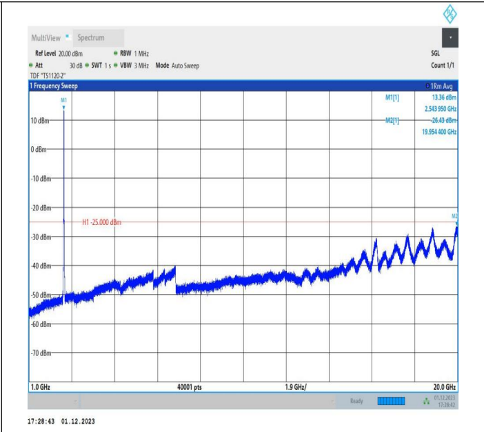
7-7-15MHz-20MHz-16QAM-16QAM-21179-21350-75RB#0-100 RB#0-1000~20000MHz-PASS
