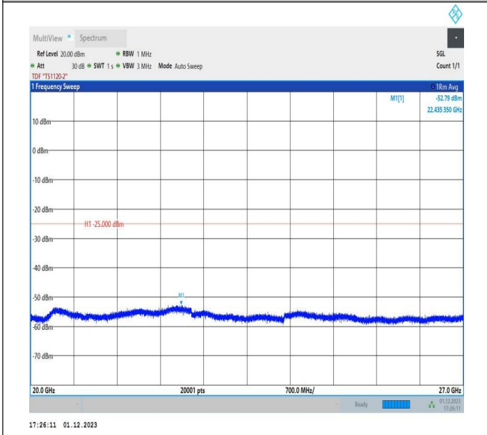
7-7-15MHz-20MHz-QPSK-QPSK-21179-21350-1RB#0-1RB#9 9-20000~27000MHz-PASS
