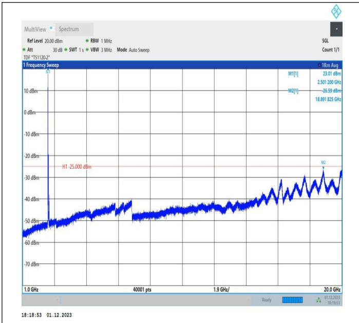
7-7-20MHz-10MHz-16QAM-16QAM-20850-20994-1RB#0-ORB #0-1000~20000MHz-PASS
