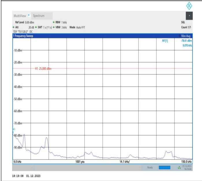
7-7-20MHz-10MHz-64QAM-64QAM-20850-20994-1RB#0-ORB #0-0.009~0.15MHz-PASS
