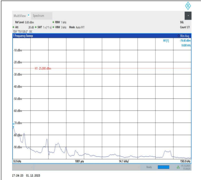
7-7-15MHz-20MHz-16QAM-16QAM-21179-21350-1RB#74-0R B#0-0.009~0.15MHz-PASS
