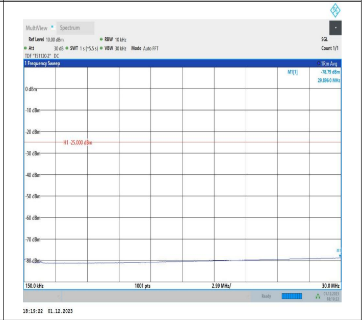
7-7-20MHz-10MHz-64QAM-64QAM-20850-20994-1RB#0-ORB #0-0.15~30MHz-PASS
