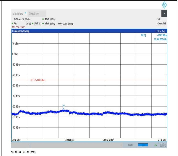
7-7-20MHz-10MHz-16QAM-16QAM-21051-21195-1RB#0-ORB #0-20000~27000MHz-PASS
