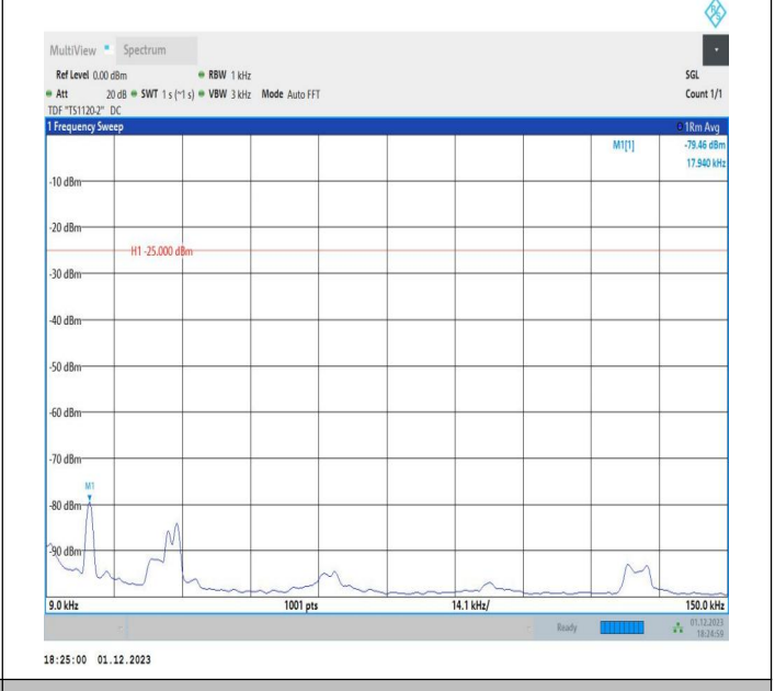
7-7-20MHz-10MHz-64QAM-64QAM-20850-20994-100RB#0-5 ORB#0-0.009~0.15MHz-PASS
