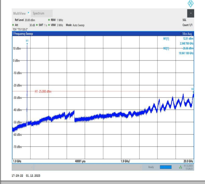
7-7-15MHz-20MHz-64QAM-64QAM-21179-21350-75RB#0-100 RB#0-1000~20000MHz-PASS
