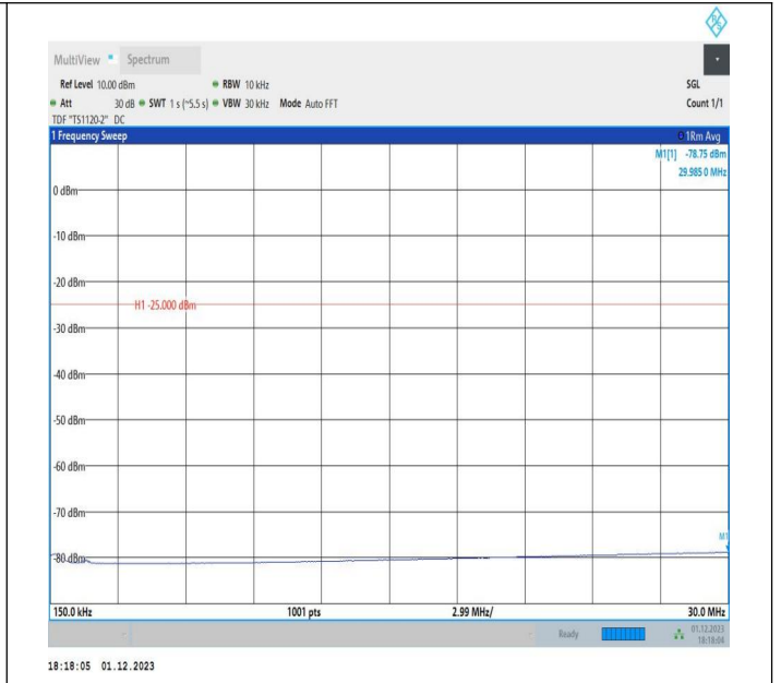
7-7-20MHz-10MHz-QPSK-QPSK-20850-20994-1RB#0-0RB#0 -0.15~30MHz-PASS
