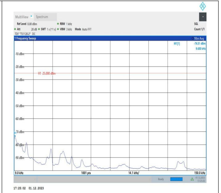
7-7-15MHz-20MHz-64QAM-64QAM-21179-21350-1RB#74-0R B#0-0.009~0.15MHz-PASS
