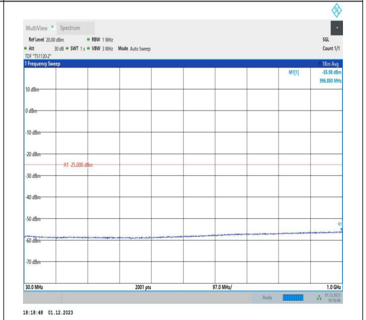
7-7-20MHz-10MHz-16QAM-16QAM-20850-20994-1RB#0-0RB #0-30~1000MHz-PASS
