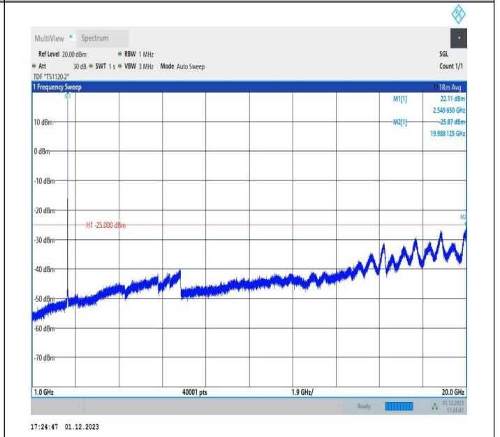
7-7-15MHz-20MHz-16QAM-16QAM-21179-21350-1RB#74-0R B#0-1000~20000MHz-PASS
