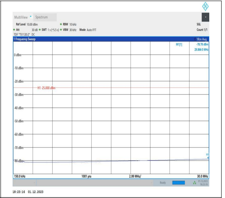
7-7-20MHz-10MHz-64QAM-64QAM-20850-20994-1RB#0-1RB #49-0.15~30MHz-PASS
