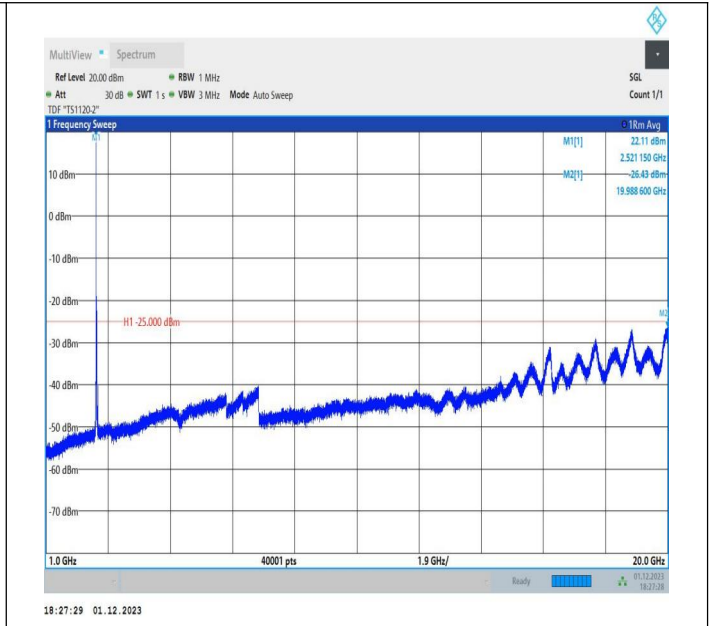
7-7-20MHz-10MHz-64QAM-64QAM-21051-21195-1RB#0-ORB #0-1000~20000MHz-PASS
