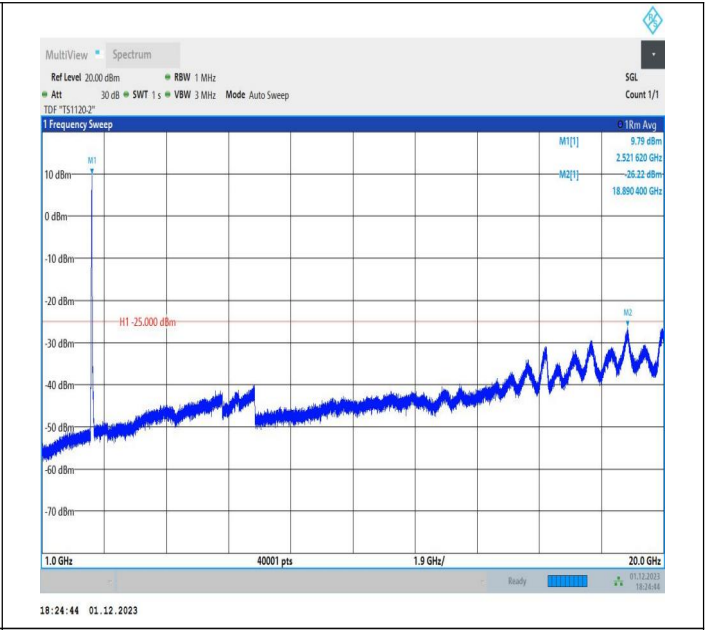
7-7-20MHz-10MHz-16QAM-16QAM-20850-20994-100RB#0-5 ORB#0-1000~20000MHz-PASS
