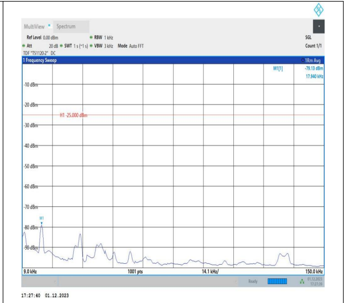
7-7-15MHz-20MHz-QPSK-QPSK-21179-21350-75RB#0-100R B#0-0.009~0.15MHz-PASS
