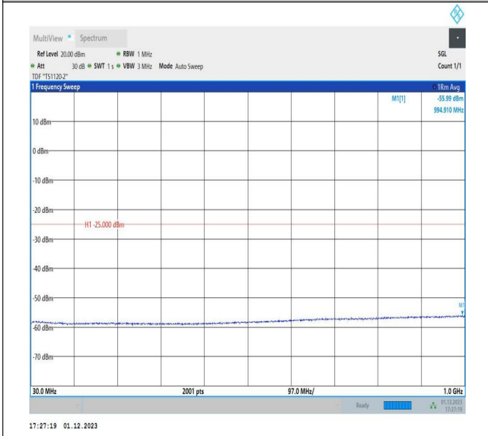
7-7-15MHz-20MHz-64QAM-64QAM-21179-21350-1RB#0-1RB #99-30~1000MHz-PASS
