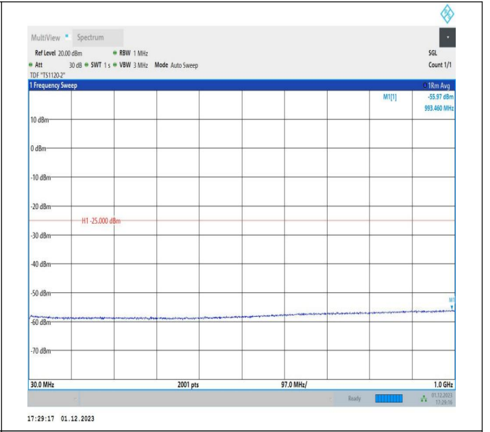
7-7-15MHz-20MHz-64QAM-64QAM-21179-21350-75RB#0-100 RB#0-30~1000MHz-PASS
