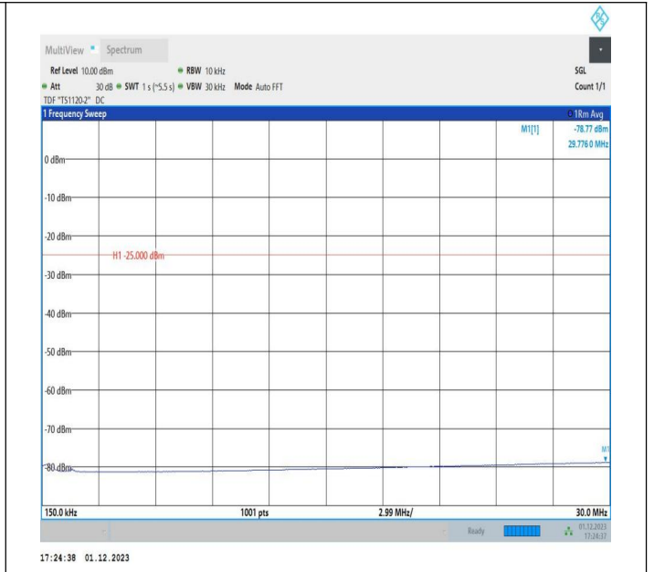
7-7-15MHz-20MHz-16QAM-16QAM-21179-21350-1RB#74-0R B#0-0.15~30MHz-PASS
