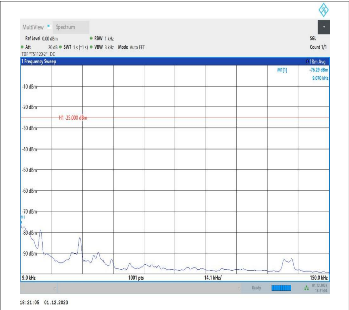
7-7-20MHz-10MHz-64QAM-64QAM-20850-20994-1RB#99-0R B#0-0.009~0.15MHz-PASS
