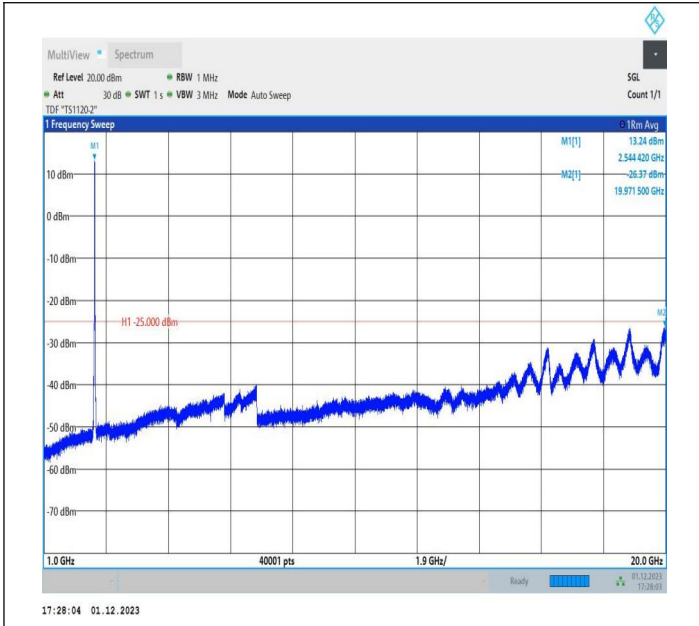
7-7-15MHz-20MHz-QPSK-QPSK-21179-21350-75RB#0-100R B#0-1000~20000MHz-PASS
