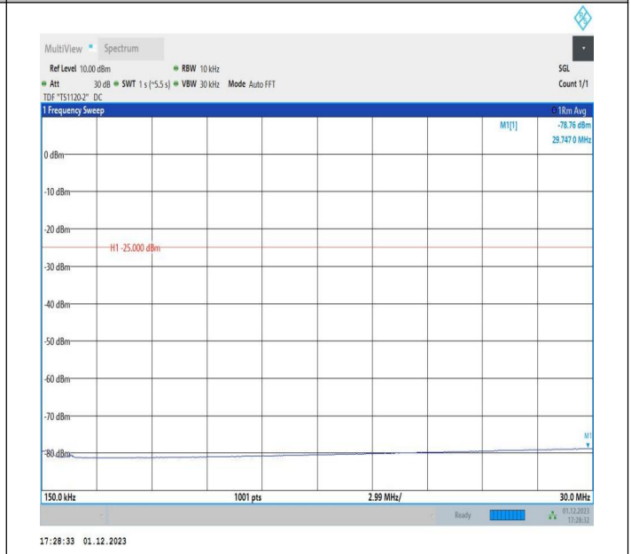
7-7-15MHz-20MHz-16QAM-16QAM-21179-21350-75RB#0-100 RB#0-0.15~30MHz-PASS
