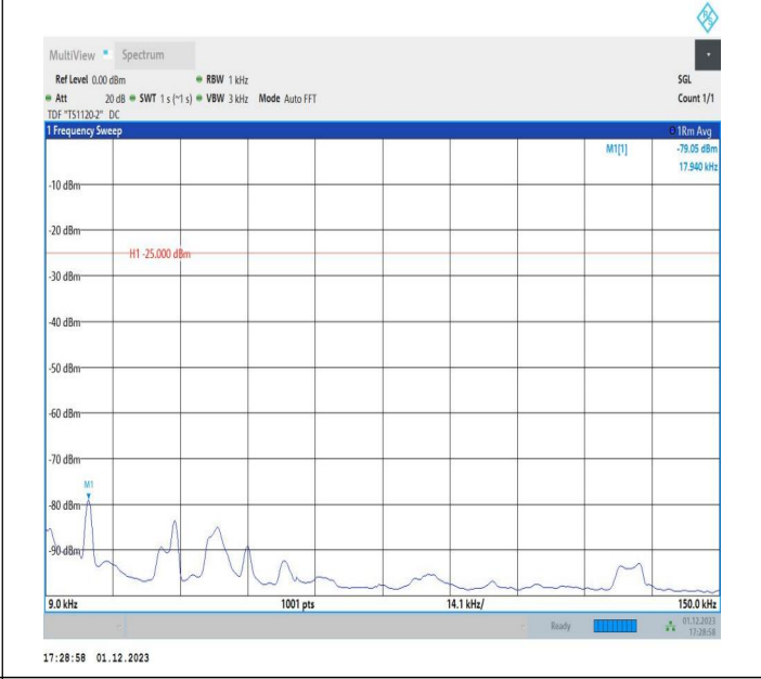
7-7-15MHz-20MHz-64QAM-64QAM-21179-21350-75RB#0-100 RB#0-0.009~0.15MHz-PASS
