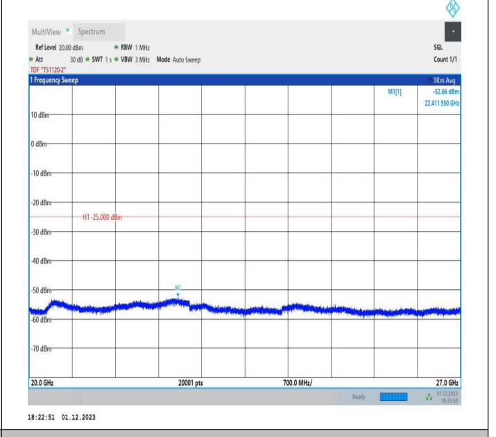
7-7-20MHz-10MHz-16QAM-16QAM-20850-20994-1RB#0-1RB #49-20000~27000MHz-PASS
