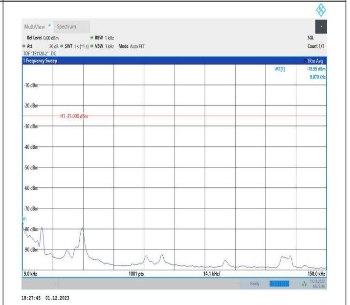
7-7-20MHz-10MHz-QPSK-QPSK-21051-21195-1RB#99-ORB# 0-0.009~0.15MHz-PASS
