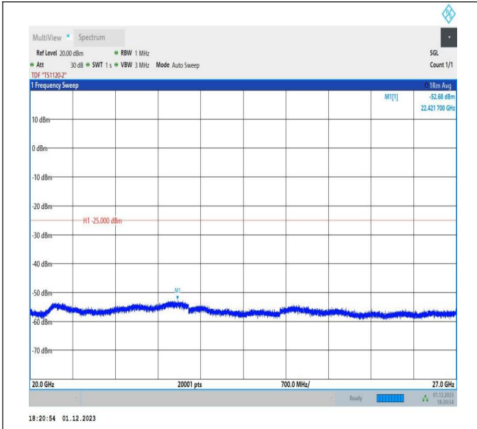
7-7-20MHz-10MHz-16QAM-16QAM-20850-20994-1RB#99-0R B#0-20000~27000MHz-PASS
