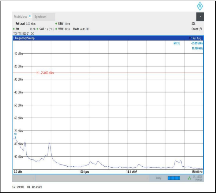
7-7-15MHz-20MHz-64QAM-64QAM-20828-20999-1RB#74-0R B#0-0.009~0.15MHz-PASS
