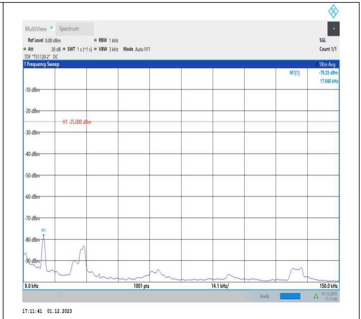
7-7-15MHz-20MHz-QPSK-QPSK-20828-20999-75RB#0-100R B#0-0.009~0.15MHz-PASS
