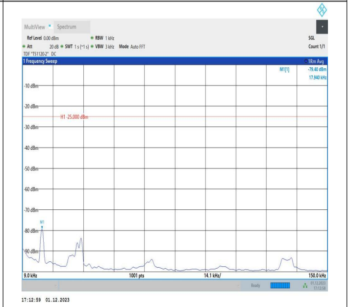
7-7-15MHz-20MHz-64QAM-64QAM-20828-20999-75RB#0-10 ORB#0-0.009~0.15MHz-PASS
