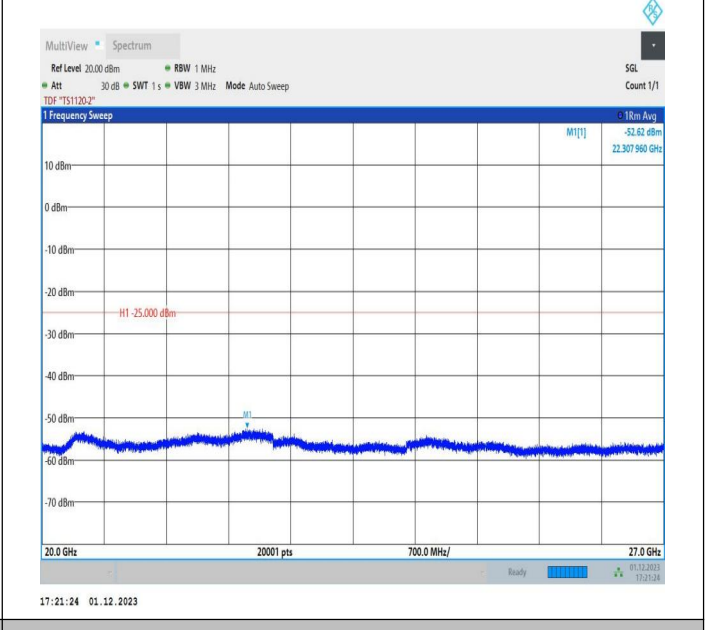
7-7-15MHz-20MHz-64QAM-64QAM-21003-21174-75RB#0-100 RB#0-20000~27000MHz-PASS
