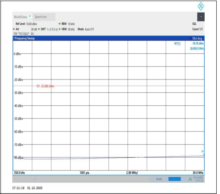
7-7-15MHz-20MHz-64QAM-64QAM-20828-20999-1RB#0-1RB #99-0.15~30MHz-PASS
