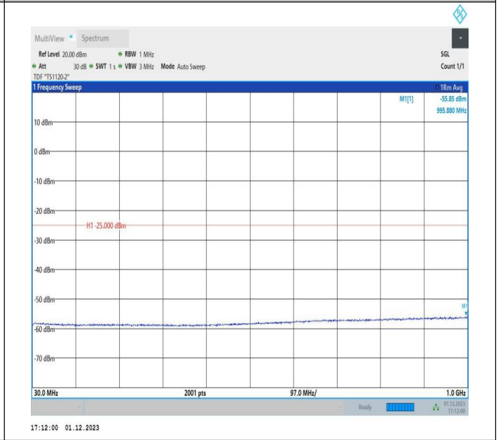
7-7-15MHz-20MHz-QPSK-QPSK-20828-20999-75RB#0-100R B#0-30~1000MHz-PASS
