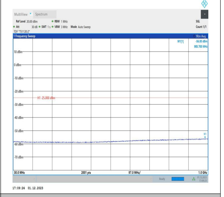
7-7-15MHz-20MHz-64QAM-64QAM-20828-20999-1RB#74-0R B#0-30~1000MHz-PASS
