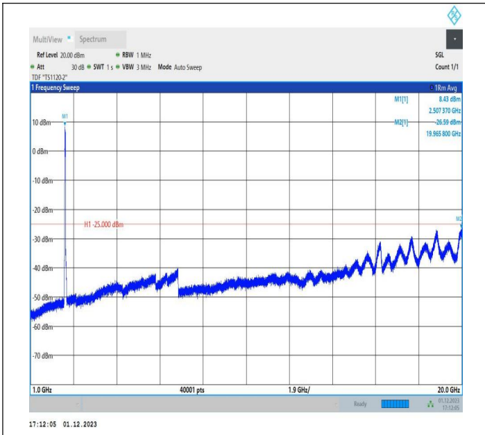
7-7-15MHz-20MHz-QPSK-QPSK-20828-20999-75RB#0-100R B#0-1000~20000MHz-PASS
