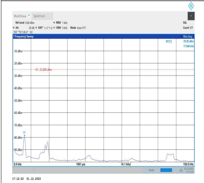
7-7-15MHz-20MHz-16QAM-16QAM-20828-20999-75RB#0-10 ORB#0-0.009~0.15MHz-PASS
