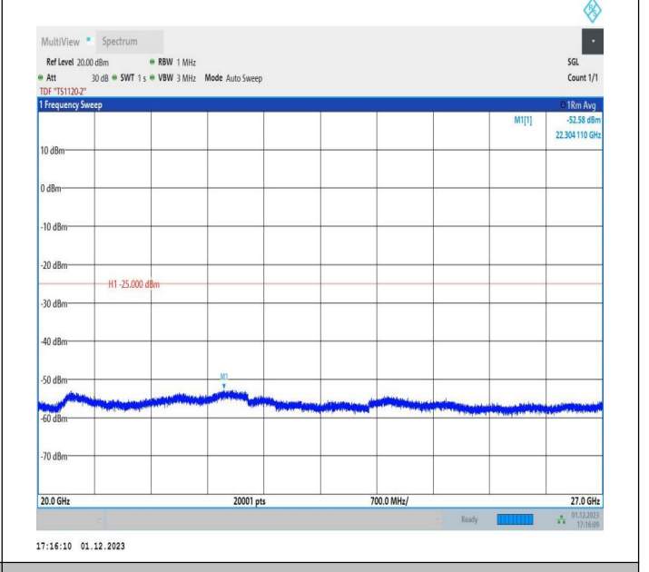
7-7-15MHz-20MHz-QPSK-QPSK-21003-21174-1RB#74-0RB# 0-20000~27000MHz-PASS
