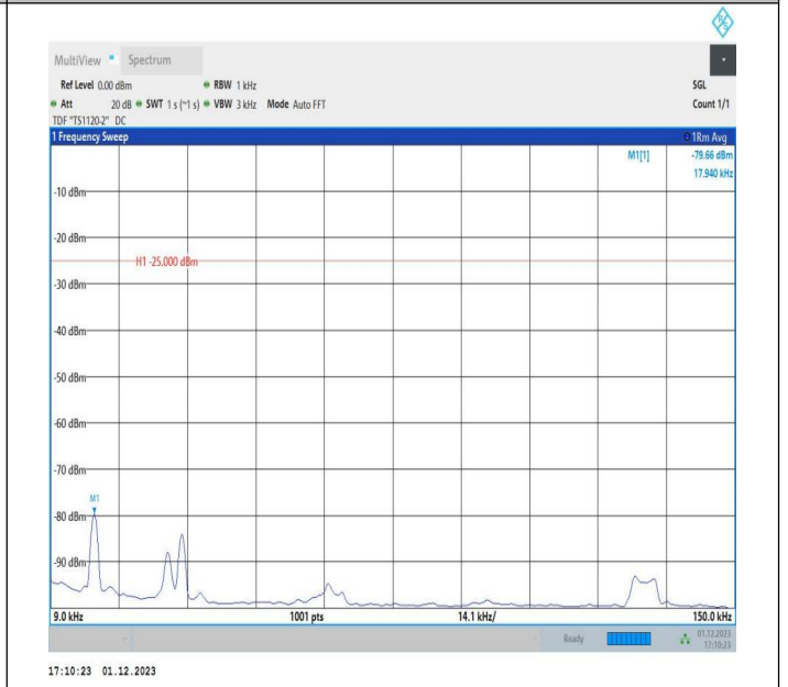
7-7-15MHz-20MHz-16QAM-16QAM-20828-20999-1RB#0-1RB #99-0.009~0.15MHz-PASS
