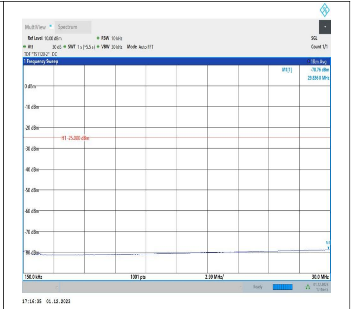
7-7-15MHz-20MHz-16QAM-16QAM-21003-21174-1RB#74-0R B#0-0.15~30MHz-PASS
