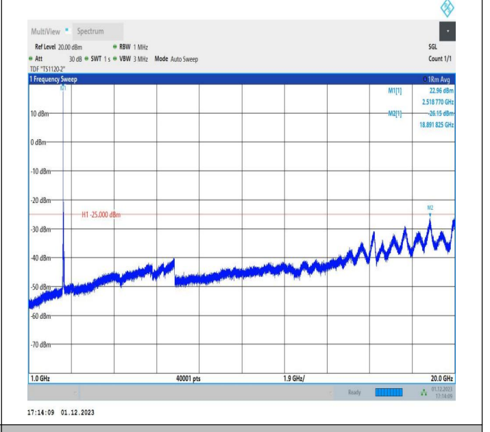
7-7-15MHz-20MHz-QPSK-QPSK-21003-21174-1RB#0-ORB#0-1000~20000MHz-PASS
