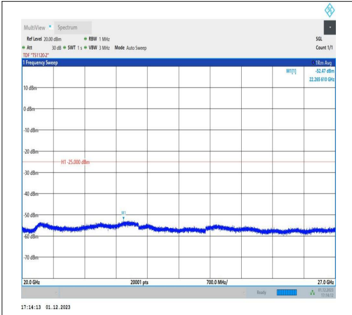
7-7-15MHz-20MHz-QPSK-QPSK-21003-21174-1RB#0-ORB#0-20000~27000MHz-PASS
