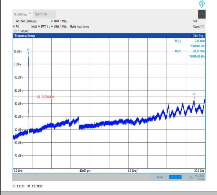
7-7-15MHz-20MHz-64QAM-64QAM-20828-20999-75RB#0-10 ORB#0-1000~20000MHz-PASS
