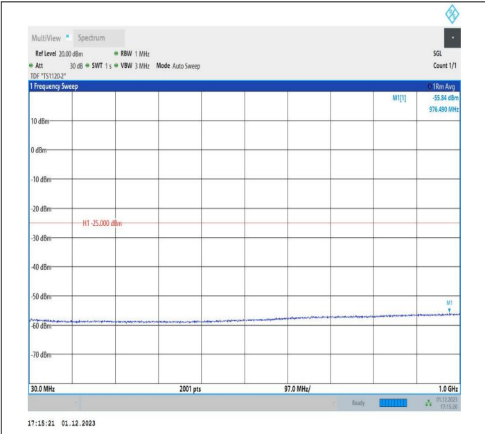
7-7-15MHz-20MHz-64QAM-64QAM-21003-21174-1RB#0-ORB #0-30~1000MHz-PASS
