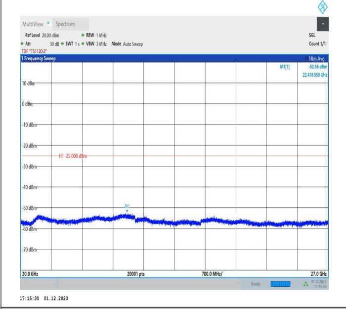
7-7-15MHz-20MHz-64QAM-64QAM-21003-21174-1RB#0-ORB #0-20000~27000MHz-PASS
