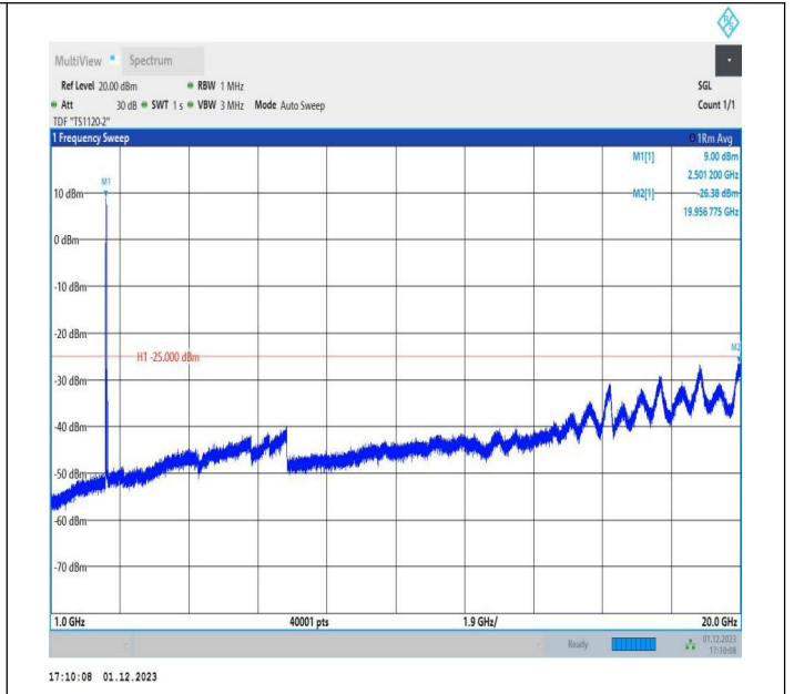
7-7-15MHz-20MHz-QPSK-QPSK-20828-20999-1RB#0-1RB#9 9-1000~20000MHz-PASS
