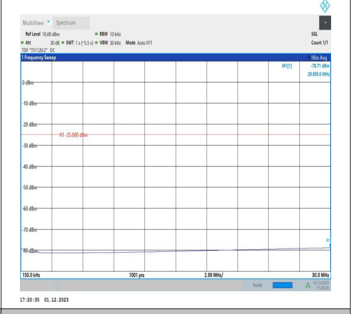
7-7-15MHz-20MHz-16QAM-16QAM-21003-21174-75RB#0-100 RB#0-0.15~30MHz-PASS
