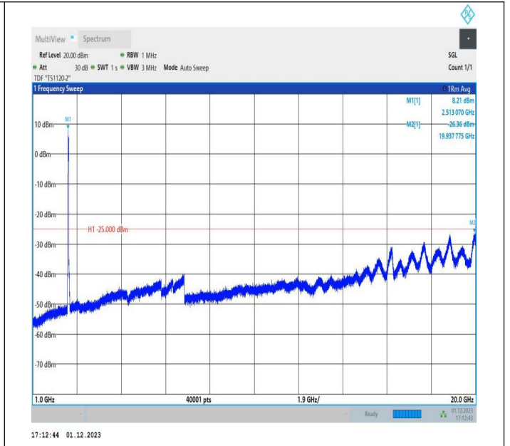
7-7-15MHz-20MHz-16QAM-16QAM-20828-20999-75RB#0-10 ORB#0-1000~20000MHz-PASS
