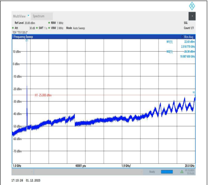
7-7-15MHz-20MHz-64QAM-64QAM-21003-21174-1RB#0-ORB #0-1000~20000MHz-PASS
