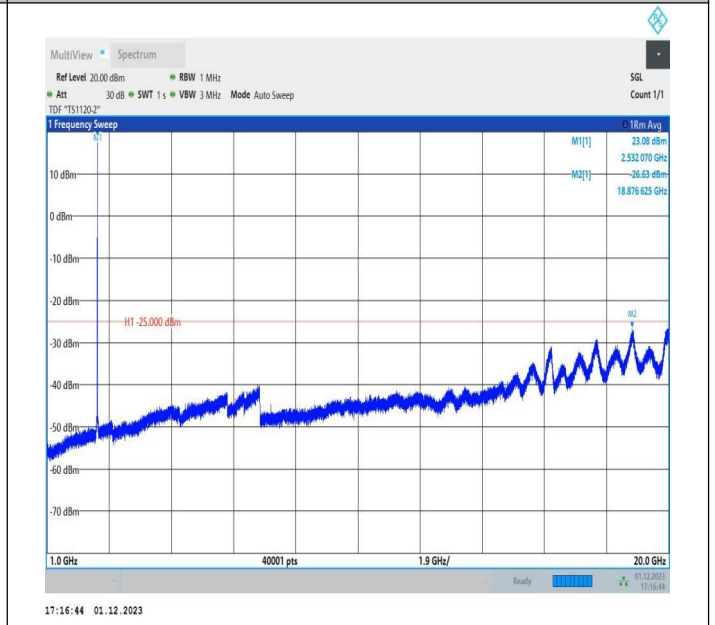
7-7-15MHz-20MHz-16QAM-16QAM-21003-21174-1RB#74-0R B#0-1000~20000MHz-PASS
