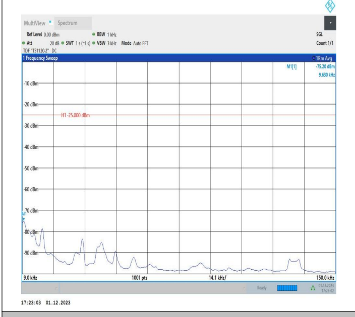
7-7-15MHz-20MHz-64QAM-64QAM-21179-21350-1RB#0-ORB #0-0.009~0.15MHz-PASS
