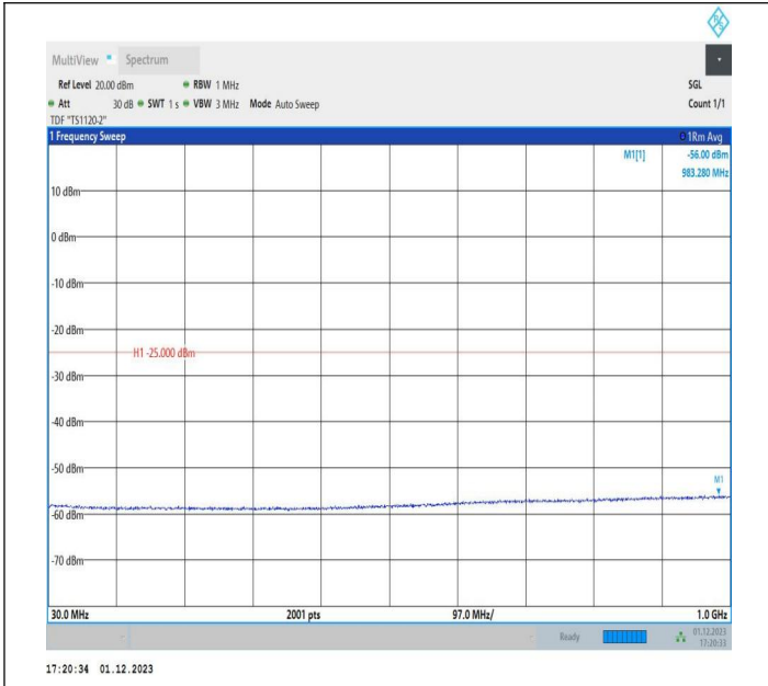
7-7-15MHz-20MHz-16QAM-16QAM-21003-21174-75RB#0-100 RB#0-30~1000MHz-PASS
