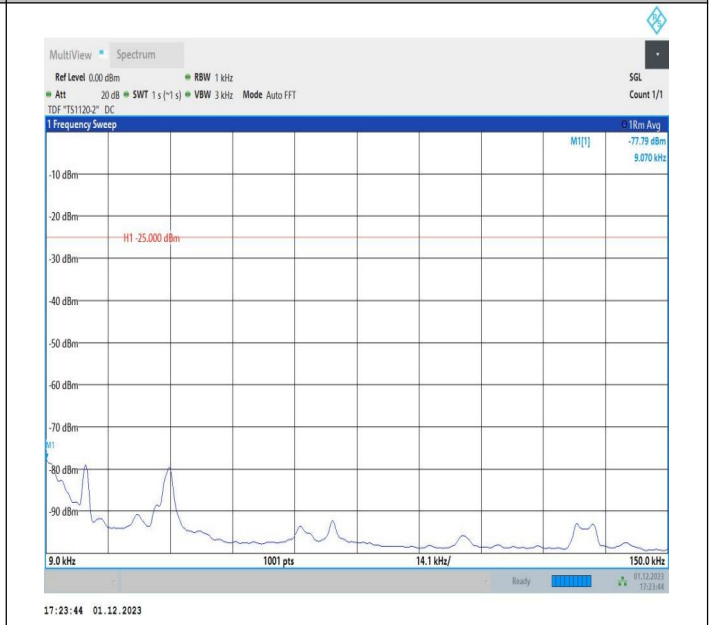
7-7-15MHz-20MHz-QPSK-QPSK-21179-21350-1RB#74-ORB# 0-0.009~0.15MHz-PASS
