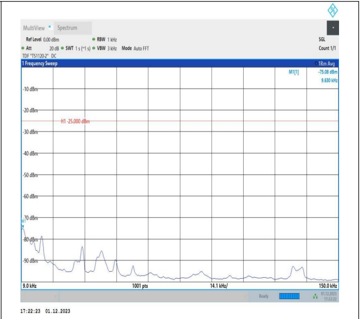
7-7-15MHz-20MHz-16QAM-16QAM-21179-21350-1RB#0-ORB#0-0.009~0.15MHz-PASS
