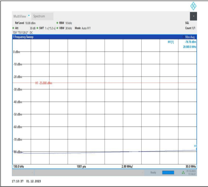
7-7-15MHz-20MHz-16QAM-16QAM-20828-20999-1RB#0-1RB #99-0.15~30MHz-PASS
