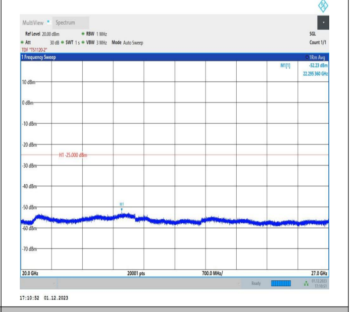
7-7-15MHz-20MHz-16QAM-16QAM-20828-20999-1RB#0-1RB #99-20000~27000MHz-PASS
