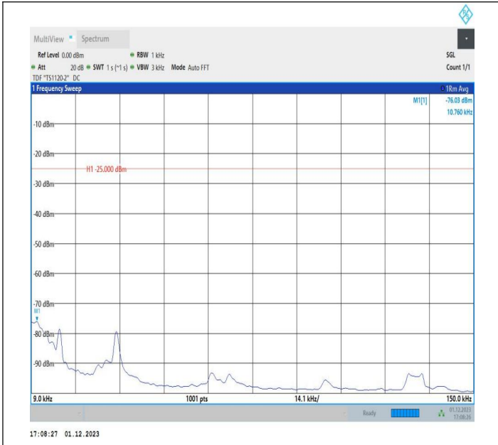
7-7-15MHz-20MHz-16QAM-16QAM-20828-20999-1RB#74-0R B#0-0.009~0.15MHz-PASS
