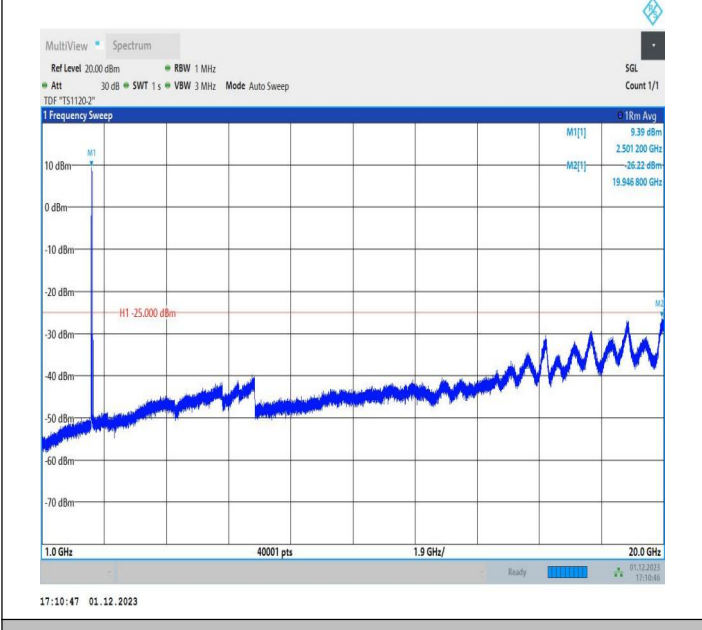
7-7-15MHz-20MHz-16QAM-16QAM-20828-20999-1RB#0-1RB #99-1000~20000MHz-PASS
