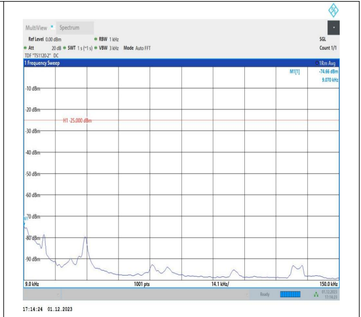
7-7-15MHz-20MHz-16QAM-16QAM-21003-21174-1RB#0-ORB#0-0.009~0.15MHz-PASS
