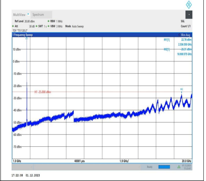
7-7-15MHz-20MHz-QPSK-QPSK-21179-21350-1RB#0-ORB#0-1000~20000MHz-PASS
