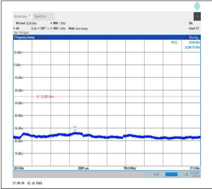
7-7-15MHz-20MHz-16QAM-16QAM-20828-20999-1RB#74-0R B#0-20000~27000MHz-PASS
