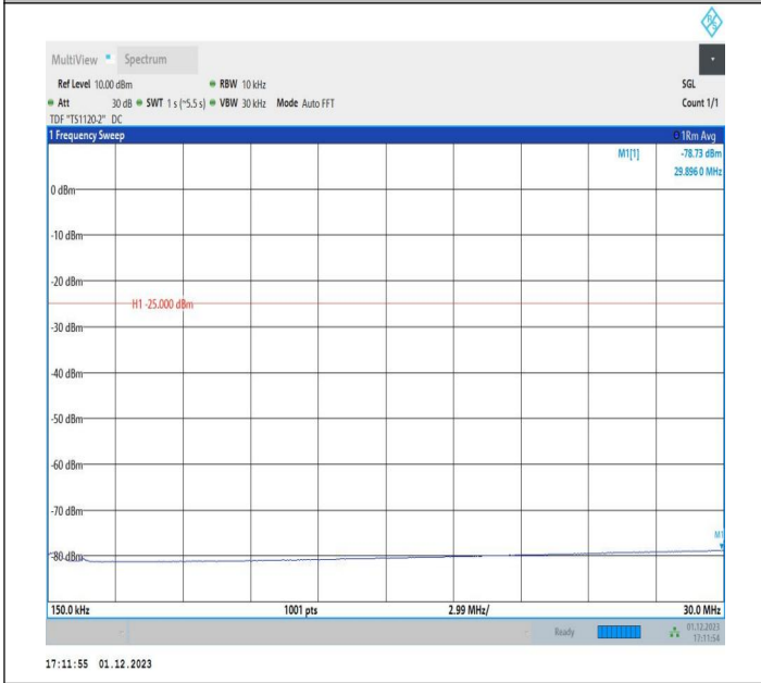
7-7-15MHz-20MHz-QPSK-QPSK-20828-20999-75RB#0-100R B#0-0.15~30MHz-PASS
