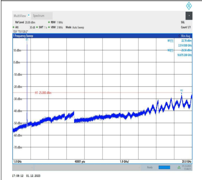
7-7-15MHz-20MHz-QPSK-QPSK-20828-20999-1RB#74-0RB# 0-1000~20000MHz-PASS
