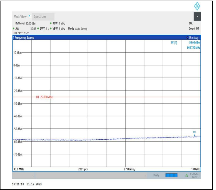
7-7-15MHz-20MHz-64QAM-64QAM-21003-21174-75RB#0-100 RB#0-30~1000MHz-PASS
