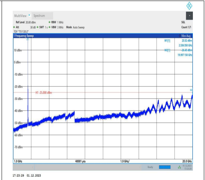
7-7-15MHz-20MHz-64QAM-64QAM-21179-21350-1RB#0-ORB #0-1000~20000MHz-PASS
