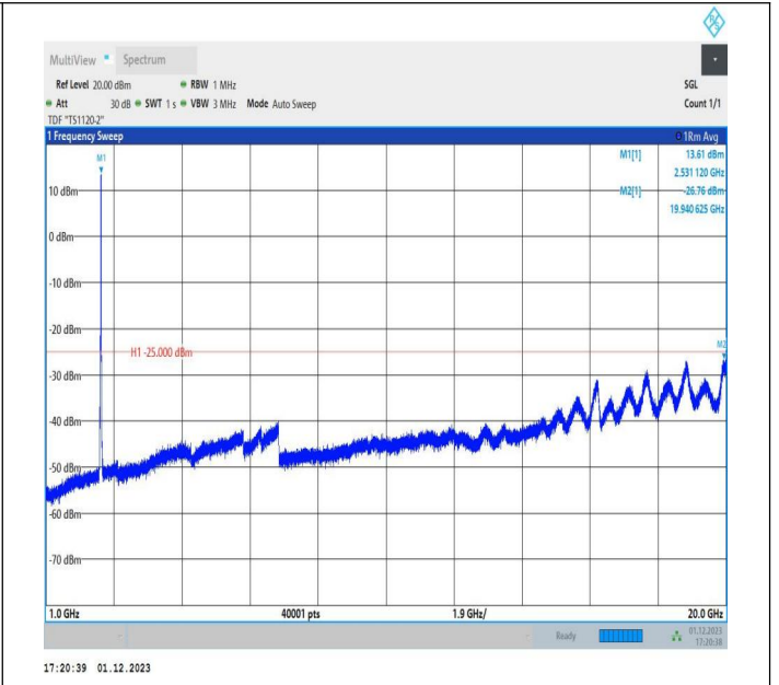
7-7-15MHz-20MHz-16QAM-16QAM-21003-21174-75RB#0-100 RB#0-1000~20000MHz-PASS
