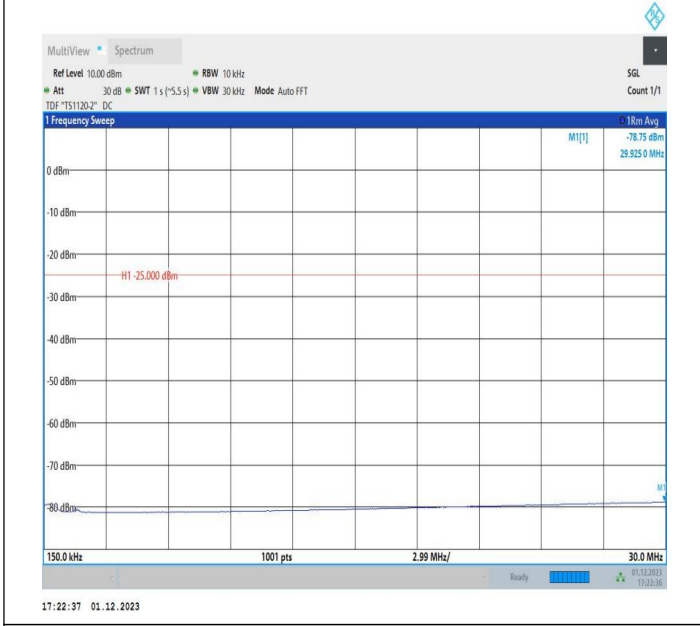
7-7-15MHz-20MHz-16QAM-16QAM-21179-21350-1RB#0-ORB#0-0.15~30MHz-PASS
