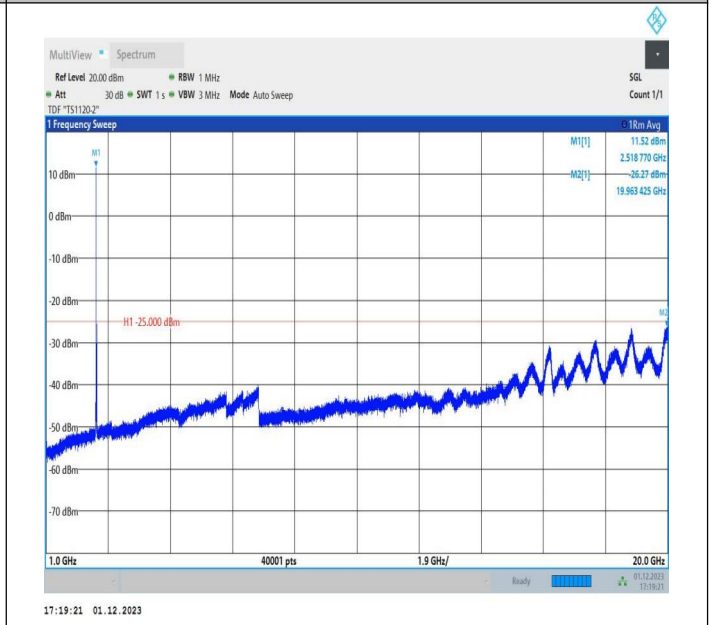
7-7-15MHz-20MHz-64QAM-64QAM-21003-21174-1RB#0-1RB #99-1000~20000MHz-PASS
