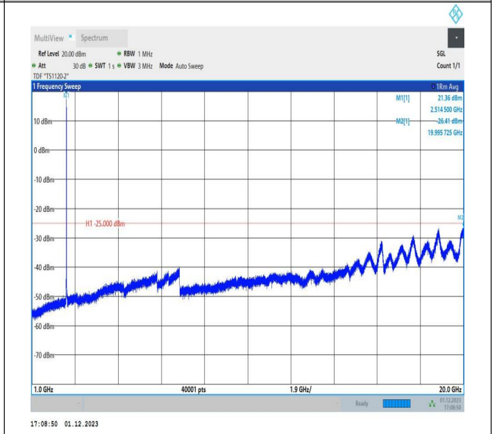
7-7-15MHz-20MHz-16QAM-16QAM-20828-20999-1RB#74-0R B#0-1000~20000MHz-PASS
