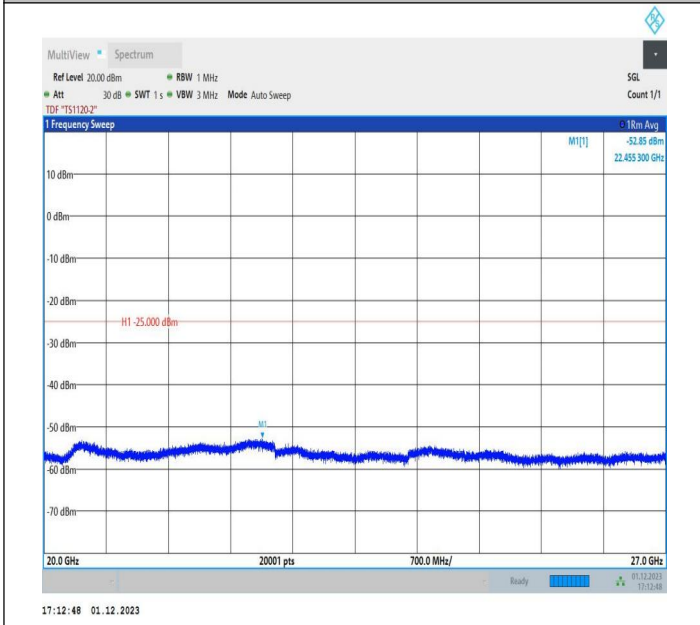
7-7-15MHz-20MHz-16QAM-16QAM-20828-20999-75RB#0-10 ORB#0-20000~27000MHz-PASS
