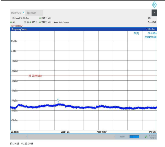
7-7-15MHz-20MHz-QPSK-QPSK-20828-20999-1RB#0-1RB#9 9-20000~27000MHz-PASS
