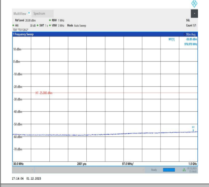
7-7-15MHz-20MHz-QPSK-QPSK-21003-21174-1RB#0-ORB#0-30~1000MHz-PASS
