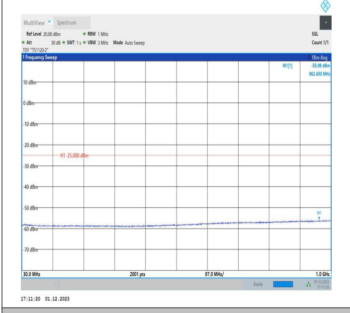
7-7-15MHz-20MHz-64QAM-64QAM-20828-20999-1RB#0-1RB #99-30~1000MHz-PASS
