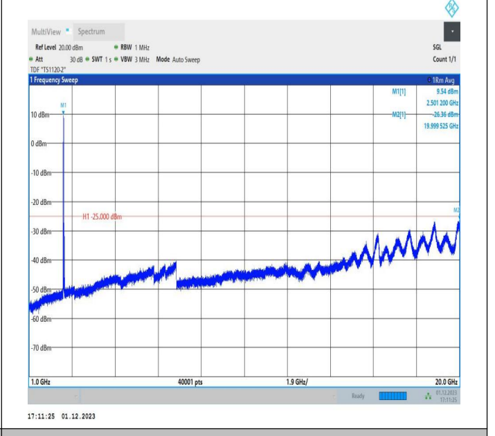
7-7-15MHz-20MHz-64QAM-64QAM-20828-20999-1RB#0-1RB #99-1000~20000MHz-PASS
