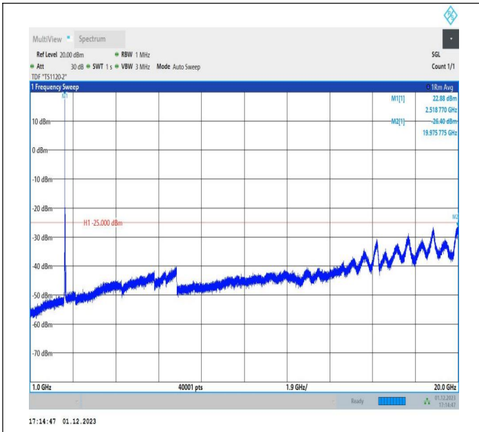
7-7-15MHz-20MHz-16QAM-16QAM-21003-21174-1RB#0-ORB #0-1000~20000MHz-PASS
