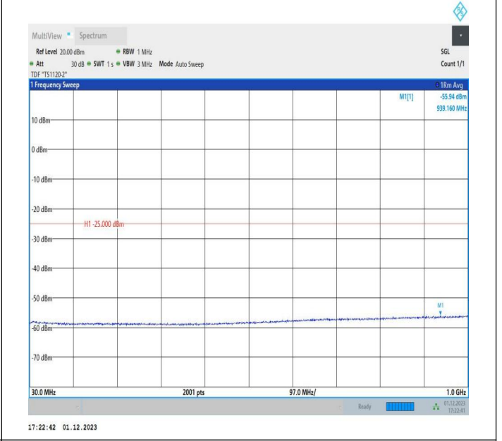
7-7-15MHz-20MHz-16QAM-16QAM-21179-21350-1RB#0-ORB#0-30~1000MHz-PASS
