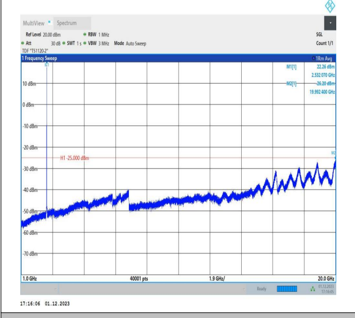
7-7-15MHz-20MHz-QPSK-QPSK-21003-21174-1RB#74-0RB# 0-1000~20000MHz-PASS
