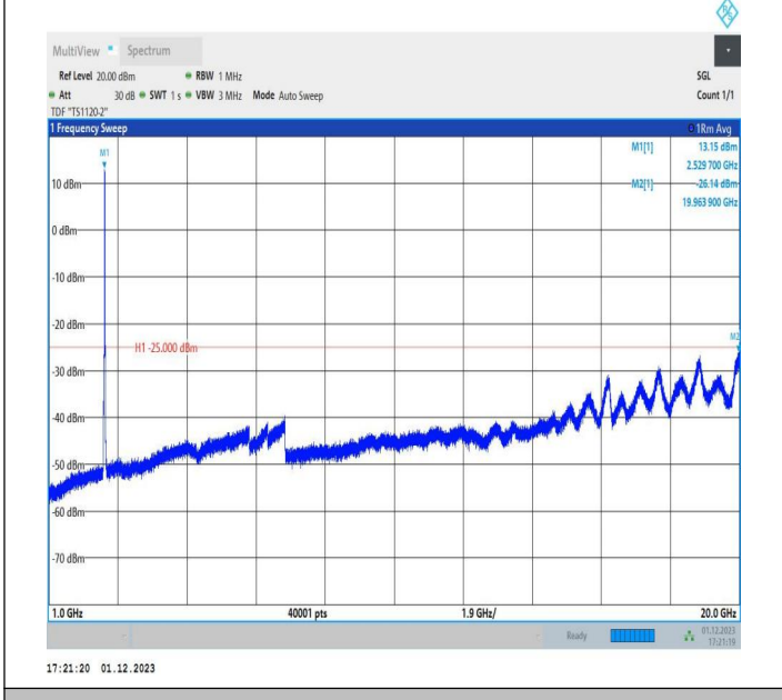
7-7-15MHz-20MHz-64QAM-64QAM-21003-21174-75RB#0-100 RB#0-1000~20000MHz-PASS
