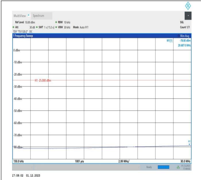
7-7-15MHz-20MHz-QPSK-QPSK-20828-20999-1RB#74-0RB# 0-0.15~30MHz-PASS
