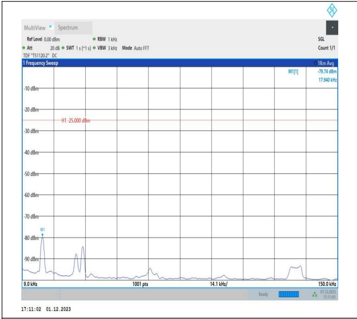
7-7-15MHz-20MHz-64QAM-64QAM-20828-20999-1RB#0-1RB #99-0.009~0.15MHz-PASS
