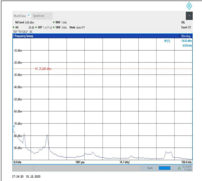
7-7-15MHz-20MHz-16QAM-16QAM-21003-21174-1RB#74-0R B#0-0.009~0.15MHz-PASS
