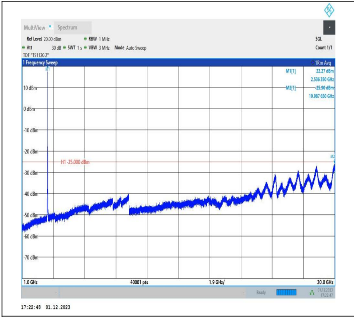
7-7-15MHz-20MHz-16QAM-16QAM-21179-21350-1RB#0-ORB #0-1000~20000MHz-PASS
