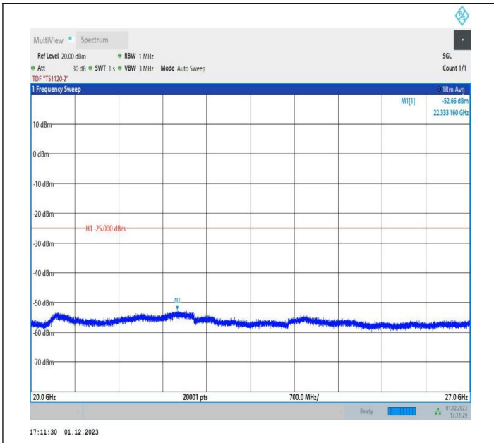
7-7-15MHz-20MHz-64QAM-64QAM-20828-20999-1RB#0-1RB #99-20000~27000MHz-PASS
