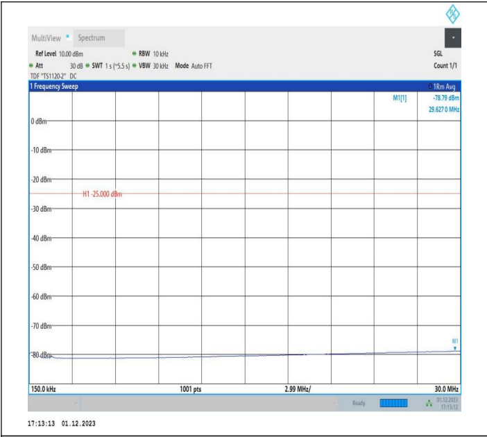
7-7-15MHz-20MHz-64QAM-64QAM-20828-20999-75RB#0-10 ORB#0-0.15~30MHz-PASS
