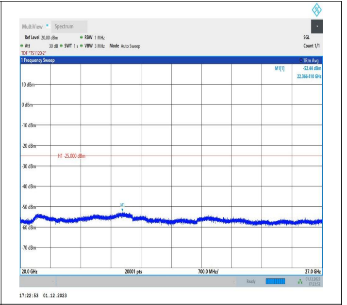
7-7-15MHz-20MHz-16QAM-16QAM-21179-21350-1RB#0-ORB #0-20000~27000MHz-PASS
