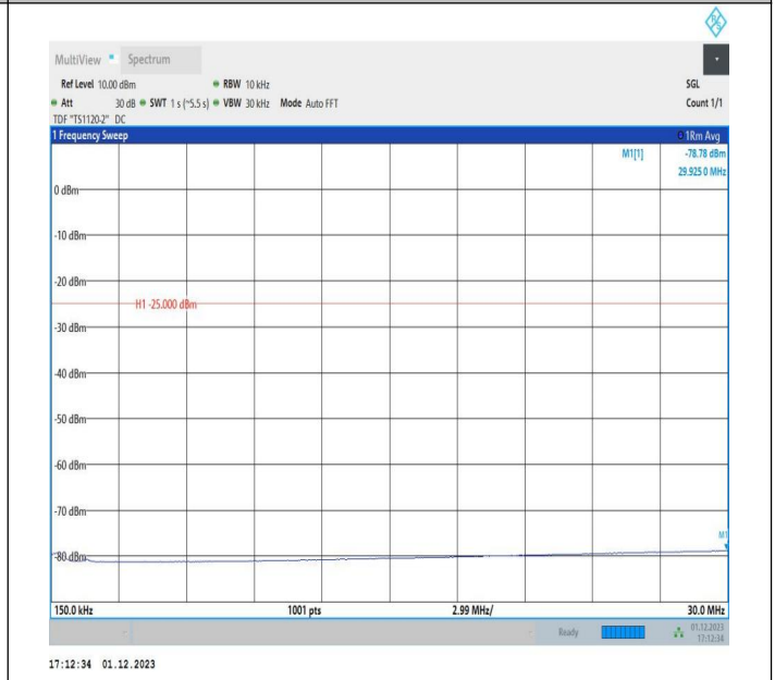
7-7-15MHz-20MHz-16QAM-16QAM-20828-20999-75RB#0-10 ORB#0-0.15~30MHz-PASS
