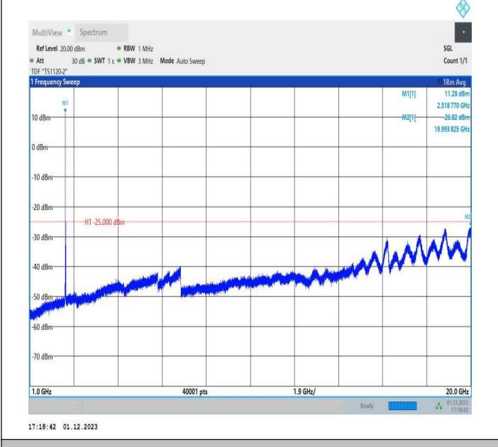
7-7-15MHz-20MHz-16QAM-16QAM-21003-21174-1RB#0-1RB #99-1000~20000MHz-PASS
