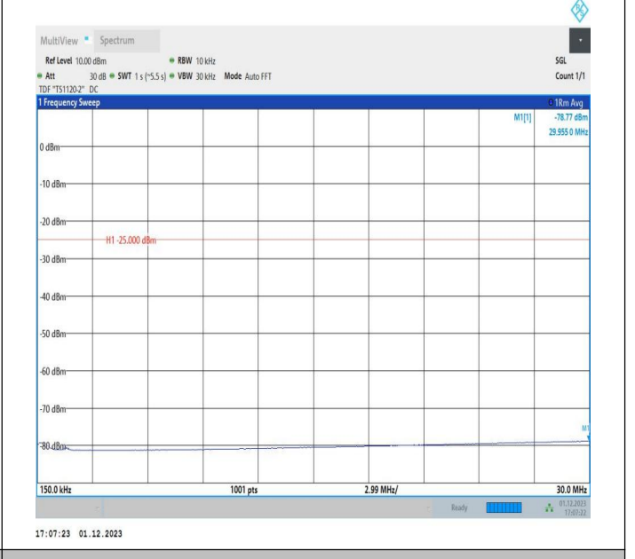
7-7-15MHz-20MHz-64QAM-64QAM-20828-20999-1RB#0-ORB #0-0.15~30MHz-PASS
