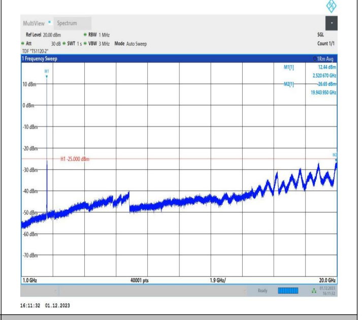
7-7-15MHz-15MHz-64QAM-64QAM-21025-21175-1RB#0-1RB #74-1000~20000MHz-PASS
