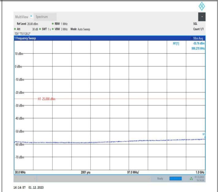
7-7-15MHz-15MHz-16QAM-16QAM-21225-21375-1RB#0-0RB #0-30~1000MHz-PASS
