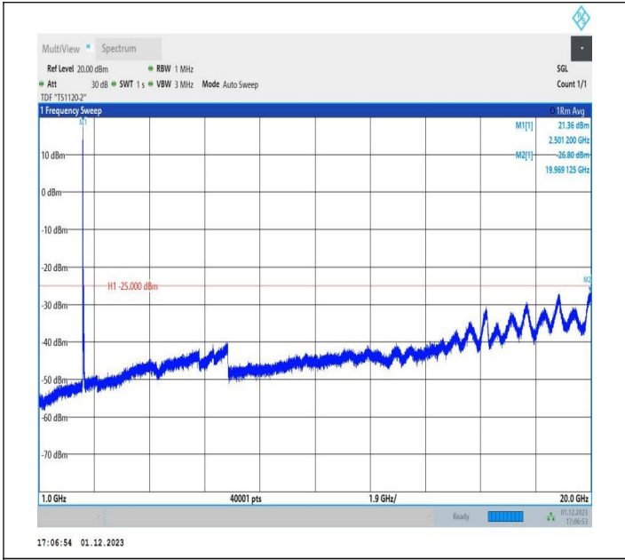
7-7-15MHz-20MHz-16QAM-16QAM-20828-20999-1RB#0-ORB #0-1000~20000MHz-PASS
