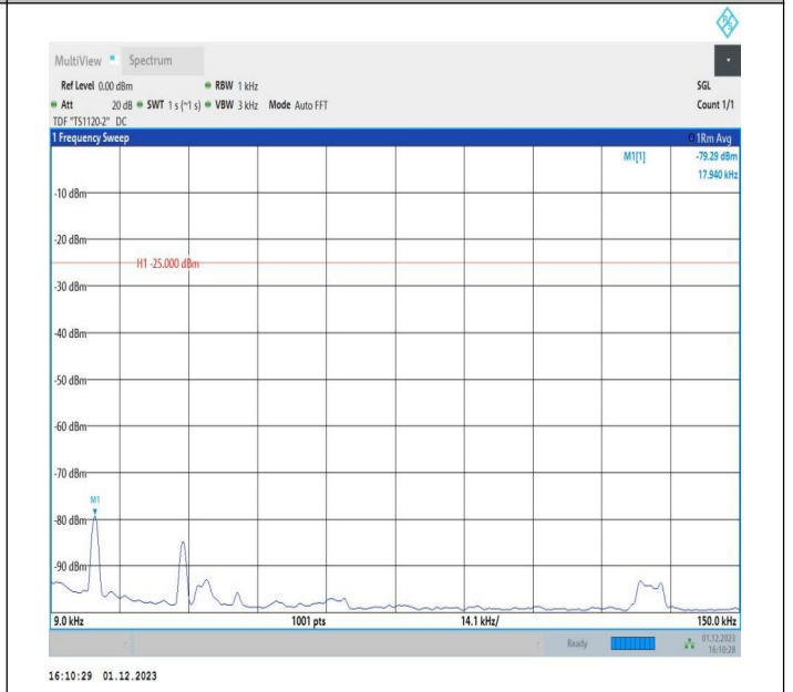
7-7-15MHz-15MHz-16QAM-16QAM-21025-21175-1RB#0-1RB #74-0.009~0.15MHz-PASS
