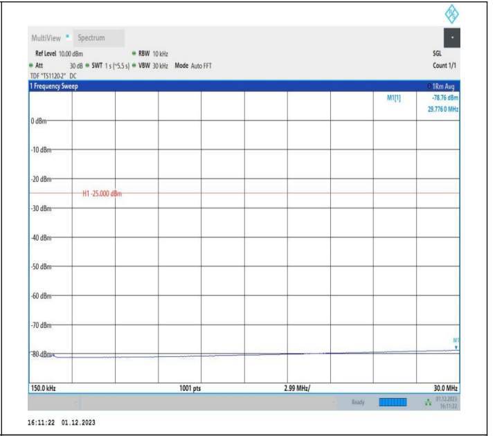
7-7-15MHz-15MHz-64QAM-64QAM-21025-21175-1RB#0-1RB #74-0.15~30MHz-PASS
