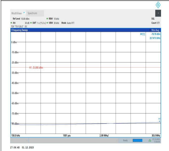
7-7-15MHz-20MHz-16QAM-16QAM-20828-20999-1RB#0-0RB #0-0.15~30MHz-PASS
