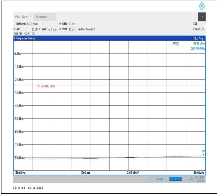
7-7-15MHz-15MHz-16QAM-16QAM-21025-21175-1RB#0-1RB #74-0.15~30MHz-PASS
