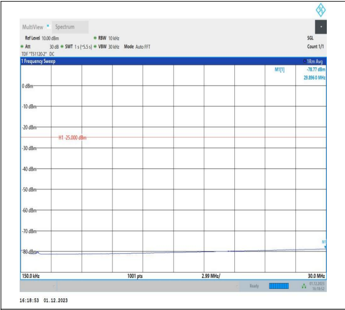
7-7-15MHz-15MHz-16QAM-16QAM-21225-21375-1RB#0-1RB #74-0.15~30MHz-PASS
