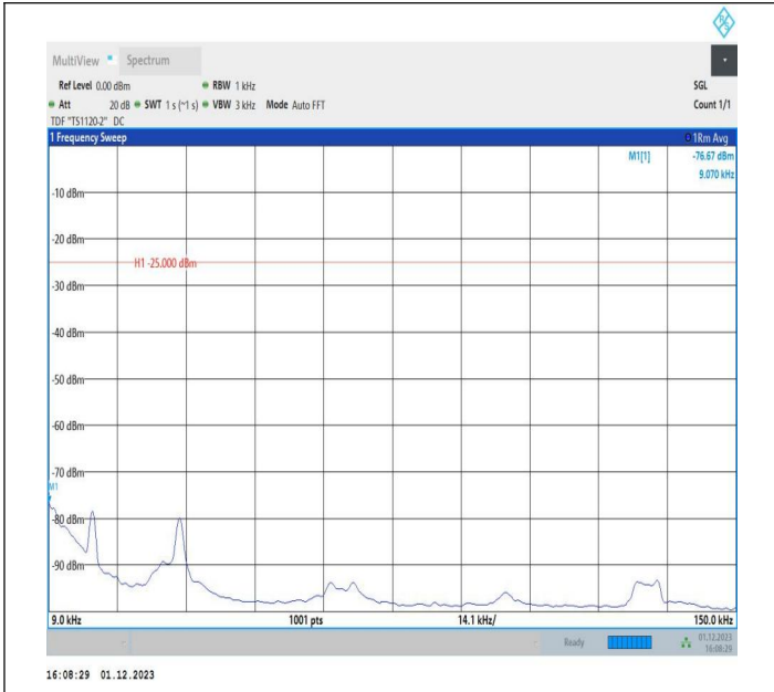
7-7-15MHz-15MHz-16QAM-16QAM-21025-21175-1RB#74-0R B#0-0.009~0.15MHz-PASS
