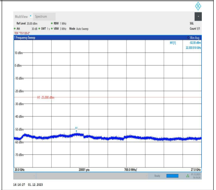
7-7-15MHz-15MHz-QPSK-QPSK-21225-21375-1RB#74-0RB# 0-20000~27000MHz-PASS
