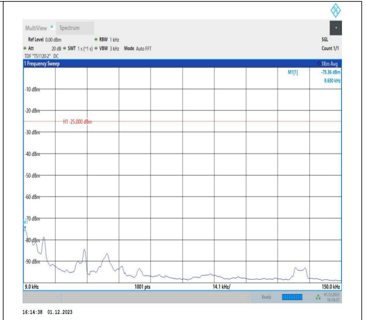
7-7-15MHz-15MHz-16QAM-16QAM-21225-21375-1RB#0-0RB #0-0.009~0.15MHz-PASS
