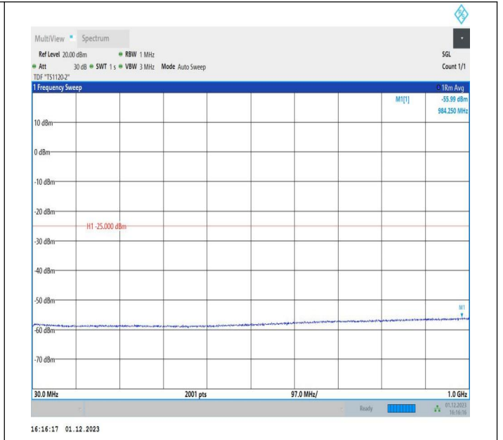
7-7-15MHz-15MHz-QPSK-QPSK-21225-21375-1RB#74-0RB# 0-30~1000MHz-PASS
