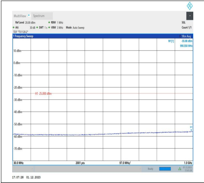
7-7-15MHz-20MHz-64QAM-64QAM-20828-20999-1RB#0-ORB #0-30~1000MHz-PASS
