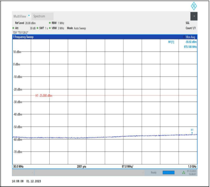
7-7-15MHz-15MHz-QPSK-QPSK-21025-21175-1RB#74-0RB# 0-30~1000MHz-PASS
