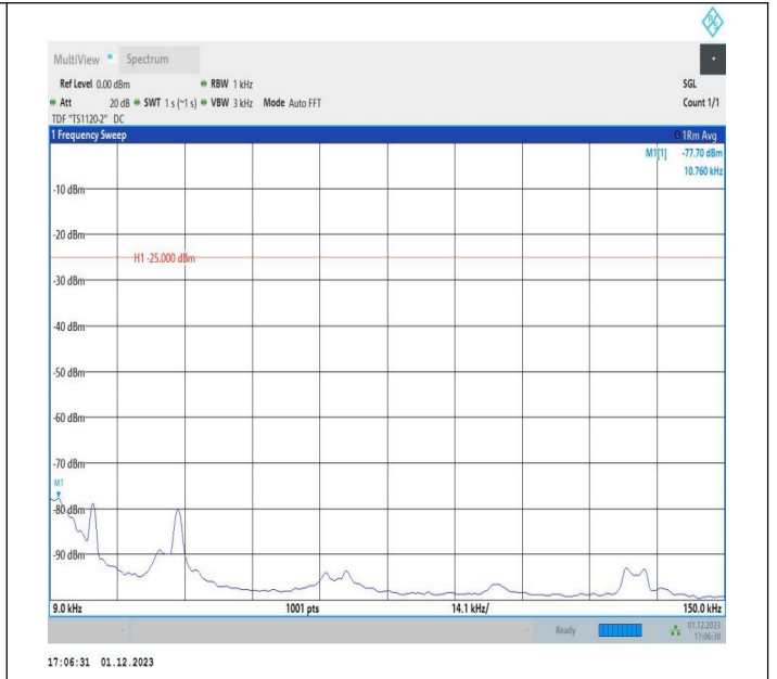
7-7-15MHz-20MHz-16QAM-16QAM-20828-20999-1RB#0-0RB #0-0.009~0.15MHz-PASS
