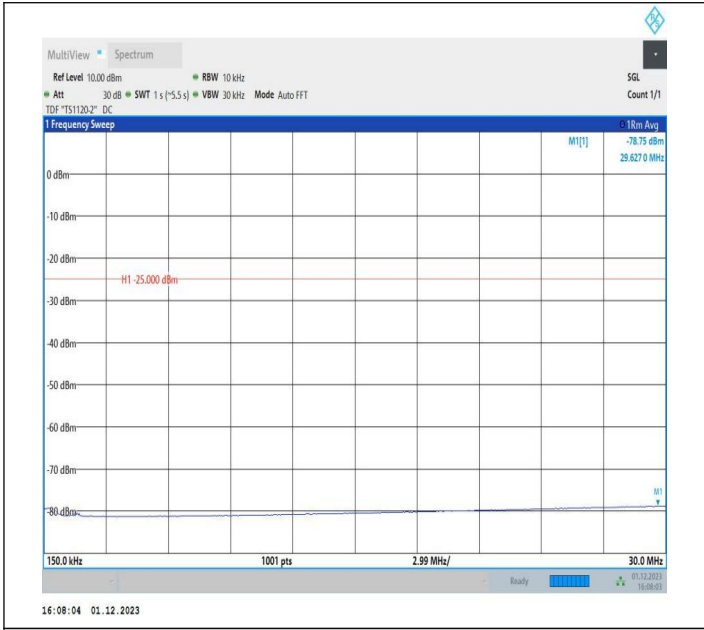
7-7-15MHz-15MHz-QPSK-QPSK-21025-21175-1RB#74-0RB# 0-0.15~30MHz-PASS
