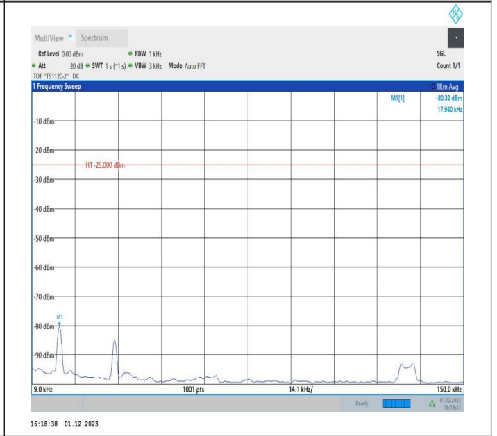
7-7-15MHz-15MHz-16QAM-16QAM-21225-21375-1RB#0-1RB #74-0.009~0.15MHz-PASS
