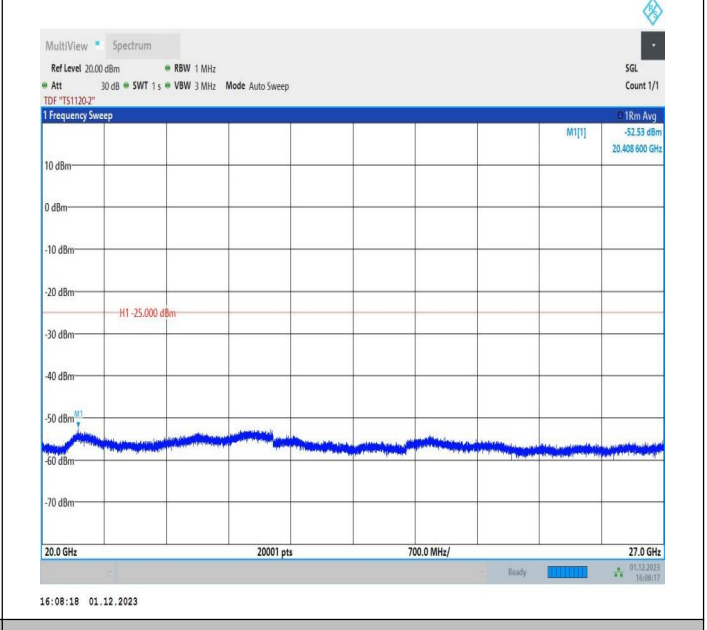
7-7-15MHz-15MHz-QPSK-QPSK-21025-21175-1RB#74-0RB# 0-20000~27000MHz-PASS
