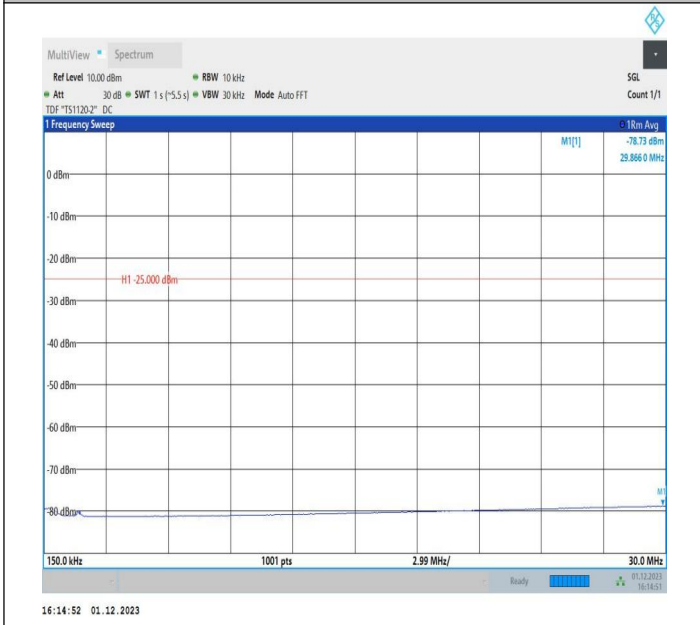
7-7-15MHz-15MHz-16QAM-16QAM-21225-21375-1RB#0-0RB #0-0.15~30MHz-PASS
