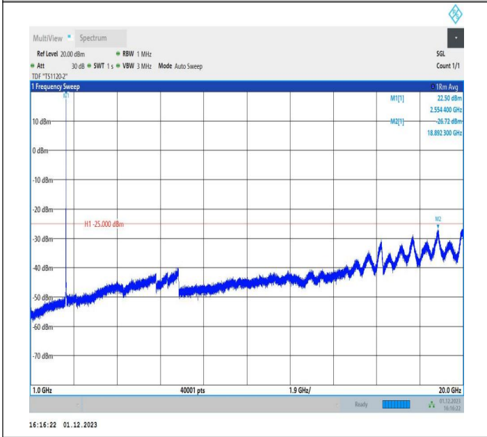
7-7-15MHz-15MHz-QPSK-QPSK-21225-21375-1RB#74-0RB# 0-1000~20000MHz-PASS
