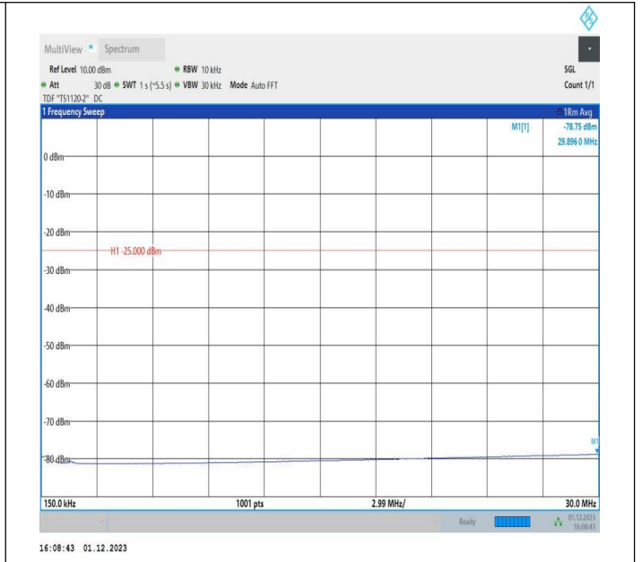
7-7-15MHz-15MHz-16QAM-16QAM-21025-21175-1RB#74-0R B#0-0.15~30MHz-PASS
