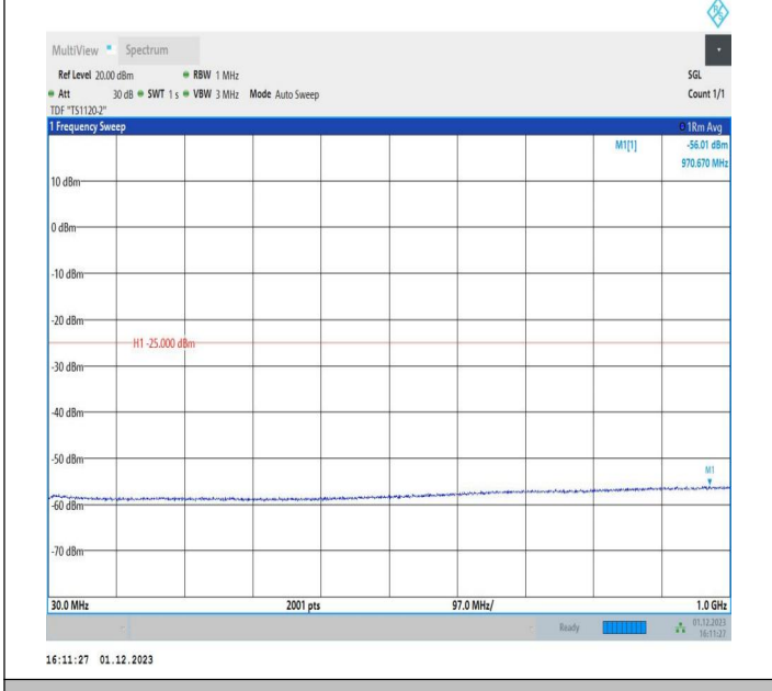
7-7-15MHz-15MHz-64QAM-64QAM-21025-21175-1RB#0-1RB #74-30~1000MHz-PASS
