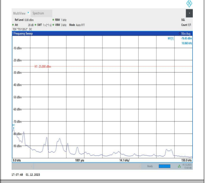
7-7-15MHz-20MHz-QPSK-QPSK-20828-20999-1RB#74-ORB# 0-0.009~0.15MHz-PASS
