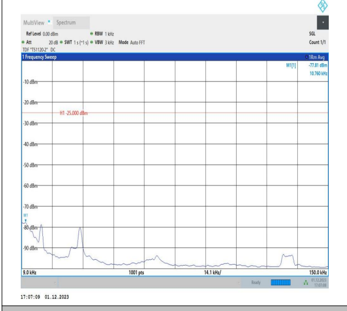
7-7-15MHz-20MHz-64QAM-64QAM-20828-20999-1RB#0-ORB #0-0.009~0.15MHz-PASS
