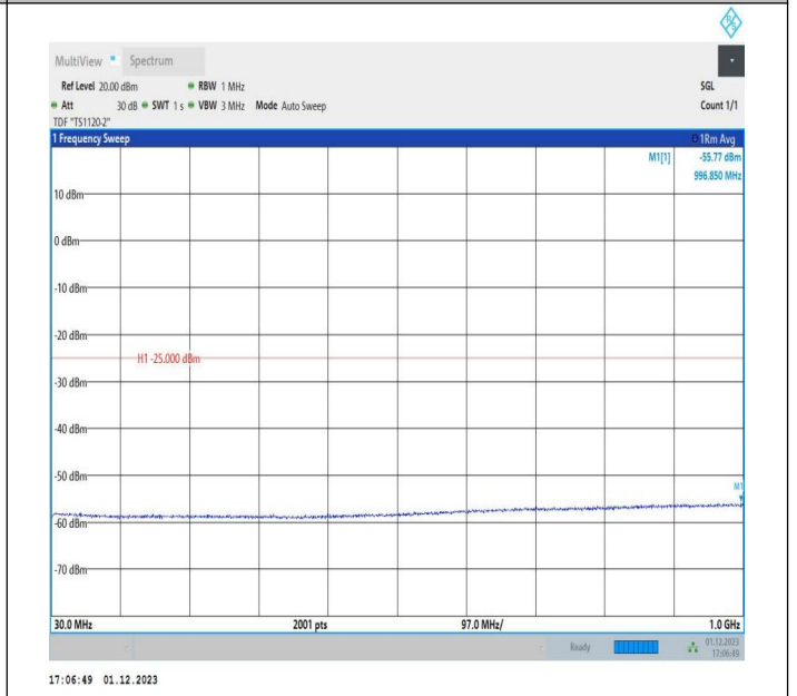
7-7-15MHz-20MHz-16QAM-16QAM-20828-20999-1RB#0-0RB #0-30~1000MHz-PASS
