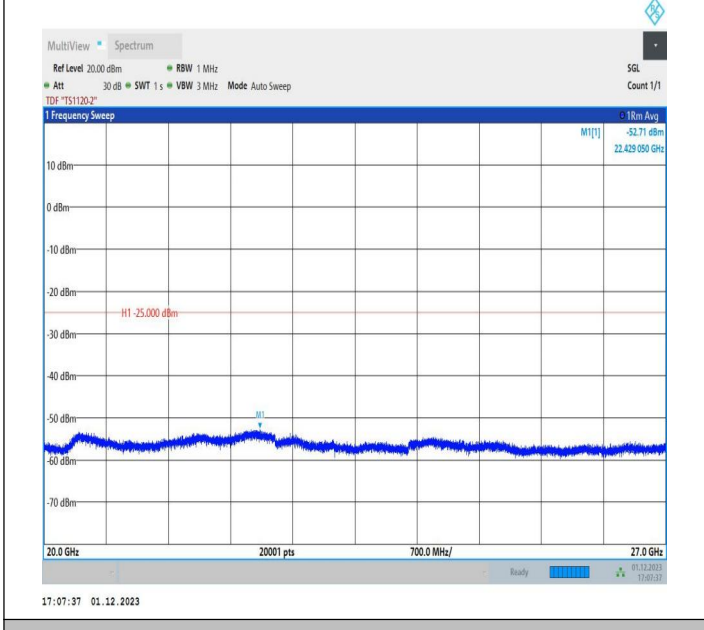
7-7-15MHz-20MHz-64QAM-64QAM-20828-20999-1RB#0-ORB #0-20000~27000MHz-PASS
