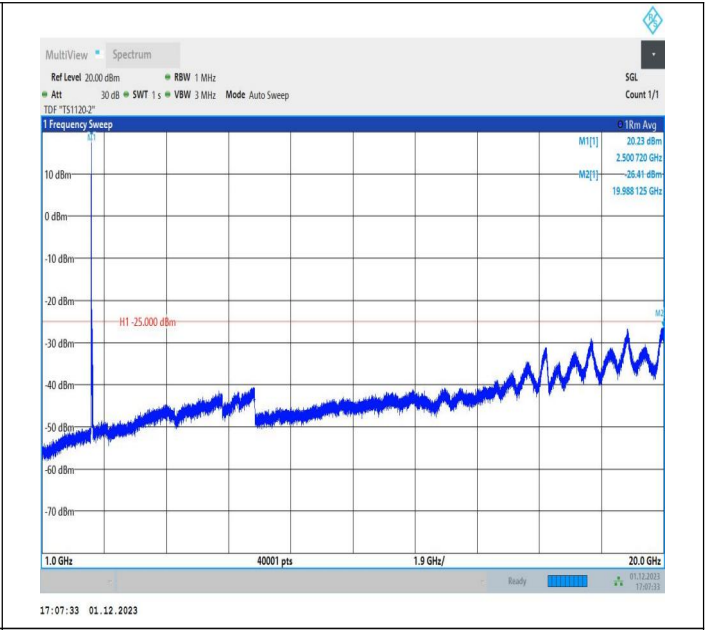
7-7-15MHz-20MHz-64QAM-64QAM-20828-20999-1RB#0-ORB #0-1000~20000MHz-PASS
