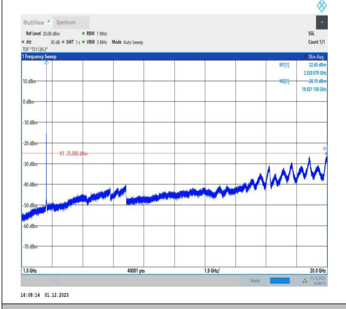
7-7-15MHz-15MHz-QPSK-QPSK-21025-21175-1RB#74-0RB# 0-1000~20000MHz-PASS
