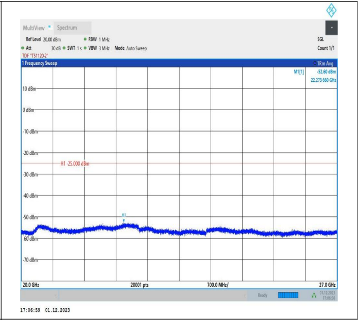
7-7-15MHz-20MHz-16QAM-16QAM-20828-20999-1RB#0-ORB #0-20000~27000MHz-PASS
