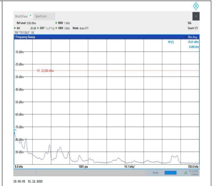
7-7-15MHz-10MHz-16QAM-16QAM-21277-21397-1RB#0-0RB #0-0.009~0.15MHz-PASS
