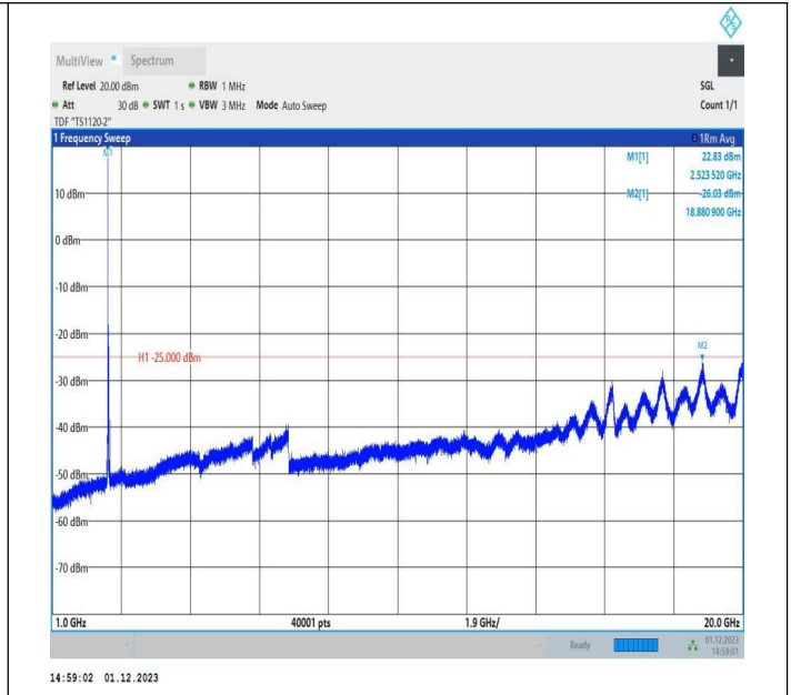
7-7-15MHz-10MHz-64QAM-64QAM-21051-21171-1RB#0-ORB #0-1000~20000MHz-PASS
