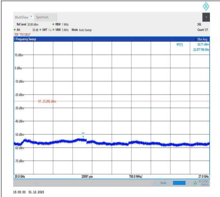
7-7-15MHz-10MHz-QPSK-QPSK-21277-21397-1RB#0-0RB#0 -20000~27000MHz-PASS
