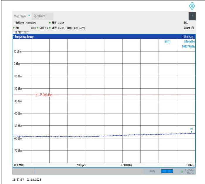
7-7-15MHz-10MHz-QPSK-QPSK-21051-21171-1RB#0-ORB#0-30~1000MHz-PASS
