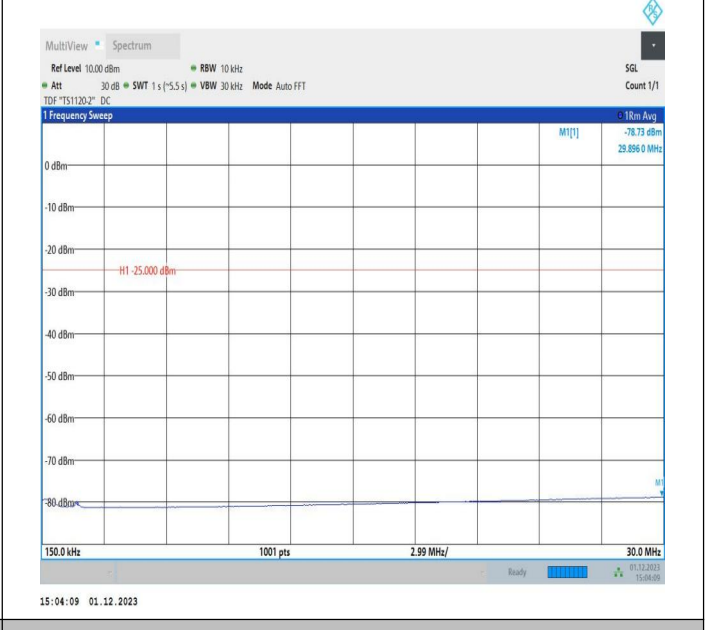
7-7-15MHz-10MHz-16QAM-16QAM-21051-21171-75RB#0-50 RB#0-0.15~30MHz-PASS
