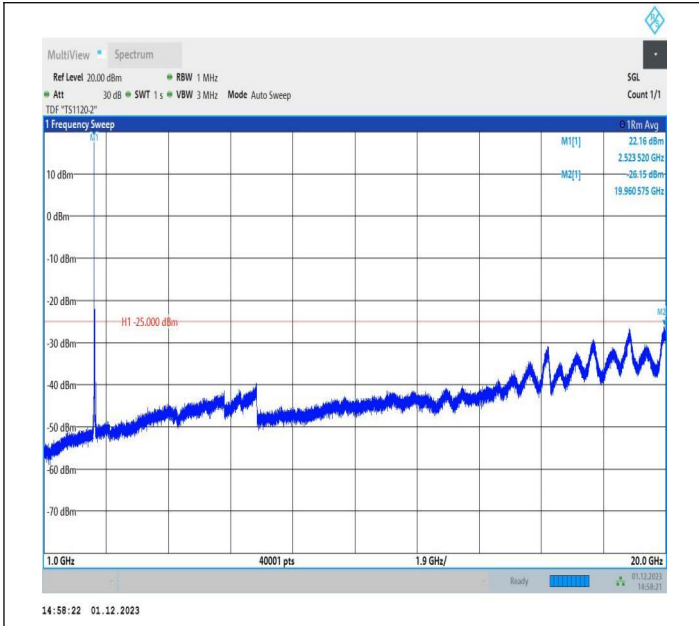
7-7-15MHz-10MHz-16QAM-16QAM-21051-21171-1RB#0-ORB #0-1000~20000MHz-PASS
