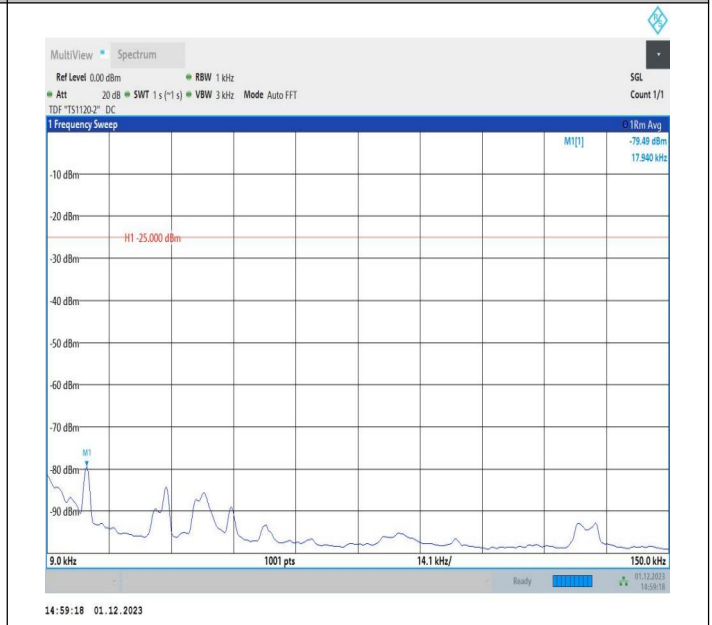
7-7-15MHz-10MHz-QPSK-QPSK-21051-21171-1RB#74-ORB# 0-0.009~0.15MHz-PASS
