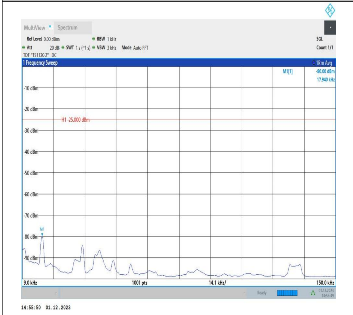
7-7-15MHz-10MHz-16QAM-16QAM-20825-20945-75RB#0-50 RB#0-0.009~0.15MHz-PASS
