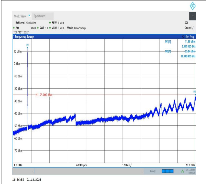
7-7-15MHz-10MHz-64QAM-64QAM-20825-20945-75RB#0-50 RB#0-1000~20000MHz-PASS
