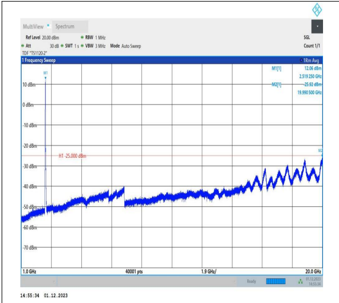
7-7-15MHz-10MHz-QPSK-QPSK-20825-20945-75RB#0-50RB #0-1000~20000MHz-PASS
