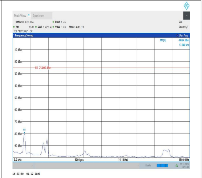
7-7-15MHz-10MHz-16QAM-16QAM-20825-20945-1RB#0-1RB #49-0.009~0.15MHz-PASS
