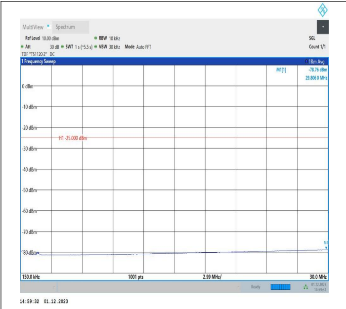
7-7-15MHz-10MHz-QPSK-QPSK-21051-21171-1RB#74-0RB# 0-0.15~30MHz-PASS
