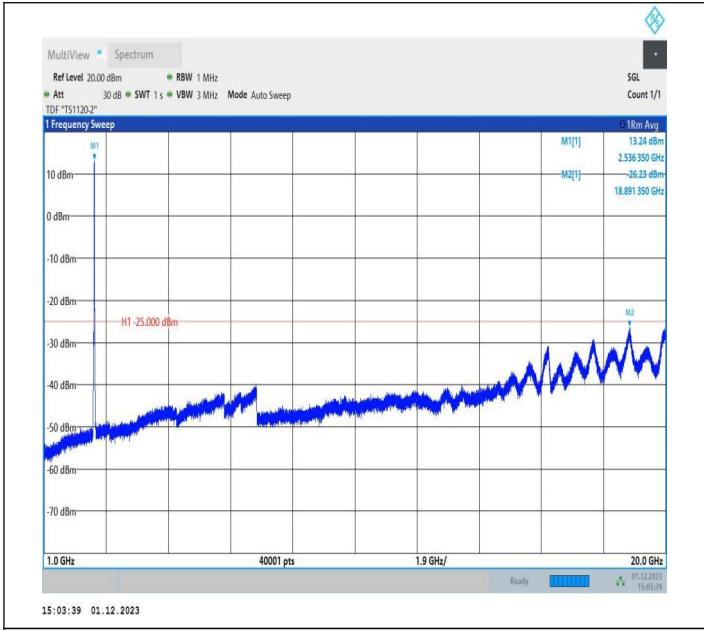
7-7-15MHz-10MHz-QPSK-QPSK-21051-21171-75RB#0-50RB #0-1000~20000MHz-PASS
