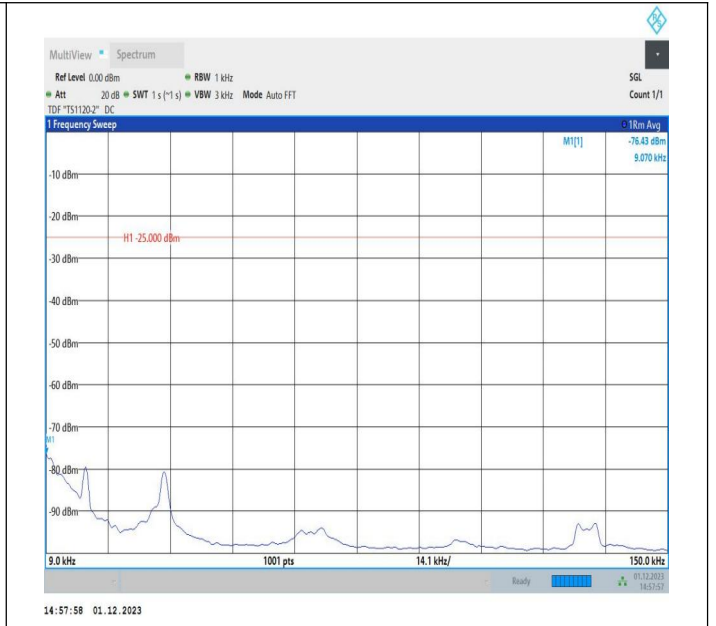
7-7-15MHz-10MHz-16QAM-16QAM-21051-21171-1RB#0-ORB#0-0.009~0.15MHz-PASS
