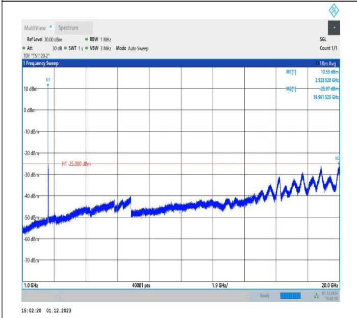
7-7-15MHz-10MHz-16QAM-16QAM-21051-21171-1RB#0-1RB #49-1000~20000MHz-PASS
