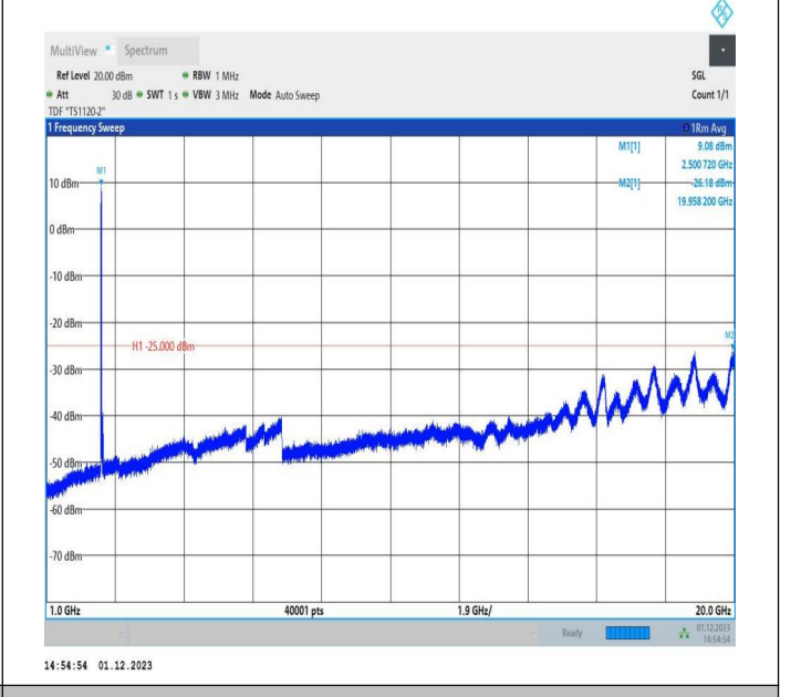
7-7-15MHz-10MHz-64QAM-64QAM-20825-20945-1RB#0-1RB #49-1000~20000MHz-PASS
