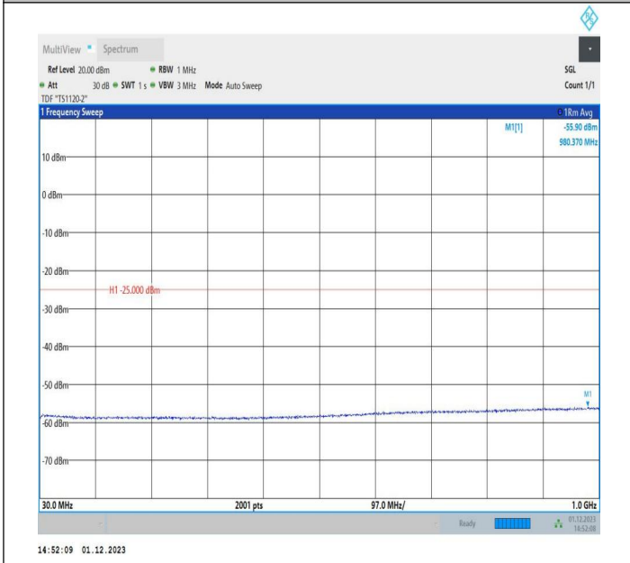
7-7-15MHz-10MHz-16QAM-16QAM-20825-20945-1RB#74-OR B#0-30~1000MHz-PASS
