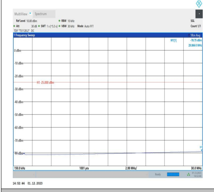
7-7-15MHz-10MHz-64QAM-64QAM-20825-20945-1RB#74-0R B#0-0.15~30MHz-PASS
