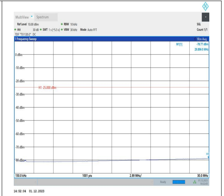
7-7-15MHz-10MHz-16QAM-16QAM-20825-20945-1RB#74-OR B#0-0.15~30MHz-PASS
