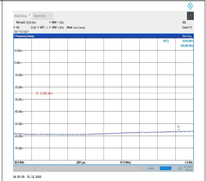
7-7-15MHz-10MHz-QPSK-QPSK-20825-20945-75RB#0-50RB #0-30~1000MHz-PASS
