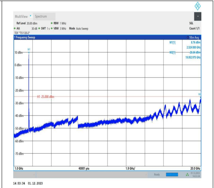
7-7-15MHz-10MHz-QPSK-QPSK-20825-20945-1RB#0-1RB#4 9-1000~20000MHz-PASS
