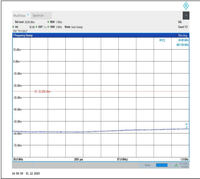
7-7-15MHz-10MHz-16QAM-16QAM-20825-20945-75RB#0-50 RB#0-30~1000MHz-PASS
