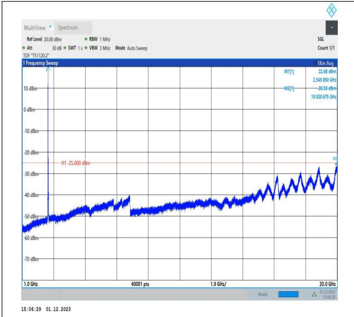
7-7-15MHz-10MHz-16QAM-16QAM-21277-21397-1RB#0-ORB #0-1000~20000MHz-PASS
