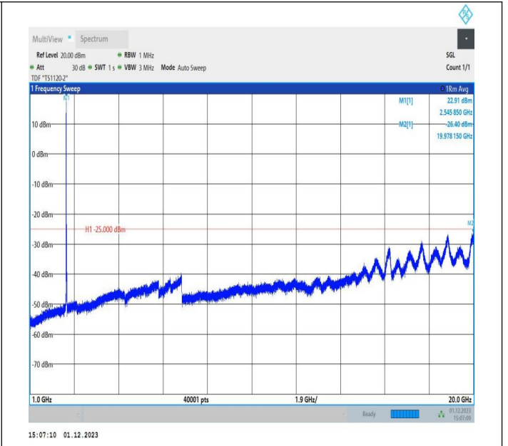
7-7-15MHz-10MHz-64QAM-64QAM-21277-21397-1RB#0-ORB #0-1000~20000MHz-PASS
