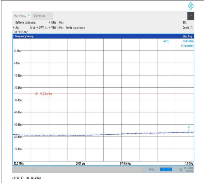
7-7-15MHz-10MHz-16QAM-16QAM-21051-21171-1RB#74-0R B#0-30~1000MHz-PASS
