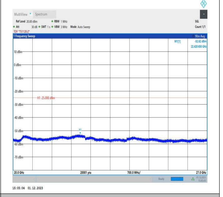
7-7-15MHz-10MHz-64QAM-64QAM-21051-21171-75RB#0-50 RB#0-20000~27000MHz-PASS
