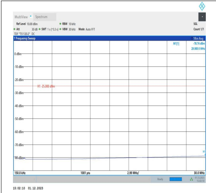
7-7-15MHz-10MHz-16QAM-16QAM-21051-21171-1RB#0-1RB #49-0.15~30MHz-PASS
