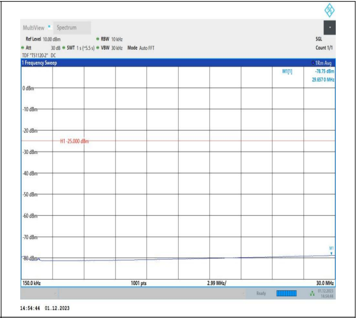
7-7-15MHz-10MHz-64QAM-64QAM-20825-20945-1RB#0-1RB #49-0.15~30MHz-PASS
