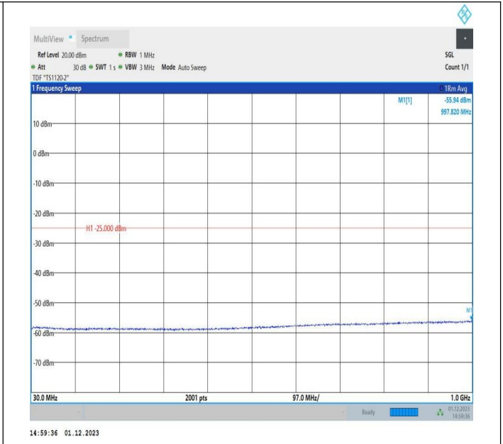
7-7-15MHz-10MHz-QPSK-QPSK-21051-21171-1RB#74-0RB# 0-30~1000MHz-PASS
