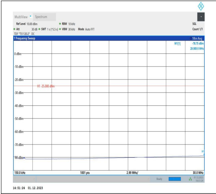
7-7-15MHz-10MHz-QPSK-QPSK-20825-20945-1RB#74-0RB# 0-0.15~30MHz-PASS
