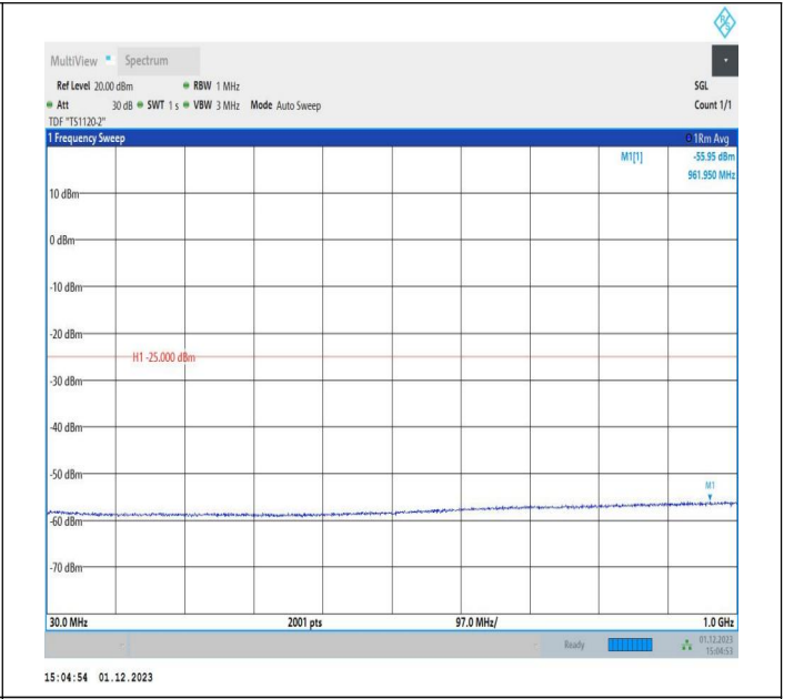
7-7-15MHz-10MHz-64QAM-64QAM-21051-21171-75RB#0-50 RB#0-30~1000MHz-PASS
