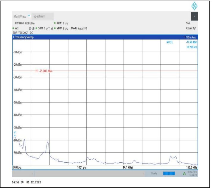
7-7-15MHz-10MHz-64QAM-64QAM-20825-20945-1RB#74-0R B#0-0.009~0.15MHz-PASS
