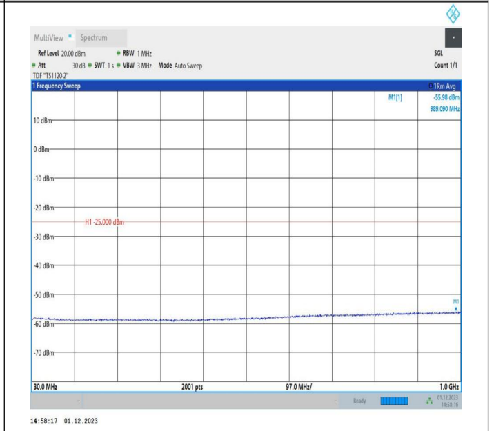
7-7-15MHz-10MHz-16QAM-16QAM-21051-21171-1RB#0-ORB#0-30~1000MHz-PASS
