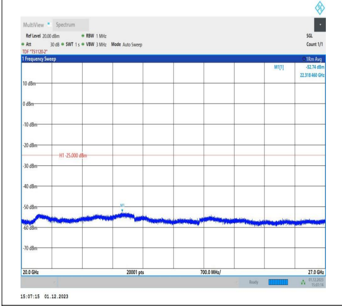
7-7-15MHz-10MHz-64QAM-64QAM-21277-21397-1RB#0-ORB #0-20000~27000MHz-PASS
