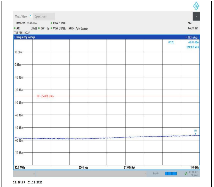
7-7-15MHz-10MHz-64QAM-64QAM-20825-20945-75RB#0-50 RB#0-30~1000MHz-PASS
