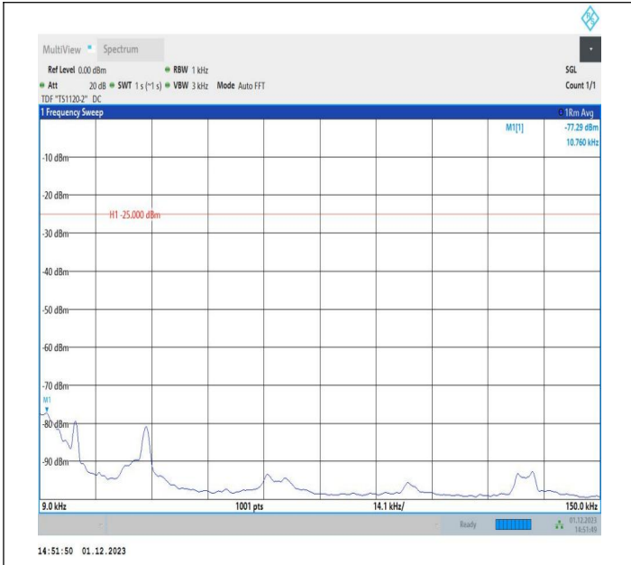
7-7-15MHz-10MHz-16QAM-16QAM-20825-20945-1RB#74-OR B#0-0.009~0.15MHz-PASS
