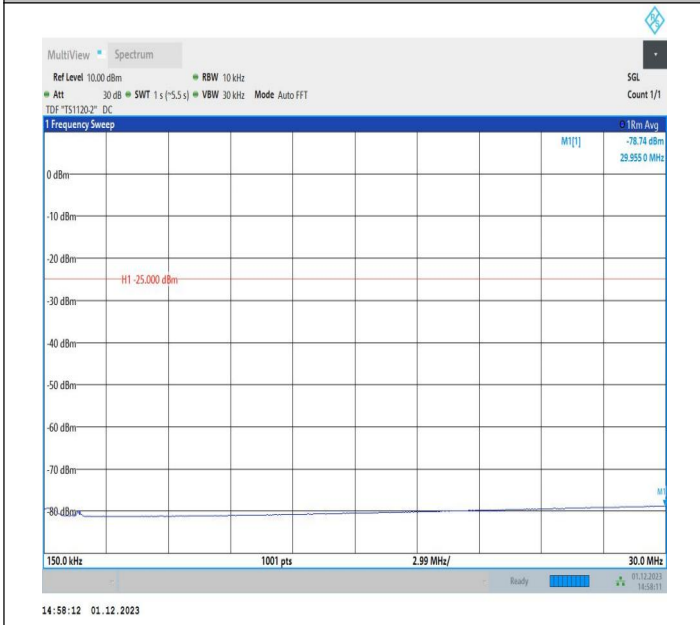
7-7-15MHz-10MHz-16QAM-16QAM-21051-21171-1RB#0-ORB#0-0.15~30MHz-PASS
