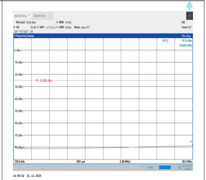
7-7-15MHz-10MHz-64QAM-64QAM-21051-21171-1RB#0-ORB #0-0.15~30MHz-PASS
