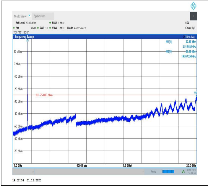
7-7-15MHz-10MHz-64QAM-64QAM-20825-20945-1RB#74-0R B#0-1000~20000MHz-PASS
