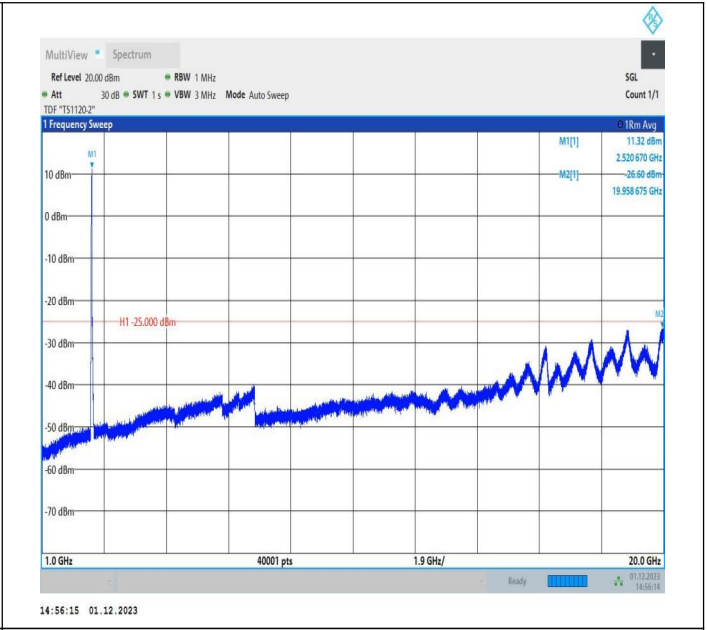
7-7-15MHz-10MHz-16QAM-16QAM-20825-20945-75RB#0-50 RB#0-1000~20000MHz-PASS
