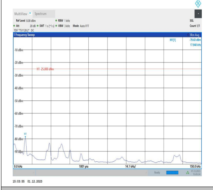
7-7-15MHz-10MHz-16QAM-16QAM-21051-21171-75RB#0-50 RB#0-0.009~0.15MHz-PASS
