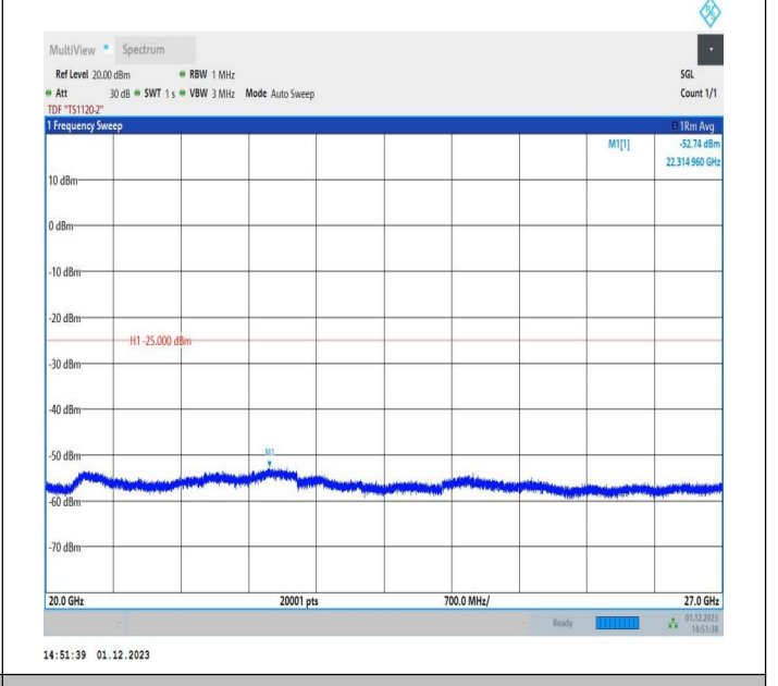
7-7-15MHz-10MHz-QPSK-QPSK-20825-20945-1RB#74-0RB# 0-20000~27000MHz-PASS
