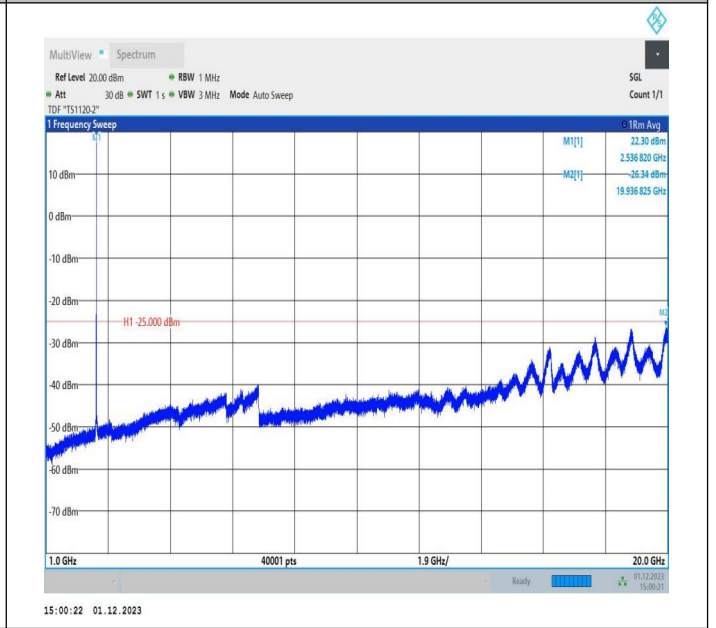
7-7-15MHz-10MHz-16QAM-16QAM-21051-21171-1RB#74-0R B#0-1000~20000MHz-PASS
