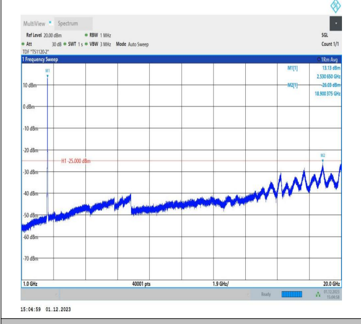
7-7-15MHz-10MHz-64QAM-64QAM-21051-21171-75RB#0-50 RB#0-1000~20000MHz-PASS
