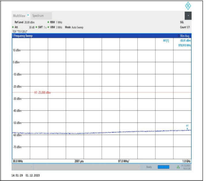
7-7-15MHz-10MHz-QPSK-QPSK-20825-20945-1RB#74-0RB# 0-30~1000MHz-PASS
