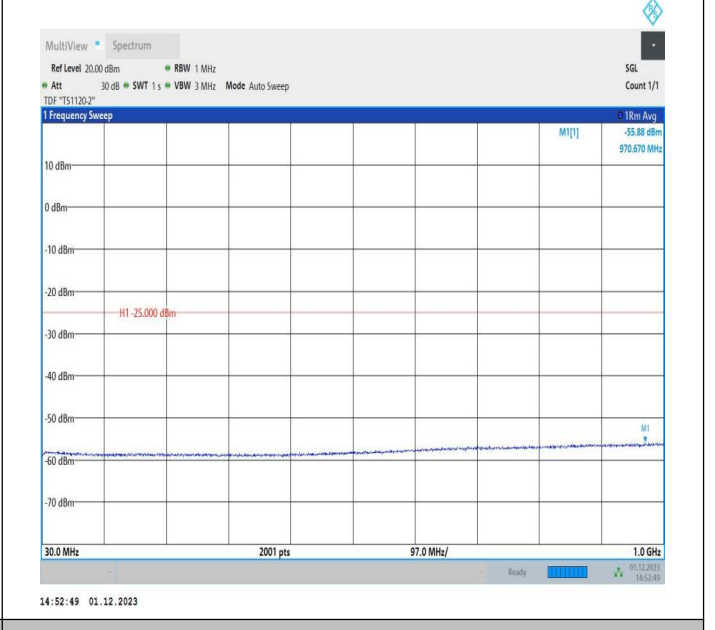
7-7-15MHz-10MHz-64QAM-64QAM-20825-20945-1RB#74-0R B#0-30~1000MHz-PASS
