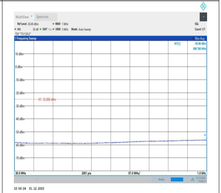
7-7-15MHz-10MHz-16QAM-16QAM-21277-21397-1RB#0-0RB #0-30~1000MHz-PASS
