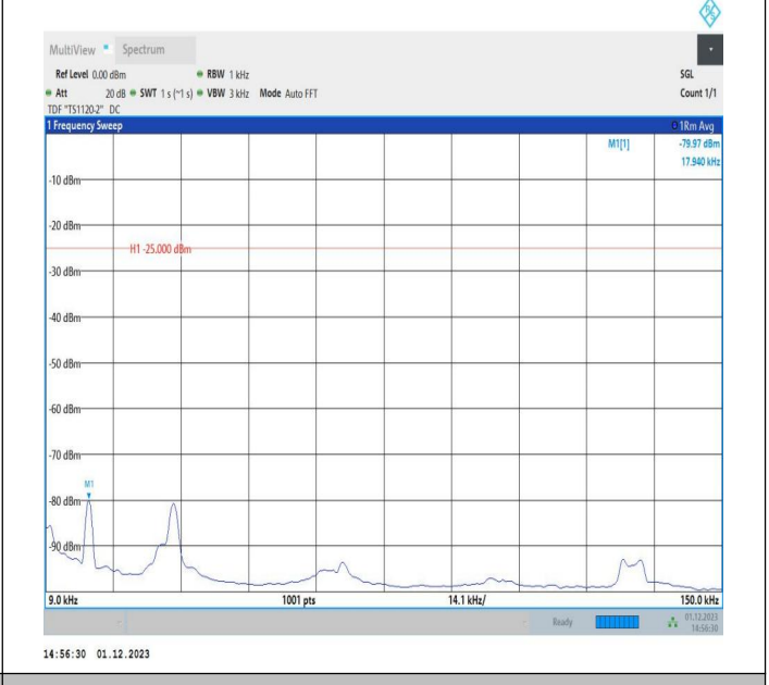
7-7-15MHz-10MHz-64QAM-64QAM-20825-20945-75RB#0-50 RB#0-0.009~0.15MHz-PASS
