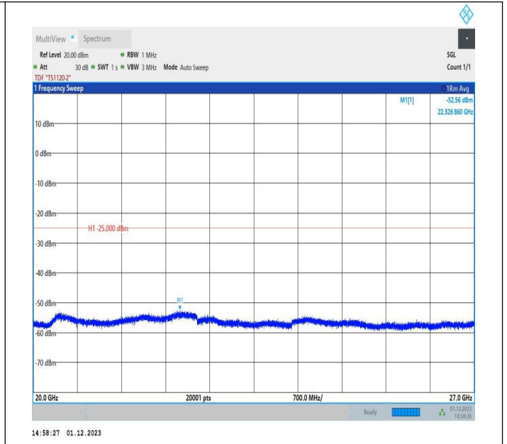
7-7-15MHz-10MHz-16QAM-16QAM-21051-21171-1RB#0-ORB #0-20000~27000MHz-PASS
