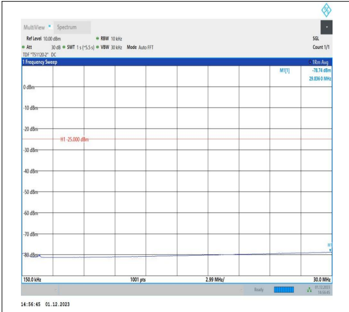
7-7-15MHz-10MHz-64QAM-64QAM-20825-20945-75RB#0-50 RB#0-0.15~30MHz-PASS
