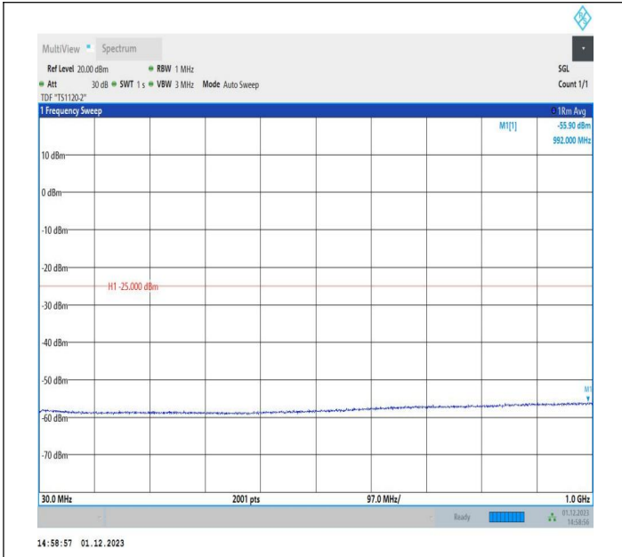
7-7-15MHz-10MHz-64QAM-64QAM-21051-21171-1RB#0-ORB #0-30~1000MHz-PASS
