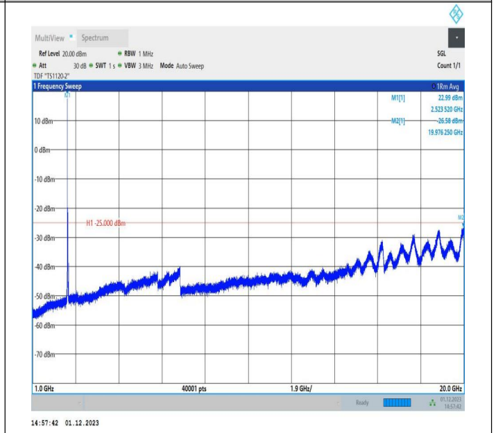
7-7-15MHz-10MHz-QPSK-QPSK-21051-21171-1RB#0-ORB#0-1000~20000MHz-PASS
