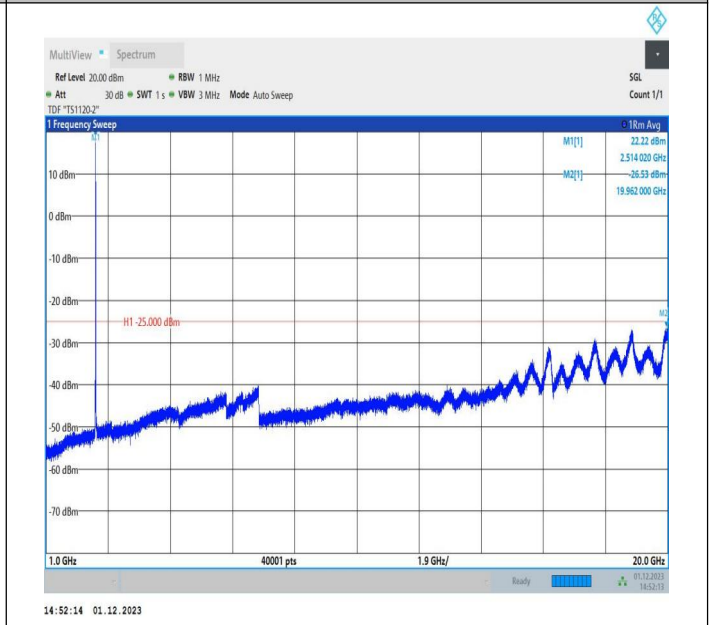
7-7-15MHz-10MHz-16QAM-16QAM-20825-20945-1RB#74-OR B#0-1000~20000MHz-PASS
