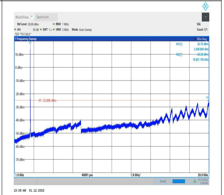
7-7-15MHz-10MHz-QPSK-QPSK-21277-21397-1RB#0-0RB#0 -1000~20000MHz-PASS
