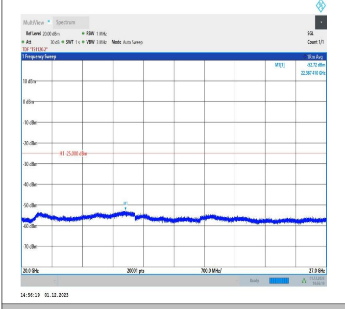
7-7-15MHz-10MHz-16QAM-16QAM-20825-20945-75RB#0-50 RB#0-20000~27000MHz-PASS
