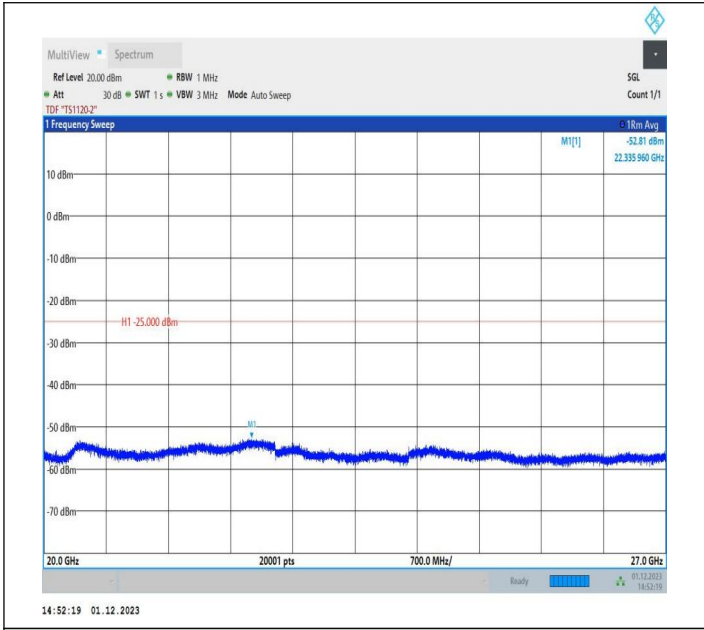
7-7-15MHz-10MHz-16QAM-16QAM-20825-20945-1RB#74-0R B#0-20000~27000MHz-PASS
