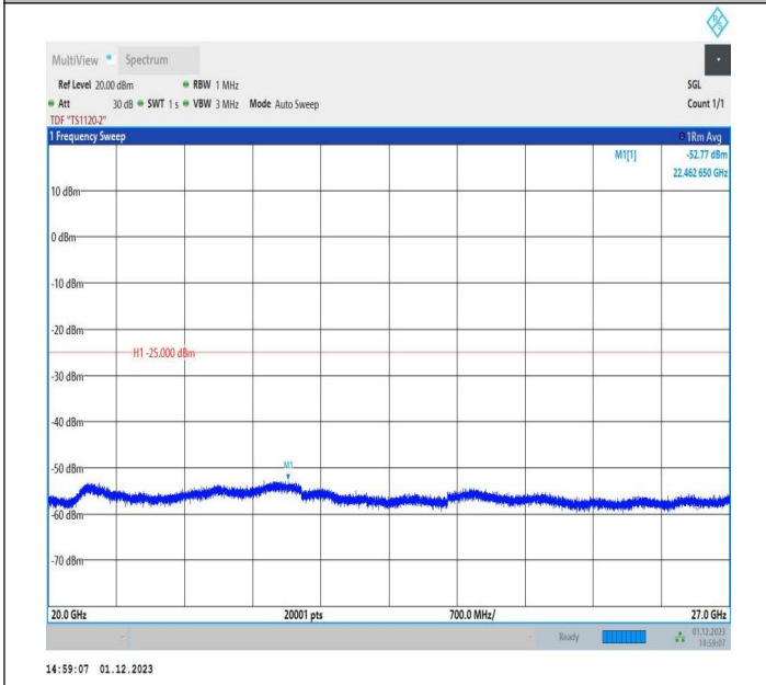
7-7-15MHz-10MHz-64QAM-64QAM-21051-21171-1RB#0-ORB #0-20000~27000MHz-PASS
