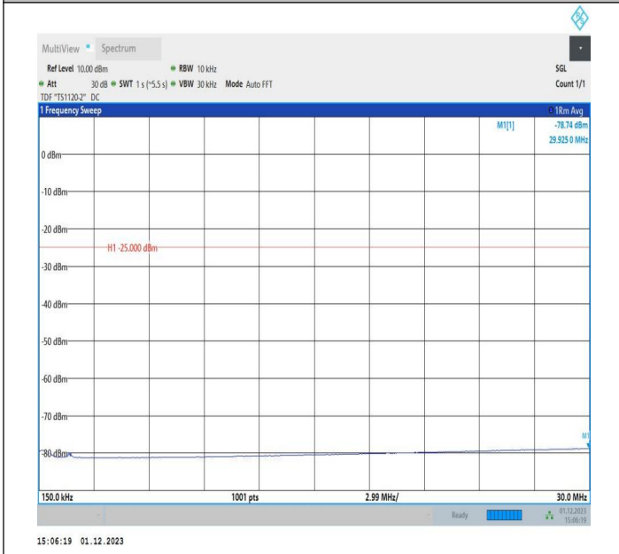
7-7-15MHz-10MHz-16QAM-16QAM-21277-21397-1RB#0-0RB #0-0.15~30MHz-PASS
