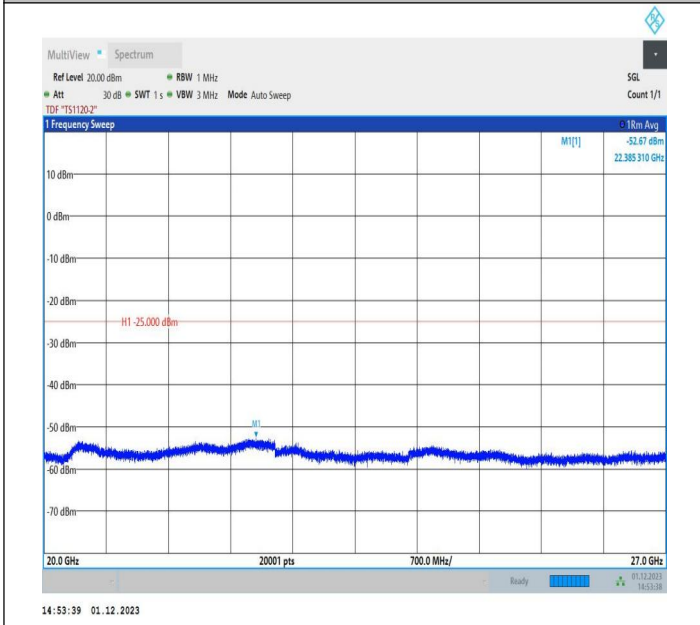
7-7-15MHz-10MHz-QPSK-QPSK-20825-20945-1RB#0-1RB#4 9-20000~27000MHz-PASS
