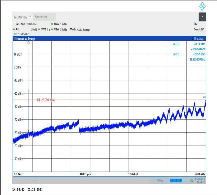
7-7-15MHz-10MHz-QPSK-QPSK-21051-21171-1RB#74-0RB# 0-1000~20000MHz-PASS
