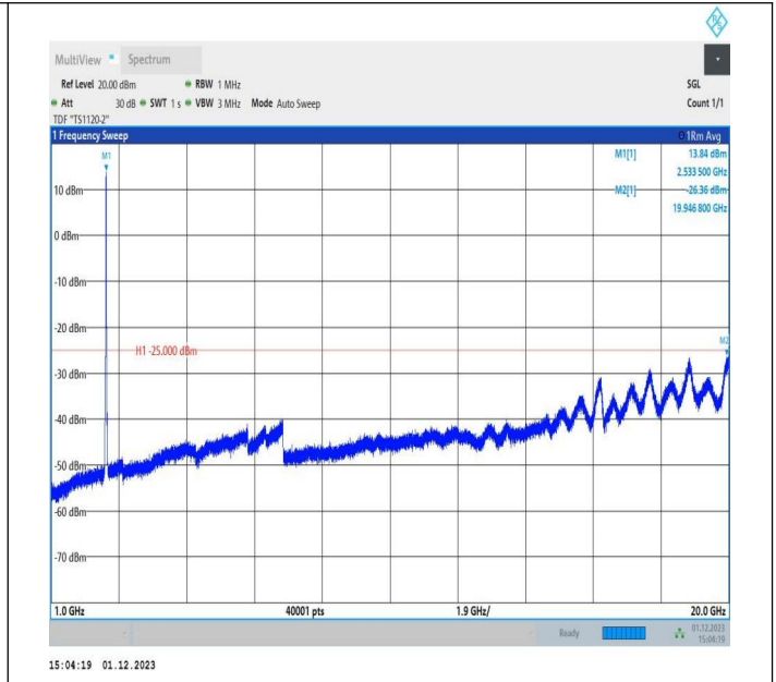
7-7-15MHz-10MHz-16QAM-16QAM-21051-21171-75RB#0-50 RB#0-1000~20000MHz-PASS
