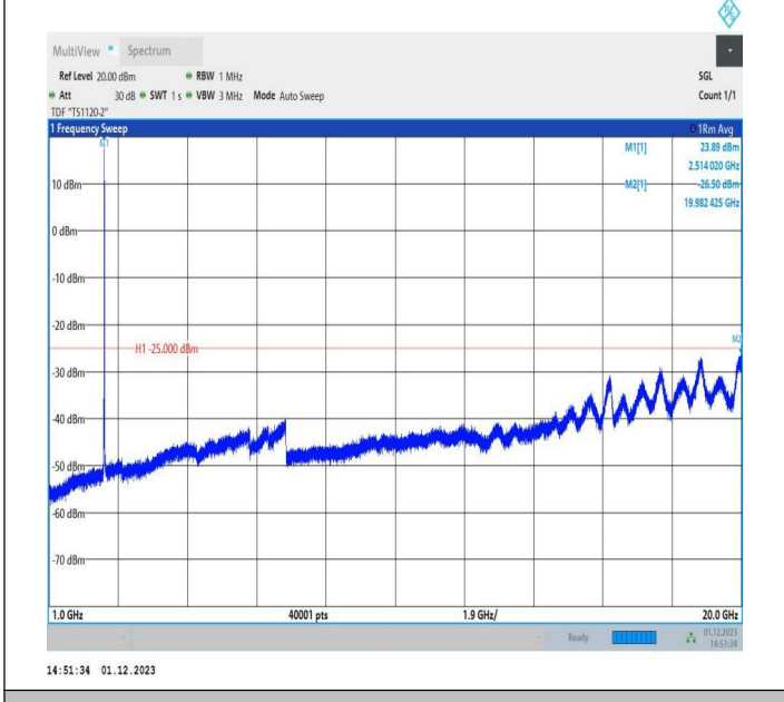
7-7-15MHz-10MHz-QPSK-QPSK-20825-20945-1RB#74-0RB# 0-1000~20000MHz-PASS
