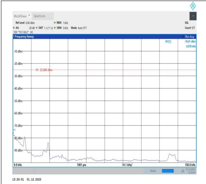
7-7-10MHz-20MHz-16QAM-16QAM-21006-21150-1RB#49-OR B#0-0.009~0.15MHz-PASS
