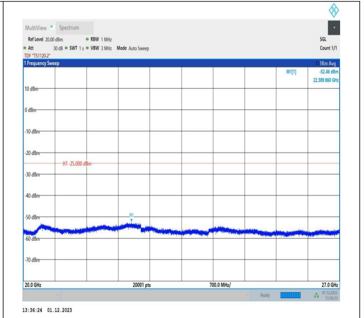
7-7-10MHz-20MHz-16QAM-16QAM-21206-21350-1RB#0-ORB #0-20000~27000MHz-PASS
