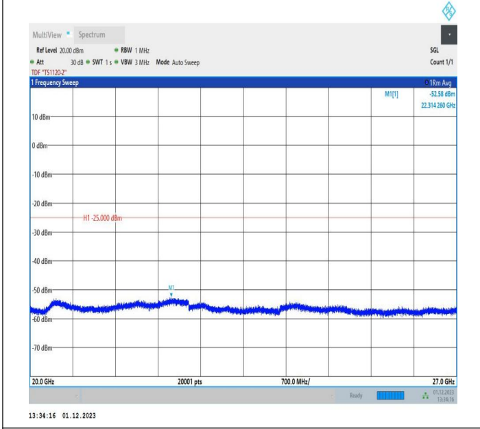
7-7-10MHz-20MHz-16QAM-16QAM-21006-21150-50RB#0-100 RB#0-20000~27000MHz-PASS
