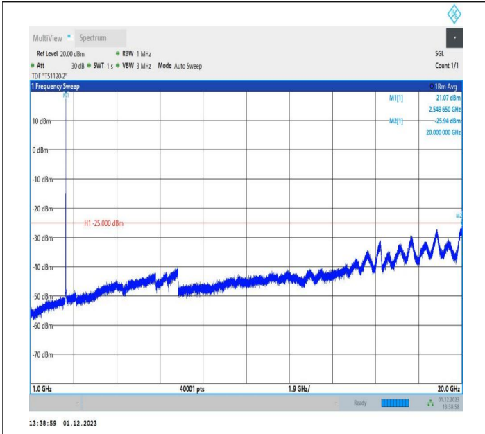
7-7-10MHz-20MHz-64QAM-64QAM-21206-21350-1RB#49-0R B#0-1000~20000MHz-PASS
