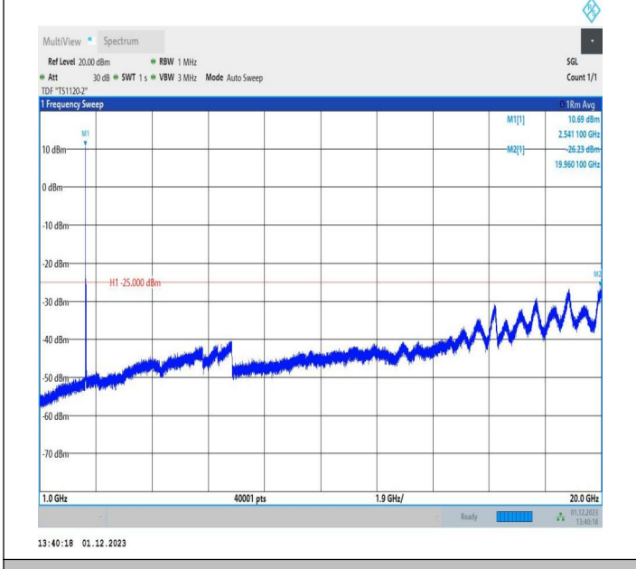
7-7-10MHz-20MHz-16QAM-16QAM-21206-21350-1RB#0-1RB #99-1000~20000MHz-PASS
