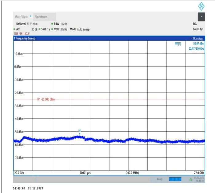
7-7-15MHz-10MHz-QPSK-QPSK-20825-20945-1RB#0-0RB#0 -20000~27000MHz-PASS
