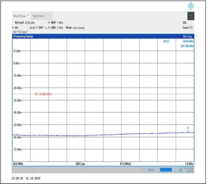
7-7-10MHz-20MHz-QPSK-QPSK-21006-21150-1RB#49-0RB# 0-30~1000MHz-PASS
