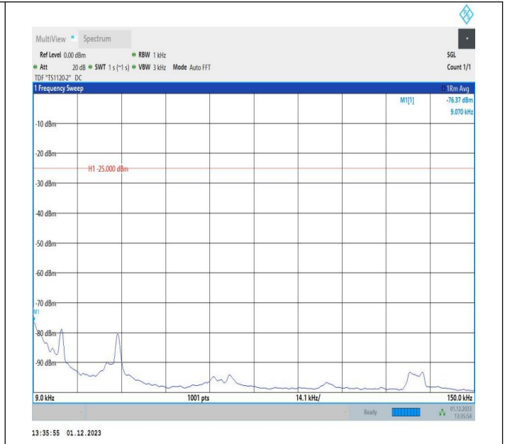
7-7-10MHz-20MHz-16QAM-16QAM-21206-21350-1RB#0-0RB #0-0.009~0.15MHz-PASS
