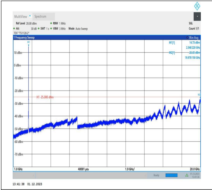
7-7-10MHz-20MHz-QPSK-QPSK-21206-21350-50RB#0-100R B#0-1000~20000MHz-PASS
