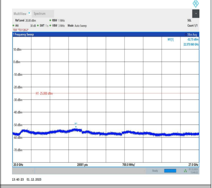
7-7-10MHz-20MHz-16QAM-16QAM-21206-21350-1RB#0-1RB #99-20000~27000MHz-PASS
