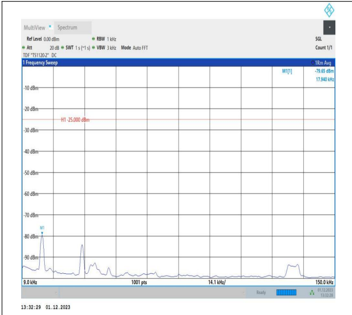
7-7-10MHz-20MHz-64QAM-64QAM-21006-21150-1RB#0-1RB #99-0.009~0.15MHz-PASS
