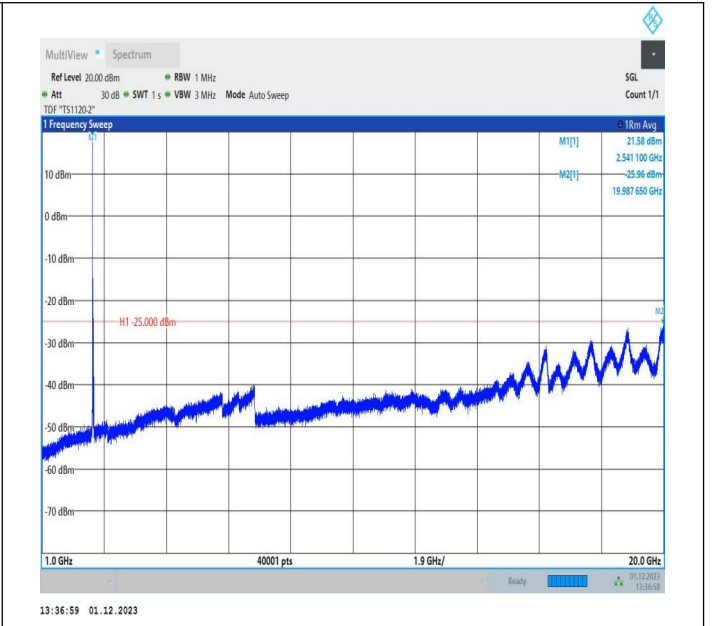
7-7-10MHz-20MHz-64QAM-64QAM-21206-21350-1RB#0-ORB #0-1000~20000MHz-PASS
