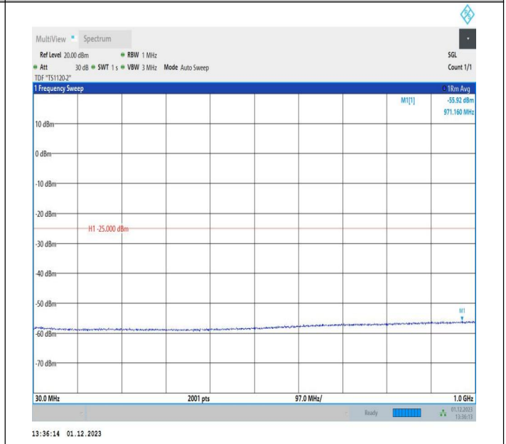
7-7-10MHz-20MHz-16QAM-16QAM-21206-21350-1RB#0-0RB #0-30~1000MHz-PASS
