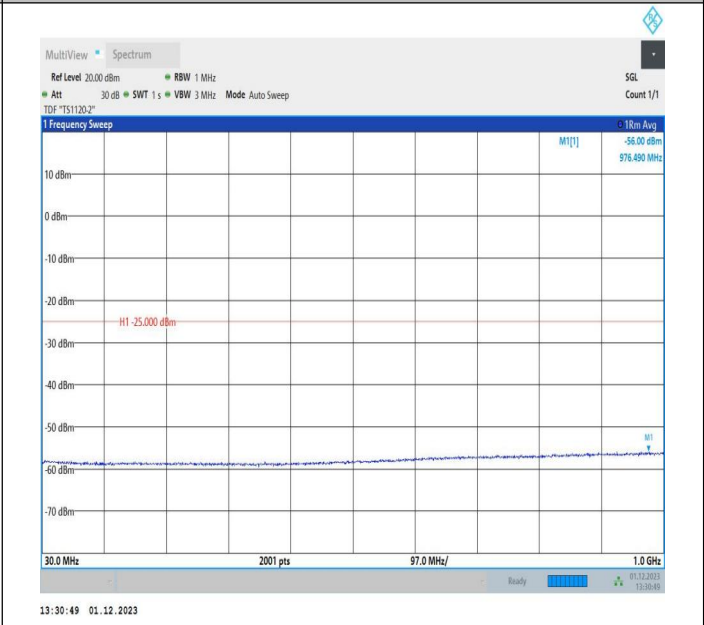
7-7-10MHz-20MHz-64QAM-64QAM-21006-21150-1RB#49-OR B#0-30~1000MHz-PASS
