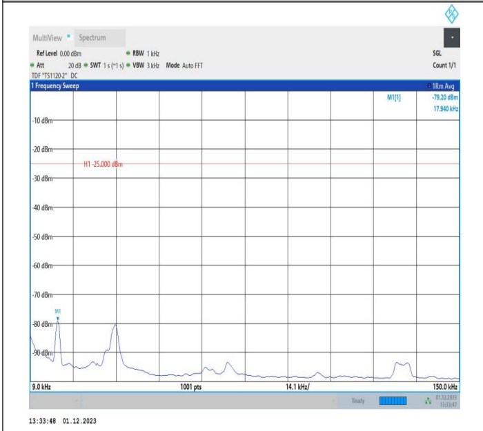
7-7-10MHz-20MHz-16QAM-16QAM-21006-21150-50RB#0-100 RB#0-0.009~0.15MHz-PASS
