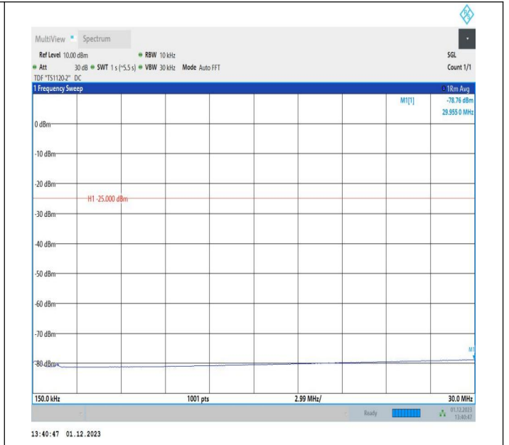
7-7-10MHz-20MHz-64QAM-64QAM-21206-21350-1RB#0-1RB #99-0.15~30MHz-PASS
