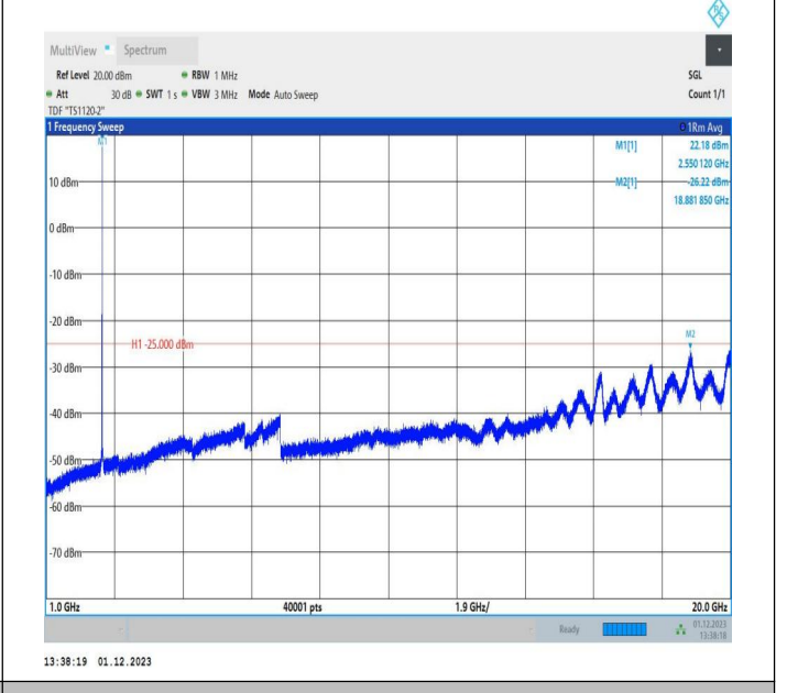
7-7-10MHz-20MHz-16QAM-16QAM-21206-21350-1RB#49-OR B#0-1000~20000MHz-PASS
