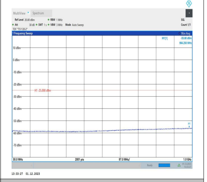
7-7-10MHz-20MHz-QPSK-QPSK-21006-21150-50RB#0-100R B#0-30~1000MHz-PASS
