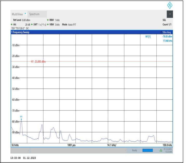
7-7-10MHz-20MHz-QPSK-QPSK-21006-21150-50RB#0-100R B#0-0.009~0.15MHz-PASS
