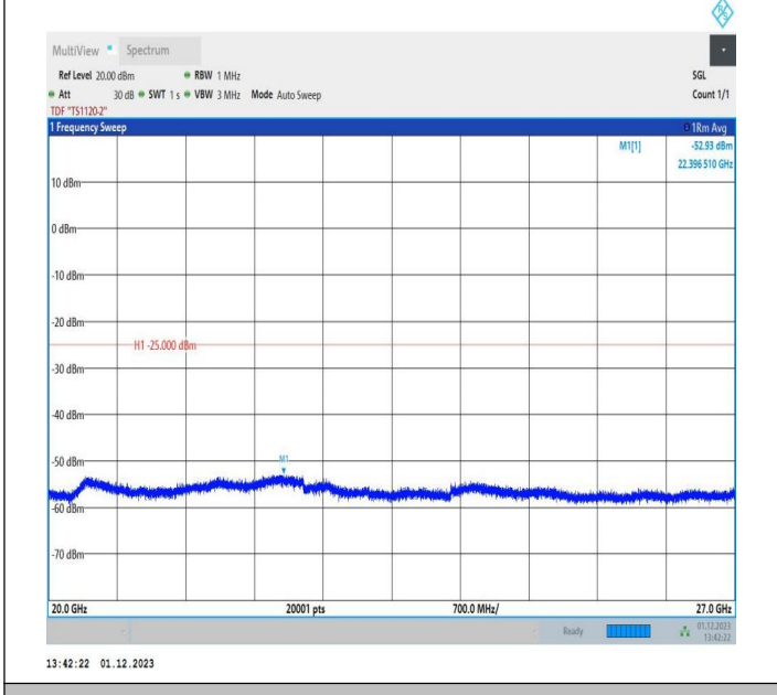
7-7-10MHz-20MHz-16QAM-16QAM-21206-21350-50RB#0-10 ORB#0-20000~27000MHz-PASS
