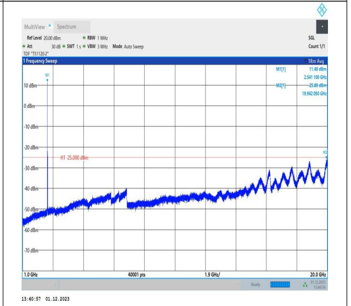
7-7-10MHz-20MHz-64QAM-64QAM-21206-21350-1RB#0-1RB #99-1000~20000MHz-PASS
