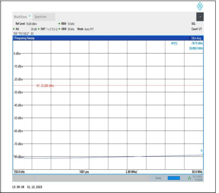
7-7-10MHz-20MHz-16QAM-16QAM-21206-21350-1RB#49-OR B#0-0.15~30MHz-PASS
