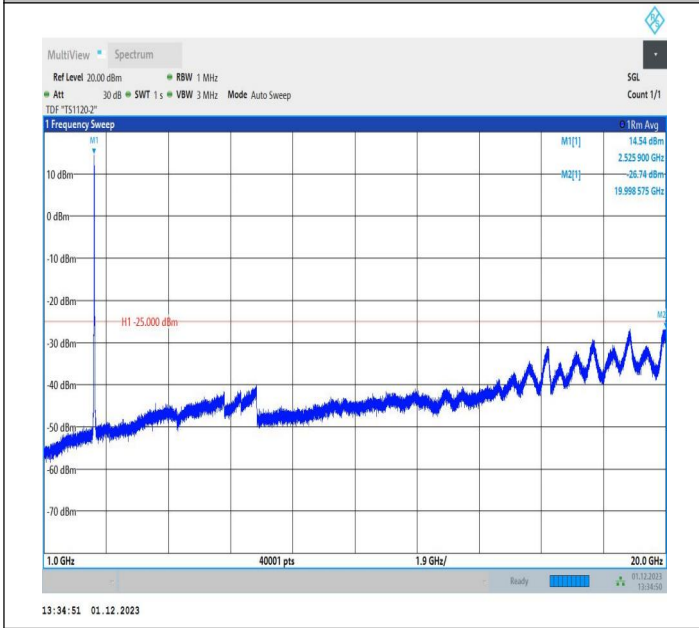
7-7-10MHz-20MHz-64QAM-64QAM-21006-21150-50RB#0-100 RB#0-1000~20000MHz-PASS
