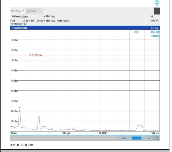
7-7-10MHz-20MHz-16QAM-16QAM-21006-21150-1RB#0-1RB #99-0.009~0.15MHz-PASS
