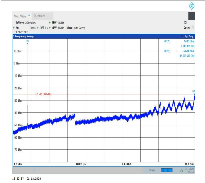
7-7-10MHz-20MHz-64QAM-64QAM-21206-21350-50RB#0-10 ORB#0-1000~20000MHz-PASS
