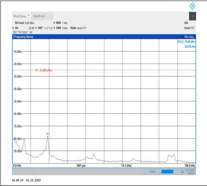
7-7-15MHz-10MHz-QPSK-QPSK-20825-20945-1RB#0-0RB#0 -0.009~0.15MHz-PASS
