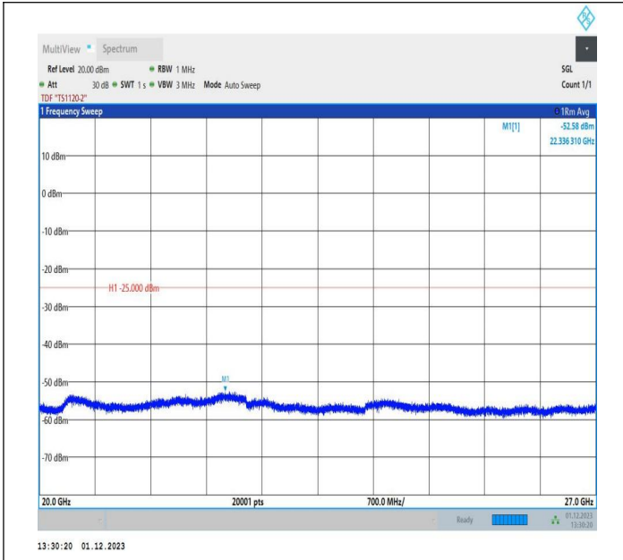
7-7-10MHz-20MHz-16QAM-16QAM-21006-21150-1RB#49-OR B#0-20000~27000MHz-PASS
