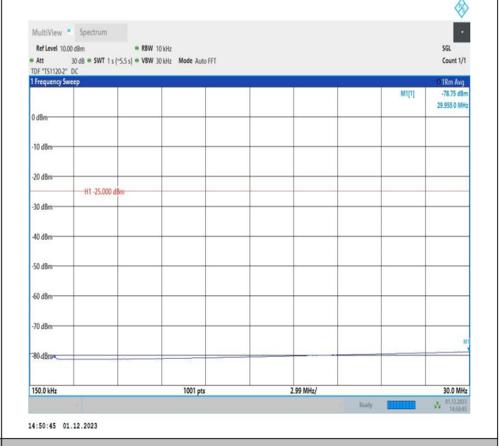
7-7-15MHz-10MHz-64QAM-64QAM-20825-20945-1RB#0-ORB #0-0.15~30MHz-PASS
