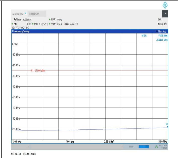
7-7-10MHz-20MHz-64QAM-64QAM-21006-21150-1RB#0-1RB #99-0.15~30MHz-PASS
