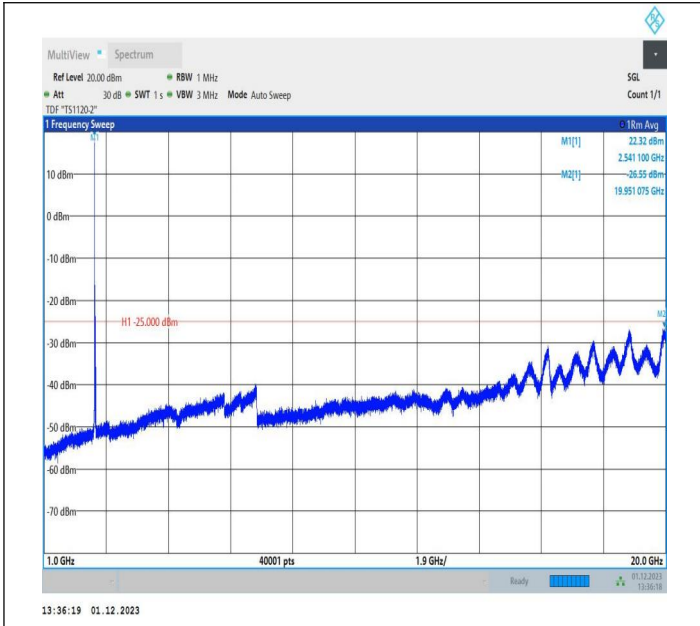
7-7-10MHz-20MHz-16QAM-16QAM-21206-21350-1RB#0-ORB #0-1000~20000MHz-PASS
