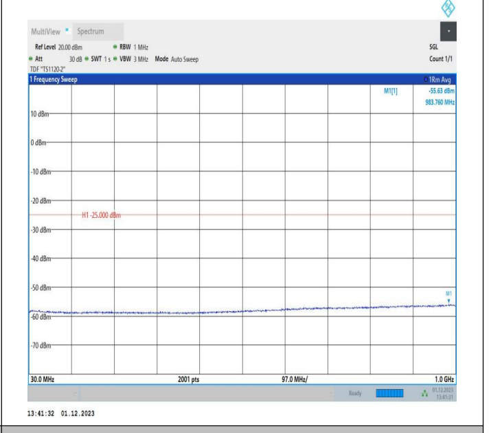
7-7-10MHz-20MHz-QPSK-QPSK-21206-21350-50RB#0-100R B#0-30~1000MHz-PASS
