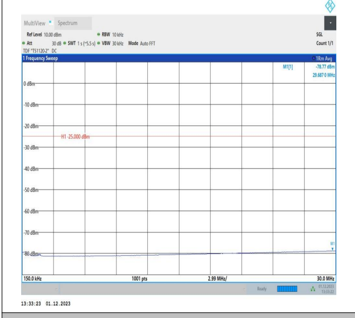
7-7-10MHz-20MHz-QPSK-QPSK-21006-21150-50RB#0-100R B#0-0.15~30MHz-PASS
