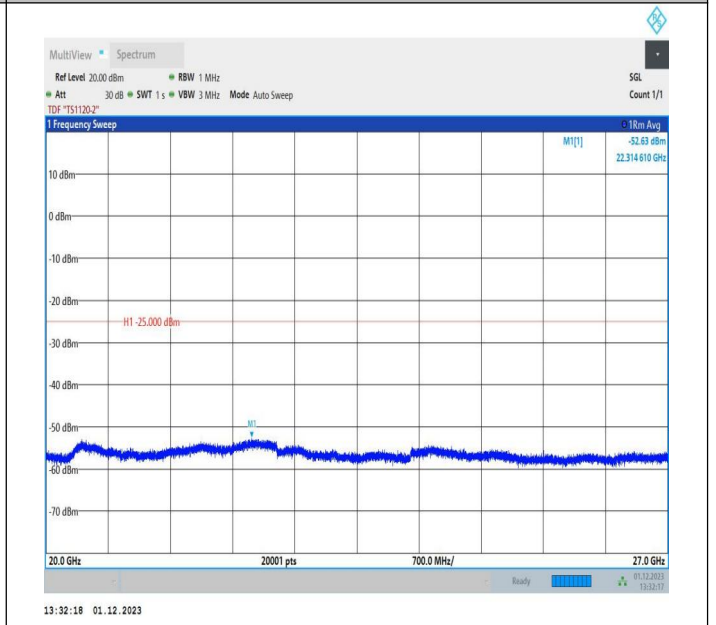
7-7-10MHz-20MHz-16QAM-16QAM-21006-21150-1RB#0-1RB #99-20000~27000MHz-PASS
