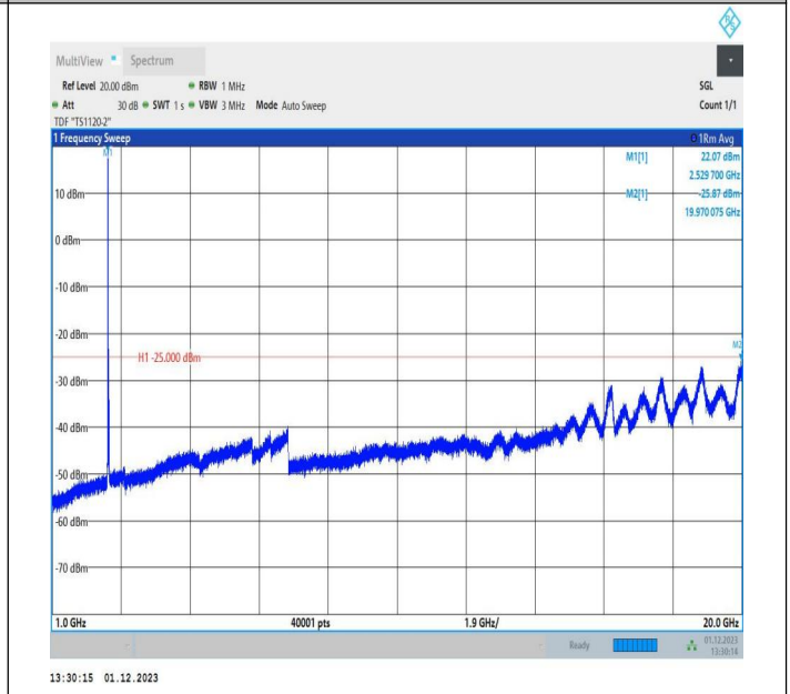
7-7-10MHz-20MHz-16QAM-16QAM-21006-21150-1RB#49-OR B#0-1000~20000MHz-PASS
