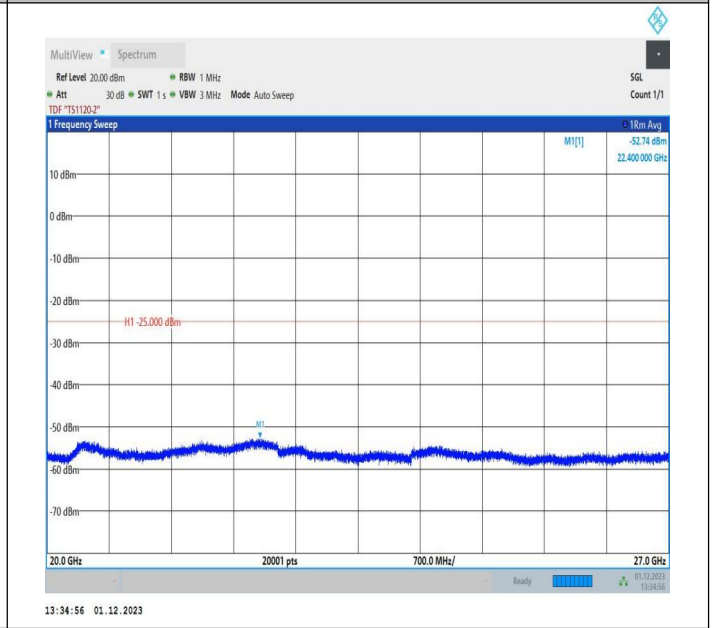
7-7-10MHz-20MHz-64QAM-64QAM-21006-21150-50RB#0-100 RB#0-20000~27000MHz-PASS
