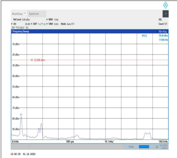
7-7-10MHz-20MHz-64QAM-64QAM-21206-21350-1RB#0-1RB #99-0.009~0.15MHz-PASS
