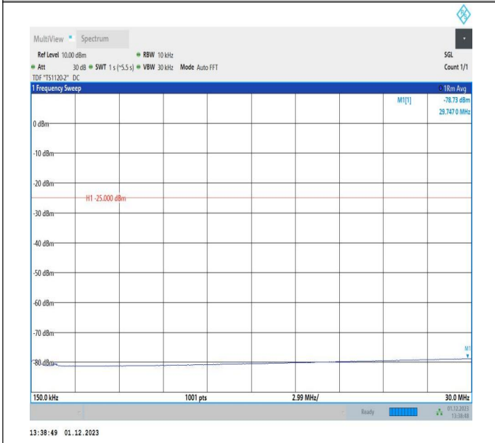
7-7-10MHz-20MHz-64QAM-64QAM-21206-21350-1RB#49-0R B#0-0.15~30MHz-PASS
