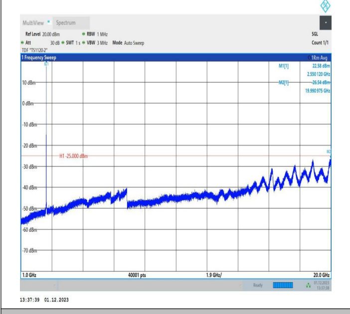
7-7-10MHz-20MHz-QPSK-QPSK-21206-21350-1RB#49-0RB# 0-1000~20000MHz-PASS
