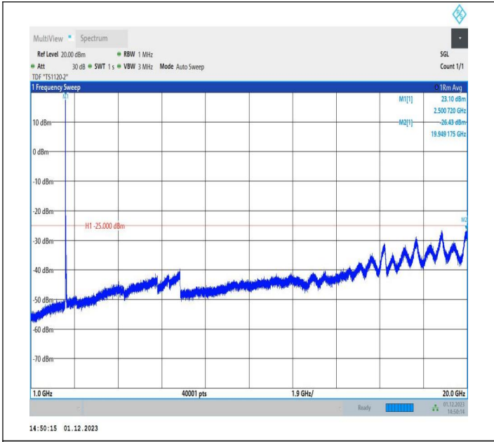
7-7-15MHz-10MHz-16QAM-16QAM-20825-20945-1RB#0-ORB #0-1000~20000MHz-PASS
