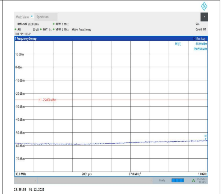
7-7-10MHz-20MHz-64QAM-64QAM-21206-21350-1RB#49-0R B#0-30~1000MHz-PASS
