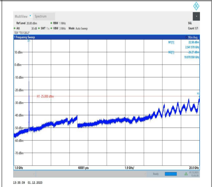
7-7-10MHz-20MHz-QPSK-QPSK-21206-21350-1RB#0-0RB#0 -1000~20000MHz-PASS
