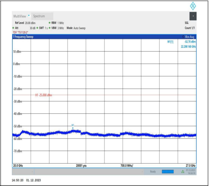
7-7-15MHz-10MHz-16QAM-16QAM-20825-20945-1RB#0-ORB #0-20000~27000MHz-PASS
