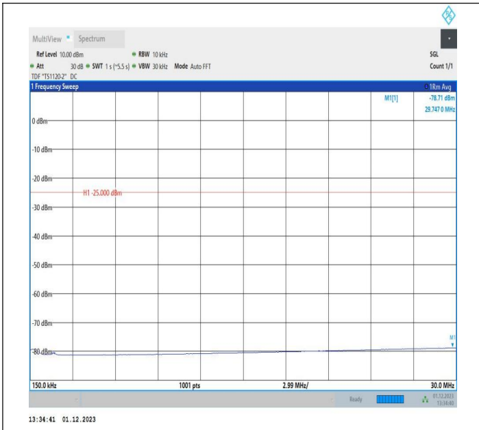
7-7-10MHz-20MHz-64QAM-64QAM-21006-21150-50RB#0-100 RB#0-0.15~30MHz-PASS
