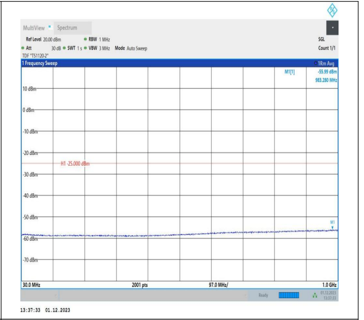
7-7-10MHz-20MHz-QPSK-QPSK-21206-21350-1RB#49-0RB# 0-30~1000MHz-PASS
