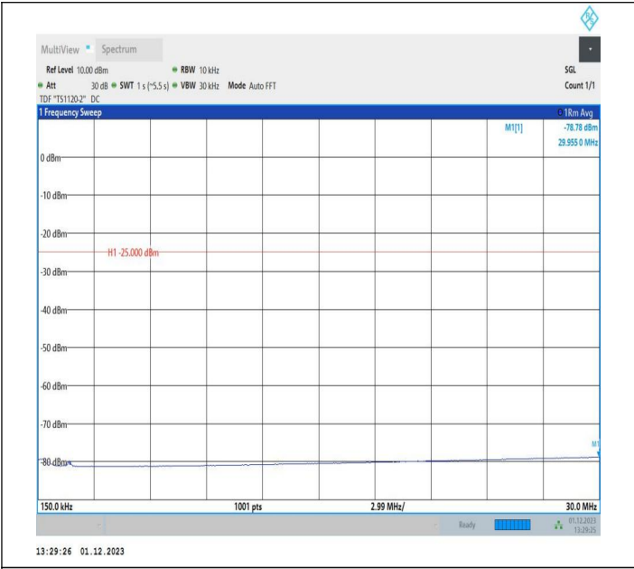
7-7-10MHz-20MHz-QPSK-QPSK-21006-21150-1RB#49-0RB# 0-0.15~30MHz-PASS
