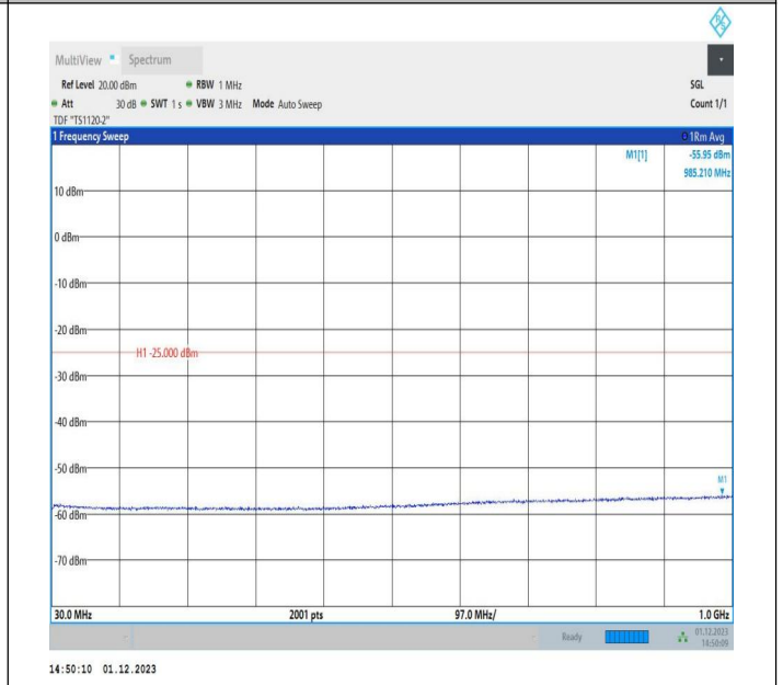
7-7-15MHz-10MHz-16QAM-16QAM-20825-20945-1RB#0-0RB #0-30~1000MHz-PASS
