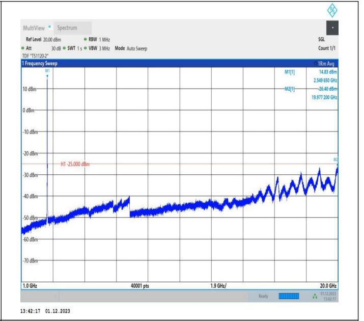
7-7-10MHz-20MHz-16QAM-16QAM-21206-21350-50RB#0-10 ORB#0-1000~20000MHz-PASS
