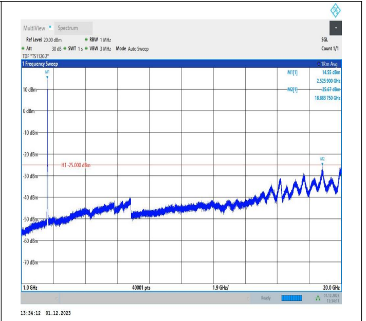
7-7-10MHz-20MHz-16QAM-16QAM-21006-21150-50RB#0-100 RB#0-1000~20000MHz-PASS
