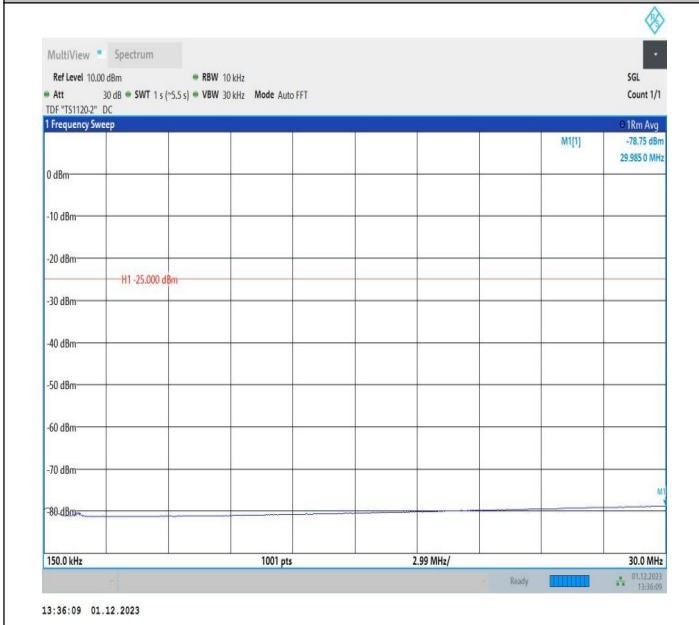
7-7-10MHz-20MHz-16QAM-16QAM-21206-21350-1RB#0-0RB #0-0.15~30MHz-PASS
