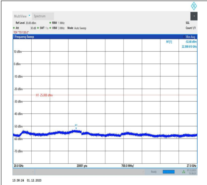
7-7-10MHz-20MHz-16QAM-16QAM-21206-21350-1RB#49-0R B#0-20000~27000MHz-PASS
