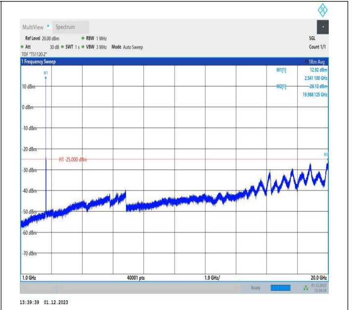
7-7-10MHz-20MHz-QPSK-QPSK-21206-21350-1RB#0-1RB#9 9-1000~20000MHz-PASS
