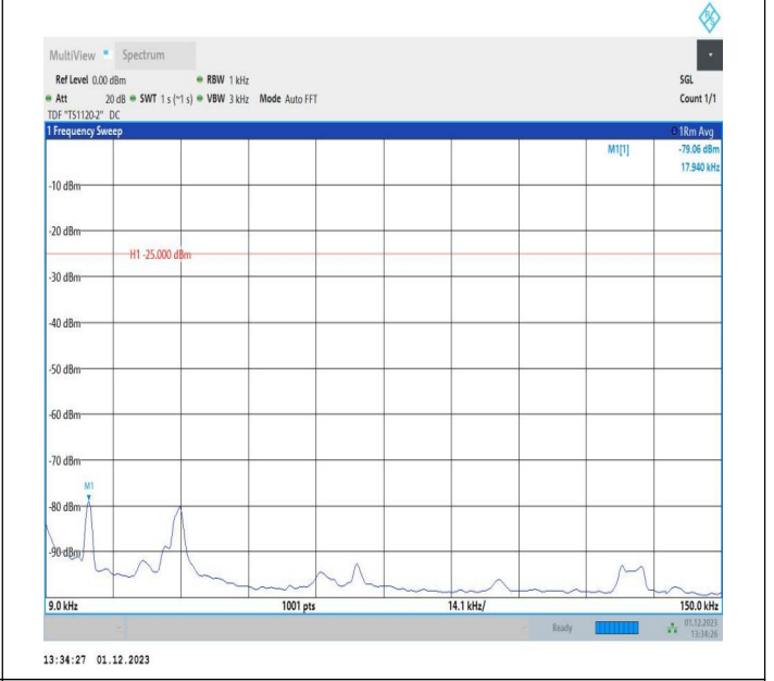
7-7-10MHz-20MHz-64QAM-64QAM-21006-21150-50RB#0-100 RB#0-0.009~0.15MHz-PASS
