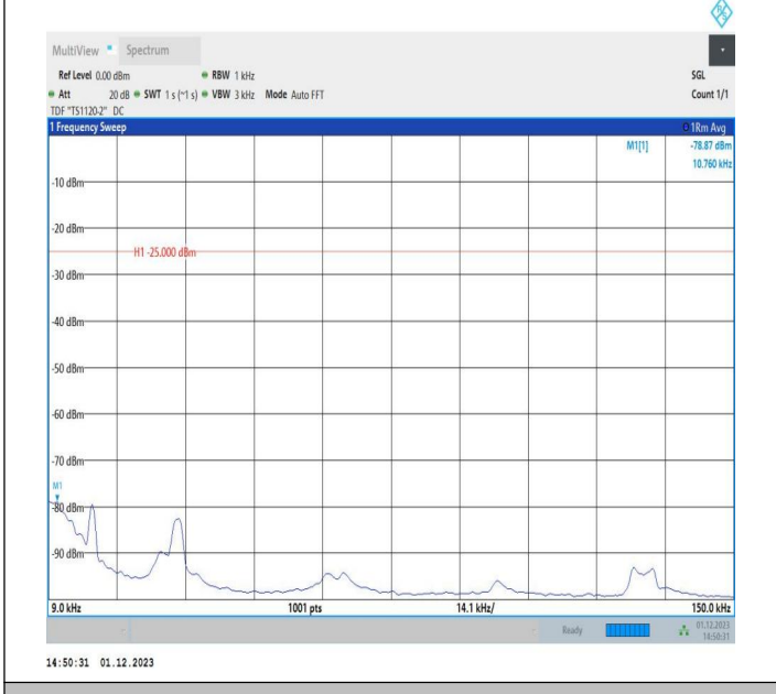
7-7-15MHz-10MHz-64QAM-64QAM-20825-20945-1RB#0-ORB #0-0.009~0.15MHz-PASS
