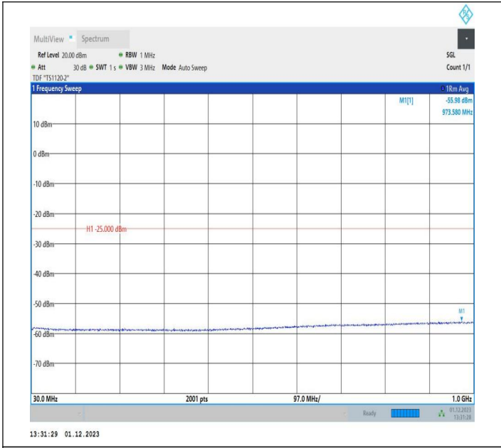
7-7-10MHz-20MHz-QPSK-QPSK-21006-21150-1RB#0-1RB#9 9-30~1000MHz-PASS
