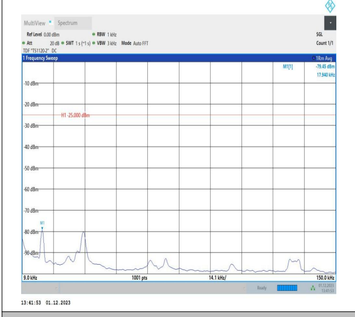
7-7-10MHz-20MHz-16QAM-16QAM-21206-21350-50RB#0-10 ORB#0-0.009~0.15MHz-PASS
