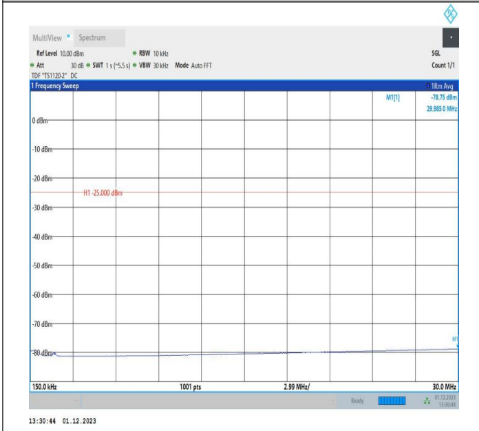
7-7-10MHz-20MHz-64QAM-64QAM-21006-21150-1RB#49-OR B#0-0.15~30MHz-PASS
