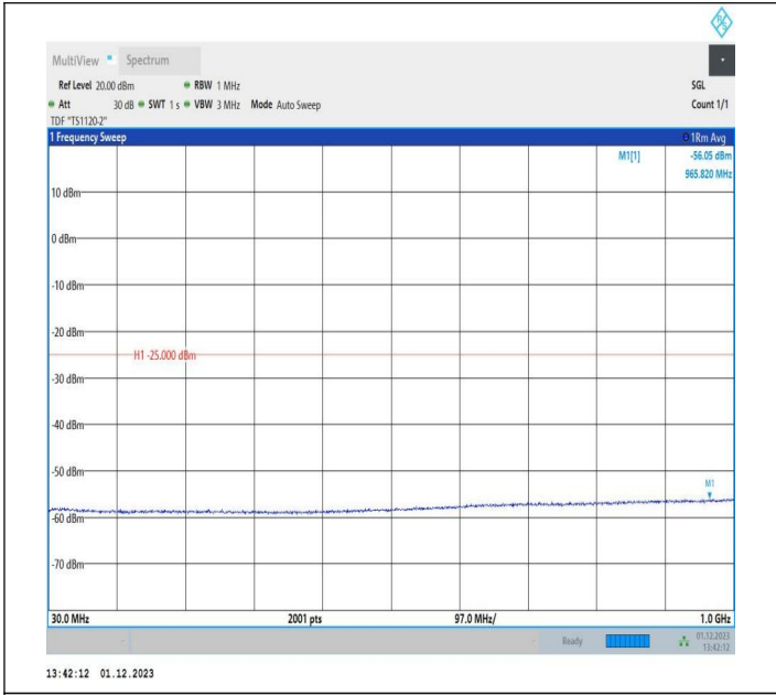
7-7-10MHz-20MHz-16QAM-16QAM-21206-21350-50RB#0-10 ORB#0-30~1000MHz-PASS
