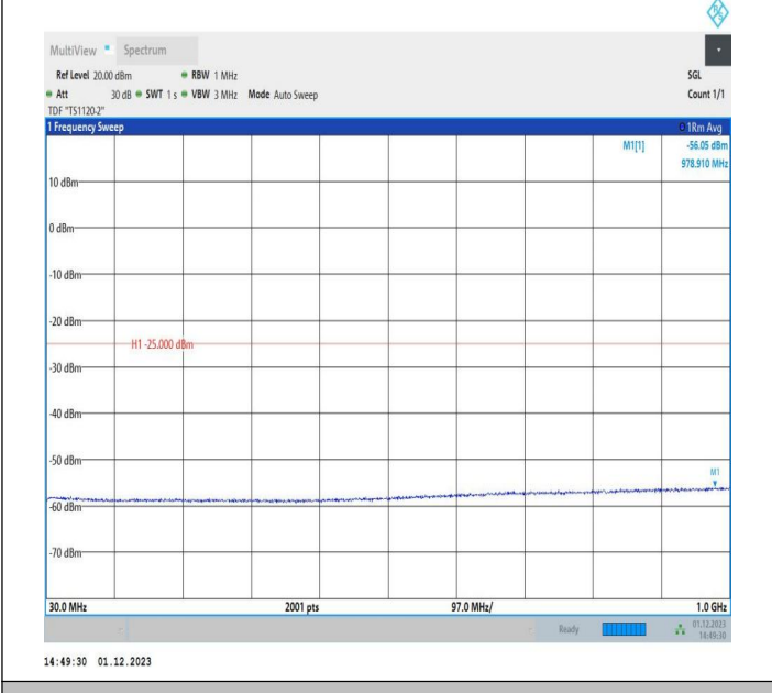
7-7-15MHz-10MHz-QPSK-QPSK-20825-20945-1RB#0-0RB#0 -30~1000MHz-PASS
