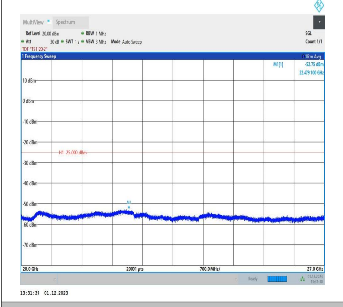
7-7-10MHz-20MHz-QPSK-QPSK-21006-21150-1RB#0-1RB#9 9-20000~27000MHz-PASS
