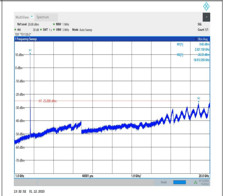
7-7-10MHz-20MHz-64QAM-64QAM-21006-21150-1RB#0-1RB #99-1000~20000MHz-PASS
