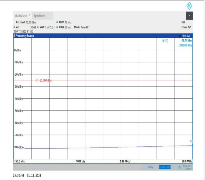
7-7-10MHz-20MHz-16QAM-16QAM-21006-21150-1RB#49-OR B#0-0.15~30MHz-PASS
