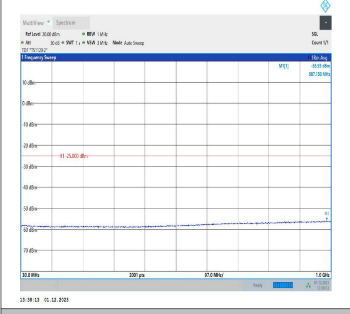
7-7-10MHz-20MHz-16QAM-16QAM-21206-21350-1RB#49-OR B#0-30~1000MHz-PASS
