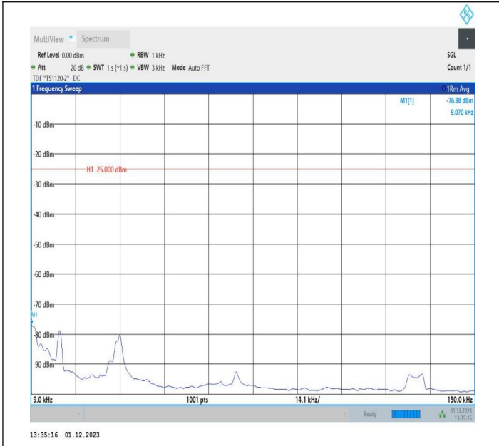
7-7-10MHz-20MHz-QPSK-QPSK-21206-21350-1RB#0-0RB#0 -0.009~0.15MHz-PASS
