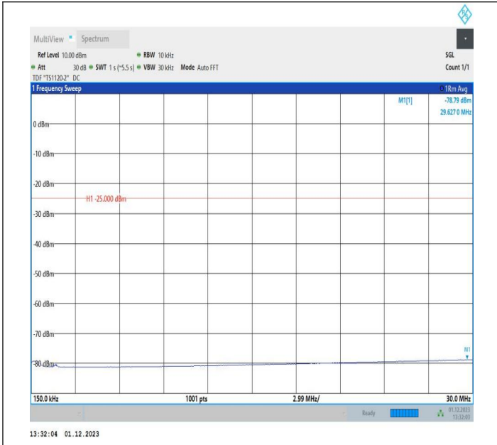
7-7-10MHz-20MHz-16QAM-16QAM-21006-21150-1RB#0-1RB #99-0.15~30MHz-PASS
