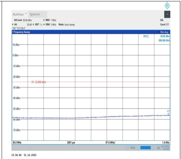
7-7-10MHz-20MHz-64QAM-64QAM-21006-21150-50RB#0-100 RB#0-30~1000MHz-PASS
