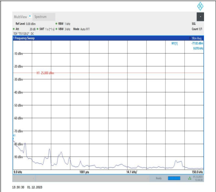
7-7-10MHz-20MHz-64QAM-64QAM-21006-21150-1RB#49-OR B#0-0.009~0.15MHz-PASS
