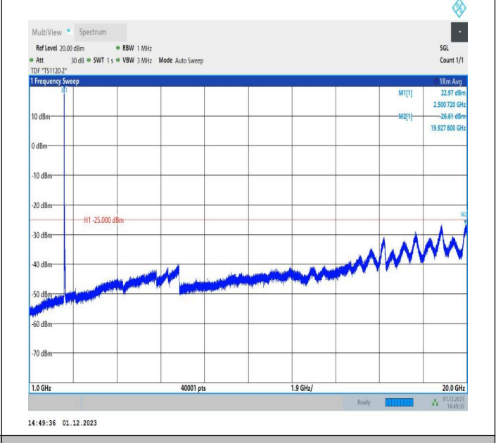
7-7-15MHz-10MHz-QPSK-QPSK-20825-20945-1RB#0-0RB#0 -1000~20000MHz-PASS
