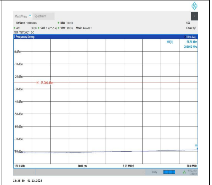
7-7-10MHz-20MHz-64QAM-64QAM-21206-21350-1RB#0-ORB #0-0.15~30MHz-PASS
