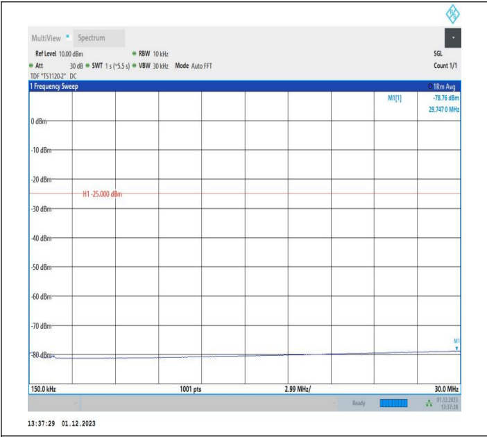
7-7-10MHz-20MHz-QPSK-QPSK-21206-21350-1RB#49-0RB# 0-0.15~30MHz-PASS
