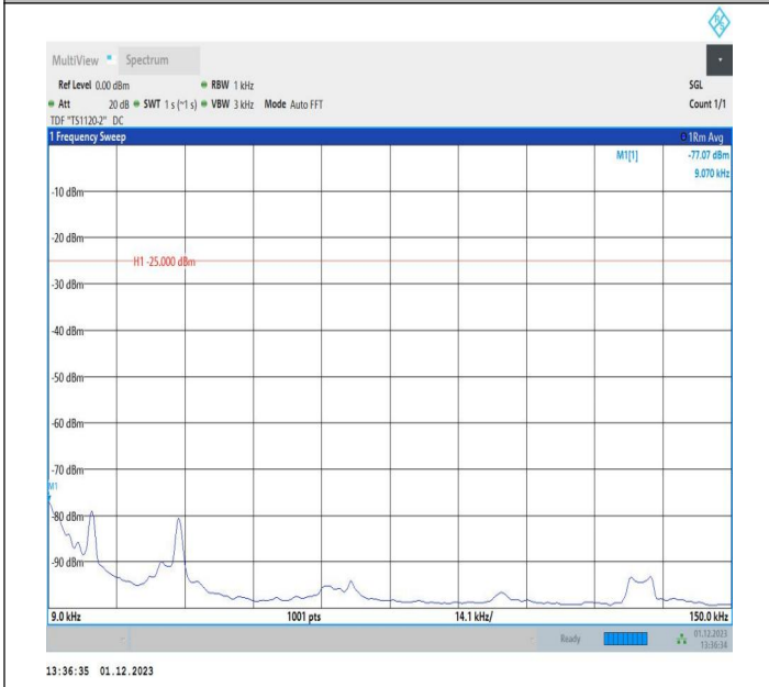
7-7-10MHz-20MHz-64QAM-64QAM-21206-21350-1RB#0-ORB #0-0.009~0.15MHz-PASS
