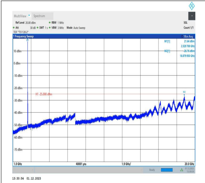
7-7-10MHz-20MHz-64QAM-64QAM-21006-21150-1RB#49-0R B#0-1000~20000MHz-PASS
