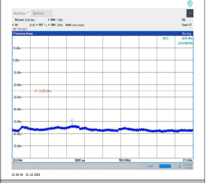
7-7-10MHz-20MHz-QPSK-QPSK-21006-21150-1RB#49-0RB# 0-20000~27000MHz-PASS
