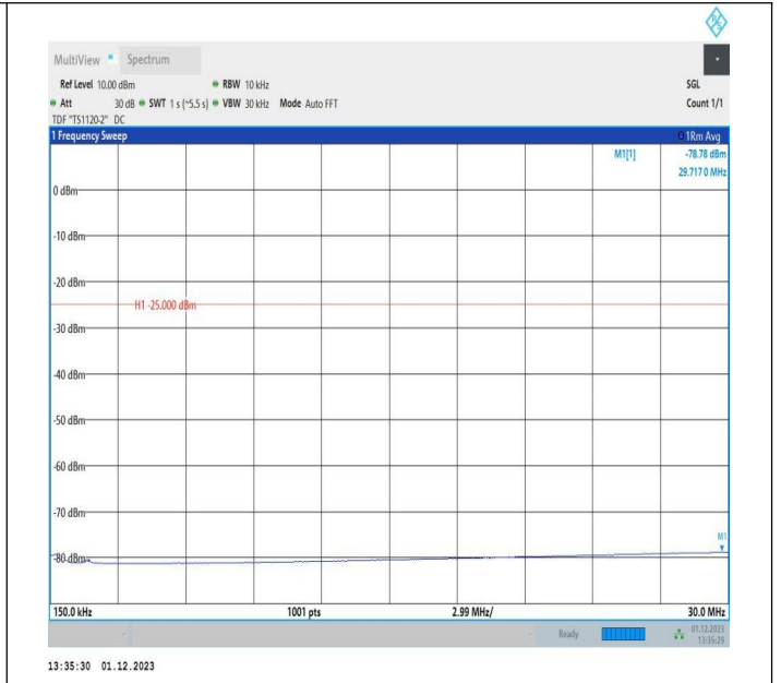
7-7-10MHz-20MHz-QPSK-QPSK-21206-21350-1RB#0-0RB#0 -0.15~30MHz-PASS
