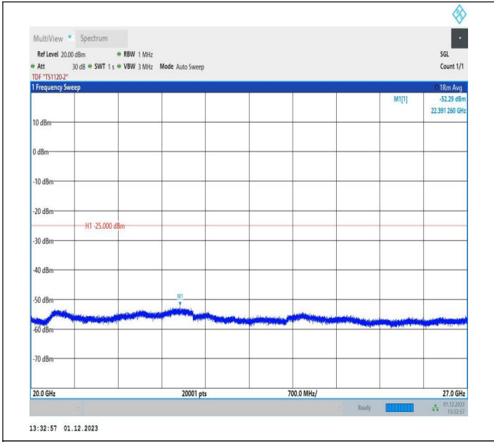
7-7-10MHz-20MHz-64QAM-64QAM-21006-21150-1RB#0-1RB #99-20000~27000MHz-PASS
