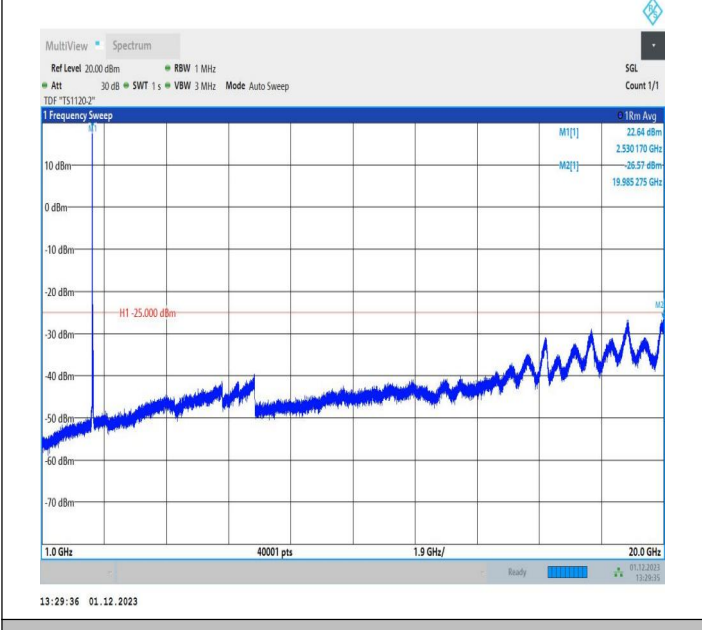
7-7-10MHz-20MHz-QPSK-QPSK-21006-21150-1RB#49-0RB# 0-1000~20000MHz-PASS
