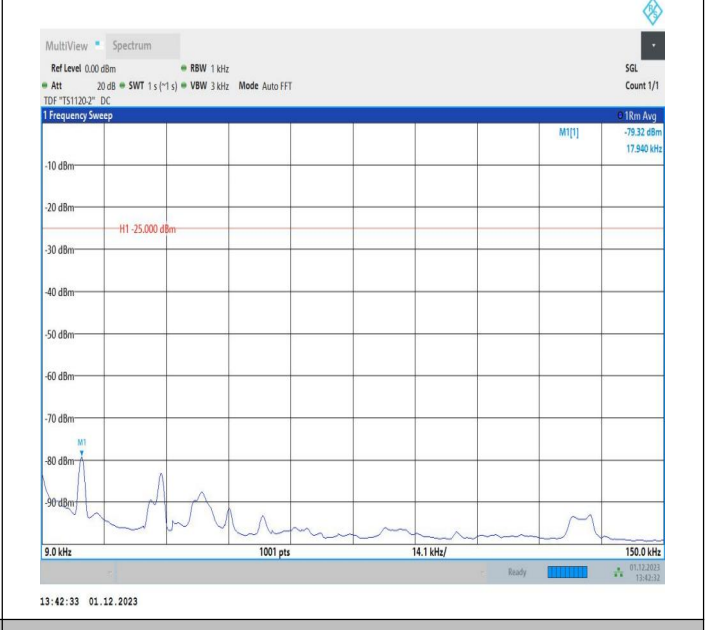
7-7-10MHz-20MHz-64QAM-64QAM-21206-21350-50RB#0-10 ORB#0-0.009~0.15MHz-PASS
