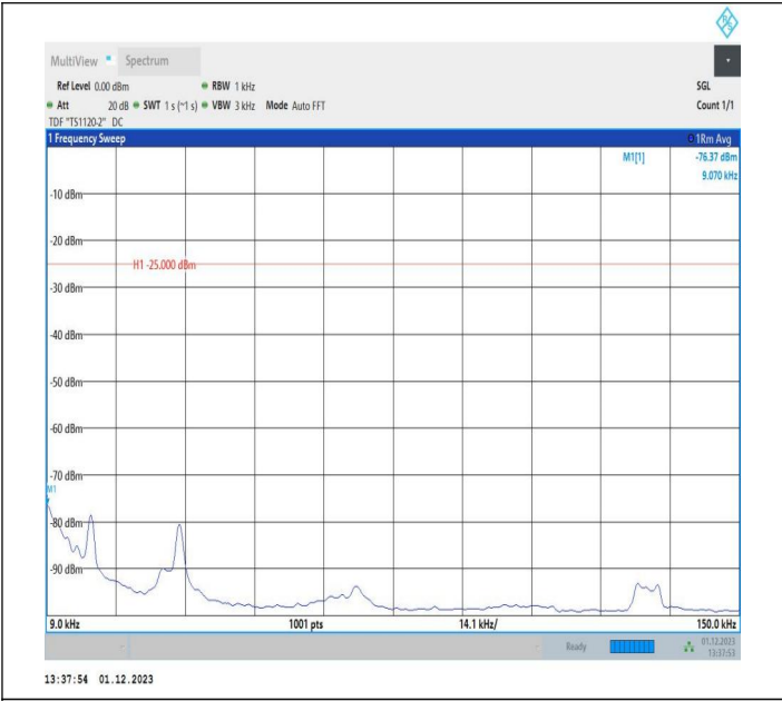
7-7-10MHz-20MHz-16QAM-16QAM-21206-21350-1RB#49-OR B#0-0.009~0.15MHz-PASS
