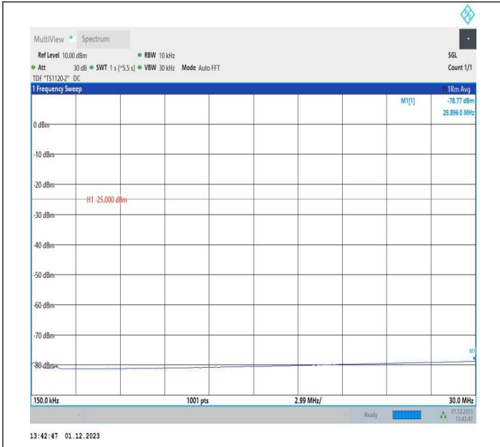
7-7-10MHz-20MHz-64QAM-64QAM-21206-21350-50RB#0-10 ORB#0-0.15~30MHz-PASS
