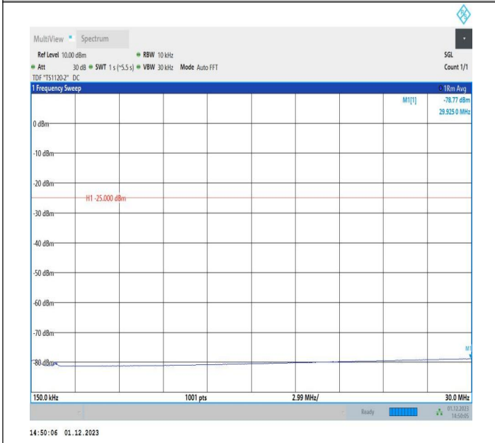
7-7-15MHz-10MHz-16QAM-16QAM-20825-20945-1RB#0-0RB #0-0.15~30MHz-PASS
