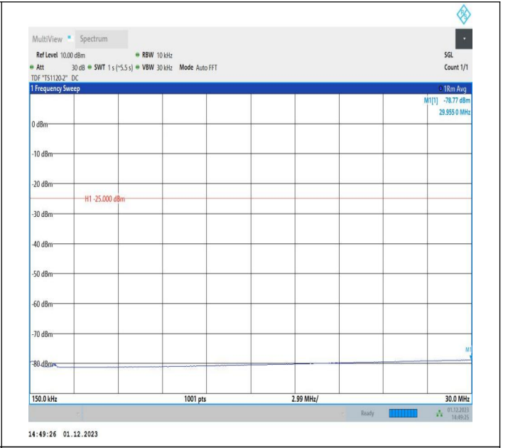
7-7-15MHz-10MHz-QPSK-QPSK-20825-20945-1RB#0-0RB#0 -0.15~30MHz-PASS
