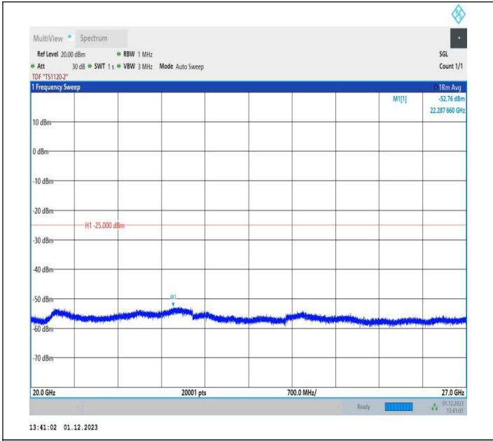
7-7-10MHz-20MHz-64QAM-64QAM-21206-21350-1RB#0-1RB #99-20000~27000MHz-PASS
