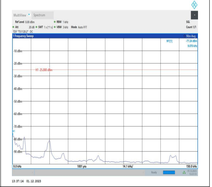
7-7-10MHz-20MHz-QPSK-QPSK-21206-21350-1RB#49-ORB# 0-0.009~0.15MHz-PASS
