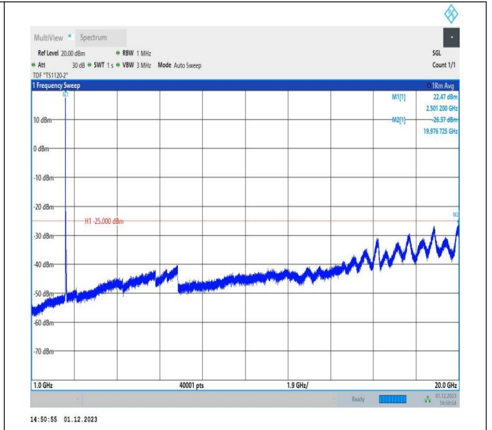
7-7-15MHz-10MHz-64QAM-64QAM-20825-20945-1RB#0-ORB #0-1000~20000MHz-PASS
