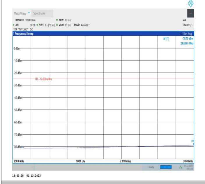
7-7-10MHz-20MHz-QPSK-QPSK-21206-21350-50RB#0-100R B#0-0.15~30MHz-PASS
