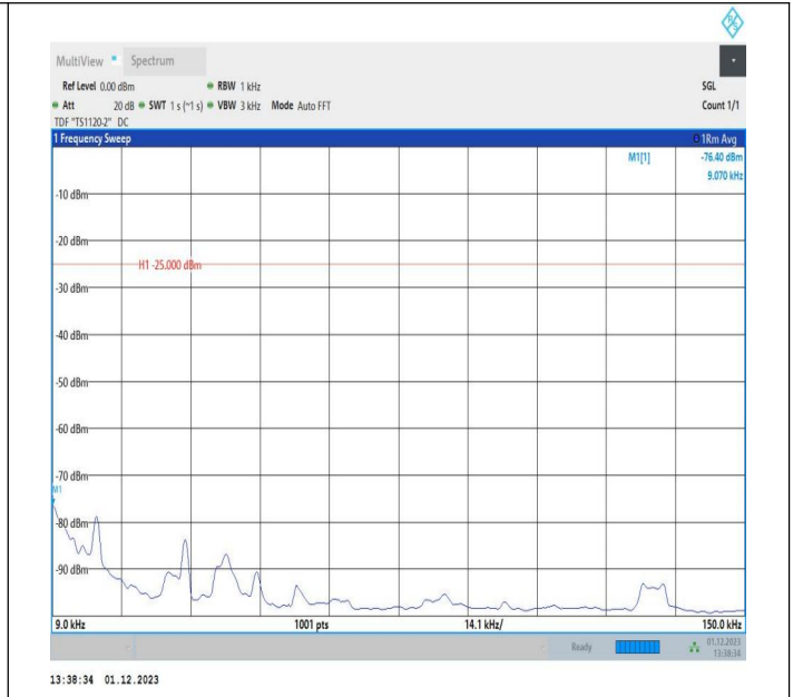
7-7-10MHz-20MHz-64QAM-64QAM-21206-21350-1RB#49-0R B#0-0.009~0.15MHz-PASS
