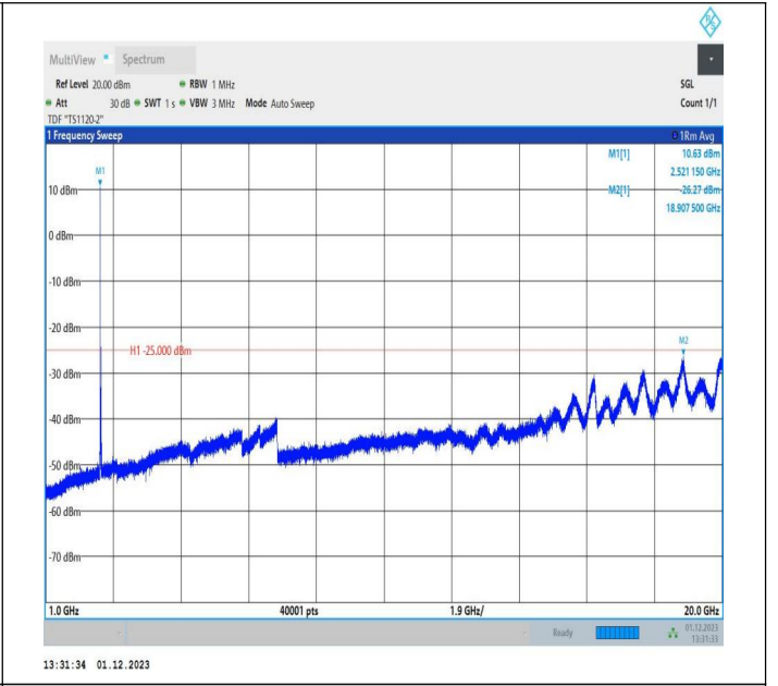
7-7-10MHz-20MHz-QPSK-QPSK-21006-21150-1RB#0-1RB#9 9-1000~20000MHz-PASS
