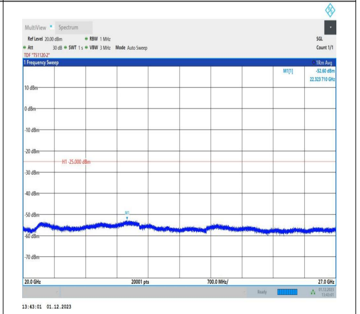
7-7-10MHz-20MHz-64QAM-64QAM-21206-21350-50RB#0-10 ORB#0-20000~27000MHz-PASS
