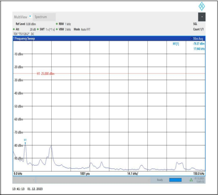
7-7-10MHz-20MHz-QPSK-QPSK-21206-21350-50RB#0-100R B#0-0.009~0.15MHz-PASS
