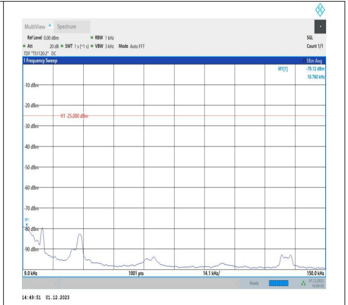
7-7-15MHz-10MHz-16QAM-16QAM-20825-20945-1RB#0-0RB #0-0.009~0.15MHz-PASS
