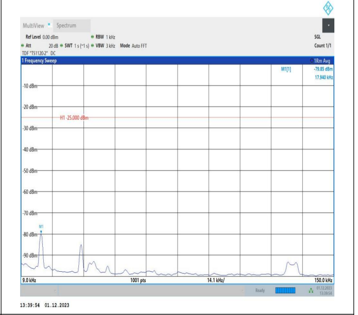
7-7-10MHz-20MHz-16QAM-16QAM-21206-21350-1RB#0-1RB #99-0.009~0.15MHz-PASS
