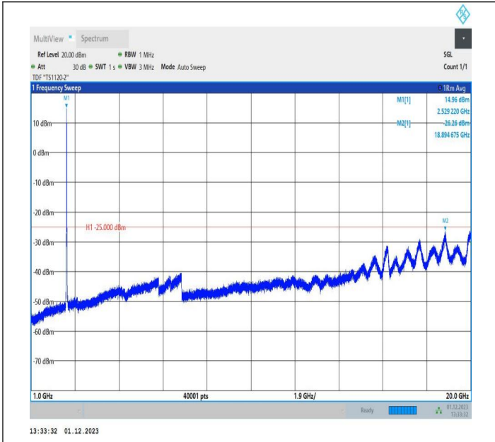
7-7-10MHz-20MHz-QPSK-QPSK-21006-21150-50RB#0-100R B#0-1000~20000MHz-PASS
