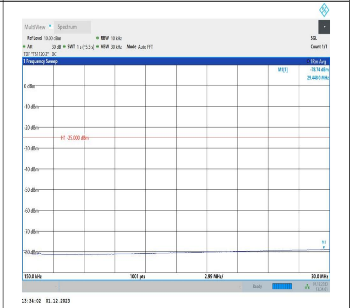
7-7-10MHz-20MHz-16QAM-16QAM-21006-21150-50RB#0-100 RB#0-0.15~30MHz-PASS
