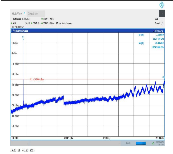
7-7-10MHz-20MHz-16QAM-16QAM-21006-21150-1RB#0-1RB #99-1000~20000MHz-PASS
