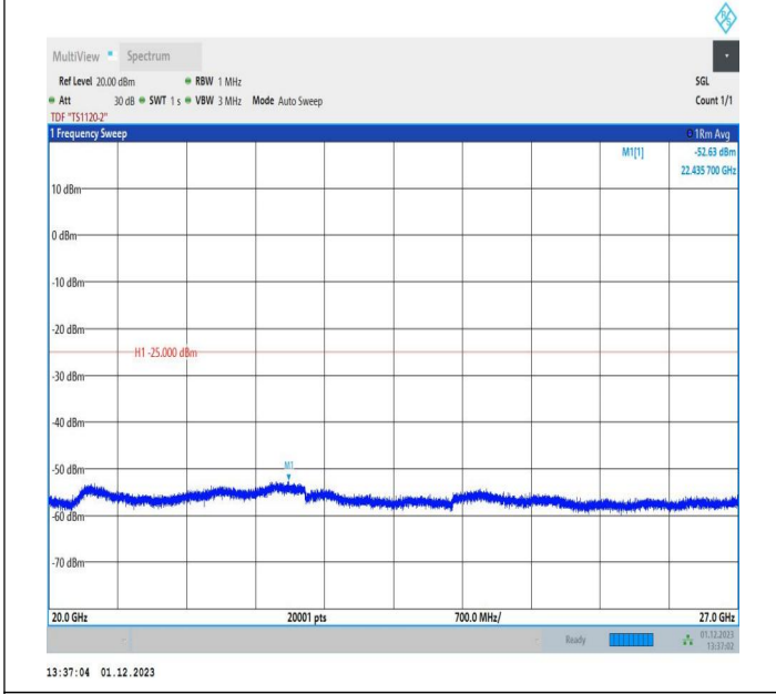
7-7-10MHz-20MHz-64QAM-64QAM-21206-21350-1RB#0-ORB #0-20000~27000MHz-PASS
