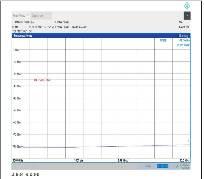
7-7-15MHz-5MHz-16QAM-16QAM-21327-21420-1RB#74-0RB #0-0.15~30MHz-PASS
