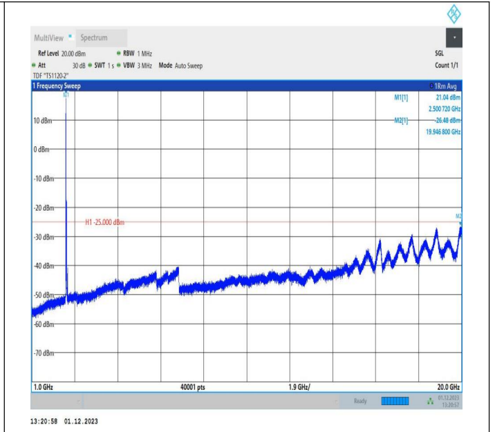
7-7-10MHz-20MHz-64QAM-64QAM-20805-20949-1RB#0-ORB #0-1000~20000MHz-PASS
