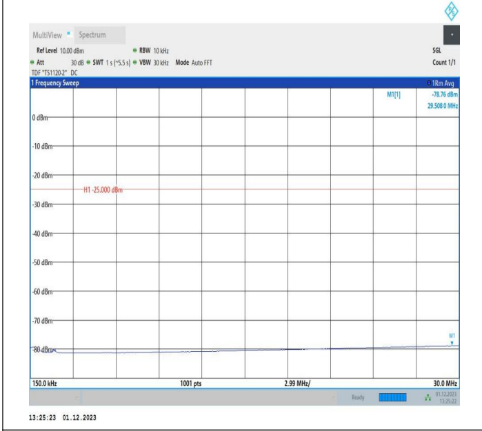
7-7-10MHz-20MHz-QPSK-QPSK-20805-20949-50RB#0-100R B#0-0.15~30MHz-PASS
