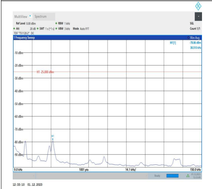
7-7-15MHz-5MHz-16QAM-16QAM-21327-21420-75RB#0-25R B#0-0.009~0.15MHz-PASS
