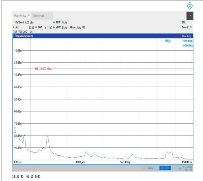
7-7-10MHz-20MHz-16QAM-16QAM-20805-20949-1RB#49-OR B#0-0.009~0.15MHz-PASS
