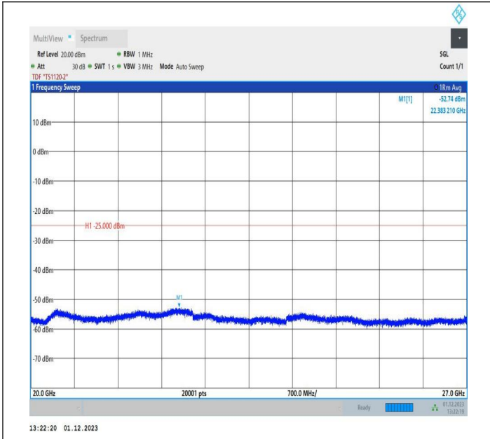
7-7-10MHz-20MHz-16QAM-16QAM-20805-20949-1RB#49-0R B#0-20000~27000MHz-PASS
