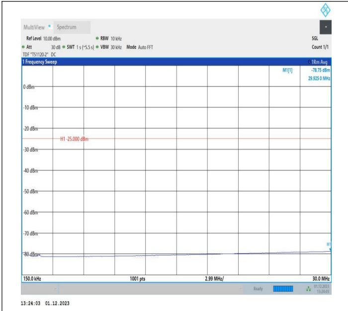
7-7-10MHz-20MHz-16QAM-16QAM-20805-20949-1RB#0-1RB #99-0.15~30MHz-PASS
