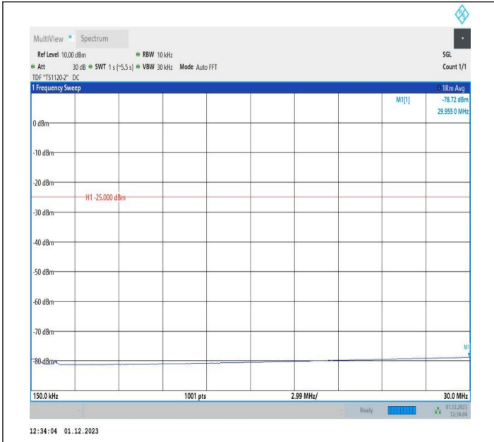
7-7-15MHz-5MHz-64QAM-64QAM-21327-21420-75RB#0-25R B#0-0.15~30MHz-PASS
