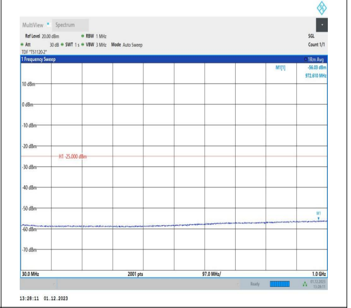
7-7-10MHz-20MHz-16QAM-16QAM-21006-21150-1RB#0-ORB#0-30~1000MHz-PASS
