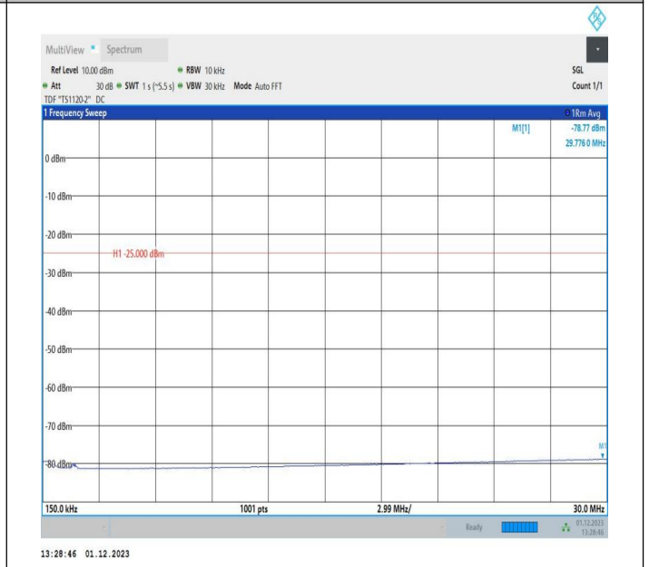
7-7-10MHz-20MHz-64QAM-64QAM-21006-21150-1RB#0-ORB #0-0.15~30MHz-PASS
