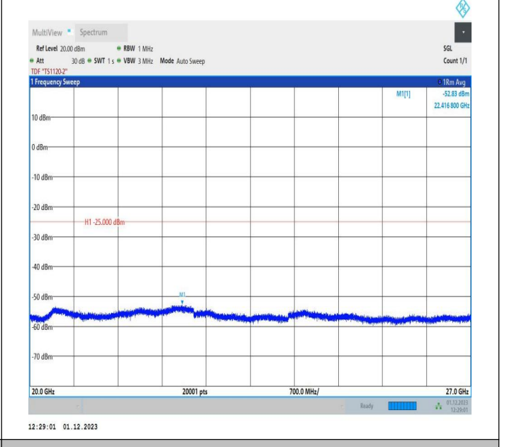
7-7-15MHz-5MHz-QPSK-QPSK-21327-21420-1RB#74-0RB#0 -20000~27000MHz-PASS
