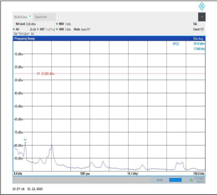
7-7-10MHz-20MHz-QPSK-QPSK-21006-21150-1RB#0-ORB#0-0.009~0.15MHz-PASS
