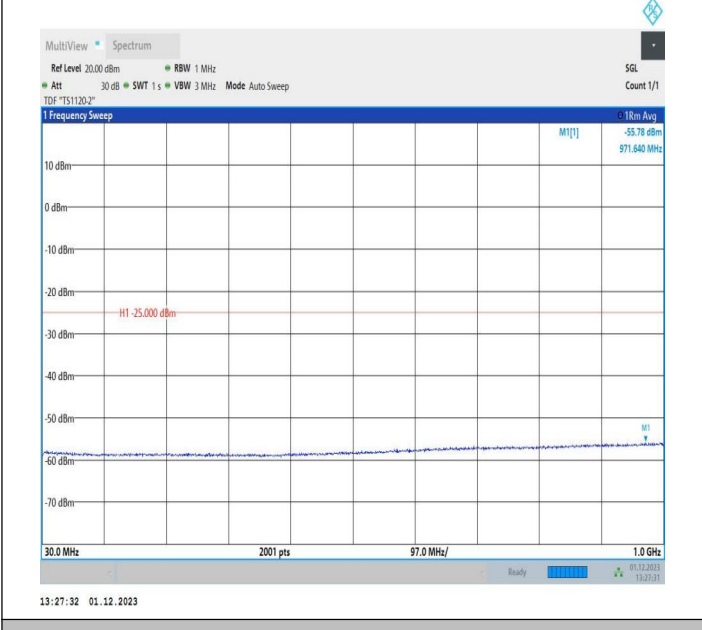
7-7-10MHz-20MHz-QPSK-QPSK-21006-21150-1RB#0-ORB#0-30~1000MHz-PASS
