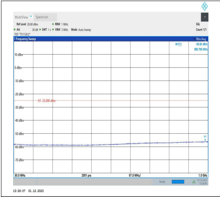
7-7-10MHz-20MHz-16QAM-16QAM-20805-20949-50RB#0-10 ORB#0-30~1000MHz-PASS
