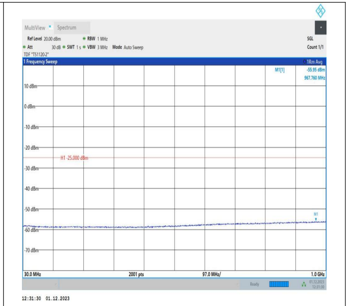
7-7-15MHz-5MHz-16QAM-16QAM-21327-21420-1RB#0-1RB# 24-30~1000MHz-PASS
