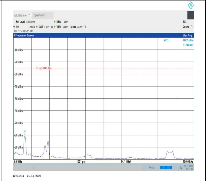
7-7-15MHz-5MHz-16QAM-16QAM-21327-21420-1RB#0-1RB#24 24-0.009~0.15MHz-PASS
