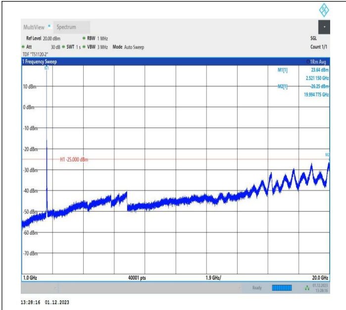
7-7-10MHz-20MHz-16QAM-16QAM-21006-21150-1RB#0-ORB #0-1000~20000MHz-PASS
