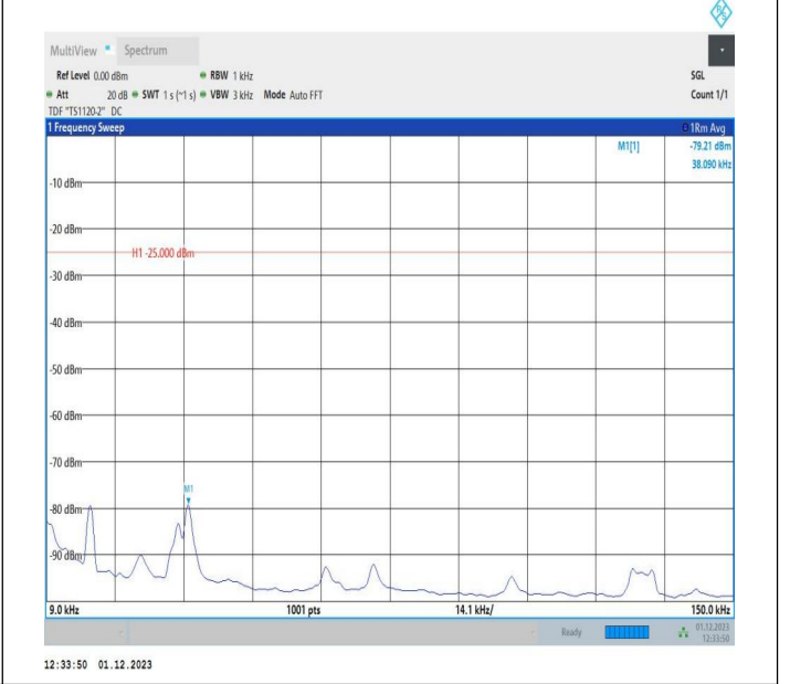
7-7-15MHz-5MHz-64QAM-64QAM-21327-21420-75RB#0-25R B#0-0.009~0.15MHz-PASS
