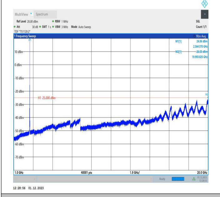
7-7-15MHz-5MHz-QPSK-QPSK-21327-21420-1RB#74-0RB#0 -1000~20000MHz-PASS
