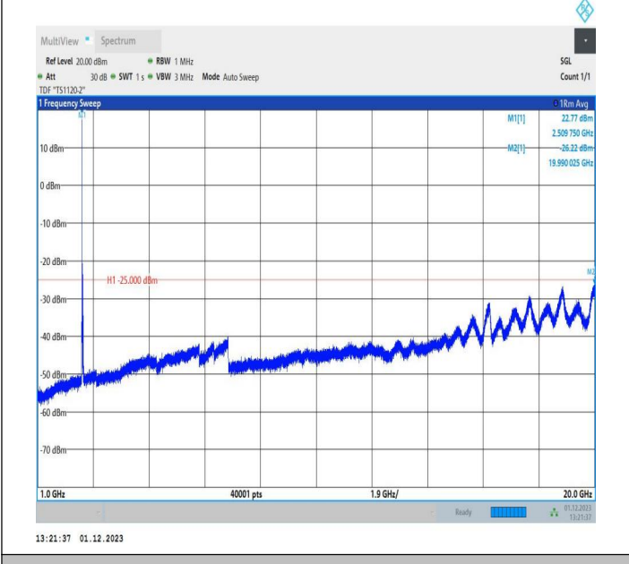
7-7-10MHz-20MHz-QPSK-QPSK-20805-20949-1RB#49-0RB# 0-1000~20000MHz-PASS
