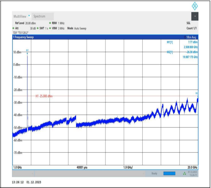
7-7-10MHz-20MHz-16QAM-16QAM-20805-20949-50RB#0-10 ORB#0-1000~20000MHz-PASS
