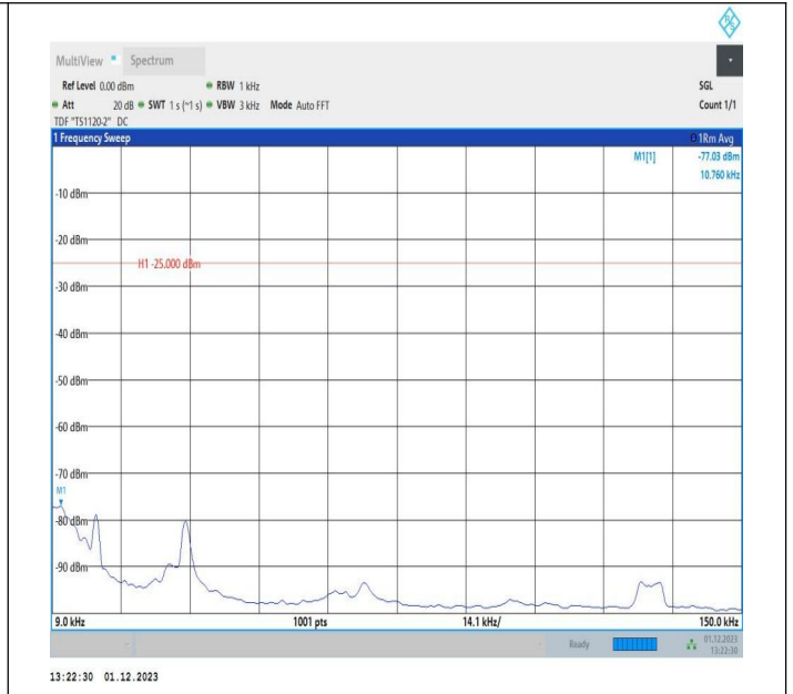
7-7-10MHz-20MHz-64QAM-64QAM-20805-20949-1RB#49-0R B#0-0.009~0.15MHz-PASS
