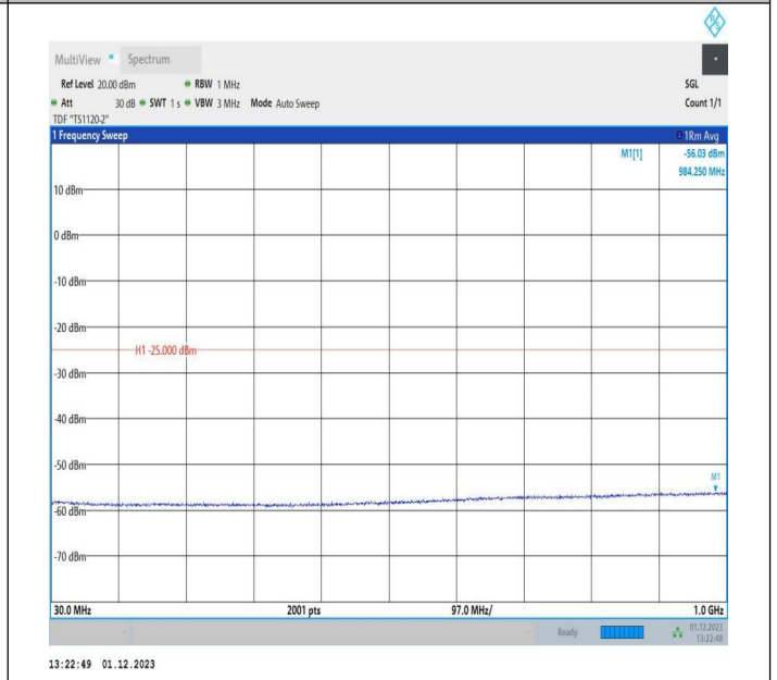
7-7-10MHz-20MHz-64QAM-64QAM-20805-20949-1RB#49-0R B#0-30~1000MHz-PASS
