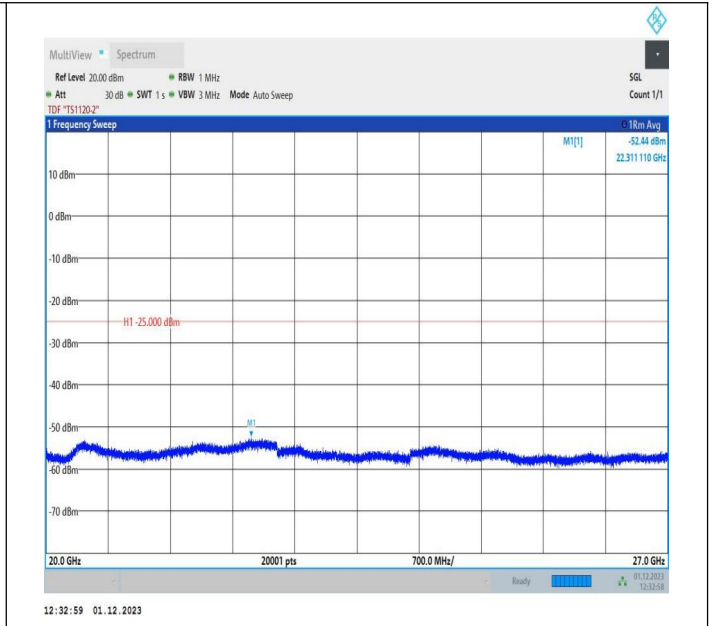
7-7-15MHz-5MHz-QPSK-QPSK-21327-21420-75RB#0-25RB# 0-20000~27000MHz-PASS
