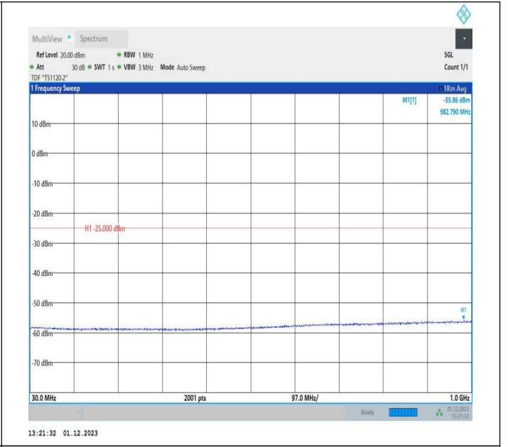
7-7-10MHz-20MHz-QPSK-QPSK-20805-20949-1RB#49-0RB# 0-30~1000MHz-PASS
