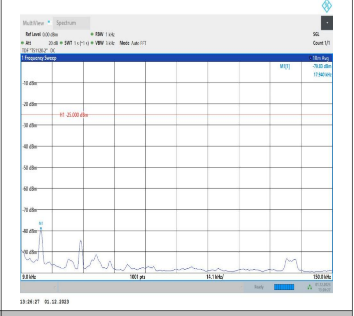
7-7-10MHz-20MHz-64QAM-64QAM-20805-20949-50RB#0-10 ORB#0-0.009~0.15MHz-PASS
