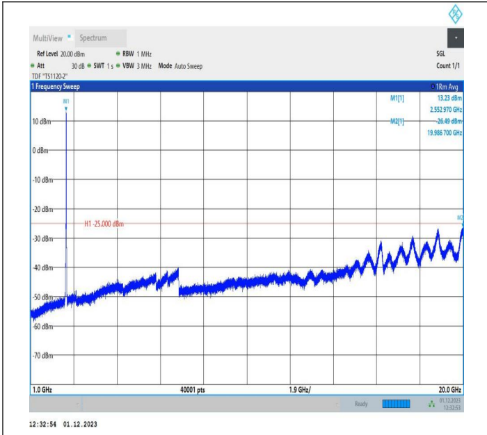
7-7-15MHz-5MHz-QPSK-QPSK-21327-21420-75RB#0-25RB# 0-1000~20000MHz-PASS
