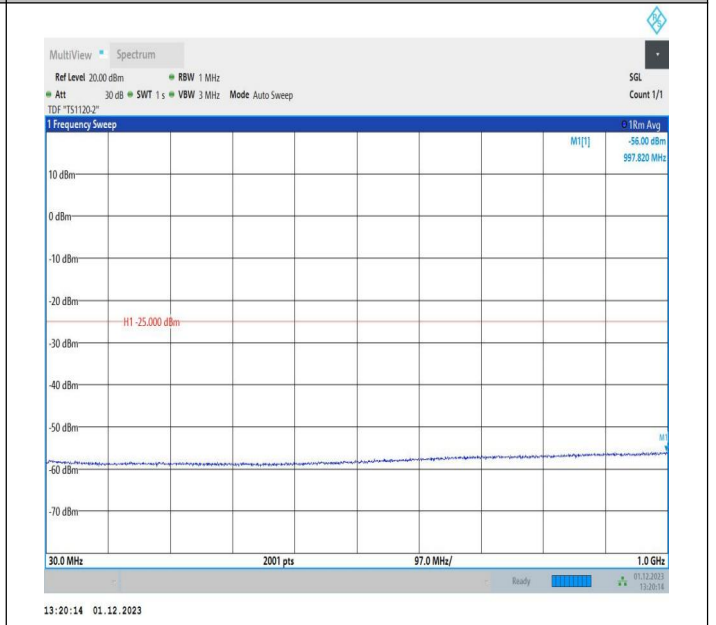
7-7-10MHz-20MHz-16QAM-16QAM-20805-20949-1RB#0-0RB #0-30~1000MHz-PASS
