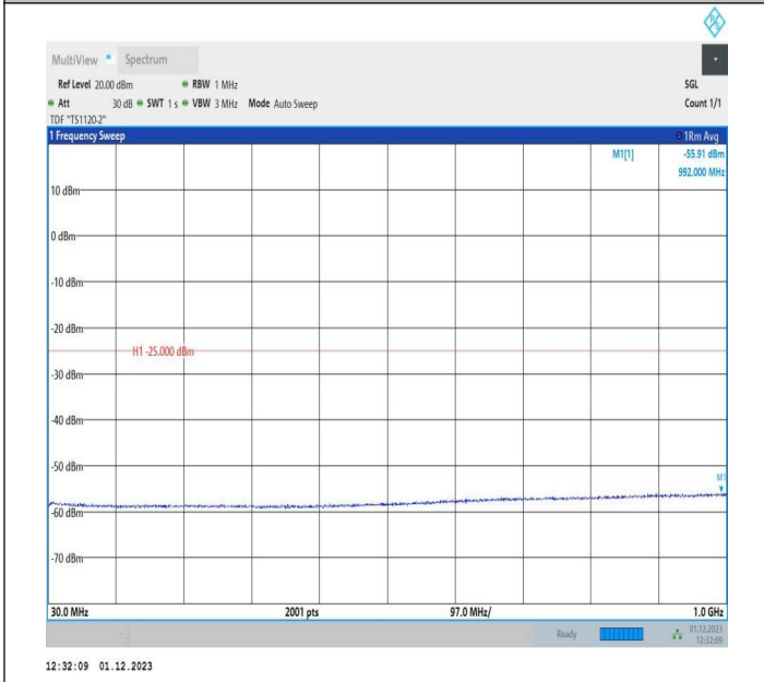
7-7-15MHz-5MHz-64QAM-64QAM-21327-21420-1RB#0-1RB# 24-30~1000MHz-PASS
