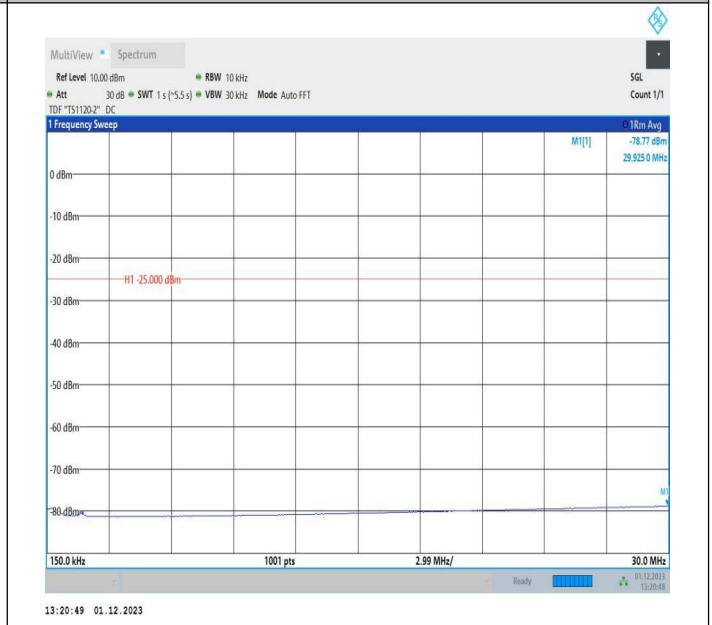
7-7-10MHz-20MHz-64QAM-64QAM-20805-20949-1RB#0-ORB #0-0.15~30MHz-PASS
