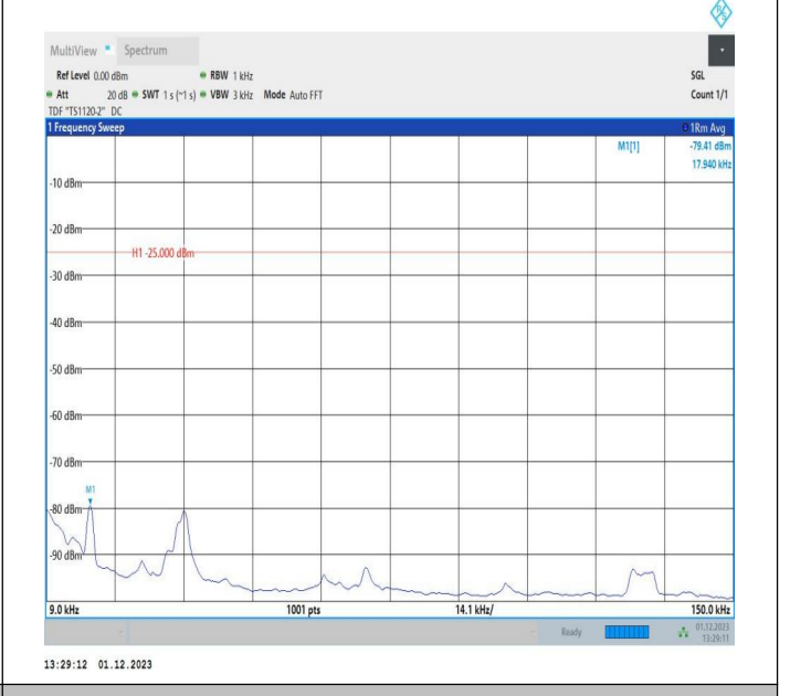
7-7-10MHz-20MHz-QPSK-QPSK-21006-21150-1RB#49-ORB# 0-0.009~0.15MHz-PASS
