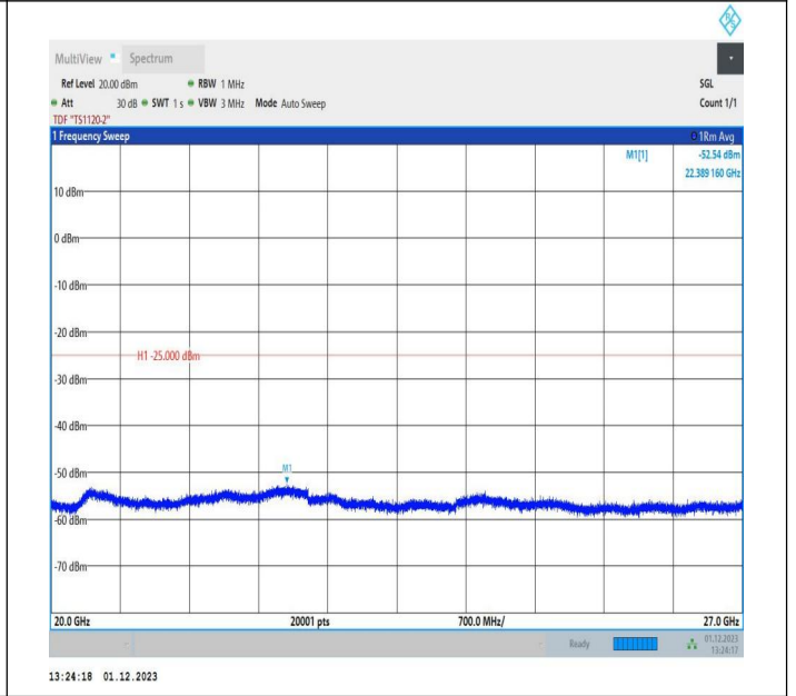
7-7-10MHz-20MHz-16QAM-16QAM-20805-20949-1RB#0-1RB #99-20000~27000MHz-PASS
