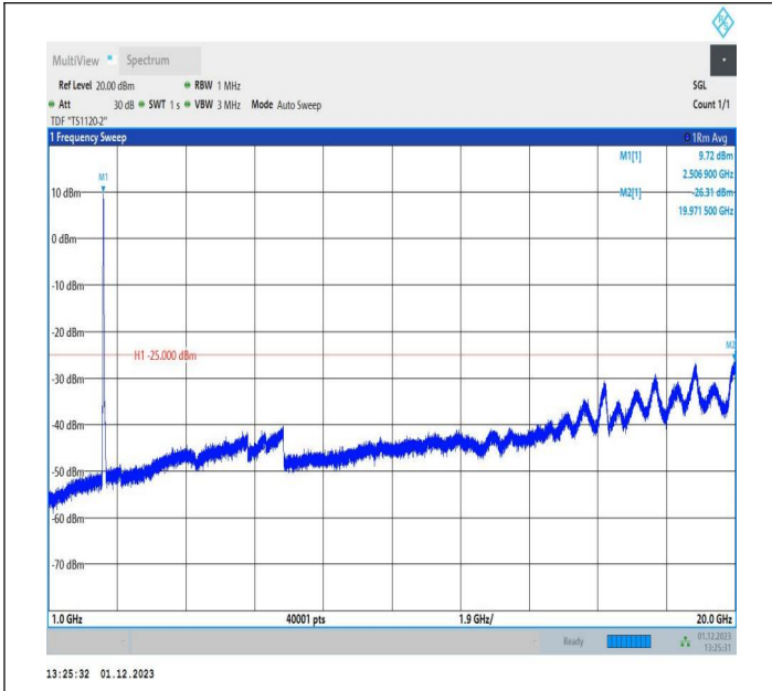
7-7-10MHz-20MHz-QPSK-QPSK-20805-20949-50RB#0-100R B#0-1000~20000MHz-PASS
