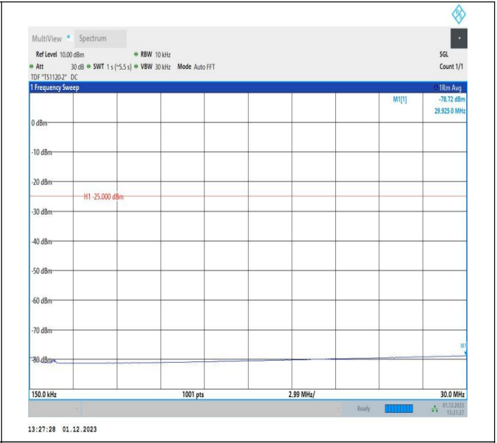
7-7-10MHz-20MHz-QPSK-QPSK-21006-21150-1RB#0-ORB#0-0.15~30MHz-PASS
