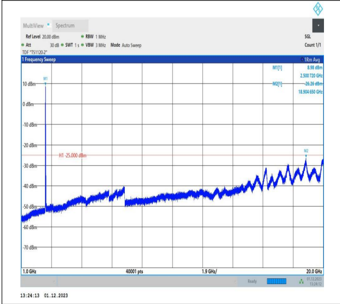
7-7-10MHz-20MHz-16QAM-16QAM-20805-20949-1RB#0-1RB #99-1000~20000MHz-PASS
