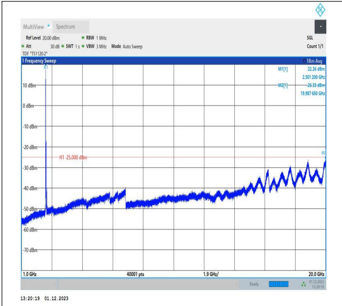
7-7-10MHz-20MHz-16QAM-16QAM-20805-20949-1RB#0-ORB #0-1000~20000MHz-PASS
