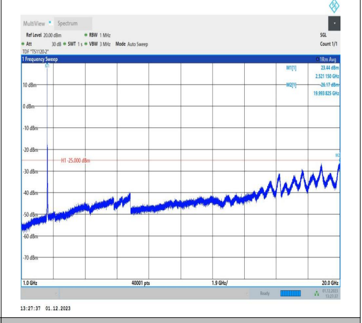
7-7-10MHz-20MHz-QPSK-QPSK-21006-21150-1RB#0-ORB#0-1000~20000MHz-PASS
