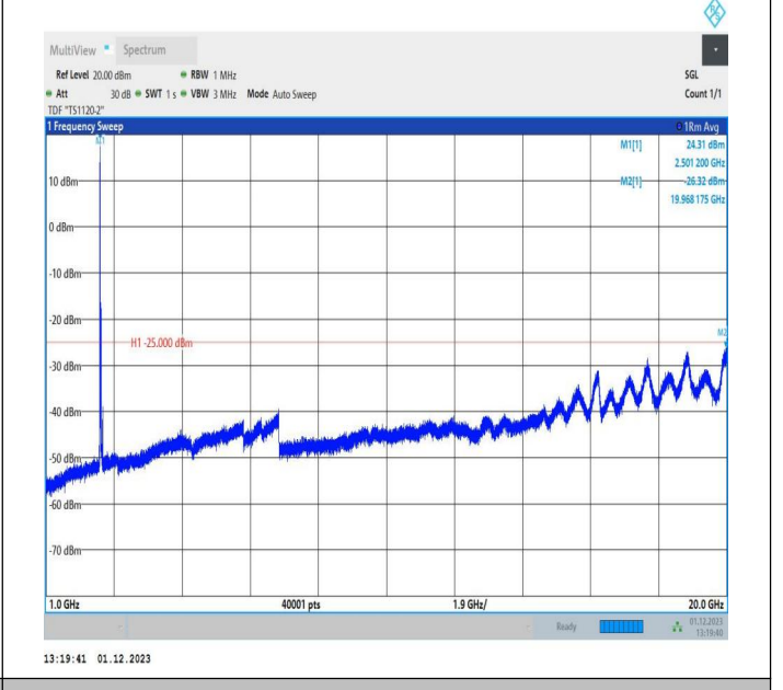
7-7-10MHz-20MHz-QPSK-QPSK-20805-20949-1RB#0-0RB#0 -1000~20000MHz-PASS
