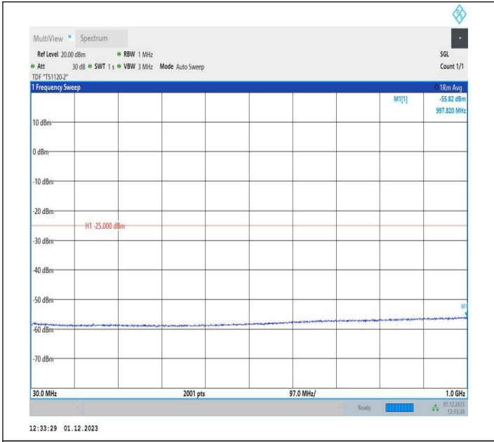
7-7-15MHz-5MHz-16QAM-16QAM-21327-21420-75RB#0-25R B#0-30~1000MHz-PASS
