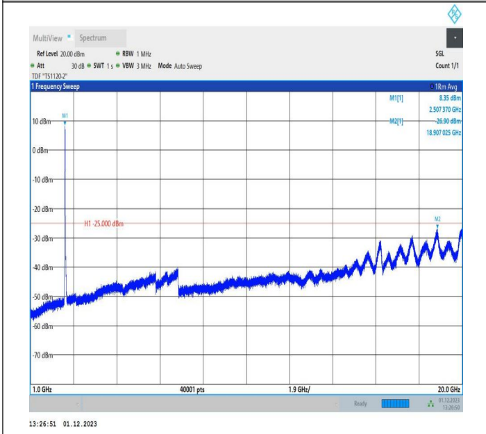
7-7-10MHz-20MHz-64QAM-64QAM-20805-20949-50RB#0-10 ORB#0-1000~20000MHz-PASS
