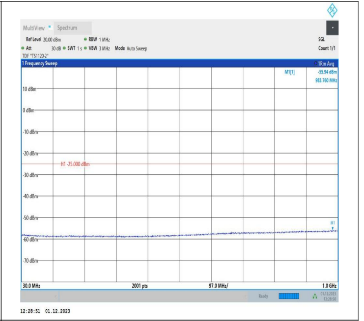
7-7-15MHz-5MHz-QPSK-QPSK-21327-21420-1RB#74-0RB#0 -30~1000MHz-PASS
