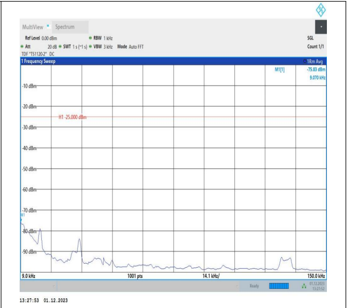
7-7-10MHz-20MHz-16QAM-16QAM-21006-21150-1RB#0-ORB#0-0.009~0.15MHz-PASS
