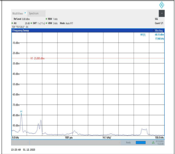
7-7-10MHz-20MHz-16QAM-16QAM-20805-20949-1RB#0-1RB #99-0.009~0.15MHz-PASS
