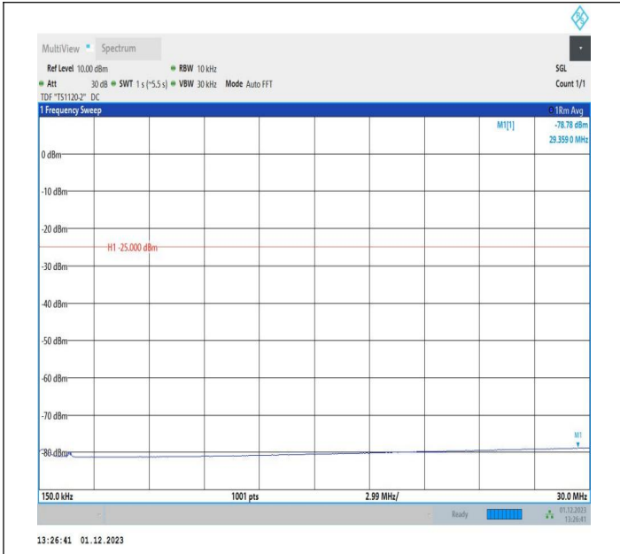
7-7-10MHz-20MHz-64QAM-64QAM-20805-20949-50RB#0-10 ORB#0-0.15~30MHz-PASS
