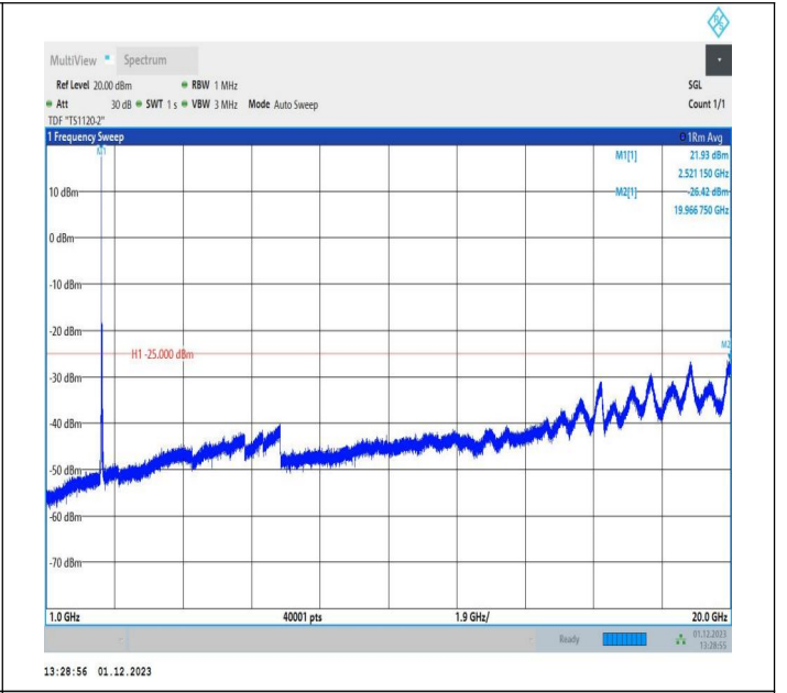
7-7-10MHz-20MHz-64QAM-64QAM-21006-21150-1RB#0-ORB #0-1000~20000MHz-PASS
