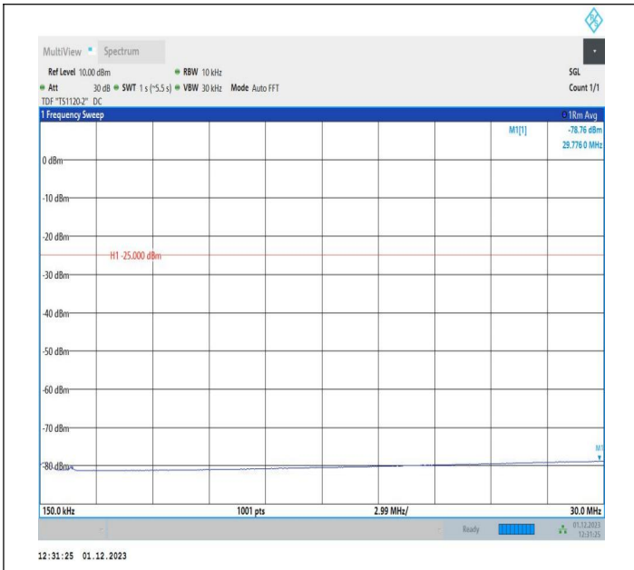
7-7-15MHz-5MHz-16QAM-16QAM-21327-21420-1RB#0-1RB# 24-0.15~30MHz-PASS
