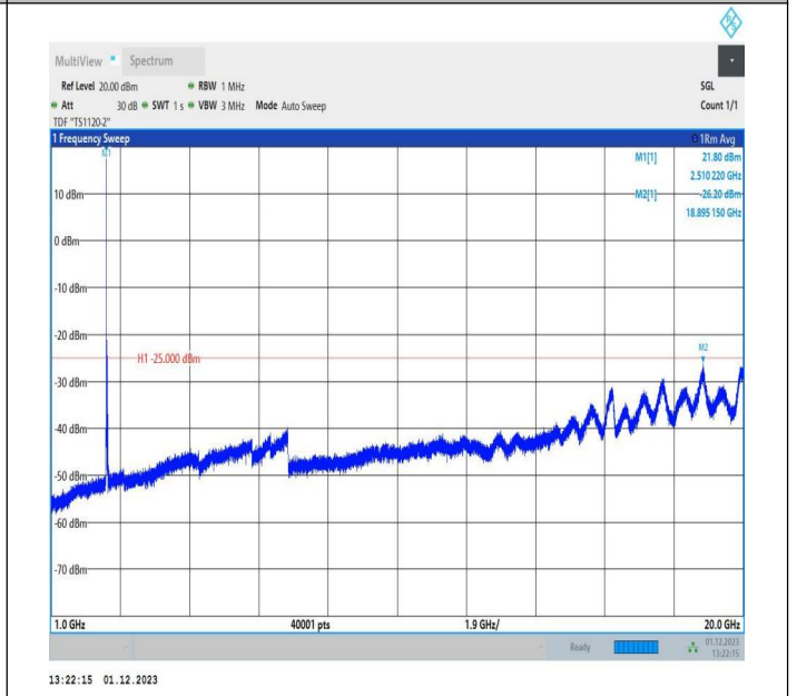
7-7-10MHz-20MHz-16QAM-16QAM-20805-20949-1RB#49-OR B#0-1000~20000MHz-PASS
