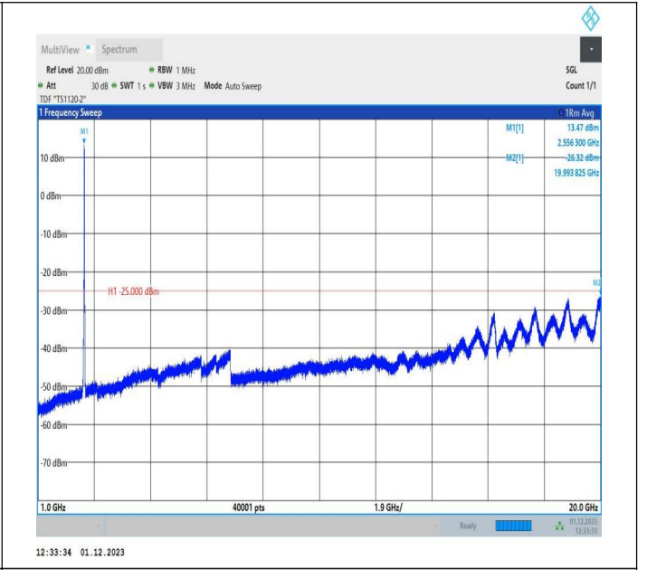
7-7-15MHz-5MHz-16QAM-16QAM-21327-21420-75RB#0-25R B#0-1000~20000MHz-PASS
