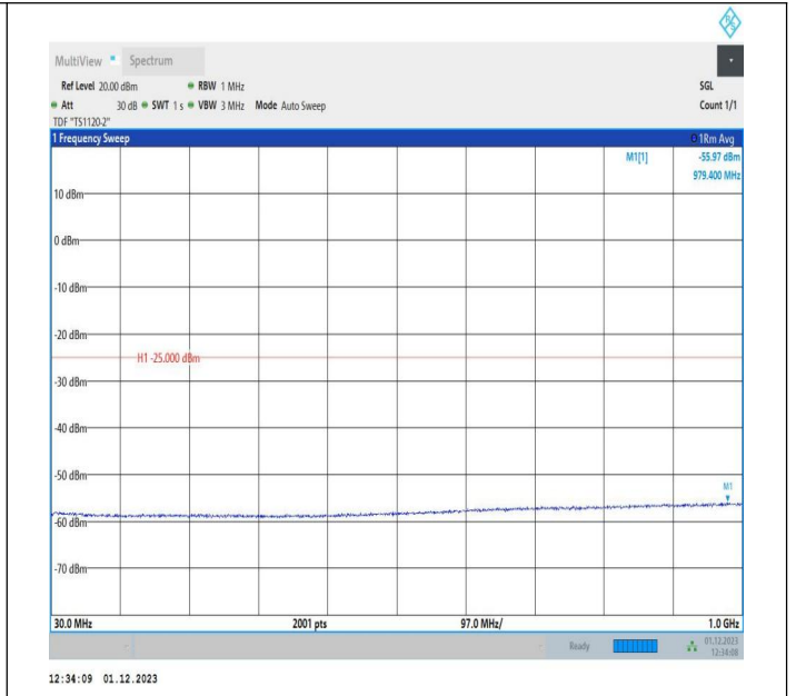
7-7-15MHz-5MHz-64QAM-64QAM-21327-21420-75RB#0-25R B#0-30~1000MHz-PASS
