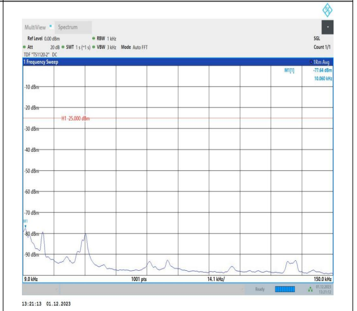
7-7-10MHz-20MHz-QPSK-QPSK-20805-20949-1RB#49-ORB# 0-0.009~0.15MHz-PASS
