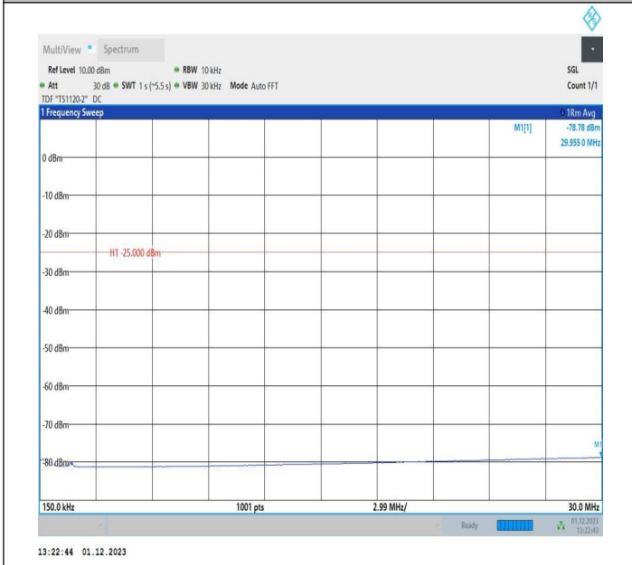
7-7-10MHz-20MHz-64QAM-64QAM-20805-20949-1RB#49-0R B#0-0.15~30MHz-PASS
