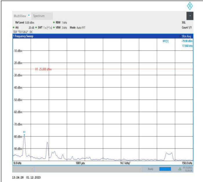
7-7-10MHz-20MHz-64QAM-64QAM-20805-20949-1RB#0-1RB #99-0.009~0.15MHz-PASS
