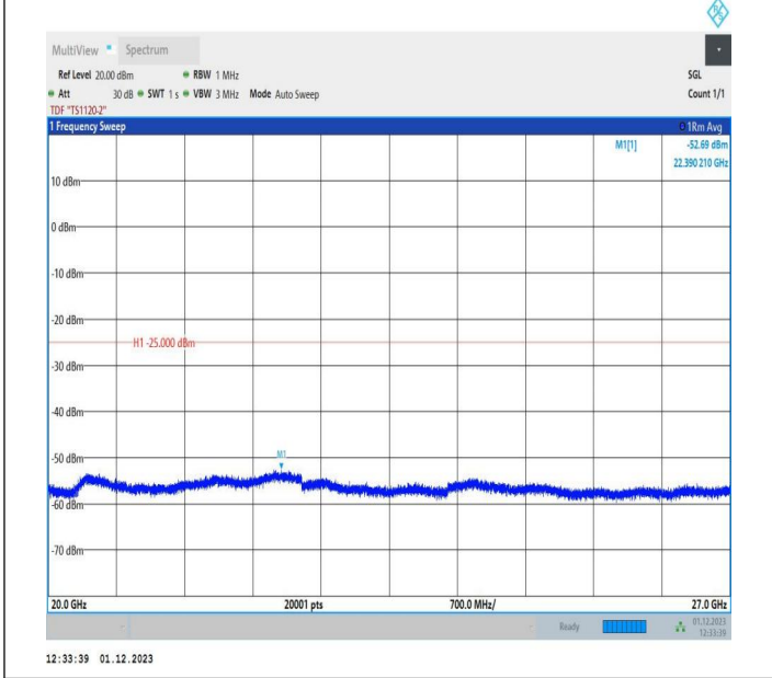
7-7-15MHz-5MHz-16QAM-16QAM-21327-21420-75RB#0-25R B#0-20000~27000MHz-PASS
