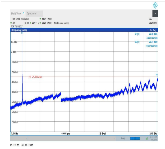
7-7-10MHz-20MHz-64QAM-64QAM-20805-20949-1RB#49-0R B#0-1000~20000MHz-PASS
