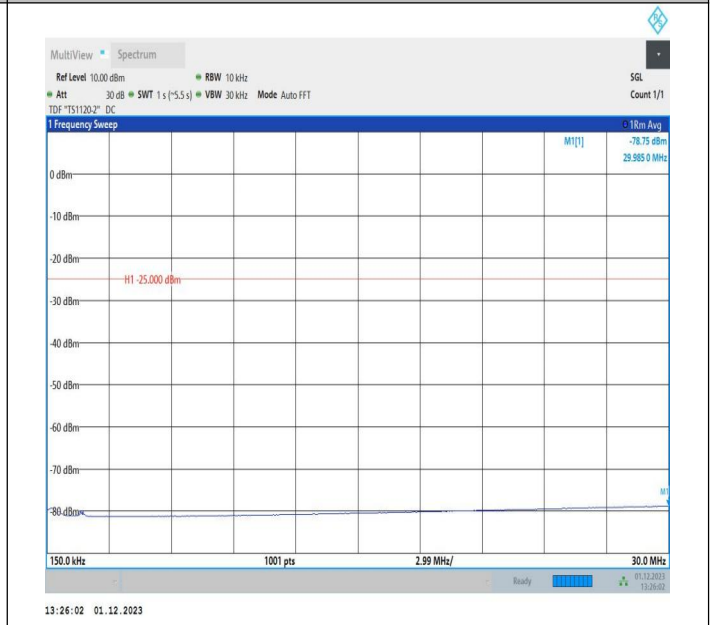
7-7-10MHz-20MHz-16QAM-16QAM-20805-20949-50RB#0-10 ORB#0-0.15~30MHz-PASS
