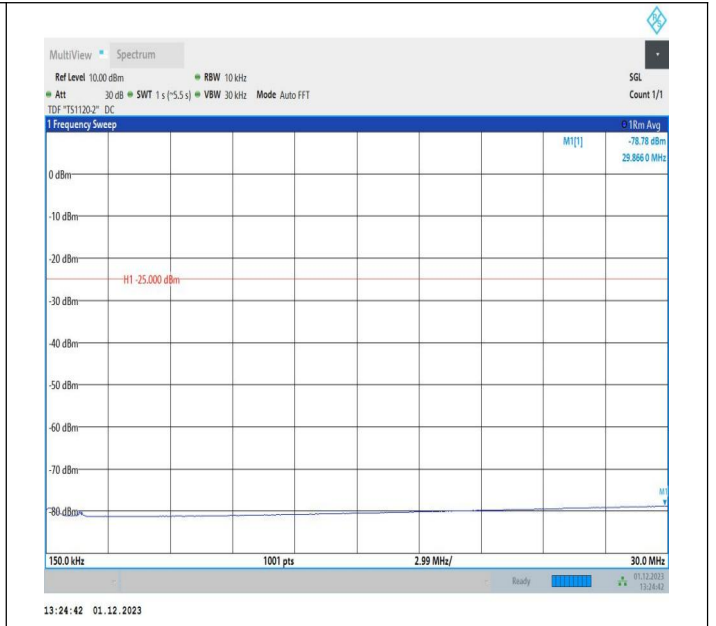
7-7-10MHz-20MHz-64QAM-64QAM-20805-20949-1RB#0-1RB #99-0.15~30MHz-PASS
