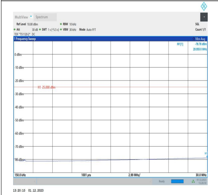
7-7-10MHz-20MHz-16QAM-16QAM-20805-20949-1RB#0-0RB #0-0.15~30MHz-PASS
