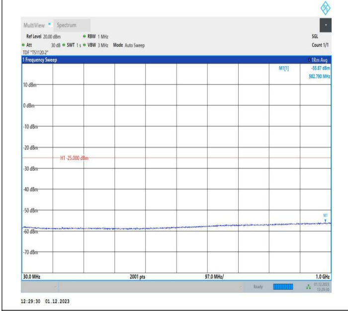
7-7-15MHz-5MHz-16QAM-16QAM-21327-21420-1RB#74-0RB #0-30~1000MHz-PASS
