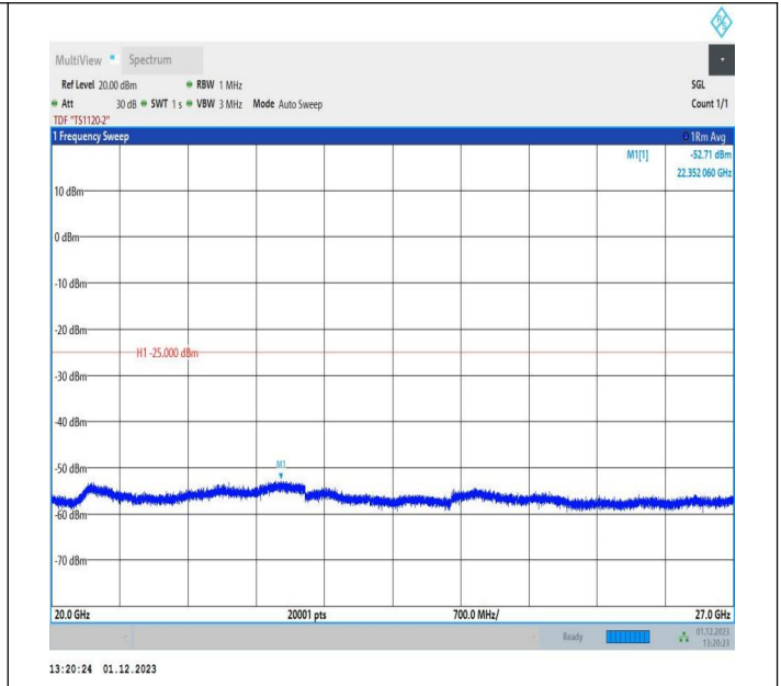
7-7-10MHz-20MHz-16QAM-16QAM-20805-20949-1RB#0-ORB #0-20000~27000MHz-PASS
