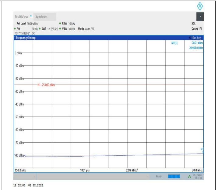
7-7-15MHz-5MHz-64QAM-64QAM-21327-21420-1RB#0-1RB# 24-0.15~30MHz-PASS
