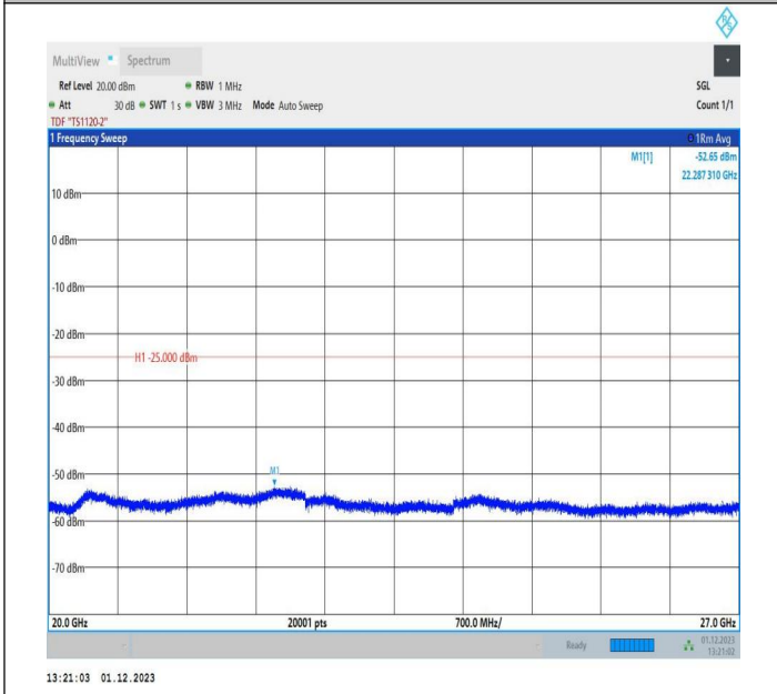
7-7-10MHz-20MHz-64QAM-64QAM-20805-20949-1RB#0-ORB #0-20000~27000MHz-PASS
