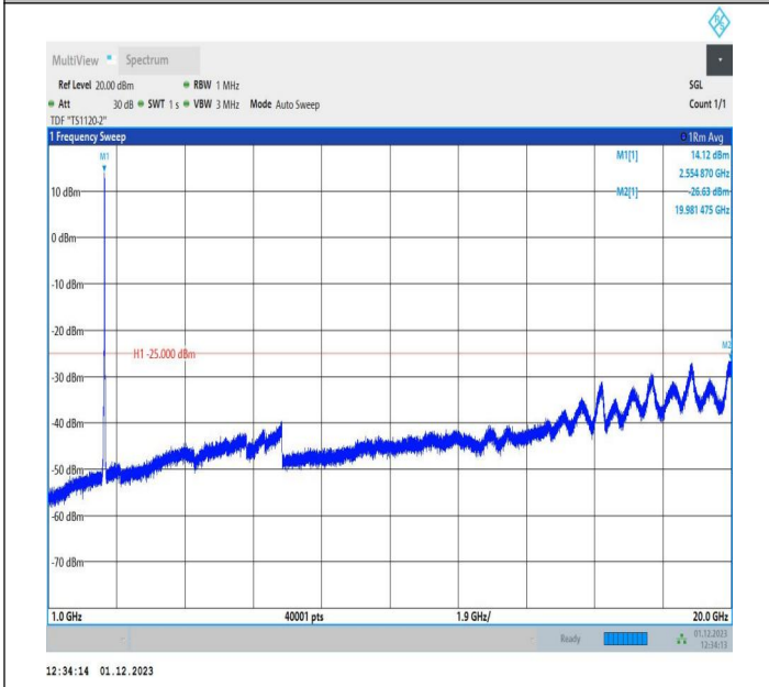
7-7-15MHz-5MHz-64QAM-64QAM-21327-21420-75RB#0-25R B#0-1000~20000MHz-PASS
