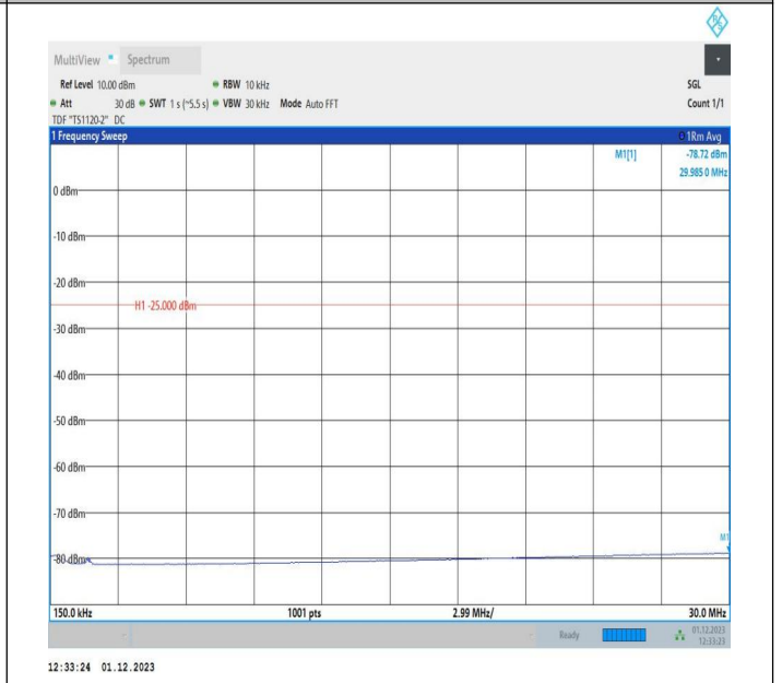
7-7-15MHz-5MHz-16QAM-16QAM-21327-21420-75RB#0-25R B#0-0.15~30MHz-PASS
