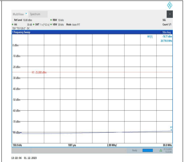
7-7-10MHz-20MHz-16QAM-16QAM-20805-20949-1RB#49-OR B#0-0.15~30MHz-PASS
