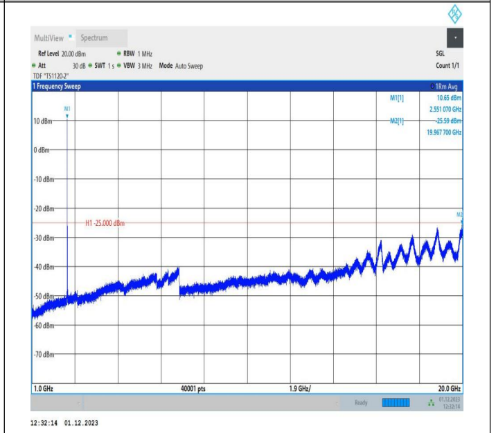
7-7-15MHz-5MHz-64QAM-64QAM-21327-21420-1RB#0-1RB# 24-1000~20000MHz-PASS
