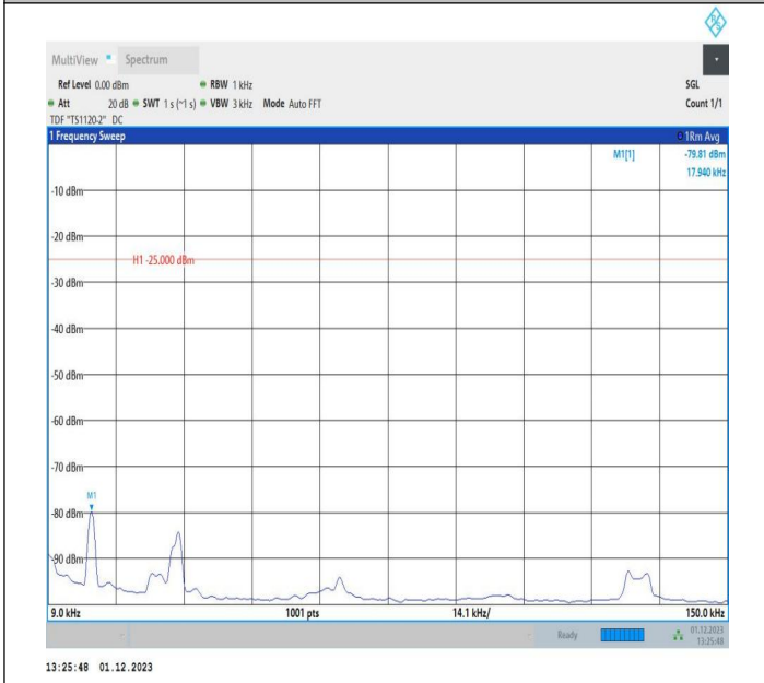
7-7-10MHz-20MHz-16QAM-16QAM-20805-20949-50RB#0-10 ORB#0-0.009~0.15MHz-PASS
