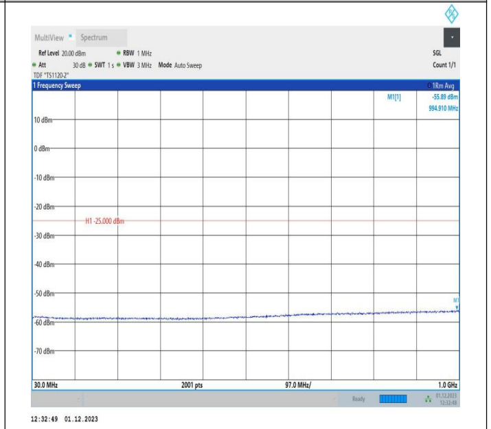
7-7-15MHz-5MHz-QPSK-QPSK-21327-21420-75RB#0-25RB# 0-30~1000MHz-PASS
