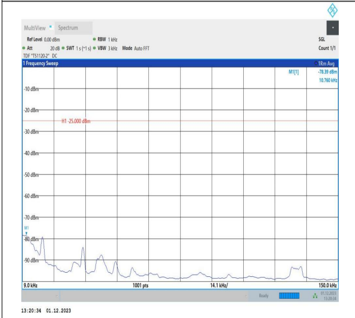
7-7-10MHz-20MHz-64QAM-64QAM-20805-20949-1RB#0-ORB #0-0.009~0.15MHz-PASS
