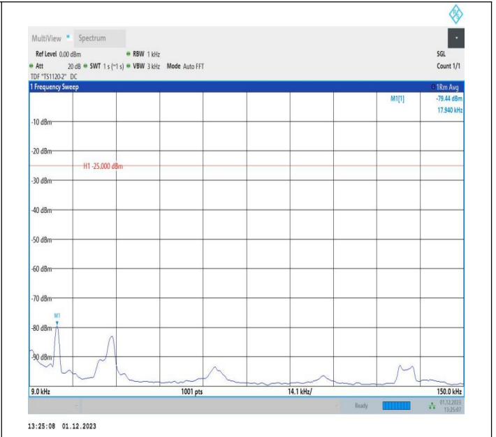
7-7-10MHz-20MHz-QPSK-QPSK-20805-20949-50RB#0-100R B#0-0.009~0.15MHz-PASS
