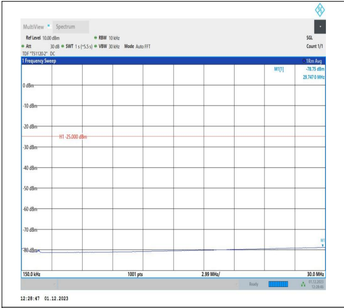
7-7-15MHz-5MHz-QPSK-QPSK-21327-21420-1RB#74-0RB#0 -0.15~30MHz-PASS
