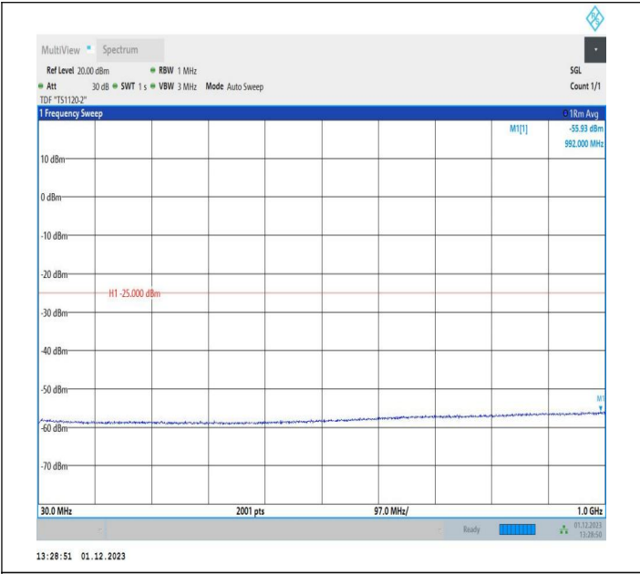
7-7-10MHz-20MHz-64QAM-64QAM-21006-21150-1RB#0-ORB #0-30~1000MHz-PASS
