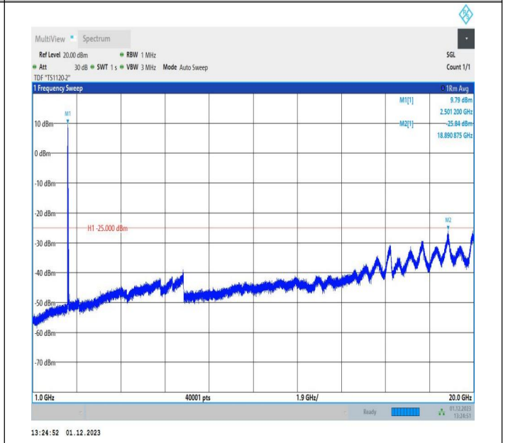
7-7-10MHz-20MHz-64QAM-64QAM-20805-20949-1RB#0-1RB #99-1000~20000MHz-PASS
