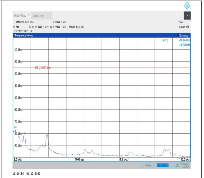
7-7-10MHz-20MHz-16QAM-16QAM-20805-20949-1RB#0-0RB #0-0.009~0.15MHz-PASS
