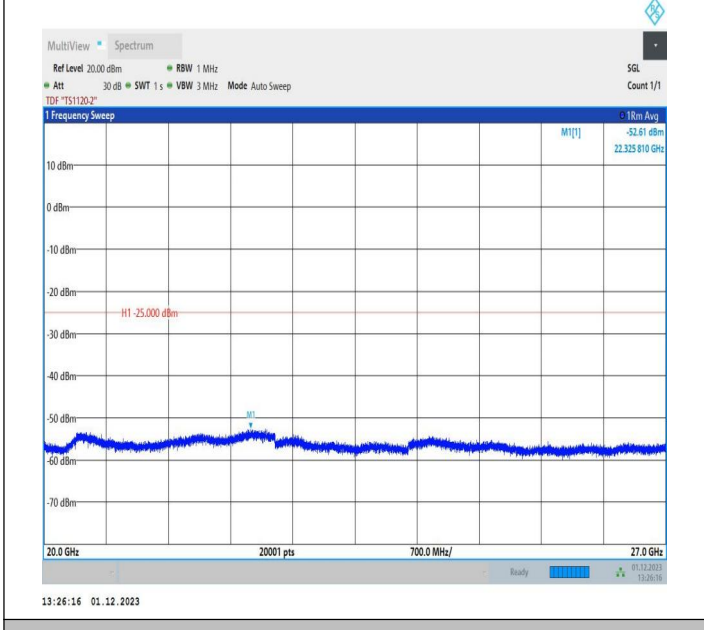
7-7-10MHz-20MHz-16QAM-16QAM-20805-20949-50RB#0-10 ORB#0-20000~27000MHz-PASS
