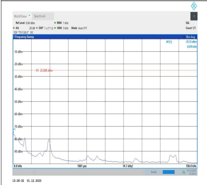
7-7-10MHz-20MHz-64QAM-64QAM-21006-21150-1RB#0-ORB #0-0.009~0.15MHz-PASS
