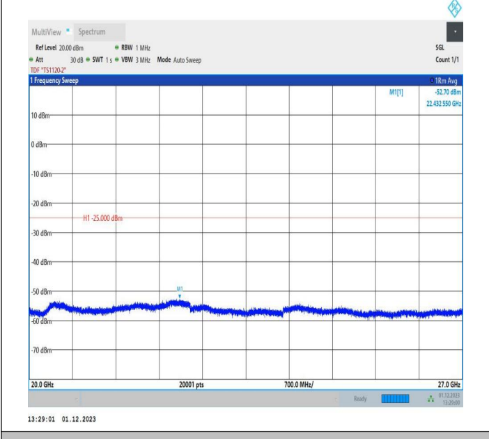
7-7-10MHz-20MHz-64QAM-64QAM-21006-21150-1RB#0-ORB #0-20000~27000MHz-PASS
