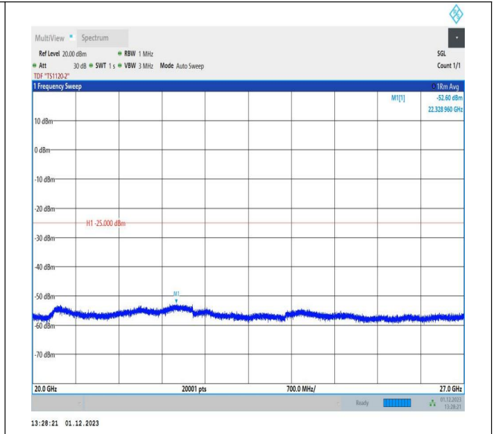
7-7-10MHz-20MHz-16QAM-16QAM-21006-21150-1RB#0-ORB #0-20000~27000MHz-PASS
