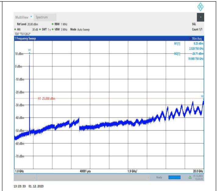
7-7-10MHz-20MHz-QPSK-QPSK-20805-20949-1RB#0-1RB#9 9-1000~20000MHz-PASS
