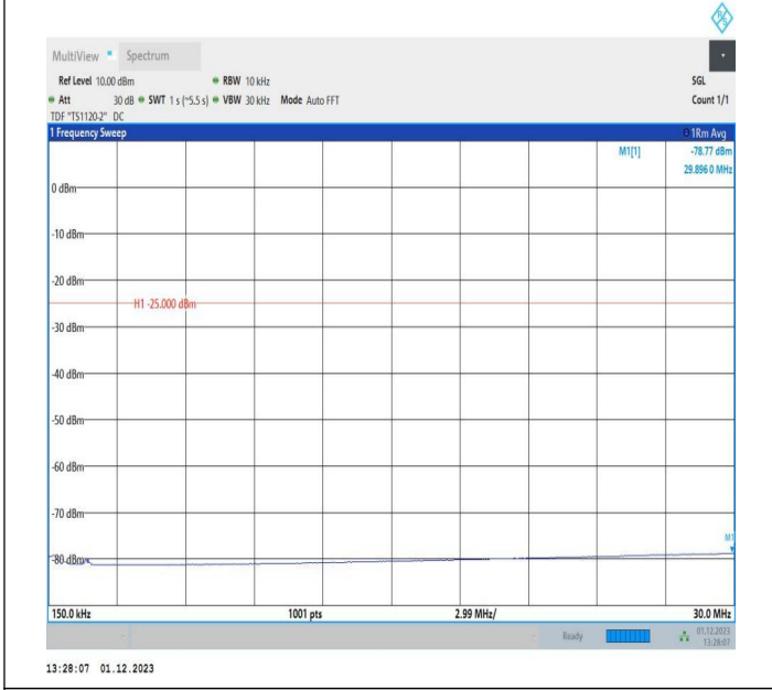
7-7-10MHz-20MHz-16QAM-16QAM-21006-21150-1RB#0-ORB#0-0.15~30MHz-PASS
