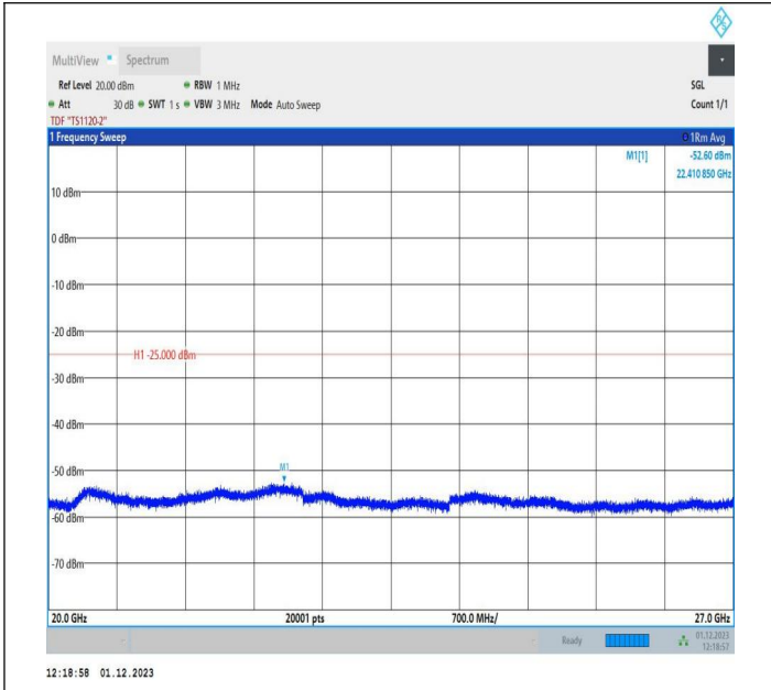
7-7-15MHz-5MHz-QPSK-QPSK-21076-21169-1RB#0-0RB#0-2 0000~27000MHz-PASS
