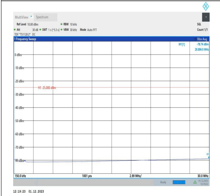
7-7-15MHz-5MHz-16QAM-16QAM-21076-21169-1RB#0-0RB# 0-0.15~30MHz-PASS
