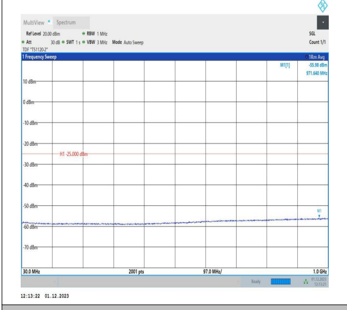
7-7-15MHz-5MHz-16QAM-16QAM-20825-20918-1RB#74-ORB #0-30~1000MHz-PASS
