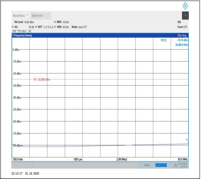
7-7-15MHz-5MHz-16QAM-16QAM-20825-20918-1RB#74-ORB #0-0.15~30MHz-PASS
