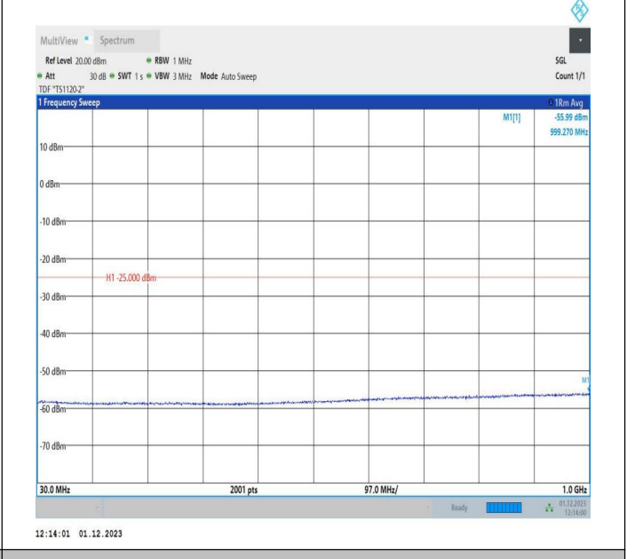
7-7-15MHz-5MHz-64QAM-64QAM-20825-20918-1RB#74-ORB #0-30~1000MHz-PASS
