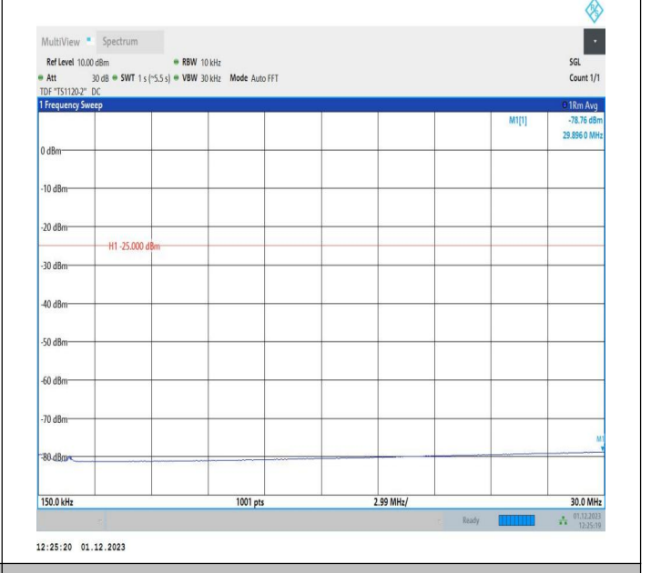
7-7-15MHz-5MHz-16QAM-16QAM-21076-21169-75RB#0-25R B#0-0.15~30MHz-PASS
