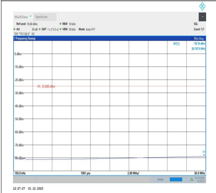
7-7-15MHz-5MHz-16QAM-16QAM-21327-21420-1RB#0-0RB#0-0-0.15~30MHz-PASS
