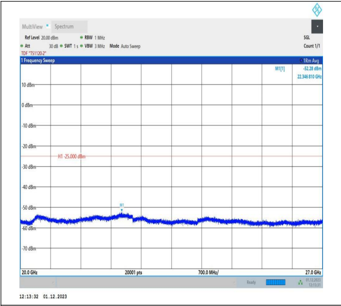
7-7-15MHz-5MHz-16QAM-16QAM-20825-20918-1RB#74-ORB #0-20000~27000MHz-PASS
