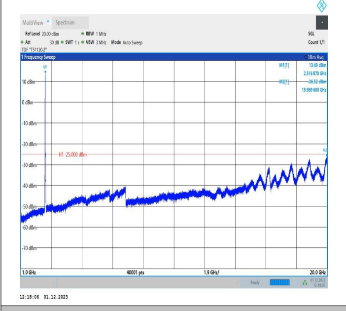
7-7-15MHz-5MHz-64QAM-64QAM-20825-20918-75RB#0-25R B#0-1000~20000MHz-PASS
