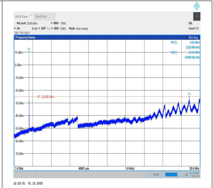
7-7-15MHz-5MHz-QPSK-QPSK-21076-21169-1RB#0-1RB#24-1000~20000MHz-PASS
