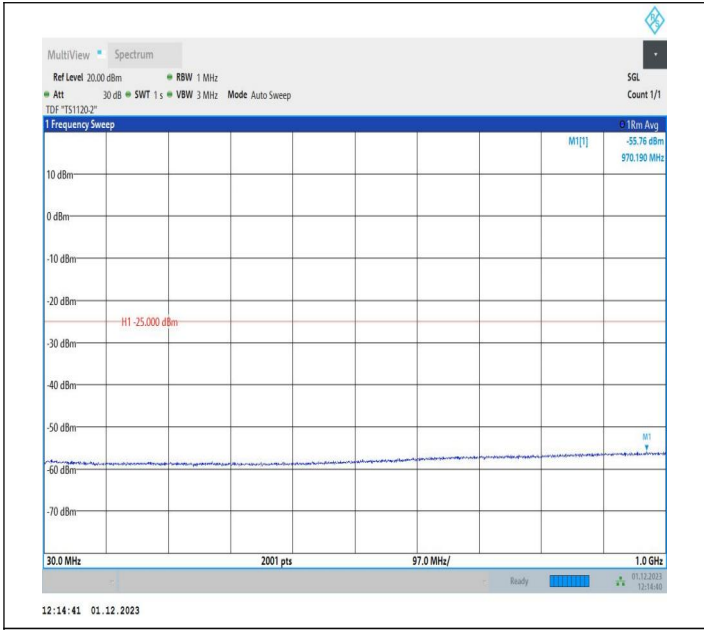
7-7-15MHz-5MHz-QPSK-QPSK-20825-20918-1RB#0-1RB#24 -30~1000MHz-PASS
