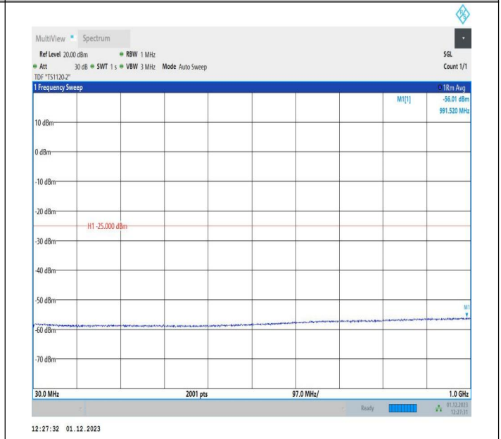
7-7-15MHz-5MHz-16QAM-16QAM-21327-21420-1RB#0-0RB#0-0-30~1000MHz-PASS
