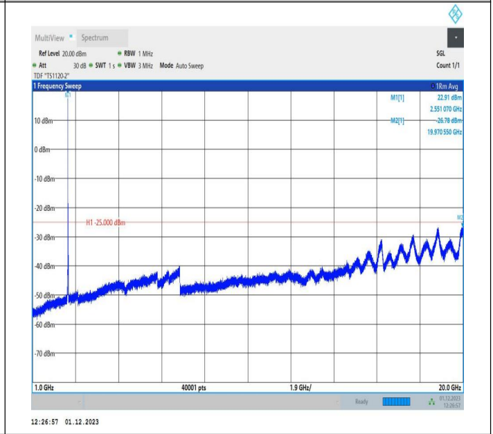
7-7-15MHz-5MHz-QPSK-QPSK-21327-21420-1RB#0-0RB#0-1000~20000MHz-PASS
