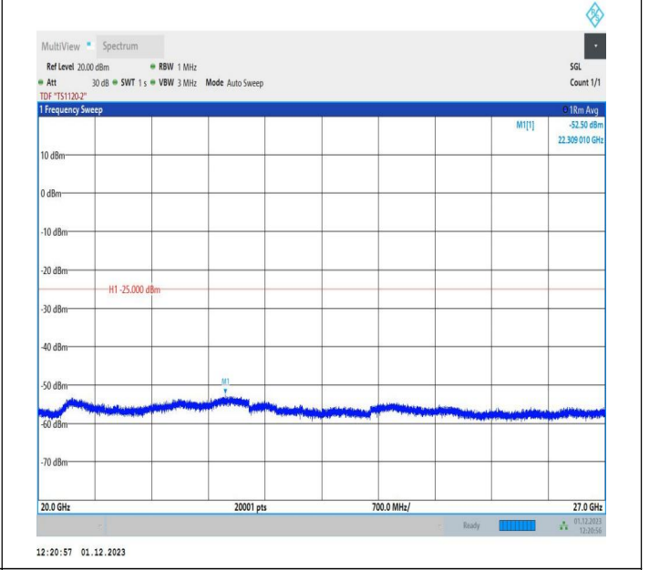
7-7-15MHz-5MHz-QPSK-QPSK-21076-21169-1RB#74-ORB#0-20000~27000MHz-PASS
