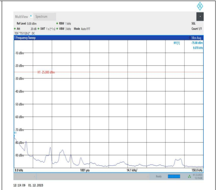
7-7-15MHz-5MHz-16QAM-16QAM-21076-21169-1RB#0-0RB# 0-0.009~0.15MHz-PASS
