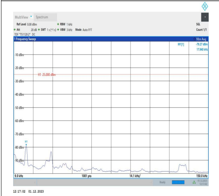
7-7-15MHz-5MHz-16QAM-16QAM-20825-20918-75RB#0-25R B#0-0.009~0.15MHz-PASS
