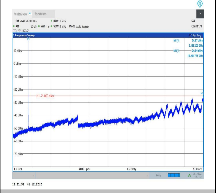
7-7-15MHz-5MHz-16QAM-16QAM-21076-21169-1RB#74-ORB #0-1000~20000MHz-PASS
