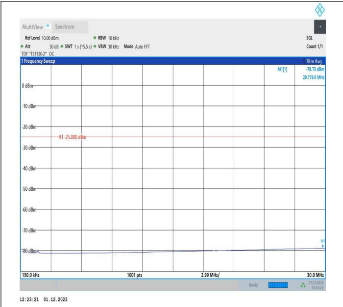
7-7-15MHz-5MHz-16QAM-16QAM-21076-21169-1RB#0-1RB# 24-0.15~30MHz-PASS
