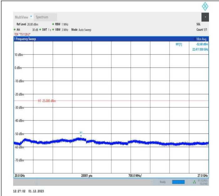
7-7-15MHz-5MHz-QPSK-QPSK-21327-21420-1RB#0-0RB#0-20000~27000MHz-PASS
