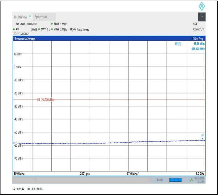
7-7-15MHz-5MHz-QPSK-QPSK-20825-20918-1RB#74-0RB#0 -30~1000MHz-PASS
