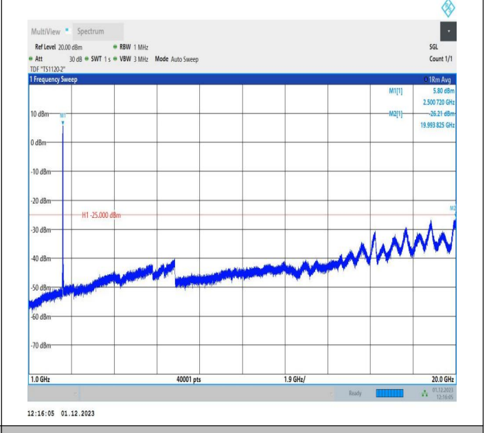
7-7-15MHz-5MHz-64QAM-64QAM-20825-20918-1RB#0-1RB# 24-1000~20000MHz-PASS
