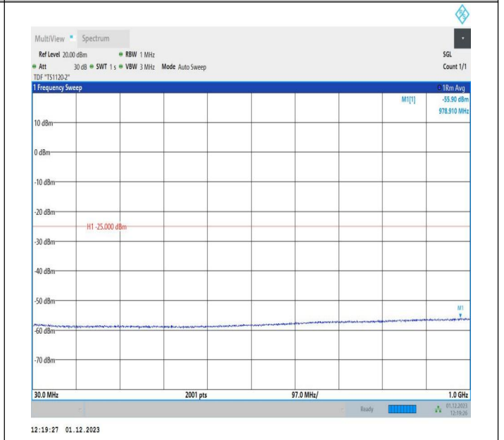
7-7-15MHz-5MHz-16QAM-16QAM-21076-21169-1RB#0-0RB# 0-30~1000MHz-PASS
