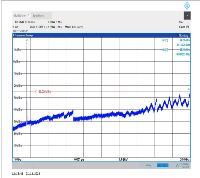
7-7-15MHz-5MHz-QPSK-QPSK-20825-20918-75RB#0-25RB# 0-1000~20000MHz-PASS
