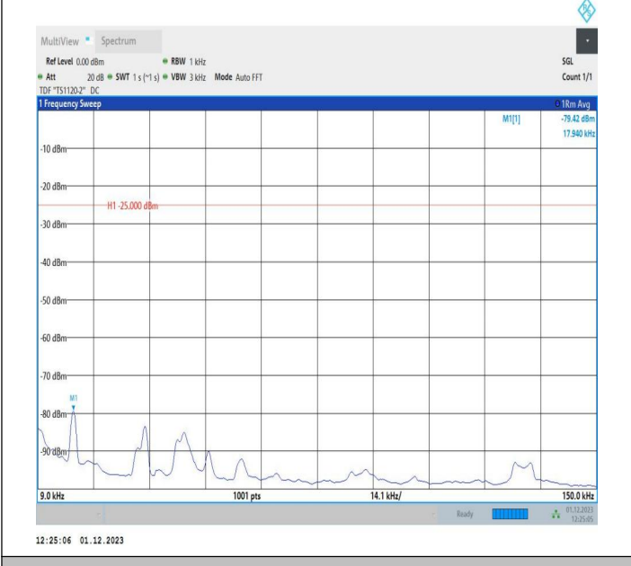
7-7-15MHz-5MHz-16QAM-16QAM-21076-21169-75RB#0-25R B#0-0.009~0.15MHz-PASS
