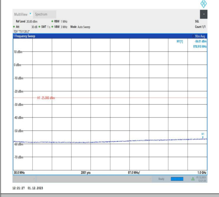
7-7-15MHz-5MHz-16QAM-16QAM-21076-21169-1RB#74-ORB #0-30~1000MHz-PASS
