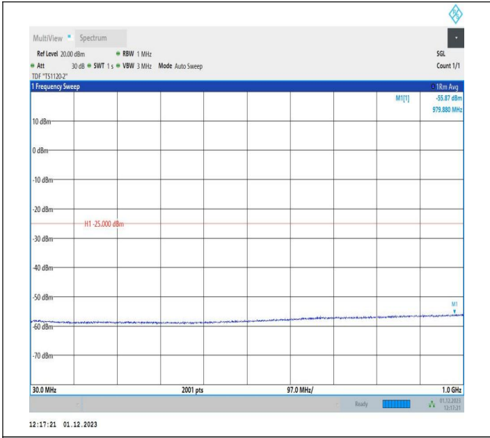
7-7-15MHz-5MHz-16QAM-16QAM-20825-20918-75RB#0-25R B#0-30~1000MHz-PASS
