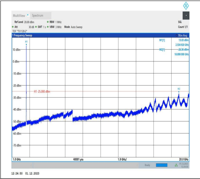
7-7-15MHz-5MHz-QPSK-QPSK-21076-21169-75RB#0-25RB# 0-1000~20000MHz-PASS
