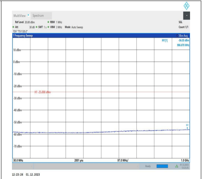
7-7-15MHz-5MHz-16QAM-16QAM-21076-21169-1RB#0-1RB# 24-30~1000MHz-PASS
