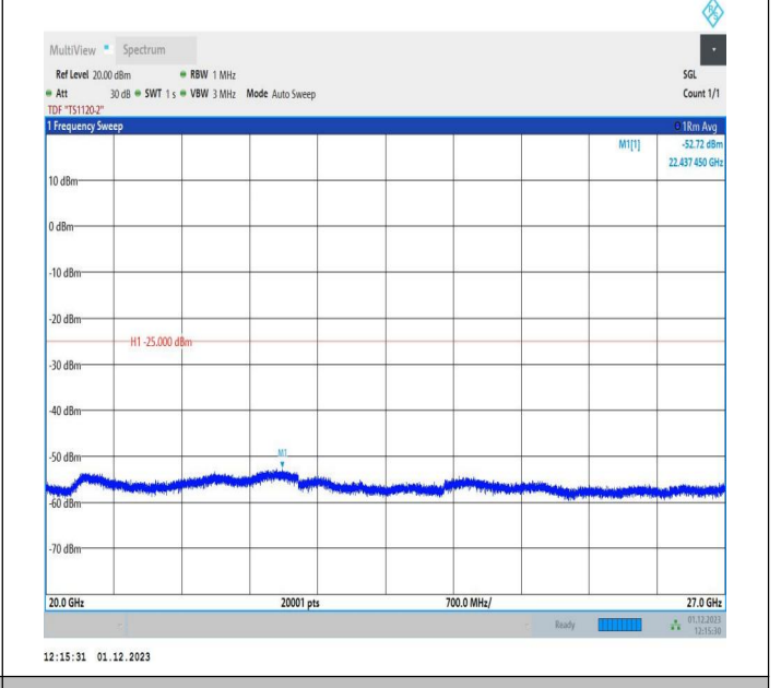
7-7-15MHz-5MHz-16QAM-16QAM-20825-20918-1RB#0-1RB# 24-20000~27000MHz-PASS
