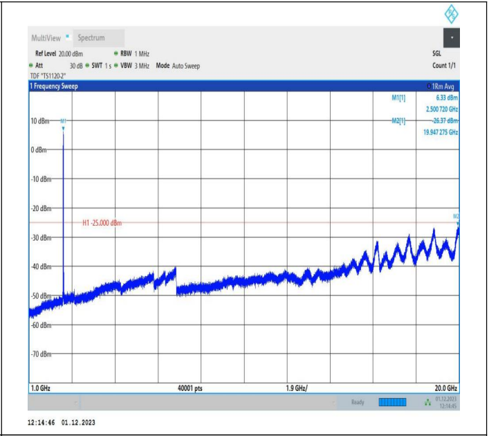
7-7-15MHz-5MHz-QPSK-QPSK-20825-20918-1RB#0-1RB#24 -1000~20000MHz-PASS
