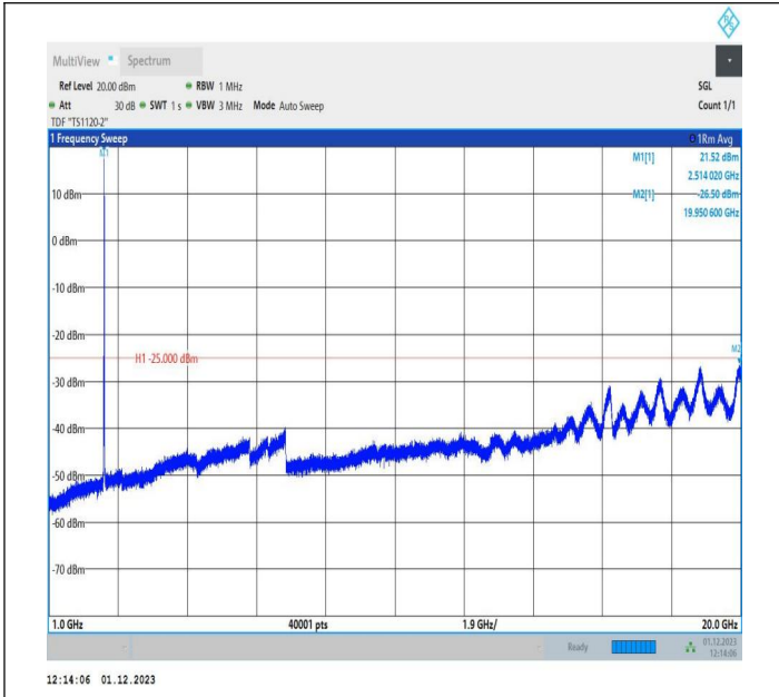
7-7-15MHz-5MHz-64QAM-64QAM-20825-20918-1RB#74-0RB #0-1000~20000MHz-PASS
