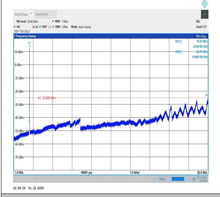
7-7-15MHz-5MHz-64QAM-64QAM-21076-21169-75RB#0-25R B#0-1000~20000MHz-PASS
