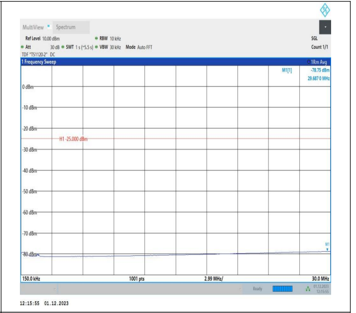
7-7-15MHz-5MHz-64QAM-64QAM-20825-20918-1RB#0-1RB# 24-0.15~30MHz-PASS
