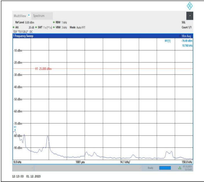
7-7-15MHz-5MHz-16QAM-16QAM-20825-20918-1RB#74-ORB #0-0.009~0.15MHz-PASS
