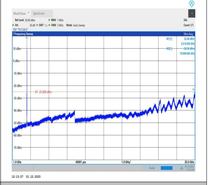
7-7-15MHz-5MHz-16QAM-16QAM-20825-20918-1RB#74-ORB #0-1000~20000MHz-PASS
