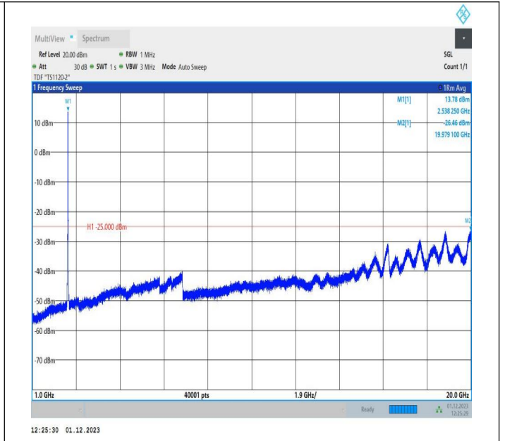
7-7-15MHz-5MHz-16QAM-16QAM-21076-21169-75RB#0-25R B#0-1000~20000MHz-PASS
