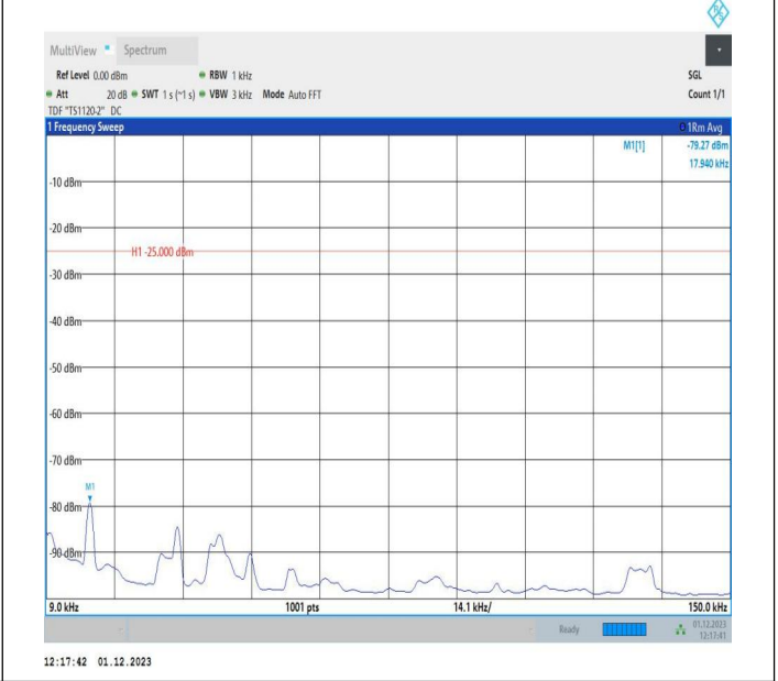
7-7-15MHz-5MHz-64QAM-64QAM-20825-20918-75RB#0-25R B#0-0.009~0.15MHz-PASS
