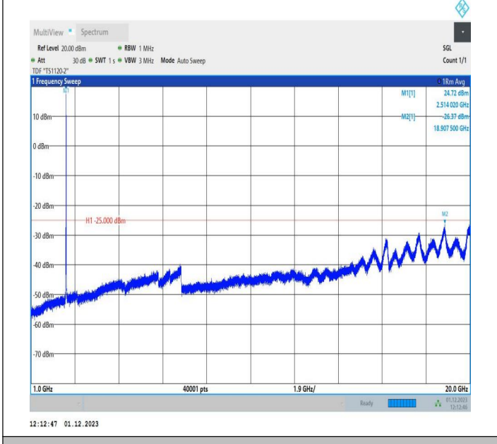
7-7-15MHz-5MHz-QPSK-QPSK-20825-20918-1RB#74-0RB#0 -1000~20000MHz-PASS
