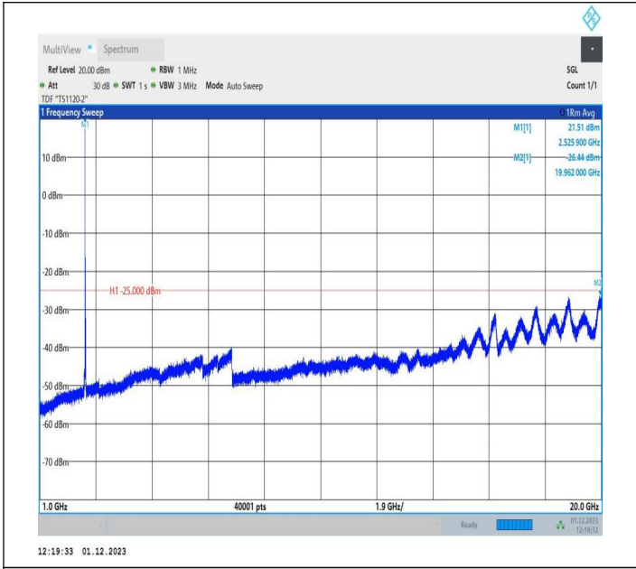
7-7-15MHz-5MHz-16QAM-16QAM-21076-21169-1RB#0-0RB# 0-1000~20000MHz-PASS
