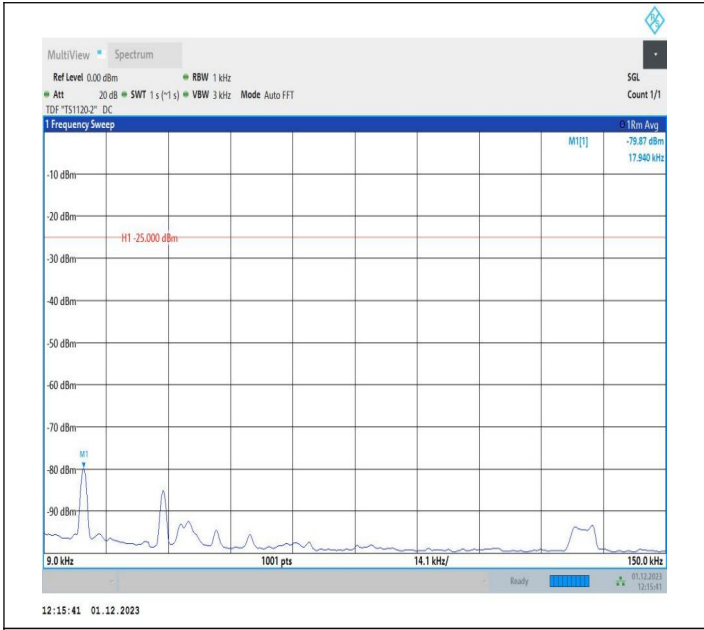
7-7-15MHz-5MHz-64QAM-64QAM-20825-20918-1RB#0-1RB# 24-0.009~0.15MHz-PASS
