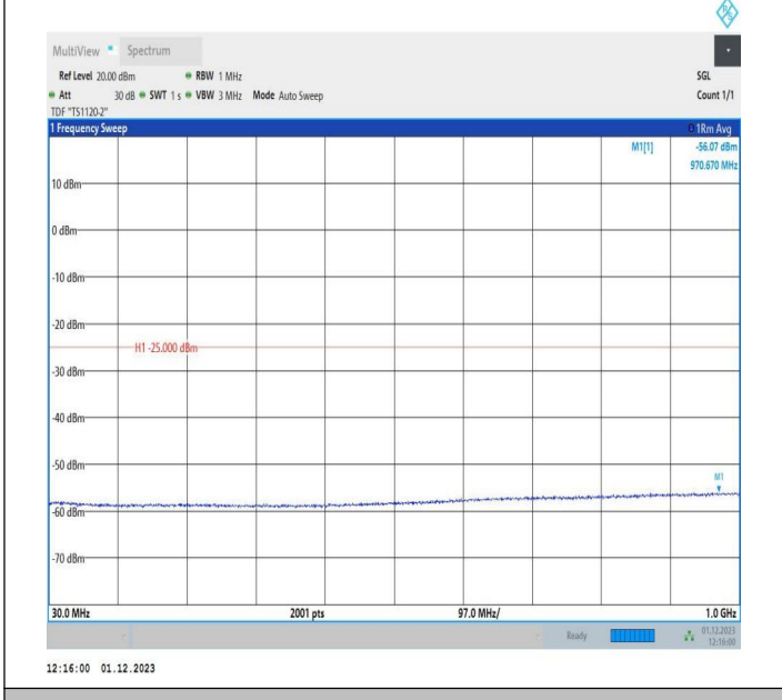
7-7-15MHz-5MHz-64QAM-64QAM-20825-20918-1RB#0-1RB# 24-30~1000MHz-PASS
