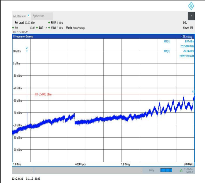
7-7-15MHz-5MHz-16QAM-16QAM-21076-21169-1RB#0-1RB# 24-1000~20000MHz-PASS
