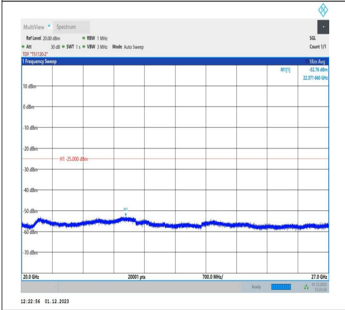
7-7-15MHz-5MHz-QPSK-QPSK-21076-21169-1RB#0-1RB#24-20000~27000MHz-PASS
