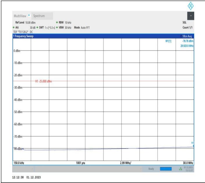
7-7-15MHz-5MHz-QPSK-QPSK-20825-20918-1RB#74-0RB#0 -0.15~30MHz-PASS
