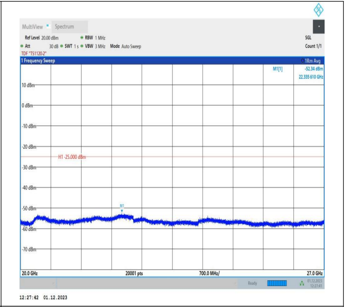
7-7-15MHz-5MHz-16QAM-16QAM-21327-21420-1RB#0-0RB# 0-20000~27000MHz-PASS
