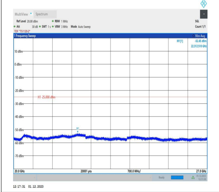
7-7-15MHz-5MHz-16QAM-16QAM-20825-20918-75RB#0-25R B#0-20000~27000MHz-PASS
