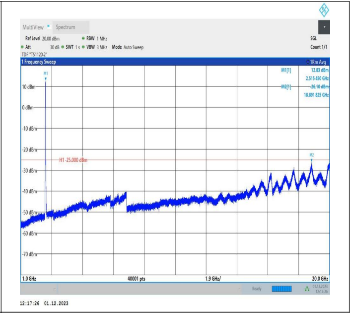
7-7-15MHz-5MHz-16QAM-16QAM-20825-20918-75RB#0-25R B#0-1000~20000MHz-PASS
