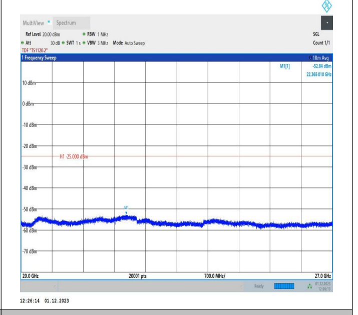
7-7-15MHz-5MHz-64QAM-64QAM-21076-21169-75RB#0-25R B#0-20000~27000MHz-PASS
