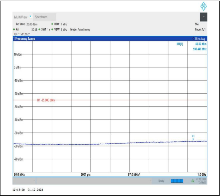
7-7-15MHz-5MHz-64QAM-64QAM-20825-20918-75RB#0-25R B#0-30~1000MHz-PASS
