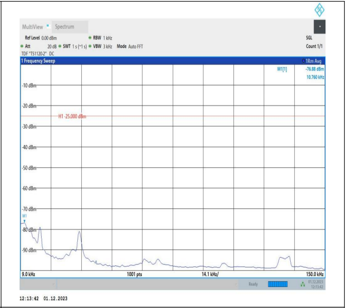
7-7-15MHz-5MHz-64QAM-64QAM-20825-20918-1RB#74-ORB #0-0.009~0.15MHz-PASS
