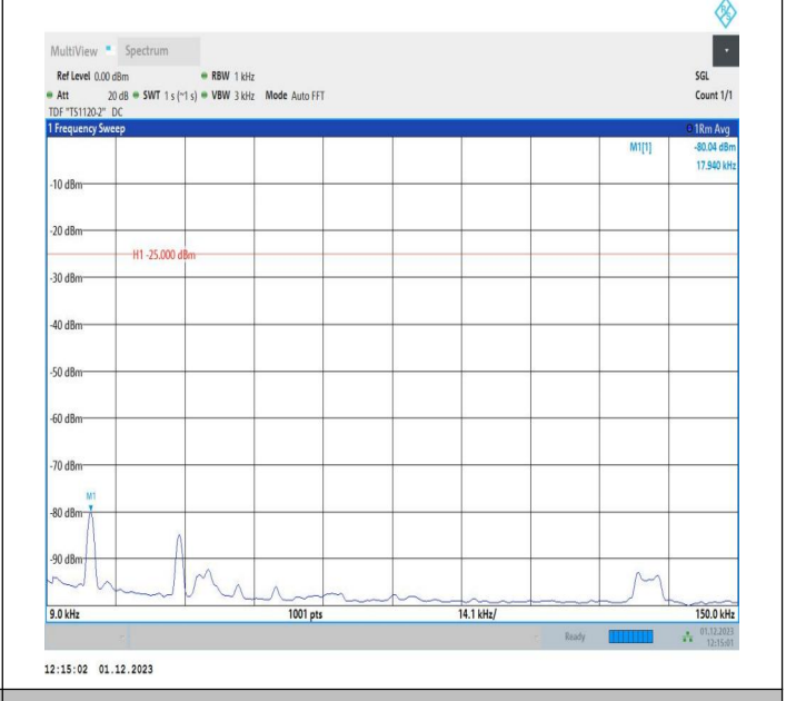
7-7-15MHz-5MHz-16QAM-16QAM-20825-20918-1RB#0-1RB# 24-0.009~0.15MHz-PASS
