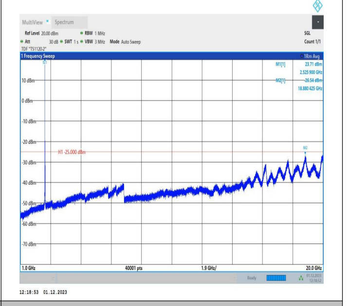
7-7-15MHz-5MHz-QPSK-QPSK-21076-21169-1RB#0-0RB#0-1 000~20000MHz-PASS
