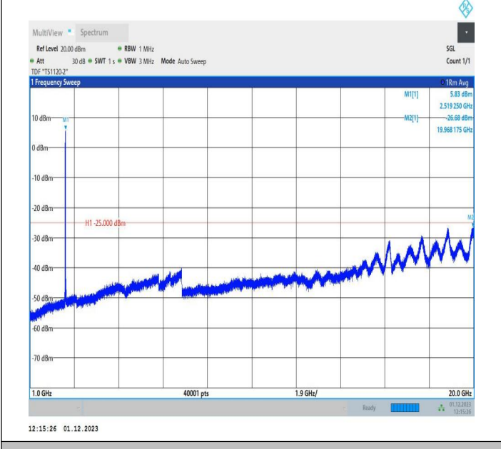
7-7-15MHz-5MHz-16QAM-16QAM-20825-20918-1RB#0-1RB# 24-1000~20000MHz-PASS
