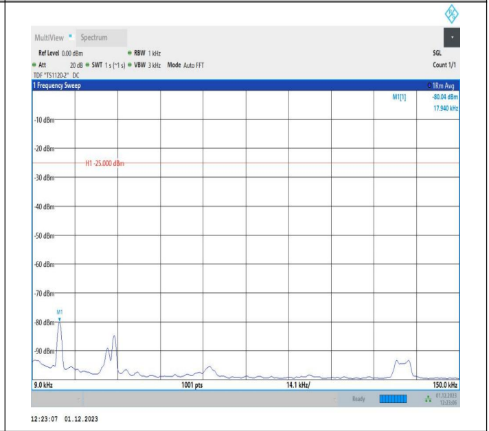
7-7-15MHz-5MHz-16QAM-16QAM-21076-21169-1RB#0-1RB#24-0.009~0.15MHz-PASS
