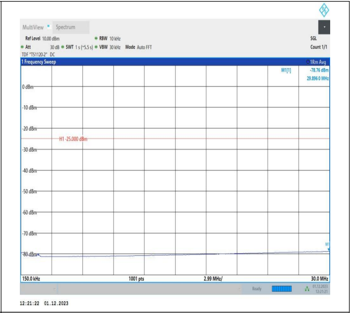
7-7-15MHz-5MHz-16QAM-16QAM-21076-21169-1RB#74-ORB #0-0.15~30MHz-PASS
