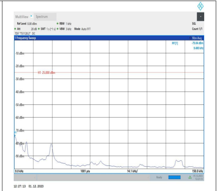
7-7-15MHz-5MHz-16QAM-16QAM-21327-21420-1RB#0-0RB#0-0-0.009~0.15MHz-PASS
