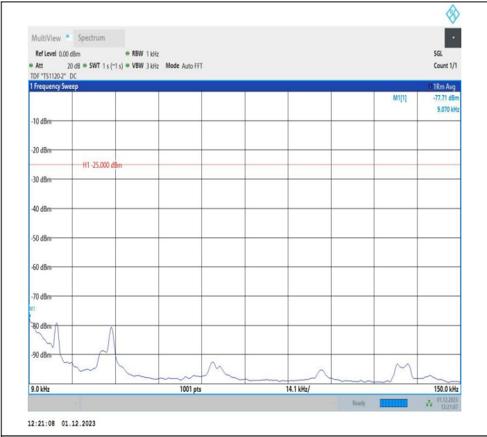
7-7-15MHz-5MHz-16QAM-16QAM-21076-21169-1RB#74-ORB #0-0.009~0.15MHz-PASS
