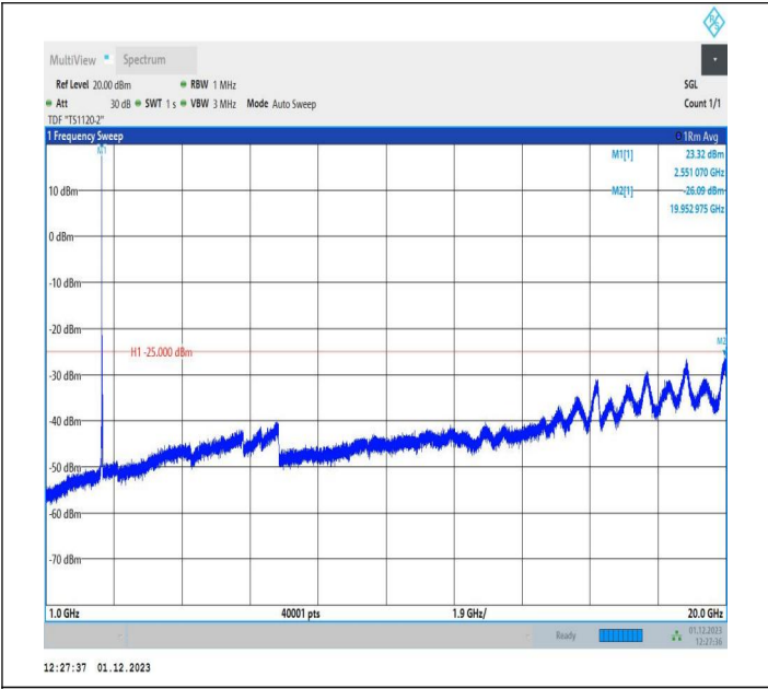
7-7-15MHz-5MHz-16QAM-16QAM-21327-21420-1RB#0-0RB# 0-1000~20000MHz-PASS
