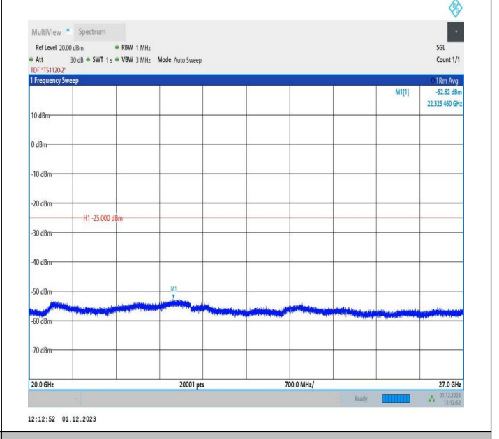
7-7-15MHz-5MHz-QPSK-QPSK-20825-20918-1RB#74-0RB#0 -20000~27000MHz-PASS
