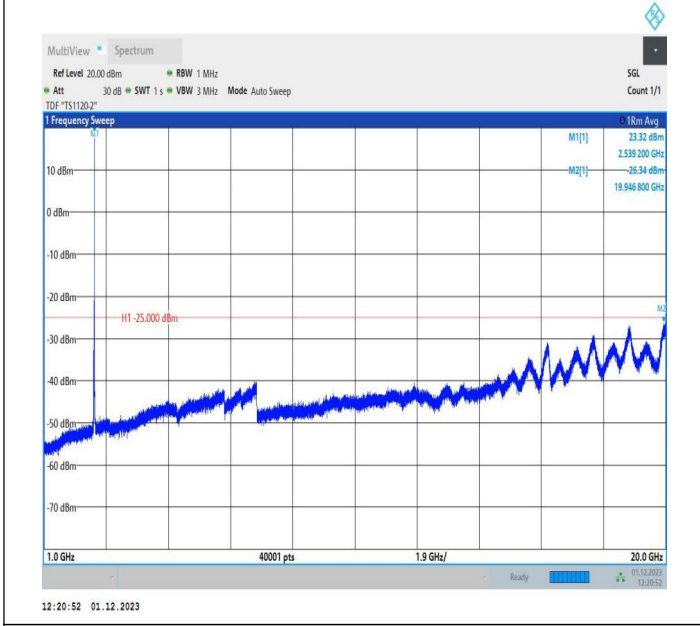
7-7-15MHz-5MHz-QPSK-QPSK-21076-21169-1RB#74-ORB#0-1000~20000MHz-PASS
