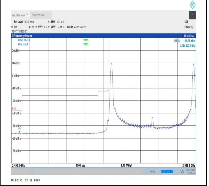
20MHz-20MHz_64QAM@64QAM-64QAM@64QAM_20850-2 1048_1RB#0@100RB#0-1RB#99@100RB#0
