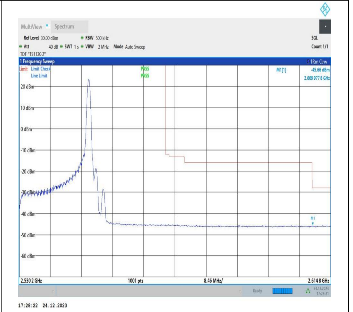
20MHz-20MHz_QPSK@QPSK-QPSK@QPSK_21152-21350_1RB#99@100RB#0-0RB#0@100RB#0
