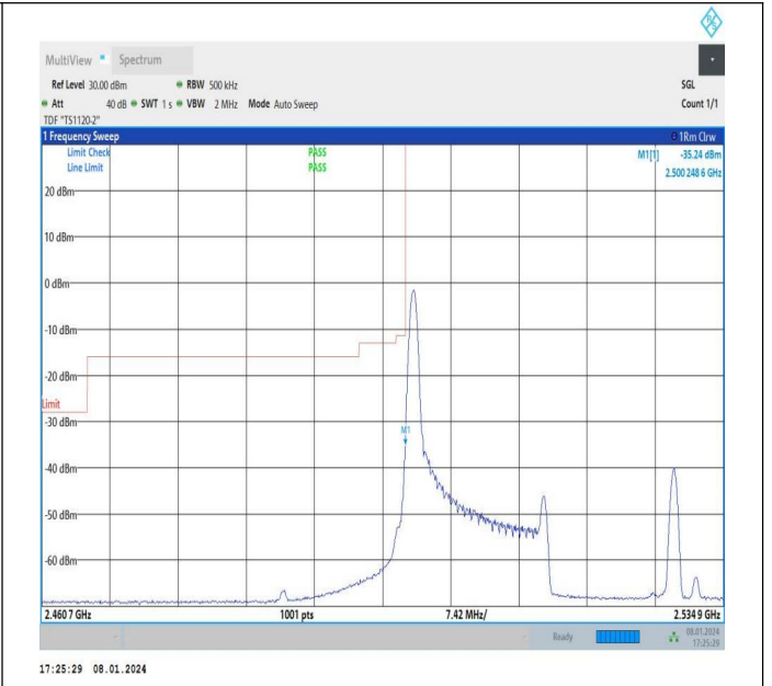
15MHz-20MHz_64QAM@64QAM-64QAM@64QAM_20828-20999_1RB#0@75RB#0-0RB#0@100RB#0
