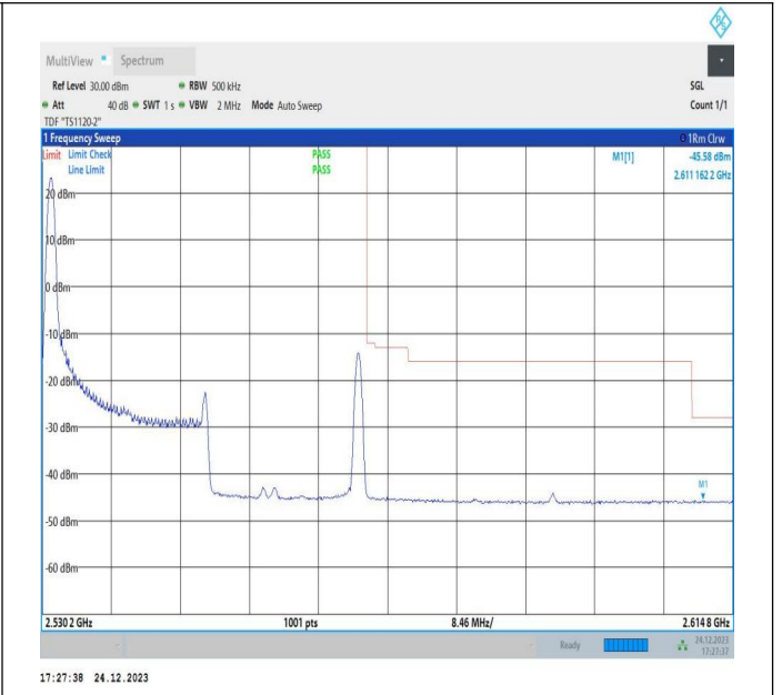
20MHz-20MHz_QPSK@QPSK-QPSK@QPSK_21152-21350_1RB#0@100RB#0-0RB#0@100RB#0
