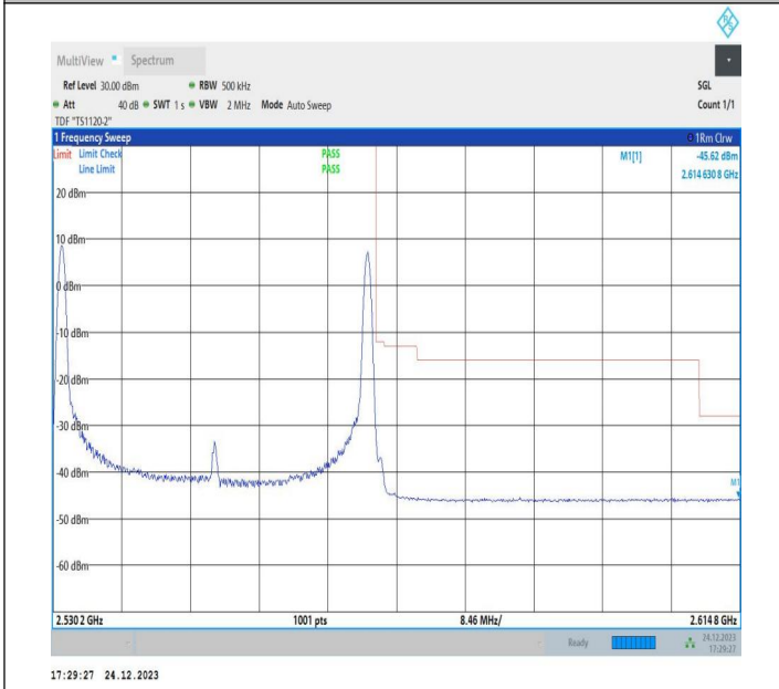
20MHz-20MHz_16QAM@16QAM-16QAM@16QAM_21152-21350_1RB#0@100RB#0-1RB#99@100RB#0
