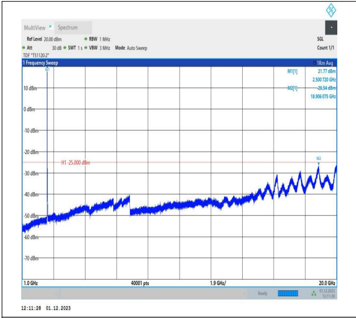
7-7-15MHz-5MHz-16QAM-16QAM-20825-20918-1RB#0-0RB# 0-1000~20000MHz-PASS
