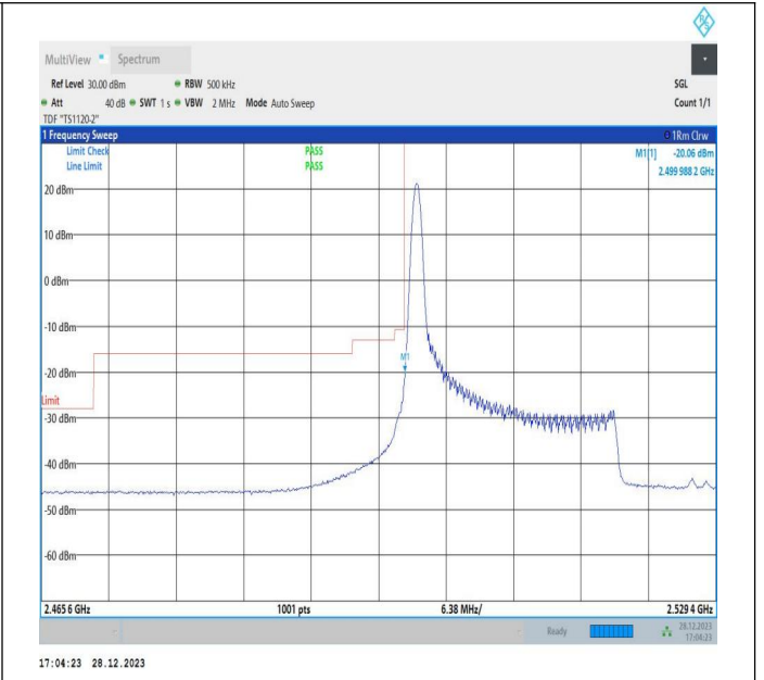
20MHz-10MHz_64QAM@64QAM-64QAM@64QAM_20850-2 0994_1RB#0@100RB#0-0RB#0@50RB#0
