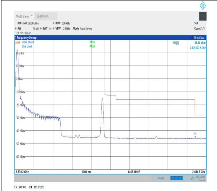
20MHz-20MHz_16QAM@16QAM-16QAM@16QAM_21152-21350_350_1RB#0@100RB#0-0RB#0@100RB#0
