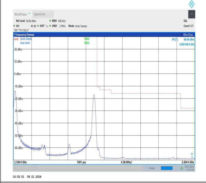
10MHz-20MHz_64QAM@64QAM-64QAM@64QAM_21206-21350_1RB#0@50RB#0-1RB#99@100RB#0
