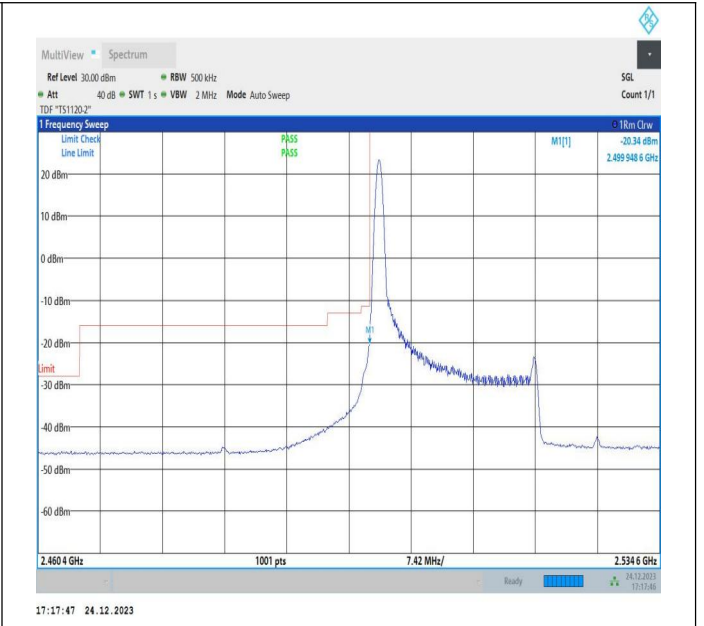
20MHz-15MHz_QPSK@QPSK-QPSK@QPSK_20850-21021_1RB#0@100RB#0-0RB#0@75RB#0
