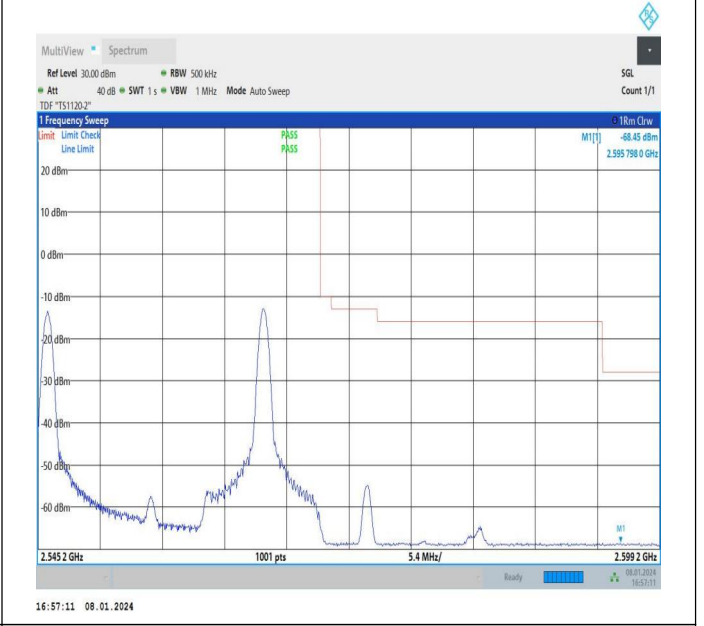
15MHz-10MHz_64QAM@64QAM-64QAM@64QAM_21277-21397_1RB#0@50RB#0-1RB#99@100RB#0
