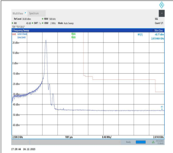
20MHz-20MHz_16QAM@16QAM-16QAM@16QAM_21152-21350_1RB#99@100RB#0-0RB#0@100RB#0
