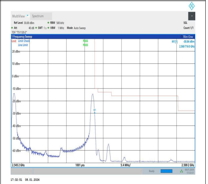
15MHz-10MHz_64QAM@64QAM-64QAM@64QAM_21277-2 1397_1RB#0@75RB#0-1RB#49@50RB#0
