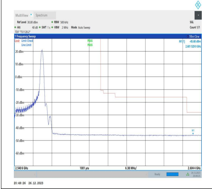
10MHz-20MHz_64QAM@64QAM-64QAM@64QAM_21206-21 350_1RB#49@50RB#0-0RB#0@100RB#0
