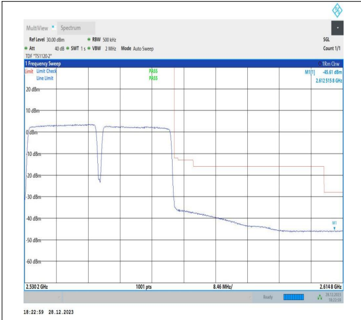
20MHz-20MHz_64QAM@64QAM-64QAM@64QAM_21152-21350_100RB#0@100RB#0-100RB#0@100RB#0
