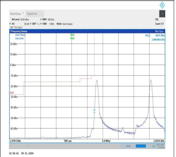
15MHz-10MHz_16QAM@16QAM-16QAM@16QAM_20825-20945_1RB#0@50RB#0-1RB#99@100RB#0
