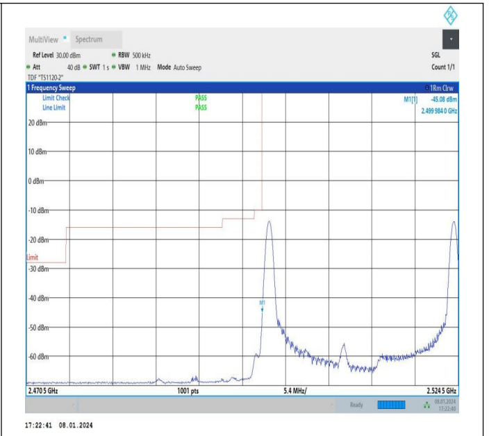
15MHz-10MHz_16QAM@16QAM-16QAM@16QAM_20825-0945_1RB#0@75RB#0-1RB#49@49RB#0
