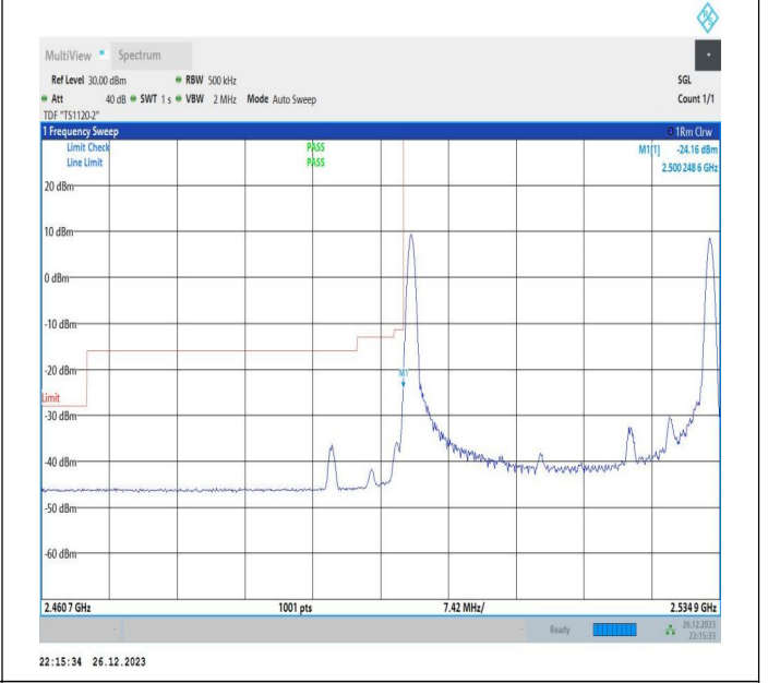
15MHz-20MHz_64QAM@64QAM-64QAM@64QAM_20828-20999_1RB#0@75RB#0-1RB#99@100RB#0
