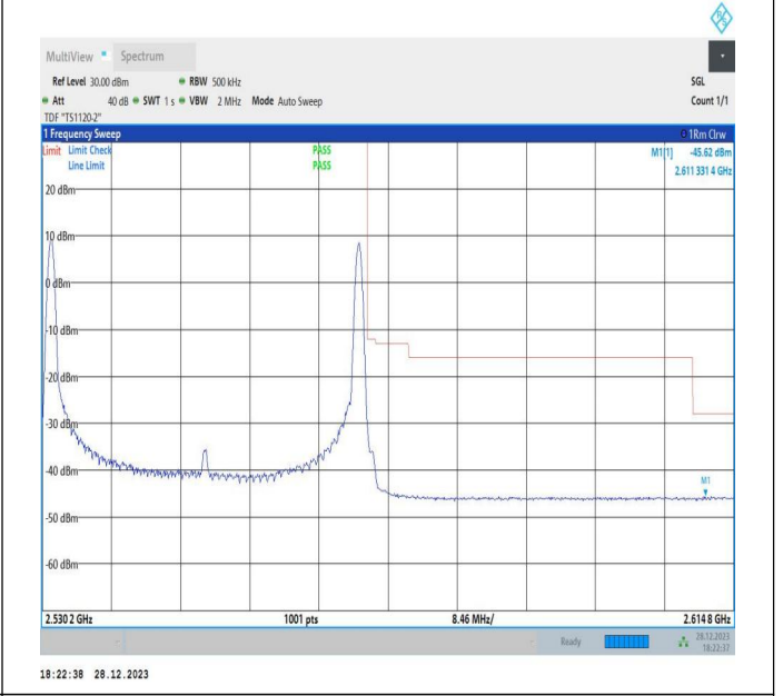
20MHz-20MHz_64QAM@64QAM-64QAM@64QAM_21152-21350_1RB#0@100RB#0-1RB#99@100RB#0
