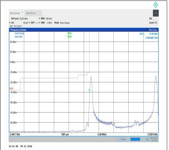
10MHz-20MHz_64QAM@64QAM-64QAM@64QAM_20805-2 0949_1RB#0@50RB#0-1RB#99@100RB#0
