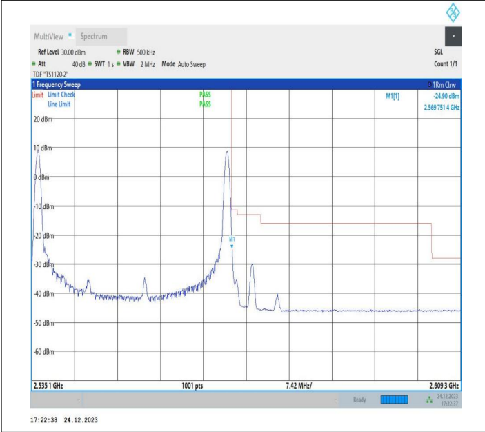
20MHz-15MHz_16QAM@16QAM-16QAM@16QAM_21201-21372_1RB#0@100RB#0-1RB#74@75RB#0
