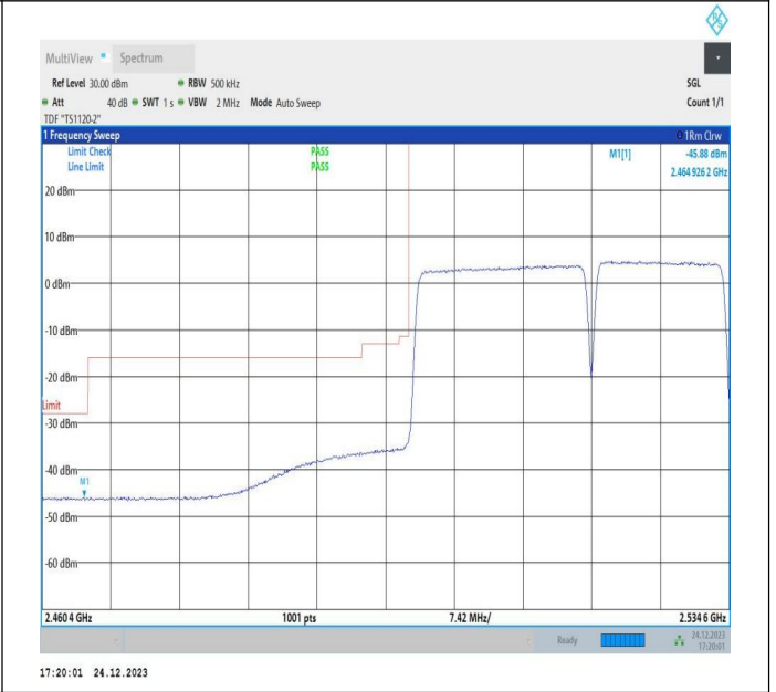
20MHz-15MHz_QPSK@QPSK-QPSK@QPSK_20850-21021_100RB#0@100RB#0-75RB#0@75RB#0
