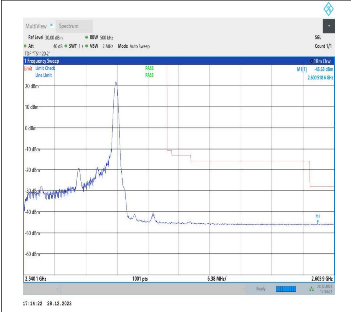
20MHz-10MHz_64QAM@64QAM-64QAM@64QAM_21251-21395_1RB#99@100RB#0-0RB#0@50RB#0
