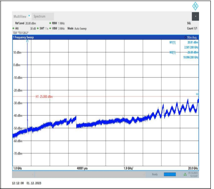
7-7-15MHz-5MHz-64QAM-64QAM-20825-20918-1RB#0-0RB# 0-1000~20000MHz-PASS
