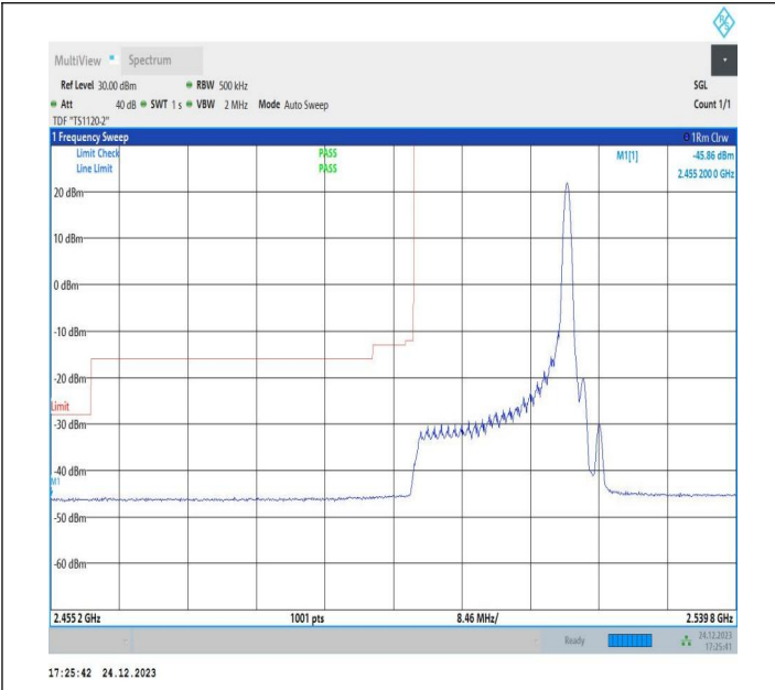
20MHz-20MHz_16QAM@16QAM-16QAM@16QAM_20850-21048_1RB#99@100RB#0-0RB#0@100RB#0
