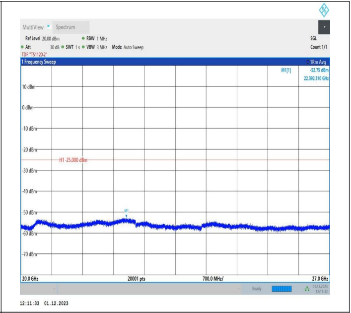
7-7-15MHz-5MHz-16QAM-16QAM-20825-20918-1RB#0-0RB# 0-20000~27000MHz-PASS
