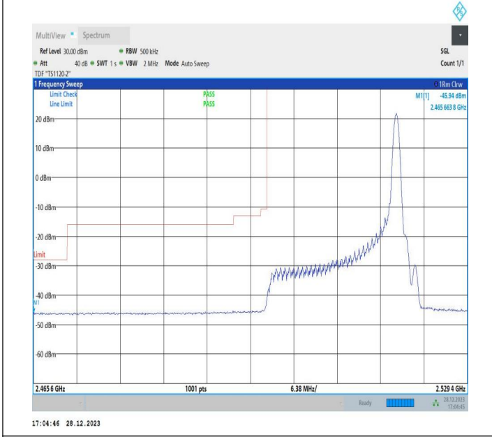
20MHz-10MHz_64QAM@64QAM-64QAM@64QAM_20850-20 994_1RB#99@100RB#0-0RB#0@50RB#0
