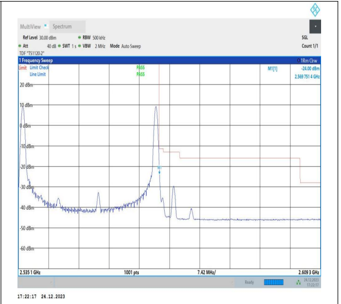
20MHz-15MHz_QPSK@QPSK-QPSK@QPSK_21201-21372_1RB#0@100RB#0-1RB#74@75RB#0
