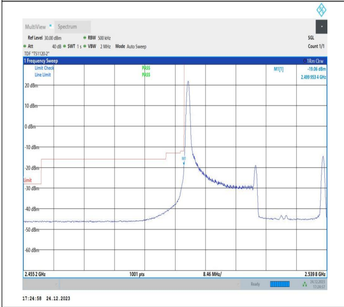
20MHz-20MHz_16QAM@16QAM-16QAM@16QAM_20850-21048_1RB#0@100RB#0-0RB#0@100RB#0
