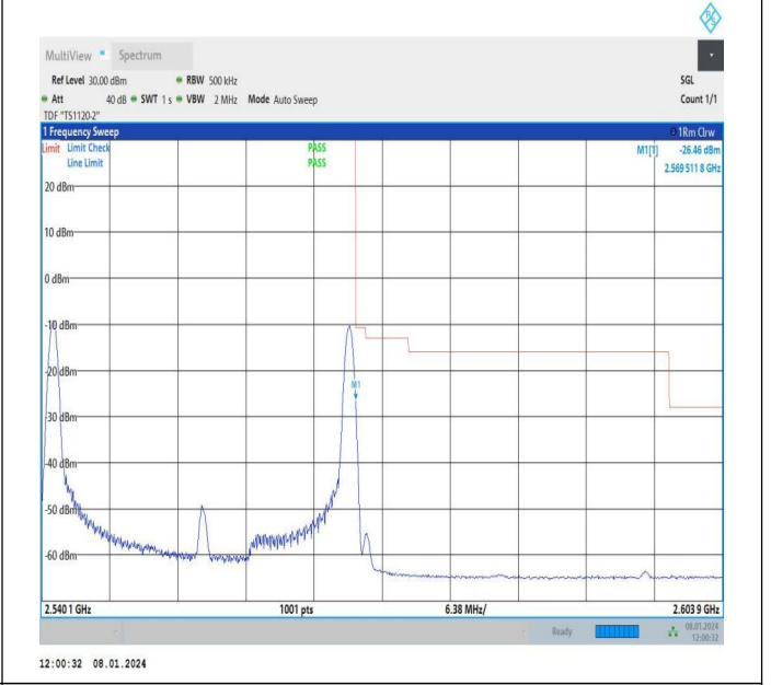
20MHz-10MHz_64QAM@64QAM-64QAM@64QAM_21251-2 1395_1RB#0@100RB#0-1RB#49@50RB#0
