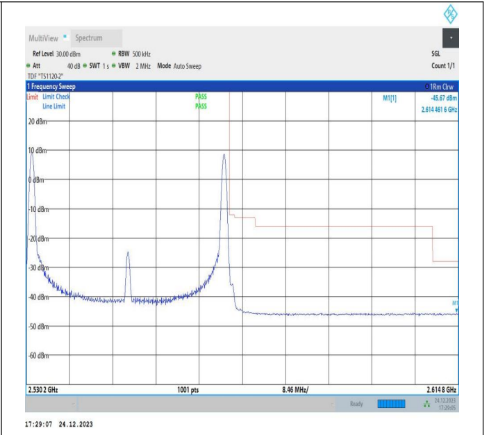
20MHz-20MHz_QPSK@QPSK-QPSK@QPSK_21152-21350_1RB#0@100RB#0-1RB#99@100RB#0
