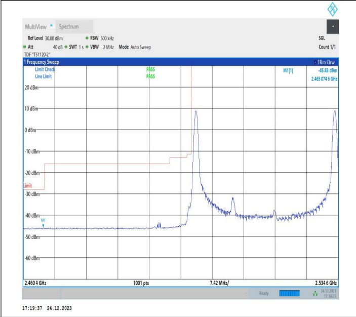
20MHz-15MHz_16QAM@16QAM-16QAM@16QAM_20850-21021_1RB#0@100RB#0-1RB#74@75RB#0
