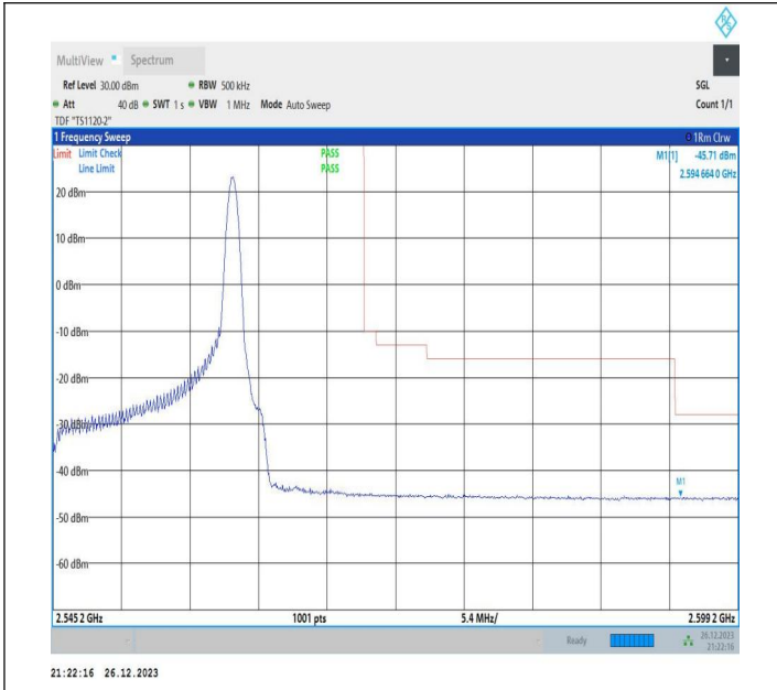
15MHz-10MHz_64QAM@64QAM-64QAM@64QAM_21277-21 397_1RB#74@75RB#0-0RB#0@50RB#0
