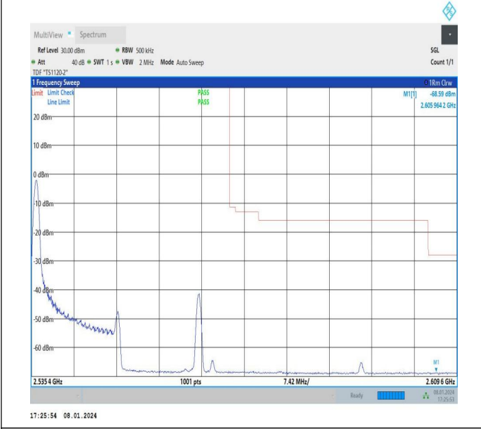
15MHz-20MHz_64QAM@64QAM-64QAM@64QAM_21179-21350_1RB#0@75RB#0-0RB#0@100RB#0
