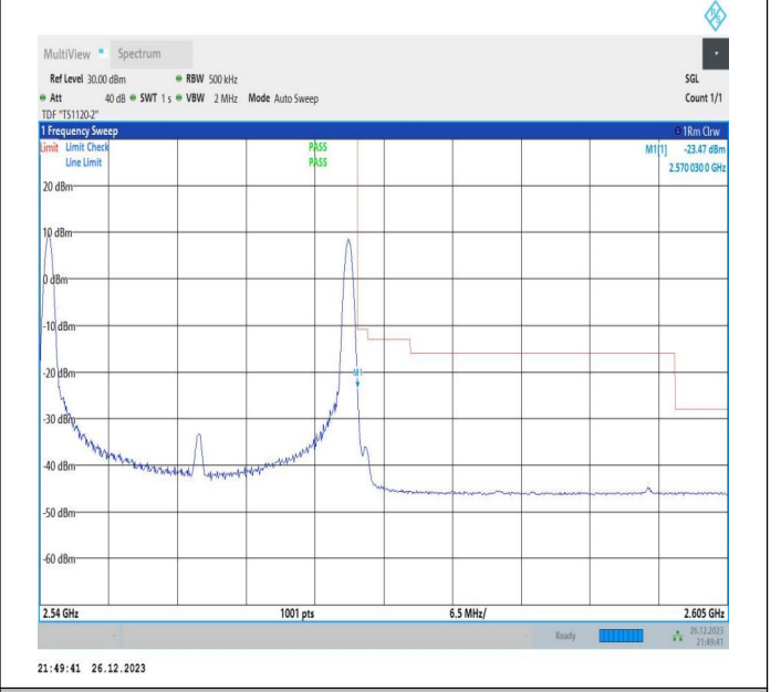
15MHz-15MHz_64QAM@64QAM-64QAM@64QAM_21225-21375_1RB#0@75RB#0-1RB#74@75RB#0
