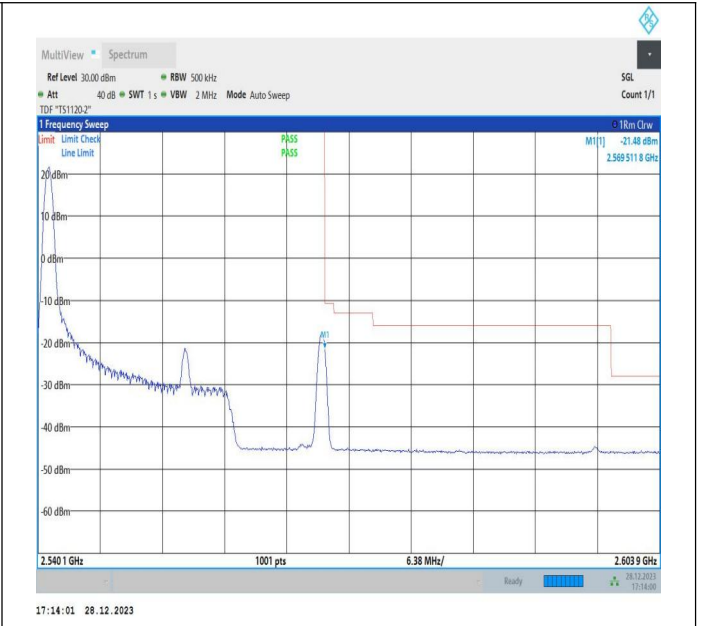
20MHz-10MHz_64QAM@64QAM-64QAM@64QAM_21251-21395_1RB#0@100RB#0-0RB#0@50RB#0
