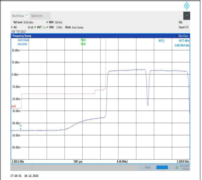
20MHz-20MHz_QPSK@QPSK-QPSK@QPSK_20850-21048_100RB#0@100RB#0-100RB#0@100RB#0
