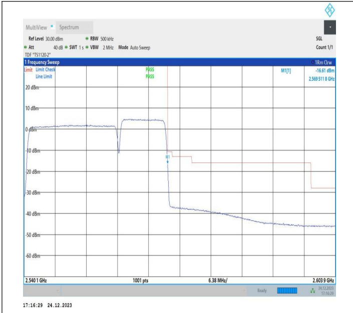
20MHz-10MHz_16QAM@16QAM-16QAM@16QAM_21251-21395_100RB#0@100RB#0-50RB#0@50RB#0
