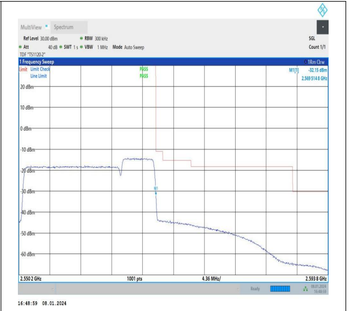
15MHz-5MHz_64QAM@64QAM-64QAM@64QAM_21327-21420_75RB#0@75RB#0-25RB#0@25RB#0
