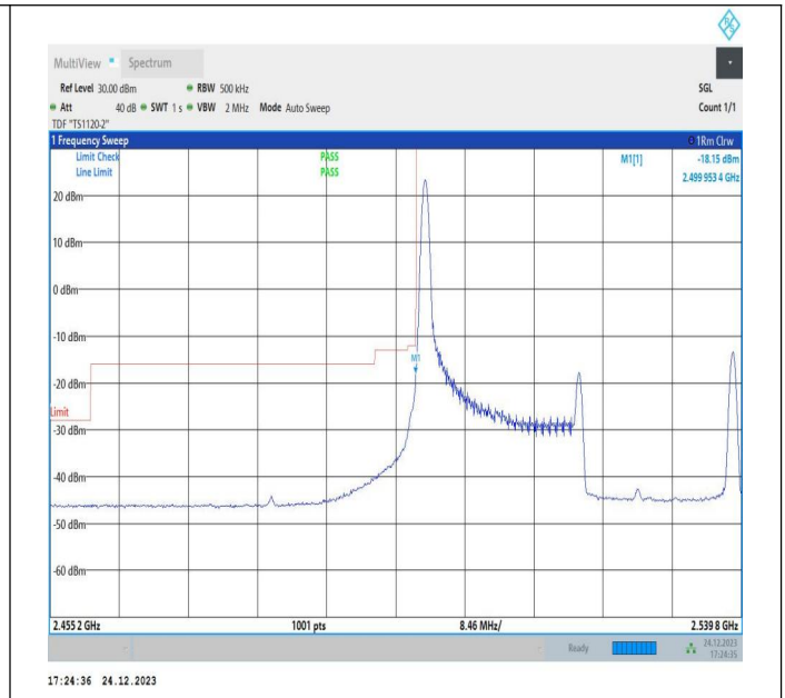
20MHz-20MHz_QPSK@QPSK-QPSK@QPSK_20850-21048_1RB#0@100RB#0-0RB#0@100RB#0
