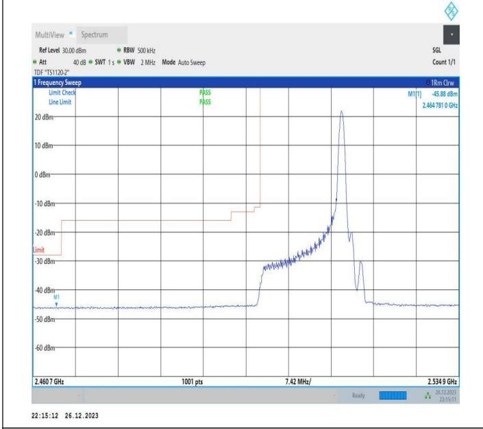
15MHz-20MHz_64QAM@64QAM-64QAM@64QAM_20828-20999_1RB#74@75RB#0-0RB#0@100RB#0
