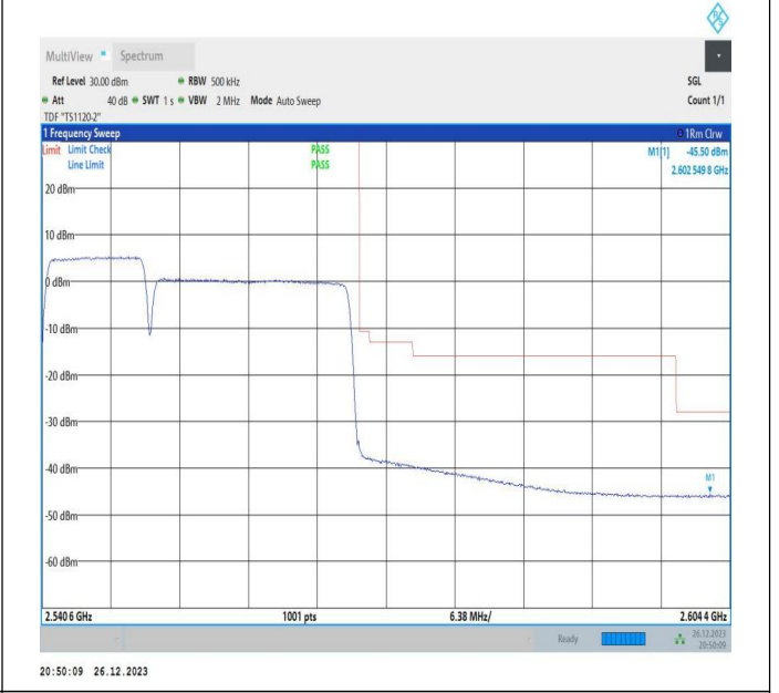
10MHz-20MHz_64QAM@64QAM-64QAM@64QAM_21206-2 1350_50RB#0@50RB#0-100RB#0@100RB#0
