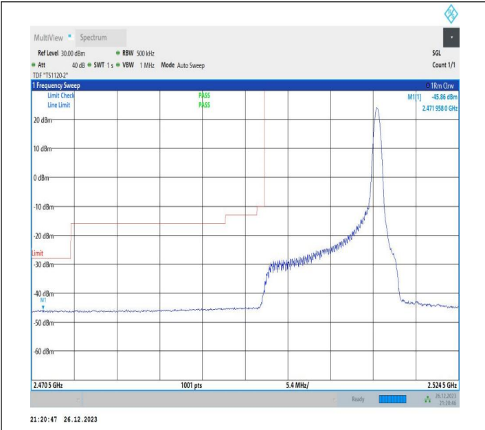
15MHz-10MHz_64QAM@64QAM-64QAM@64QAM_20825-20945_1RB#74@75RB#0-0RB#0@50RB#0
