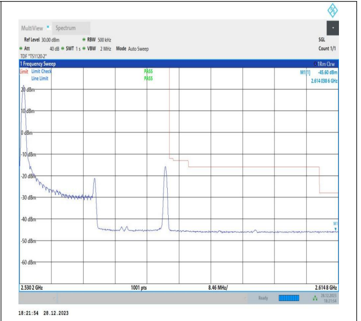
20MHz-20MHz_64QAM@64QAM-64QAM@64QAM_21152-21350_1RB#0@100RB#0-0RB#0@100RB#0
