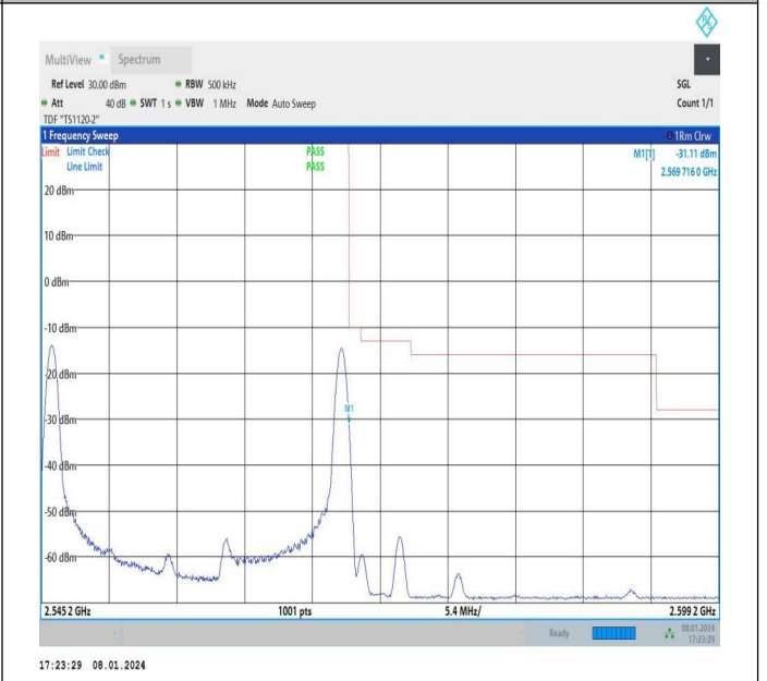
15MHz-10MHz_QPSK@QPSK-QPSK@QPSK_21277-21397_1RB#0@75RB#0-1RB#49@49RB#0
