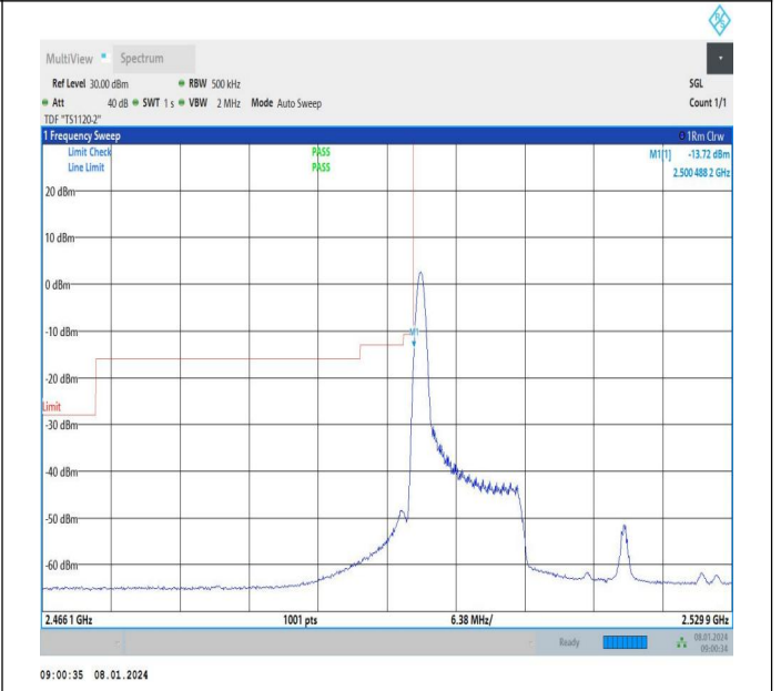
10MHz-20MHz_64QAM@64QAM-64QAM@64QAM_20805-20949_1RB#0@50RB#0-0RB#0@100RB#0
