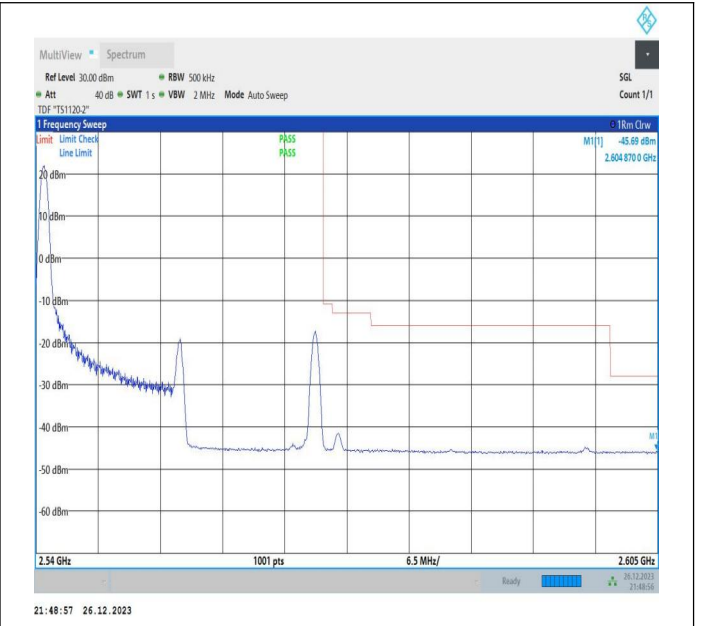
15MHz-15MHz_64QAM@64QAM-64QAM@64QAM_21225-21375_1RB#0@75RB#0-0RB#0@75RB#0
