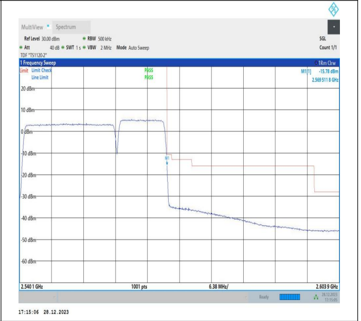
20MHz-10MHz_64QAM@64QAM-64QAM@64QAM_21251-21395_100RB#0@100RB#0-50RB#0@50RB#0
