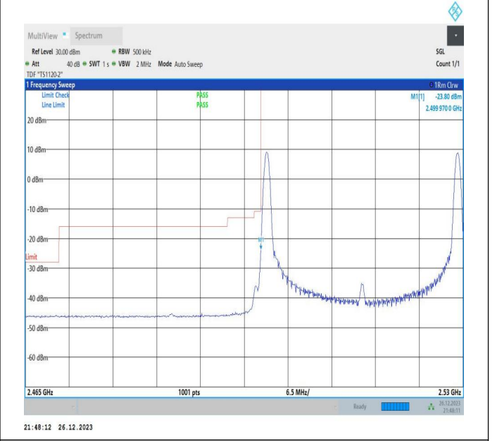
15MHz-15MHz_64QAM@64QAM-64QAM@64QAM_20825-20975_1RB#0@75RB#0-1RB#74@75RB#0
