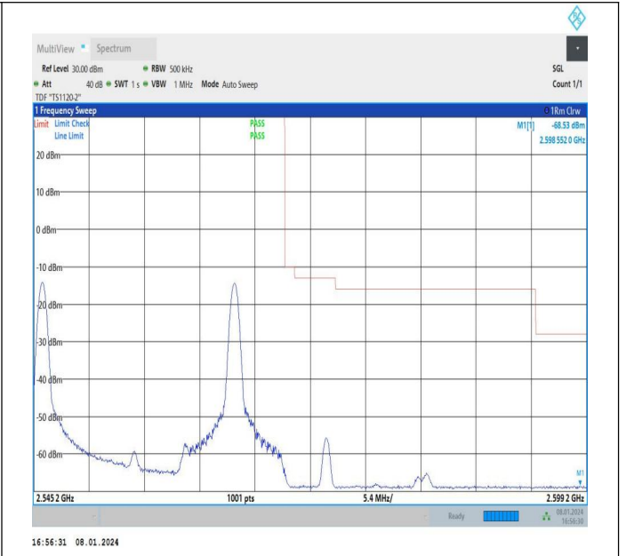
15MHz-10MHz_QPSK@QPSK-QPSK@QPSK_21277-21397_1RB#0@50RB#0-1RB#99@100RB#0
