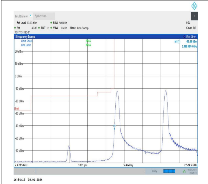
15MHz-10MHz_QPSK@QPSK-QPSK@QPSK_20825-20945_1RB#0@50RB#0-1RB#99@100RB#0
