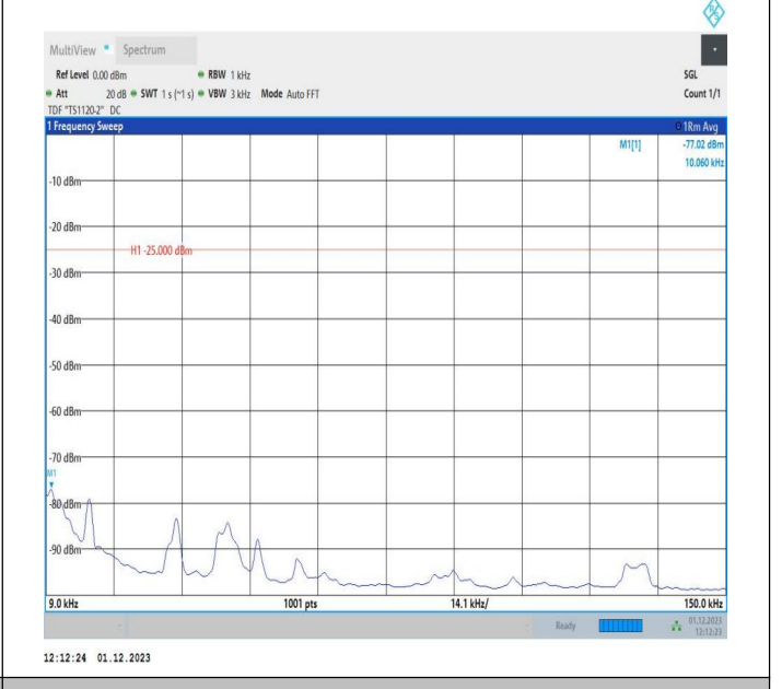
7-7-15MHz-5MHz-QPSK-QPSK-20825-20918-1RB#74-0RB#0 -0.009~0.15MHz-PASS
