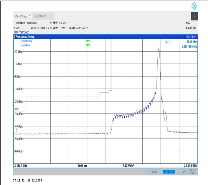
20MHz-15MHz_16QAM@16QAM-16QAM@16QAM_20850-21021_1RB#99@100RB#0-0RB#0@75RB#0
