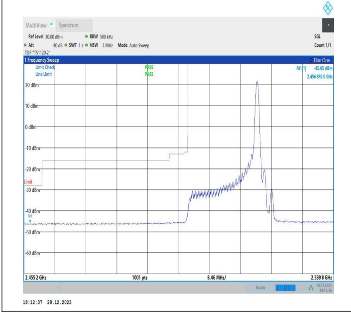
20MHz-20MHz_64QAM@64QAM-64QAM@64QAM_20850-21 048_1RB#99@100RB#0-0RB#0@100RB#0
