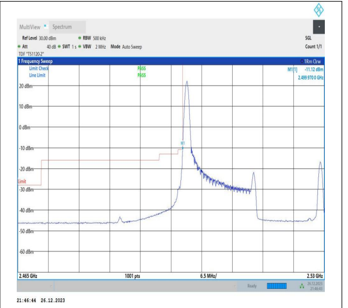
15MHz-15MHz_64QAM@64QAM-64QAM@64QAM_20825-20975_1RB#0@75RB#0-0RB#0@75RB#0
