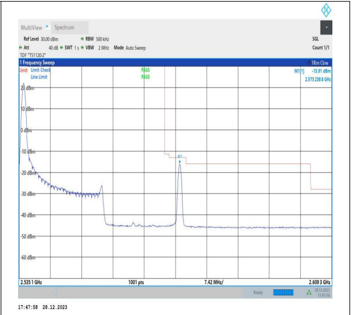
20MHz-15MHz_64QAM@64QAM-64QAM@64QAM_21201-21372_1RB#0@100RB#0-0RB#0@75RB#0
