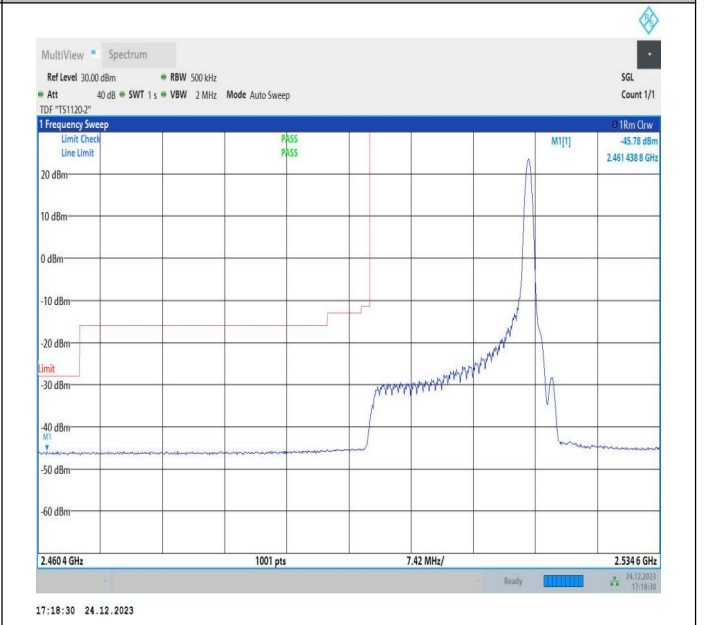
20MHz-15MHz_QPSK@QPSK-QPSK@QPSK_20850-21021_1RB#99@100RB#0-0RB#0@75RB#0
