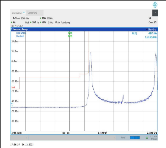
20MHz-20MHz_16QAM@16QAM-16QAM@16QAM_20850-21048_1RB#0@100RB#0-1RB#99@100RB#0
