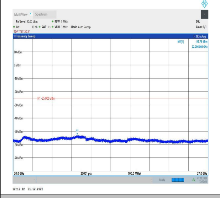
7-7-15MHz-5MHz-64QAM-64QAM-20825-20918-1RB#0-0RB# 0-20000~27000MHz-PASS
