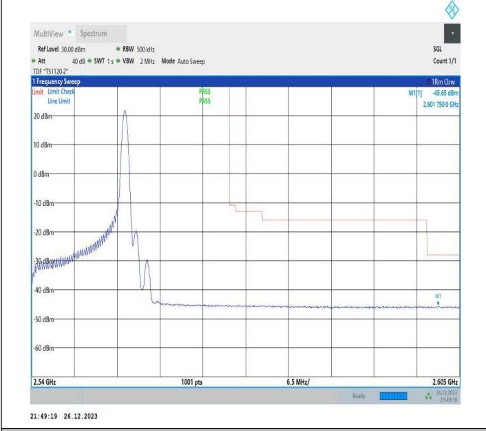
15MHz-15MHz_64QAM@64QAM-64QAM@64QAM_21225-21375_1RB#74@75RB#0-0RB#0@75RB#0
