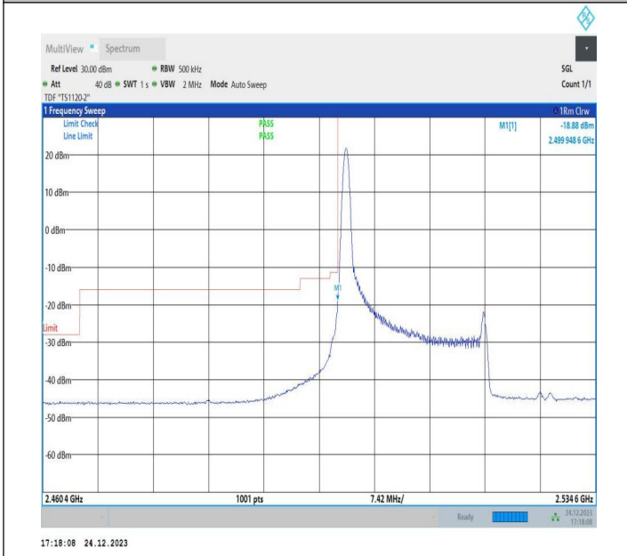
20MHz-15MHz_16QAM@16QAM-16QAM@16QAM_20850-21021_021_1RB#0@100RB#0-0RB#0@75RB#0
