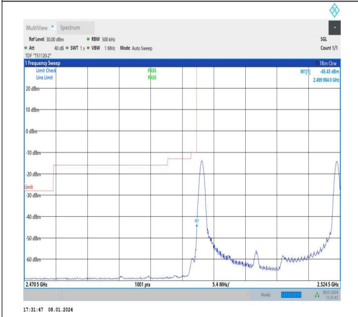
15MHz-10MHz_64QAM@64QAM-64QAM@64QAM_20825-20 945_1RB#0@75RB#0-1RB#49@50RB#0
