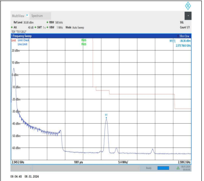
15MHz-10MHz_64QAM@64QAM-64QAM@64QAM_21277-2 1397_1RB#0@75RB#0-0RB#0@50RB#0
