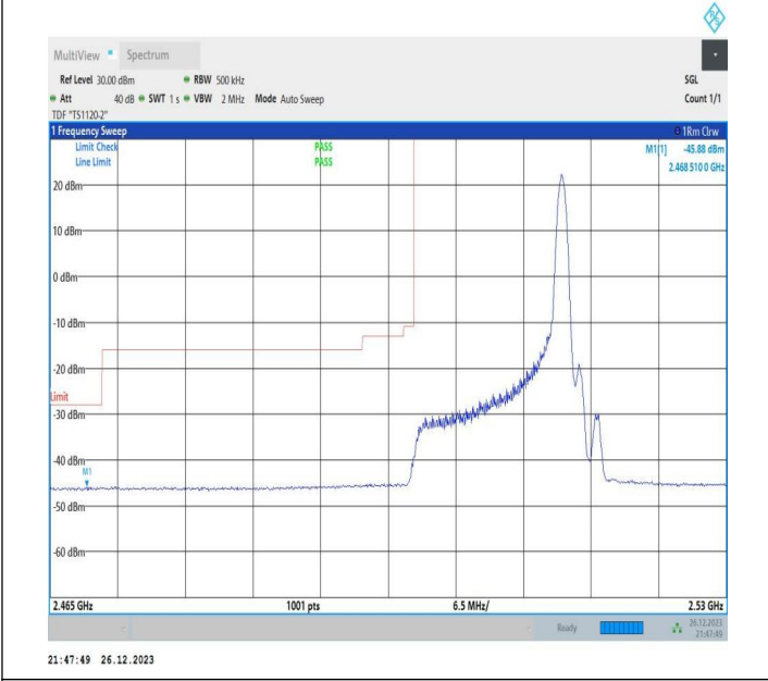
15MHz-15MHz_64QAM@64QAM-64QAM@64QAM_20825-20975_1RB#74@75RB#0-0RB#0@75RB#0
