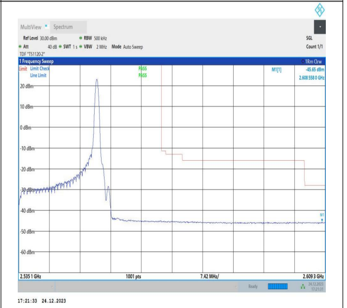
20MHz-15MHz_QPSK@QPSK-QPSK@QPSK_21201-21372_1RB#99@100RB#0-0RB#0@75RB#0
