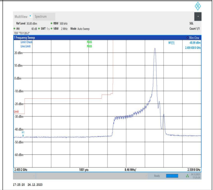
20MHz-20MHz_QPSK@QPSK-QPSK@QPSK_20850-21048_1RB#99@100RB#0-0RB#0@100RB#0
