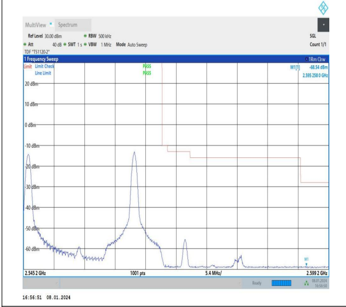
15MHz-10MHz_16QAM@16QAM-16QAM@16QAM_21277-21397_1RB#0@50RB#0-1RB#99@100RB#0
