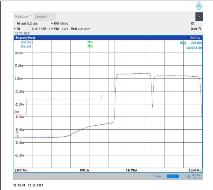
15MHz-20MHz_64QAM@64QAM-64QAM@64QAM_20828-20999_75RB#0@75RB#0-100RB#0@100RB#0
