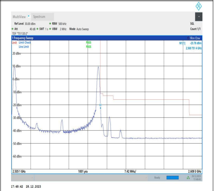
20MHz-15MHz_64QAM@64QAM-64QAM@64QAM_21201-21372_1RB#0@100RB#0-1RB#74@75RB#0
