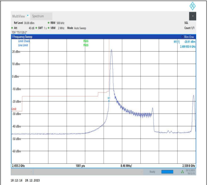
20MHz-20MHz_64QAM@64QAM-64QAM@64QAM_20850-2 1048_1RB#0@100RB#0-0RB#0@100RB#0
