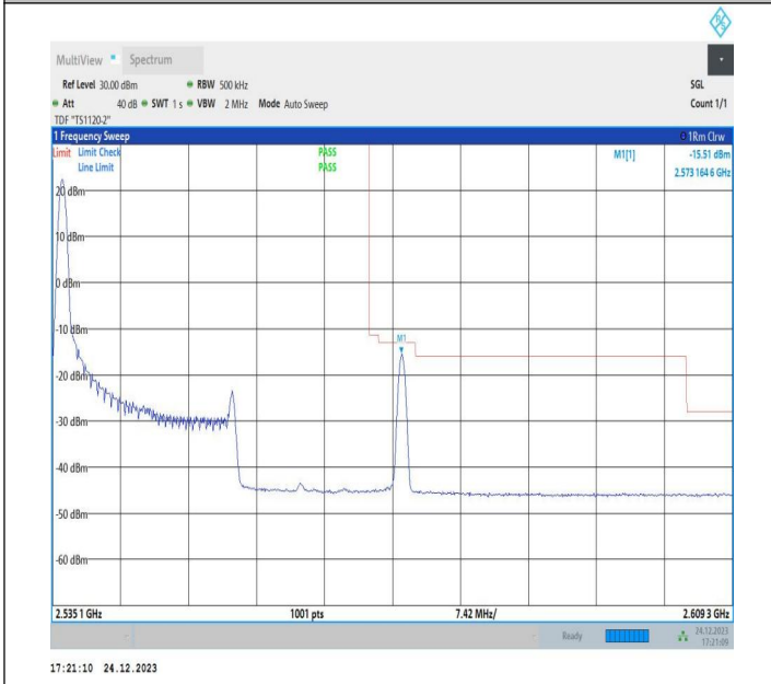
20MHz-15MHz_16QAM@16QAM-16QAM@16QAM_21201-21372_372_1RB#0@100RB#0-0RB#0@75RB#0
