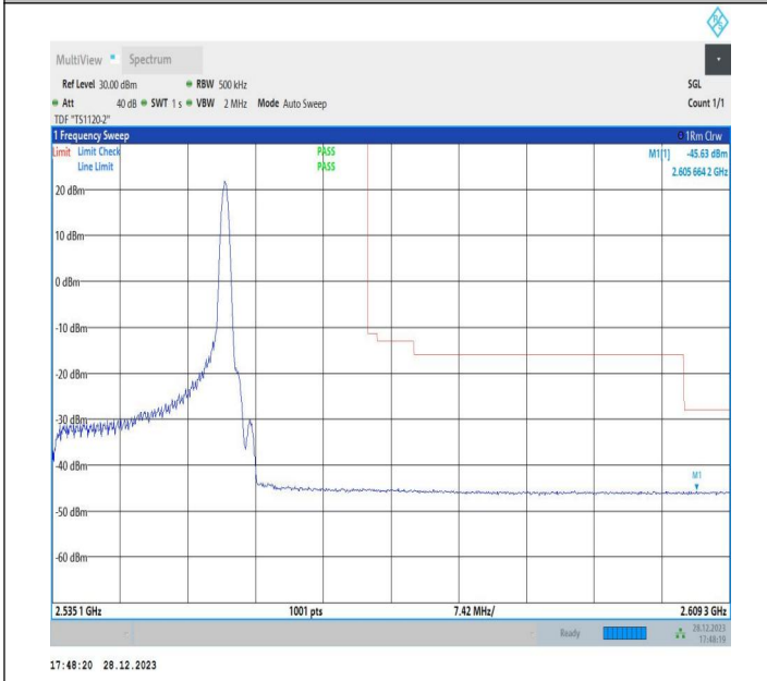
20MHz-15MHz_64QAM@64QAM-64QAM@64QAM_21201-21372_1RB#99@100RB#0-0RB#0@75RB#0
