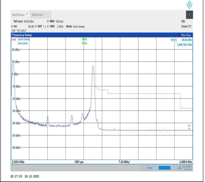
15MHz-20MHz_64QAM@64QAM-64QAM@64QAM_21179-21350_1RB#0@75RB#0-1RB#99@100RB#0
