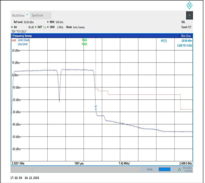
20MHz-15MHz_QPSK@QPSK-QPSK@QPSK_21201-21372_100RB#0@100RB#0-75RB#0@75RB#0
