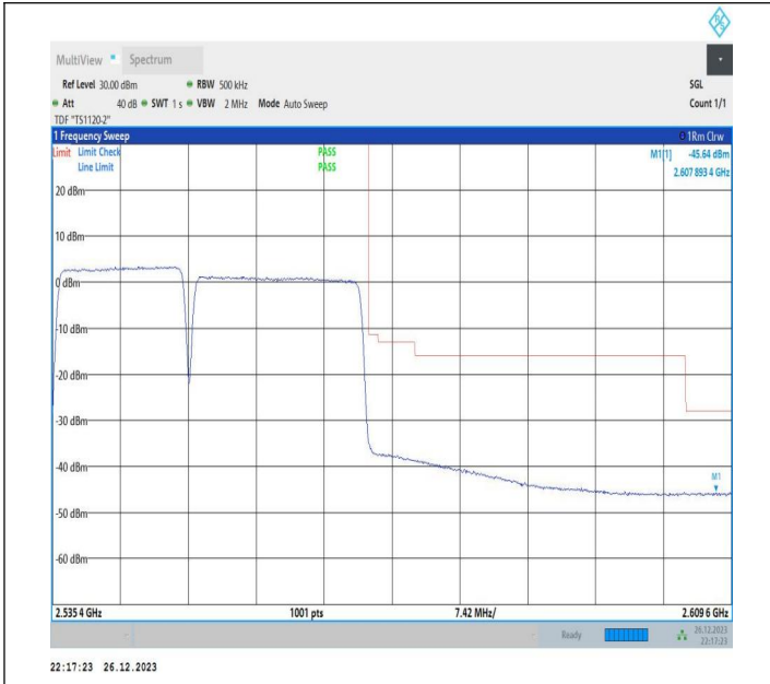
15MHz-20MHz_64QAM@64QAM-64QAM@64QAM_21179-21 350_75RB#0@75RB#0-100RB#0@100RB#0
