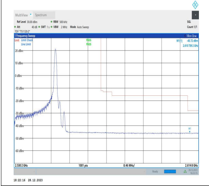
20MHz-20MHz_64QAM@64QAM-64QAM@64QAM_21152-21350_1RB#99@100RB#0-0RB#0@100RB#0
