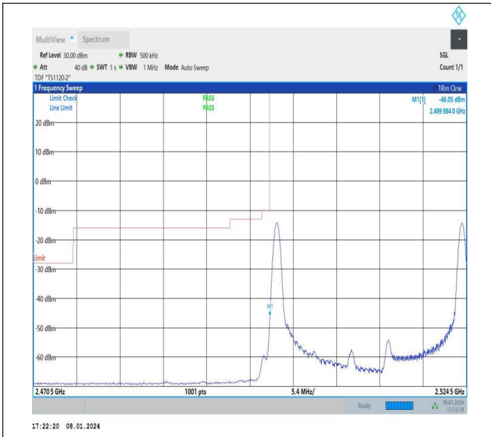
15MHz-10MHz_QPSK@QPSK-QPSK@QPSK_20825-20945_1 RB#0@75RB#0-1RB#49@49RB#0
