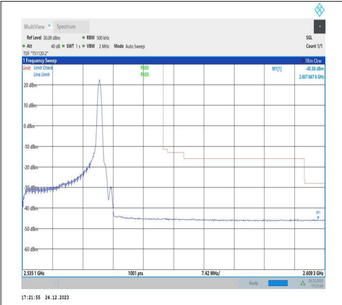
20MHz-15MHz_16QAM@16QAM-16QAM@16QAM_21201-21372_1RB#99@100RB#0-0RB#0@75RB#0
