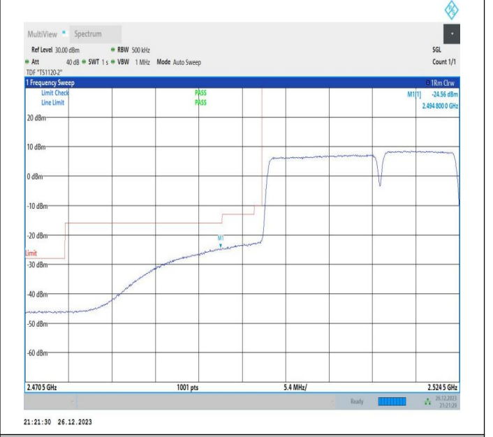
15MHz-10MHz_64QAM@64QAM-64QAM@64QAM_20825-20945_75RB#0@75RB#0-50RB#0@50RB#0
