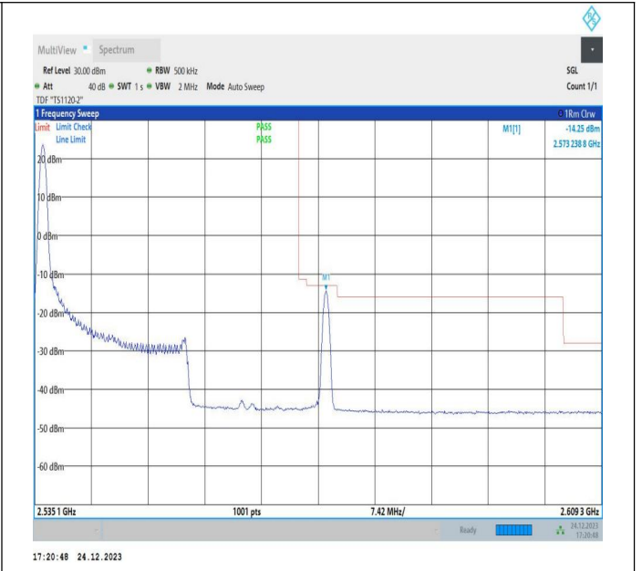
20MHz-15MHz_QPSK@QPSK-QPSK@QPSK_21201-21372_1RB#0@100RB#0-0RB#0@75RB#0
