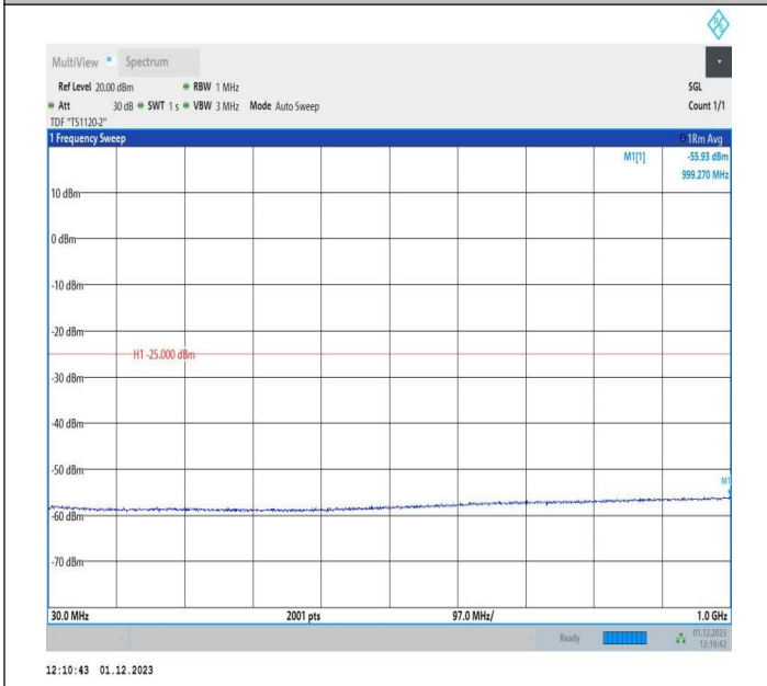
7-7-15MHz-5MHz-QPSK-QPSK-20825-20918-1RB#0-0RB#0-30~1000MHz-PASS
