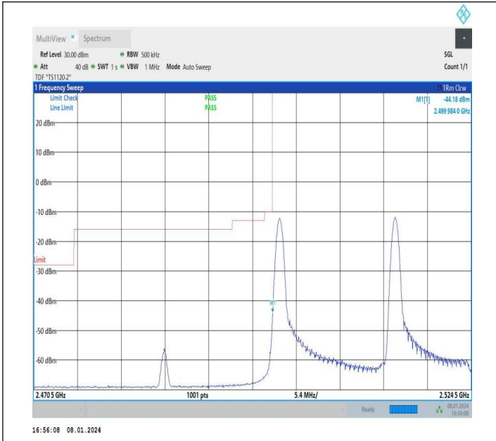
15MHz-10MHz_64QAM@64QAM-64QAM_20825-20945_1RB#0@50RB#0-1RB#99@100RB#0
