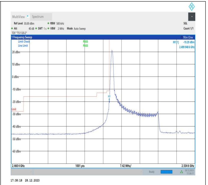
20MHz-15MHz_64QAM@64QAM-64QAM@64QAM_20850-21021_1RB#0@100RB#0-0RB#0@75RB#0
