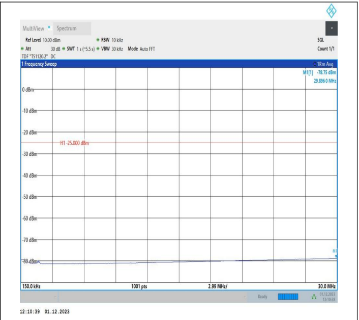
7-7-15MHz-5MHz-QPSK-QPSK-20825-20918-1RB#0-0RB#0-0.15~30MHz-PASS
