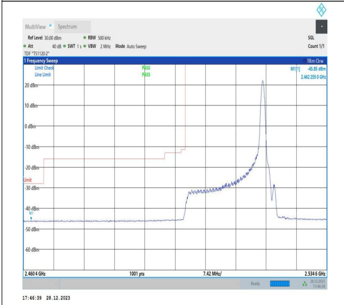
20MHz-15MHz_64QAM@64QAM-64QAM@64QAM_20850-21021_1RB#99@100RB#0-0RB#0@75RB#0
