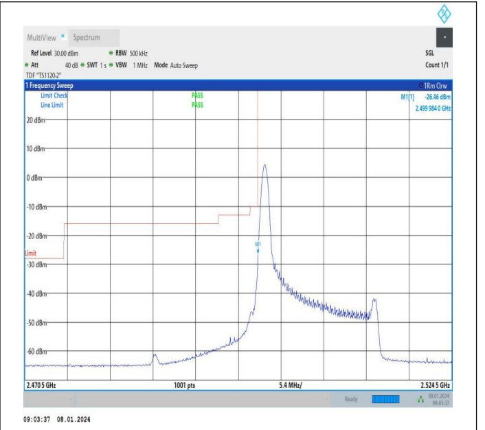
15MHz-10MHz_64QAM@64QAM-64QAM@64QAM_20825-20945_1RB#0@75RB#0-0RB#0@50RB#0
