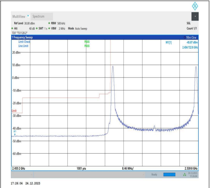
20MHz-20MHz_QPSK@QPSK-QPSK@QPSK_20850-21048_1RB#0@100RB#0-1RB#99@100RB#0
