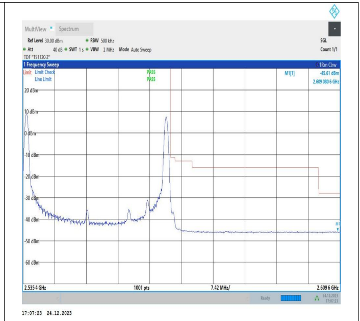
15MHz-20MHz_QPSK@QPSK-QPSK@QPSK_21179-21350_1RB#0@75RB#0-1RB#99@100RB#0
