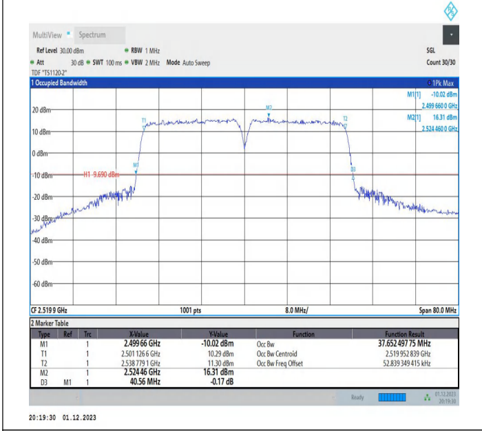
7-7-20MHz-20MHz-16QAM-16QAM-20850-21048-100RB#0-1 00RB#0-PASS
