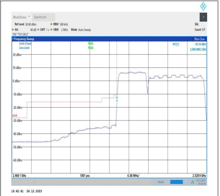
10MHz-20MHz_QPSK@QPSK-QPSK@QPSK_20805-20949_50RB#0@50RB#0-100RB#0@100RB#0
