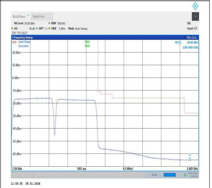
15MHz-15MHz_16QAM@16QAM-16QAM@16QAM_21225-1375_75RB#0@75RB#0-75RB#0@75RB#0
