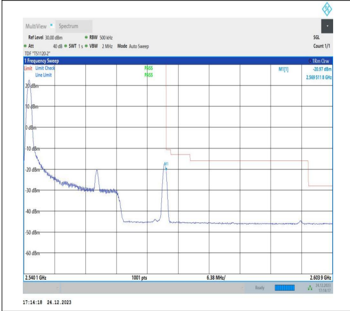
20MHz-10MHz_16QAM@16QAM-16QAM@16QAM_21251-21395_1RB#0@100RB#0-0RB#0@50RB#0
