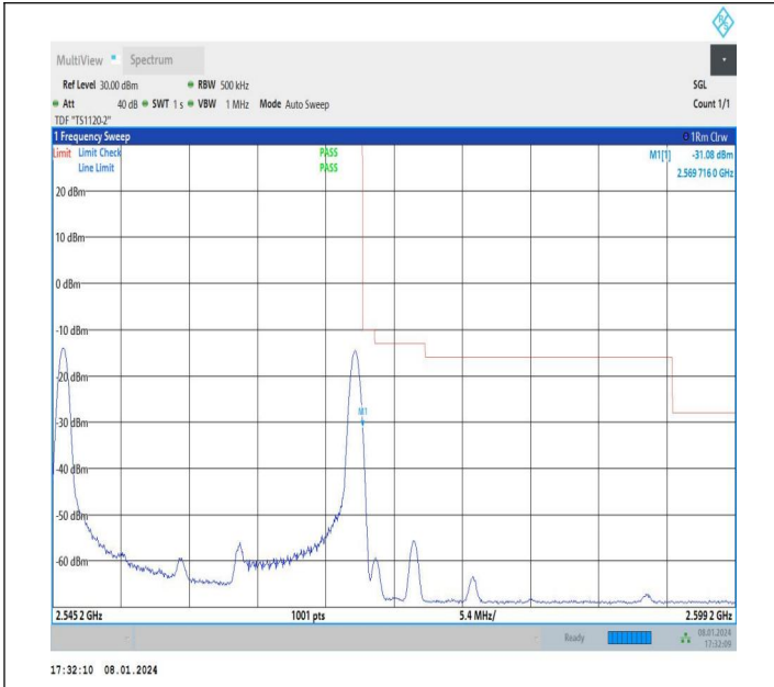
15MHz-10MHz_QPSK@QPSK-QPSK@QPSK_21277-21397_1 RB#0@75RB#0-1RB#49@50RB#0
