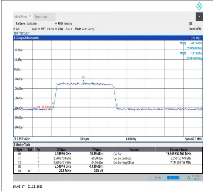
7-7-20MHz-10MHz-QPSK-QPSK-21251-21395-100RB#0-50R B#0-PASS
