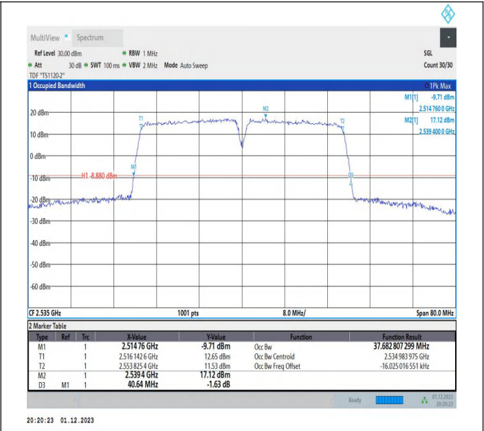
7-7-20MHz-20MHz-QPSK-QPSK-21001-21199-100RB#0-100 RB#0-PASS
