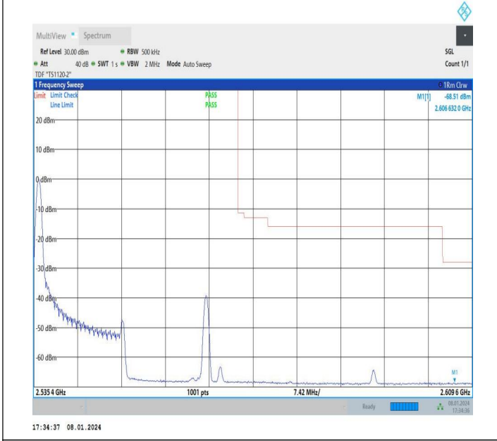
15MHz-20MHz_QPSK@QPSK-QPSK@QPSK_21179-21350_1RB#0@75RB#0-0RB#0@100RB#0
