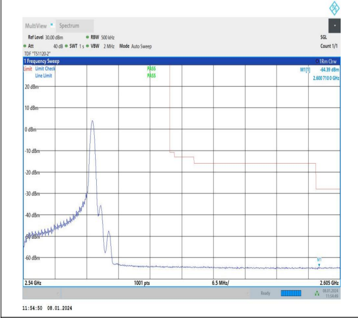
15MHz-15MHz_QPSK@QPSK-QPSK@QPSK_21225-21375_1 RB#74@75RB#0-0RB#0@75RB#0
