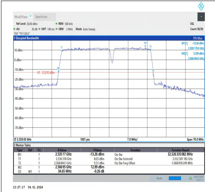
7-7-20MHz-15MHz-64QAM-64QAM-21201-21372-100RB#0-7 5RB#0-PASS
