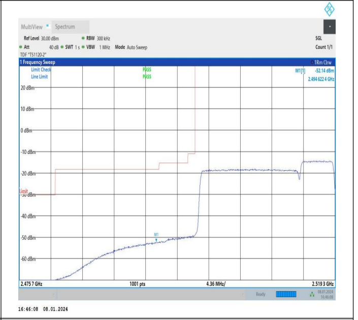
15MHz-5MHz_QPSK@QPSK-QPSK@QPSK_20825-20918_75RB#0@75RB#0-25RB#0@25RB#0
