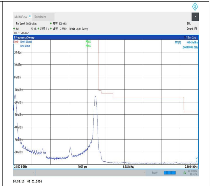
10MHz-20MHz_QPSK@QPSK-QPSK@QPSK_21206-21350_1RB#0@50RB#0-1RB#99@100RB#0
