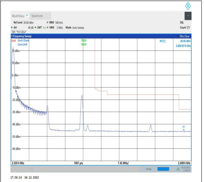
15MHz-20MHz_16QAM@16QAM-16QAM@16QAM_21179-21350_1RB#0@75RB#0-0RB#0@100RB#0
