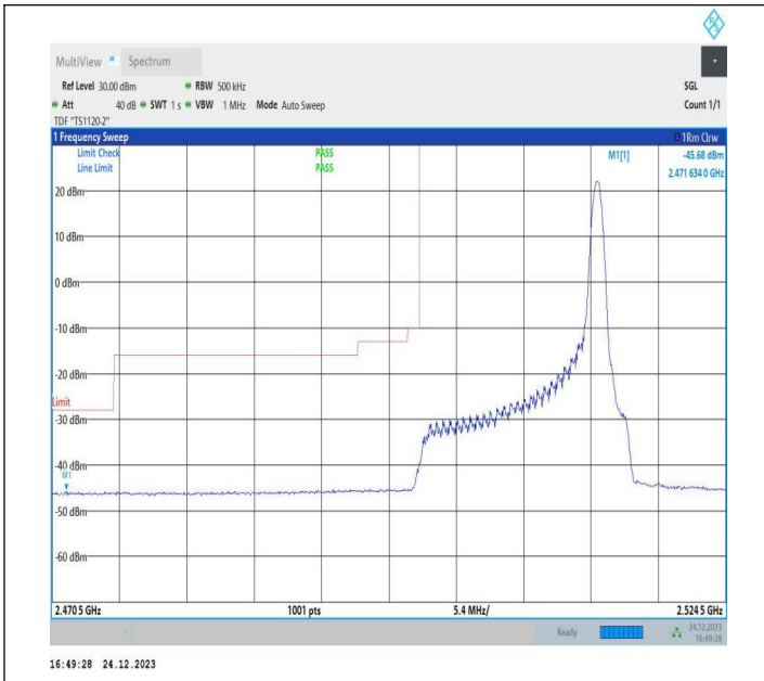
15MHz-10MHz_16QAM@16QAM-16QAM@16QAM_20825-20945_1RB#74@75RB#0-0RB#0@50RB#0
