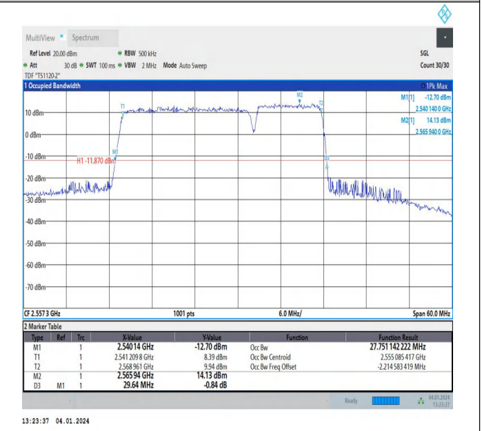
7-7-20MHz-10MHz-64QAM-64QAM-21251-21395-100RB#0-5 0RB#0-PASS
