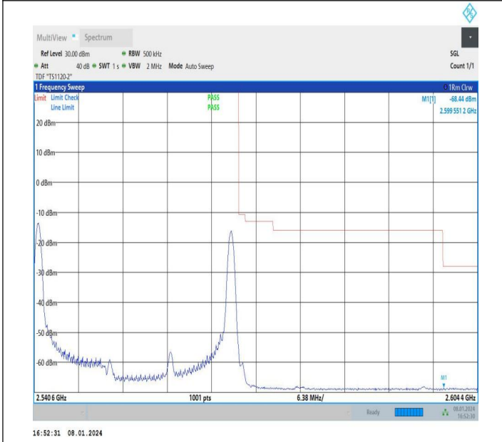
10MHz-20MHz_16QAM@16QAM-16QAM@16QAM_21206-21350_1RB#0@50RB#0-1RB#99@100RB#0
