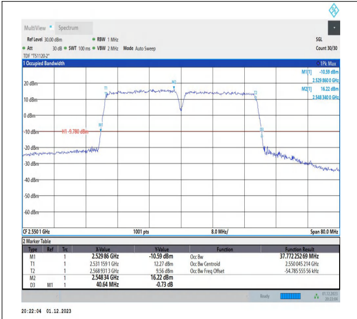
7-7-20MHz-20MHz-16QAM-16QAM-21152-21350-100RB#0-10 ORB#0-PASS
