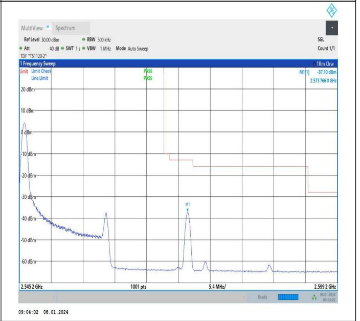
15MHz-10MHz_QPSK@QPSK-QPSK@QPSK_21277-21397_1RB#0@75RB#0-0RB#0@50RB#0
