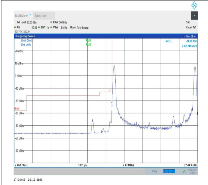
15MHz-20MHz_16QAM@16QAM-16QAM@16QAM_20828-20999_1RB#0@75RB#0-1RB#99@100RB#0
