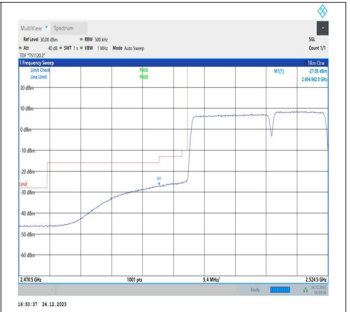
15MHz-10MHz_QPSK@QPSK-QPSK@QPSK_20825-20945_75RB#0@75RB#0-50RB#0@50RB#0
