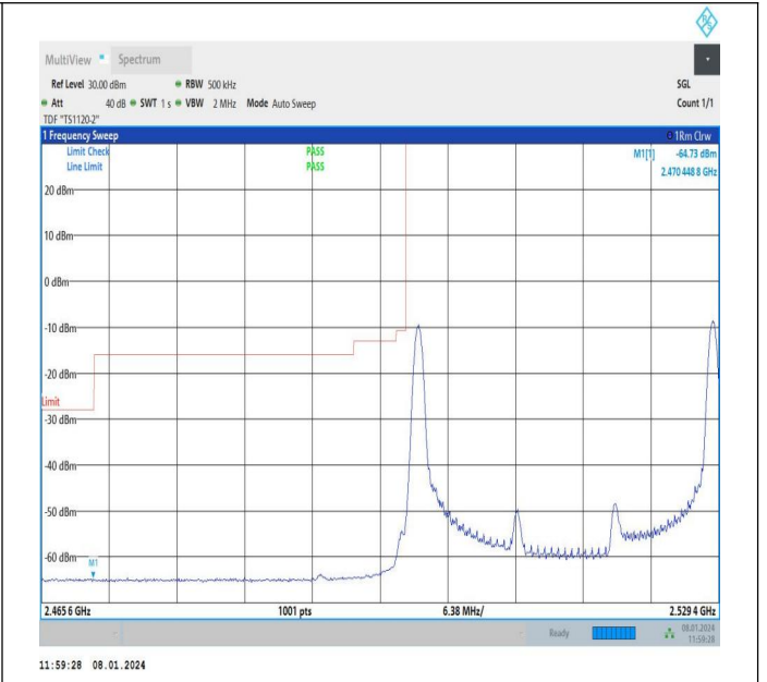
20MHz-10MHz_64QAM@64QAM-64QAM@64QAM_20850-20994_1RB#0@100RB#0-1RB#49@50RB#0
