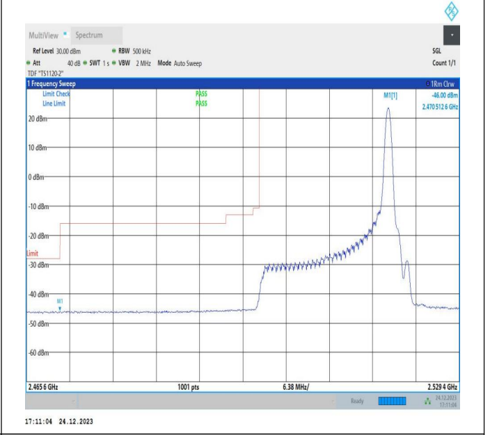
20MHz-10MHz_QPSK@QPSK-QPSK@QPSK_20850-20994_1RB#99@100RB#0-0RB#0@50RB#0
