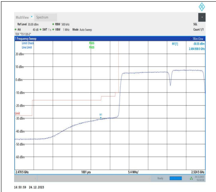
15MHz-10MHz_16QAM@16QAM-16QAM@16QAM_20825-20945_75RB#0@75RB#0-50RB#0@50RB#0
