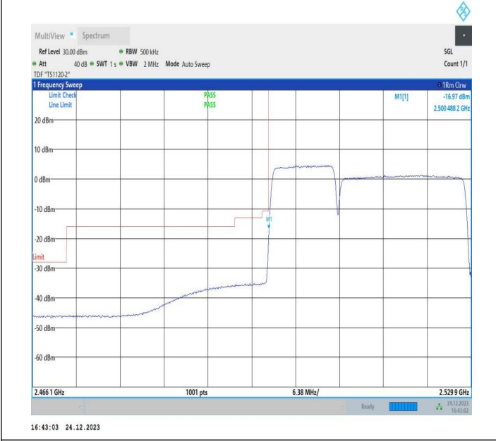
10MHz-20MHz_16QAM@16QAM-16QAM@16QAM_20805-20949_50RB#0@50RB#0-100RB#0@100RB#0
