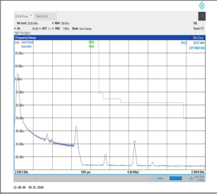
15MHz-5MHz_QPSK@QPSK-QPSK@QPSK_21327-21420_1 RB#0@75RB#0-0RB#0@25RB#0
