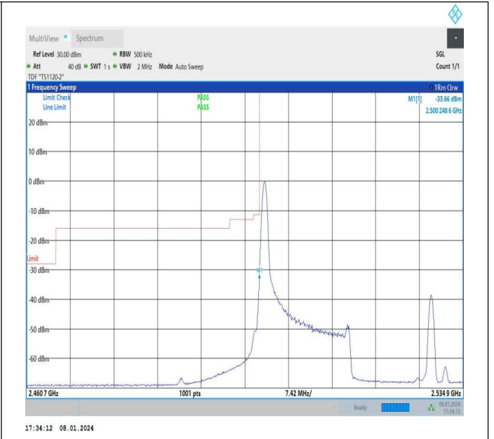
15MHz-20MHz_QPSK@QPSK-QPSK@QPSK_20828-20999 _1RB#0@75RB#0-0RB#0@100RB#0
