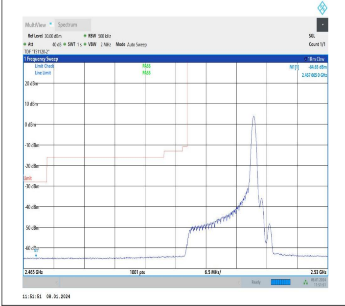
15MHz-15MHz_QPSK@QPSK-QPSK@QPSK_20825-20975_1 RB#74@75RB#0-0RB#0@75RB#0
