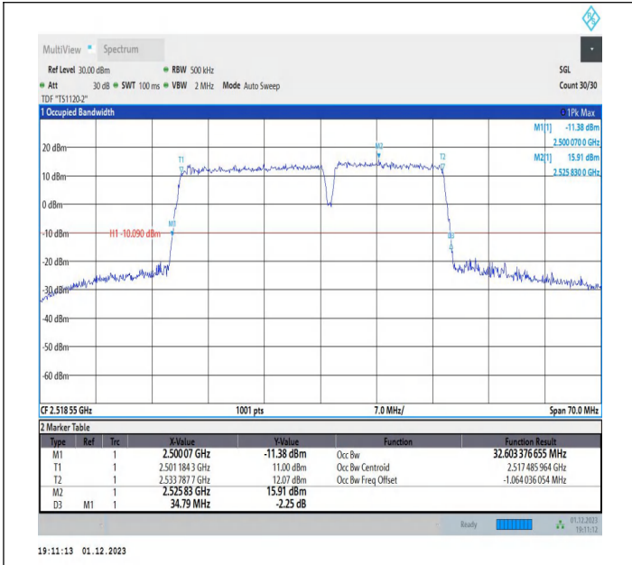
7-7-20MHz-15MHz-QPSK-QPSK-20850-21021-100RB#0-75R B#0-PASS
