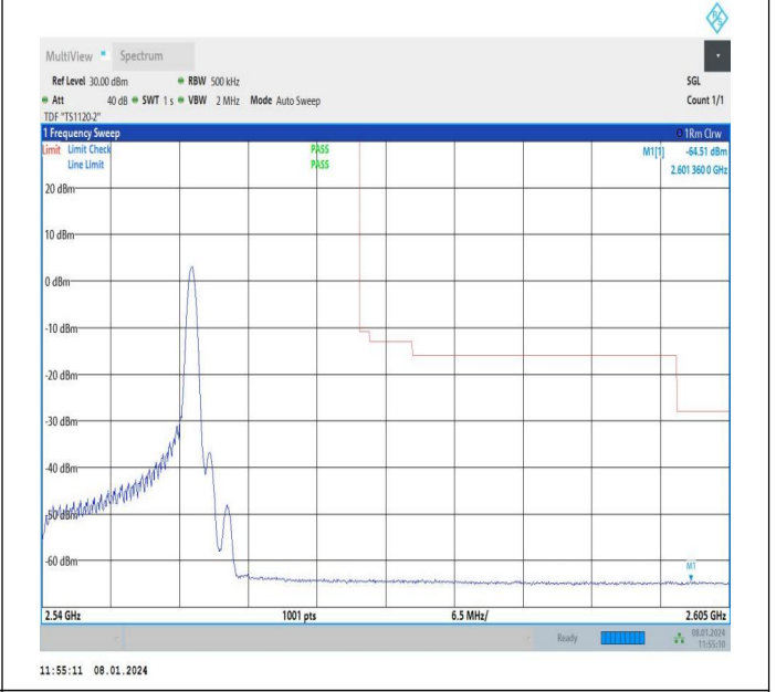
15MHz-15MHz_16QAM@16QAM-16QAM@16QAM_21225-1375_1RB#74@75RB#0-0RB#0@75RB#0
