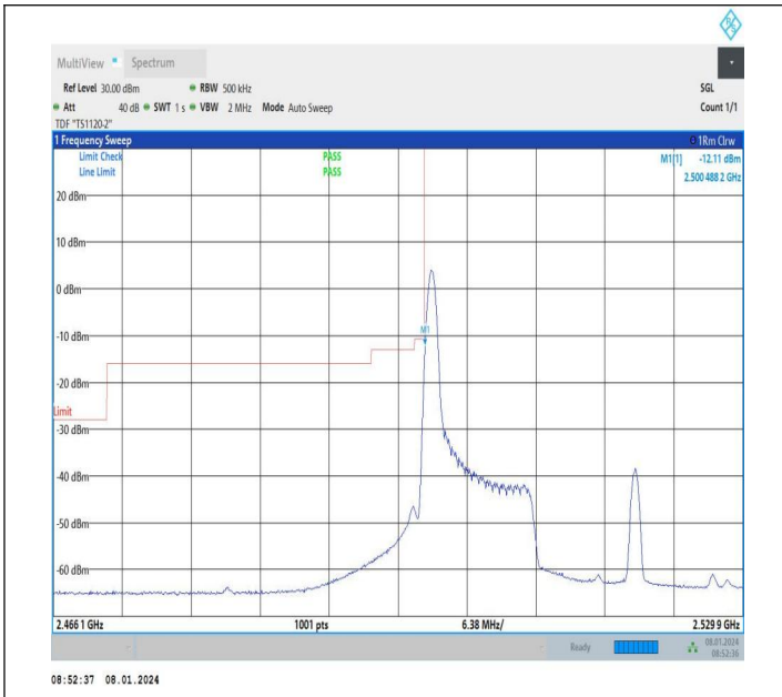
10MHz-20MHz_QPSK@QPSK-QPSK@QPSK_20805-20949_1 RB#0@50RB#0-0RB#0@100RB#0
