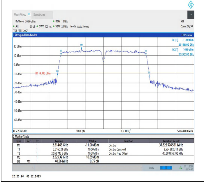
7-7-20MHz-20MHz-16QAM-16QAM-21001-21199-100RB#0-10 0RB#0-PASS
