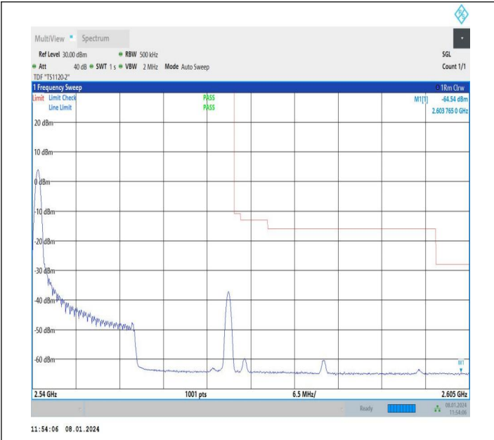
15MHz-15MHz_QPSK@QPSK-QPSK@QPSK_21225-21375_1 RB#0@75RB#0-0RB#0@75RB#0
