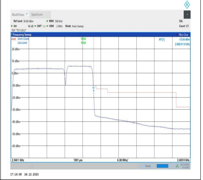
20MHz-10MHz_QPSK@QPSK-QPSK@QPSK_21251-21395_100RB#0@100RB#0-50RB#0@50RB#0
