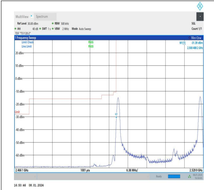
10MHz-20MHz_16QAM@16QAM-16QAM@16QAM_20805-20949_1RB#0@50RB#0-1RB#99@100RB#0
