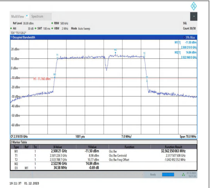
7-7-20MHz-15MHz-16QAM-16QAM-20850-21021-100RB#0-7 5RB#0-PASS
