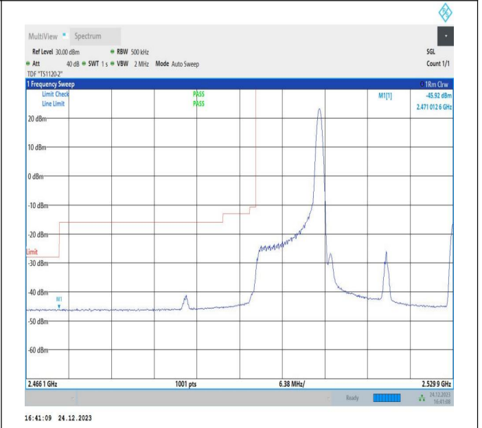
10MHz-20MHz_QPSK@QPSK-QPSK@QPSK_20805-20949_1RB#49@50RB#0-0RB#0@100RB#0
