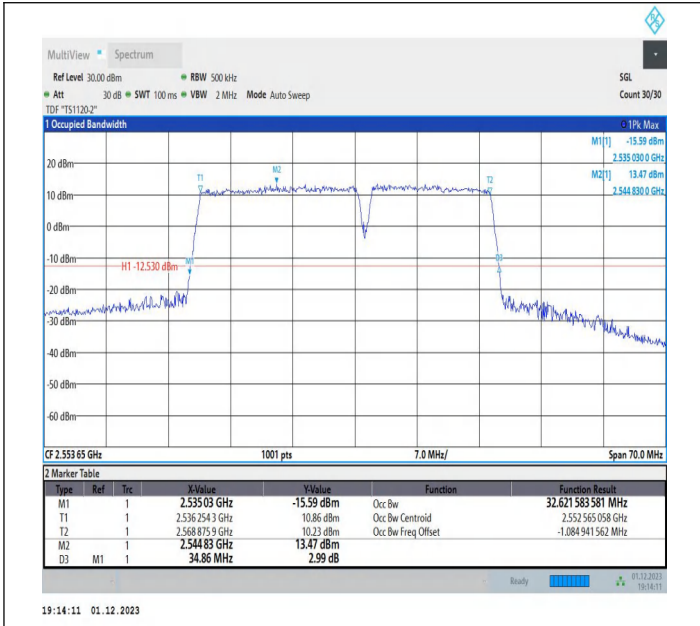
7-7-20MHz-15MHz-16QAM-16QAM-21201-21372-100RB#0-7 5RB#0-PASS
