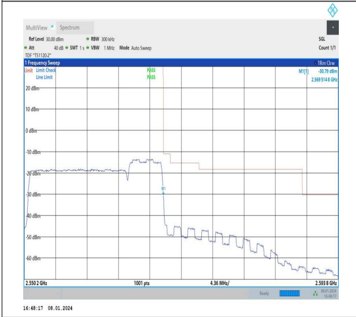
15MHz-5MHz_QPSK@QPSK-QPSK@QPSK_21327-21420_75 RB#0@75RB#0-25RB#0@25RB#0
