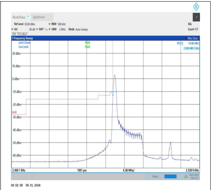
10MHz-20MHz_16QAM@16QAM-16QAM@16QAM_20805-20949_1RB#0@50RB#0-0RB#0@100RB#0
