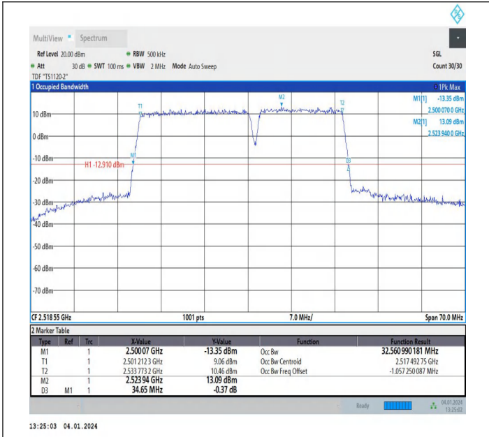
7-7-20MHz-15MHz-64QAM-64QAM-20850-21021-100RB#0-7 5RB#0-PASS
