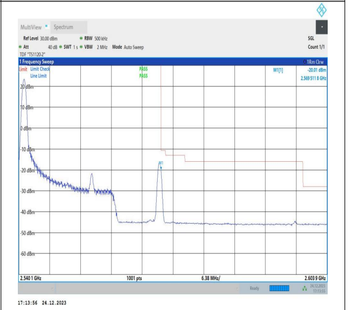
20MHz-10MHz_QPSK@QPSK-QPSK@QPSK_21251-21395_1RB#0@100RB#0-0RB#0@50RB#0
