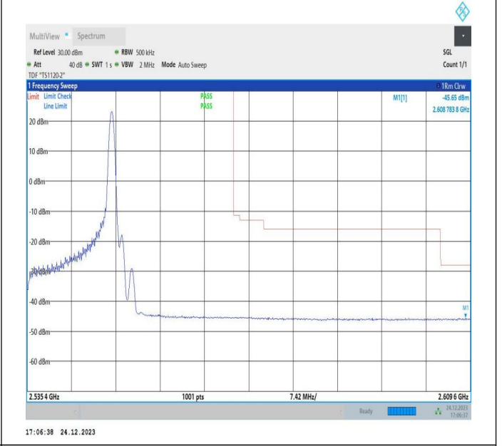
15MHz-20MHz_QPSK@QPSK-QPSK@QPSK_21179-21350_1RB#74@75RB#0-0RB#0@100RB#0
