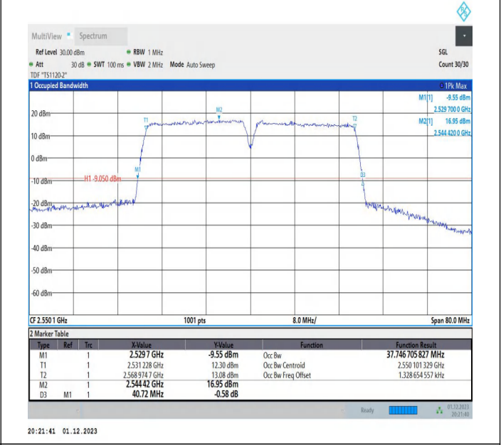
7-7-20MHz-20MHz-QPSK-QPSK-21152-21350-100RB#0-100 RB#0-PASS
