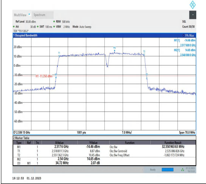
7-7-20MHz-15MHz-16QAM-16QAM-21026-21197-100RB#0-75 RB#0-PASS
