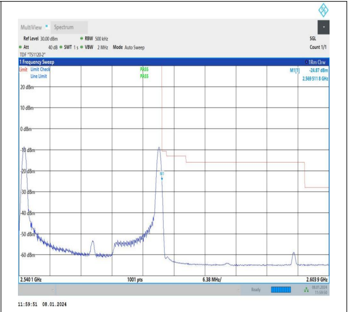
20MHz-10MHz_QPSK@QPSK-QPSK@QPSK_21251-21395_1RB#0@100RB#0-1RB#49@50RB#0
