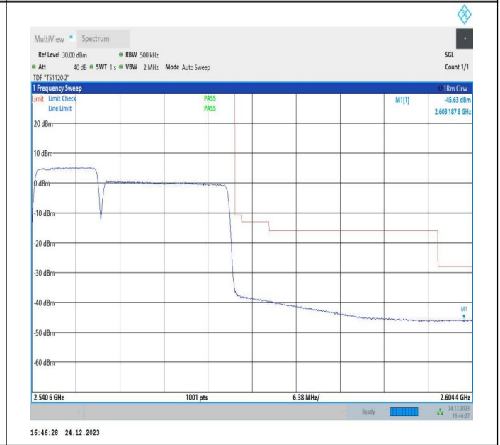
10MHz-20MHz_16QAM@16QAM-16QAM@16QAM_21206-21350_50RB#0@50RB#0-100RB#0@100RB#0
