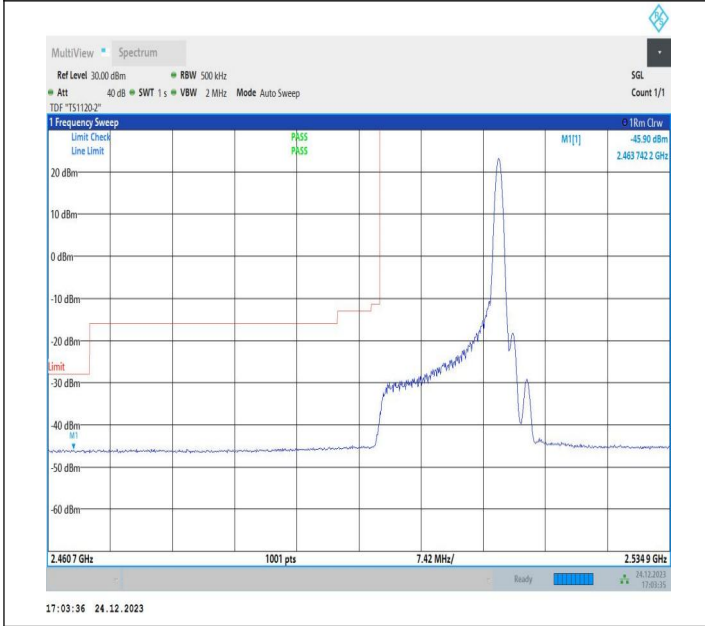
15MHz-20MHz_QPSK@QPSK-QPSK@QPSK_20828-20999_1 RB#74@75RB#0-0RB#0@100RB#0
