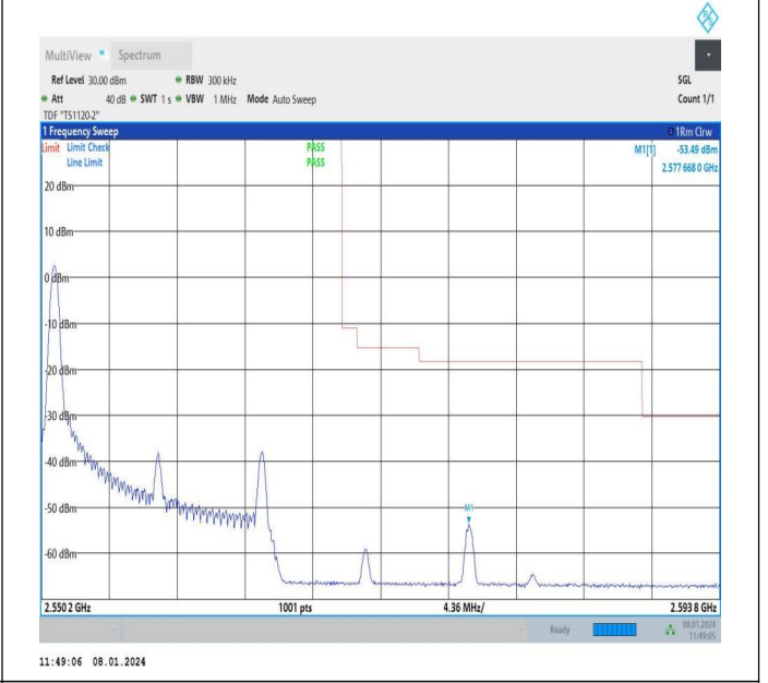
15MHz-5MHz_16QAM@16QAM-16QAM@16QAM_21327-21420_1RB#0@75RB#0-0RB#0@25RB#0
