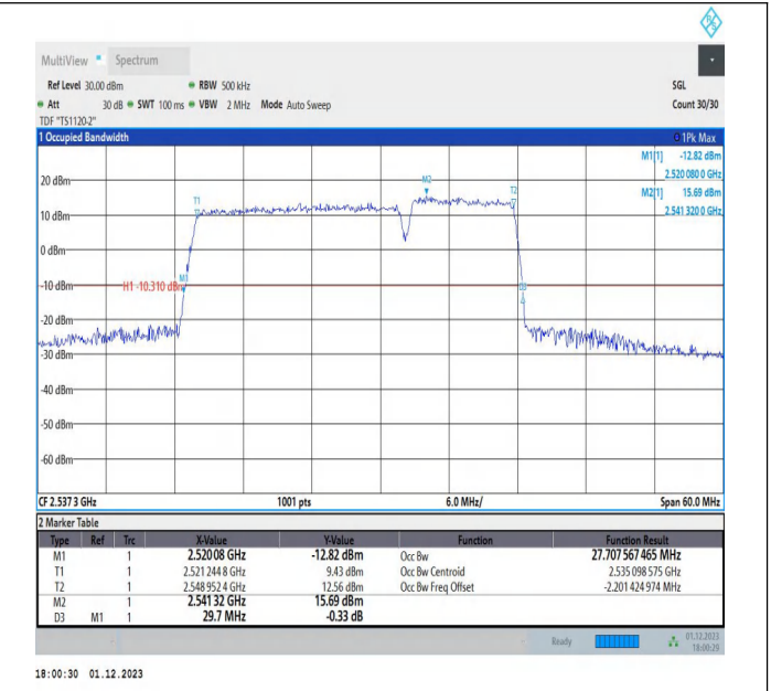
7-7-20MHz-10MHz-16QAM-16QAM-21051-21195-100RB#0-50 RB#0-PASS
