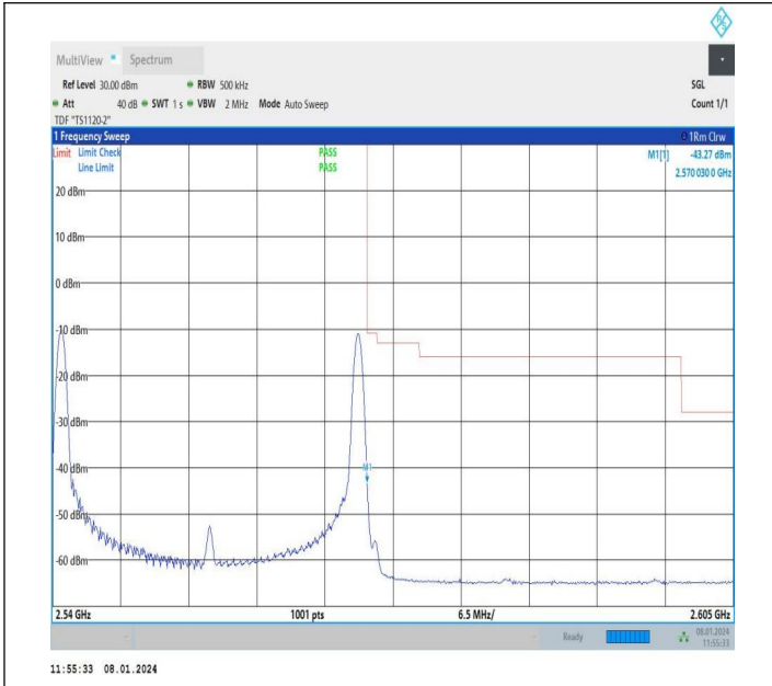
15MHz-15MHz_QPSK@QPSK-QPSK@QPSK_21225-21375_1 RB#0@75RB#0-1RB#74@75RB#0
