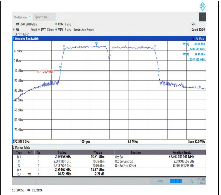
7-7-20MHz-20MHz-64QAM-64QAM-20850-21048-100RB#0-1 00RB#0-PASS
