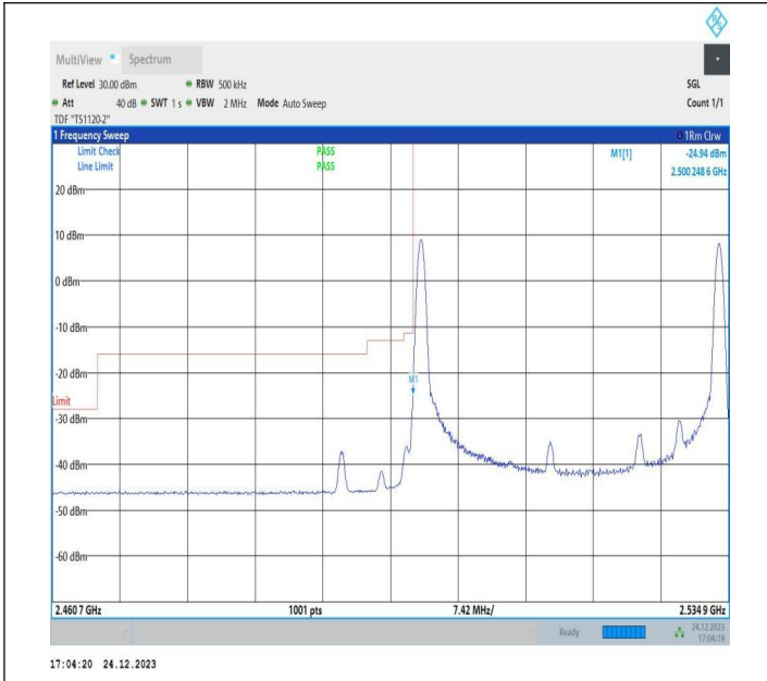
15MHz-20MHz_QPSK@QPSK-QPSK@QPSK_20828-20999_1 RB#0@75RB#0-1RB#99@100RB#0
