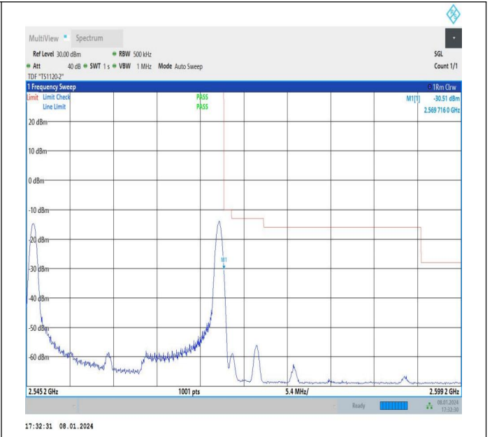
15MHz-10MHz_16QAM@16QAM-16QAM@16QAM_21277-21397_1 RB#0@75RB#0-1RB#49@50RB#0
