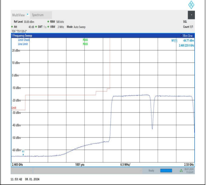
15MHz-15MHz_16QAM@16QAM-16QAM@16QAM_20825-0975_75RB#0@75RB#0-75RB#0@75RB#0
