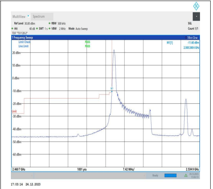
15MHz-20MHz_16QAM@16QAM-16QAM@16QAM_20828-20999_1RB#0@75RB#0-0RB#0@100RB#0
