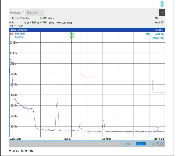
10MHz-20MHz_QPSK@QPSK-QPSK@QPSK_21206-21350_1RB#0@50RB#0-0RB#0@100RB#0
