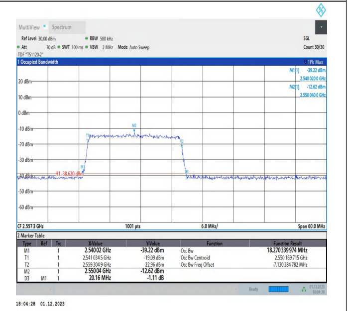
7-7-20MHz-10MHz-16QAM-16QAM-21251-21395-100RB#0-50 ORB#0-PASS
