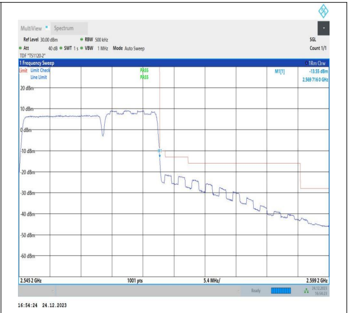
15MHz-10MHz_QPSK@QPSK-QPSK@QPSK_21277-21397_75RB#0@75RB#0-50RB#0@50RB#0
