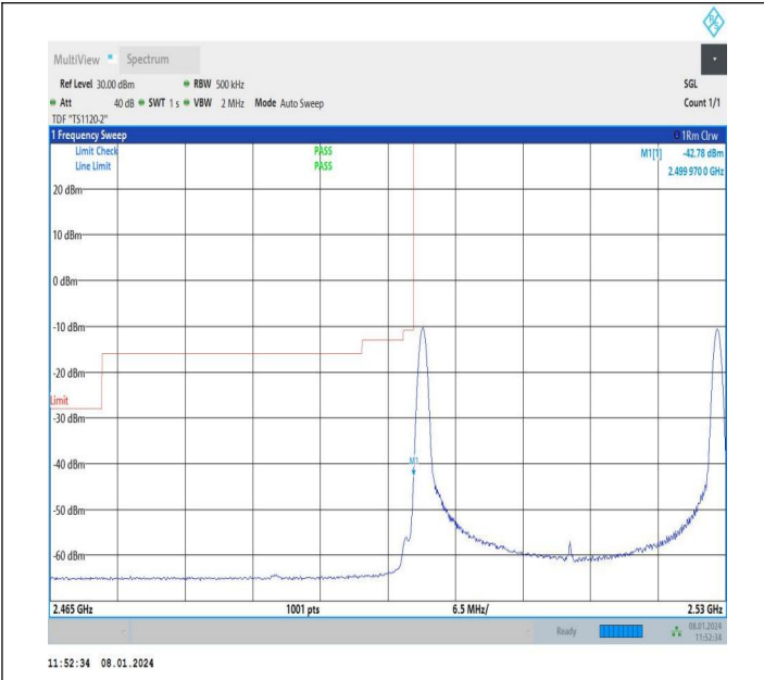
15MHz-15MHz_QPSK@QPSK-QPSK@QPSK_20825-20975_1 RB#0@75RB#0-1RB#74@75RB#0
