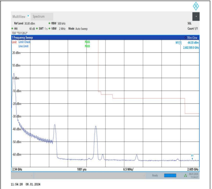
15MHz-15MHz_16QAM@16QAM-16QAM@16QAM_21225-1375_1RB#0@75RB#0-0RB#0@75RB#0
