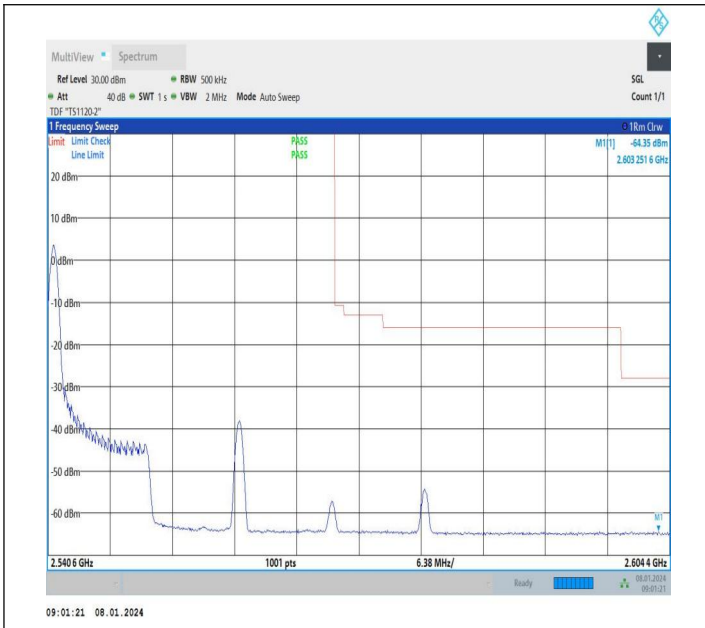
10MHz-20MHz_16QAM@16QAM-16QAM@16QAM_21206-21350_1RB#0@50RB#0-0RB#0@100RB#0
