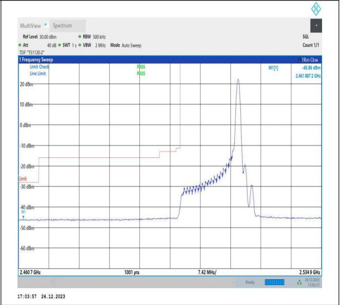
15MHz-20MHz_16QAM@16QAM-16QAM@16QAM_20828-20999_1RB#74@75RB#0-0RB#0@100RB#0
