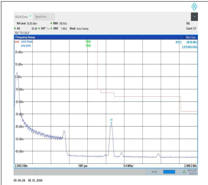
15MHz-10MHz_16QAM@16QAM-16QAM@16QAM_21277-21397_1RB#0@75RB#0-0RB#0@50RB#0
