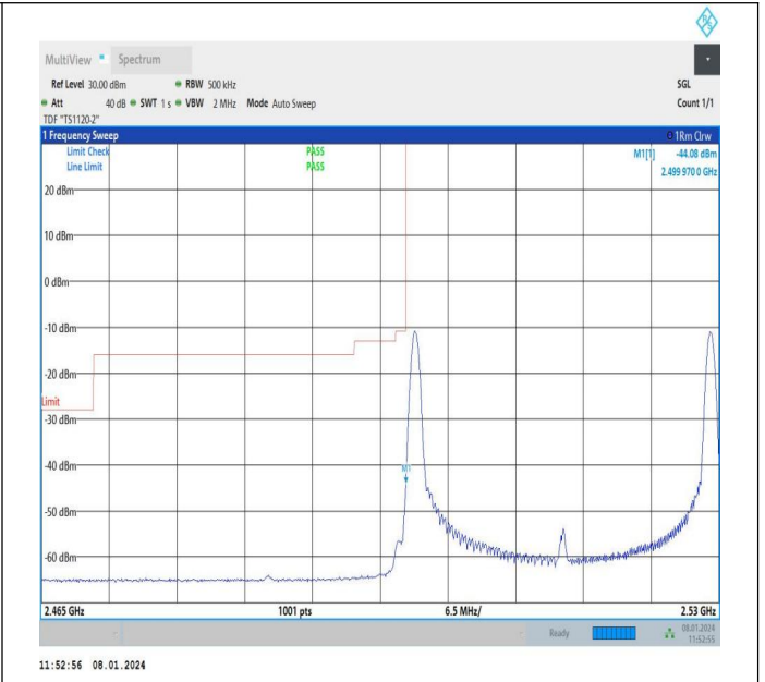
15MHz-15MHz_16QAM@16QAM-16QAM@16QAM_20825-0975_1RB#0@75RB#0-1RB#74@75RB#0
