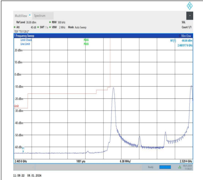
20MHz-10MHz_16QAM@16QAM-16QAM@16QAM_20850-20994_1RB#0@100RB#0-1RB#49@50RB#0
