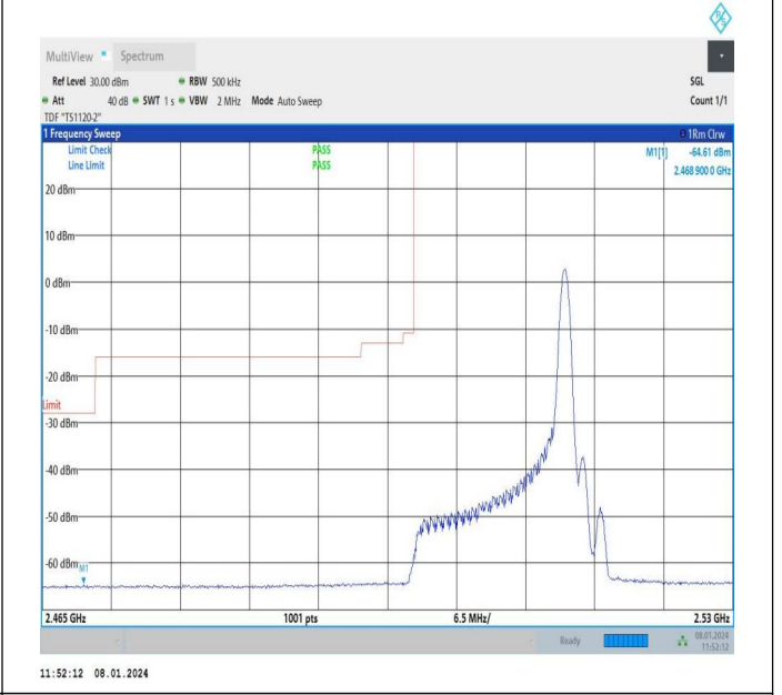
15MHz-15MHz_16QAM@16QAM-16QAM@16QAM_20825-20975_1 RB#74@75RB#0-0RB#0@75RB#0
