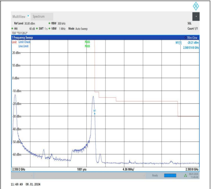
15MHz-5MHz_16QAM@16QAM-16QAM@16QAM_21327-21420_1RB#0@75RB#0-1RB#24@25RB#0
