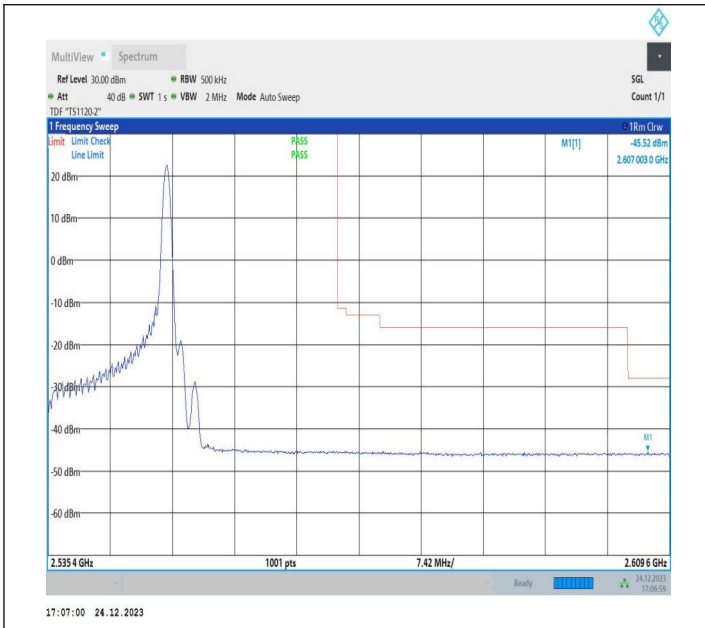
15MHz-20MHz_16QAM@16QAM-16QAM@16QAM_21179-21350_1RB#74@75RB#0-0RB#0@100RB#0
