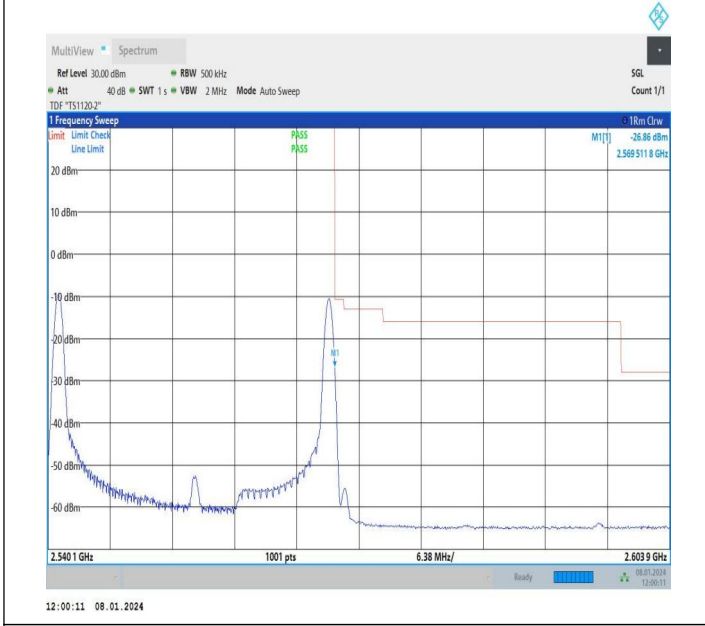
20MHz-10MHz_16QAM@16QAM-16QAM@16QAM_21251-21395_1RB#0@100RB#0-1RB#49@50RB#0
