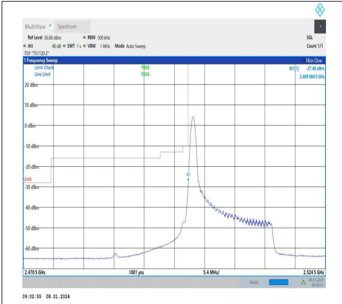
15MHz-10MHz_QPSK@QPSK-QPSK@QPSK_20825-20945_1 RB#0@75RB#0-0RB#0@50RB#0
