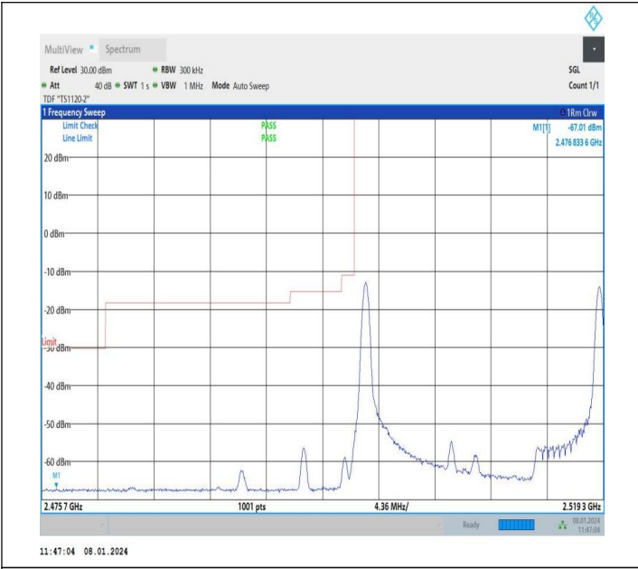
15MHz-5MHz_QPSK@QPSK-QPSK@QPSK_20825-20918_1 RB#0@75RB#0-1RB#24@25RB#0
