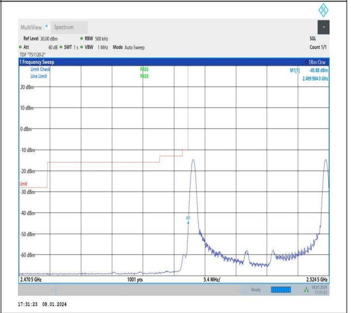
15MHz-10MHz_16QAM@16QAM-16QAM@16QAM_20825-20945_1RB#0@75RB#0-1RB#49@50RB#0
