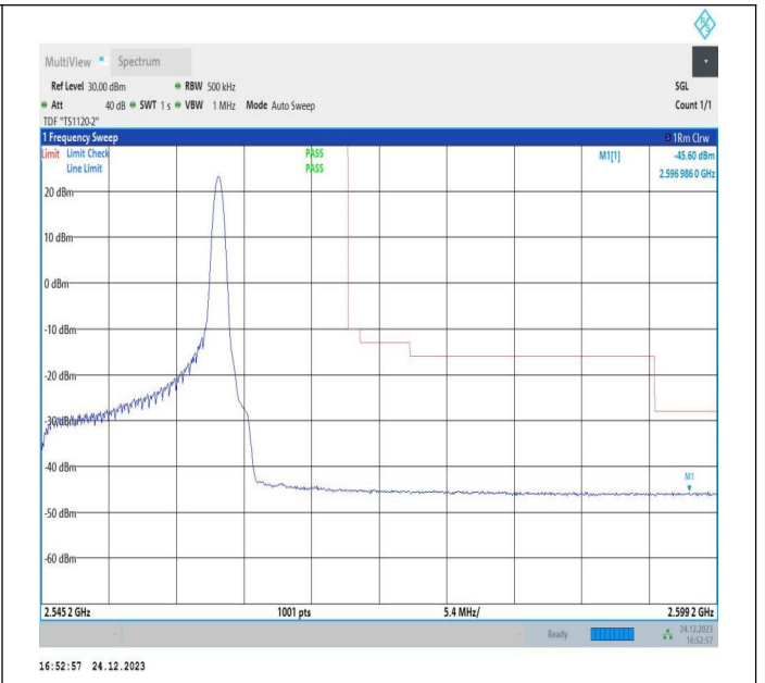
15MHz-10MHz_QPSK@QPSK-QPSK@QPSK_21277-21397_1RB#74@75RB#0-0RB#0@50RB#0
