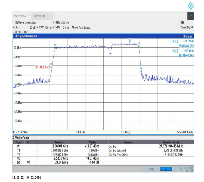
7-7-20MHz-10MHz-64QAM-64QAM-20850-20994-100RB#0-5 ORB#0-PASS
