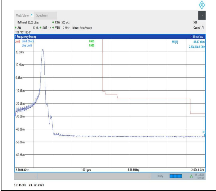
10MHz-20MHz_16QAM@16QAM-16QAM@16QAM_21206-21350_1RB#49@50RB#0-0RB#0@100RB#0
