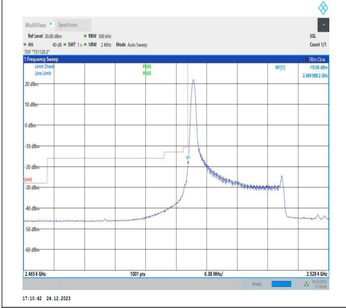
20MHz-10MHz_16QAM@16QAM-16QAM@16QAM_20850-20994_994_1RB#0@100RB#0-0RB#0@50RB#0
