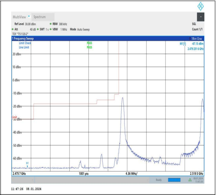
15MHz-5MHz_16QAM@16QAM-16QAM@16QAM_20825-20918_1 RB#0@75RB#0-1RB#24@25RB#0
