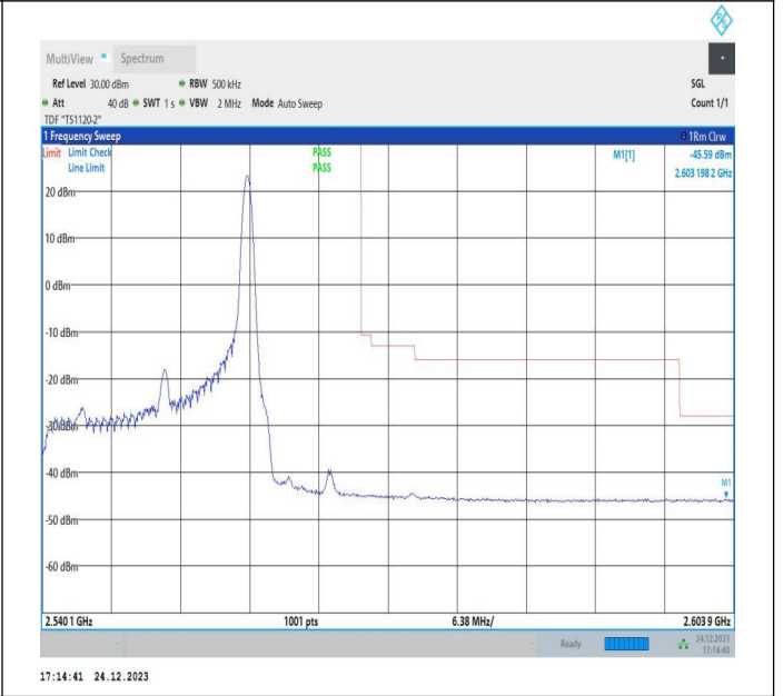
20MHz-10MHz_QPSK@QPSK-QPSK@QPSK_21251-21395_1RB#99@100RB#0-0RB#0@50RB#0
