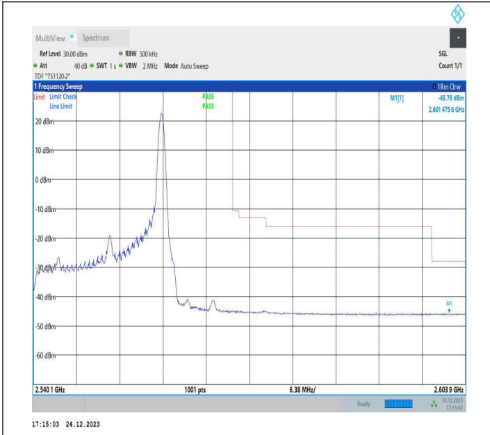
20MHz-10MHz_16QAM@16QAM-16QAM@16QAM_21251-21395_1RB#99@100RB#0-0RB#0@50RB#0
