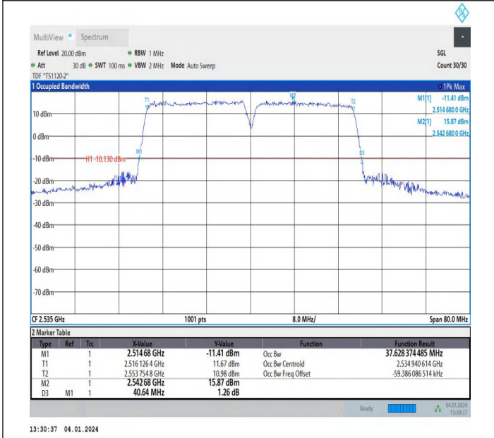
7-7-20MHz-20MHz-64QAM-64QAM-21001-21199-100RB#0-10 ORB#0-PASS
