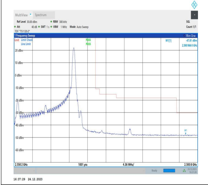
15MHz-5MHz_16QAM@16QAM-16QAM@16QAM_21327-21420_1RB#74@75RB#0-0RB#0@25RB#0
