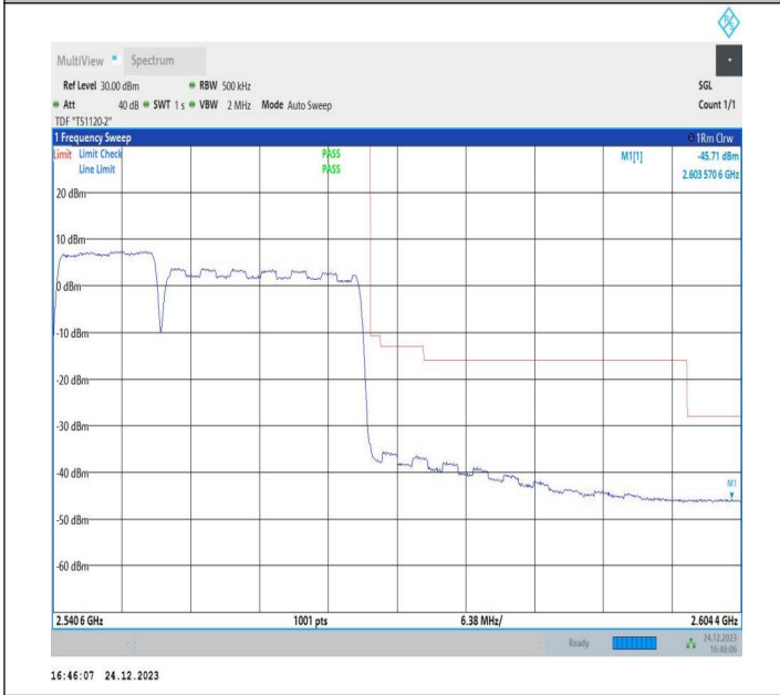
10MHz-20MHz_QPSK@QPSK-QPSK@QPSK_21206-21350_5_0RB#0@50RB#0-100RB#0@100RB#0
