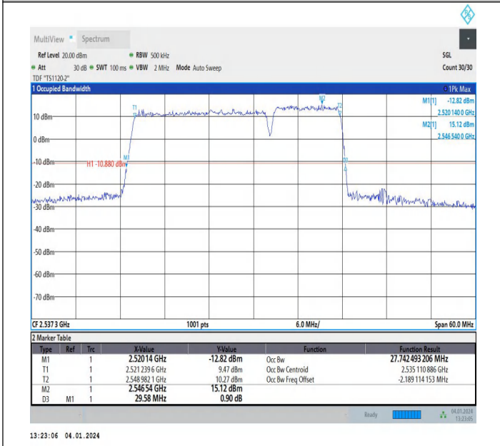
7-7-20MHz-10MHz-64QAM-64QAM-21051-21195-100RB#0-50 RB#0-PASS
