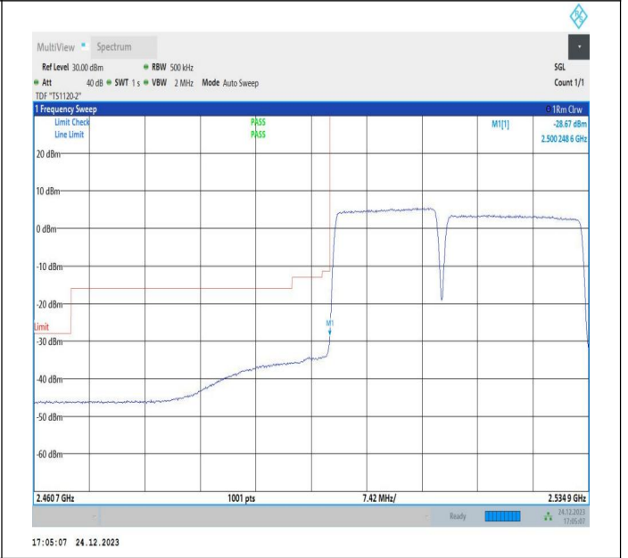
15MHz-20MHz_QPSK@QPSK-QPSK@QPSK_20828-20999_75RB#0@75RB#0-100RB#0@100RB#0
