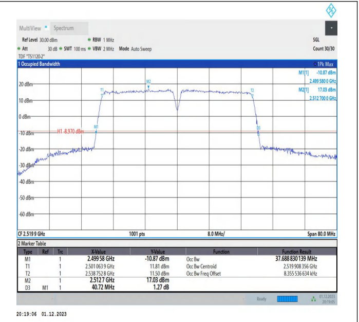
7-7-20MHz-20MHz-QPSK-QPSK-20850-21048-100RB#0-100 RB#0-PASS
