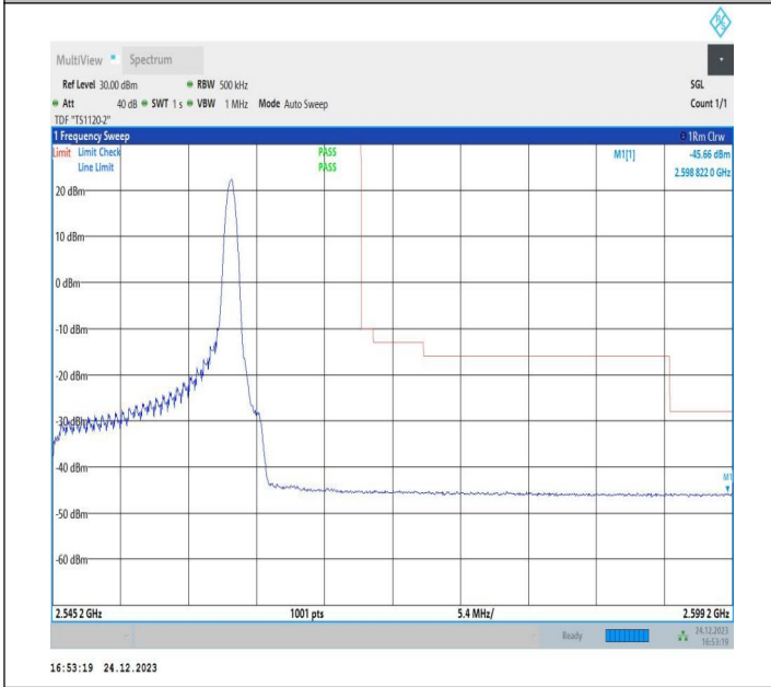
15MHz-10MHz_16QAM@16QAM-16QAM@16QAM_21277-21397_1RB#74@75RB#0-0RB#0@50RB#0
