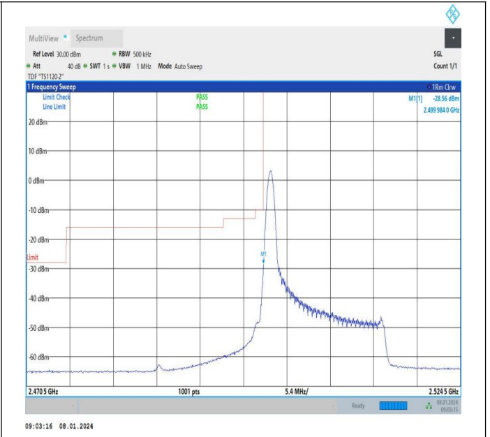
15MHz-10MHz_16QAM@16QAM-16QAM@16QAM_20825-0945_1RB#0@75RB#0-0RB#0@50RB#0
