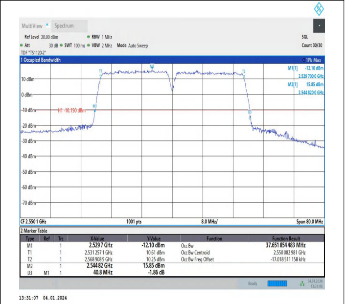
7-7-20MHz-20MHz-64QAM-64QAM-21152-21350-100RB#0-10 ORB#0-PASS
