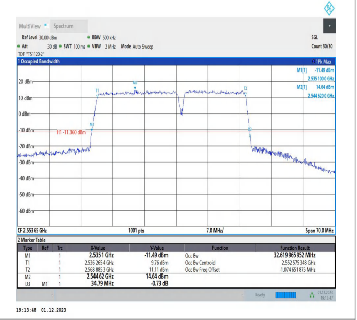
7-7-20MHz-15MHz-QPSK-QPSK-21201-21372-100RB#0-75R B#0-PASS
