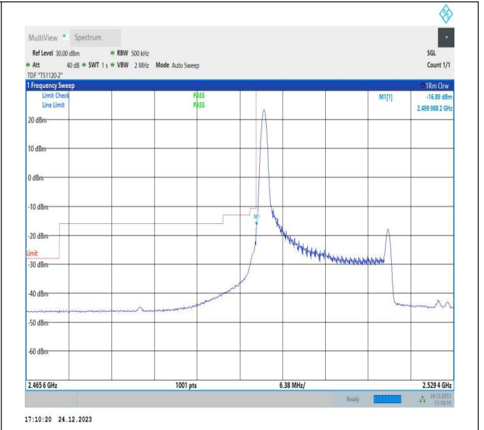
20MHz-10MHz_QPSK@QPSK-QPSK@QPSK_20850-20994_1RB#0@100RB#0-0RB#0@50RB#0
