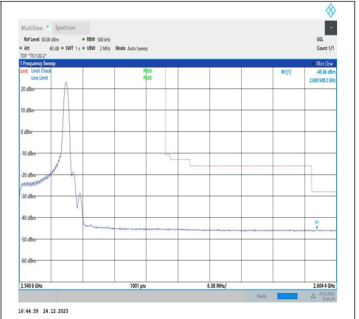
10MHz-20MHz_QPSK@QPSK-QPSK@QPSK_21206-21350_1RB#49@50RB#0-0RB#0@100RB#0
