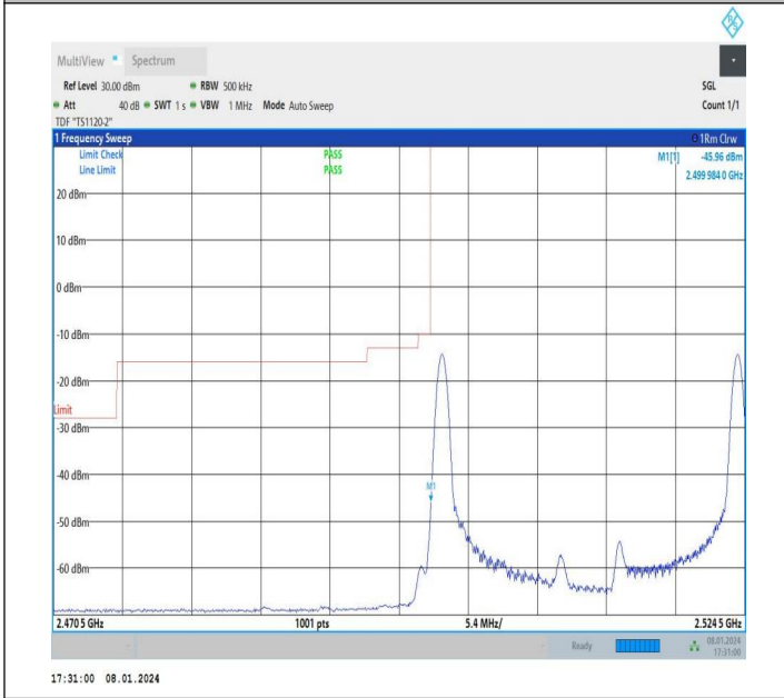
15MHz-10MHz_QPSK@QPSK-QPSK@QPSK_20825-20945_1RB#0@75RB#0-1RB#49@50RB#0
