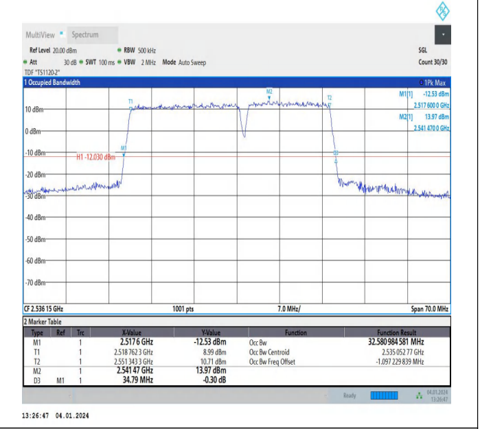
7-7-20MHz-15MHz-64QAM-64QAM-21026-21197-100RB#0-75 RB#0-PASS
