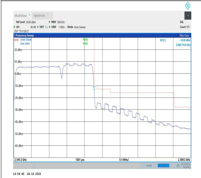
15MHz-10MHz_16QAM@16QAM-16QAM@16QAM_21277-21397_75RB#0@75RB#0-50RB#0@50RB#0
