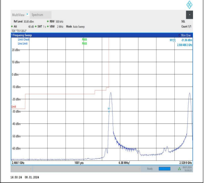
10MHz-20MHz_QPSK@QPSK-QPSK@QPSK_20805-20949_1RB#0@50RB#0-1RB#99@100RB#0
