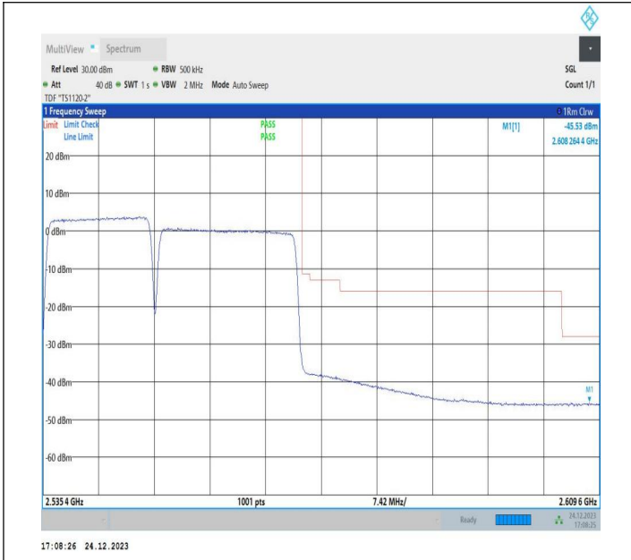
15MHz-20MHz_16QAM@16QAM-16QAM@16QAM_21179-21350_75RB#0@75RB#0-100RB#0@100RB#0
