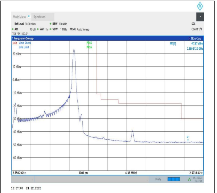
15MHz-5MHz_QPSK@QPSK-QPSK@QPSK_21327-21420_1RB#74@75RB#0-0RB#0@25RB#0
