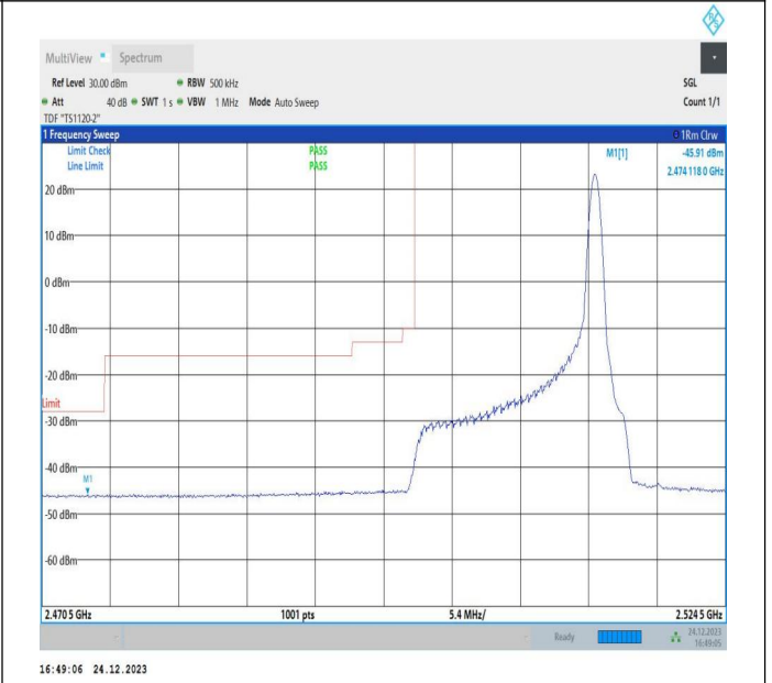
15MHz-10MHz_QPSK@QPSK-QPSK@QPSK_20825-20945_1RB#74@75RB#0-0RB#0@50RB#0
