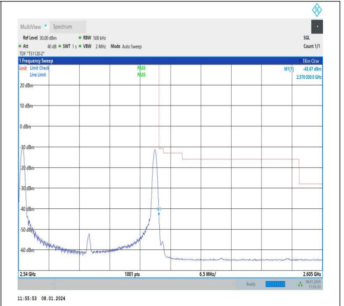
15MHz-15MHz_16QAM@16QAM-16QAM@16QAM_21225-1375_1RB#0@75RB#0-1RB#74@75RB#0
