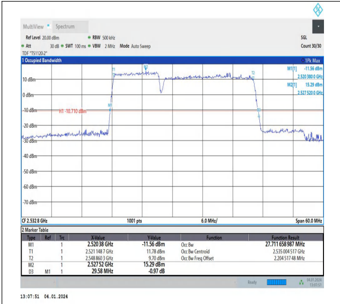
7-7-10MHz-20MHz-64QAM-64QAM-21006-21150-50RB#0-100 RB#0-PASS
