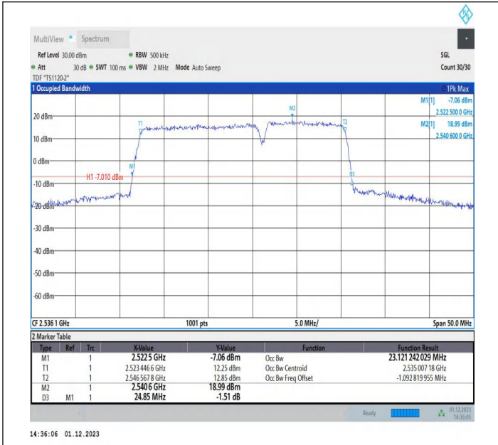
7-7-15MHz-10MHz-16QAM-16QAM-21051-21171-75RB#0-50 RB#0-PASS
