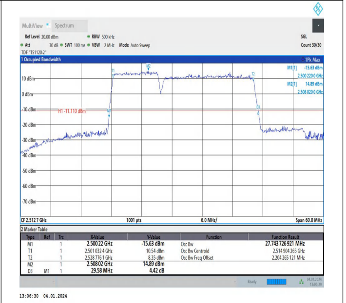
7-7-10MHz-20MHz-64QAM-64QAM-20805-20949-50RB#0-10 ORB#0-PASS
