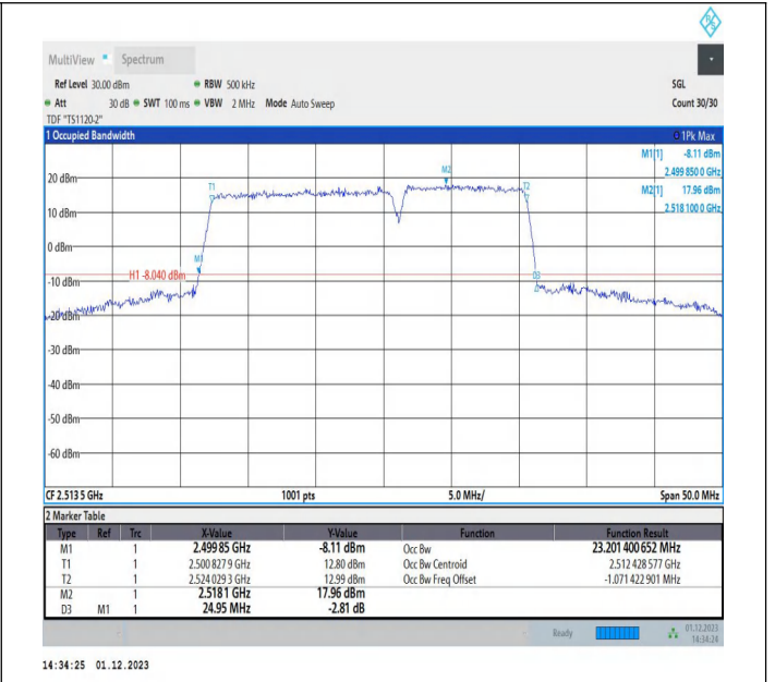
7-7-15MHz-10MHz-QPSK-QPSK-20825-20945-75RB#0-50RB #0-PASS
