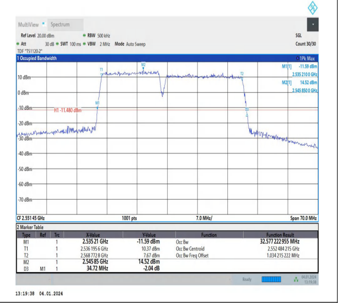
7-7-15MHz-20MHz-64QAM-64QAM-21179-21350-75RB#0-100 RB#0-PASS
