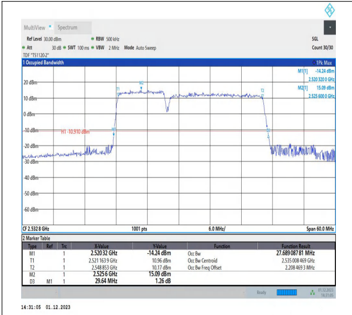
7-7-10MHz-20MHz-16QAM-16QAM-21006-21150-50RB#0-100 RB#0-PASS
