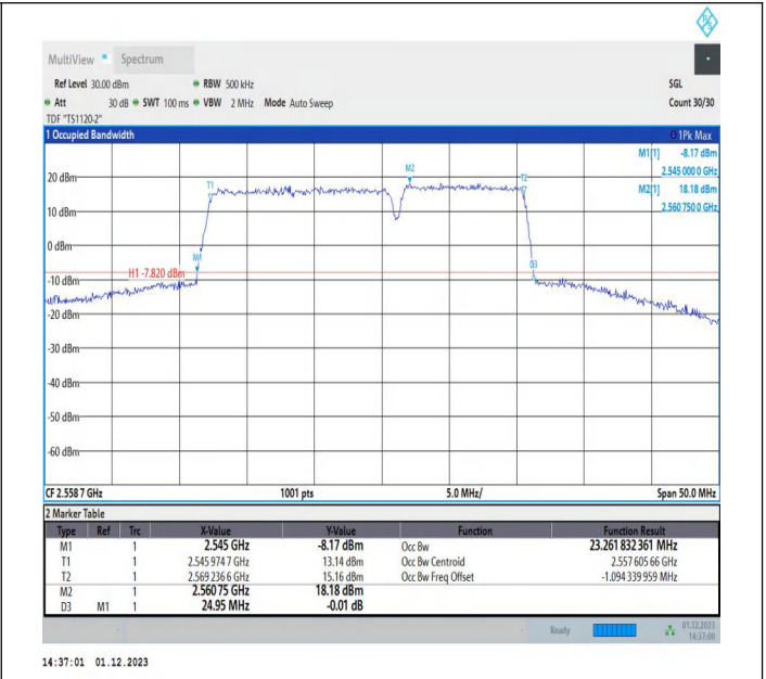
7-7-15MHz-10MHz-QPSK-QPSK-21277-21397-75RB#0-50RB #0-PASS
