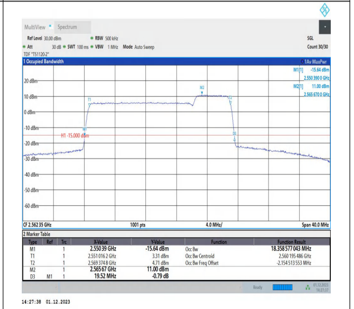
7-7-15MHz-5MHz-16QAM-16QAM-21327-21420-75RB#0-25R B#0-PASS
