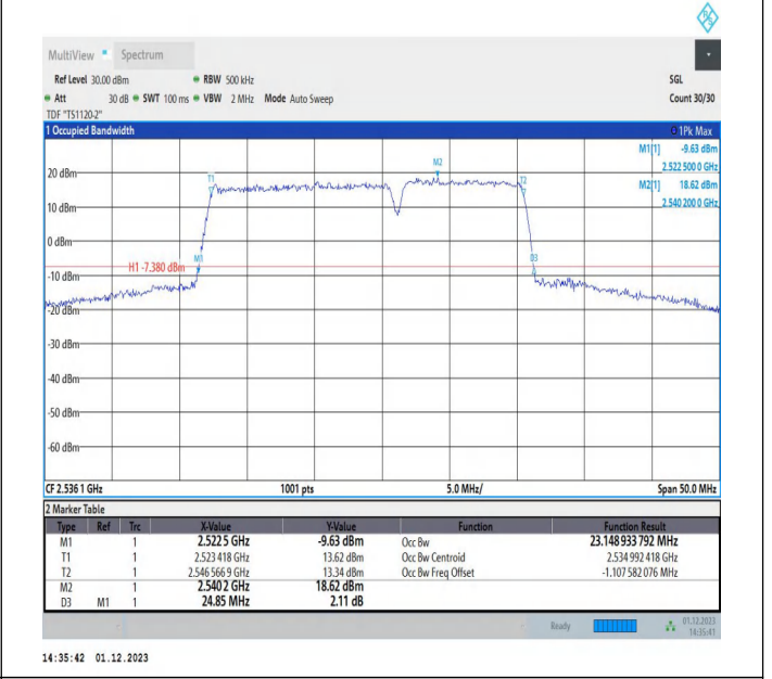
7-7-15MHz-10MHz-QPSK-QPSK-21051-21171-75RB#0-50RB #0-PASS
