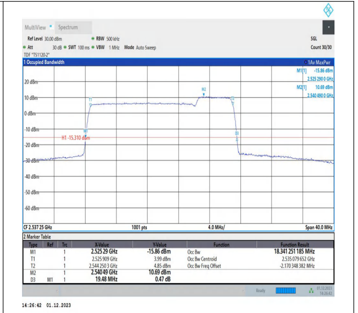
7-7-15MHz-5MHz-64QAM-64QAM-21076-21169-75RB#0-25R B#0-PASS
