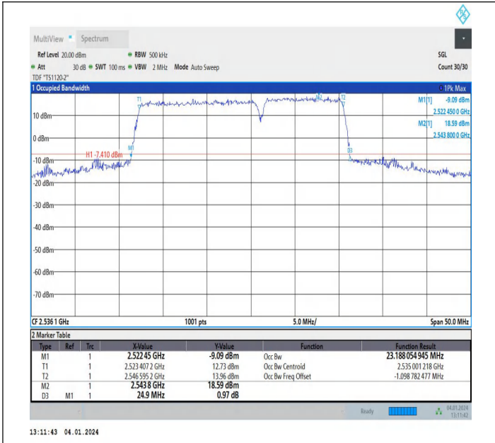
7-7-15MHz-10MHz-64QAM-64QAM-21051-21171-75RB#0-50 RB#0-PASS
