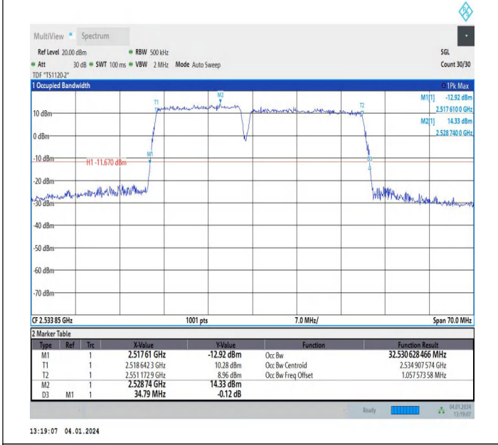
7-7-15MHz-20MHz-64QAM-64QAM-21003-21174-75RB#0-100 RB#0-PASS
