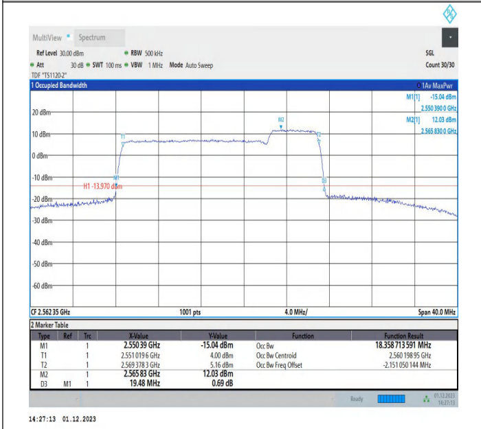
7-7-15MHz-5MHz-QPSK-QPSK-21327-21420-75RB#0-25RB#0-PASS
