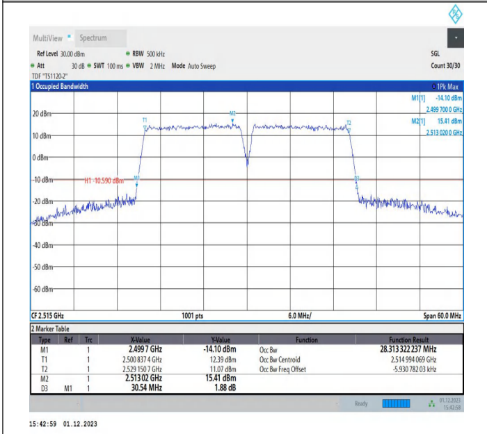
7-7-15MHz-15MHz-QPSK-QPSK-20825-20975-75RB#0-75RB#0-PASS
