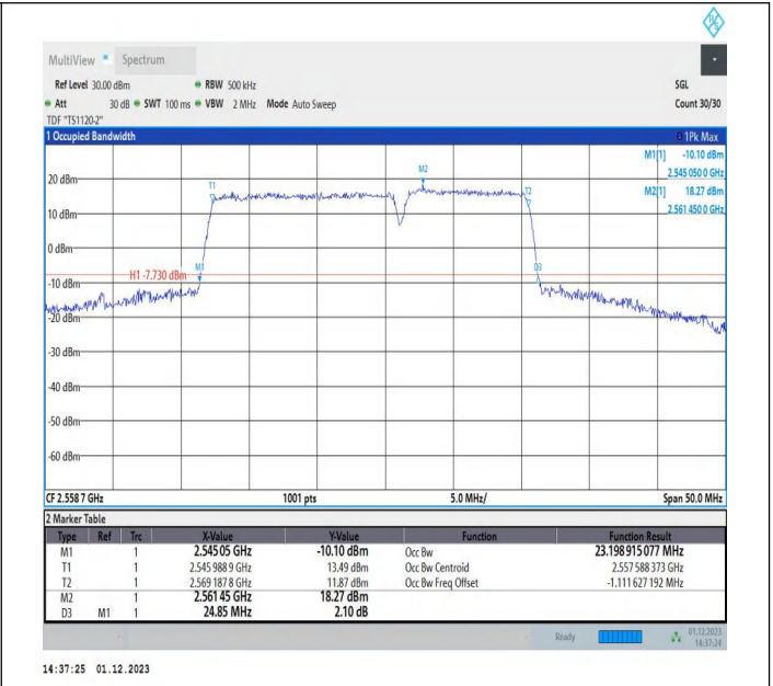
7-7-15MHz-10MHz-16QAM-16QAM-21277-21397-75RB#0-50 RB#0-PASS
