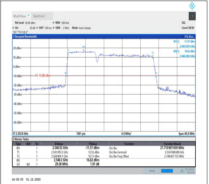
7-7-10MHz-20MHz-QPSK-QPSK-21206-21350-50RB#0-100R B#0-PASS
