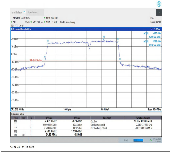
7-7-15MHz-10MHz-16QAM-16QAM-20825-20945-75RB#0-50 RB#0-PASS
