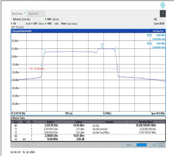
7-7-15MHz-5MHz-16QAM-16QAM-21076-21169-75RB#0-25R B#0-PASS
