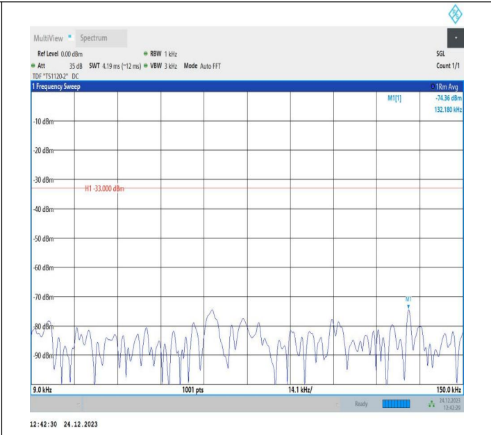
5-5-10MHz-10MHz-QPSK-QPSK-20501-20600-1RB#49-ORB# 0-0.009~0.15MHz-PASS
