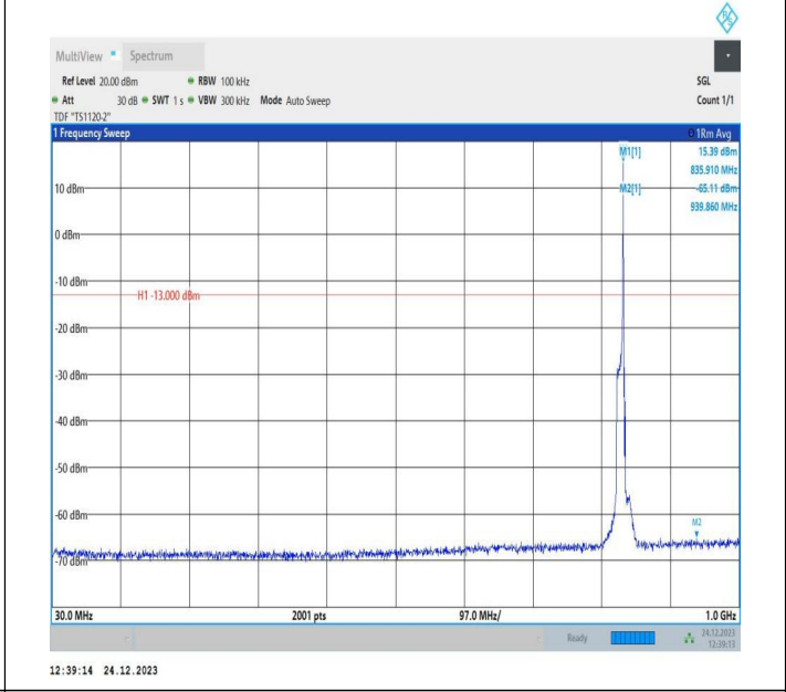
5-5-10MHz-10MHz-QPSK-QPSK-20476-20575-1RB#49-ORB# 0-30~1000MHz-PASS
