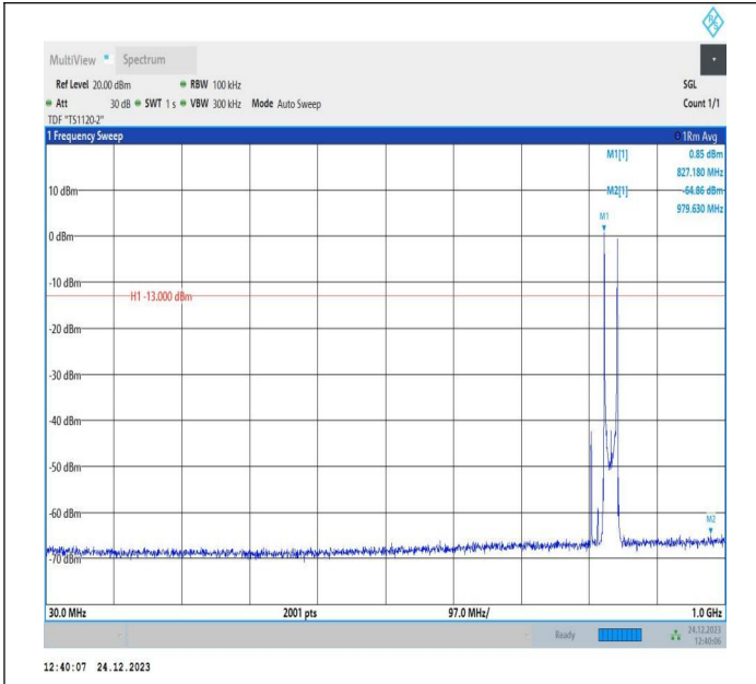
5-5-10MHz-10MHz-QPSK-QPSK-20476-20575-1RB#0-1RB#4 9-30~1000MHz-PASS
