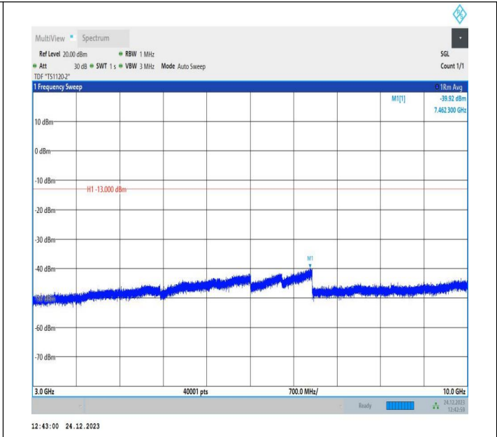
5-5-10MHz-10MHz-QPSK-QPSK-20501-20600-1RB#49-0RB# 0-3000~10000MHz-PASS
