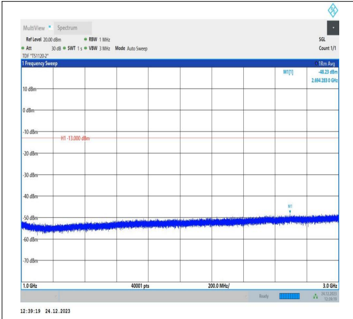
5-5-10MHz-10MHz-QPSK-QPSK-20476-20575-1RB#49-0RB# 0-1000~3000MHz-PASS
