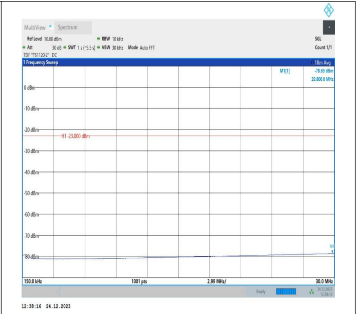
5-5-10MHz-10MHz-QPSK-QPSK-20476-20575-1RB#0-0RB#0 0.15~30MHz-PASS
