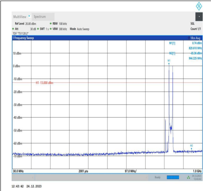
5-5-10MHz-10MHz-QPSK-QPSK-20501-20600-1RB#0-1RB#4 9-30~1000MHz-PASS
