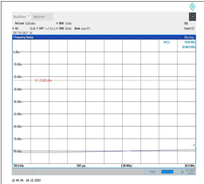
5-5-10MHz-10MHz-QPSK-QPSK-20476-20575-50RB#0-50RB #0-0.15~30MHz-PASS
