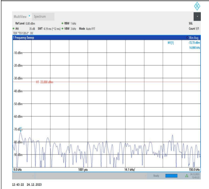
5-5-10MHz-10MHz-QPSK-QPSK-20501-20600-1RB#0-1RB#4 9-0.009~0.15MHz-PASS
