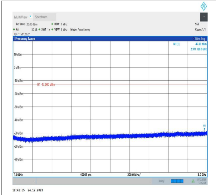
5-5-10MHz-10MHz-QPSK-QPSK-20501-20600-1RB#49-0RB# 0-1000~3000MHz-PASS
