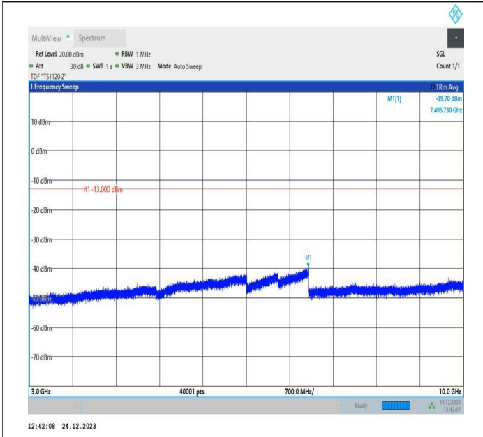
5-5-10MHz-10MHz-QPSK-QPSK-20501-20600-1RB#0-ORB#0 -3000~10000MHz-PASS
