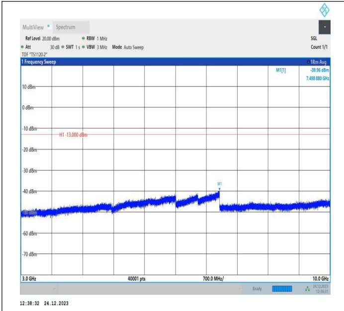
5-5-10MHz-10MHz-QPSK-QPSK-20476-20575-1RB#0-ORB#0 -3000~10000MHz-PASS
