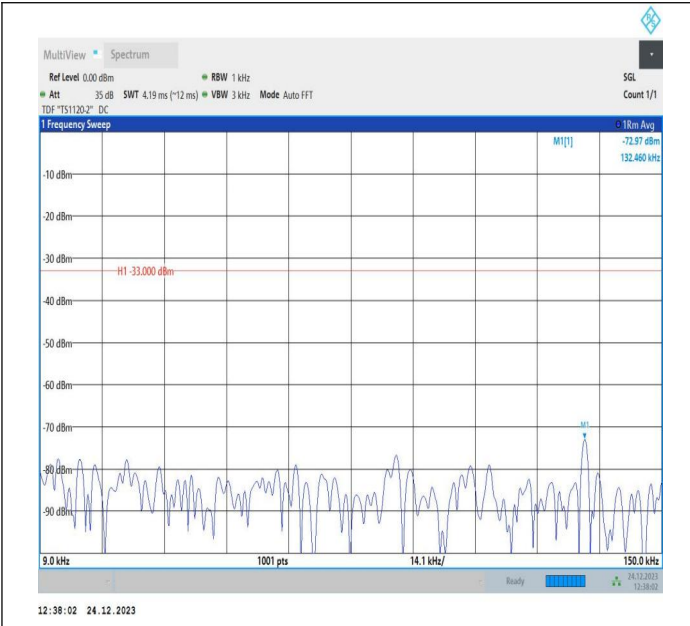
5-5-10MHz-10MHz-QPSK-QPSK-20476-20575-1RB#0-0RB#0 -0.009~0.15MHz-PASS
