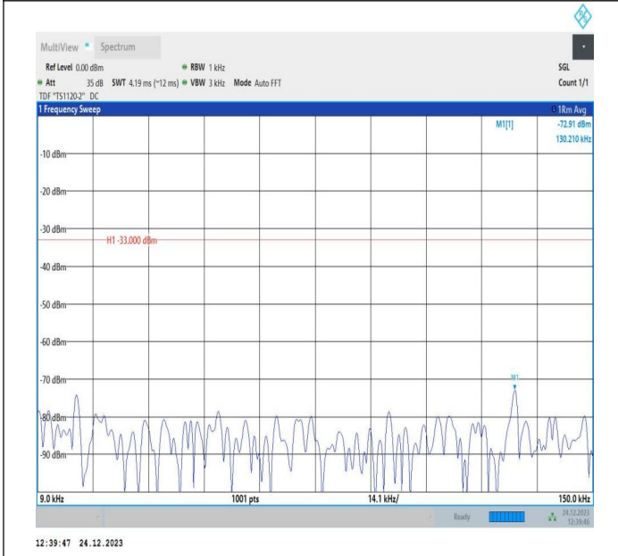
5-5-10MHz-10MHz-QPSK-QPSK-20476-20575-1RB#0-1RB#4 9-0.009~0.15MHz-PASS
