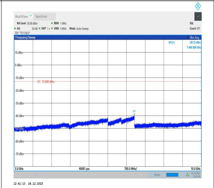
5-5-10MHz-10MHz-QPSK-QPSK-20476-20575-50RB#0-50RB #0-3000~10000MHz-PASS
