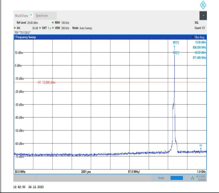
5-5-10MHz-10MHz-QPSK-QPSK-20501-20600-1RB#49-ORB# 0-30~1000MHz-PASS
