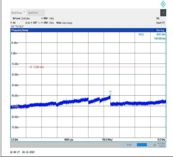
5-5-10MHz-10MHz-QPSK-QPSK-20476-20575-1RB#0-1RB#4 9-3000~10000MHz-PASS
