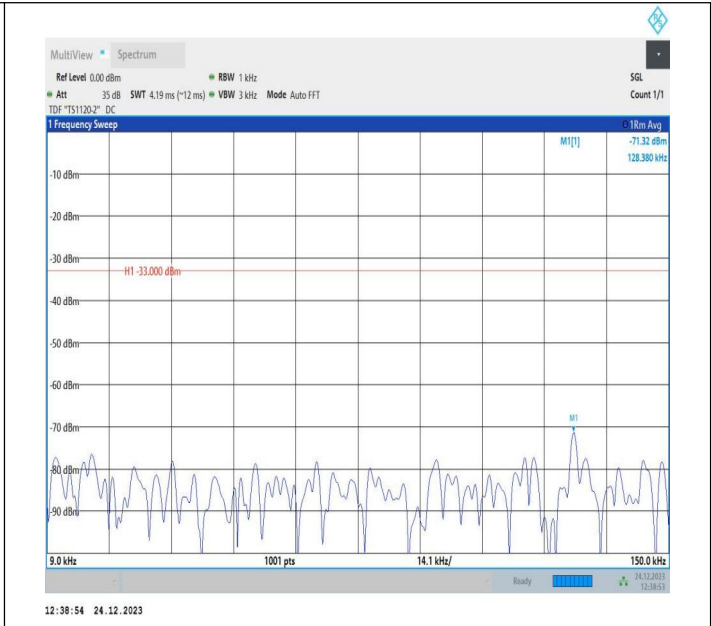
5-5-10MHz-10MHz-QPSK-QPSK-20476-20575-1RB#49-ORB# 0-0.009~0.15MHz-PASS
