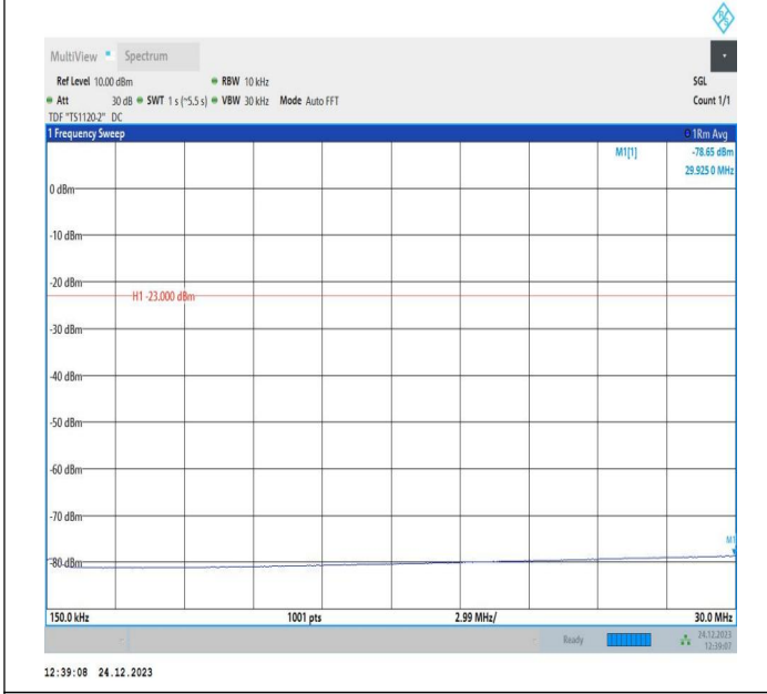
5-5-10MHz-10MHz-QPSK-QPSK-20476-20575-1RB#49-ORB# 0-0.15~30MHz-PASS
