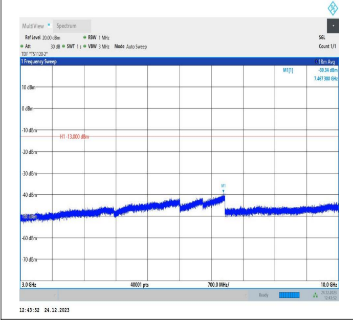
5-5-10MHz-10MHz-QPSK-QPSK-20501-20600-1RB#0-1RB#4 9-3000~10000MHz-PASS
