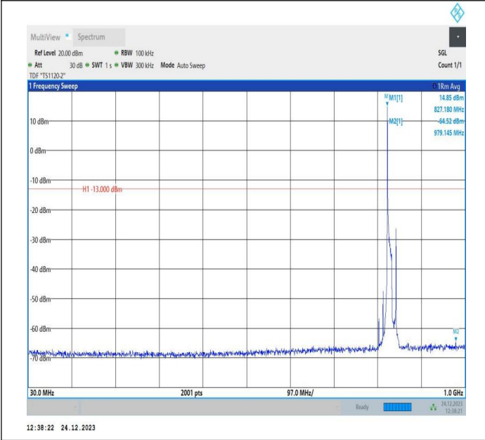
5-5-10MHz-10MHz-QPSK-QPSK-20476-20575-1RB#0-0RB#0 -30~1000MHz-PASS
