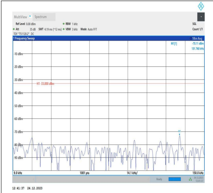
5-5-10MHz-10MHz-QPSK-QPSK-20501-20600-1RB#0-0RB#0 -0.009~0.15MHz-PASS
