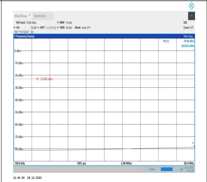
5-5-10MHz-10MHz-QPSK-QPSK-20501-20600-1RB#0-1RB#4 9-0.15~30MHz-PASS
