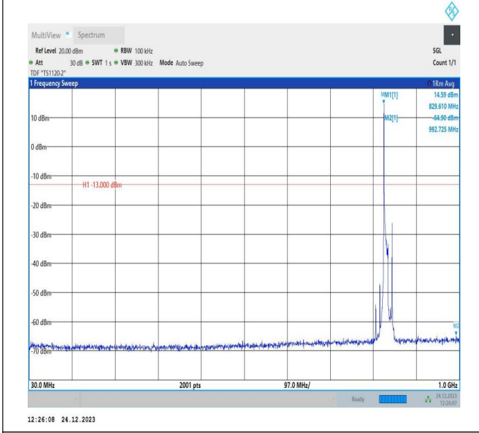
5-5-10MHz-5MHz-QPSK-QPSK-20500-20572-1RB#0-0RB#0-30~1000MHz-PASS
