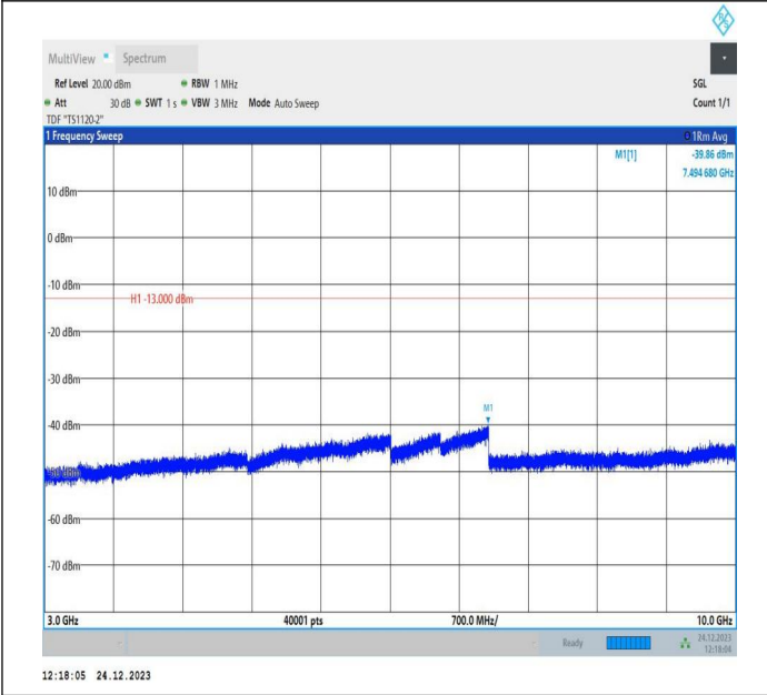
5-5-5MHz-10MHz-QPSK-QPSK-20528-20600-1RB#0-1RB#49 -3000~10000MHz-PASS
