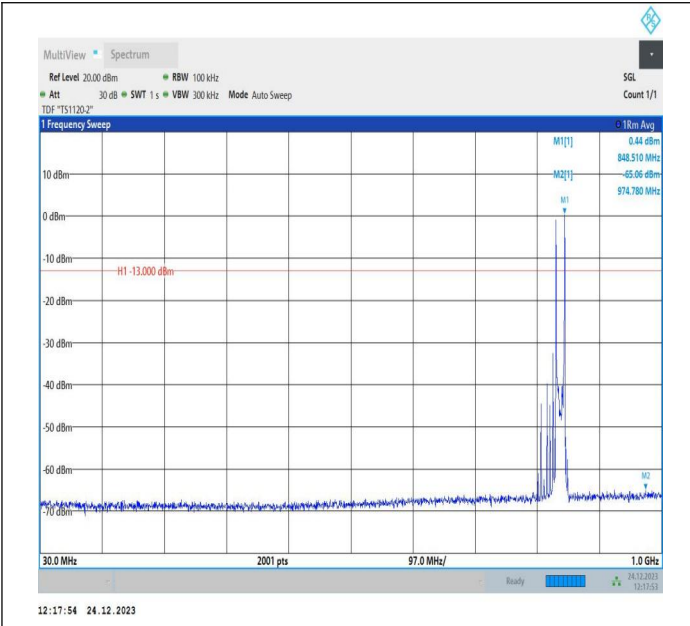
5-5-5MHz-10MHz-QPSK-QPSK-20528-20600-1RB#0-1RB#49 -30~1000MHz-PASS
