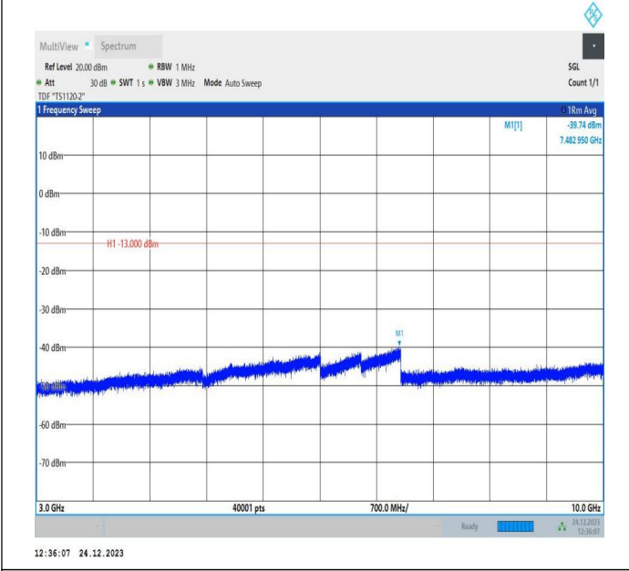
5-5-10MHz-10MHz-QPSK-QPSK-20450-20549-1RB#0-1RB#4 9-3000~10000MHz-PASS
