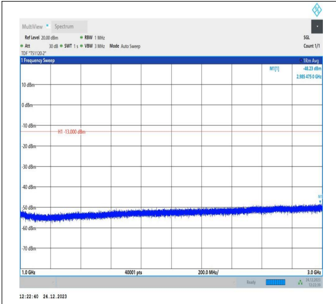
5-5-10MHz-5MHz-QPSK-QPSK-20450-20522-1RB#49-0RB#0 -1000~3000MHz-PASS
