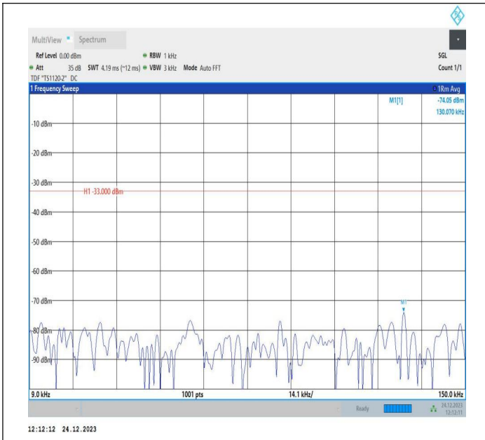
5-5-5MHz-10MHz-QPSK-QPSK-20478-20550-1RB#0-0RB#0-0.009~0.15MHz-PASS
