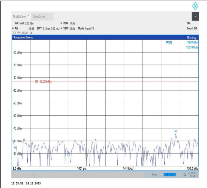
5-5-10MHz-10MHz-QPSK-QPSK-20450-20549-1RB#0-0RB#0 -0.009~0.15MHz-PASS
