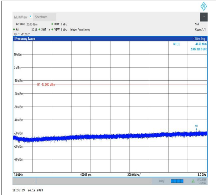
5-5-10MHz-10MHz-QPSK-QPSK-20450-20549-1RB#49-0RB# 0-1000~3000MHz-PASS
