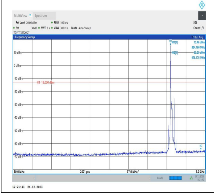
5-5-10MHz-5MHz-QPSK-QPSK-20450-20522-1RB#0-0RB#0-30~1000MHz-PASS
