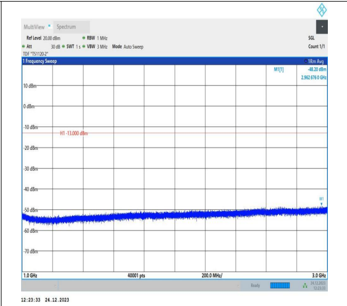
5-5-10MHz-5MHz-QPSK-QPSK-20450-20522-1RB#0-1RB#24- 1000~3000MHz-PASS
