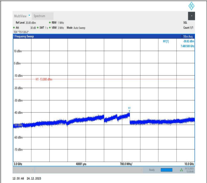
5-5-10MHz-5MHz-QPSK-QPSK-20550-20622-1RB#49-0RB#0- 3000~10000MHz-PASS
