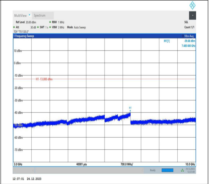
5-5-10MHz-10MHz-QPSK-QPSK-20450-20549-50RB#0-50RB #0-3000~10000MHz-PASS
