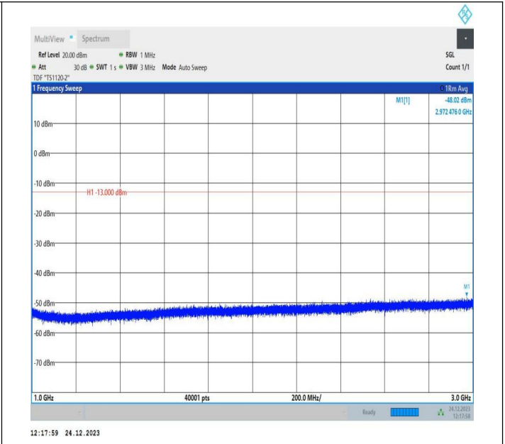
5-5-5MHz-10MHz-QPSK-QPSK-20528-20600-1RB#0-1RB#49- 1000~3000MHz-PASS
