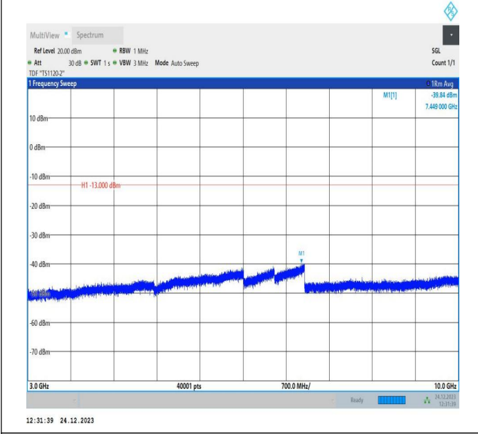
5-5-10MHz-5MHz-QPSK-QPSK-20550-20622-1RB#0-1RB#24 -3000~10000MHz-PASS
