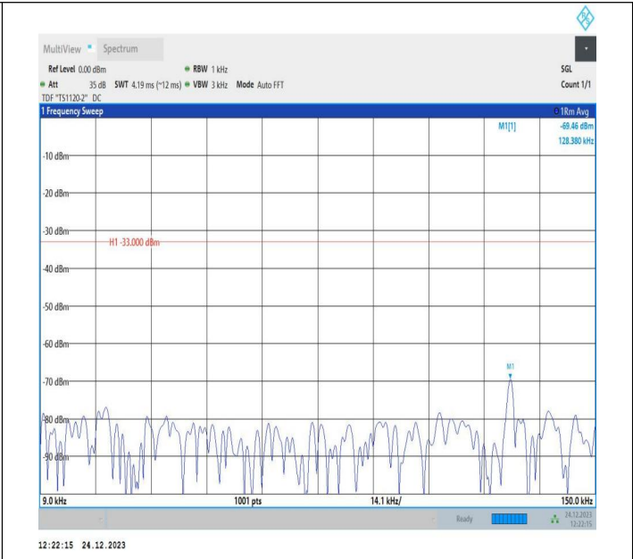
5-5-10MHz-5MHz-QPSK-QPSK-20450-20522-1RB#49-0RB#0-0.009~0.15MHz-PASS
