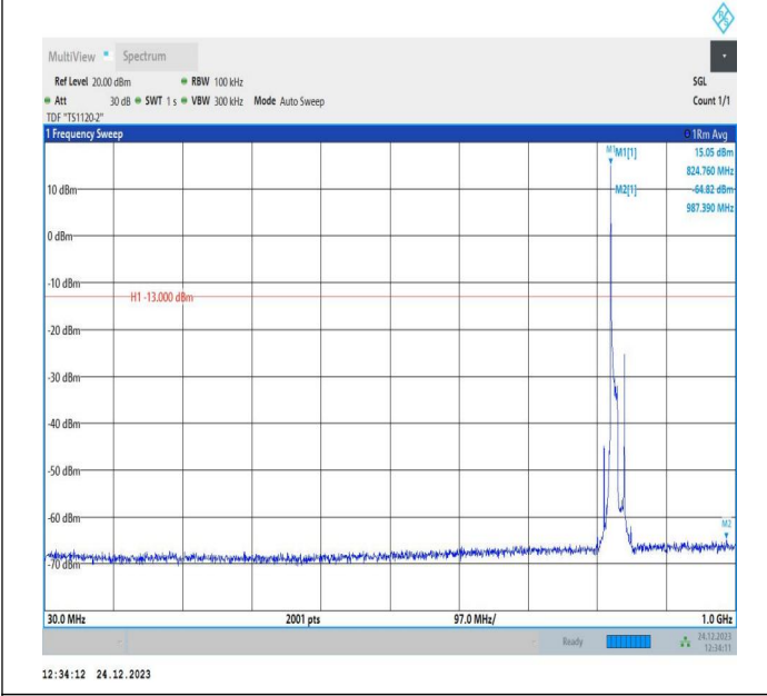
5-5-10MHz-10MHz-QPSK-QPSK-20450-20549-1RB#0-0RB#0 -30~1000MHz-PASS
