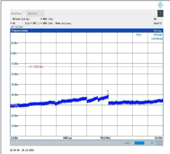
5-5-10MHz-5MHz-QPSK-QPSK-20550-20622-1RB#0-0RB#0-3000~10000MHz-PASS
