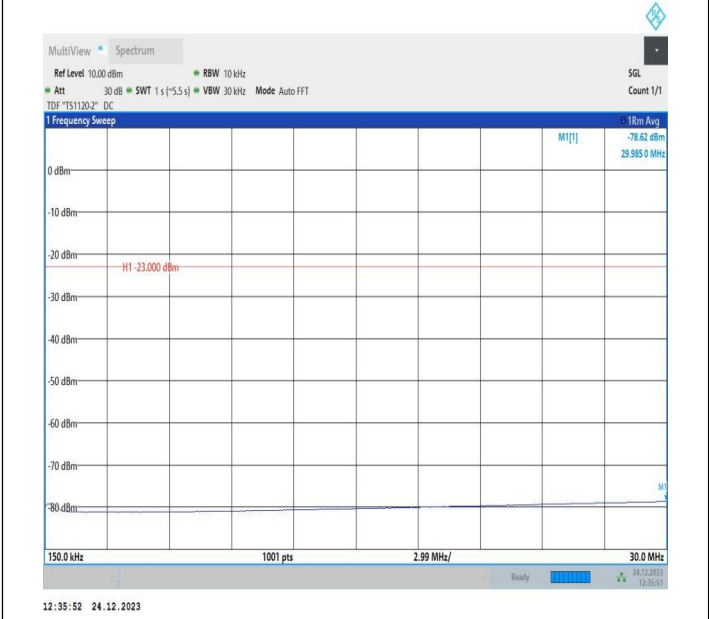
5-5-10MHz-10MHz-QPSK-QPSK-20450-20549-1RB#0-1RB#4 9-0.15~30MHz-PASS
