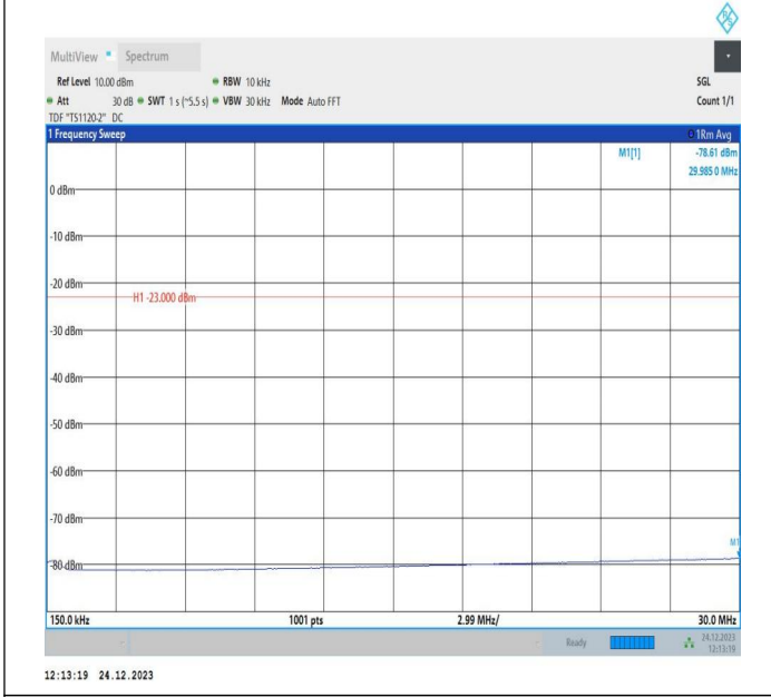
5-5-5MHz-10MHz-QPSK-QPSK-20478-20550-1RB#24-0RB#0-0.15~30MHz-PASS
