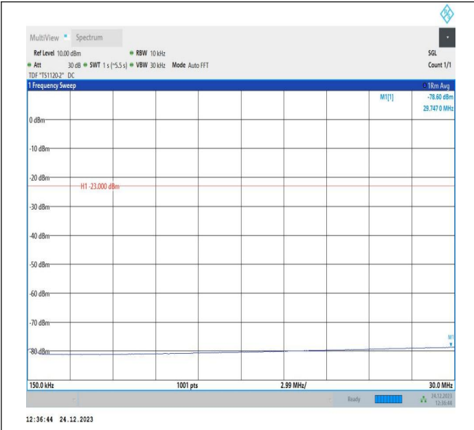
5-5-10MHz-10MHz-QPSK-QPSK-20450-20549-50RB#0-50RB #0-0.15~30MHz-PASS
