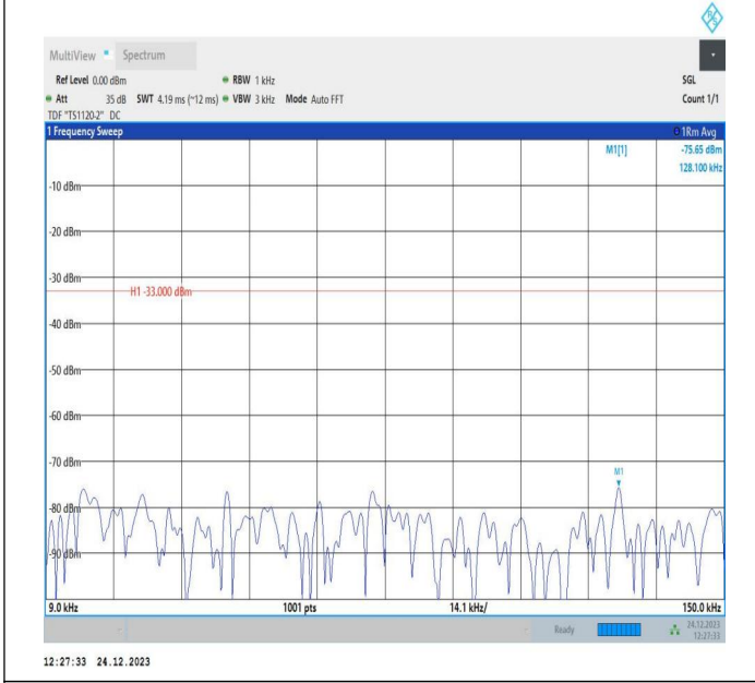
5-5-10MHz-5MHz-QPSK-QPSK-20500-20572-1RB#0-1RB#24 -0.009~0.15MHz-PASS
