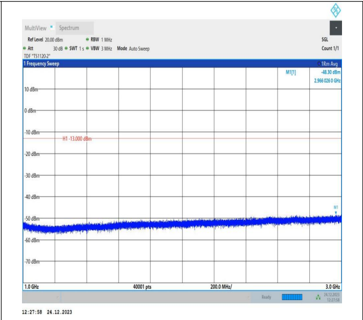
5-5-10MHz-5MHz-QPSK-QPSK-20500-20572-1RB#0-1RB#24- 1000~3000MHz-PASS
