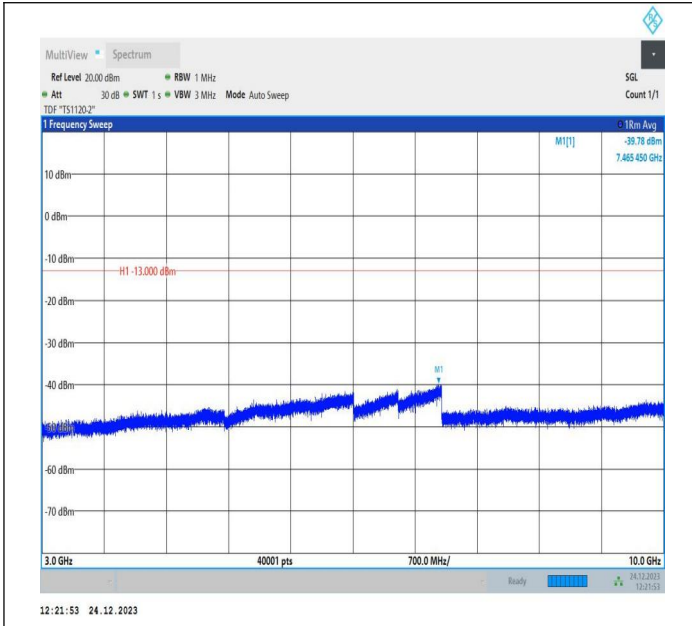
5-5-10MHz-5MHz-QPSK-QPSK-20450-20522-1RB#0-0RB#0-3000~10000MHz-PASS
