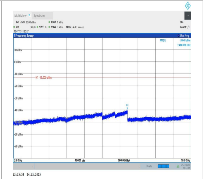
5-5-5MHz-10MHz-QPSK-QPSK-20478-20550-1RB#24-0RB#0 3000~10000MHz-PASS
