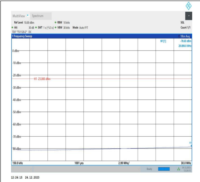
5-5-10MHz-5MHz-QPSK-QPSK-20450-20522-50RB#0-25RB# 0-0.15~30MHz-PASS
