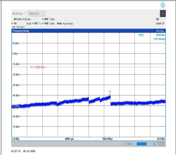
5-5-10MHz-5MHz-QPSK-QPSK-20500-20572-1RB#49-0RB#0- 3000~10000MHz-PASS
