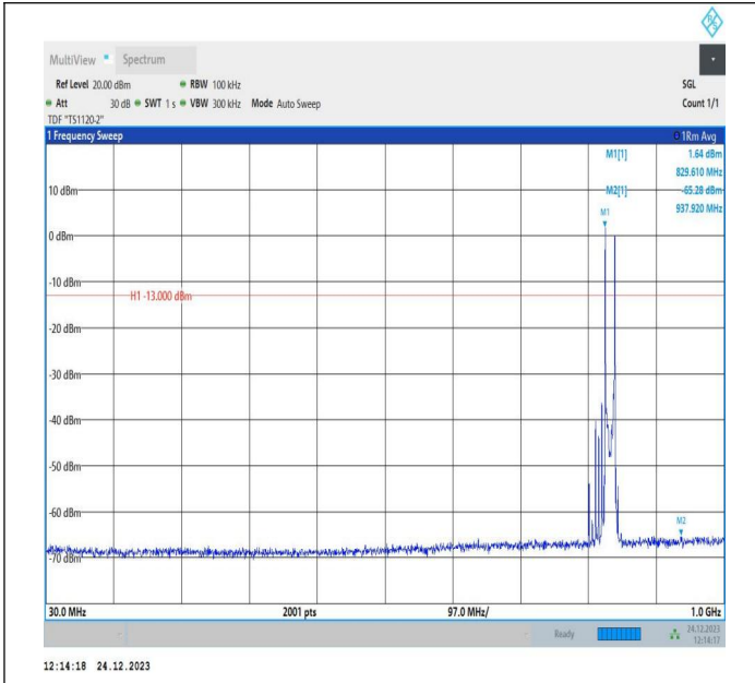
5-5-5MHz-10MHz-QPSK-QPSK-20478-20550-1RB#0-1RB#49 -30~1000MHz-PASS
