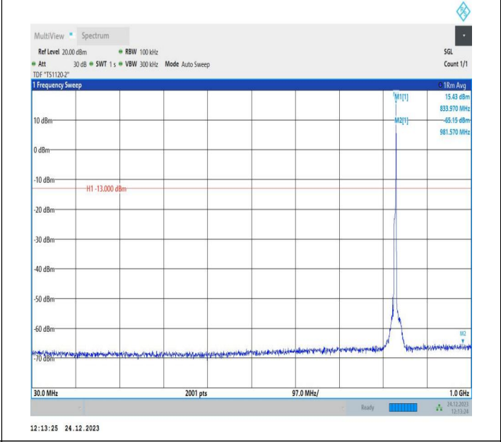
5-5-5MHz-10MHz-QPSK-QPSK-20478-20550-1RB#24-0RB#0-30~1000MHz-PASS
