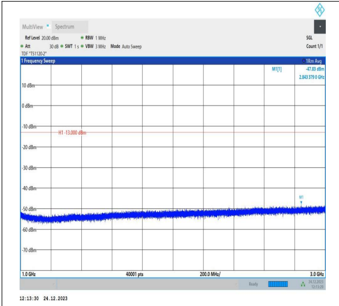
5-5-5MHz-10MHz-QPSK-QPSK-20478-20550-1RB#24-0RB#0 -1000~3000MHz-PASS
