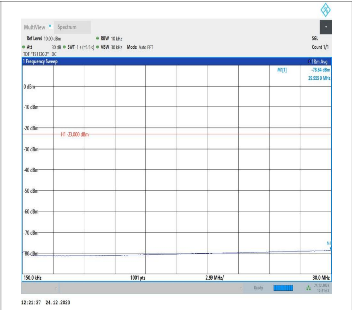
5-5-10MHz-5MHz-QPSK-QPSK-20450-20522-1RB#0-0RB#0-0.15~30MHz-PASS
