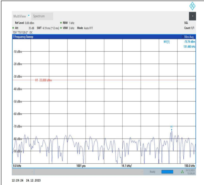
5-5-10MHz-5MHz-QPSK-QPSK-20550-20622-1RB#0-0RB#0-0.009~0.15MHz-PASS
