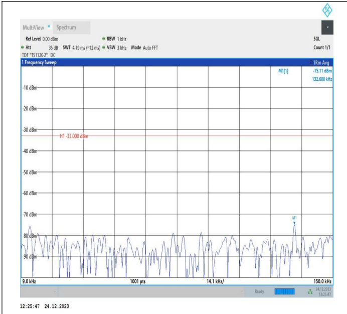
5-5-10MHz-5MHz-QPSK-QPSK-20500-20572-1RB#0-0RB#0-0.009~0.15MHz-PASS
