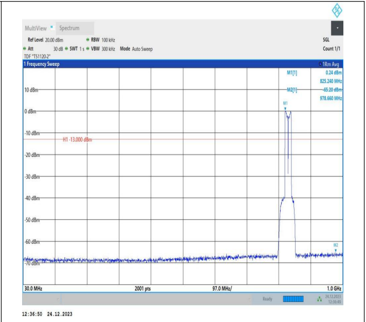
5-5-10MHz-10MHz-QPSK-QPSK-20450-20549-50RB#0-50RB #0-30~1000MHz-PASS
