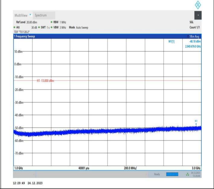
5-5-10MHz-5MHz-QPSK-QPSK-20550-20622-1RB#0-0RB#0-1000~3000MHz-PASS
