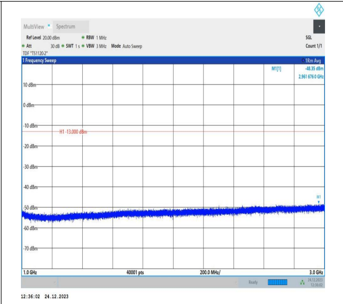
5-5-10MHz-10MHz-QPSK-QPSK-20450-20549-1RB#0-1RB#4 9-1000~3000MHz-PASS
