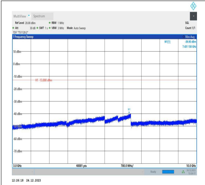
5-5-10MHz-5MHz-QPSK-QPSK-20500-20572-1RB#0-0RB#0-3000~10000MHz-PASS
