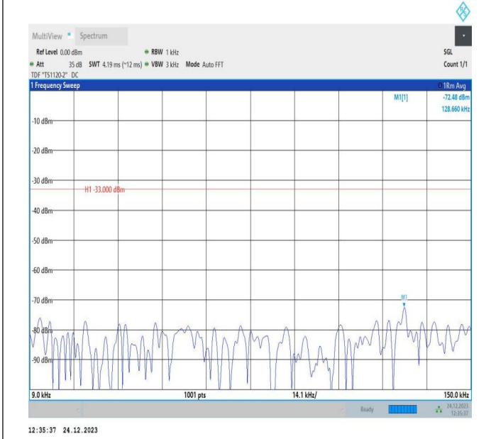
5-5-10MHz-10MHz-QPSK-QPSK-20450-20549-1RB#0-1RB#4 9-0.009~0.15MHz-PASS
