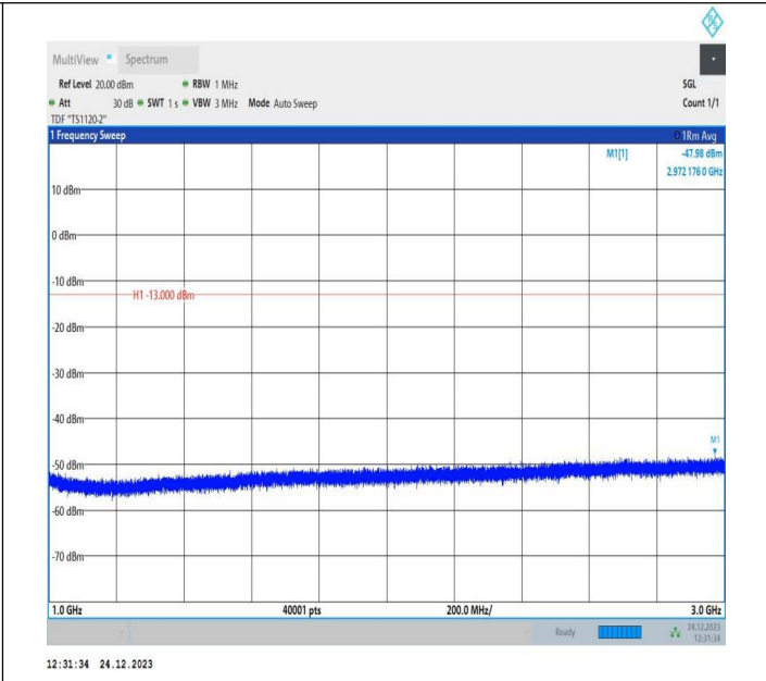
5-5-10MHz-5MHz-QPSK-QPSK-20550-20622-1RB#0-1RB#24- 1000~3000MHz-PASS
