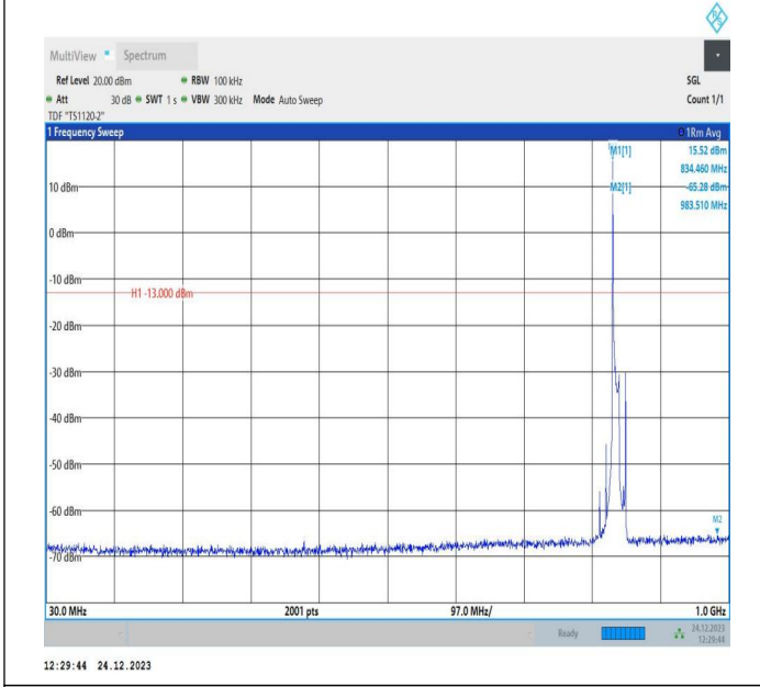
5-5-10MHz-5MHz-QPSK-QPSK-20550-20622-1RB#0-0RB#0-30~1000MHz-PASS
