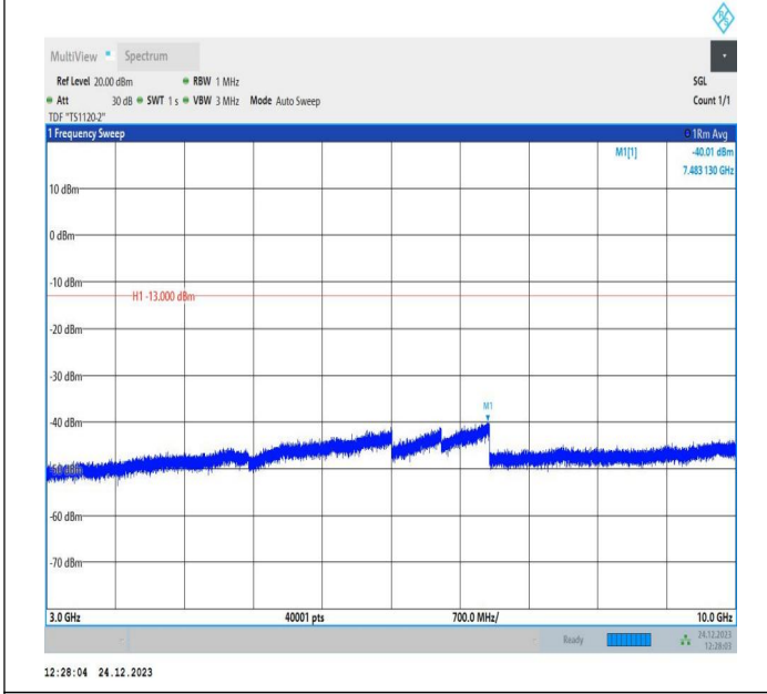
5-5-10MHz-5MHz-QPSK-QPSK-20500-20572-1RB#0-1RB#24 -3000~10000MHz-PASS
