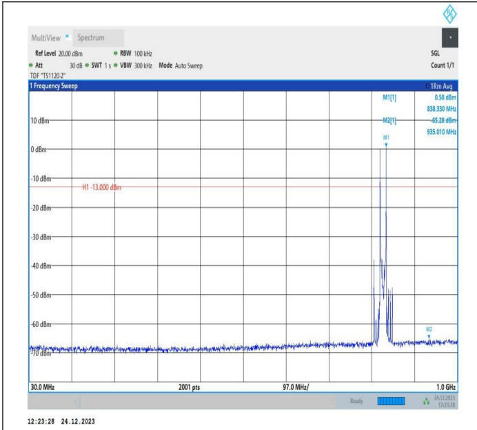
5-5-10MHz-5MHz-QPSK-QPSK-20450-20522-1RB#0-1RB#24 -30~1000MHz-PASS
