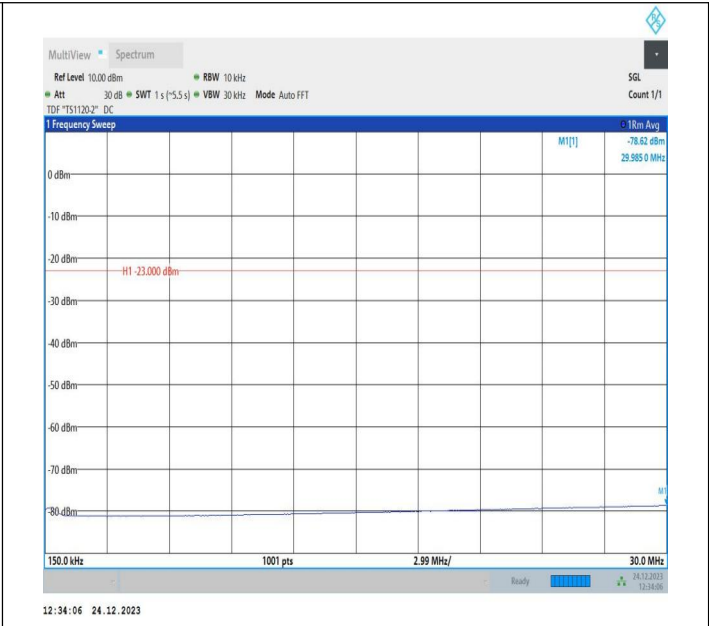
5-5-10MHz-10MHz-QPSK-QPSK-20450-20549-1RB#0-0RB#0 0.15~30MHz-PASS
