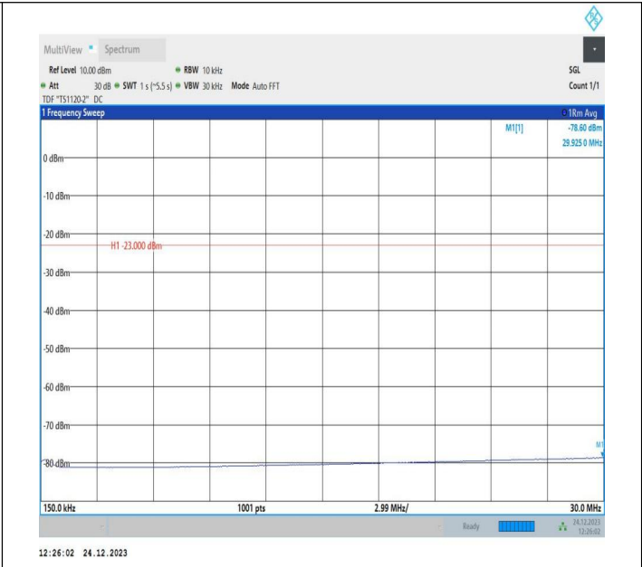
5-5-10MHz-5MHz-QPSK-QPSK-20500-20572-1RB#0-0RB#0-0.15~30MHz-PASS
