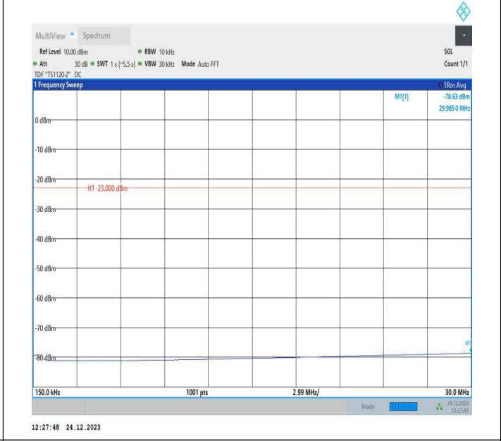
5-5-10MHz-5MHz-QPSK-QPSK-20500-20572-1RB#0-1RB#24- 0.15~30MHz-PASS
