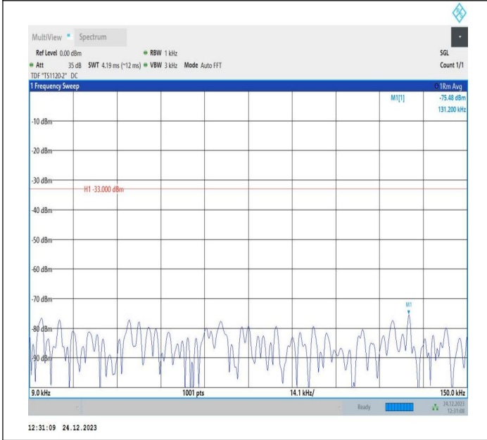
5-5-10MHz-5MHz-QPSK-QPSK-20550-20622-1RB#0-1RB#24 -0.009~0.15MHz-PASS
