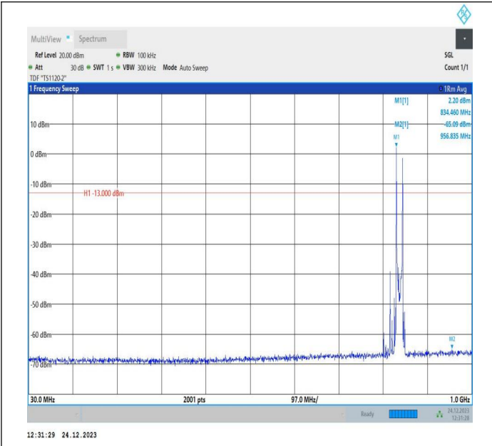
5-5-10MHz-5MHz-QPSK-QPSK-20550-20622-1RB#0-1RB#24 -30~1000MHz-PASS
