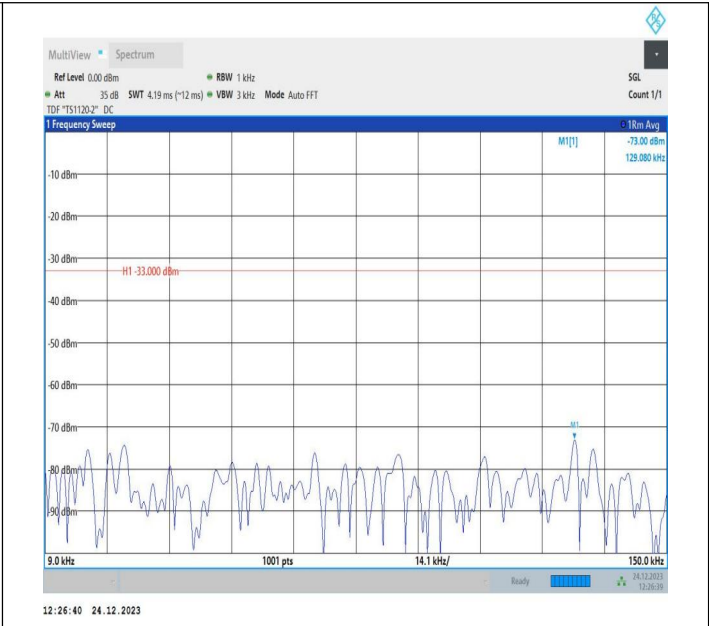
5-5-10MHz-5MHz-QPSK-QPSK-20500-20572-1RB#49-0RB#0-0.009~0.15MHz-PASS
