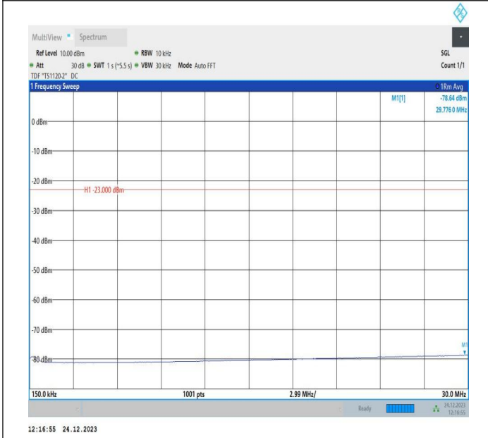
5-5-5MHz-10MHz-QPSK-QPSK-20528-20600-1RB#24-0RB#0-0.15~30MHz-PASS
