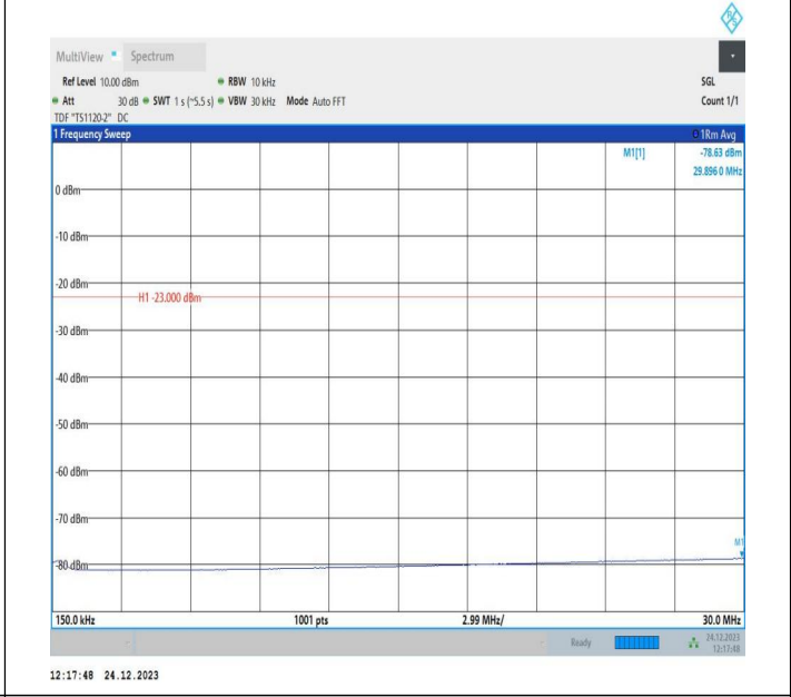
5-5-5MHz-10MHz-QPSK-QPSK-20528-20600-1RB#0-1RB#49 0.15~30MHz-PASS
