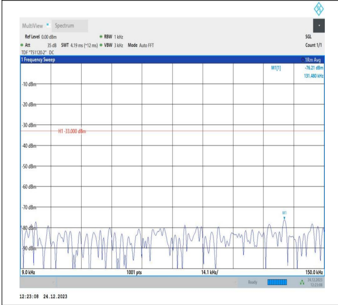
5-5-10MHz-5MHz-QPSK-QPSK-20450-20522-1RB#0-1RB#24 -0.009~0.15MHz-PASS
