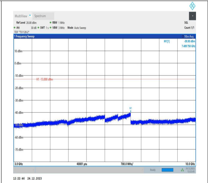
5-5-10MHz-5MHz-QPSK-QPSK-20450-20522-1RB#49-0RB#0- 3000~10000MHz-PASS
