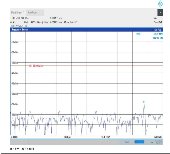
5-5-5MHz-10MHz-QPSK-QPSK-20478-20550-1RB#0-1RB#49 -0.009~0.15MHz-PASS
