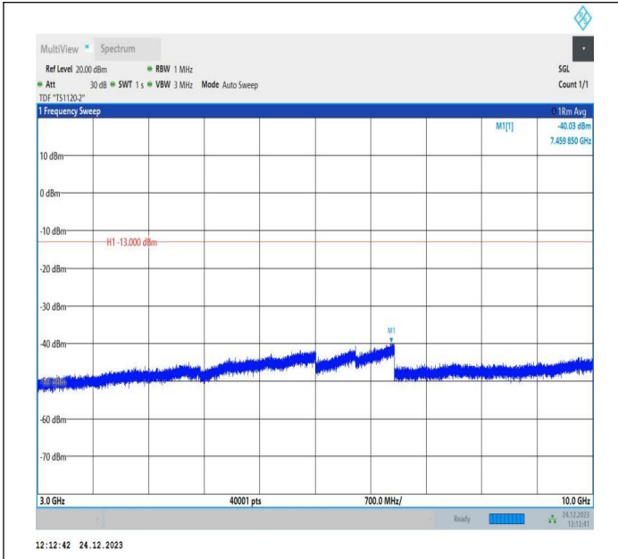
5-5-5MHz-10MHz-QPSK-QPSK-20478-20550-1RB#0-0RB#0-3000~10000MHz-PASS
