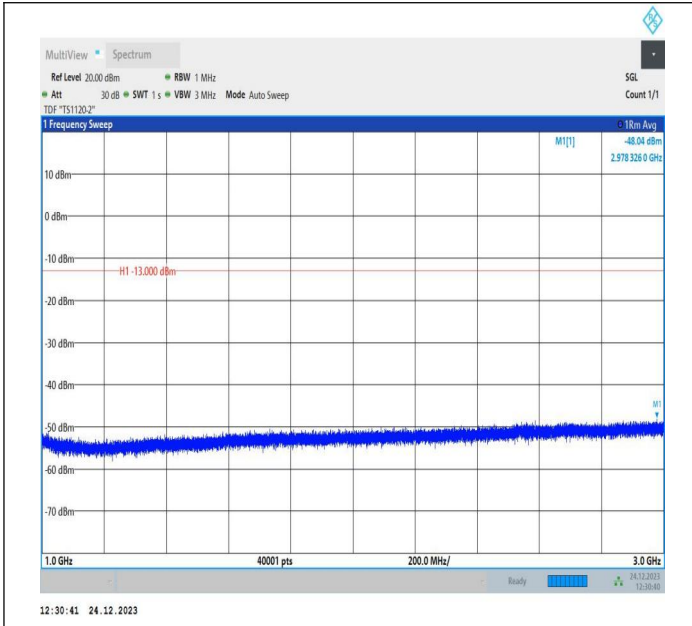
5-5-10MHz-5MHz-QPSK-QPSK-20550-20622-1RB#49-0RB#0 -1000~3000MHz-PASS
