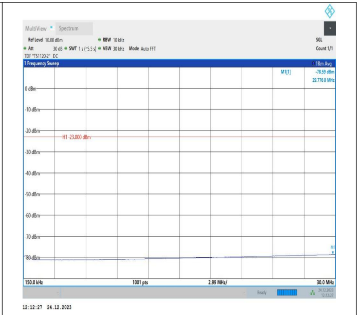
5-5-5MHz-10MHz-QPSK-QPSK-20478-20550-1RB#0-0RB#0-0.15~30MHz-PASS
