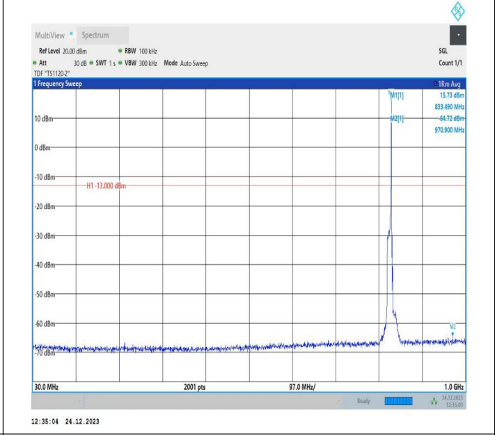
5-5-10MHz-10MHz-QPSK-QPSK-20450-20549-1RB#49-ORB# 0-30~1000MHz-PASS
