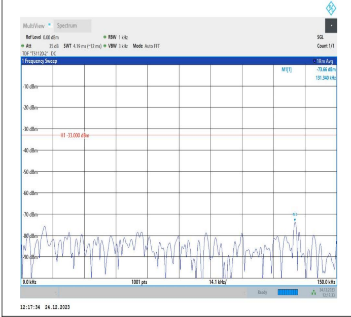
5-5-5MHz-10MHz-QPSK-QPSK-20528-20600-1RB#0-1RB#49 -0.009~0.15MHz-PASS
