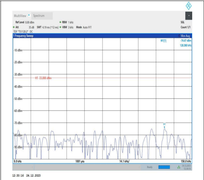
5-5-10MHz-5MHz-QPSK-QPSK-20550-20622-1RB#49-0RB#0-0.009~0.15MHz-PASS
