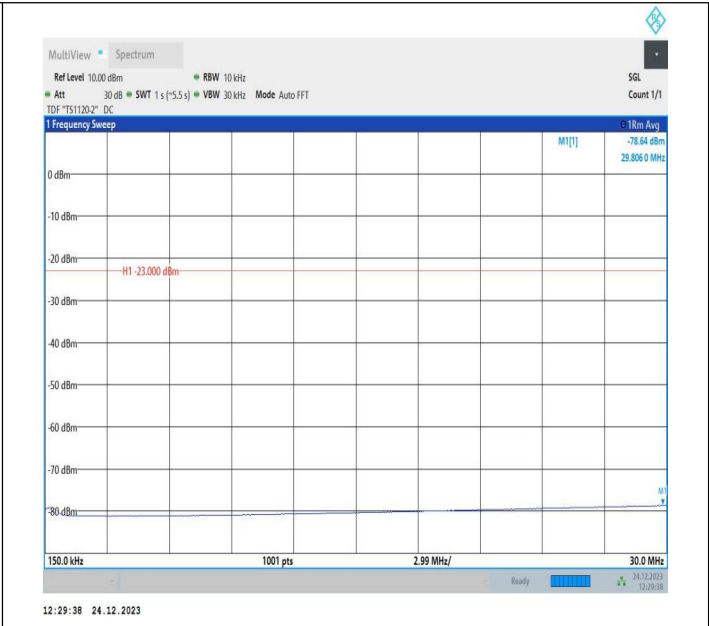
5-5-10MHz-5MHz-QPSK-QPSK-20550-20622-1RB#0-0RB#0-0.15~30MHz-PASS
