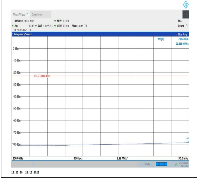
5-5-10MHz-5MHz-QPSK-QPSK-20450-20522-1RB#49-0RB#0-0.15~30MHz-PASS
