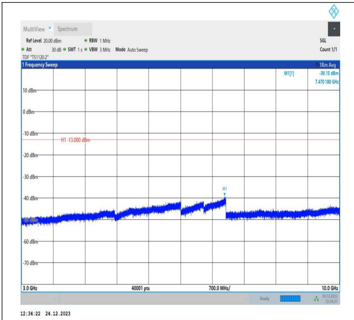
5-5-10MHz-10MHz-QPSK-QPSK-20450-20549-1RB#0-ORB#0 -3000~10000MHz-PASS
