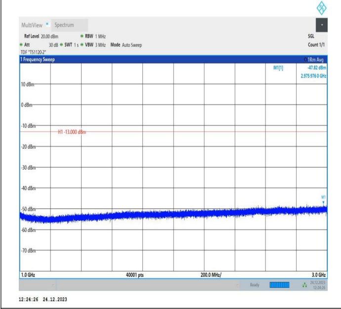
5-5-10MHz-5MHz-QPSK-QPSK-20450-20522-50RB#0-25RB# 0-1000~3000MHz-PASS
