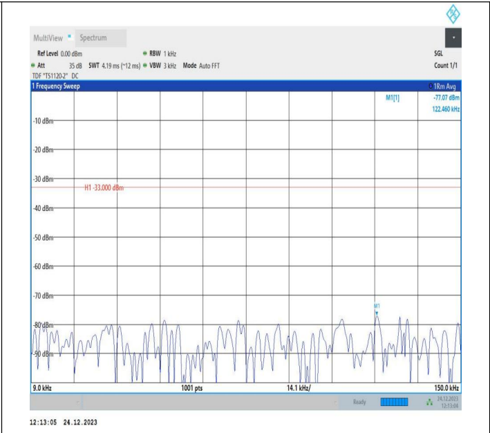
5-5-5MHz-10MHz-QPSK-QPSK-20478-20550-1RB#24-0RB#0-0.009~0.15MHz-PASS
