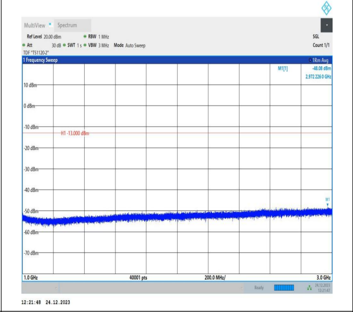
5-5-10MHz-5MHz-QPSK-QPSK-20450-20522-1RB#0-0RB#0-1000~3000MHz-PASS
