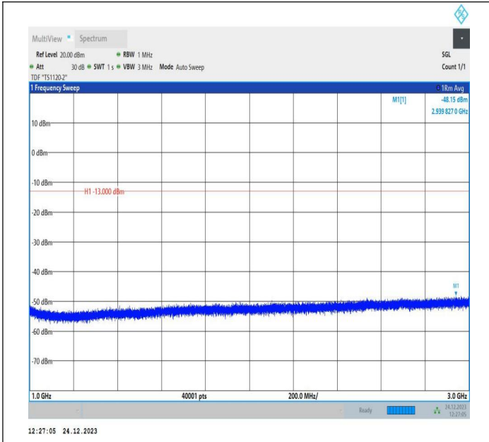
5-5-10MHz-5MHz-QPSK-QPSK-20500-20572-1RB#49-0RB#0 -1000~3000MHz-PASS
