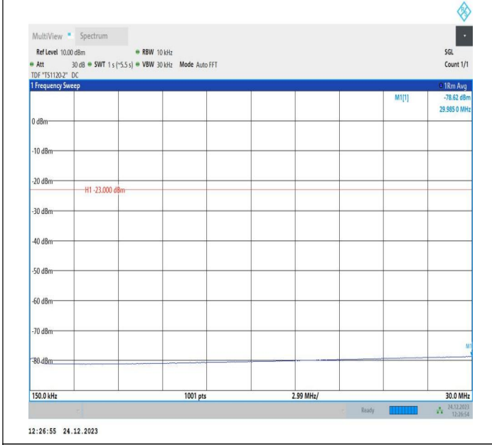
5-5-10MHz-5MHz-QPSK-QPSK-20500-20572-1RB#49-0RB#0-0.15~30MHz-PASS
