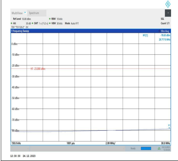
5-5-10MHz-5MHz-QPSK-QPSK-20550-20622-1RB#49-0RB#0-0.15~30MHz-PASS
