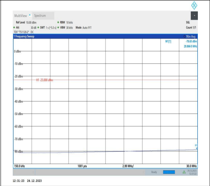
5-5-10MHz-5MHz-QPSK-QPSK-20550-20622-1RB#0-1RB#24- 0.15~30MHz-PASS
