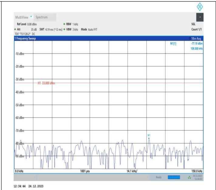
5-5-10MHz-10MHz-QPSK-QPSK-20450-20549-1RB#49-ORB# 0-0.009~0.15MHz-PASS
