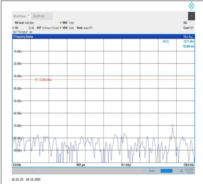
5-5-10MHz-5MHz-QPSK-QPSK-20450-20522-1RB#0-0RB#0-0.009~0.15MHz-PASS
