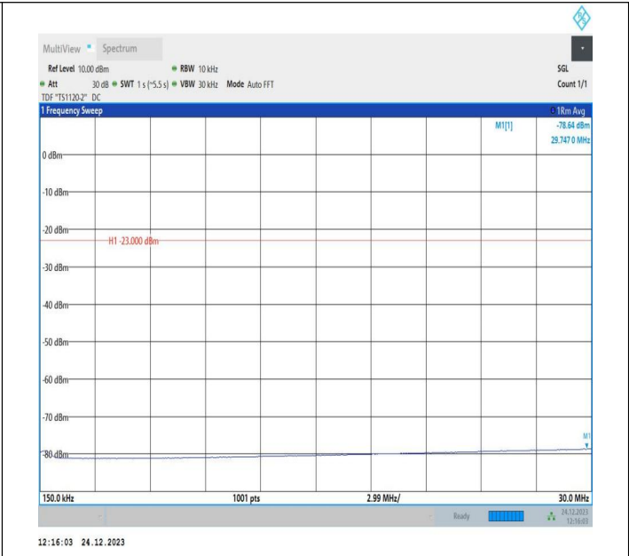
5-5-5MHz-10MHz-QPSK-QPSK-20528-20600-1RB#0-0RB#0-0.15~30MHz-PASS
