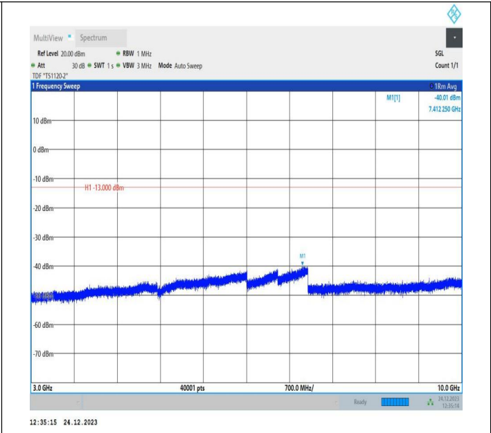
5-5-10MHz-10MHz-QPSK-QPSK-20450-20549-1RB#49-0RB# 0-3000~10000MHz-PASS
