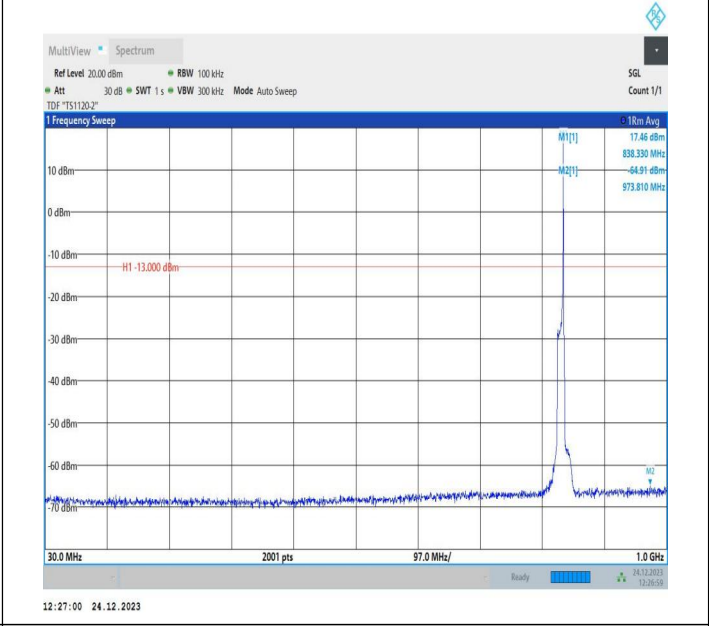
5-5-10MHz-5MHz-QPSK-QPSK-20500-20572-1RB#49-0RB#0-30~1000MHz-PASS
