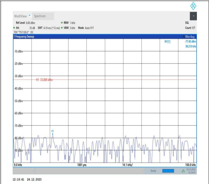
5-5-5MHz-10MHz-QPSK-QPSK-20528-20600-1RB#24-0RB#0-0.009~0.15MHz-PASS
