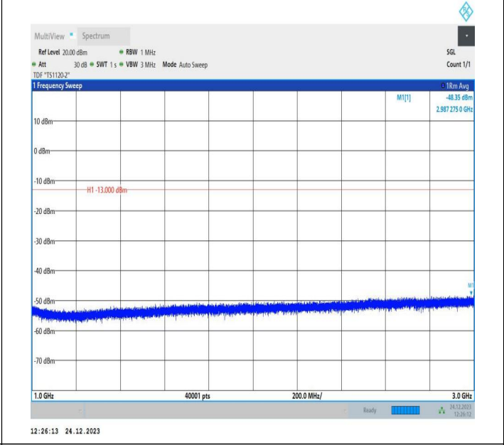
5-5-10MHz-5MHz-QPSK-QPSK-20500-20572-1RB#0-0RB#0-1000~3000MHz-PASS
