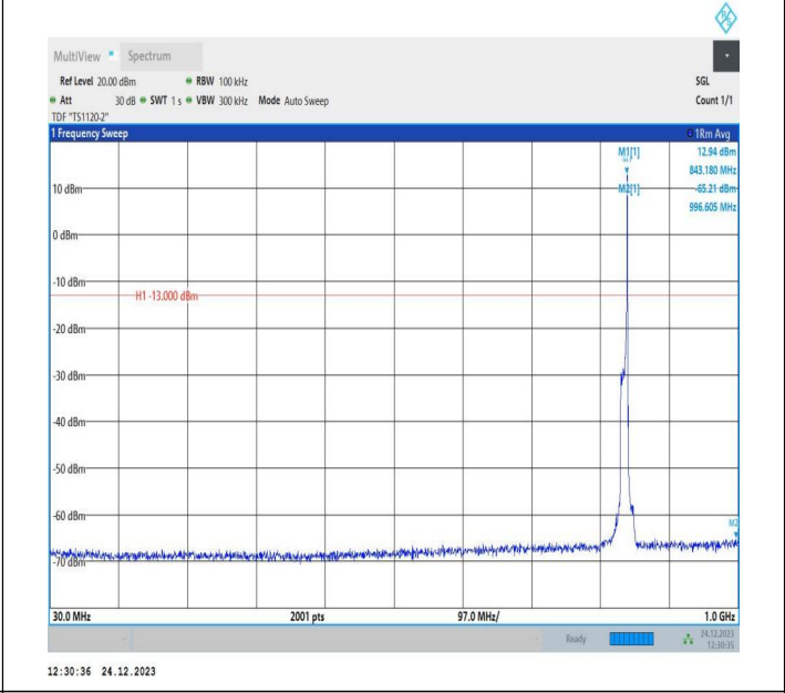
5-5-10MHz-5MHz-QPSK-QPSK-20550-20622-1RB#49-0RB#0-30~1000MHz-PASS
