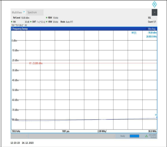
5-5-10MHz-5MHz-QPSK-QPSK-20450-20522-1RB#0-1RB#24- 0.15~30MHz-PASS
