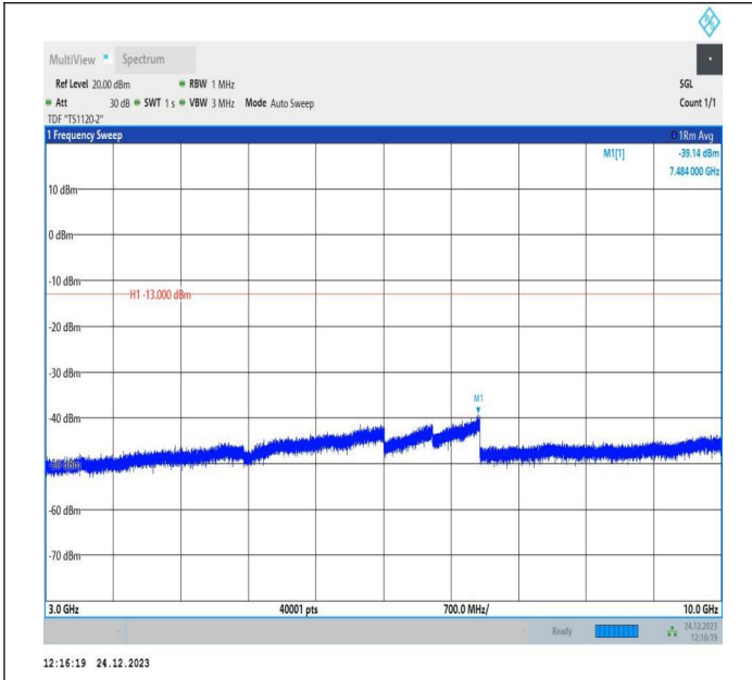
5-5-5MHz-10MHz-QPSK-QPSK-20528-20600-1RB#0-0RB#0-3000~10000MHz-PASS
