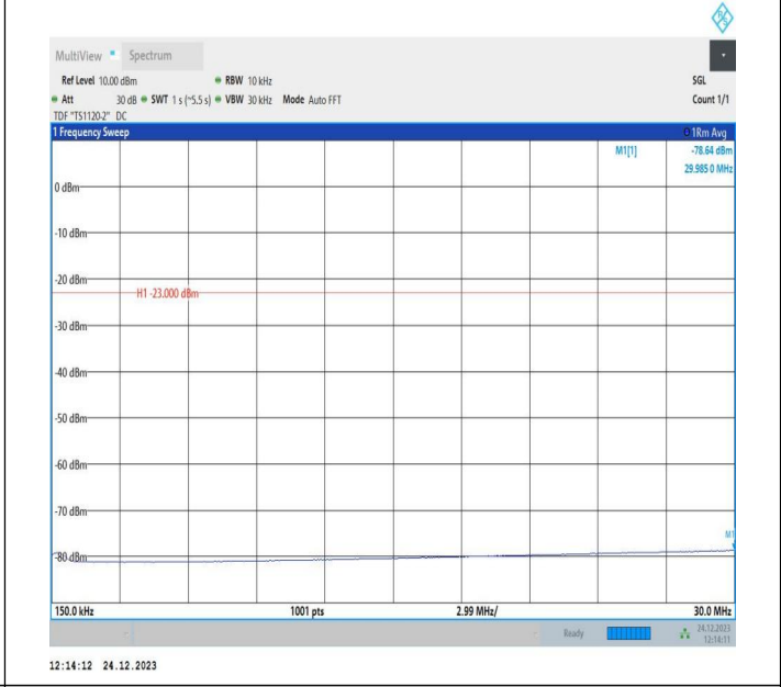
5-5-5MHz-10MHz-QPSK-QPSK-20478-20550-1RB#0-1RB#49 0.15~30MHz-PASS
