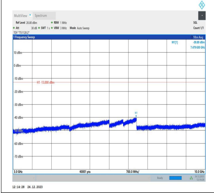
5-5-5MHz-10MHz-QPSK-QPSK-20478-20550-1RB#0-1RB#49 -3000~10000MHz-PASS
