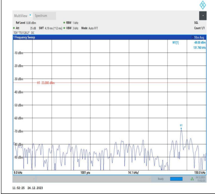
5-5-3MHz-5MHz-QPSK-QPSK-20586-20625-1RB#0-1RB#24-0.009~0.15MHz-PASS
