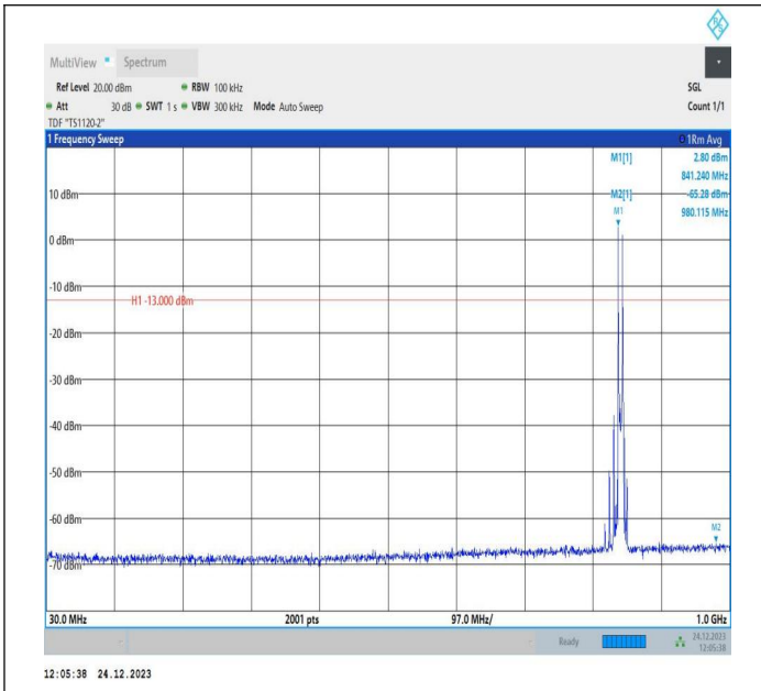
5-5-5MHz-3MHz-QPSK-QPSK-20595-20634-1RB#0-1RB#15-30~1000MHz-PASS
