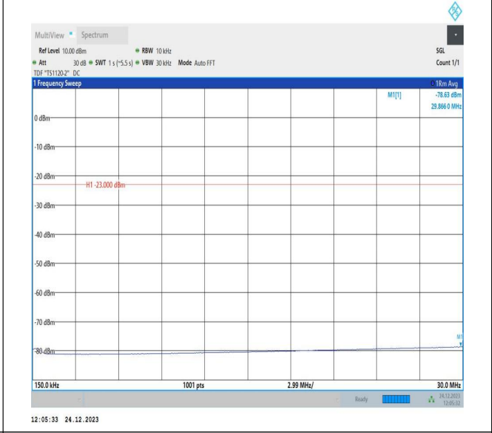
5-5-5MHz-3MHz-QPSK-QPSK-20595-20634-1RB#0-1RB#15-0.15~30MHz-PASS
