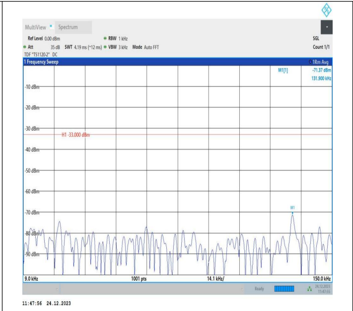
5-5-3MHz-5MHz-QPSK-QPSK-20501-20540-1RB#14-0RB#0-0 .009~0.15MHz-PASS
