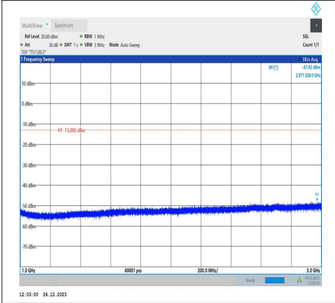
5-5-5MHz-3MHz-QPSK-QPSK-20510-20549-25RB#0-15RB#0 -1000~3000MHz-PASS
