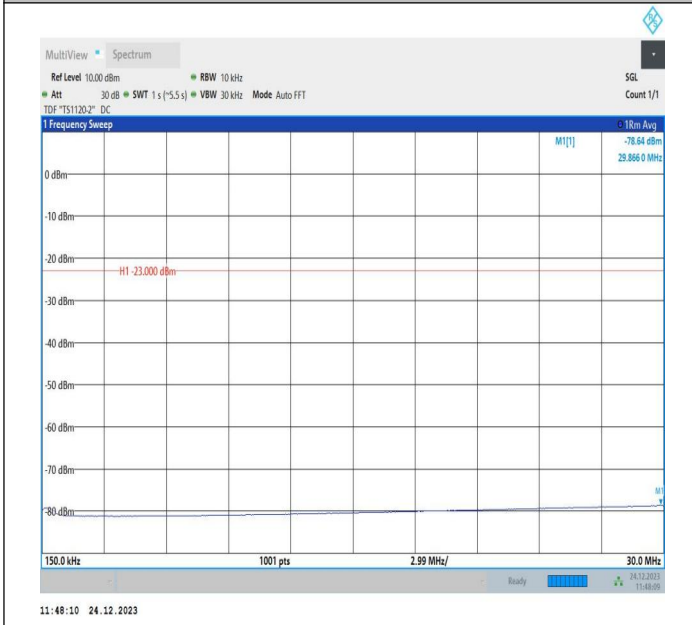
5-5-3MHz-5MHz-QPSK-QPSK-20501-20540-1RB#14-0RB#0-0 0.15~30MHz-PASS
