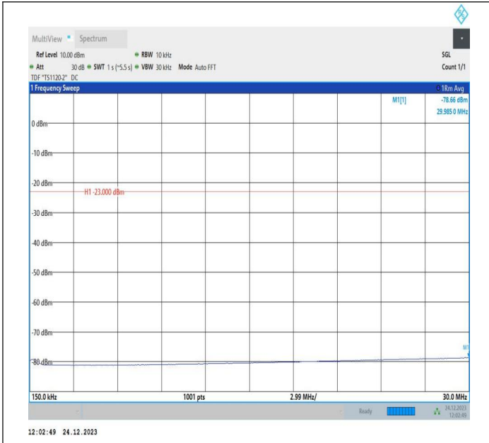
5-5-5MHz-3MHz-QPSK-QPSK-20510-20549-25RB#0-15RB#0 -0.15~30MHz-PASS
