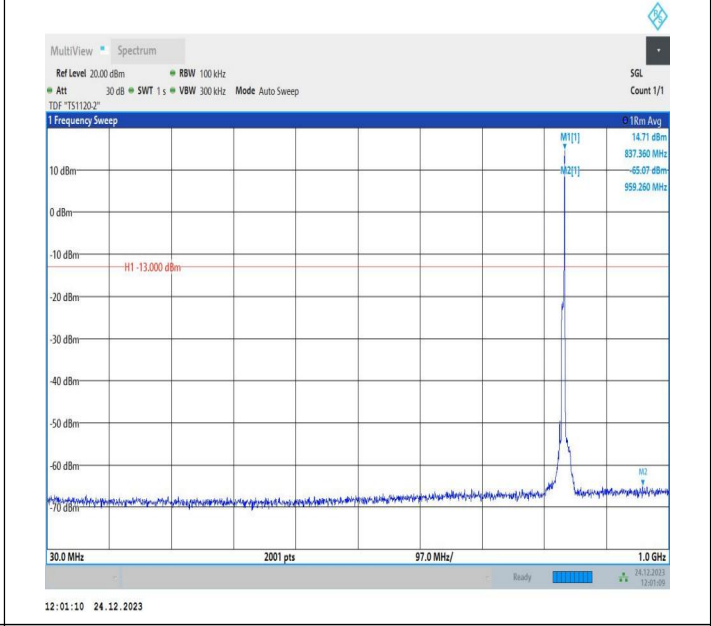
5-5-5MHz-3MHz-QPSK-QPSK-20510-20549-1RB#24-0RB#0-3 0~1000MHz-PASS
