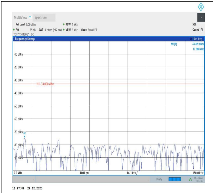
5-5-3MHz-5MHz-QPSK-QPSK-20501-20540-1RB#0-0RB#0-0.009~0.15MHz-PASS
