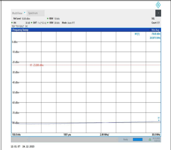
5-5-5MHz-3MHz-QPSK-QPSK-20510-20549-1RB#0-1RB#15-0.15~30MHz-PASS
