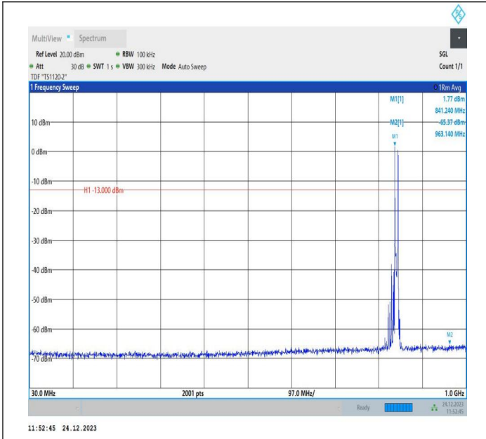
5-5-3MHz-5MHz-QPSK-QPSK-20586-20625-1RB#0-1RB#24-30~1000MHz-PASS
