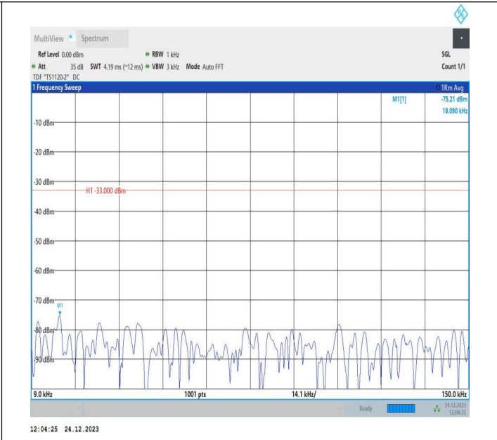
5-5-5MHz-3MHz-QPSK-QPSK-20595-20634-1RB#24-0RB#0-0 .009~0.15MHz-PASS
