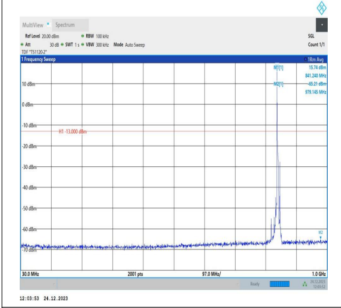
5-5-5MHz-3MHz-QPSK-QPSK-20595-20634-1RB#0-0RB#0-3 0~1000MHz-PASS
