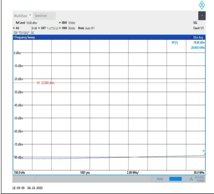
5-5-5MHz-10MHz-QPSK-QPSK-20428-20500-1RB#24-0RB#0-0.15~30MHz-PASS
