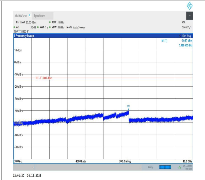
5-5-5MHz-3MHz-QPSK-QPSK-20510-20549-1RB#24-0RB#0-3000~10000MHz-PASS
