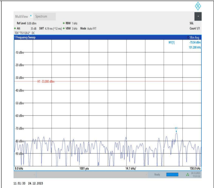
5-5-3MHz-5MHz-QPSK-QPSK-20586-20625-1RB#14-0RB#0-0 .009~0.15MHz-PASS
