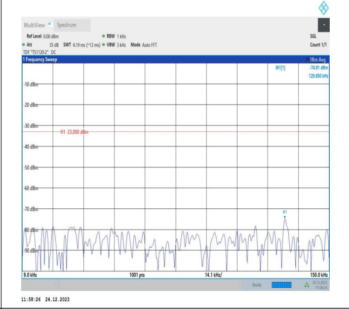
5-5-5MHz-3MHz-QPSK-QPSK-20425-20464-25RB#0-15RB#0-0.009~0.15MHz-PASS
