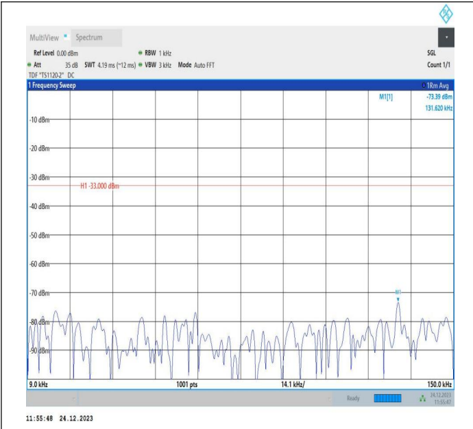
5-5-5MHz-3MHz-QPSK-QPSK-20425-20464-1RB#0-0RB#0-0. 009~0.15MHz-PASS
