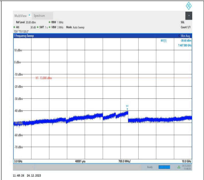
5-5-3MHz-5MHz-QPSK-QPSK-20501-20540-1RB#14-0RB#0-3000~10000MHz-PASS
