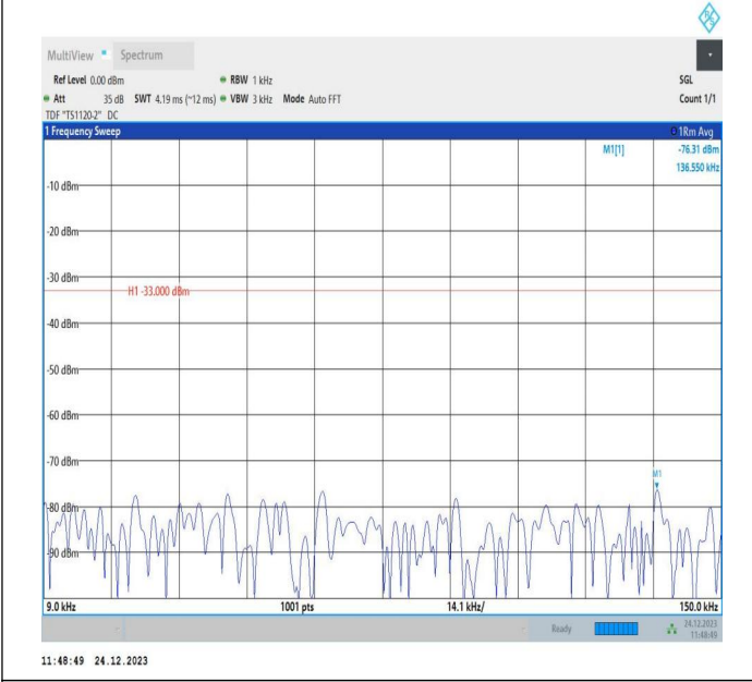
5-5-3MHz-5MHz-QPSK-QPSK-20501-20540-1RB#0-1RB#24-0.009~0.15MHz-PASS
