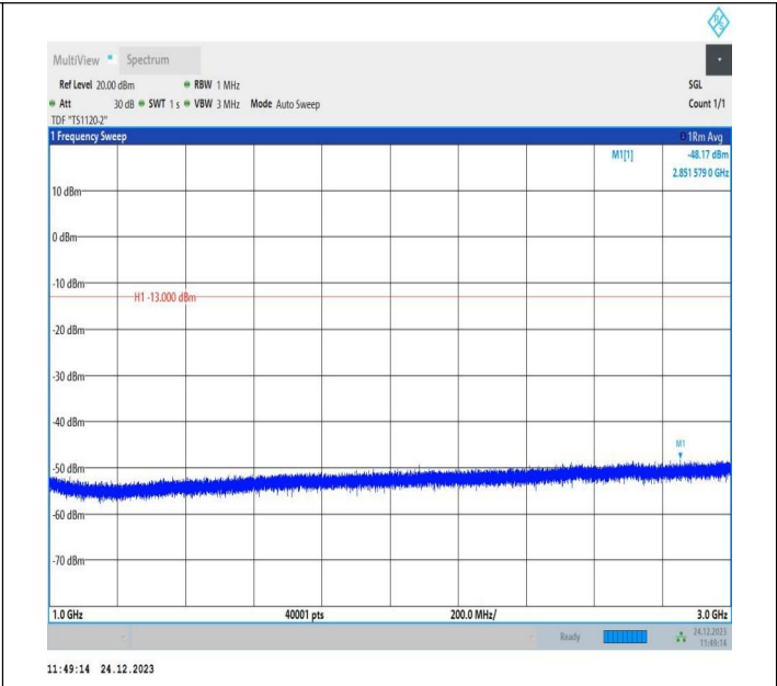
5-5-3MHz-5MHz-QPSK-QPSK-20501-20540-1RB#0-1RB#24-1000~3000MHz-PASS
