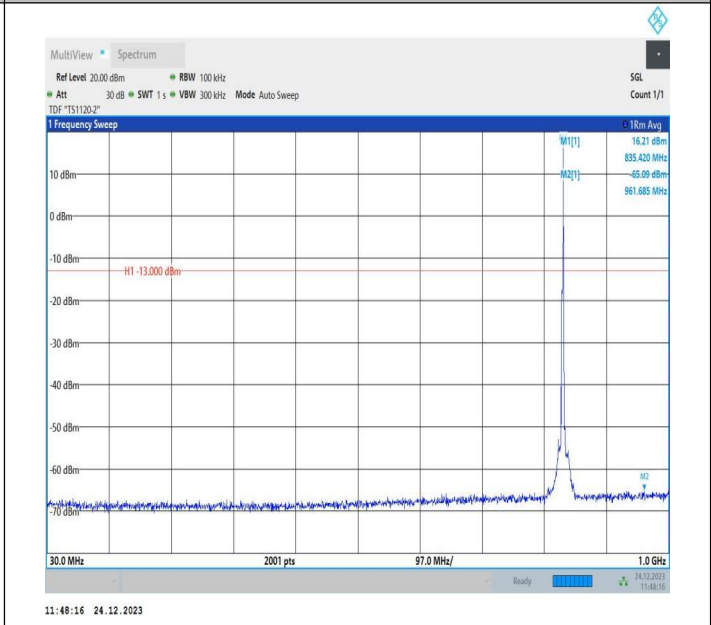
5-5-3MHz-5MHz-QPSK-QPSK-20501-20540-1RB#14-0RB#0-3 0~1000MHz-PASS
