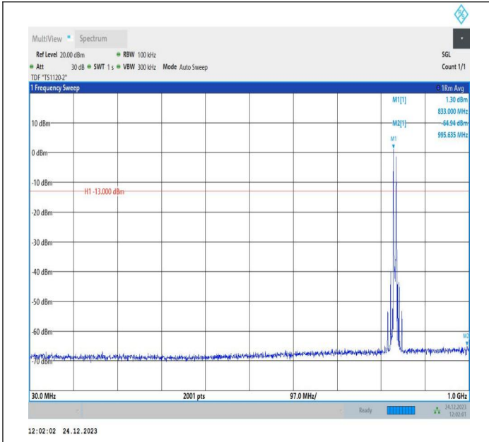
5-5-5MHz-3MHz-QPSK-QPSK-20510-20549-1RB#0-1RB#15-30~1000MHz-PASS
