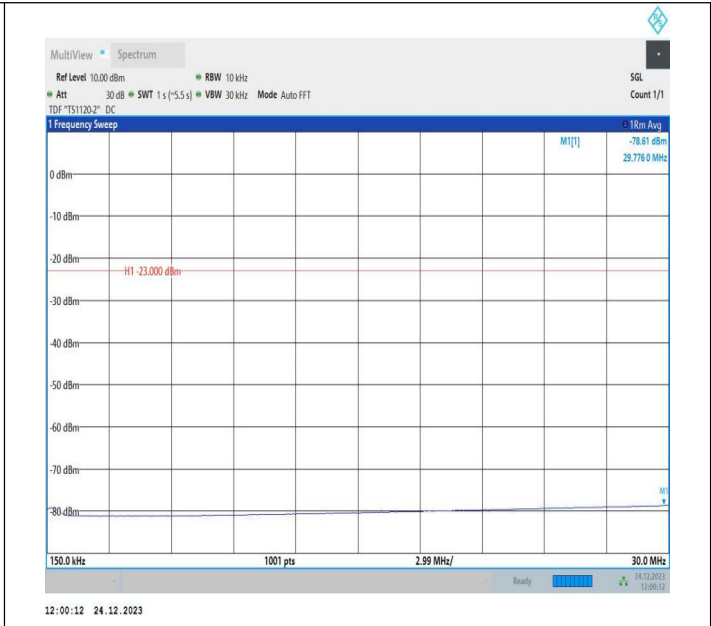
5-5-5MHz-3MHz-QPSK-QPSK-20510-20549-1RB#0-0RB#0-0. 15~30MHz-PASS
