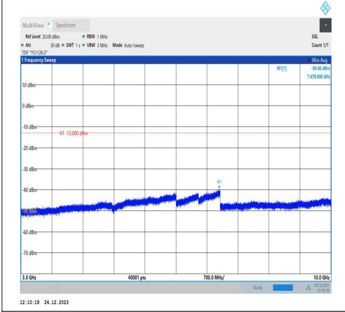
5-5-5MHz-10MHz-QPSK-QPSK-20428-20500-1RB#0-1RB#49 -3000~10000MHz-PASS
