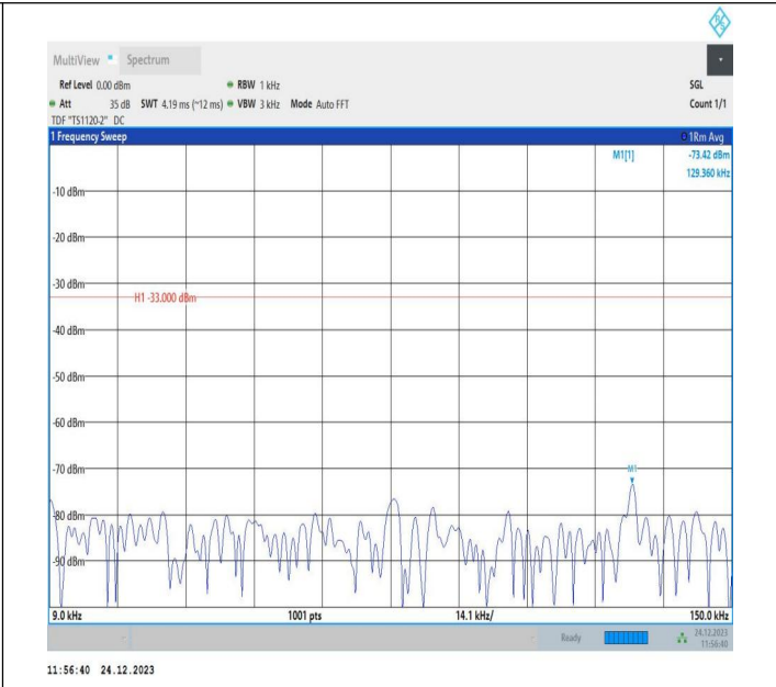
5-5-5MHz-3MHz-QPSK-QPSK-20425-20464-1RB#24-0RB#0-0 .009~0.15MHz-PASS
