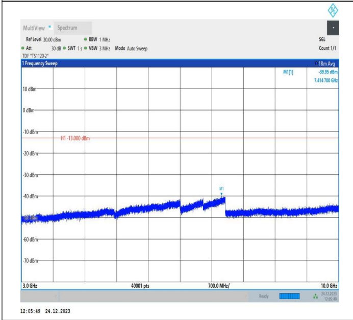
5-5-5MHz-3MHz-QPSK-QPSK-20595-20634-1RB#0-1RB#15-3000~10000MHz-PASS
