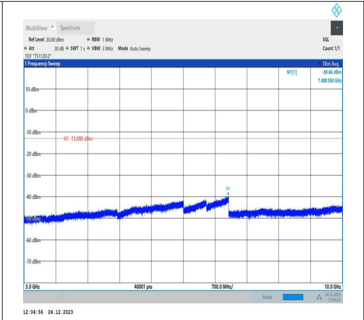
5-5-5MHz-3MHz-QPSK-QPSK-20595-20634-1RB#24-0RB#0-3000~10000MHz-PASS
