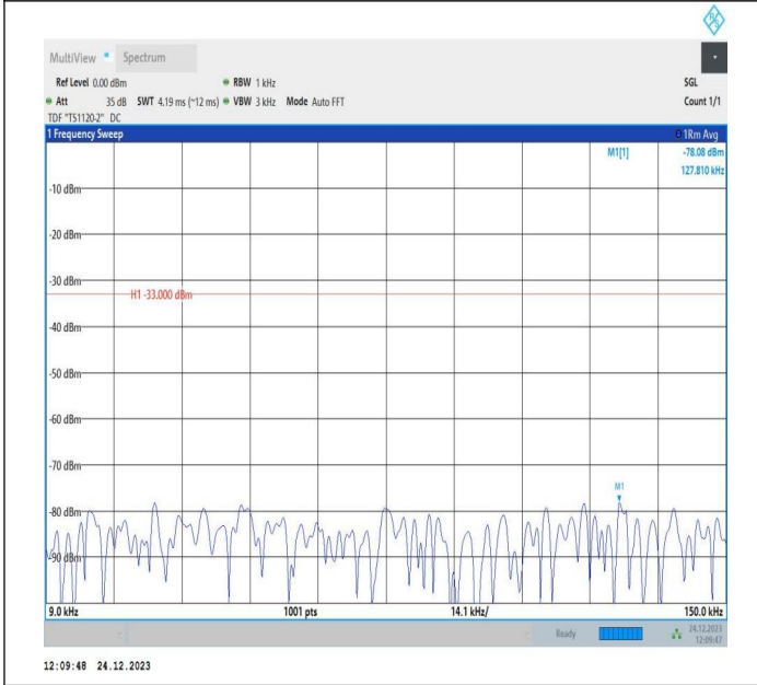
5-5-5MHz-10MHz-QPSK-QPSK-20428-20500-1RB#0-1RB#49 -0.009~0.15MHz-PASS
