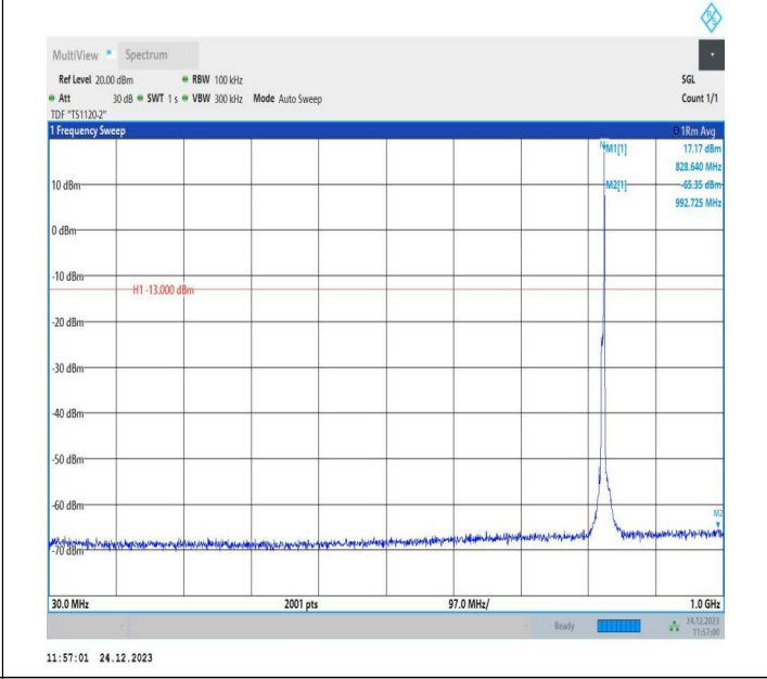
5-5-5MHz-3MHz-QPSK-QPSK-20425-20464-1RB#24-0RB#0-3 0~1000MHz-PASS
