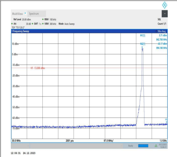
5-5-5MHz-3MHz-QPSK-QPSK-20595-20634-25RB#0-15RB#0- 30~1000MHz-PASS
