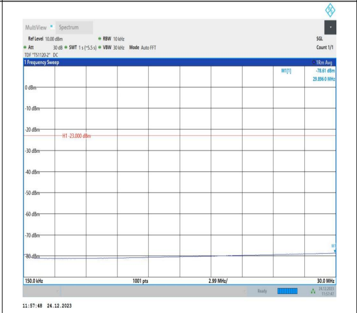
5-5-5MHz-3MHz-QPSK-QPSK-20425-20464-1RB#0-1RB#15-0.15~30MHz-PASS
