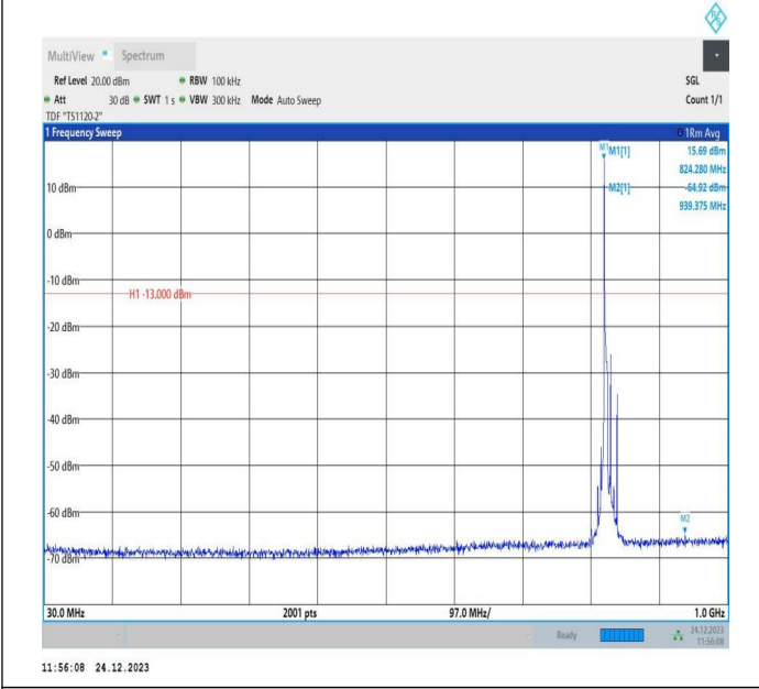
5-5-5MHz-3MHz-QPSK-QPSK-20425-20464-1RB#0-0RB#0-3 0~1000MHz-PASS
