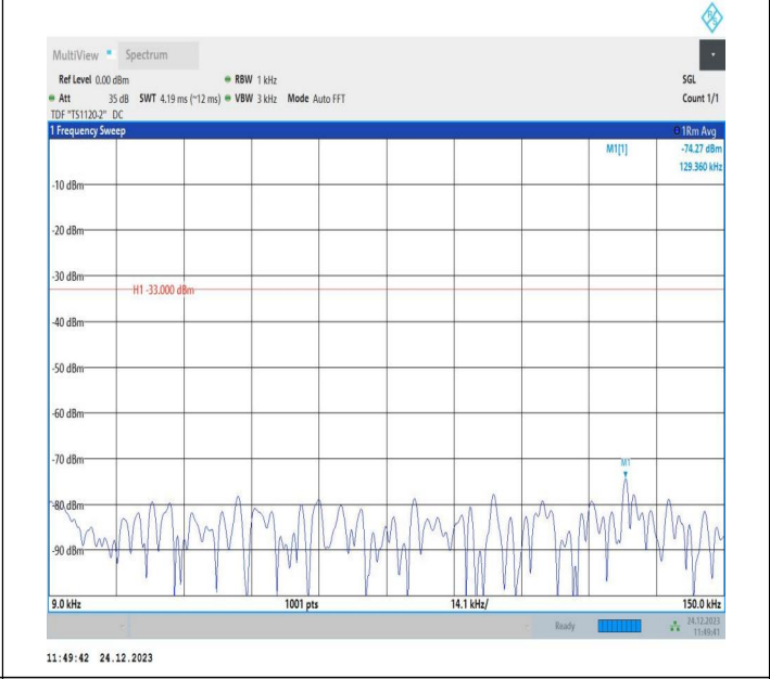
5-5-3MHz-5MHz-QPSK-QPSK-20501-20540-15RB#0-25RB#0-0.009~0.15MHz-PASS
