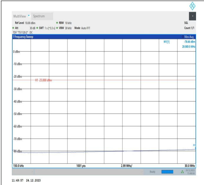
5-5-3MHz-5MHz-QPSK-QPSK-20501-20540-15RB#0-25RB#0 -0.15~30MHz-PASS
