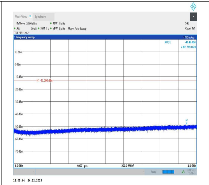
5-5-5MHz-3MHz-QPSK-QPSK-20595-20634-1RB#0-1RB#15-1000~3000MHz-PASS
