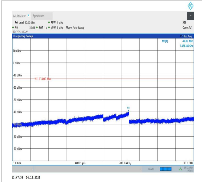
5-5-3MHz-5MHz-QPSK-QPSK-20501-20540-1RB#0-0RB#0-3 000~1000MHz-PASS
