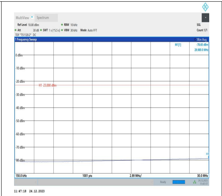
5-5-3MHz-5MHz-QPSK-QPSK-20501-20540-1RB#0-0RB#0-0.15~30MHz-PASS
