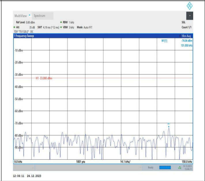
5-5-5MHz-3MHz-QPSK-QPSK-20595-20634-25RB#0-15RB#0-0.009~0.15MHz-PASS
