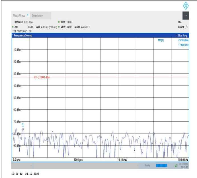
5-5-5MHz-3MHz-QPSK-QPSK-20510-20549-1RB#0-1RB#15-0.009~0.15MHz-PASS
