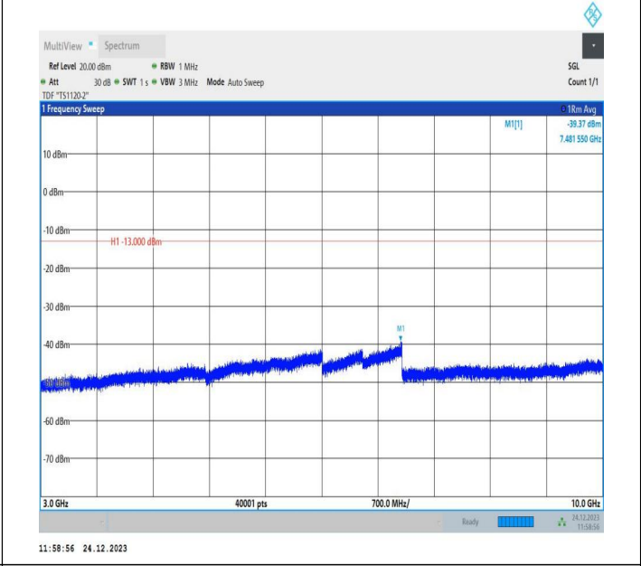
5-5-5MHz-3MHz-QPSK-QPSK-20425-20464-25RB#0-15RB#0- 3000~10000MHz-PASS
