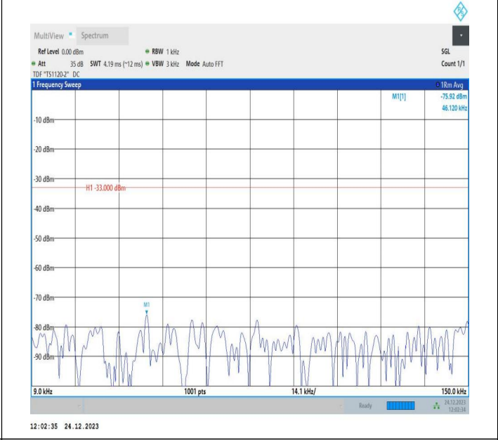
5-5-5MHz-3MHz-QPSK-QPSK-20510-20549-25RB#0-15RB#0-0.009~0.15MHz-PASS
