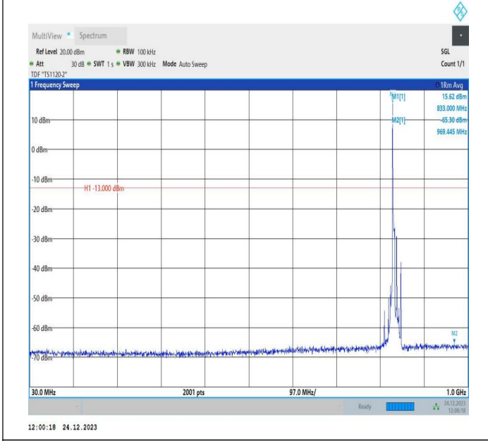
5-5-5MHz-3MHz-QPSK-QPSK-20510-20549-1RB#0-0RB#0-3 0~1000MHz-PASS
