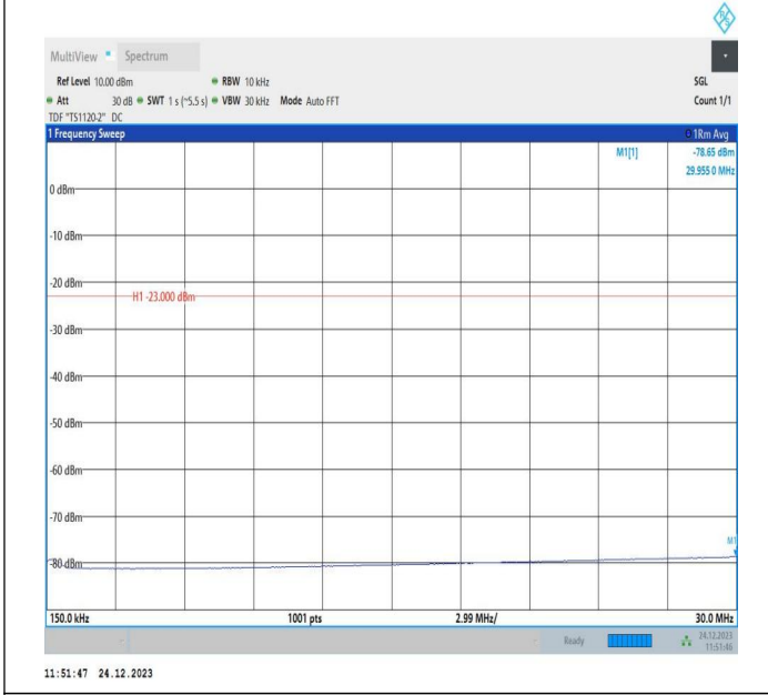
5-5-3MHz-5MHz-QPSK-QPSK-20586-20625-1RB#14-0RB#0-0 0.15~30MHz-PASS
