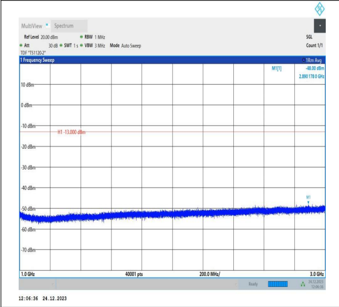
5-5-5MHz-3MHz-QPSK-QPSK-20595-20634-25RB#0-15RB#0 -1000~3000MHz-PASS
