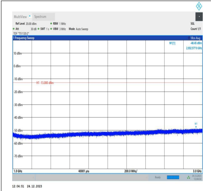
5-5-5MHz-3MHz-QPSK-QPSK-20595-20634-1RB#24-0RB#0-1000~3000MHz-PASS
