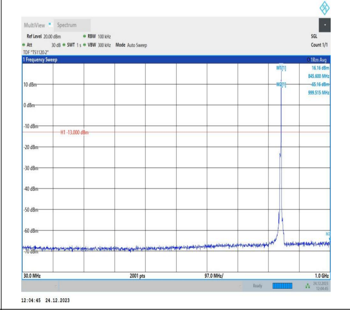
5-5-5MHz-3MHz-QPSK-QPSK-20595-20634-1RB#24-0RB#0-3 0~1000MHz-PASS
