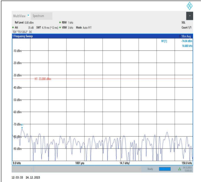
5-5-5MHz-3MHz-QPSK-QPSK-20595-20634-1RB#0-0RB#0-0. 009~0.15MHz-PASS
