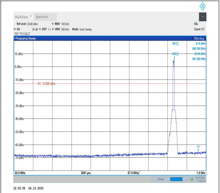
5-5-5MHz-3MHz-QPSK-QPSK-20510-20549-25RB#0-15RB#0- 30~1000MHz-PASS
