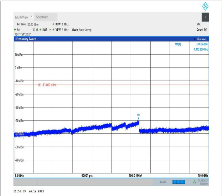
5-5-3MHz-5MHz-QPSK-QPSK-20586-20625-1RB#14-0RB#0-3000~10000MHz-PASS
