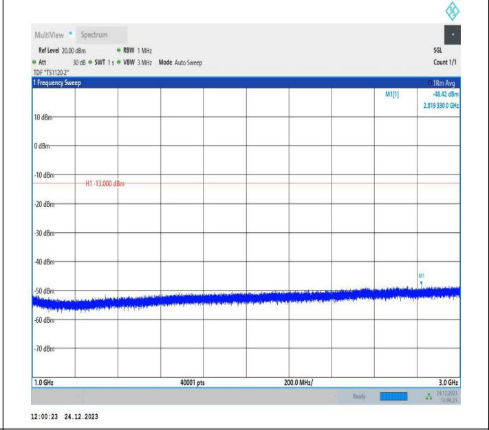
5-5-5MHz-3MHz-QPSK-QPSK-20510-20549-1RB#0-0RB#0-10 00~3000MHz-PASS
