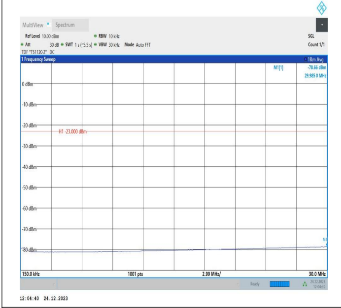
5-5-5MHz-3MHz-QPSK-QPSK-20595-20634-1RB#24-0RB#0-0 0.15~30MHz-PASS
