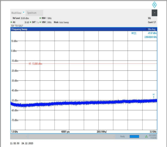
5-5-3MHz-5MHz-QPSK-QPSK-20586-20625-1RB#0-1RB#24-1000~3000MHz-PASS
