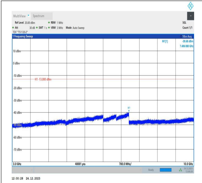
5-5-5MHz-3MHz-QPSK-QPSK-20510-20549-1RB#0-0RB#0-3 000~1000MHz-PASS
