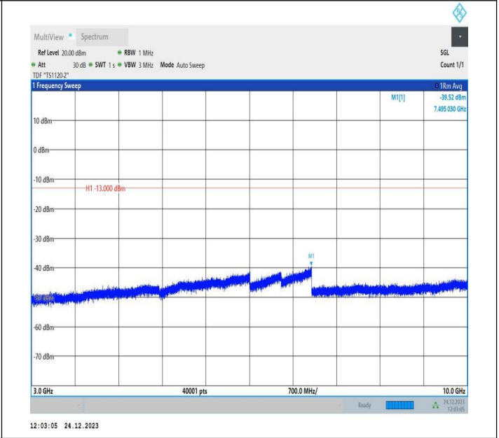
5-5-5MHz-3MHz-QPSK-QPSK-20510-20549-25RB#0-15RB#0- 3000~10000MHz-PASS
