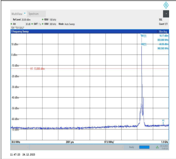
5-5-3MHz-5MHz-QPSK-QPSK-20501-20540-1RB#0-0RB#0-0.0~1000MHz-PASS
