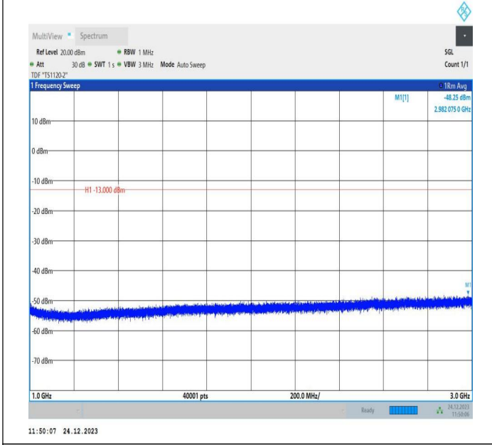
5-5-3MHz-5MHz-QPSK-QPSK-20501-20540-15RB#0-25RB#0 -1000~3000MHz-PASS
