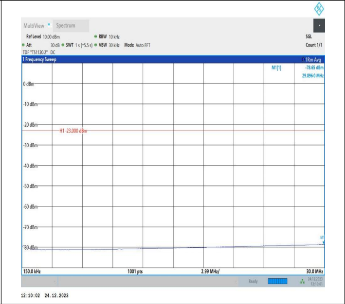
5-5-5MHz-10MHz-QPSK-QPSK-20428-20500-1RB#0-1RB#49- 0.15~30MHz-PASS
