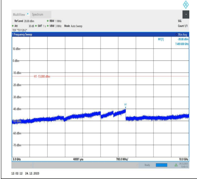
5-5-5MHz-3MHz-QPSK-QPSK-20510-20549-1RB#0-1RB#15-3000~10000MHz-PASS
