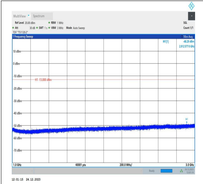
5-5-5MHz-3MHz-QPSK-QPSK-20510-20549-1RB#24-0RB#0-1000~3000MHz-PASS
