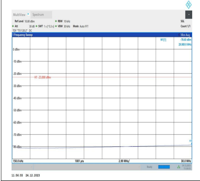
5-5-5MHz-3MHz-QPSK-QPSK-20425-20464-1RB#24-0RB#0-0 0.15~30MHz-PASS
