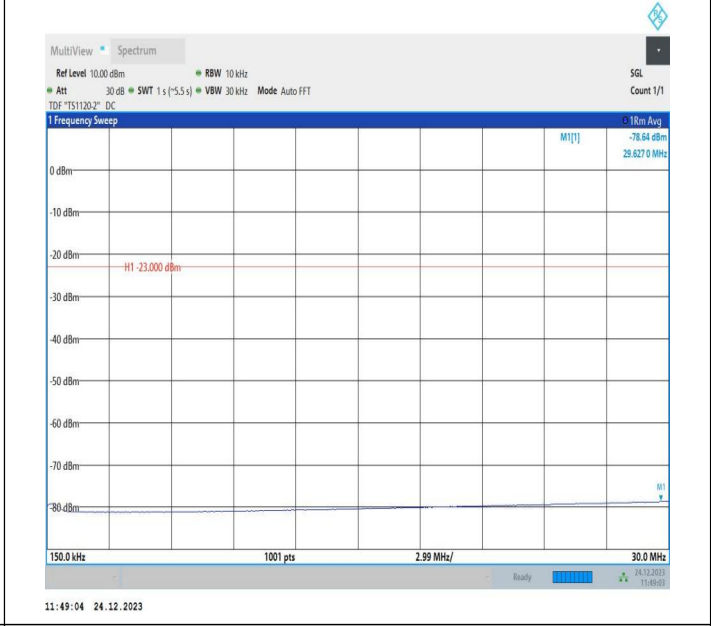
5-5-3MHz-5MHz-QPSK-QPSK-20501-20540-1RB#0-1RB#24-0.15~30MHz-PASS
