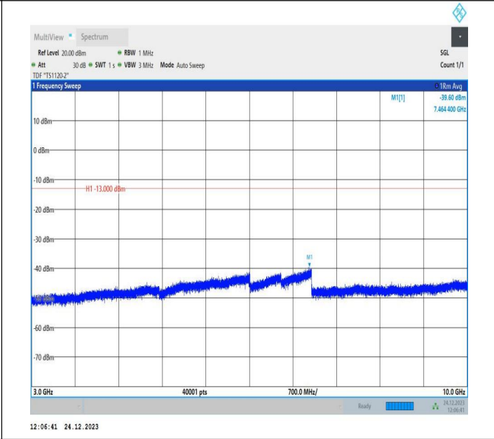
5-5-5MHz-3MHz-QPSK-QPSK-20595-20634-25RB#0-15RB#0- 3000~10000MHz-PASS
