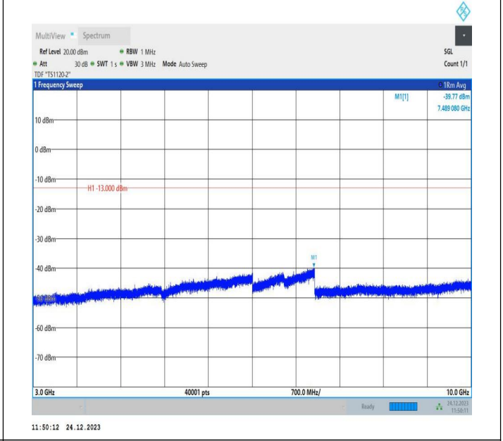
5-5-3MHz-5MHz-QPSK-QPSK-20501-20540-15RB#0-25RB#0- 3000~10000MHz-PASS
