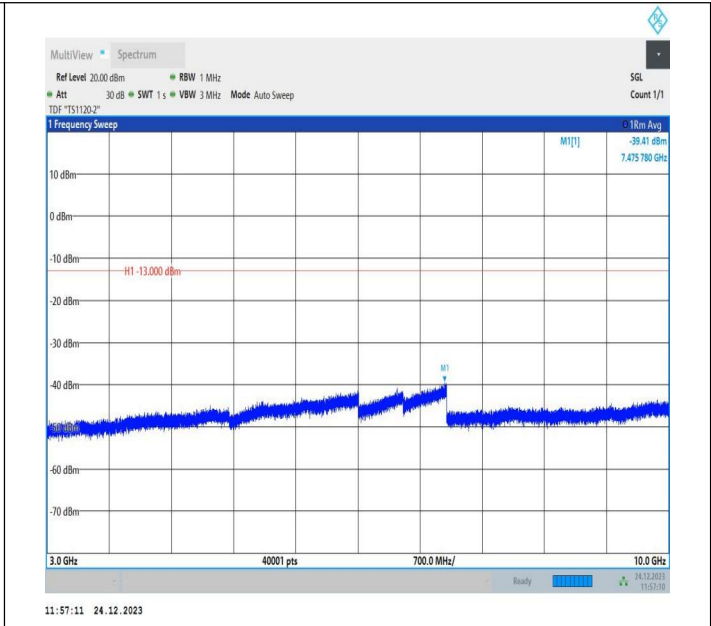
5-5-5MHz-3MHz-QPSK-QPSK-20425-20464-1RB#24-0RB#0-3000~10000MHz-PASS
