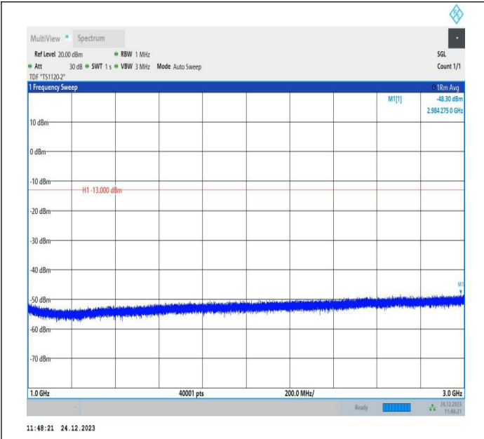
5-5-3MHz-5MHz-QPSK-QPSK-20501-20540-1RB#14-0RB#0-1000~3000MHz-PASS
