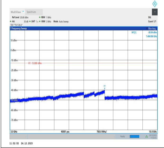
5-5-3MHz-5MHz-QPSK-QPSK-20586-20625-1RB#0-1RB#24-3000~10000MHz-PASS
