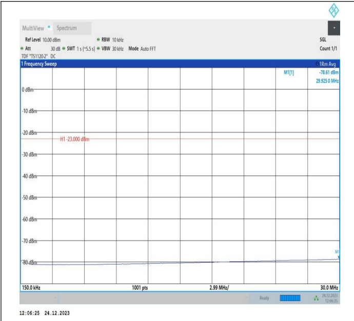
5-5-5MHz-3MHz-QPSK-QPSK-20595-20634-25RB#0-15RB#0 -0.15~30MHz-PASS
