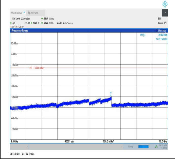
5-5-3MHz-5MHz-QPSK-QPSK-20501-20540-1RB#0-1RB#24-3000~10000MHz-PASS
