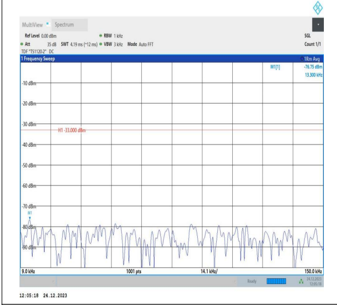
5-5-5MHz-3MHz-QPSK-QPSK-20595-20634-1RB#0-1RB#15-0.009~0.15MHz-PASS
