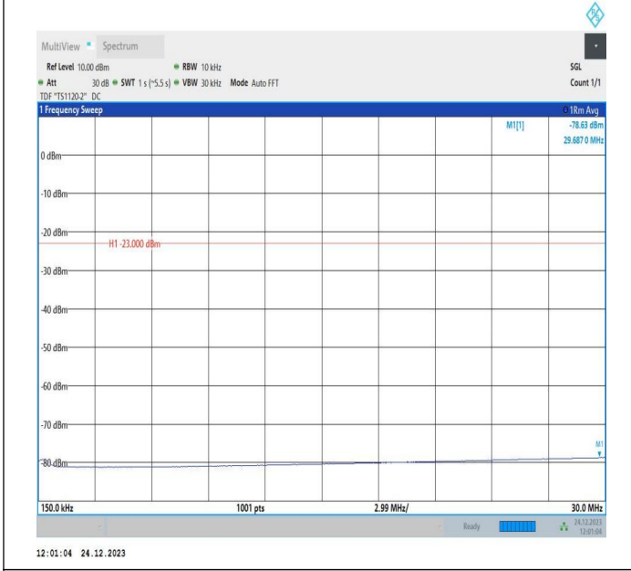
5-5-5MHz-3MHz-QPSK-QPSK-20510-20549-1RB#24-0RB#0-0 0.15~30MHz-PASS
