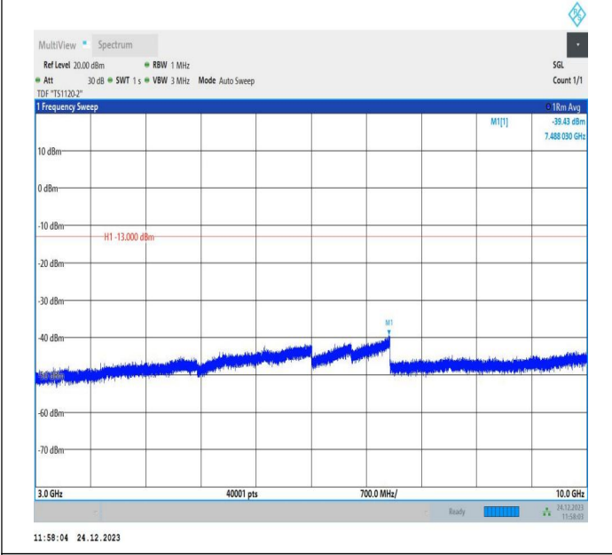
5-5-5MHz-3MHz-QPSK-QPSK-20425-20464-1RB#0-1RB#15-3000~10000MHz-PASS
