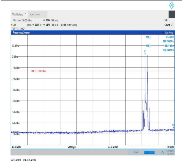
5-5-5MHz-10MHz-QPSK-QPSK-20428-20500-1RB#0-1RB#49 -30~1000MHz-PASS
