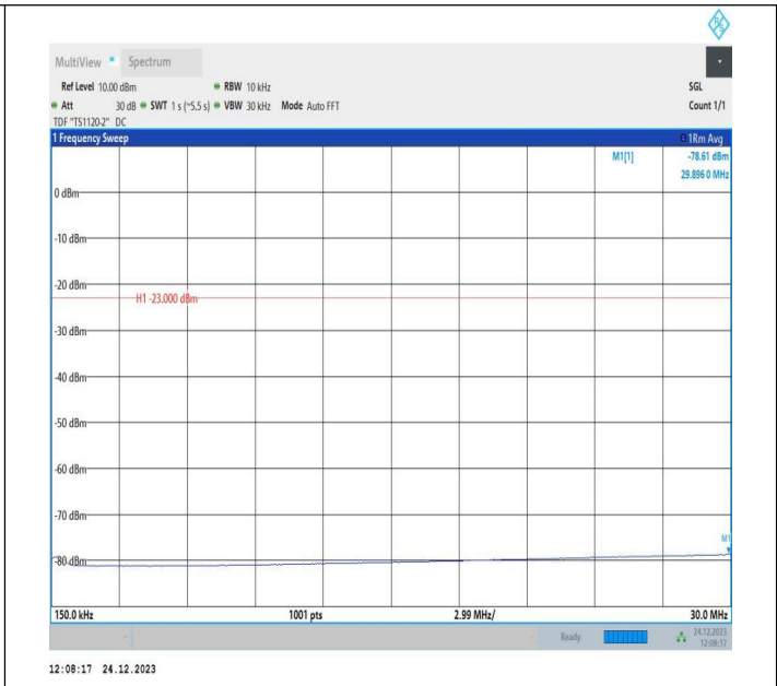
5-5-5MHz-10MHz-QPSK-QPSK-20428-20500-1RB#0-0RB#0-0.15~30MHz-PASS
