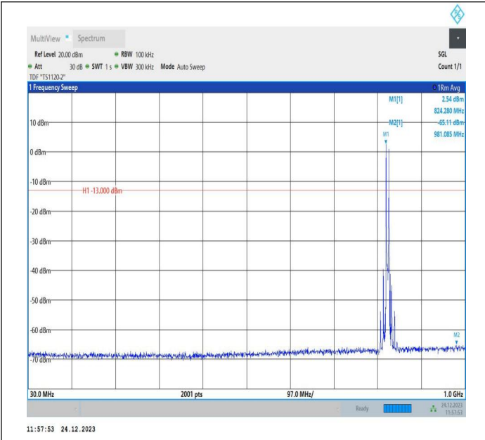
5-5-5MHz-3MHz-QPSK-QPSK-20425-20464-1RB#0-1RB#15-30~1000MHz-PASS
