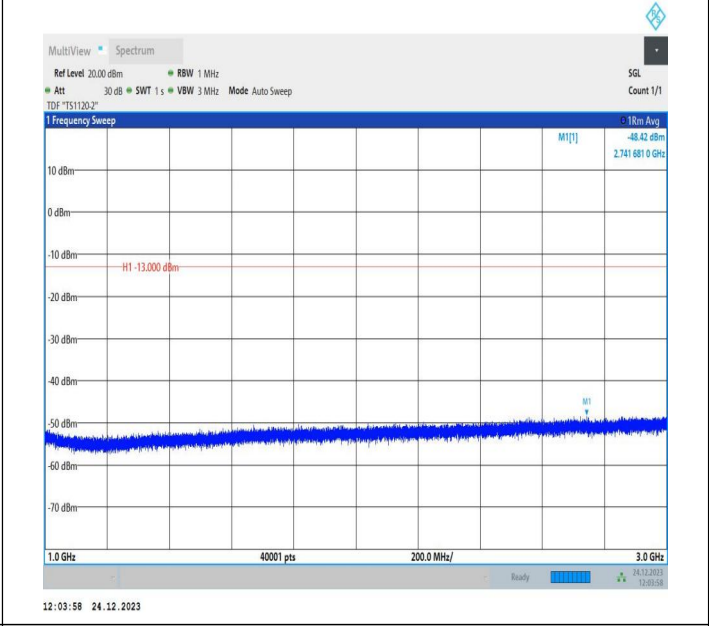
5-5-5MHz-3MHz-QPSK-QPSK-20595-20634-1RB#0-0RB#0-10 00~3000MHz-PASS
