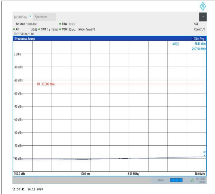
5-5-5MHz-3MHz-QPSK-QPSK-20425-20464-25RB#0-15RB#0 -0.15~30MHz-PASS
