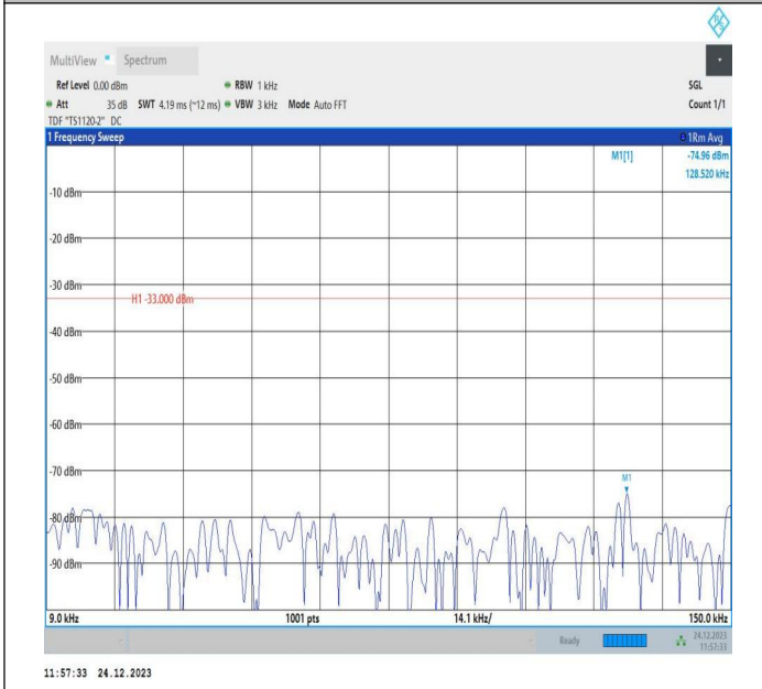
5-5-5MHz-3MHz-QPSK-QPSK-20425-20464-1RB#0-1RB#15-0.009~0.15MHz-PASS
