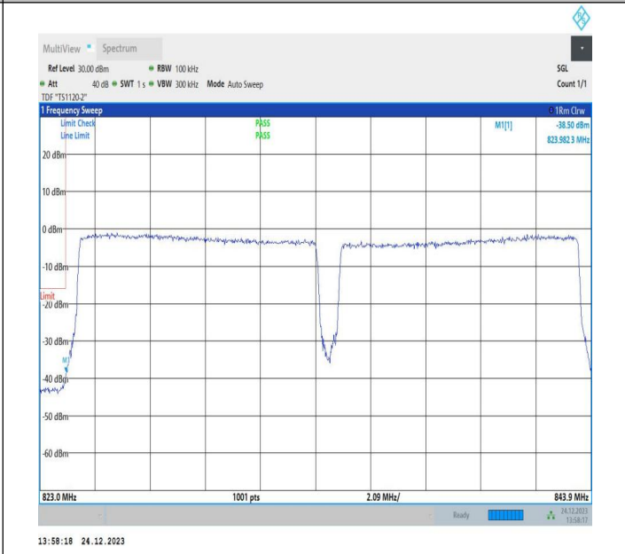
10MHz-10MHz_16QAM@16QAM-16QAM@16QAM_20450-20549_50RB#0@50RB#0-50RB#0@50RB#0
