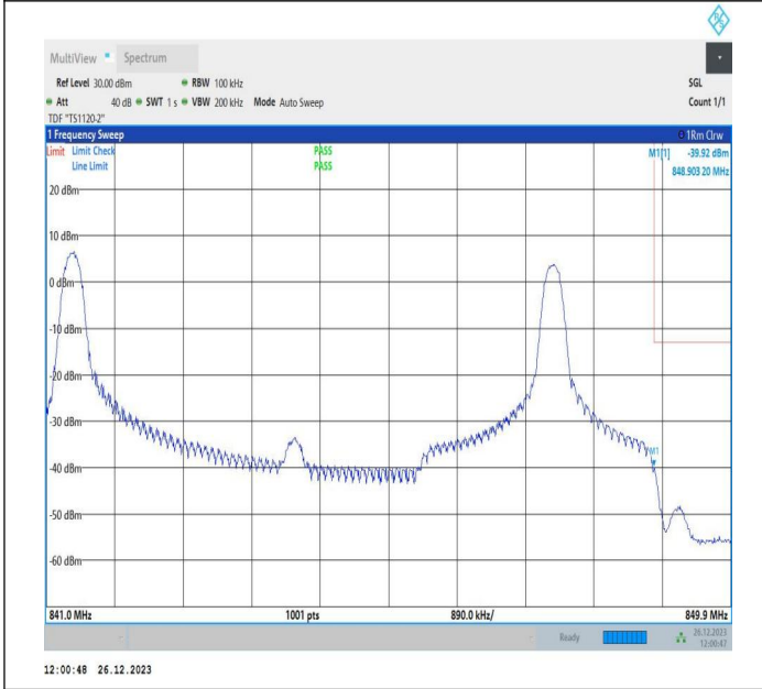
5MHz-3MHz_64QAM@64QAM-64QAM@64QAM_20595-20634_1RB#0@25RB#0-1RB#15@15RB#0
