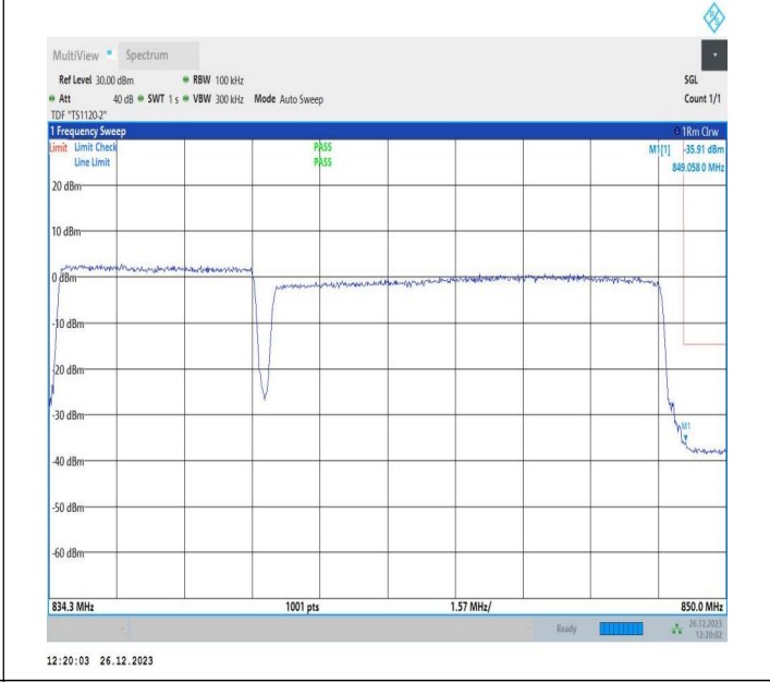
5MHz-10MHz_64QAM@64QAM-64QAM@64QAM_20528-206 00_25RB#0@25RB#0-50RB#0@50RB#0
