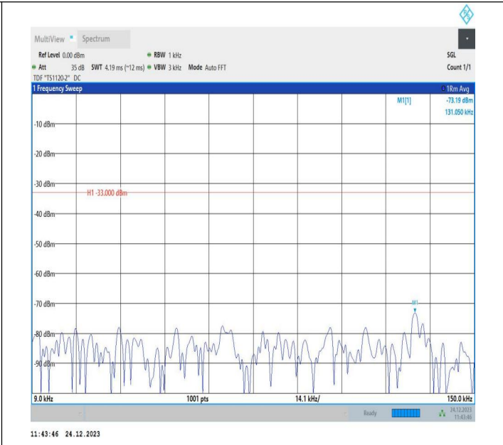
5-5-3MHz-5MHz-QPSK-QPSK-20416-20455-1RB#14-0RB#0-0 .009~0.15MHz-PASS
