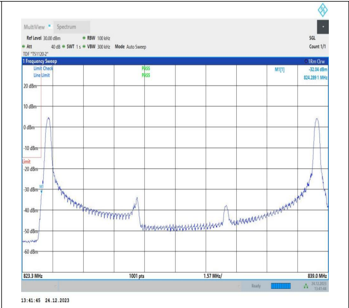
5MHz-10MHz_16QAM@16QAM-16QAM@16QAM_20428-20500_1 RB#0@25RB#0-1RB#49@50RB#0
