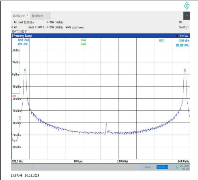
10MHz-10MHz_QPSK@QPSK-QPSK@QPSK_20450-20549_1RB#0@50RB#0-1RB#49@50RB#0
