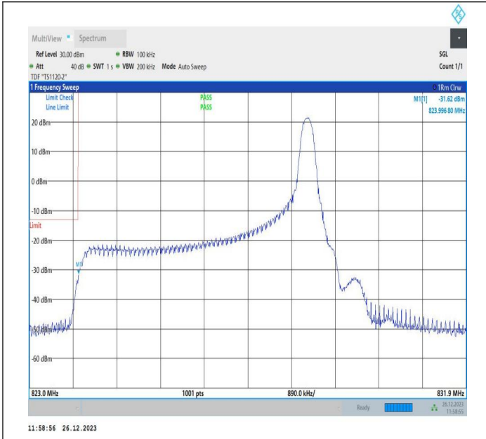
5MHz-3MHz_64QAM@64QAM-64QAM@64QAM_20425-20464_1RB#24@25RB#0-0RB#0@15RB#0
