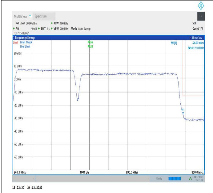
3MHz-5MHz_QPSK@QPSK-QPSK@QPSK_20586-20625_15 RB#0@15RB#0-25RB#0@25RB#0
