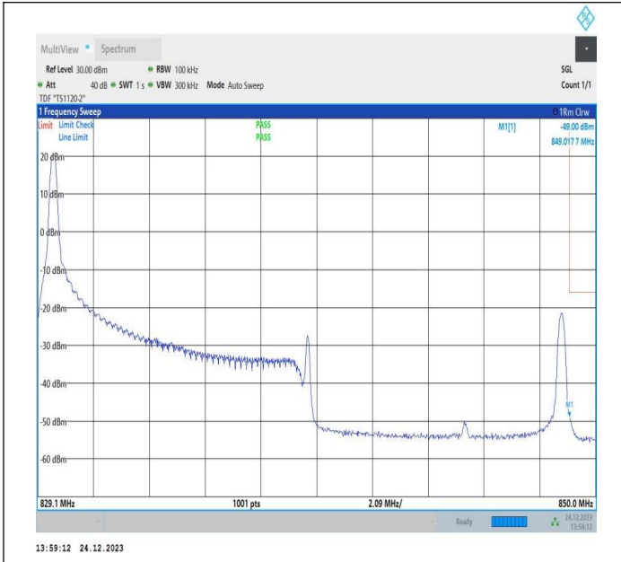
10MHz-10MHz_QPSK@QPSK-QPSK@QPSK_20501-20600_1RB#0@50RB#0-0RB#0@50RB#0
