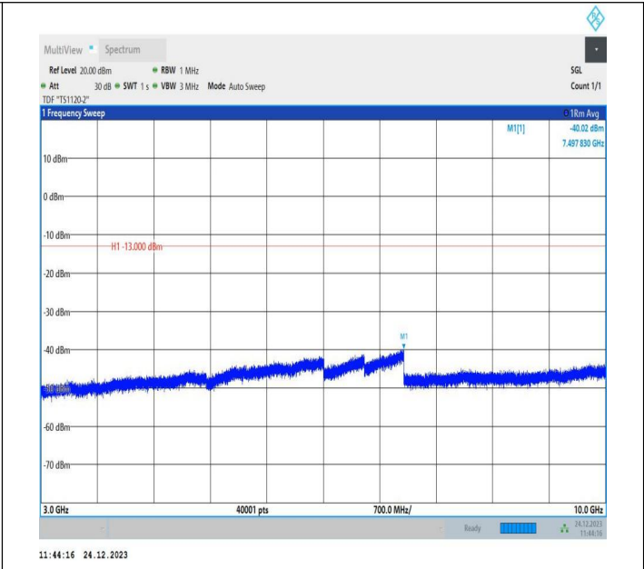
5-5-3MHz-5MHz-QPSK-QPSK-20416-20455-1RB#14-0RB#0-3000~10000MHz-PASS
