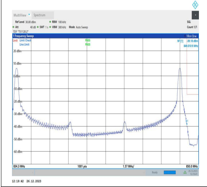
5MHz-10MHz_64QAM@64QAM-64QAM@64QAM_20528-20 600_1RB#0@25RB#0-1RB#49@50RB#0
