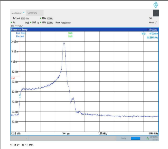
5MHz-10MHz_64QAM@64QAM-64QAM@64QAM_20428-205 00_1RB#24@25RB#0-0RB#0@50RB#0
