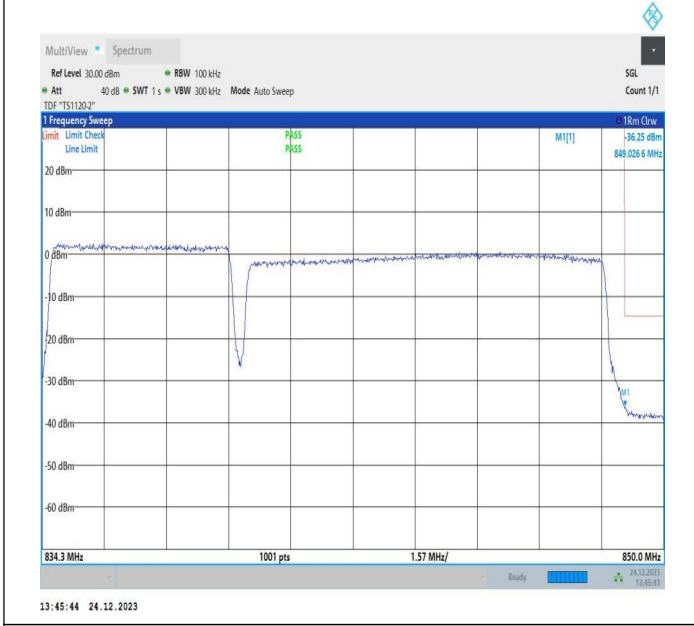
5MHz-10MHz_QPSK@QPSK-QPSK@QPSK_20528-20600_2 5RB#0@25RB#0-50RB#0@50RB#0
