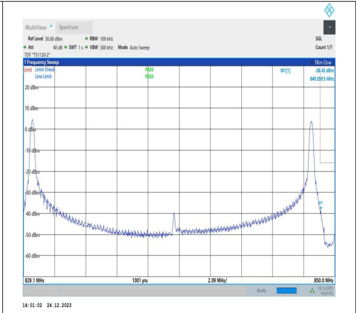
10MHz-10MHz_16QAM@16QAM-16QAM@16QAM_20501-20600_1RB#0@50RB#0-1RB#49@50RB#0
