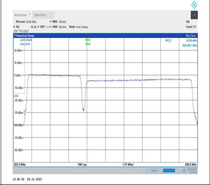
5MHz-10MHz_16QAM@16QAM-16QAM@16QAM_20428-20500_25RB#0@25RB#0-50RB#0@50RB#0
