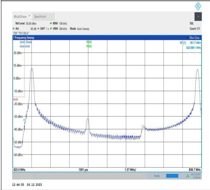
10MHz-5MHz_64QAM@64QAM-64QAM@64QAM_20450-20522_1RB#0@50RB#0-1RB#24@25RB#0
