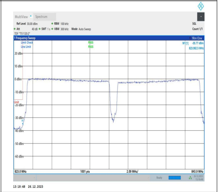
10MHz-10MHz_64QAM@64QAM-64QAM@64QAM_20450-20 549_50RB#0@50RB#0-50RB#0@50RB#0
