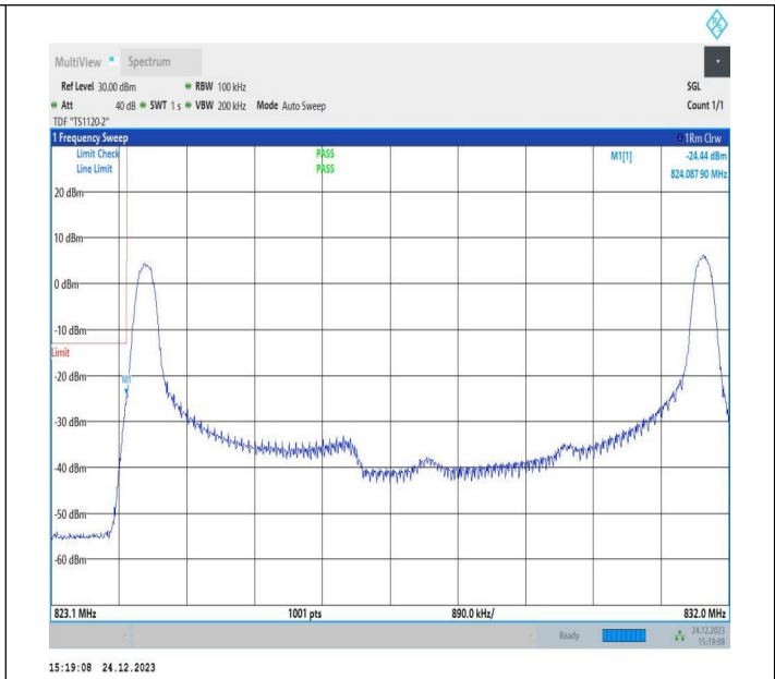
3MHz-5MHz_16QAM@16QAM-16QAM@16QAM_20416-2045 5_1RB#0@15RB#0-1RB#24@25RB#0
