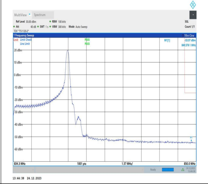
5MHz-10MHz_16QAM@16QAM-16QAM@16QAM_20528-20600_1 RB#24@25RB#0-0RB#0@50RB#0
