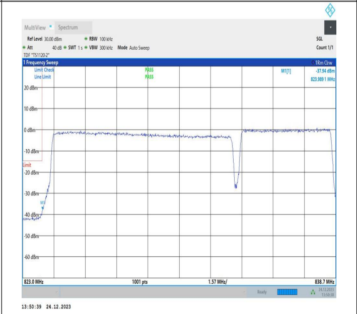
10MHz-5MHz_16QAM@16QAM-16QAM@16QAM_20450-20522_50RB#0@50RB#0-25RB#0@25RB#0
