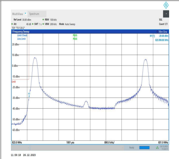
5MHz-3MHz_64QAM@64QAM-64QAM@64QAM_20425-20464_1RB#0@25RB#0-1RB#15@15RB#0
