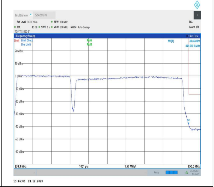
5MHz-10MHz_16QAM@16QAM-16QAM@16QAM_20528-20600_25RB#0@25RB#0-50RB#0@50RB#0
