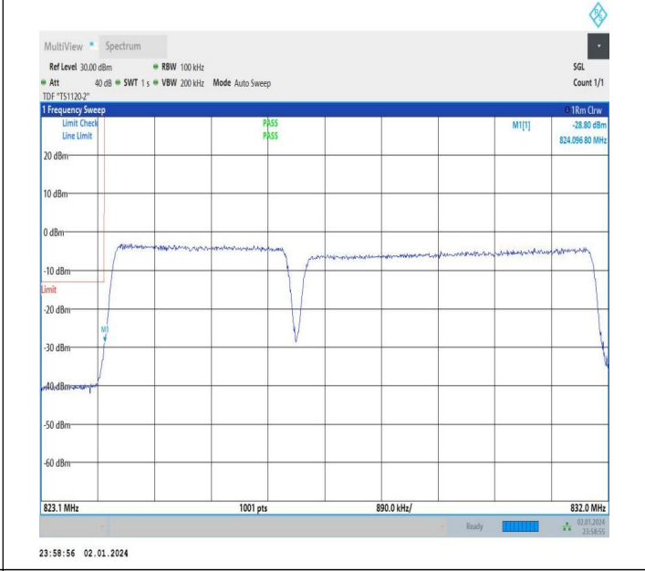
3MHz-5MHz_64QAM@64QAM-64QAM@64QAM_20416-20455_15RB#0@15RB#0-25RB#0@25RB#0
