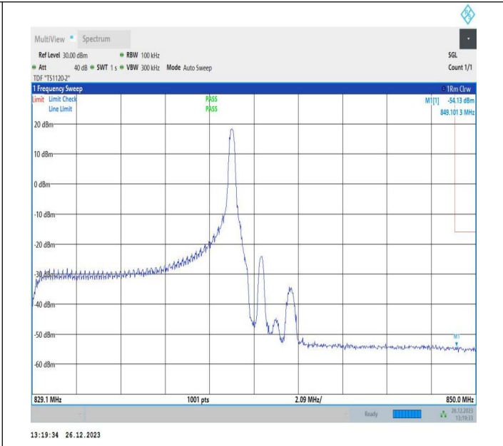
10MHz-10MHz_64QAM@64QAM-64QAM@64QAM_20501-20 600_1RB#49@50RB#0-0RB#0@50RB#0
