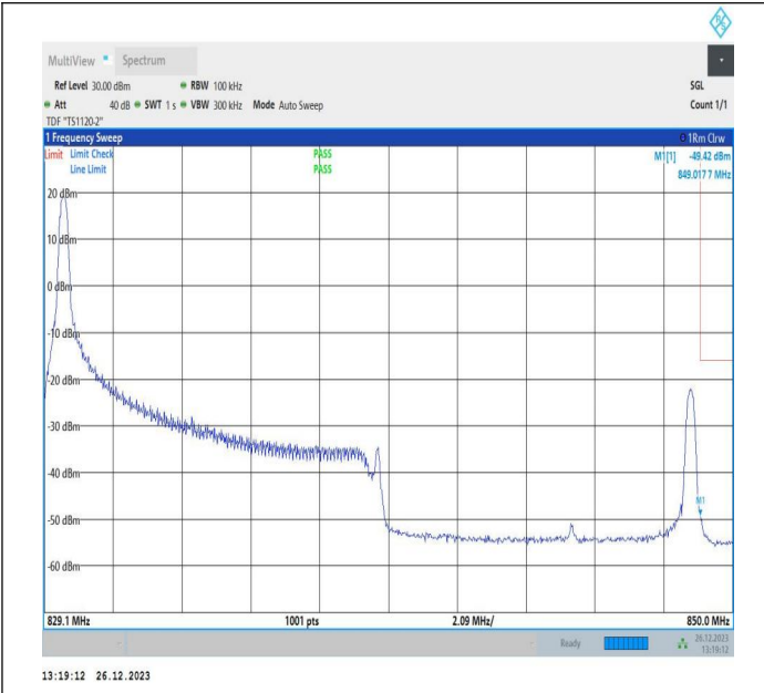
10MHz-10MHz_64QAM@64QAM-64QAM@64QAM_20501-2 0600_1RB#0@50RB#0-0RB#0@50RB#0
