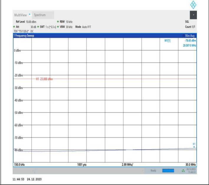
5-5-3MHz-5MHz-QPSK-QPSK-20416-20455-1RB#0-1RB#24-0.15~30MHz-PASS
