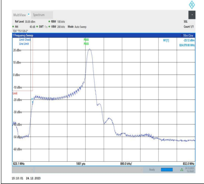
3MHz-5MHz_QPSK@QPSK-QPSK@QPSK_20416-20455_1 RB#14@15RB#0-0RB#0@25RB#0
