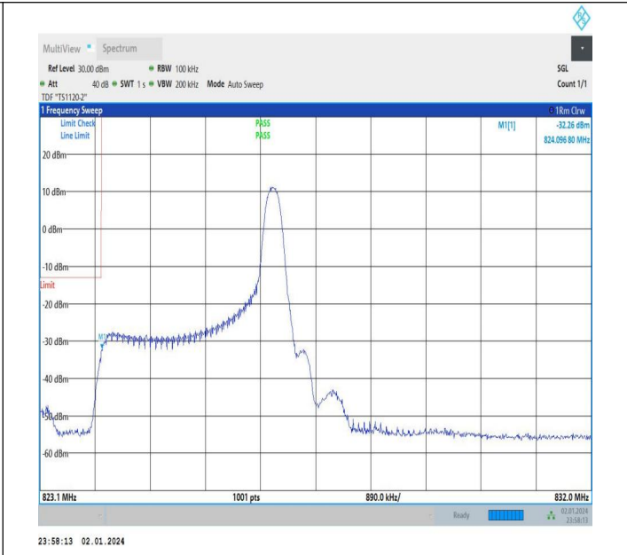
3MHz-5MHz_64QAM@64QAM-64QAM@64QAM_20416-20455_1RB#14@15RB#0-0RB#0@25RB#0
