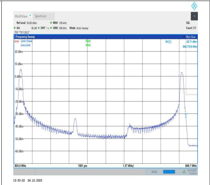
10MHz-5MHz_16QAM@16QAM-16QAM@16QAM_20550-20622_1RB#0@50RB#0-1RB#24@25RB#0
