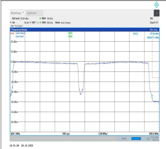
10MHz-10MHz_QPSK@QPSK-QPSK@QPSK_20501-20600_50RB#0@50RB#0-50RB#0@50RB#0
