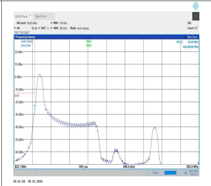
3MHz-5MHz_16QAM@16QAM-16QAM@16QAM_20416-20455_1 RB#0@15RB#0-0RB#0@25RB#0
