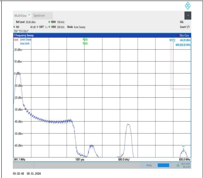
3MHz-5MHz_16QAM@16QAM-16QAM@16QAM_20586-20625_1RB#0@15RB#0-0RB#0@25RB#0
