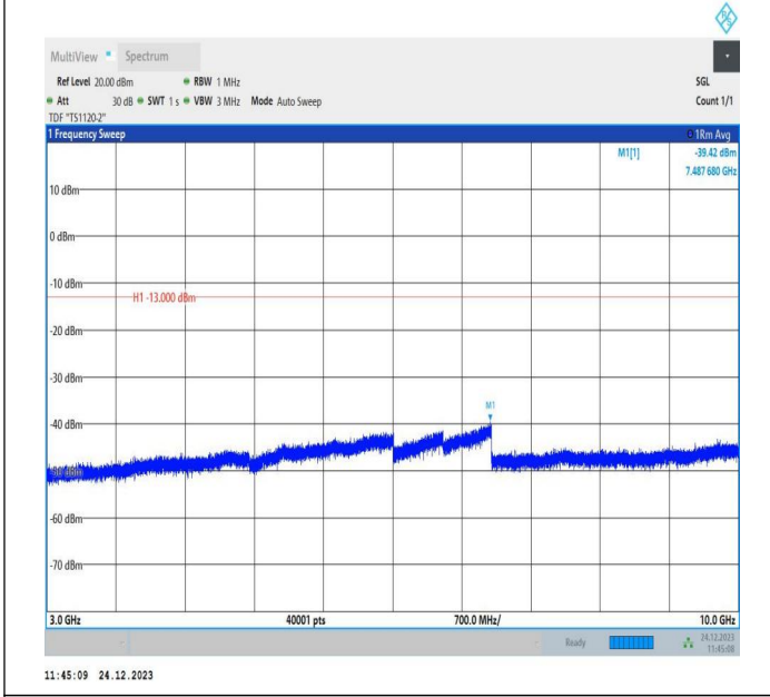
5-5-3MHz-5MHz-QPSK-QPSK-20416-20455-1RB#0-1RB#24-3000~10000MHz-PASS
