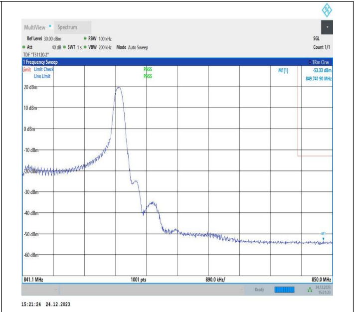
3MHz-5MHz_16QAM@16QAM-16QAM@16QAM_20586-20625_1 RB#14@15RB#0-0RB#0@25RB#0
