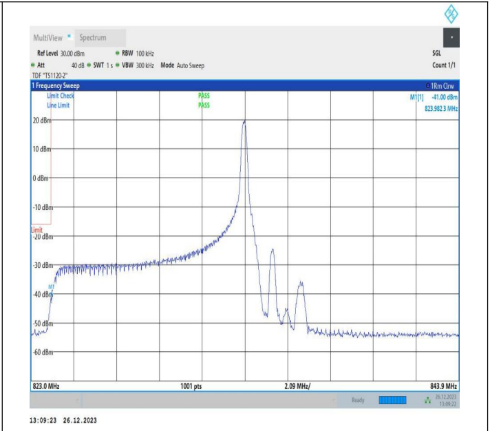
10MHz-10MHz_64QAM@64QAM-64QAM@64QAM_20450-20 549_1RB#49@50RB#0-0RB#0@50RB#0
