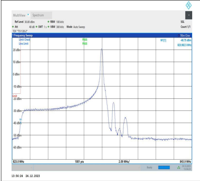
10MHz-10MHz_QPSK@QPSK-QPSK@QPSK_20450-20549_1RB#49@50RB#0-0RB#0@50RB#0
