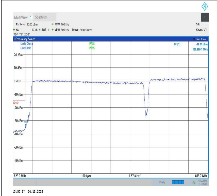
10MHz-5MHz_QPSK@QPSK-QPSK@QPSK_20450-20522_5 0RB#0@50RB#0-25RB#0@25RB#0
