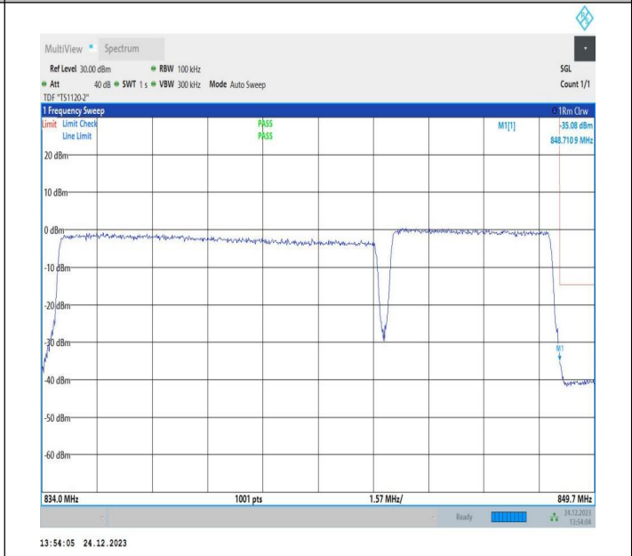
10MHz-5MHz_16QAM@16QAM-16QAM@16QAM_20550-20622_50RB#0@50RB#0-25RB#0@25RB#0
