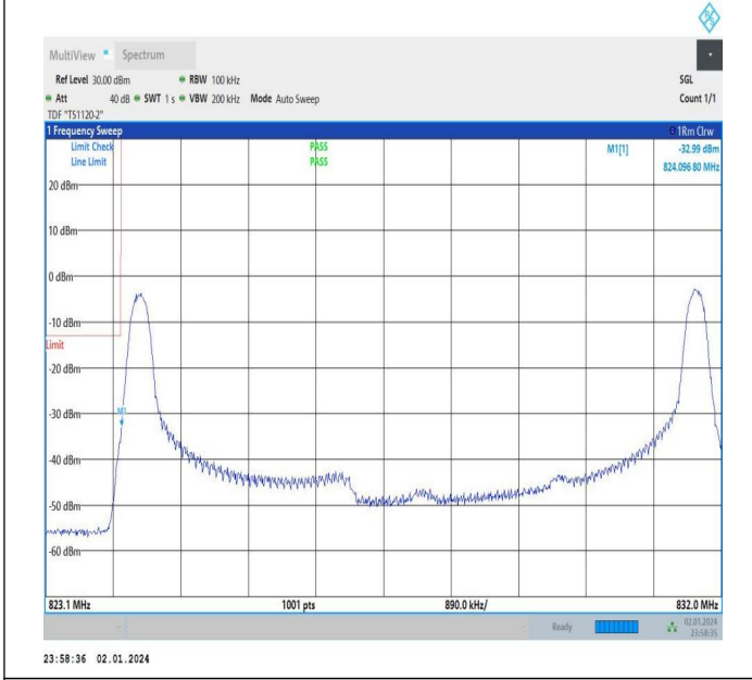
3MHz-5MHz_64QAM@64QAM-64QAM@64QAM_20416-20455_1RB#0@15RB#0-1RB#24@25RB#0
