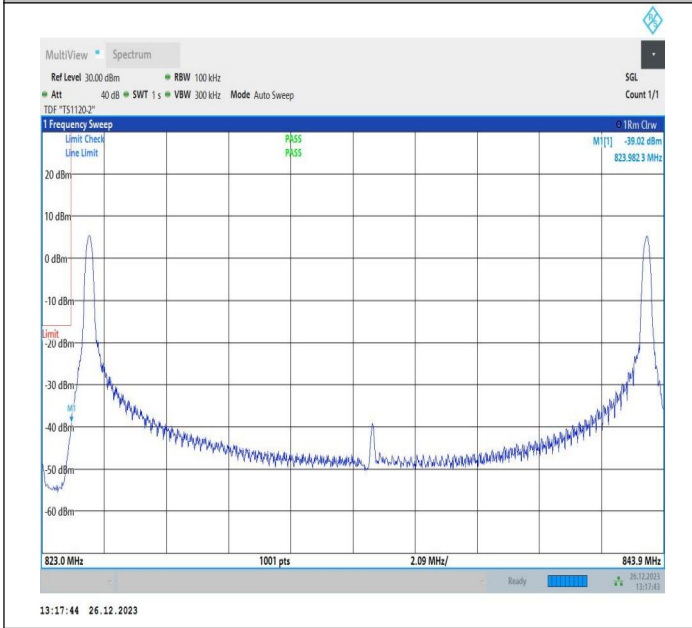
10MHz-10MHz_64QAM@64QAM-64QAM@64QAM_20450-2 0549_1RB#0@50RB#0-1RB#49@50RB#0
