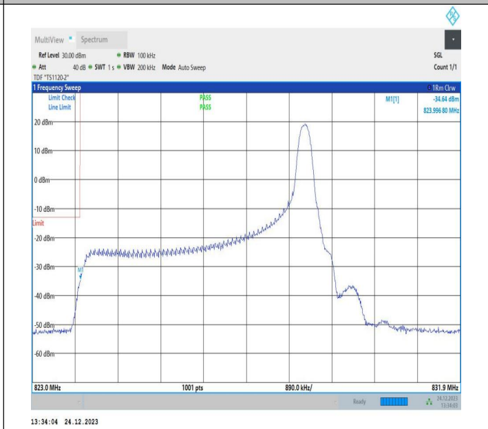
5MHz-3MHz_16QAM@16QAM-16QAM@16QAM_20425-20464_4_1RB#24@25RB#0-0RB#0@15RB#0
