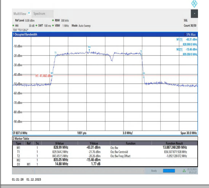
5-5-10MHz-5MHz-QPSK-QPSK-20500-20572-50RB#0-25RB#0-PASS
