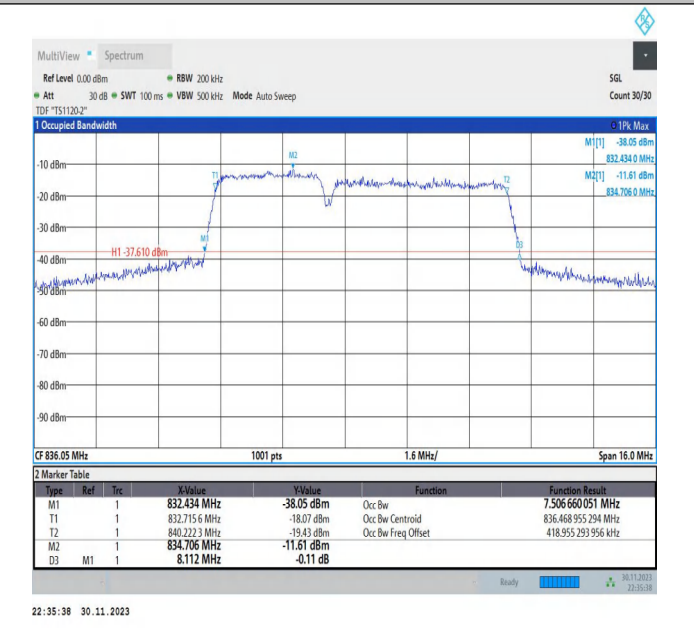
5-5-3MHz-5MHz-16QAM-16QAM-20501-20540-15RB#0-25RB#0-PASS
