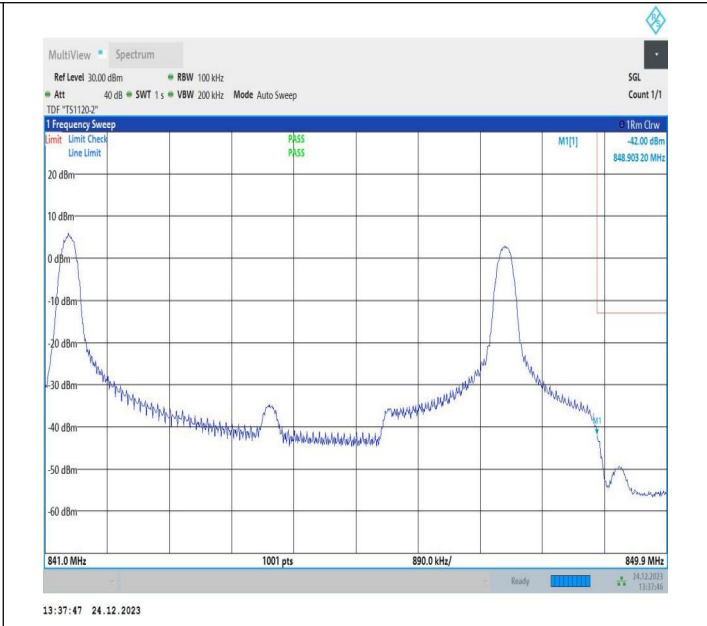
5MHz-3MHz_16QAM@16QAM-16QAM@16QAM_20595-20634_1RB#0@25RB#0-1RB#15@15RB#0
