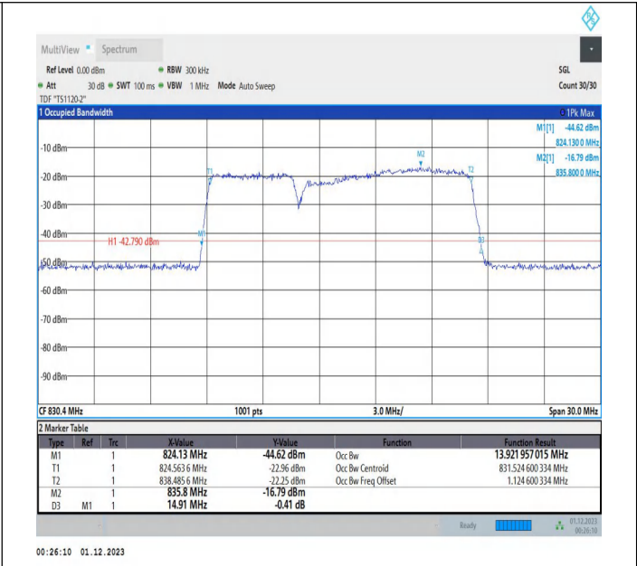
5-5-5MHz-10MHz-16QAM-16QAM-20428-20500-25RB#0-50RB#0-PASS
