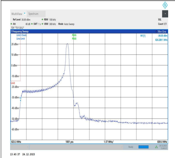
5MHz-10MHz_QPSK@QPSK-QPSK@QPSK_20428-20500_1 RB#24@25RB#0-0RB#0@50RB#0
