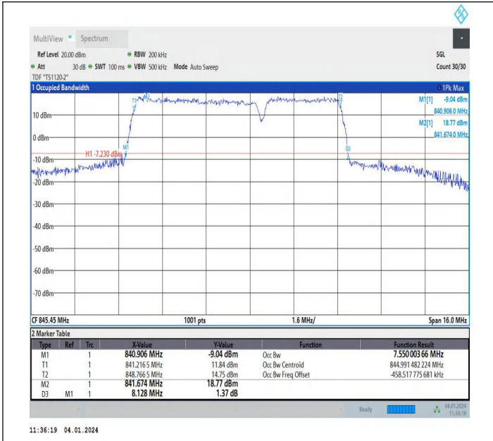
5-5-5MHz-3MHz-64QAM-64QAM-20595-20634-25RB#0-15RB #0-PASS
