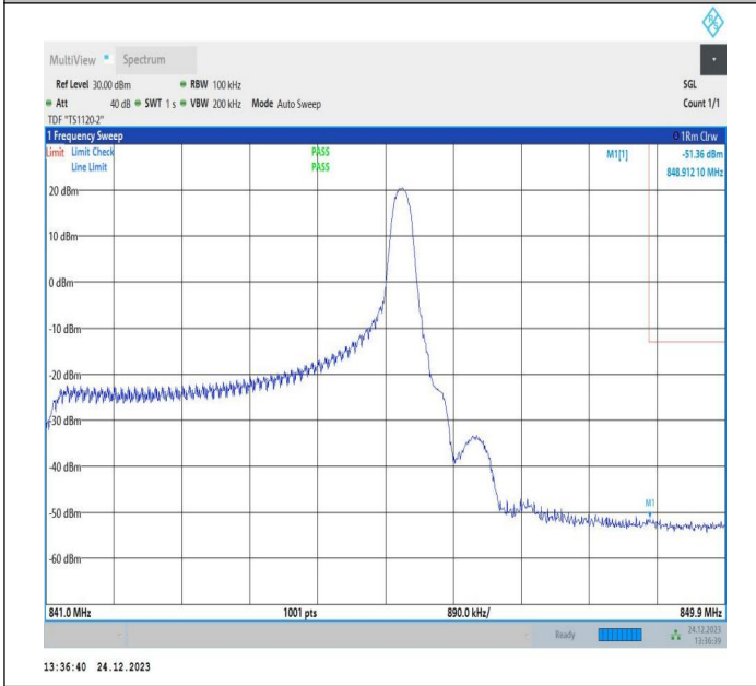
5MHz-3MHz_QPSK@QPSK-QPSK@QPSK_20595-20634_1RB#24@25RB#0-0RB#0@15RB#0
