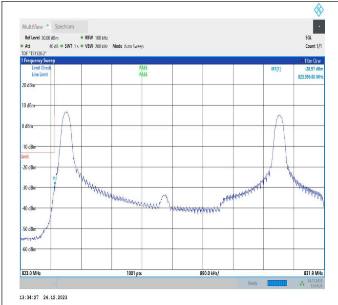
5MHz-3MHz_QPSK@QPSK-QPSK@QPSK_20425-20464_1 RB#0@25RB#0-1RB#15@15RB#0
