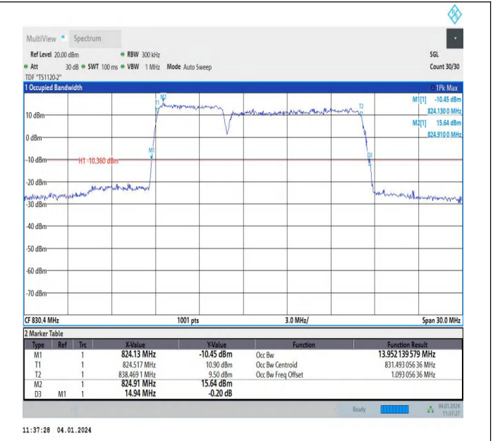
5-5-5MHz-10MHz-64QAM-64QAM-20428-20500-25RB#0-50R B#0-PASS
