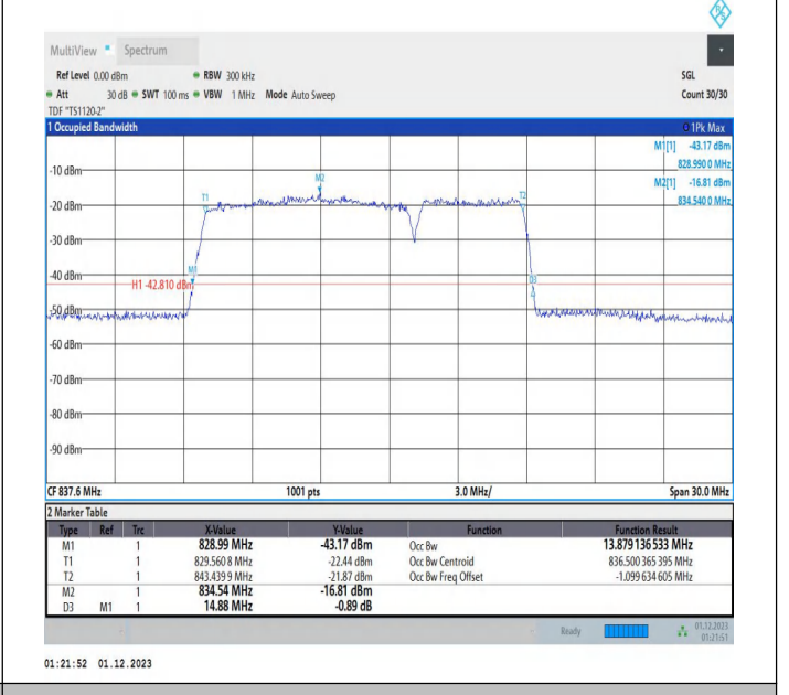
5-5-10MHz-5MHz-16QAM-16QAM-20500-20572-50RB#0-25R B#0-PASS
