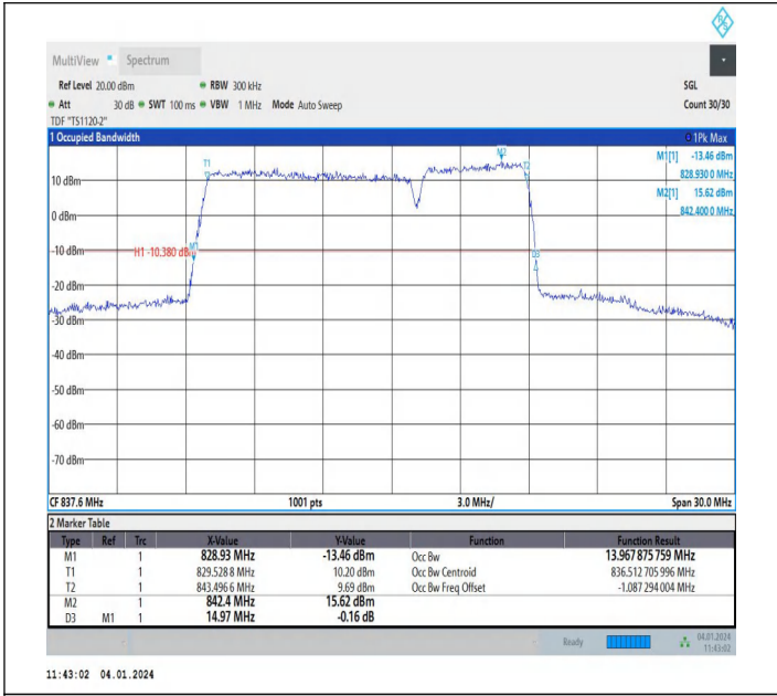
5-5-10MHz-5MHz-64QAM-64QAM-20500-20572-50RB#0-25R B#0-PASS
