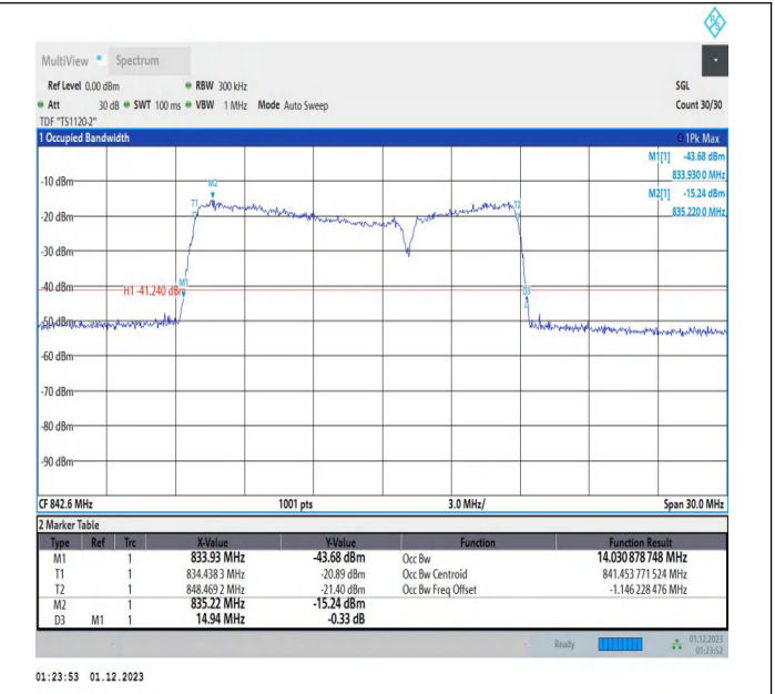
5-5-10MHz-5MHz-16QAM-16QAM-20550-20622-50RB#0-25RB#0-PASS
