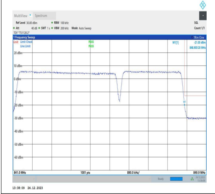
5MHz-3MHz_QPSK@QPSK-QPSK@QPSK_20595-20634_25 RB#0@25RB#0-15RB#0@15RB#0
