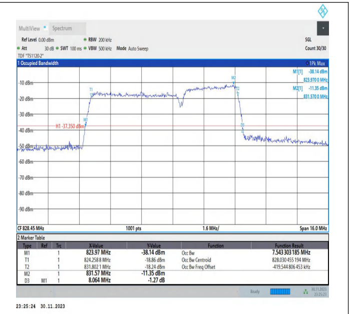
5-5-5MHz-3MHz-16QAM-16QAM-20425-20464-25RB#0-15RB#0-PASS
