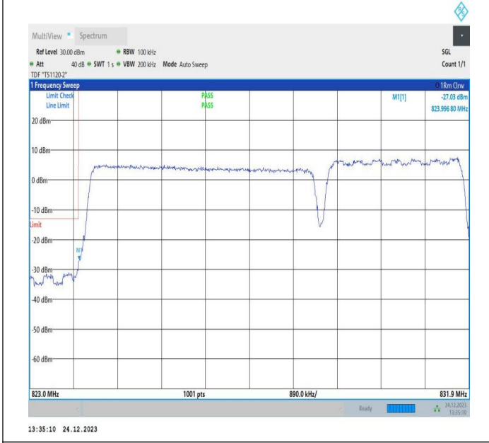
5MHz-3MHz_QPSK@QPSK-QPSK@QPSK_20425-20464_25 RB#0@25RB#0-15RB#0@15RB#0
