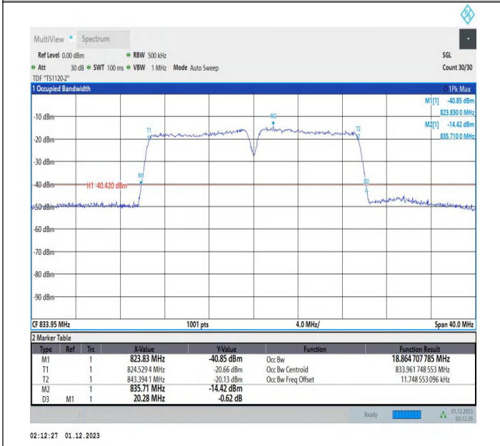
5-5-10MHz-10MHz-QPSK-QPSK-20450-20549-50RB#0-50RB#0-PASS
