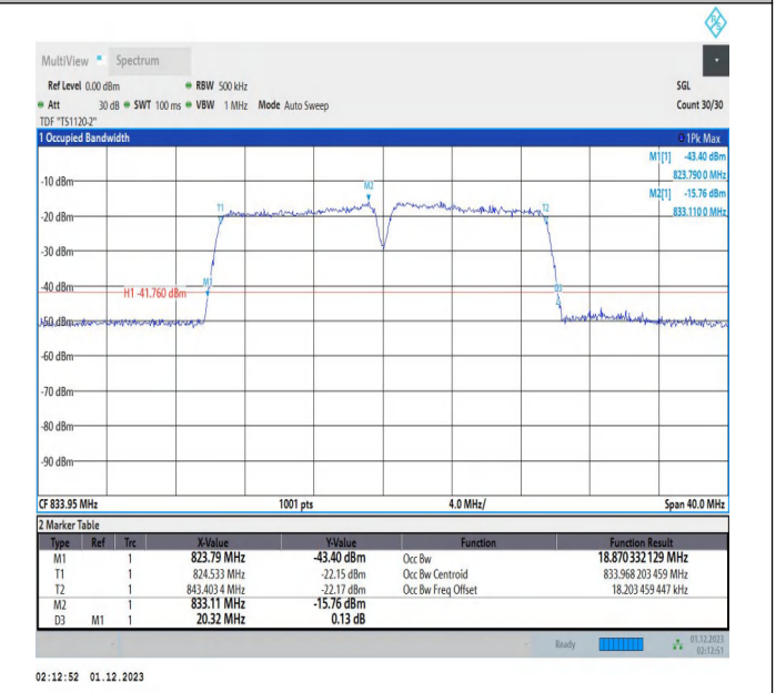
5-5-10MHz-10MHz-16QAM-16QAM-20450-20549-50RB#0-50RB#0-PASS
