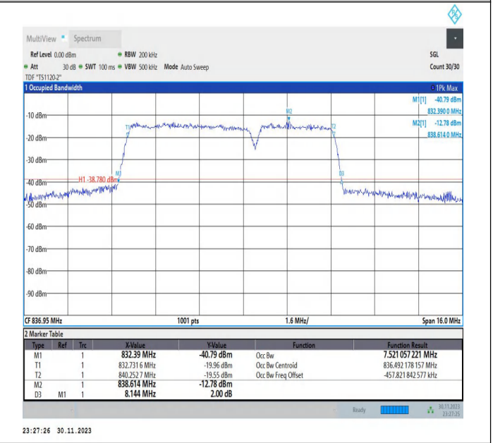
5-5-5MHz-3MHz-16QAM-16QAM-20510-20549-25RB#0-15RB#0-PASS
