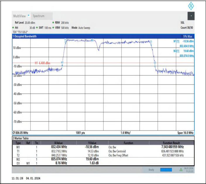
5-5-3MHz-5MHz-64QAM-64QAM-20501-20540-15RB#0-25RB #0-PASS
