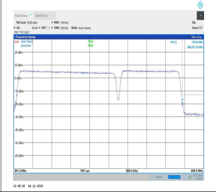
5MHz-3MHz_16QAM@16QAM-16QAM@16QAM_20595-20634_25RB#0@25RB#0-15RB#0@15RB#0
