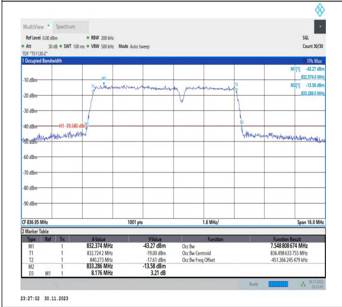
5-5-5MHz-3MHz-QPSK-QPSK-20510-20549-25RB#0-15RB#0-PASS
