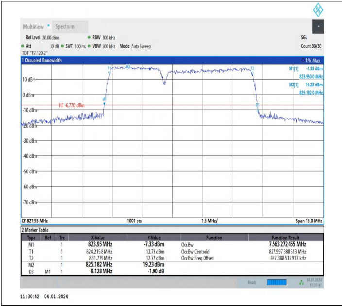
5-5-3MHz-5MHz-64QAM-64QAM-20416-20455-15RB#0-25RB #0-PASS
