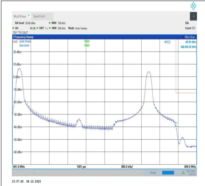
5MHz-3MHz_QPSK@QPSK-QPSK@QPSK_20595-20634_1 RB#0@25RB#0-1RB#15@15RB#0
