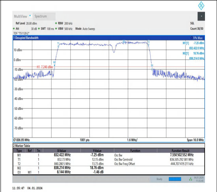
5-5-5MHz-3MHz-64QAM-64QAM-20510-20549-25RB#0-15RB#0-PASS
