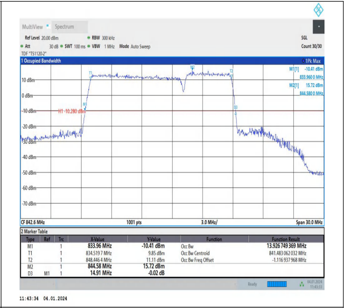
5-5-10MHz-5MHz-64QAM-64QAM-20550-20622-50RB#0-25R B#0-PASS
