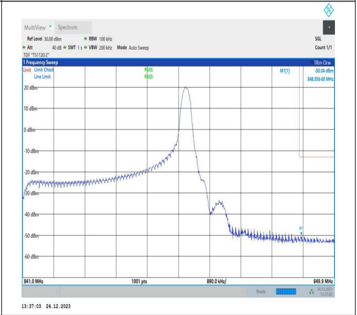
5MHz-3MHz_16QAM@16QAM-16QAM@16QAM_20595-20634_1RB#24@25RB#0-0RB#0@15RB#0
