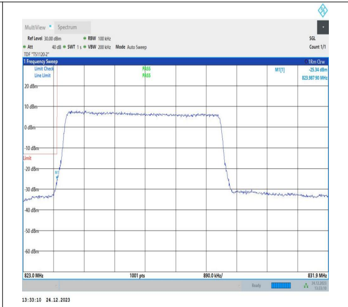
5MHz-3MHz_16QAM@16QAM-16QAM@16QAM_20425-20464_4_1RB#0@25RB#0-0RB#0@15RB#0
