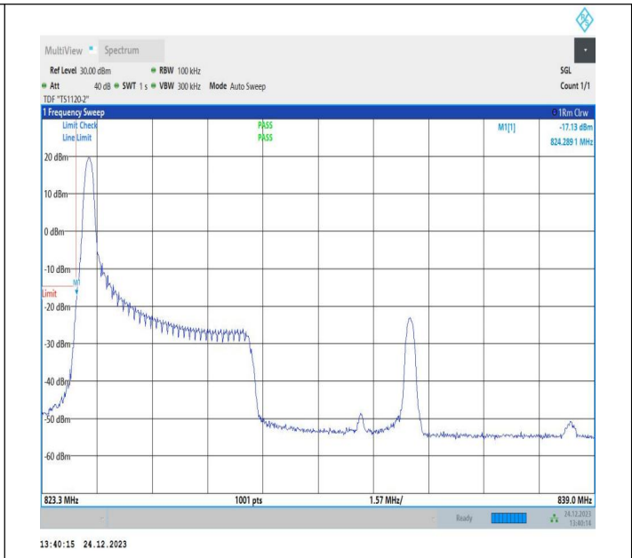
5MHz-10MHz_16QAM@16QAM-16QAM@16QAM_20428-20500_1 RB#0@25RB#0-0RB#0@50RB#0
