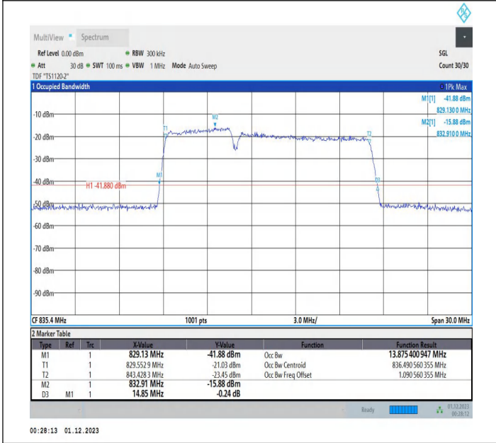
5-5-5MHz-10MHz-16QAM-16QAM-20478-20550-25RB#0-50R B#0-PASS
