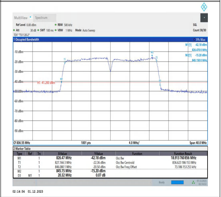
5-5-10MHz-10MHz-16QAM-16QAM-20476-20575-50RB#0-50RB RB#0-PASS
