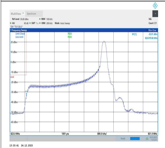
5MHz-3MHz_QPSK@QPSK-QPSK@QPSK_20425-20464_1RB#24@25RB#0-0RB#0@15RB#0
