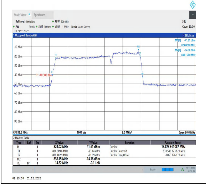
5-5-10MHz-5MHz-16QAM-16QAM-20450-20522-50RB#0-25R B#0-PASS
