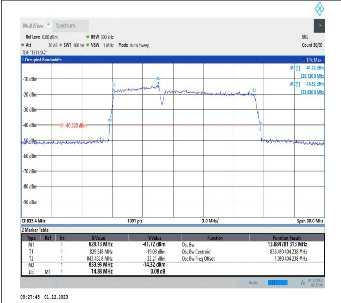
5-5-5MHz-10MHz-QPSK-QPSK-20478-20550-25RB#0-50RB#0-PASS
