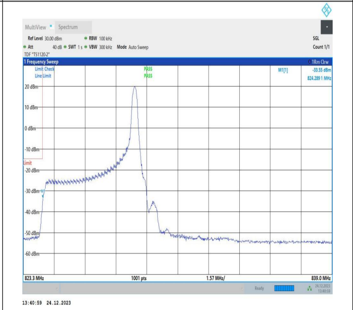
5MHz-10MHz_16QAM@16QAM-16QAM@16QAM_20428-20500_1 RB#24@25RB#0-0RB#0@50RB#0
