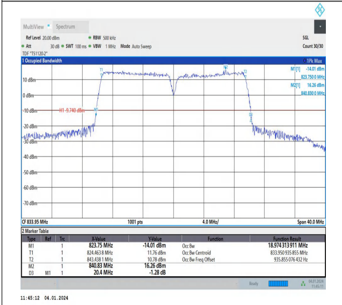
5-5-10MHz-10MHz-64QAM-64QAM-20450-20549-50RB#0-50RB #0-PASS
