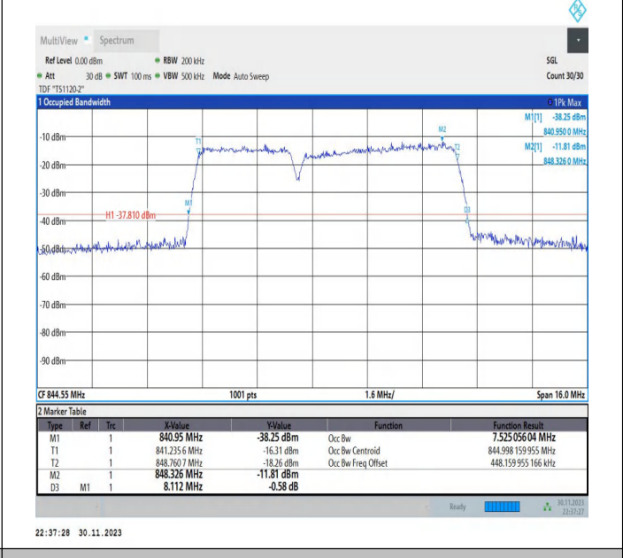
5-5-3MHz-5MHz-16QAM-16QAM-20586-20625-15RB#0-25RB #0-PASS
