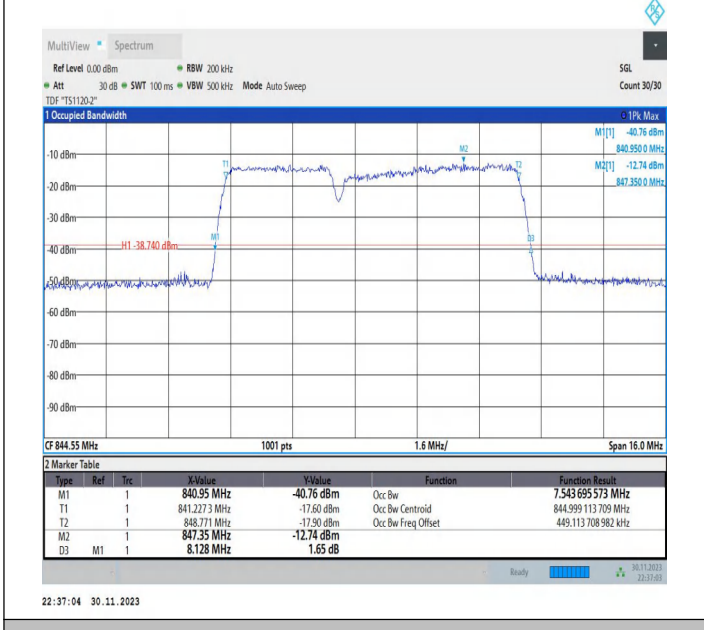
5-5-3MHz-5MHz-QPSK-QPSK-20586-20625-15RB#0-25RB#0-PASS
