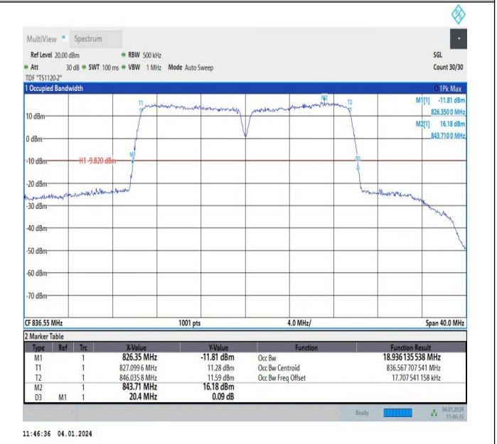
5-5-10MHz-10MHz-64QAM-64QAM-20476-20575-50RB#0-50RB #0-PASS
