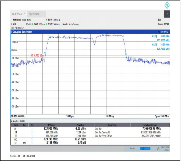
5-5-5MHz-3MHz-64QAM-64QAM-20425-20464-25RB#0-15RB #0-PASS
