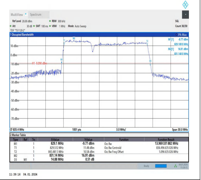
5-5-5MHz-10MHz-64QAM-64QAM-20478-20550-25RB#0-50R B#0-PASS
