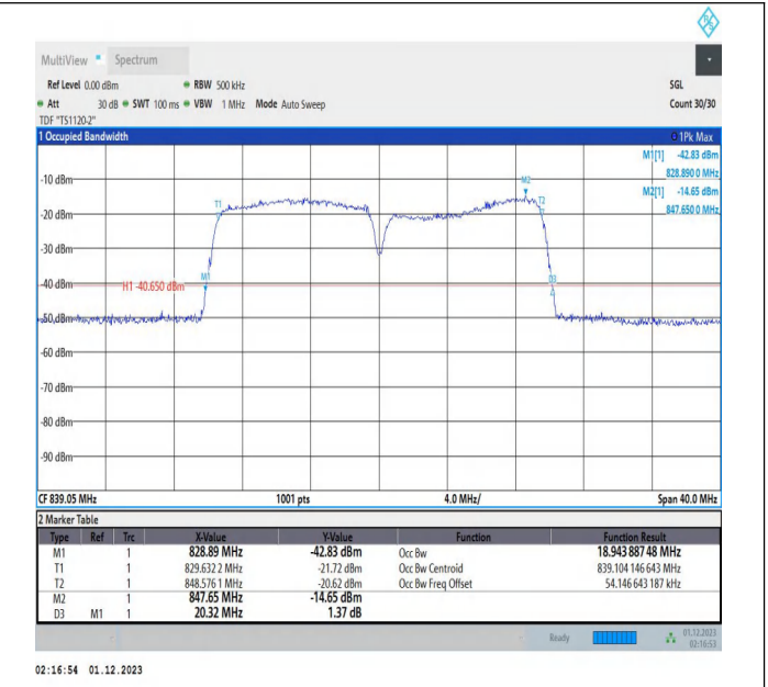
5-5-10MHz-10MHz-16QAM-16QAM-20501-20600-50RB#0-50RB #0-PASS
