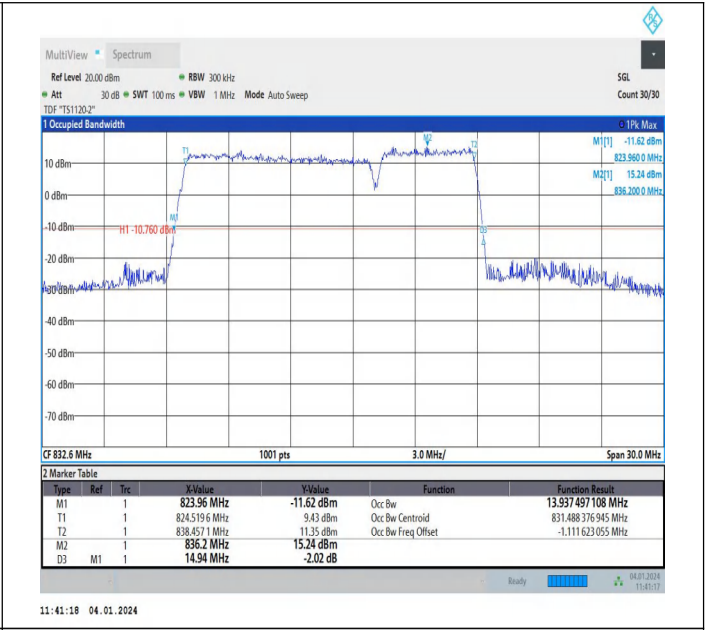
5-5-10MHz-5MHz-64QAM-64QAM-20450-20522-50RB#0-25R B#0-PASS
