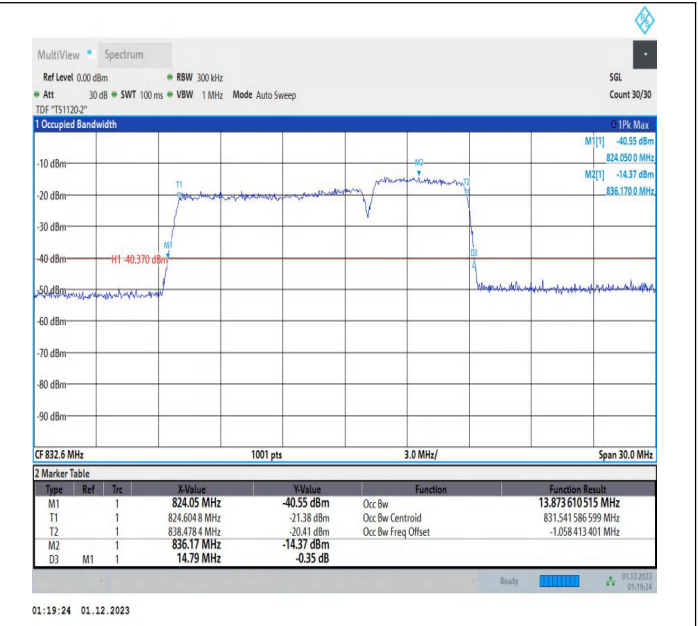
5-5-10MHz-5MHz-QPSK-QPSK-20450-20522-50RB#0-25RB#0-PASS
