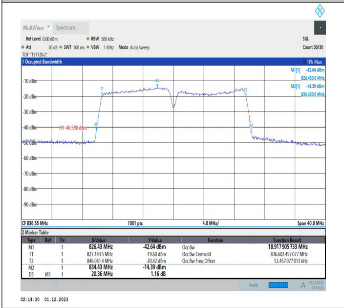
5-5-10MHz-10MHz-QPSK-QPSK-20476-20575-50RB#0-50RB #0-PASS
