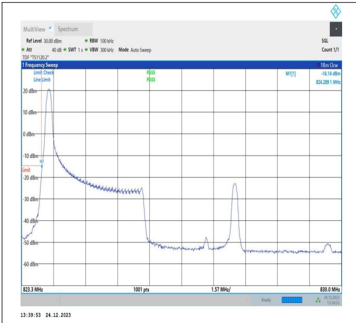
5MHz-10MHz_QPSK@QPSK-QPSK@QPSK_20428-20500_1 RB#0@25RB#0-0RB#0@50RB#0
