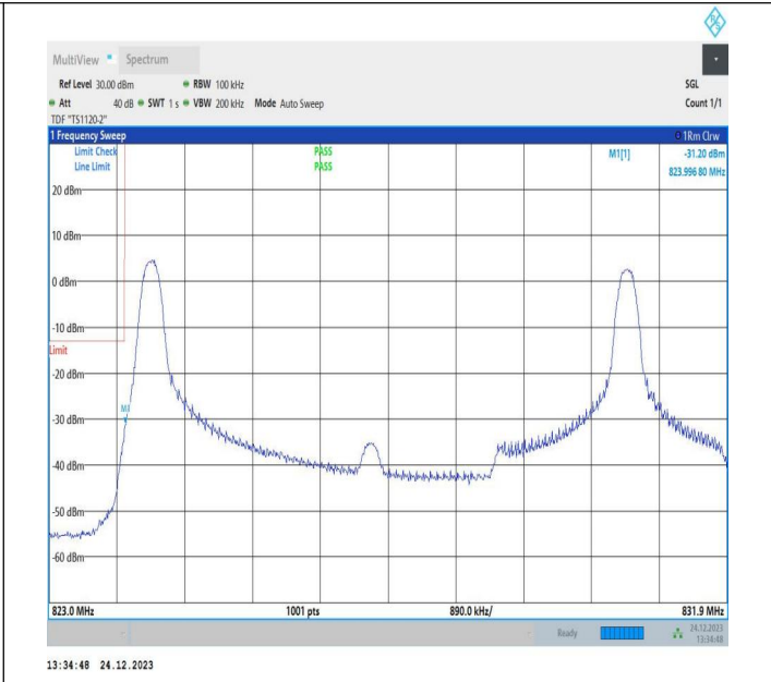
5MHz-3MHz_16QAM@16QAM-16QAM@16QAM_20425-20464_4_1RB#0@25RB#0-1RB#15@15RB#0
