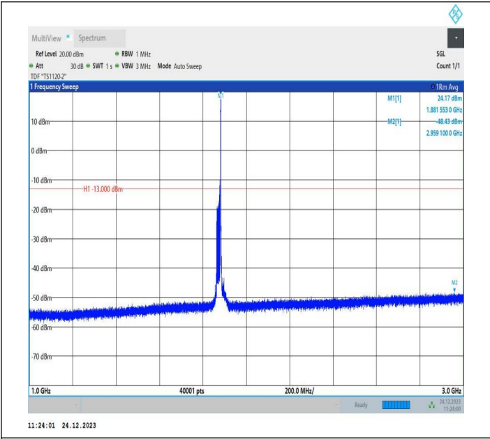
2-2-20MHz-15MHz-QPSK-QPSK-18826-18997-1RB#99-0RB# 0-1000~3000MHz-PASS
