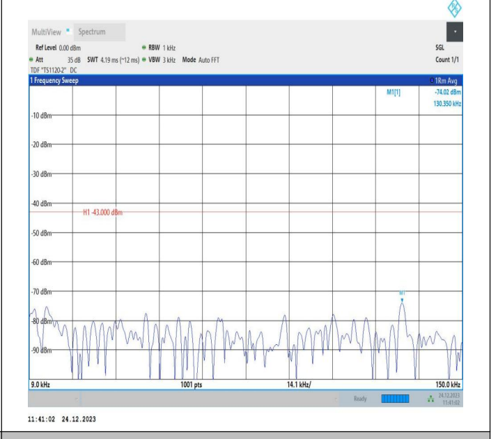
2-2-20MHz-20MHz-QPSK-QPSK-18902-19100-100RB#0-100 RB#0-0.009~0.15MHz-PASS
