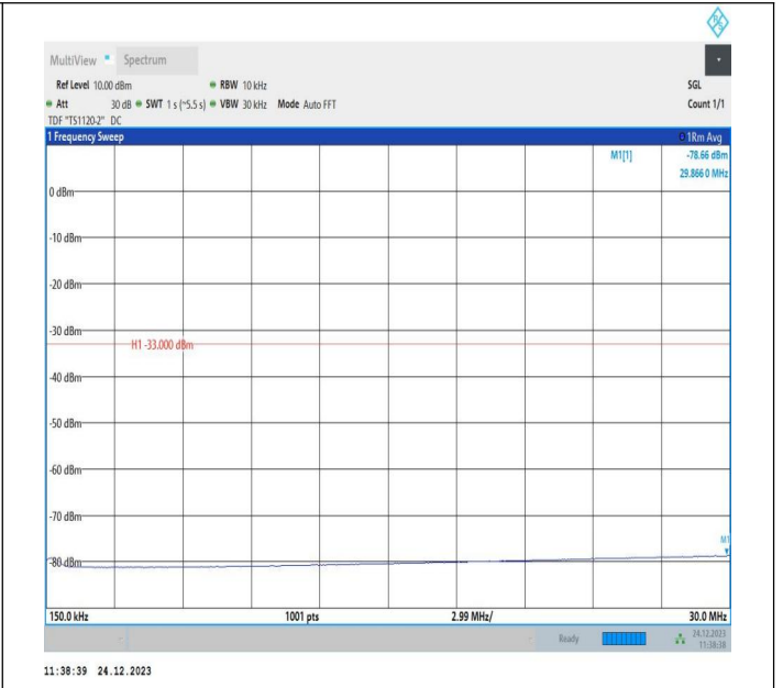
2-2-20MHz-20MHz-QPSK-QPSK-18902-19100-1RB#0-0RB#0 -0.15~30MHz-PASS
