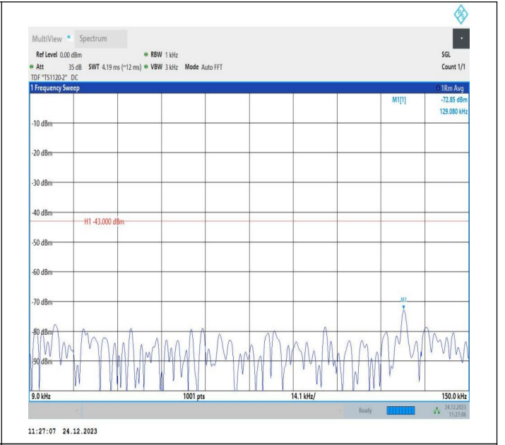
2-2-20MHz-15MHz-QPSK-QPSK-18951-19122-1RB#99-0RB#0 0-0.009~0.15MHz-PASS
