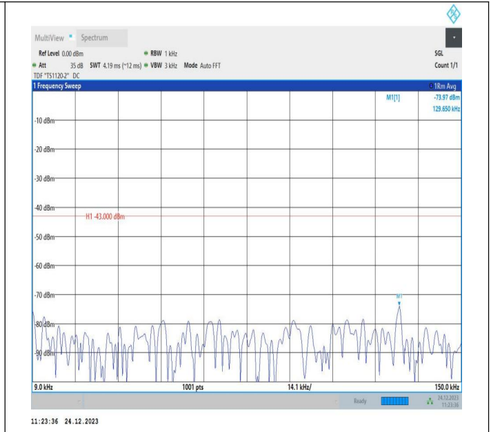
2-2-20MHz-15MHz-QPSK-QPSK-18826-18997-1RB#99-0RB#9 0-0.009~0.15MHz-PASS
