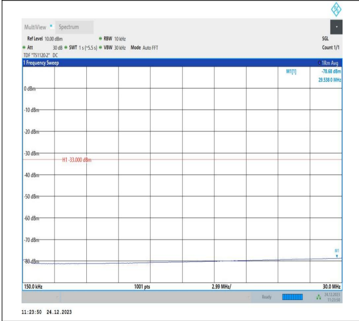
2-2-20MHz-15MHz-QPSK-QPSK-18826-18997-1RB#99-0RB#9 0-0.15~30MHz-PASS
