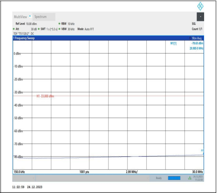
2-2-20MHz-15MHz-QPSK-QPSK-18826-18997-1RB#0-0RB#0 -0.15~30MHz-PASS
