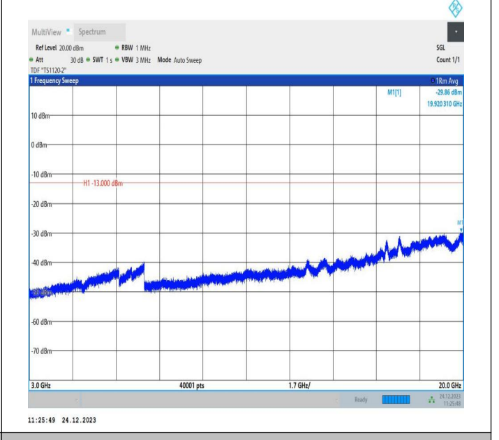
2-2-20MHz-15MHz-QPSK-QPSK-18826-18997-100RB#0-75R B#0-3000~20000MHz-PASS
