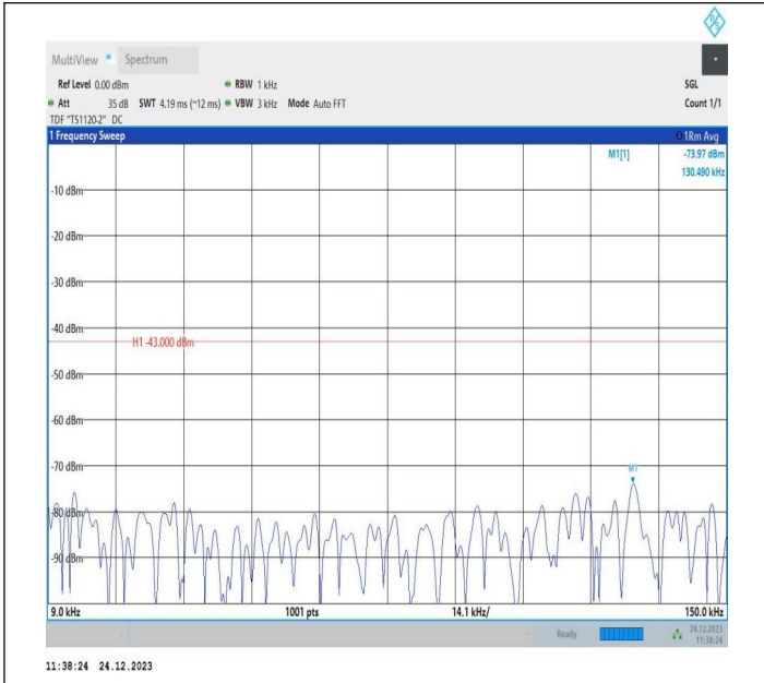
2-2-20MHz-20MHz-QPSK-QPSK-18902-19100-1RB#0-0RB#0 -0.009~0.15MHz-PASS
