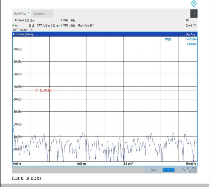
2-2-20MHz-15MHz-QPSK-QPSK-18951-19122-100RB#0-75R B#0-0.009~0.15MHz-PASS
