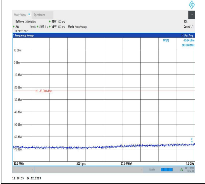
2-2-20MHz-15MHz-QPSK-QPSK-18951-19122-1RB#0-0RB#0 -30~1000MHz-PASS
