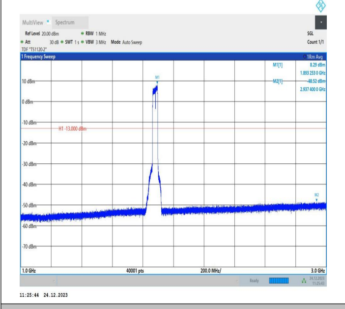
2-2-20MHz-15MHz-QPSK-QPSK-18826-18997-100RB#0-75R B#0-1000~3000MHz-PASS
