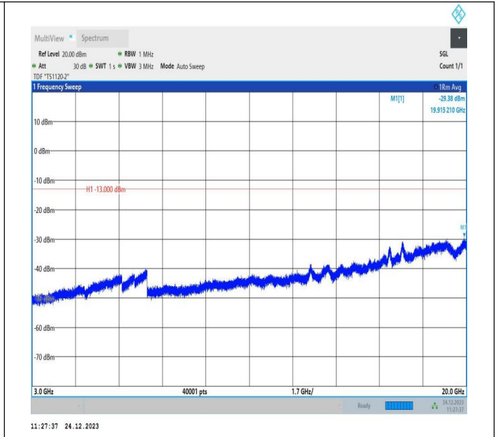
2-2-20MHz-15MHz-QPSK-QPSK-18951-19122-1RB#99-0RB# 0-3000~20000MHz-PASS
