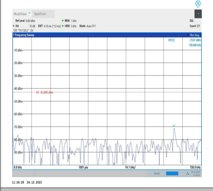
2-2-20MHz-15MHz-QPSK-QPSK-18826-18997-1RB#0-1RB#7 4-0.009~0.15MHz-PASS
