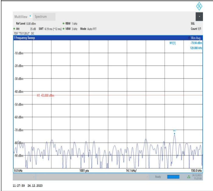
2-2-20MHz-15MHz-QPSK-QPSK-18951-19122-1RB#0-1RB#7 4-0.009~0.15MHz-PASS
