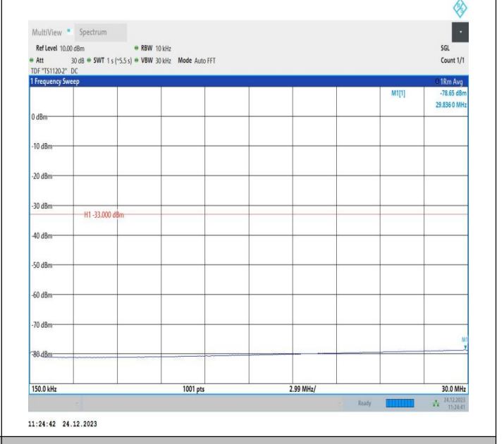
2-2-20MHz-15MHz-QPSK-QPSK-18826-18997-1RB#0-1RB#7 4-0.15~30MHz-PASS
