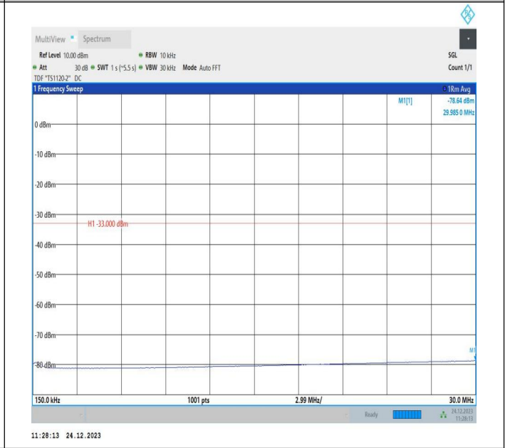
2-2-20MHz-15MHz-QPSK-QPSK-18951-19122-1RB#0-1RB#7 4-0.15~30MHz-PASS
