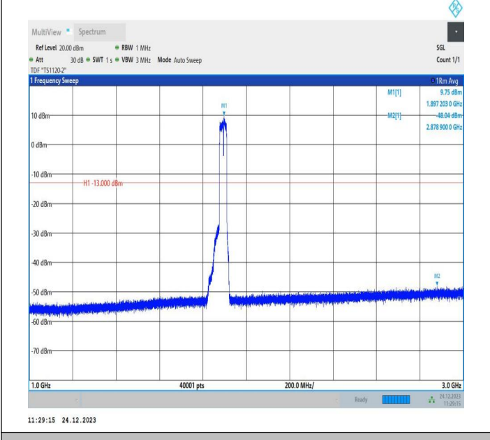
2-2-20MHz-15MHz-QPSK-QPSK-18951-19122-100RB#0-75R B#0-1000~3000MHz-PASS
