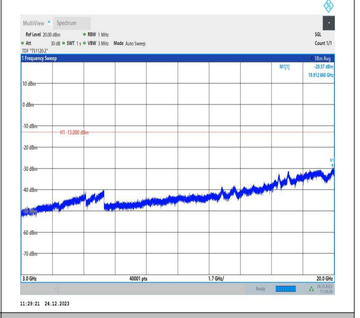
2-2-20MHz-15MHz-QPSK-QPSK-18951-19122-100RB#0-75R B#0-3000~20000MHz-PASS
