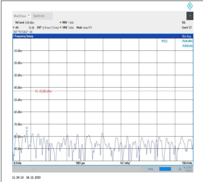
2-2-20MHz-15MHz-QPSK-QPSK-18951-19122-1RB#0-0RB#0 -0.009~0.15MHz-PASS
