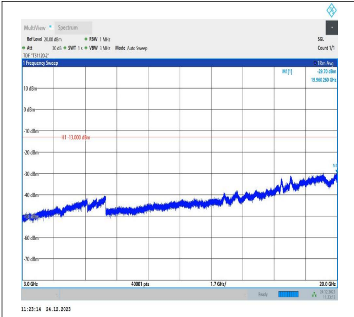
2-2-20MHz-15MHz-QPSK-QPSK-18826-18997-1RB#0-0RB#0 -3000~20000MHz-PASS
