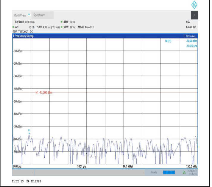
2-2-20MHz-15MHz-QPSK-QPSK-18826-18997-100RB#0-75R B#0-0.009~0.15MHz-PASS
