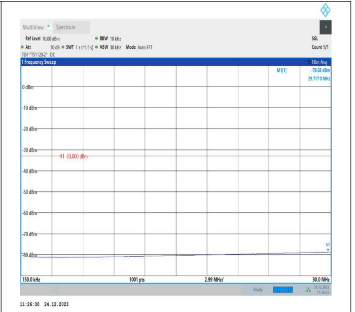
2-2-20MHz-15MHz-QPSK-QPSK-18951-19122-1RB#0-0RB#0 -0.15~30MHz-PASS
