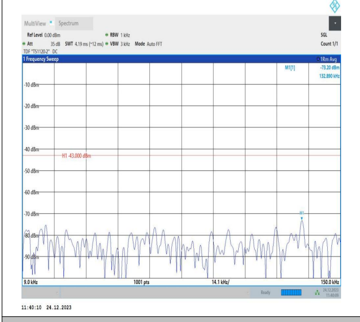
2-2-20MHz-20MHz-QPSK-QPSK-18902-19100-1RB#0-1RB#9 9-0.009~0.15MHz-PASS
