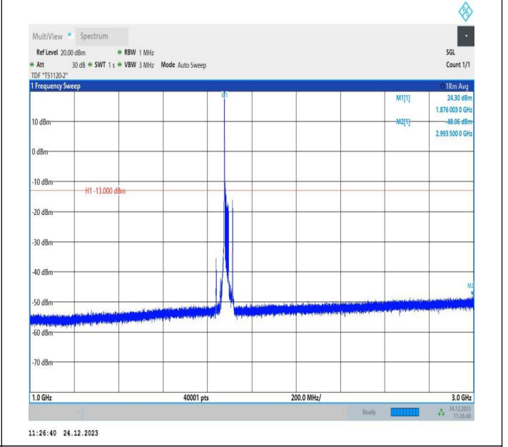
2-2-20MHz-15MHz-QPSK-QPSK-18951-19122-1RB#0-0RB#0 -1000~3000MHz-PASS
