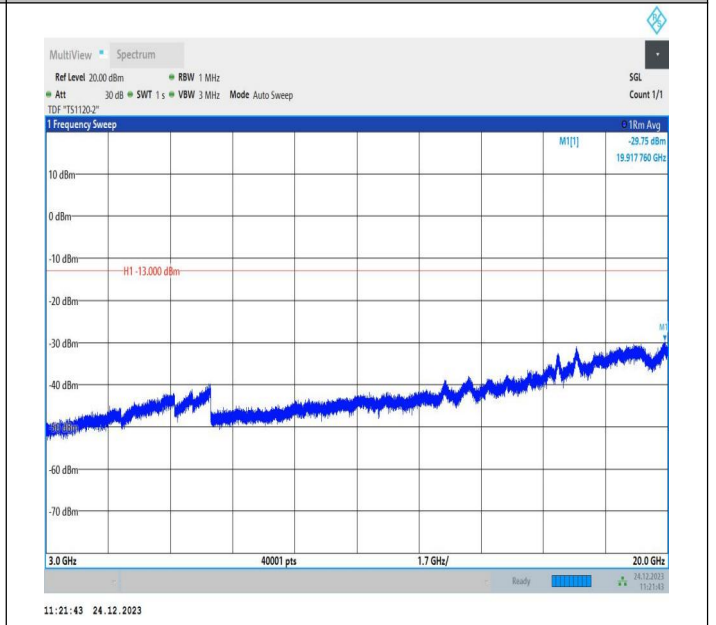
2-2-20MHz-15MHz-QPSK-QPSK-18700-18871-100RB#0-75R B#0-3000~20000MHz-PASS
