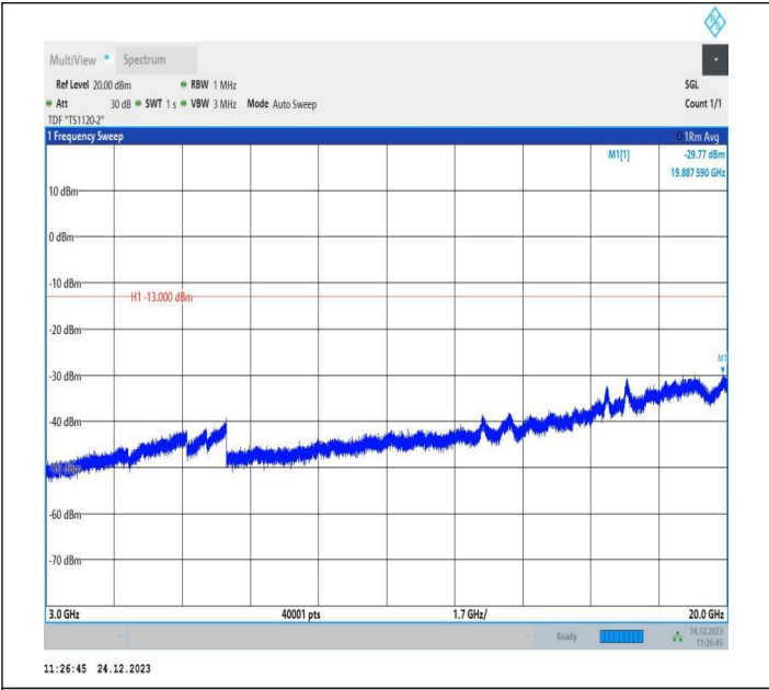
2-2-20MHz-15MHz-QPSK-QPSK-18951-19122-1RB#0-0RB#0 -3000~20000MHz-PASS
