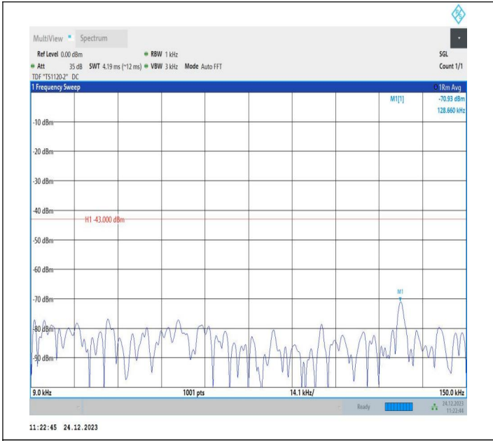
2-2-20MHz-15MHz-QPSK-QPSK-18826-18997-1RB#0-0RB#0 -0.009~0.15MHz-PASS
