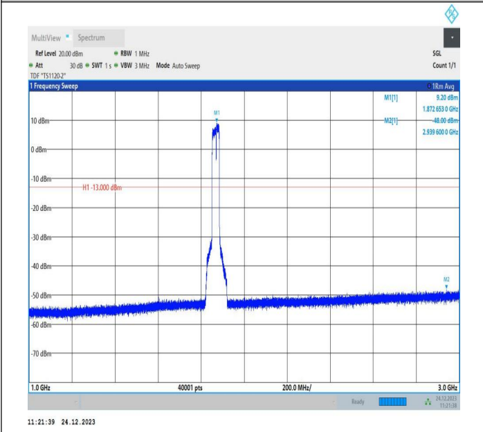
2-2-20MHz-15MHz-QPSK-QPSK-18700-18871-100RB#0-75R B#0-1000~3000MHz-PASS
