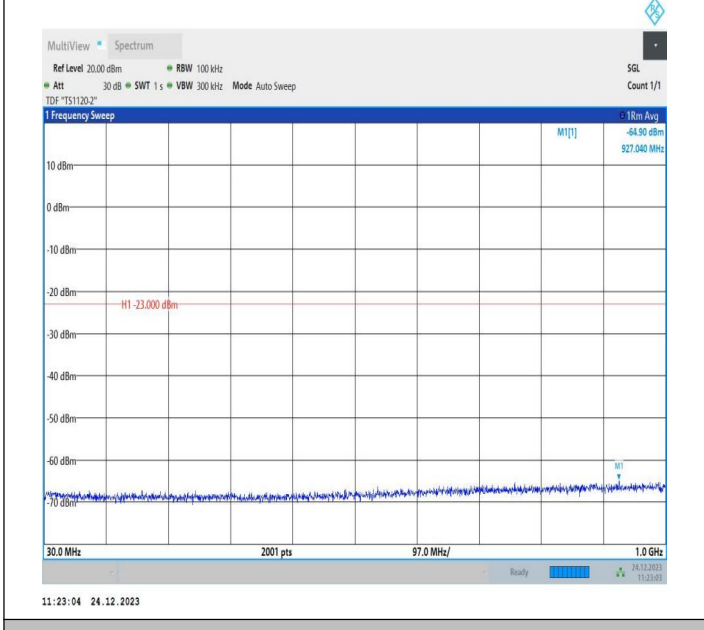
2-2-20MHz-15MHz-QPSK-QPSK-18826-18997-1RB#0-0RB#0 -30~1000MHz-PASS
