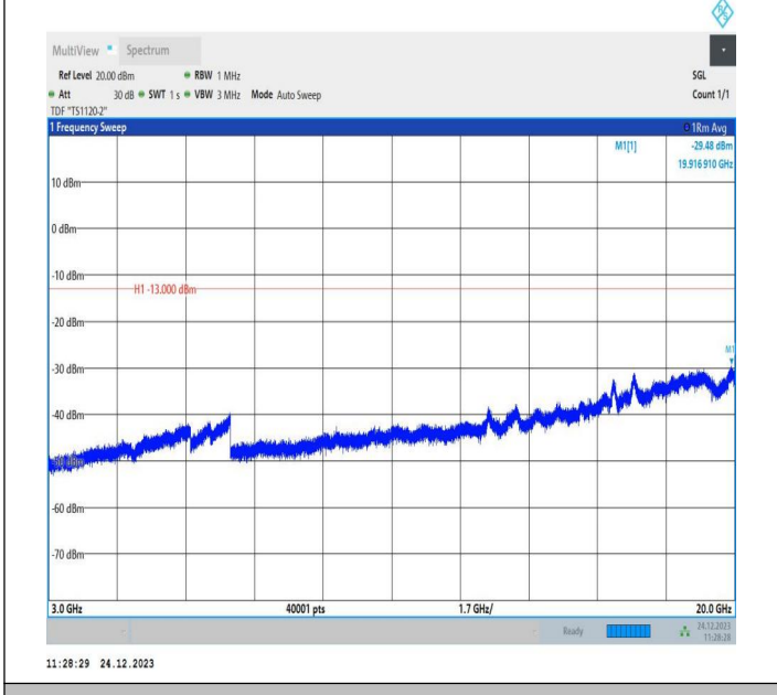
2-2-20MHz-15MHz-QPSK-QPSK-18951-19122-1RB#0-1RB#7 4-3000~20000MHz-PASS
