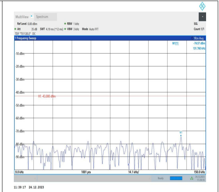
2-2-20MHz-20MHz-QPSK-QPSK-18902-19100-1RB#99-0RB#0 0-0.009~0.15MHz-PASS
