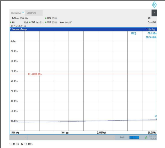
2-2-20MHz-15MHz-QPSK-QPSK-18700-18871-100RB#0-75R B#0-0.15~30MHz-PASS
