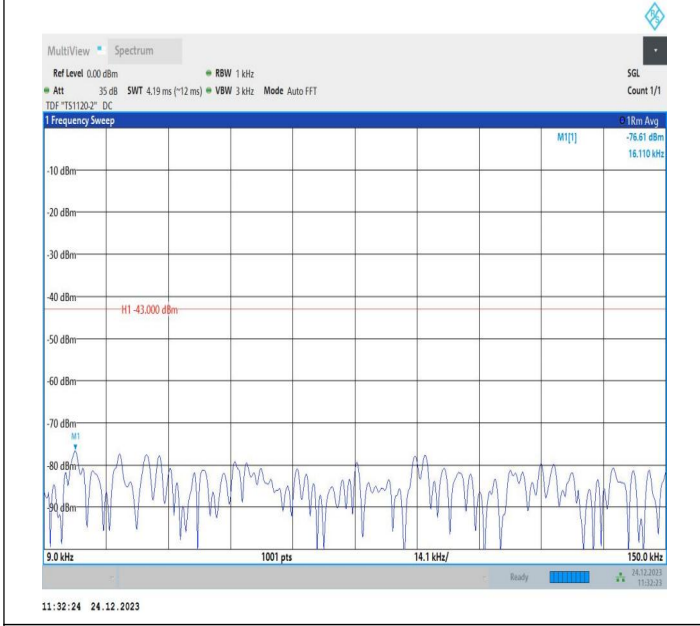
2-2-20MHz-20MHz-QPSK-QPSK-18700-18898-1RB#0-1RB#9 9-0.009~0.15MHz-PASS
