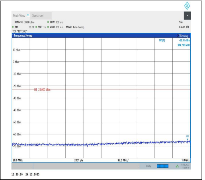
2-2-20MHz-15MHz-QPSK-QPSK-18951-19122-100RB#0-75R B#0-30~100MHz-PASS
