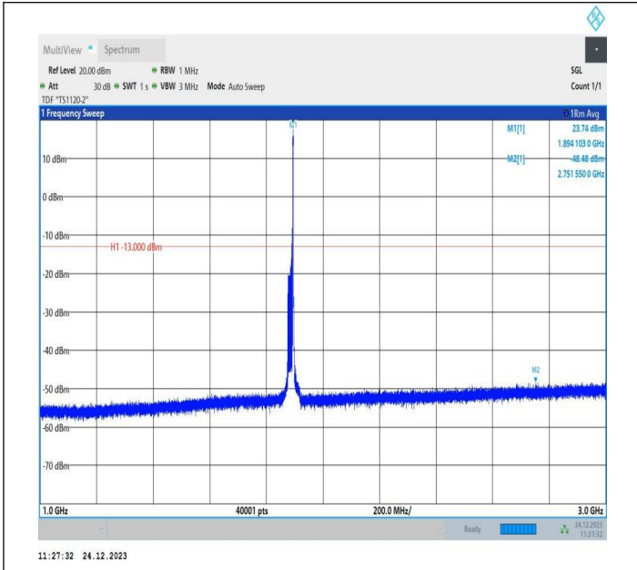
2-2-20MHz-15MHz-QPSK-QPSK-18951-19122-1RB#99-0RB# 0-1000~3000MHz-PASS
