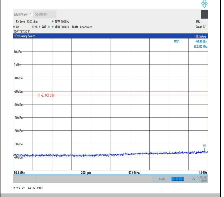
2-2-20MHz-15MHz-QPSK-QPSK-18951-19122-1RB#99-0RB#0 0-30~1000MHz-PASS
