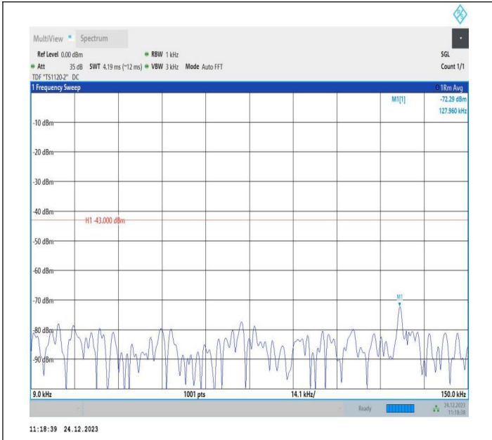
2-2-20MHz-15MHz-QPSK-QPSK-18700-18871-1RB#0-0RB#0 -0.009~0.15MHz-PASS
