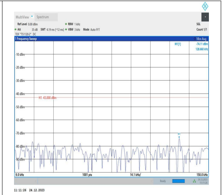
2-2-20MHz-5MHz-QPSK-QPSK-18875-18992-1RB#99-0RB#0-0.009~0.15MHz-PASS
