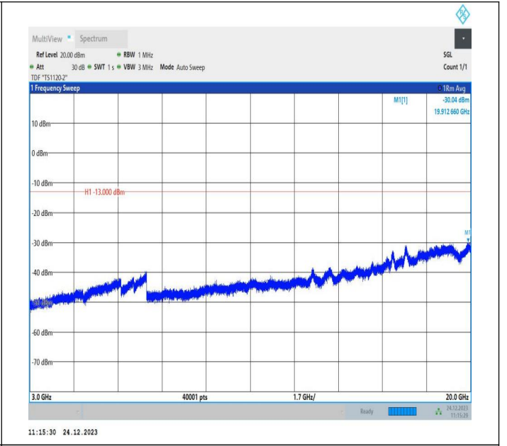
2-2-20MHz-5MHz-QPSK-QPSK-19050-19167-1RB#99-0RB#0 -3000~20000MHz-PASS
