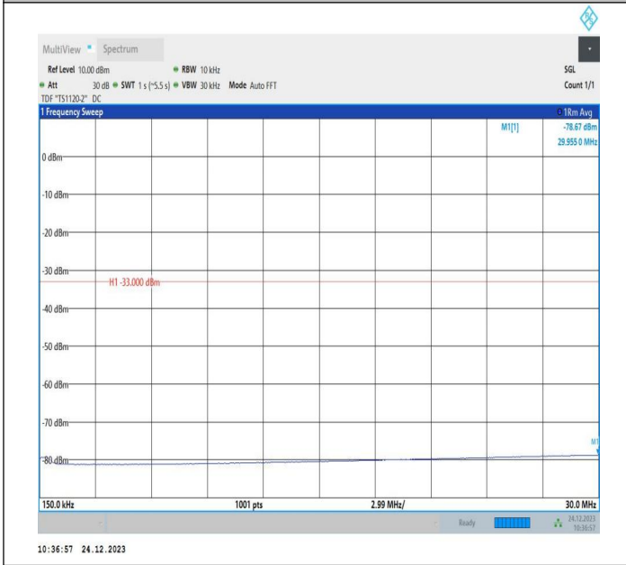
2-2-15MHz-20MHz-QPSK-QPSK-18929-19100-1RB#74-0RB#0 0-0.15~30MHz-PASS
