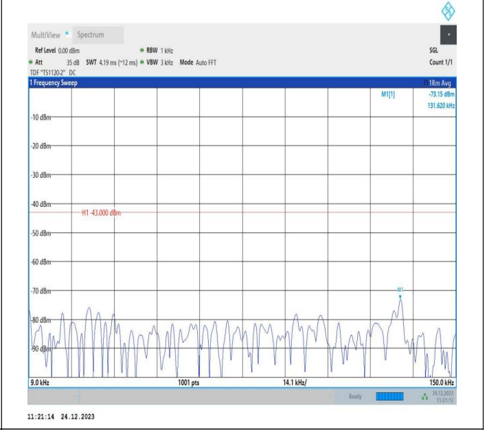
2-2-20MHz-15MHz-QPSK-QPSK-18700-18871-100RB#0-75R B#0-0.009~0.15MHz-PASS
