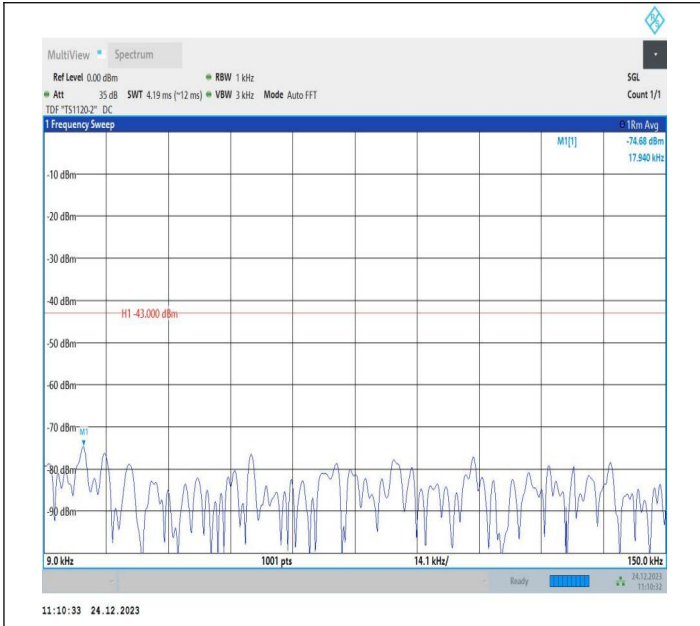
2-2-20MHz-5MHz-QPSK-QPSK-18875-18992-1RB#0-0RB#0-0.009~0.15MHz-PASS
