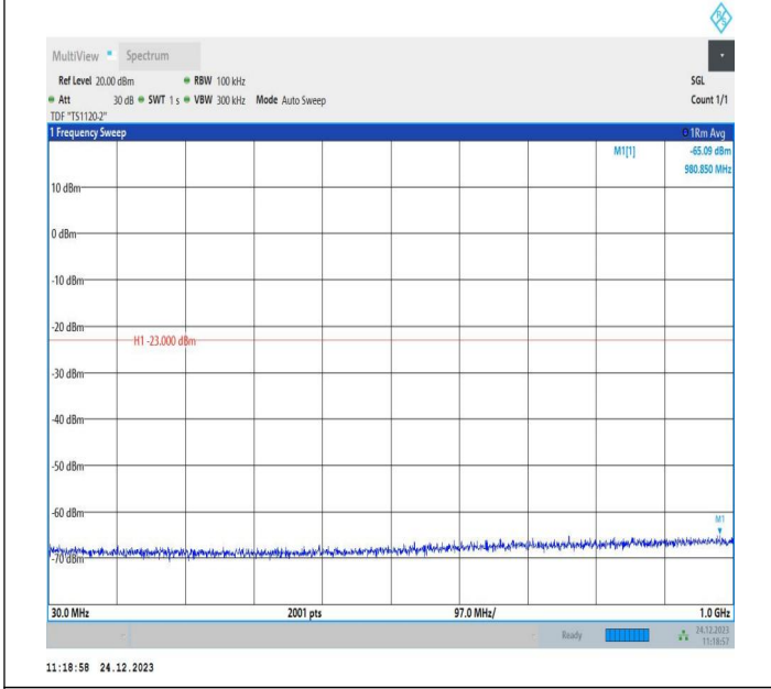
2-2-20MHz-15MHz-QPSK-QPSK-18700-18871-1RB#0-0RB#0 -30~1000MHz-PASS
