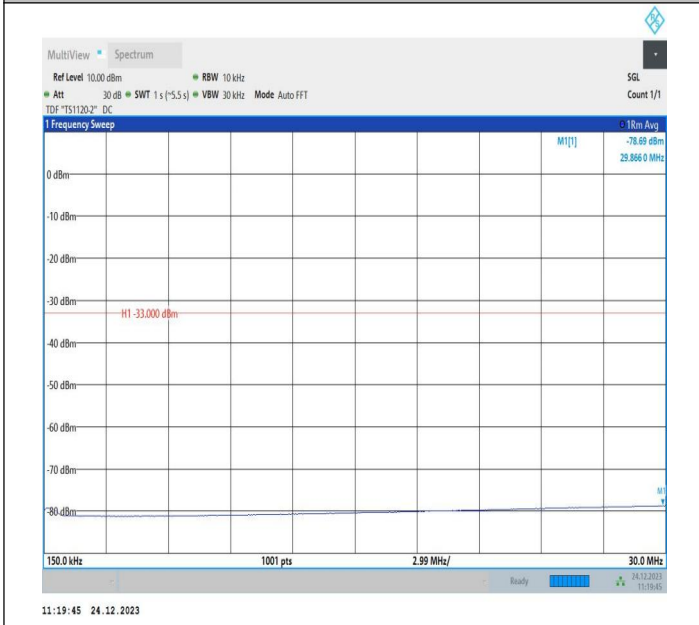
2-2-20MHz-15MHz-QPSK-QPSK-18700-18871-1RB#99-0RB#9 0-0.15~30MHz-PASS
