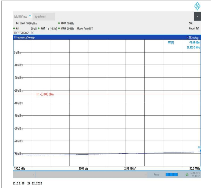
2-2-20MHz-5MHz-QPSK-QPSK-19050-19167-100RB#0-25RB #0-0.15~30MHz-PASS
