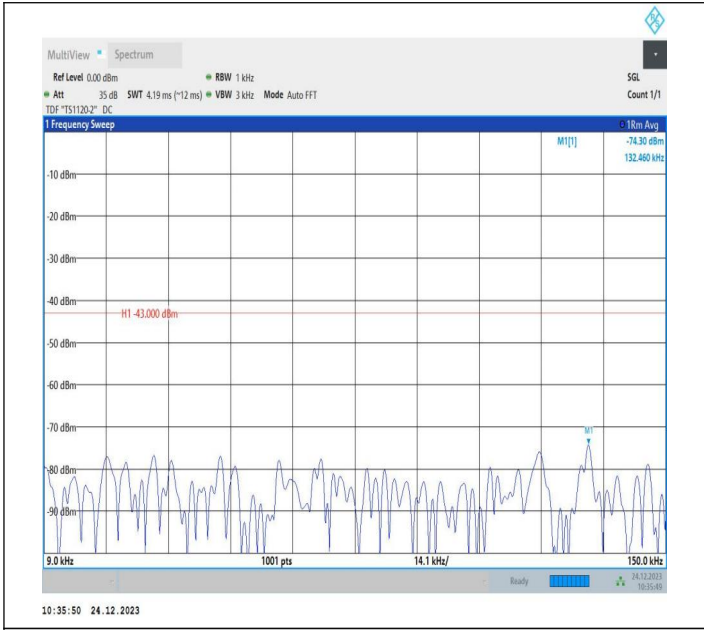
2-2-15MHz-20MHz-QPSK-QPSK-18929-19100-1RB#0-0RB#0 -0.009~0.15MHz-PASS
