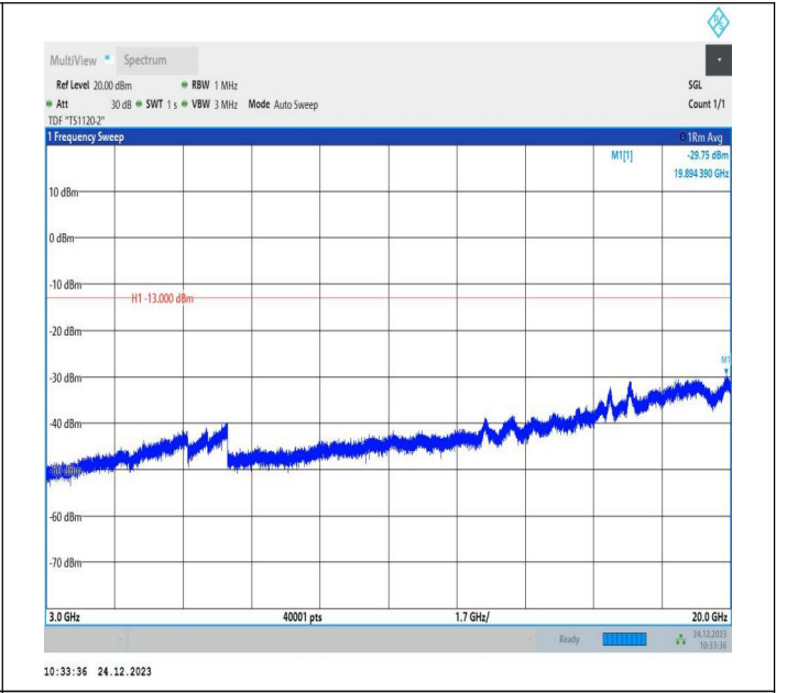
2-2-15MHz-20MHz-QPSK-QPSK-18803-18974-1RB#74-0RB# 0-3000~20000MHz-PASS
