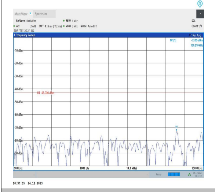
2-2-15MHz-20MHz-QPSK-QPSK-18929-19100-1RB#0-1RB#9 9-0.009~0.15MHz-PASS
