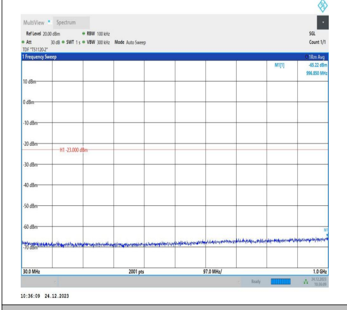
2-2-15MHz-20MHz-QPSK-QPSK-18929-19100-1RB#0-0RB#0 -30~1000MHz-PASS
