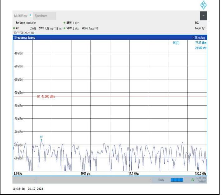
2-2-15MHz-20MHz-QPSK-QPSK-18929-19100-75RB#0-100R B#0-0.009~0.15MHz-PASS
