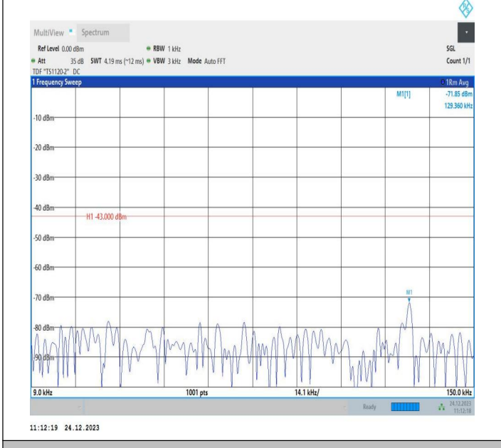
2-2-20MHz-5MHz-QPSK-QPSK-18875-18992-1RB#0-1RB#24 -0.009~0.15MHz-PASS
