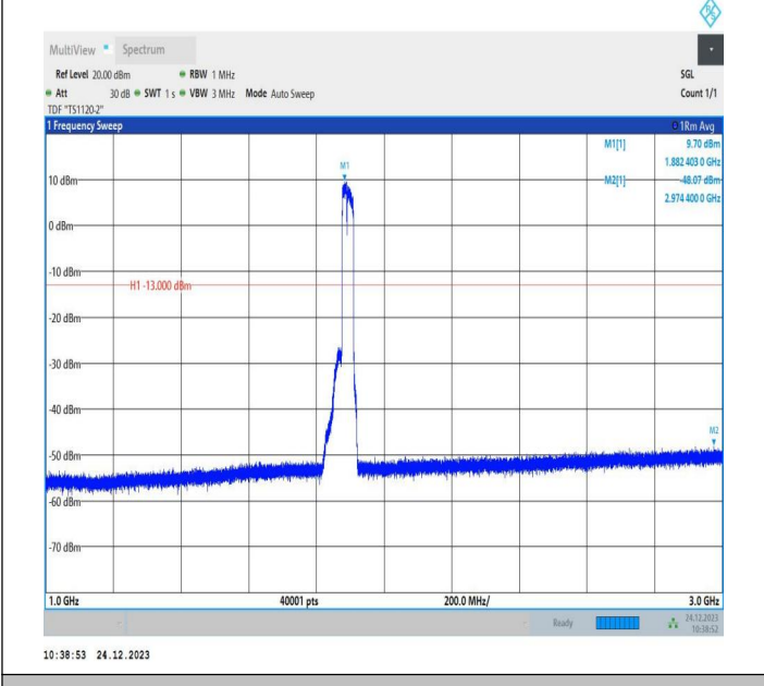
2-2-15MHz-20MHz-QPSK-QPSK-18929-19100-75RB#0-100R B#0-1000~3000MHz-PASS
