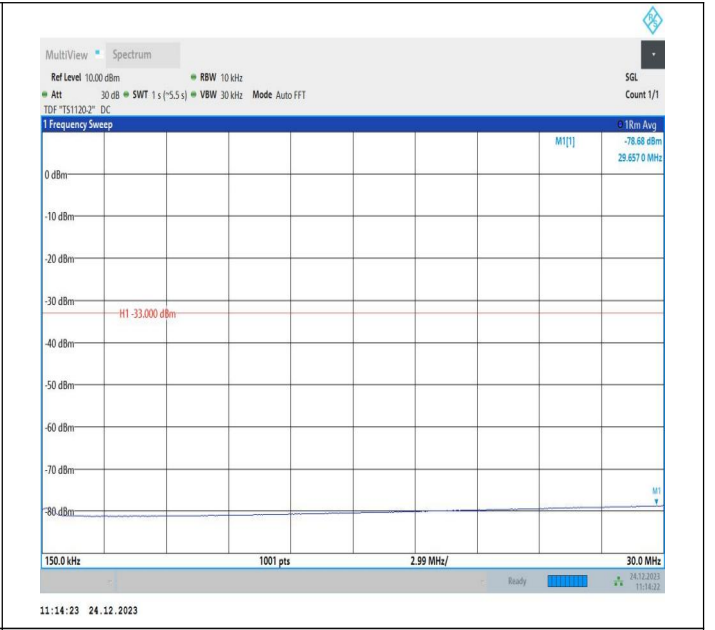
2-2-20MHz-5MHz-QPSK-QPSK-19050-19167-1RB#0-0RB#0-0.15~30MHz-PASS
