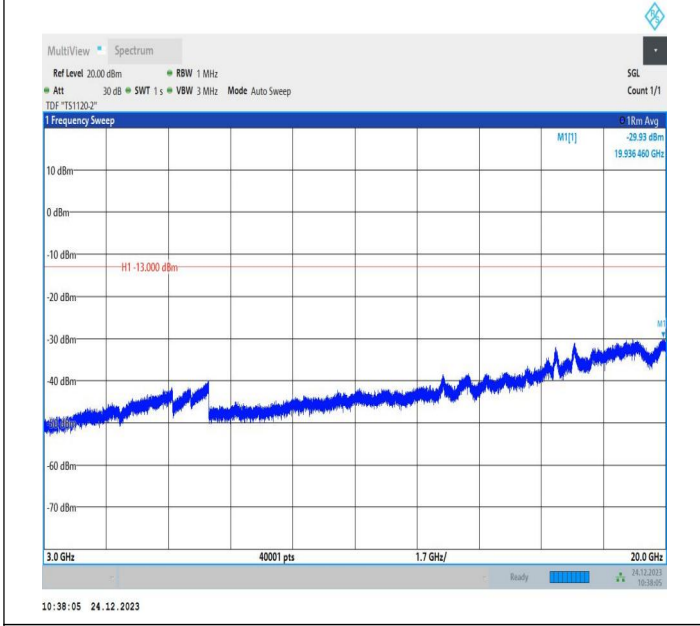
2-2-15MHz-20MHz-QPSK-QPSK-18929-19100-1RB#0-1RB#9 9-3000~20000MHz-PASS
