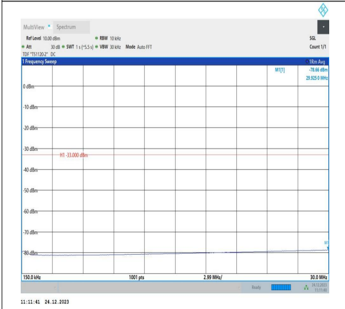
2-2-20MHz-5MHz-QPSK-QPSK-18875-18992-1RB#99-0RB#0-0.15~30MHz-PASS
