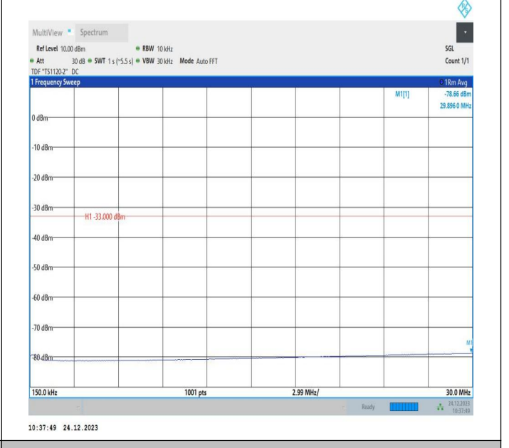
2-2-15MHz-20MHz-QPSK-QPSK-18929-19100-1RB#0-1RB#9 9-0.15~30MHz-PASS
