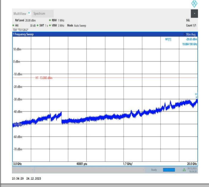
2-2-15MHz-20MHz-QPSK-QPSK-18803-18974-1RB#0-1RB#9 9-3000~20000MHz-PASS
