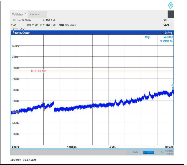
2-2-20MHz-15MHz-QPSK-QPSK-18700-18871-1RB#99-0RB# 0-3000~20000MHz-PASS
