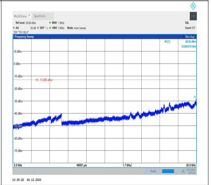
2-2-15MHz-20MHz-QPSK-QPSK-18803-18974-75RB#0-100R B#0-3000~20000MHz-PASS
