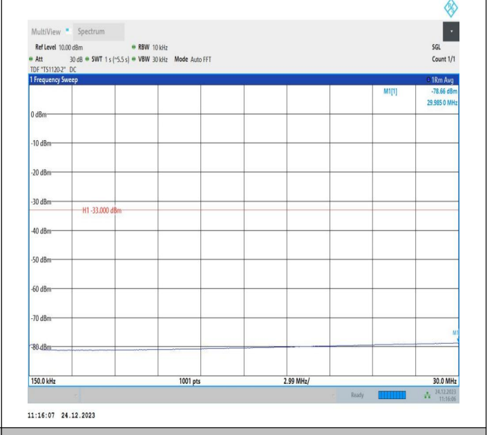
2-2-20MHz-5MHz-QPSK-QPSK-19050-19167-1RB#0-1RB#24 -0.15~30MHz-PASS
