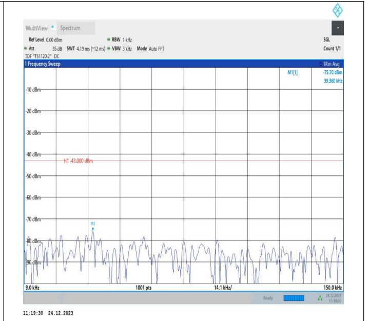
2-2-20MHz-15MHz-QPSK-QPSK-18700-18871-1RB#99-0RB#9 0-0.009~0.15MHz-PASS
