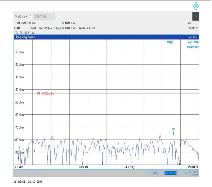
2-2-20MHz-5MHz-QPSK-QPSK-19050-19167-100RB#0-25RB #0-0.009~0.15MHz-PASS
