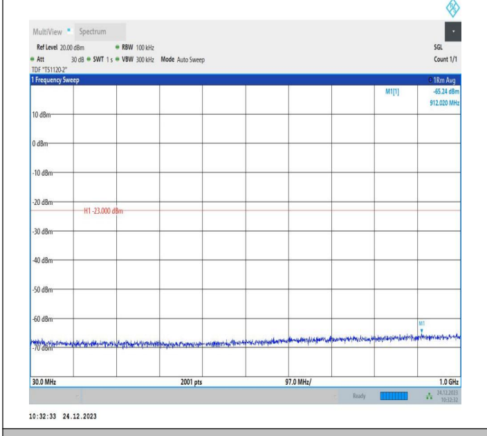
2-2-15MHz-20MHz-QPSK-QPSK-18803-18974-1RB#0-0RB#0 -30~1000MHz-PASS
