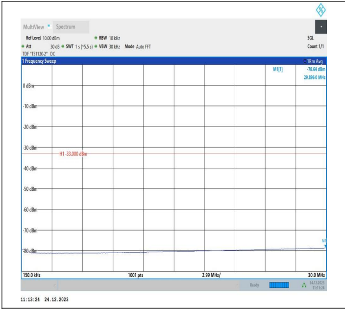
2-2-20MHz-5MHz-QPSK-QPSK-18875-18992-100RB#0-25RB #0-0.15~30MHz-PASS
