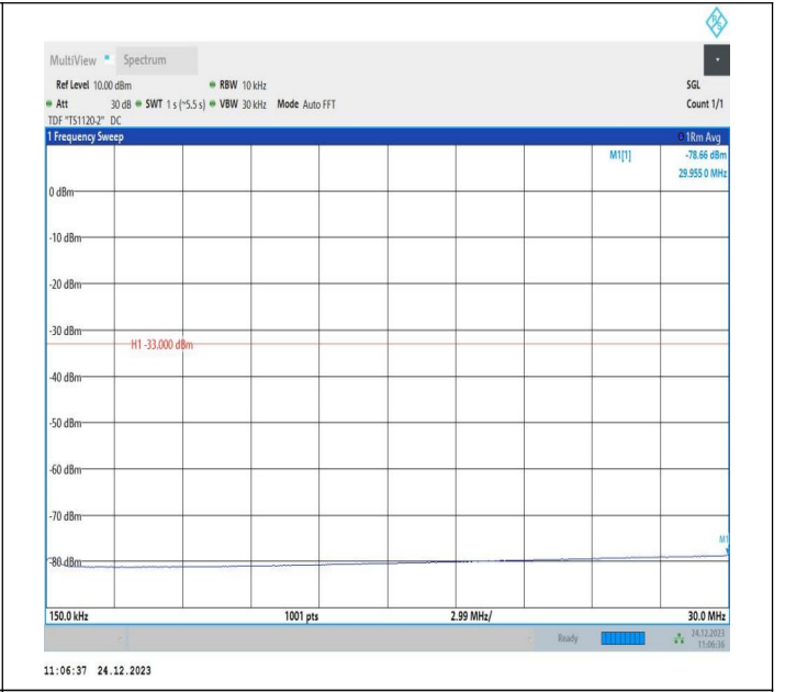
2-2-20MHz-5MHz-QPSK-QPSK-18700-18817-1RB#0-0RB#0-0.15~30MHz-PASS
