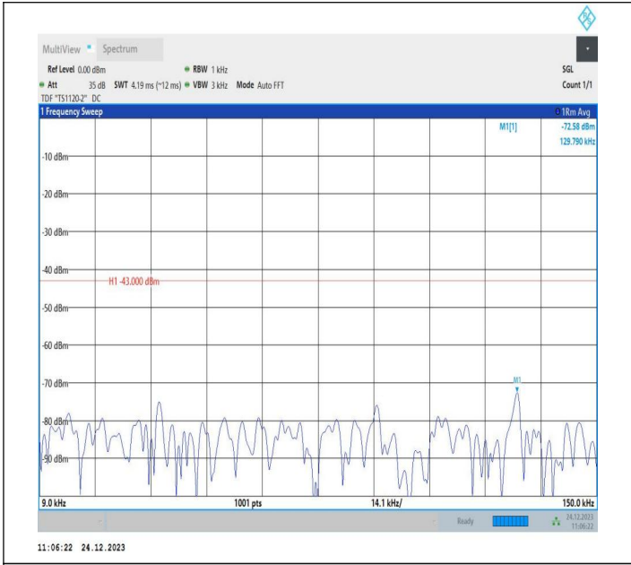
2-2-20MHz-5MHz-QPSK-QPSK-18700-18817-1RB#0-0RB#0-0.009~0.15MHz-PASS
