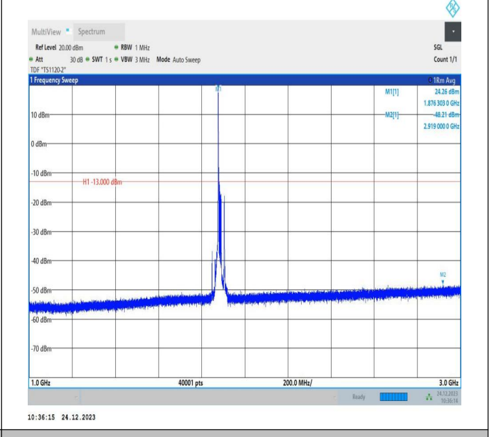
2-2-15MHz-20MHz-QPSK-QPSK-18929-19100-1RB#0-0RB#0 -1000~3000MHz-PASS
