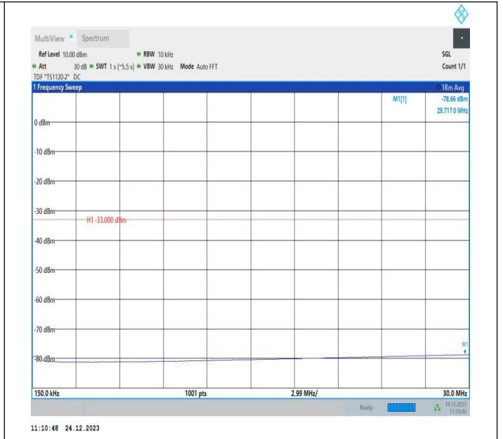
2-2-20MHz-5MHz-QPSK-QPSK-18875-18992-1RB#0-0RB#0-0.15~30MHz-PASS
