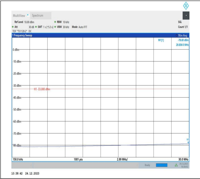
2-2-15MHz-20MHz-QPSK-QPSK-18929-19100-75RB#0-100R B#0-0.15~30MHz-PASS
