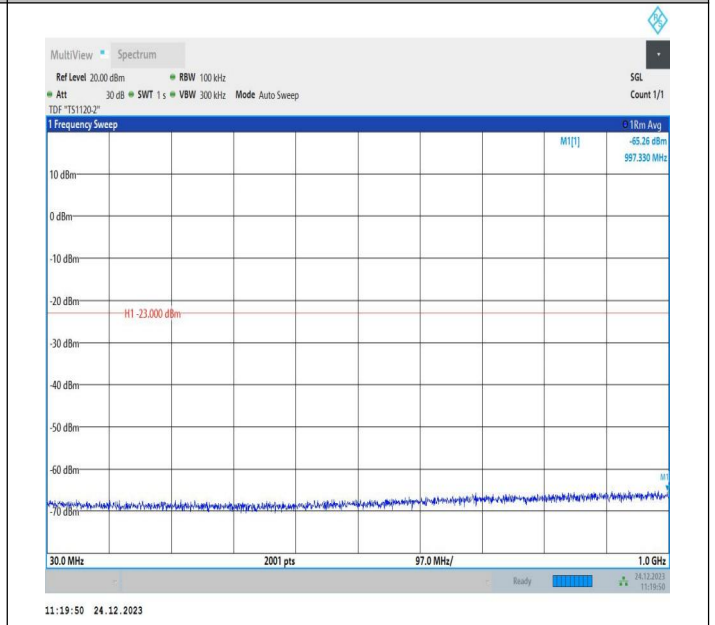
2-2-20MHz-15MHz-QPSK-QPSK-18700-18871-1RB#99-0RB#9 0-30~1000MHz-PASS
