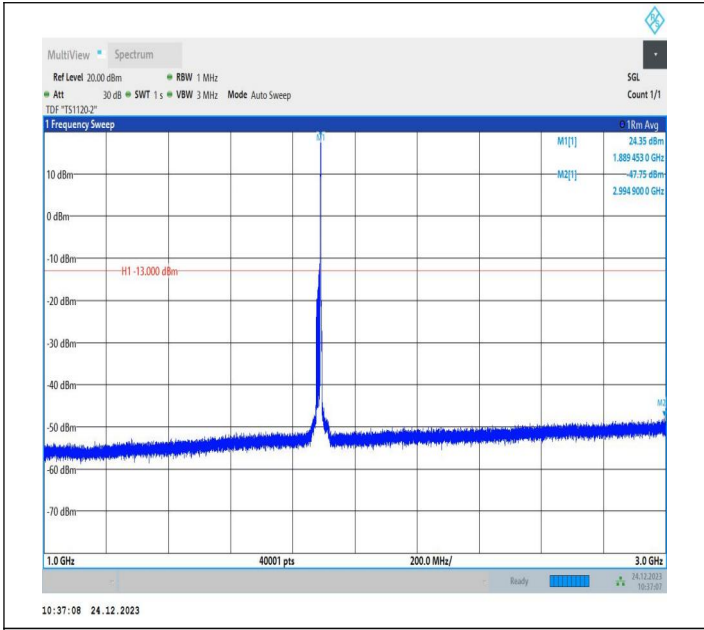
2-2-15MHz-20MHz-QPSK-QPSK-18929-19100-1RB#74-0RB# 0-1000~3000MHz-PASS
