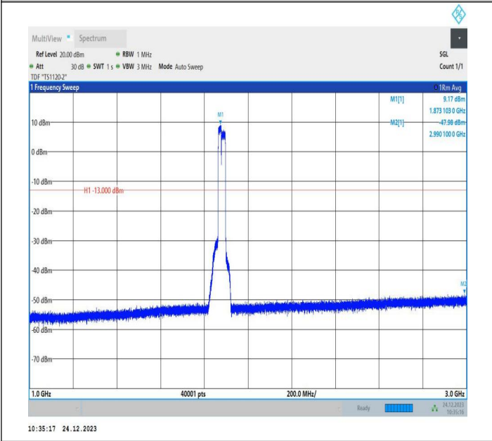
2-2-15MHz-20MHz-QPSK-QPSK-18803-18974-75RB#0-100R B#0-1000~3000MHz-PASS
