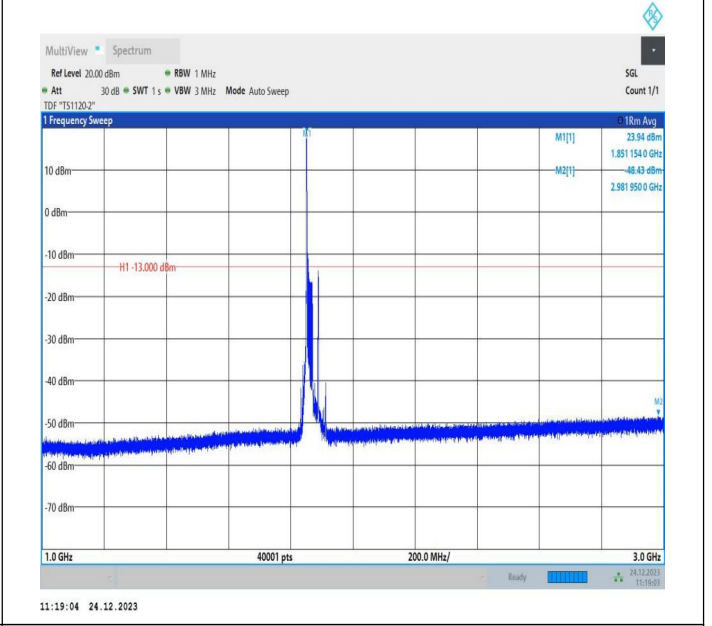
2-2-20MHz-15MHz-QPSK-QPSK-18700-18871-1RB#0-0RB#0 -1000~3000MHz-PASS
