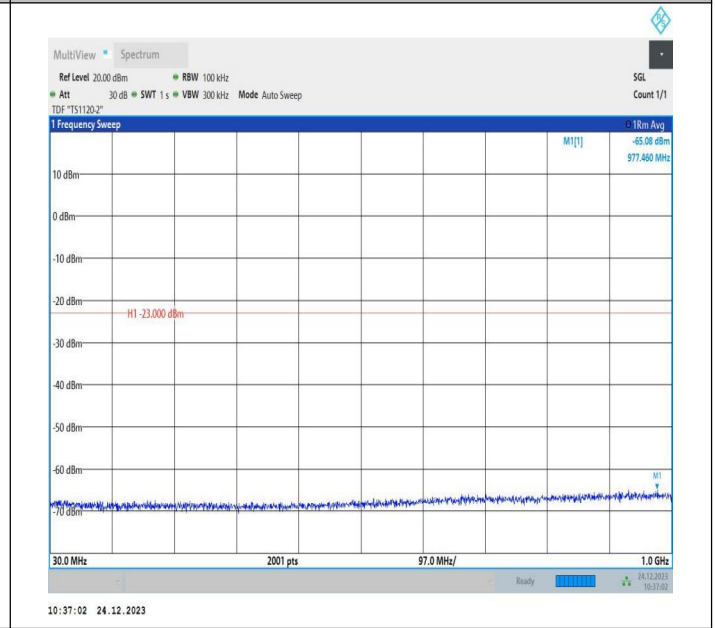
2-2-15MHz-20MHz-QPSK-QPSK-18929-19100-1RB#74-0RB#0 0-30~1000MHz-PASS
