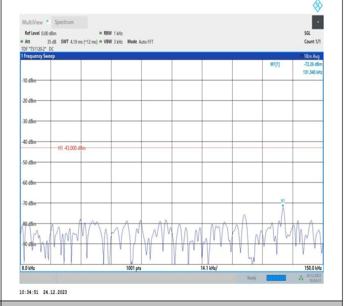
2-2-15MHz-20MHz-QPSK-QPSK-18803-18974-75RB#0-100R B#0-0.009~0.15MHz-PASS
