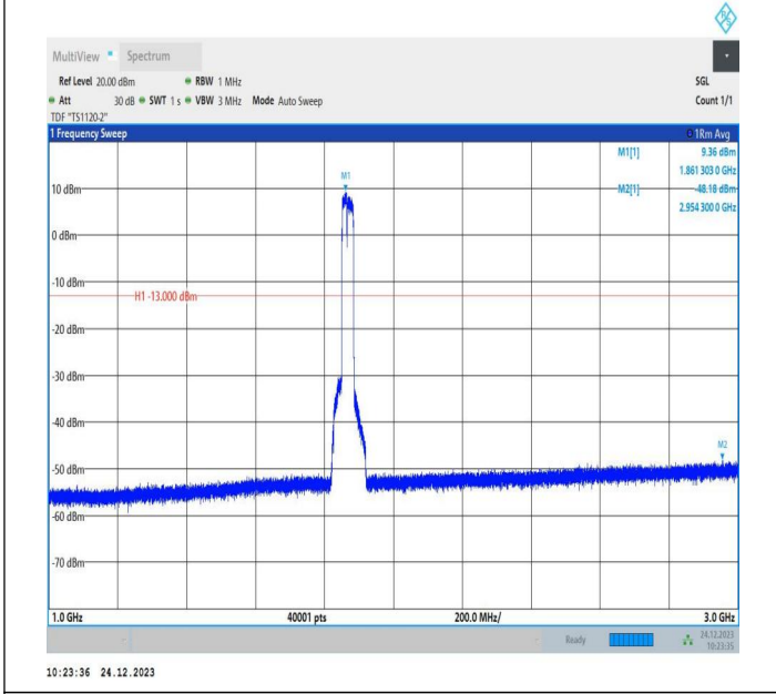
2-2-15MHz-20MHz-QPSK-QPSK-18678-18849-75RB#0-100R B#0-1000~3000MHz-PASS
