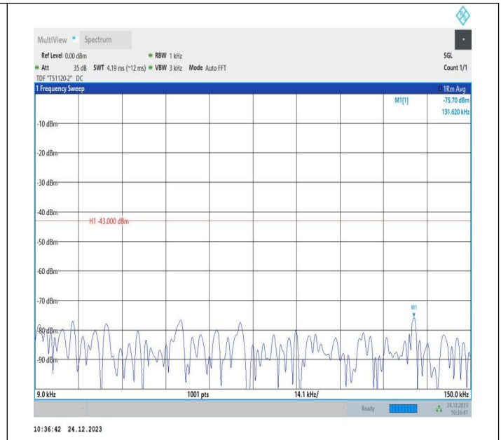
2-2-15MHz-20MHz-QPSK-QPSK-18929-19100-1RB#74-0RB#0 0-0.009~0.15MHz-PASS
