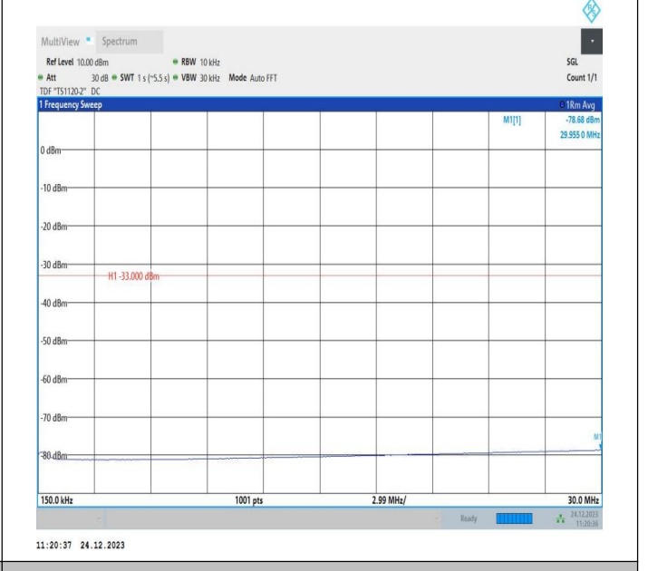
2-2-20MHz-15MHz-QPSK-QPSK-18700-18871-1RB#0-1RB#7 4-0.15~30MHz-PASS
