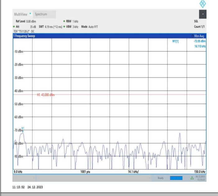
2-2-20MHz-5MHz-QPSK-QPSK-19050-19167-1RB#0-1RB#24 -0.009~0.15MHz-PASS
