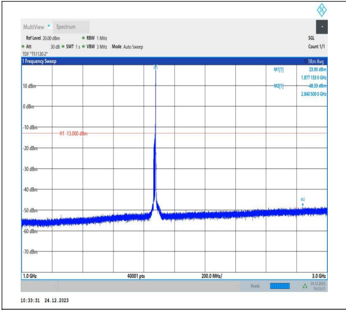
2-2-15MHz-20MHz-QPSK-QPSK-18803-18974-1RB#74-0RB# 0-1000~3000MHz-PASS
