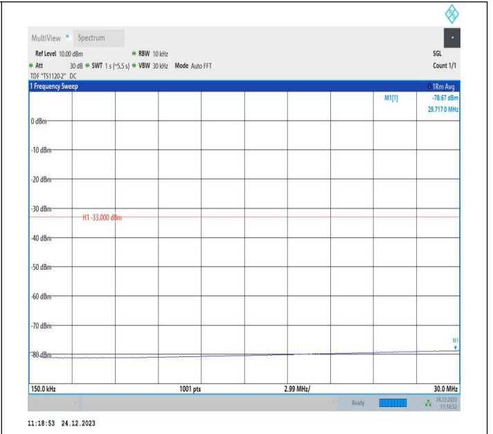
2-2-20MHz-15MHz-QPSK-QPSK-18700-18871-1RB#0-0RB#0 -0.15~30MHz-PASS
