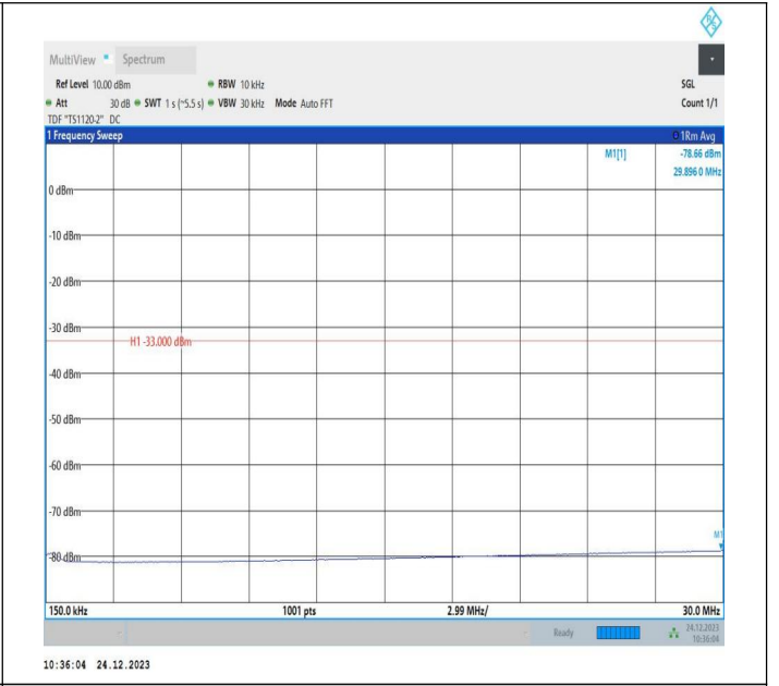
2-2-15MHz-20MHz-QPSK-QPSK-18929-19100-1RB#0-0RB#0 -0.15~30MHz-PASS
