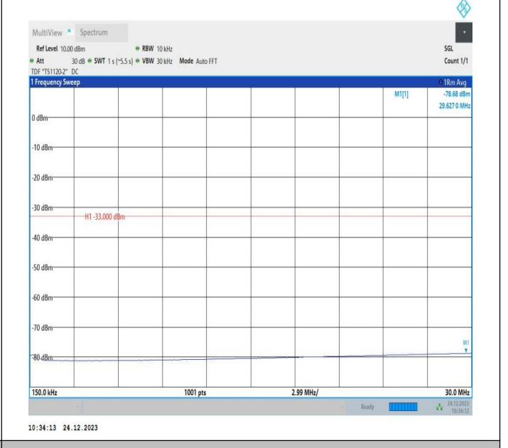
2-2-15MHz-20MHz-QPSK-QPSK-18803-18974-1RB#0-1RB#9 9-0.15~30MHz-PASS
