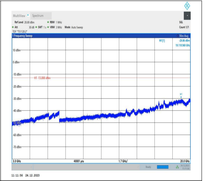
2-2-20MHz-5MHz-QPSK-QPSK-18875-18992-1RB#99-0RB#0 -3000~20000MHz-PASS
