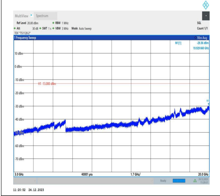
2-2-20MHz-15MHz-QPSK-QPSK-18700-18871-1RB#0-1RB#7 4-3000~20000MHz-PASS
