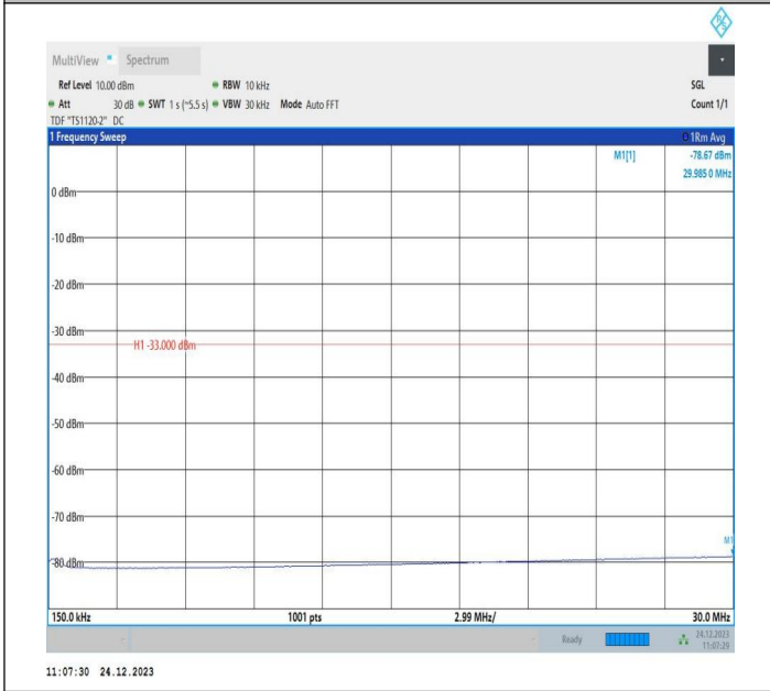
2-2-20MHz-5MHz-QPSK-QPSK-18700-18817-1RB#99-0RB#0-0.15~30MHz-PASS
