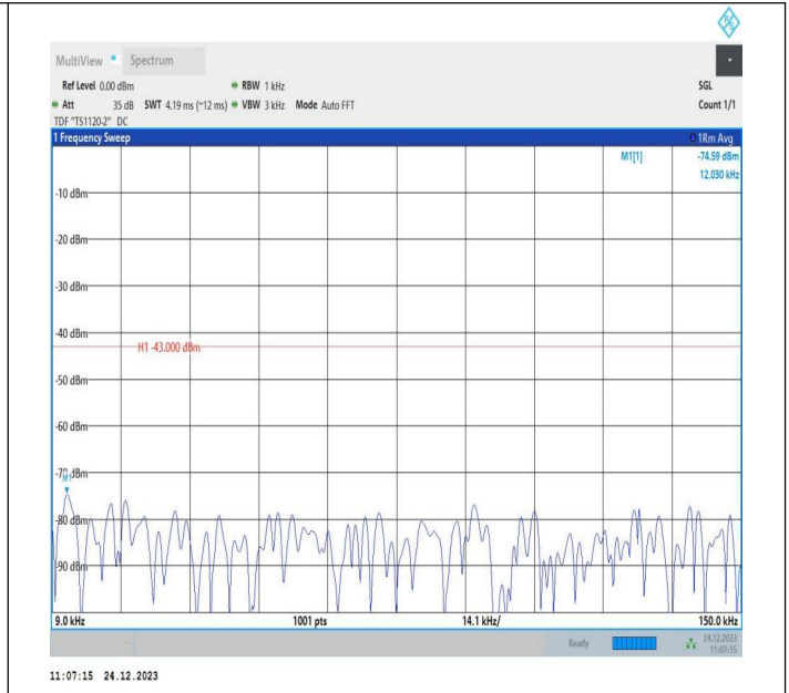
2-2-20MHz-5MHz-QPSK-QPSK-18700-18817-1RB#99-0RB#0-0.009~0.15MHz-PASS
