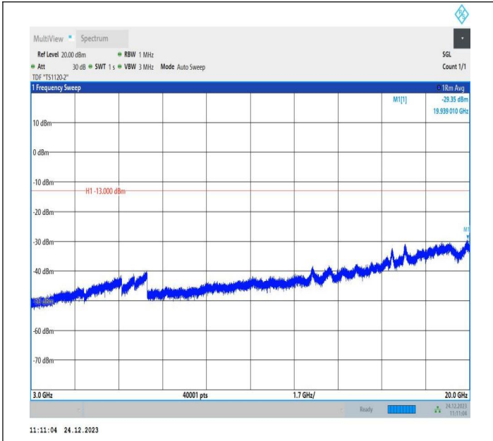
2-2-20MHz-5MHz-QPSK-QPSK-18875-18992-1RB#0-0RB#0-3000~20000MHz-PASS
