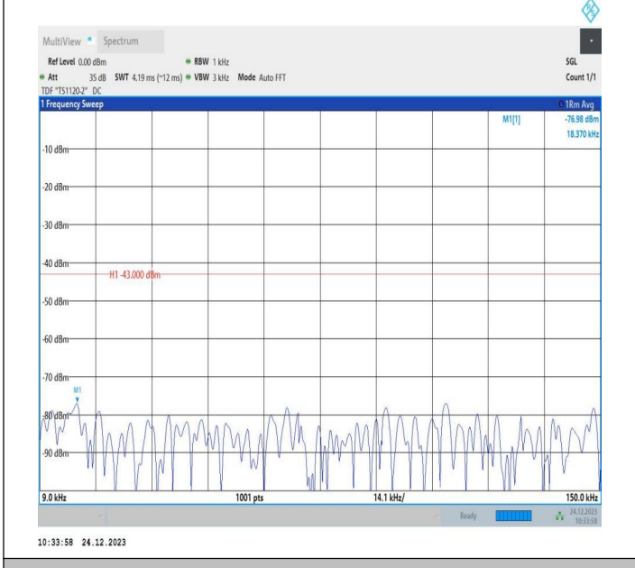
2-2-15MHz-20MHz-QPSK-QPSK-18803-18974-1RB#0-1RB#9 9-0.009~0.15MHz-PASS
