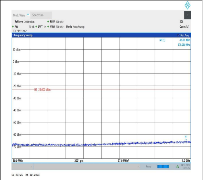
2-2-15MHz-20MHz-QPSK-QPSK-18803-18974-1RB#74-0RB# 0-30~1000MHz-PASS
