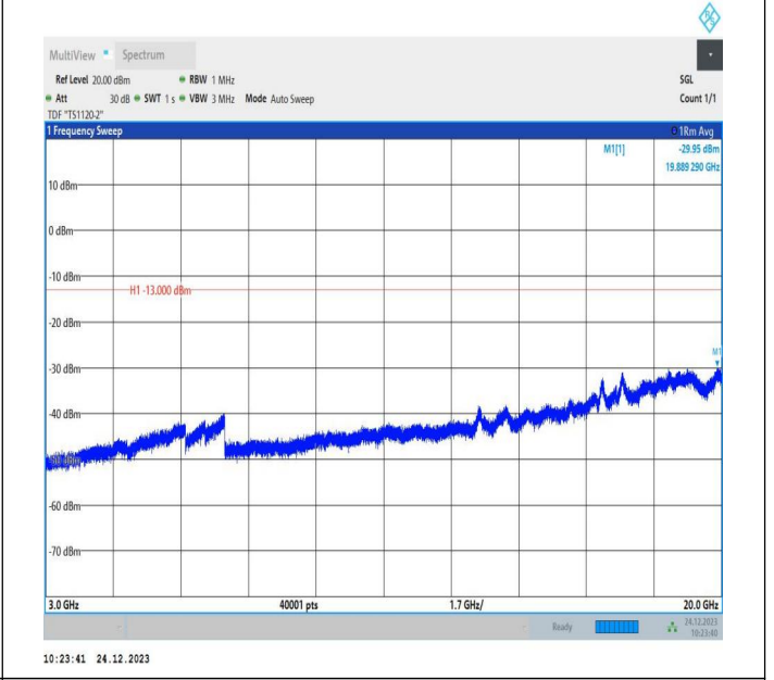
2-2-15MHz-20MHz-QPSK-QPSK-18678-18849-75RB#0-100R B#0-3000~20000MHz-PASS
