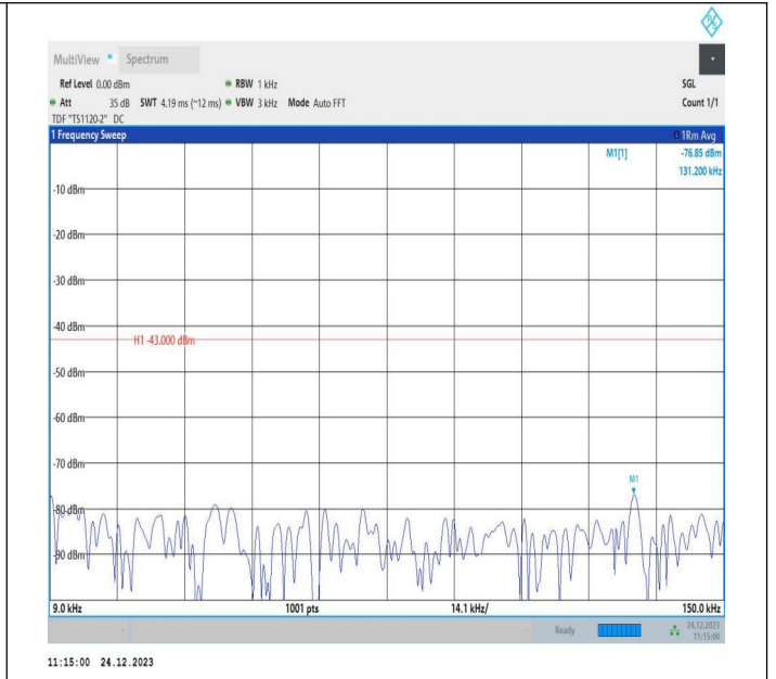
2-2-20MHz-5MHz-QPSK-QPSK-19050-19167-1RB#99-0RB#0-0.009~0.15MHz-PASS
