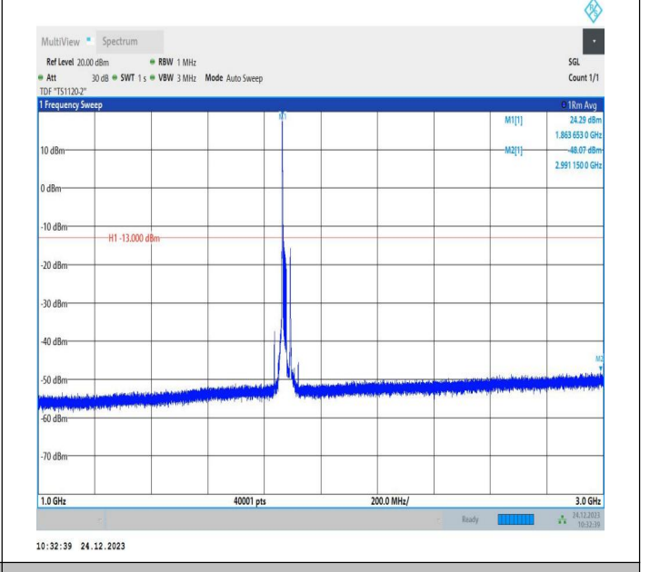
2-2-15MHz-20MHz-QPSK-QPSK-18803-18974-1RB#0-0RB#0 -1000~3000MHz-PASS
