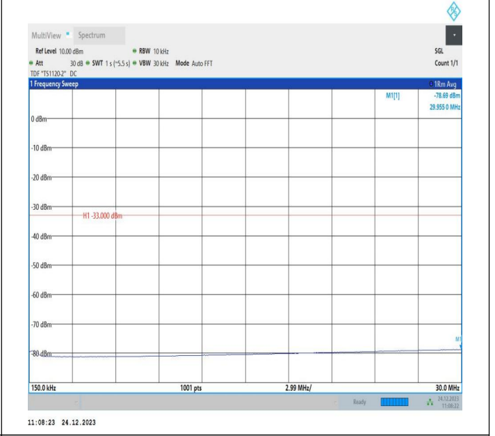
2-2-20MHz-5MHz-QPSK-QPSK-18700-18817-1RB#0-1RB#24 -0.15~30MHz-PASS
