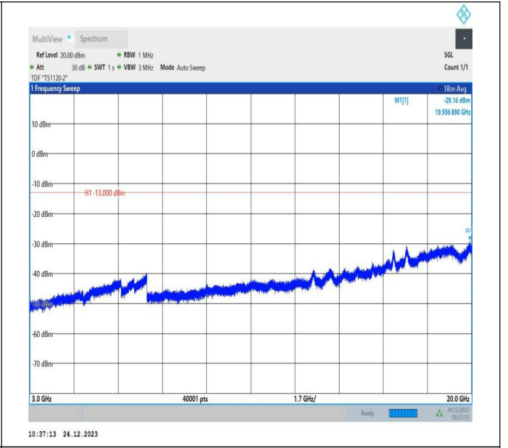
2-2-15MHz-20MHz-QPSK-QPSK-18929-19100-1RB#74-0RB# 0-3000~20000MHz-PASS
