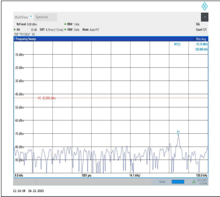
2-2-20MHz-5MHz-QPSK-QPSK-19050-19167-1RB#0-0RB#0-0.009~0.15MHz-PASS
