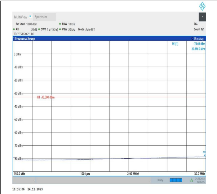
2-2-15MHz-20MHz-QPSK-QPSK-18803-18974-75RB#0-100R B#0-0.15~30MHz-PASS
