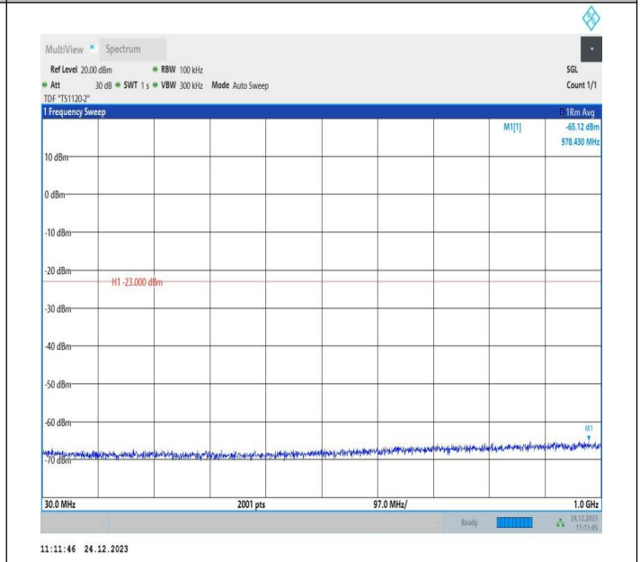
2-2-20MHz-5MHz-QPSK-QPSK-18875-18992-1RB#99-0RB#0-30~1000MHz-PASS
