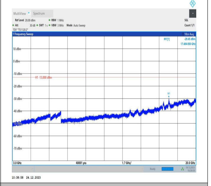
2-2-15MHz-20MHz-QPSK-QPSK-18929-19100-75RB#0-100R B#0-3000~20000MHz-PASS
