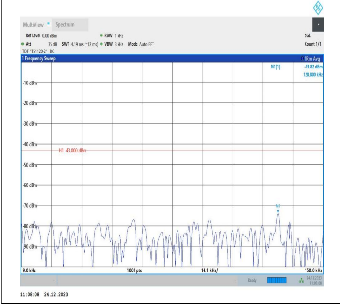
2-2-20MHz-5MHz-QPSK-QPSK-18700-18817-1RB#0-1RB#24 -0.009~0.15MHz-PASS
