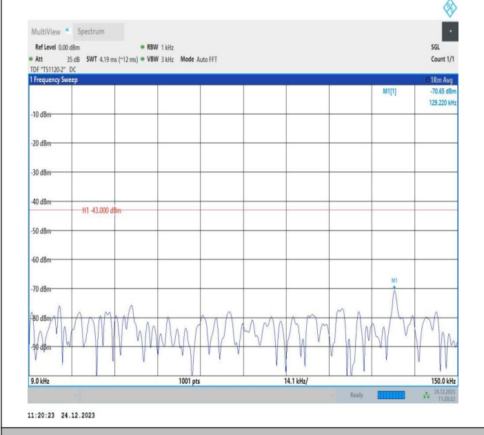
2-2-20MHz-15MHz-QPSK-QPSK-18700-18871-1RB#0-1RB#7 4-0.009~0.15MHz-PASS
