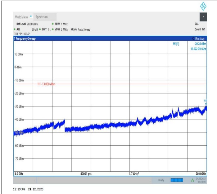
2-2-20MHz-15MHz-QPSK-QPSK-18700-18871-1RB#0-0RB#0 -3000~20000MHz-PASS
