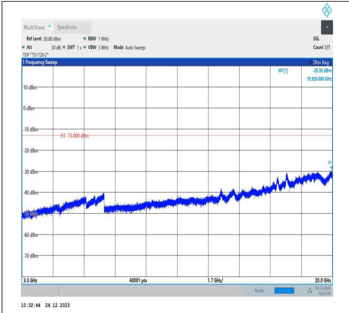
2-2-15MHz-20MHz-QPSK-QPSK-18803-18974-1RB#0-0RB# -3000~20000MHz-PASS
