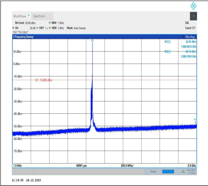
2-2-20MHz-15MHz-QPSK-QPSK-18700-18871-1RB#99-0RB# 0-1000~3000MHz-PASS
