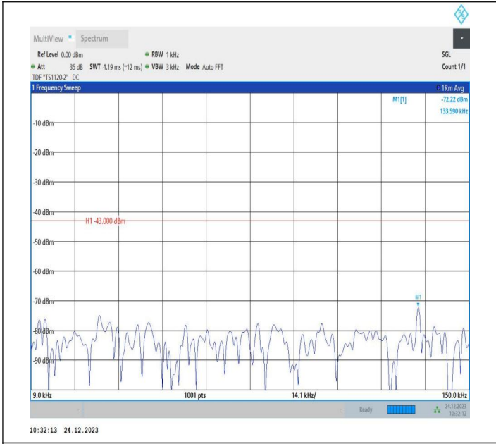
2-2-15MHz-20MHz-QPSK-QPSK-18803-18974-1RB#0-0RB#0 -0.009~0.15MHz-PASS
