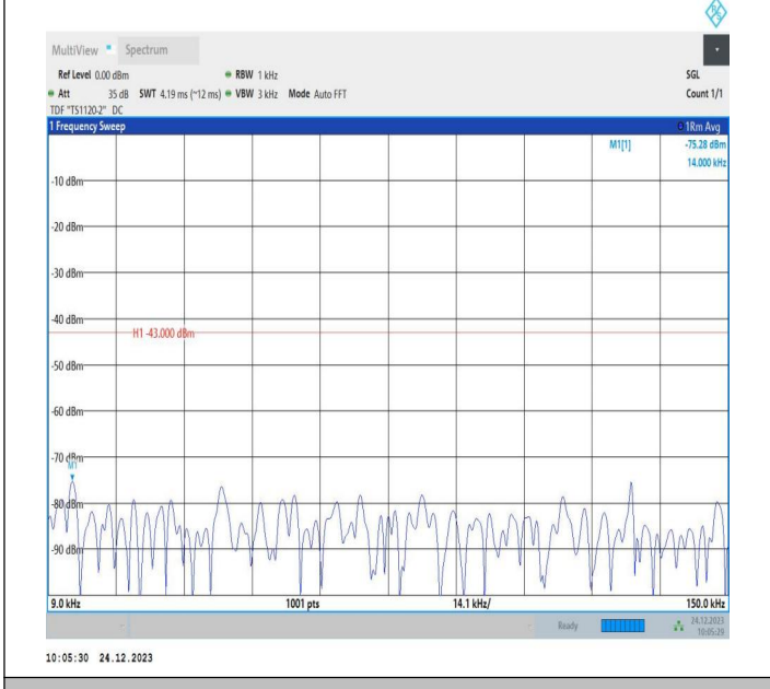
2-2-15MHz-10MHz-QPSK-QPSK-19027-19147-1RB#0-1RB#4 9-0.009~0.15MHz-PASS
