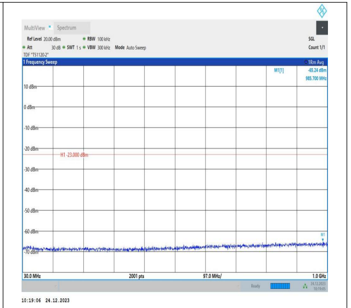
2-2-15MHz-15MHz-QPSK-QPSK-18975-19125-75RB#0-75RB #0-30~1000MHz-PASS
