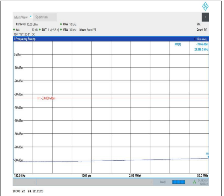
2-2-15MHz-10MHz-QPSK-QPSK-18851-18971-1RB#0-0RB#0 -0.15~30MHz-PASS
