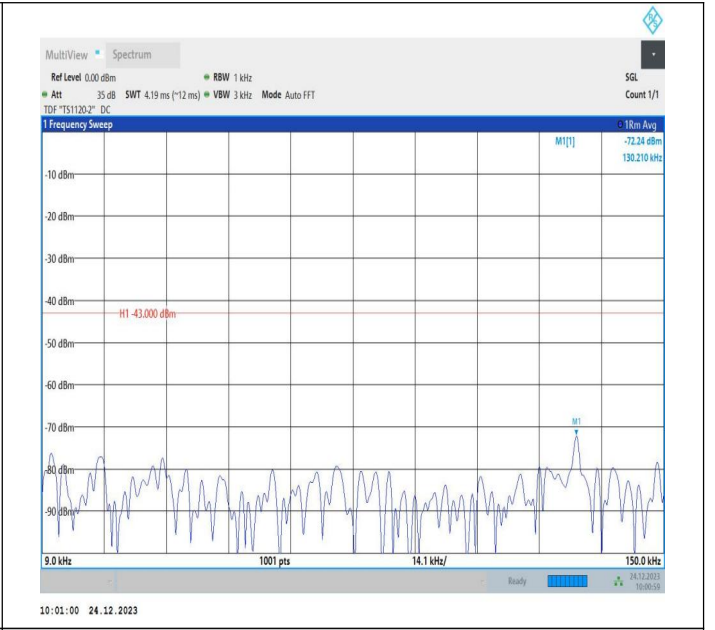
2-2-15MHz-10MHz-QPSK-QPSK-18851-18971-1RB#74-0RB# 0-0.009~0.15MHz-PASS
