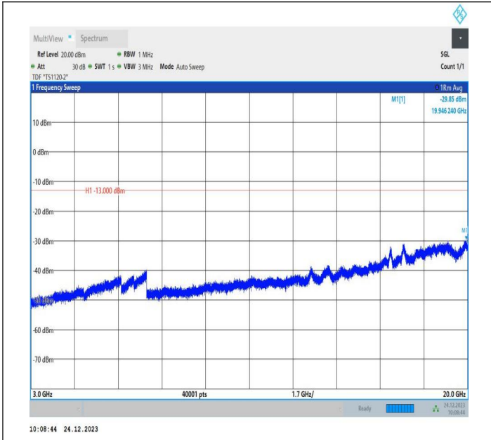
2-2-15MHz-15MHz-QPSK-QPSK-18675-18825-1RB#0-0RB# -3000~20000MHz-PASS
