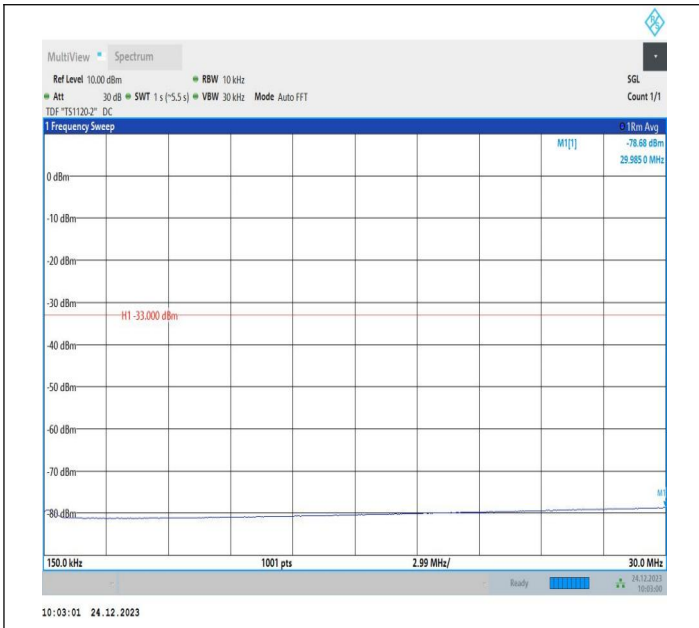
2-2-15MHz-10MHz-QPSK-QPSK-18851-18971-75RB#0-50RB #0-0.15~30MHz-PASS
