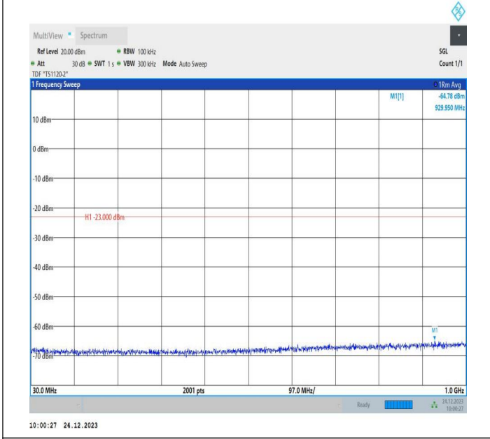
2-2-15MHz-10MHz-QPSK-QPSK-18851-18971-1RB#0-0RB#0 -30~1000MHz-PASS
