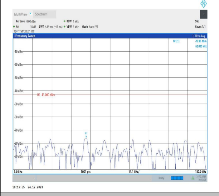
2-2-15MHz-15MHz-QPSK-QPSK-18975-19125-1RB#0-1RB#7 4-0.009~0.15MHz-PASS
