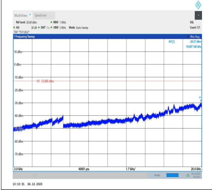
2-2-15MHz-15MHz-QPSK-QPSK-18675-18825-1RB#0-1RB#7 4-3000~20000MHz-PASS
