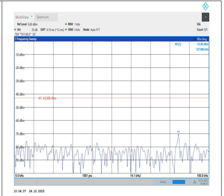
2-2-15MHz-10MHz-QPSK-QPSK-19027-19147-1RB#74-0RB#0 0-0.009~0.15MHz-PASS
