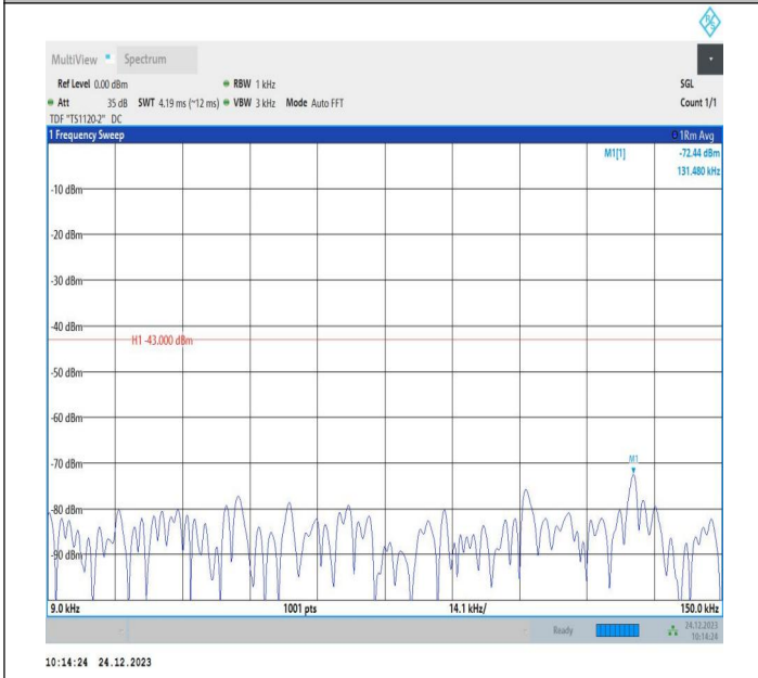
2-2-15MHz-15MHz-QPSK-QPSK-18825-18975-1RB#0-1RB#7 4-0.009~0.15MHz-PASS
