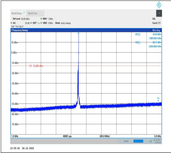
2-2-15MHz-10MHz-QPSK-QPSK-19027-19147-1RB#74-0RB# 0-1000~3000MHz-PASS
