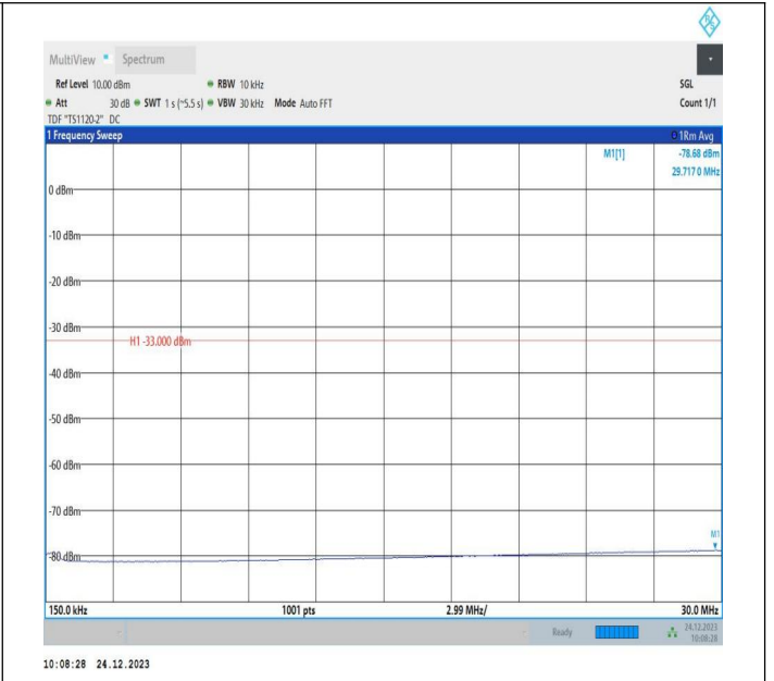
2-2-15MHz-15MHz-QPSK-QPSK-18675-18825-1RB#0-0RB#0 -0.15~30MHz-PASS
