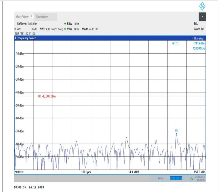
2-2-15MHz-15MHz-QPSK-QPSK-18675-18825-1RB#74-0RB# 0-0.009~0.15MHz-PASS
