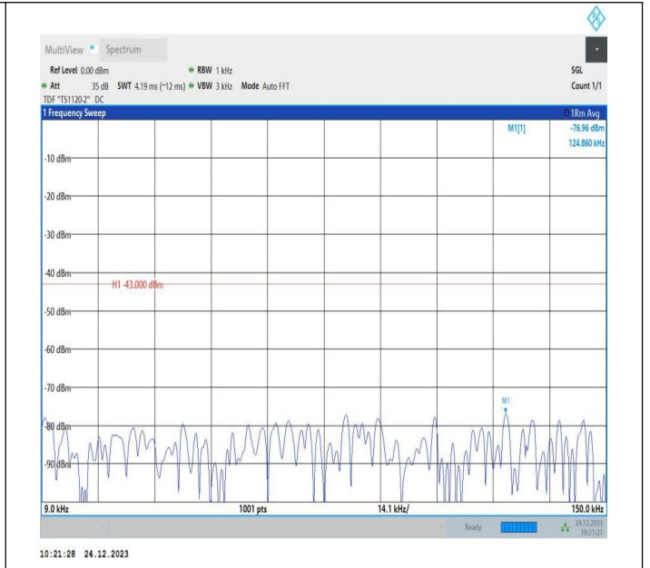
2-2-15MHz-20MHz-QPSK-QPSK-18678-18849-1RB#74-0RB#0 0-0.009~0.15MHz-PASS
