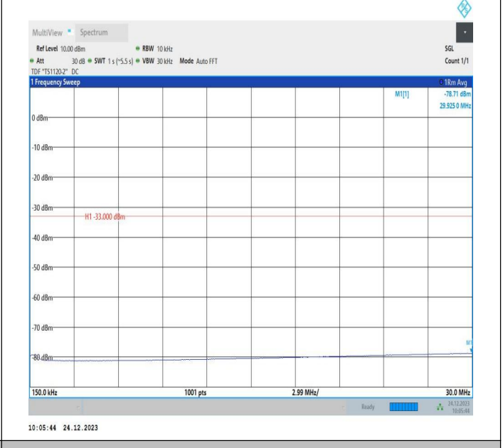
2-2-15MHz-10MHz-QPSK-QPSK-19027-19147-1RB#0-1RB#4 9-0.15~30MHz-PASS
