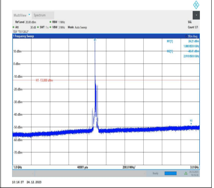
2-2-15MHz-15MHz-QPSK-QPSK-18975-19125-1RB#0-0RB#0 -1000~3000MHz-PASS
