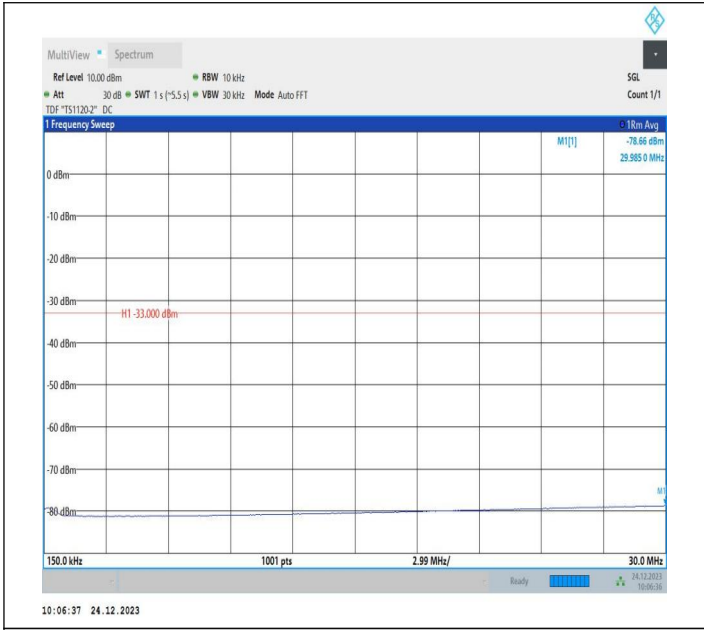
2-2-15MHz-10MHz-QPSK-QPSK-19027-19147-75RB#0-50RB #0-0.15~30MHz-PASS
