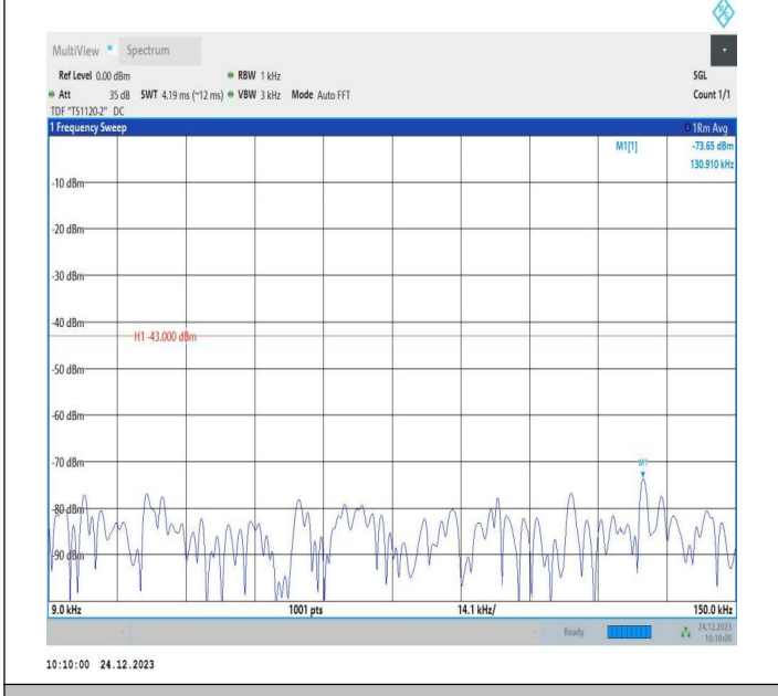
2-2-15MHz-15MHz-QPSK-QPSK-18675-18825-1RB#0-1RB#7 4-0.009~0.15MHz-PASS
