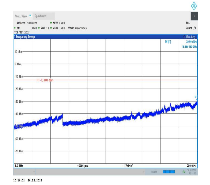
2-2-15MHz-15MHz-QPSK-QPSK-18825-18975-1RB#74-0RB# 0-3000~20000MHz-PASS
