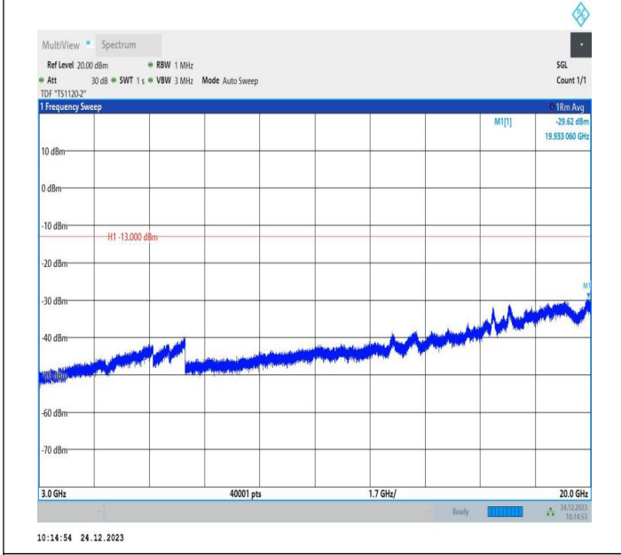
2-2-15MHz-15MHz-QPSK-QPSK-18825-18975-1RB#0-1RB#7 4-3000~20000MHz-PASS
