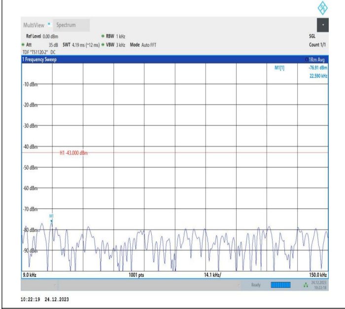
2-2-15MHz-20MHz-QPSK-QPSK-18678-18849-1RB#0-1RB#9 9-0.009~0.15MHz-PASS
