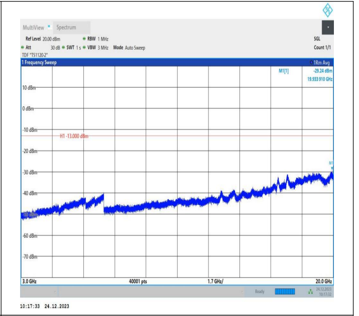
2-2-15MHz-15MHz-QPSK-QPSK-18975-19125-1RB#74-0RB# 0-3000~20000MHz-PASS
