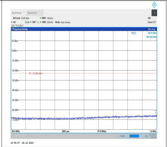
2-2-15MHz-15MHz-QPSK-QPSK-18675-18825-1RB#74-0RB# 0-30~1000MHz-PASS
