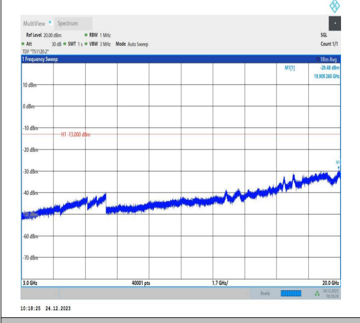
2-2-15MHz-15MHz-QPSK-QPSK-18975-19125-1RB#0-1RB#7 4-3000~20000MHz-PASS
