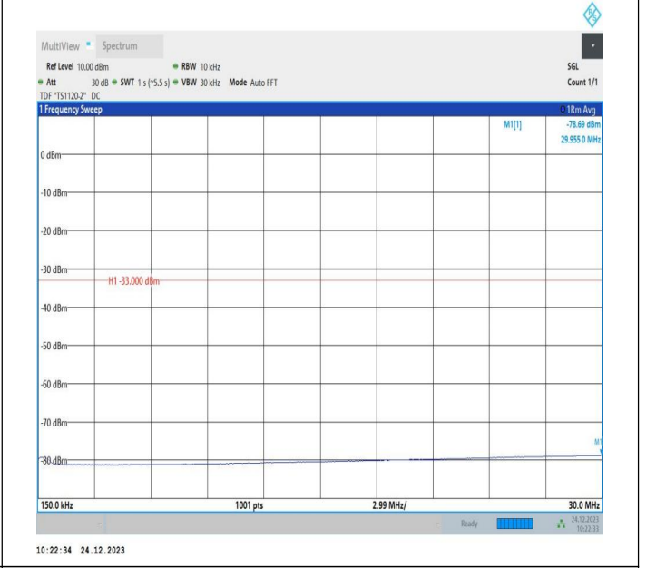
2-2-15MHz-20MHz-QPSK-QPSK-18678-18849-1RB#0-1RB#9 9-0.15~30MHz-PASS
