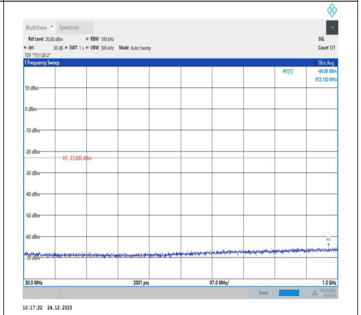
2-2-15MHz-15MHz-QPSK-QPSK-18975-19125-1RB#74-0RB#7 0-30~1000MHz-PASS
