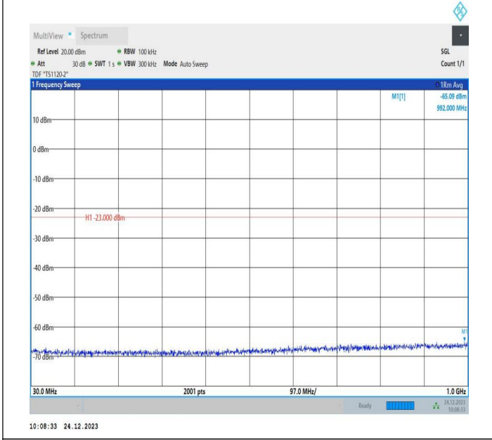
2-2-15MHz-15MHz-QPSK-QPSK-18675-18825-1RB#0-0RB#0 -30~1000MHz-PASS
