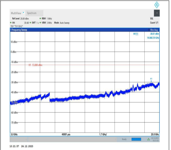
2-2-15MHz-20MHz-QPSK-QPSK-18678-18849-1RB#74-0RB# 0-3000~20000MHz-PASS
