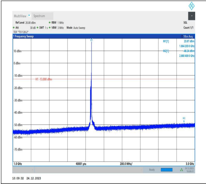
2-2-15MHz-15MHz-QPSK-QPSK-18675-18825-1RB#74-0RB# 0-1000~3000MHz-PASS
