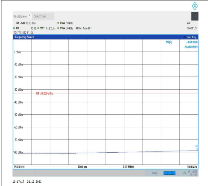
2-2-15MHz-15MHz-QPSK-QPSK-18975-19125-1RB#74-0RB#7 0-0.15~30MHz-PASS
