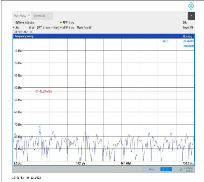
2-2-15MHz-10MHz-QPSK-QPSK-18851-18971-1RB#0-1RB#4 9-0.009~0.15MHz-PASS
