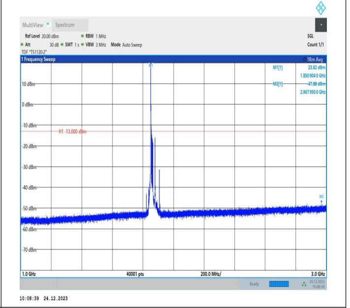
2-2-15MHz-15MHz-QPSK-QPSK-18675-18825-1RB#0-0RB#0 -1000~3000MHz-PASS
