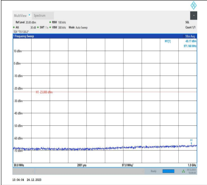
2-2-15MHz-10MHz-QPSK-QPSK-19027-19147-1RB#0-0RB#0 -30~1000MHz-PASS
