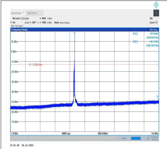
2-2-15MHz-20MHz-QPSK-QPSK-18678-18849-1RB#74-0RB# 0-1000~3000MHz-PASS
