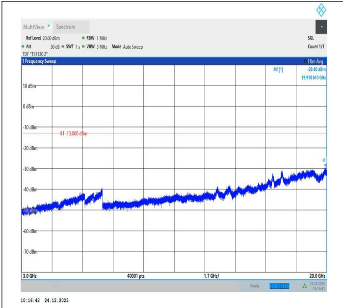
2-2-15MHz-15MHz-QPSK-QPSK-18975-19125-1RB#0-0RB#0 -3000~20000MHz-PASS
