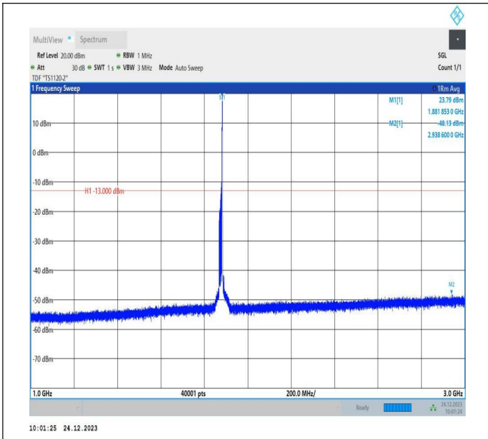
2-2-15MHz-10MHz-QPSK-QPSK-18851-18971-1RB#74-0RB# 0-1000~3000MHz-PASS
