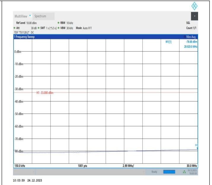
2-2-15MHz-10MHz-QPSK-QPSK-19027-19147-1RB#0-0RB#0 -0.15~30MHz-PASS
