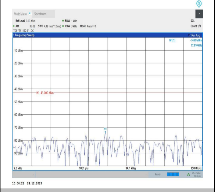
2-2-15MHz-10MHz-QPSK-QPSK-19027-19147-75RB#0-50RB #0-0.009~0.15MHz-PASS
