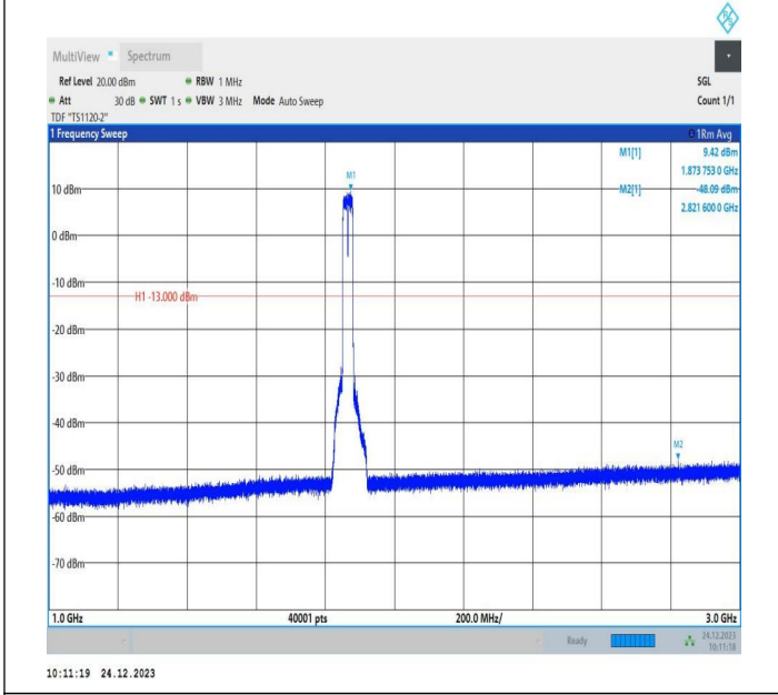
2-2-15MHz-15MHz-QPSK-QPSK-18675-18825-75RB#0-75RB #0-1000~3000MHz-PASS
