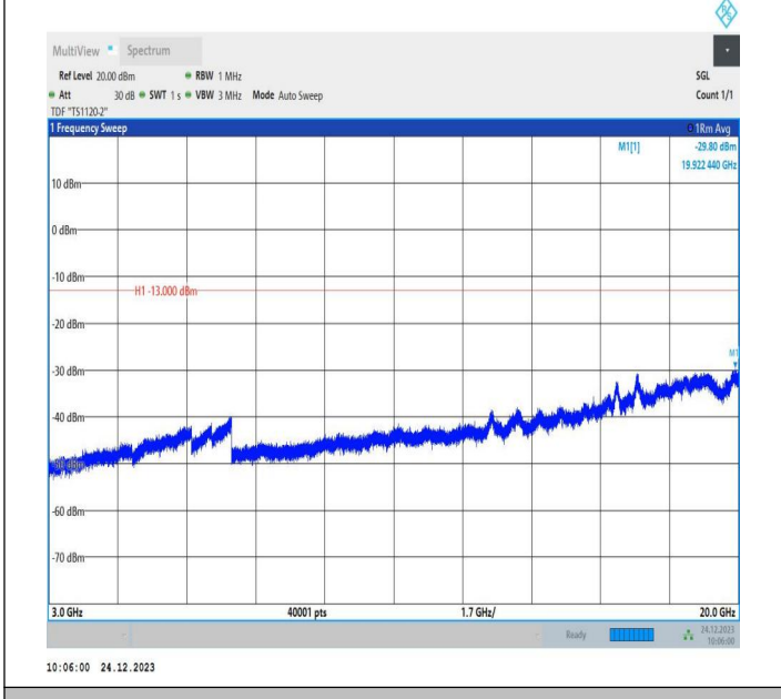
2-2-15MHz-10MHz-QPSK-QPSK-19027-19147-1RB#0-1RB#4 9-3000~20000MHz-PASS
