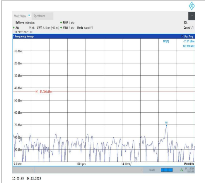
2-2-15MHz-10MHz-QPSK-QPSK-19027-19147-1RB#0-0RB#0 -0.009~0.15MHz-PASS
