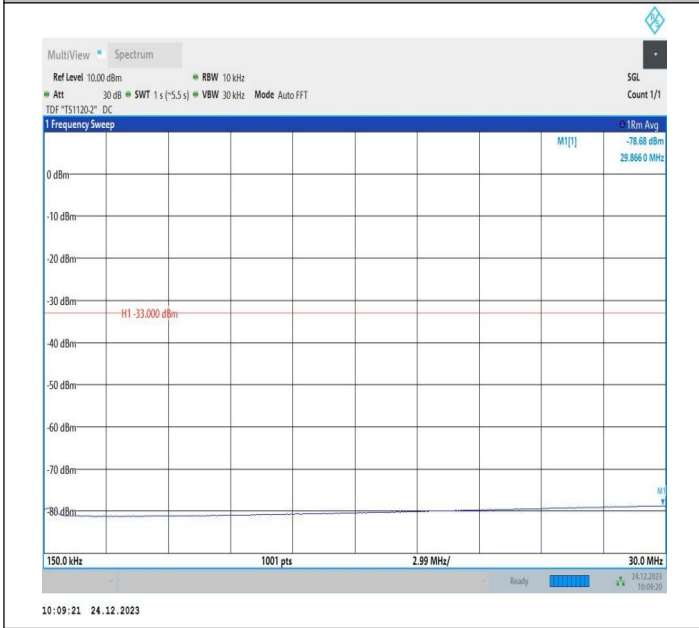
2-2-15MHz-15MHz-QPSK-QPSK-18675-18825-1RB#74-0RB# 0-0.15~30MHz-PASS
