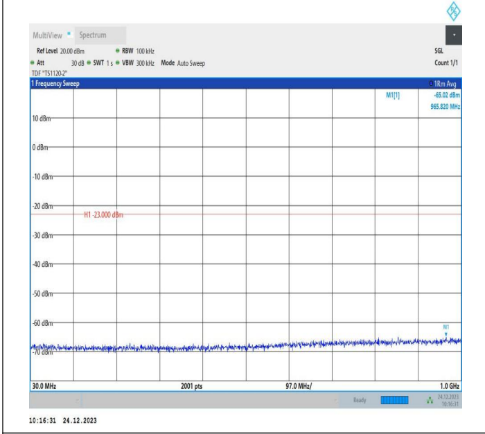
2-2-15MHz-15MHz-QPSK-QPSK-18975-19125-1RB#0-0RB#0 -30~1000MHz-PASS
