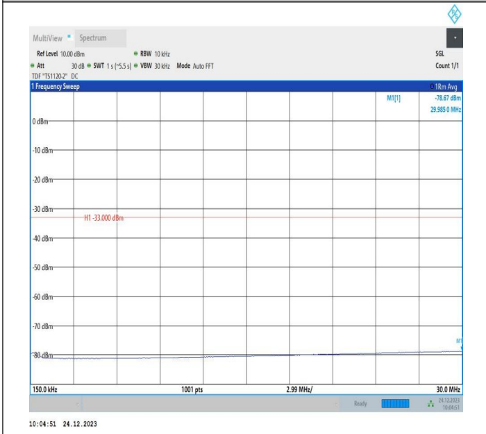
2-2-15MHz-10MHz-QPSK-QPSK-19027-19147-1RB#74-0RB#0 0-0.15~30MHz-PASS
