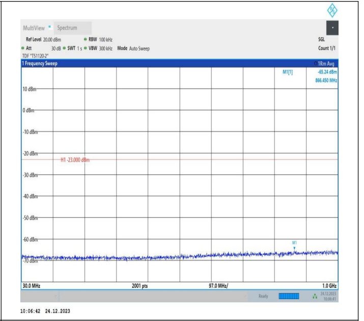
2-2-15MHz-10MHz-QPSK-QPSK-19027-19147-75RB#0-50RB #0-30~1000MHz-PASS
