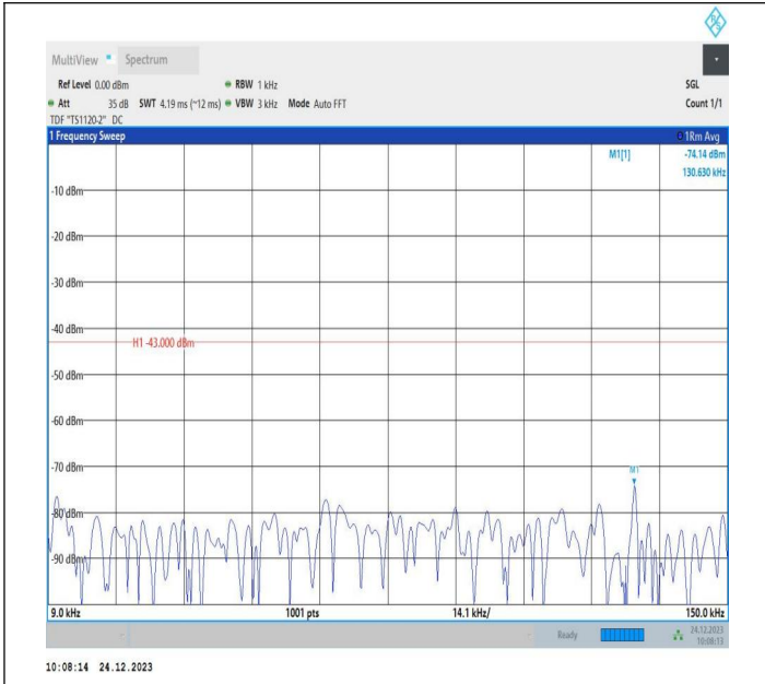
2-2-15MHz-15MHz-QPSK-QPSK-18675-18825-1RB#0-0RB#0 -0.009~0.15MHz-PASS
