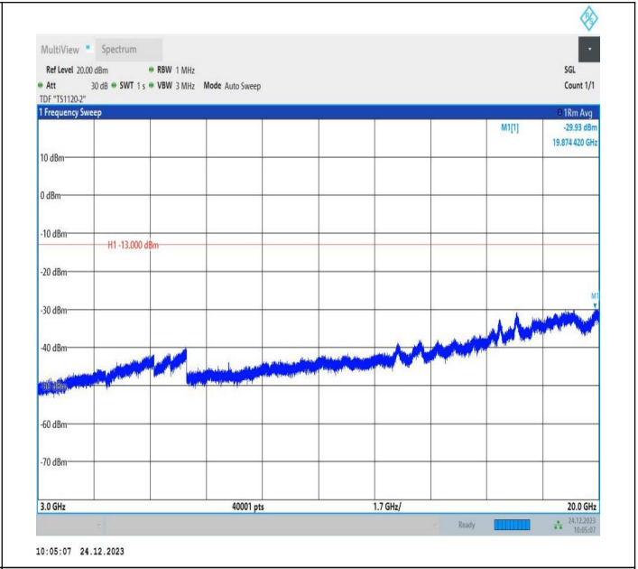
2-2-15MHz-10MHz-QPSK-QPSK-19027-19147-1RB#74-0RB# 0-3000~20000MHz-PASS
