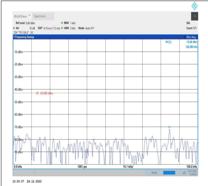
2-2-15MHz-10MHz-QPSK-QPSK-18851-18971-1RB#0-0RB#0 -0.009~0.15MHz-PASS
