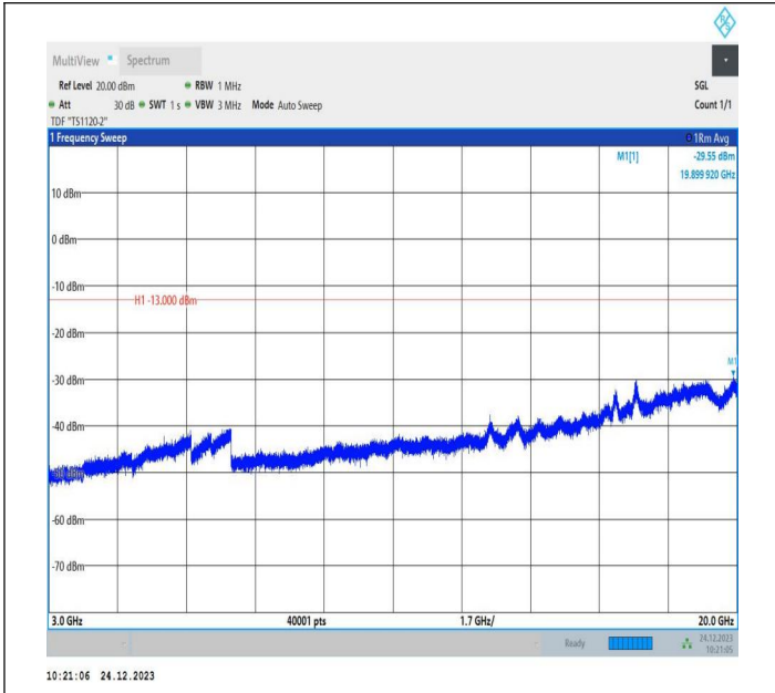
2-2-15MHz-20MHz-QPSK-QPSK-18678-18849-1RB#0-0RB#0 -3000~20000MHz-PASS
