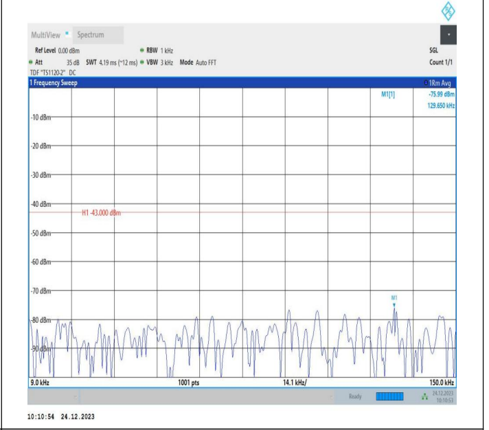
2-2-15MHz-15MHz-QPSK-QPSK-18675-18825-75RB#0-75RB #0-0.009~0.15MHz-PASS
