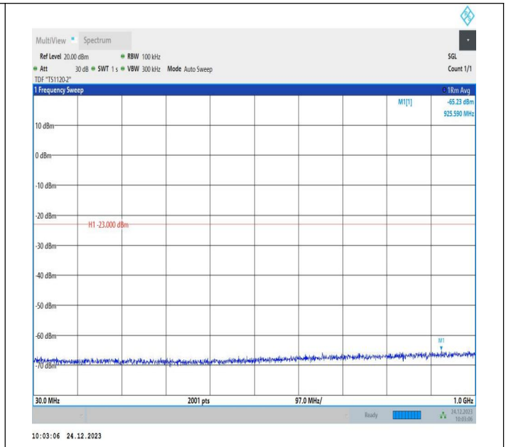
2-2-15MHz-10MHz-QPSK-QPSK-18851-18971-75RB#0-50RB #0-30~1000MHz-PASS
