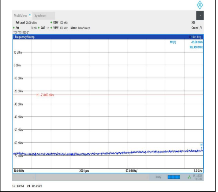
2-2-15MHz-15MHz-QPSK-QPSK-18825-18975-1RB#74-0RB#74 0-30~1000MHz-PASS
