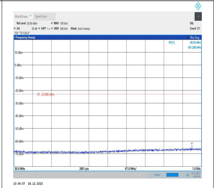
2-2-15MHz-10MHz-QPSK-QPSK-19027-19147-1RB#74-0RB#0 0-30~1000MHz-PASS
