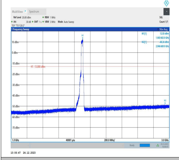
2-2-15MHz-10MHz-QPSK-QPSK-19027-19147-75RB#0-50RB #0-1000~3000MHz-PASS
