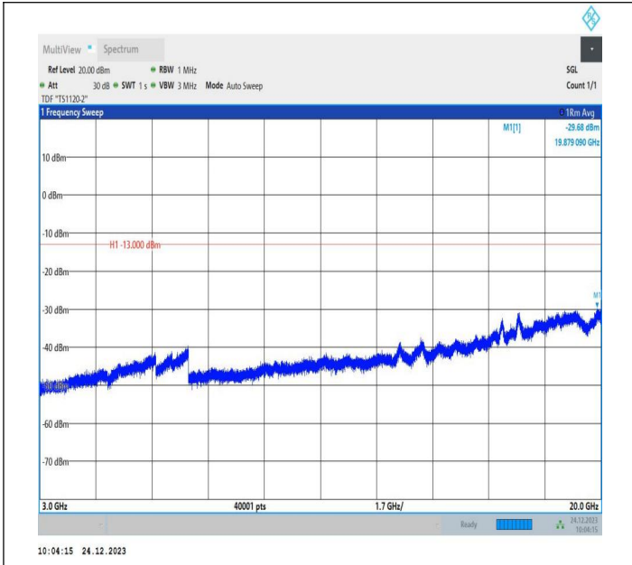
2-2-15MHz-10MHz-QPSK-QPSK-19027-19147-1RB#0-0RB#0 -3000~20000MHz-PASS
