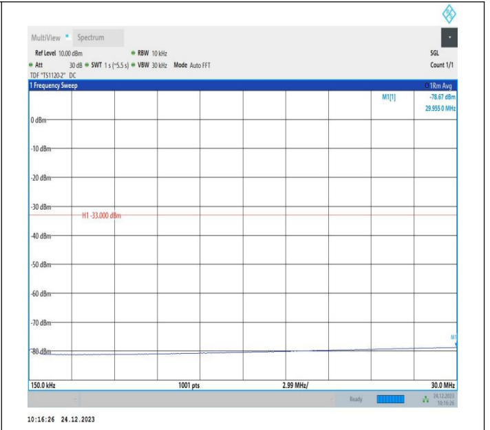
2-2-15MHz-15MHz-QPSK-QPSK-18975-19125-1RB#0-0RB#0 -0.15~30MHz-PASS
