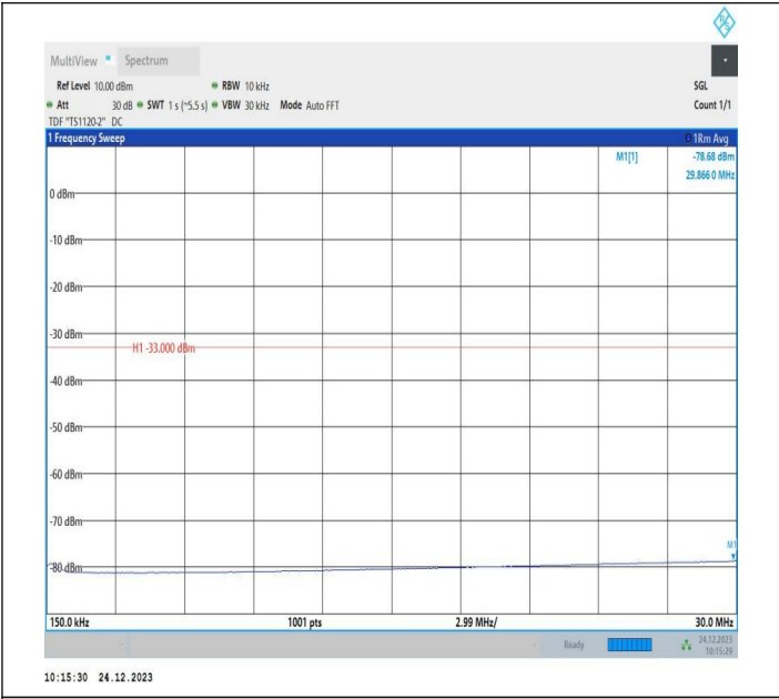
2-2-15MHz-15MHz-QPSK-QPSK-18825-18975-75RB#0-75RB #0-0.15~30MHz-PASS
