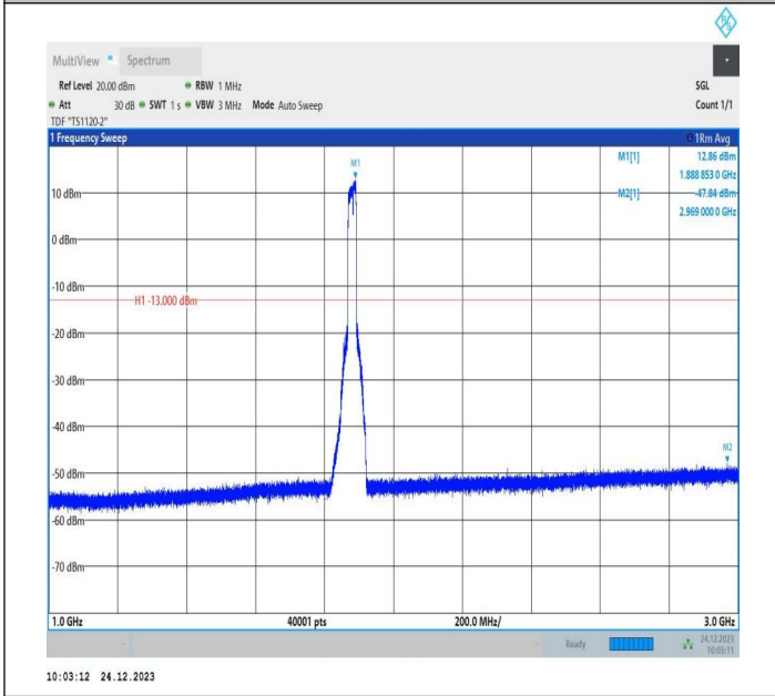
2-2-15MHz-10MHz-QPSK-QPSK-18851-18971-75RB#0-50RB #0-1000~3000MHz-PASS
