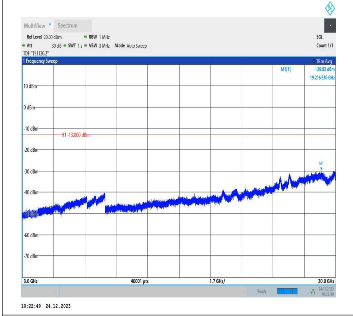
2-2-15MHz-20MHz-QPSK-QPSK-18678-18849-1RB#0-1RB#9 9-3000~20000MHz-PASS
