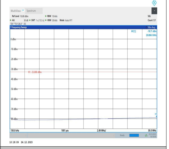
2-2-15MHz-15MHz-QPSK-QPSK-18975-19125-1RB#0-1RB#7 4-0.15~30MHz-PASS
