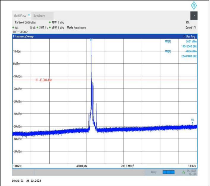
2-2-15MHz-20MHz-QPSK-QPSK-18678-18849-1RB#0-0RB#0 -1000~3000MHz-PASS
