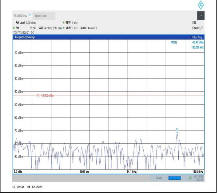
2-2-15MHz-10MHz-QPSK-QPSK-18851-18971-75RB#0-50RB #0-0.009~0.15MHz-PASS
