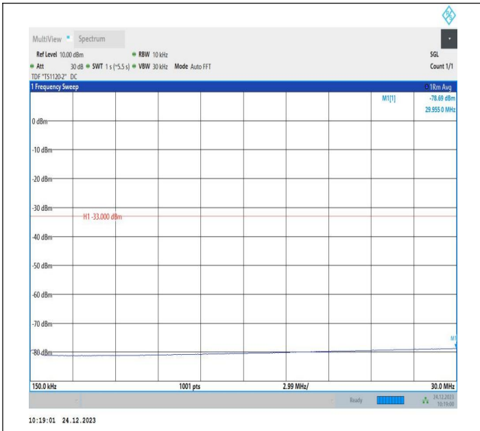
2-2-15MHz-15MHz-QPSK-QPSK-18975-19125-75RB#0-75RB #0-0.15~30MHz-PASS
