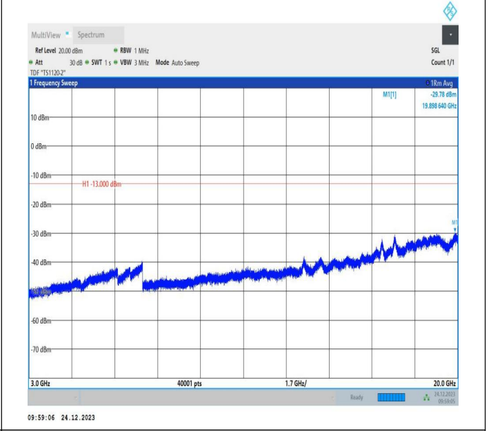
2-2-15MHz-10MHz-QPSK-QPSK-18675-18795-75RB#0-50RB #0-3000~20000MHz-PASS
