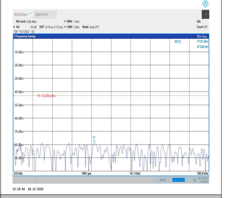
2-2-15MHz-15MHz-QPSK-QPSK-18975-19125-75RB#0-75RB #0-0.009~0.15MHz-PASS
