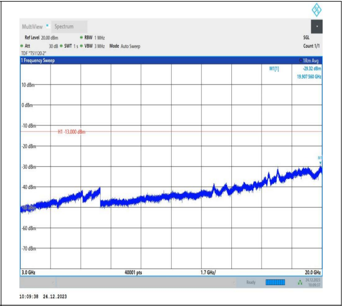
2-2-15MHz-15MHz-QPSK-QPSK-18675-18825-1RB#74-0RB# 0-3000~20000MHz-PASS
