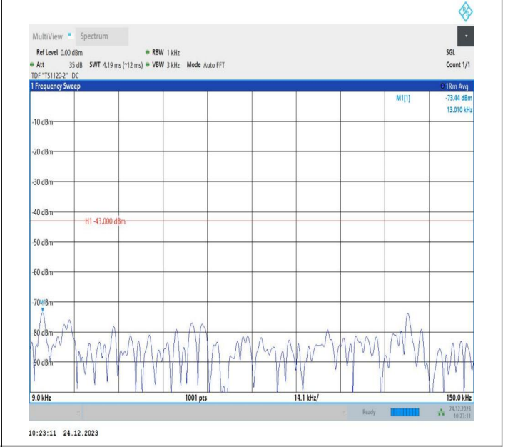
2-2-15MHz-20MHz-QPSK-QPSK-18678-18849-75RB#0-100R B#0-0.009~0.15MHz-PASS
