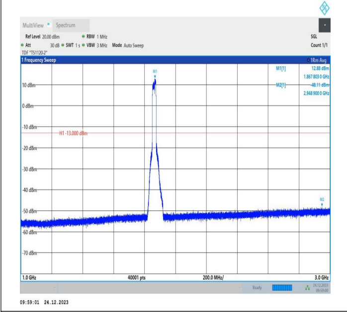
2-2-15MHz-10MHz-QPSK-QPSK-18675-18795-75RB#0-50RB #0-1000~3000MHz-PASS
