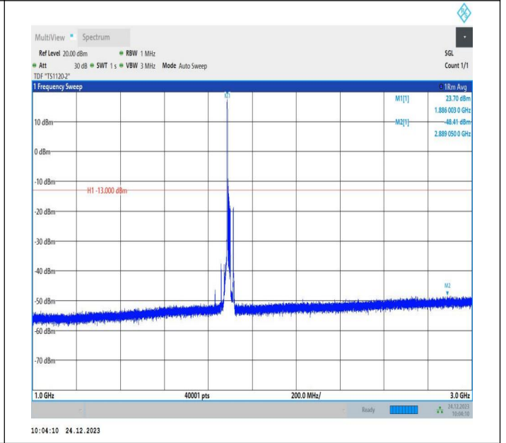
2-2-15MHz-10MHz-QPSK-QPSK-19027-19147-1RB#0-0RB#0 -1000~3000MHz-PASS
