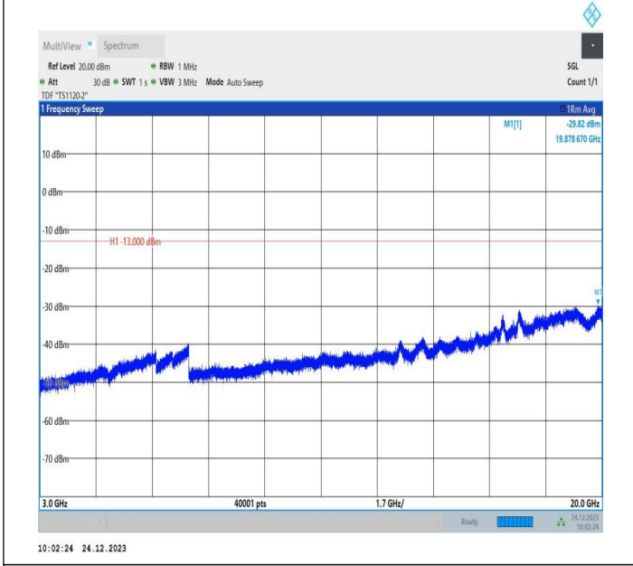
2-2-15MHz-10MHz-QPSK-QPSK-18851-18971-1RB#0-1RB#4 9-3000~20000MHz-PASS
