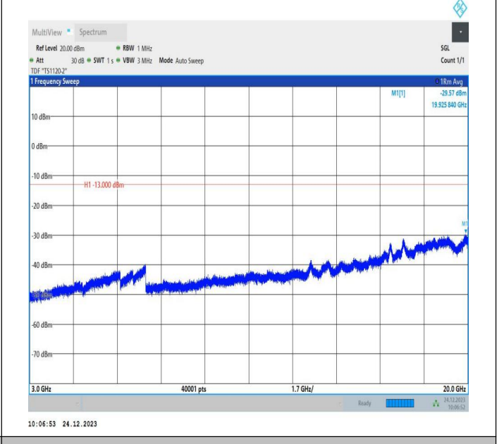
2-2-15MHz-10MHz-QPSK-QPSK-19027-19147-75RB#0-50RB #0-3000~20000MHz-PASS
