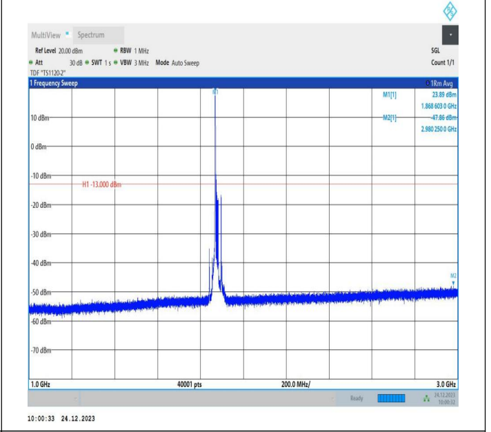
2-2-15MHz-10MHz-QPSK-QPSK-18851-18971-1RB#0-0RB#0 -1000~3000MHz-PASS
