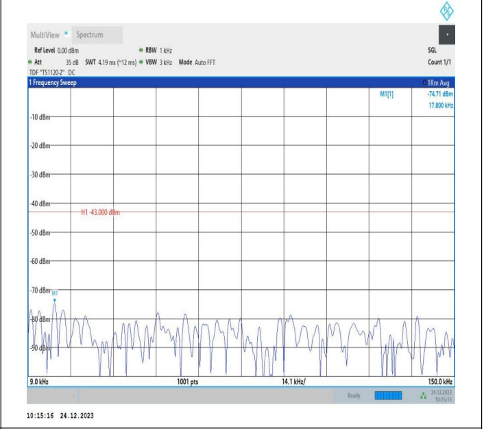
2-2-15MHz-15MHz-QPSK-QPSK-18825-18975-75RB#0-75RB #0-0.009~0.15MHz-PASS
