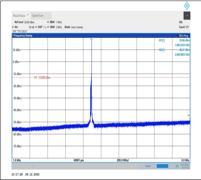
2-2-15MHz-15MHz-QPSK-QPSK-18975-19125-1RB#74-0RB# 0-1000~3000MHz-PASS
