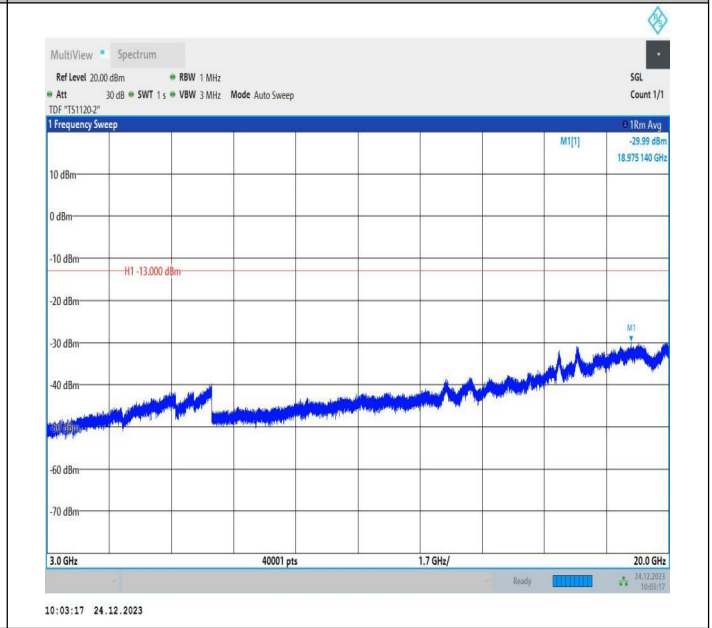
2-2-15MHz-10MHz-QPSK-QPSK-18851-18971-75RB#0-50RB #0-3000~20000MHz-PASS
