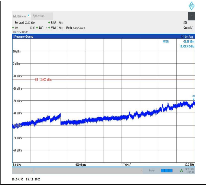
2-2-15MHz-10MHz-QPSK-QPSK-18851-18971-1RB#0-0RB# -3000~20000MHz-PASS
