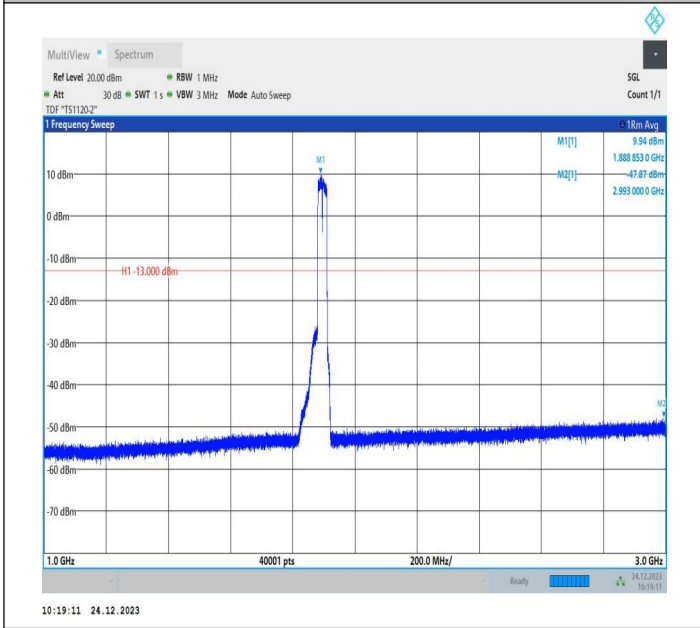
2-2-15MHz-15MHz-QPSK-QPSK-18975-19125-75RB#0-75RB #0-1000~3000MHz-PASS
