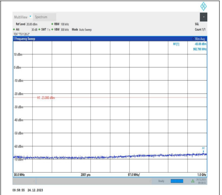
2-2-15MHz-10MHz-QPSK-QPSK-18675-18795-75RB#0-50RB #0-30~1000MHz-PASS
