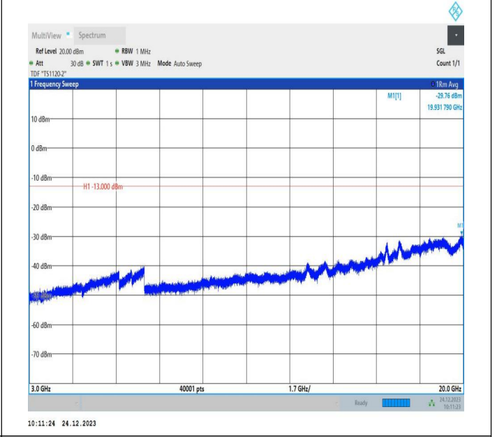
2-2-15MHz-15MHz-QPSK-QPSK-18675-18825-75RB#0-75RB #0-3000~20000MHz-PASS
