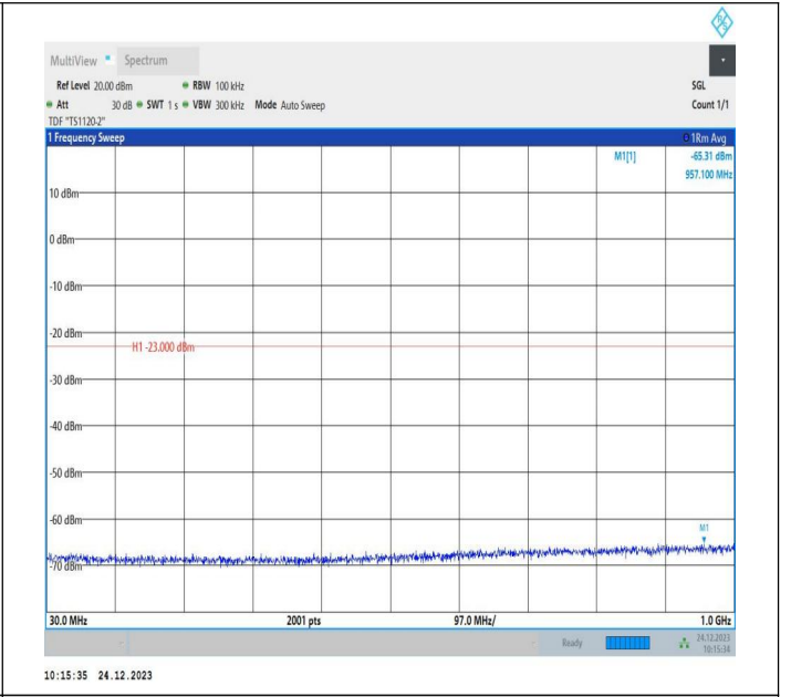
2-2-15MHz-15MHz-QPSK-QPSK-18825-18975-75RB#0-75RB #0-30~1000MHz-PASS
