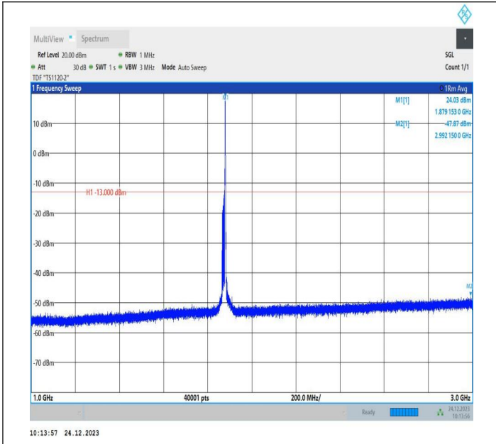
2-2-15MHz-15MHz-QPSK-QPSK-18825-18975-1RB#74-0RB# 0-1000~3000MHz-PASS
