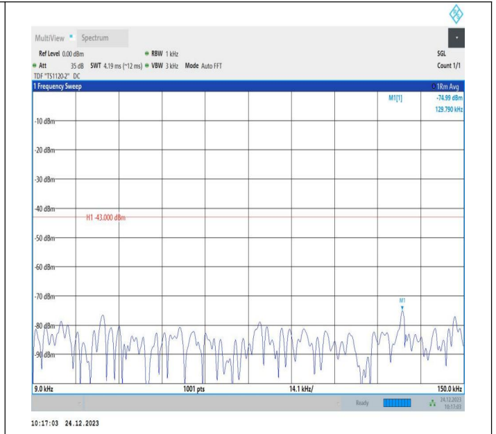
2-2-15MHz-15MHz-QPSK-QPSK-18975-19125-1RB#74-0RB#7 0-0.009~0.15MHz-PASS
