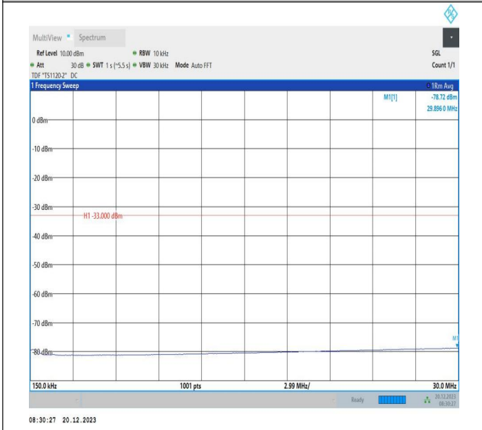
2-2-20MHz-10MHz-64QAM-64QAM-19001-19145-1RB#99-0R B#0-0.15~30MHz-PASS
