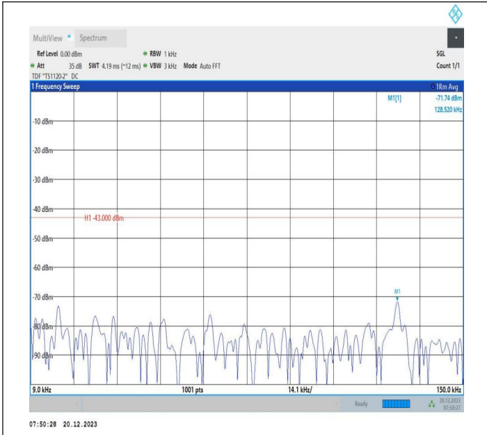
2-2-20MHz-10MHz-16QAM-16QAM-18851-18995-1RB#0-ORB #0-0.009~0.15MHz-PASS
