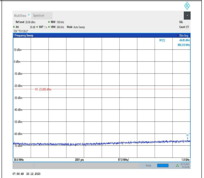
2-2-20MHz-10MHz-64QAM-64QAM-18851-18995-1RB#99-0R B#0-30~1000MHz-PASS
