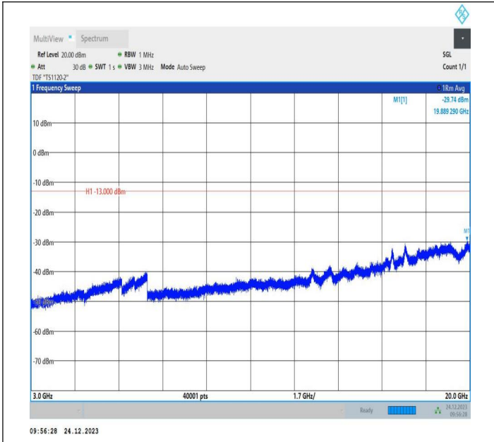
2-2-15MHz-10MHz-QPSK-QPSK-18675-18795-1RB#0-0RB# -3000~20000MHz-PASS
