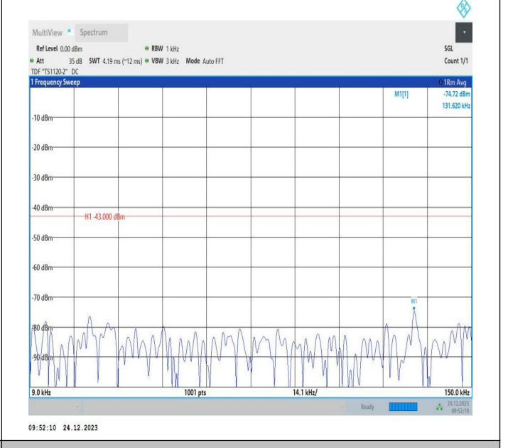
2-2-20MHz-10MHz-QPSK-QPSK-19001-19145-1RB#99-ORB# 0-0.009~0.15MHz-PASS
