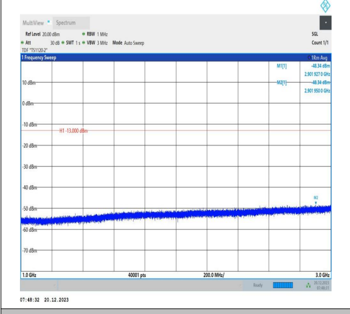
2-2-20MHz-10MHz-64QAM-64QAM-18700-18844-100RB#0-4 ORB#0-1000~3000MHz-PASS
