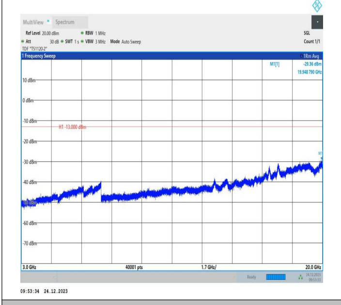
2-2-20MHz-10MHz-QPSK-QPSK-19001-19145-1RB#0-1RB#4 9-3000~20000MHz-PASS
