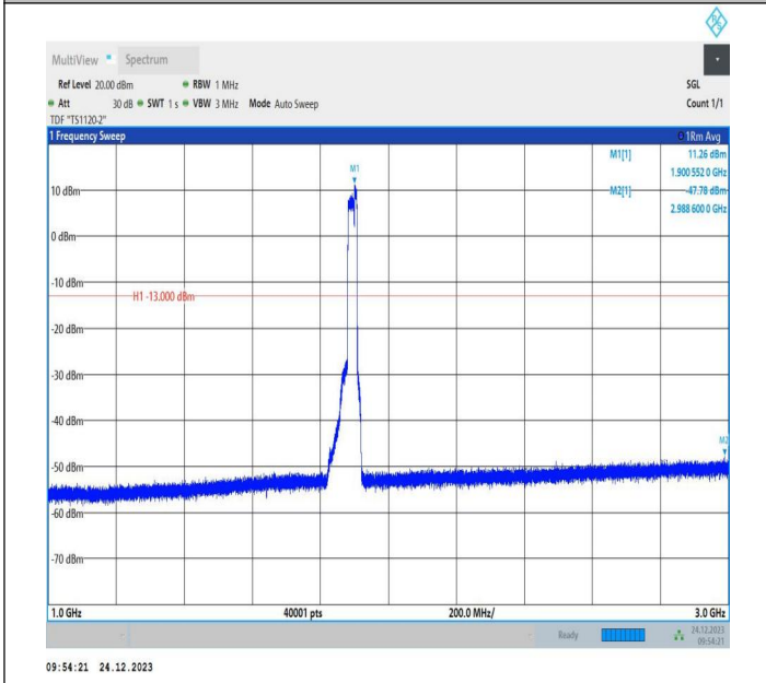
2-2-20MHz-10MHz-QPSK-QPSK-19001-19145-100RB#0-40R B#0-1000~3000MHz-PASS
