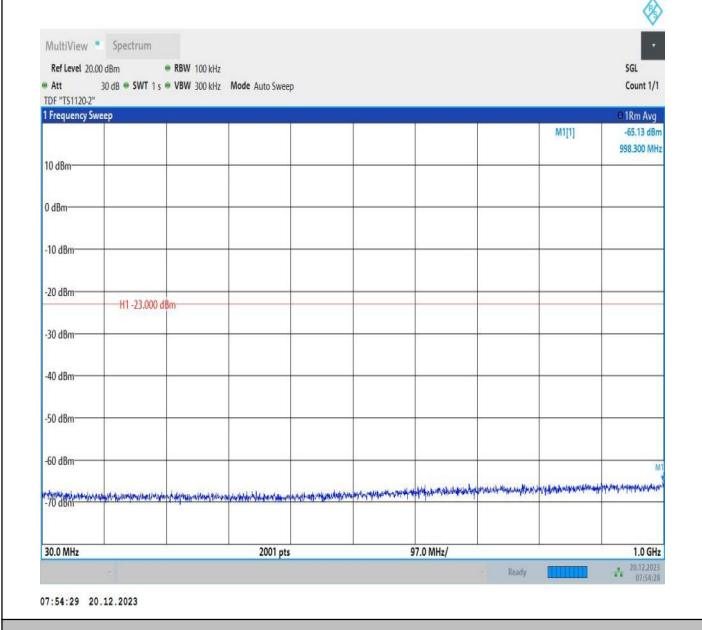
2-2-20MHz-10MHz-16QAM-16QAM-18851-18995-1RB#99-0R B#0-30~1000MHz-PASS
