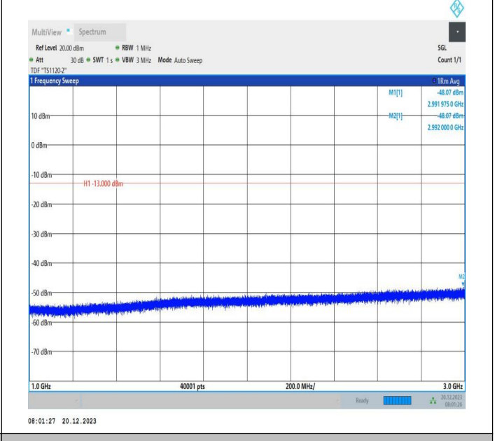
2-2-20MHz-10MHz-64QAM-64QAM-18851-18995-1RB#0-1RB #49-1000~3000MHz-PASS
