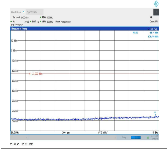
2-2-20MHz-10MHz-16QAM-16QAM-18851-18995-1RB#0-ORB #0-30~1000MHz-PASS
