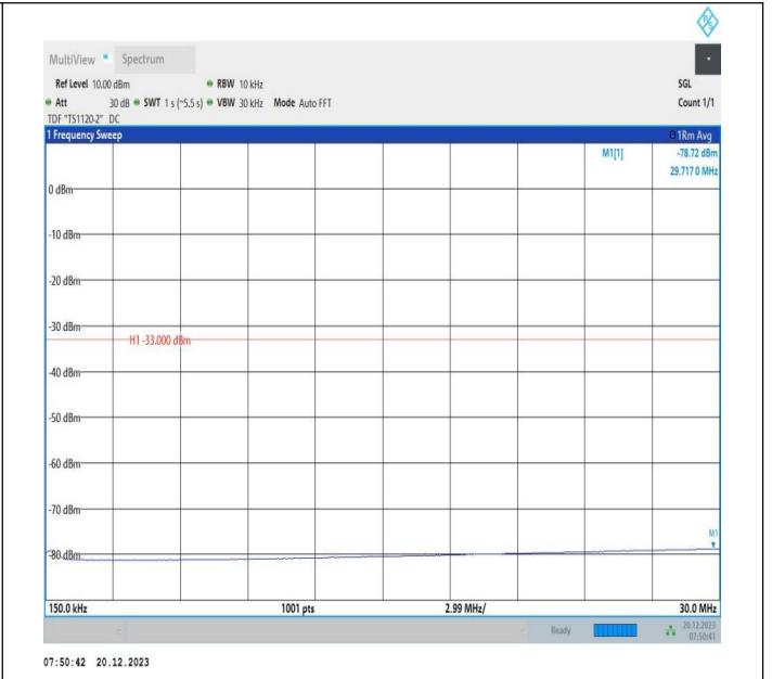
2-2-20MHz-10MHz-16QAM-16QAM-18851-18995-1RB#0-ORB #0-0.15~30MHz-PASS
