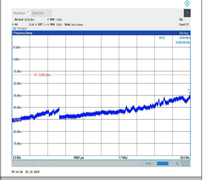
2-2-20MHz-10MHz-64QAM-64QAM-18851-18995-100RB#0-4 ORB#0-3000~20000MHz-PASS
