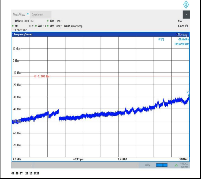
2-2-20MHz-10MHz-QPSK-QPSK-18851-18995-1RB#0-1RB#4 9-3000~20000MHz-PASS
