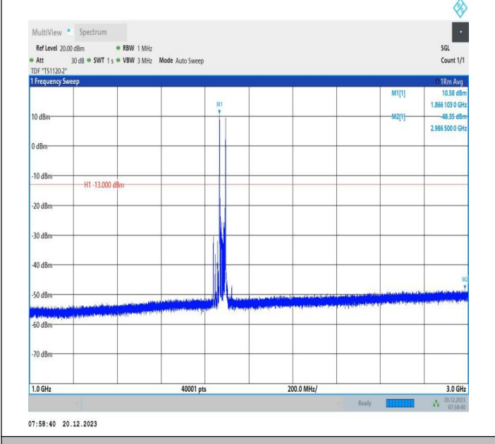
2-2-20MHz-10MHz-16QAM-16QAM-18851-18995-1RB#0-1RB #49-1000~3000MHz-PASS
