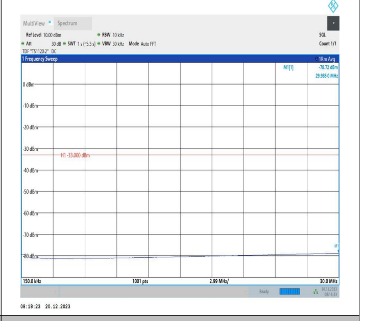
2-2-20MHz-10MHz-64QAM-64QAM-19001-19145-1RB#0-ORB #0-0.15~30MHz-PASS
