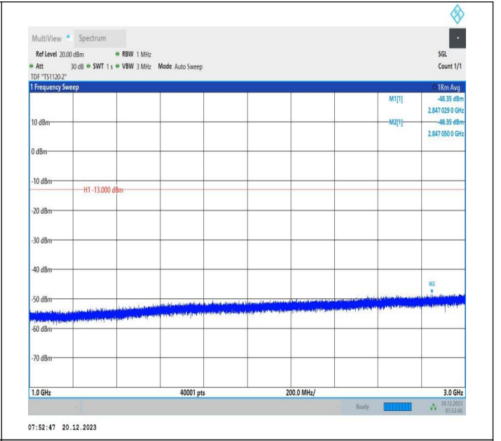
2-2-20MHz-10MHz-64QAM-64QAM-18851-18995-1RB#0-ORB #0-1000~3000MHz-PASS
