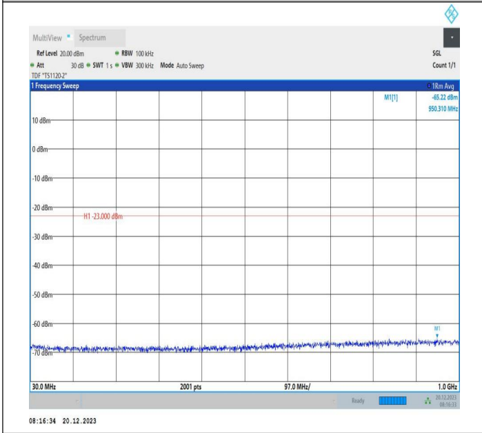
2-2-20MHz-10MHz-16QAM-16QAM-19001-19145-1RB#0-ORB #0-30~1000MHz-PASS
