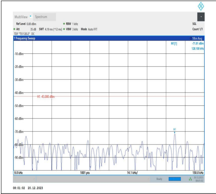
2-2-20MHz-10MHz-64QAM-64QAM-18851-18995-1RB#0-1RB #49-0.009~0.15MHz-PASS
