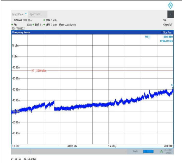
2-2-20MHz-10MHz-16QAM-16QAM-18851-18995-1RB#0-ORB #0-3000~20000MHz-PASS
