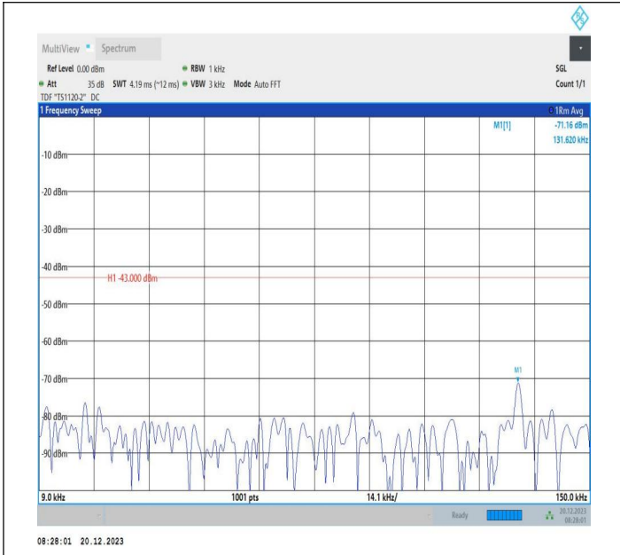
2-2-20MHz-10MHz-16QAM-16QAM-19001-19145-1RB#99-0R B#0-0.009~0.15MHz-PASS
