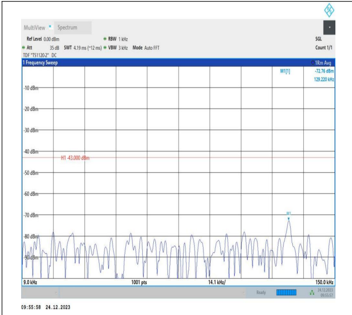
2-2-15MHz-10MHz-QPSK-QPSK-18675-18795-1RB#0-0RB#0 -0.009~0.15MHz-PASS
