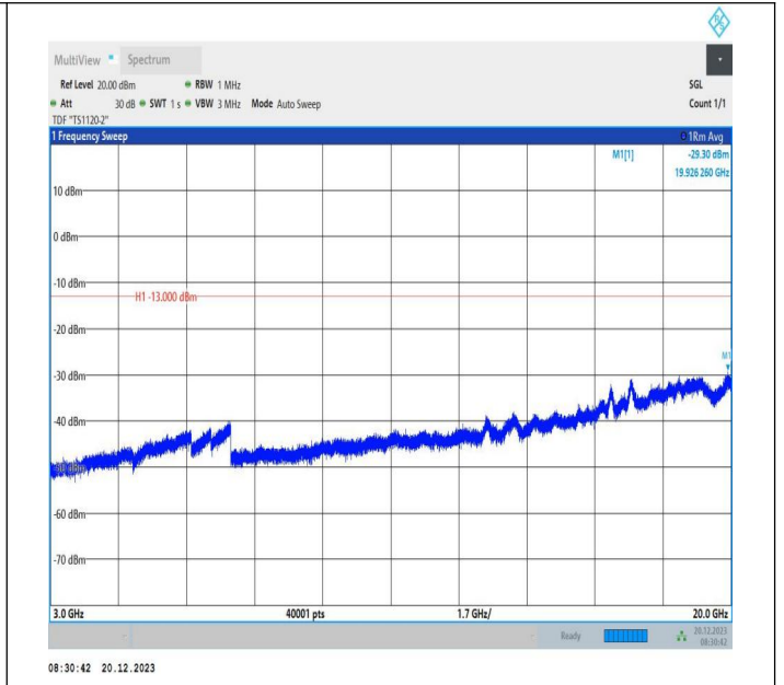
2-2-20MHz-10MHz-64QAM-64QAM-19001-19145-1RB#99-0R B#0-3000~20000MHz-PASS
