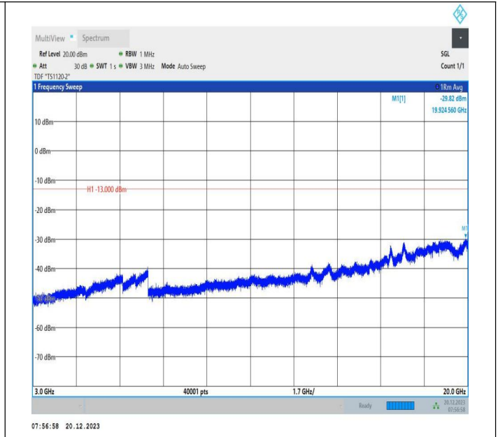
2-2-20MHz-10MHz-64QAM-64QAM-18851-18995-1RB#99-0R B#0-3000~20000MHz-PASS
