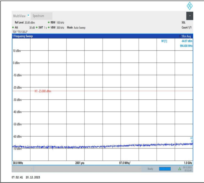
2-2-20MHz-10MHz-64QAM-64QAM-18851-18995-1RB#0-ORB #0-30~1000MHz-PASS
