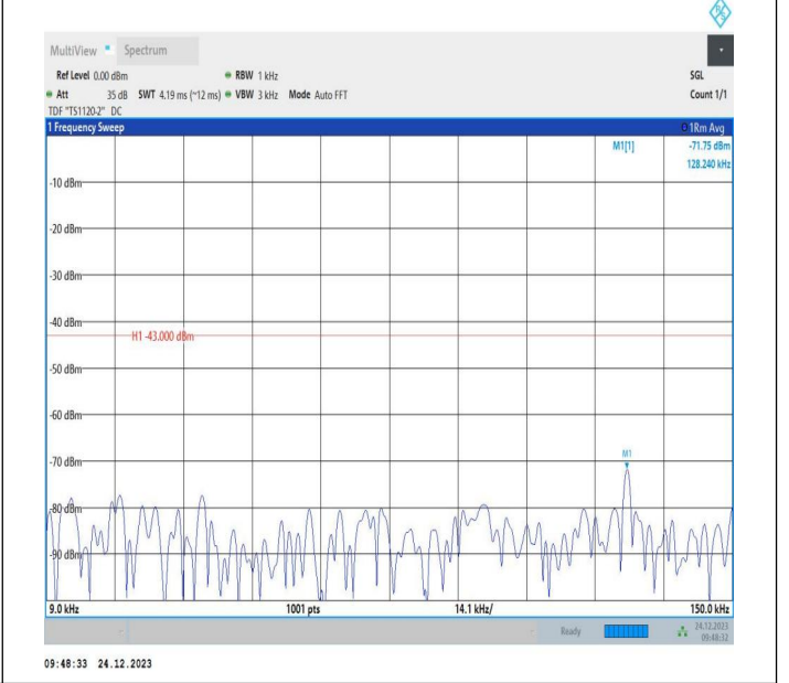
2-2-20MHz-10MHz-QPSK-QPSK-18851-18995-1RB#99-ORB# 0-0.009~0.15MHz-PASS
