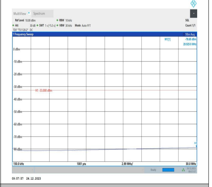
2-2-15MHz-10MHz-QPSK-QPSK-18675-18795-1RB#0-1RB# 9-0.15~30MHz-PASS
