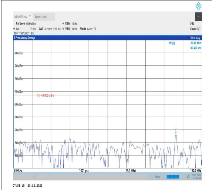
2-2-20MHz-10MHz-16QAM-16QAM-18851-18995-1RB#0-1RB #49-0.009~0.15MHz-PASS
