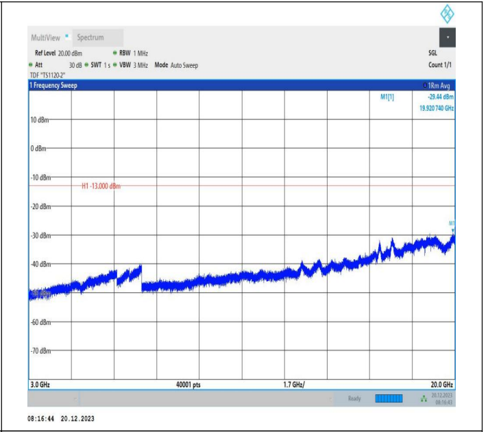
2-2-20MHz-10MHz-16QAM-16QAM-19001-19145-1RB#0-ORB #0-3000~20000MHz-PASS
