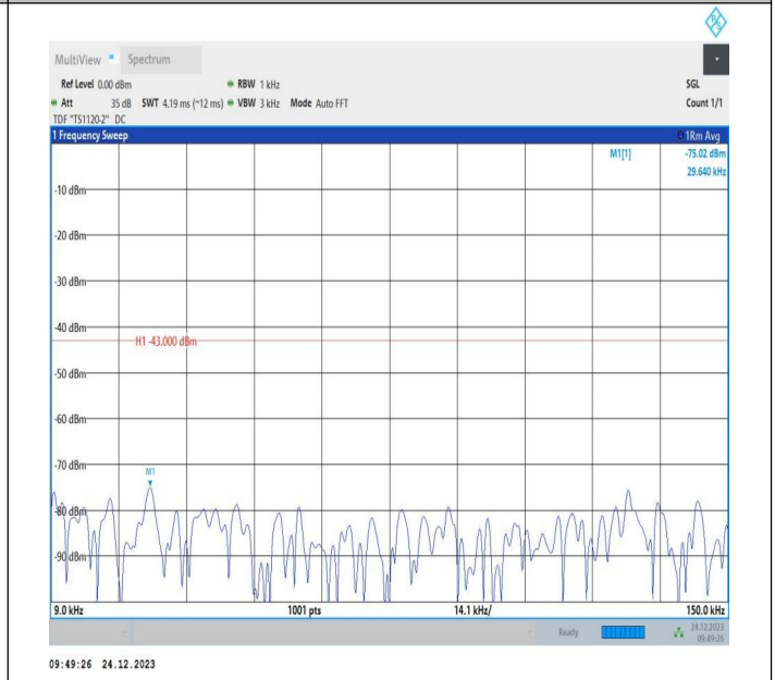
2-2-20MHz-10MHz-QPSK-QPSK-18851-18995-1RB#0-1RB#4 9-0.009~0.15MHz-PASS
