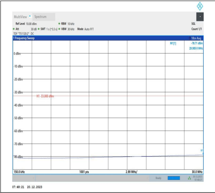
2-2-20MHz-10MHz-64QAM-64QAM-18700-18844-100RB#0-4 ORB#0-0.15~30MHz-PASS
