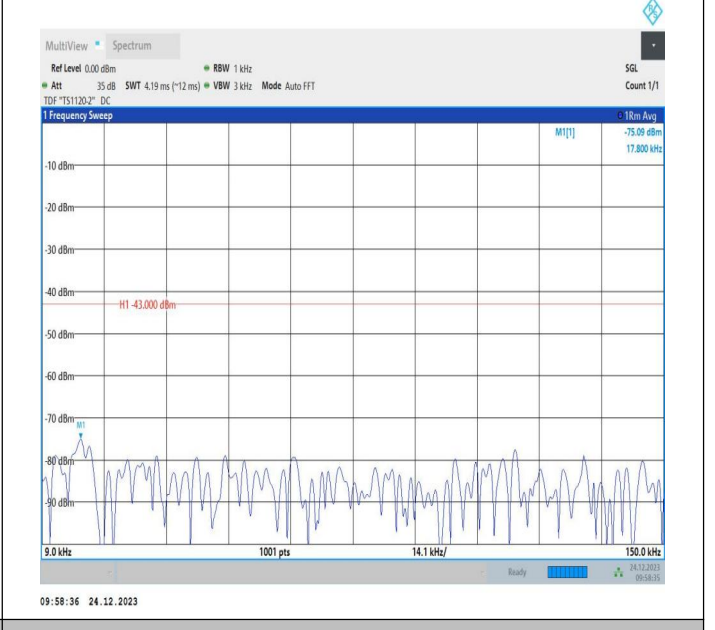
2-2-15MHz-10MHz-QPSK-QPSK-18675-18795-75RB#0-50RB #0-0.009~0.15MHz-PASS
