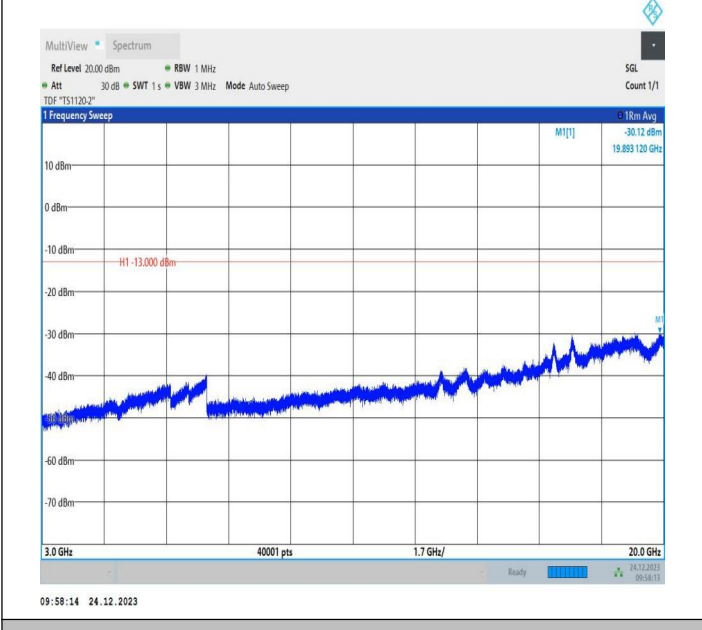
2-2-15MHz-10MHz-QPSK-QPSK-18675-18795-1RB#0-1RB#4 9-3000~20000MHz-PASS
