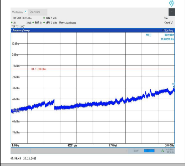
2-2-20MHz-10MHz-16QAM-16QAM-18851-18995-1RB#0-1RB #49-3000~20000MHz-PASS
