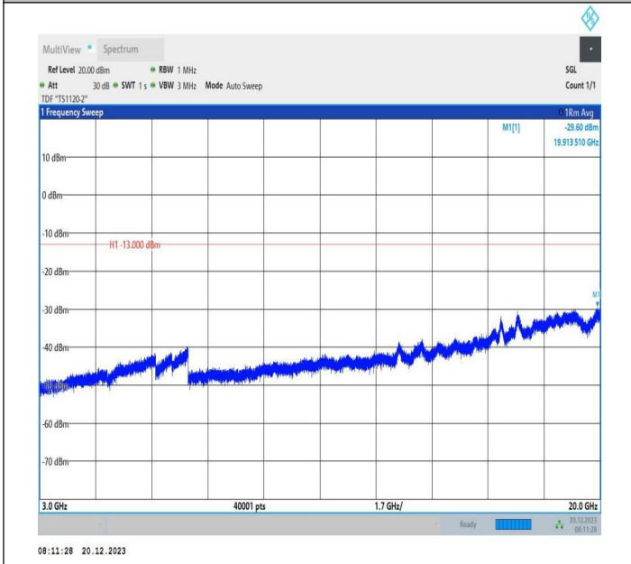
2-2-20MHz-10MHz-16QAM-16QAM-18851-18995-100RB#0-4 ORB#0-3000~20000MHz-PASS
