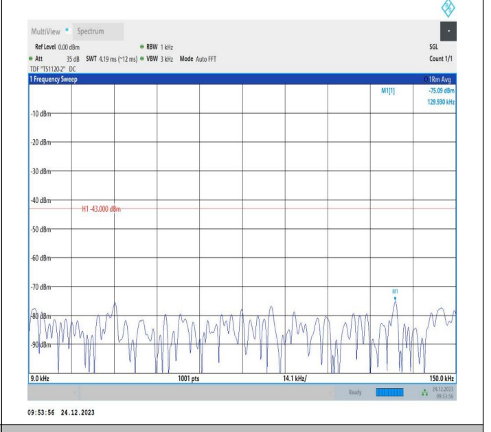
2-2-20MHz-10MHz-QPSK-QPSK-19001-19145-100RB#0-40R B#0-0.009~0.15MHz-PASS
