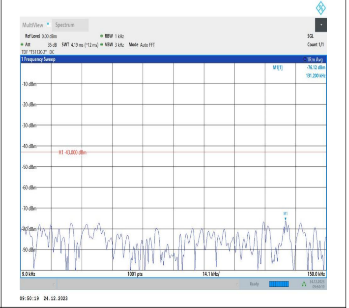
2-2-20MHz-10MHz-QPSK-QPSK-18851-18995-100RB#0-40R B#0-0.009~0.15MHz-PASS
