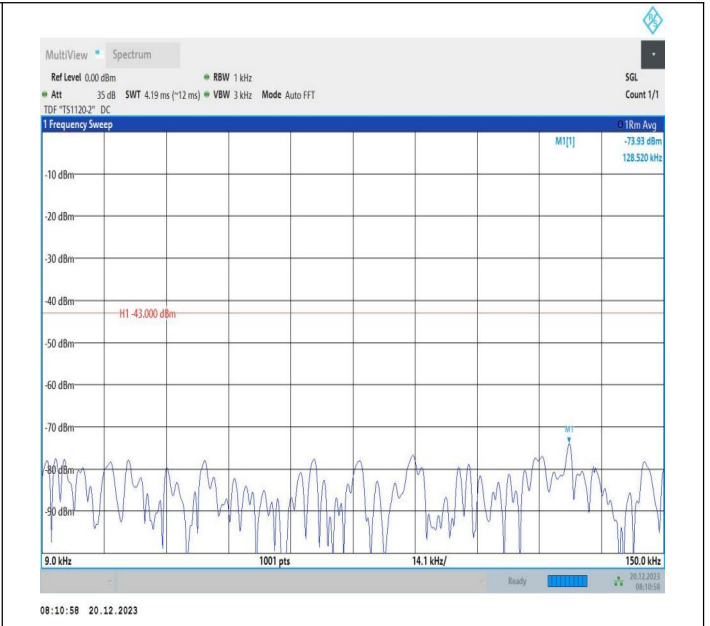
2-2-20MHz-10MHz-16QAM-16QAM-18851-18995-100RB#0-4 ORB#0-0.009~0.15MHz-PASS
