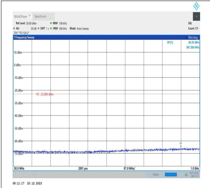
2-2-20MHz-10MHz-16QAM-16QAM-18851-18995-100RB#0-4 ORB#0-30~1000MHz-PASS
