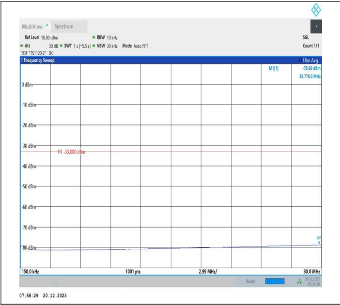
2-2-20MHz-10MHz-16QAM-16QAM-18851-18995-1RB#0-1RB #49-0.15~30MHz-PASS
