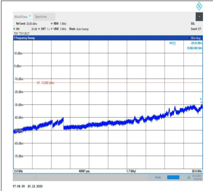
2-2-20MHz-10MHz-16QAM-16QAM-18851-18995-1RB#99-0R B#0-3000~20000MHz-PASS
