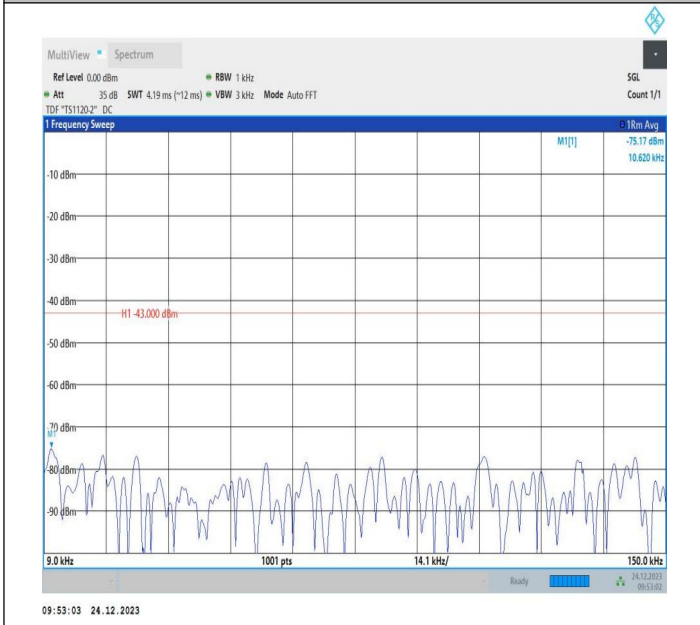
2-2-20MHz-10MHz-QPSK-QPSK-19001-19145-1RB#0-1RB#4 9-0.009~0.15MHz-PASS
