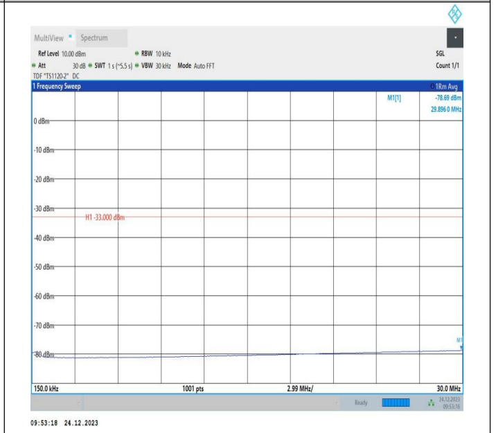
2-2-20MHz-10MHz-QPSK-QPSK-19001-19145-1RB#0-1RB#4 9-0.15~30MHz-PASS
