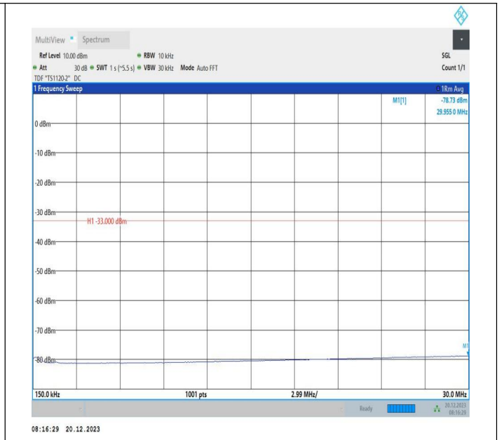
2-2-20MHz-10MHz-16QAM-16QAM-19001-19145-1RB#0-ORB #0-0.15~30MHz-PASS
