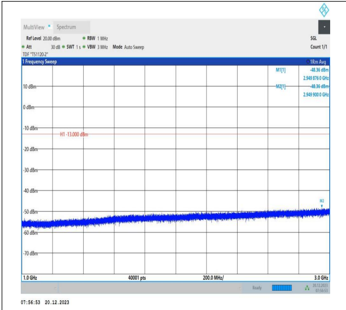
2-2-20MHz-10MHz-64QAM-64QAM-18851-18995-1RB#99-0R B#0-1000~3000MHz-PASS
