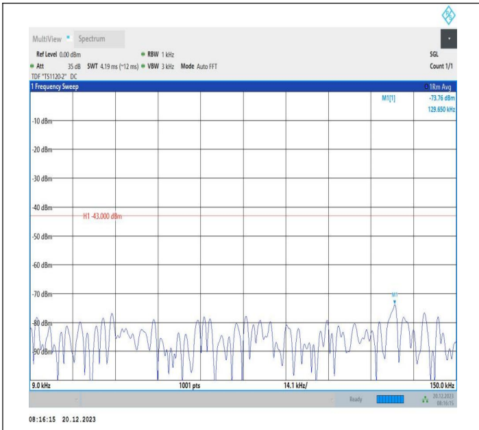
2-2-20MHz-10MHz-16QAM-16QAM-19001-19145-1RB#0-ORB #0-0.009~0.15MHz-PASS
