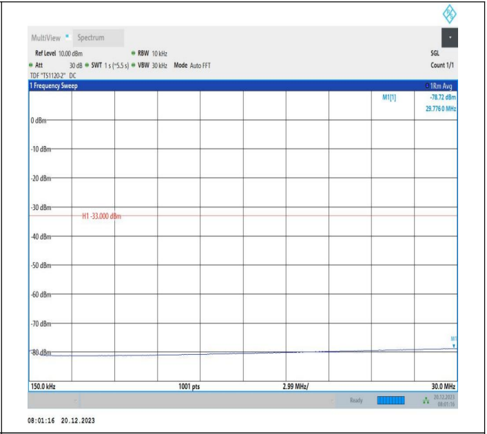
2-2-20MHz-10MHz-64QAM-64QAM-18851-18995-1RB#0-1RB #49-0.15~30MHz-PASS
