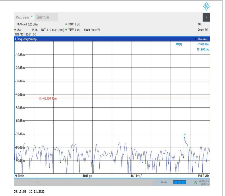
2-2-20MHz-10MHz-64QAM-64QAM-18851-18995-100RB#0-4 ORB#0-0.009~0.15MHz-PASS
