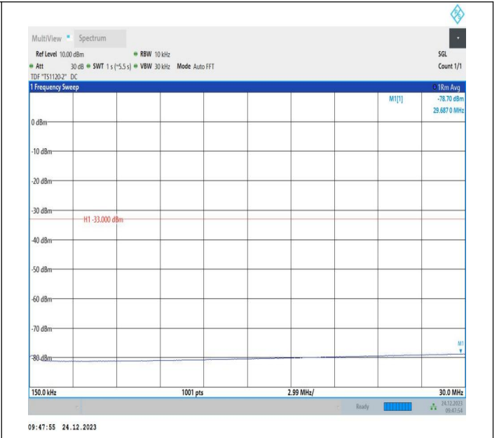
2-2-20MHz-10MHz-QPSK-QPSK-18851-18995-1RB#0-0RB#0 -0.15~30MHz-PASS
