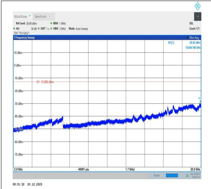
2-2-20MHz-10MHz-64QAM-64QAM-18851-18995-1RB#0-1RB #49-3000~20000MHz-PASS
