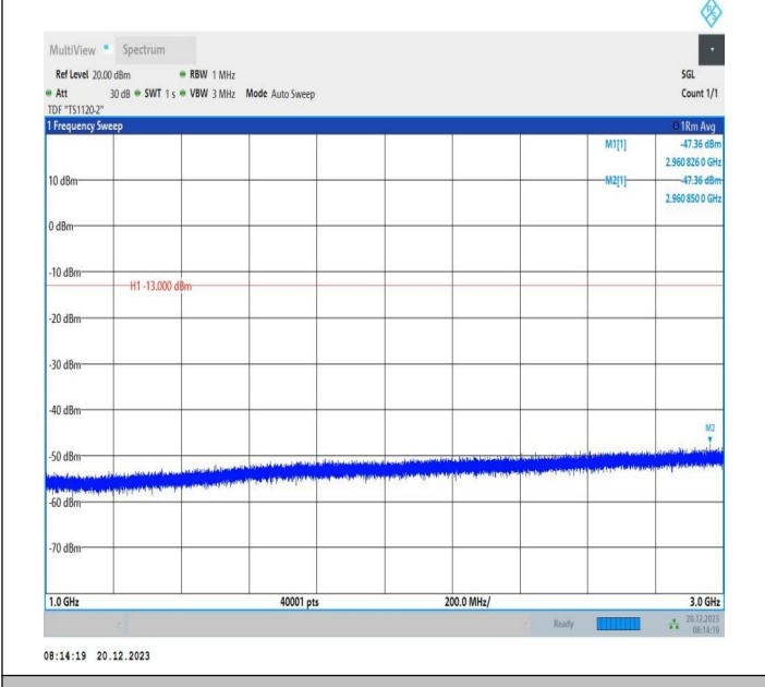
2-2-20MHz-10MHz-64QAM-64QAM-18851-18995-100RB#0-4 ORB#0-1000~3000MHz-PASS
