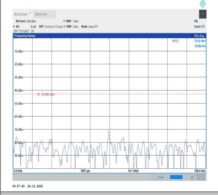
2-2-15MHz-10MHz-QPSK-QPSK-18675-18795-1RB#0-1RB# 9-0.009~0.15MHz-PASS
