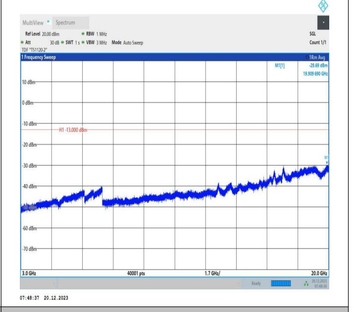
2-2-20MHz-10MHz-64QAM-64QAM-18700-18844-100RB#0-4 ORB#0-3000~20000MHz-PASS
