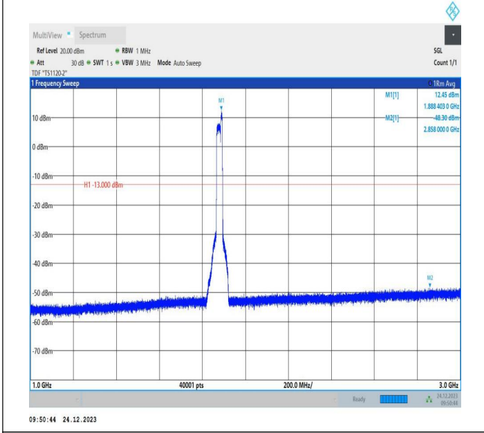
2-2-20MHz-10MHz-QPSK-QPSK-18851-18995-100RB#0-40R B#0-1000~3000MHz-PASS
