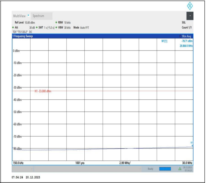
2-2-20MHz-10MHz-16QAM-16QAM-18851-18995-1RB#99-0R B#0-0.15~30MHz-PASS
