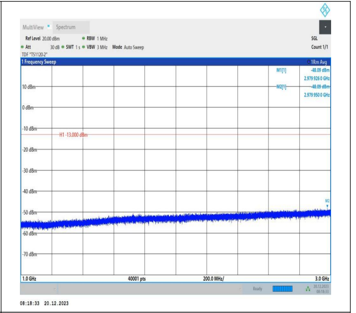
2-2-20MHz-10MHz-64QAM-64QAM-19001-19145-1RB#0-ORB #0-1000~3000MHz-PASS
