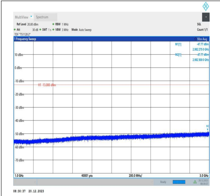
2-2-20MHz-10MHz-64QAM-64QAM-19001-19145-1RB#99-0R B#0-1000~3000MHz-PASS
