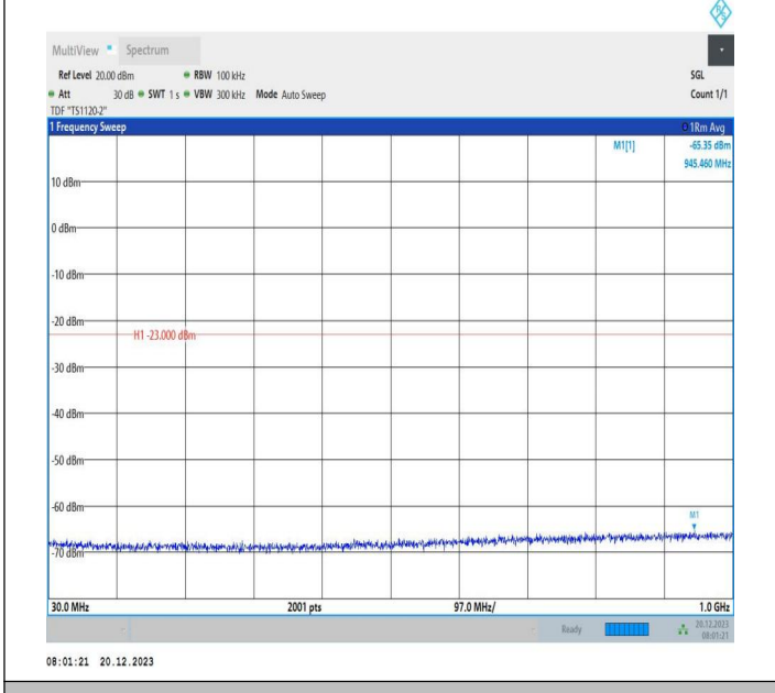
2-2-20MHz-10MHz-64QAM-64QAM-18851-18995-1RB#0-1RB #49-30~1000MHz-PASS
