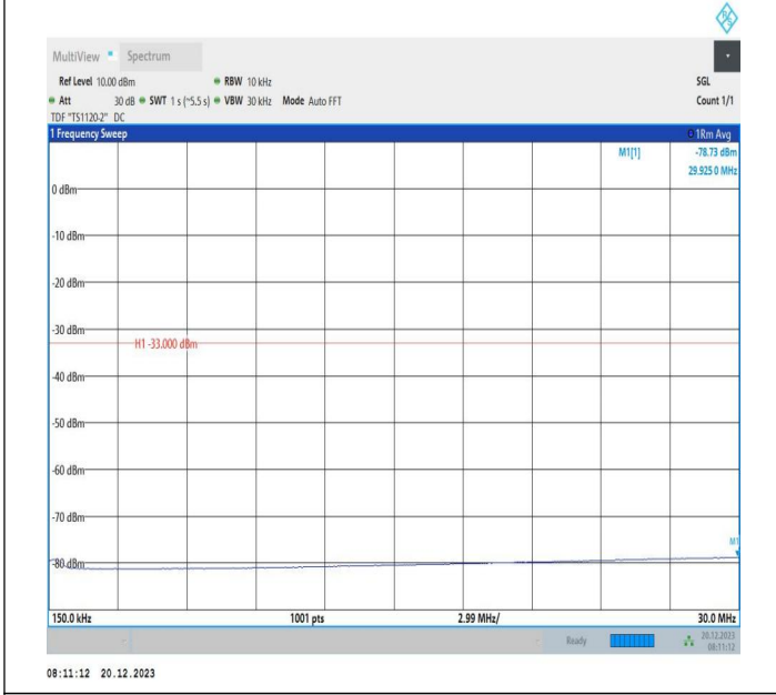
2-2-20MHz-10MHz-16QAM-16QAM-18851-18995-100RB#0-4 ORB#0-0.15~30MHz-PASS
