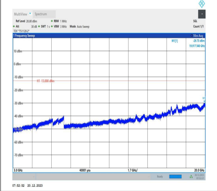
2-2-20MHz-10MHz-64QAM-64QAM-18851-18995-1RB#0-ORB #0-3000~20000MHz-PASS
