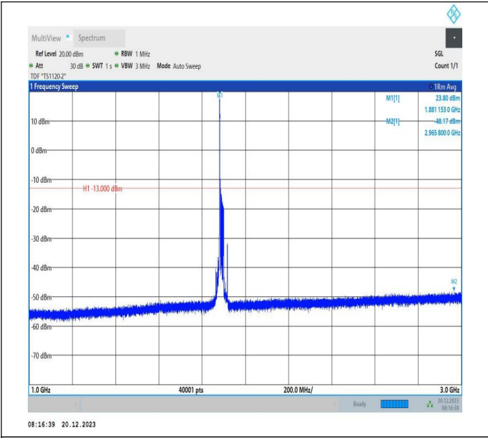
2-2-20MHz-10MHz-16QAM-16QAM-19001-19145-1RB#0-ORB #0-1000~3000MHz-PASS
