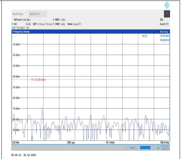
2-2-20MHz-10MHz-64QAM-64QAM-19001-19145-1RB#99-0R B#0-0.009~0.15MHz-PASS
