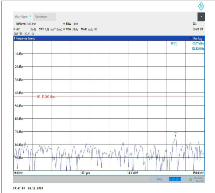
2-2-20MHz-10MHz-QPSK-QPSK-18851-18995-1RB#0-0RB#0 -0.009~0.15MHz-PASS
