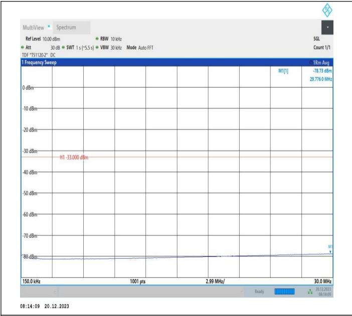
2-2-20MHz-10MHz-64QAM-64QAM-18851-18995-100RB#0-4 ORB#0-0.15~30MHz-PASS
