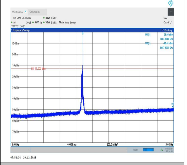
2-2-20MHz-10MHz-16QAM-16QAM-18851-18995-1RB#99-0R B#0-1000~3000MHz-PASS
