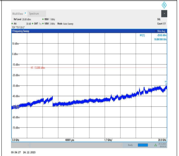
2-2-20MHz-10MHz-QPSK-QPSK-19001-19145-100RB#0-40R B#0-3000~20000MHz-PASS
