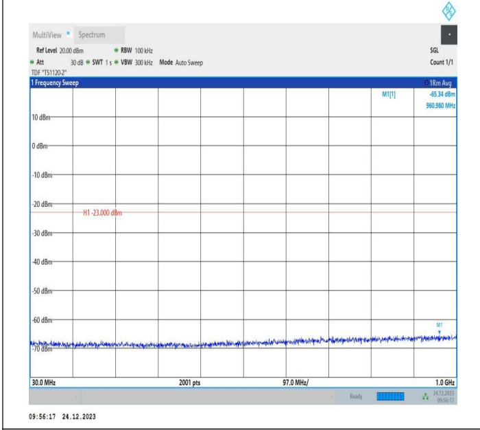
2-2-15MHz-10MHz-QPSK-QPSK-18675-18795-1RB#0-0RB#0 -30~1000MHz-PASS
