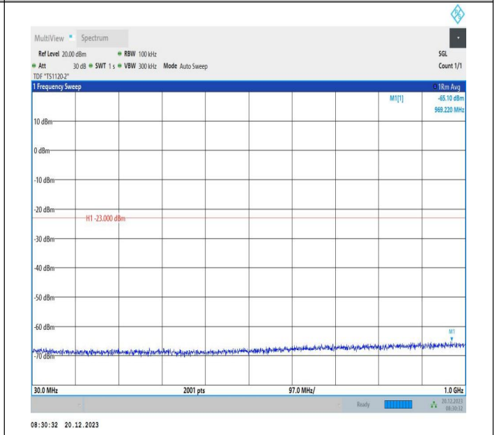
2-2-20MHz-10MHz-64QAM-64QAM-19001-19145-1RB#99-0R B#0-30~1000MHz-PASS
