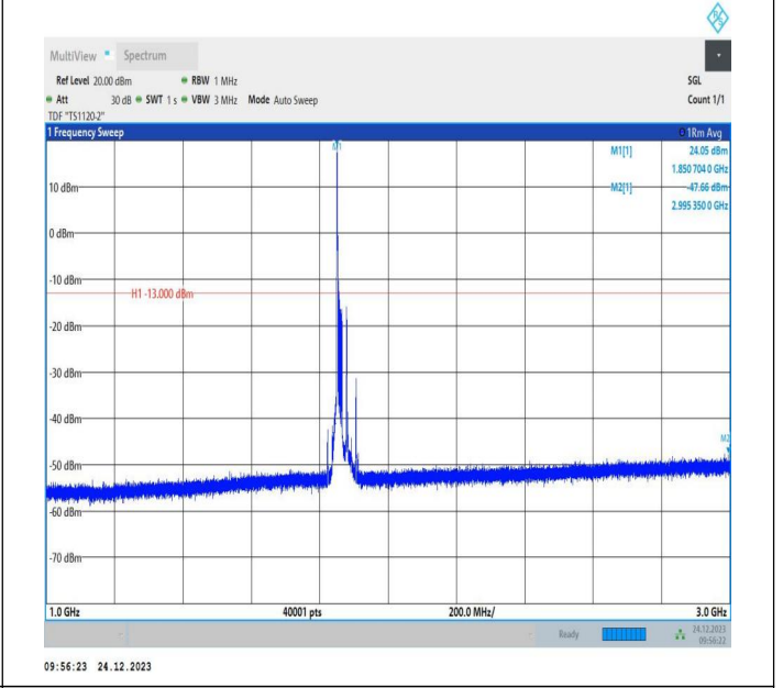
2-2-15MHz-10MHz-QPSK-QPSK-18675-18795-1RB#0-0RB#0 -1000~3000MHz-PASS
