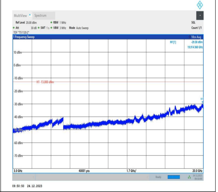
2-2-20MHz-10MHz-QPSK-QPSK-18851-18995-100RB#0-40R B#0-3000~20000MHz-PASS
