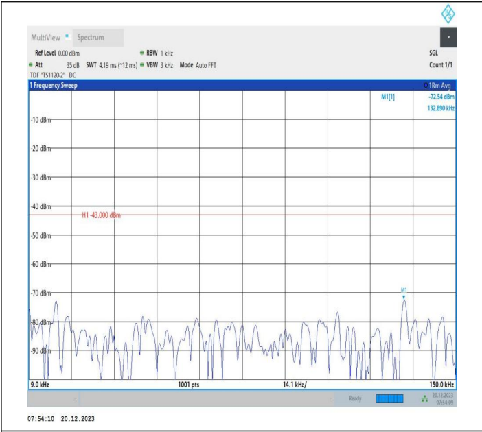
2-2-20MHz-10MHz-16QAM-16QAM-18851-18995-1RB#99-0R B#0-0.009~0.15MHz-PASS
