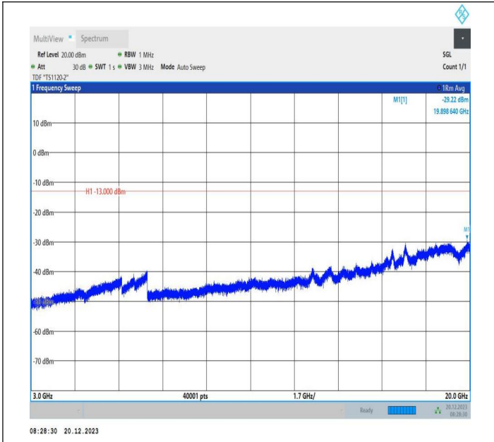
2-2-20MHz-10MHz-16QAM-16QAM-19001-19145-1RB#99-0R B#0-3000~20000MHz-PASS
