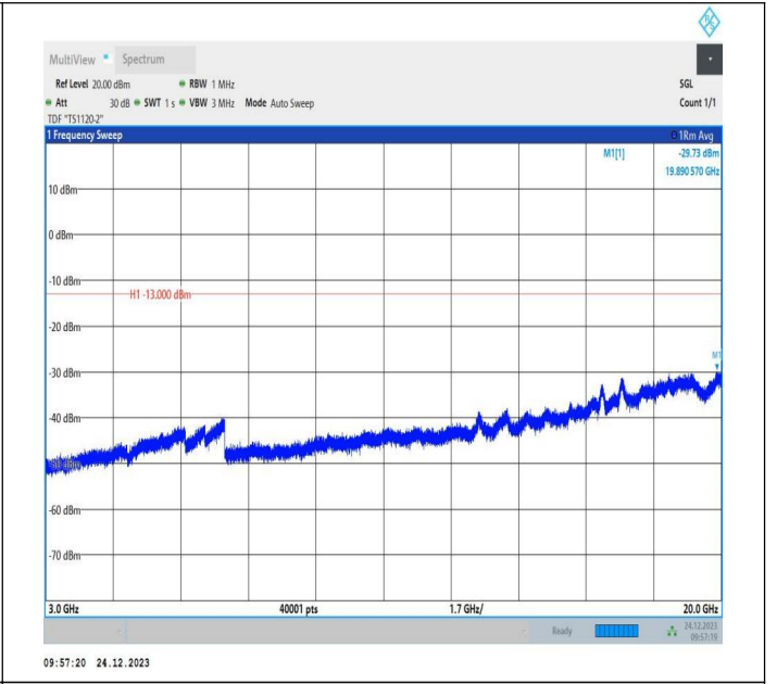
2-2-15MHz-10MHz-QPSK-QPSK-18675-18795-1RB#74-0RB# 0-3000~20000MHz-PASS
