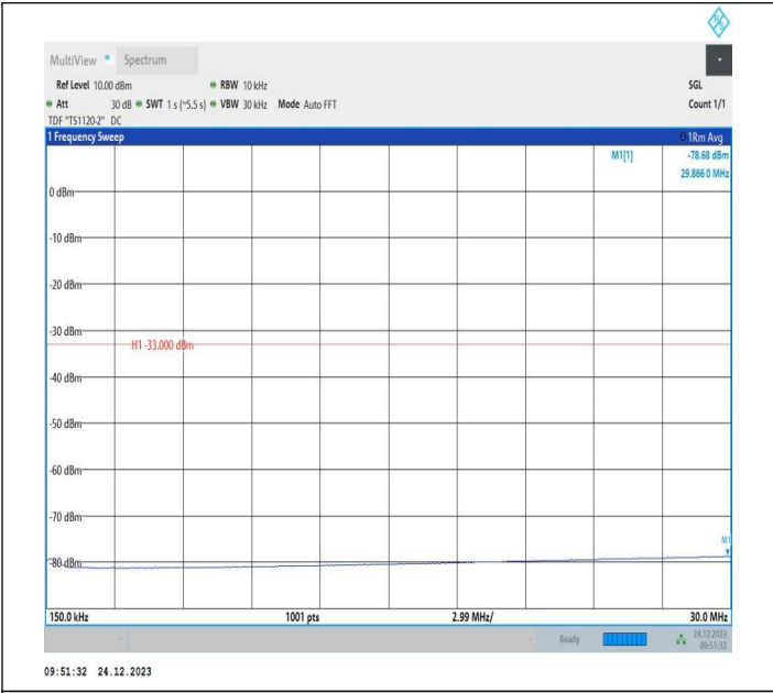
2-2-20MHz-10MHz-QPSK-QPSK-19001-19145-1RB#0-0RB#0 -0.15~30MHz-PASS
