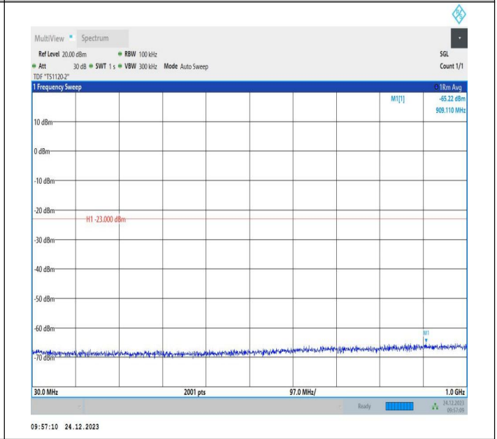
2-2-15MHz-10MHz-QPSK-QPSK-18675-18795-1RB#74-0RB# 0-30~1000MHz-PASS
