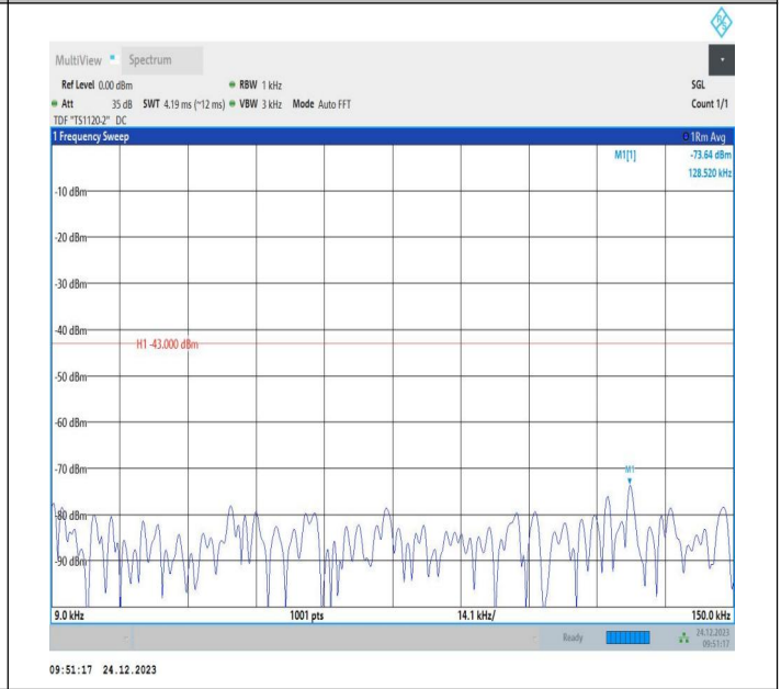
2-2-20MHz-10MHz-QPSK-QPSK-19001-19145-1RB#0-ORB#0 -0.009~0.15MHz-PASS
