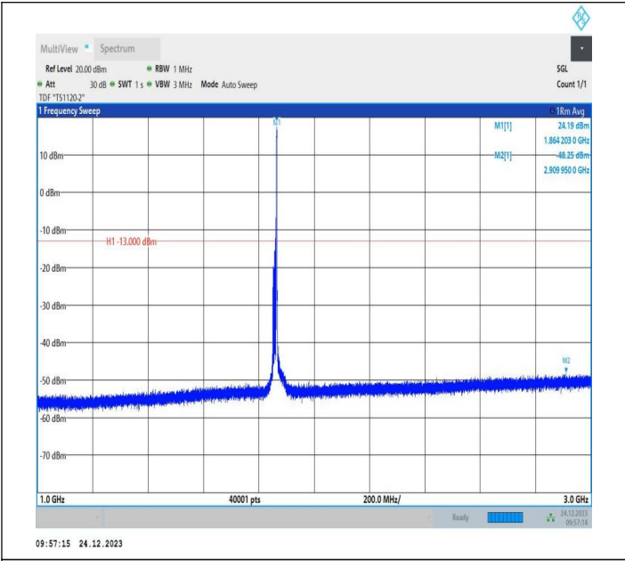
2-2-15MHz-10MHz-QPSK-QPSK-18675-18795-1RB#74-0RB# 0-1000~3000MHz-PASS
