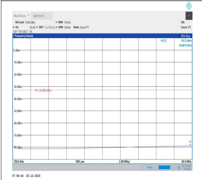
2-2-20MHz-10MHz-64QAM-64QAM-18851-18995-1RB#99-0R B#0-0.15~30MHz-PASS
