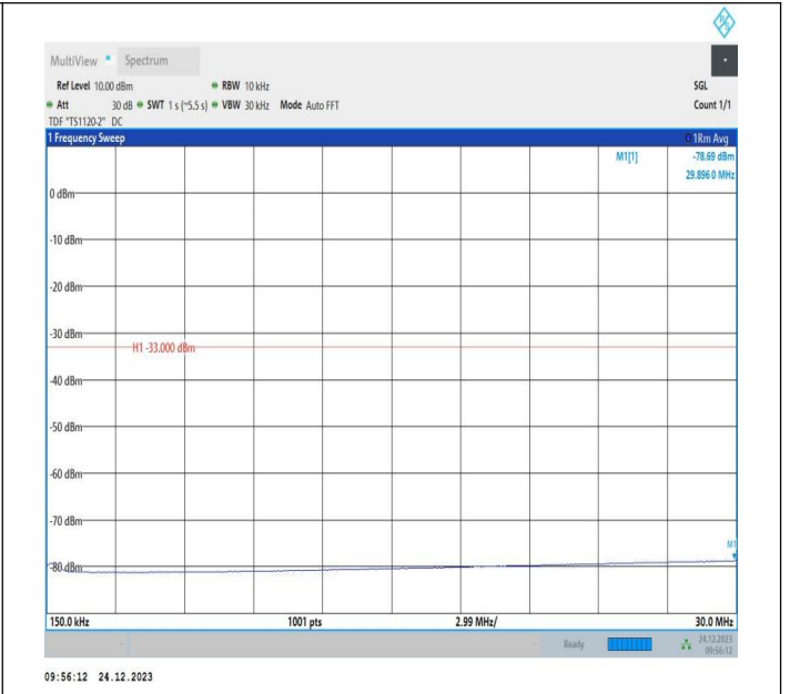
2-2-15MHz-10MHz-QPSK-QPSK-18675-18795-1RB#0-0RB#0 -0.15~30MHz-PASS
