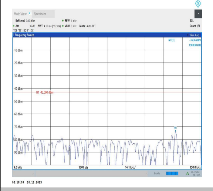
2-2-20MHz-10MHz-64QAM-64QAM-19001-19145-1RB#0-ORB #0-0.009~0.15MHz-PASS
