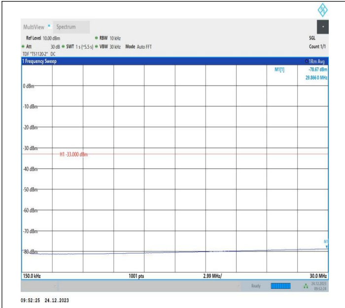
2-2-20MHz-10MHz-QPSK-QPSK-19001-19145-1RB#99-0RB# 0-0.15~30MHz-PASS
