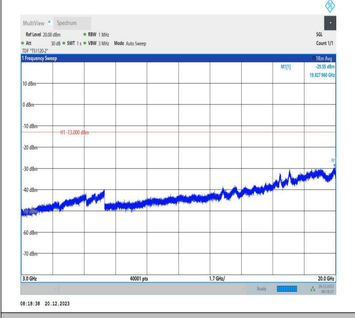
2-2-20MHz-10MHz-64QAM-64QAM-19001-19145-1RB#0-ORB #0-3000~20000MHz-PASS
