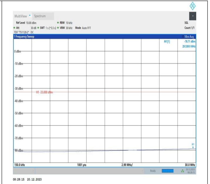
2-2-20MHz-10MHz-16QAM-16QAM-19001-19145-1RB#99-0R B#0-0.15~30MHz-PASS
