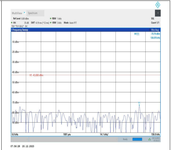
2-2-20MHz-10MHz-64QAM-64QAM-18851-18995-1RB#99-0R B#0-0.009~0.15MHz-PASS
