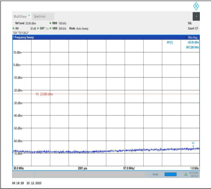
2-2-20MHz-10MHz-64QAM-64QAM-19001-19145-1RB#0-ORB #0-30~1000MHz-PASS
