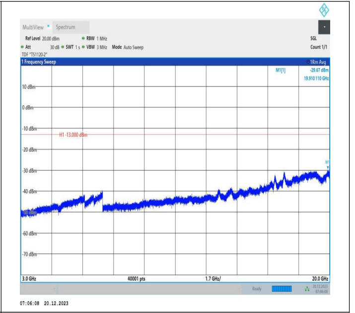
2-2-10MHz-20MHz-64QAM-64QAM-18956-19100-1RB#49-0R B#0-3000~20000MHz-PASS
