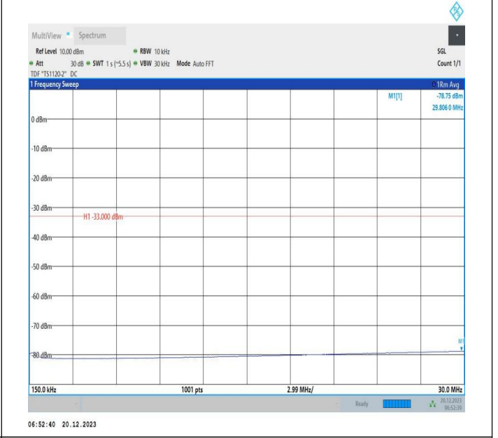
2-2-10MHz-20MHz-64QAM-64QAM-18956-19100-1RB#0-ORB #0-0.15~30MHz-PASS
