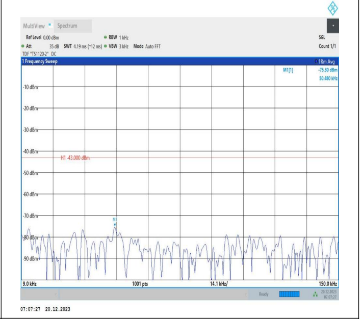
2-2-10MHz-20MHz-16QAM-16QAM-18956-19100-1RB#0-1RB #99-0.009~0.15MHz-PASS
