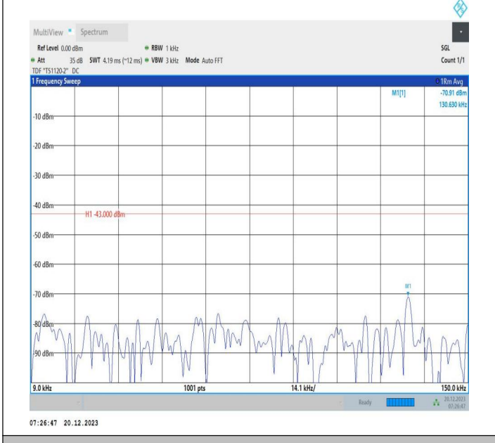
2-2-20MHz-10MHz-64QAM-64QAM-18700-18844-1RB#0-ORB #0-0.009~0.15MHz-PASS
