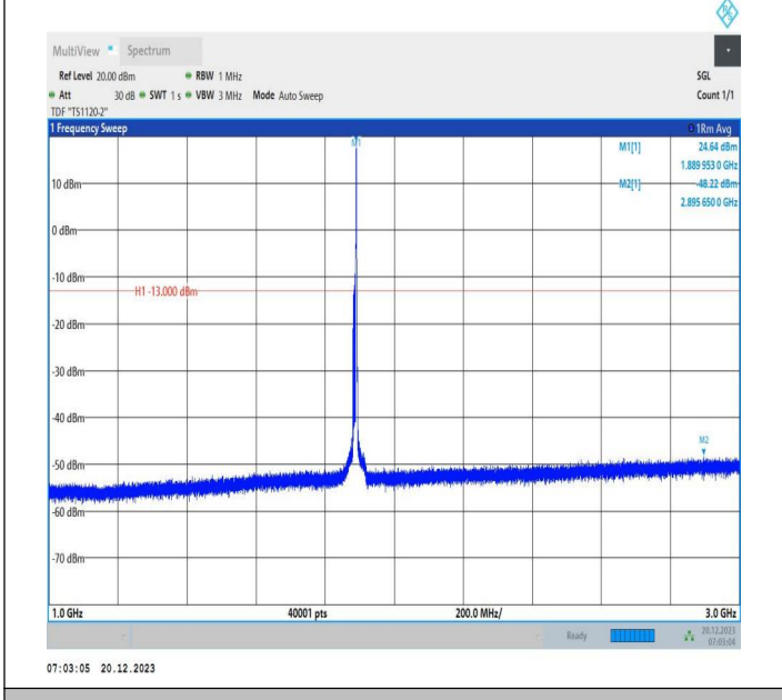
2-2-10MHz-20MHz-QPSK-QPSK-18956-19100-1RB#49-0RB# 0-1000~3000MHz-PASS
