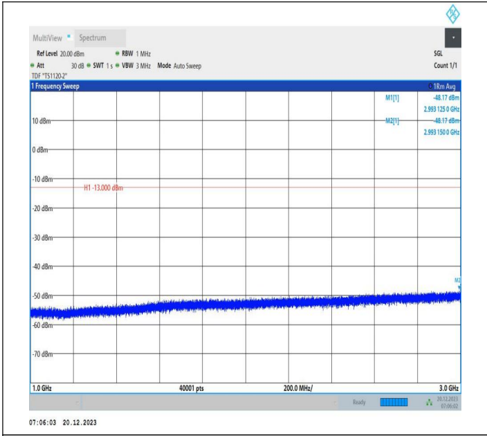
2-2-10MHz-20MHz-64QAM-64QAM-18956-19100-1RB#49-0R B#0-1000~3000MHz-PASS
