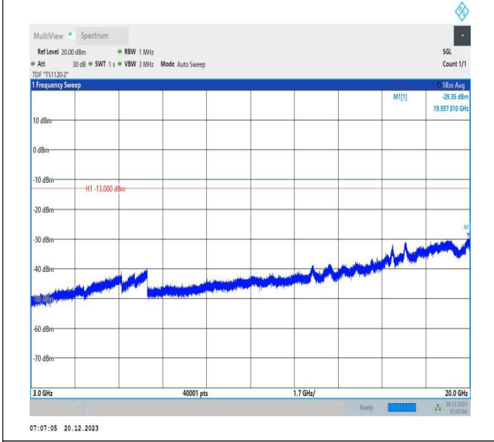
2-2-10MHz-20MHz-QPSK-QPSK-18956-19100-1RB#0-1RB#9 9-3000~20000MHz-PASS
