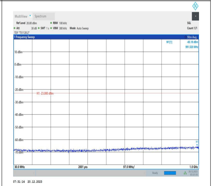
2-2-20MHz-10MHz-64QAM-64QAM-18700-18844-1RB#99-0R B#0-30~1000MHz-PASS
