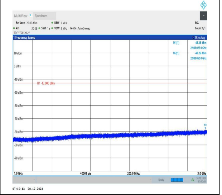
2-2-10MHz-20MHz-64QAM-64QAM-18956-19100-1RB#0-1RB #99-1000~3000MHz-PASS
