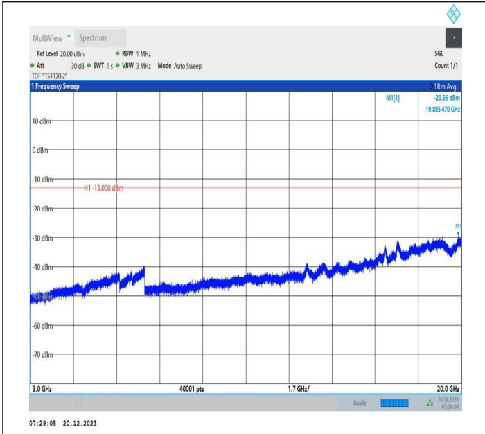
2-2-20MHz-10MHz-16QAM-16QAM-18700-18844-1RB#99-0R B#0-3000~20000MHz-PASS
