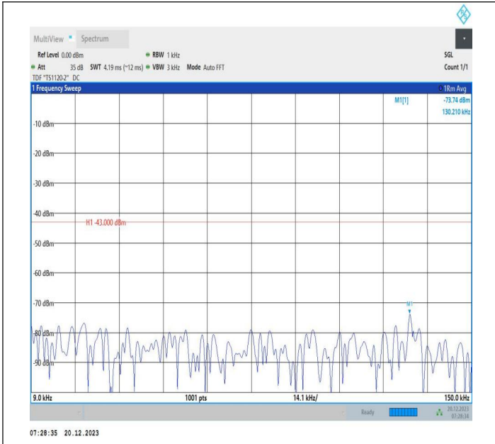
2-2-20MHz-10MHz-16QAM-16QAM-18700-18844-1RB#99-0R B#0-0.009~0.15MHz-PASS
