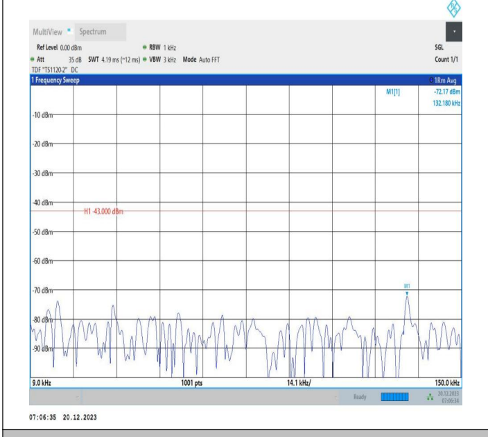
2-2-10MHz-20MHz-QPSK-QPSK-18956-19100-1RB#0-1RB#9 9-0.009~0.15MHz-PASS
