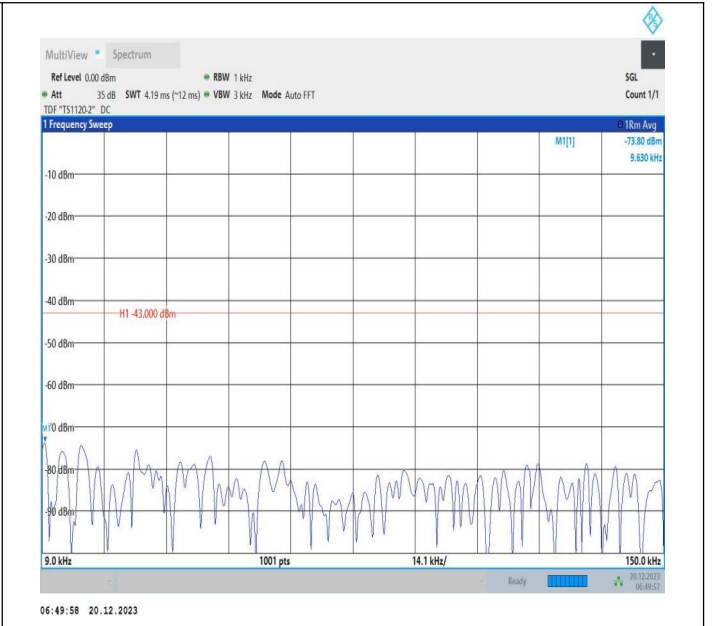
2-2-10MHz-20MHz-16QAM-16QAM-18956-19100-1RB#0-0RB #0-0.009~0.15MHz-PASS
