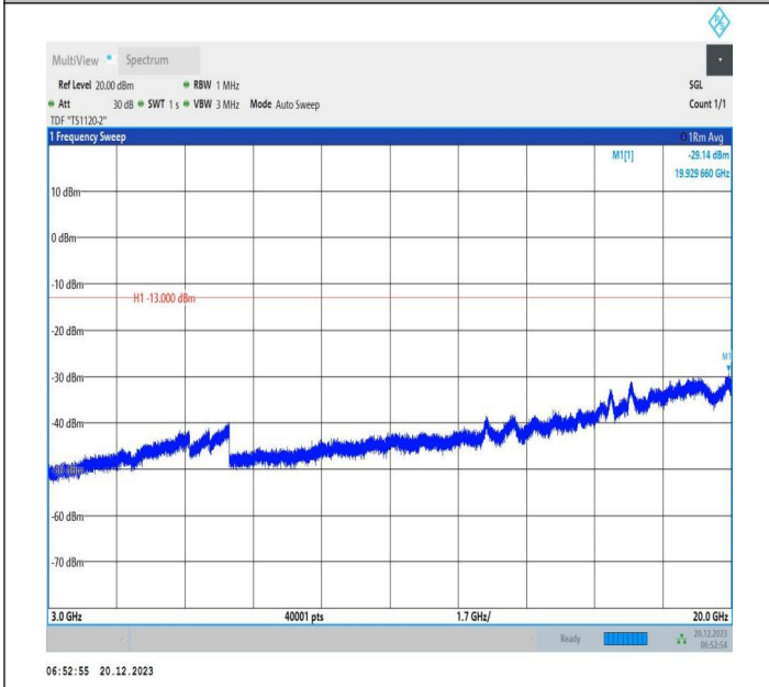
2-2-10MHz-20MHz-64QAM-64QAM-18956-19100-1RB#0-ORB #0-3000~20000MHz-PASS
