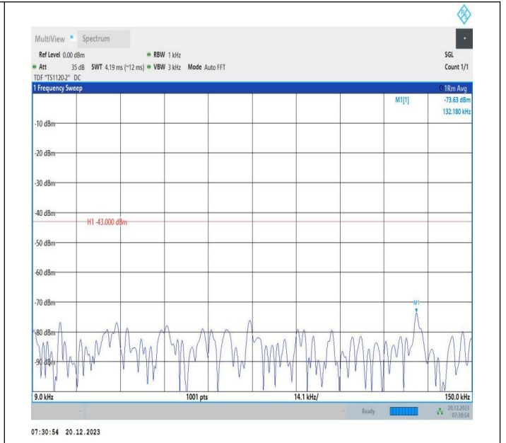
2-2-20MHz-10MHz-64QAM-64QAM-18700-18844-1RB#99-0R B#0-0.009~0.15MHz-PASS
