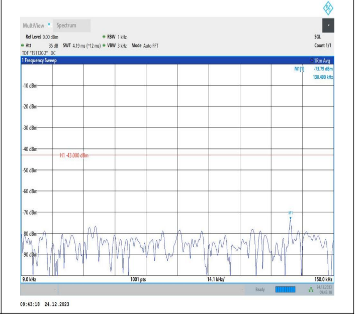
2-2-20MHz-10MHz-QPSK-QPSK-18700-18844-1RB#0-ORB#0 -0.009~0.15MHz-PASS
