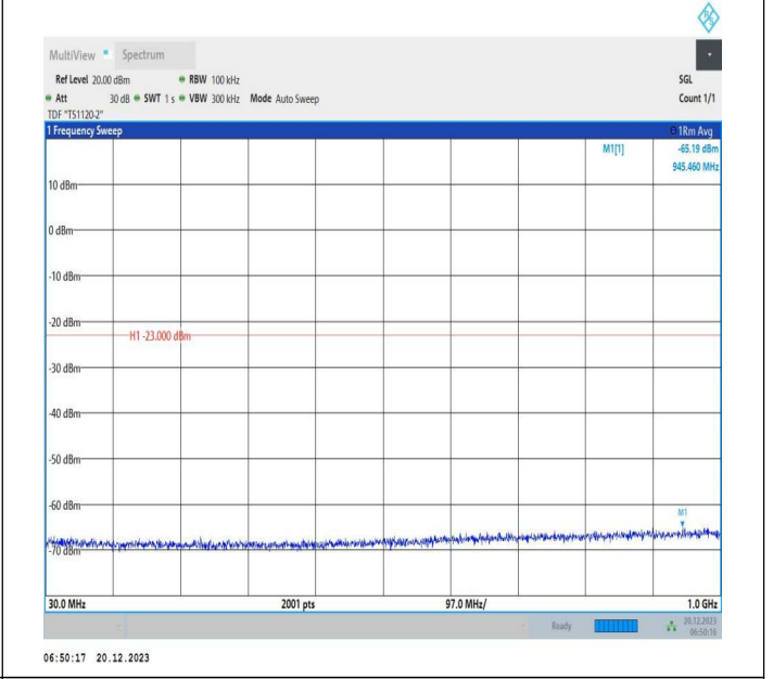
2-2-10MHz-20MHz-16QAM-16QAM-18956-19100-1RB#0-0RB #0-30~1000MHz-PASS
