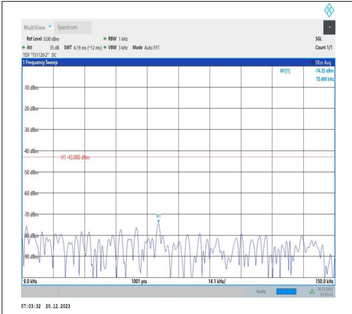
2-2-10MHz-20MHz-16QAM-16QAM-18956-19100-1RB#49-0R B#0-0.009~0.15MHz-PASS
