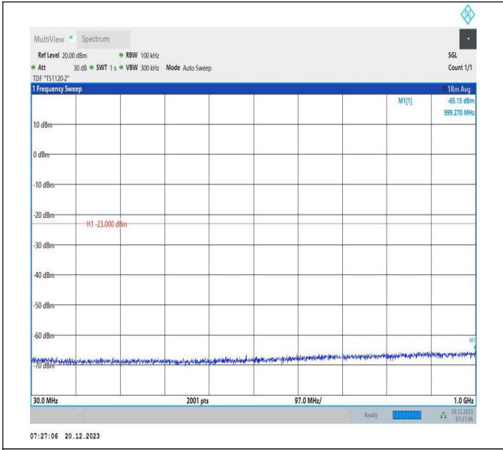
2-2-20MHz-10MHz-64QAM-64QAM-18700-18844-1RB#0-ORB #0-30~1000MHz-PASS
