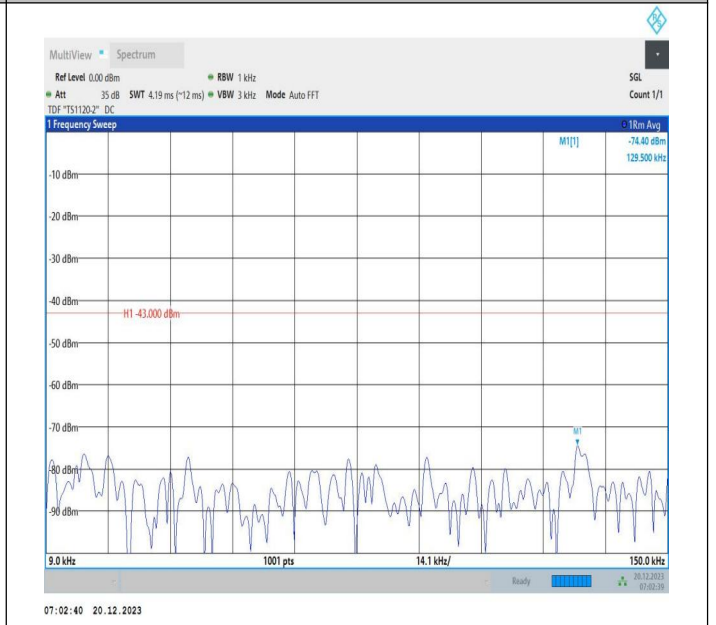
2-2-10MHz-20MHz-QPSK-QPSK-18956-19100-1RB#49-ORB# 0-0.009~0.15MHz-PASS
