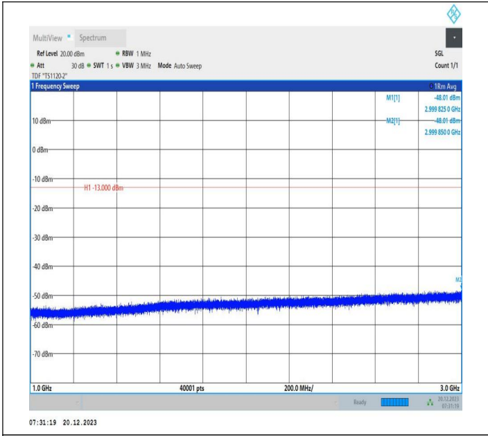
2-2-20MHz-10MHz-64QAM-64QAM-18700-18844-1RB#99-0R B#0-1000~3000MHz-PASS
