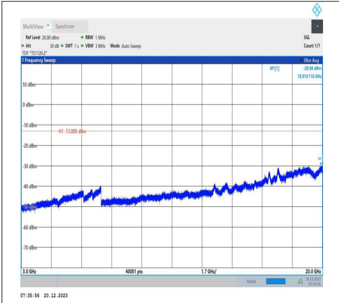
2-2-20MHz-10MHz-64QAM-64QAM-18700-18844-1RB#0-1RB #49-3000~20000MHz-PASS
