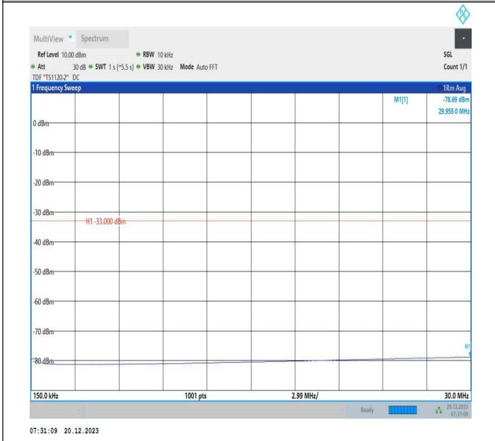
2-2-20MHz-10MHz-64QAM-64QAM-18700-18844-1RB#99-0R B#0-0.15~30MHz-PASS
