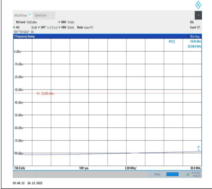
2-2-20MHz-10MHz-QPSK-QPSK-18700-18844-100RB#0-40R B#0-0.15~30MHz-PASS
