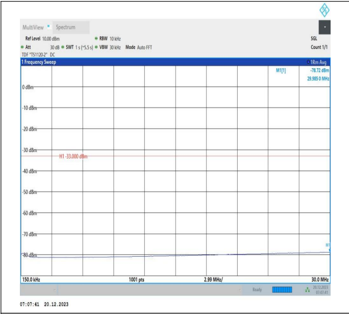
2-2-10MHz-20MHz-16QAM-16QAM-18956-19100-1RB#0-1RB #99-0.15~30MHz-PASS
