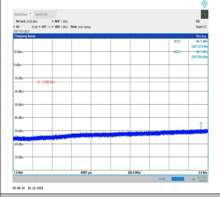
2-2-10MHz-20MHz-64QAM-64QAM-18806-18950-50RB#0-10 ORB#0-1000~3000MHz-PASS
