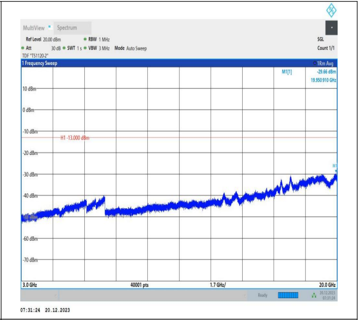
2-2-20MHz-10MHz-64QAM-64QAM-18700-18844-1RB#99-0R B#0-3000~20000MHz-PASS
