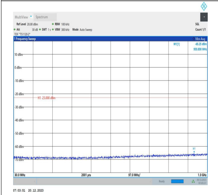
2-2-10MHz-20MHz-16QAM-16QAM-18956-19100-1RB#49-0R B#0-30~1000MHz-PASS
