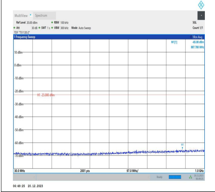
2-2-10MHz-20MHz-QPSK-QPSK-18956-19100-1RB#0-0RB#0 -30~1000MHz-PASS
