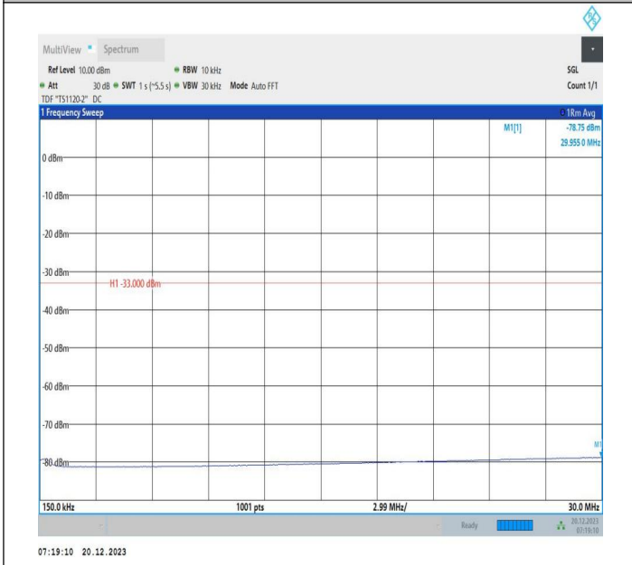
2-2-10MHz-20MHz-QPSK-QPSK-18956-19100-50RB#0-100R B#0-0.15~30MHz-PASS
