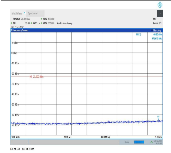
2-2-10MHz-20MHz-64QAM-64QAM-18956-19100-1RB#0-ORB #0-30~1000MHz-PASS
