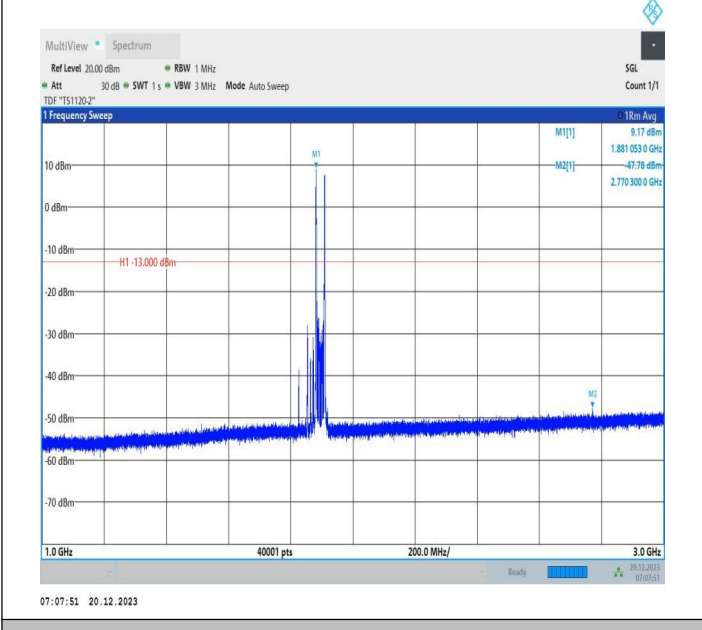
2-2-10MHz-20MHz-16QAM-16QAM-18956-19100-1RB#0-1RB #99-1000~3000MHz-PASS
