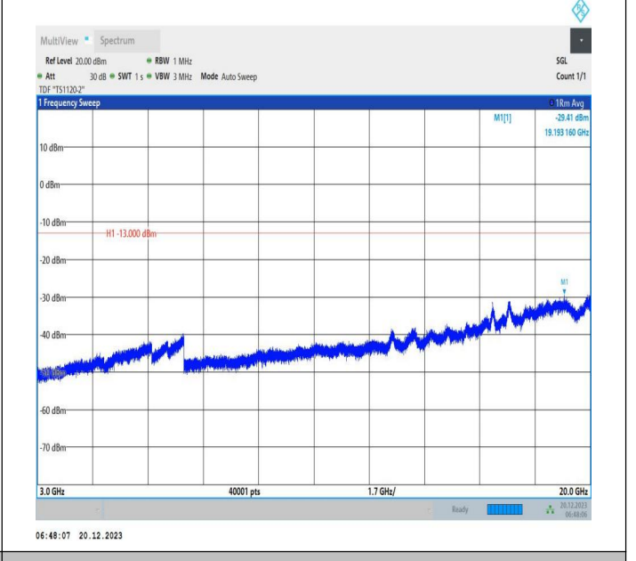
2-2-10MHz-20MHz-64QAM-64QAM-18806-18950-50RB#0-10 ORB#0-3000~20000MHz-PASS
