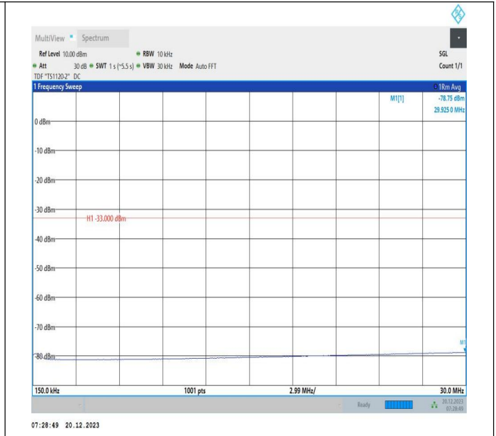
2-2-20MHz-10MHz-16QAM-16QAM-18700-18844-1RB#99-0R B#0-0.15~30MHz-PASS
