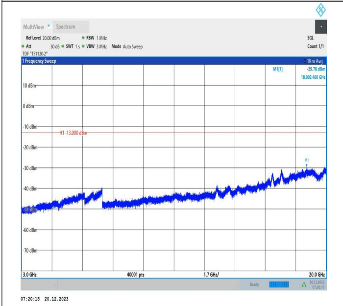
2-2-10MHz-20MHz-16QAM-16QAM-18956-19100-50RB#0-10 ORB#0-3000~20000MHz-PASS
