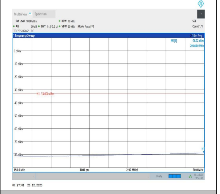
2-2-20MHz-10MHz-64QAM-64QAM-18700-18844-1RB#0-ORB #0-0.15~30MHz-PASS
