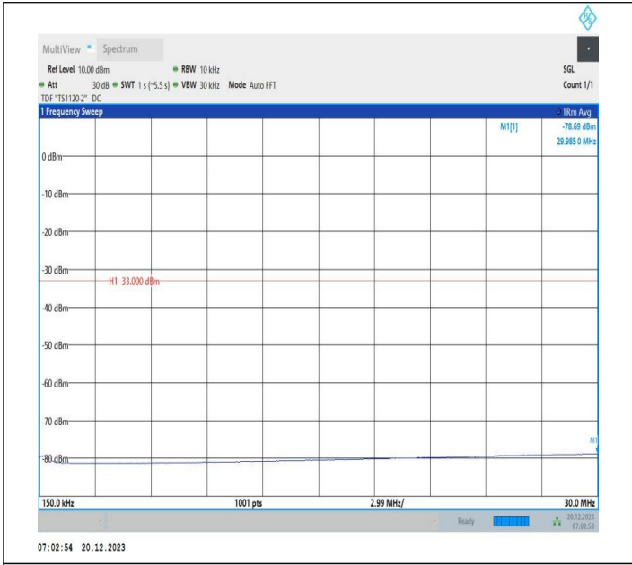
2-2-10MHz-20MHz-QPSK-QPSK-18956-19100-1RB#49-0RB# 0-0.15~30MHz-PASS
