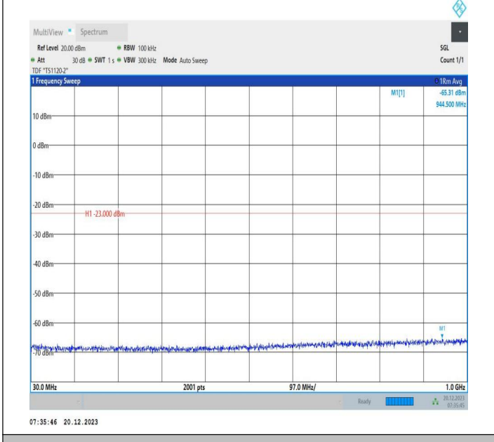
2-2-20MHz-10MHz-64QAM-64QAM-18700-18844-1RB#0-1RB #49-30~1000MHz-PASS
