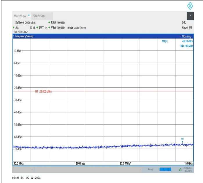
2-2-20MHz-10MHz-16QAM-16QAM-18700-18844-1RB#99-0R B#0-30~1000MHz-PASS
