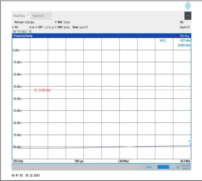
2-2-10MHz-20MHz-64QAM-64QAM-18806-18950-50RB#0-10 ORB#0-0.15~30MHz-PASS
