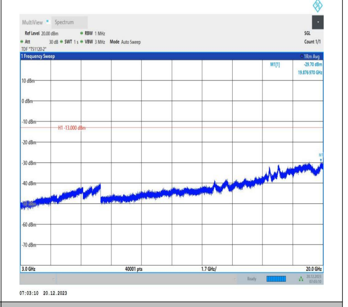
2-2-10MHz-20MHz-QPSK-QPSK-18956-19100-1RB#49-0RB# 0-3000~20000MHz-PASS
