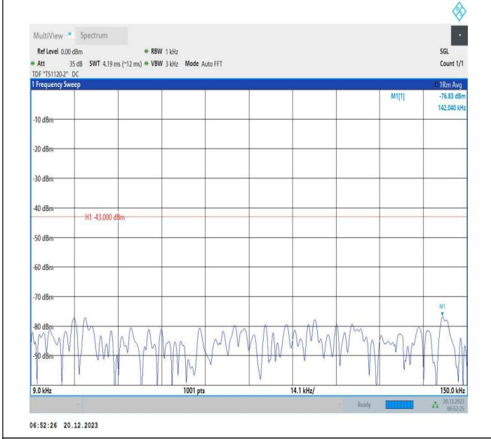
2-2-10MHz-20MHz-64QAM-64QAM-18956-19100-1RB#0-ORB #0-0.009~0.15MHz-PASS
