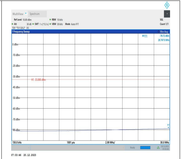
2-2-10MHz-20MHz-16QAM-16QAM-18956-19100-1RB#49-0R B#0-0.15~30MHz-PASS
