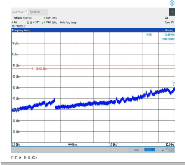
2-2-20MHz-10MHz-64QAM-64QAM-18700-18844-1RB#0-ORB #0-3000~20000MHz-PASS
