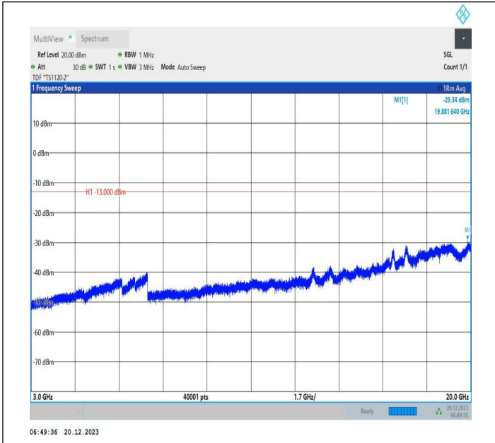
2-2-10MHz-20MHz-QPSK-QPSK-18956-19100-1RB#0-0RB#0 -3000~20000MHz-PASS
