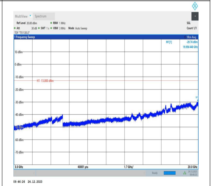
2-2-20MHz-10MHz-QPSK-QPSK-18700-18844-100RB#0-40R B#0-3000~20000MHz-PASS
