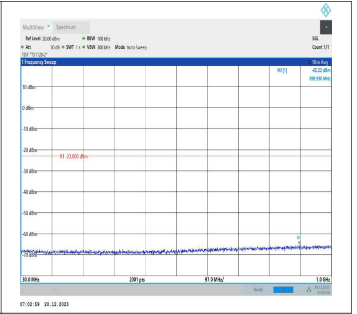
2-2-10MHz-20MHz-QPSK-QPSK-18956-19100-1RB#49-0RB# 0-30~1000MHz-PASS
