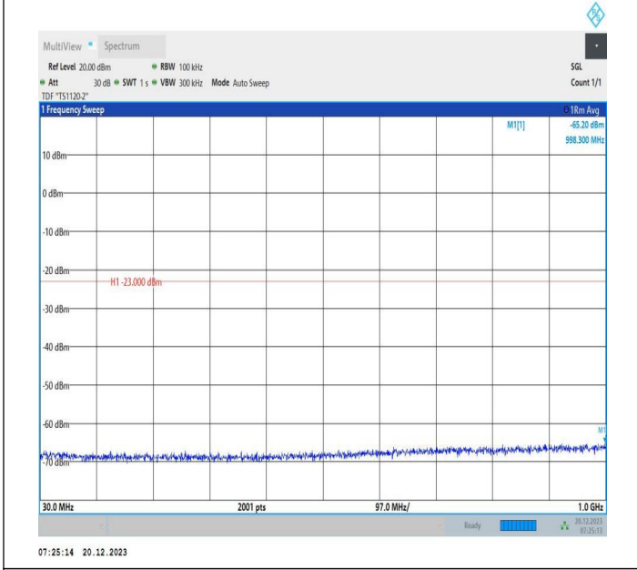
2-2-20MHz-10MHz-16QAM-16QAM-18700-18844-1RB#0-ORB #0-30~1000MHz-PASS
