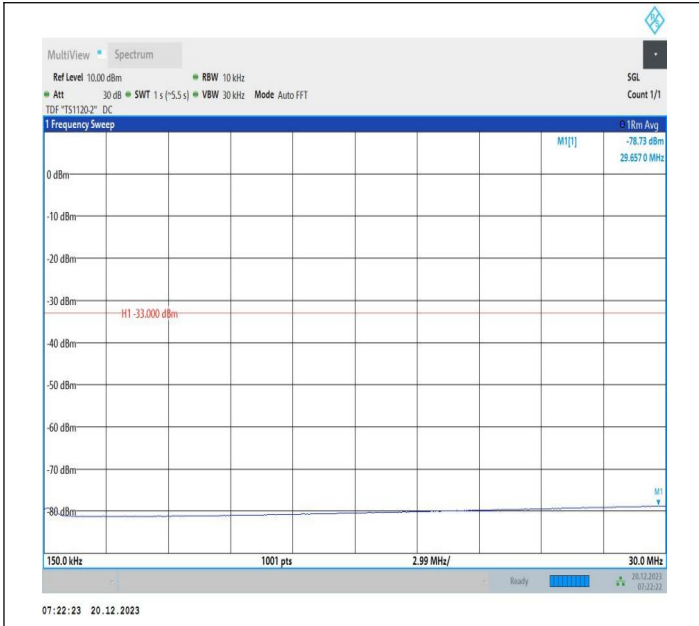
2-2-10MHz-20MHz-64QAM-64QAM-18956-19100-50RB#0-10 ORB#0-0.15~30MHz-PASS
