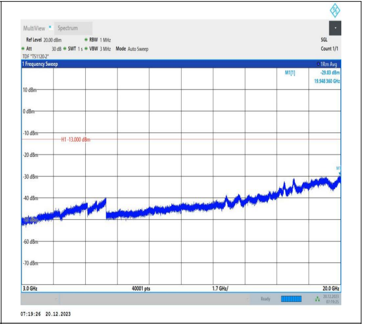
2-2-10MHz-20MHz-QPSK-QPSK-18956-19100-50RB#0-100R B#0-3000~20000MHz-PASS
