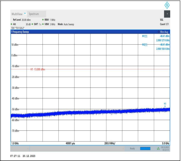
2-2-20MHz-10MHz-64QAM-64QAM-18700-18844-1RB#0-ORB #0-1000~3000MHz-PASS
