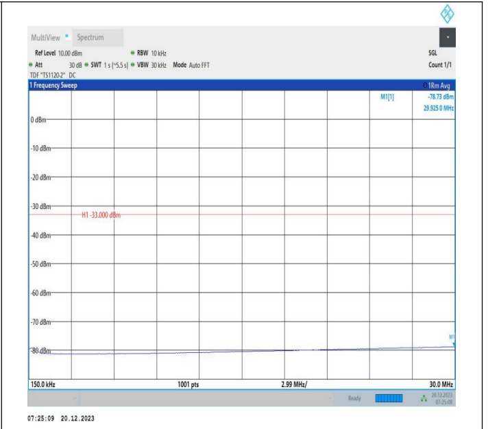
2-2-20MHz-10MHz-16QAM-16QAM-18700-18844-1RB#0-ORB #0-0.15~30MHz-PASS
