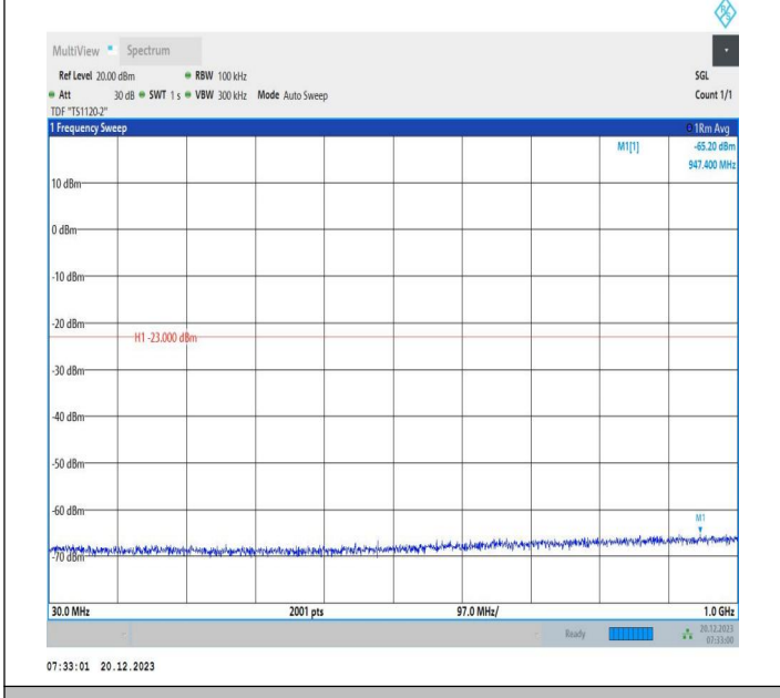
2-2-20MHz-10MHz-16QAM-16QAM-18700-18844-1RB#0-1RB #49-30~1000MHz-PASS
