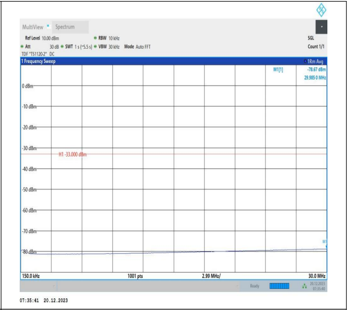
2-2-20MHz-10MHz-64QAM-64QAM-18700-18844-1RB#0-1RB #49-0.15~30MHz-PASS
