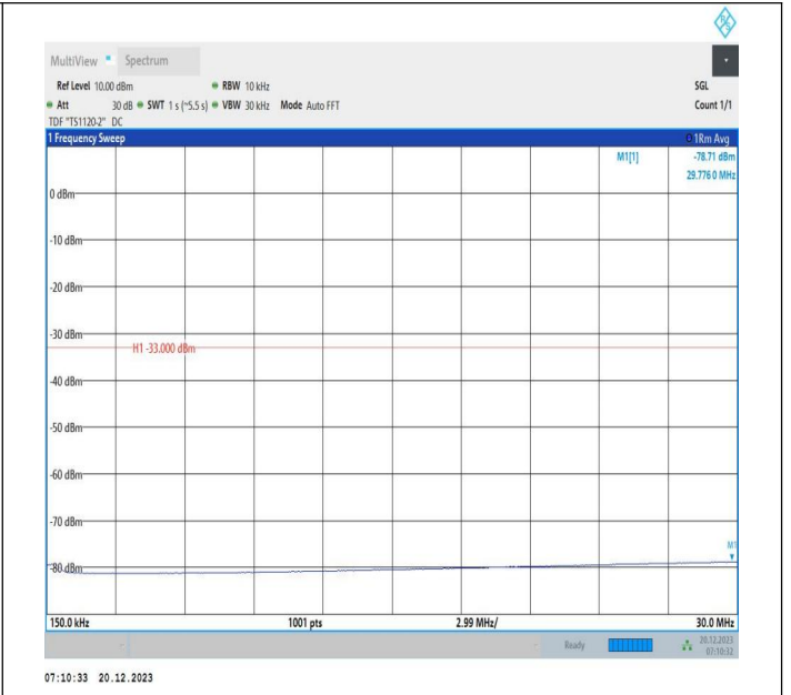
2-2-10MHz-20MHz-64QAM-64QAM-18956-19100-1RB#0-1RB #99-0.15~30MHz-PASS
