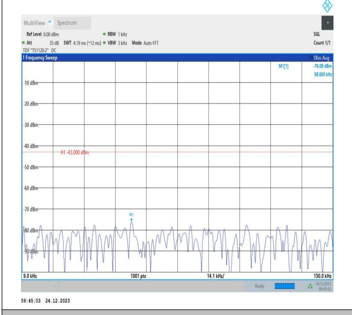
2-2-20MHz-10MHz-QPSK-QPSK-18700-18844-1RB#0-1RB#4 9-0.009~0.15MHz-PASS
