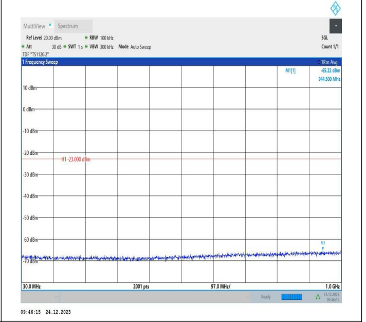
2-2-20MHz-10MHz-QPSK-QPSK-18700-18844-100RB#0-40R B#0-30~1000MHz-PASS
