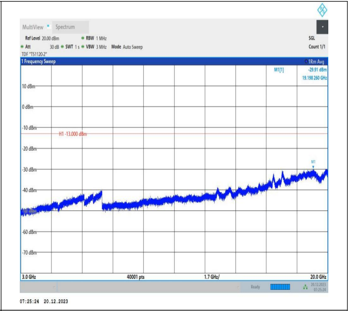
2-2-20MHz-10MHz-16QAM-16QAM-18700-18844-1RB#0-ORB #0-3000~20000MHz-PASS
