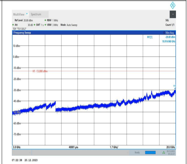
2-2-10MHz-20MHz-64QAM-64QAM-18956-19100-50RB#0-10 ORB#0-3000~20000MHz-PASS
