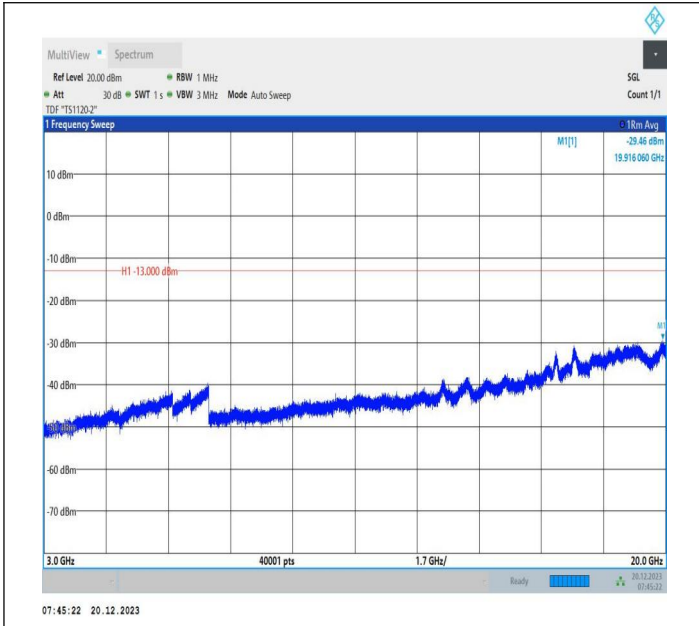
2-2-20MHz-10MHz-16QAM-16QAM-18700-18844-100RB#0-4 ORB#0-3000~20000MHz-PASS
