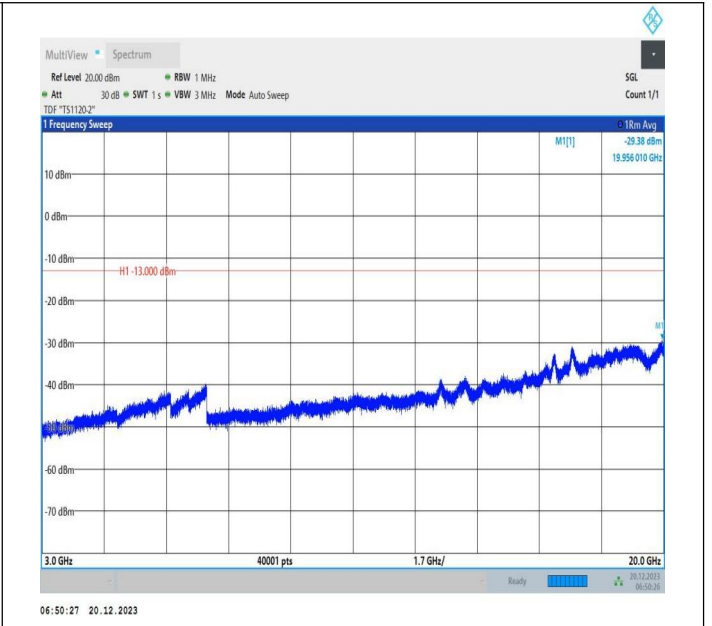
2-2-10MHz-20MHz-16QAM-16QAM-18956-19100-1RB#0-ORB #0-3000~20000MHz-PASS
