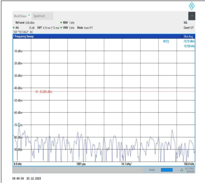
2-2-10MHz-20MHz-QPSK-QPSK-18956-19100-1RB#0-0RB#0 -0.009~0.15MHz-PASS
