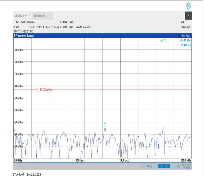
2-2-20MHz-10MHz-64QAM-64QAM-18700-18844-100RB#0-4 ORB#0-0.009~0.15MHz-PASS
