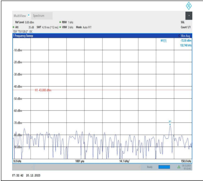
2-2-20MHz-10MHz-16QAM-16QAM-18700-18844-1RB#0-1RB #49-0.009~0.15MHz-PASS
