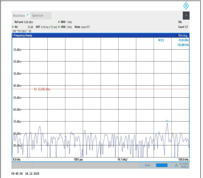
2-2-20MHz-10MHz-QPSK-QPSK-18700-18844-100RB#0-40R B#0-0.009~0.15MHz-PASS
