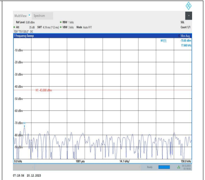
2-2-10MHz-20MHz-QPSK-QPSK-18956-19100-50RB#0-100R B#0-0.009~0.15MHz-PASS
