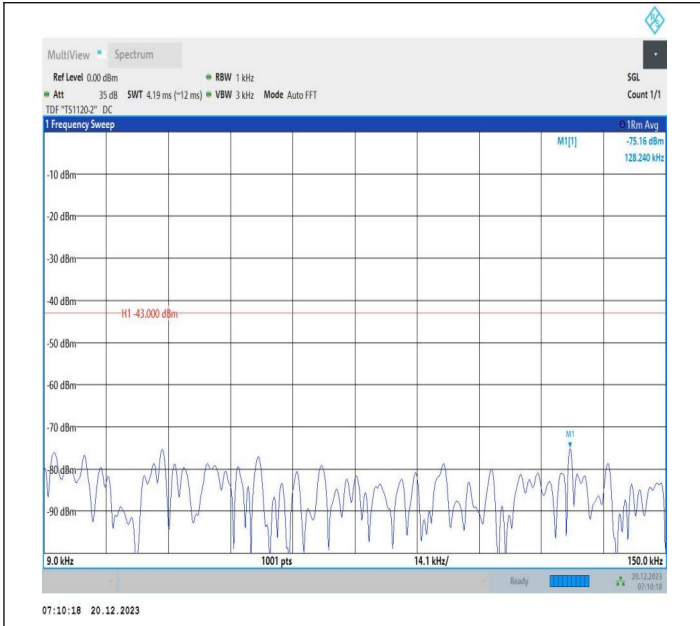
2-2-10MHz-20MHz-64QAM-64QAM-18956-19100-1RB#0-1RB #99-0.009~0.15MHz-PASS
