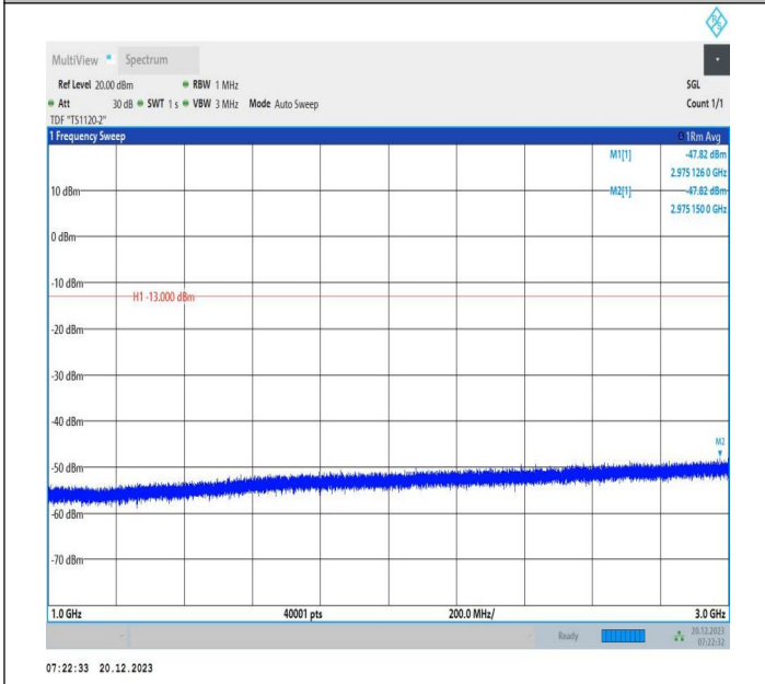
2-2-10MHz-20MHz-64QAM-64QAM-18956-19100-50RB#0-10 ORB#0-1000~3000MHz-PASS
