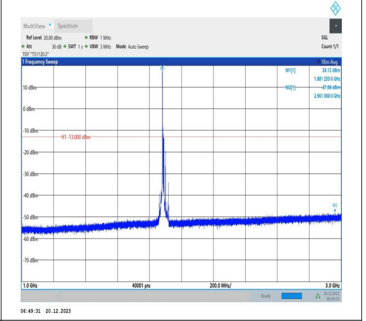
2-2-10MHz-20MHz-QPSK-QPSK-18956-19100-1RB#0-0RB#0 -1000~3000MHz-PASS
