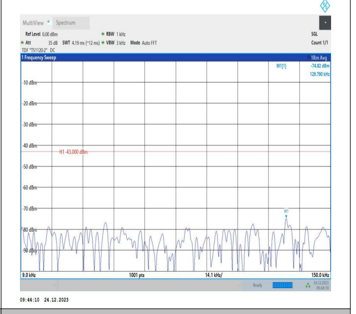
2-2-20MHz-10MHz-QPSK-QPSK-18700-18844-1RB#99-ORB# 0-0.009~0.15MHz-PASS
