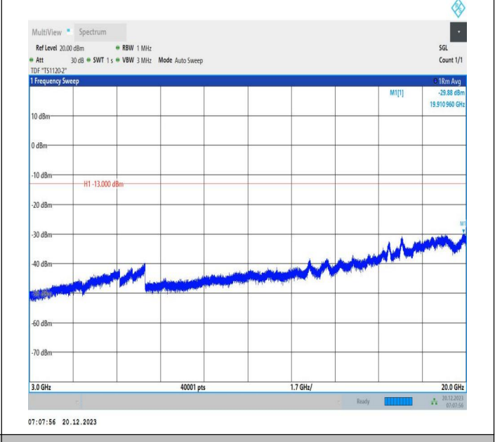
2-2-10MHz-20MHz-16QAM-16QAM-18956-19100-1RB#0-1RB #99-3000~20000MHz-PASS
