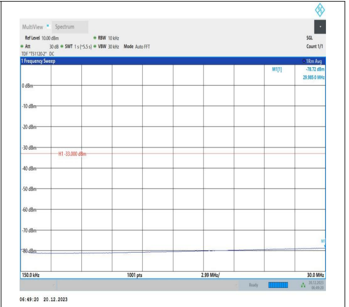
2-2-10MHz-20MHz-QPSK-QPSK-18956-19100-1RB#0-0RB#0 -0.15~30MHz-PASS
