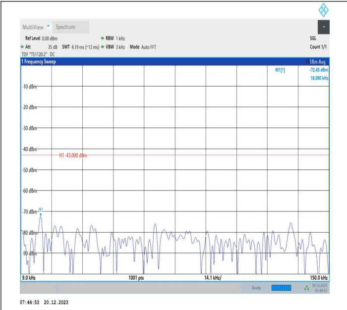
2-2-20MHz-10MHz-16QAM-16QAM-18700-18844-100RB#0-4 ORB#0-0.009~0.15MHz-PASS
