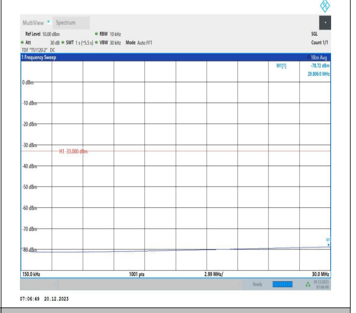
2-2-10MHz-20MHz-QPSK-QPSK-18956-19100-1RB#0-1RB#9 9-0.15~30MHz-PASS
