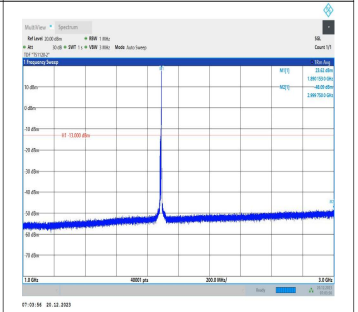
2-2-10MHz-20MHz-16QAM-16QAM-18956-19100-1RB#49-0R B#0-1000~3000MHz-PASS
