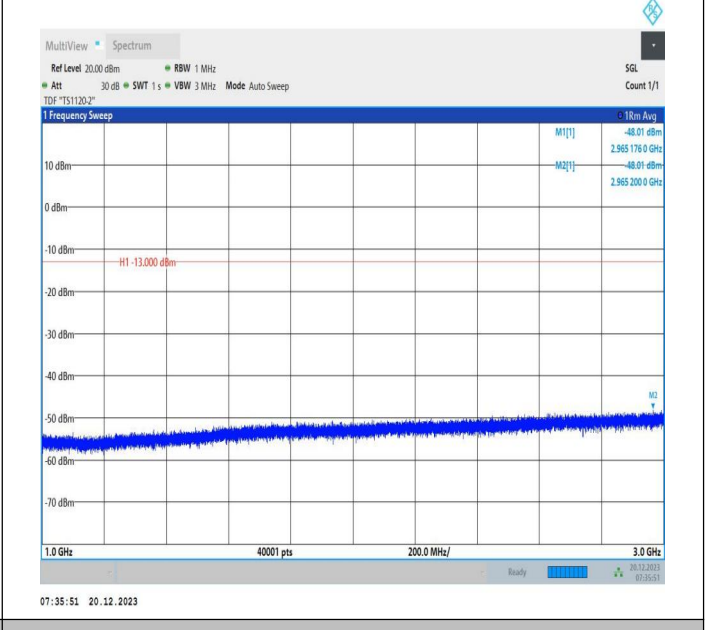
2-2-20MHz-10MHz-64QAM-64QAM-18700-18844-1RB#0-1RB #49-1000~3000MHz-PASS
