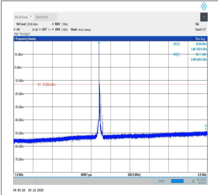
2-2-10MHz-20MHz-16QAM-16QAM-18956-19100-1RB#0-ORB #0-1000~3000MHz-PASS
