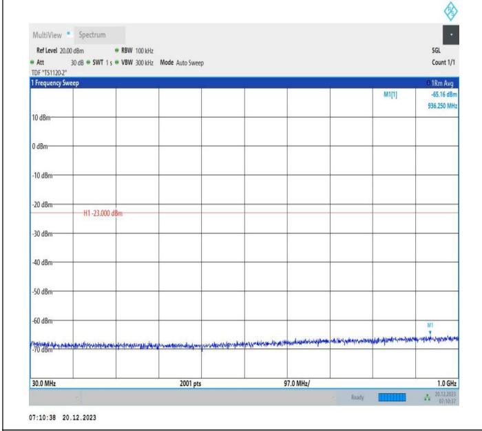
2-2-10MHz-20MHz-64QAM-64QAM-18956-19100-1RB#0-1RB #99-30~1000MHz-PASS
