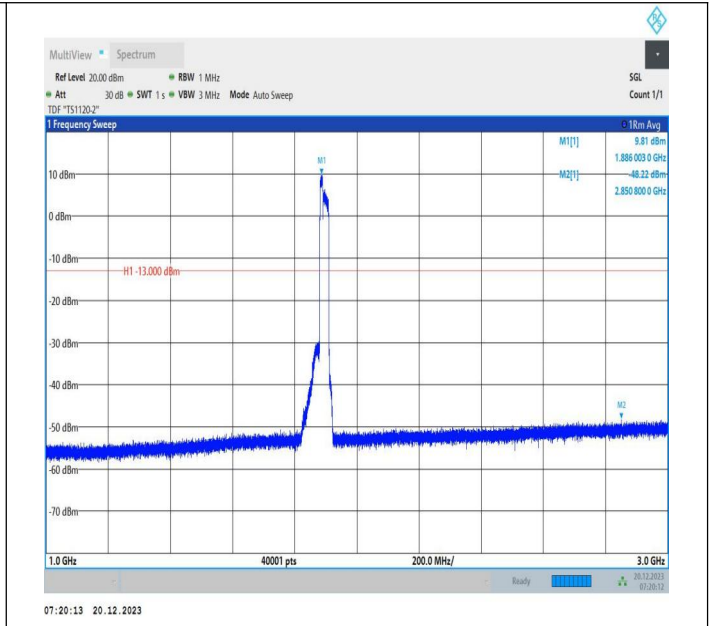
2-2-10MHz-20MHz-16QAM-16QAM-18956-19100-50RB#0-10 ORB#0-1000~3000MHz-PASS
