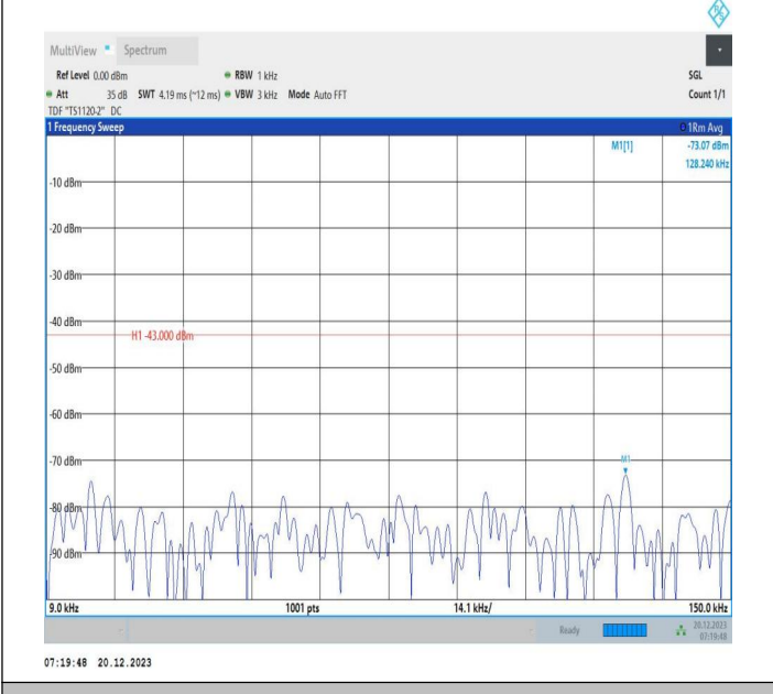
2-2-10MHz-20MHz-16QAM-16QAM-18956-19100-50RB#0-10 ORB#0-0.009~0.15MHz-PASS
