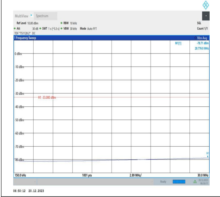
2-2-10MHz-20MHz-16QAM-16QAM-18956-19100-1RB#0-0RB #0-0.15~30MHz-PASS
