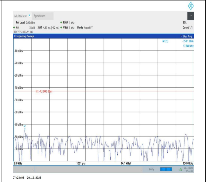
2-2-10MHz-20MHz-64QAM-64QAM-18956-19100-50RB#0-10 ORB#0-0.009~0.15MHz-PASS
