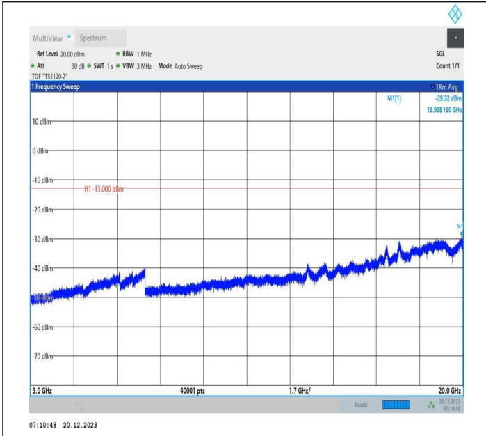
2-2-10MHz-20MHz-64QAM-64QAM-18956-19100-1RB#0-1RB #99-3000~20000MHz-PASS
