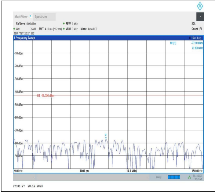
2-2-20MHz-10MHz-64QAM-64QAM-18700-18844-1RB#0-1RB #49-0.009~0.15MHz-PASS
