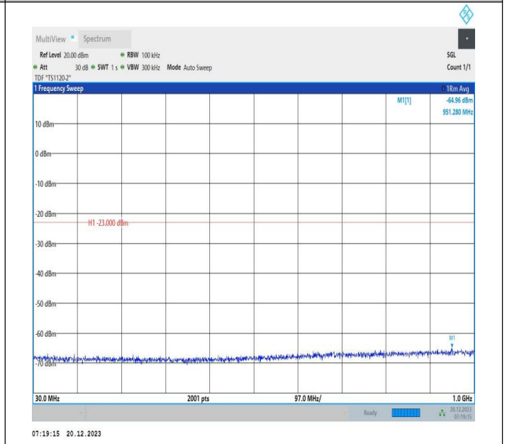
2-2-10MHz-20MHz-QPSK-QPSK-18956-19100-50RB#0-100R B#0-30~1000MHz-PASS
