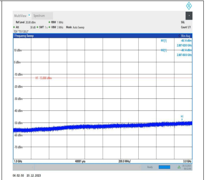
2-2-10MHz-20MHz-64QAM-64QAM-18956-19100-1RB#0-ORB #0-1000~3000MHz-PASS
