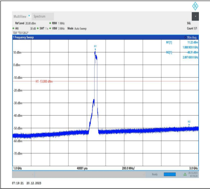
2-2-10MHz-20MHz-QPSK-QPSK-18956-19100-50RB#0-100R B#0-1000~3000MHz-PASS
