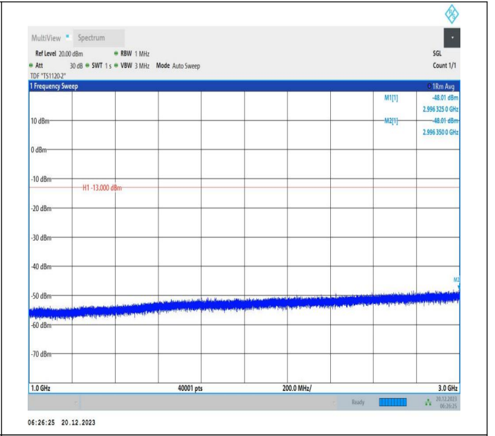
2-2-10MHz-20MHz-64QAM-64QAM-18806-18950-1RB#0-ORB #0-1000~3000MHz-PASS
