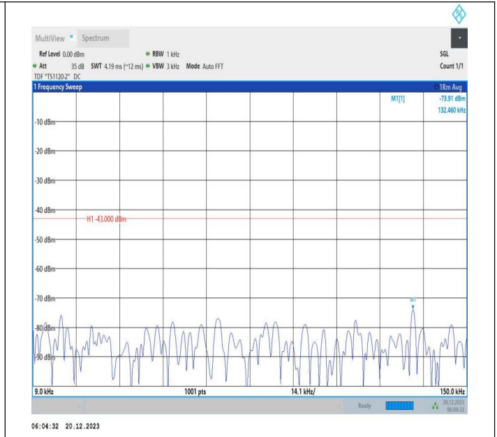
2-2-10MHz-20MHz-64QAM-64QAM-18655-18799-1RB#49-OR B#0-0.009~0.15MHz-PASS
