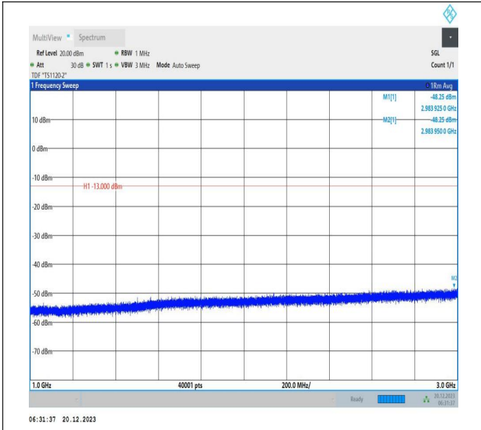
2-2-10MHz-20MHz-64QAM-64QAM-18806-18950-1RB#49-0R B#0-1000~3000MHz-PASS
