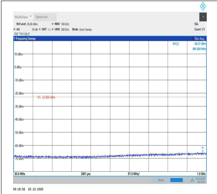
2-2-10MHz-20MHz-16QAM-16QAM-18655-18799-50RB#0-10 ORB#0-30~1000MHz-PASS
