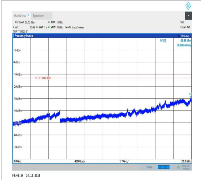
2-2-10MHz-20MHz-16QAM-16QAM-18655-18799-1RB#49-OR B#0-3000~20000MHz-PASS
