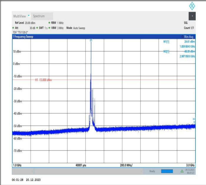
2-2-10MHz-20MHz-QPSK-QPSK-18655-18799-1RB#49-0RB# 0-1000~3000MHz-PASS
