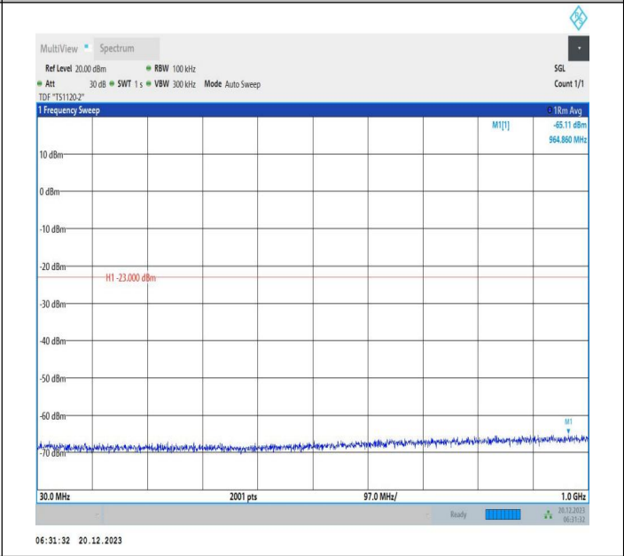
2-2-10MHz-20MHz-64QAM-64QAM-18806-18950-1RB#49-OR B#0-30~1000MHz-PASS
