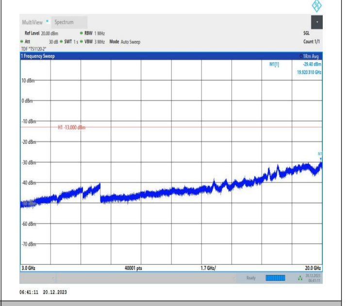
2-2-10MHz-20MHz-16QAM-16QAM-18806-18950-1RB#0-1RB #99-3000~20000MHz-PASS
