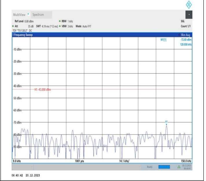
2-2-10MHz-20MHz-16QAM-16QAM-18806-18950-1RB#0-1RB #99-0.009~0.15MHz-PASS
