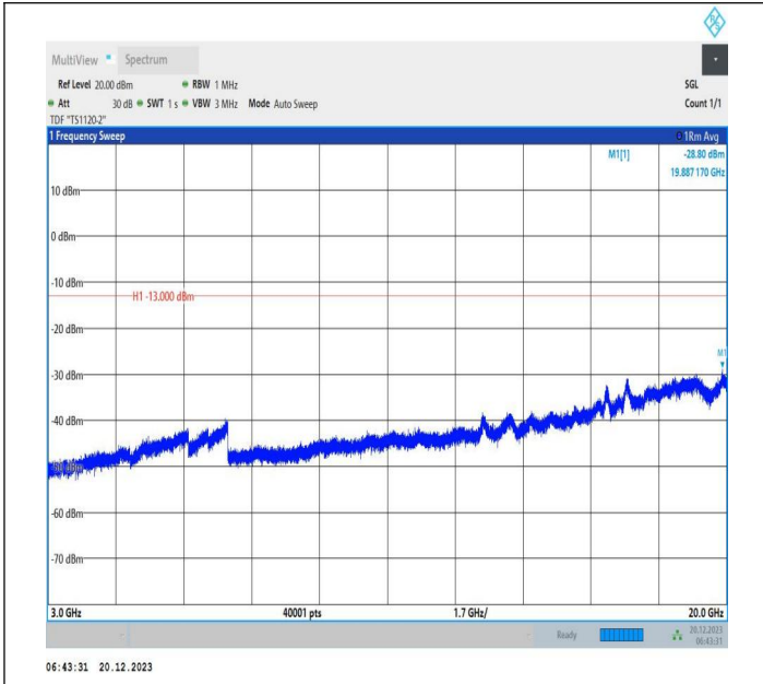
2-2-10MHz-20MHz-64QAM-64QAM-18806-18950-1RB#0-1RB #99-3000~20000MHz-PASS
