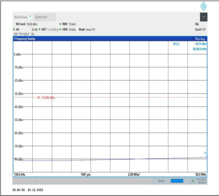
2-2-10MHz-20MHz-16QAM-16QAM-18806-18950-1RB#0-1RB #99-0.15~30MHz-PASS
