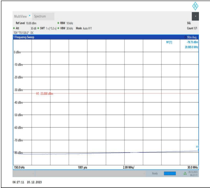
2-2-10MHz-20MHz-QPSK-QPSK-18806-18950-1RB#49-0RB# 0-0.15~30MHz-PASS
