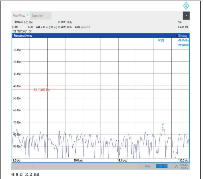
2-2-10MHz-20MHz-16QAM-16QAM-18655-18799-1RB#0-0RB #0-0.009~0.15MHz-PASS
