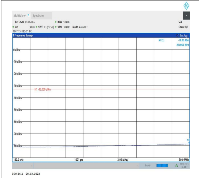
2-2-10MHz-20MHz-QPSK-QPSK-18806-18950-50RB#0-100R B#0-0.15~30MHz-PASS
