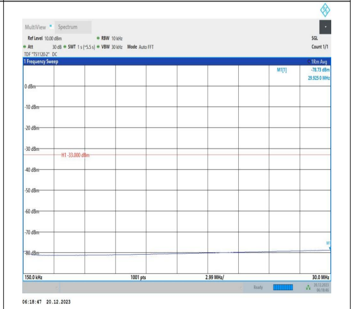
2-2-10MHz-20MHz-16QAM-16QAM-18655-18799-50RB#0-10 ORB#0-0.15~30MHz-PASS
