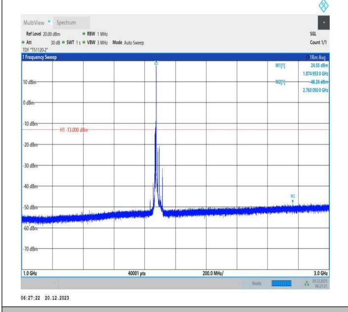
2-2-10MHz-20MHz-QPSK-QPSK-18806-18950-1RB#49-0RB# 0-1000~3000MHz-PASS
