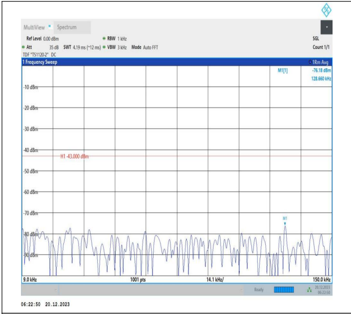
2-2-10MHz-20MHz-QPSK-QPSK-18806-18950-1RB#0-0RB#0 -0.009~0.15MHz-PASS
