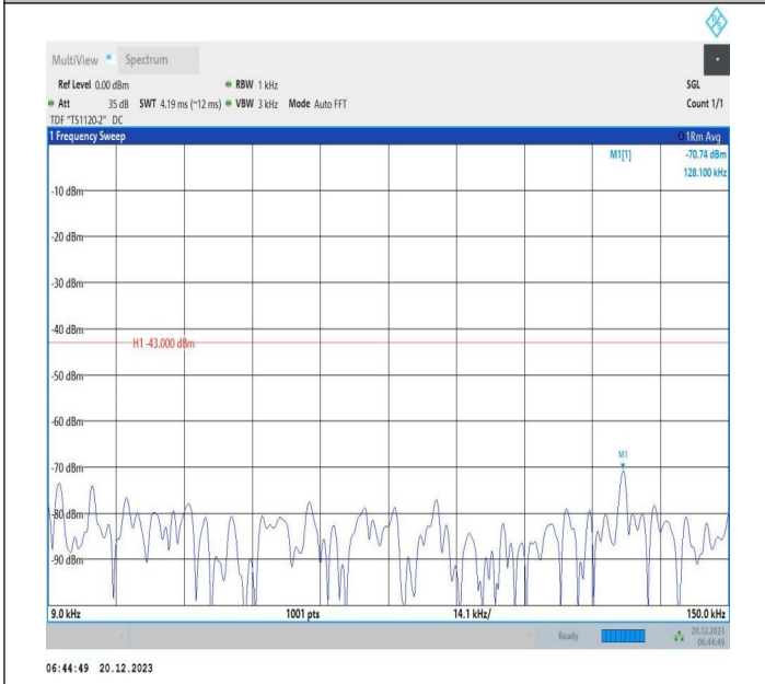
2-2-10MHz-20MHz-16QAM-16QAM-18806-18950-50RB#0-10 ORB#0-0.009~0.15MHz-PASS
