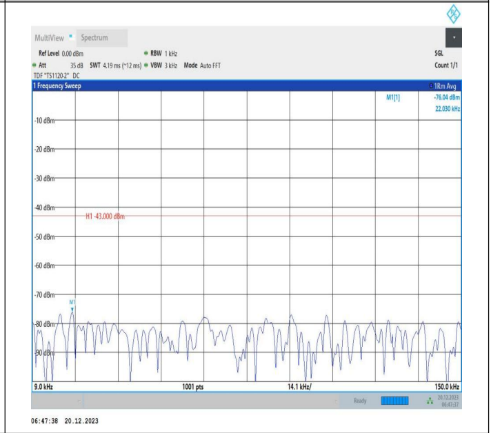
2-2-10MHz-20MHz-64QAM-64QAM-18806-18950-50RB#0-10 ORB#0-0.009~0.15MHz-PASS
