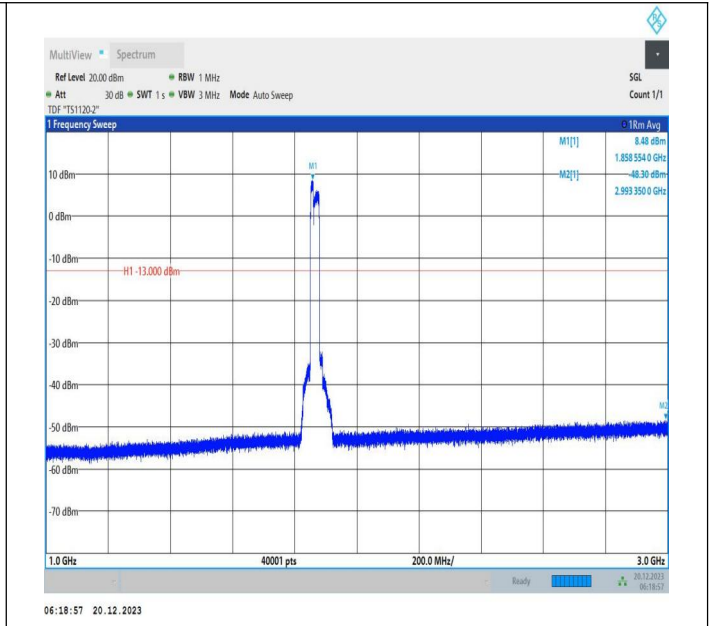
2-2-10MHz-20MHz-16QAM-16QAM-18655-18799-50RB#0-10 ORB#0-1000~3000MHz-PASS
