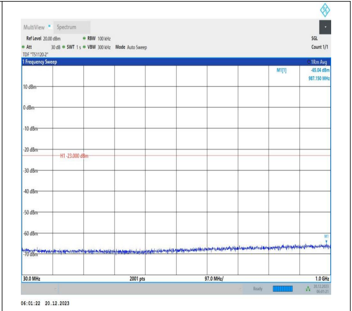
2-2-10MHz-20MHz-QPSK-QPSK-18655-18799-1RB#49-0RB# 0-30~1000MHz-PASS
