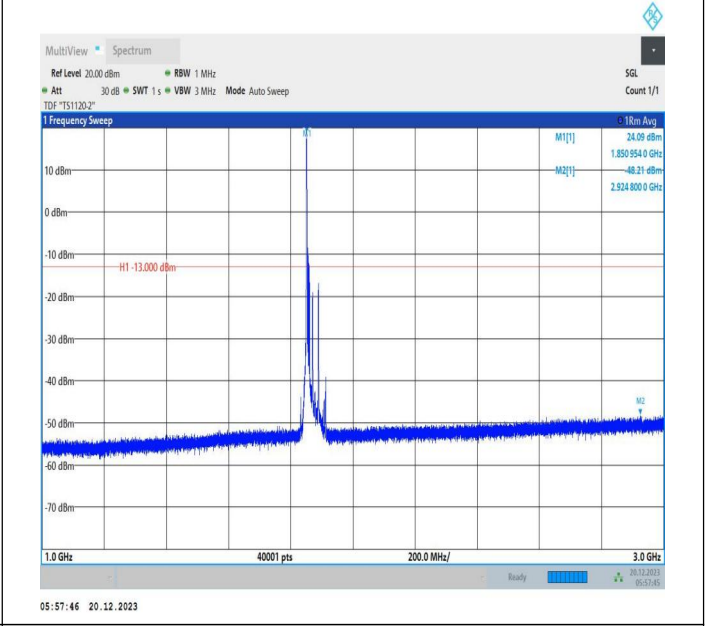
2-2-10MHz-20MHz-QPSK-QPSK-18655-18799-1RB#0-0RB#0 -1000~3000MHz-PASS
