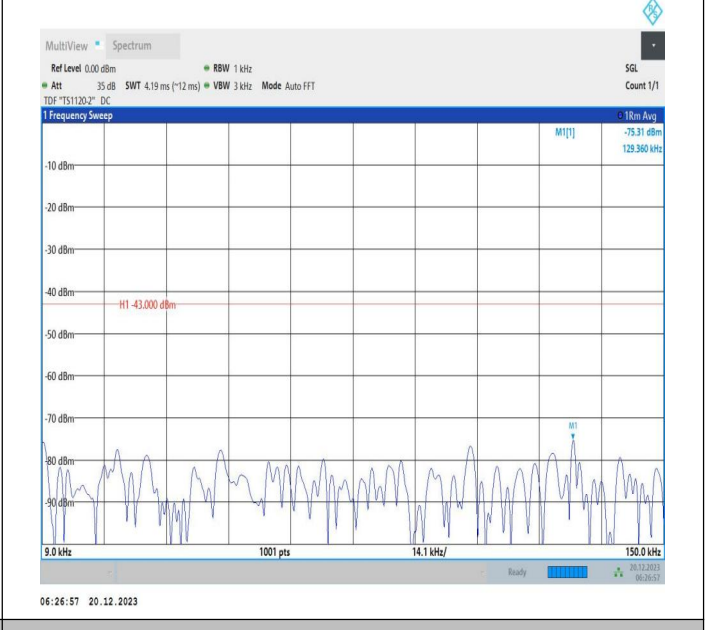
2-2-10MHz-20MHz-QPSK-QPSK-18806-18950-1RB#49-ORB# 0-0.009~0.15MHz-PASS
