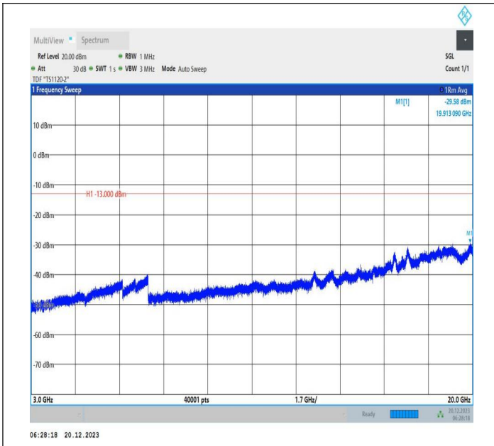
2-2-10MHz-20MHz-16QAM-16QAM-18806-18950-1RB#49-OR B#0-3000~20000MHz-PASS
