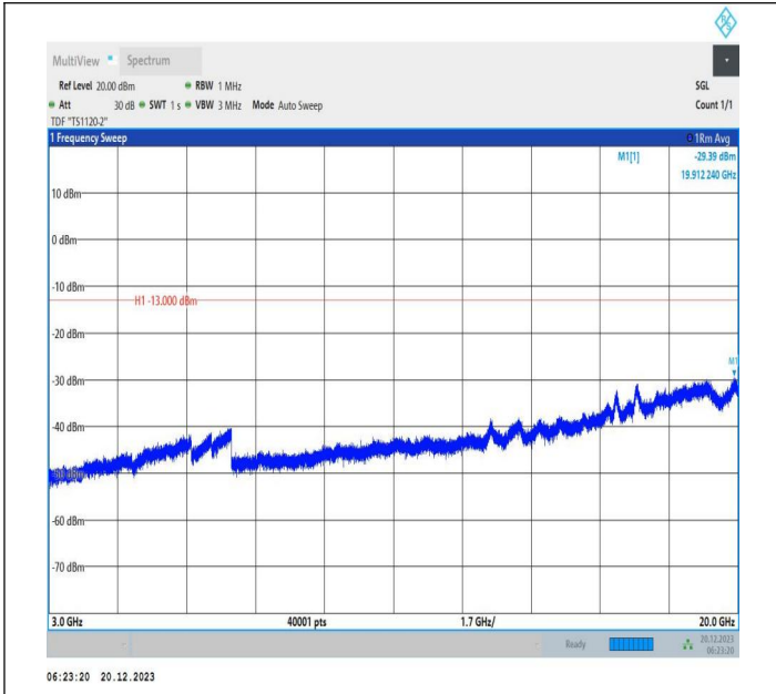
2-2-10MHz-20MHz-QPSK-QPSK-18806-18950-1RB#0-0RB#0 -3000~20000MHz-PASS
