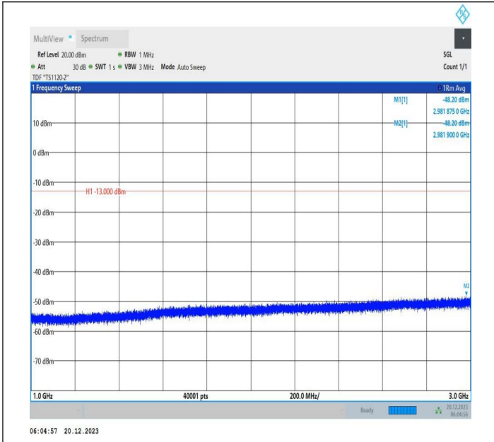
2-2-10MHz-20MHz-64QAM-64QAM-18655-18799-1RB#49-0R B#0-1000~3000MHz-PASS
