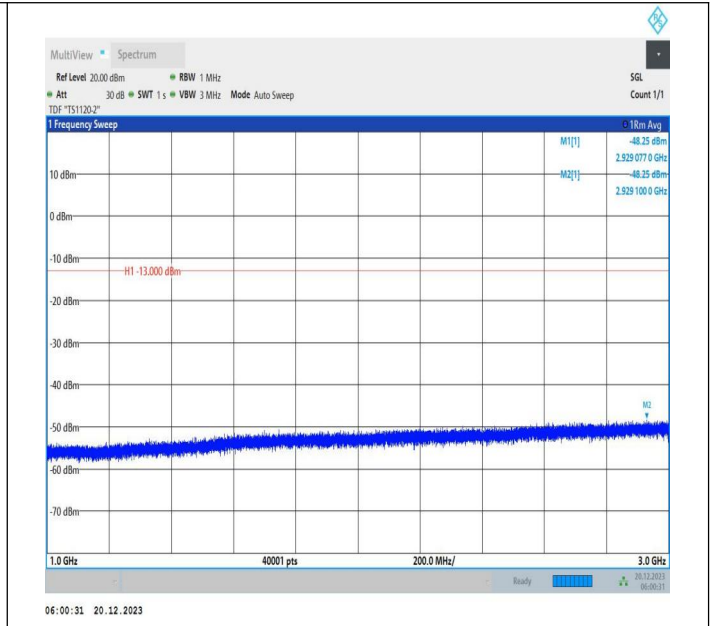
2-2-10MHz-20MHz-64QAM-64QAM-18655-18799-1RB#0-ORB #0-1000~3000MHz-PASS
