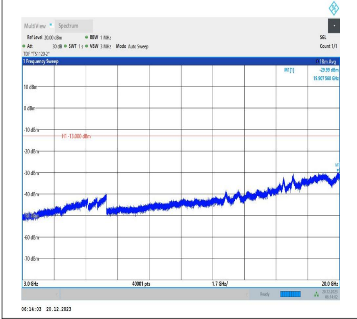
2-2-10MHz-20MHz-QPSK-QPSK-18655-18799-1RB#0-1RB#9 9-3000~20000MHz-PASS
