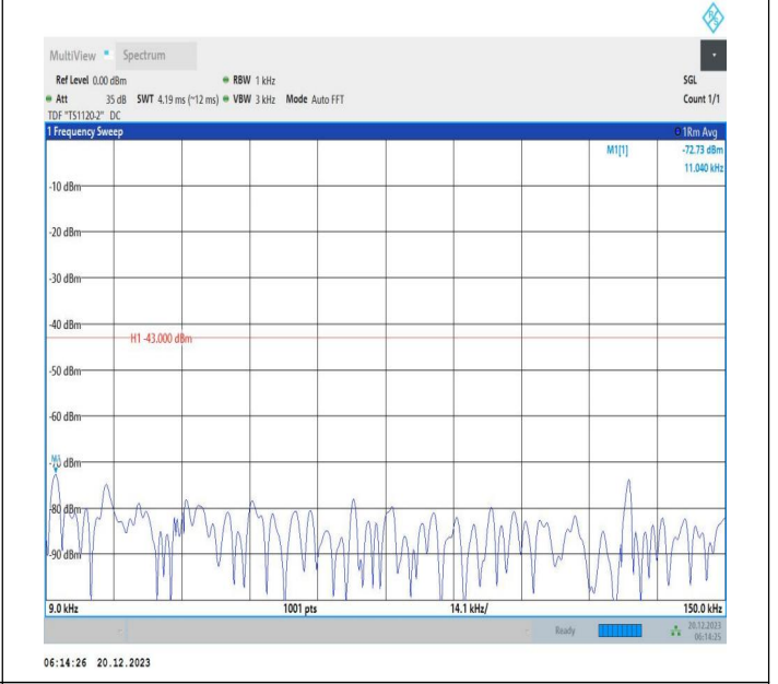
2-2-10MHz-20MHz-16QAM-16QAM-18655-18799-1RB#0-1RB #99-0.009~0.15MHz-PASS
