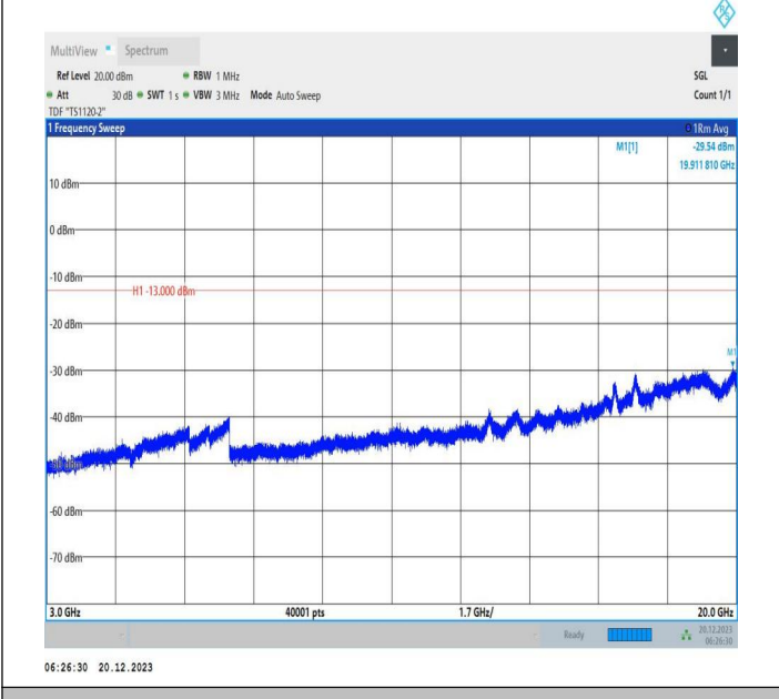
2-2-10MHz-20MHz-64QAM-64QAM-18806-18950-1RB#0-ORB #0-3000~20000MHz-PASS
