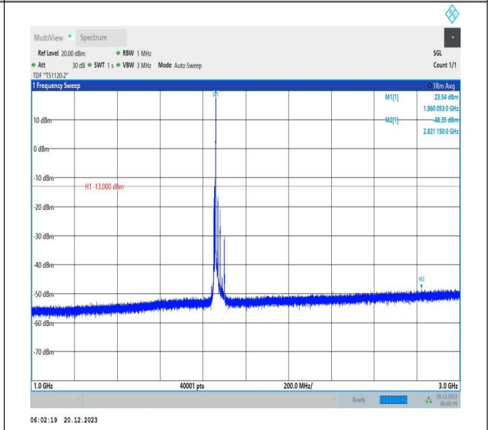
2-2-10MHz-20MHz-16QAM-16QAM-18655-18799-1RB#49-OR B#0-1000~3000MHz-PASS
