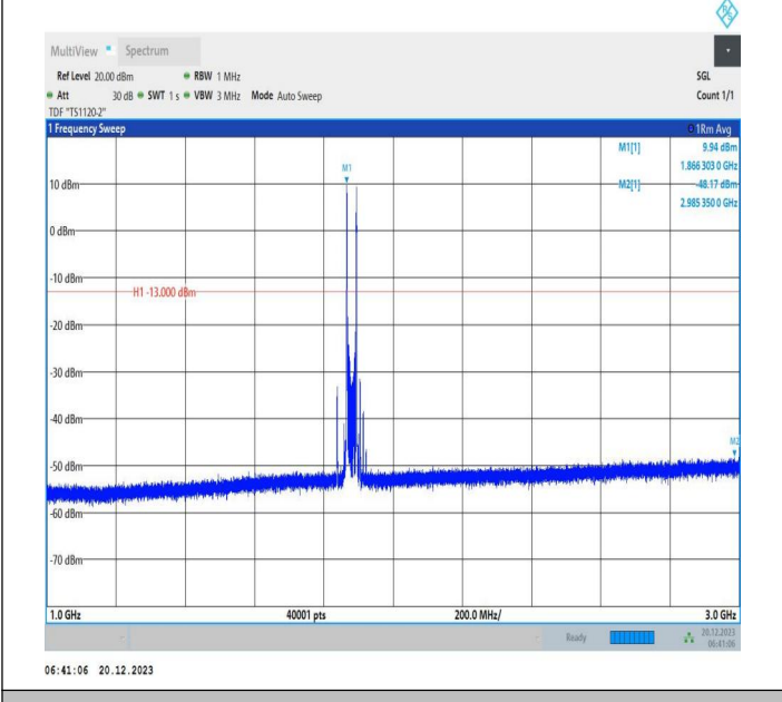
2-2-10MHz-20MHz-16QAM-16QAM-18806-18950-1RB#0-1RB #99-1000~3000MHz-PASS
