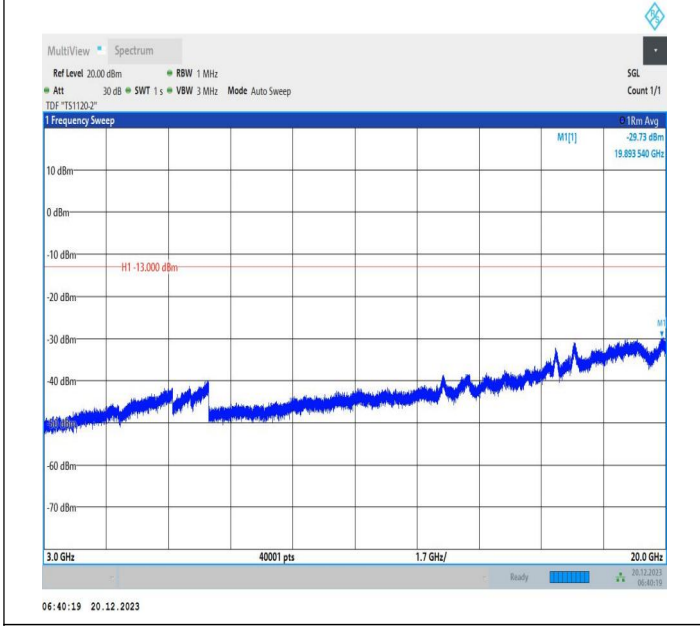
2-2-10MHz-20MHz-QPSK-QPSK-18806-18950-1RB#0-1RB#9 9-3000~20000MHz-PASS
