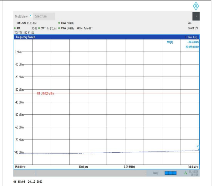
2-2-10MHz-20MHz-16QAM-16QAM-18806-18950-50RB#0-10 ORB#0-0.15~30MHz-PASS
