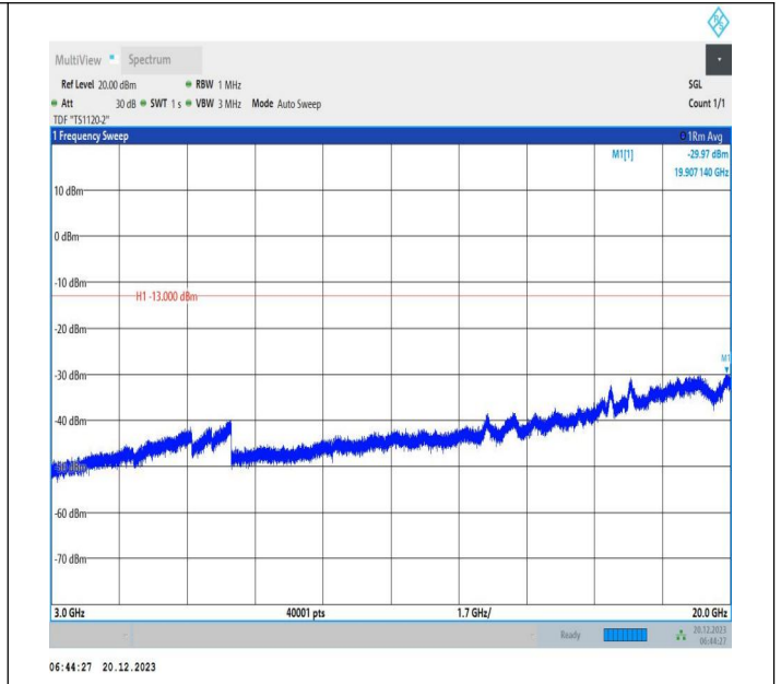
2-2-10MHz-20MHz-QPSK-QPSK-18806-18950-50RB#0-100R B#0-3000~20000MHz-PASS
