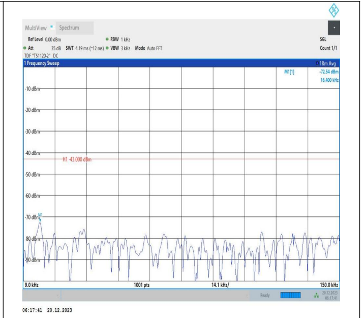
2-2-10MHz-20MHz-QPSK-QPSK-18655-18799-50RB#0-100R B#0-0.009~0.15MHz-PASS
