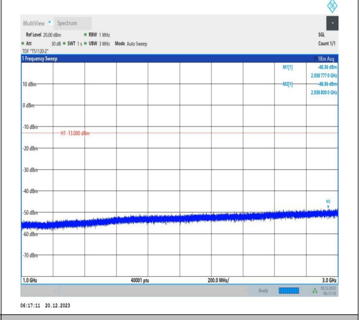
2-2-10MHz-20MHz-64QAM-64QAM-18655-18799-1RB#0-1RB #99-1000~3000MHz-PASS
