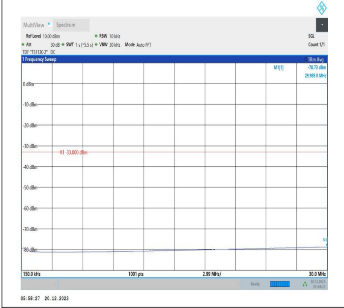
2-2-10MHz-20MHz-16QAM-16QAM-18655-18799-1RB#0-0RB #0-0.15~30MHz-PASS
