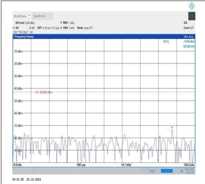
2-2-10MHz-20MHz-16QAM-16QAM-18655-18799-1RB#49-OR B#0-0.009~0.15MHz-PASS
