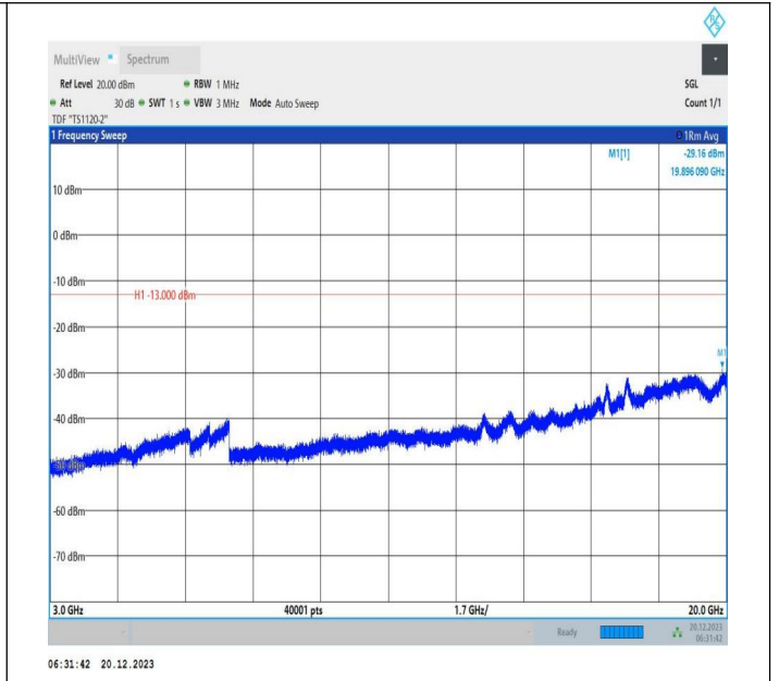
2-2-10MHz-20MHz-64QAM-64QAM-18806-18950-1RB#49-0R B#0-3000~20000MHz-PASS
