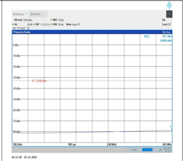
2-2-10MHz-20MHz-QPSK-QPSK-18655-18799-1RB#0-1RB#9 9-0.15~30MHz-PASS
