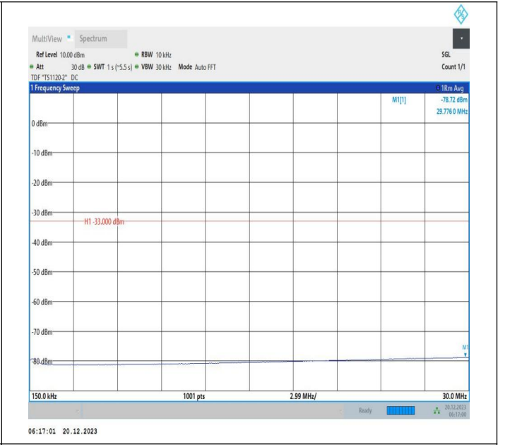
2-2-10MHz-20MHz-64QAM-64QAM-18655-18799-1RB#0-1RB #99-0.15~30MHz-PASS
