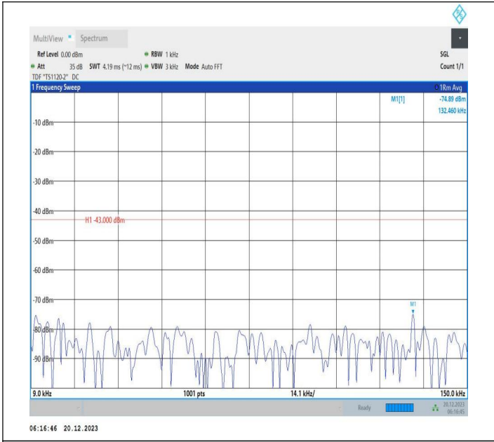
2-2-10MHz-20MHz-64QAM-64QAM-18655-18799-1RB#0-1RB #99-0.009~0.15MHz-PASS
