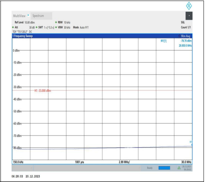
2-2-10MHz-20MHz-16QAM-16QAM-18806-18950-1RB#49-OR B#0-0.15~30MHz-PASS
