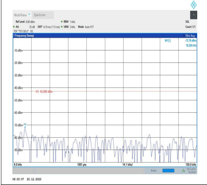
2-2-10MHz-20MHz-64QAM-64QAM-18655-18799-1RB#0-ORB #0-0.009~0.15MHz-PASS
