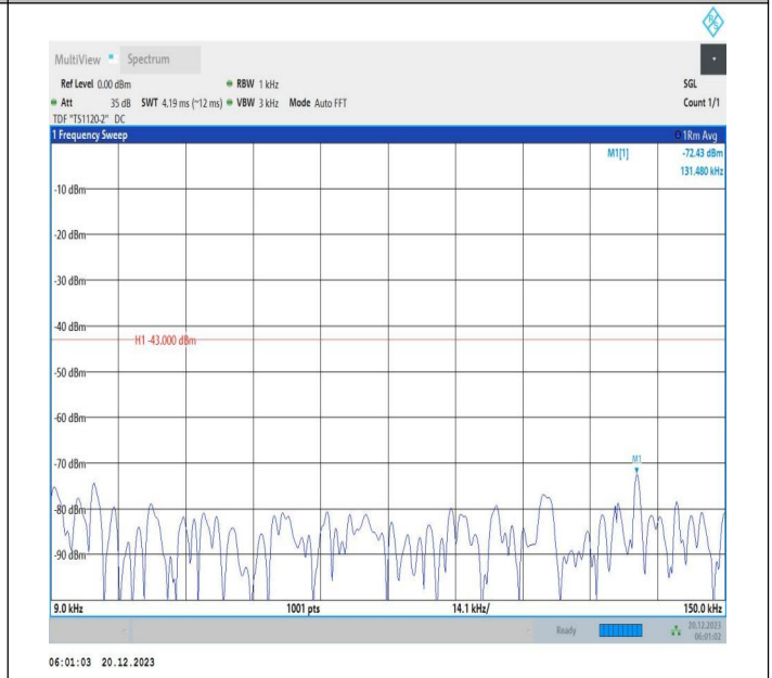
2-2-10MHz-20MHz-QPSK-QPSK-18655-18799-1RB#49-ORB# 0-0.009~0.15MHz-PASS
