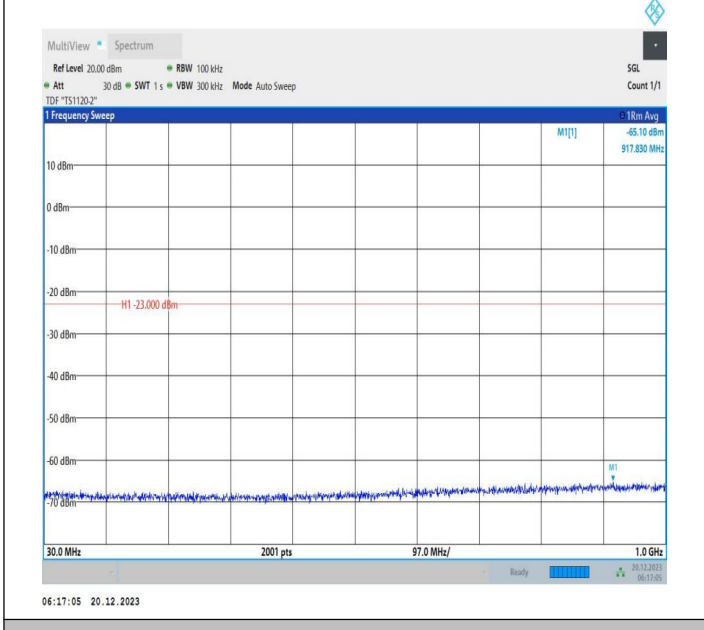
2-2-10MHz-20MHz-64QAM-64QAM-18655-18799-1RB#0-1RB #99-30~1000MHz-PASS
