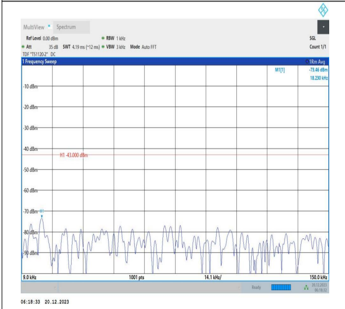
2-2-10MHz-20MHz-16QAM-16QAM-18655-18799-50RB#0-10 ORB#0-0.009~0.15MHz-PASS
