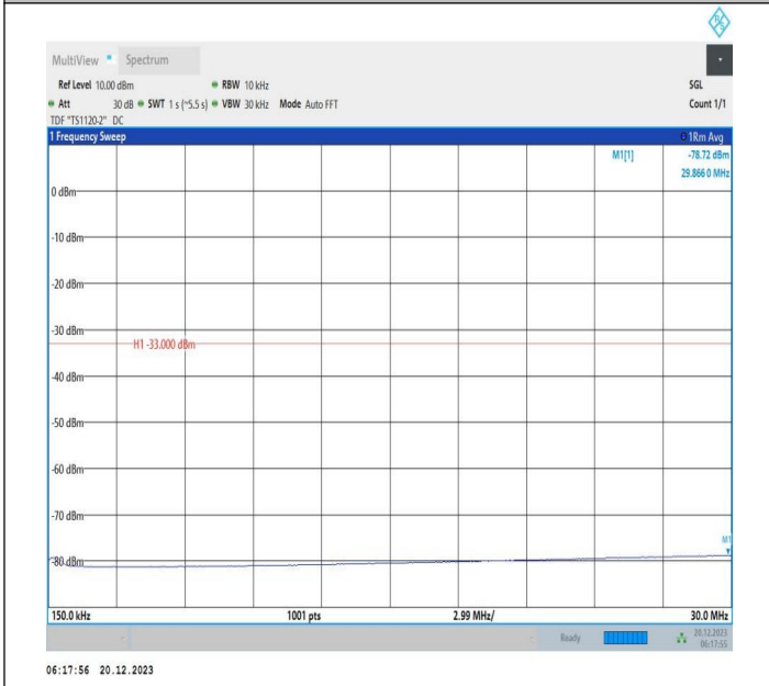
2-2-10MHz-20MHz-QPSK-QPSK-18655-18799-50RB#0-100R B#0-0.15~30MHz-PASS
