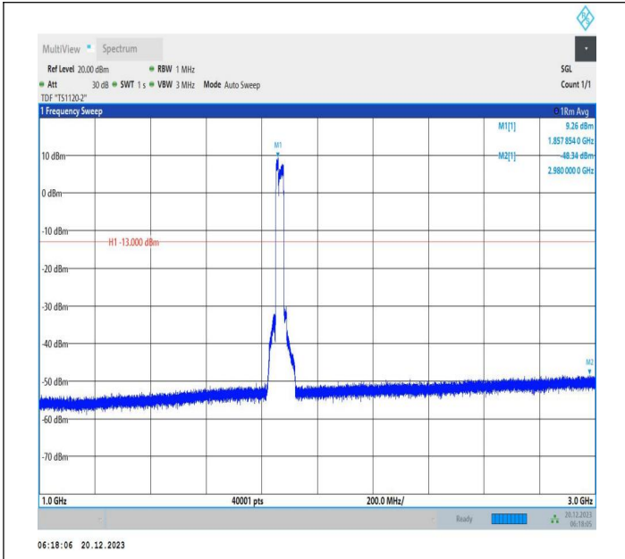
2-2-10MHz-20MHz-QPSK-QPSK-18655-18799-50RB#0-100R B#0-1000~3000MHz-PASS
