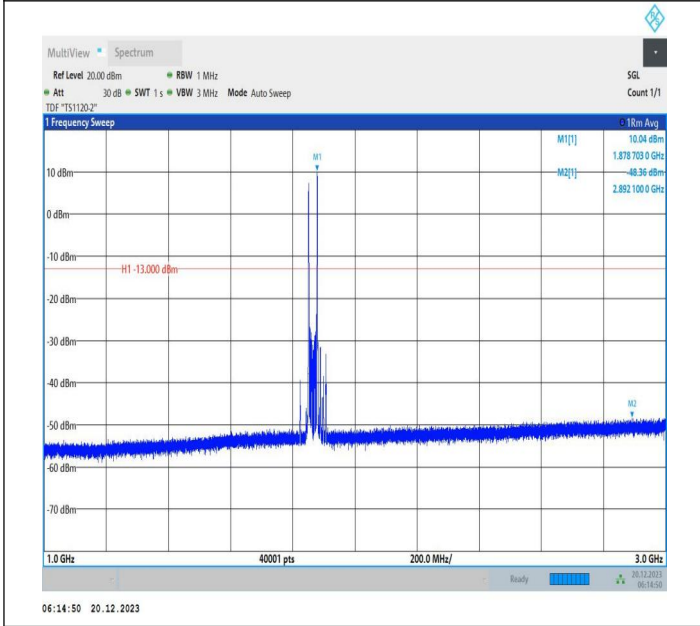
2-2-10MHz-20MHz-16QAM-16QAM-18655-18799-1RB#0-1RB #99-1000~3000MHz-PASS
