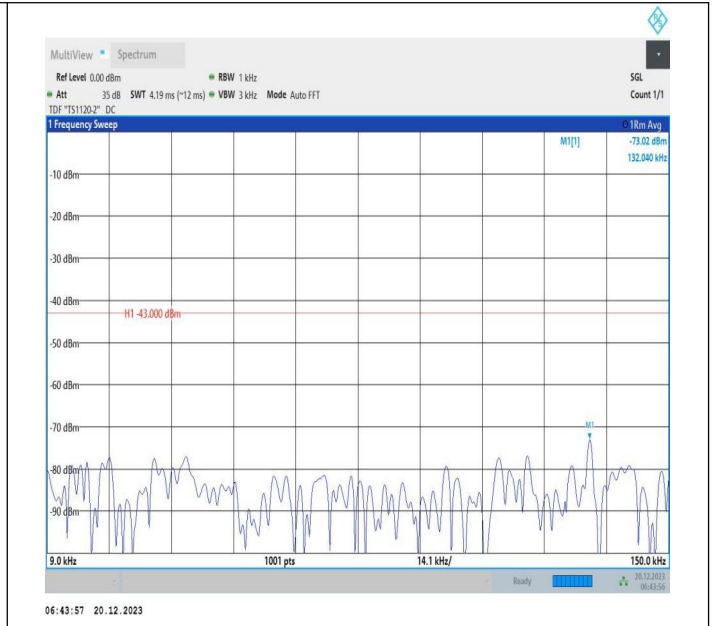
2-2-10MHz-20MHz-QPSK-QPSK-18806-18950-50RB#0-100R B#0-0.009~0.15MHz-PASS
