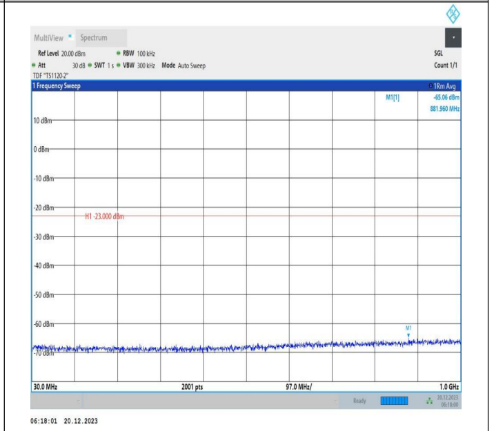
2-2-10MHz-20MHz-QPSK-QPSK-18655-18799-50RB#0-100R B#0-30~1000MHz-PASS
