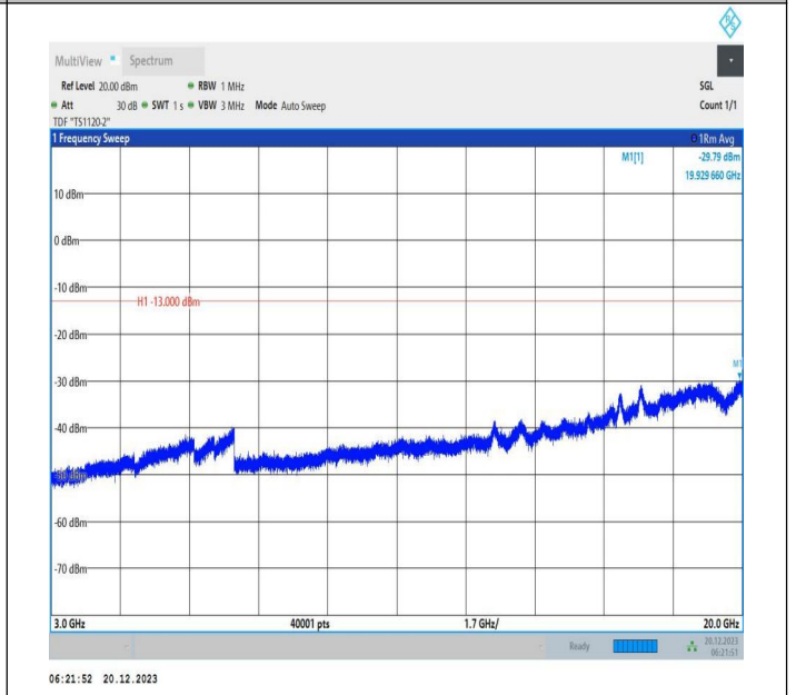
2-2-10MHz-20MHz-64QAM-64QAM-18655-18799-50RB#0-10 ORB#0-3000~20000MHz-PASS
