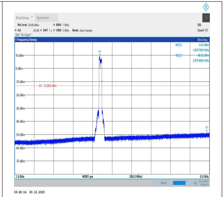
2-2-10MHz-20MHz-16QAM-16QAM-18806-18950-50RB#0-10 ORB#0-1000~3000MHz-PASS
