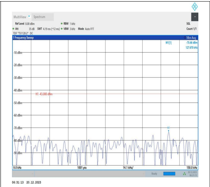
2-2-10MHz-20MHz-64QAM-64QAM-18806-18950-1RB#49-OR B#0-0.009~0.15MHz-PASS
