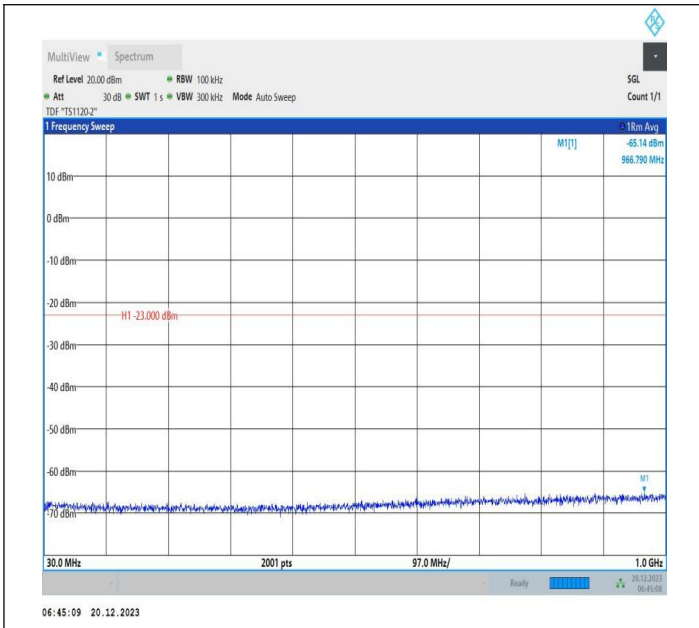
2-2-10MHz-20MHz-16QAM-16QAM-18806-18950-50RB#0-10 ORB#0-30~1000MHz-PASS
