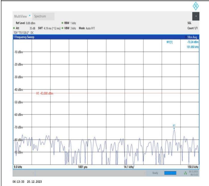
2-2-10MHz-20MHz-QPSK-QPSK-18655-18799-1RB#0-1RB#9 9-0.009~0.15MHz-PASS
