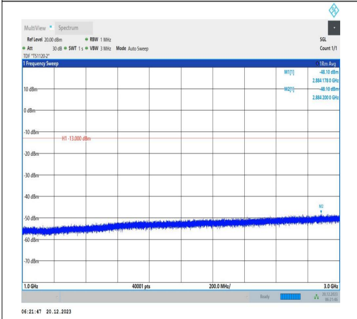
2-2-10MHz-20MHz-64QAM-64QAM-18655-18799-50RB#0-10 ORB#0-1000~3000MHz-PASS
