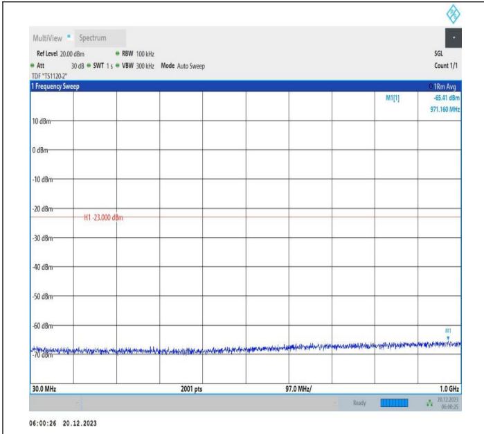
2-2-10MHz-20MHz-64QAM-64QAM-18655-18799-1RB#0-ORB #0-30~1000MHz-PASS
