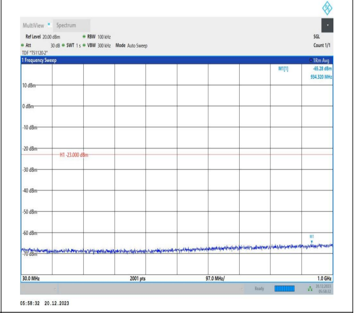
2-2-10MHz-20MHz-16QAM-16QAM-18655-18799-1RB#0-0RB #0-30~1000MHz-PASS
