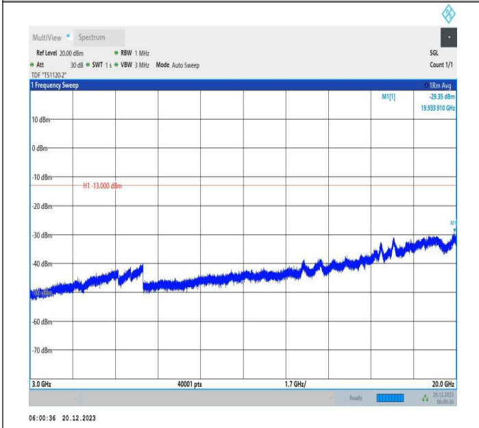
2-2-10MHz-20MHz-64QAM-64QAM-18655-18799-1RB#0-ORB #0-3000~20000MHz-PASS
