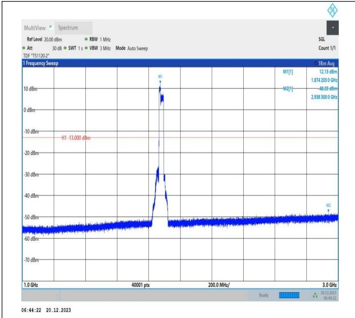
2-2-10MHz-20MHz-QPSK-QPSK-18806-18950-50RB#0-100R B#0-1000~3000MHz-PASS
