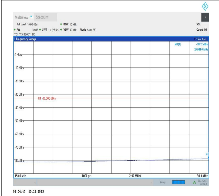
2-2-10MHz-20MHz-64QAM-64QAM-18655-18799-1RB#49-OR B#0-0.15~30MHz-PASS
