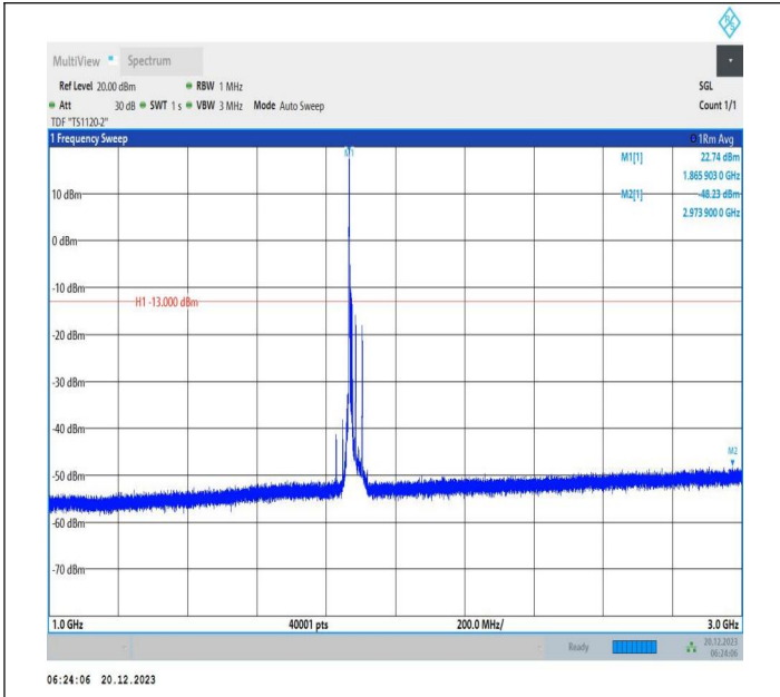
2-2-10MHz-20MHz-16QAM-16QAM-18806-18950-1RB#0-0RB #0-1000~3000MHz-PASS
