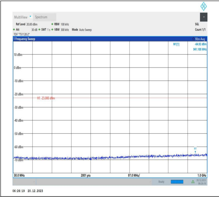
2-2-10MHz-20MHz-64QAM-64QAM-18806-18950-1RB#0-ORB #0-30~1000MHz-PASS
