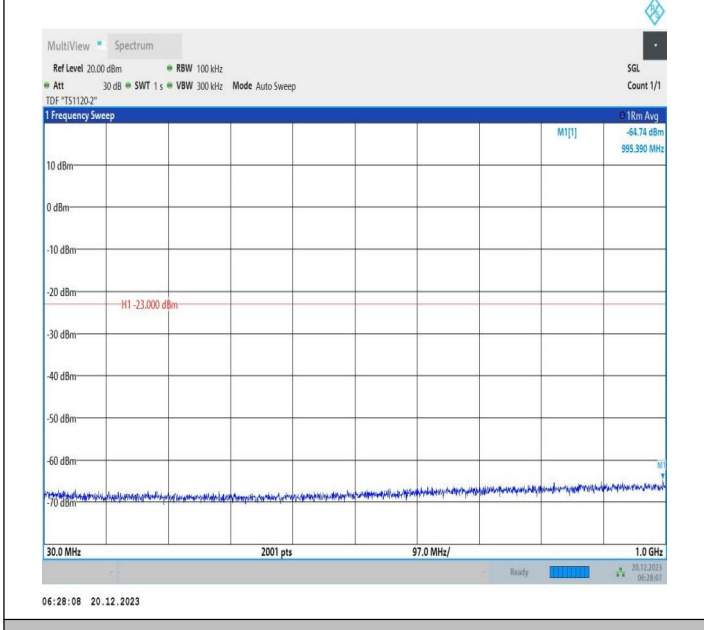
2-2-10MHz-20MHz-16QAM-16QAM-18806-18950-1RB#49-OR B#0-30~1000MHz-PASS
