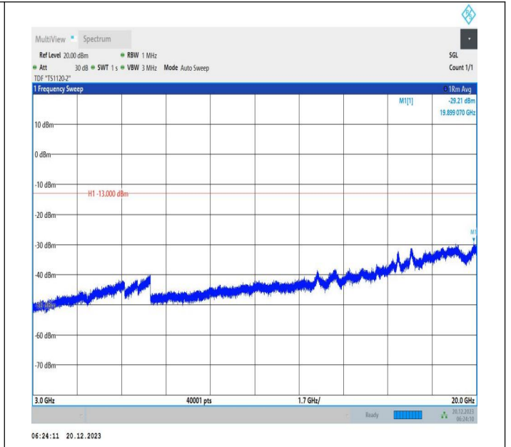
2-2-10MHz-20MHz-16QAM-16QAM-18806-18950-1RB#0-0RB #0-3000~20000MHz-PASS
