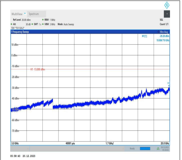
2-2-10MHz-20MHz-16QAM-16QAM-18655-18799-1RB#0-ORB #0-3000~20000MHz-PASS
