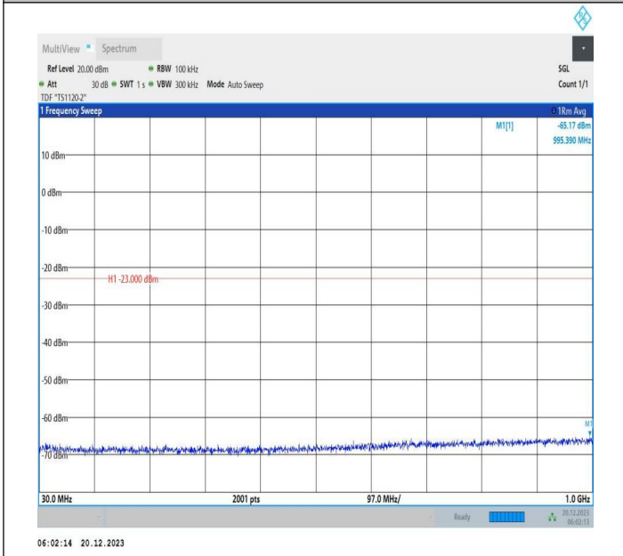
2-2-10MHz-20MHz-16QAM-16QAM-18655-18799-1RB#49-OR B#0-30~1000MHz-PASS
