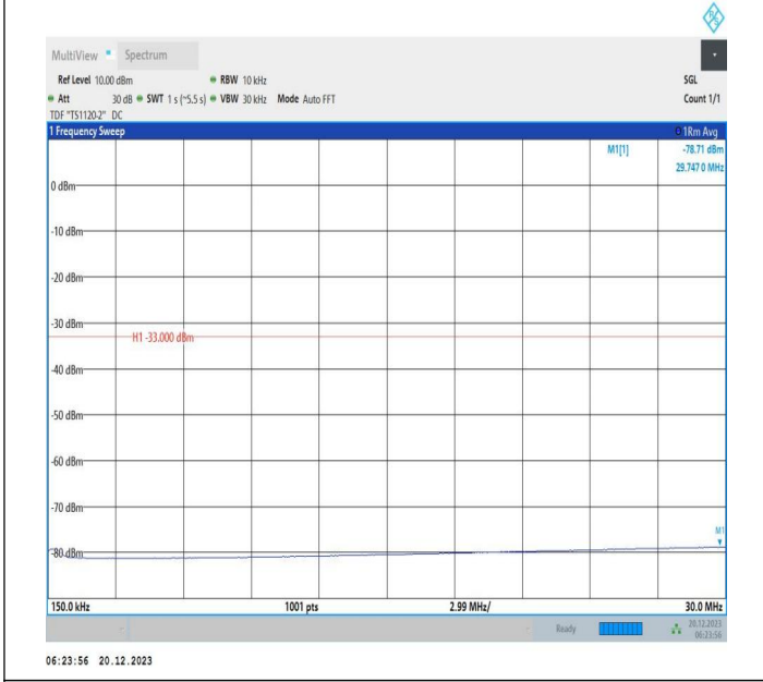
2-2-10MHz-20MHz-16QAM-16QAM-18806-18950-1RB#0-0RB #0-0.15~30MHz-PASS
