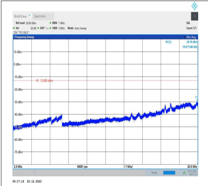
2-2-10MHz-20MHz-64QAM-64QAM-18655-18799-1RB#0-1RB #99-3000~20000MHz-PASS
