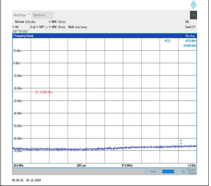
2-2-10MHz-20MHz-16QAM-16QAM-18806-18950-1RB#0-0RB #0-30~1000MHz-PASS
