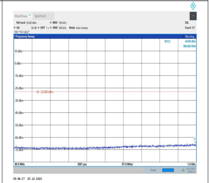
2-2-10MHz-20MHz-QPSK-QPSK-18806-18950-50RB#0-100R B#0-30~1000MHz-PASS
