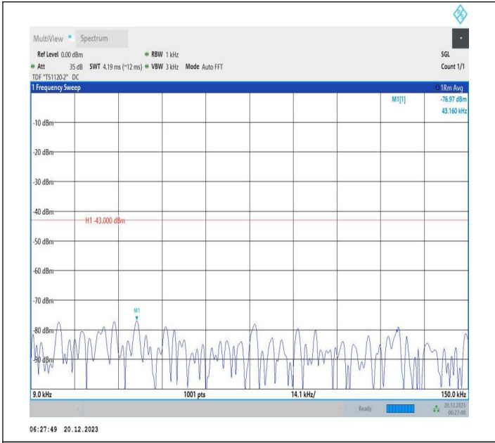
2-2-10MHz-20MHz-16QAM-16QAM-18806-18950-1RB#49-OR B#0-0.009~0.15MHz-PASS
