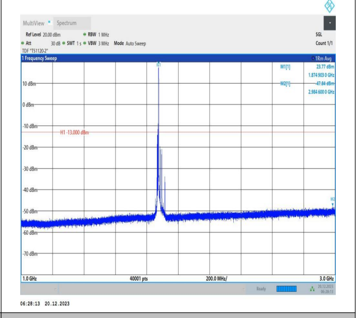
2-2-10MHz-20MHz-16QAM-16QAM-18806-18950-1RB#49-OR B#0-1000~3000MHz-PASS
