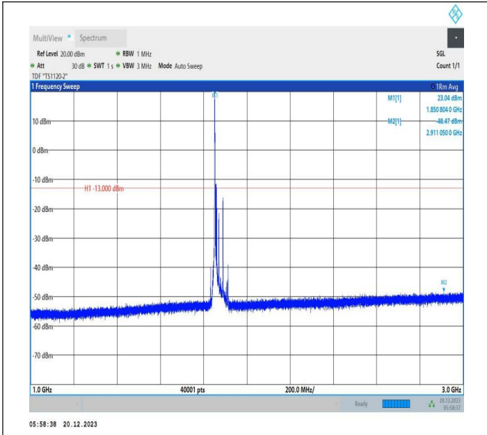
2-2-10MHz-20MHz-16QAM-16QAM-18655-18799-1RB#0-ORB #0-1000~3000MHz-PASS
