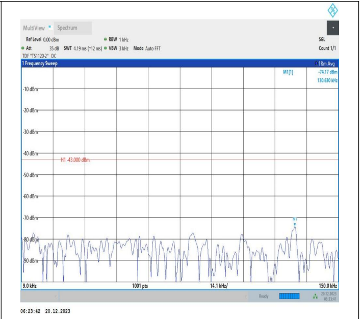
2-2-10MHz-20MHz-16QAM-16QAM-18806-18950-1RB#0-0RB #0-0.009~0.15MHz-PASS
