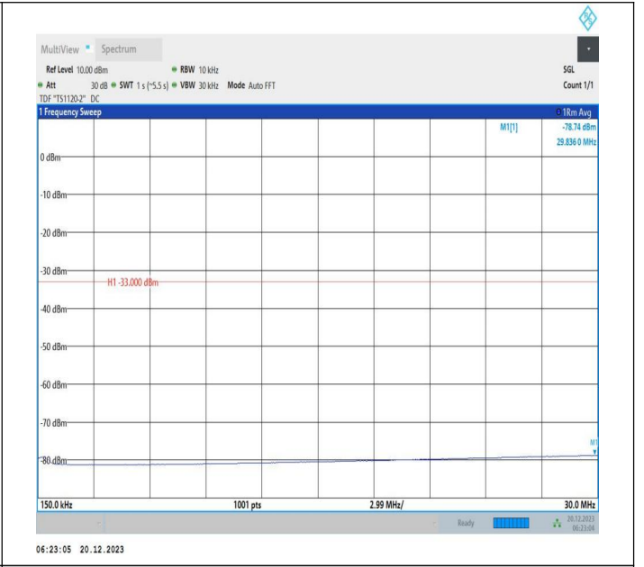
2-2-10MHz-20MHz-QPSK-QPSK-18806-18950-1RB#0-0RB#0 -0.15~30MHz-PASS
