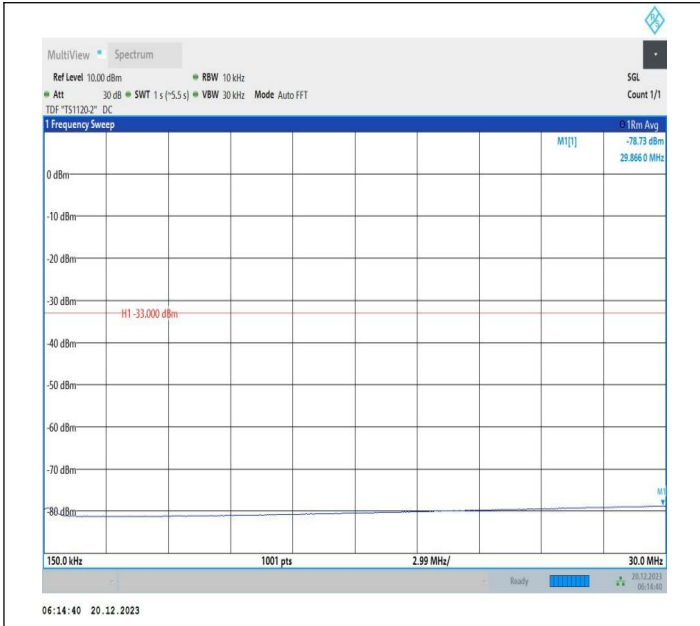
2-2-10MHz-20MHz-16QAM-16QAM-18655-18799-1RB#0-1RB #99-0.15~30MHz-PASS
