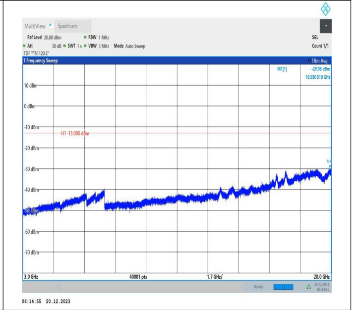
2-2-10MHz-20MHz-16QAM-16QAM-18655-18799-1RB#0-1RB #99-3000~20000MHz-PASS
