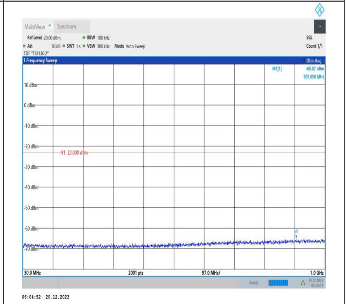
2-2-10MHz-20MHz-64QAM-64QAM-18655-18799-1RB#49-OR B#0-30~1000MHz-PASS
