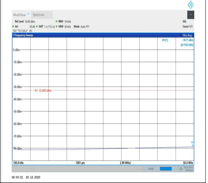
2-2-10MHz-20MHz-64QAM-64QAM-18655-18799-1RB#0-ORB #0-0.15~30MHz-PASS
