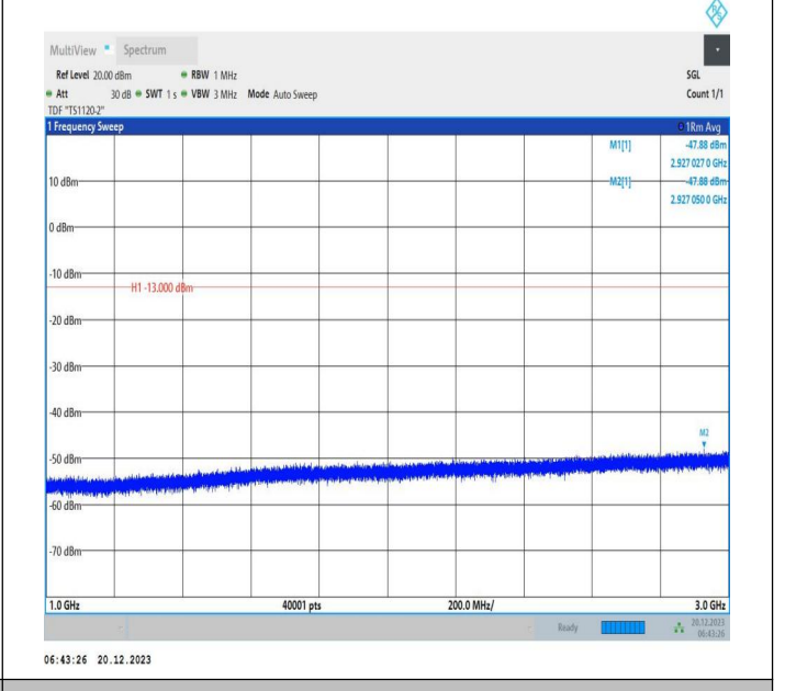
2-2-10MHz-20MHz-64QAM-64QAM-18806-18950-1RB#0-1RB #99-1000~3000MHz-PASS
