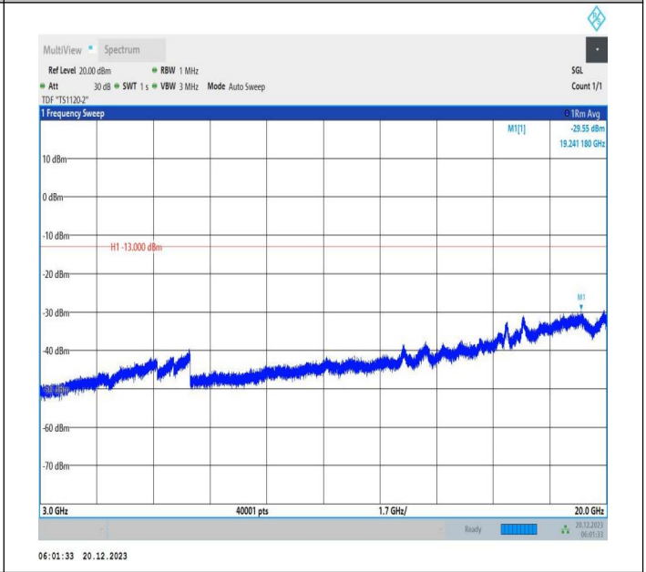
2-2-10MHz-20MHz-QPSK-QPSK-18655-18799-1RB#49-0RB# 0-3000~20000MHz-PASS
