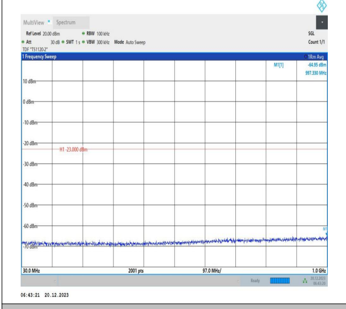
2-2-10MHz-20MHz-64QAM-64QAM-18806-18950-1RB#0-1RB #99-30~1000MHz-PASS
