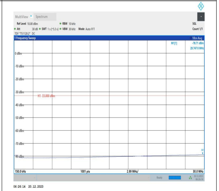
2-2-10MHz-20MHz-64QAM-64QAM-18806-18950-1RB#0-0RB #0-0.15~30MHz-PASS
