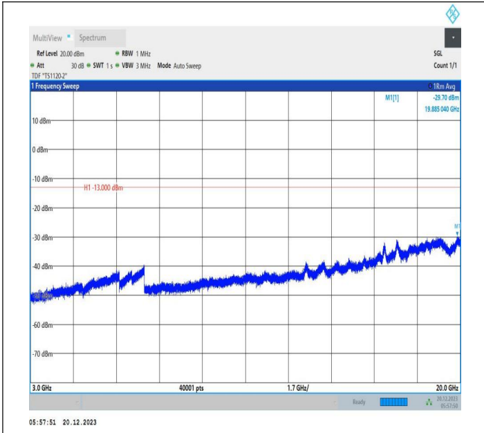
2-2-10MHz-20MHz-QPSK-QPSK-18655-18799-1RB#0-0RB#0 -3000~20000MHz-PASS
