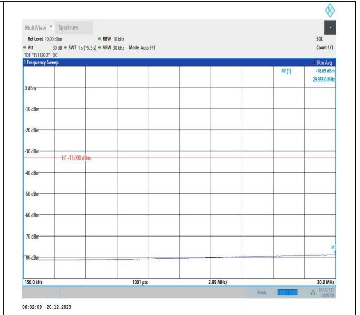
2-2-10MHz-20MHz-16QAM-16QAM-18655-18799-1RB#49-OR B#0-0.15~30MHz-PASS
