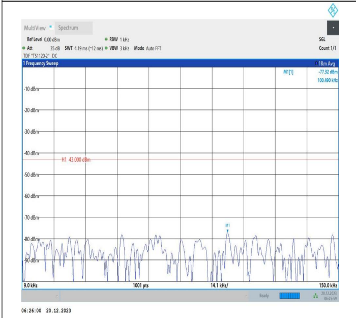
2-2-10MHz-20MHz-64QAM-64QAM-18806-18950-1RB#0-0RB #0-0.009~0.15MHz-PASS
