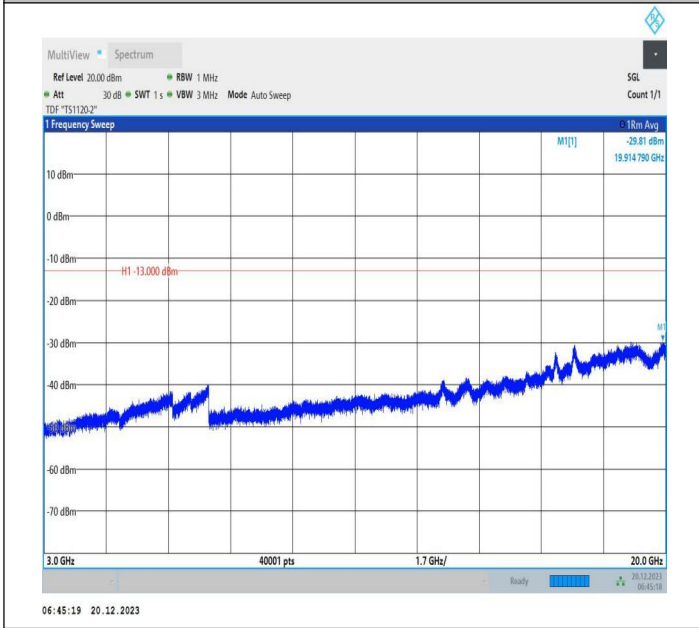
2-2-10MHz-20MHz-16QAM-16QAM-18806-18950-50RB#0-10 ORB#0-3000~20000MHz-PASS
