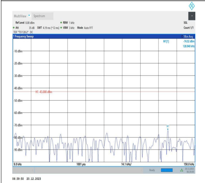
2-2-10MHz-20MHz-QPSK-QPSK-18806-18950-1RB#0-1RB#9 9-0.009~0.15MHz-PASS
